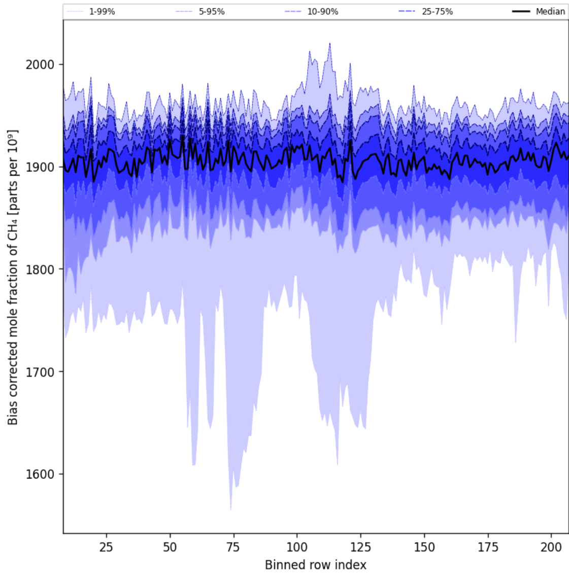
Figure 36: Along track statistics of “Bias corrected mole fraction of CH 4 ” for 2025-03-25 to 2025-03-27
