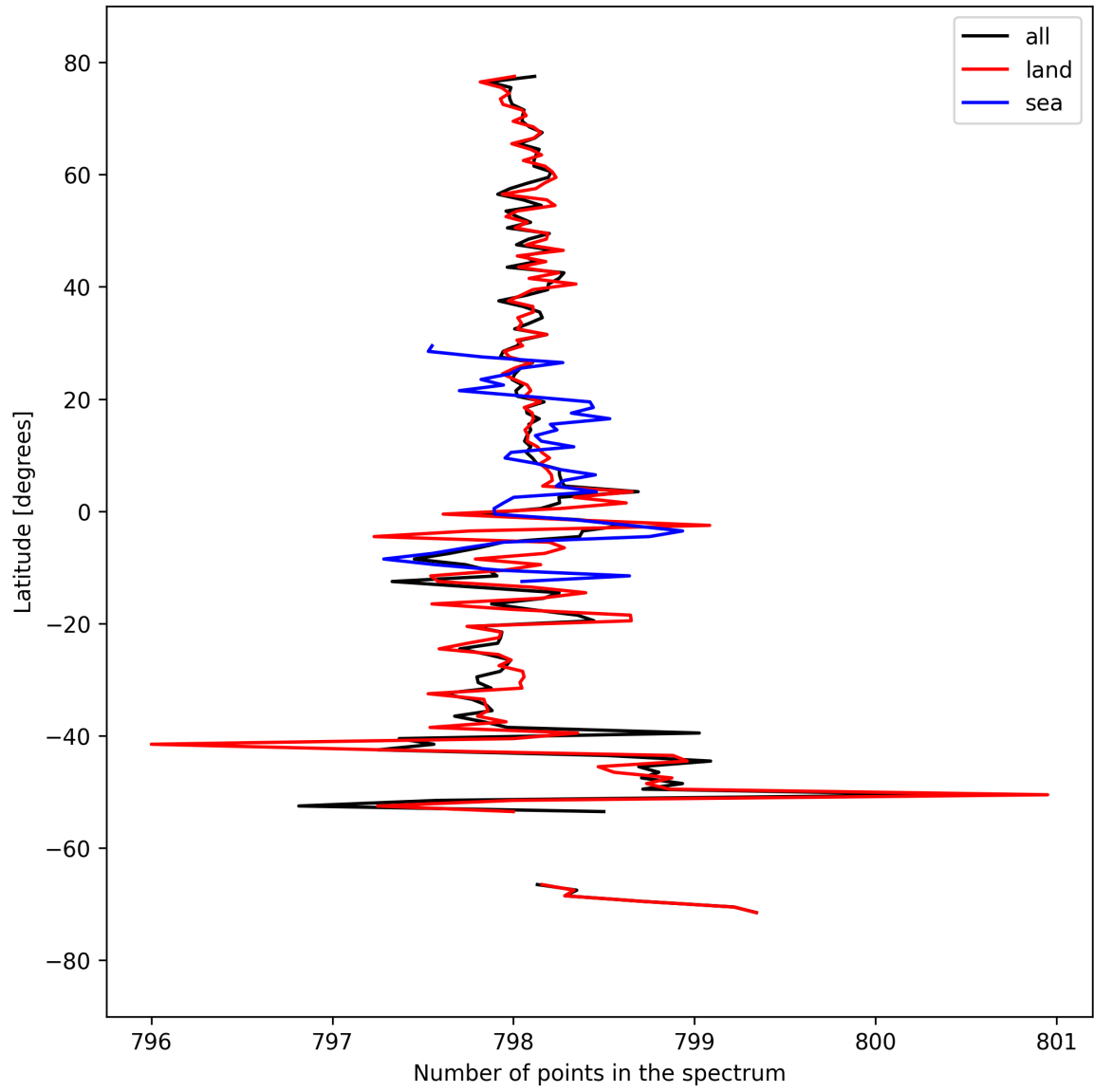
Figure 15: Zonal average of “Number of points in the spectrum” for 2025-03-25 to 2025-03-27.
