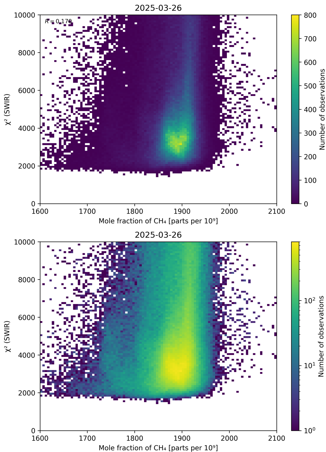
Figure 71: Scatter density plot of “Mole fraction of CH 4 ” against “ \chi^2 (SWIR)” for 2025-03-25 to 2025-03-27.
