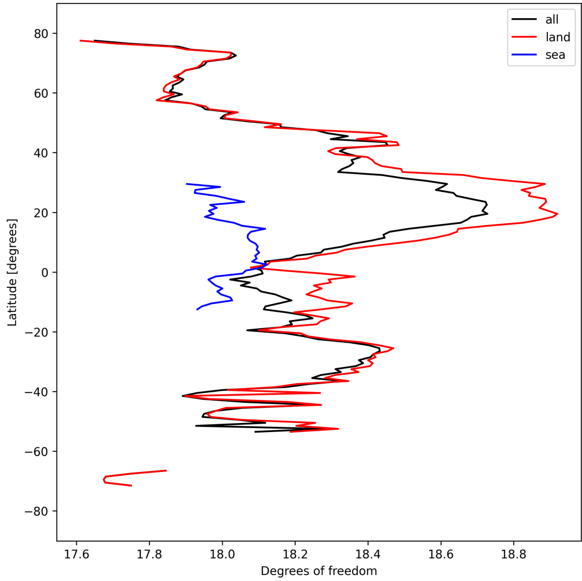
Figure 19: Zonal average of “Degrees of freedom” for 2025-03-25 to 2025-03-27.
