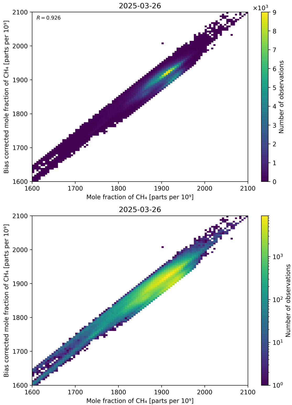
Figure 74: Scatter density plot of “Mole fraction of CH 4 ” against “Bias corrected mole fraction of CH 4 ” for 2025-03-25 to 2025-03-27.
