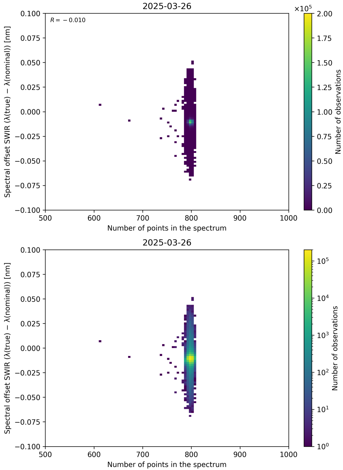
Figure 93: Scatter density plot of “Number of points in the spectrum” against “Spectral offset SWIR ( \lambda_{\text{true}} - \lambda_{\text{nominal}} )” for 2025-03-25 to 2025-03-27.
