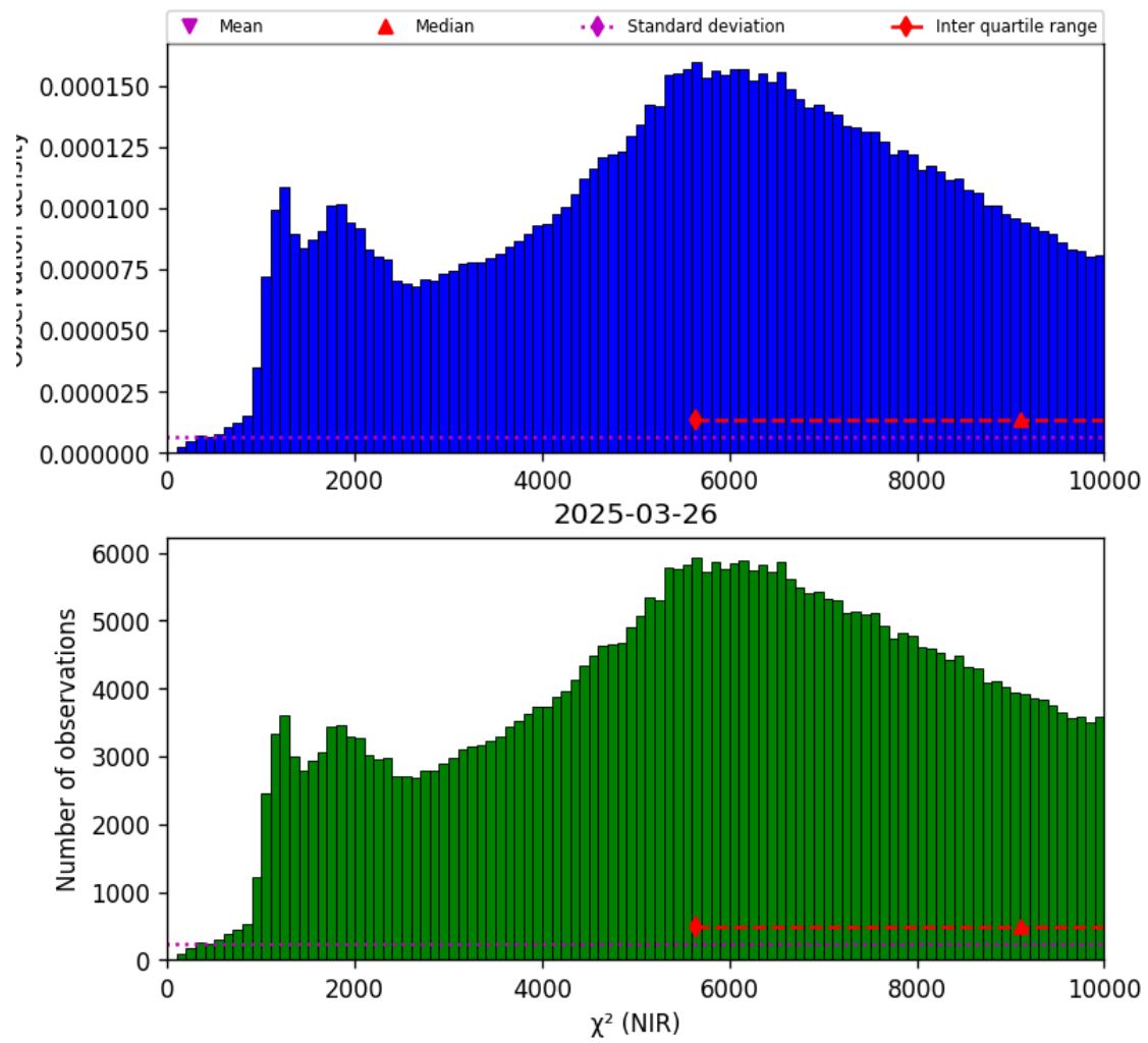
Figure 29: Histogram of “ \chi^2 (NIR)” for 2025-03-25 to 2025-03-27
