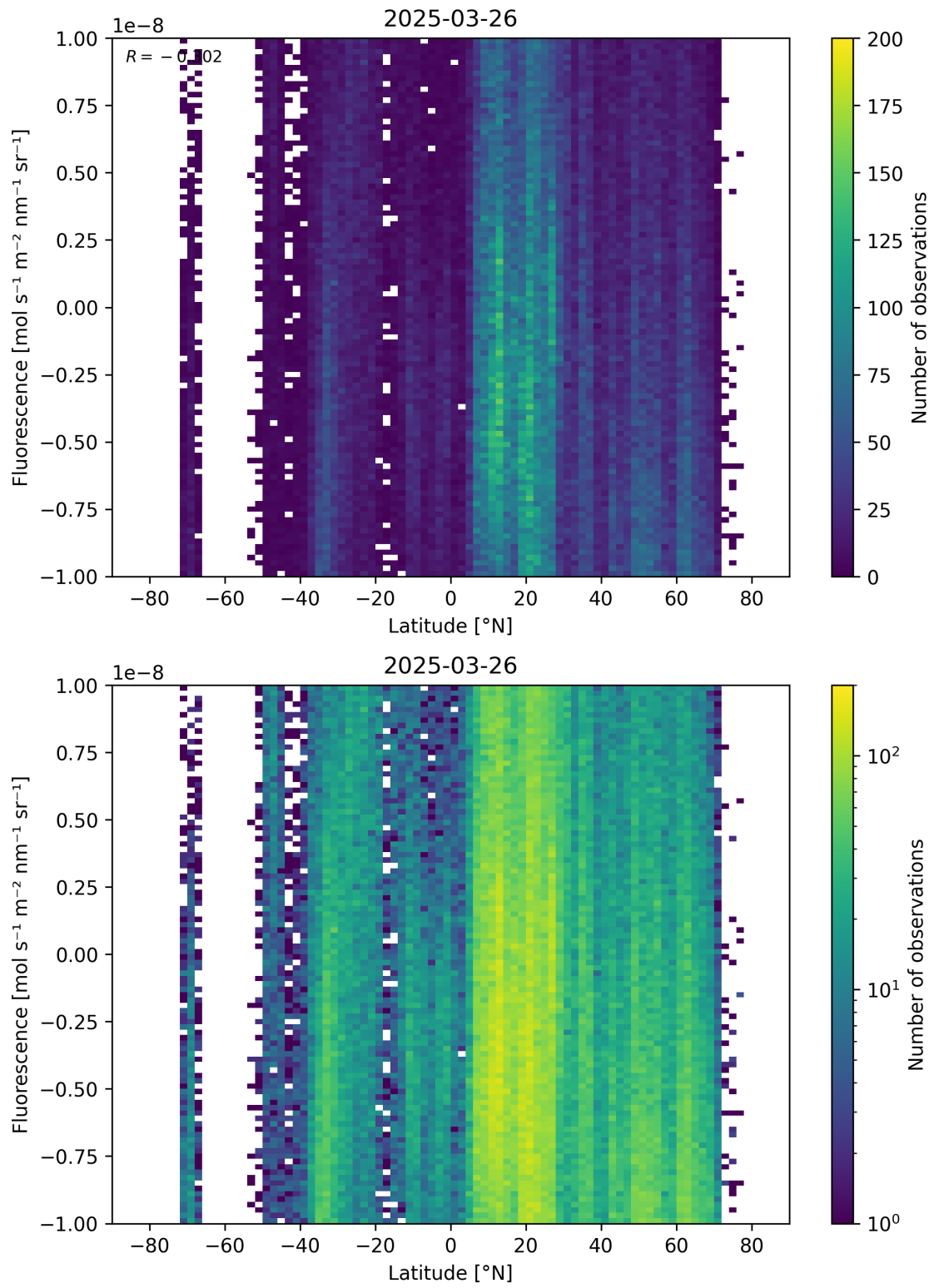
Figure 56: Scatter density plot of “Latitude” against “Fluorescence” for 2025-03-25 to 2025-03-27.
