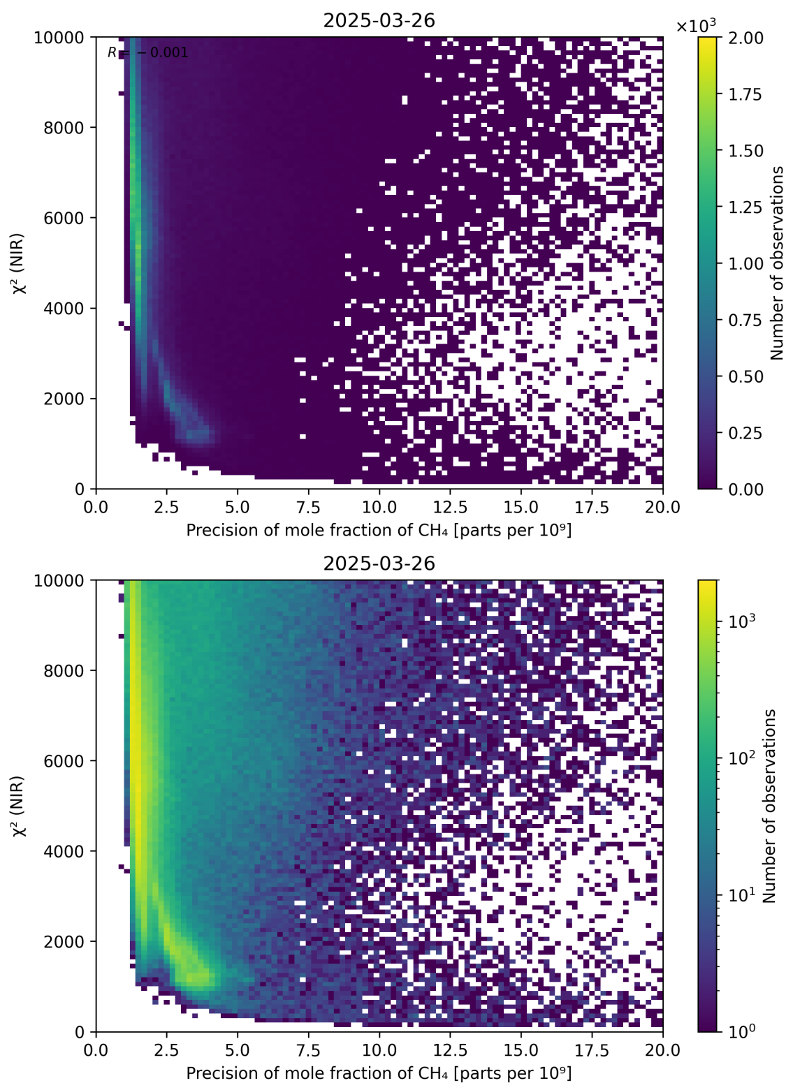
Figure 78: Scatter density plot of “Precision of mole fraction of \text{CH}_4 ” against “ \chi^2 (NIR)” for 2025-03-25 to 2025-03-27.
