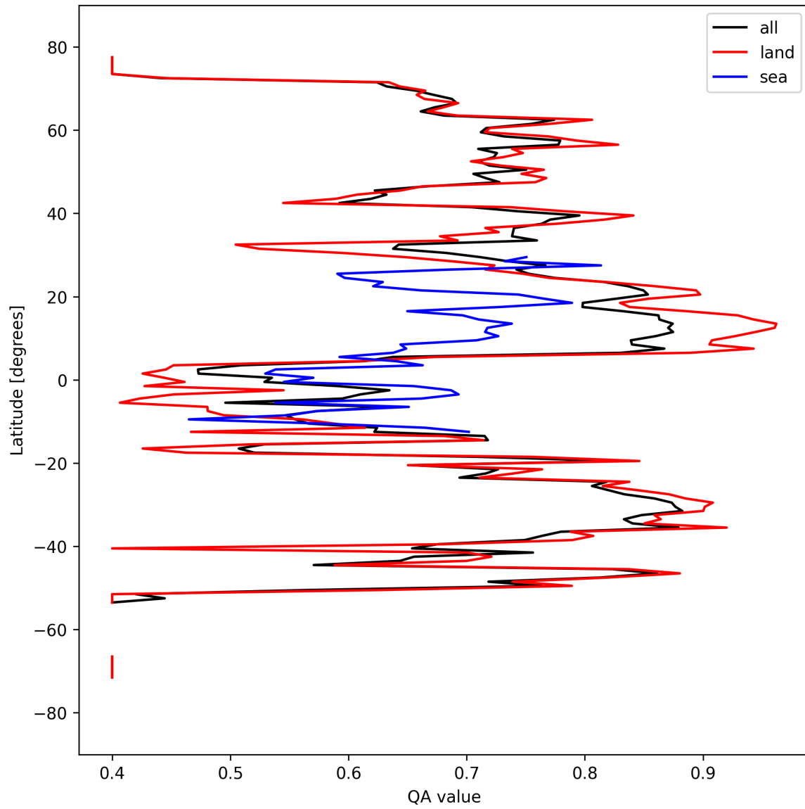
Figure 11: Zonal average of “QA value” for 2025-03-25 to 2025-03-27.
