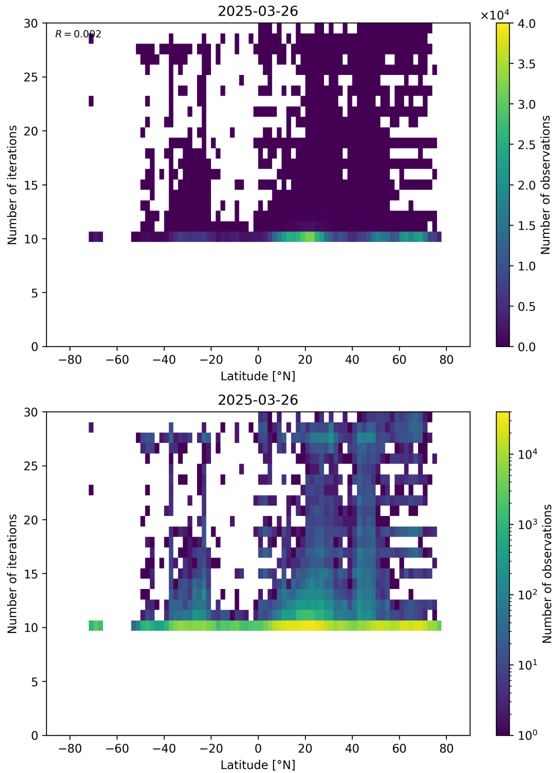
Figure 60: Scatter density plot of “Latitude” against “Number of iterations” for 2025-03-25 to 2025-03-27.
