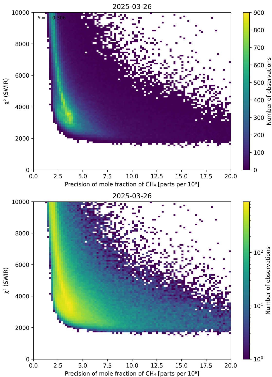
Figure 79: Scatter density plot of “Precision of mole fraction of CH 4 ” against “ \chi^2 (SWIR)” for 2025-03-25 to 2025-03-27.
