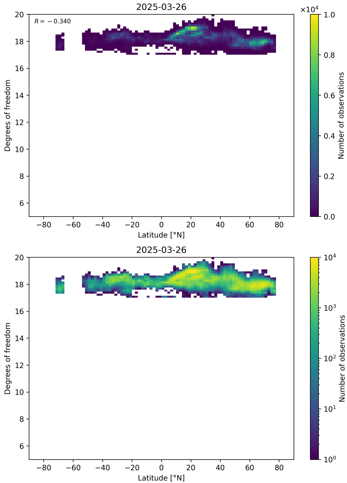
Figure 55: Scatter density plot of “Latitude” against “Degrees of freedom” for 2025-03-25 to 2025-03-27.
