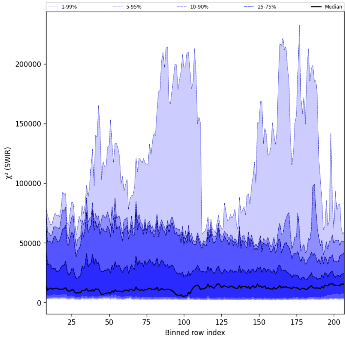
Figure 39: Along track statistics of “ \chi^2 (SWIR)” for 2025-03-25 to 2025-03-27
