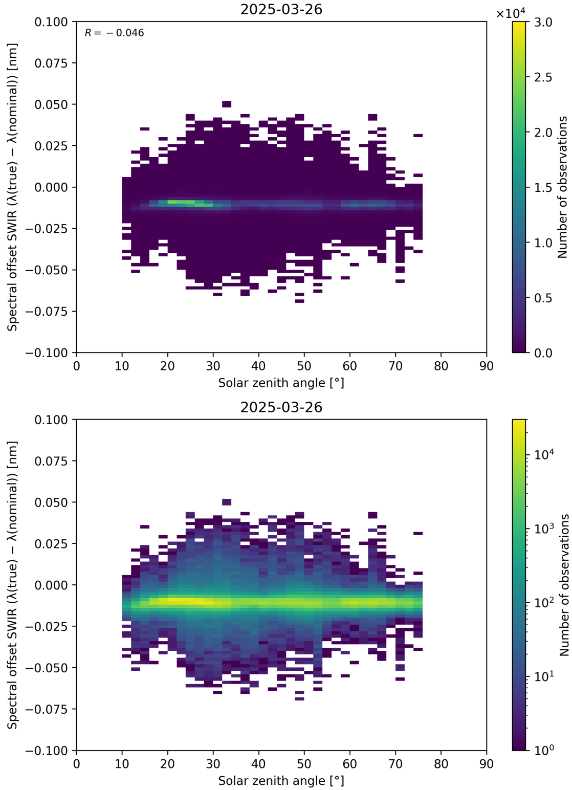
Figure 104: Scatter density plot of “Solar zenith angle” against “Spectral offset SWIR ( \lambda_{\text{true}} - \lambda_{\text{nominal}} )” for 2025-03-25 to 2025-03-27.
