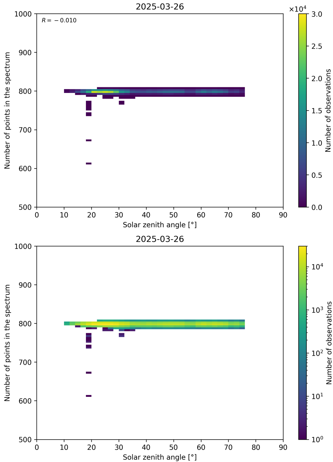
Figure 103: Scatter density plot of “Solar zenith angle” against “Number of points in the spectrum” for 2025-03-25 to 2025-03-27.
