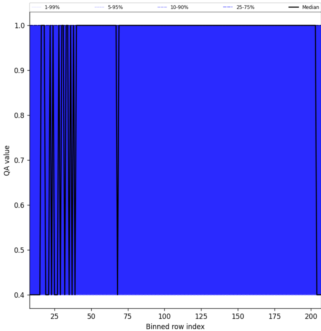
Figure 33: Along track statistics of “QA value” for 2025-03-25 to 2025-03-27
