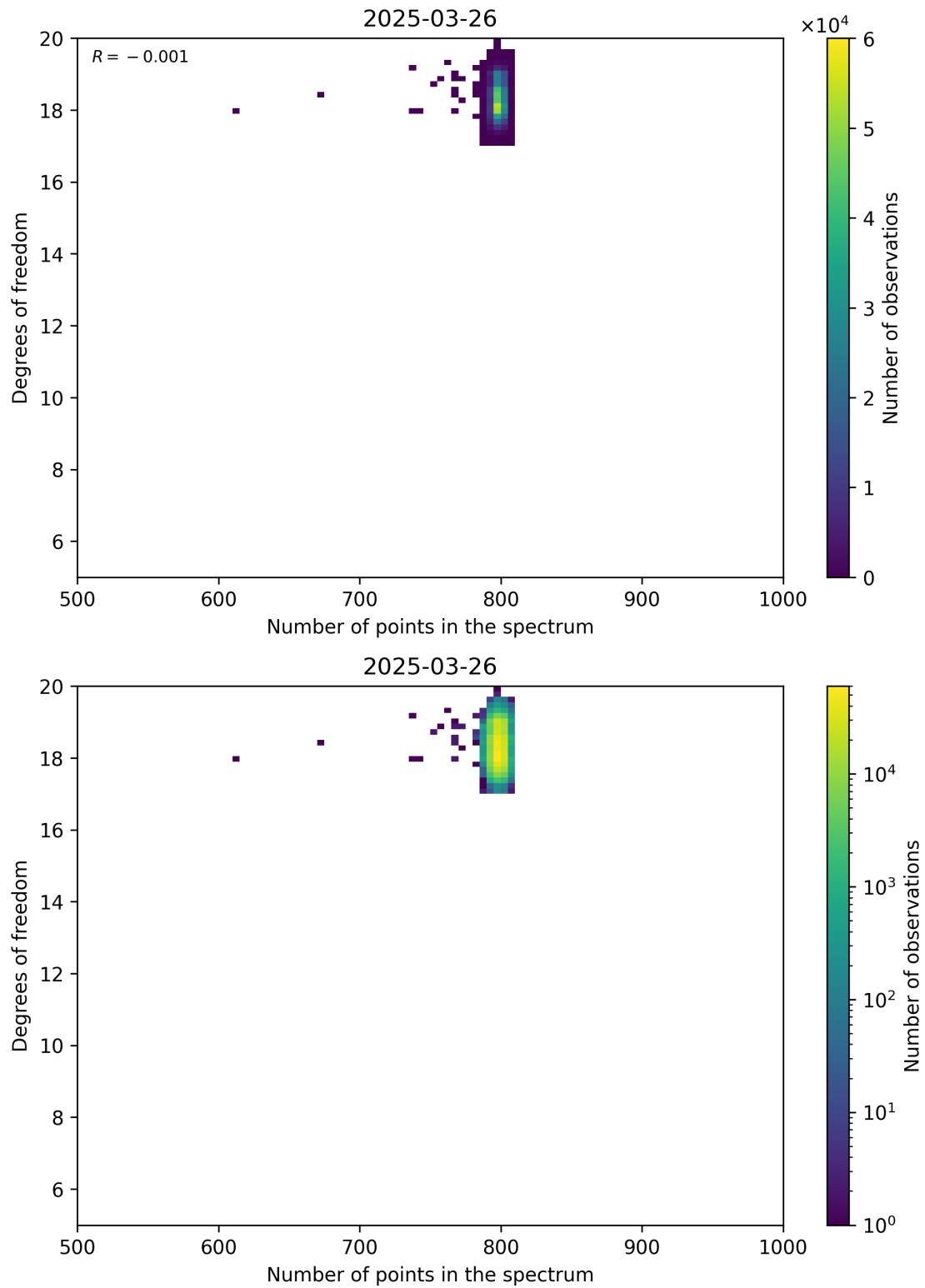
Figure 90: Scatter density plot of “Number of points in the spectrum” against “Degrees of freedom” for 2025-03-25 to 2025-03-27.
