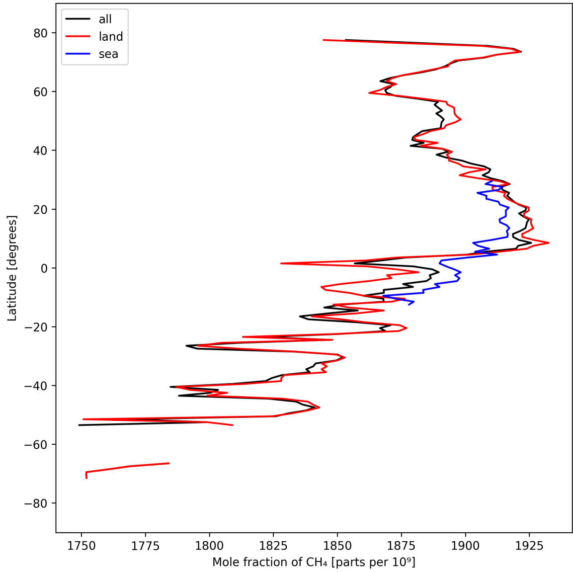
Figure 12: Zonal average of “Mole fraction of \text{CH}_4 ” for 2025-03-25 to 2025-03-27.
