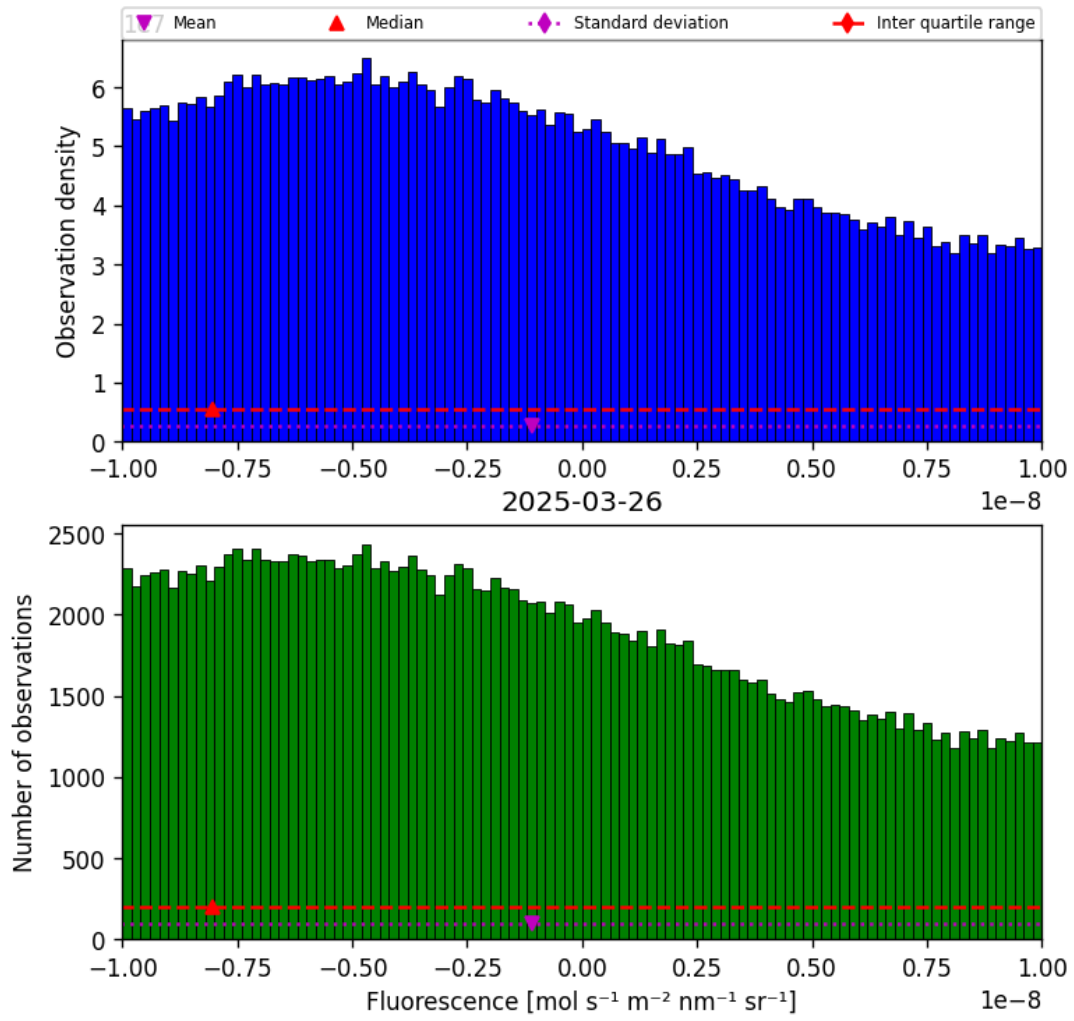
Figure 32: Histogram of “Fluorescence” for 2025-03-25 to 2025-03-27
