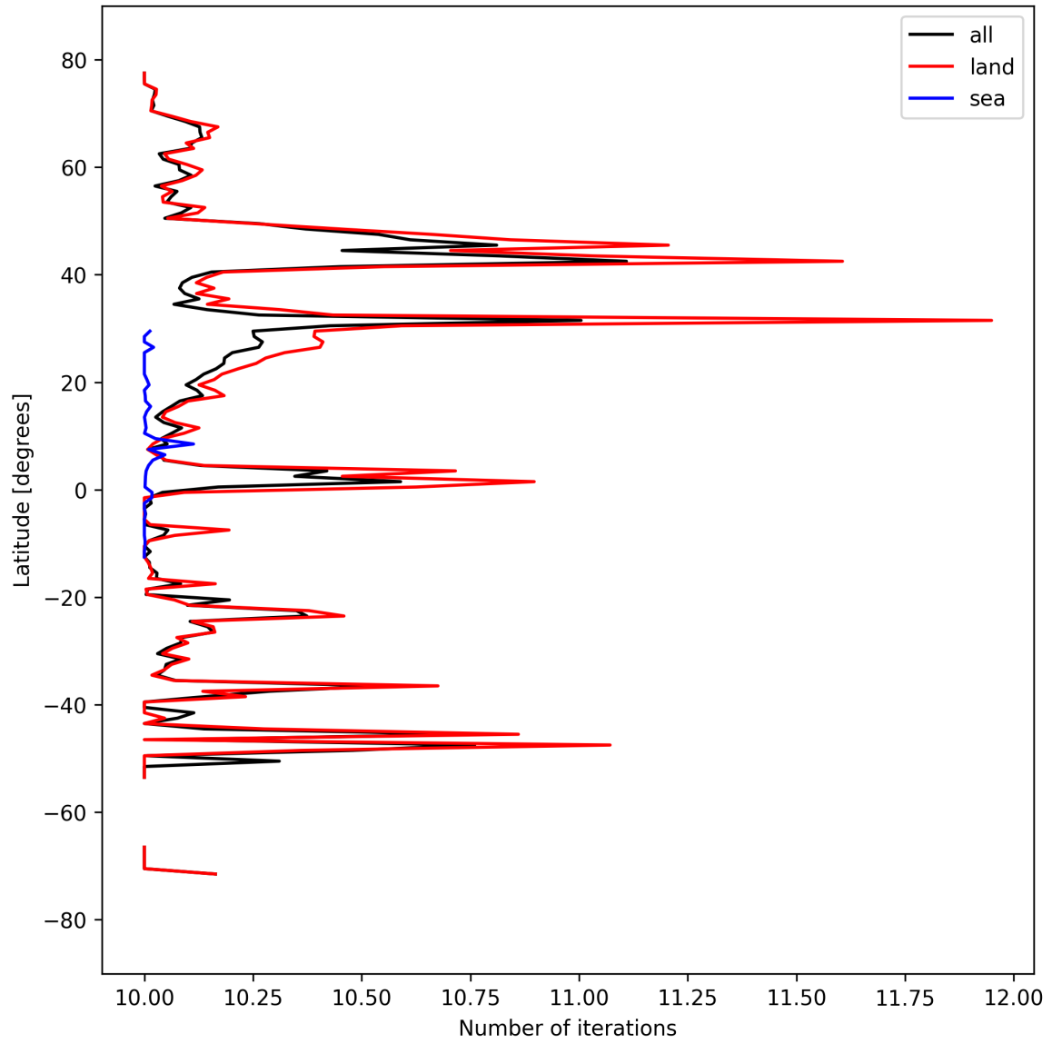
Figure 20: Zonal average of “Number of iterations” for 2025-03-25 to 2025-03-27.
