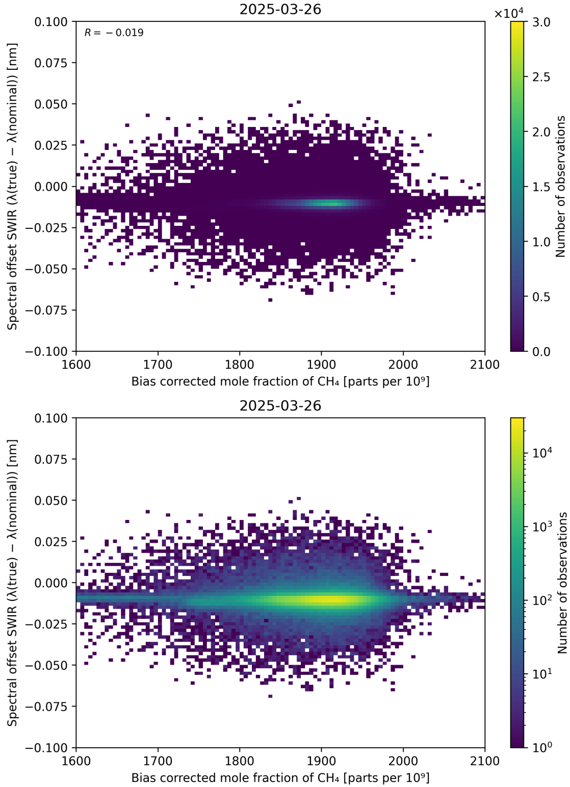
Figure 69: Scatter density plot of “Bias corrected mole fraction of \text{CH}_4 ” against “Spectral offset SWIR ( \lambda_{\text{true}} - \lambda_{\text{nominal}} )” for 2025-03-25 to 2025-03-27.
