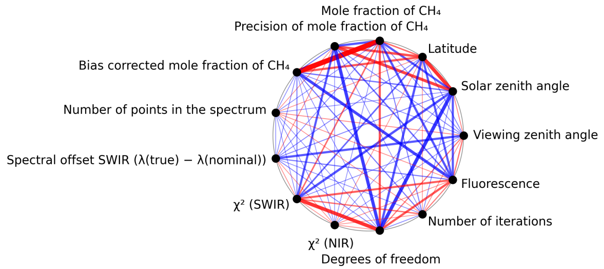
Figure 1: Map of correlation graph for 2025-03-25 to 2025-03-27.
