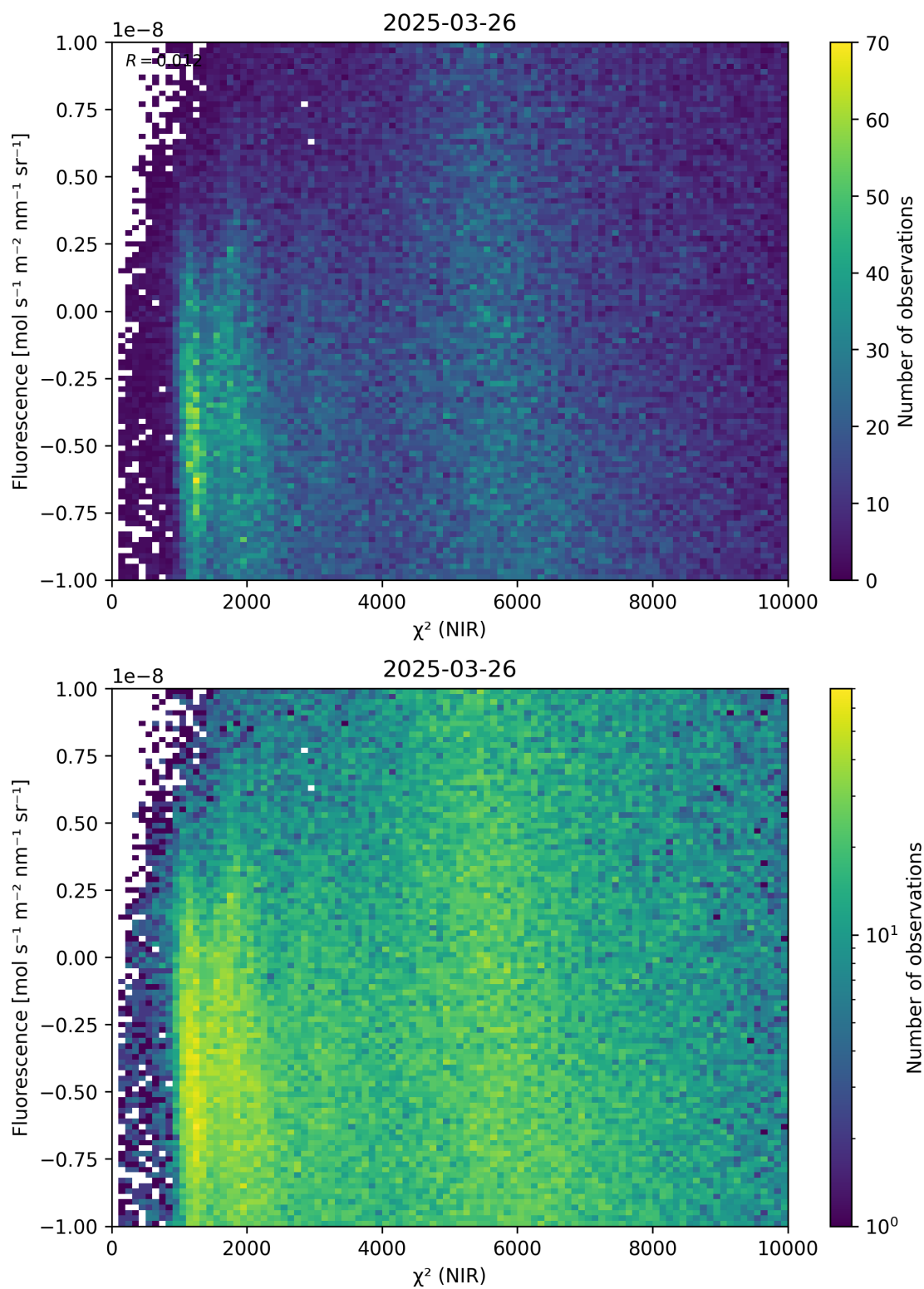
Figure 45: Scatter density plot of “ \chi^2 (NIR)” against “Fluorescence” for 2025-03-25 to 2025-03-27.
