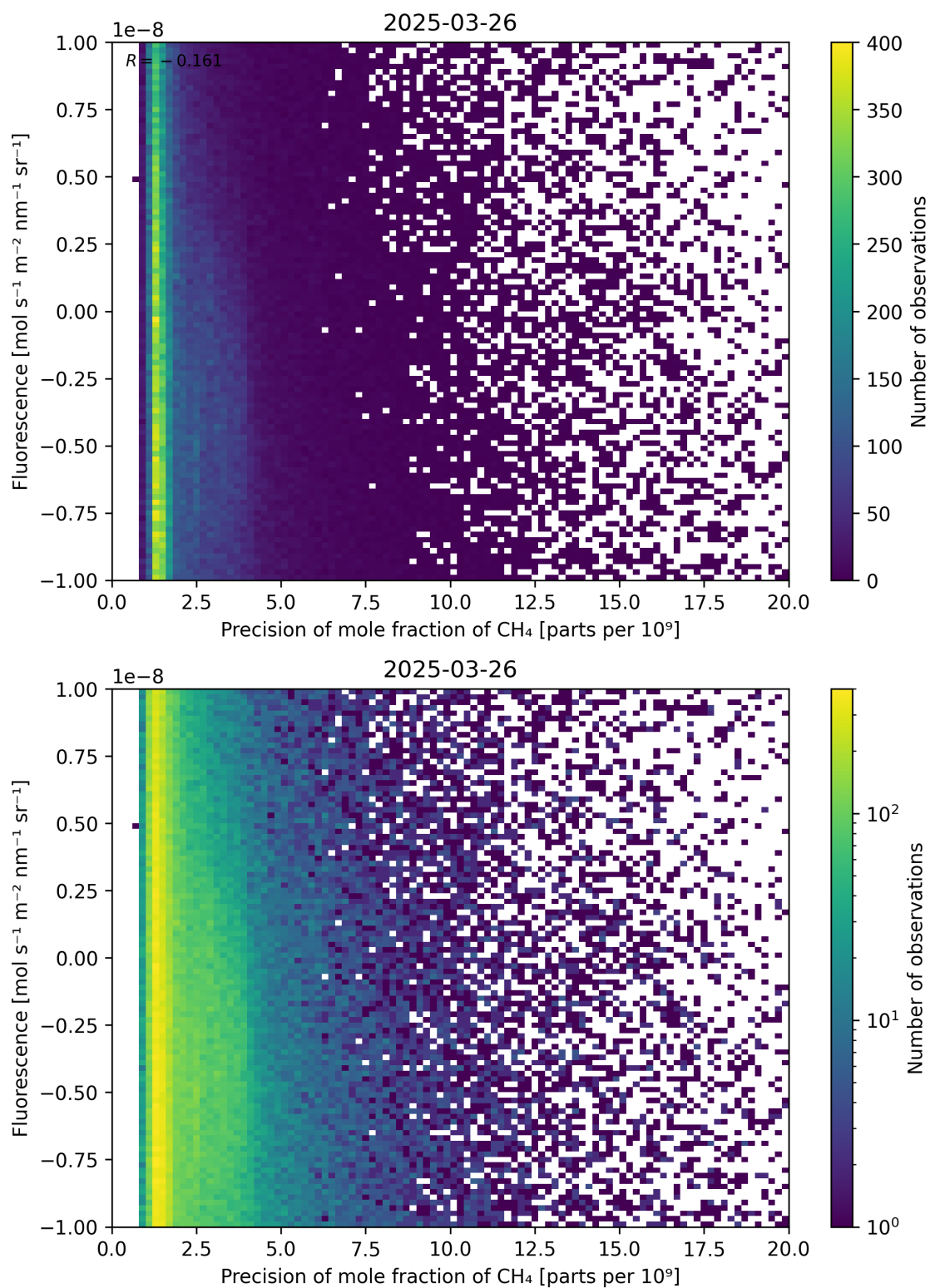
Figure 81: Scatter density plot of “Precision of mole fraction of \text{CH}_4 ” against “Fluorescence” for 2025-03-25 to 2025-03-27.
