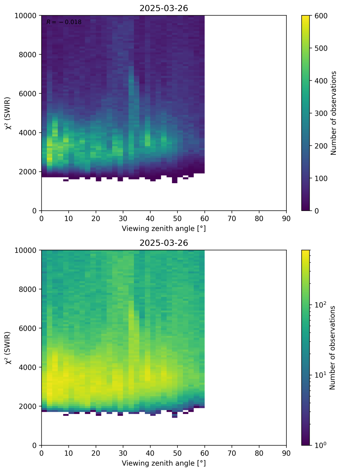
Figure 106: Scatter density plot of “Viewing zenith angle” against “ \chi^2 (SWIR)” for 2025-03-25 to 2025-03-27.
