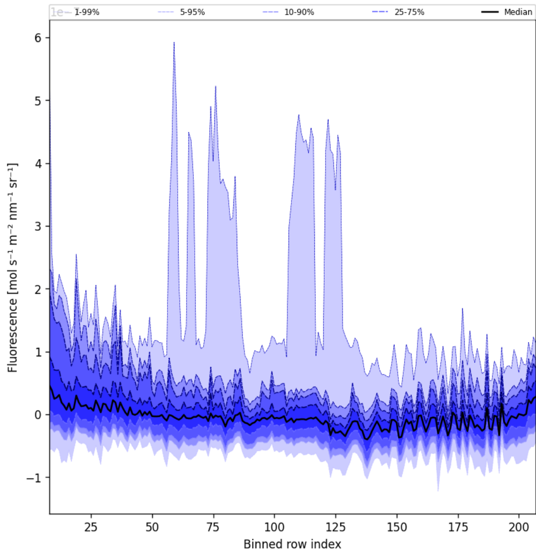
Figure 43: Along track statistics of “Fluorescence” for 2025-03-25 to 2025-03-27
