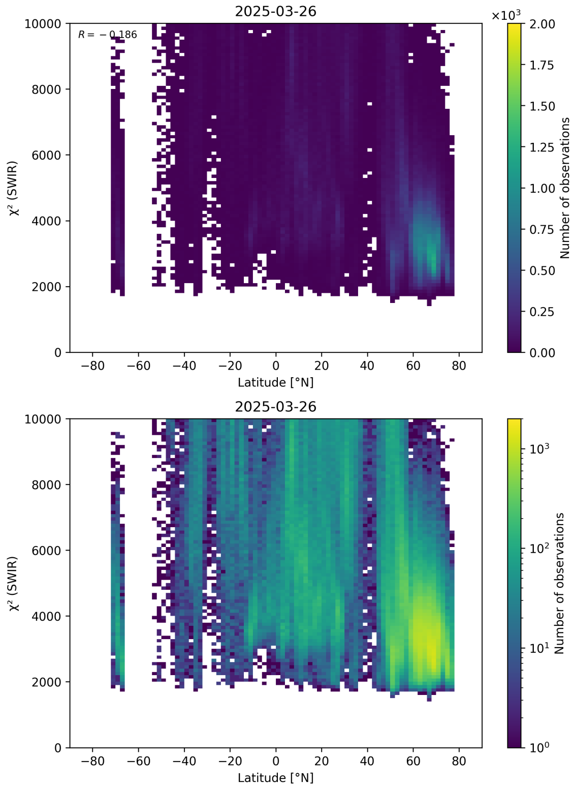
Figure 54: Scatter density plot of “Latitude” against “ \chi^2 (SWIR)” for 2025-03-25 to 2025-03-27.
