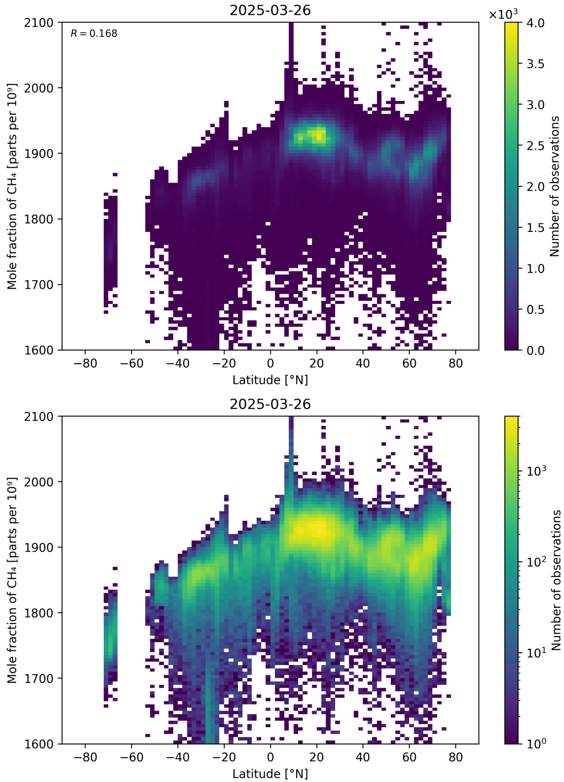
Figure 57: Scatter density plot of “Latitude” against “Mole fraction of \text{CH}_4 ” for 2025-03-25 to 2025-03-27.
