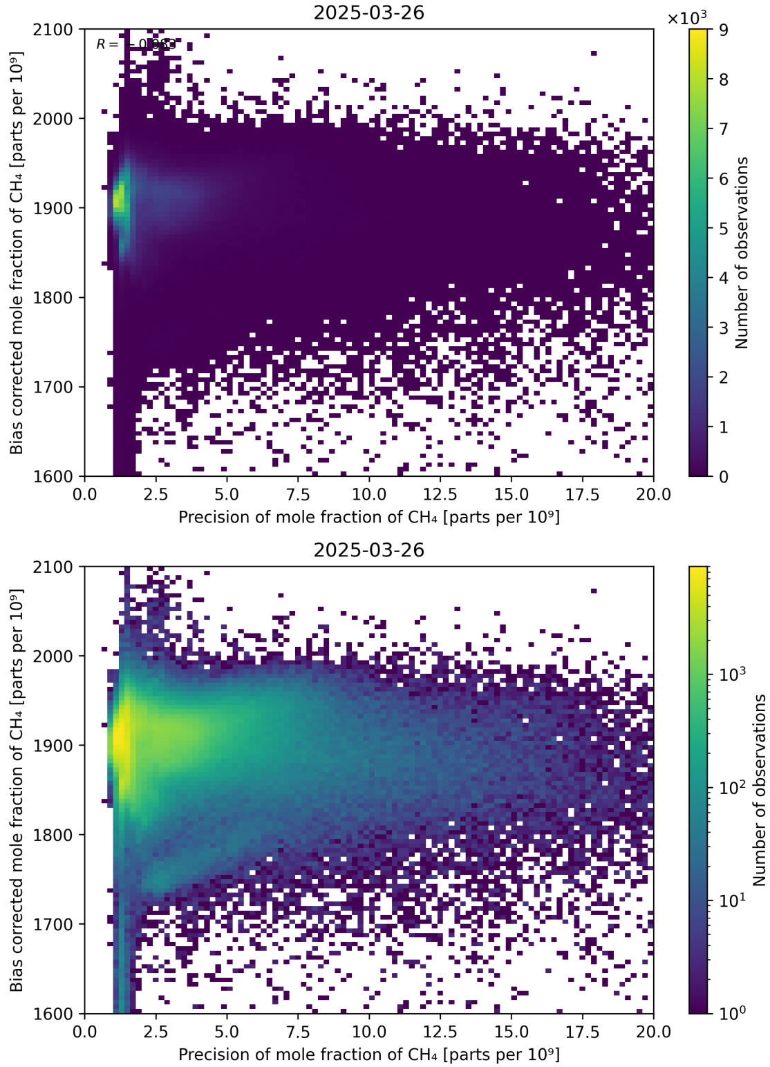
Figure 82: Scatter density plot of “Precision of mole fraction of CH 4 ” against “Bias corrected mole fraction of CH 4 ” for 2025-03-25 to 2025-03-27.
