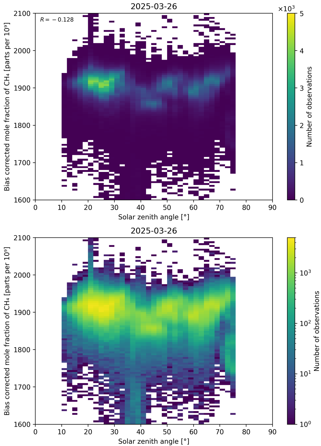
Figure 100: Scatter density plot of “Solar zenith angle” against “Bias corrected mole fraction of CH 4 ” for 2025-03-25 to 2025-03-27.
