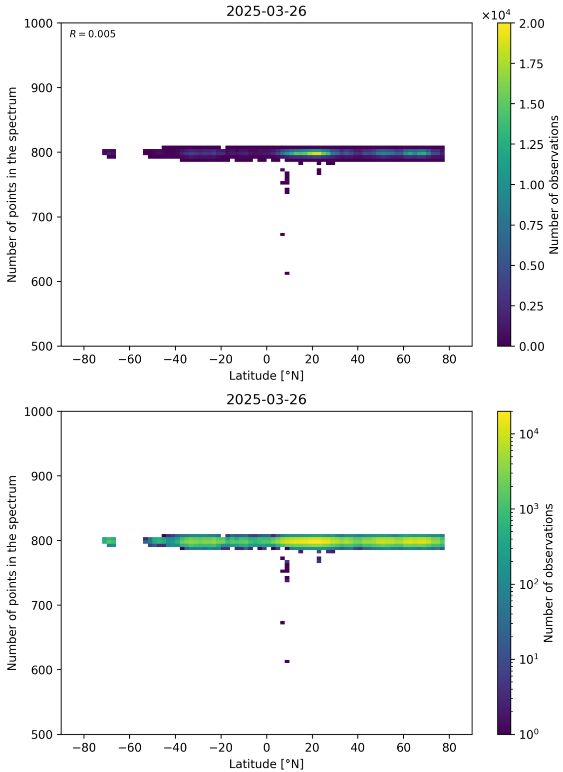
Figure 61: Scatter density plot of “Latitude” against “Number of points in the spectrum” for 2025-03-25 to 2025-03-27.
