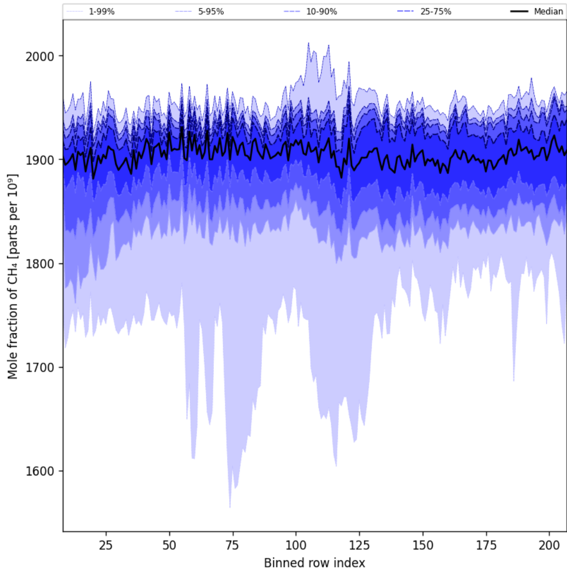
Figure 34: Along track statistics of “Mole fraction of CH 4 ” for 2025-03-25 to 2025-03-27
