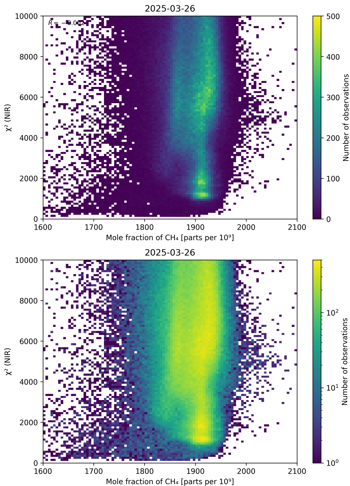
Figure 70: Scatter density plot of “Mole fraction of \text{CH}_4 ” against “ \chi^2 (NIR)” for 2025-03-25 to 2025-03-27.
