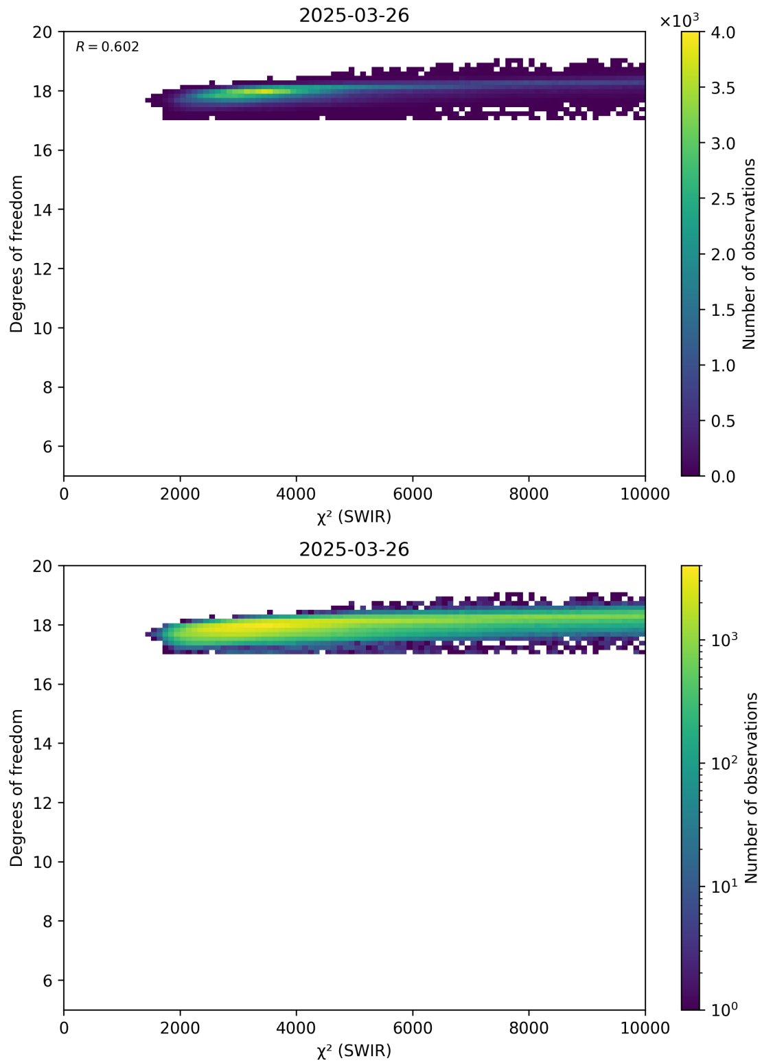
Figure 48: Scatter density plot of “ \chi^2 (SWIR)” against “Degrees of freedom” for 2025-03-25 to 2025-03-27.
