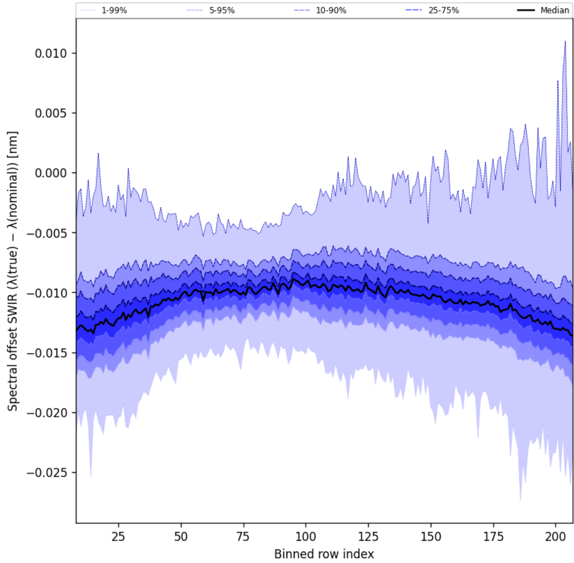
Figure 38: Along track statistics of “Spectral offset SWIR ( \lambda_{\text{true}} - \lambda_{\text{nominal}} )” for 2025-03-25 to 2025-03-27
