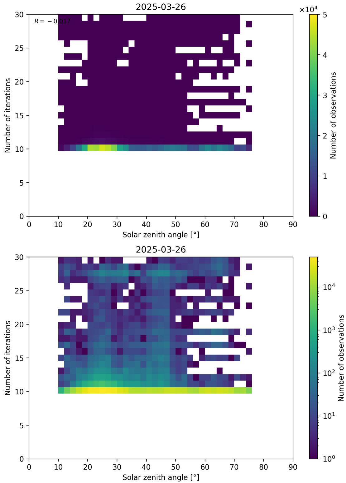
Figure 102: Scatter density plot of “Solar zenith angle” against “Number of iterations” for 2025-03-25 to 2025-03-27.
