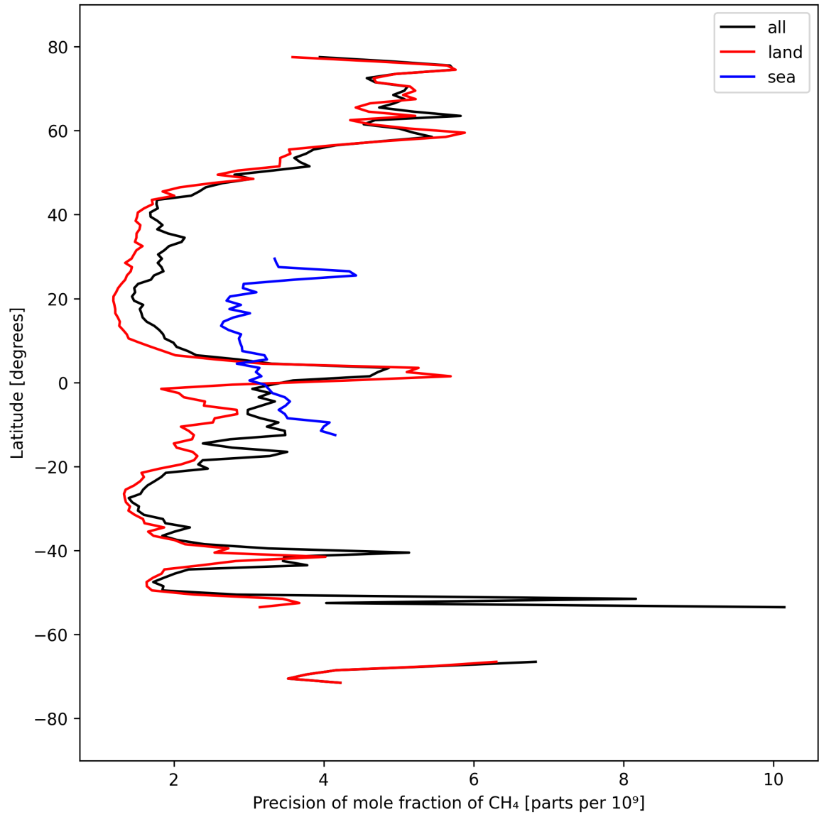
Figure 13: Zonal average of “Precision of mole fraction of CH 4 ” for 2025-03-25 to 2025-03-27.
