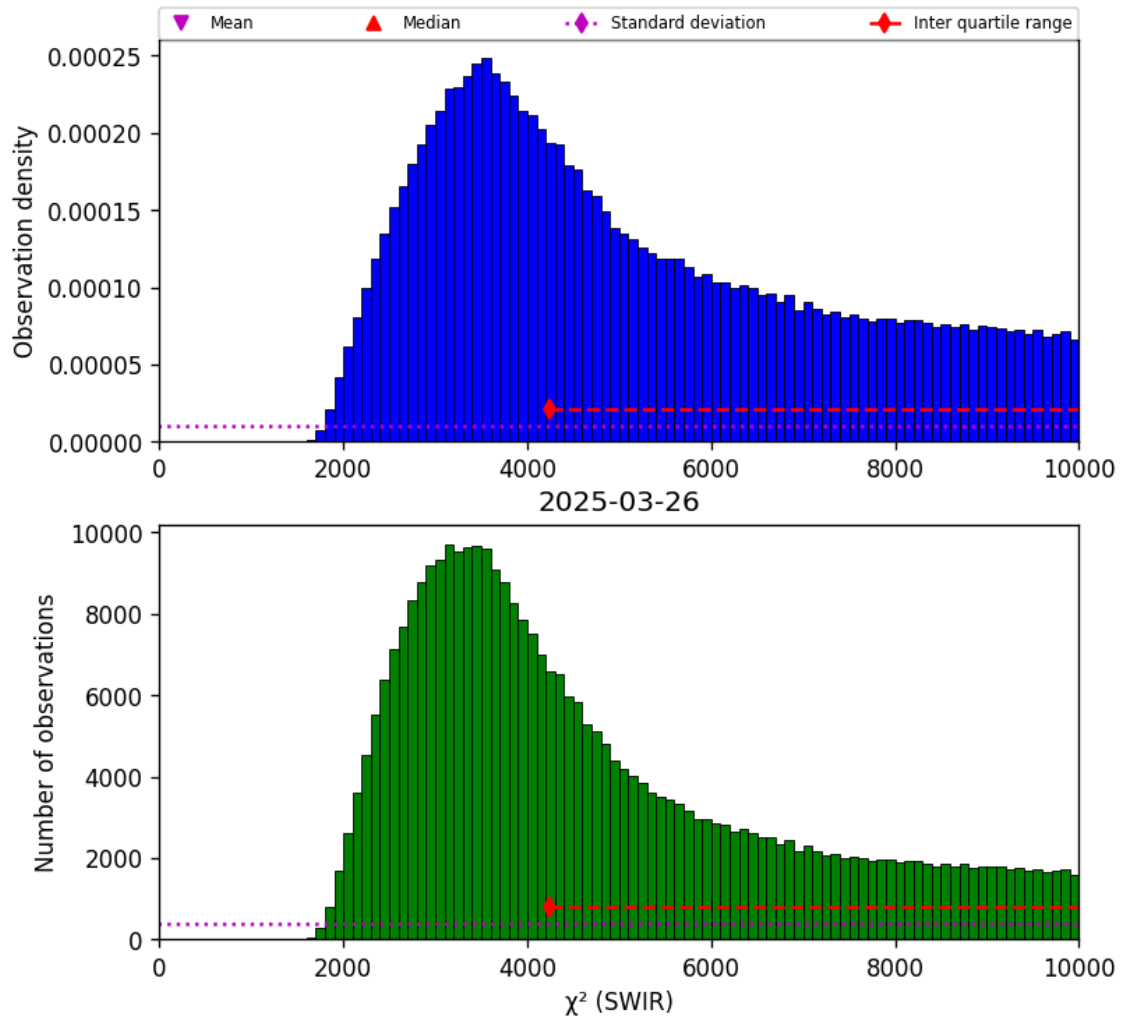
Figure 28: Histogram of " \chi^2 (SWIR)" for 2025-03-25 to 2025-03-27
