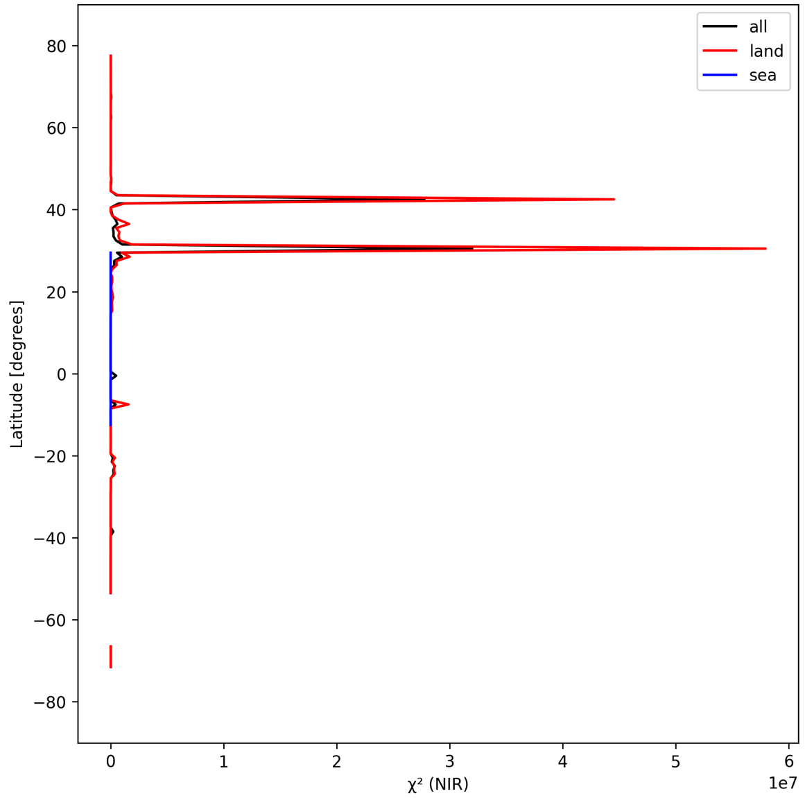
Figure 18: Zonal average of “ \chi^2 (NIR)” for 2025-03-25 to 2025-03-27.
