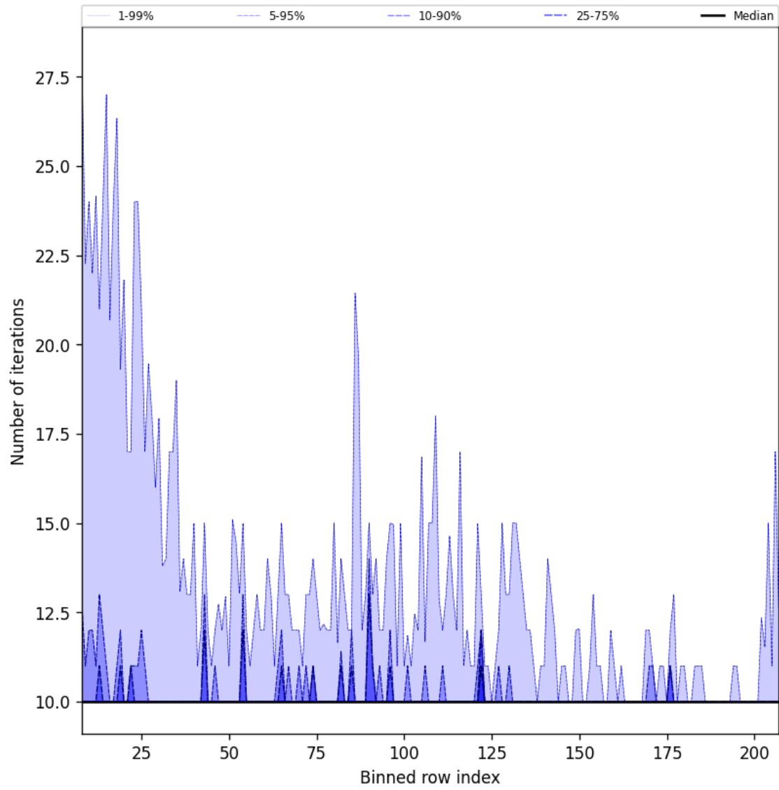
Figure 42: Along track statistics of “Number of iterations” for 2025-03-25 to 2025-03-27
