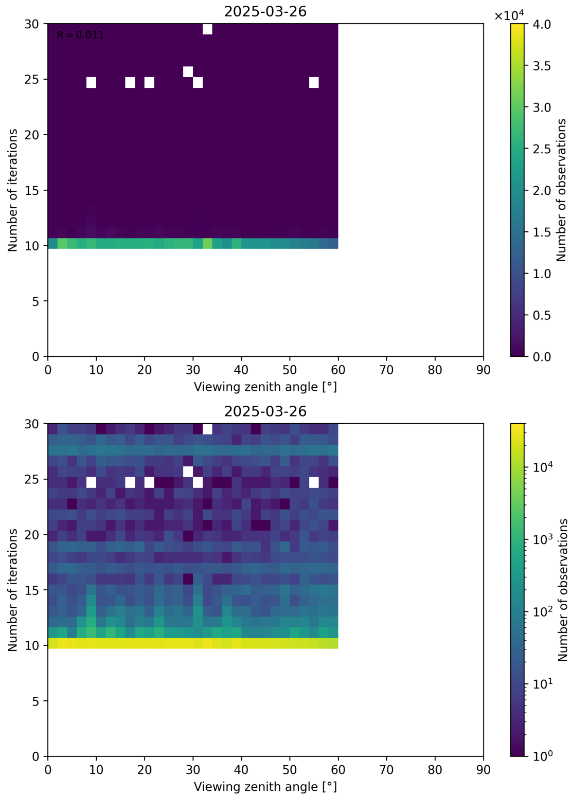
Figure 113: Scatter density plot of “Viewing zenith angle” against “Number of iterations” for 2025-03-25 to 2025-03-27.
