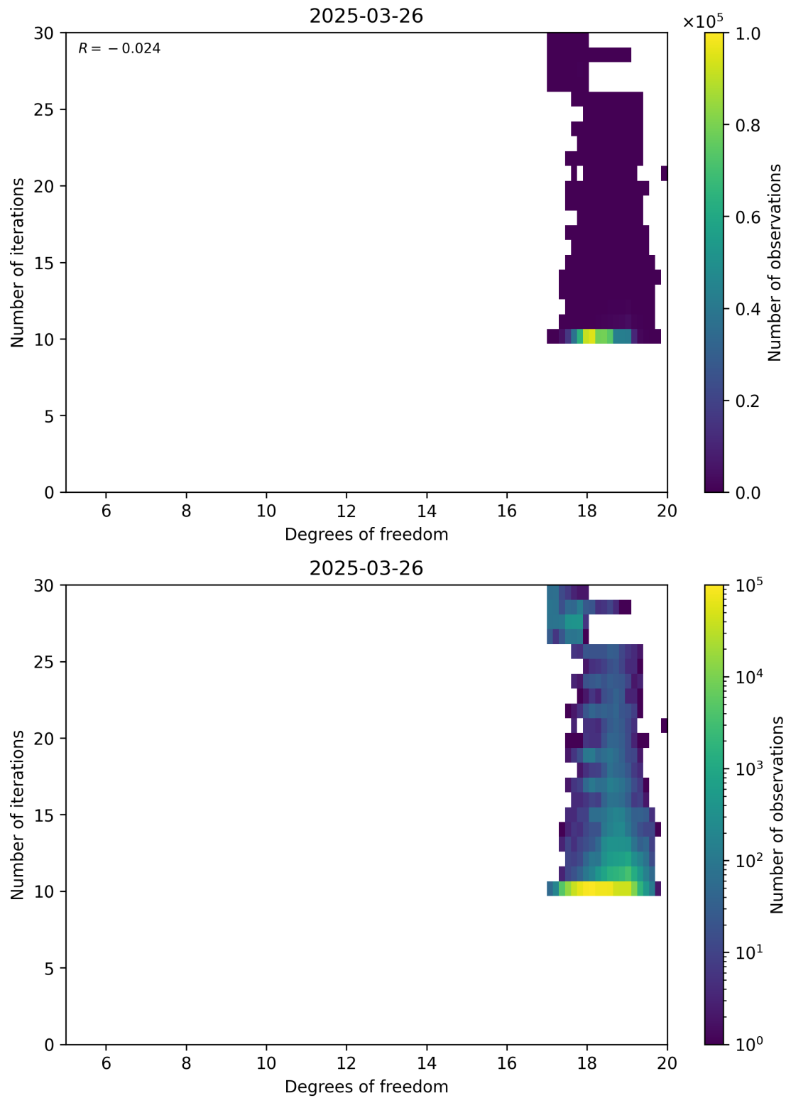
Figure 52: Scatter density plot of “Degrees of freedom” against “Number of iterations” for 2025-03-25 to 2025-03-27.
