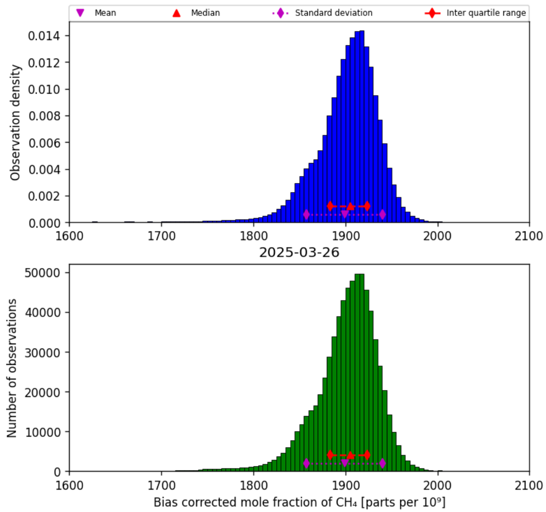
Figure 25: Histogram of “Bias corrected mole fraction of CH 4 ” for 2025-03-25 to 2025-03-27
