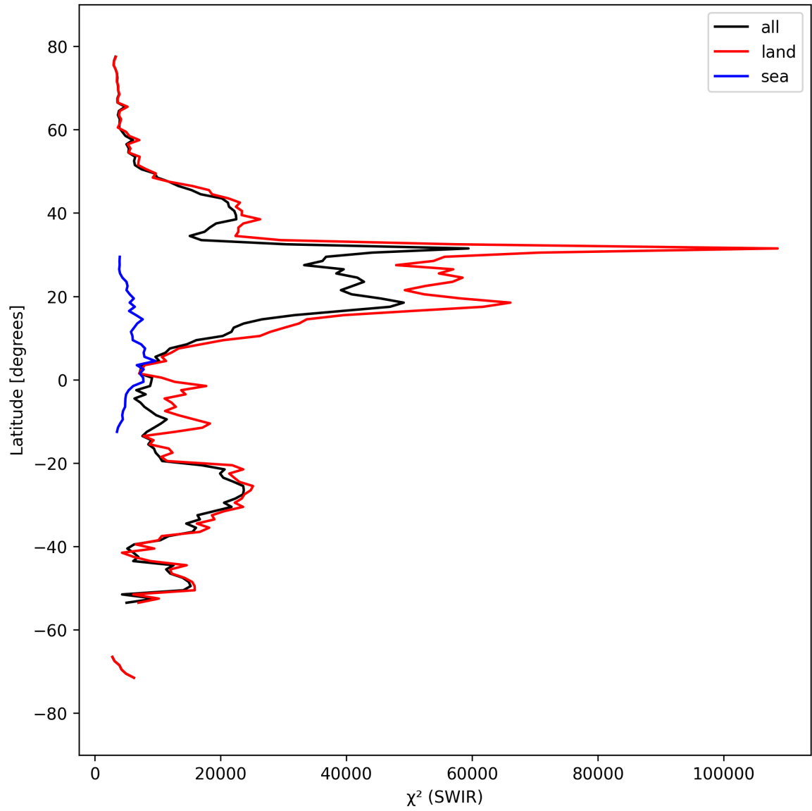
Figure 17: Zonal average of “ \chi^2 (SWIR)” for 2025-03-25 to 2025-03-27.
