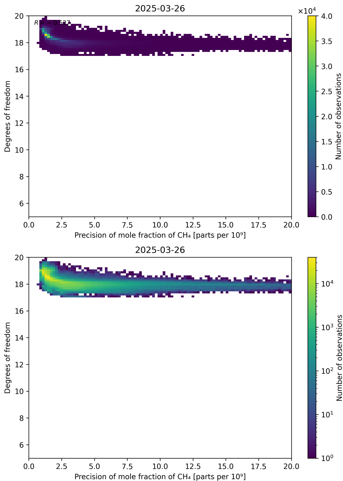
Figure 80: Scatter density plot of “Precision of mole fraction of CH 4 ” against “Degrees of freedom” for 2025-03-25 to 2025-03-27.
