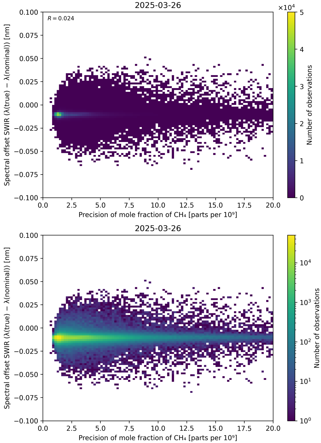
Figure 85: Scatter density plot of “Precision of mole fraction of CH 4 ” against “Spectral offset SWIR ( \lambda_{\text{true}} - \lambda_{\text{nominal}} )” for 2025-03-25 to 2025-03-27.
