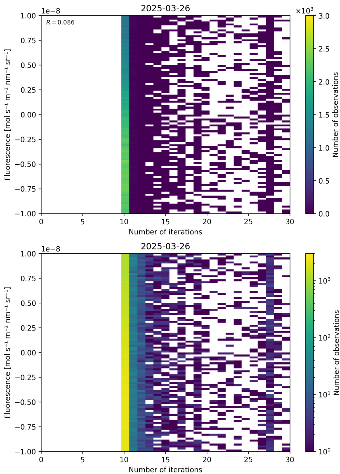
Figure 87: Scatter density plot of “Number of iterations” against “Fluorescence” for 2025-03-25 to 2025-03-27.
