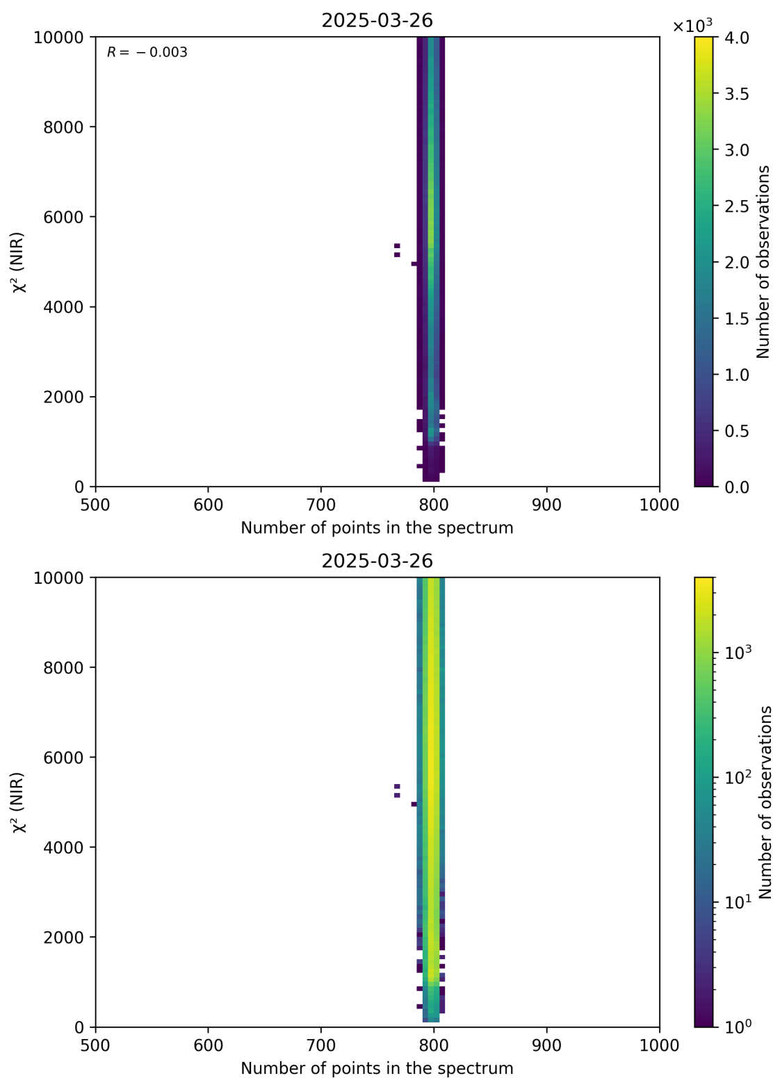
Figure 88: Scatter density plot of “Number of points in the spectrum” against “ \chi^2 (NIR)” for 2025-03-25 to 2025-03-27.
