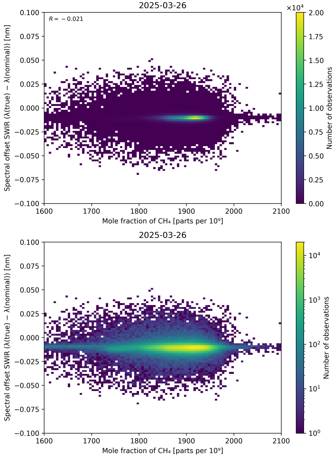
Figure 86: Scatter density plot of “Mole fraction of \text{CH}_4 ” against “Spectral offset SWIR ( \lambda_{\text{true}} - \lambda_{\text{nominal}} )” for 2025-03-25 to 2025-03-27.
