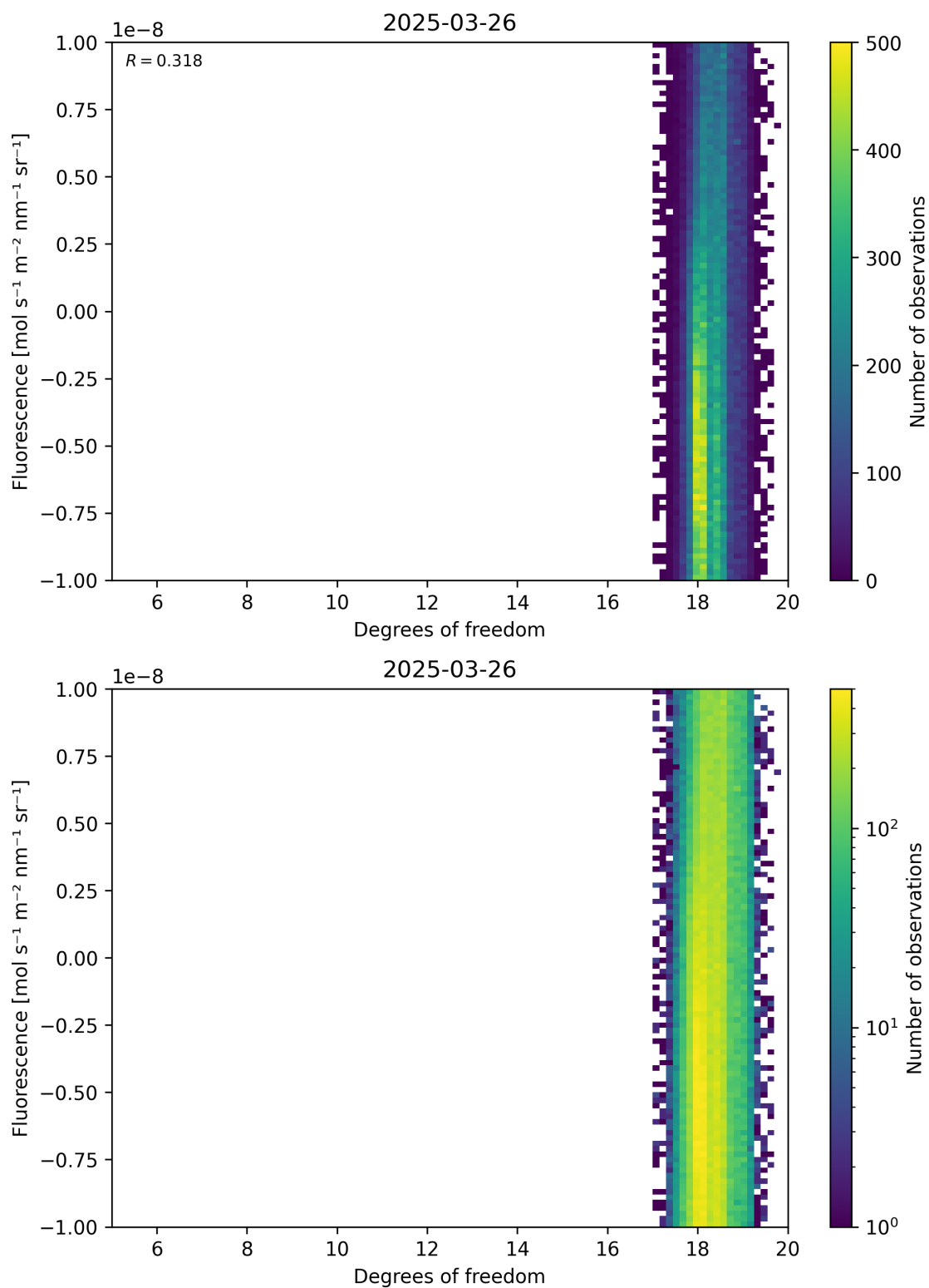
Figure 51: Scatter density plot of “Degrees of freedom” against “Fluorescence” for 2025-03-25 to 2025-03-27.
