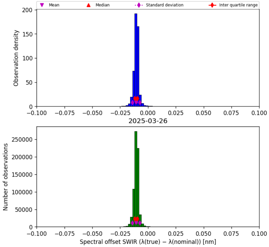
Figure 27: Histogram of “Spectral offset SWIR ( \lambda_{\text{true}} - \lambda_{\text{nominal}} )” for 2025-03-25 to 2025-03-27
