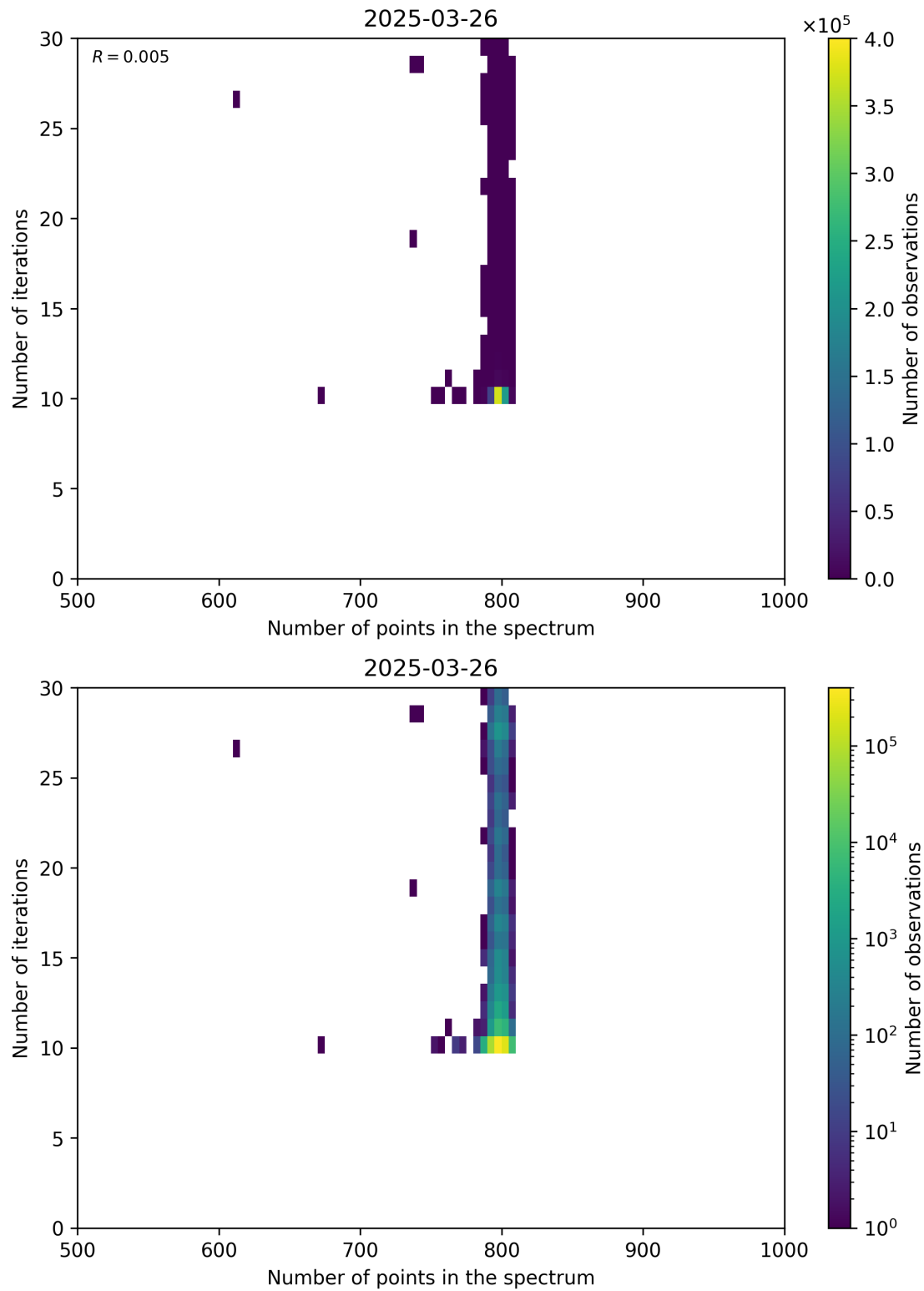
Figure 92: Scatter density plot of “Number of points in the spectrum” against “Number of iterations” for 2025-03-25 to 2025-03-27.
