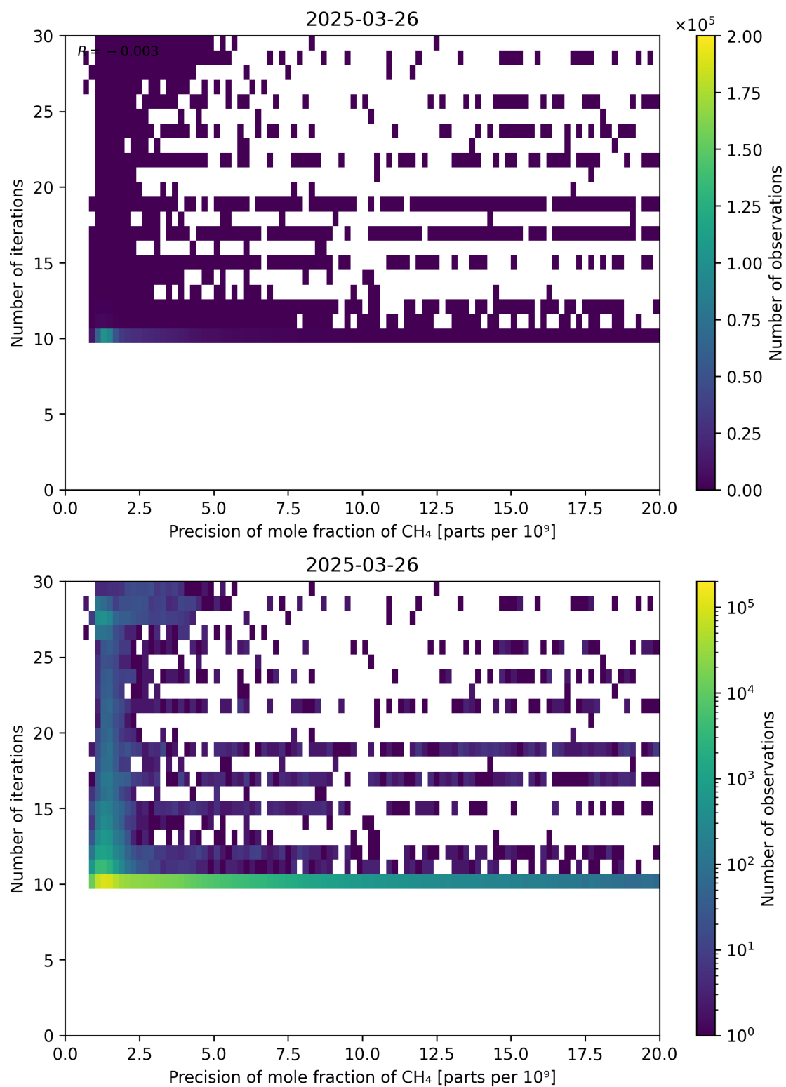
Figure 83: Scatter density plot of “Precision of mole fraction of CH 4 ” against “Number of iterations” for 2025-03-25 to 2025-03-27.
