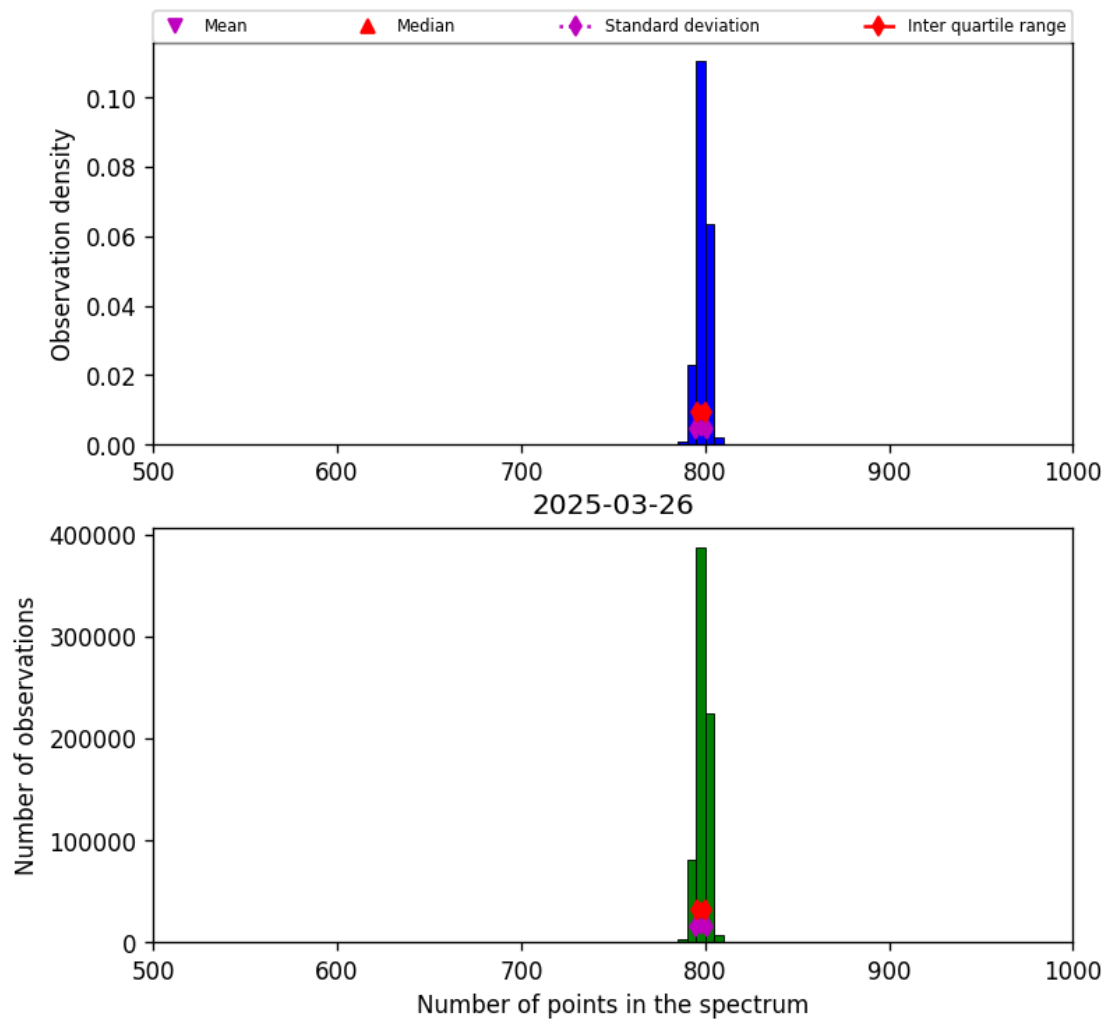
Figure 26: Histogram of “Number of points in the spectrum” for 2025-03-25 to 2025-03-27
