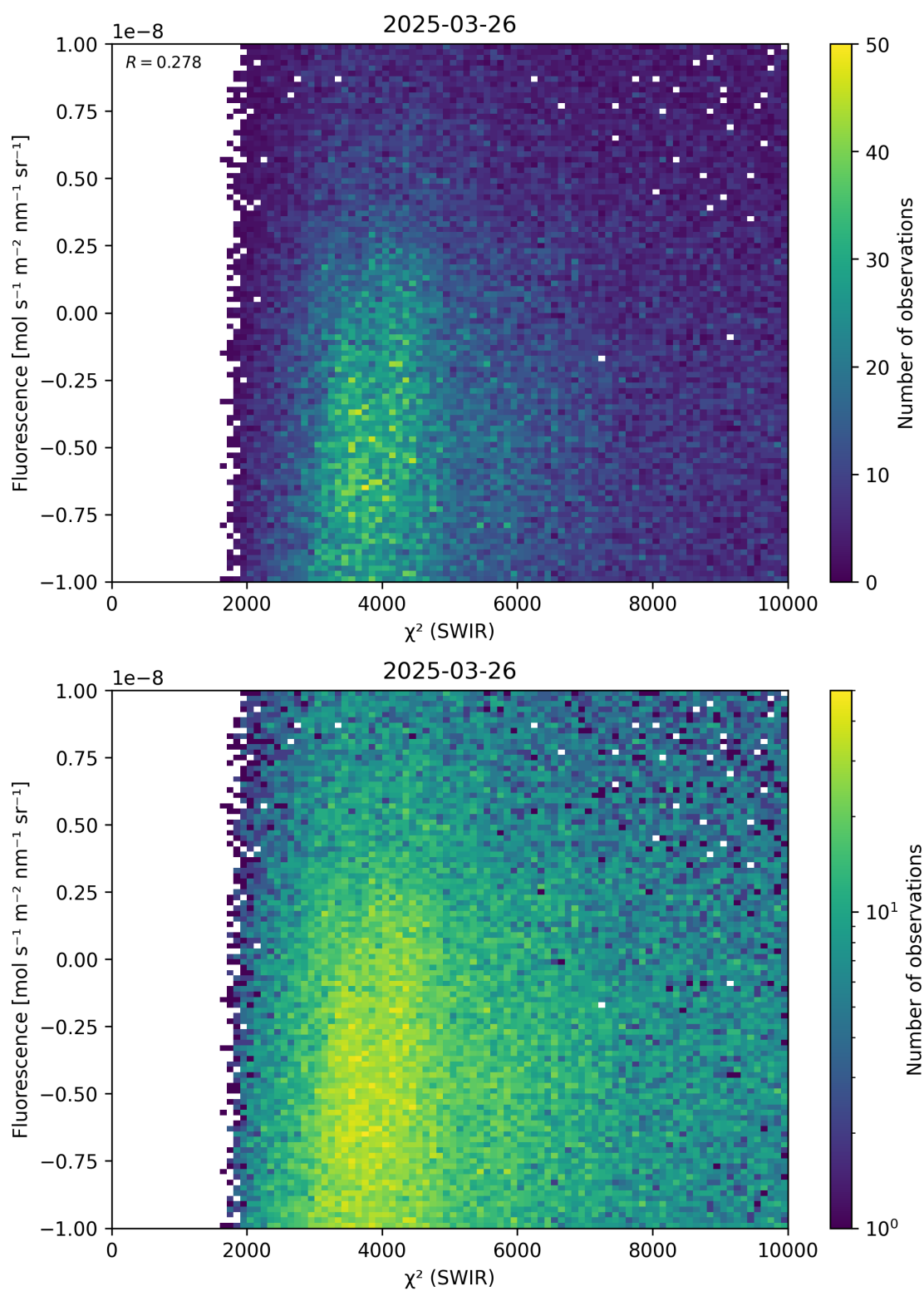
Figure 49: Scatter density plot of “ \chi^2 (SWIR)” against “Fluorescence” for 2025-03-25 to 2025-03-27.
