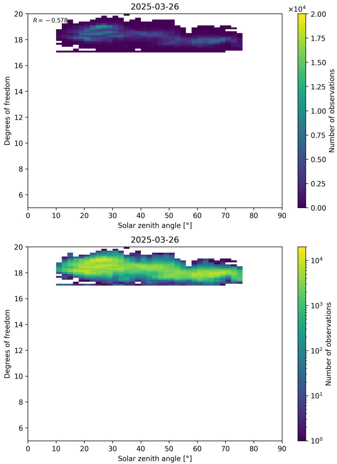
Figure 96: Scatter density plot of “Solar zenith angle” against “Degrees of freedom” for 2025-03-25 to 2025-03-27.
