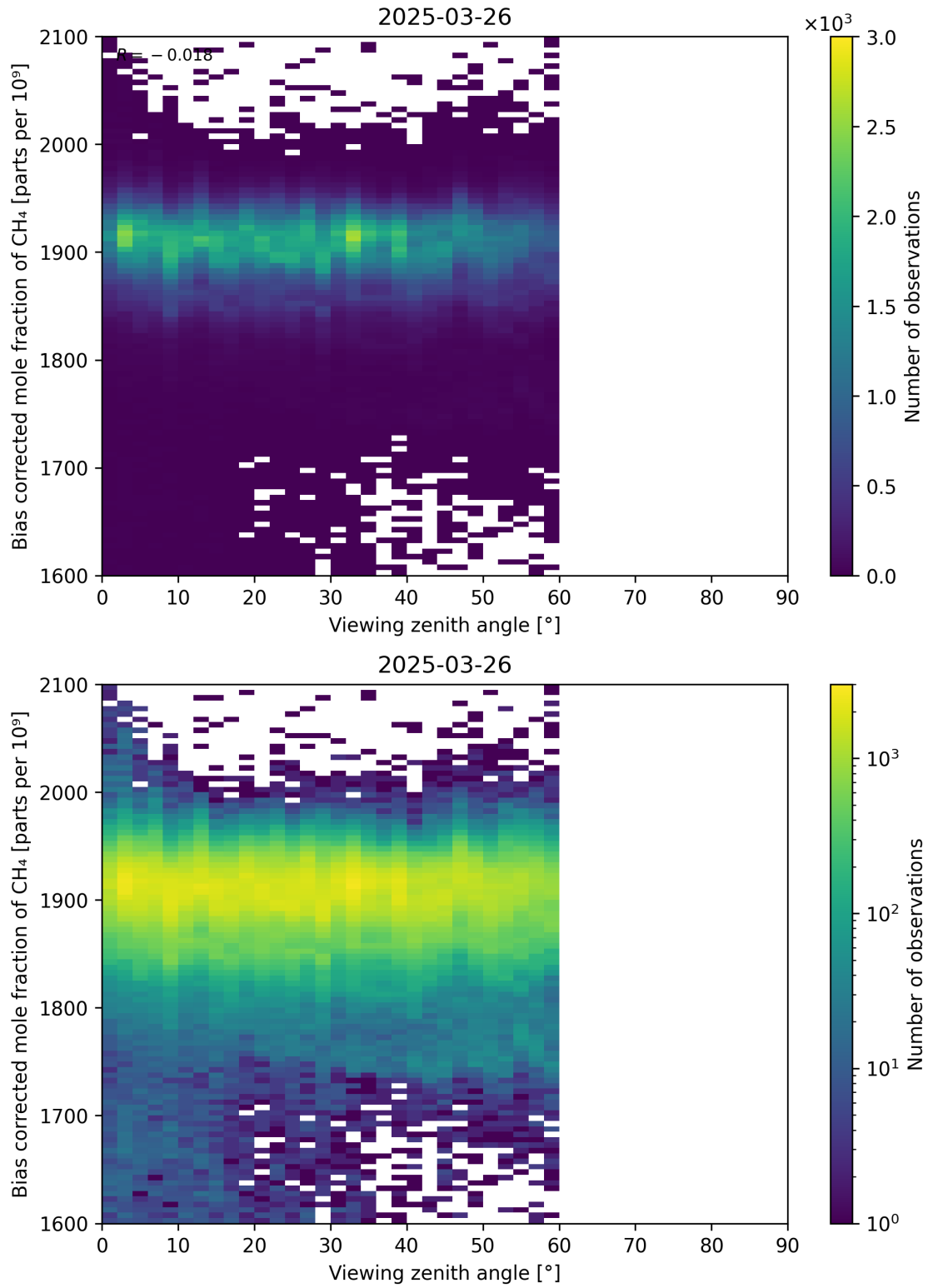
Figure 111: Scatter density plot of “Viewing zenith angle” against “Bias corrected mole fraction of CH 4 ” for 2025-03-25 to 2025-03-27.
