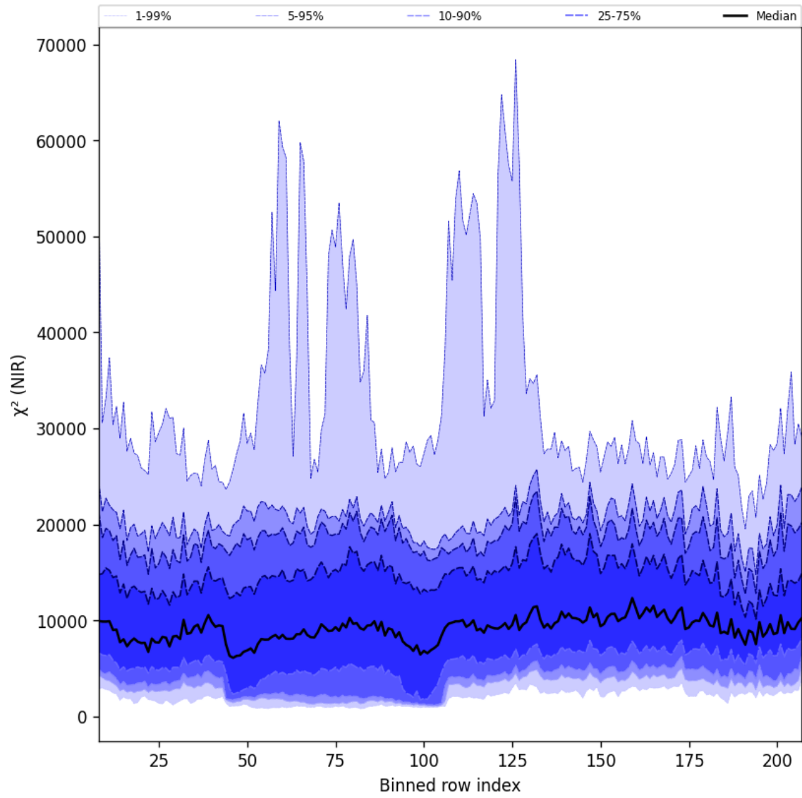
Figure 40: Along track statistics of “ \chi^2 (NIR)” for 2025-03-25 to 2025-03-27
