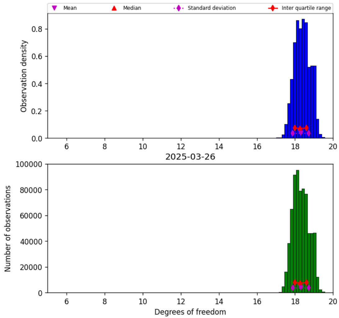
Figure 30: Histogram of “Degrees of freedom” for 2025-03-25 to 2025-03-27
