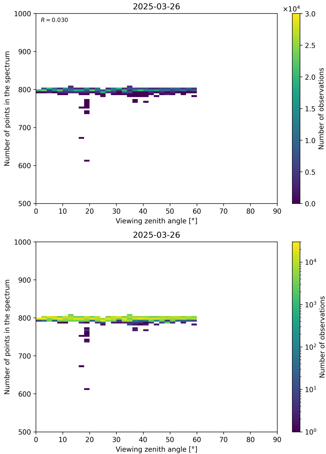
Figure 114: Scatter density plot of “Viewing zenith angle” against “Number of points in the spectrum” for 2025-03-25 to 2025-03-27.
