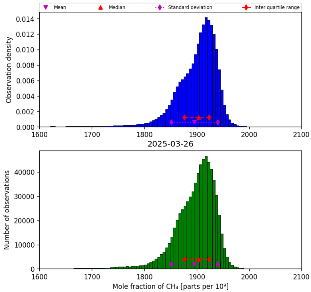
Figure 23: Histogram of “Mole fraction of CH 4 ” for 2025-03-25 to 2025-03-27
