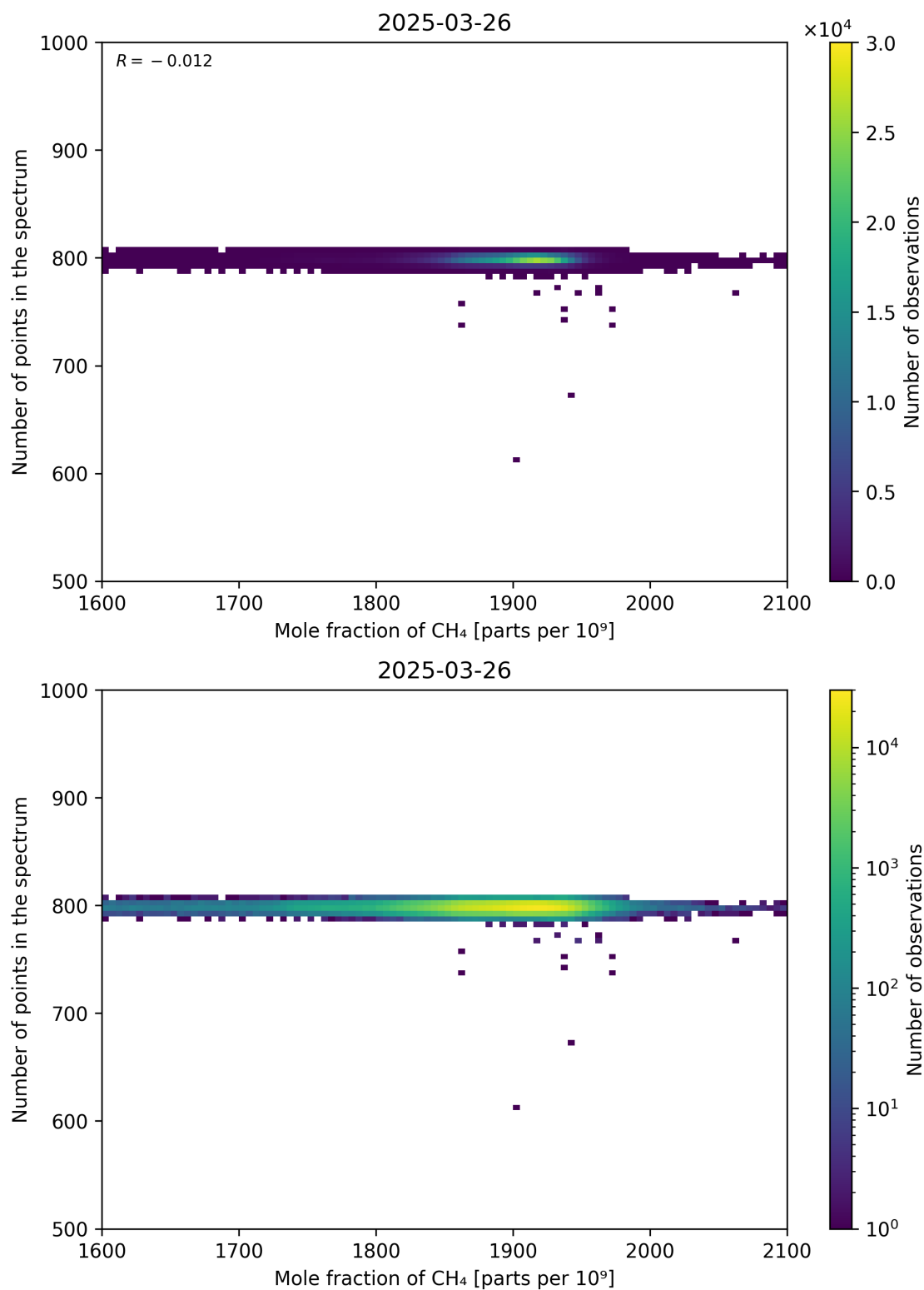
Figure 77: Scatter density plot of “Mole fraction of CH 4 ” against “Number of points in the spectrum” for 2025-03-25 to 2025-03-27.
