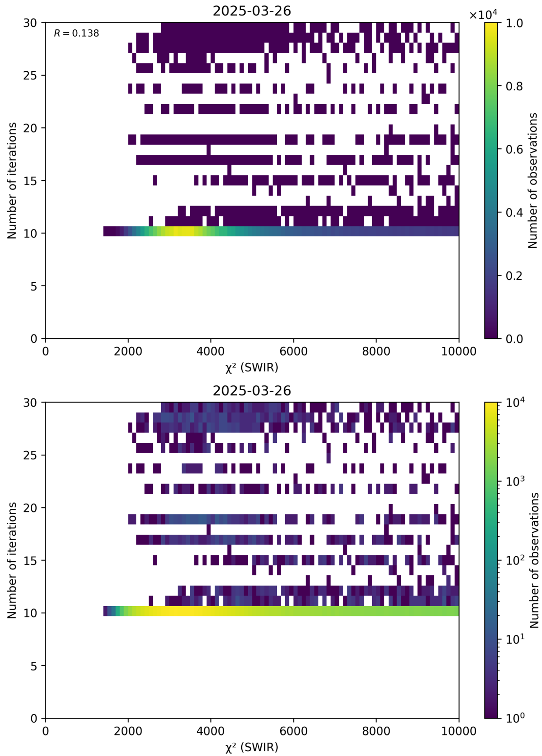
Figure 50: Scatter density plot of “ \chi^2 (SWIR)” against “Number of iterations” for 2025-03-25 to 2025-03-27.
