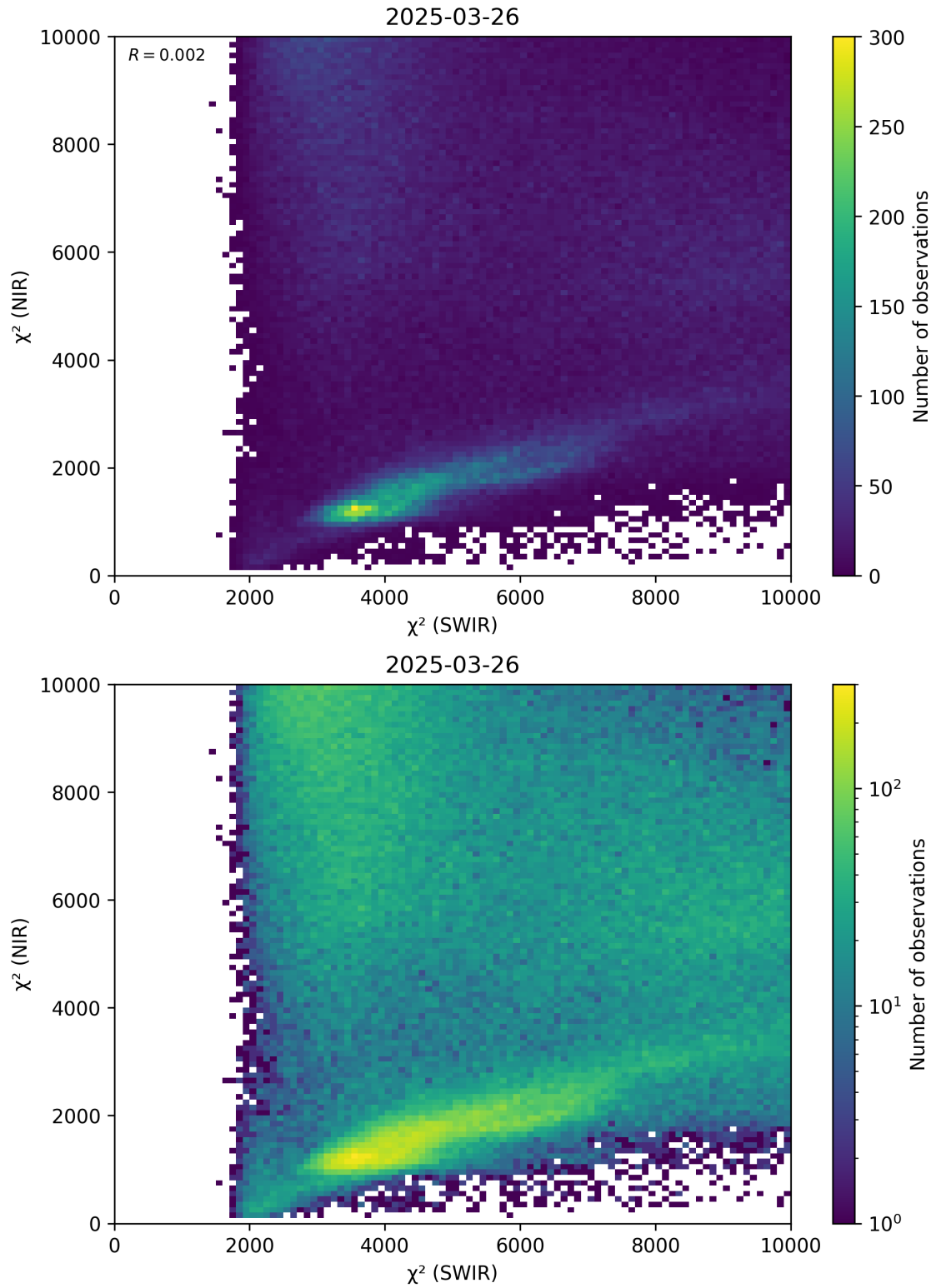
Figure 47: Scatter density plot of “ \chi^2 (SWIR)” against “ \chi^2 (NIR)” for 2025-03-25 to 2025-03-27.
