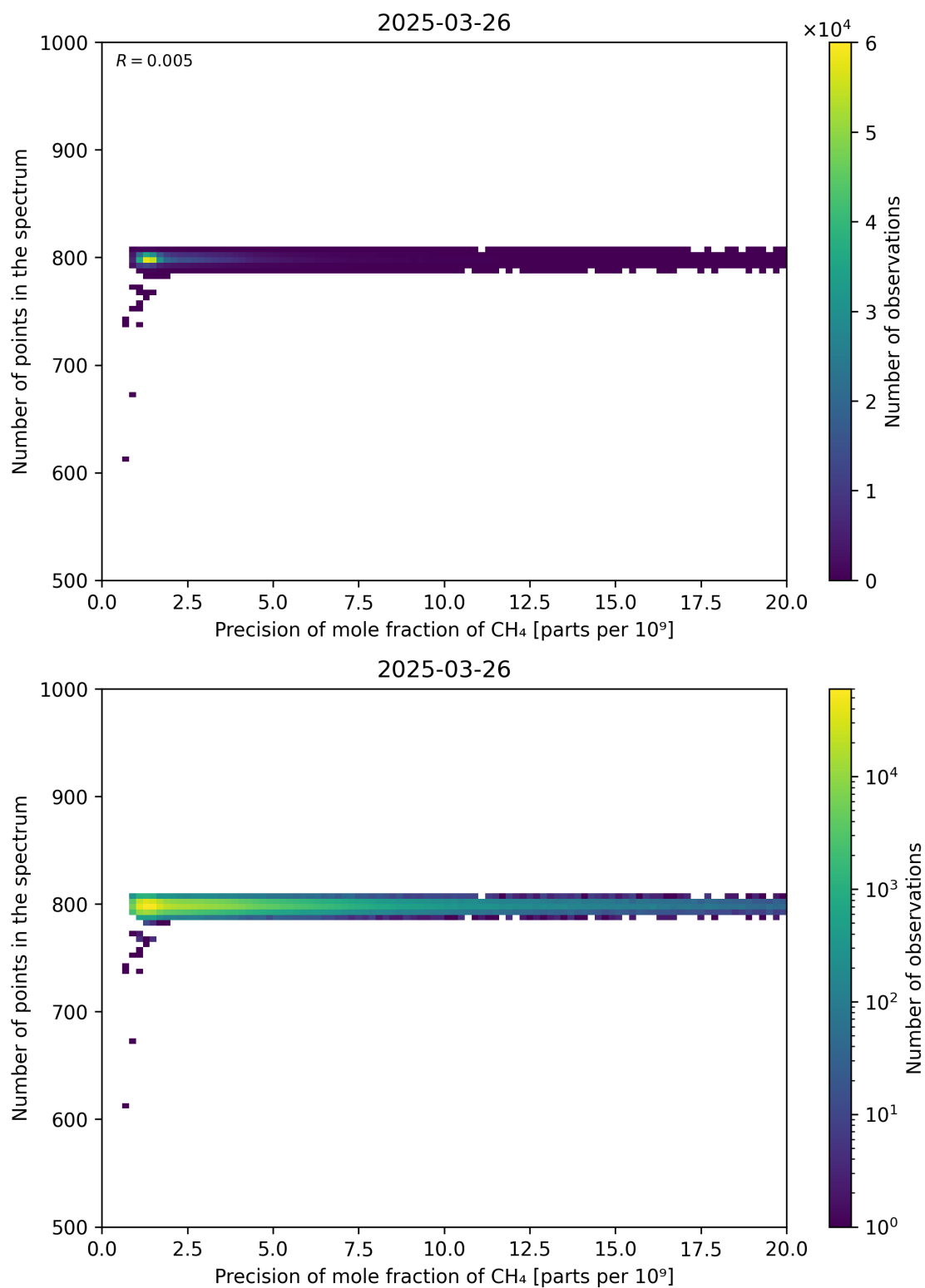
Figure 84: Scatter density plot of “Precision of mole fraction of CH 4 ” against “Number of points in the spectrum” for 2025-03-25 to 2025-03-27.
