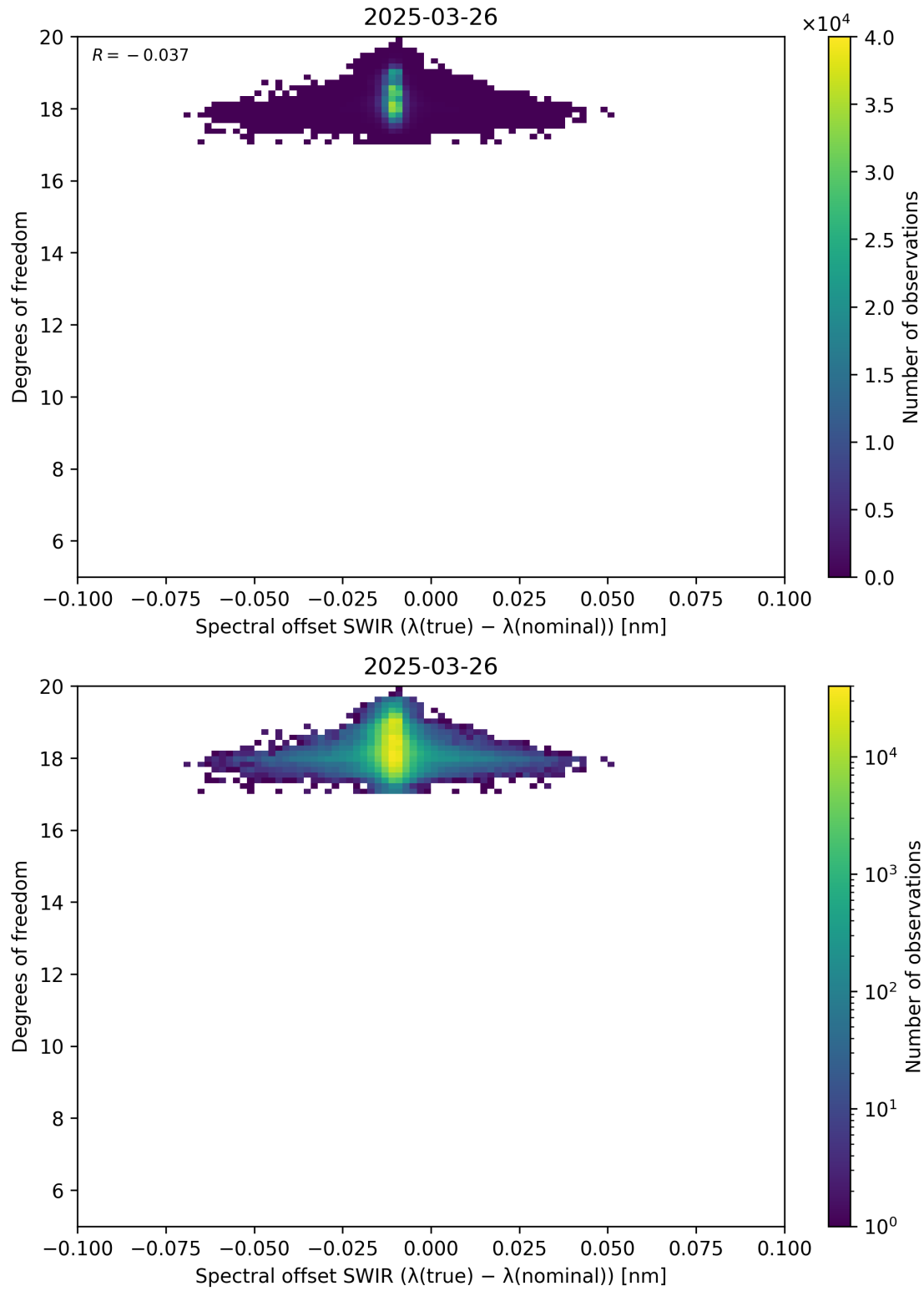
Figure 119: Scatter density plot of “Spectral offset SWIR ( \lambda_{\text{true}} - \lambda_{\text{nominal}} )” against “Degrees of freedom” for 2025-03-25 to 2025-03-27.
