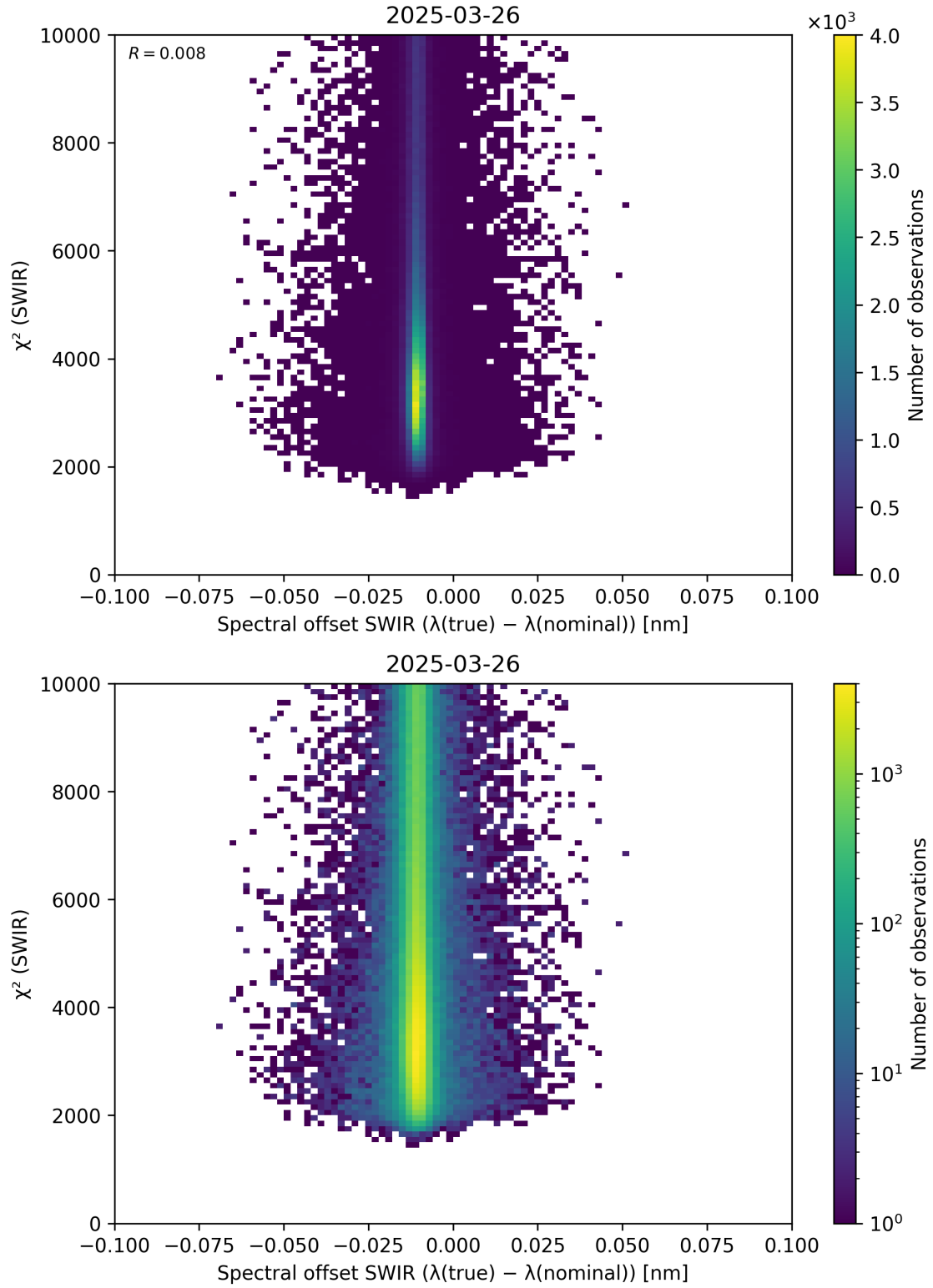
Figure 118: Scatter density plot of “Spectral offset SWIR ( \lambda_{\text{true}} - \lambda_{\text{nominal}} )” against “ \chi^2 (SWIR)” for 2025-03-25 to 2025-03-27.
