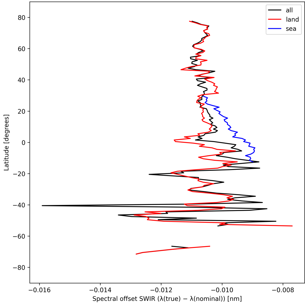
Figure 16: Zonal average of “Spectral offset SWIR ( \lambda_{\text{true}} - \lambda_{\text{nominal}} )” for 2025-03-25 to 2025-03-27.
