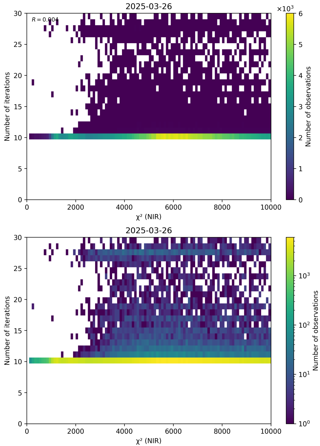
Figure 46: Scatter density plot of “ \chi^2 (NIR)” against “Number of iterations” for 2025-03-25 to 2025-03-27.
