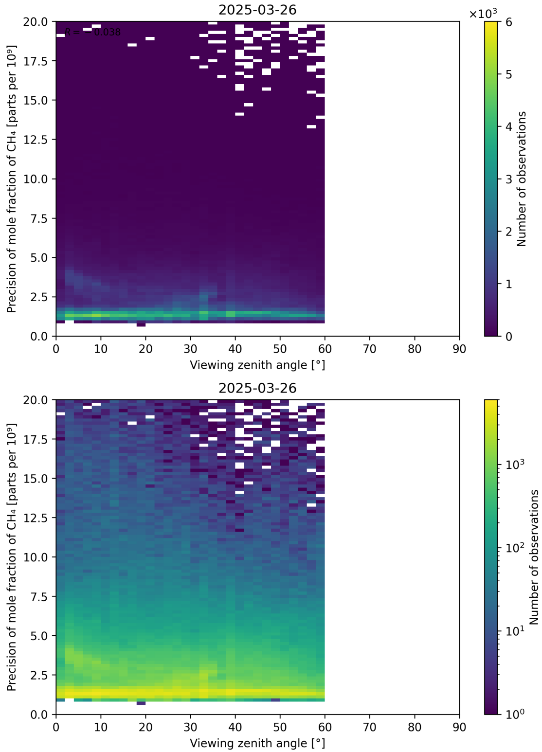
Figure 112: Scatter density plot of “Viewing zenith angle” against “Precision of mole fraction of CH 4 ” for 2025-03-25 to 2025-03-27.
