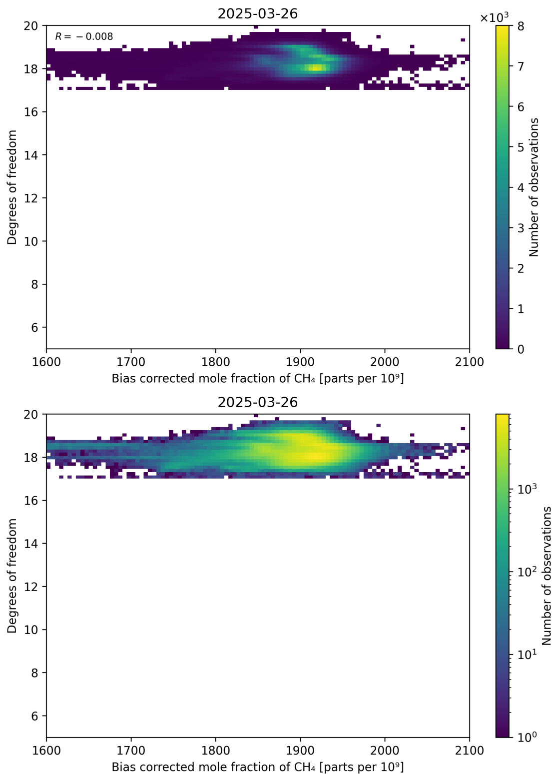
Figure 65: Scatter density plot of “Bias corrected mole fraction of CH 4 ” against “Degrees of freedom” for 2025-03-25 to 2025-03-27.
