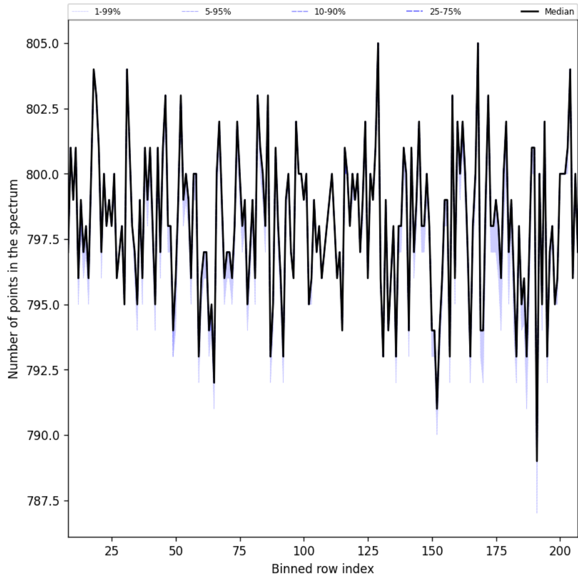
Figure 37: Along track statistics of “Number of points in the spectrum” for 2025-03-25 to 2025-03-27
