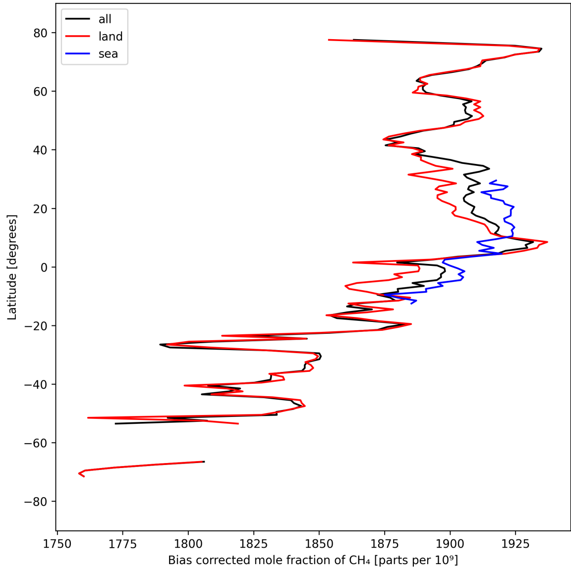
Figure 14: Zonal average of “Bias corrected mole fraction of \text{CH}_4 ” for 2025-03-25 to 2025-03-27.
