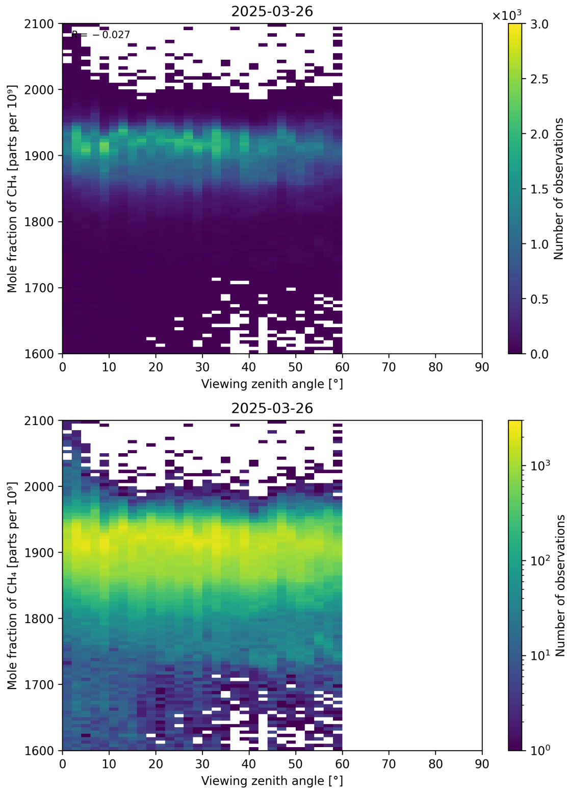
Figure 110: Scatter density plot of “Viewing zenith angle” against “Mole fraction of CH 4 ” for 2025-03-25 to 2025-03-27.
