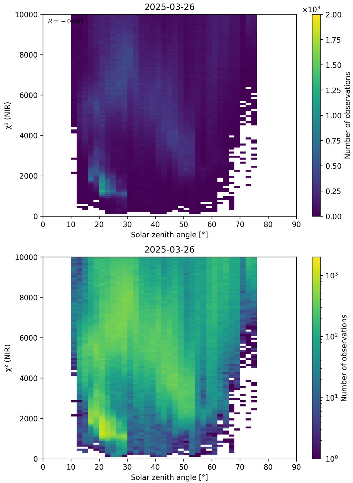
Figure 94: Scatter density plot of “Solar zenith angle” against “ \chi^2 (NIR)” for 2025-03-25 to 2025-03-27.
