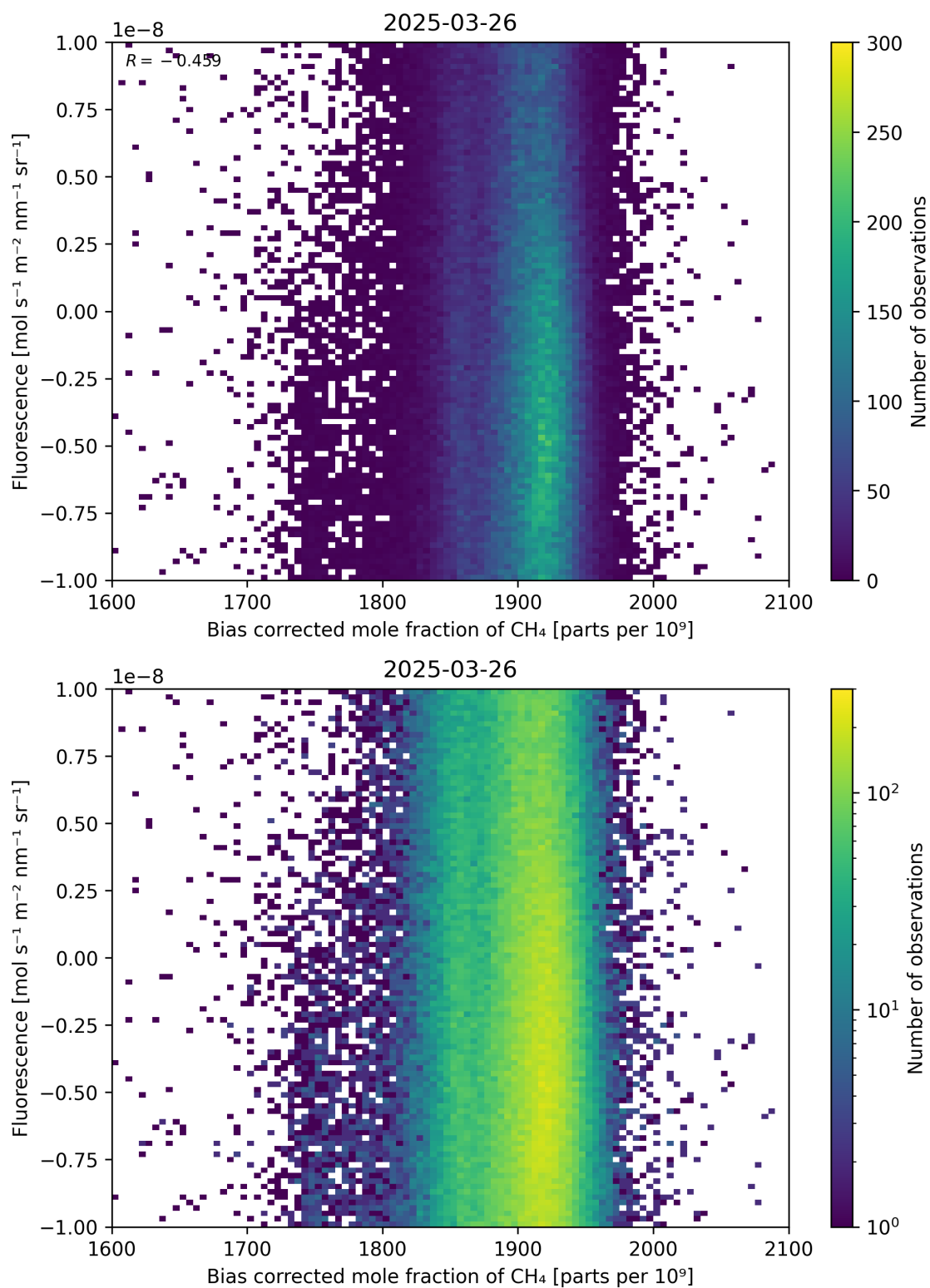
Figure 66: Scatter density plot of “Bias corrected mole fraction of \text{CH}_4 ” against “Fluorescence” for 2025-03-25 to 2025-03-27.
