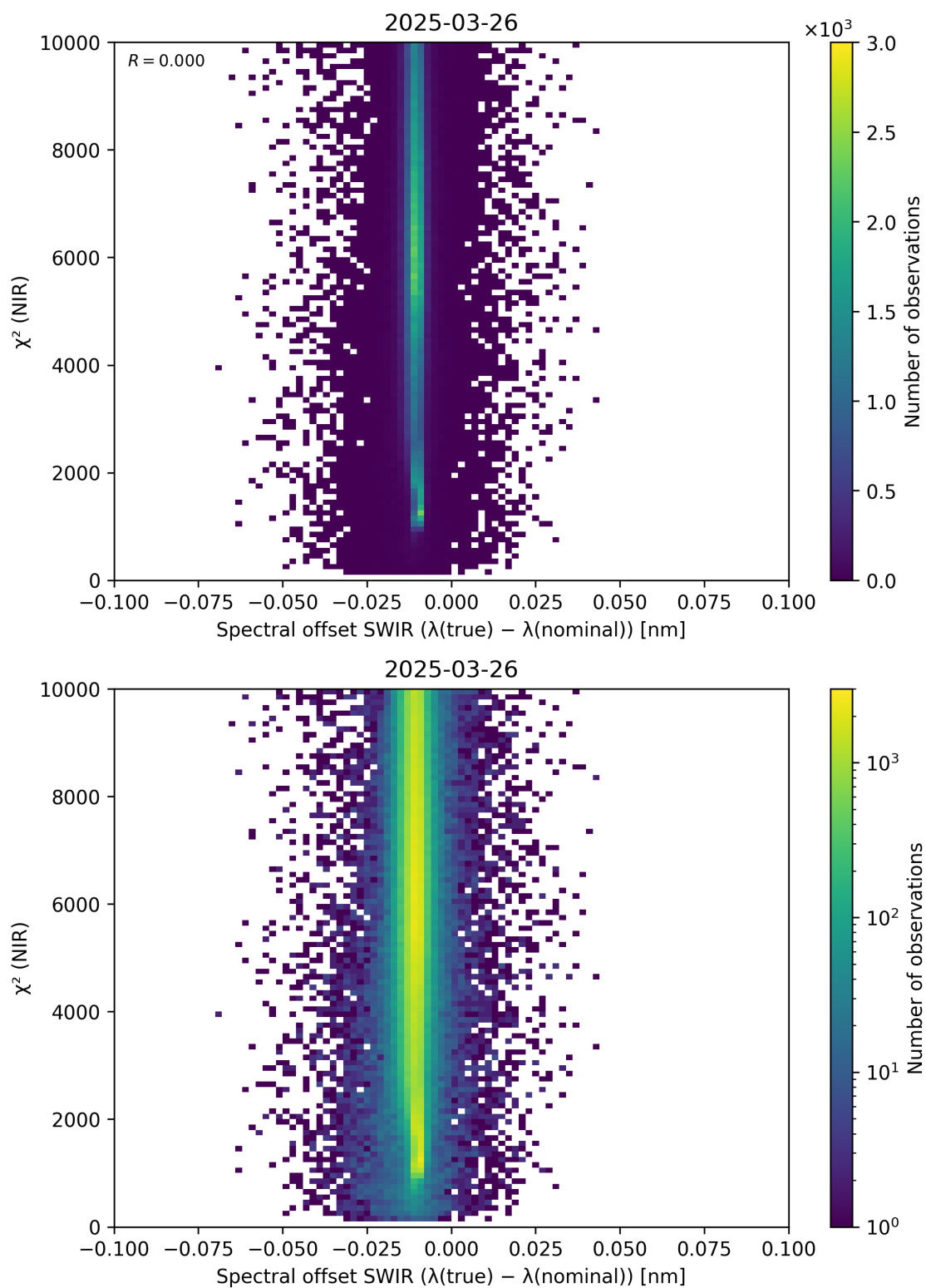
Figure 117: Scatter density plot of “Spectral offset SWIR ( \lambda_{\text{true}} - \lambda_{\text{nominal}} )” against “ \chi^2 (NIR)” for 2025-03-25 to 2025-03-27.
