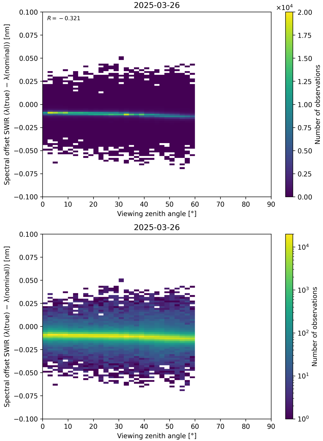
Figure 116: Scatter density plot of “Viewing zenith angle” against “Spectral offset SWIR ( \lambda_{\text{true}} - \lambda_{\text{nominal}} )” for 2025-03-25 to 2025-03-27.
