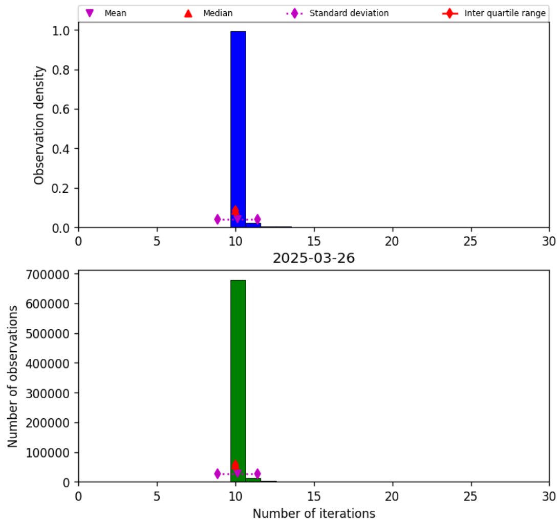
Figure 31: Histogram of “Number of iterations” for 2025-03-25 to 2025-03-27
