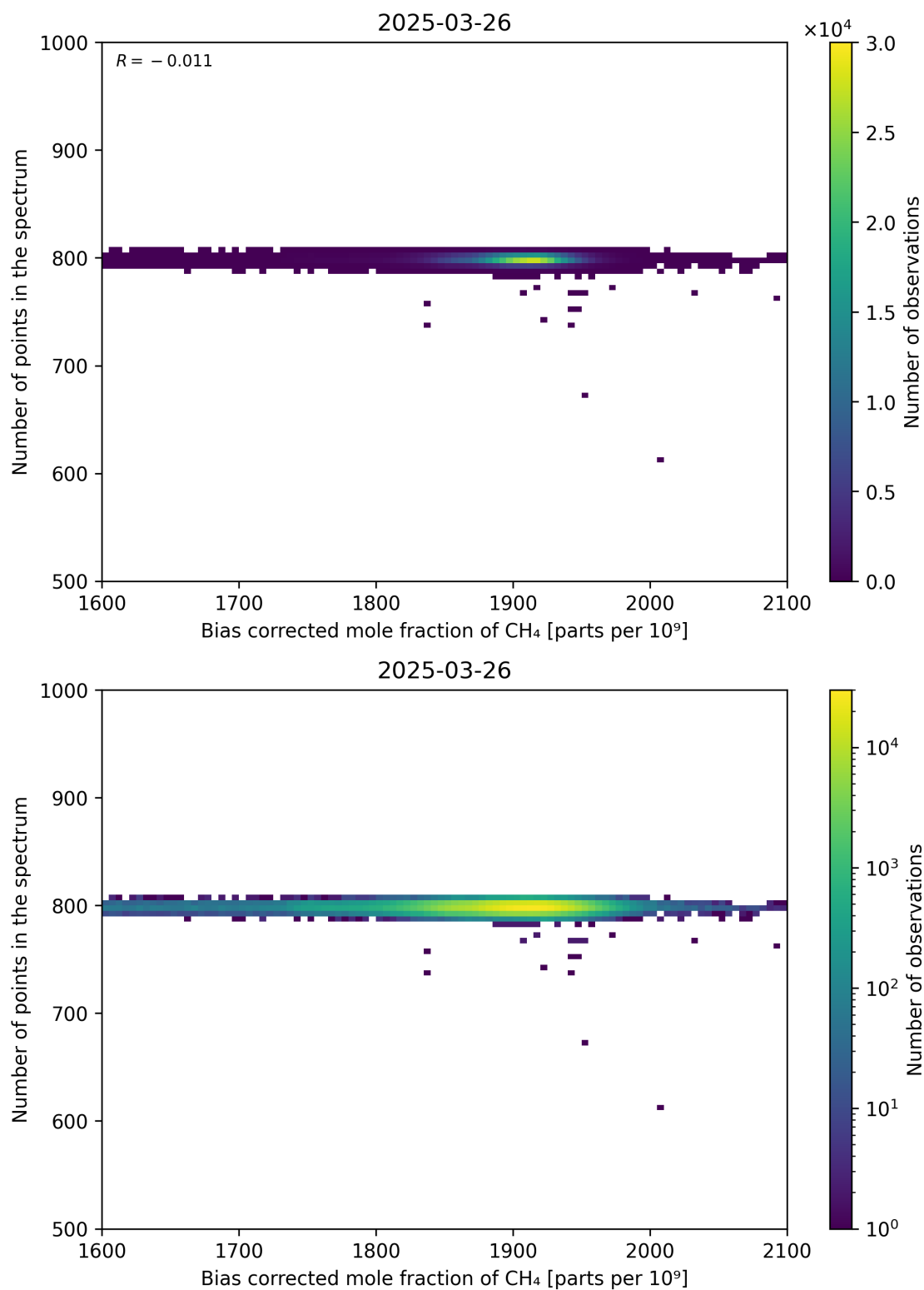
Figure 68: Scatter density plot of “Bias corrected mole fraction of CH 4 ” against “Number of points in the spectrum” for 2025-03-25 to 2025-03-27.
