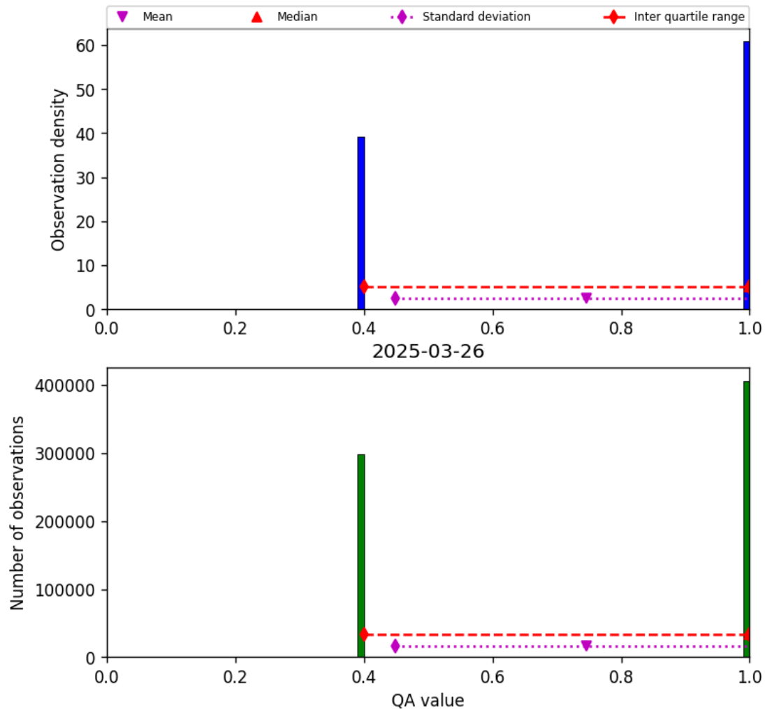
Figure 22: Histogram of “QA value” for 2025-03-25 to 2025-03-27
