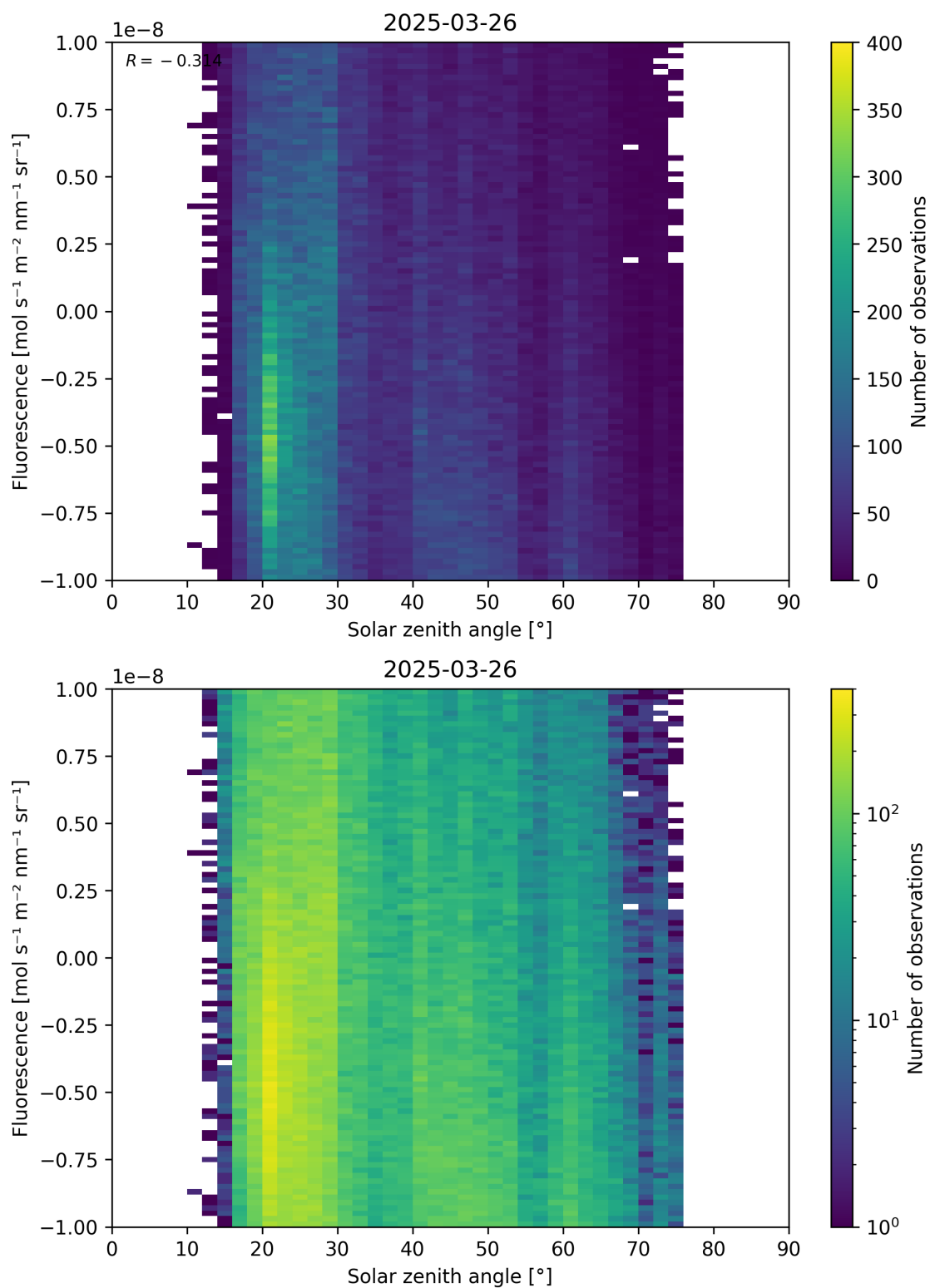
Figure 97: Scatter density plot of “Solar zenith angle” against “Fluorescence” for 2025-03-25 to 2025-03-27.
