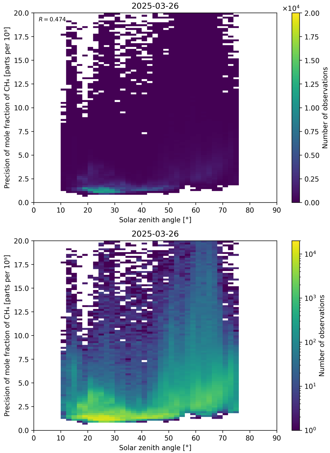
Figure 101: Scatter density plot of “Solar zenith angle” against “Precision of mole fraction of \text{CH}_4 ” for 2025-03-25 to 2025-03-27.
