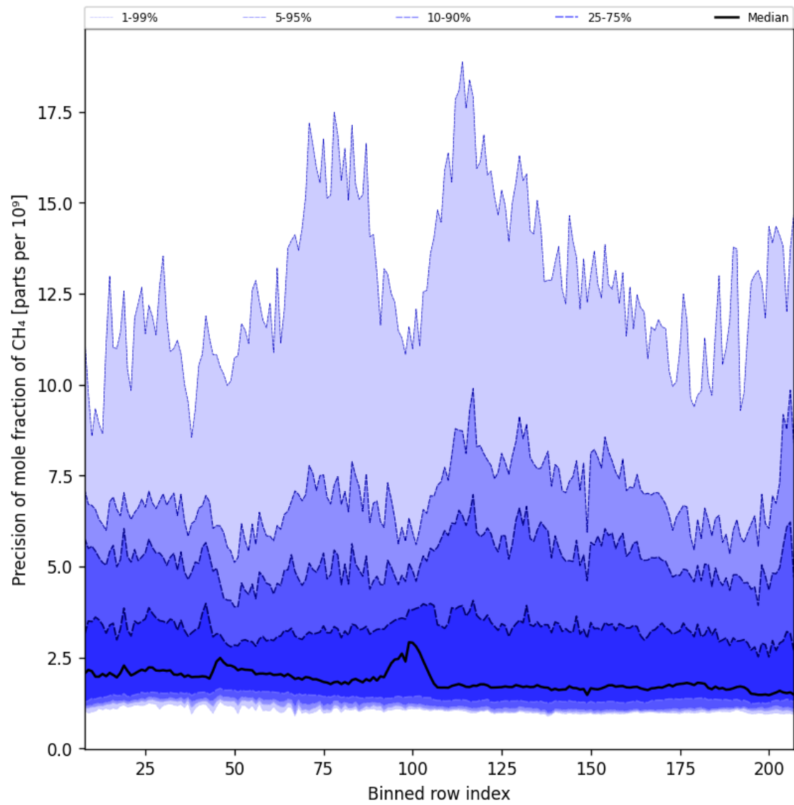
Figure 35: Along track statistics of “Precision of mole fraction of CH 4 ” for 2025-03-25 to 2025-03-27
