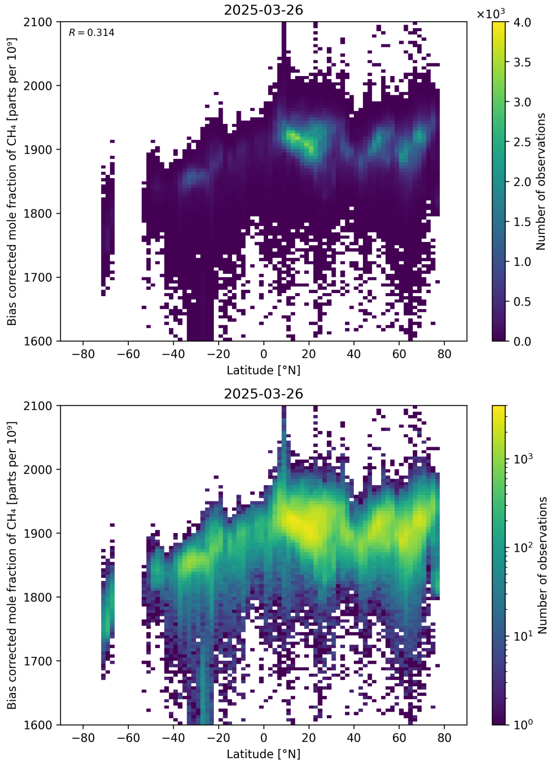
Figure 58: Scatter density plot of “Latitude” against “Bias corrected mole fraction of CH 4 ” for 2025-03-25 to 2025-03-27.
