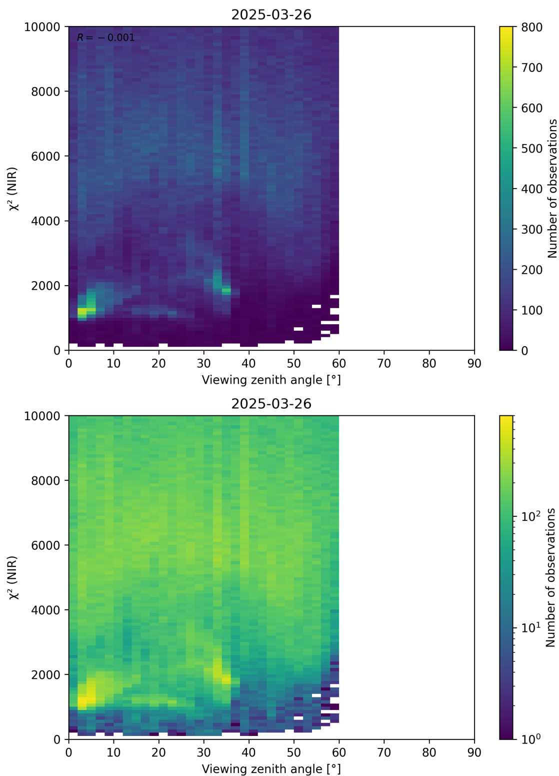
Figure 105: Scatter density plot of “Viewing zenith angle” against “ \chi^2 (NIR)” for 2025-03-25 to 2025-03-27.
