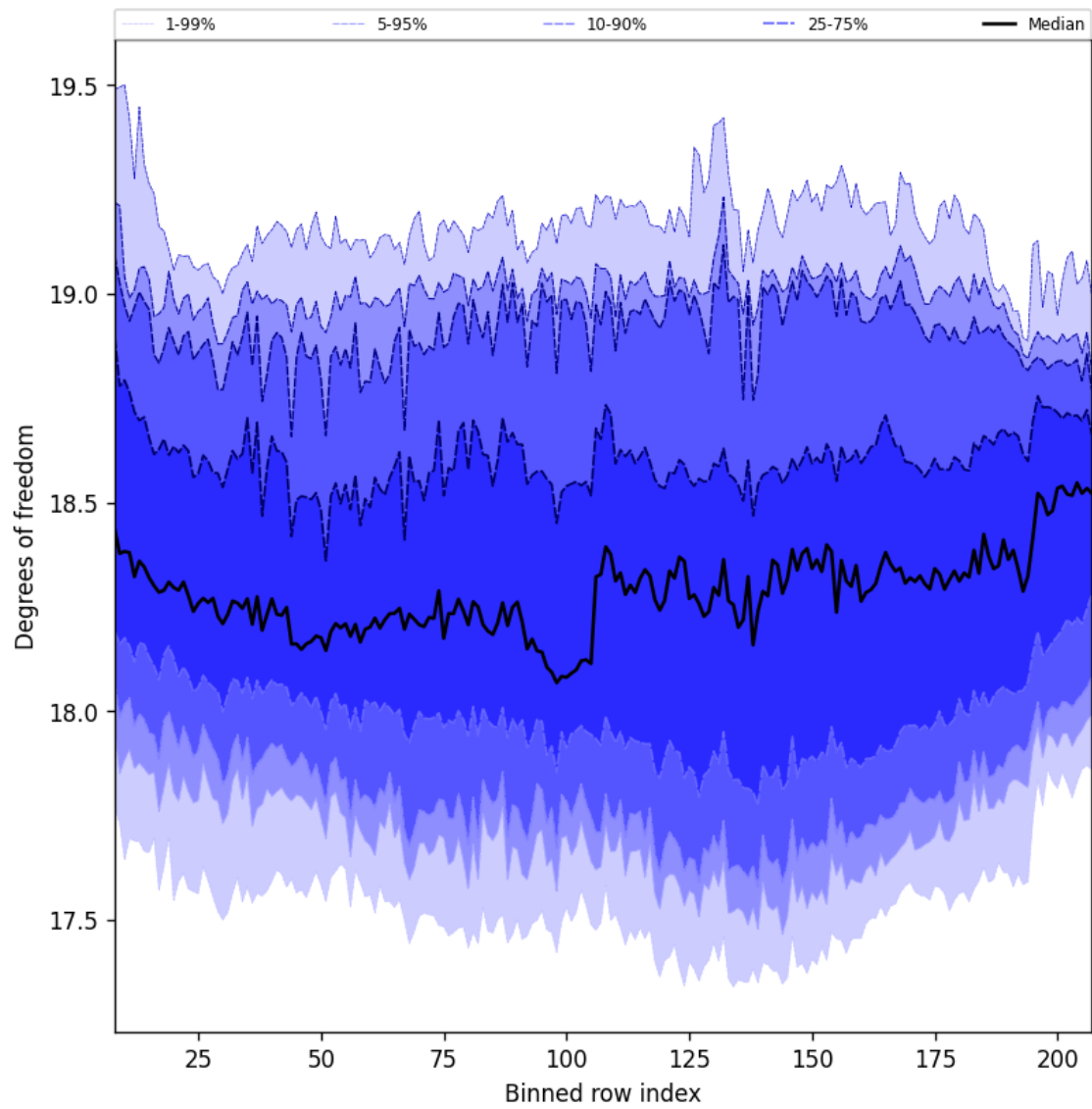
Figure 41: Along track statistics of “Degrees of freedom” for 2025-03-25 to 2025-03-27
