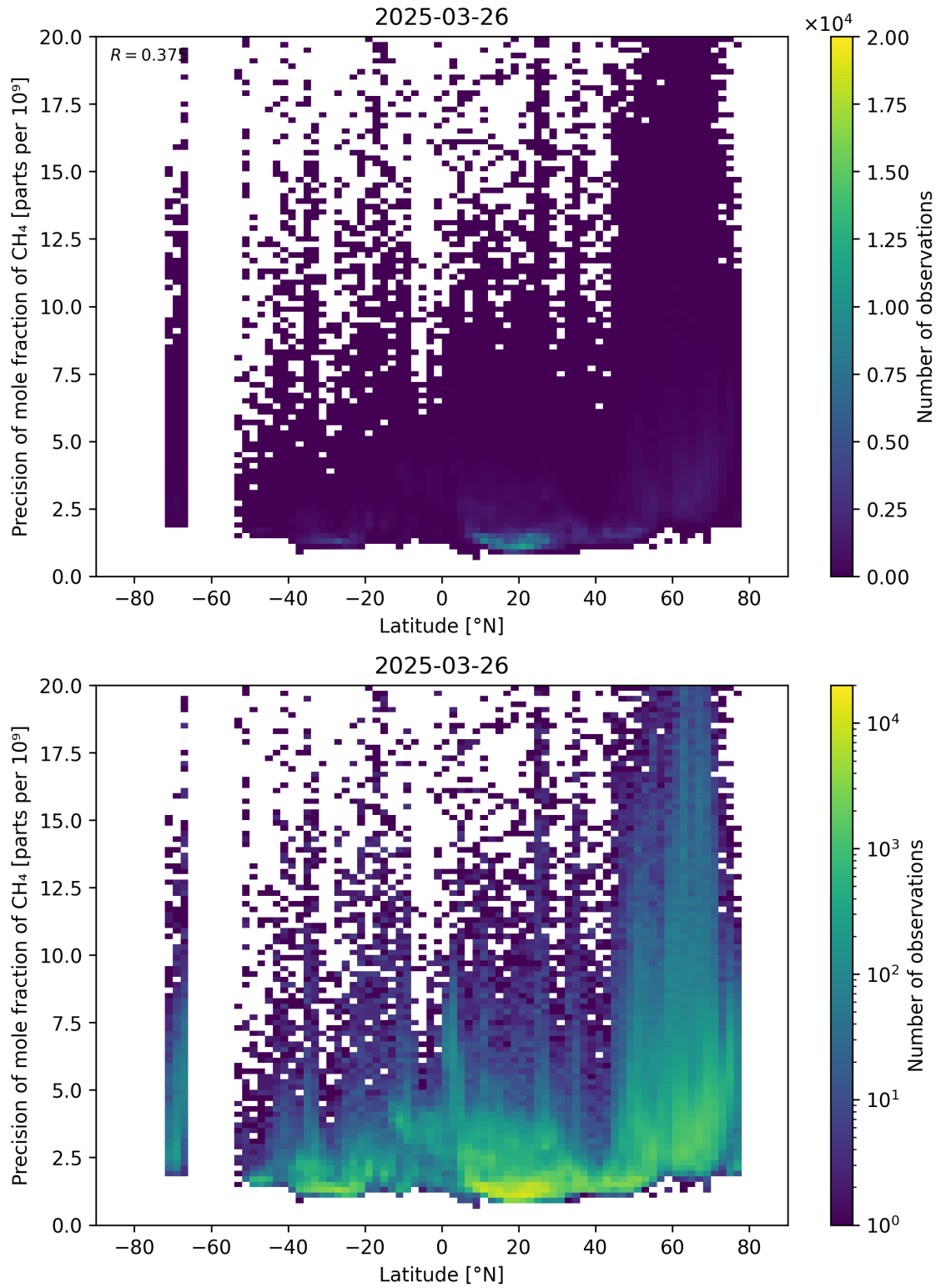
Figure 59: Scatter density plot of “Latitude” against “Precision of mole fraction of \text{CH}_4 ” for 2025-03-25 to 2025-03-27.
