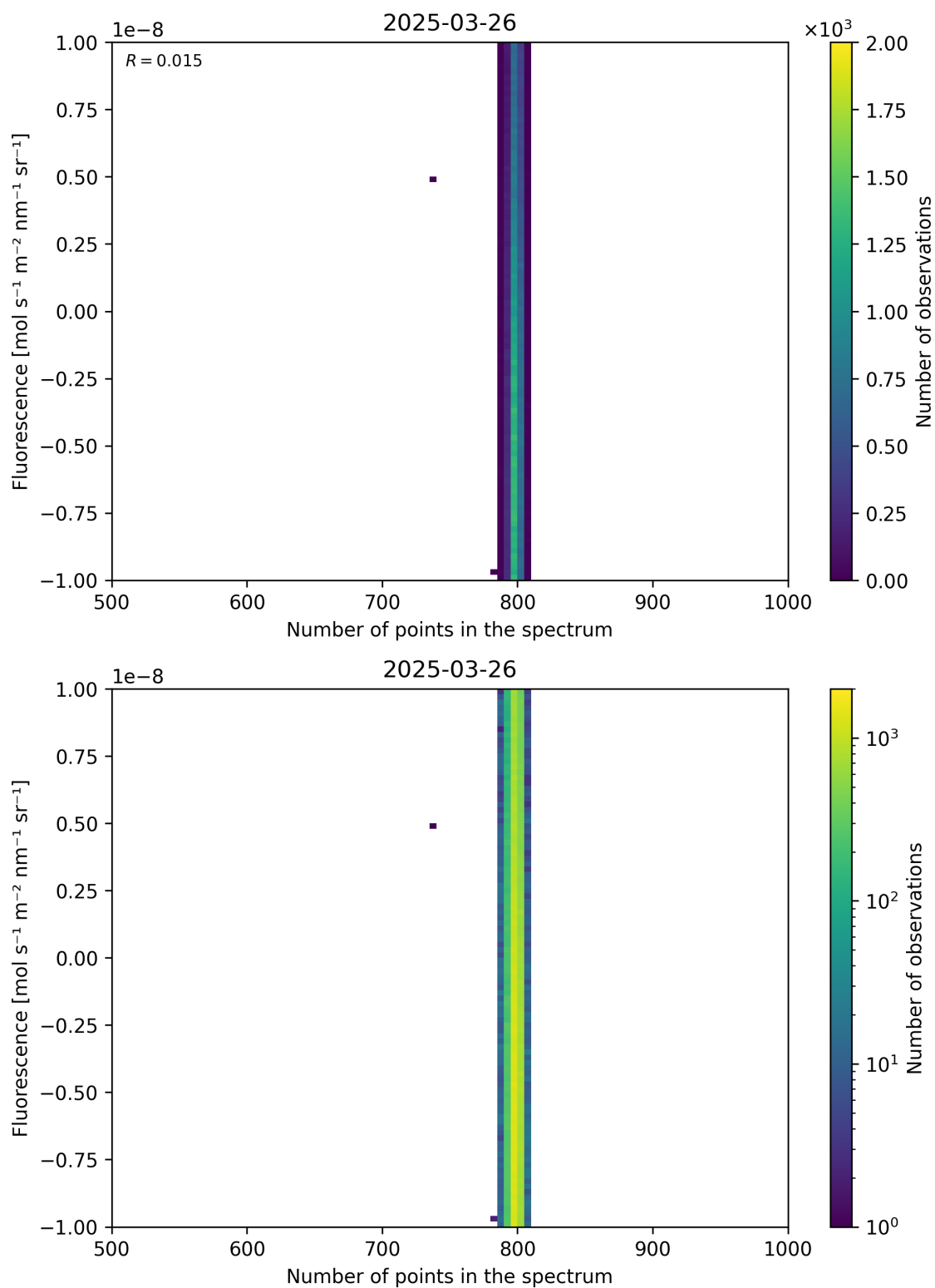
Figure 91: Scatter density plot of “Number of points in the spectrum” against “Fluorescence” for 2025-03-25 to 2025-03-27.
