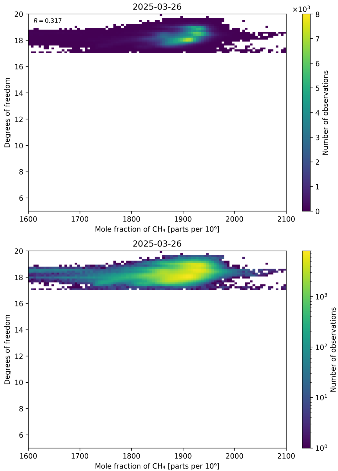
Figure 72: Scatter density plot of “Mole fraction of CH 4 ” against “Degrees of freedom” for 2025-03-25 to 2025-03-27.
