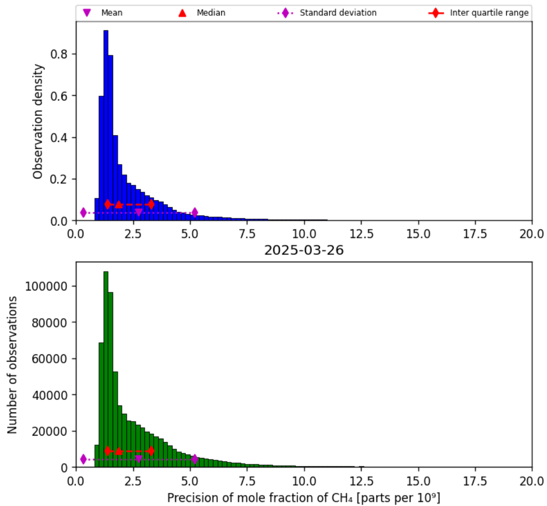
Figure 24: Histogram of “Precision of mole fraction of CH 4 ” for 2025-03-25 to 2025-03-27
