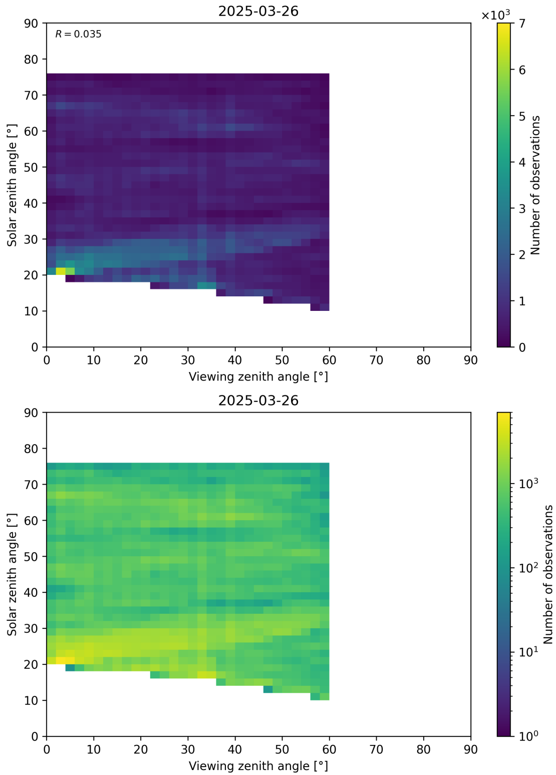
Figure 115: Scatter density plot of “Viewing zenith angle” against “Solar zenith angle” for 2025-03-25 to 2025-03-27.
