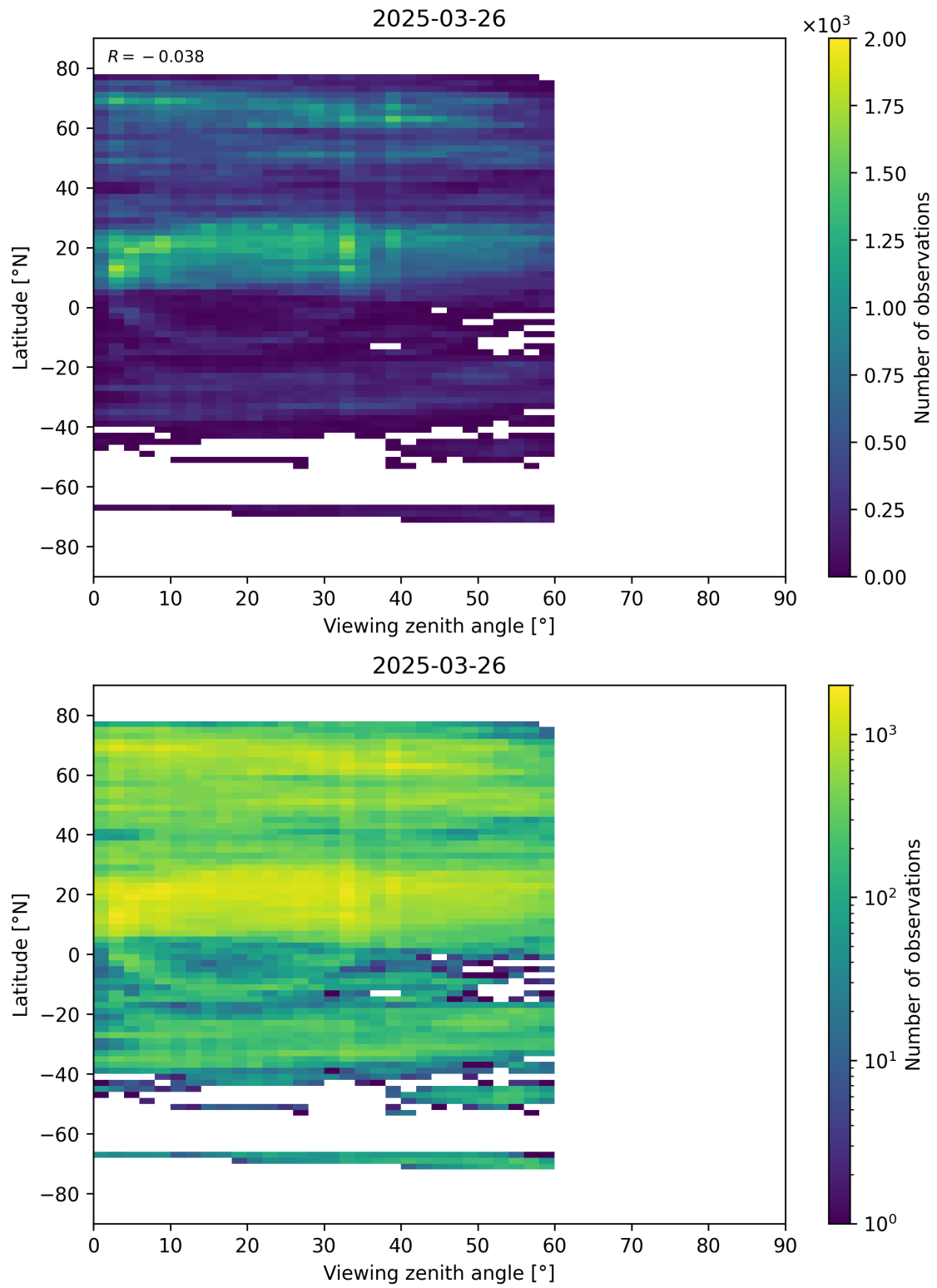
Figure 109: Scatter density plot of “Viewing zenith angle” against “Latitude” for 2025-03-25 to 2025-03-27.
