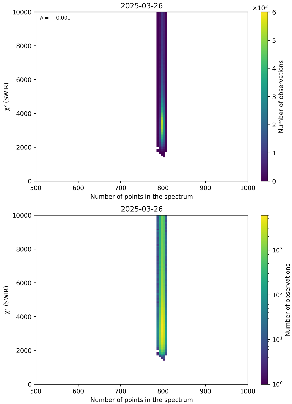
Figure 89: Scatter density plot of “Number of points in the spectrum” against “ \chi^2 (SWIR)” for 2025-03-25 to 2025-03-27.
