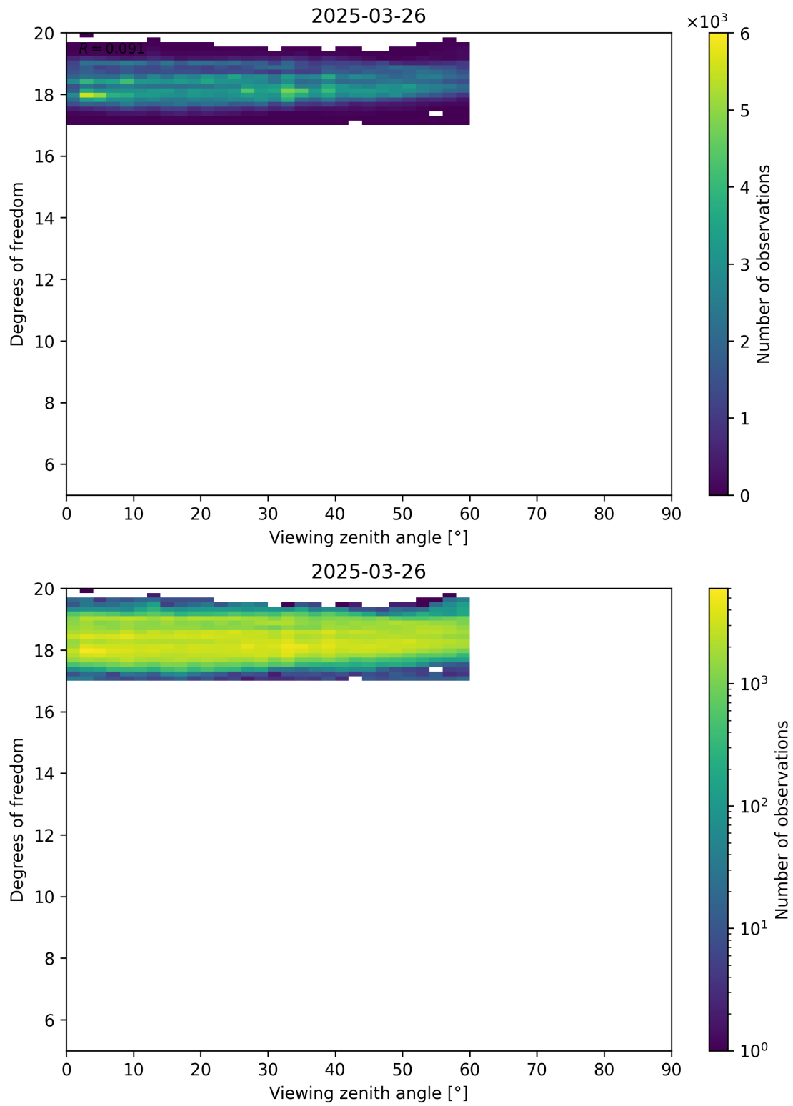
Figure 107: Scatter density plot of “Viewing zenith angle” against “Degrees of freedom” for 2025-03-25 to 2025-03-27.
