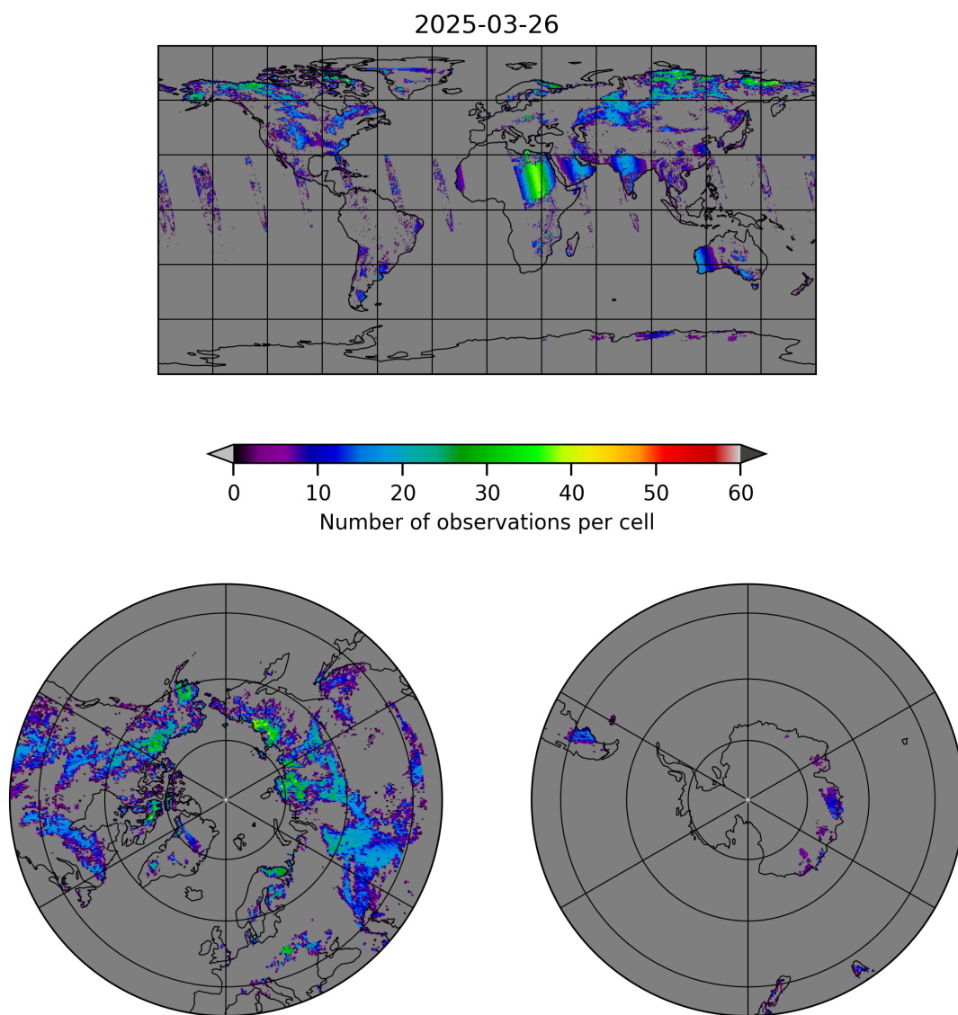
Figure 10: Map of the number of observations for 2025-03-25 to 2025-03-27
