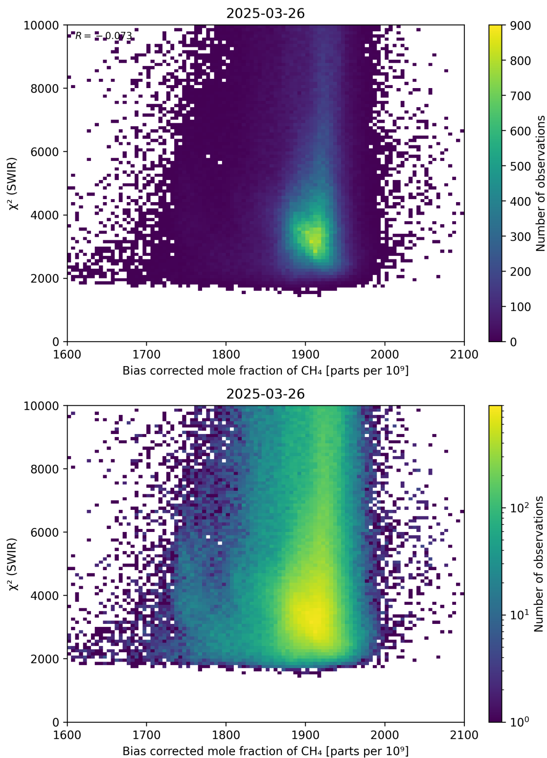
Figure 64: Scatter density plot of “Bias corrected mole fraction of \text{CH}_4 ” against “ \chi^2 (SWIR)” for 2025-03-25 to 2025-03-27.
