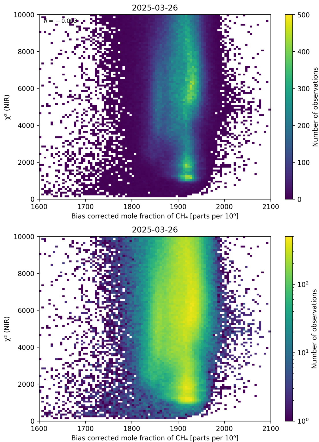
Figure 63: Scatter density plot of “Bias corrected mole fraction of \text{CH}_4 ” against “ \chi^2 (NIR)” for 2025-03-25 to 2025-03-27.
