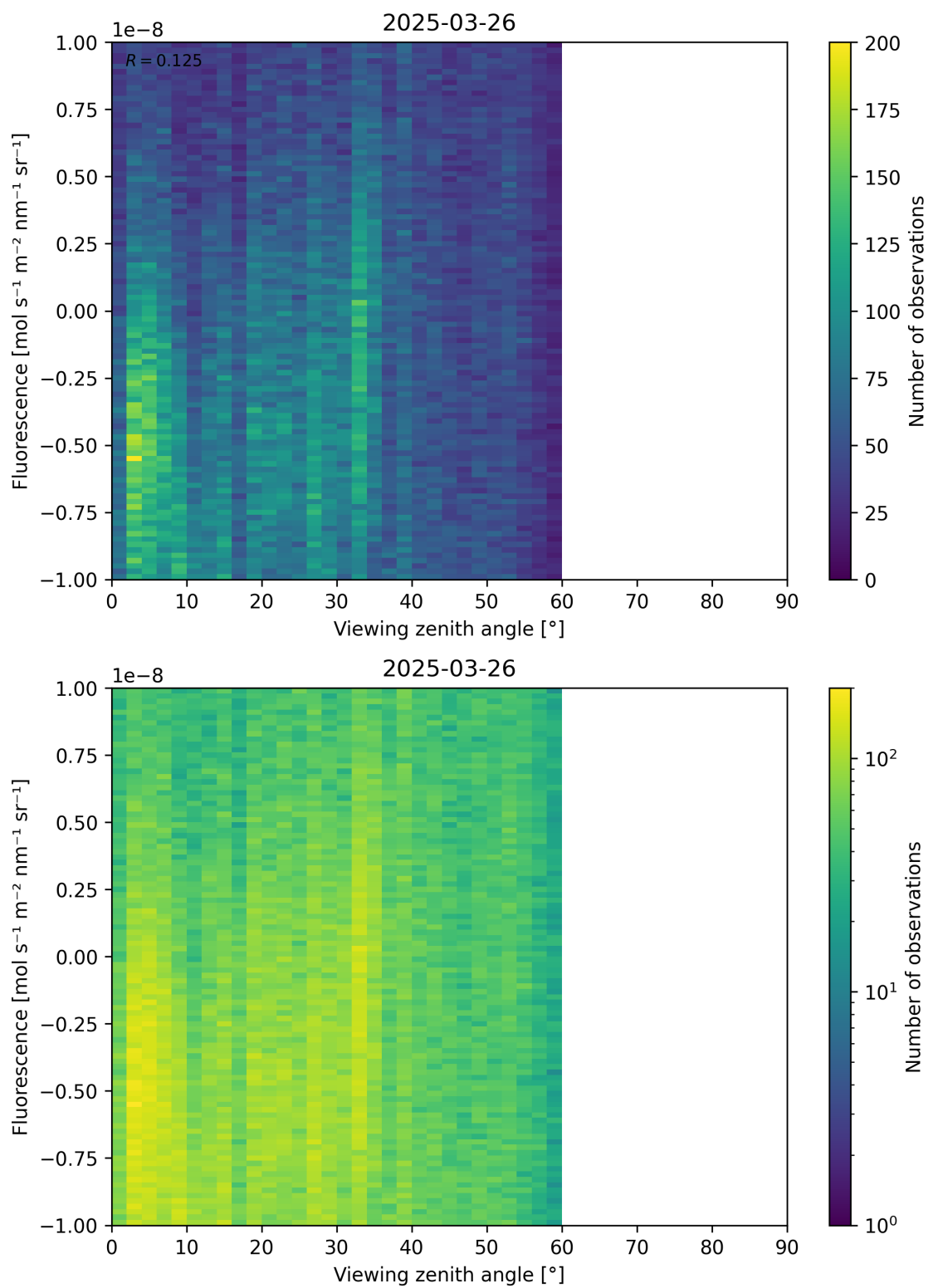
Figure 108: Scatter density plot of “Viewing zenith angle” against “Fluorescence” for 2025-03-25 to 2025-03-27.
