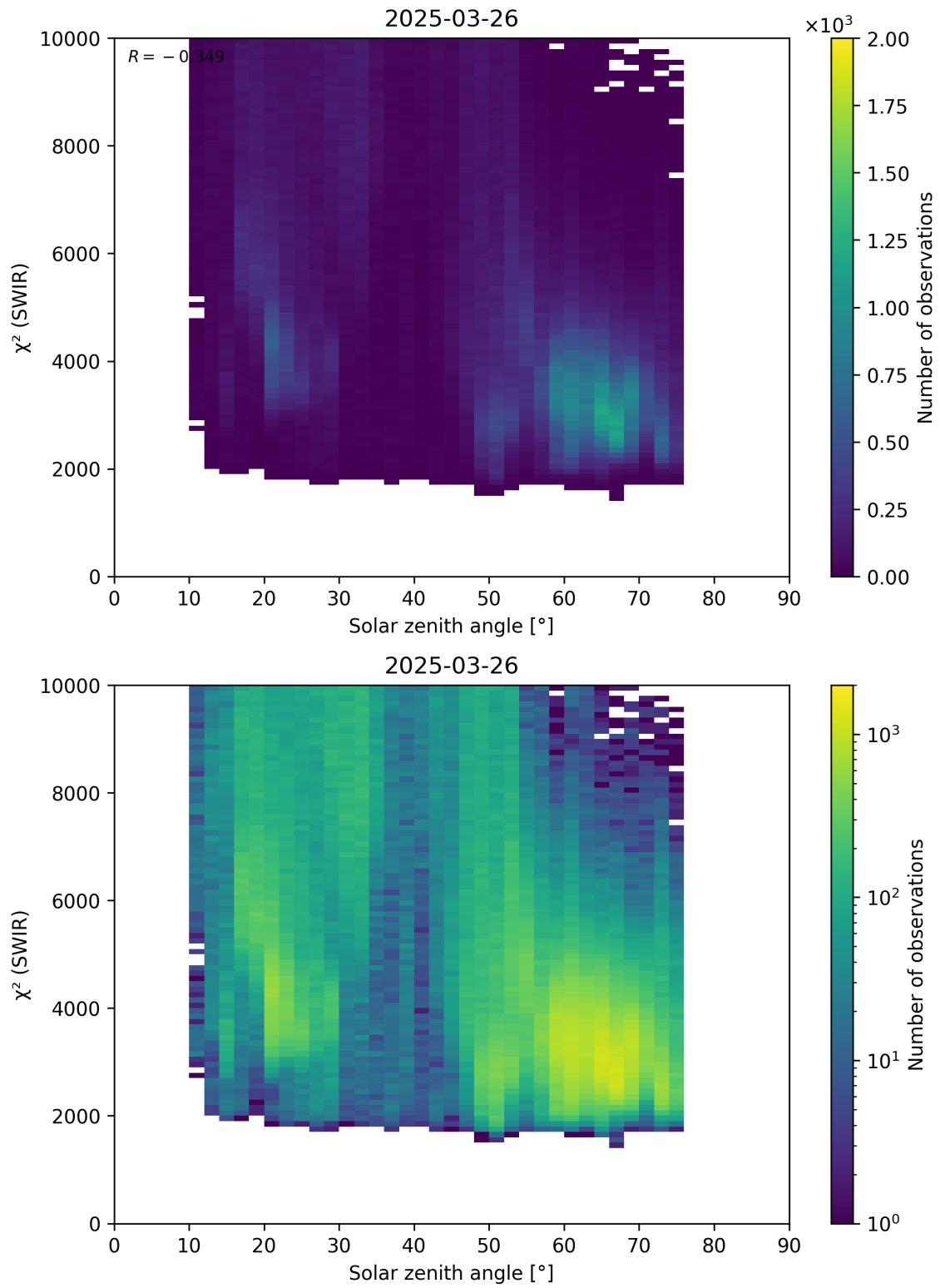
Figure 95: Scatter density plot of “Solar zenith angle” against “ \chi^2 (SWIR)” for 2025-03-25 to 2025-03-27.
