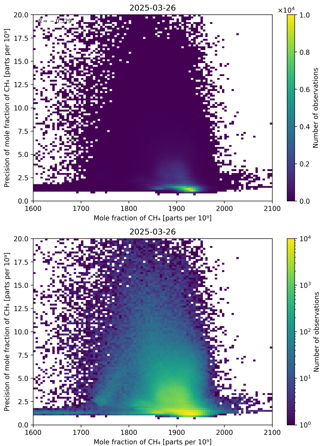
Figure 75: Scatter density plot of “Mole fraction of CH 4 ” against “Precision of mole fraction of CH 4 ” for 2025-03-25 to 2025-03-27.
