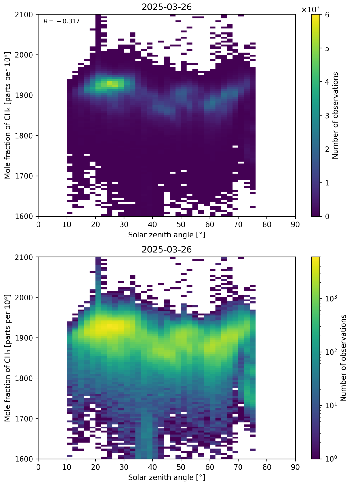
Figure 99: Scatter density plot of “Solar zenith angle” against “Mole fraction of CH 4 ” for 2025-03-25 to 2025-03-27.
