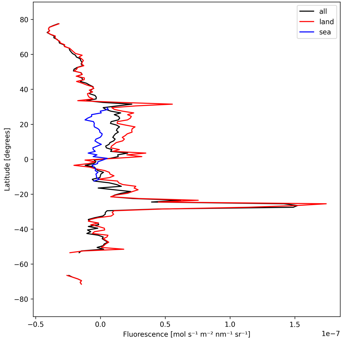
Figure 21: Zonal average of “Fluorescence” for 2025-03-25 to 2025-03-27.
