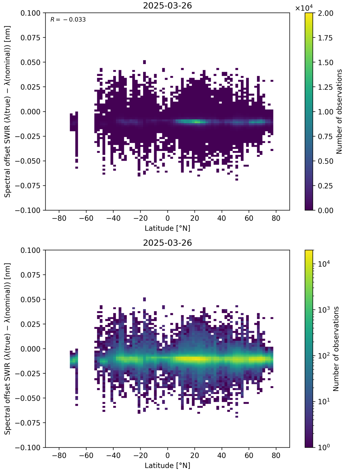
Figure 62: Scatter density plot of “Latitude” against “Spectral offset SWIR ( \lambda_{\text{true}} - \lambda_{\text{nominal}} )” for 2025-03-25 to 2025-03-27.
