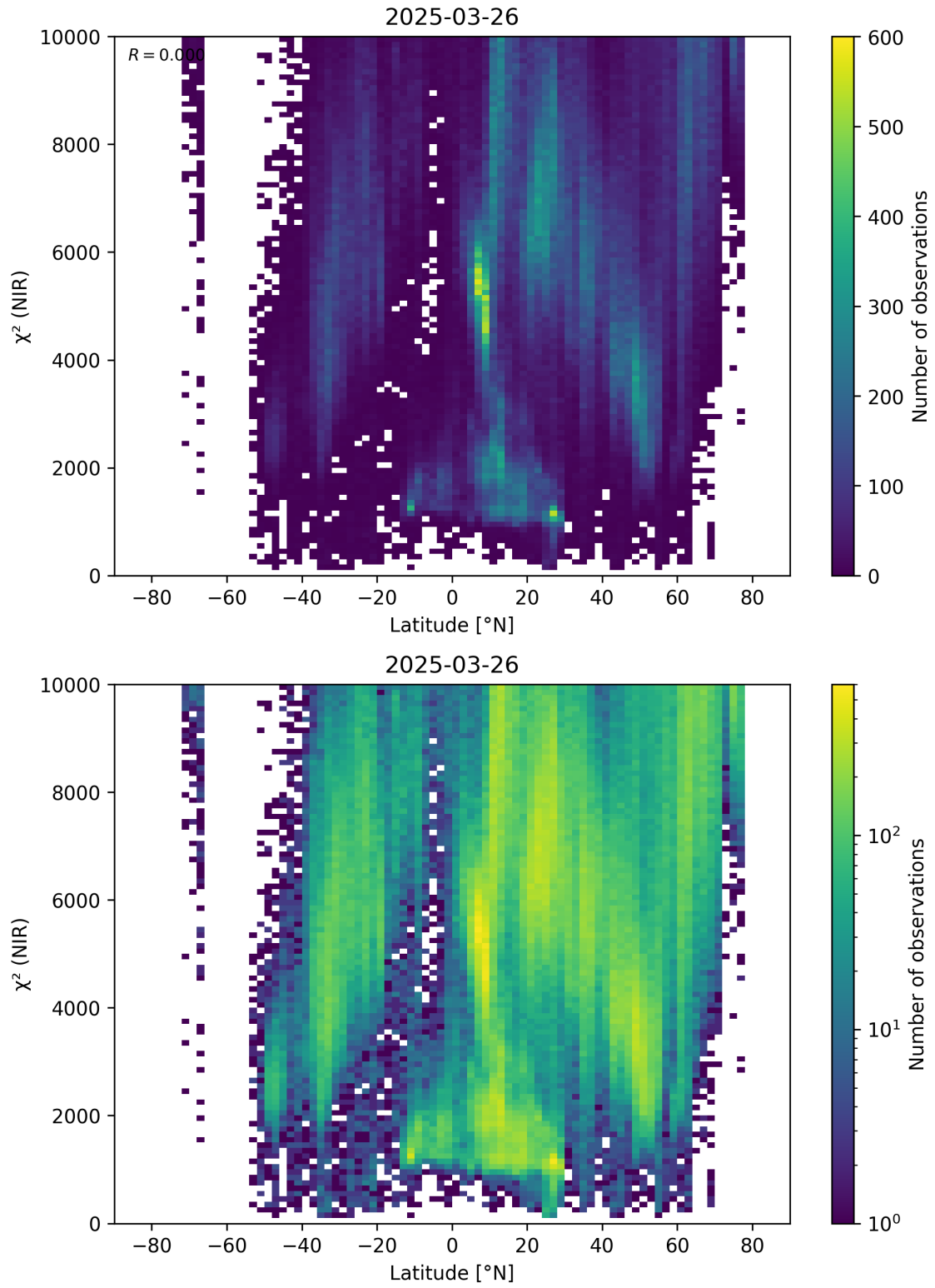
Figure 53: Scatter density plot of “Latitude” against “ \chi^2 (NIR)” for 2025-03-25 to 2025-03-27.
