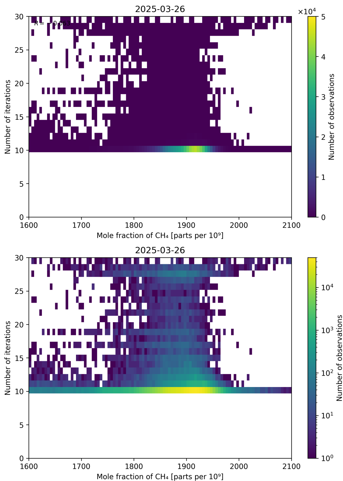
Figure 76: Scatter density plot of “Mole fraction of CH 4 ” against “Number of iterations” for 2025-03-25 to 2025-03-27.
