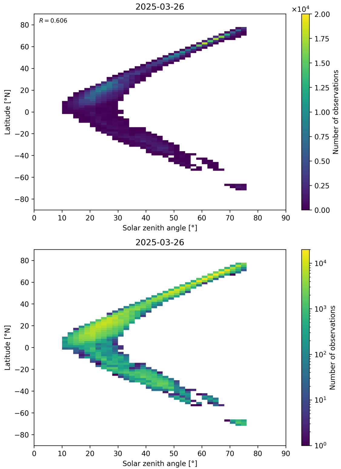
Figure 98: Scatter density plot of “Solar zenith angle” against “Latitude” for 2025-03-25 to 2025-03-27.
