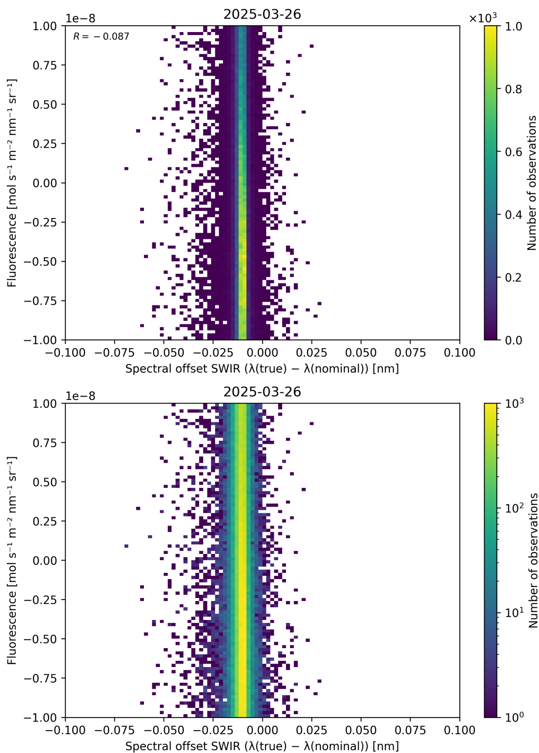
Figure 120: Scatter density plot of “Spectral offset SWIR ( \lambda_{\text{true}} - \lambda_{\text{nominal}} )” against “Fluorescence” for 2025-03-25 to 2025-03-27.
