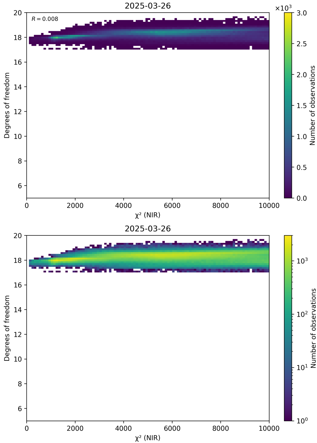
Figure 44: Scatter density plot of “ \chi^2 (NIR)” against “Degrees of freedom” for 2025-03-25 to 2025-03-27.
