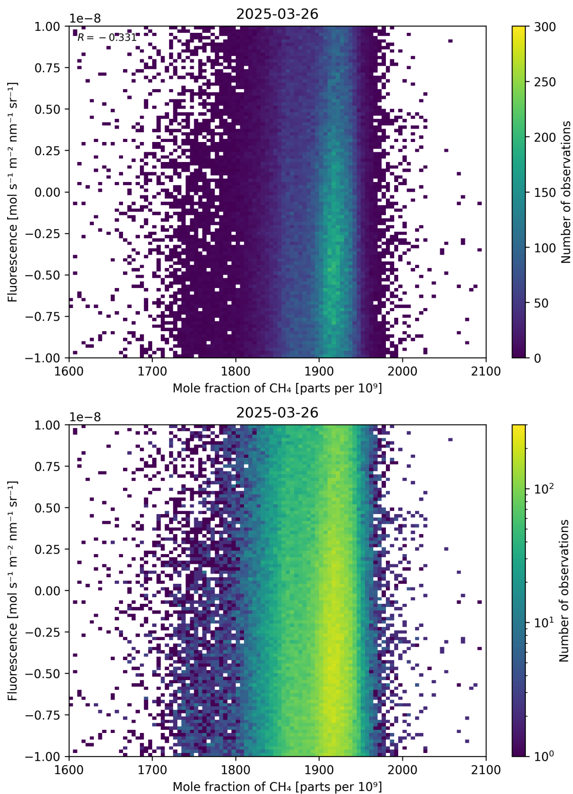
Figure 73: Scatter density plot of “Mole fraction of CH 4 ” against “Fluorescence” for 2025-03-25 to 2025-03-27.
