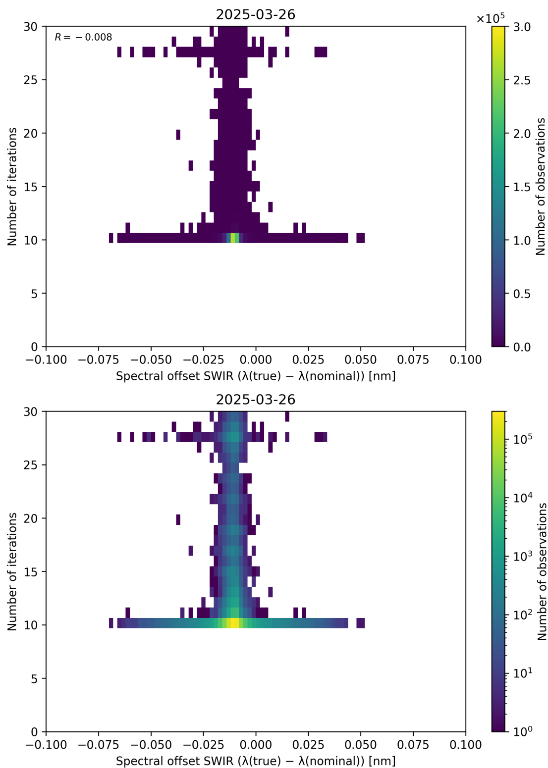
Figure 121: Scatter density plot of “Spectral offset SWIR ( \lambda_{\text{true}} - \lambda_{\text{nominal}} )” against “Number of iterations” for 2025-03-25 to 2025-03-27.
