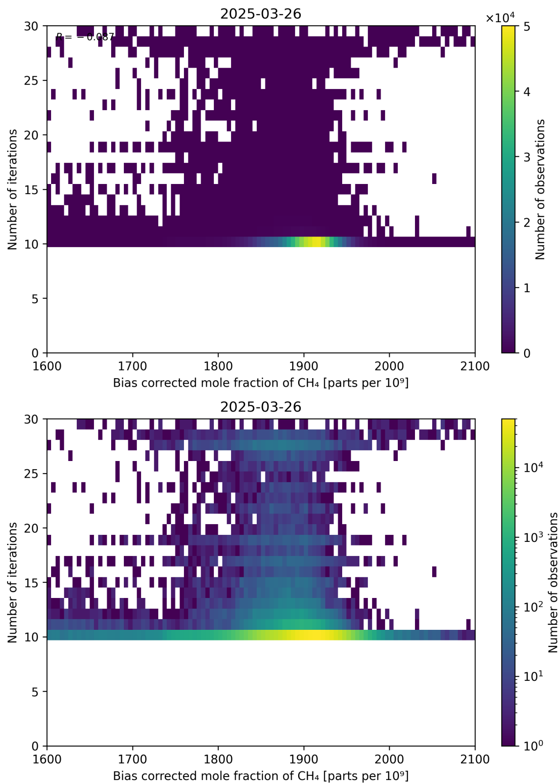
Figure 67: Scatter density plot of “Bias corrected mole fraction of CH 4 ” against “Number of iterations” for 2025-03-25 to 2025-03-27.
