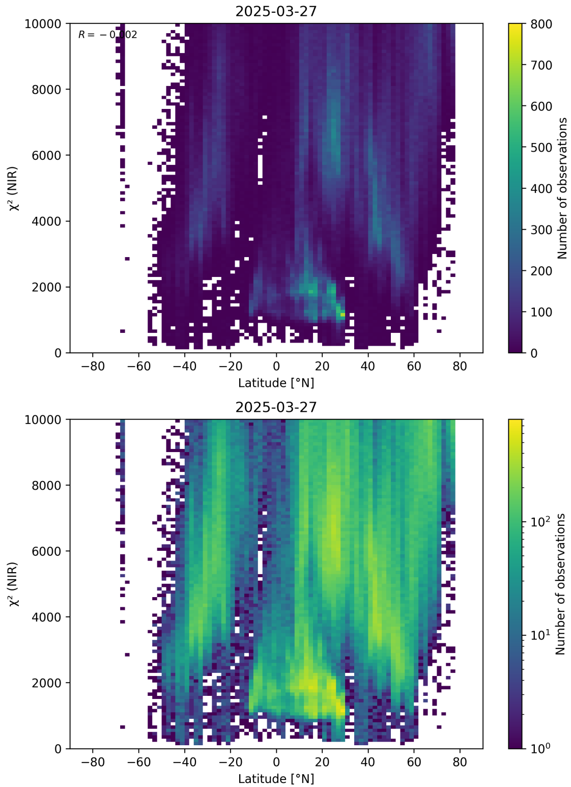
Figure 53: Scatter density plot of “Latitude” against “ \chi^2 (NIR)” for 2025-03-26 to 2025-03-28.
