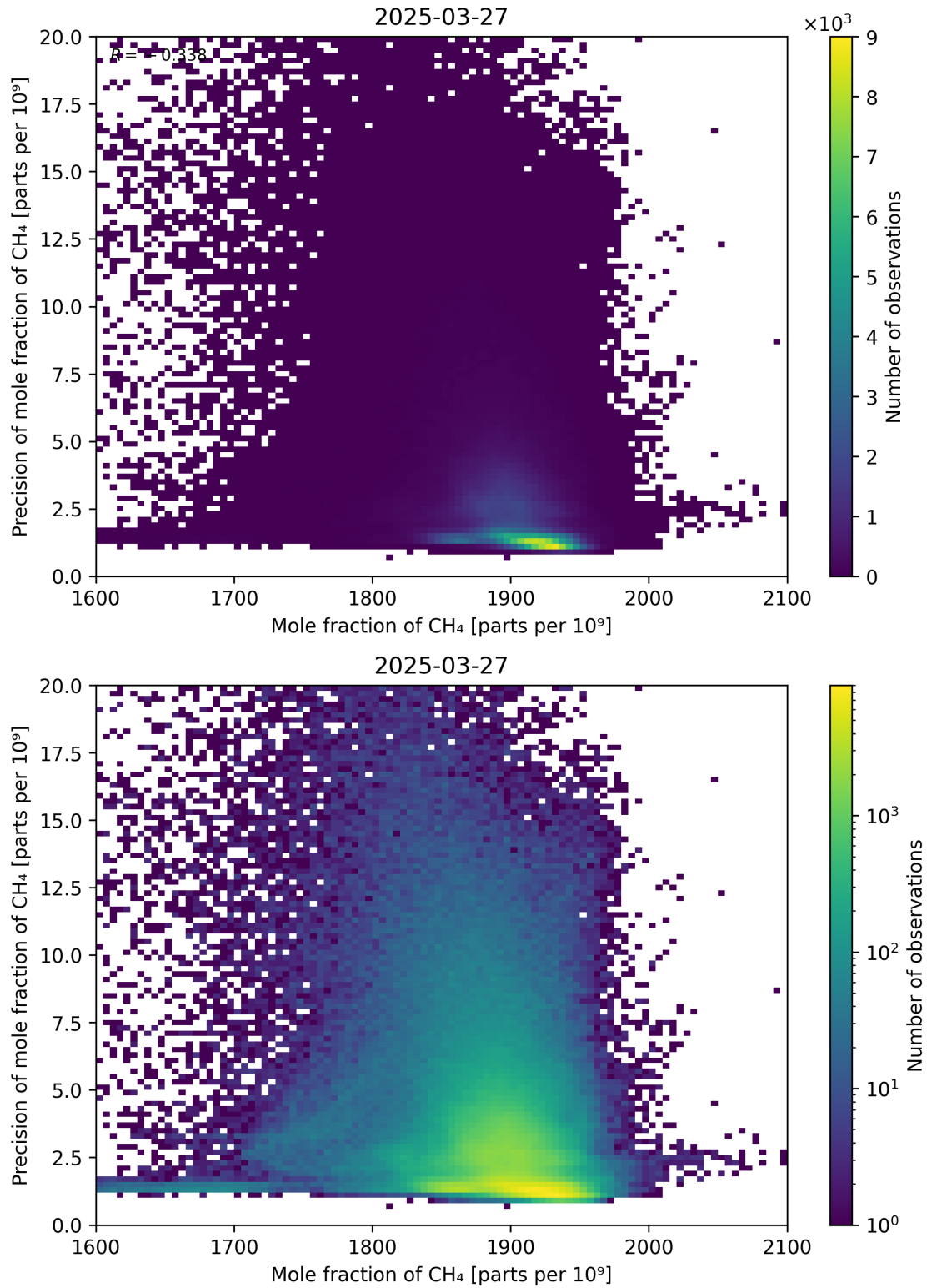
Figure 75: Scatter density plot of “Mole fraction of CH 4 ” against “Precision of mole fraction of CH 4 ” for 2025-03-26 to 2025-03-28.
