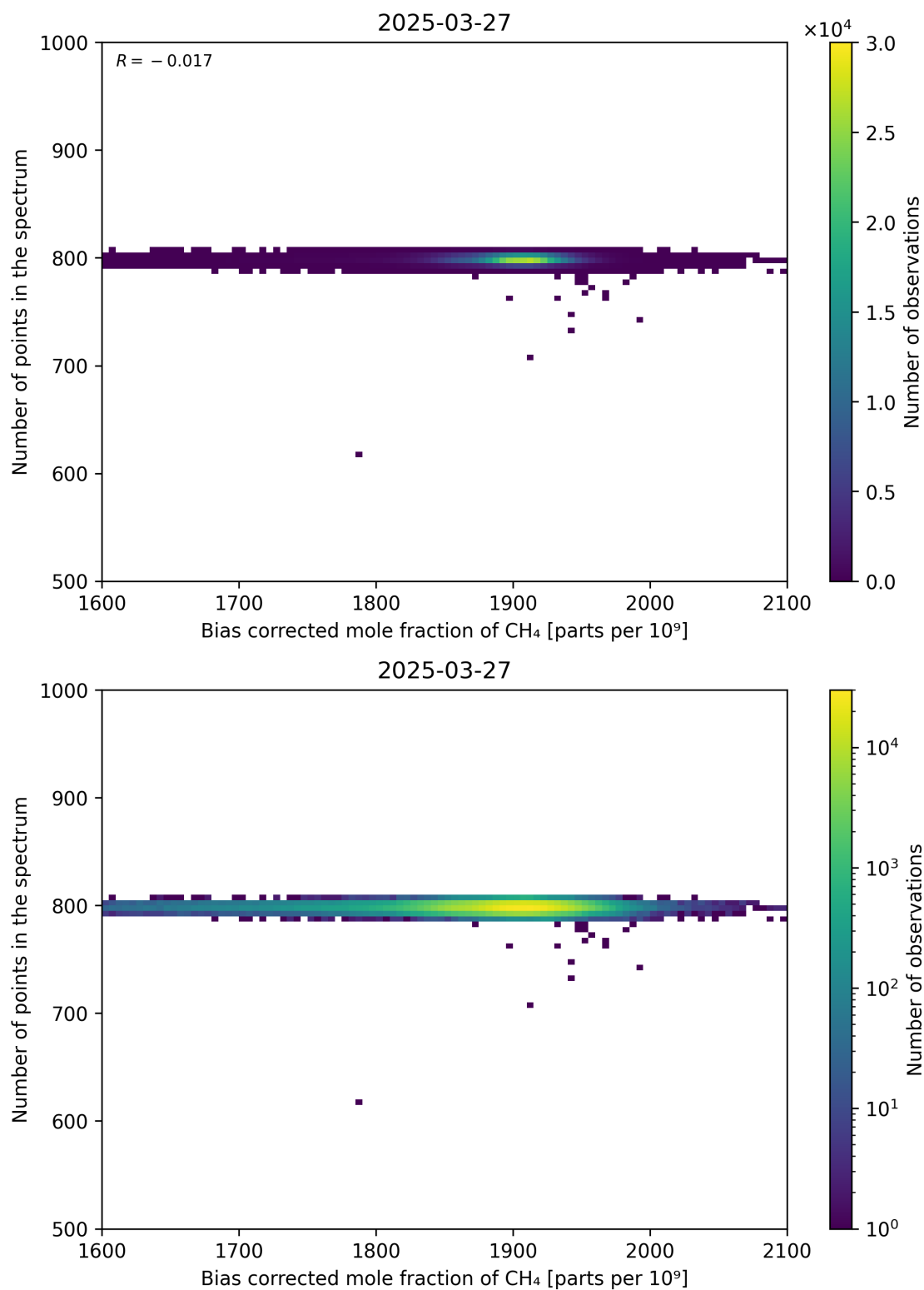
Figure 68: Scatter density plot of “Bias corrected mole fraction of CH 4 ” against “Number of points in the spectrum” for 2025-03-26 to 2025-03-28.
