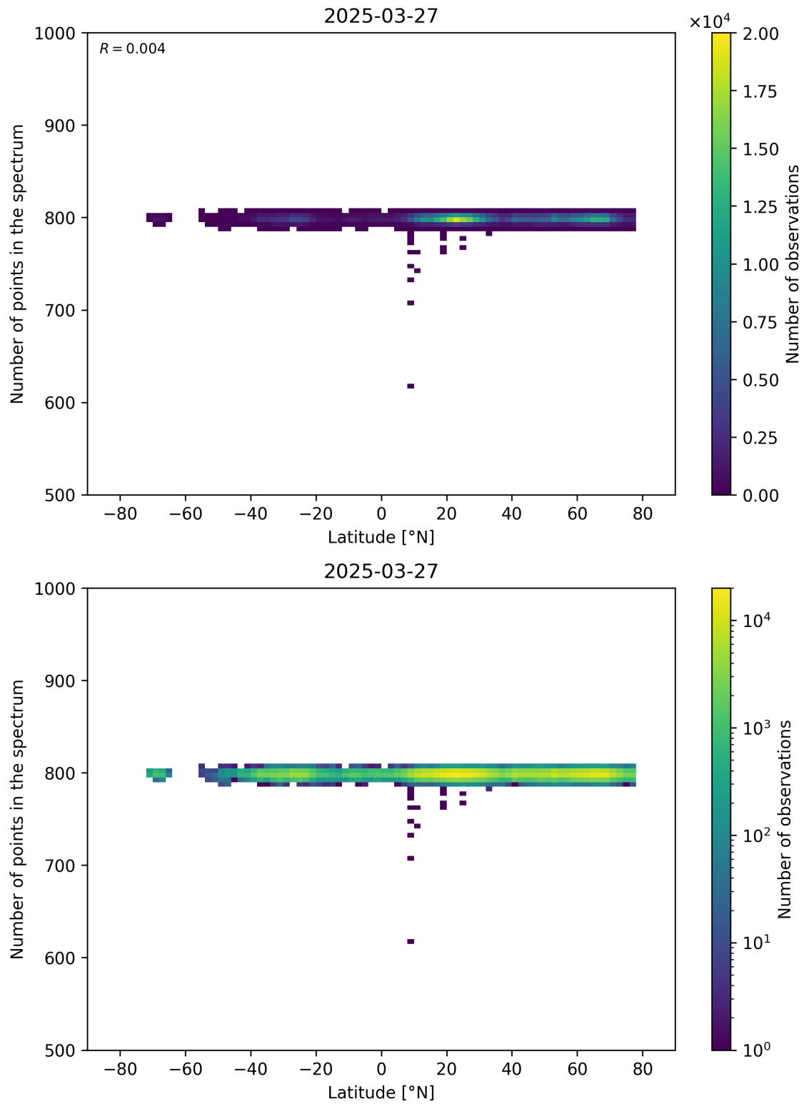
Figure 61: Scatter density plot of “Latitude” against “Number of points in the spectrum” for 2025-03-26 to 2025-03-28.
