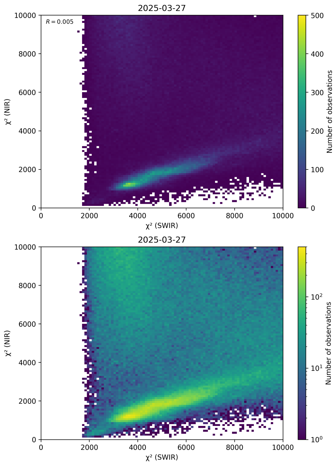
Figure 47: Scatter density plot of “ \chi^2 (SWIR)” against “ \chi^2 (NIR)” for 2025-03-26 to 2025-03-28.
