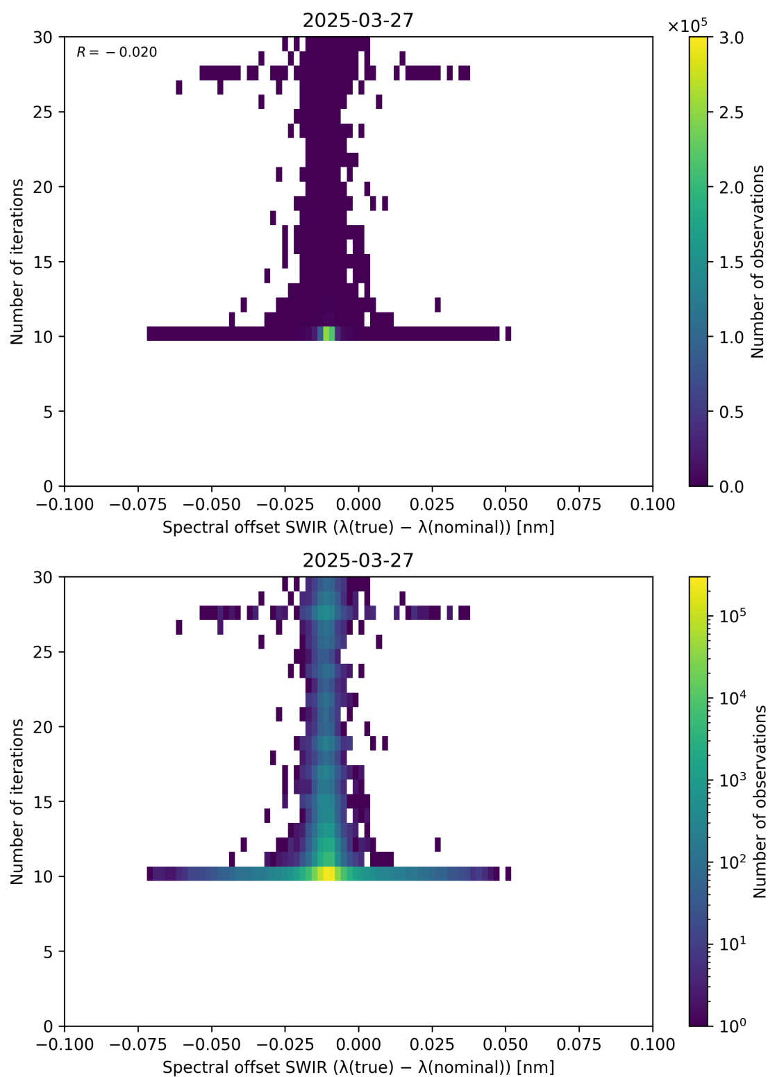
Figure 121: Scatter density plot of “Spectral offset SWIR ( \lambda_{\text{true}} - \lambda_{\text{nominal}} )” against “Number of iterations” for 2025-03-26 to 2025-03-28.
