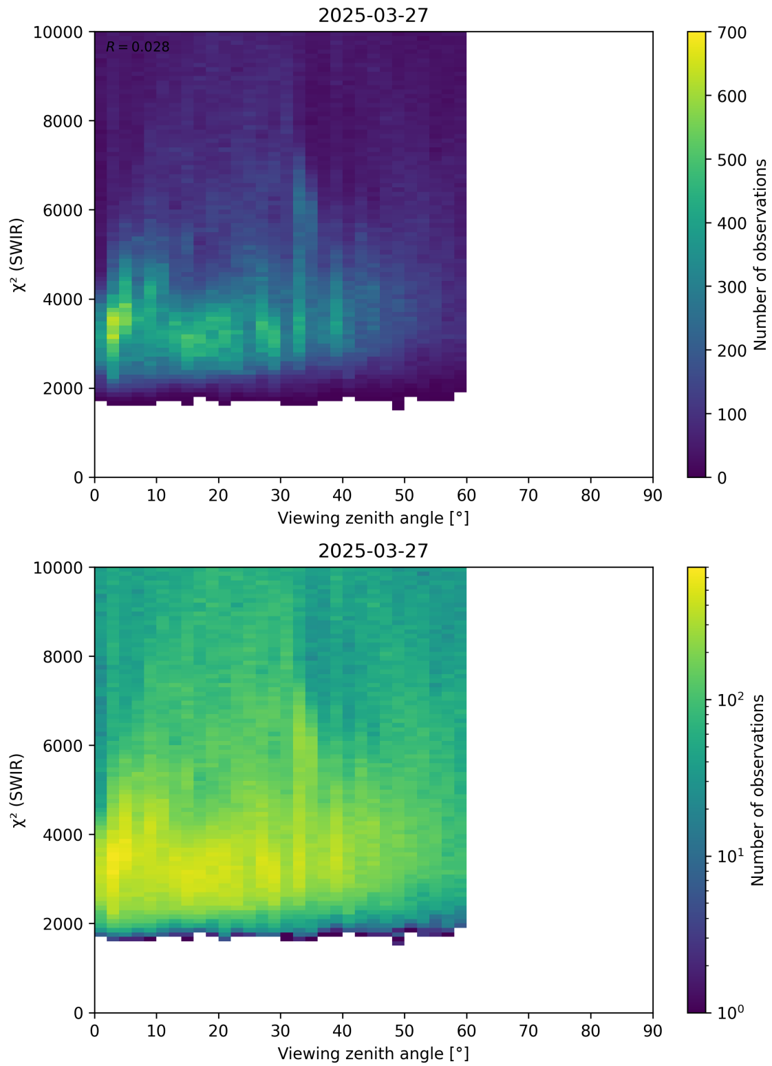
Figure 106: Scatter density plot of “Viewing zenith angle” against “ \chi^2 (SWIR)” for 2025-03-26 to 2025-03-28.
