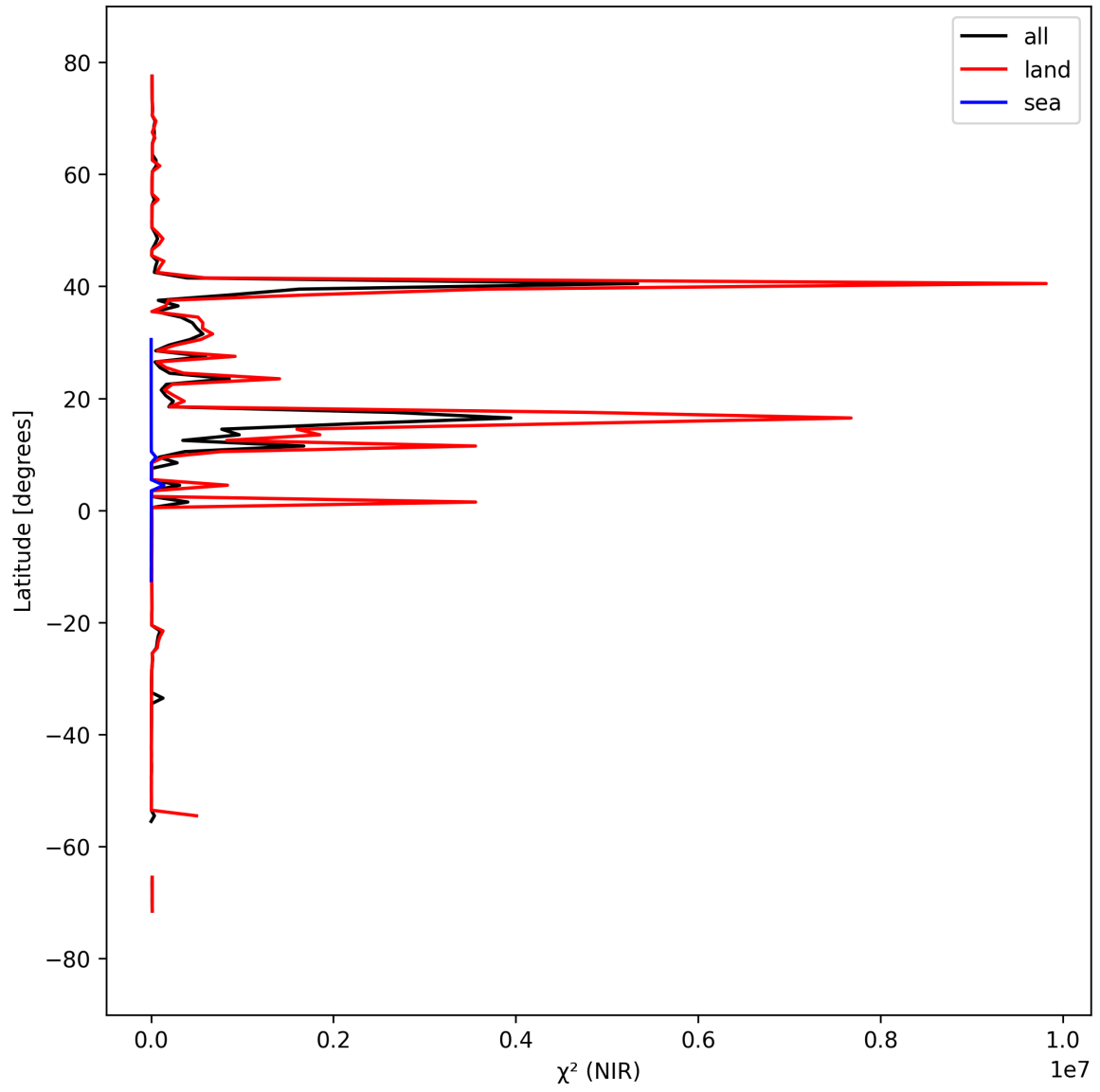
Figure 18: Zonal average of “ \chi^2 (NIR)” for 2025-03-26 to 2025-03-28.
