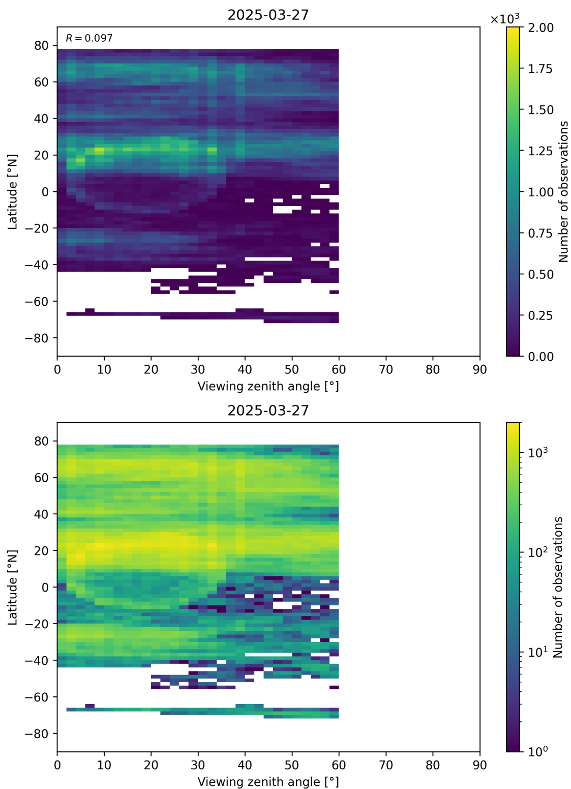
Figure 109: Scatter density plot of “Viewing zenith angle” against “Latitude” for 2025-03-26 to 2025-03-28.
