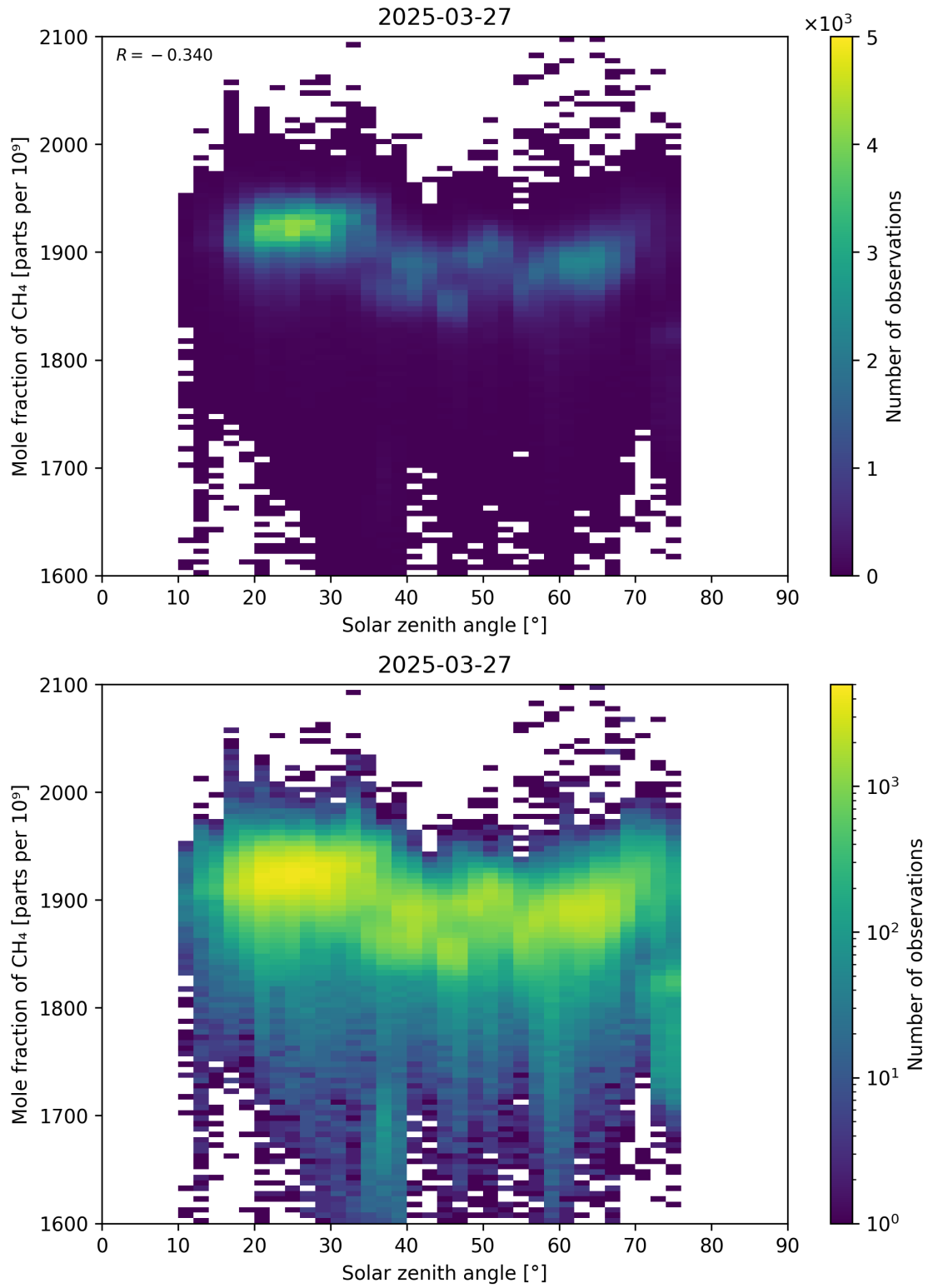
Figure 99: Scatter density plot of “Solar zenith angle” against “Mole fraction of CH 4 ” for 2025-03-26 to 2025-03-28.
