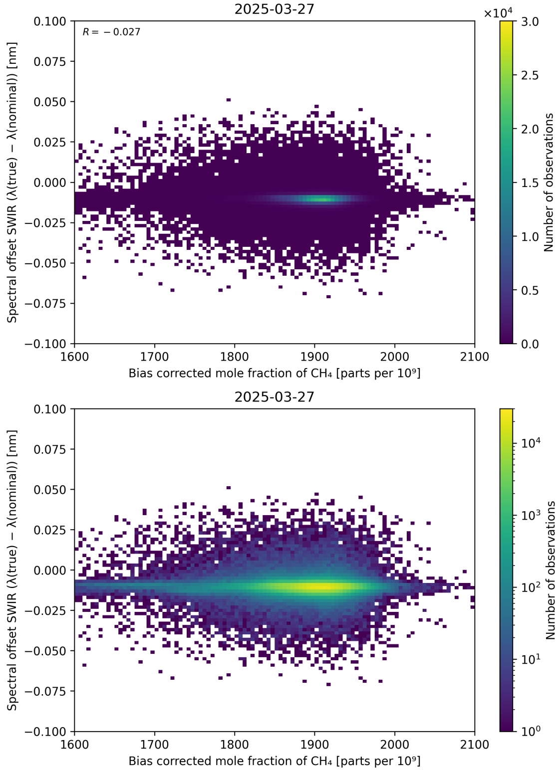
Figure 69: Scatter density plot of “Bias corrected mole fraction of \text{CH}_4 ” against “Spectral offset SWIR ( \lambda_{\text{true}} - \lambda_{\text{nominal}} )” for 2025-03-26 to 2025-03-28.
