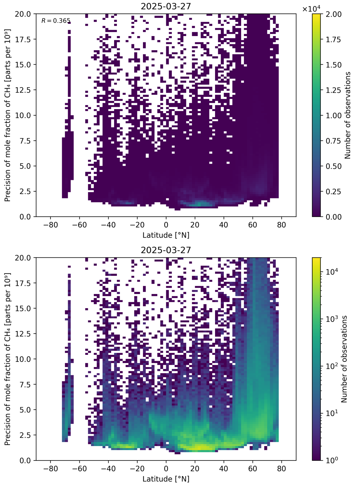
Figure 59: Scatter density plot of “Latitude” against “Precision of mole fraction of \text{CH}_4 ” for 2025-03-26 to 2025-03-28.
