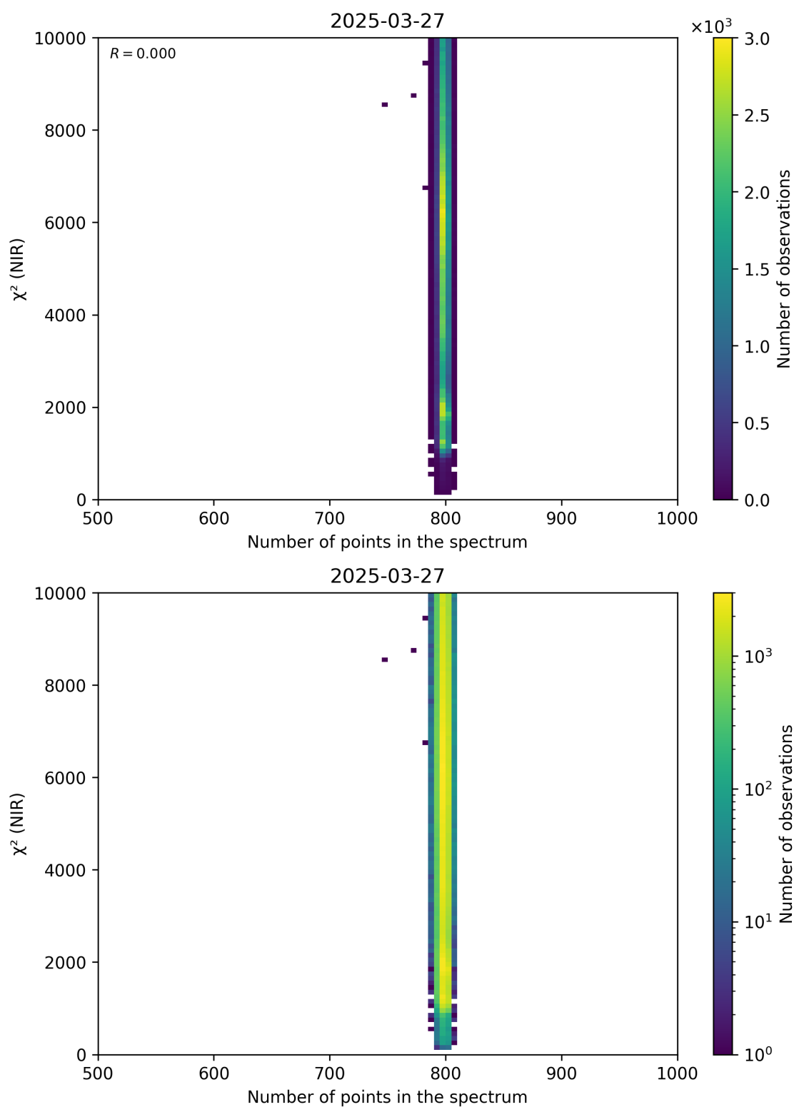
Figure 88: Scatter density plot of “Number of points in the spectrum” against “ \chi^2 (NIR)” for 2025-03-26 to 2025-03-28.
