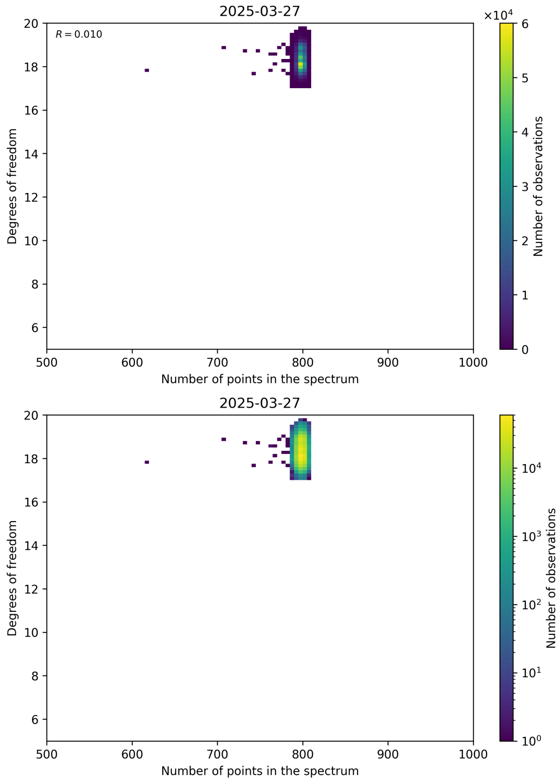
Figure 90: Scatter density plot of “Number of points in the spectrum” against “Degrees of freedom” for 2025-03-26 to 2025-03-28.
