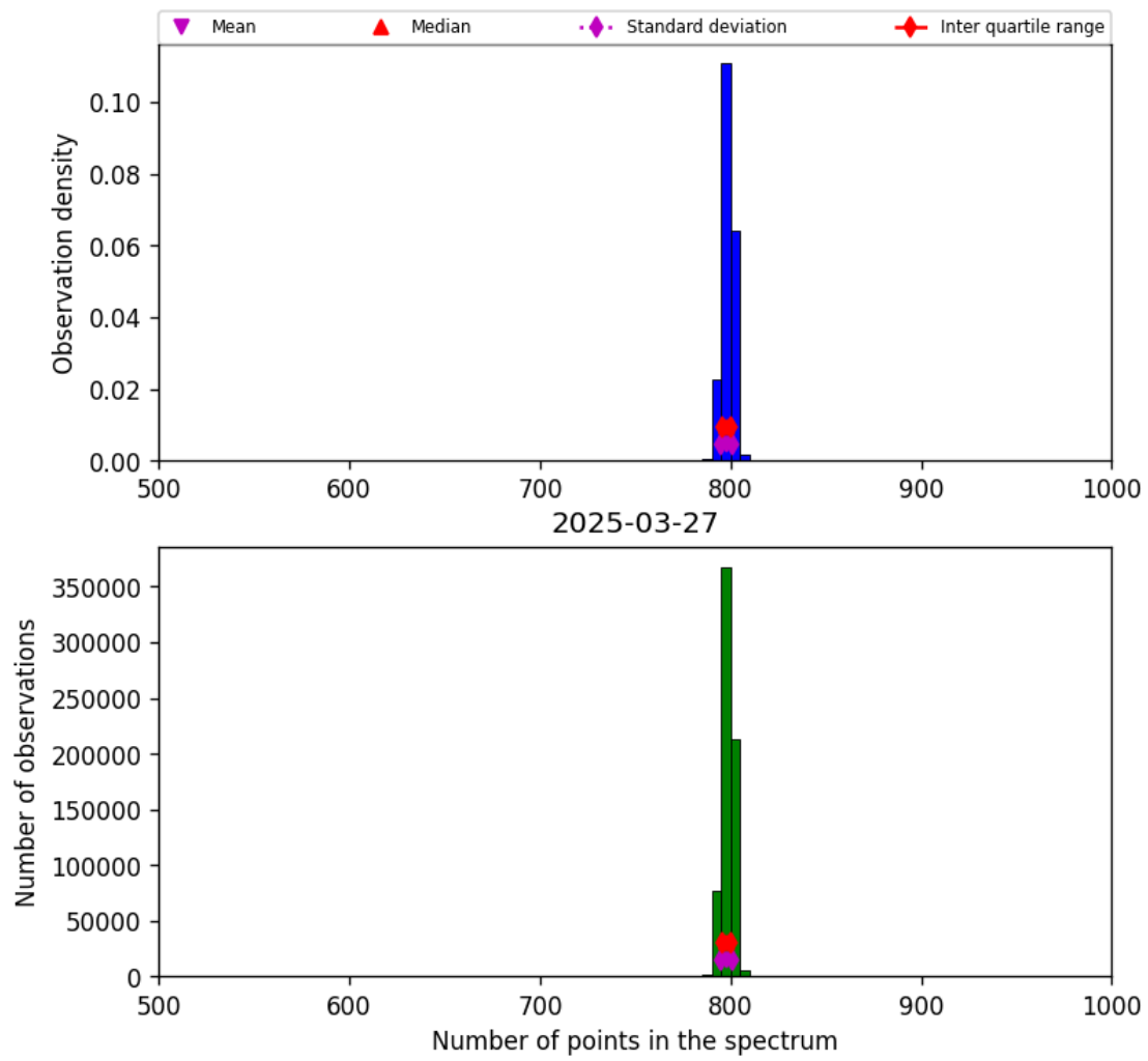
Figure 26: Histogram of “Number of points in the spectrum” for 2025-03-26 to 2025-03-28
