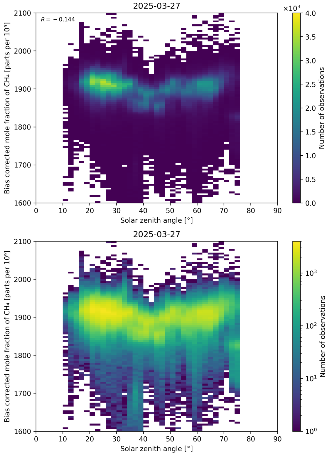
Figure 100: Scatter density plot of “Solar zenith angle” against “Bias corrected mole fraction of CH 4 ” for 2025-03-26 to 2025-03-28.
