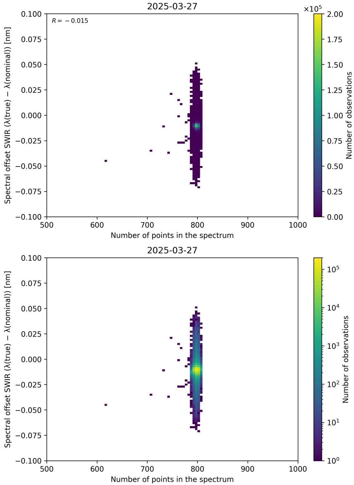
Figure 93: Scatter density plot of “Number of points in the spectrum” against “Spectral offset SWIR ( \lambda_{\text{true}} - \lambda_{\text{nominal}} )” for 2025-03-26 to 2025-03-28.
