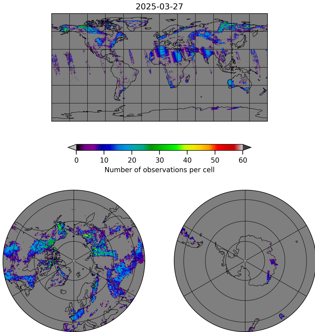
Figure 10: Map of the number of observations for 2025-03-26 to 2025-03-28
