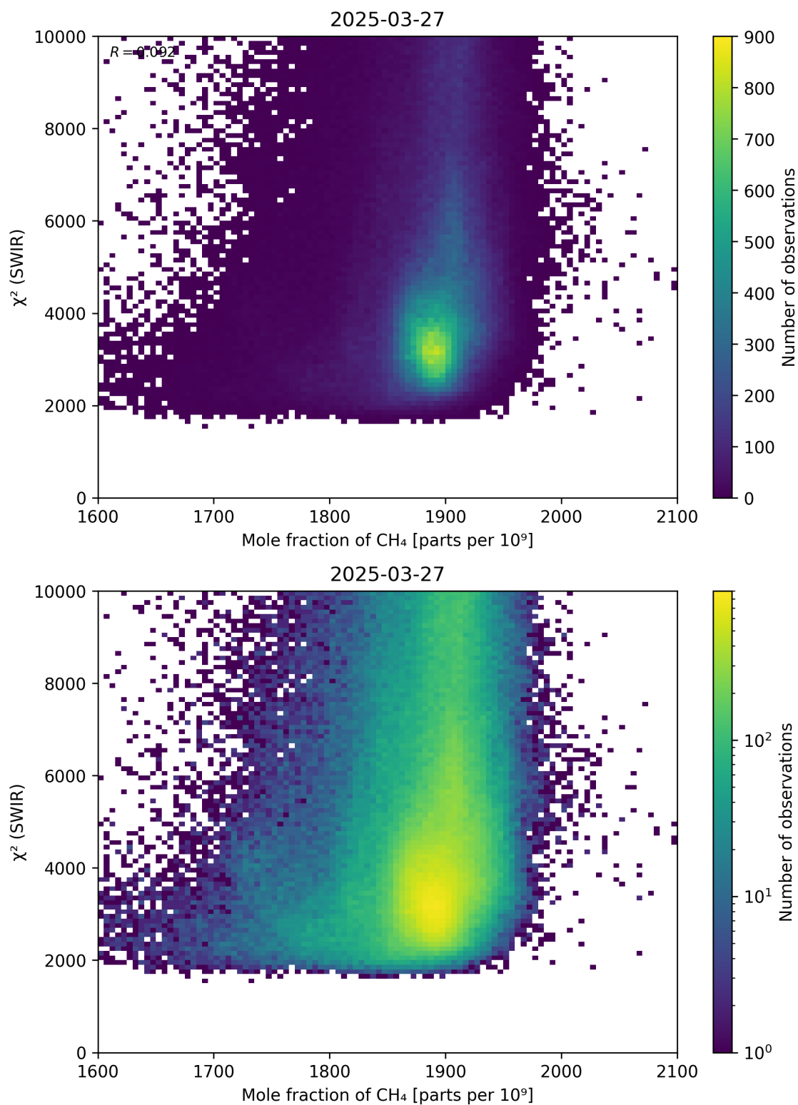
Figure 71: Scatter density plot of “Mole fraction of CH 4 ” against “ \chi^2 (SWIR)” for 2025-03-26 to 2025-03-28.
