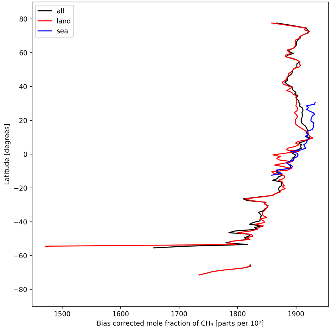
Figure 14: Zonal average of “Bias corrected mole fraction of CH 4 ” for 2025-03-26 to 2025-03-28.
