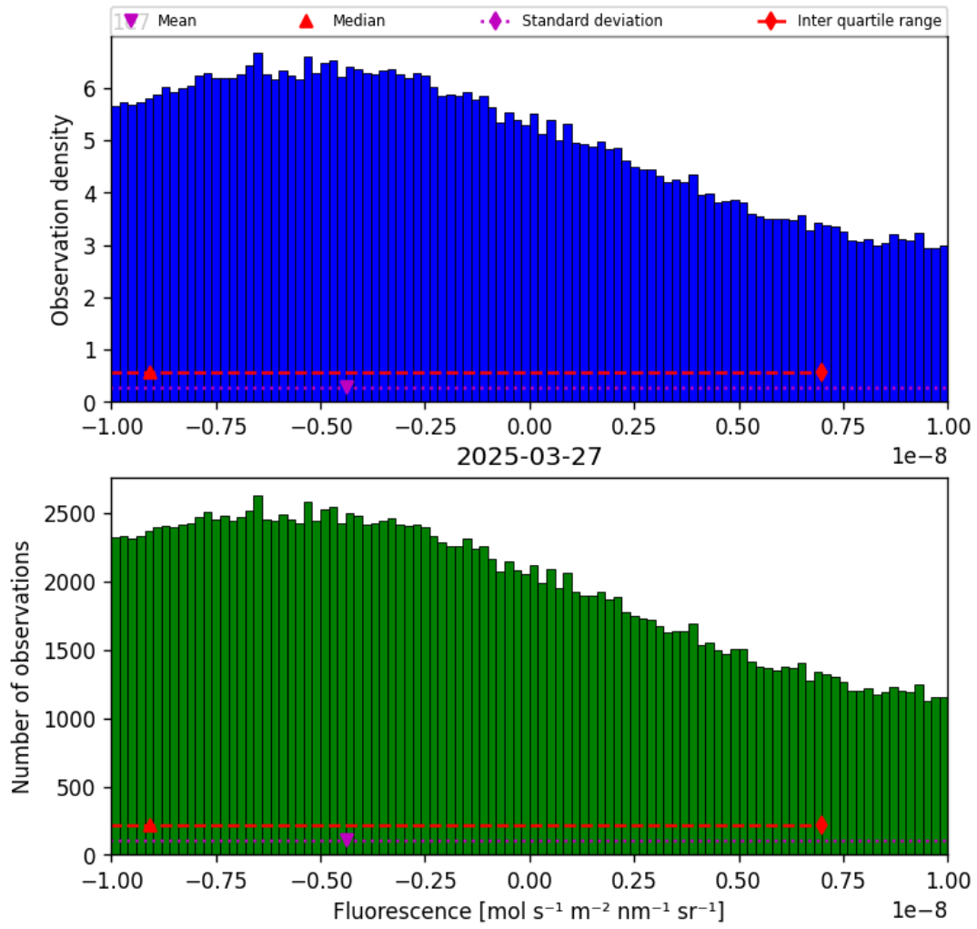
Figure 32: Histogram of “Fluorescence” for 2025-03-26 to 2025-03-28
