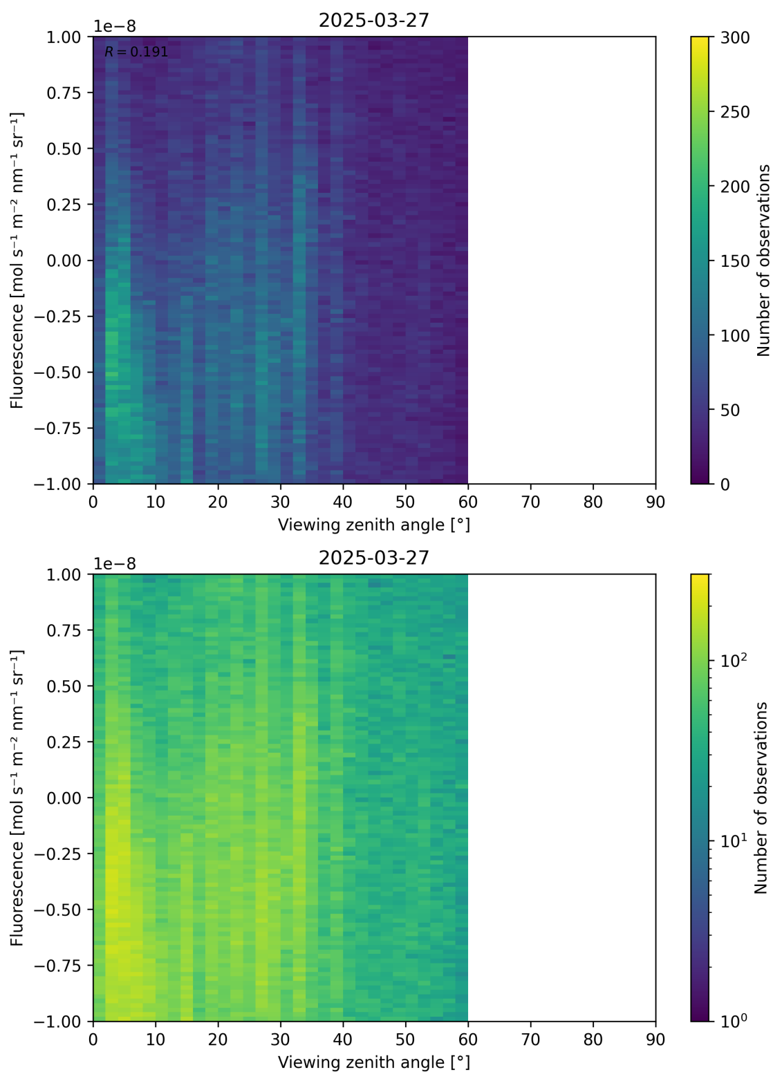
Figure 108: Scatter density plot of “Viewing zenith angle” against “Fluorescence” for 2025-03-26 to 2025-03-28.
