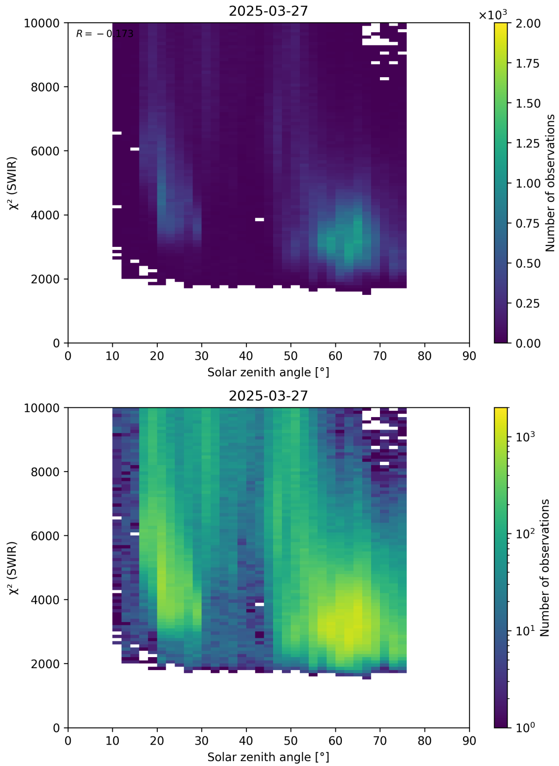
Figure 95: Scatter density plot of “Solar zenith angle” against “ \chi^2 (SWIR)” for 2025-03-26 to 2025-03-28.
