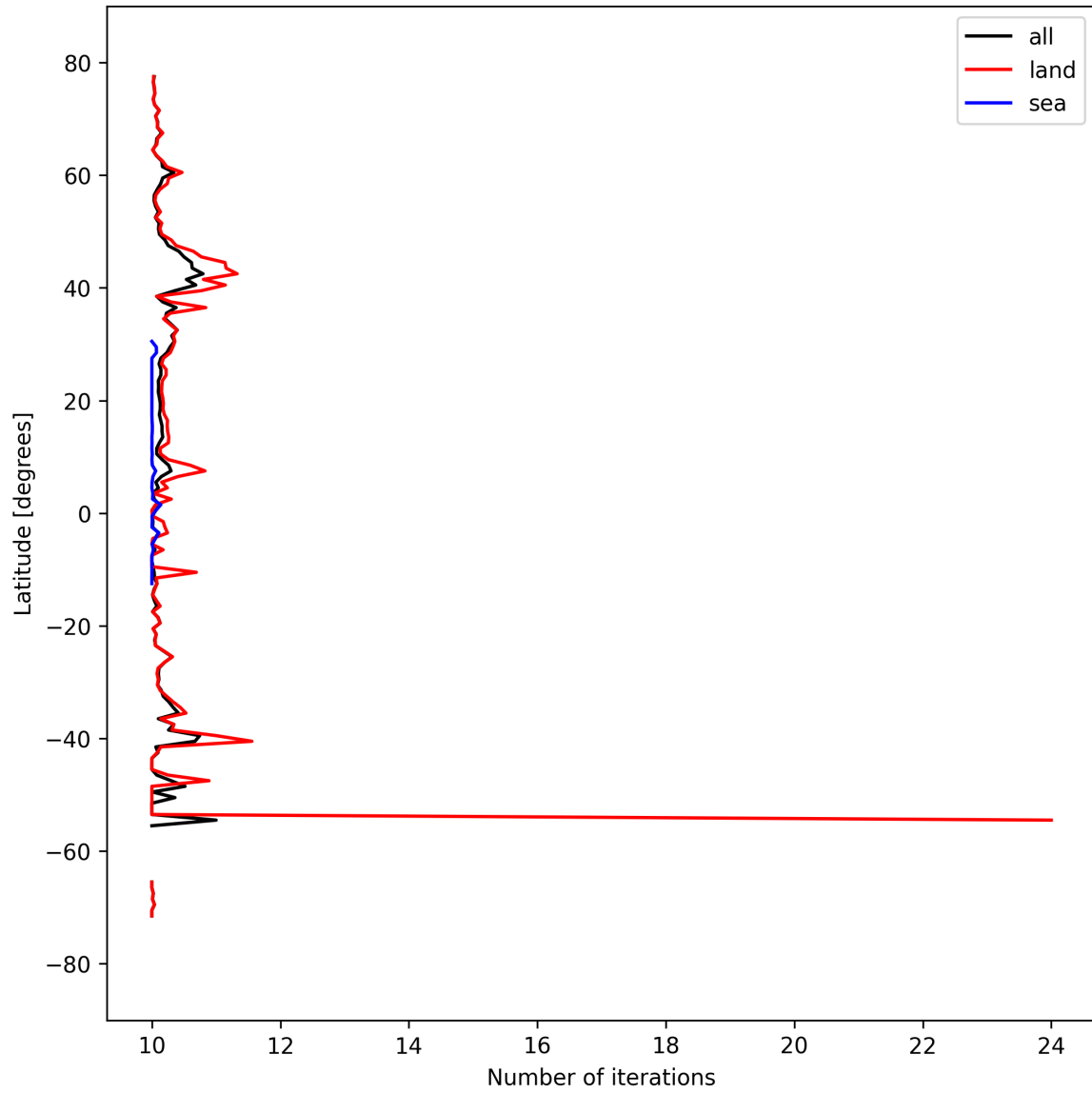
Figure 20: Zonal average of “Number of iterations” for 2025-03-26 to 2025-03-28.
