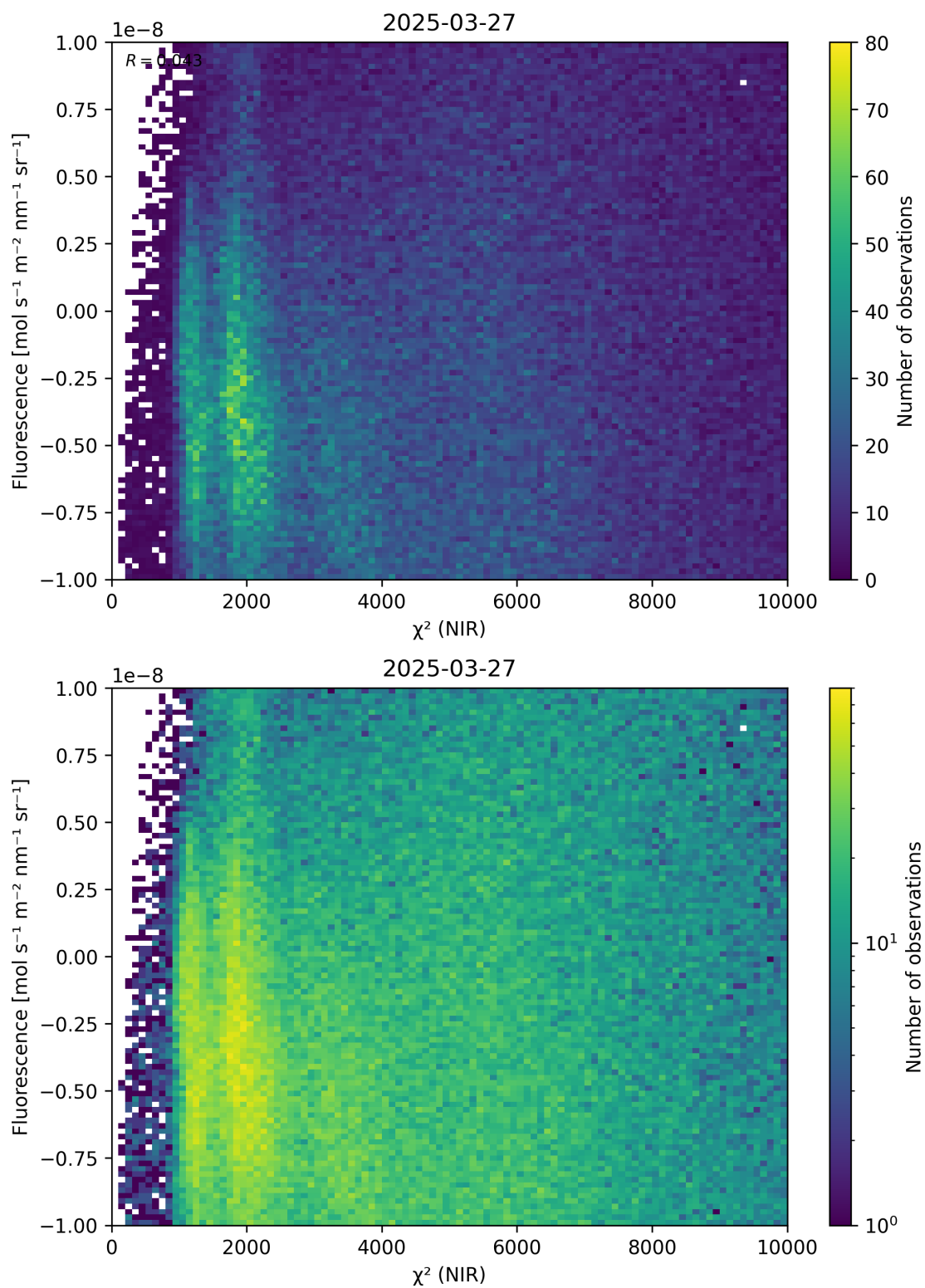
Figure 45: Scatter density plot of “ \chi^2 (NIR)” against “Fluorescence” for 2025-03-26 to 2025-03-28.
