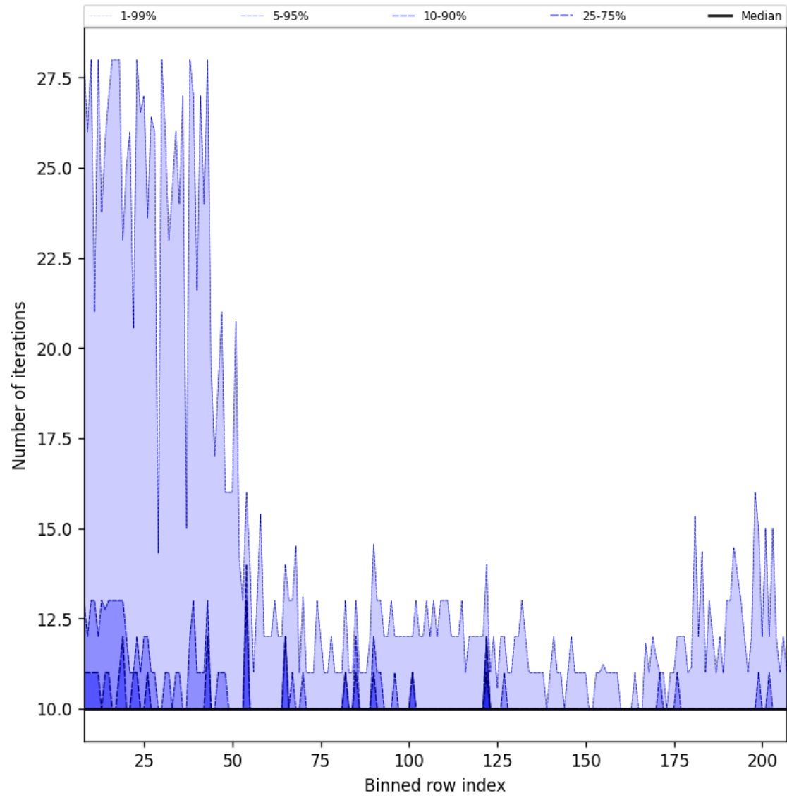
Figure 42: Along track statistics of “Number of iterations” for 2025-03-26 to 2025-03-28
