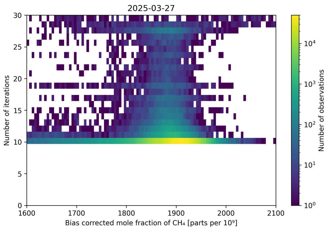
Figure 67: Scatter density plot of “Bias corrected mole fraction of CH 4 ” against “Number of iterations” for 2025-03-26 to 2025-03-28.
