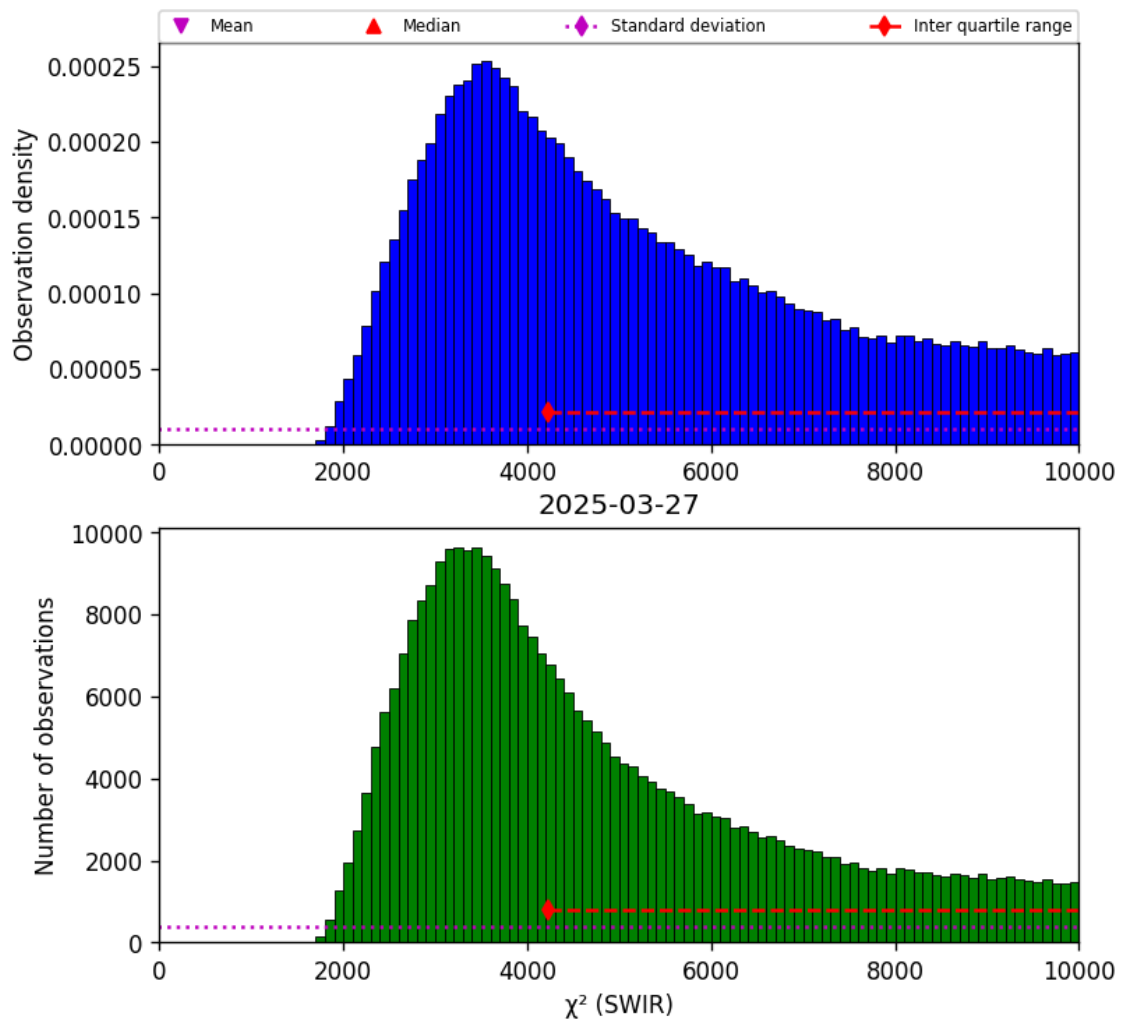
Figure 28: Histogram of “ \chi^2 (SWIR)” for 2025-03-26 to 2025-03-28
