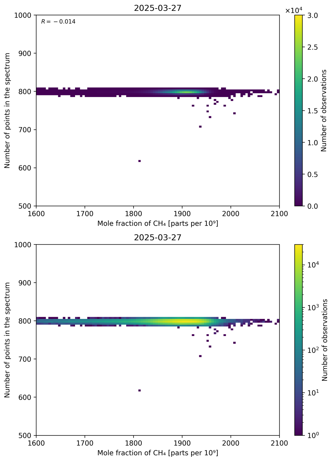
Figure 77: Scatter density plot of “Mole fraction of CH 4 ” against “Number of points in the spectrum” for 2025-03-26 to 2025-03-28.
