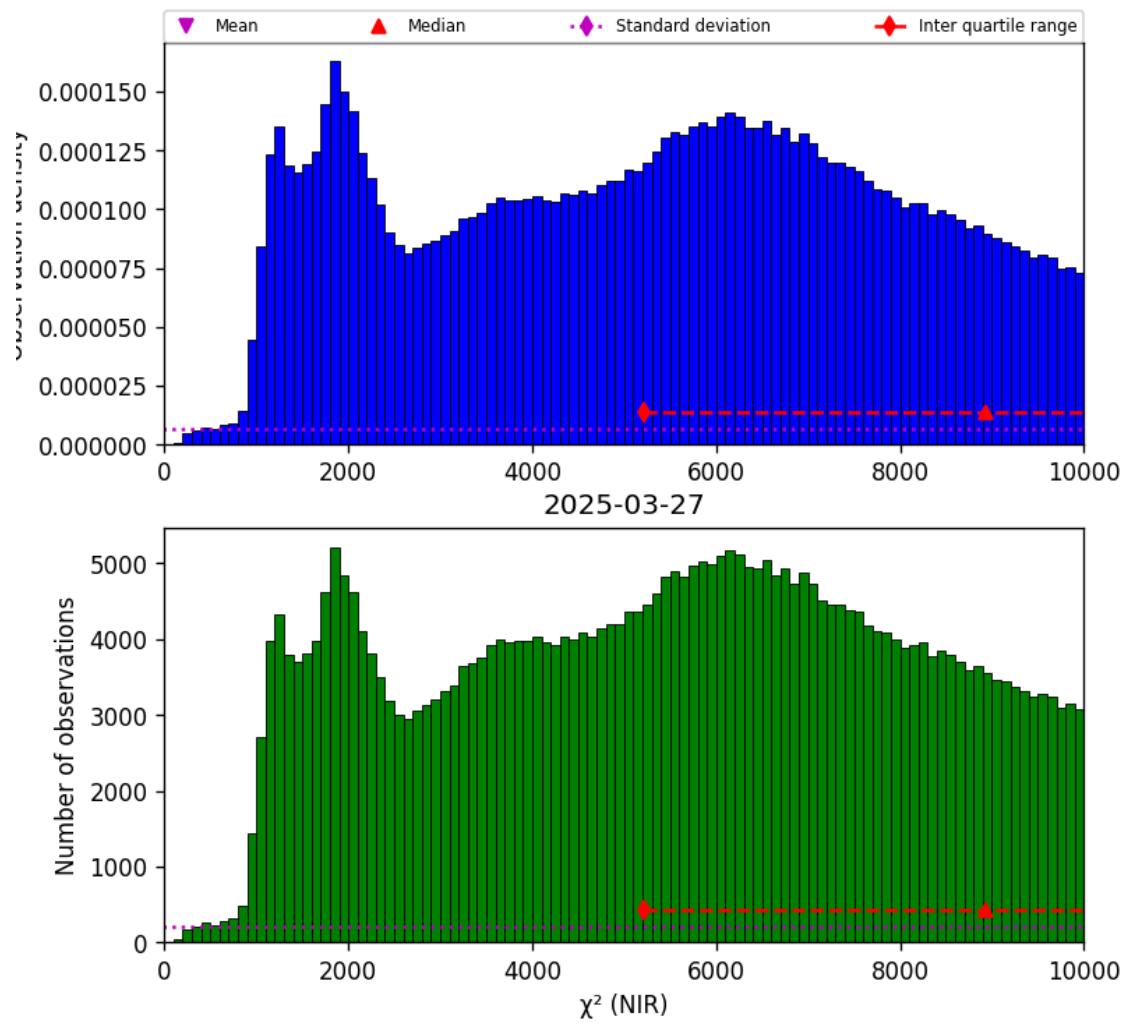
Figure 29: Histogram of “ \chi^2 (NIR)” for 2025-03-26 to 2025-03-28
