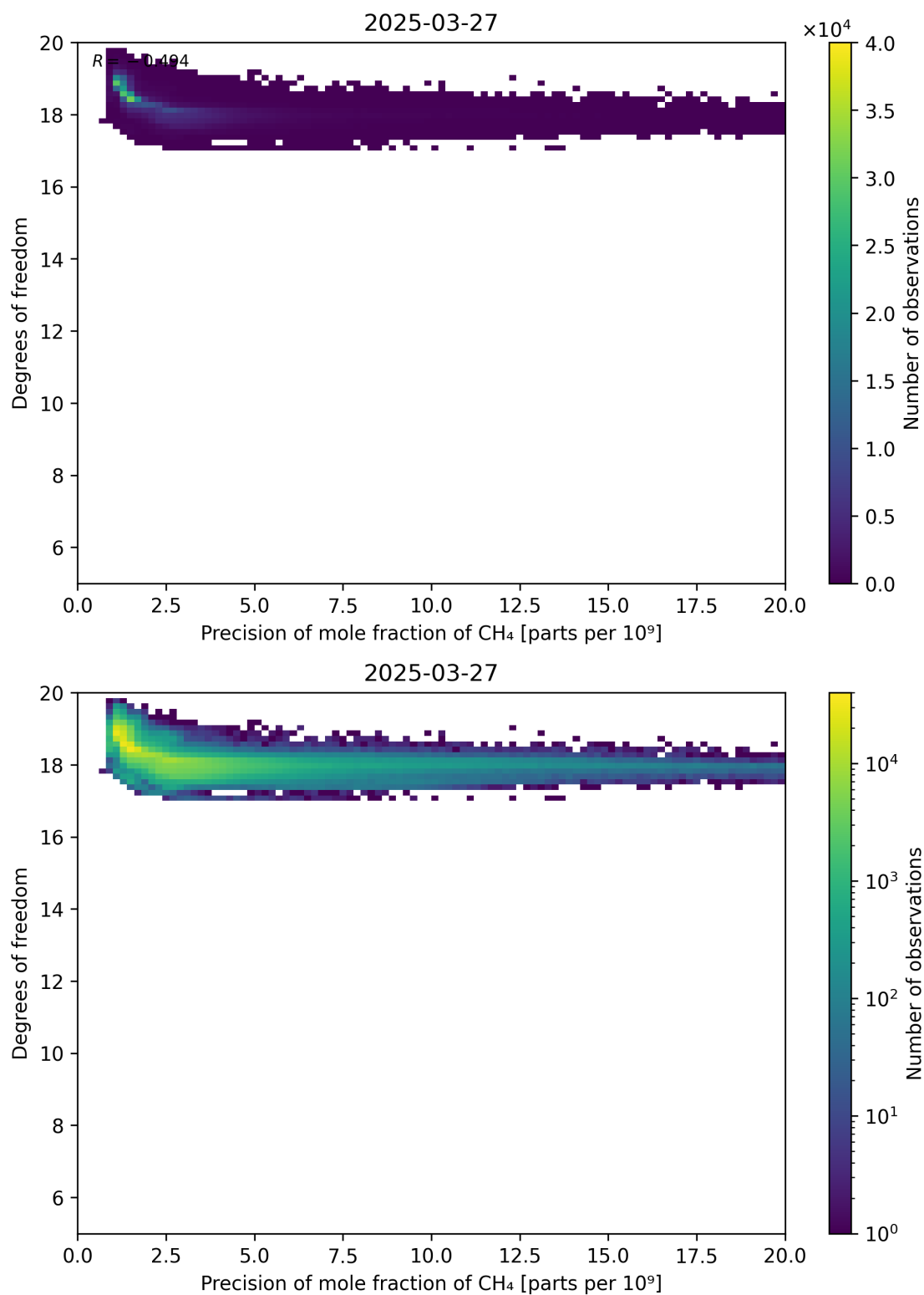
Figure 80: Scatter density plot of “Precision of mole fraction of CH 4 ” against “Degrees of freedom” for 2025-03-26 to 2025-03-28.
