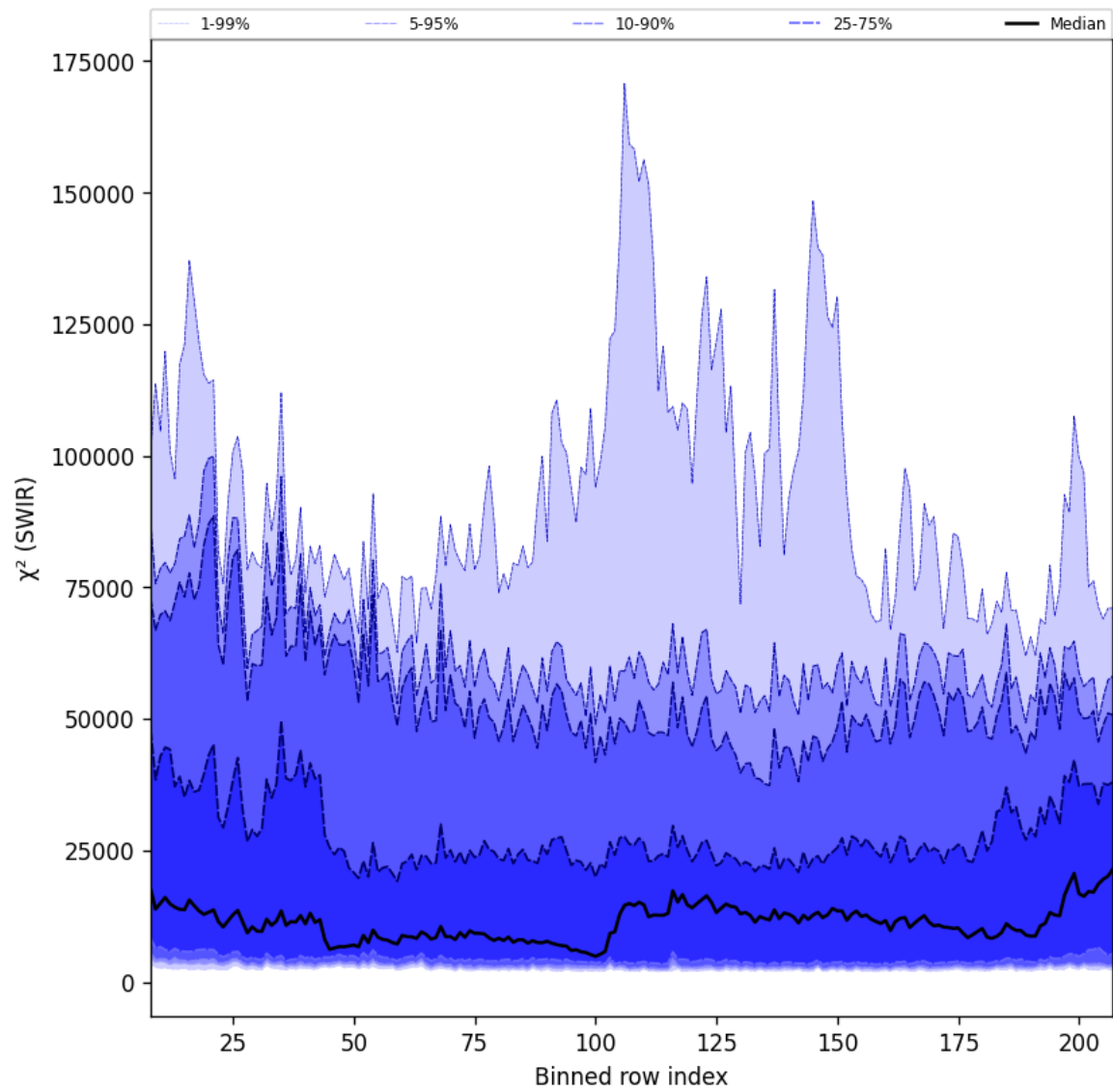
Figure 39: Along track statistics of “ \chi^2 (SWIR)” for 2025-03-26 to 2025-03-28
