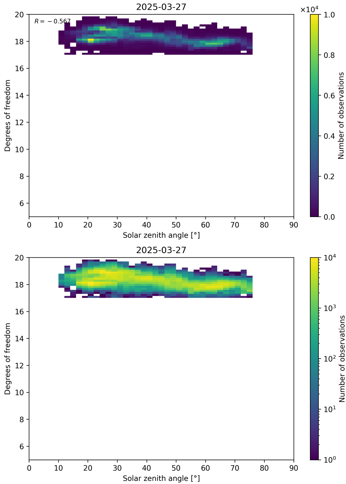
Figure 96: Scatter density plot of “Solar zenith angle” against “Degrees of freedom” for 2025-03-26 to 2025-03-28.
