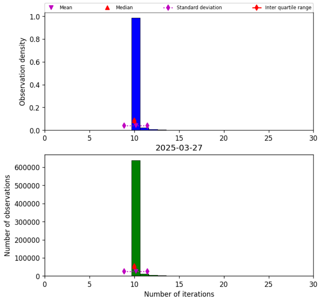
Figure 31: Histogram of “Number of iterations” for 2025-03-26 to 2025-03-28
