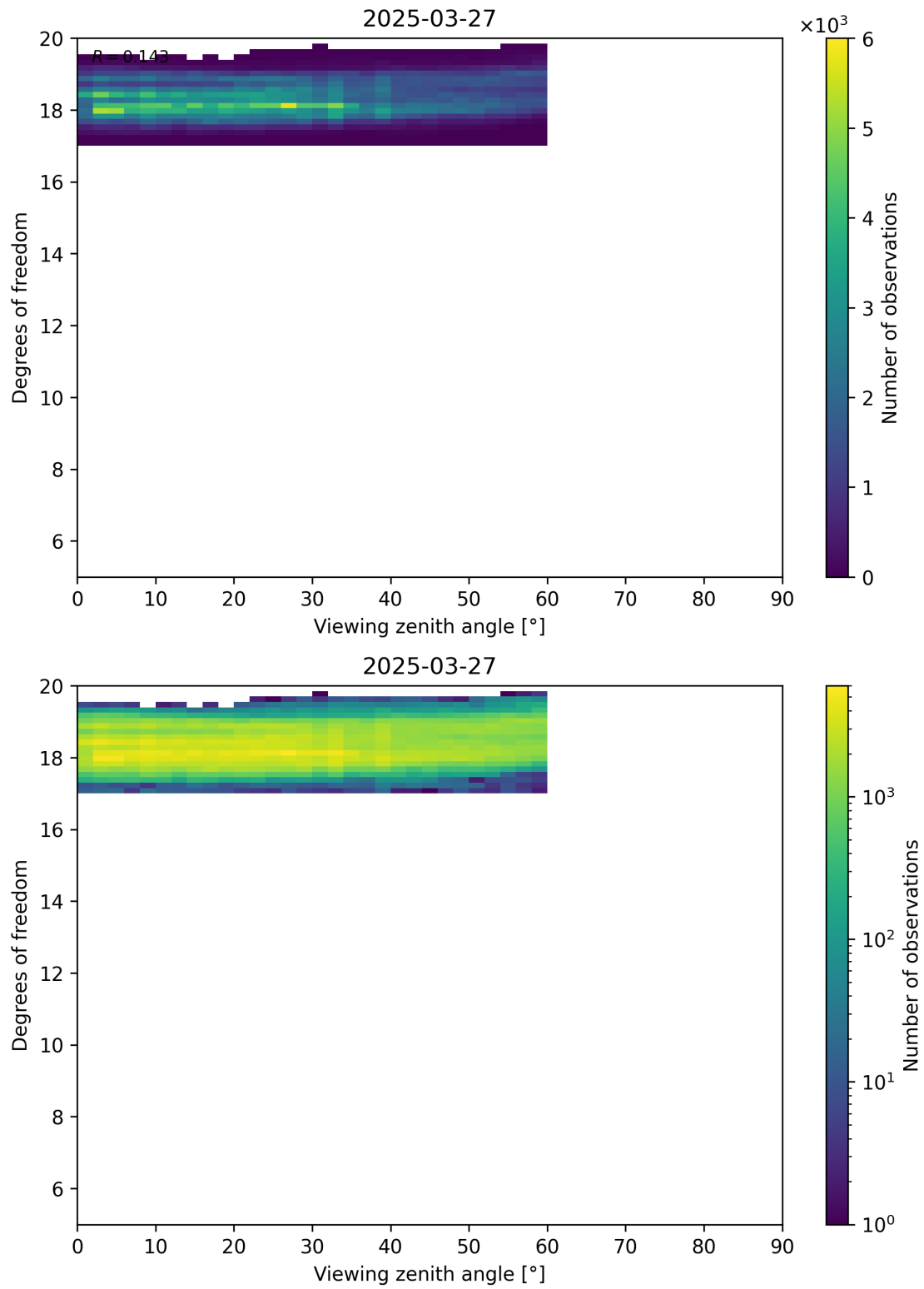
Figure 107: Scatter density plot of “Viewing zenith angle” against “Degrees of freedom” for 2025-03-26 to 2025-03-28.
