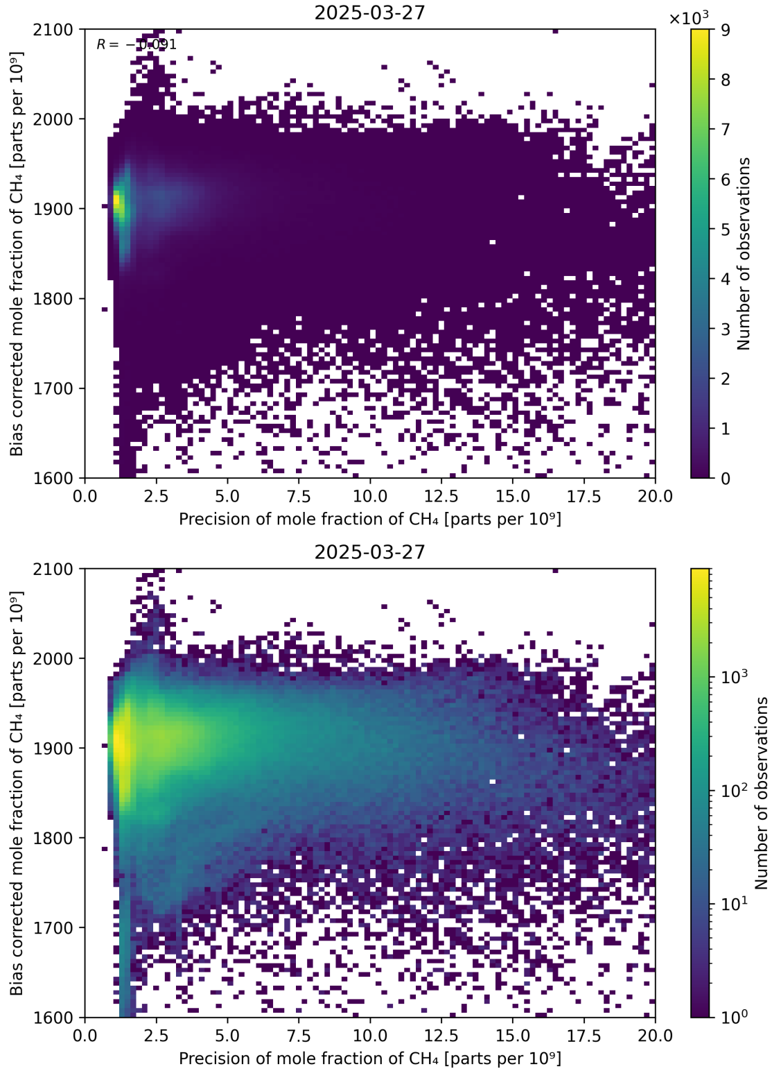
Figure 82: Scatter density plot of “Precision of mole fraction of CH 4 ” against “Bias corrected mole fraction of CH 4 ” for 2025-03-26 to 2025-03-28.
