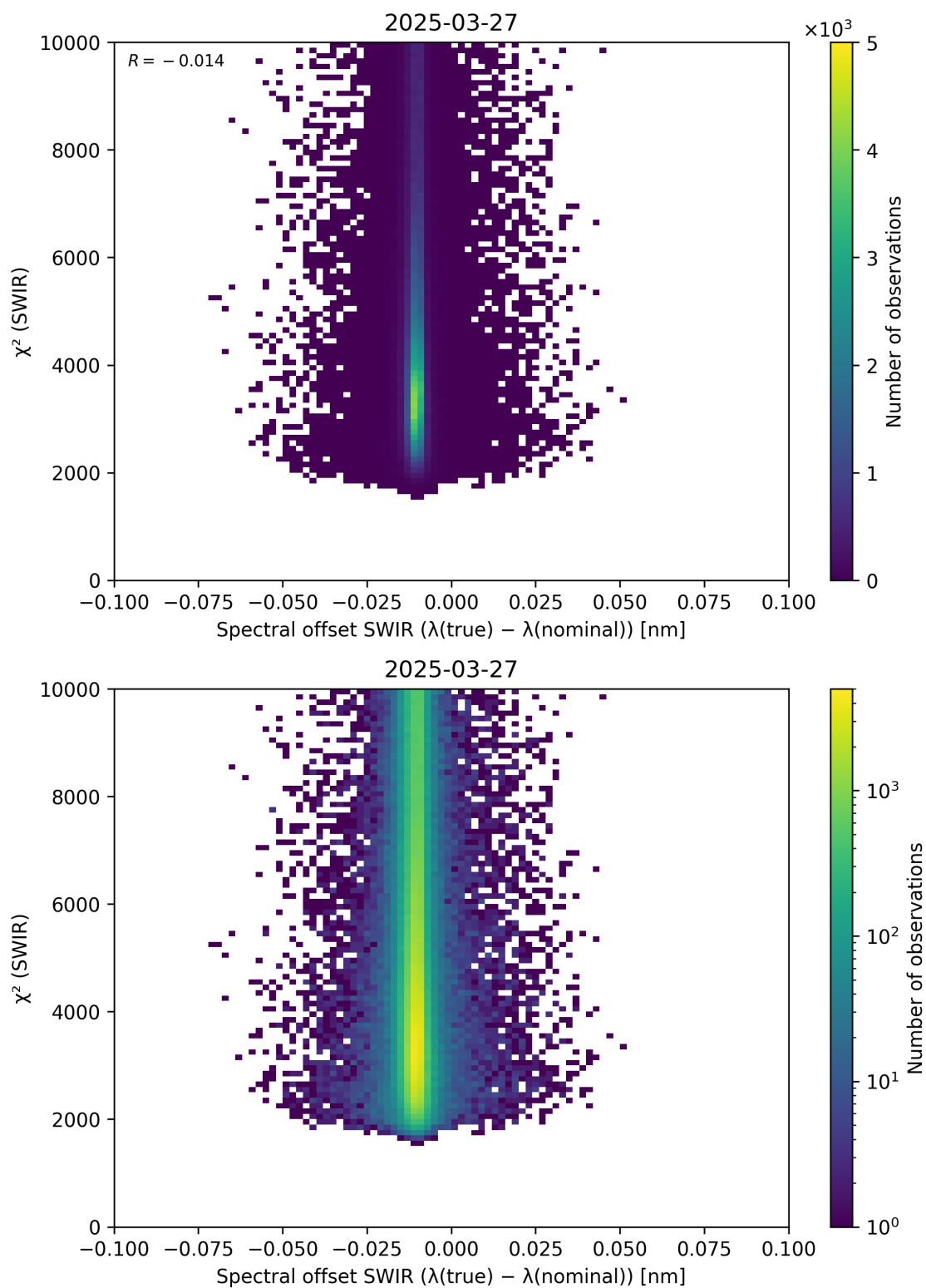
Figure 118: Scatter density plot of “Spectral offset SWIR ( \lambda_{\text{true}} - \lambda_{\text{nominal}} )” against “ \chi^2 (SWIR)” for 2025-03-26 to 2025-03-28.
