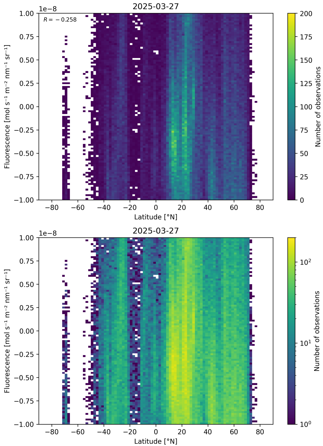
Figure 56: Scatter density plot of “Latitude” against “Fluorescence” for 2025-03-26 to 2025-03-28.
