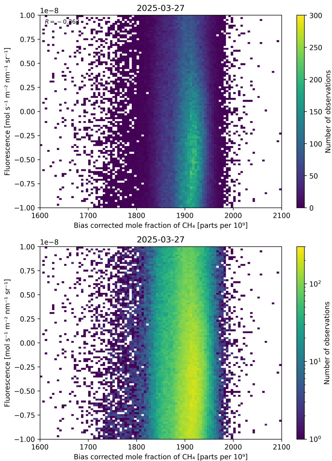
Figure 66: Scatter density plot of “Bias corrected mole fraction of \text{CH}_4 ” against “Fluorescence” for 2025-03-26 to 2025-03-28.
