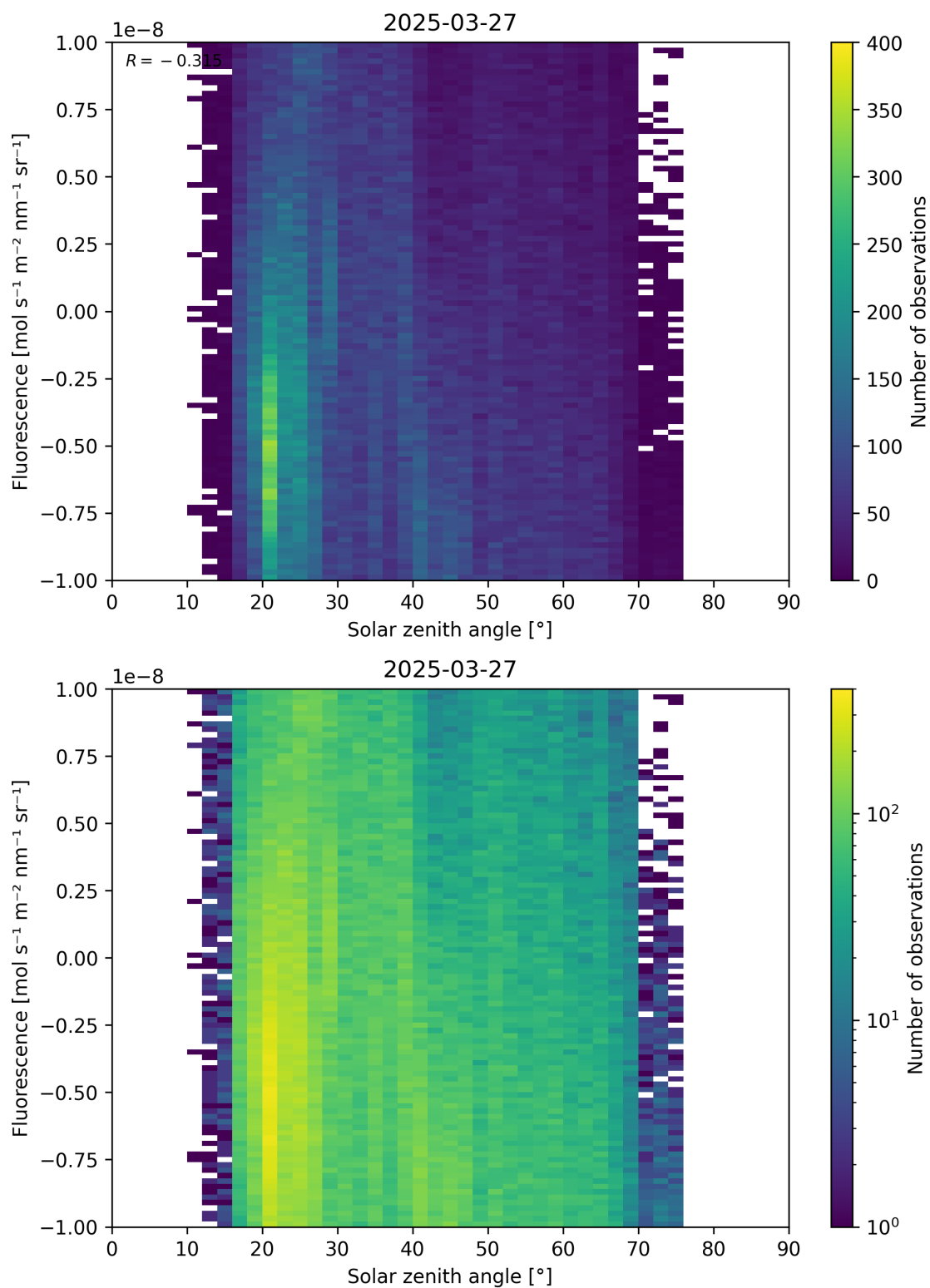
Figure 97: Scatter density plot of “Solar zenith angle” against “Fluorescence” for 2025-03-26 to 2025-03-28.
