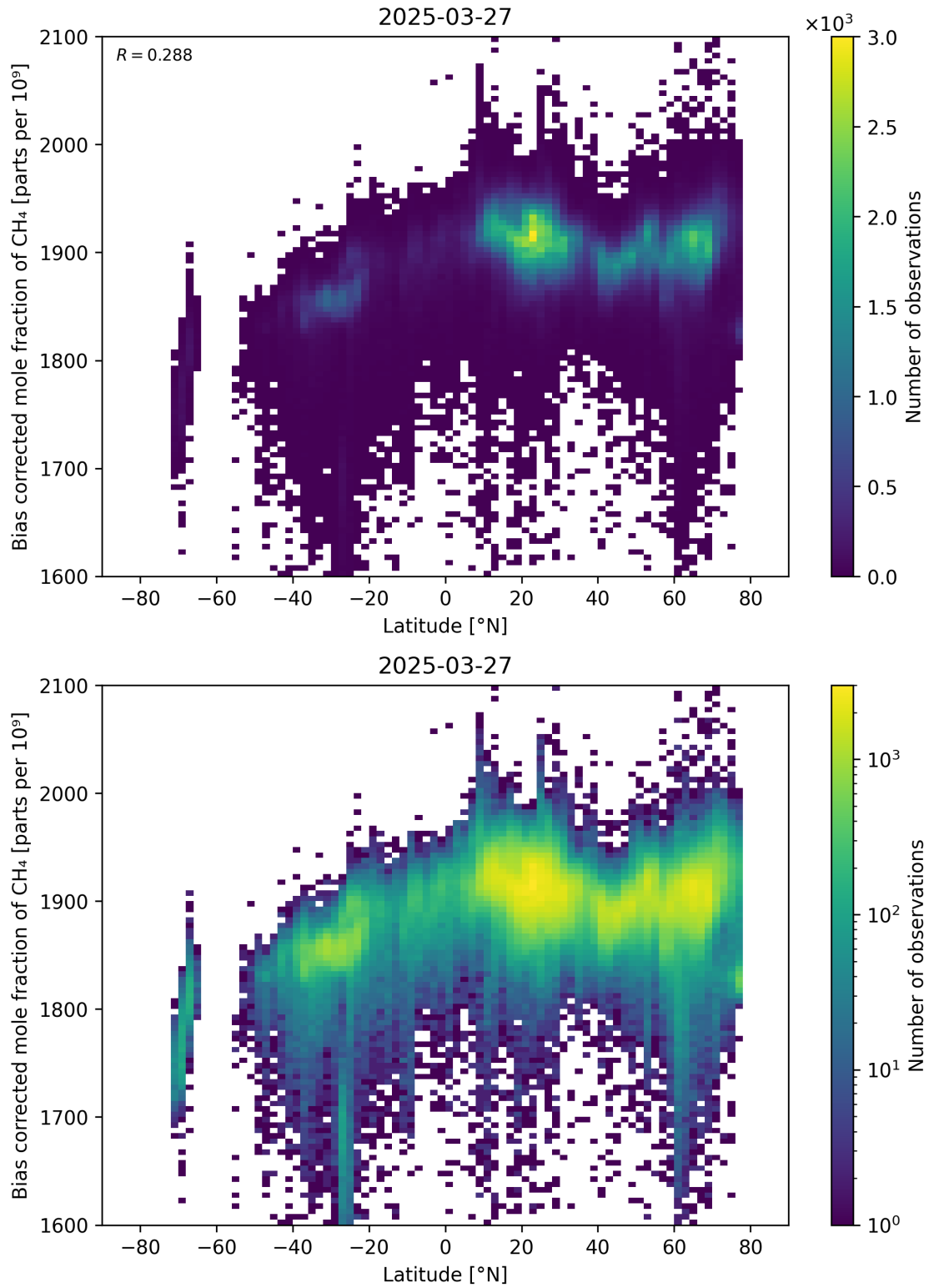
Figure 58: Scatter density plot of “Latitude” against “Bias corrected mole fraction of CH 4 ” for 2025-03-26 to 2025-03-28.
