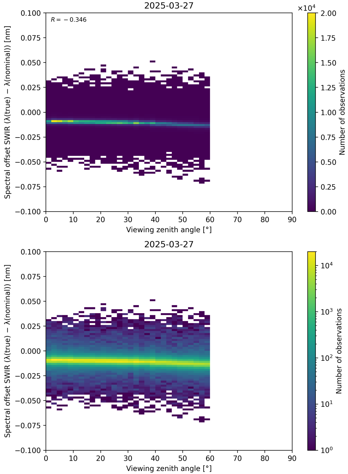
Figure 116: Scatter density plot of “Viewing zenith angle” against “Spectral offset SWIR ( \lambda_{\text{true}} - \lambda_{\text{nominal}} )” for 2025-03-26 to 2025-03-28.
