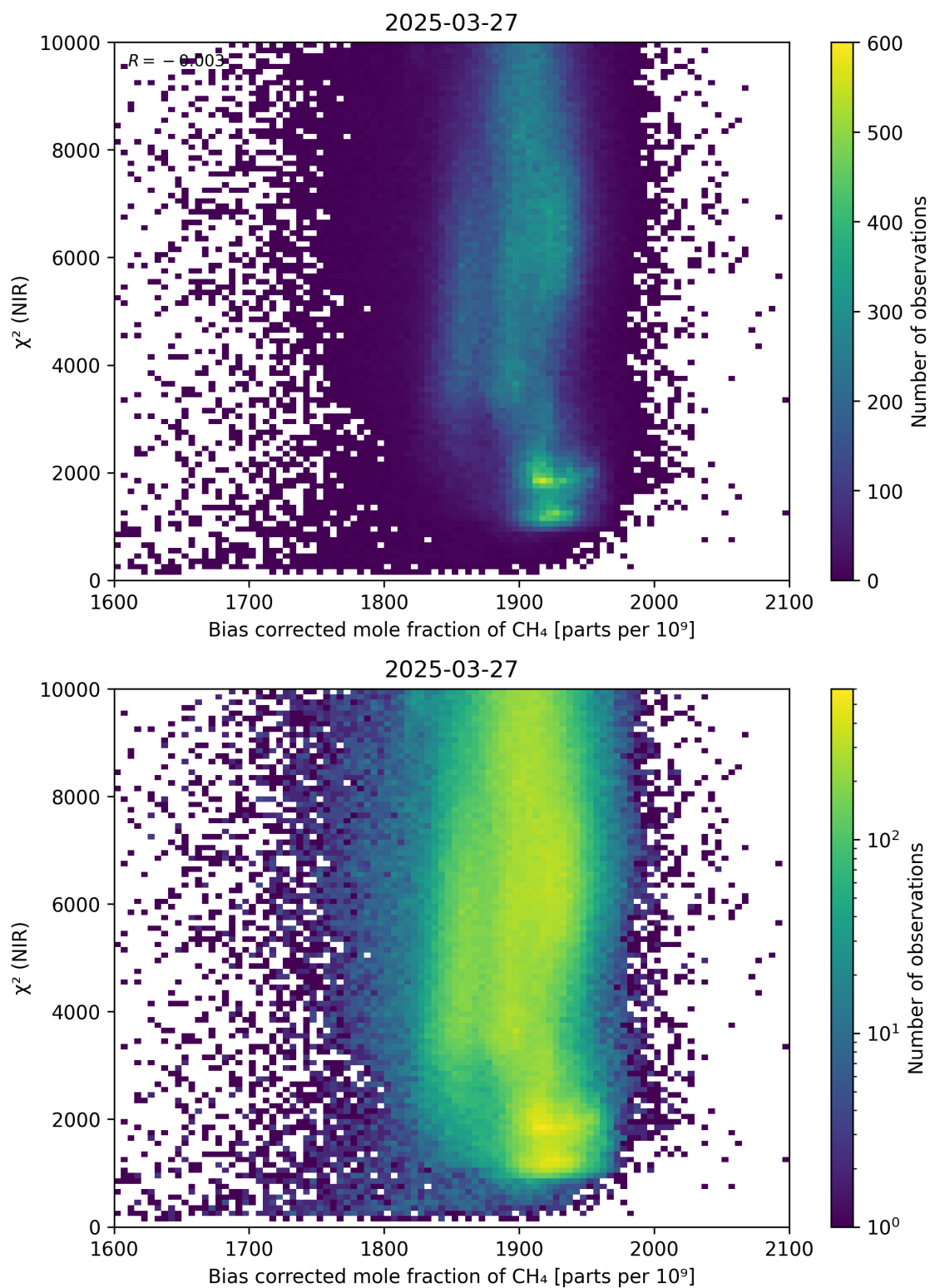
Figure 63: Scatter density plot of “Bias corrected mole fraction of CH 4 ” against “ \chi^2 (NIR)” for 2025-03-26 to 2025-03-28.
