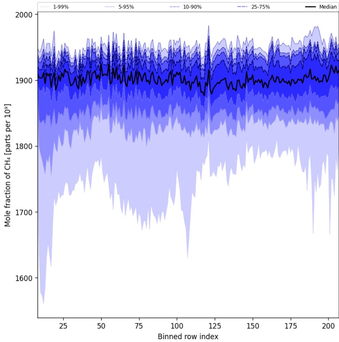
Figure 34: Along track statistics of “Mole fraction of CH 4 ” for 2025-03-26 to 2025-03-28
