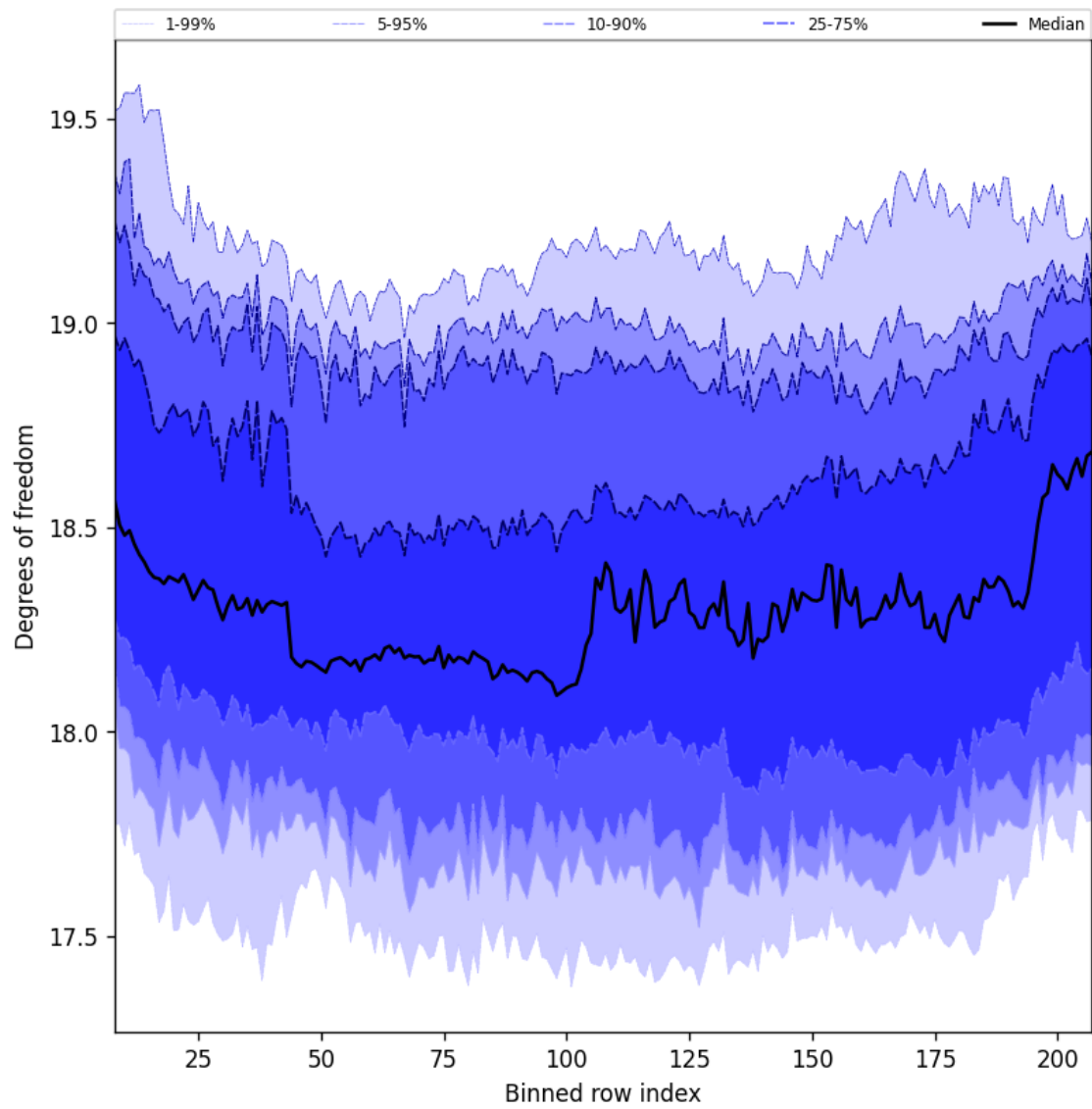
Figure 41: Along track statistics of “Degrees of freedom” for 2025-03-26 to 2025-03-28
