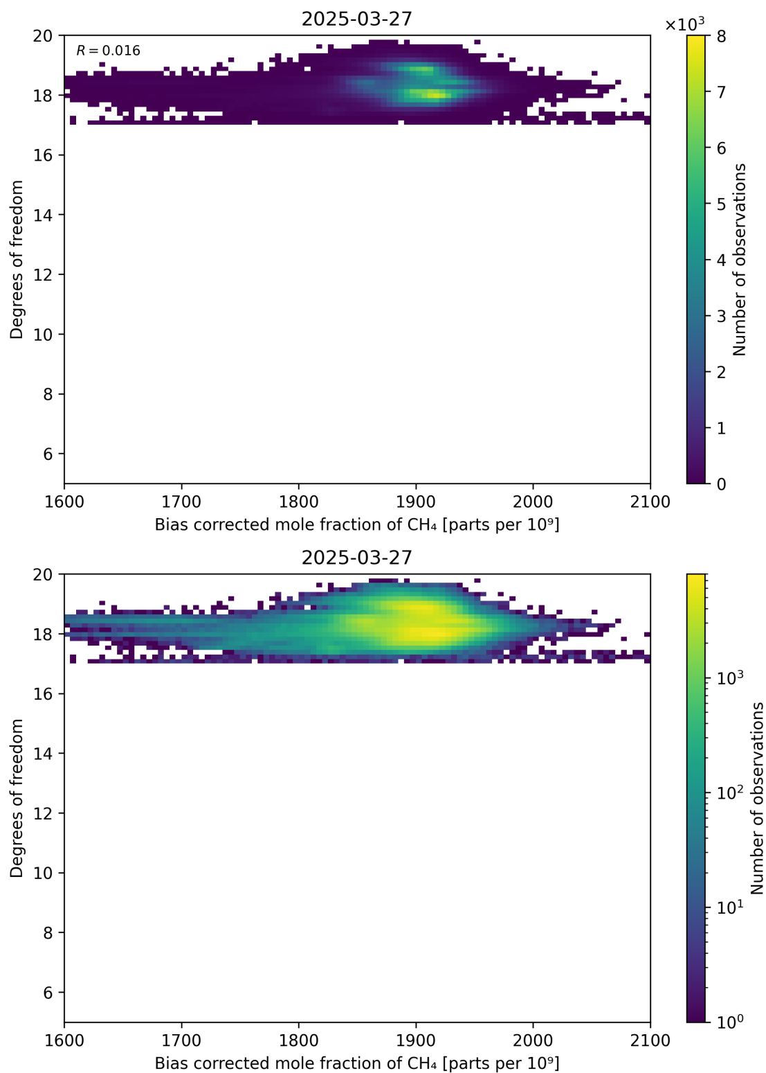
Figure 65: Scatter density plot of “Bias corrected mole fraction of CH 4 ” against “Degrees of freedom” for 2025-03-26 to 2025-03-28.
