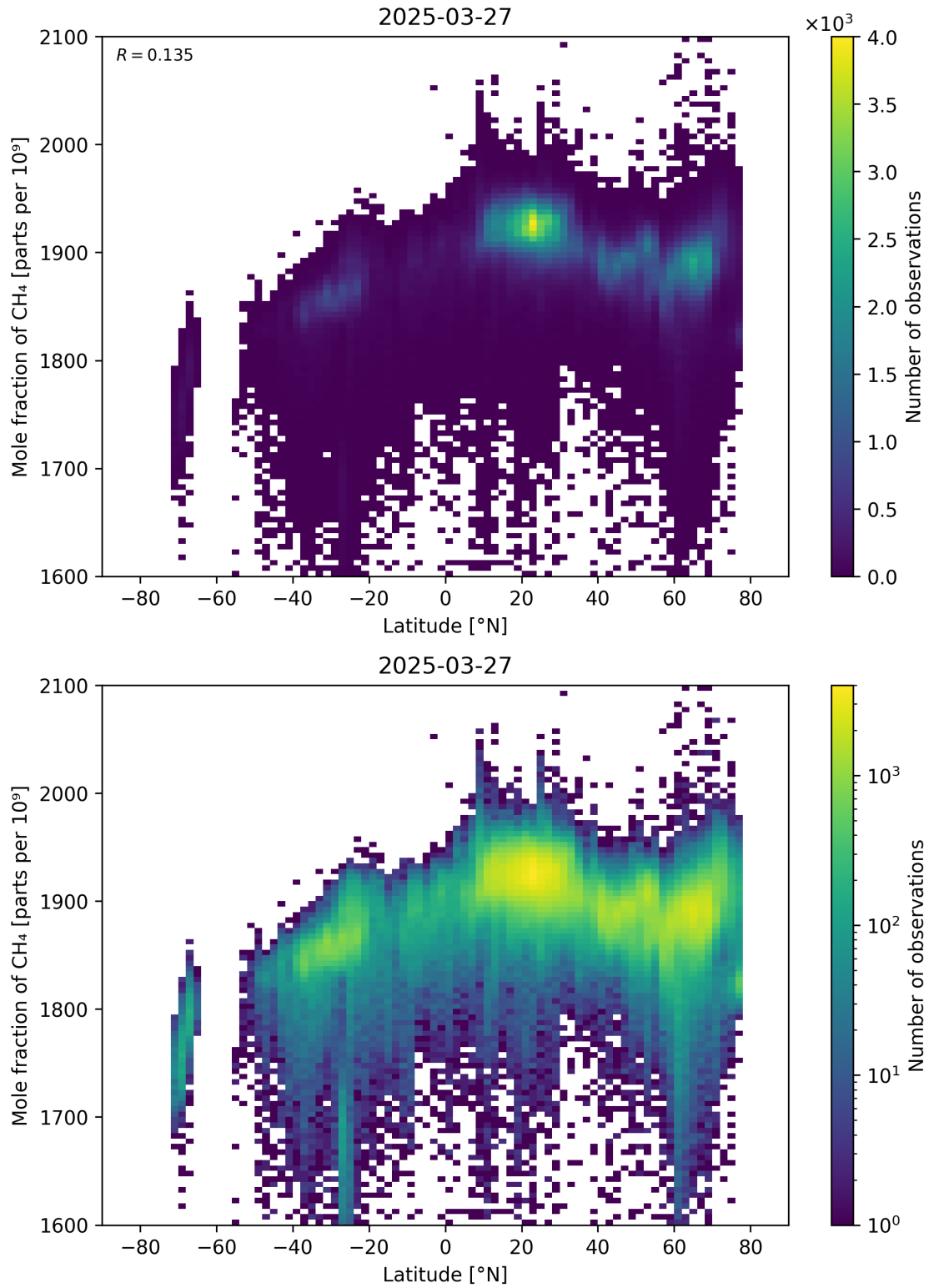
Figure 57: Scatter density plot of “Latitude” against “Mole fraction of CH 4 ” for 2025-03-26 to 2025-03-28.
