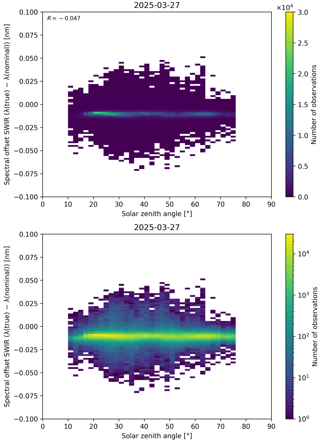
Figure 104: Scatter density plot of “Solar zenith angle” against “Spectral offset SWIR ( \lambda_{\text{true}} - \lambda_{\text{nominal}} )” for 2025-03-26 to 2025-03-28.
