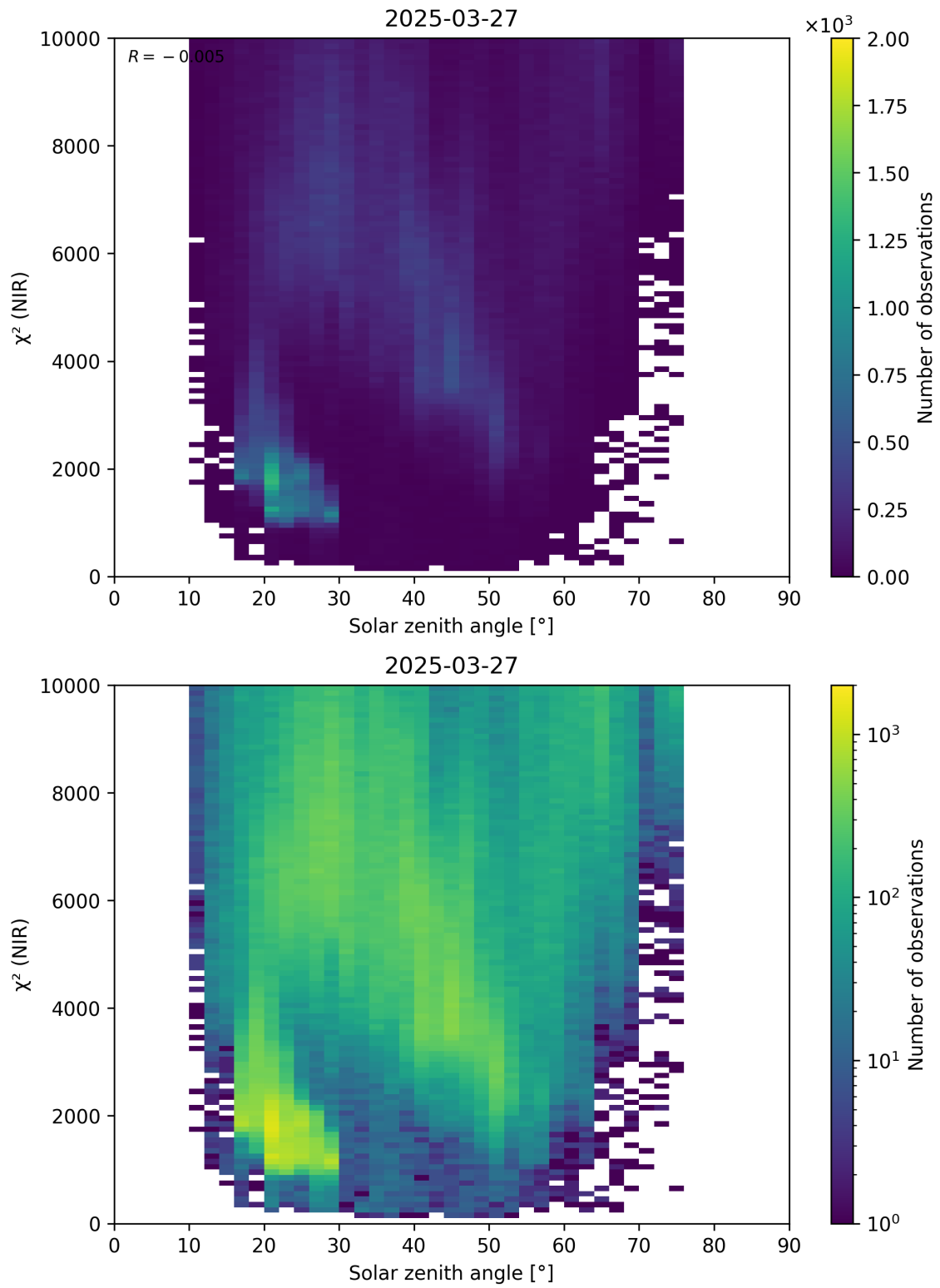
Figure 94: Scatter density plot of “Solar zenith angle” against “ \chi^2 (NIR)” for 2025-03-26 to 2025-03-28.
