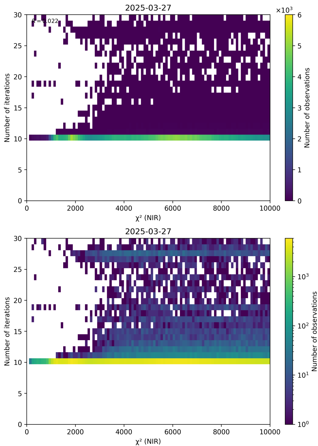
Figure 46: Scatter density plot of “ \chi^2 (NIR)” against “Number of iterations” for 2025-03-26 to 2025-03-28.
