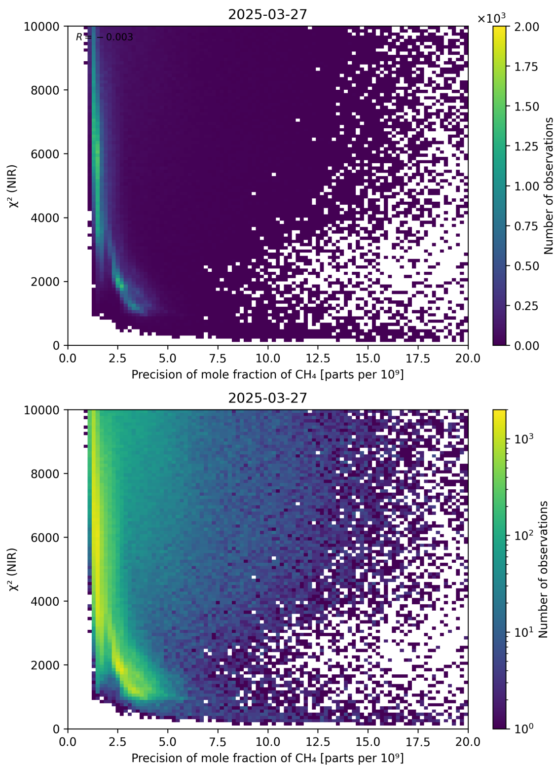
Figure 78: Scatter density plot of “Precision of mole fraction of CH 4 ” against “ \chi^2 (NIR)” for 2025-03-26 to 2025-03-28.
