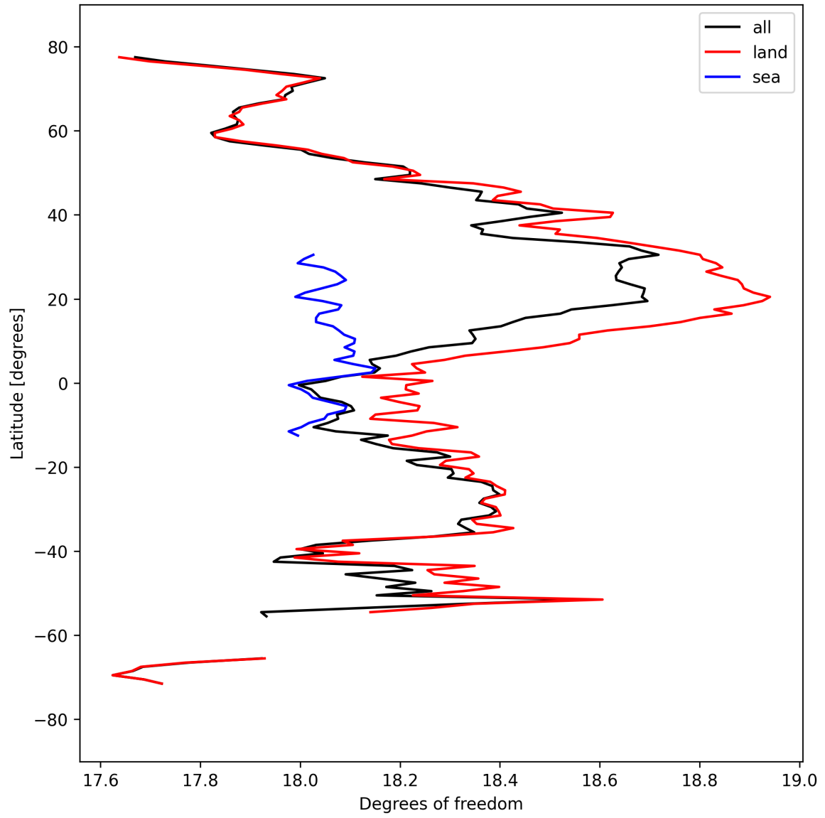
Figure 19: Zonal average of “Degrees of freedom” for 2025-03-26 to 2025-03-28.
