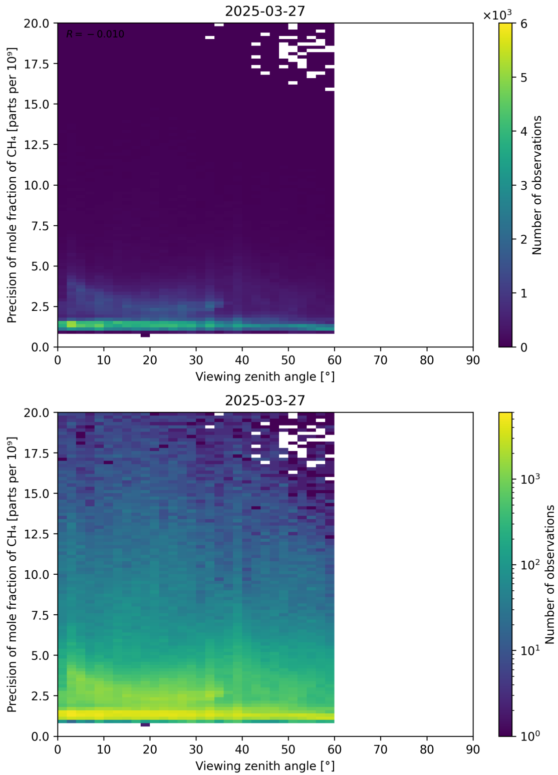
Figure 112: Scatter density plot of “Viewing zenith angle” against “Precision of mole fraction of CH 4 ” for 2025-03-26 to 2025-03-28.
