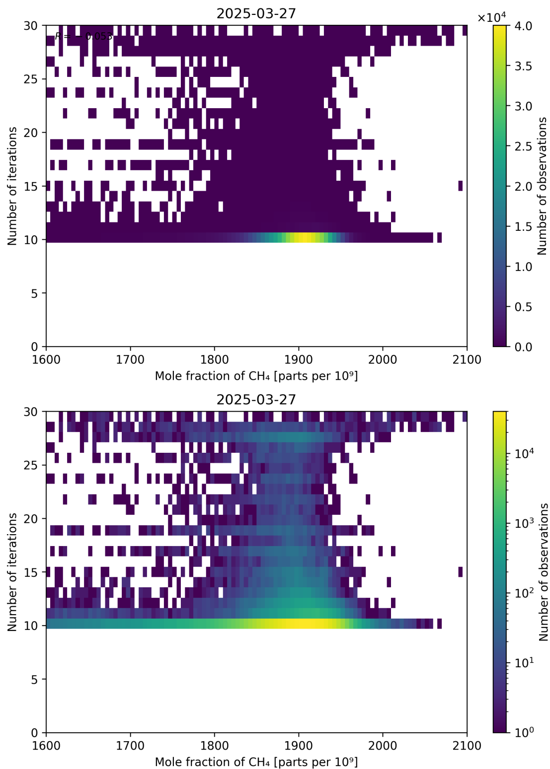
Figure 76: Scatter density plot of “Mole fraction of CH 4 ” against “Number of iterations” for 2025-03-26 to 2025-03-28.
