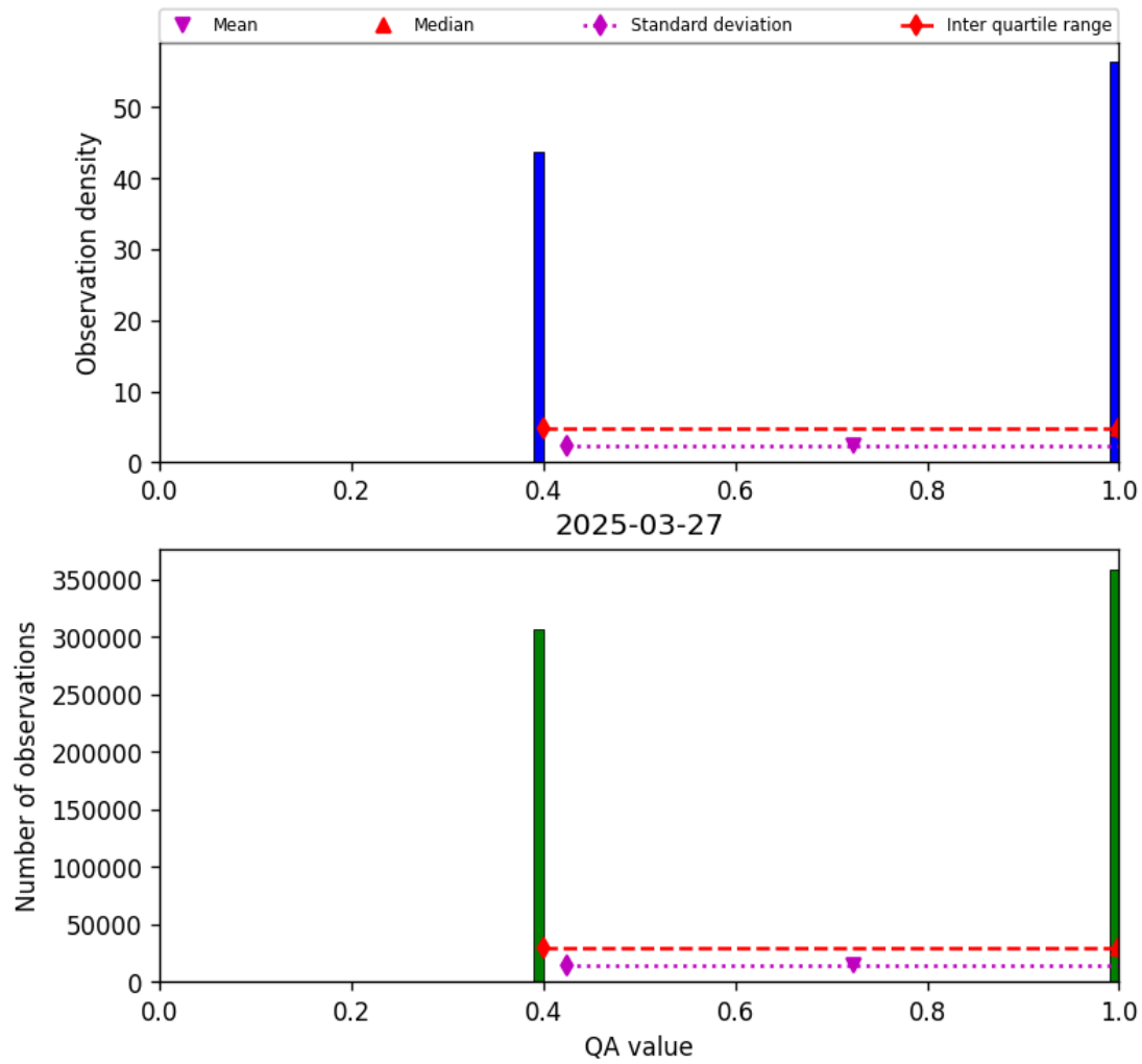
Figure 22: Histogram of “QA value” for 2025-03-26 to 2025-03-28
