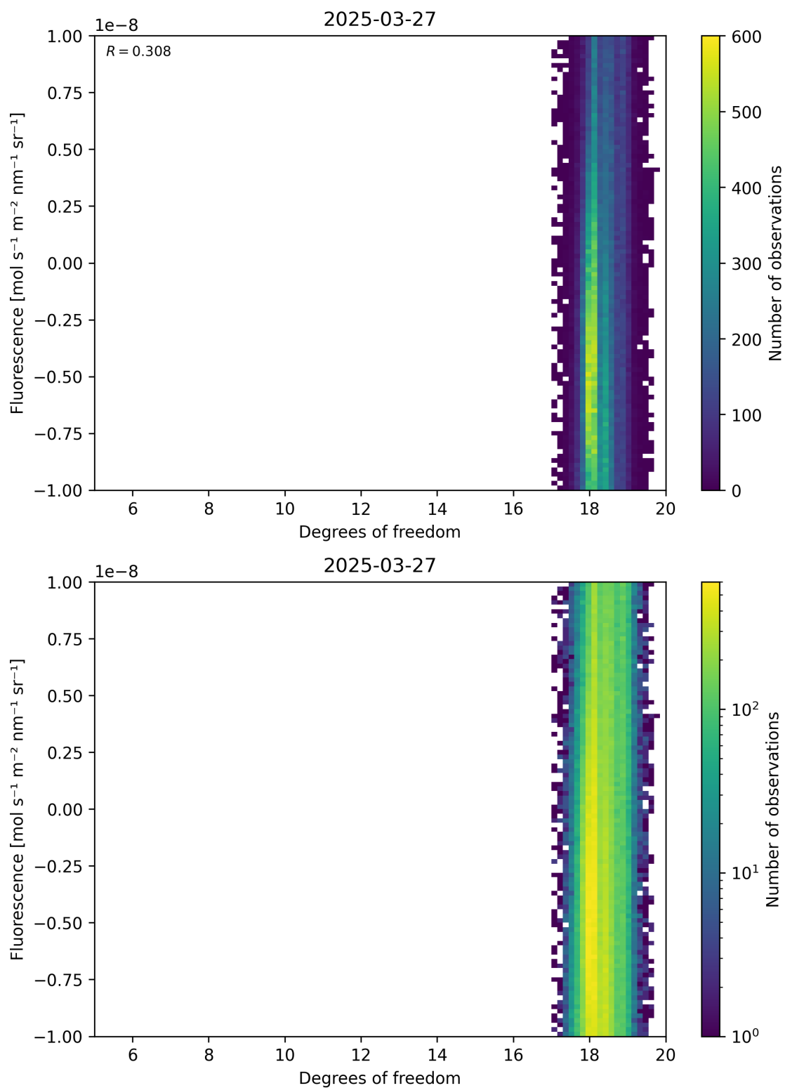
Figure 51: Scatter density plot of “Degrees of freedom” against “Fluorescence” for 2025-03-26 to 2025-03-28.
