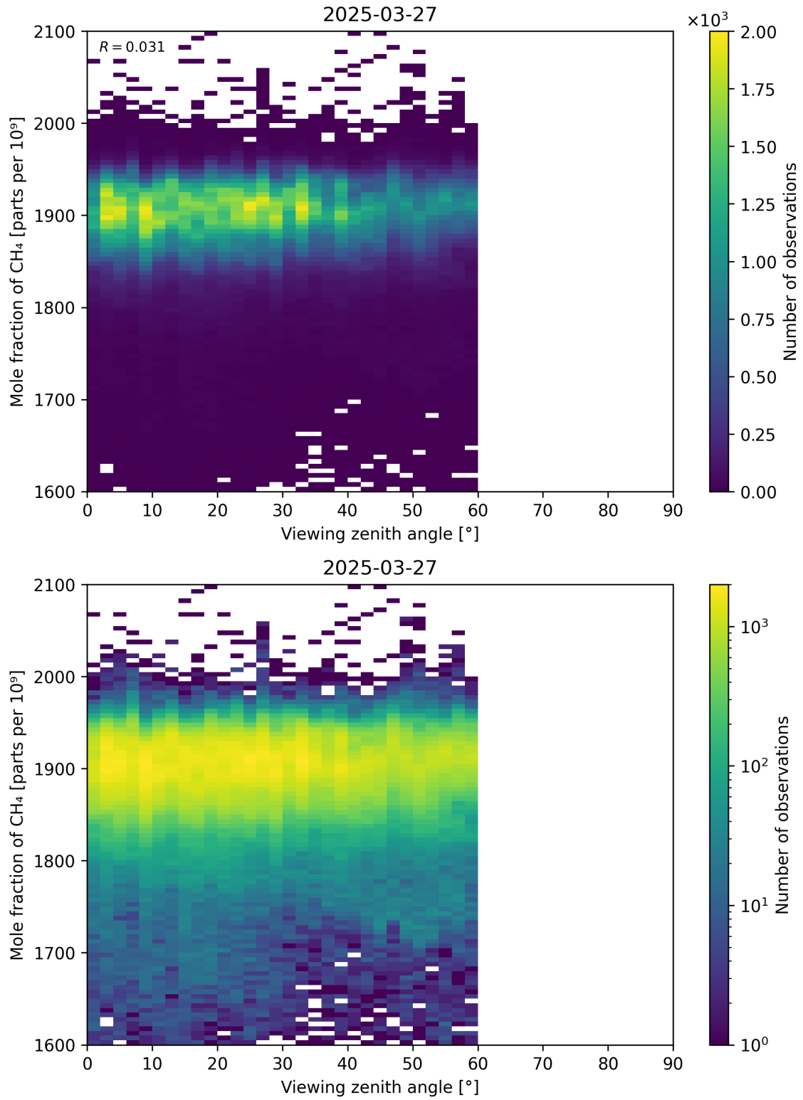
Figure 110: Scatter density plot of “Viewing zenith angle” against “Mole fraction of CH 4 ” for 2025-03-26 to 2025-03-28.
