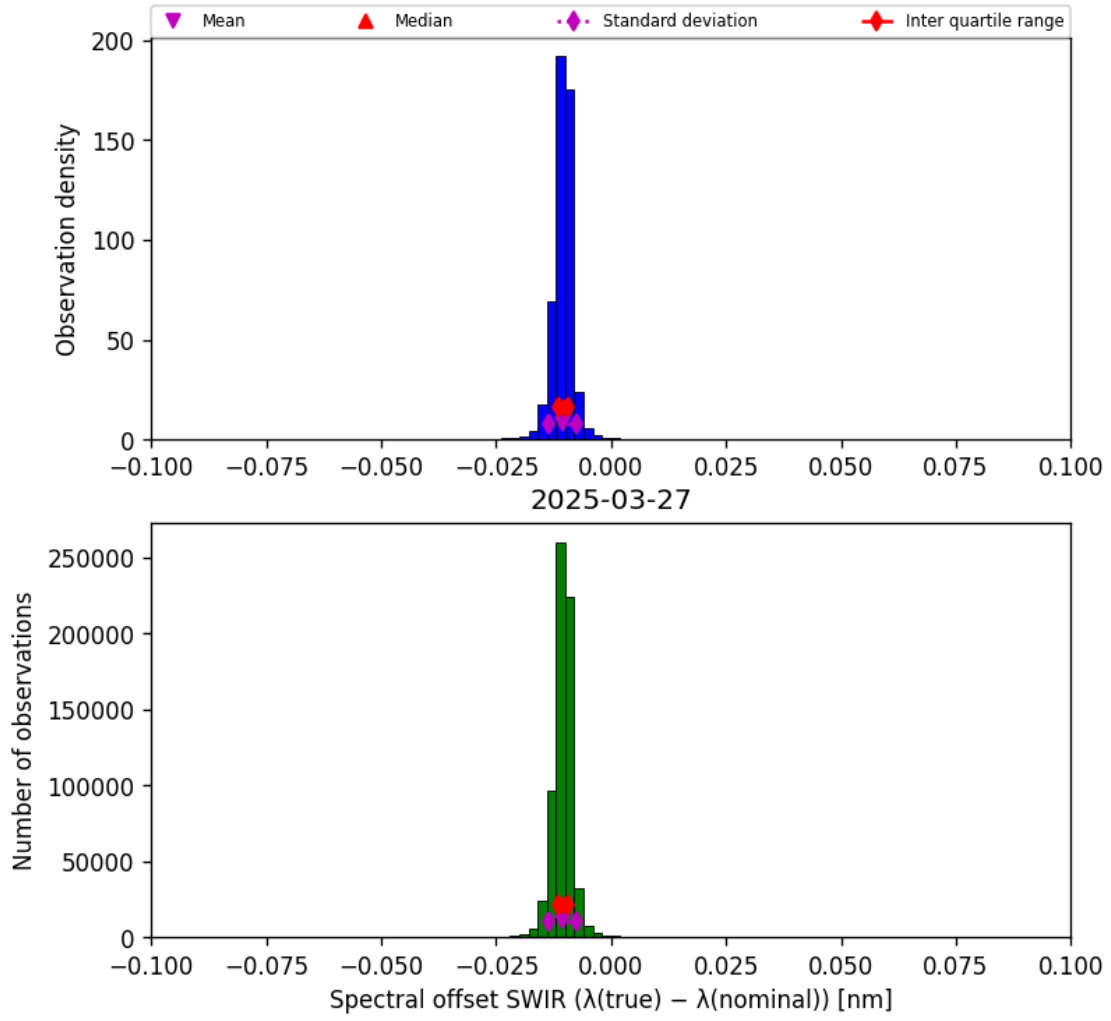
Figure 27: Histogram of “Spectral offset SWIR ( \lambda_{\text{true}} - \lambda_{\text{nominal}} )” for 2025-03-26 to 2025-03-28
