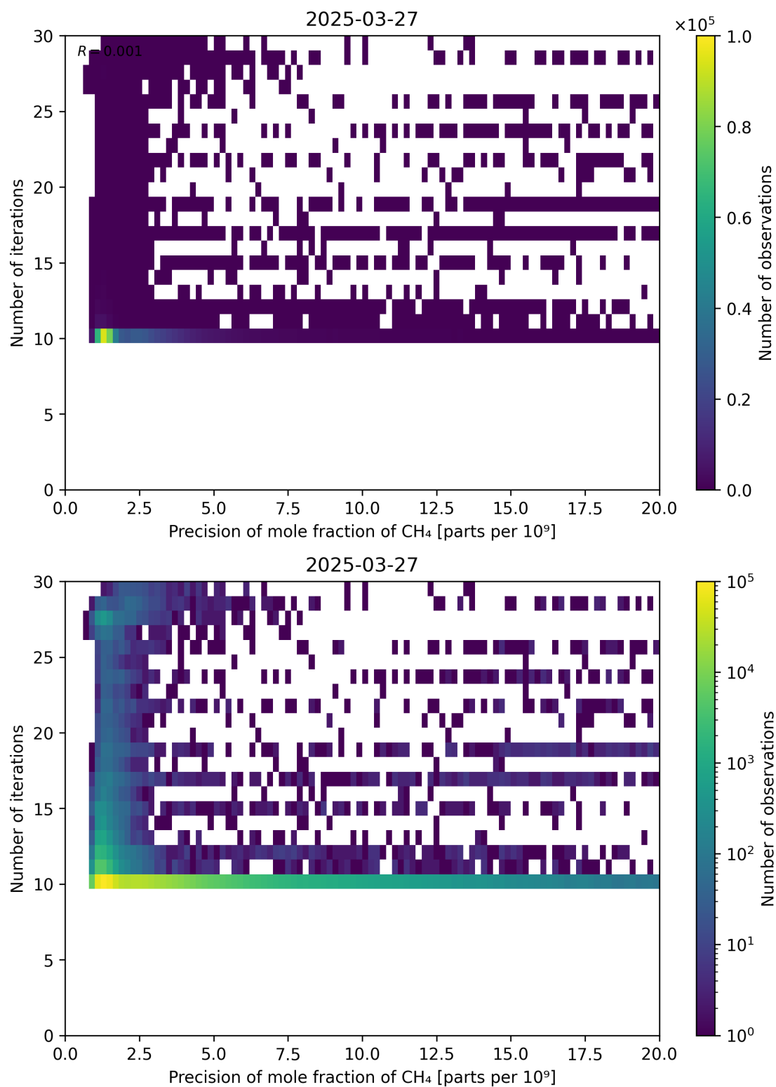
Figure 83: Scatter density plot of “Precision of mole fraction of CH 4 ” against “Number of iterations” for 2025-03-26 to 2025-03-28.
