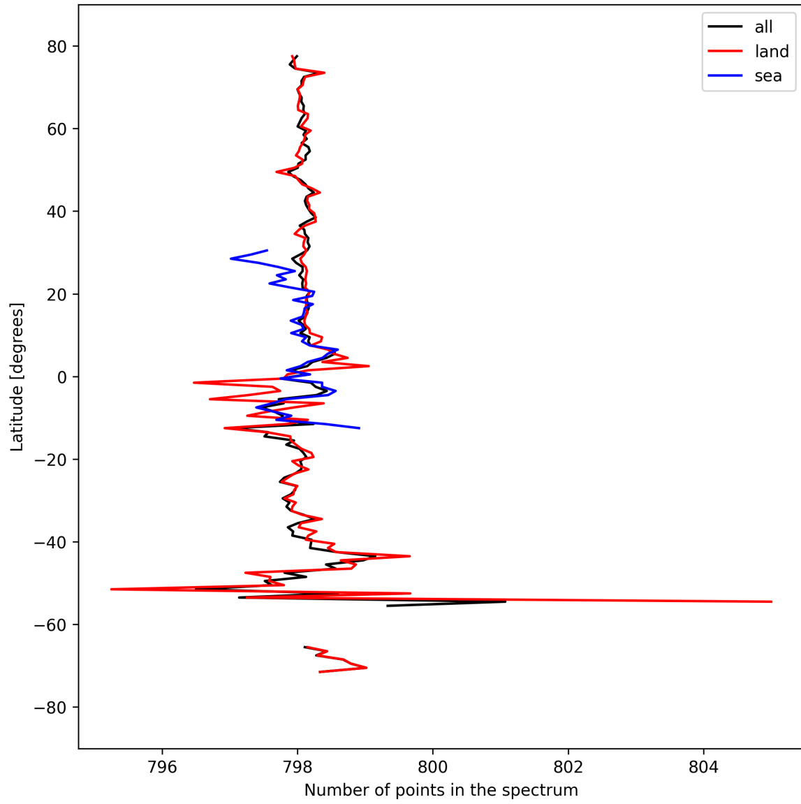
Figure 15: Zonal average of “Number of points in the spectrum” for 2025-03-26 to 2025-03-28.
