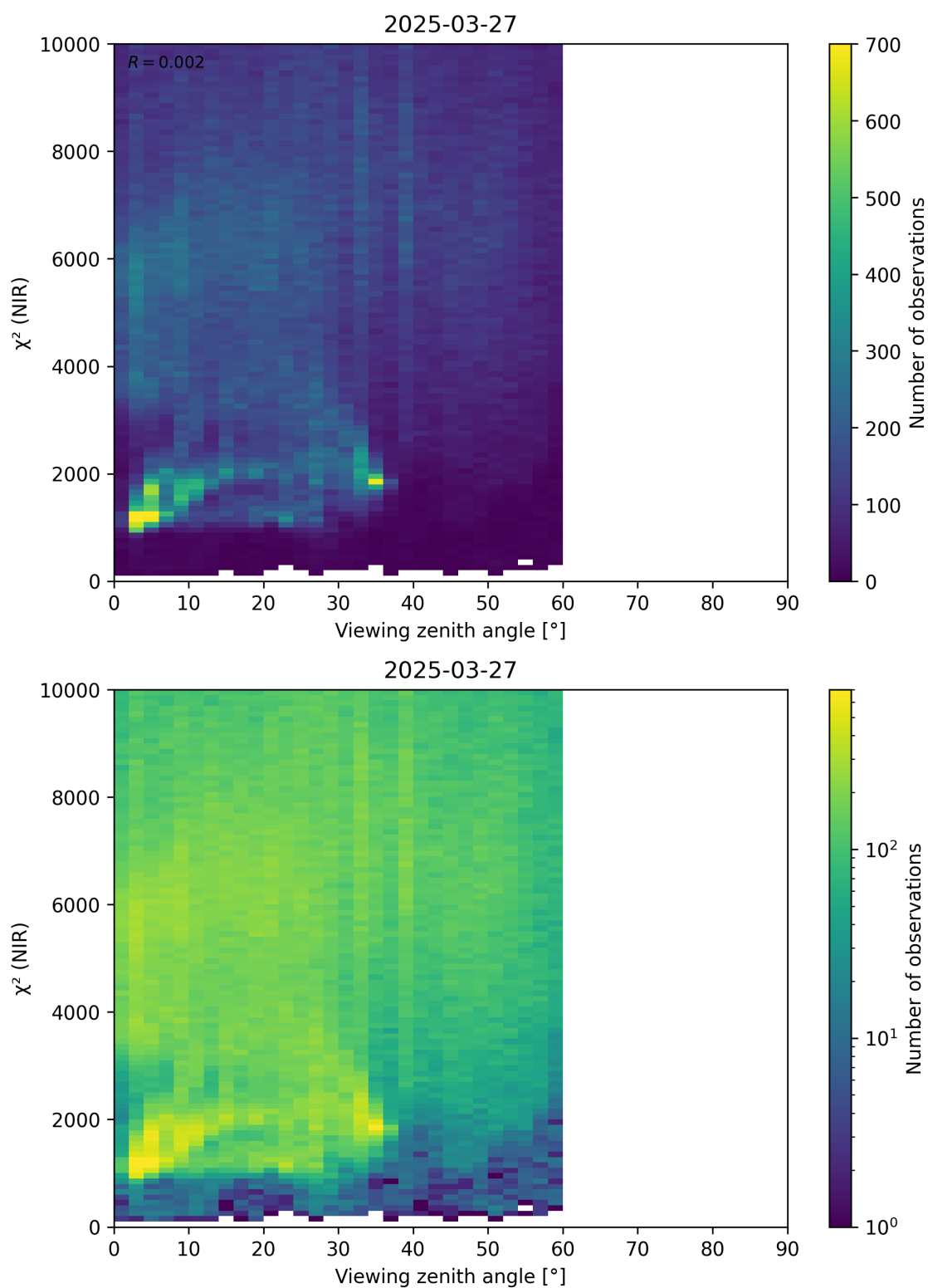
Figure 105: Scatter density plot of “Viewing zenith angle” against “ \chi^2 (NIR)” for 2025-03-26 to 2025-03-28.
