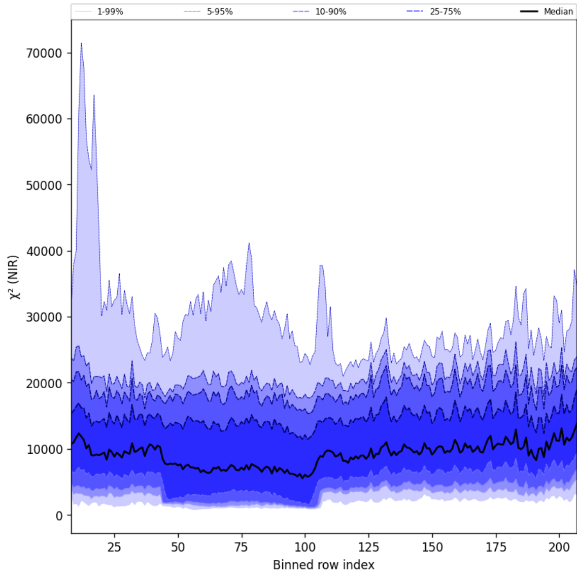
Figure 40: Along track statistics of “ \chi^2 (NIR)” for 2025-03-26 to 2025-03-28
