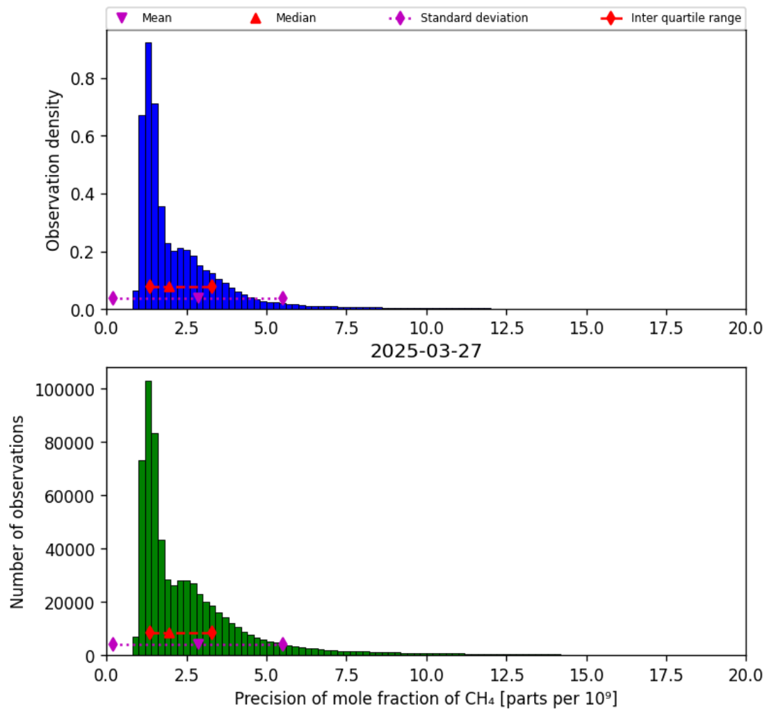
Figure 24: Histogram of “Precision of mole fraction of CH 4 ” for 2025-03-26 to 2025-03-28
