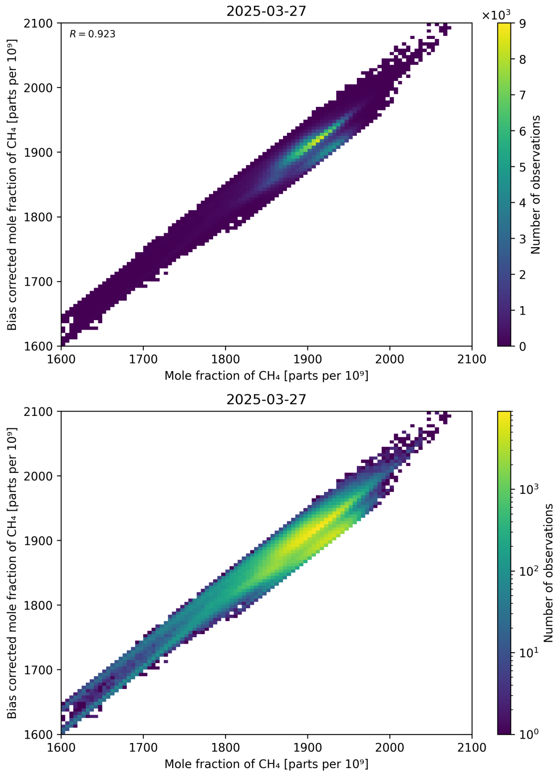
Figure 74: Scatter density plot of “Mole fraction of CH 4 ” against “Bias corrected mole fraction of CH 4 ” for 2025-03-26 to 2025-03-28.
