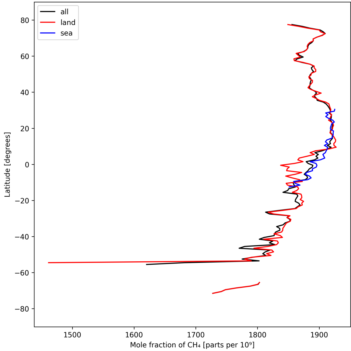
Figure 12: Zonal average of “Mole fraction of CH 4 ” for 2025-03-26 to 2025-03-28.
