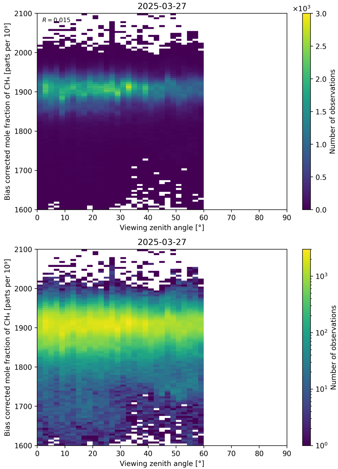
Figure 111: Scatter density plot of “Viewing zenith angle” against “Bias corrected mole fraction of CH 4 ” for 2025-03-26 to 2025-03-28.
