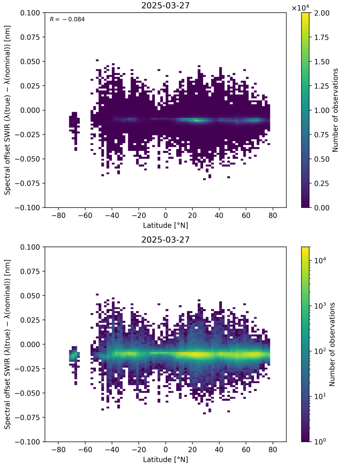
Figure 62: Scatter density plot of “Latitude” against “Spectral offset SWIR ( \lambda_{\text{true}} - \lambda_{\text{nominal}} )” for 2025-03-26 to 2025-03-28.
