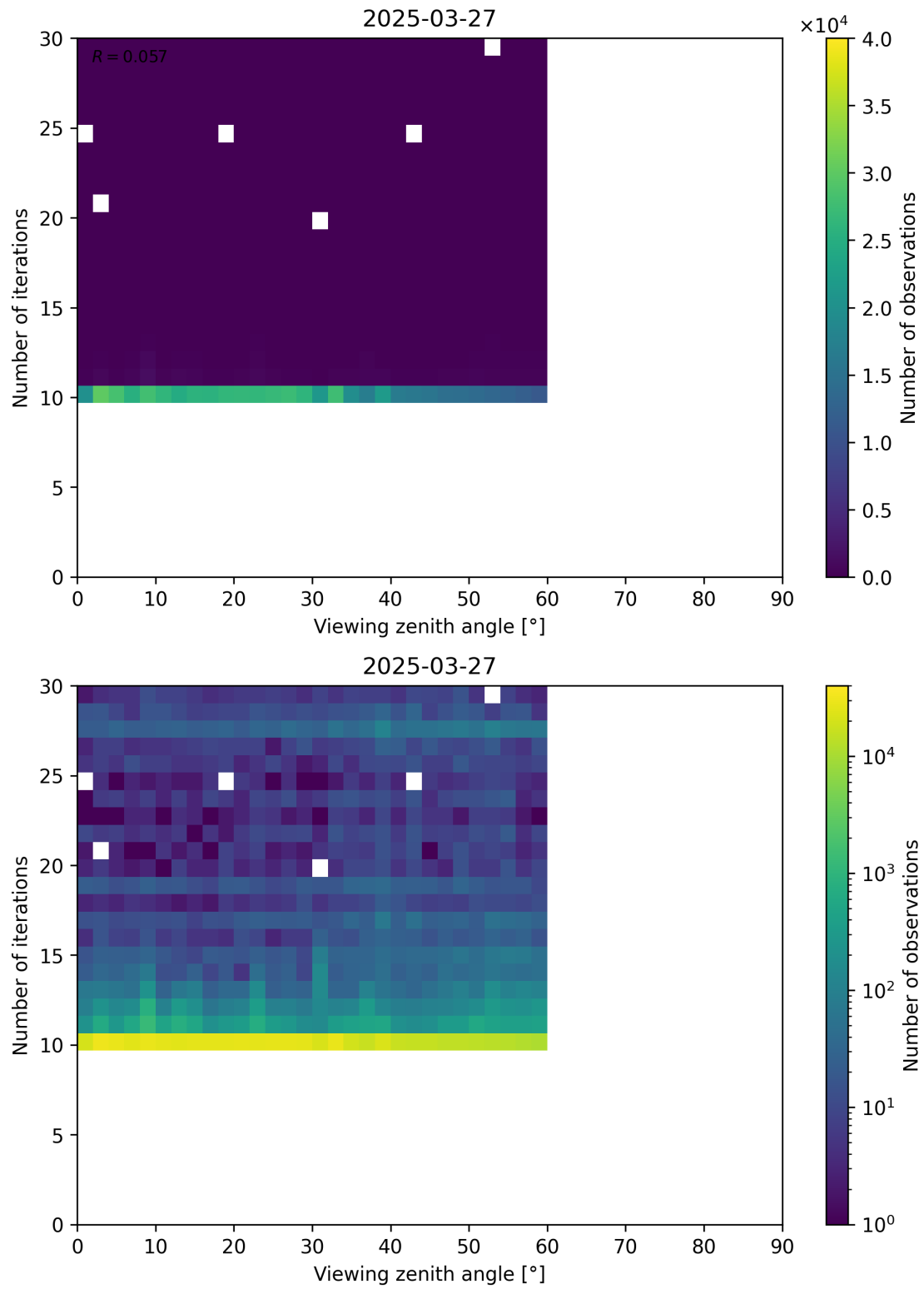
Figure 113: Scatter density plot of “Viewing zenith angle” against “Number of iterations” for 2025-03-26 to 2025-03-28.
