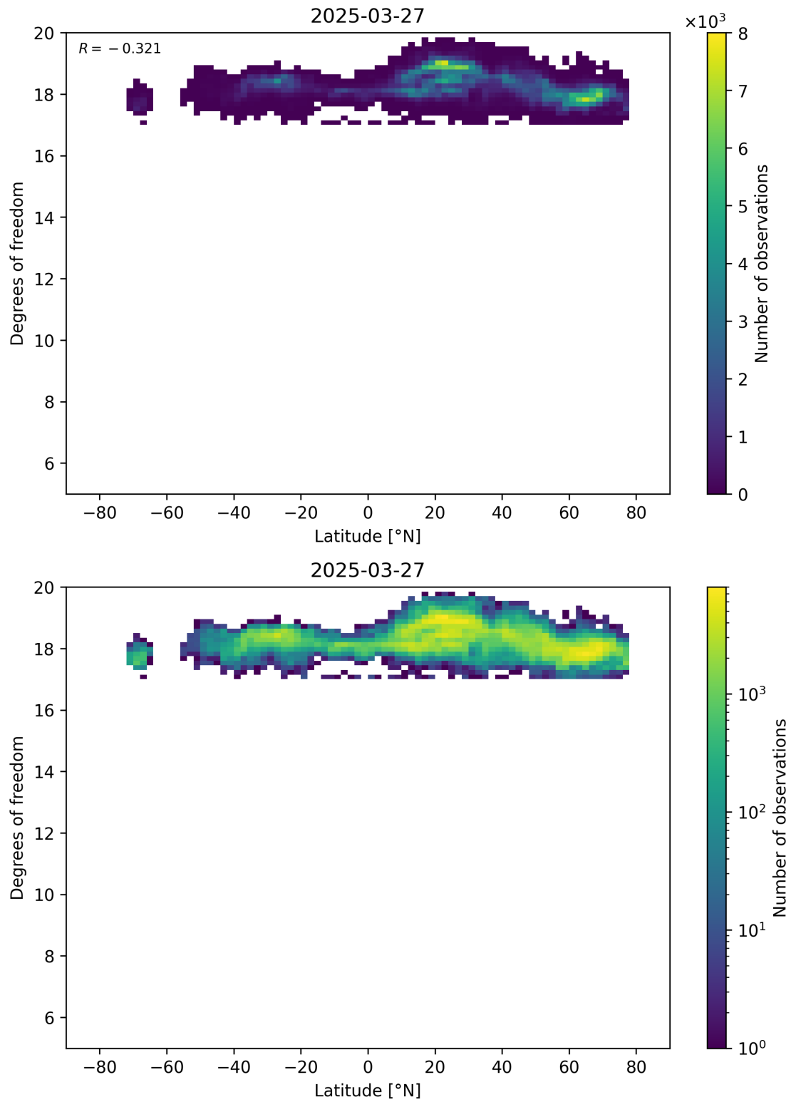
Figure 55: Scatter density plot of “Latitude” against “Degrees of freedom” for 2025-03-26 to 2025-03-28.
