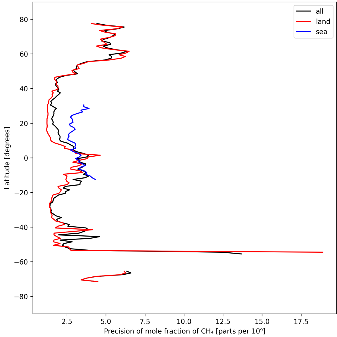
Figure 13: Zonal average of “Precision of mole fraction of CH 4 ” for 2025-03-26 to 2025-03-28.
