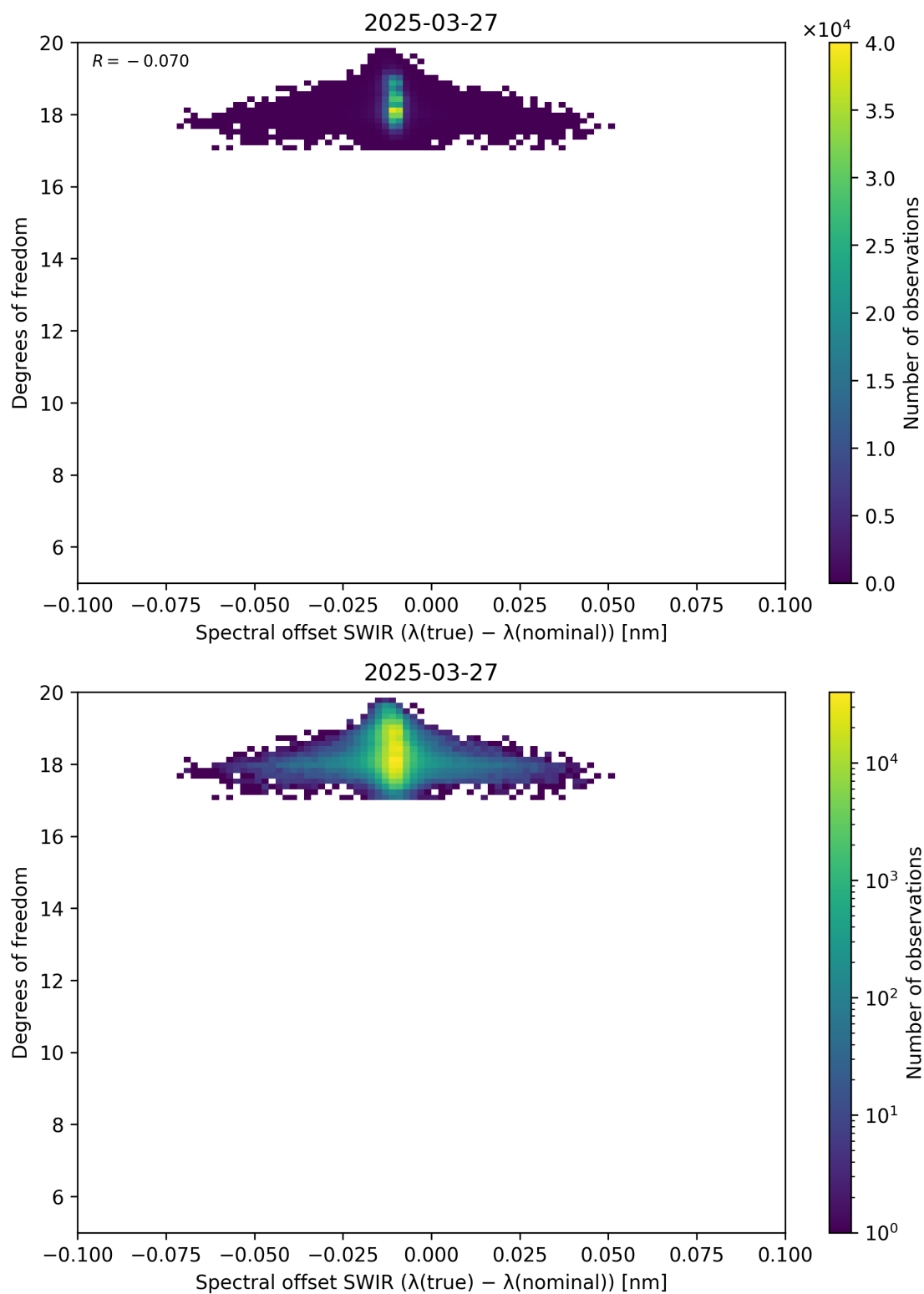
Figure 119: Scatter density plot of “Spectral offset SWIR ( \lambda_{\text{true}} - \lambda_{\text{nominal}} )” against “Degrees of freedom” for 2025-03-26 to 2025-03-28.
