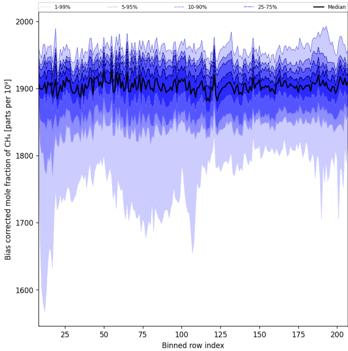
Figure 36: Along track statistics of “Bias corrected mole fraction of CH 4 ” for 2025-03-26 to 2025-03-28
