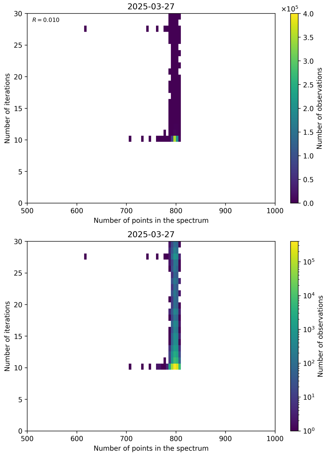
Figure 92: Scatter density plot of “Number of points in the spectrum” against “Number of iterations” for 2025-03-26 to 2025-03-28.
