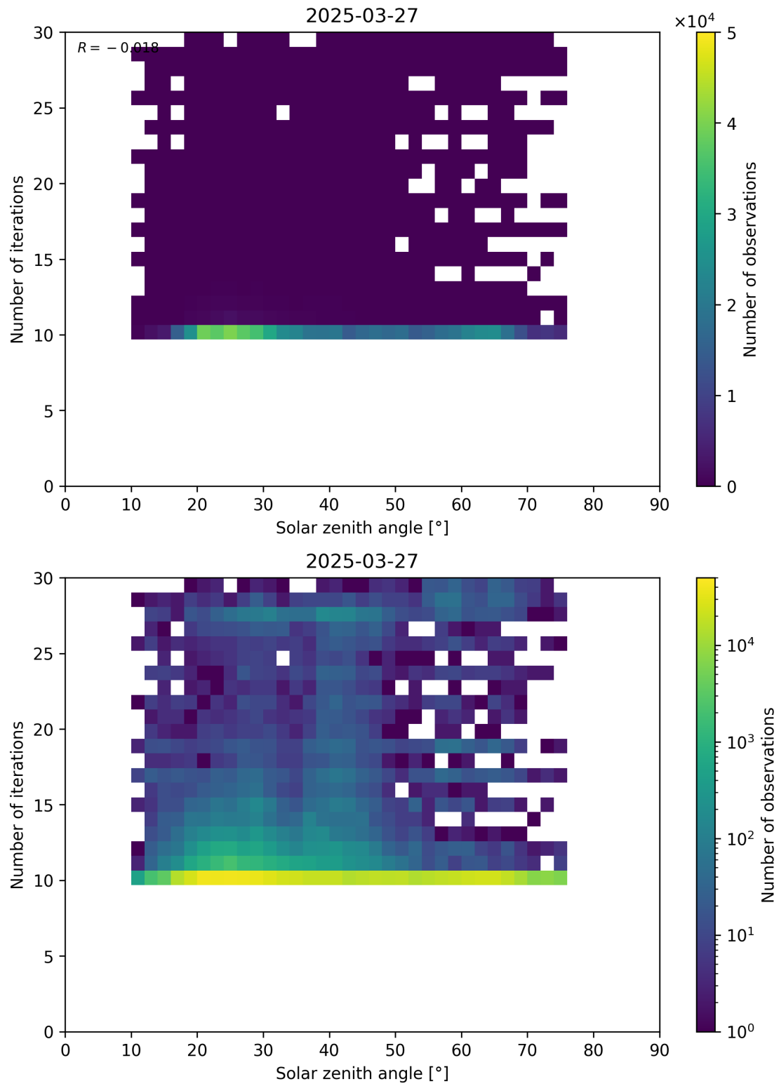
Figure 102: Scatter density plot of “Solar zenith angle” against “Number of iterations” for 2025-03-26 to 2025-03-28.
