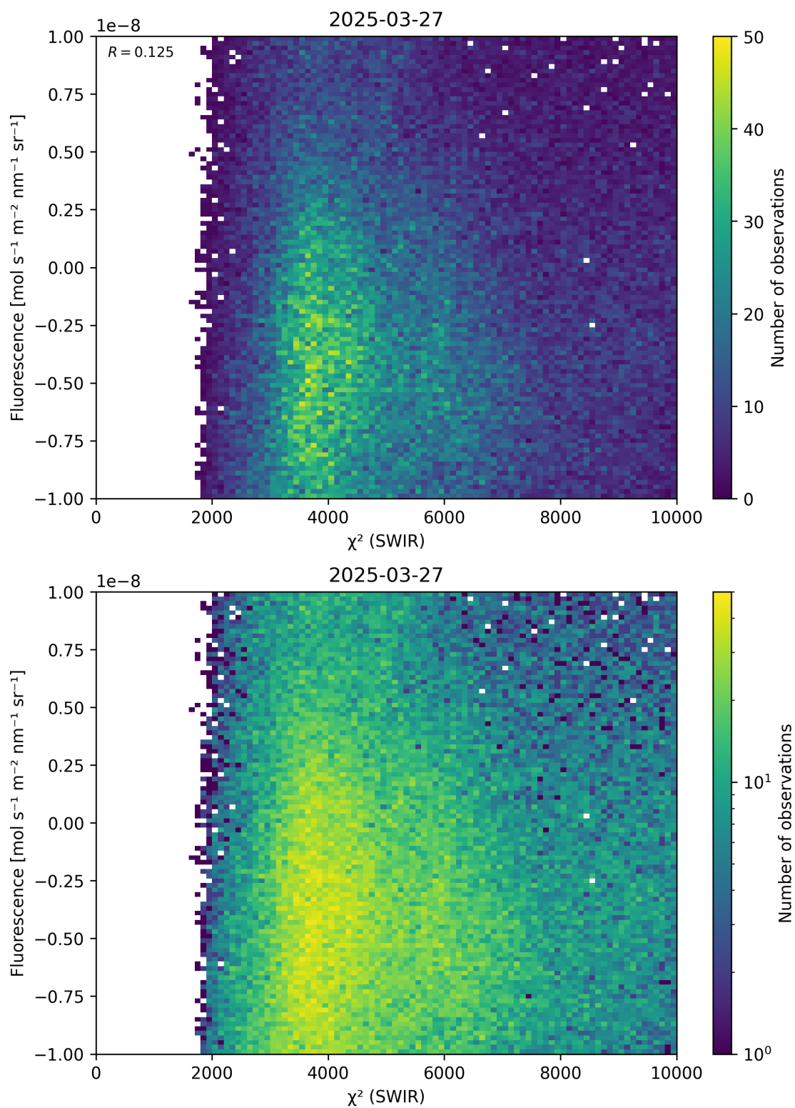
Figure 49: Scatter density plot of “ \chi^2 (SWIR)” against “Fluorescence” for 2025-03-26 to 2025-03-28.
