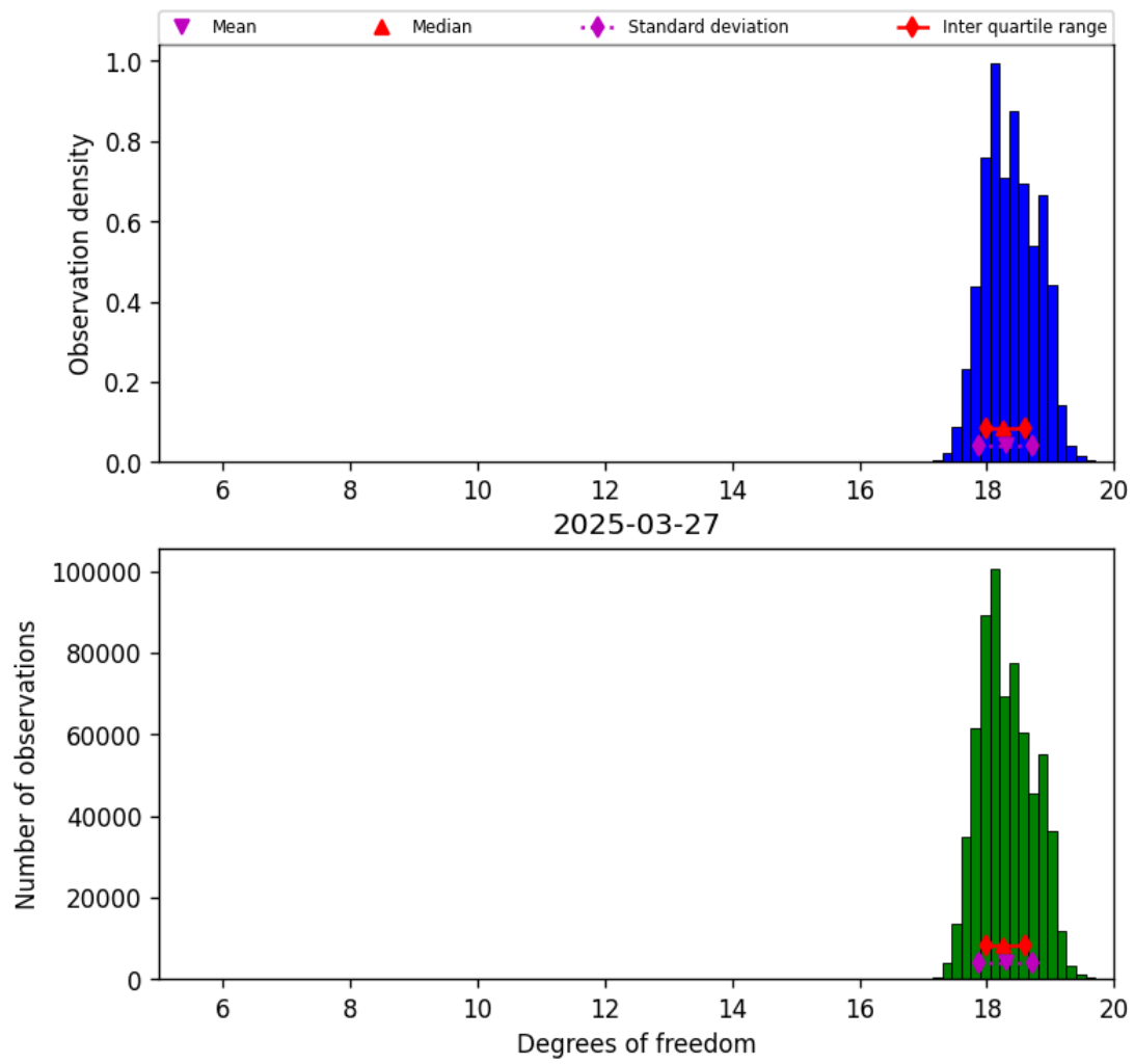
Figure 30: Histogram of “Degrees of freedom” for 2025-03-26 to 2025-03-28
