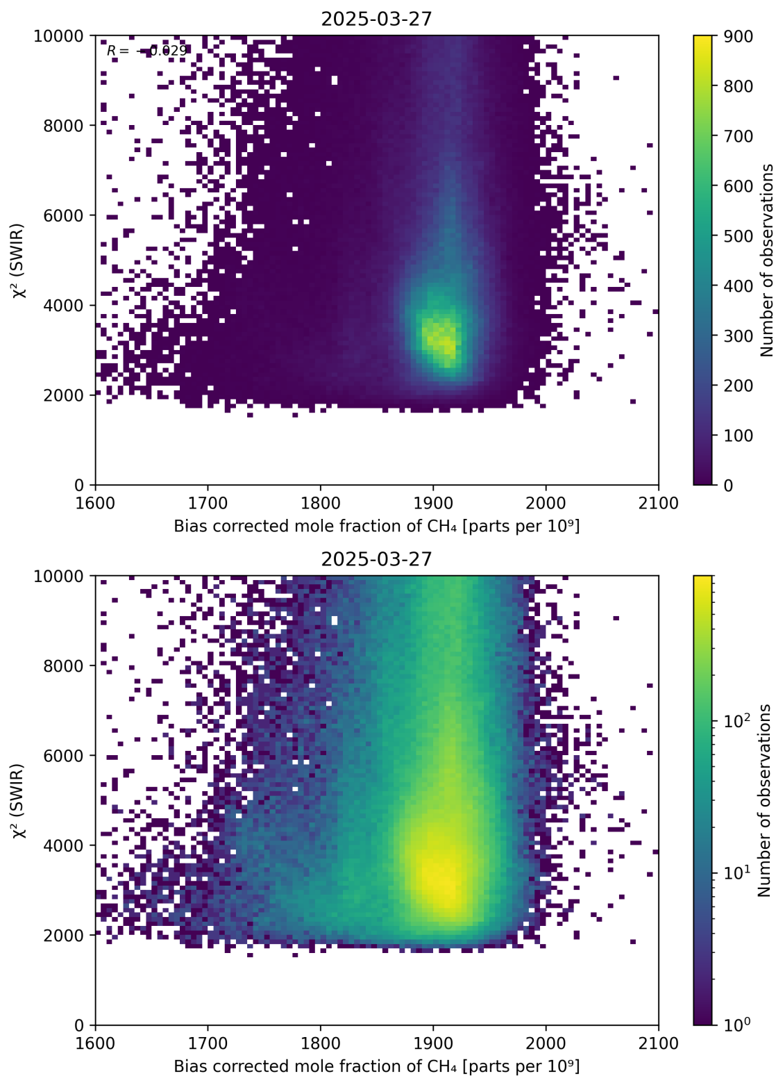
Figure 64: Scatter density plot of “Bias corrected mole fraction of \text{CH}_4 ” against “ \chi^2 (SWIR)” for 2025-03-26 to 2025-03-28.
