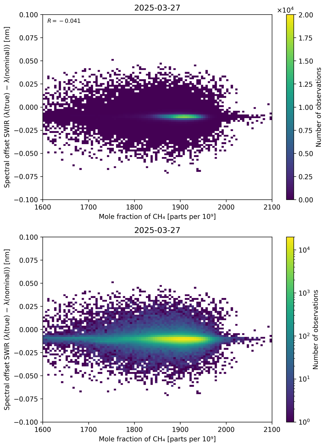
Figure 86: Scatter density plot of “Mole fraction of \text{CH}_4 ” against “Spectral offset SWIR ( \lambda_{\text{true}} - \lambda_{\text{nominal}} )” for 2025-03-26 to 2025-03-28.
