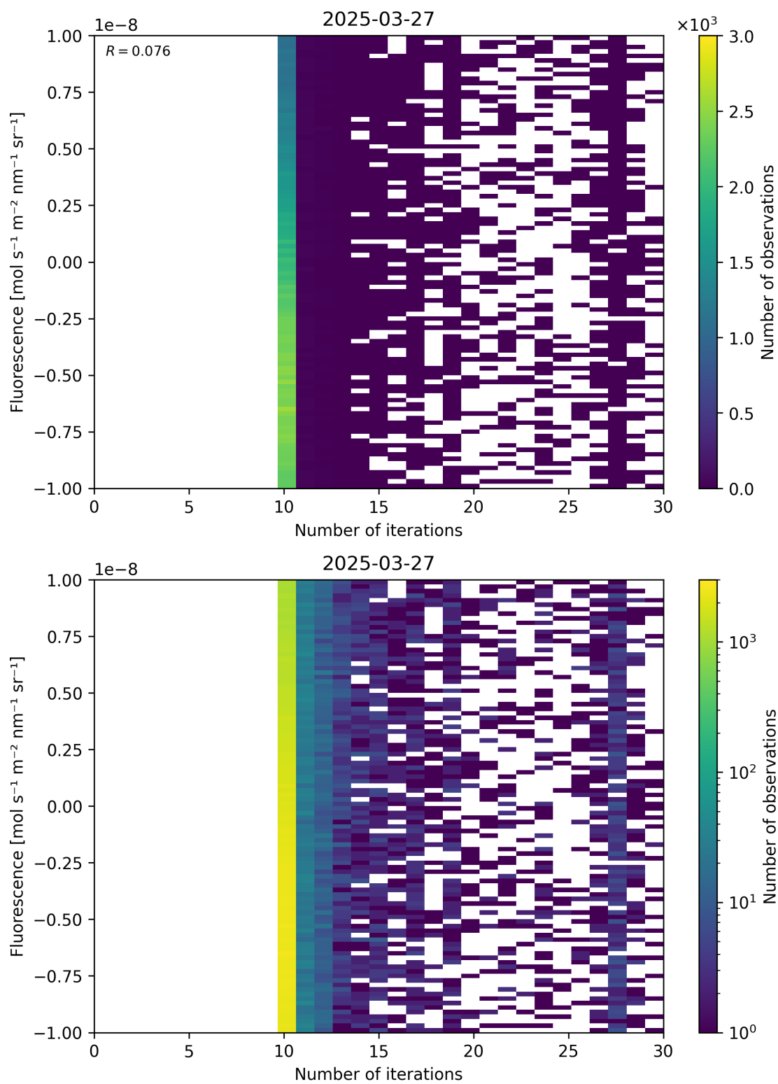
Figure 87: Scatter density plot of “Number of iterations” against “Fluorescence” for 2025-03-26 to 2025-03-28.
