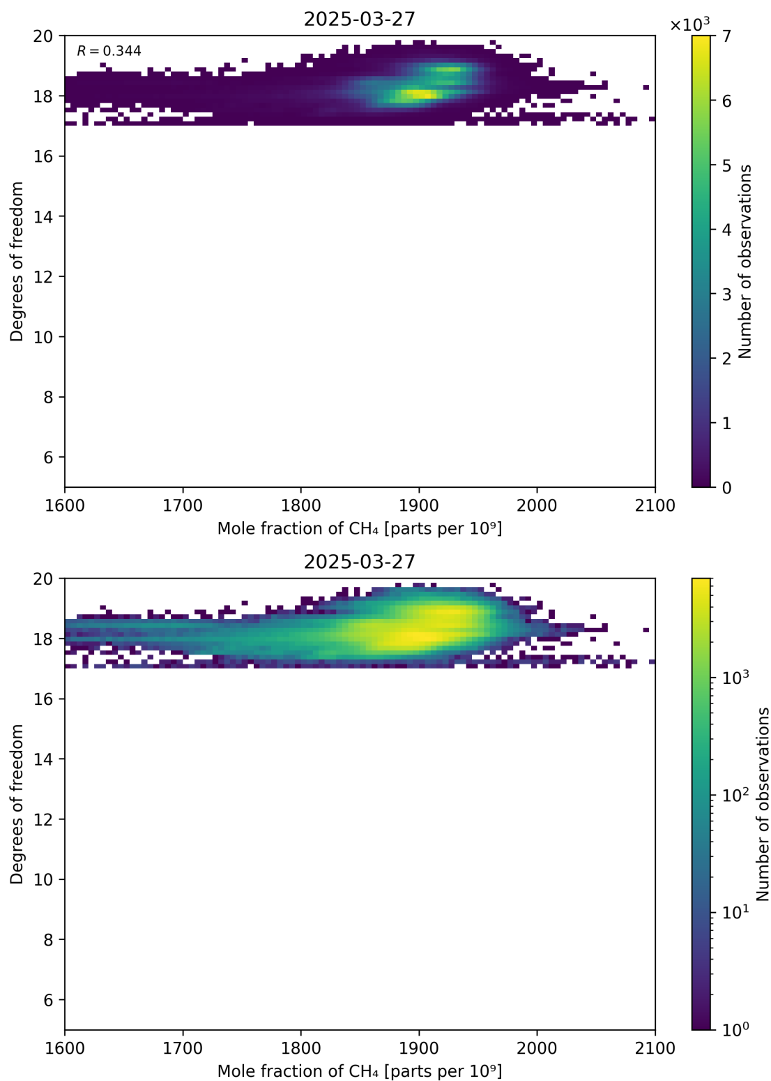
Figure 72: Scatter density plot of “Mole fraction of CH 4 ” against “Degrees of freedom” for 2025-03-26 to 2025-03-28.
