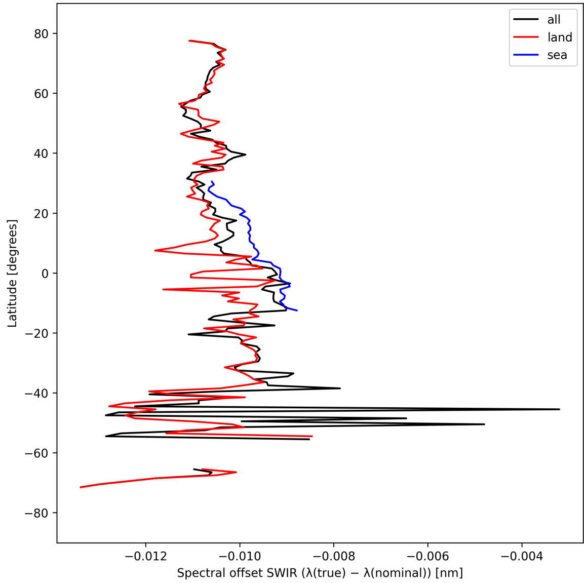
Figure 16: Zonal average of “Spectral offset SWIR ( \lambda_{\text{true}} - \lambda_{\text{nominal}} )” for 2025-03-26 to 2025-03-28.
