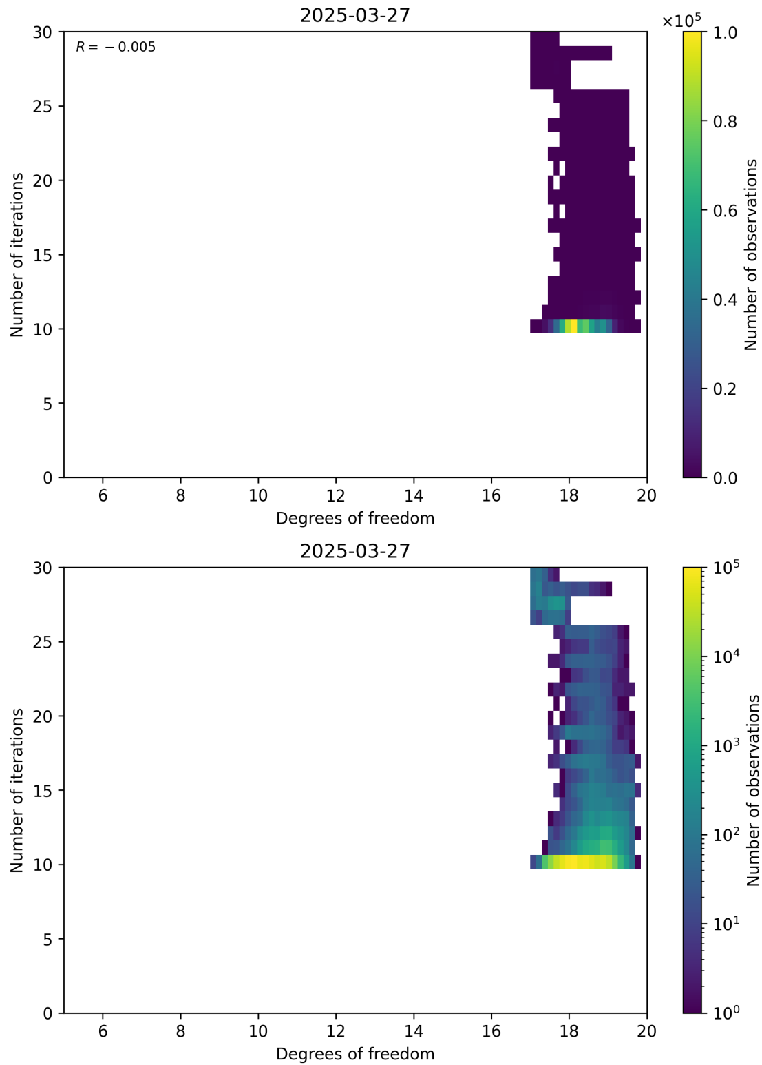
Figure 52: Scatter density plot of “Degrees of freedom” against “Number of iterations” for 2025-03-26 to 2025-03-28.
