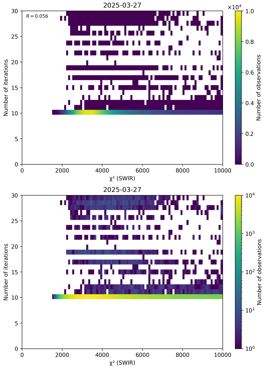
Figure 50: Scatter density plot of “ \chi^2 (SWIR)” against “Number of iterations” for 2025-03-26 to 2025-03-28.
