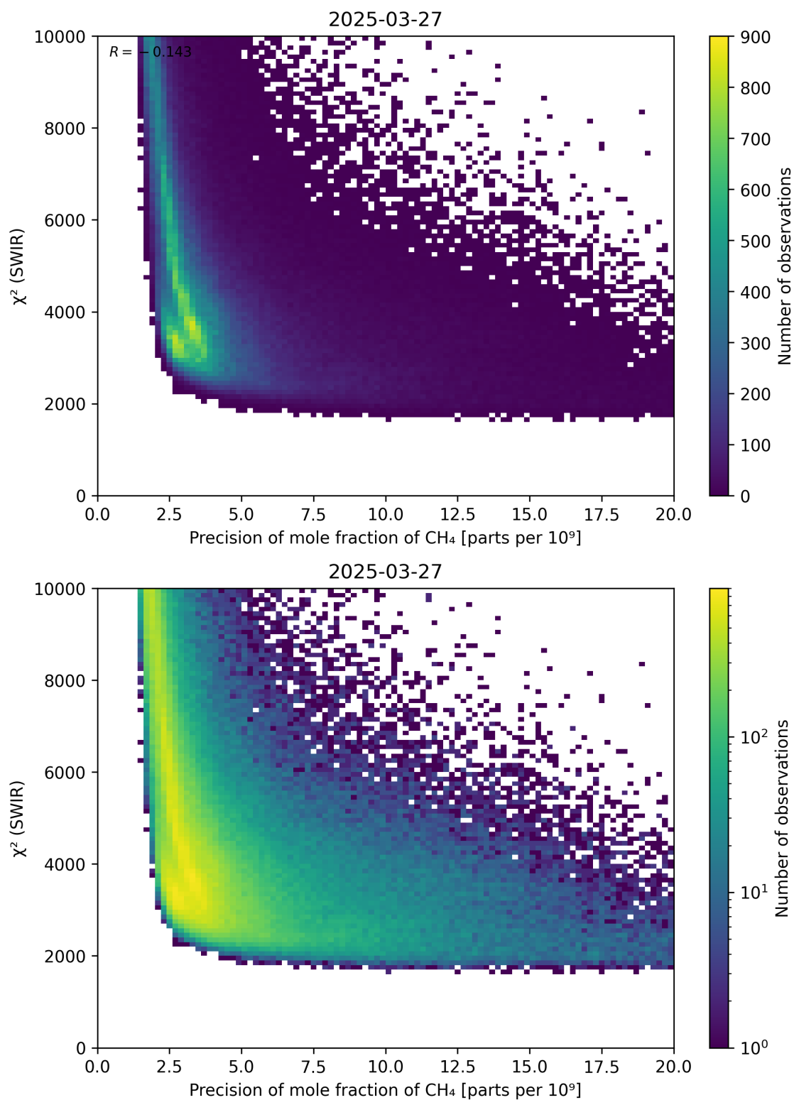
Figure 79: Scatter density plot of “Precision of mole fraction of \text{CH}_4 ” against “ \chi^2 (SWIR)” for 2025-03-26 to 2025-03-28.
