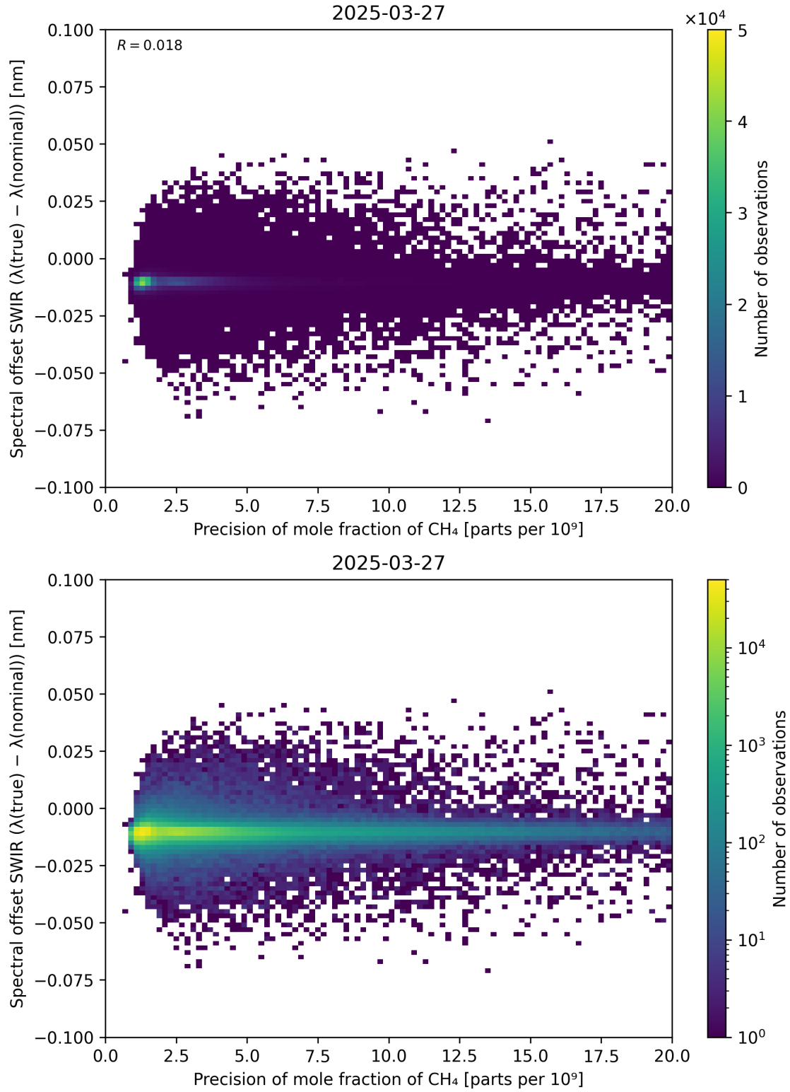
Figure 85: Scatter density plot of “Precision of mole fraction of \text{CH}_4 ” against “Spectral offset SWIR ( \lambda_{\text{true}} - \lambda_{\text{nominal}} )” for 2025-03-26 to 2025-03-28.
