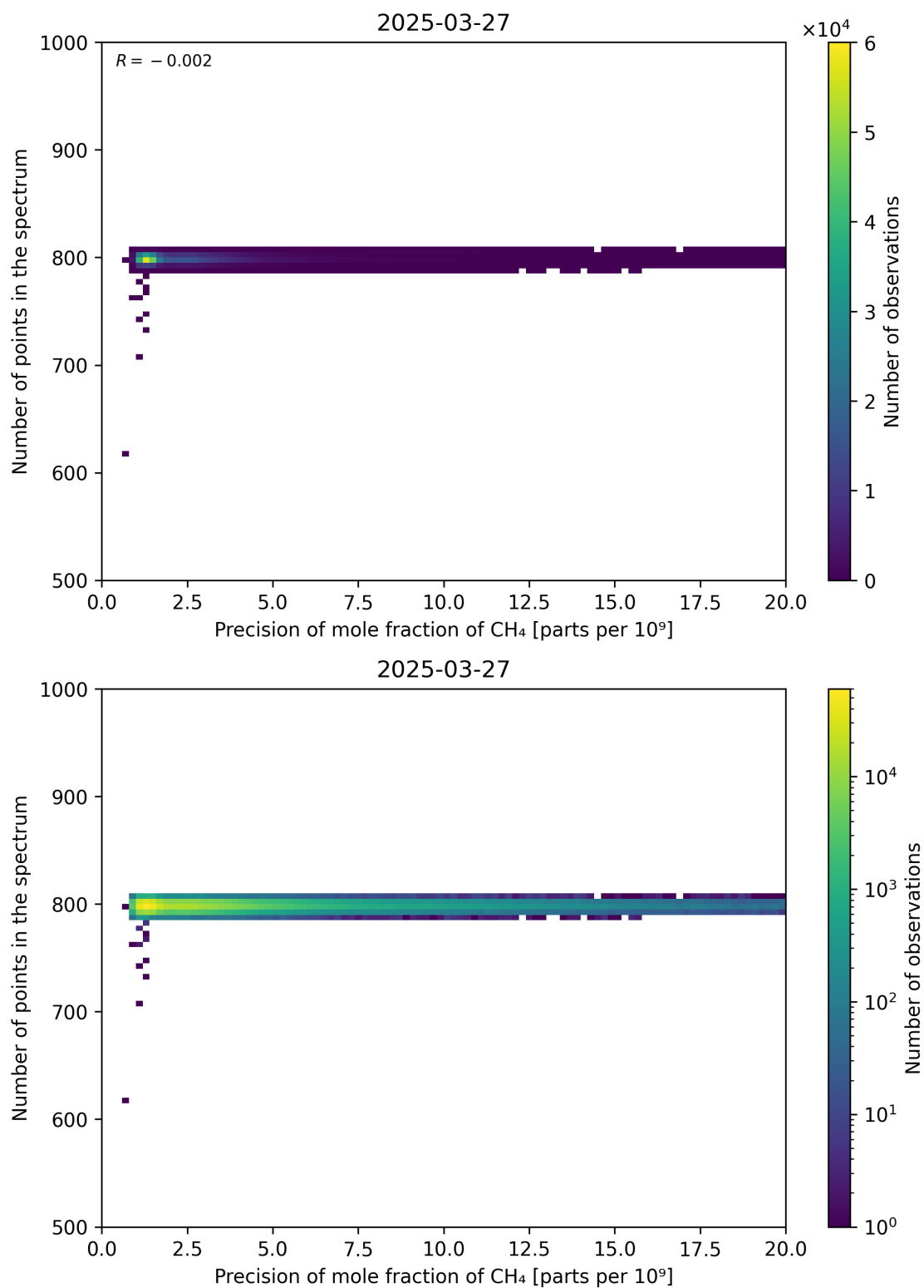
Figure 84: Scatter density plot of “Precision of mole fraction of CH 4 ” against “Number of points in the spectrum” for 2025-03-26 to 2025-03-28.
