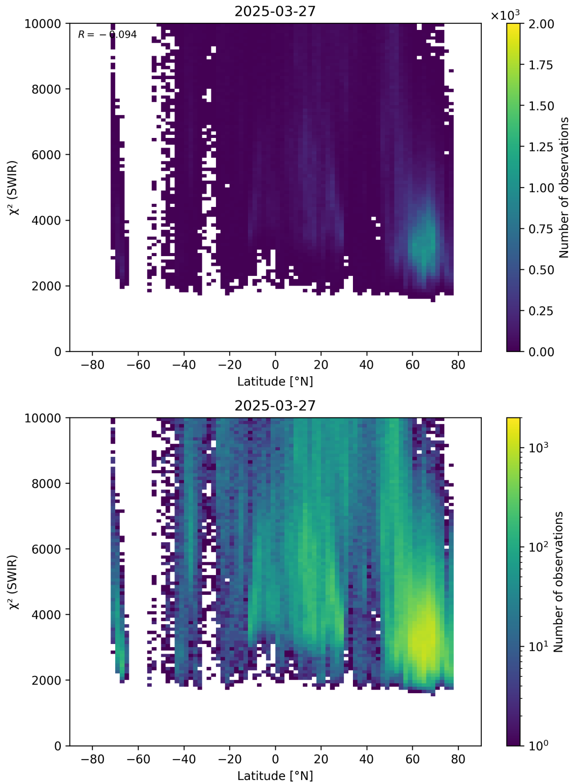
Figure 54: Scatter density plot of “Latitude” against “ \chi^2 (SWIR)” for 2025-03-26 to 2025-03-28.
