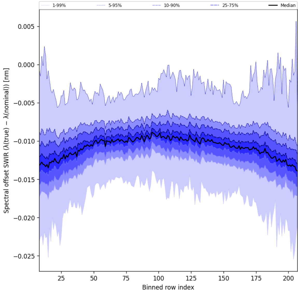
Figure 38: Along track statistics of “Spectral offset SWIR ( \lambda_{\text{true}} - \lambda_{\text{nominal}} )” for 2025-03-26 to 2025-03-28
