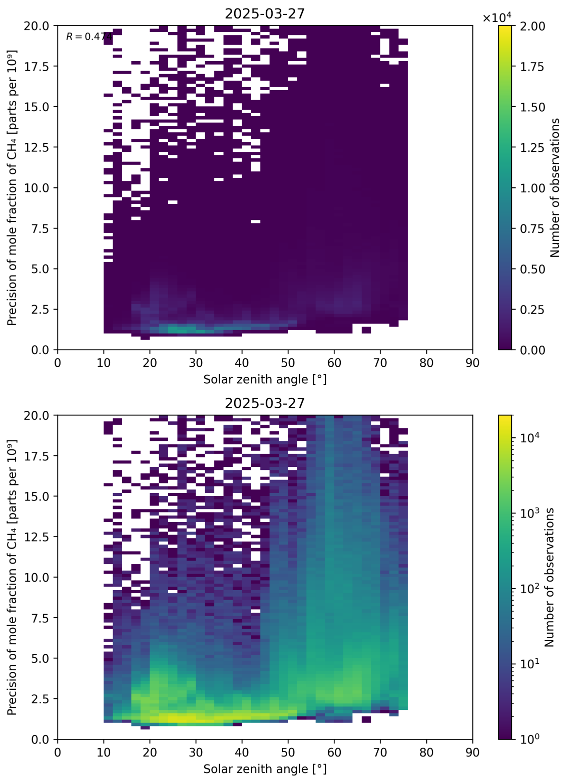
Figure 101: Scatter density plot of “Solar zenith angle” against “Precision of mole fraction of CH 4 ” for 2025-03-26 to 2025-03-28.
