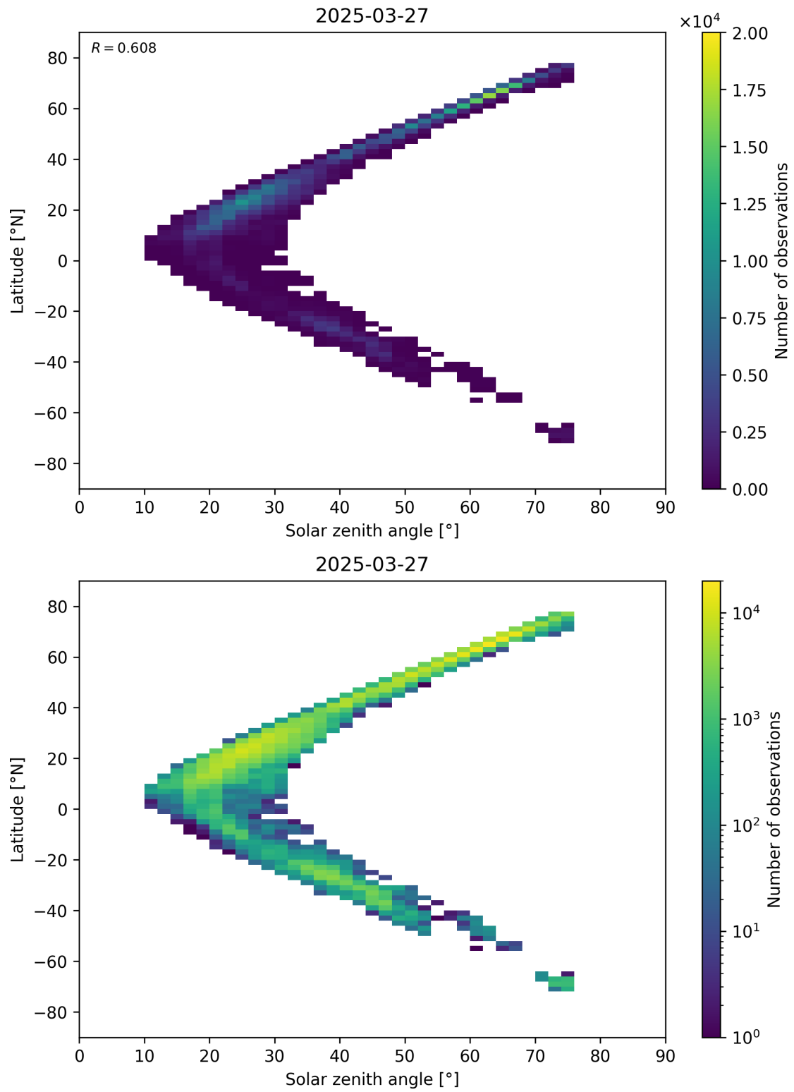
Figure 98: Scatter density plot of “Solar zenith angle” against “Latitude” for 2025-03-26 to 2025-03-28.
