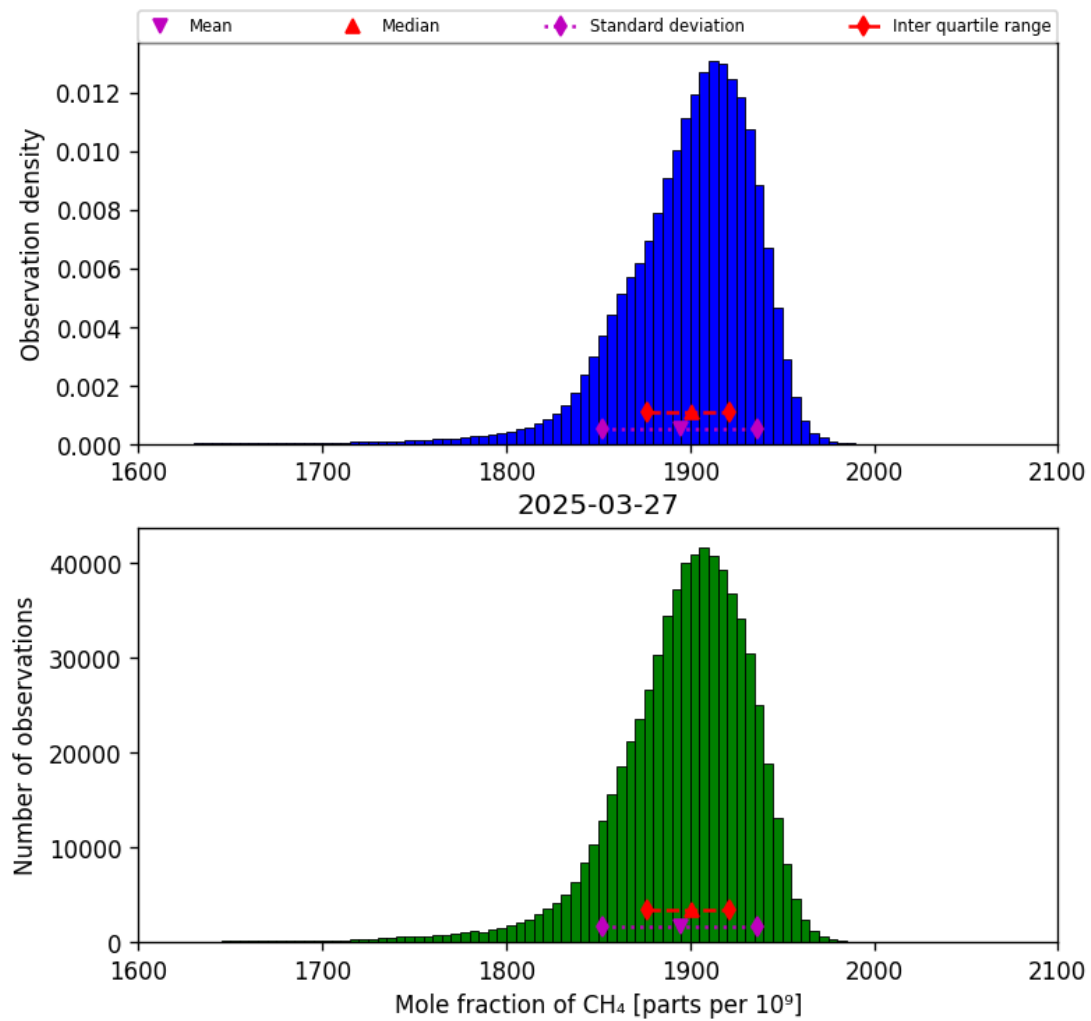
Figure 23: Histogram of “Mole fraction of CH 4 ” for 2025-03-26 to 2025-03-28
