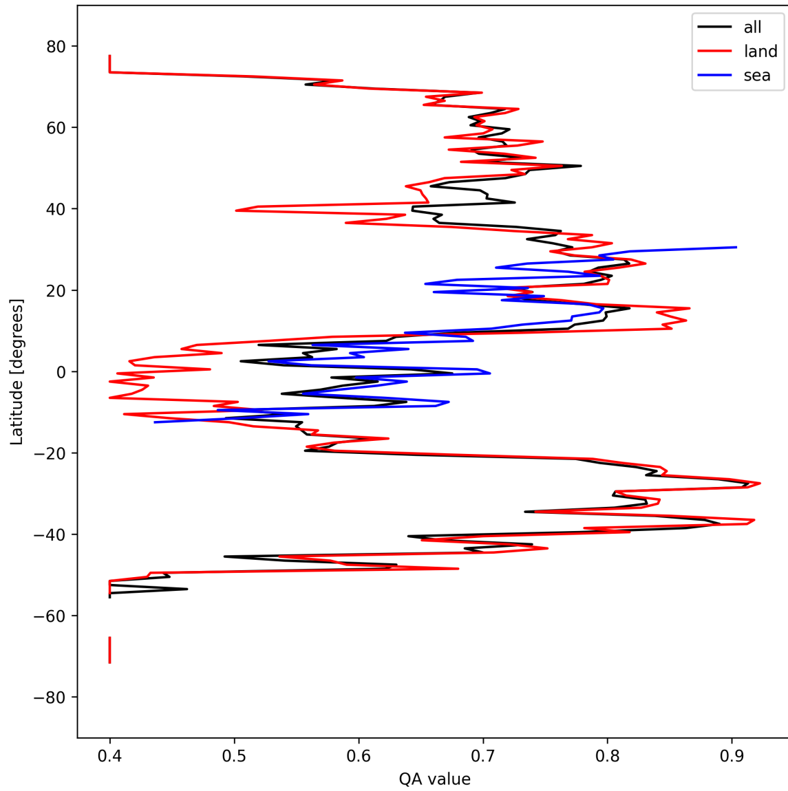
Figure 11: Zonal average of “QA value” for 2025-03-26 to 2025-03-28.
