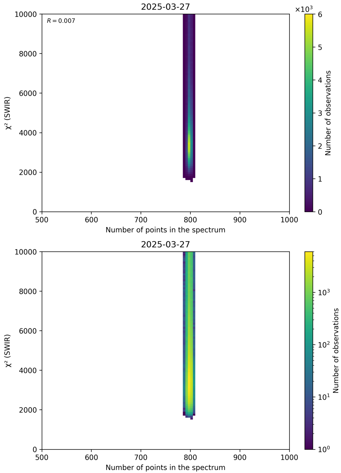
Figure 89: Scatter density plot of “Number of points in the spectrum” against “ \chi^2 (SWIR)” for 2025-03-26 to 2025-03-28.
