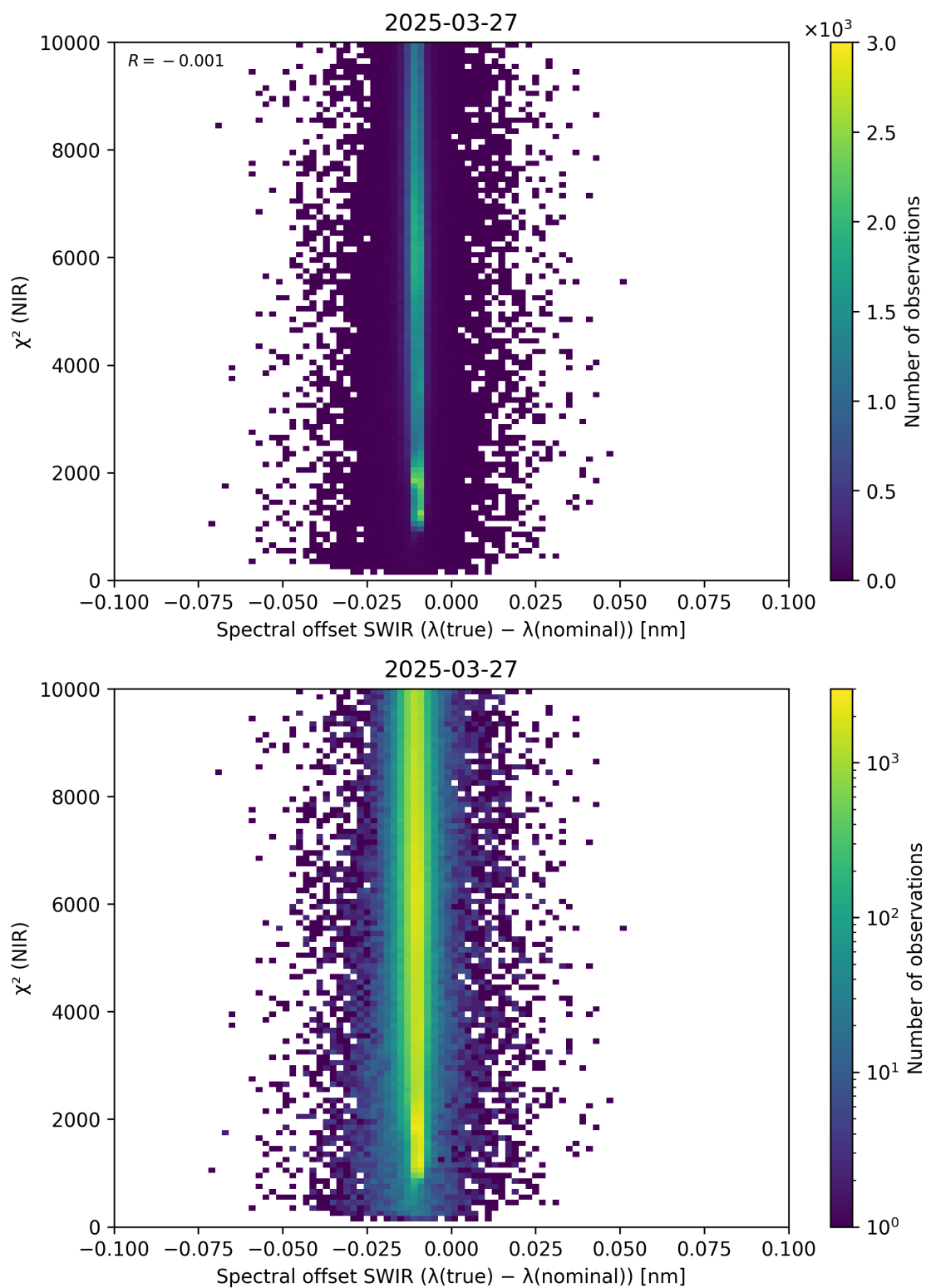
Figure 117: Scatter density plot of “Spectral offset SWIR ( \lambda_{\text{true}} - \lambda_{\text{nominal}} )” against “ \chi^2 (NIR)” for 2025-03-26 to 2025-03-28.
