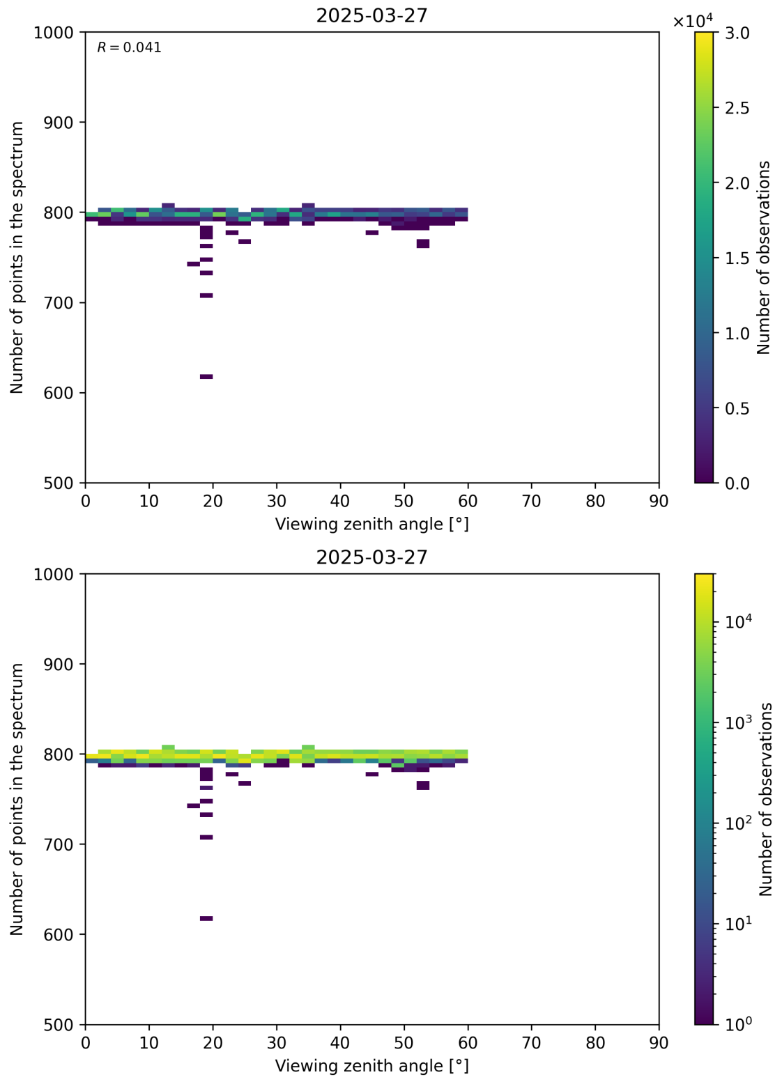
Figure 114: Scatter density plot of “Viewing zenith angle” against “Number of points in the spectrum” for 2025-03-26 to 2025-03-28.
