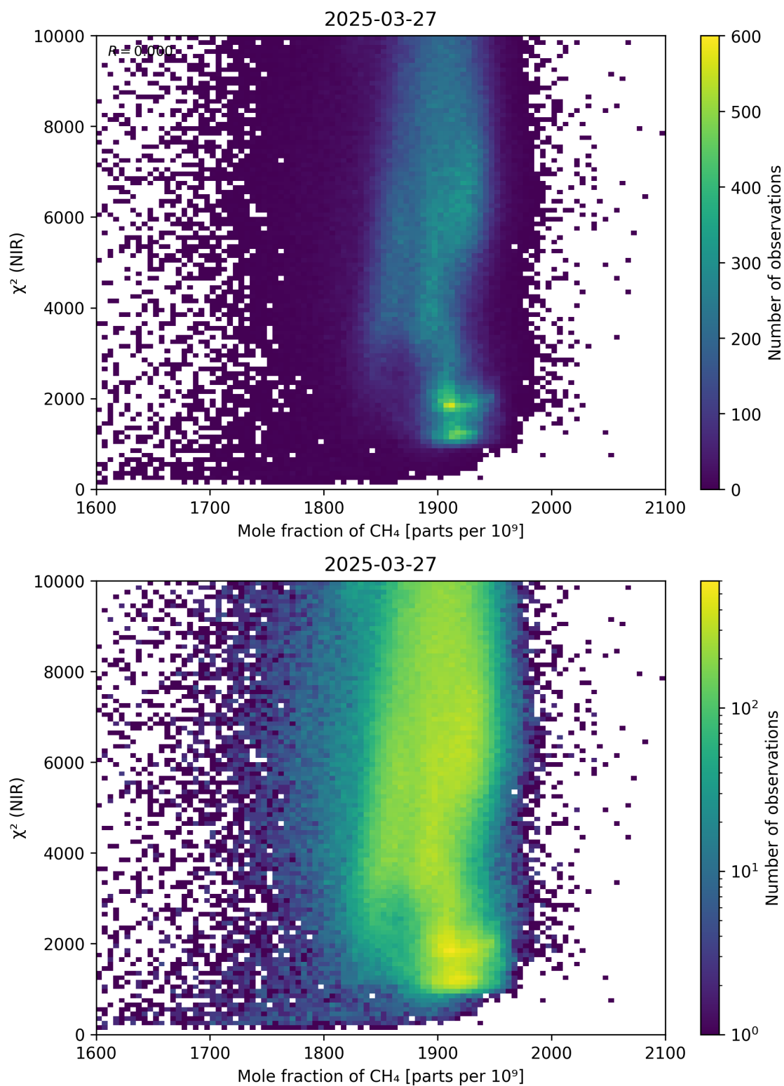
Figure 70: Scatter density plot of “Mole fraction of \text{CH}_4 ” against “ \chi^2 (NIR)” for 2025-03-26 to 2025-03-28.
