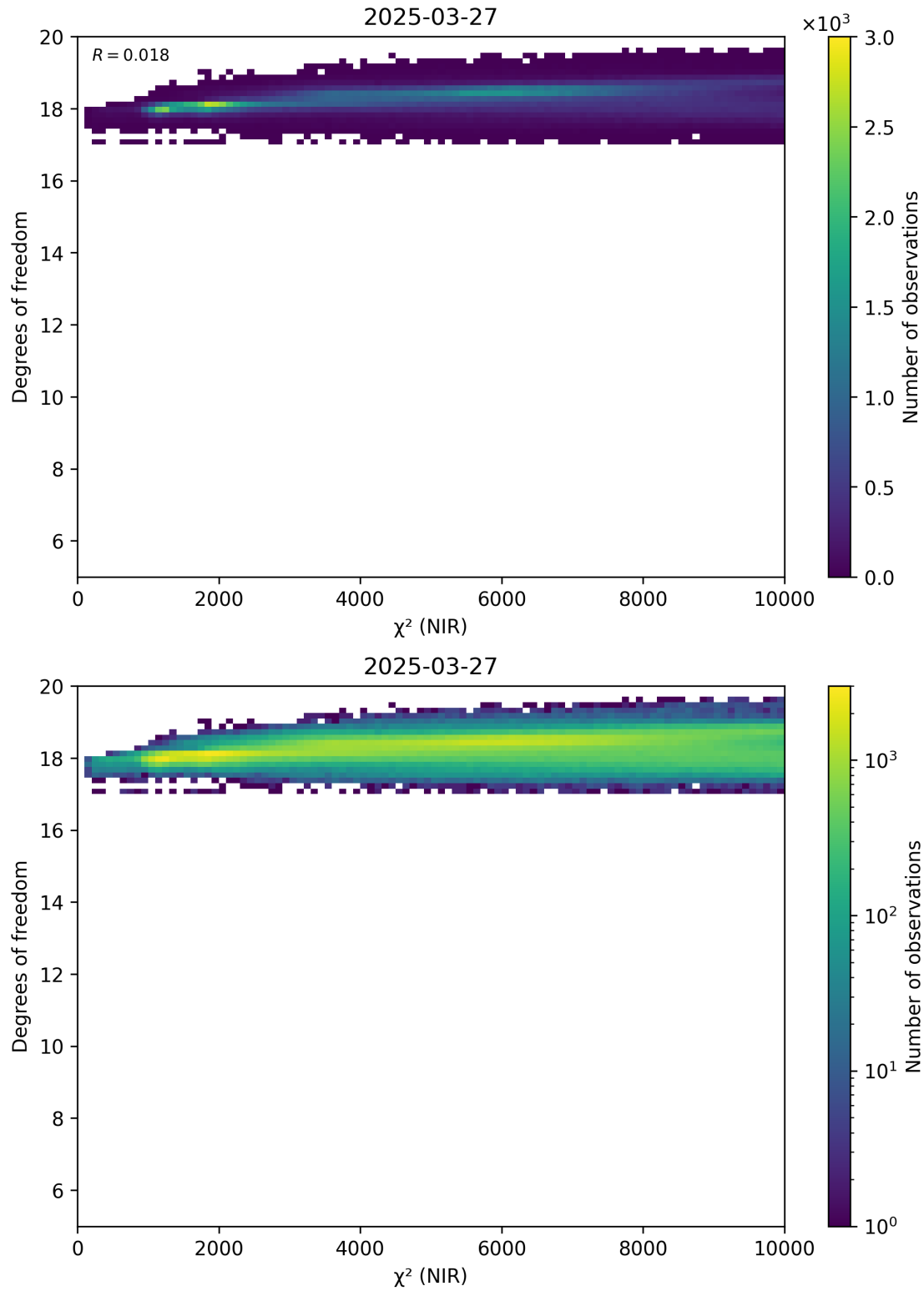
Figure 44: Scatter density plot of “ \chi^2 (NIR)” against “Degrees of freedom” for 2025-03-26 to 2025-03-28.
