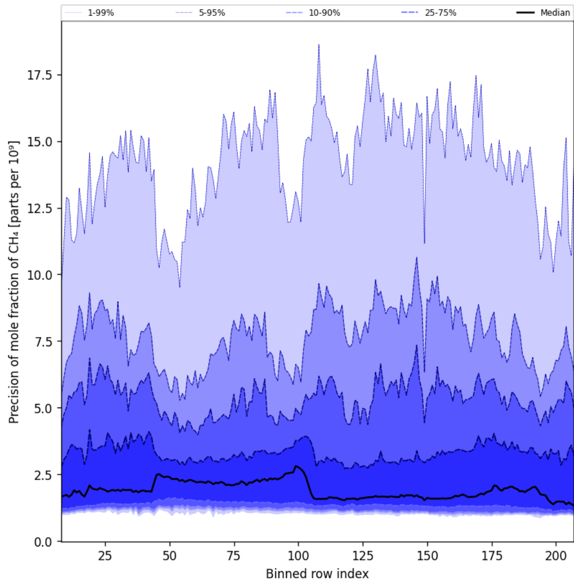
Figure 35: Along track statistics of “Precision of mole fraction of CH 4 ” for 2025-03-26 to 2025-03-28
