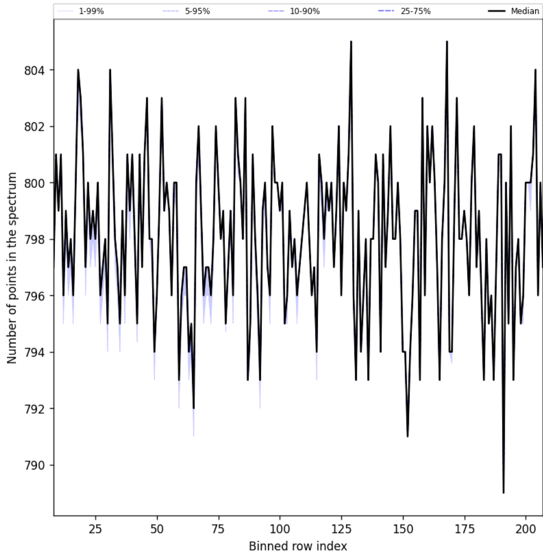
Figure 37: Along track statistics of “Number of points in the spectrum” for 2025-03-26 to 2025-03-28
