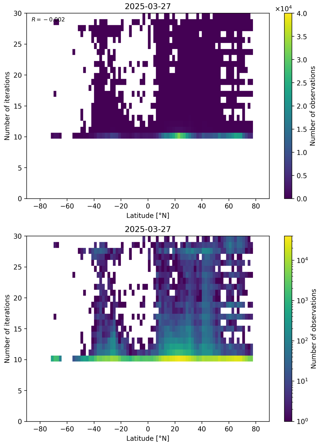
Figure 60: Scatter density plot of “Latitude” against “Number of iterations” for 2025-03-26 to 2025-03-28.
