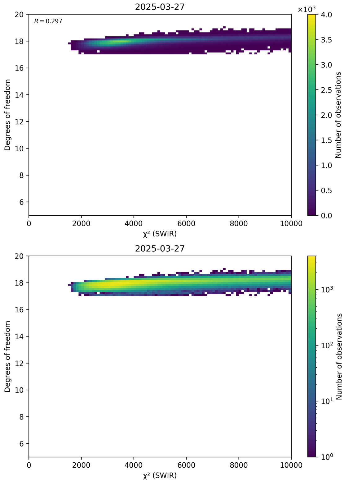
Figure 48: Scatter density plot of “ \chi^2 (SWIR)” against “Degrees of freedom” for 2025-03-26 to 2025-03-28.
