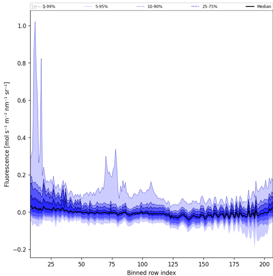
Figure 43: Along track statistics of “Fluorescence” for 2025-03-26 to 2025-03-28
