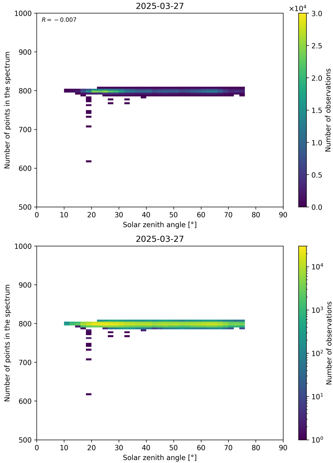
Figure 103: Scatter density plot of “Solar zenith angle” against “Number of points in the spectrum” for 2025-03-26 to 2025-03-28.
