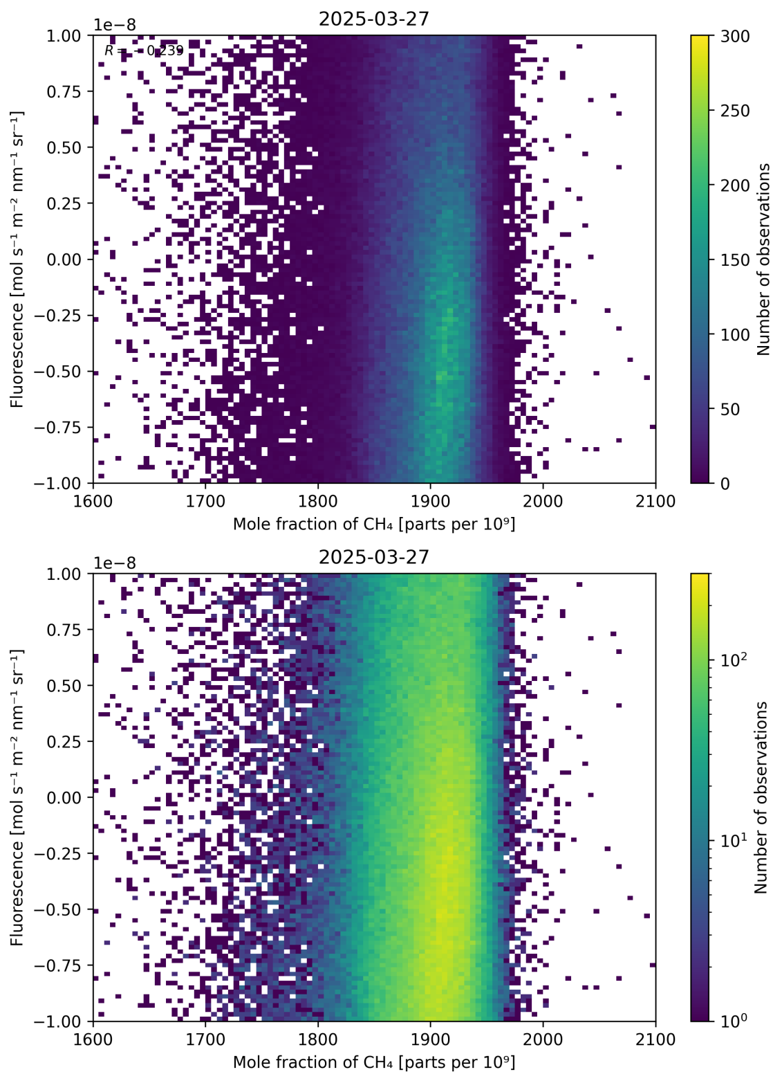
Figure 73: Scatter density plot of “Mole fraction of \text{CH}_4 ” against “Fluorescence” for 2025-03-26 to 2025-03-28.
