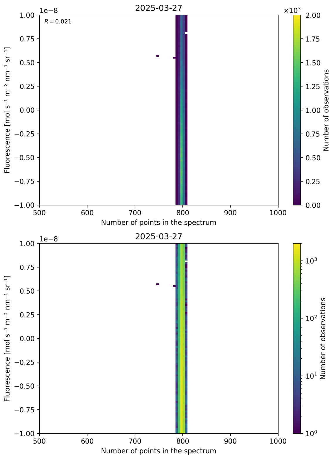
Figure 91: Scatter density plot of “Number of points in the spectrum” against “Fluorescence” for 2025-03-26 to 2025-03-28.
