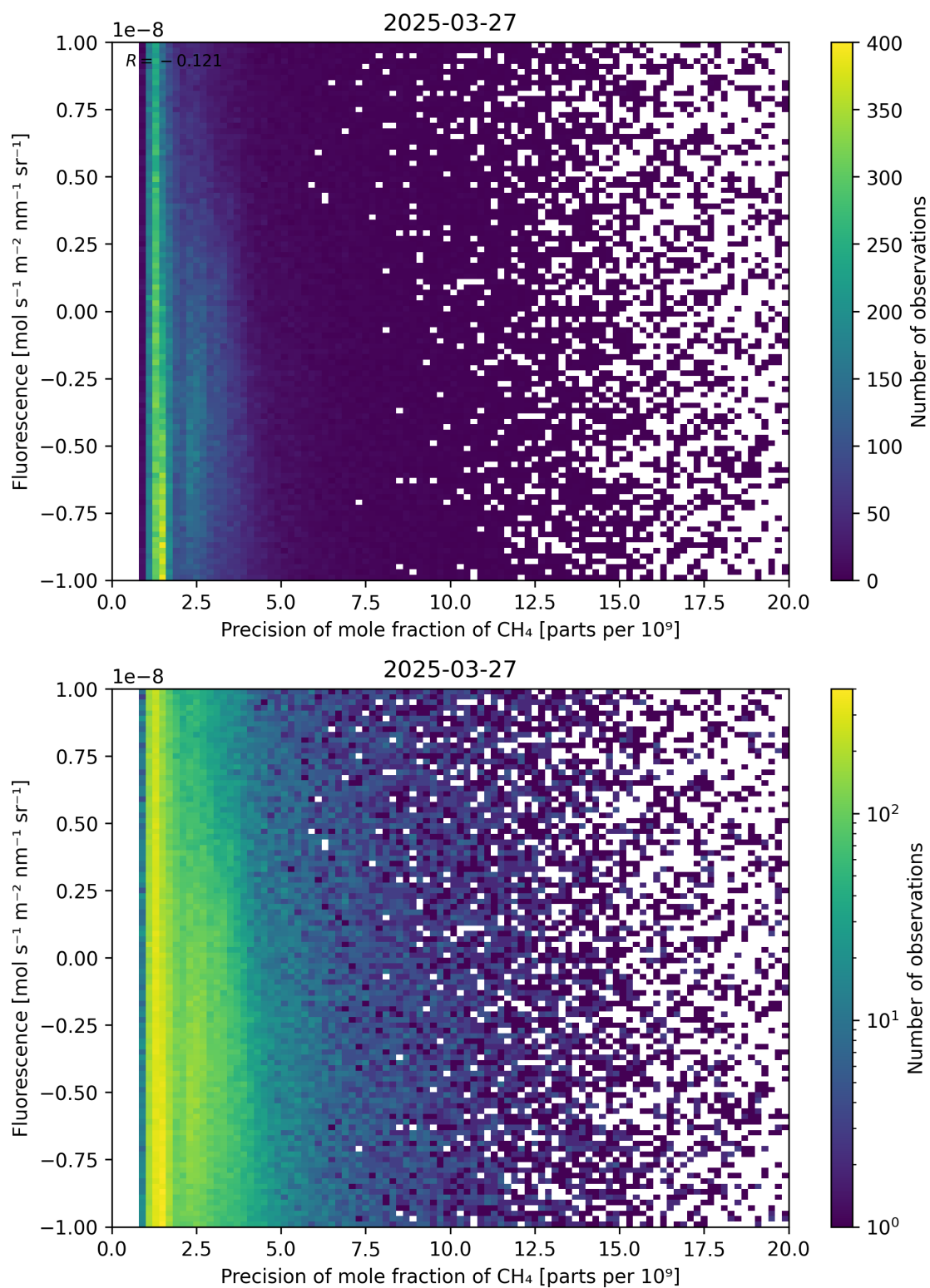
Figure 81: Scatter density plot of “Precision of mole fraction of CH 4 ” against “Fluorescence” for 2025-03-26 to 2025-03-28.
