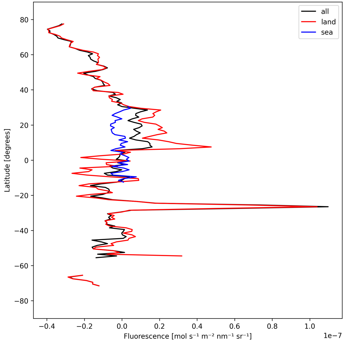
Figure 21: Zonal average of “Fluorescence” for 2025-03-26 to 2025-03-28.
