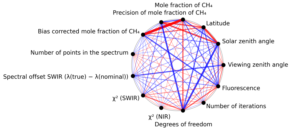
Figure 1: Map of correlation graph for 2025-03-26 to 2025-03-28.
