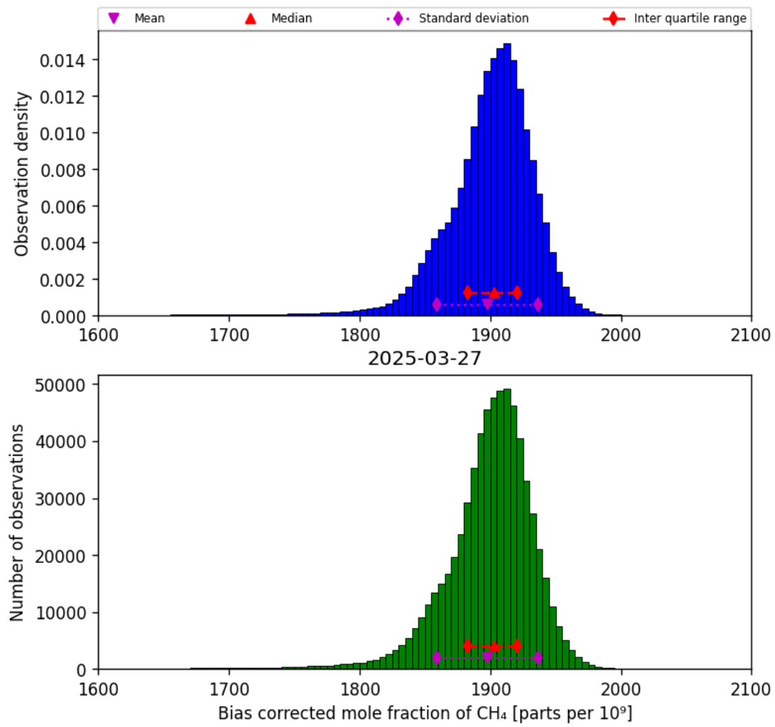
Figure 25: Histogram of “Bias corrected mole fraction of CH 4 ” for 2025-03-26 to 2025-03-28
