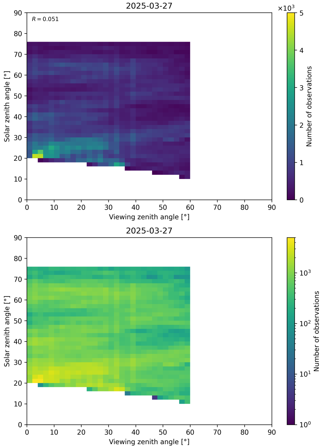
Figure 115: Scatter density plot of “Viewing zenith angle” against “Solar zenith angle” for 2025-03-26 to 2025-03-28.
