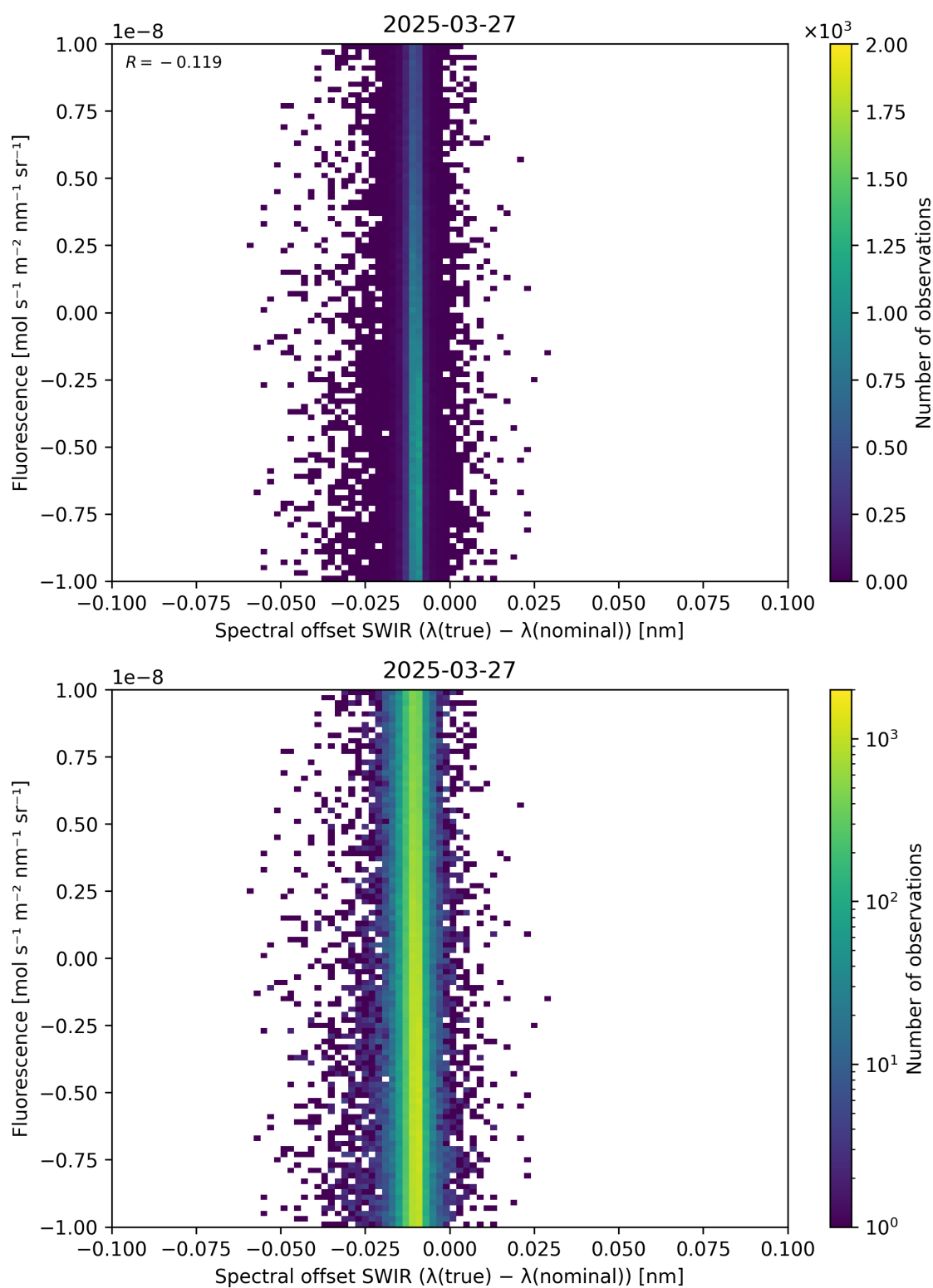
Figure 120: Scatter density plot of “Spectral offset SWIR ( \lambda_{\text{true}} - \lambda_{\text{nominal}} )” against “Fluorescence” for 2025-03-26 to 2025-03-28.
