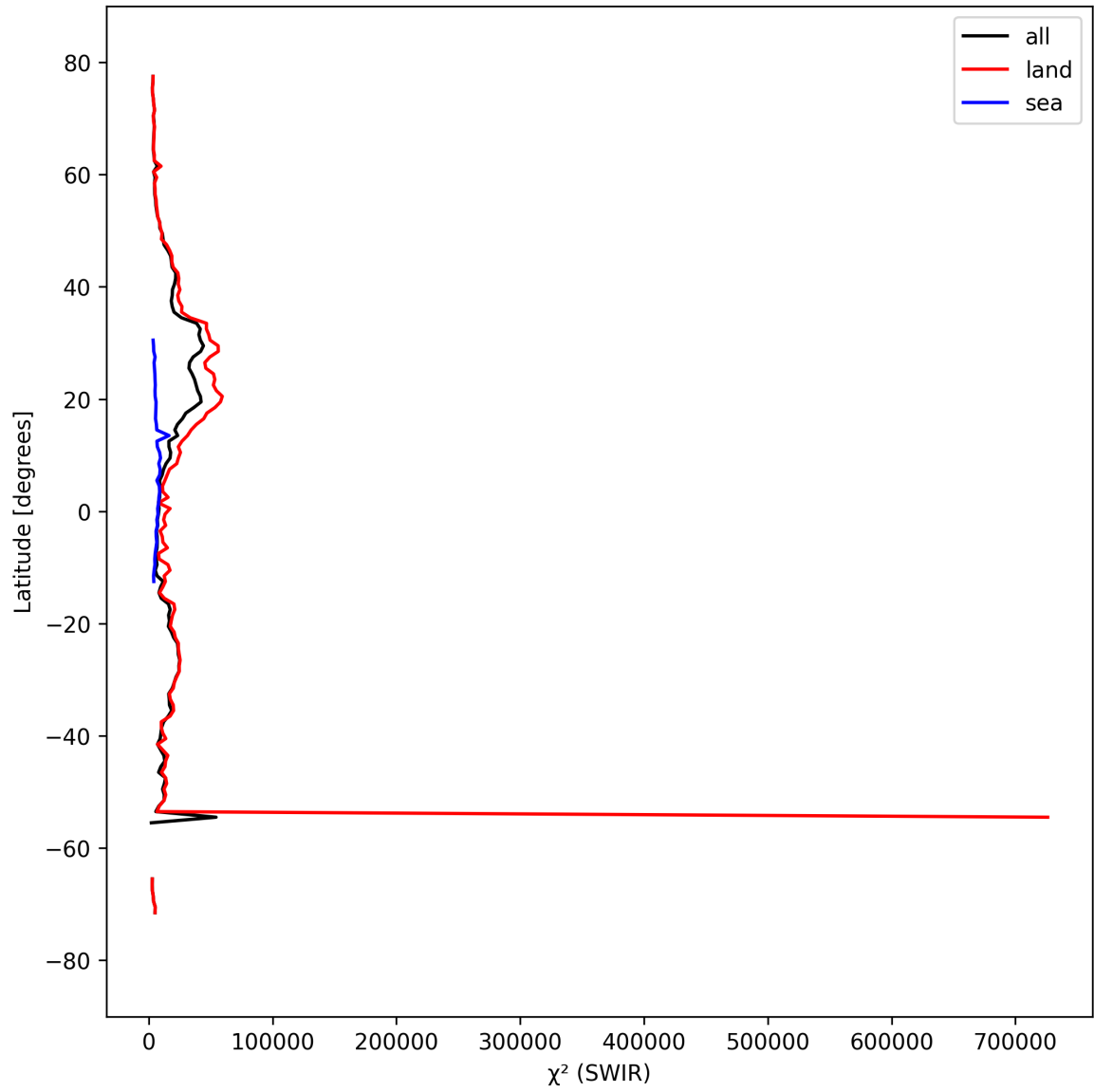
Figure 17: Zonal average of “ \chi^2 (SWIR)” for 2025-03-26 to 2025-03-28.
