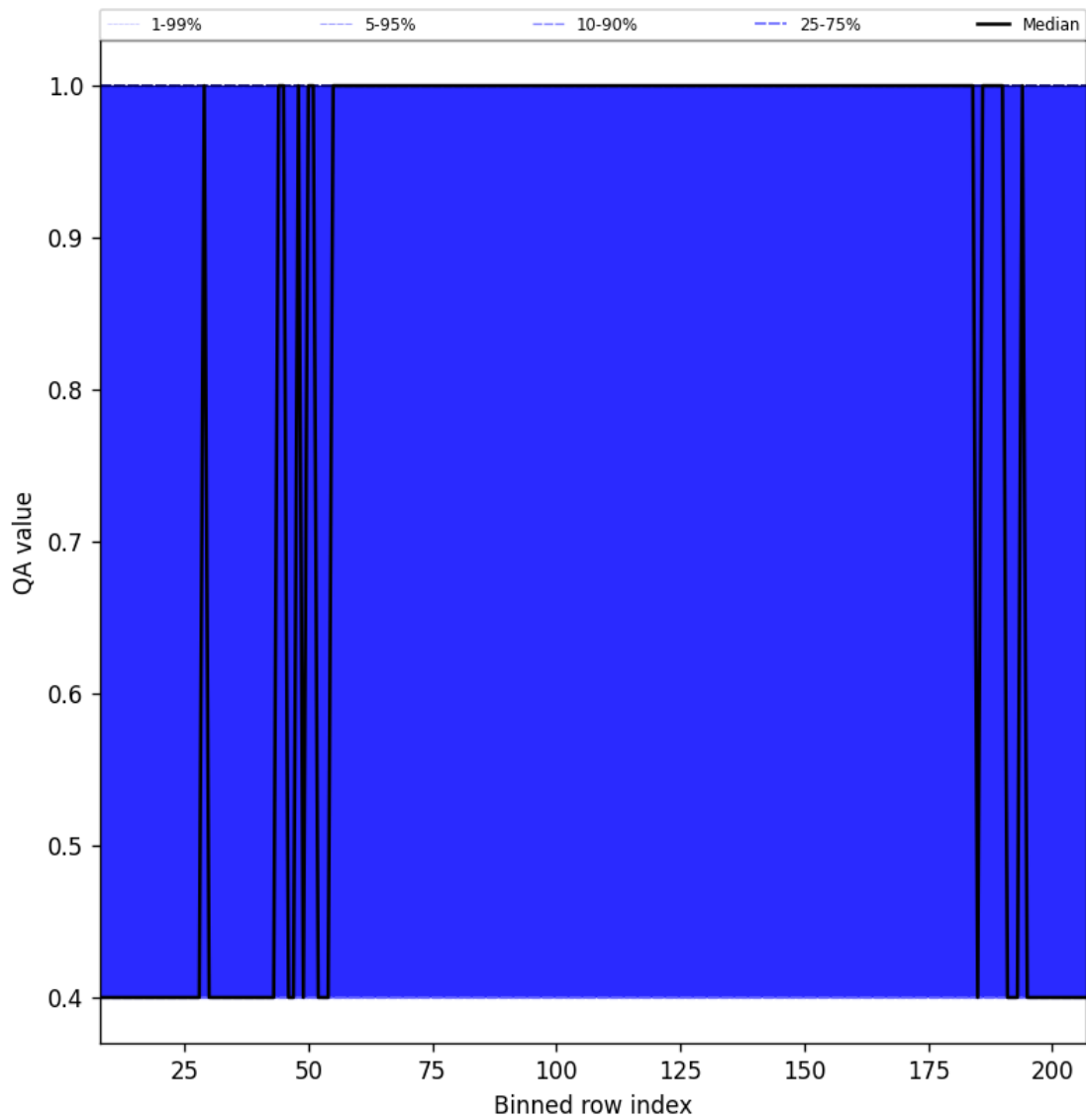
Figure 33: Along track statistics of “QA value” for 2025-03-26 to 2025-03-28
