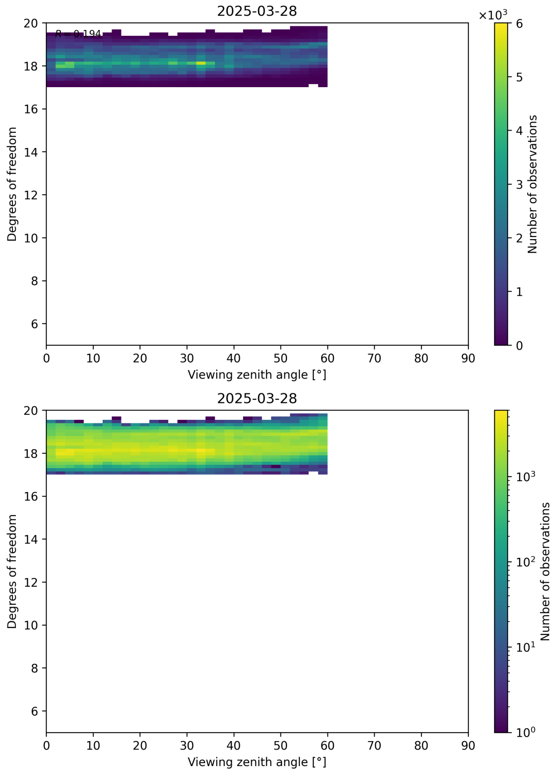
Figure 107: Scatter density plot of “Viewing zenith angle” against “Degrees of freedom” for 2025-03-28 to 2025-03-29.
