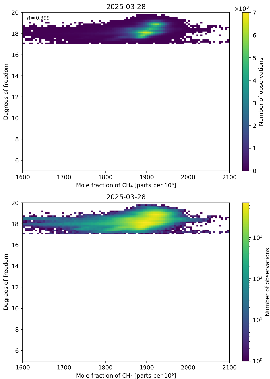
Figure 72: Scatter density plot of “Mole fraction of CH 4 ” against “Degrees of freedom” for 2025-03-28 to 2025-03-29.
