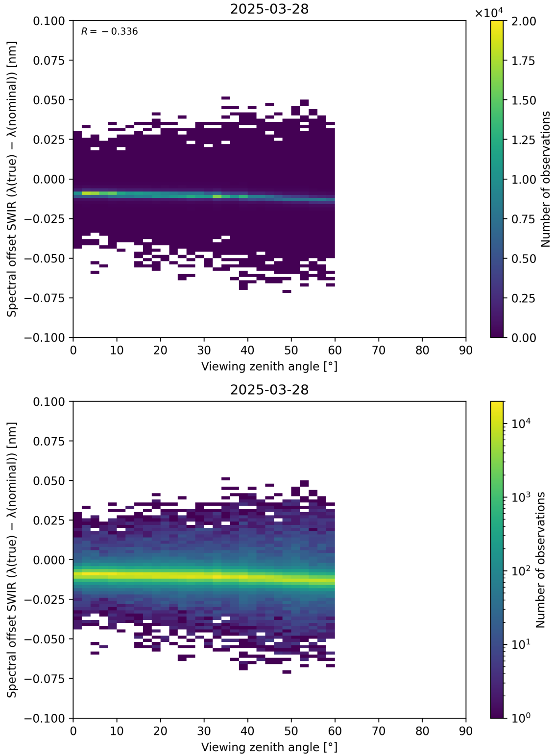
Figure 116: Scatter density plot of “Viewing zenith angle” against “Spectral offset SWIR ( \lambda_{\text{true}} - \lambda_{\text{nominal}} )” for 2025-03-28 to 2025-03-29.
