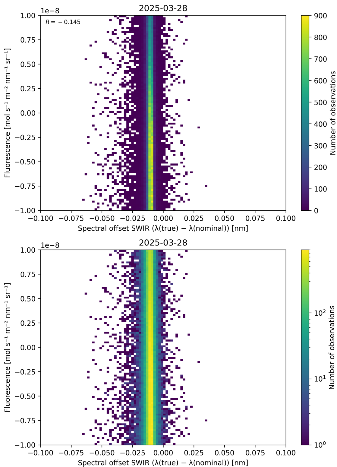
Figure 120: Scatter density plot of “Spectral offset SWIR ( \lambda_{\text{true}} - \lambda_{\text{nominal}} )” against “Fluorescence” for 2025-03-28 to 2025-03-29.
