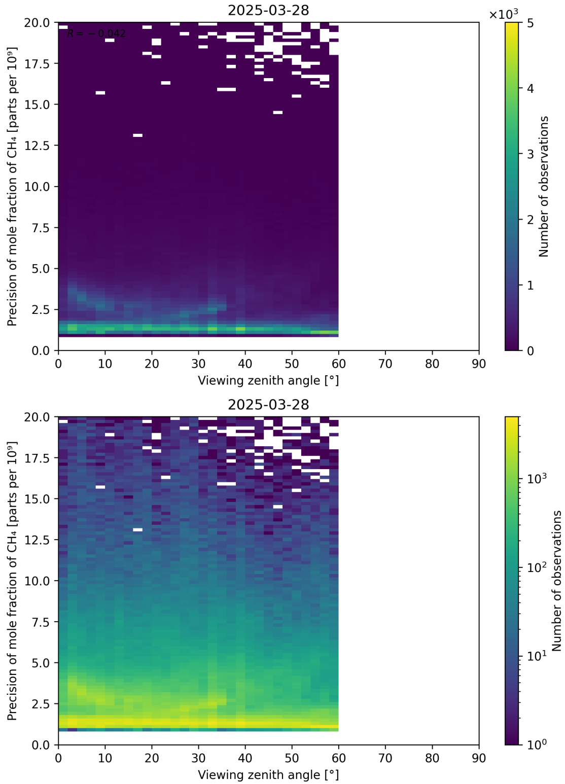
Figure 112: Scatter density plot of “Viewing zenith angle” against “Precision of mole fraction of CH 4 ” for 2025-03-28 to 2025-03-29.
