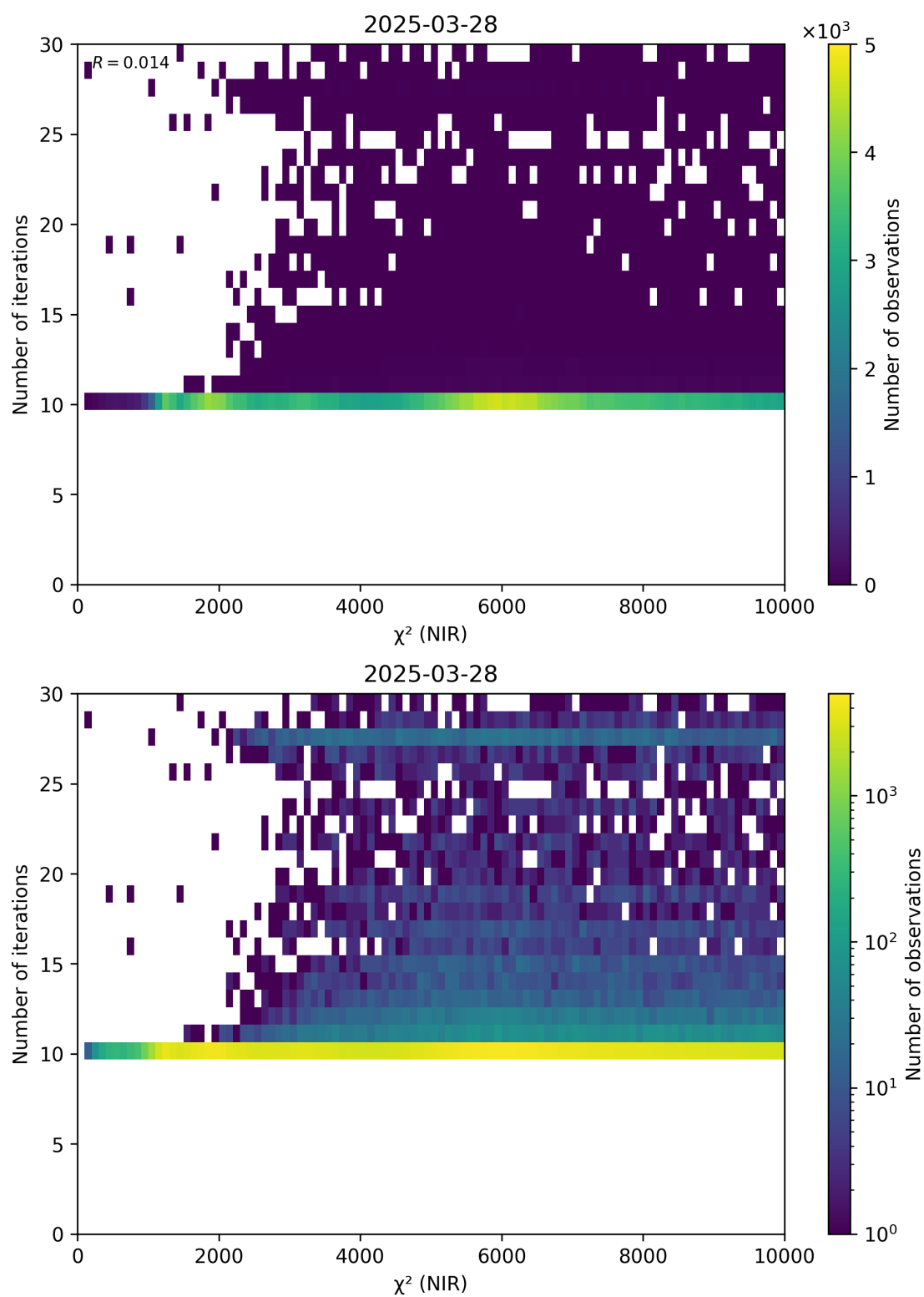
Figure 46: Scatter density plot of “ \chi^2 (NIR)” against “Number of iterations” for 2025-03-28 to 2025-03-29.
