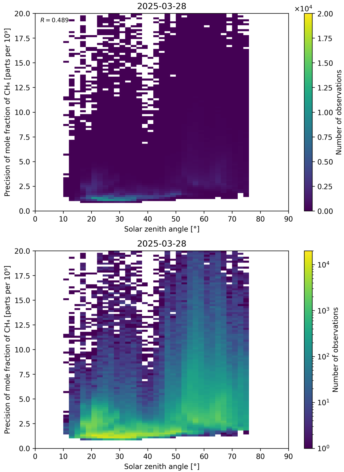
Figure 101: Scatter density plot of “Solar zenith angle” against “Precision of mole fraction of \text{CH}_4 ” for 2025-03-28 to 2025-03-29.
