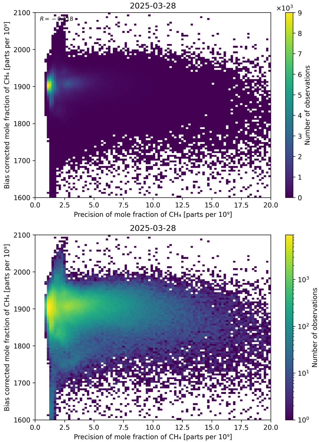
Figure 82: Scatter density plot of “Precision of mole fraction of CH 4 ” against “Bias corrected mole fraction of CH 4 ” for 2025-03-28 to 2025-03-29.
