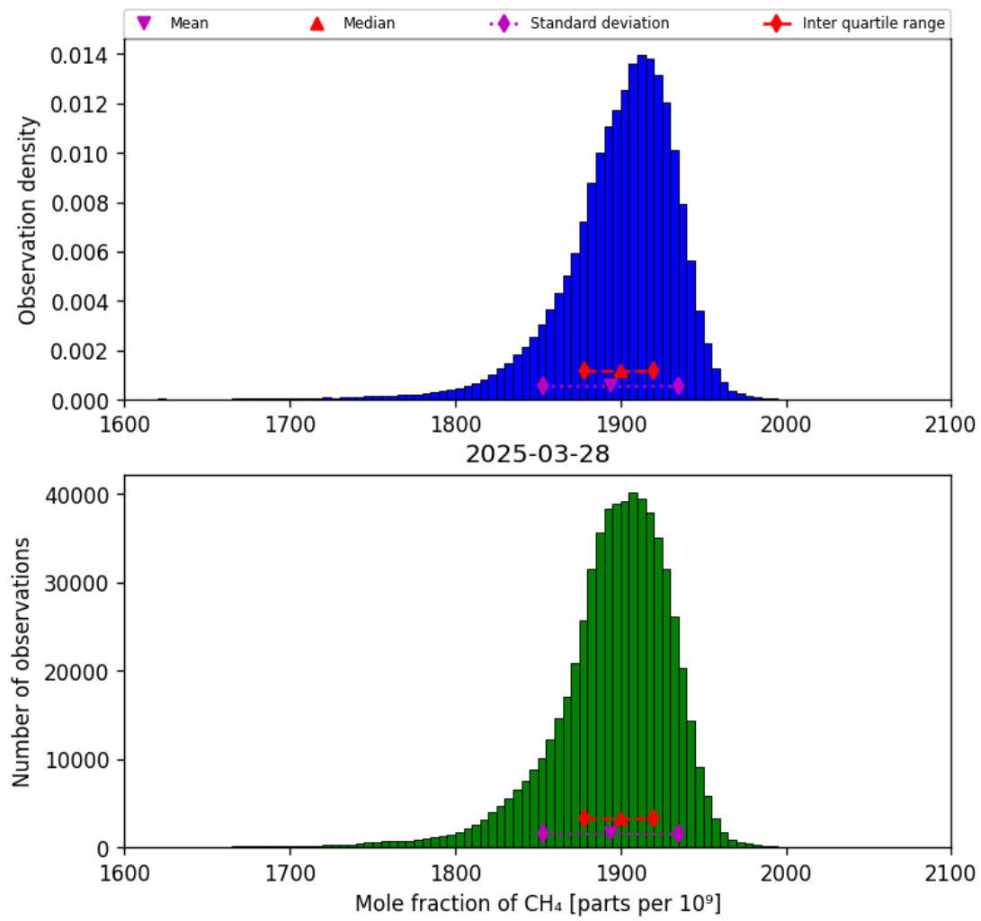
Figure 23: Histogram of “Mole fraction of CH 4 ” for 2025-03-28 to 2025-03-29
