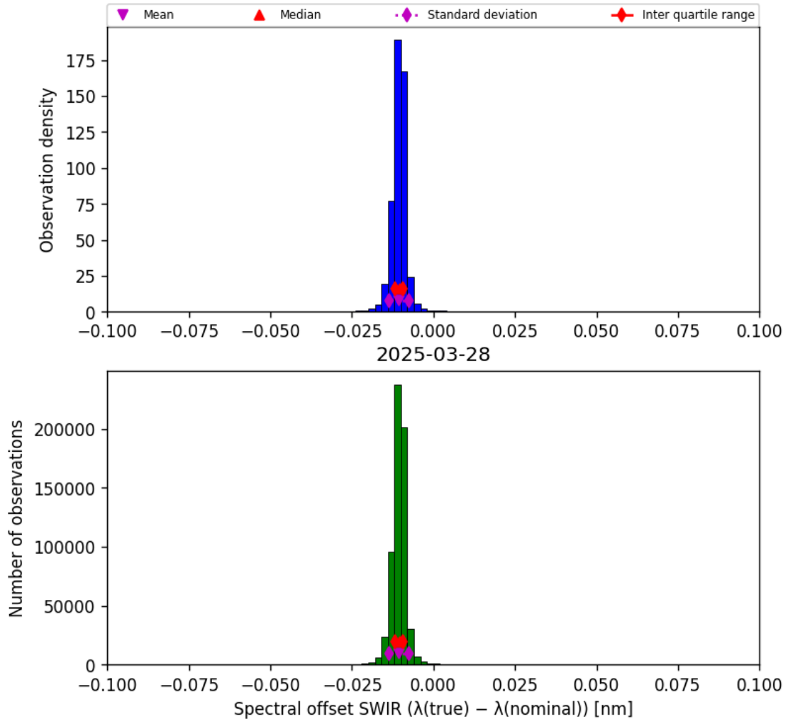
Figure 27: Histogram of “Spectral offset SWIR ( \lambda_{\text{true}} - \lambda_{\text{nominal}} )” for 2025-03-28 to 2025-03-29
