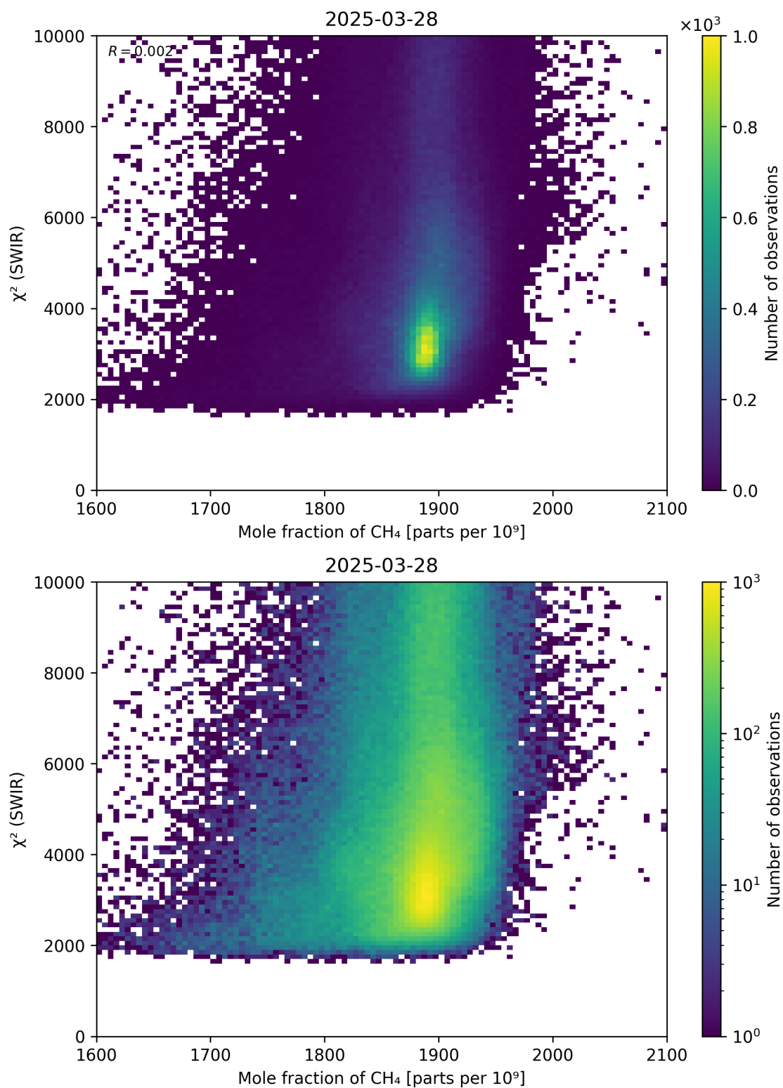
Figure 71: Scatter density plot of “Mole fraction of \text{CH}_4 ” against “ \chi^2 (SWIR)” for 2025-03-28 to 2025-03-29.
