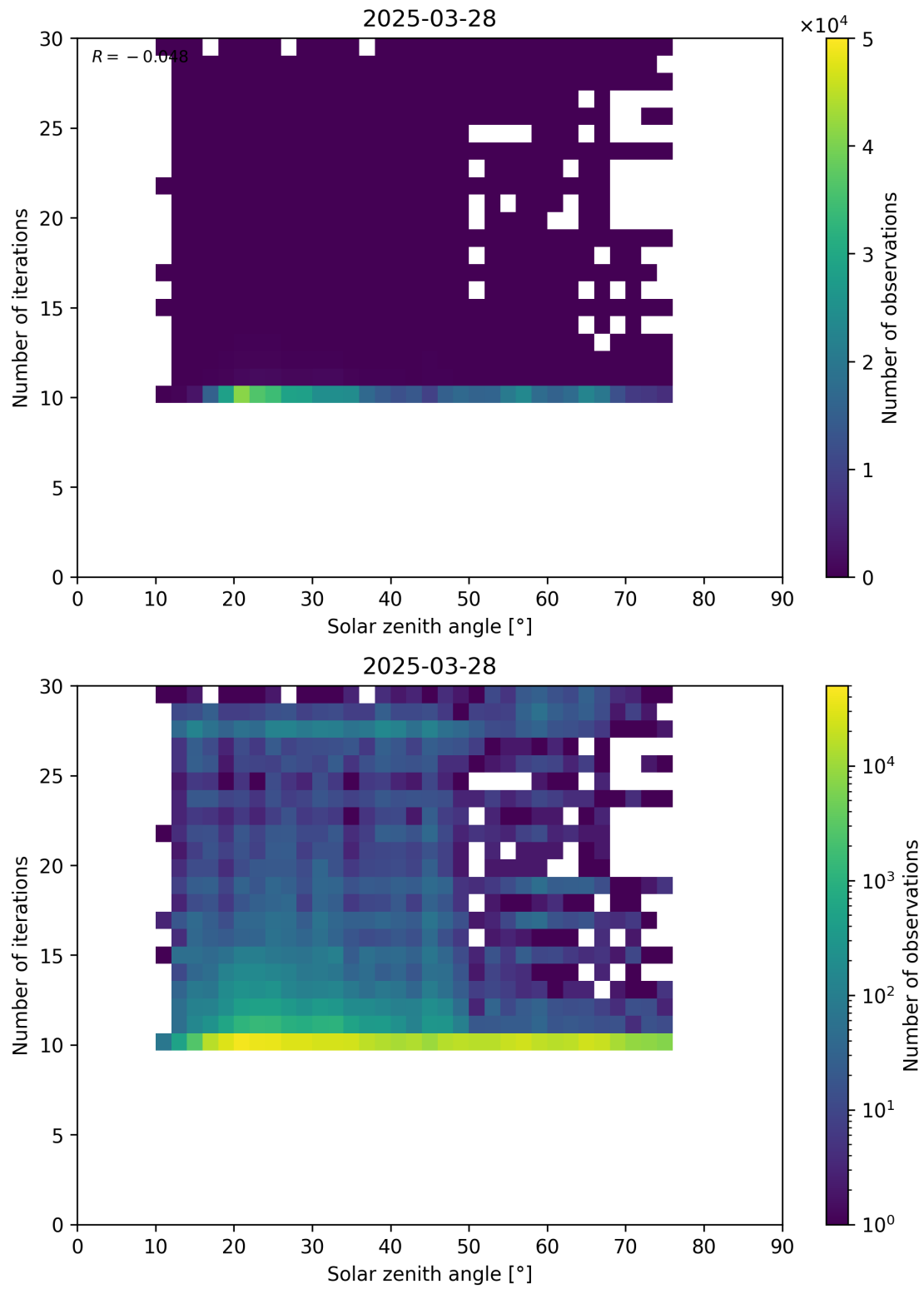
Figure 102: Scatter density plot of “Solar zenith angle” against “Number of iterations” for 2025-03-28 to 2025-03-29.
