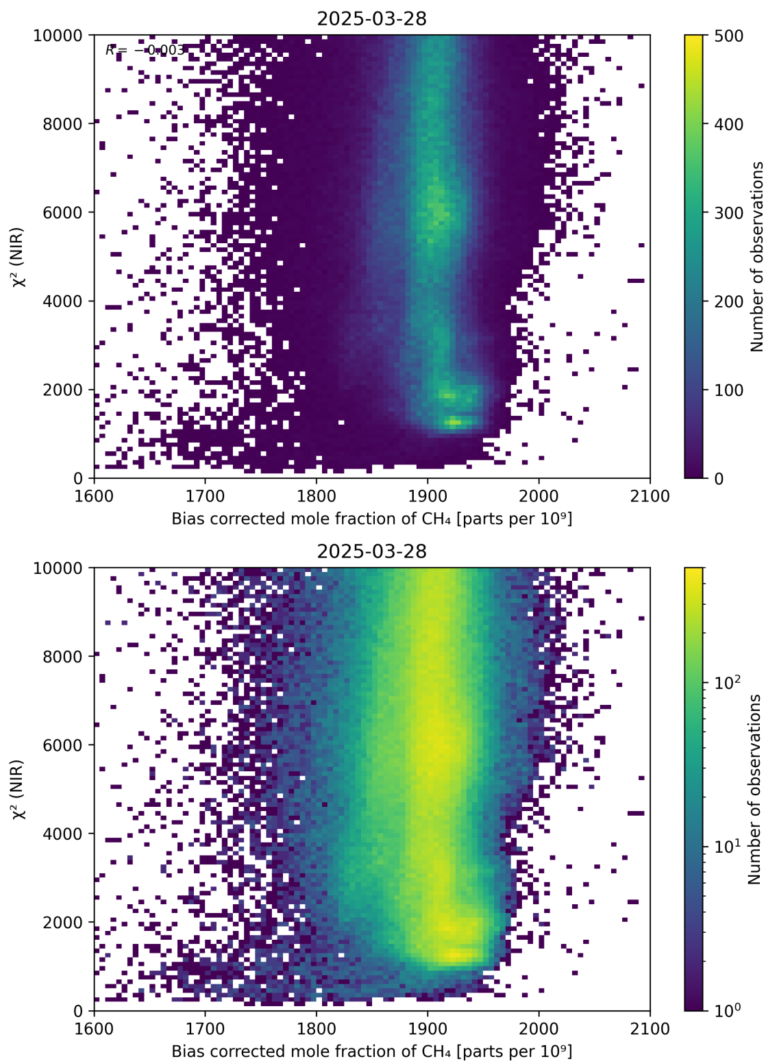
Figure 63: Scatter density plot of “Bias corrected mole fraction of \text{CH}_4 ” against “ \chi^2 (NIR)” for 2025-03-28 to 2025-03-29.
