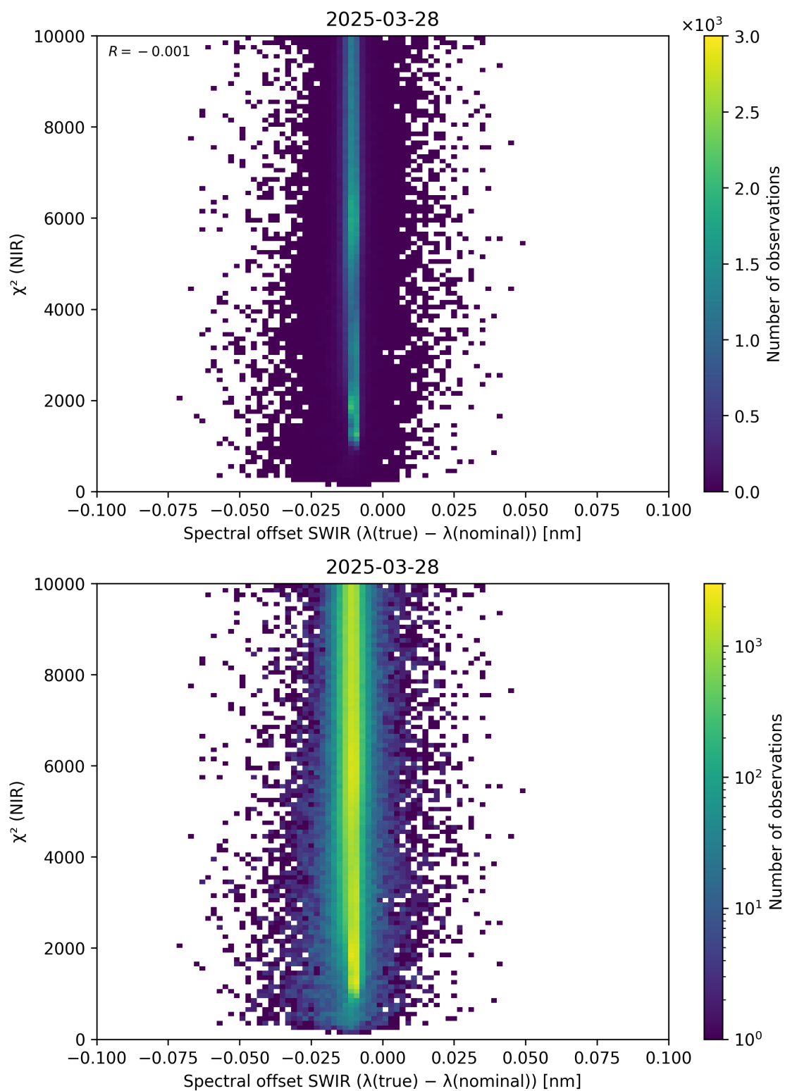
Figure 117: Scatter density plot of “Spectral offset SWIR ( \lambda_{\text{true}} - \lambda_{\text{nominal}} )” against “ \chi^2 (NIR)” for 2025-03-28 to 2025-03-29.
