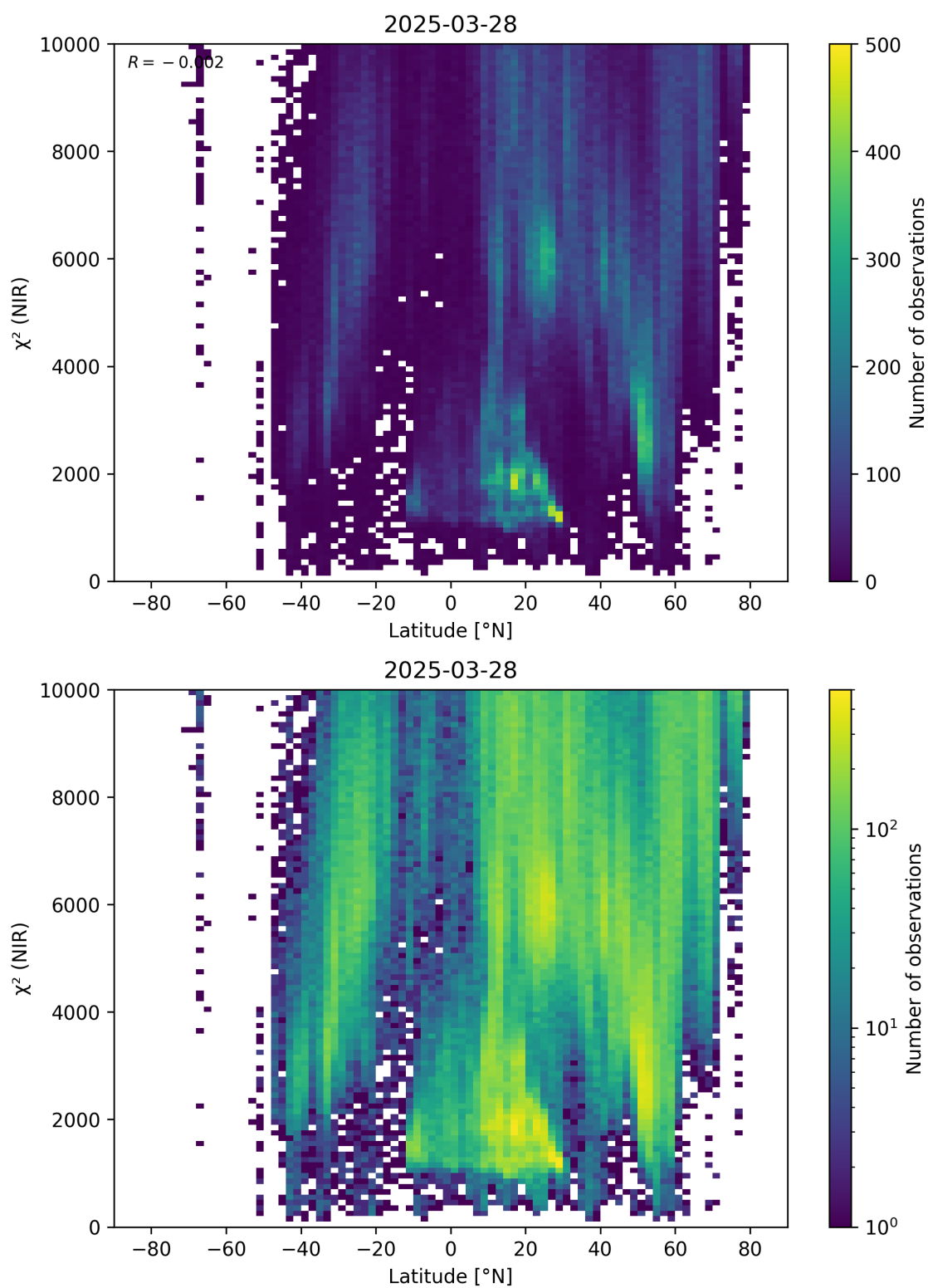
Figure 53: Scatter density plot of “Latitude” against “ \chi^2 (NIR)” for 2025-03-28 to 2025-03-29.
