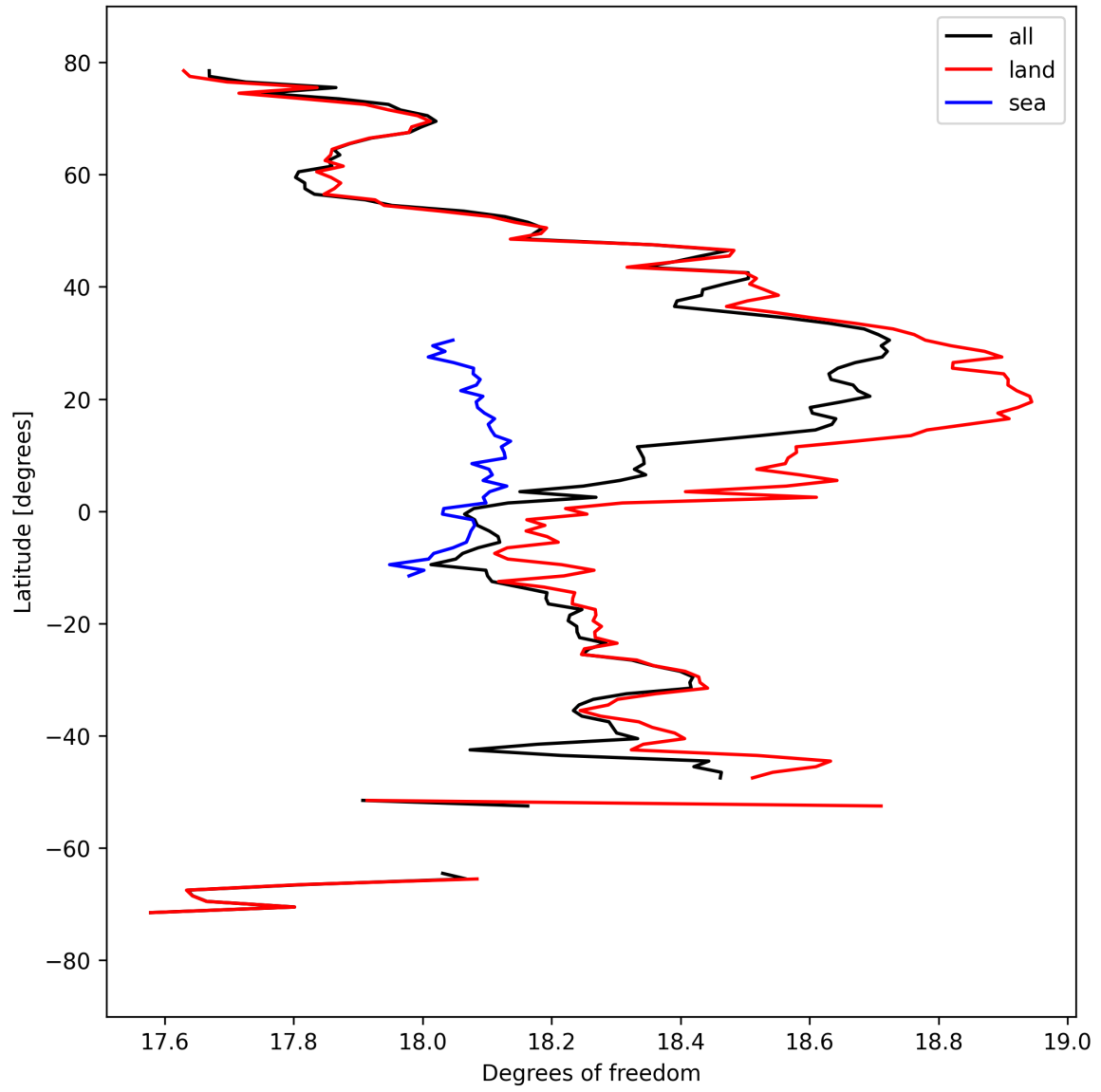
Figure 19: Zonal average of “Degrees of freedom” for 2025-03-28 to 2025-03-29.
