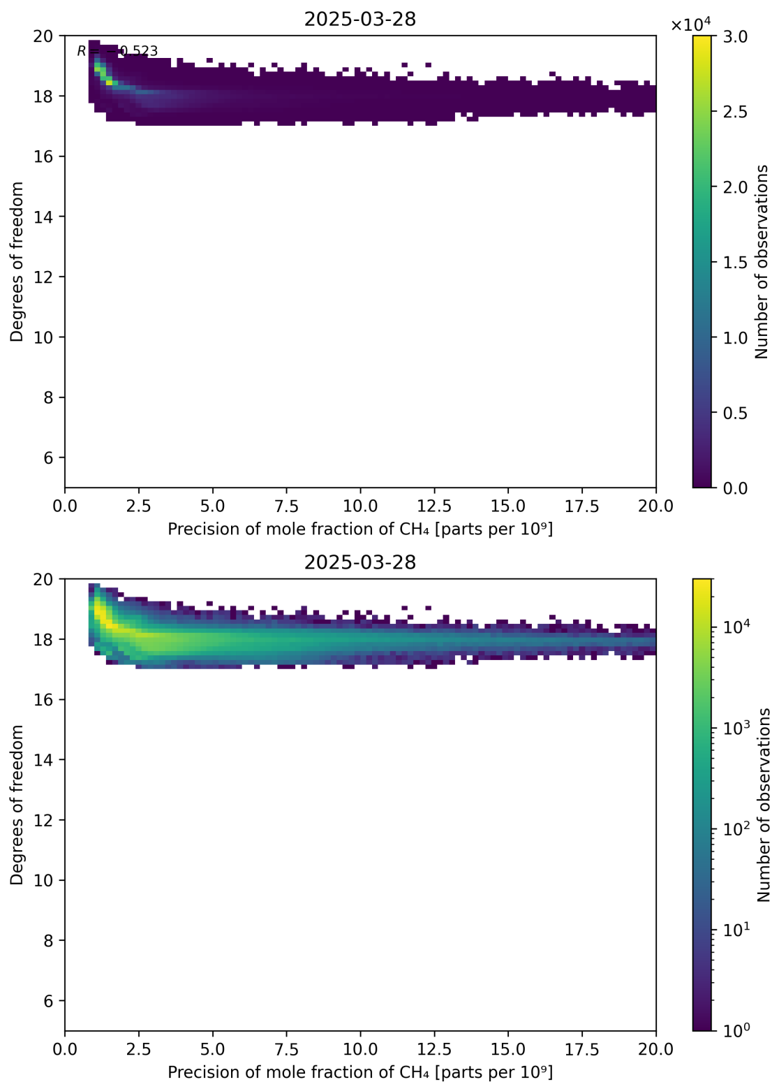
Figure 80: Scatter density plot of “Precision of mole fraction of CH 4 ” against “Degrees of freedom” for 2025-03-28 to 2025-03-29.
