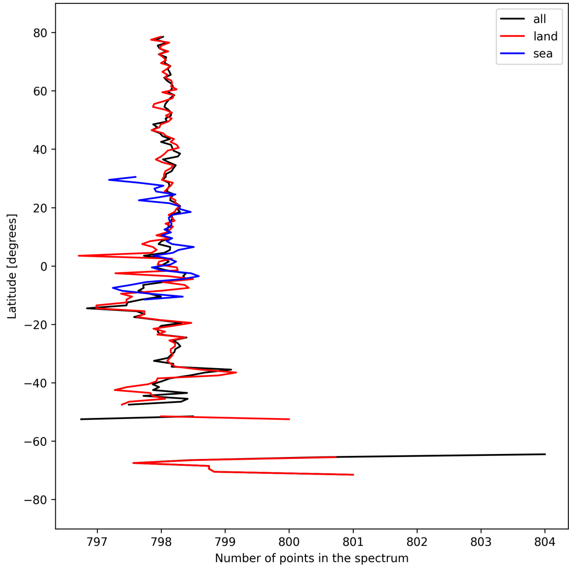
Figure 15: Zonal average of “Number of points in the spectrum” for 2025-03-28 to 2025-03-29.
