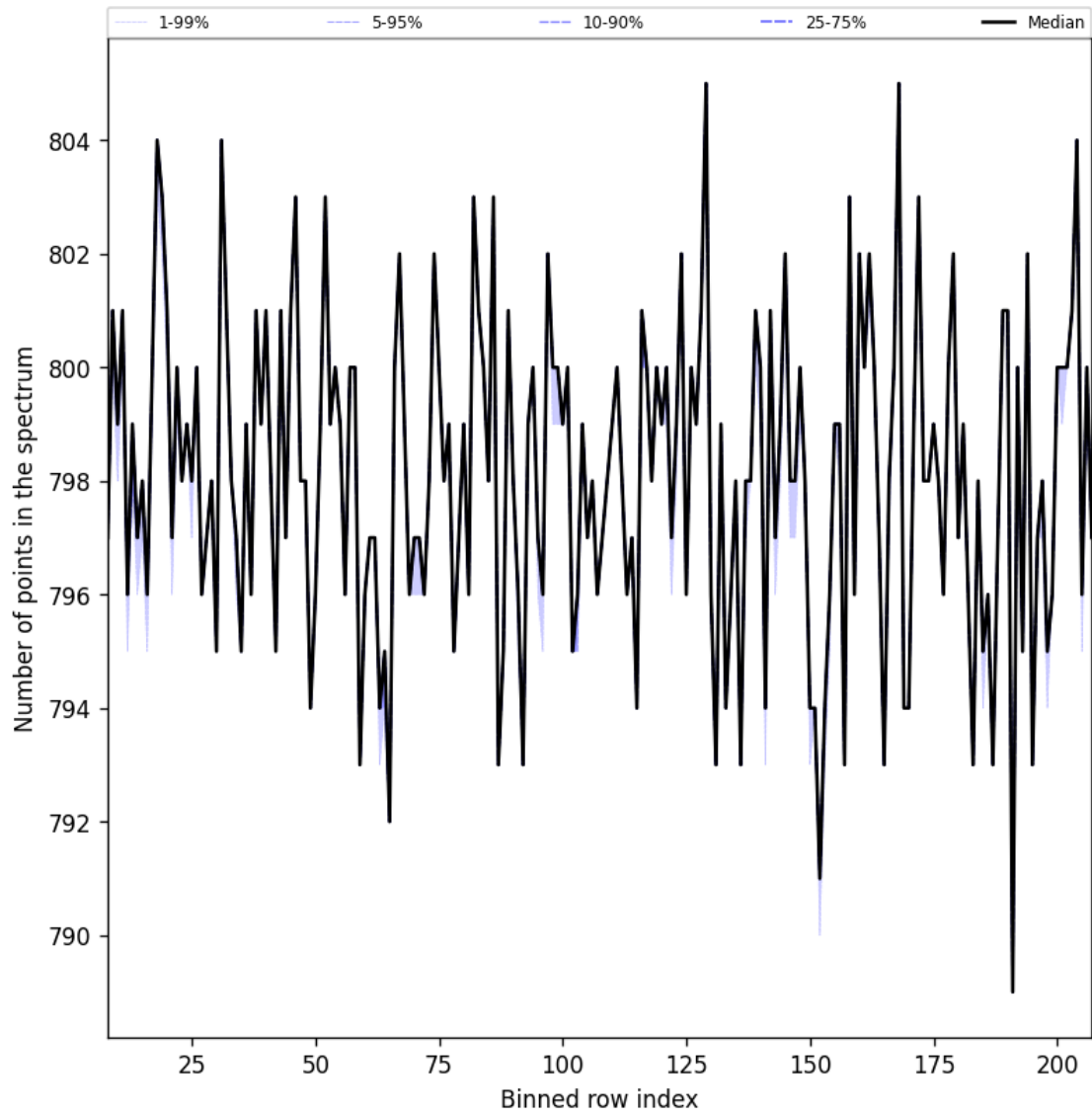
Figure 37: Along track statistics of “Number of points in the spectrum” for 2025-03-28 to 2025-03-29
