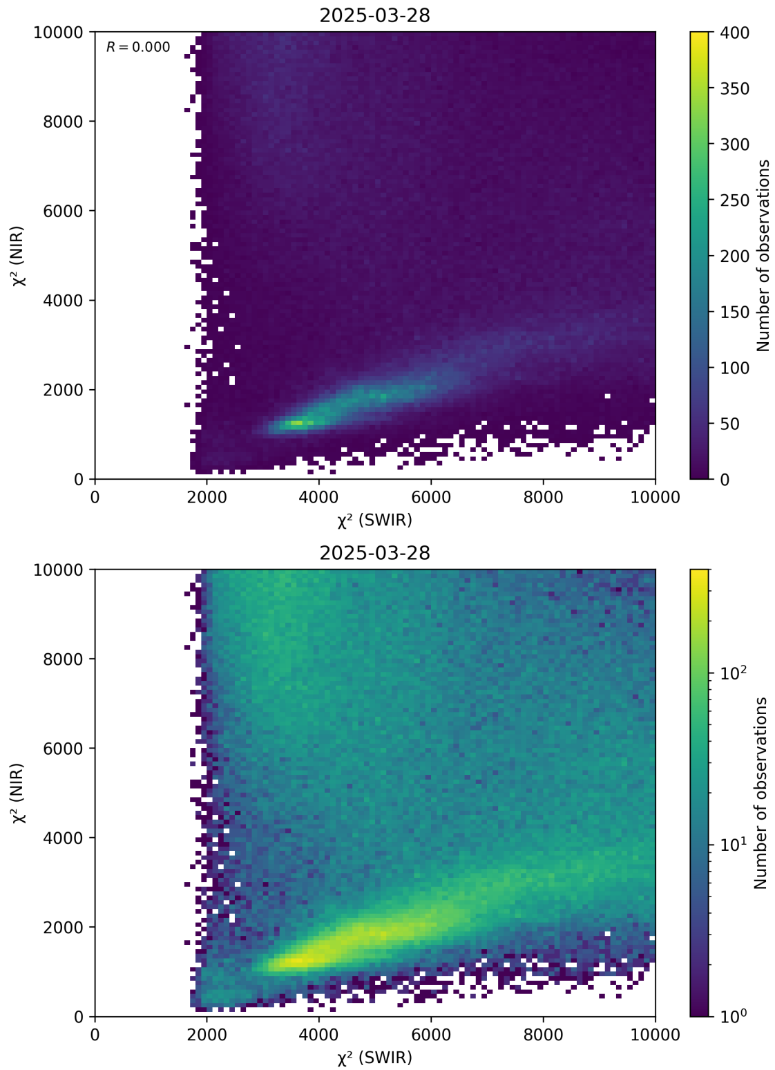
Figure 47: Scatter density plot of “ \chi^2 (SWIR)” against “ \chi^2 (NIR)” for 2025-03-28 to 2025-03-29.
