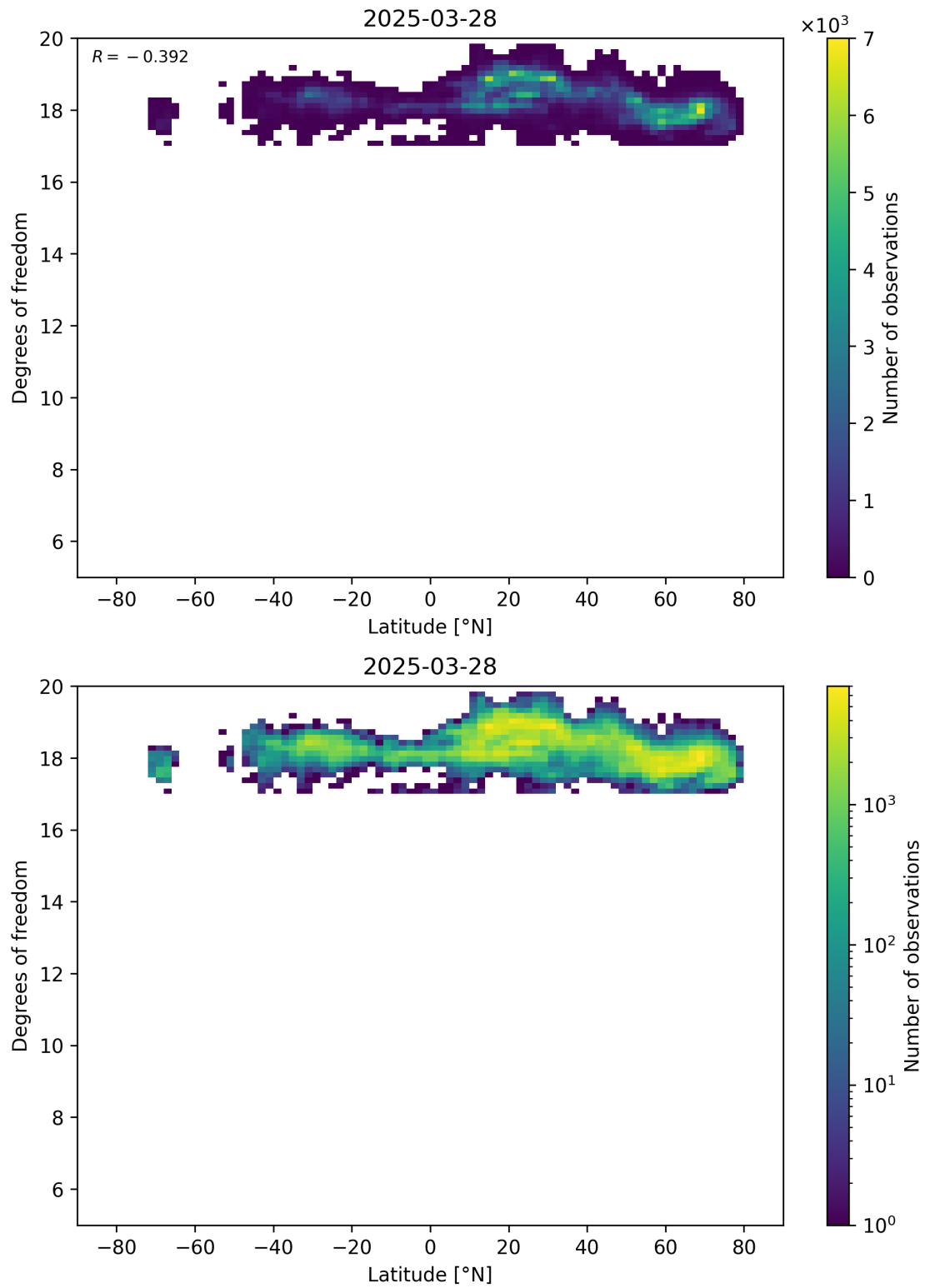
Figure 55: Scatter density plot of “Latitude” against “Degrees of freedom” for 2025-03-28 to 2025-03-29.
