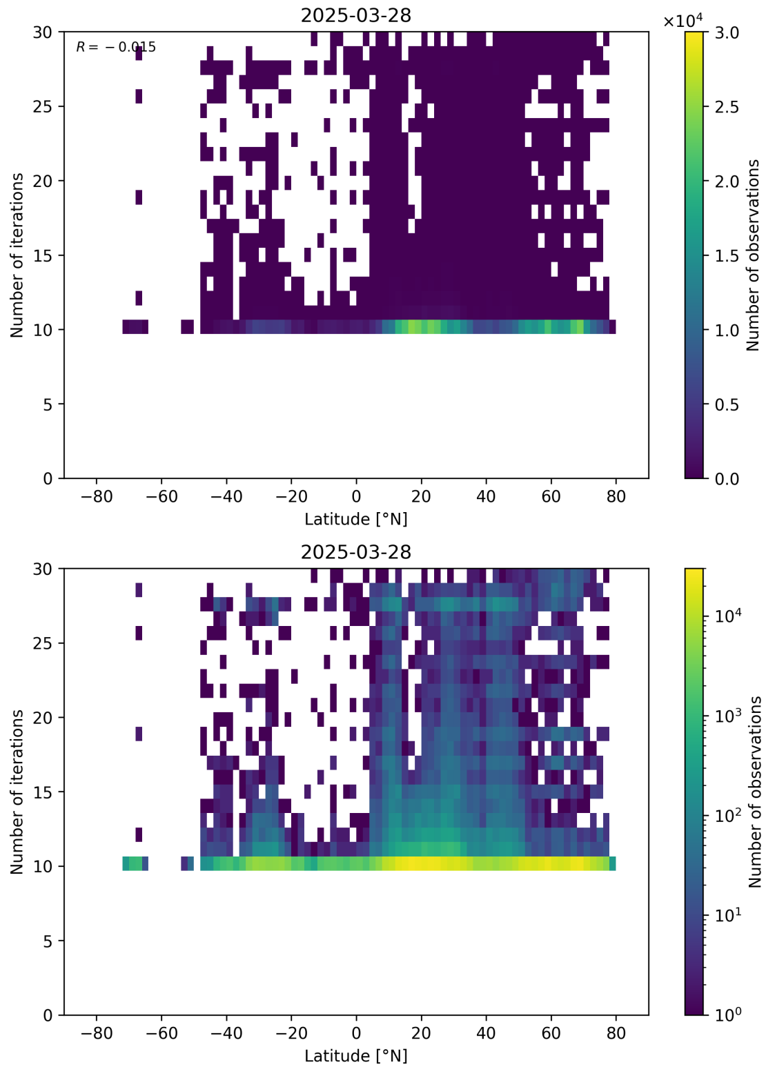
Figure 60: Scatter density plot of “Latitude” against “Number of iterations” for 2025-03-28 to 2025-03-29.
