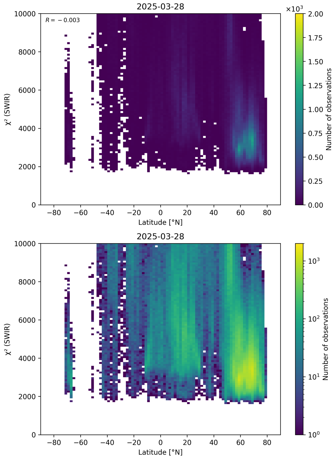
Figure 54: Scatter density plot of “Latitude” against “ \chi^2 (SWIR)” for 2025-03-28 to 2025-03-29.
