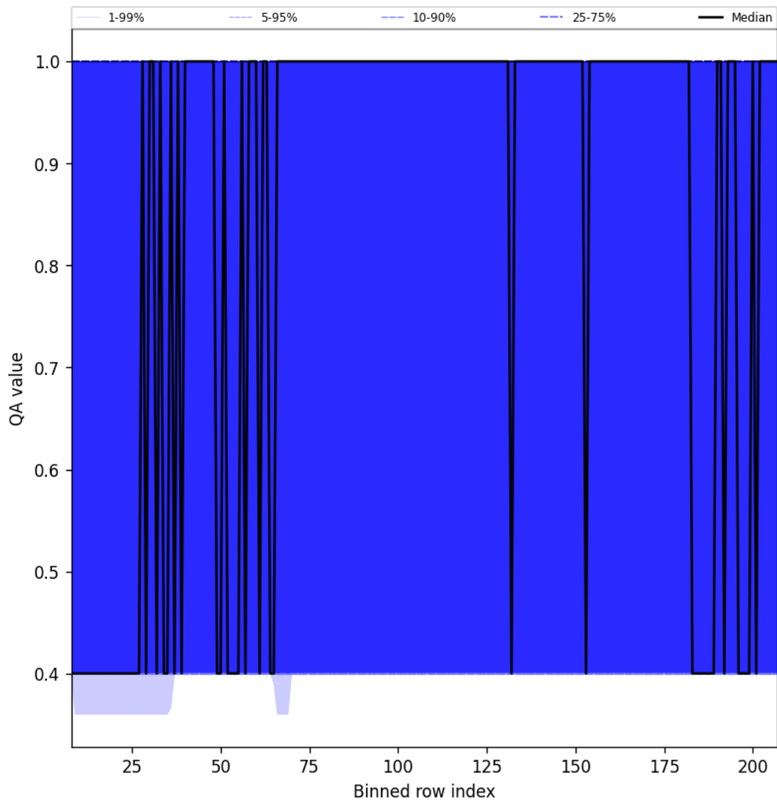
Figure 33: Along track statistics of “QA value” for 2025-03-28 to 2025-03-29
