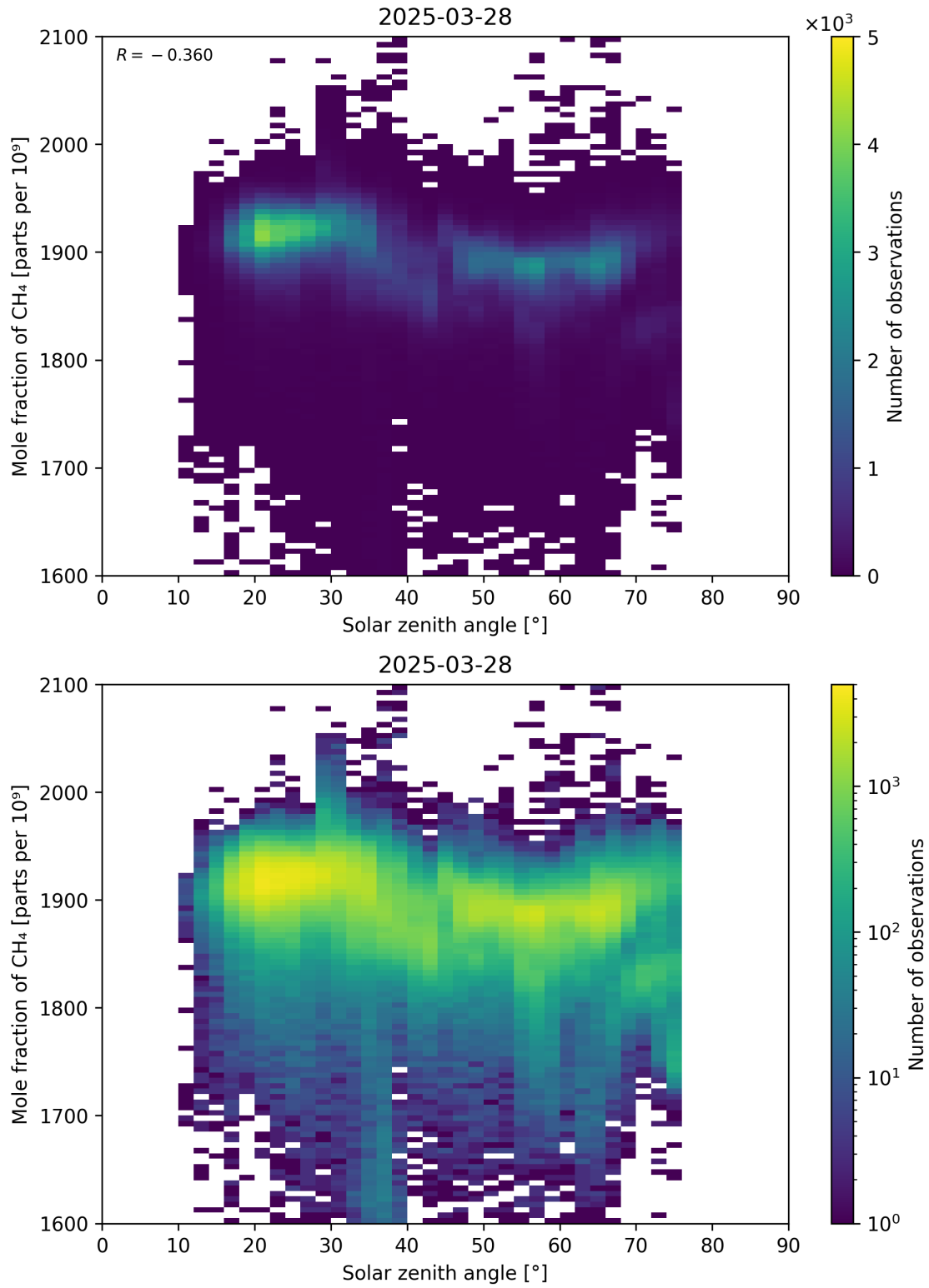
Figure 99: Scatter density plot of “Solar zenith angle” against “Mole fraction of CH 4 ” for 2025-03-28 to 2025-03-29.
