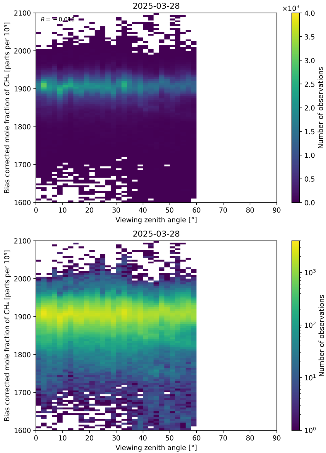
Figure 111: Scatter density plot of “Viewing zenith angle” against “Bias corrected mole fraction of CH 4 ” for 2025-03-28 to 2025-03-29.
