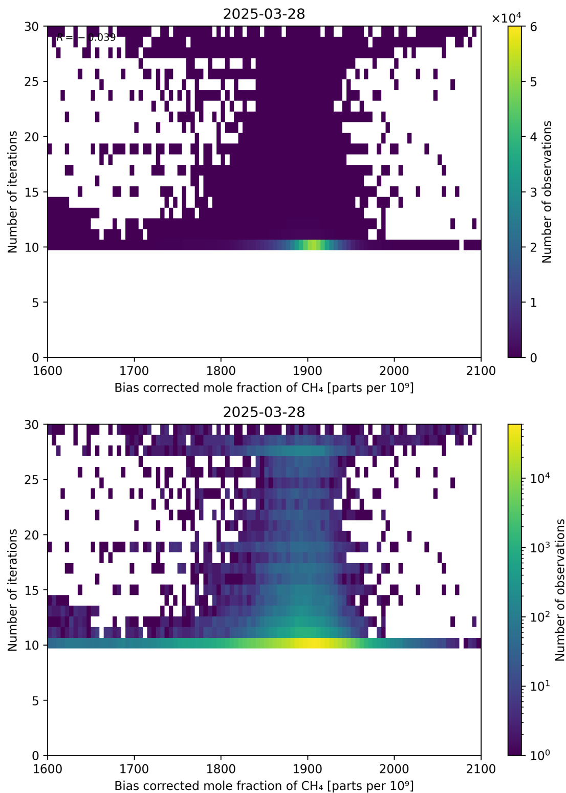
Figure 67: Scatter density plot of “Bias corrected mole fraction of \text{CH}_4 ” against “Number of iterations” for 2025-03-28 to 2025-03-29.
