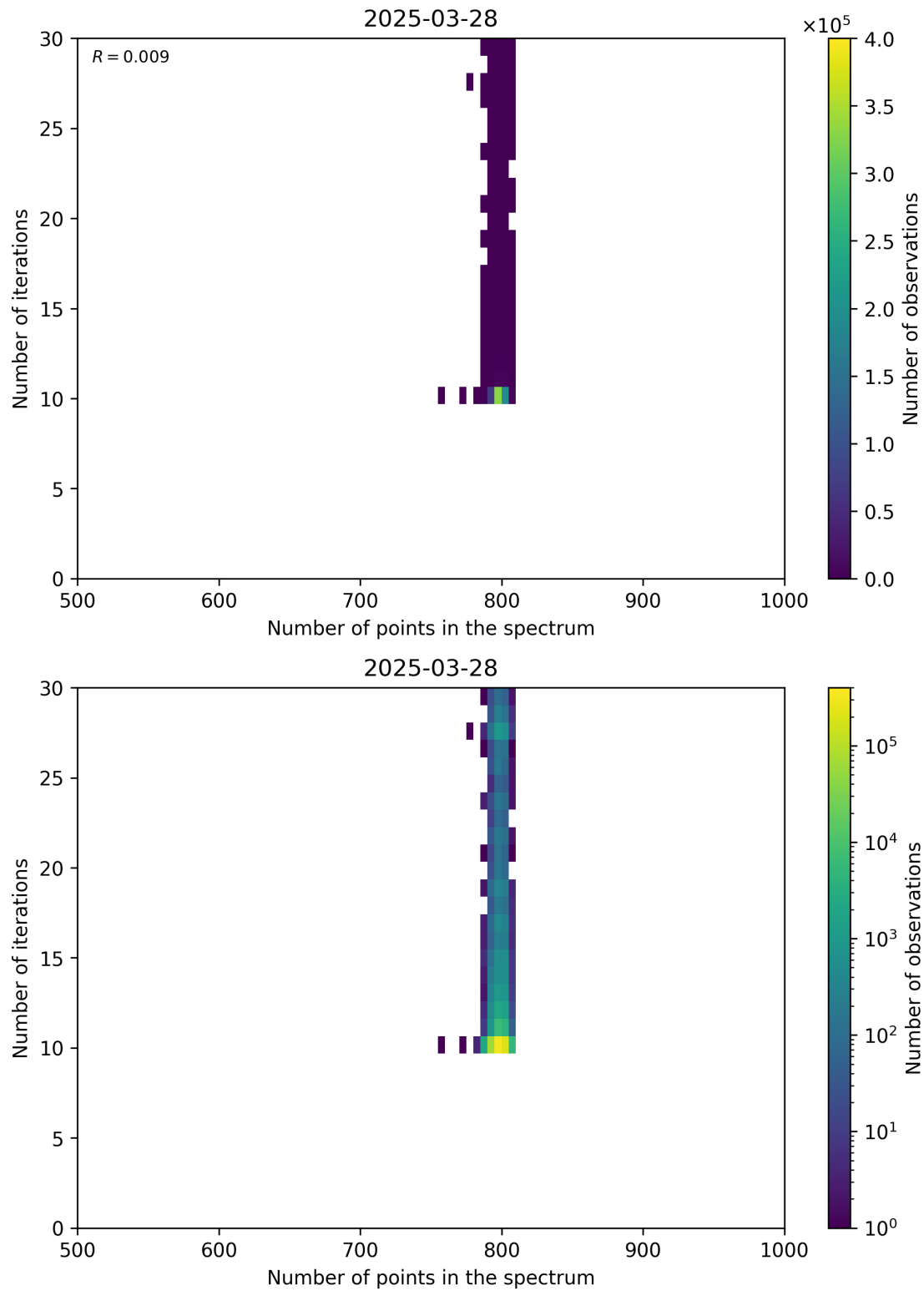
Figure 92: Scatter density plot of “Number of points in the spectrum” against “Number of iterations” for 2025-03-28 to 2025-03-29.
