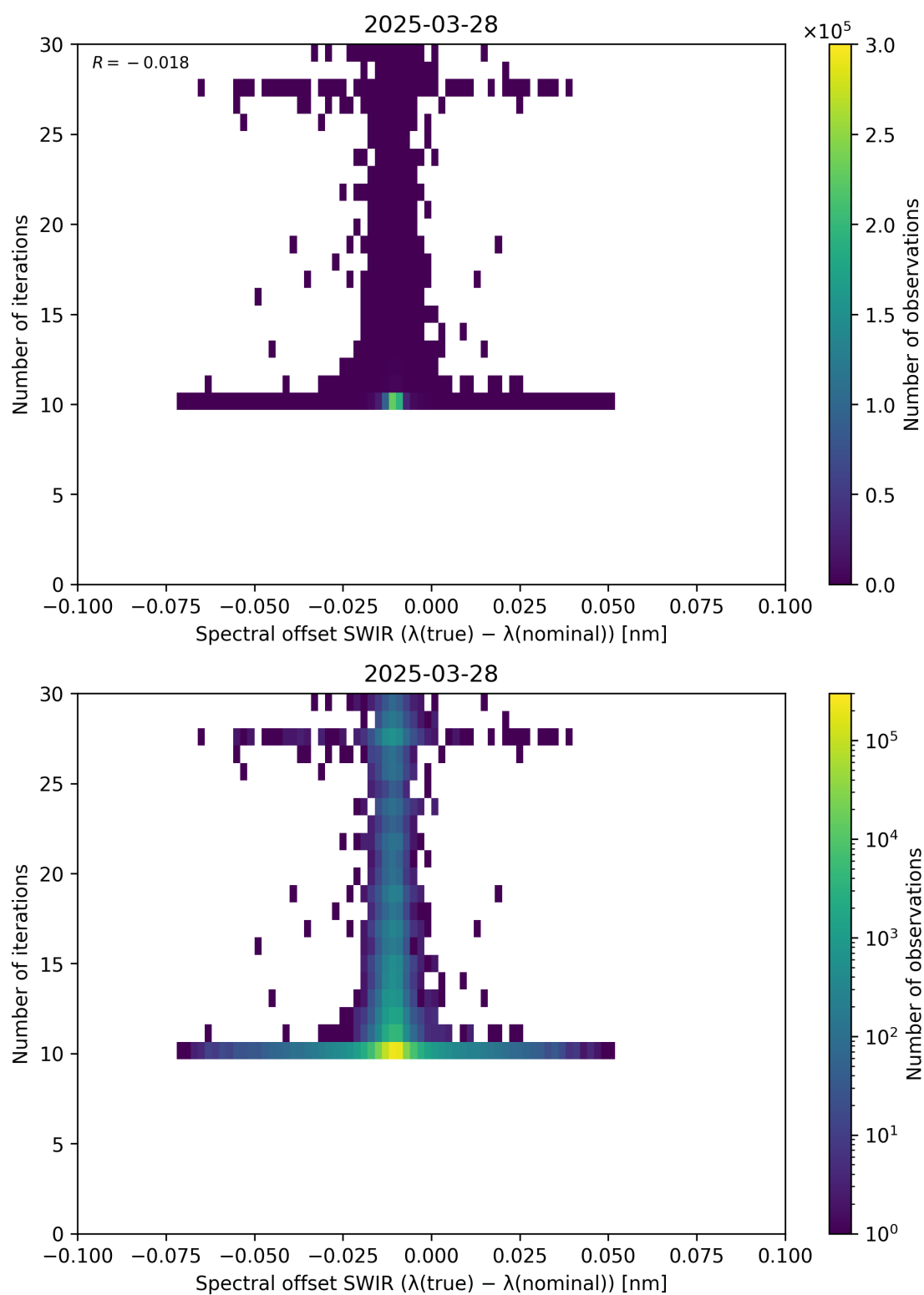
Figure 121: Scatter density plot of “Spectral offset SWIR ( \lambda_{\text{true}} - \lambda_{\text{nominal}} )” against “Number of iterations” for 2025-03-28 to 2025-03-29.
