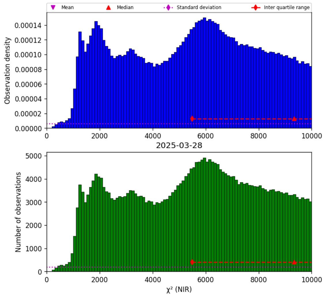
Figure 29: Histogram of “ \chi^2 (NIR)” for 2025-03-28 to 2025-03-29
