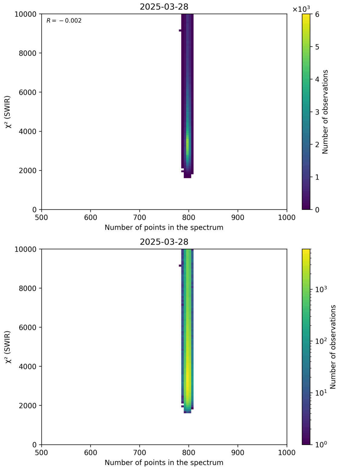
Figure 89: Scatter density plot of “Number of points in the spectrum” against “ \chi^2 (SWIR)” for 2025-03-28 to 2025-03-29.
