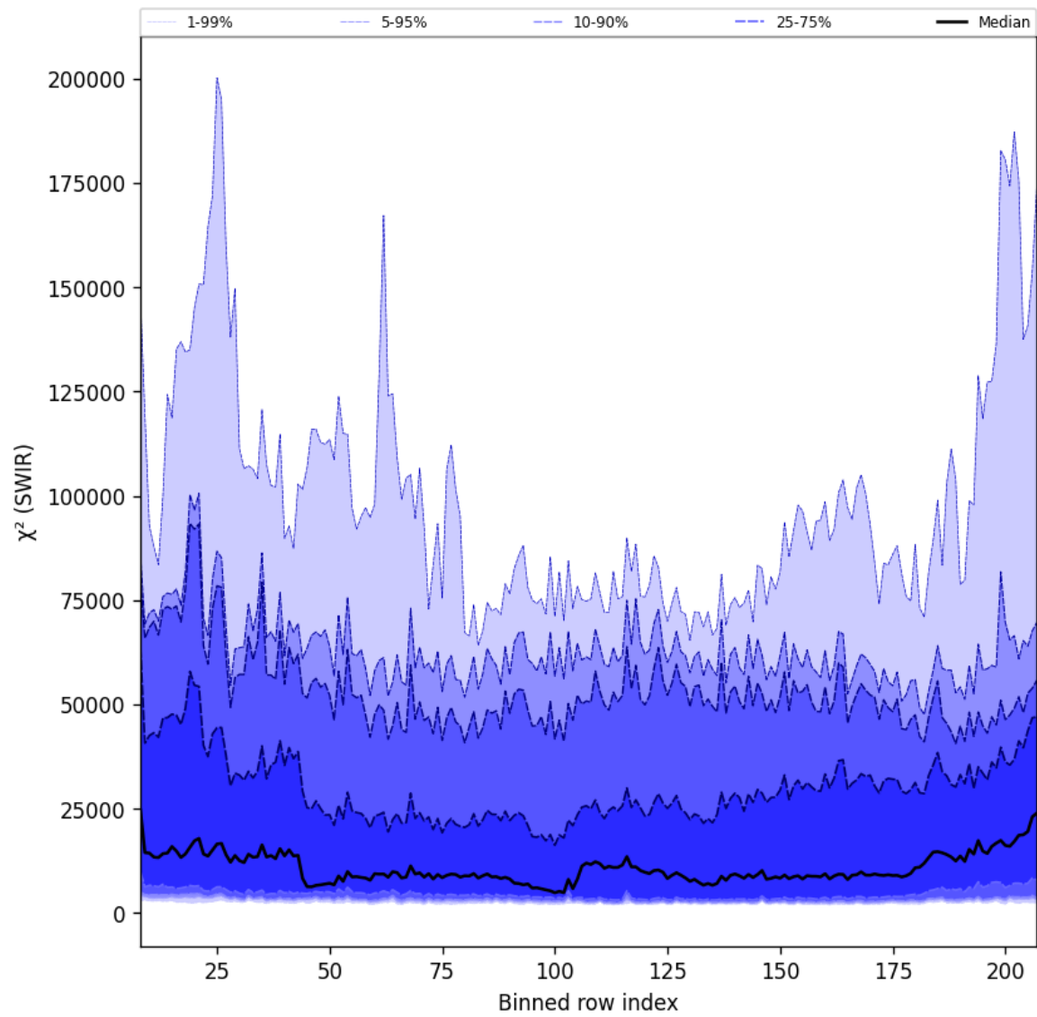
Figure 39: Along track statistics of “ \chi^2 (SWIR)” for 2025-03-28 to 2025-03-29
