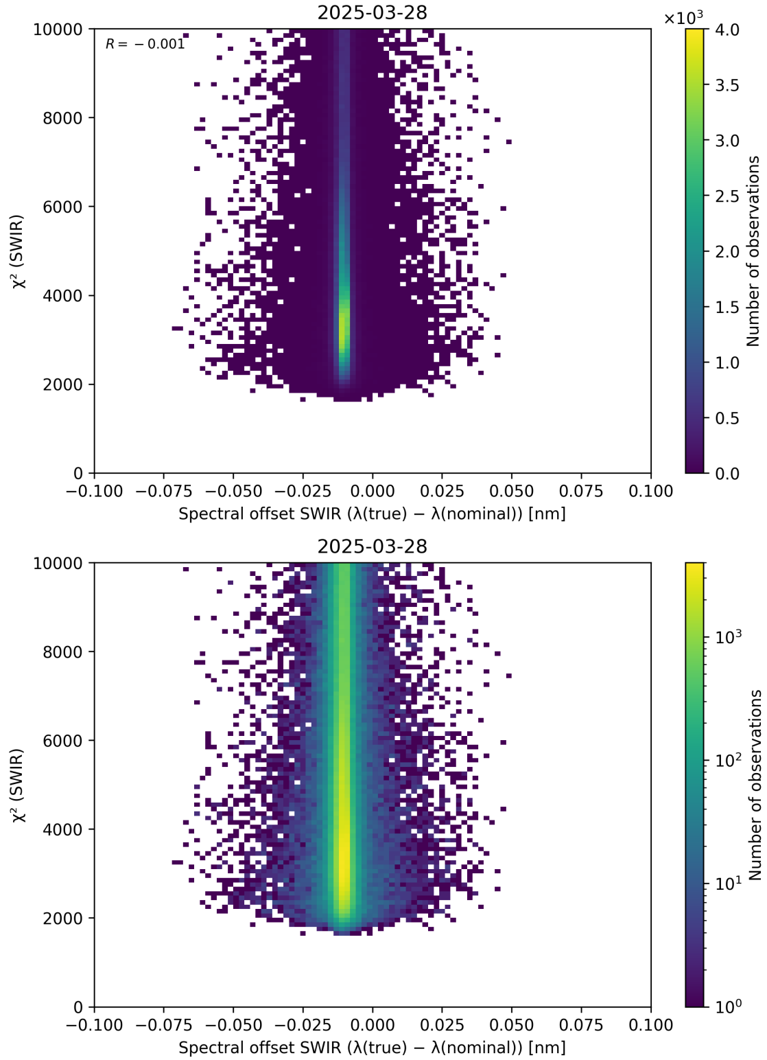
Figure 118: Scatter density plot of “Spectral offset SWIR ( \lambda_{\text{true}} - \lambda_{\text{nominal}} )” against “ \chi^2 (SWIR)” for 2025-03-28 to 2025-03-29.
