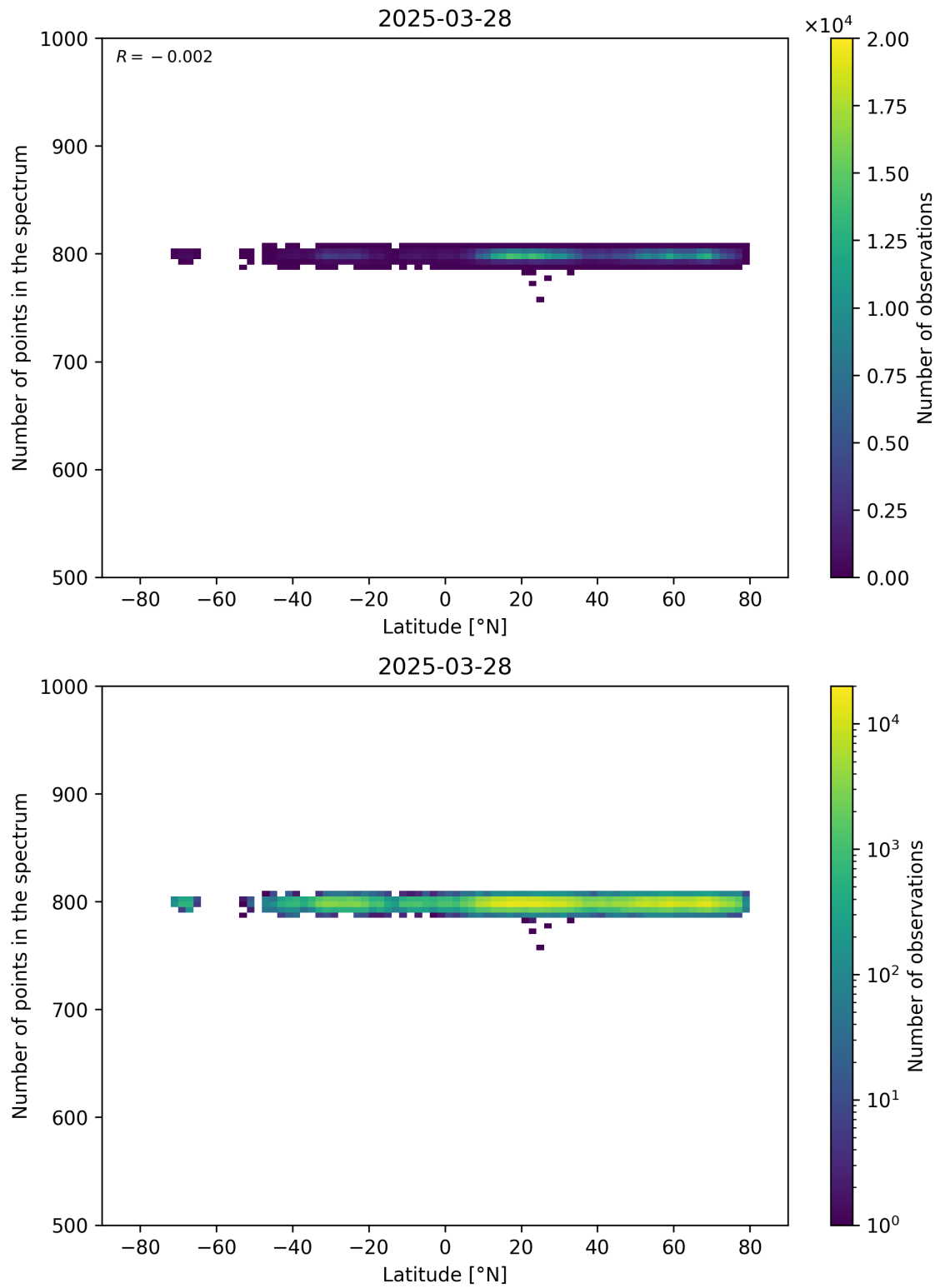
Figure 61: Scatter density plot of “Latitude” against “Number of points in the spectrum” for 2025-03-28 to 2025-03-29.
