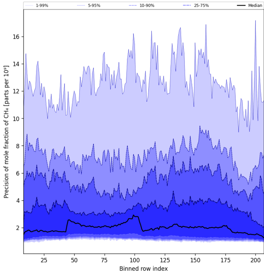
Figure 35: Along track statistics of “Precision of mole fraction of CH 4 ” for 2025-03-28 to 2025-03-29
