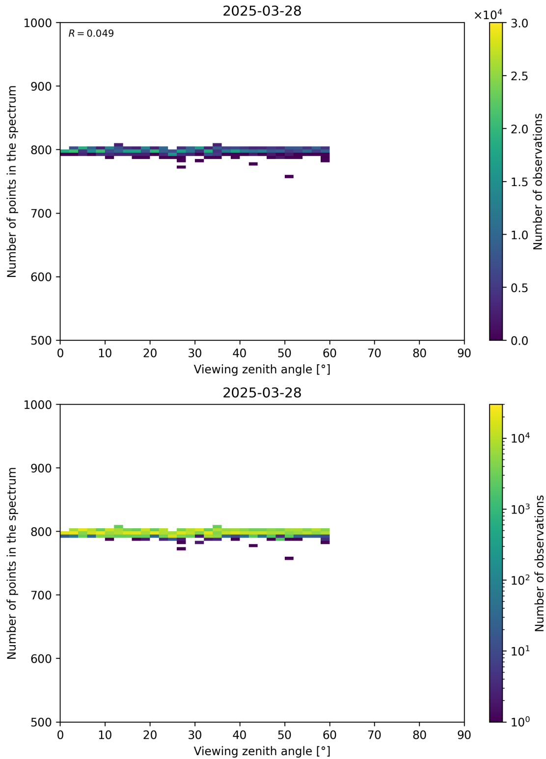
Figure 114: Scatter density plot of “Viewing zenith angle” against “Number of points in the spectrum” for 2025-03-28 to 2025-03-29.
