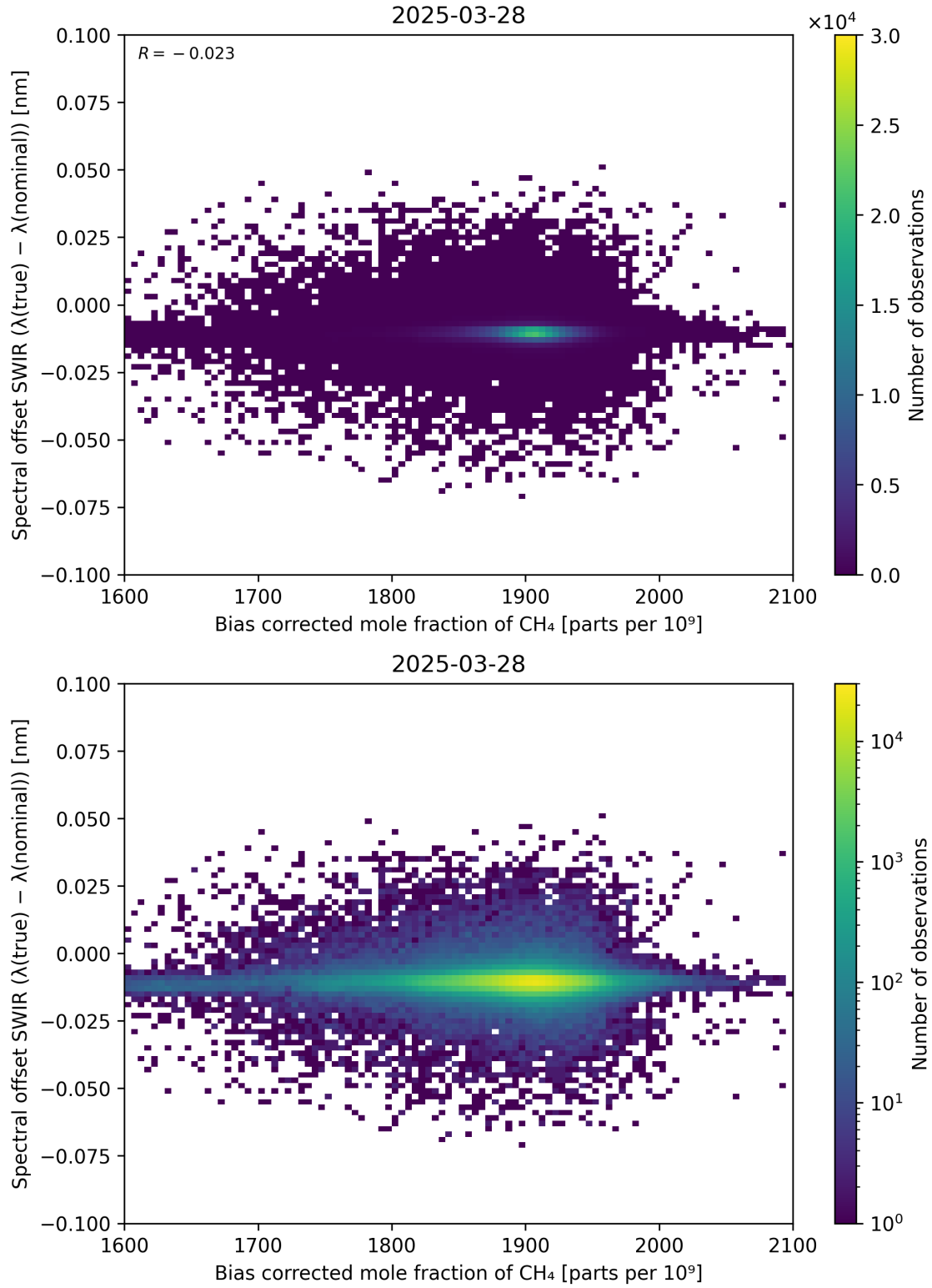
Figure 69: Scatter density plot of “Bias corrected mole fraction of \text{CH}_4 ” against “Spectral offset SWIR ( \lambda_{\text{true}} - \lambda_{\text{nominal}} )” for 2025-03-28 to 2025-03-29.
