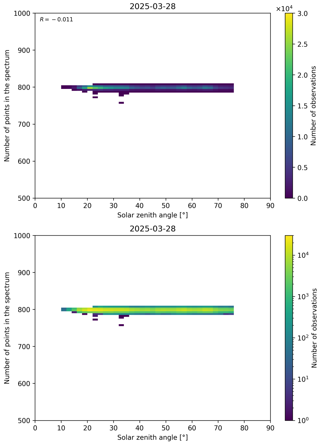
Figure 103: Scatter density plot of “Solar zenith angle” against “Number of points in the spectrum” for 2025-03-28 to 2025-03-29.
