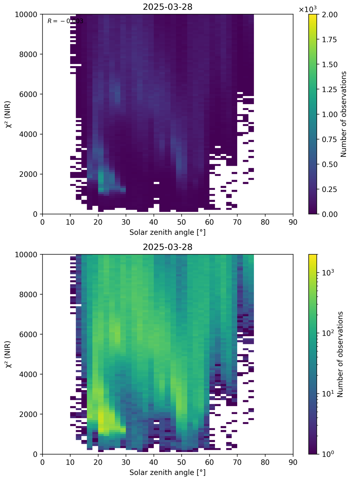
Figure 94: Scatter density plot of “Solar zenith angle” against “ \chi^2 (NIR)” for 2025-03-28 to 2025-03-29.
