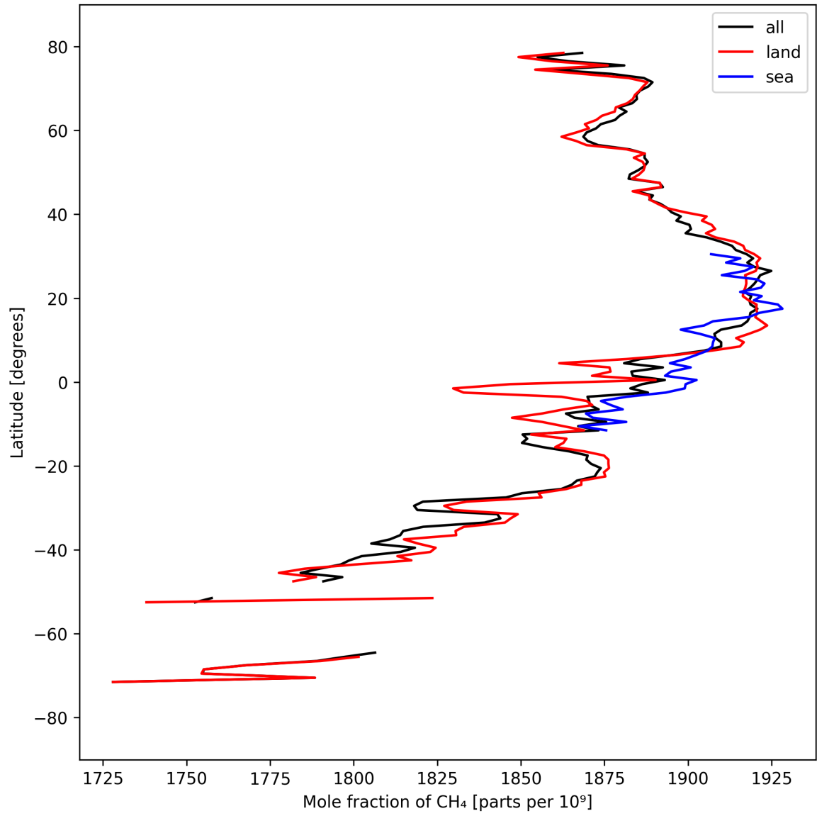
Figure 12: Zonal average of “Mole fraction of CH 4 ” for 2025-03-28 to 2025-03-29.
