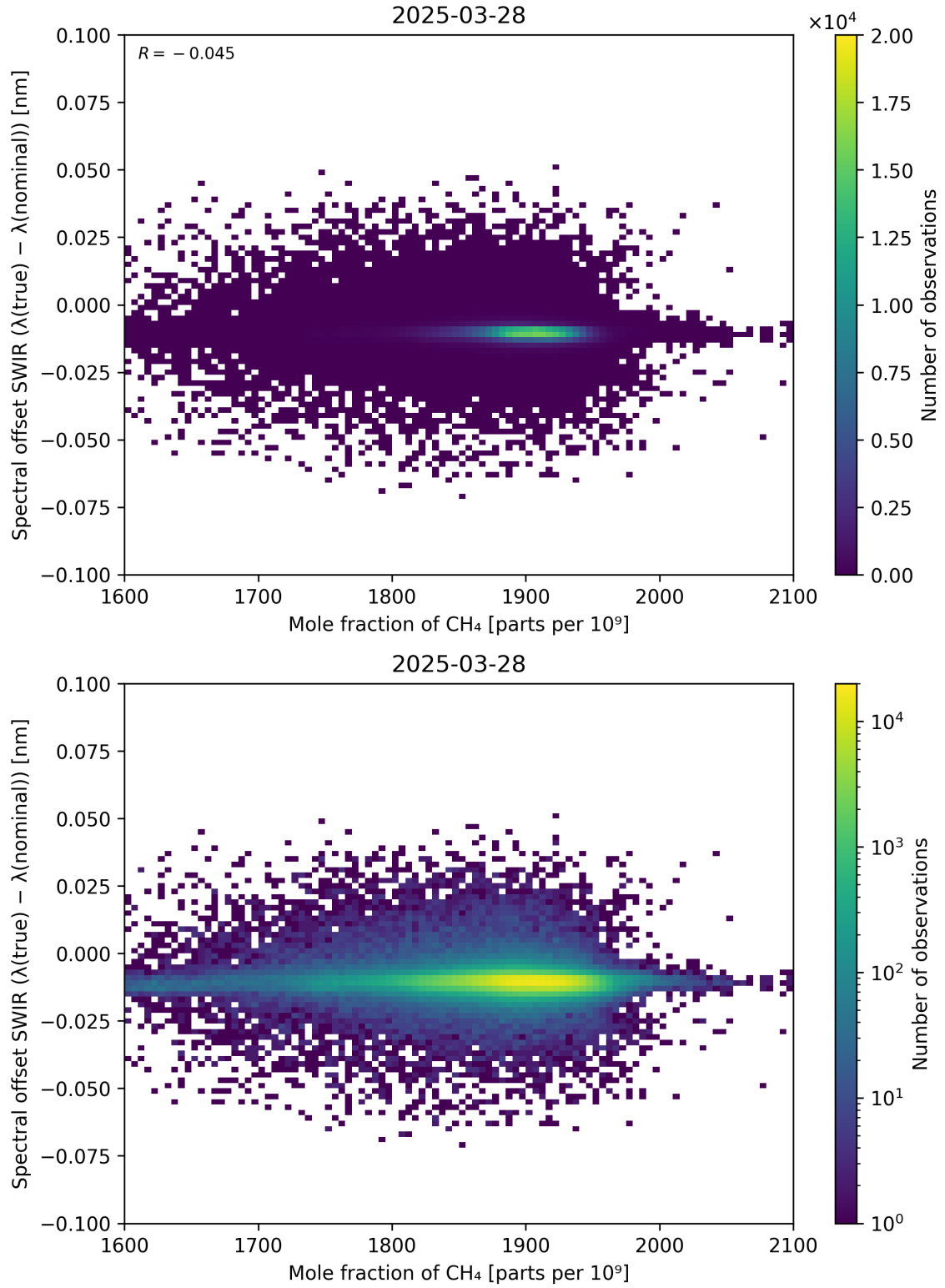
Figure 86: Scatter density plot of “Mole fraction of CH 4 ” against “Spectral offset SWIR ( \lambda_{\text{true}} - \lambda_{\text{nominal}} )” for 2025-03-28 to 2025-03-29.
