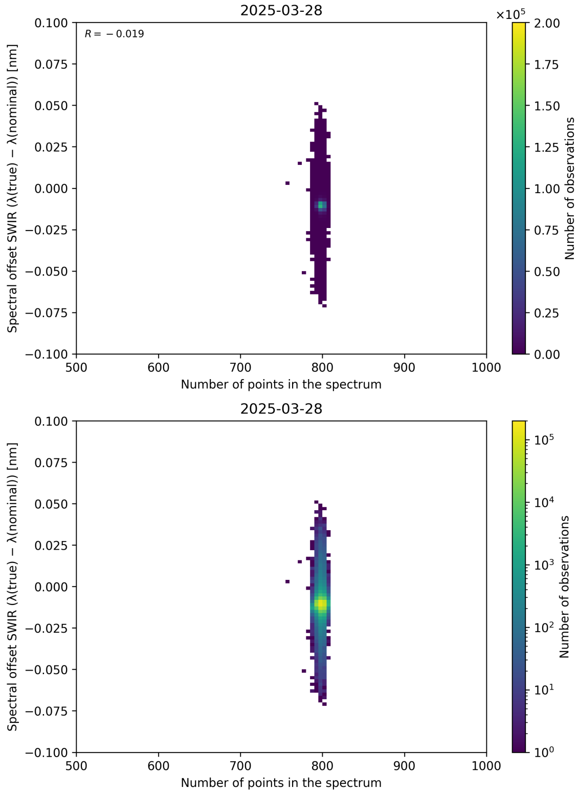
Figure 93: Scatter density plot of “Number of points in the spectrum” against “Spectral offset SWIR ( \lambda_{\text{true}} - \lambda_{\text{nominal}} )” for 2025-03-28 to 2025-03-29.
