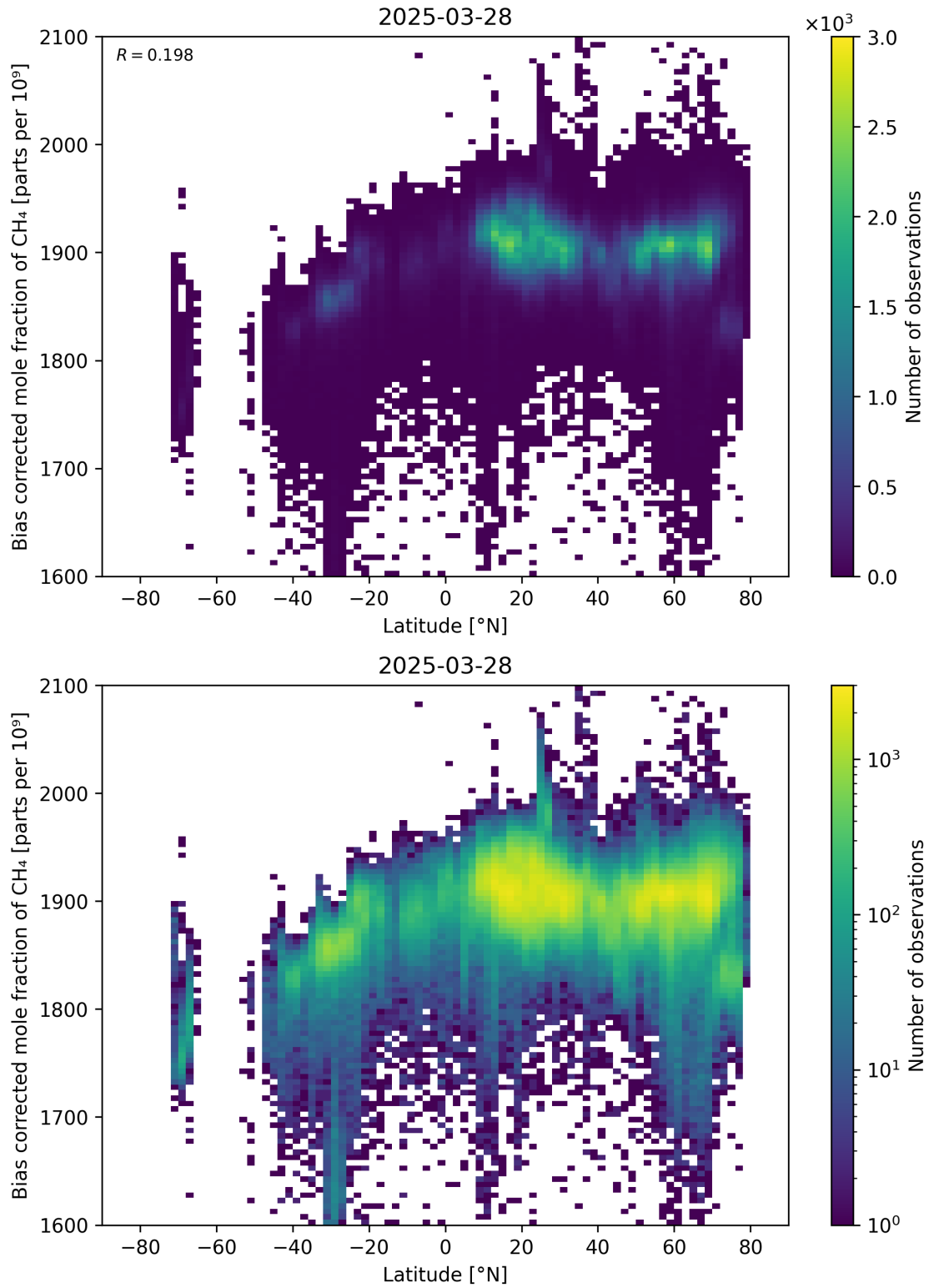
Figure 58: Scatter density plot of “Latitude” against “Bias corrected mole fraction of \text{CH}_4 ” for 2025-03-28 to 2025-03-29.
