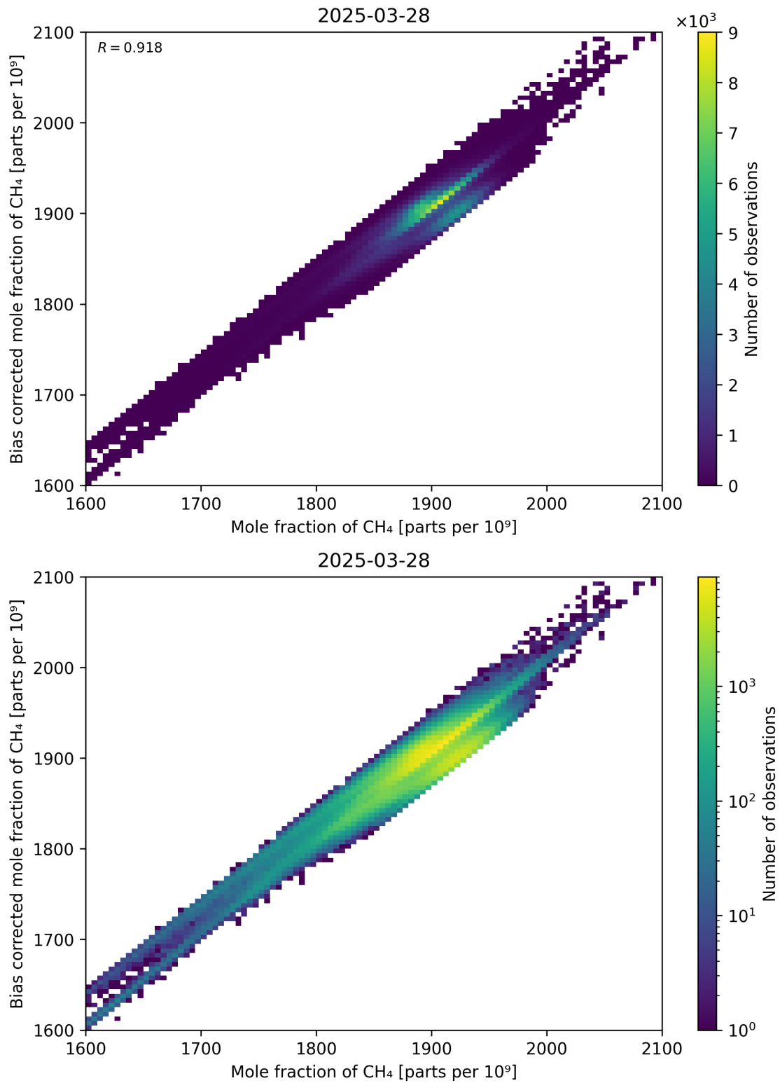
Figure 74: Scatter density plot of “Mole fraction of CH 4 ” against “Bias corrected mole fraction of CH 4 ” for 2025-03-28 to 2025-03-29.
