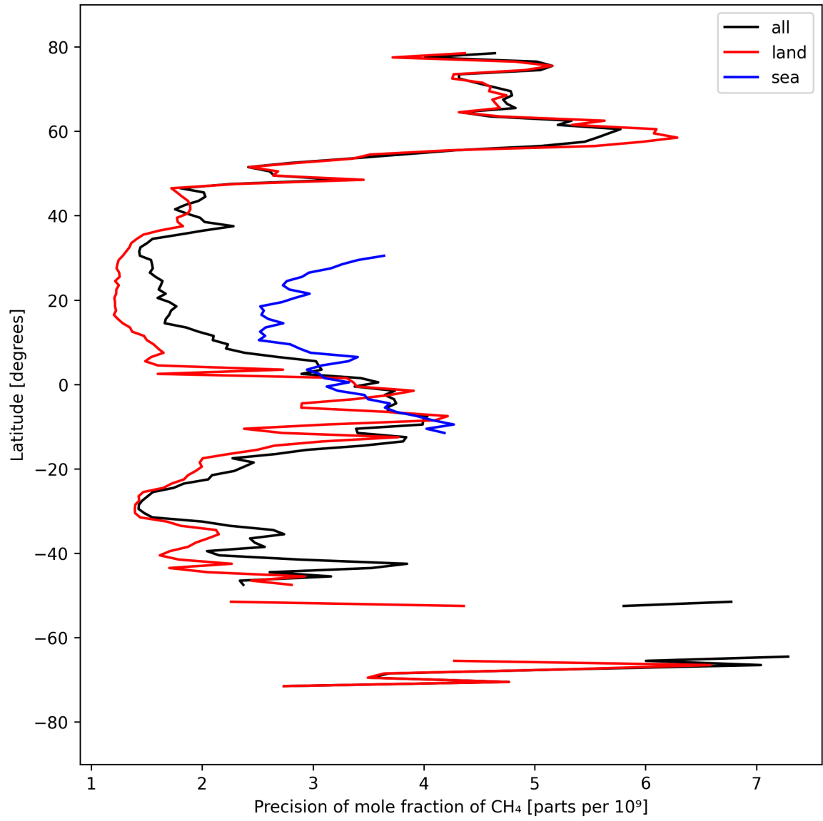
Figure 13: Zonal average of “Precision of mole fraction of CH 4 ” for 2025-03-28 to 2025-03-29.
