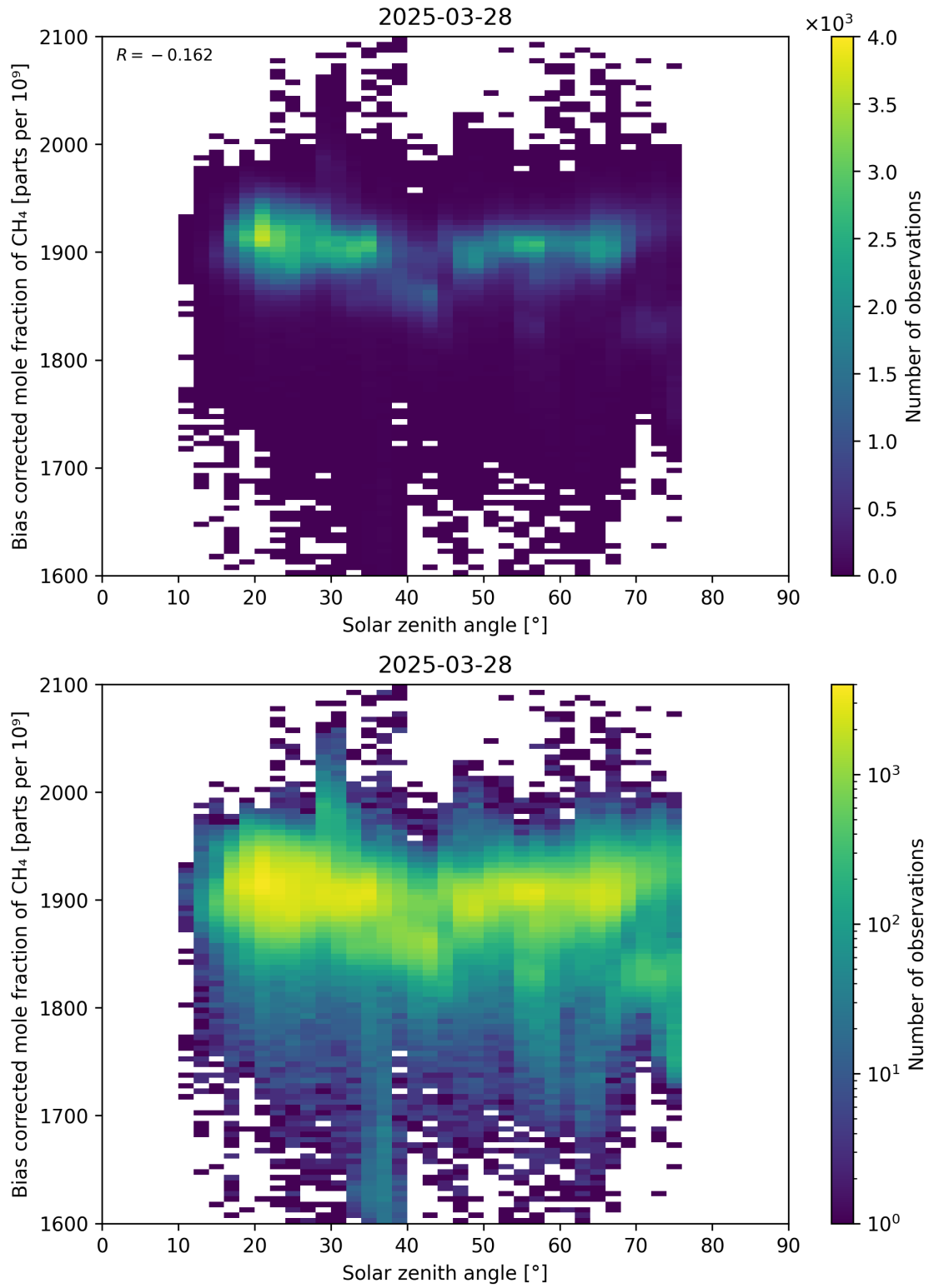
Figure 100: Scatter density plot of “Solar zenith angle” against “Bias corrected mole fraction of \text{CH}_4 ” for 2025-03-28 to 2025-03-29.
