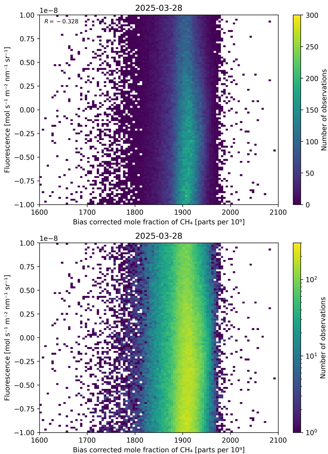
Figure 66: Scatter density plot of “Bias corrected mole fraction of \text{CH}_4 ” against “Fluorescence” for 2025-03-28 to 2025-03-29.
