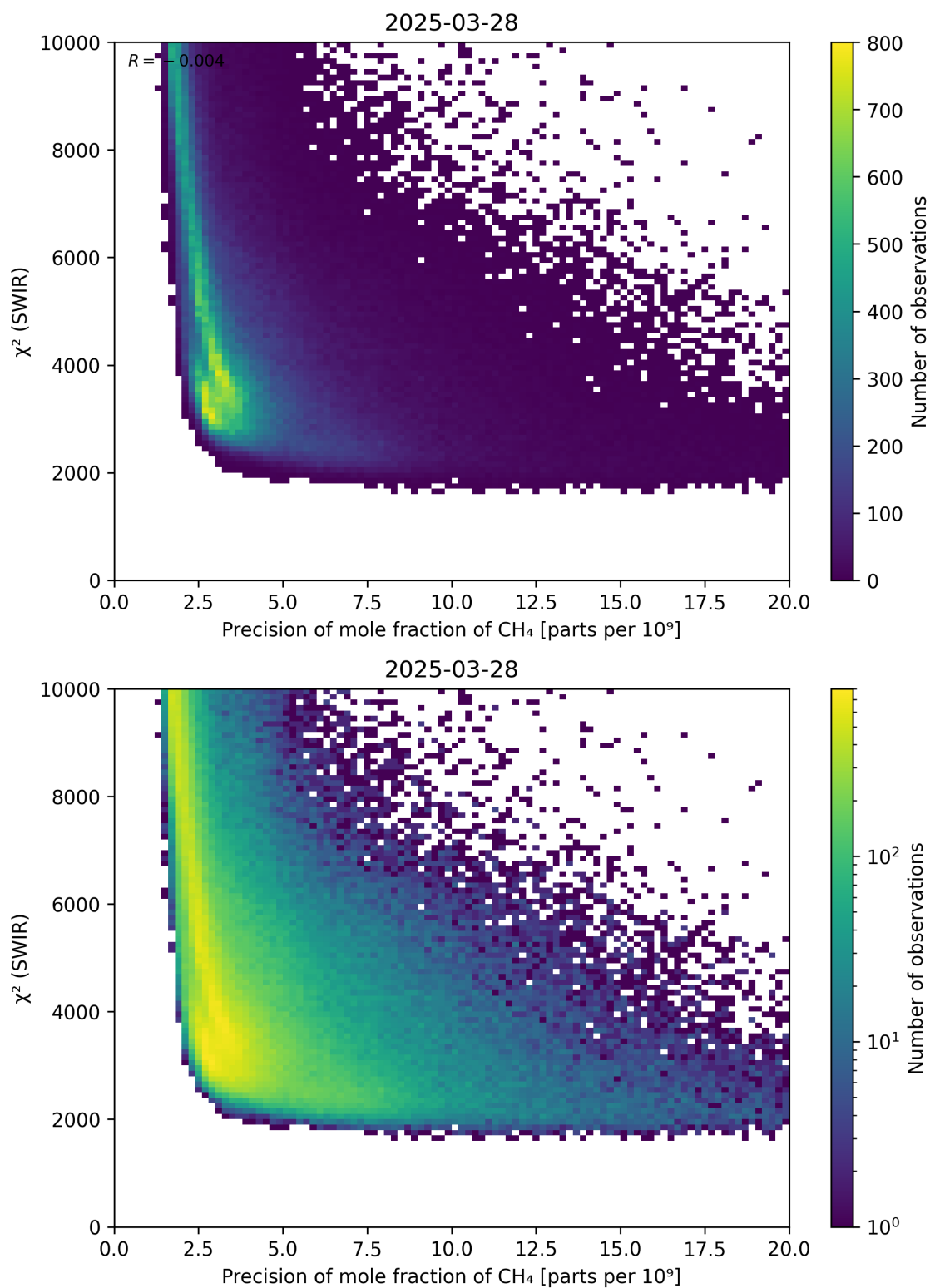
Figure 79: Scatter density plot of “Precision of mole fraction of \text{CH}_4 ” against “ \chi^2 (SWIR)” for 2025-03-28 to 2025-03-29.
