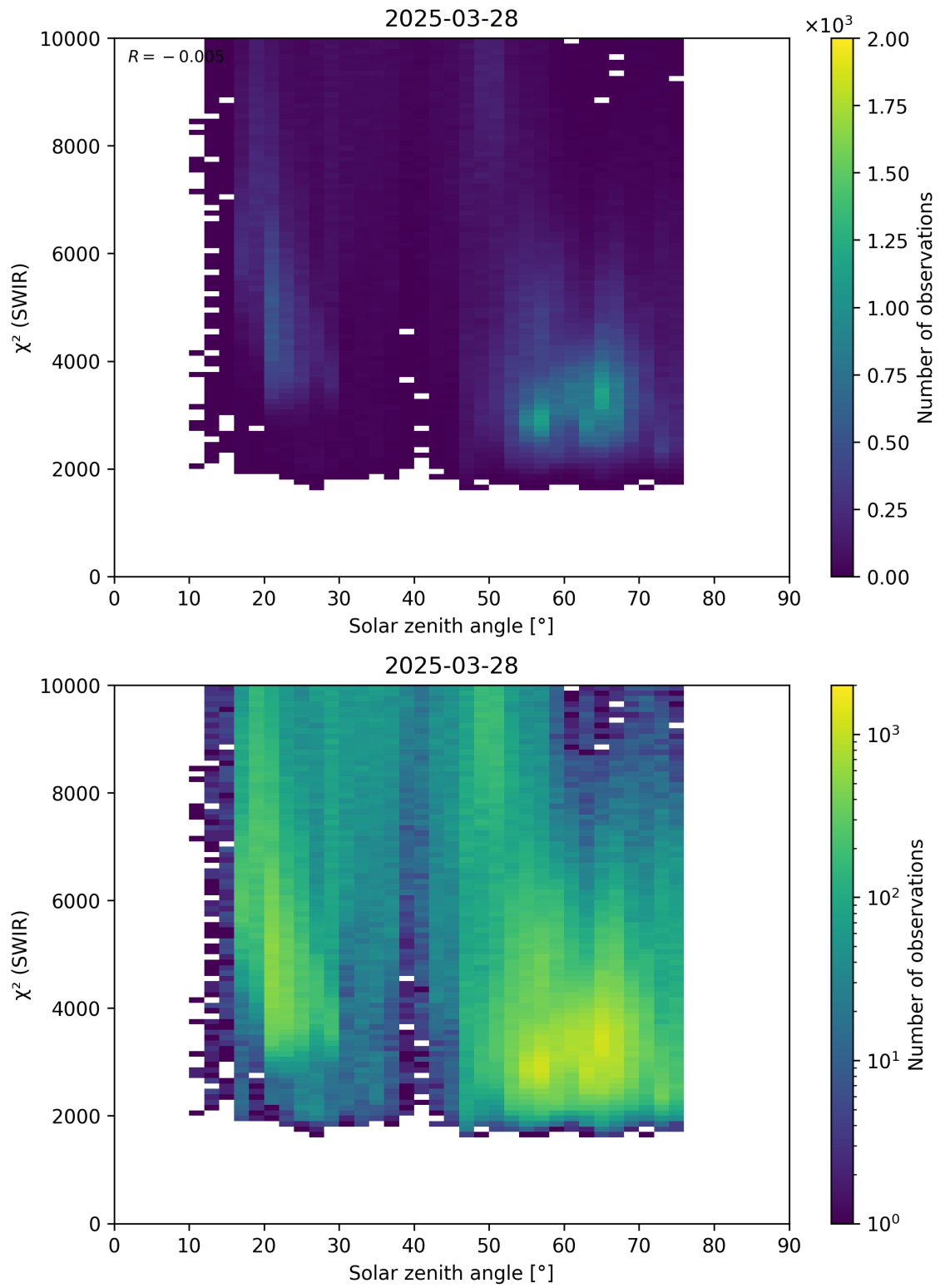
Figure 95: Scatter density plot of “Solar zenith angle” against “ \chi^2 (SWIR)” for 2025-03-28 to 2025-03-29.
