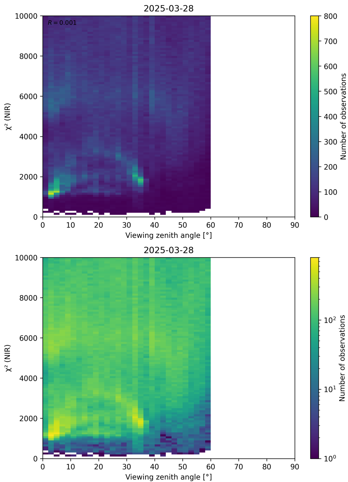
Figure 105: Scatter density plot of “Viewing zenith angle” against “ \chi^2 (NIR)” for 2025-03-28 to 2025-03-29.
