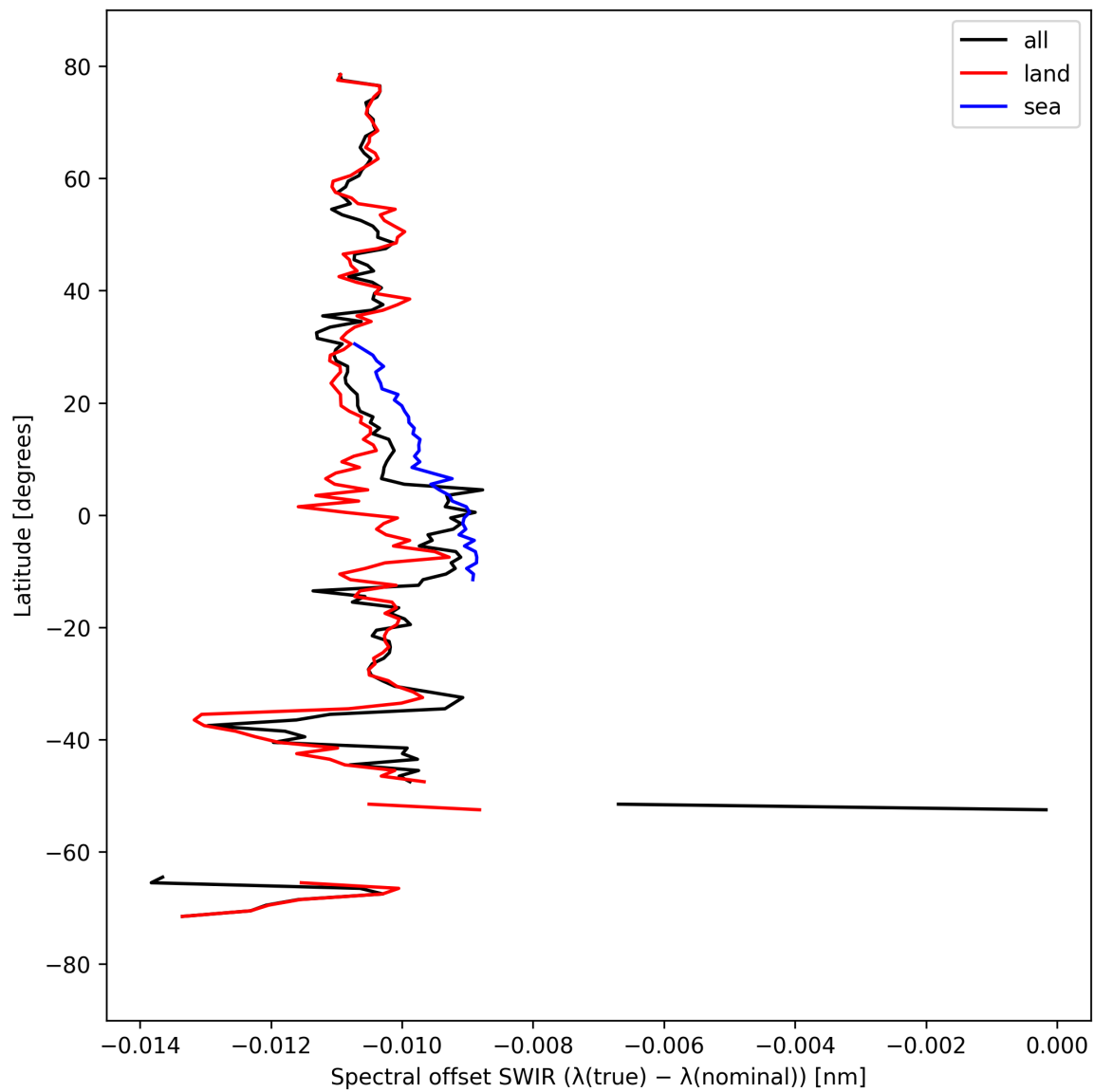
Figure 16: Zonal average of “Spectral offset SWIR ( \lambda_{\text{true}} - \lambda_{\text{nominal}} )” for 2025-03-28 to 2025-03-29.
