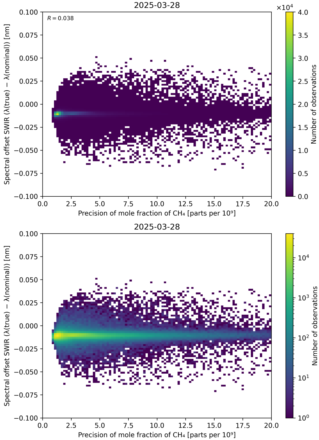
Figure 85: Scatter density plot of “Precision of mole fraction of \text{CH}_4 ” against “Spectral offset SWIR ( \lambda_{\text{true}} - \lambda_{\text{nominal}} )” for 2025-03-28 to 2025-03-29.
