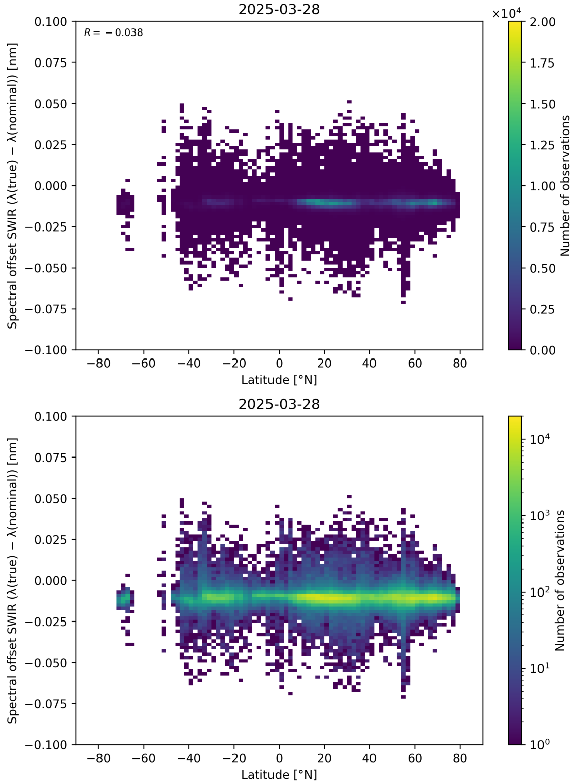
Figure 62: Scatter density plot of “Latitude” against “Spectral offset SWIR ( \lambda_{\text{true}} - \lambda_{\text{nominal}} )” for 2025-03-28 to 2025-03-29.
