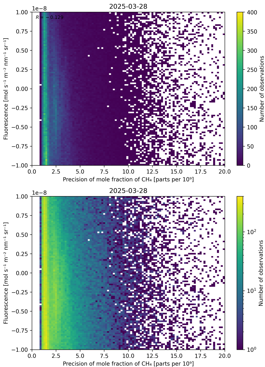
Figure 81: Scatter density plot of “Precision of mole fraction of CH 4 ” against “Fluorescence” for 2025-03-28 to 2025-03-29.
