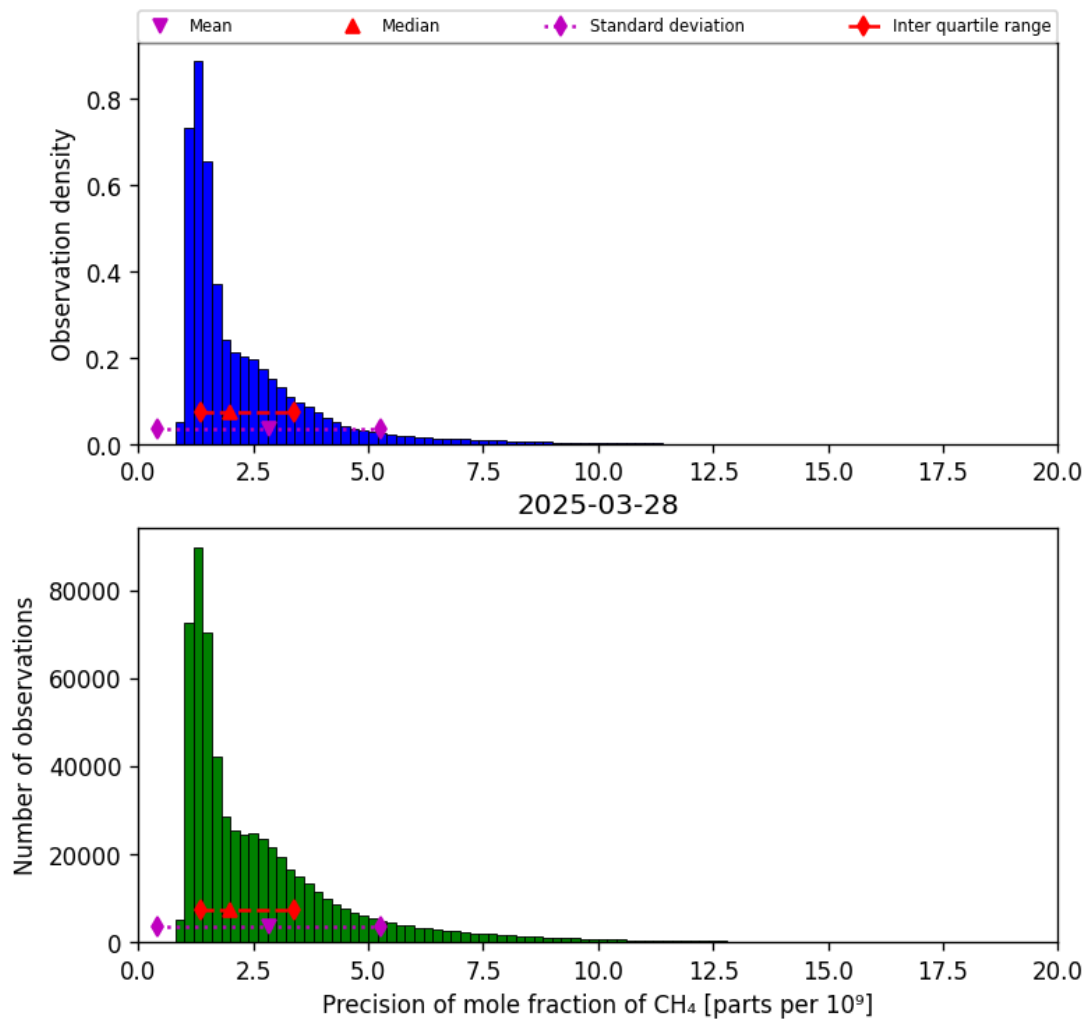
Figure 24: Histogram of “Precision of mole fraction of CH 4 ” for 2025-03-28 to 2025-03-29
