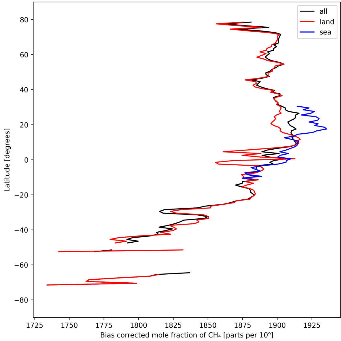
Figure 14: Zonal average of “Bias corrected mole fraction of \text{CH}_4 ” for 2025-03-28 to 2025-03-29.
