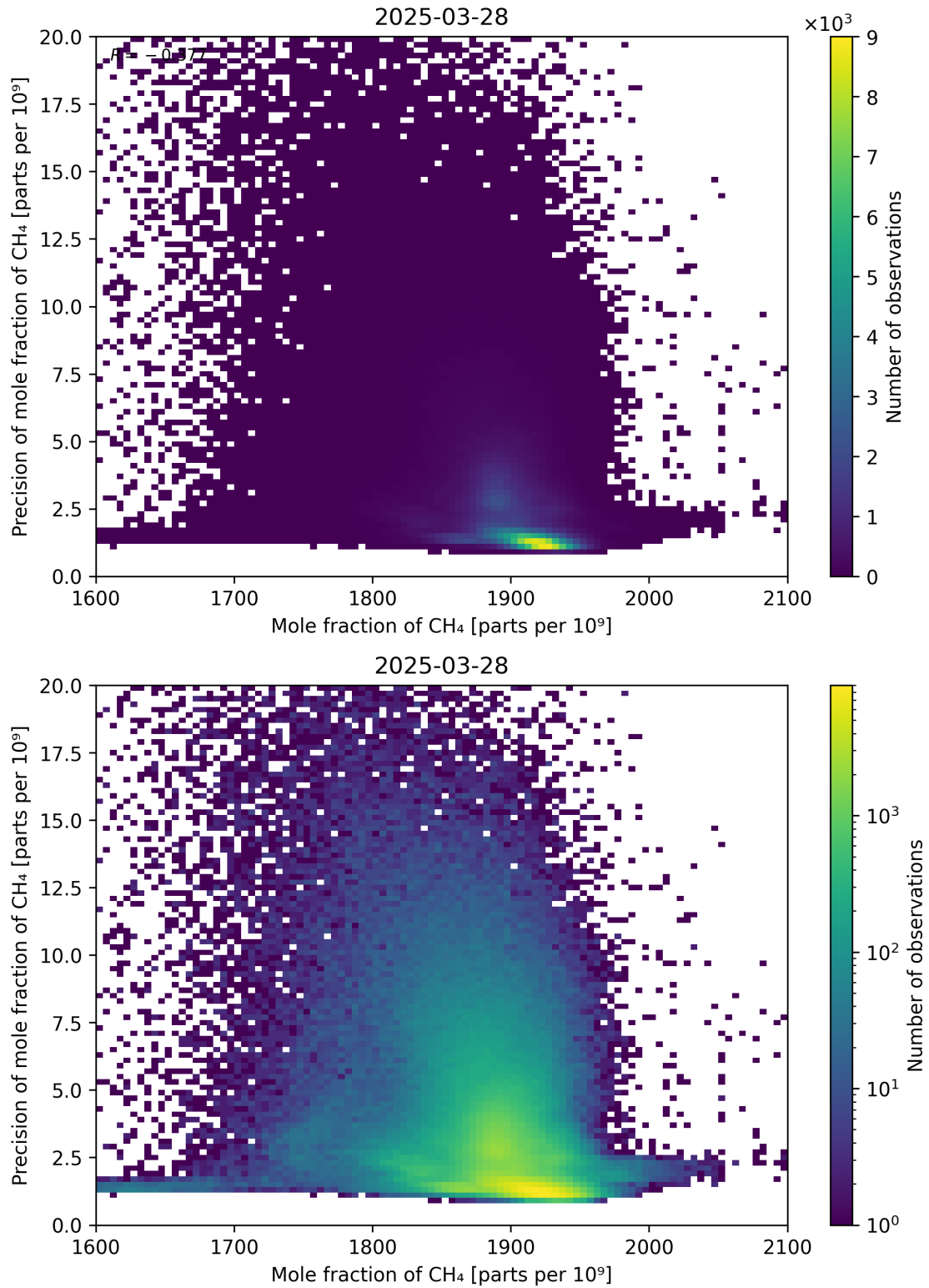
Figure 75: Scatter density plot of “Mole fraction of CH 4 ” against “Precision of mole fraction of CH 4 ” for 2025-03-28 to 2025-03-29.
