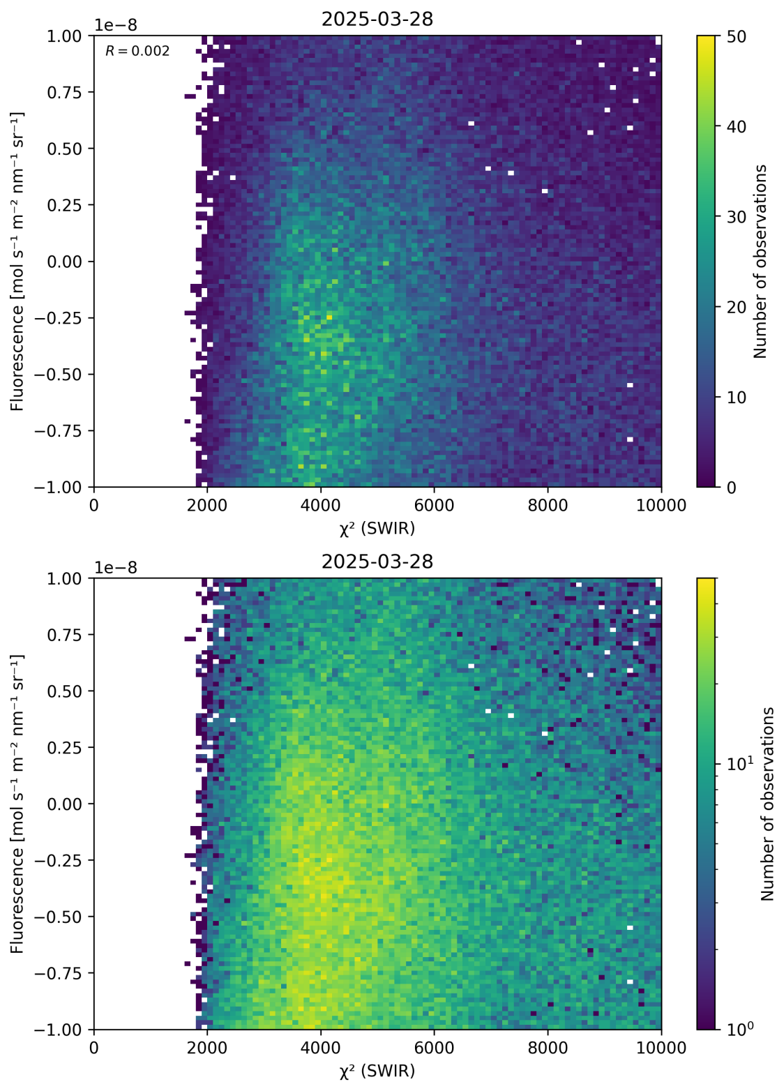
Figure 49: Scatter density plot of “ \chi^2 (SWIR)” against “Fluorescence” for 2025-03-28 to 2025-03-29.
