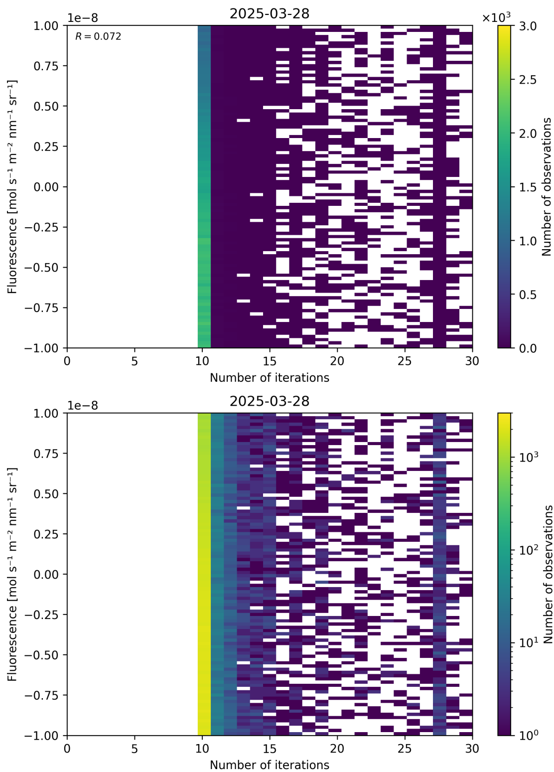
Figure 87: Scatter density plot of “Number of iterations” against “Fluorescence” for 2025-03-28 to 2025-03-29.
