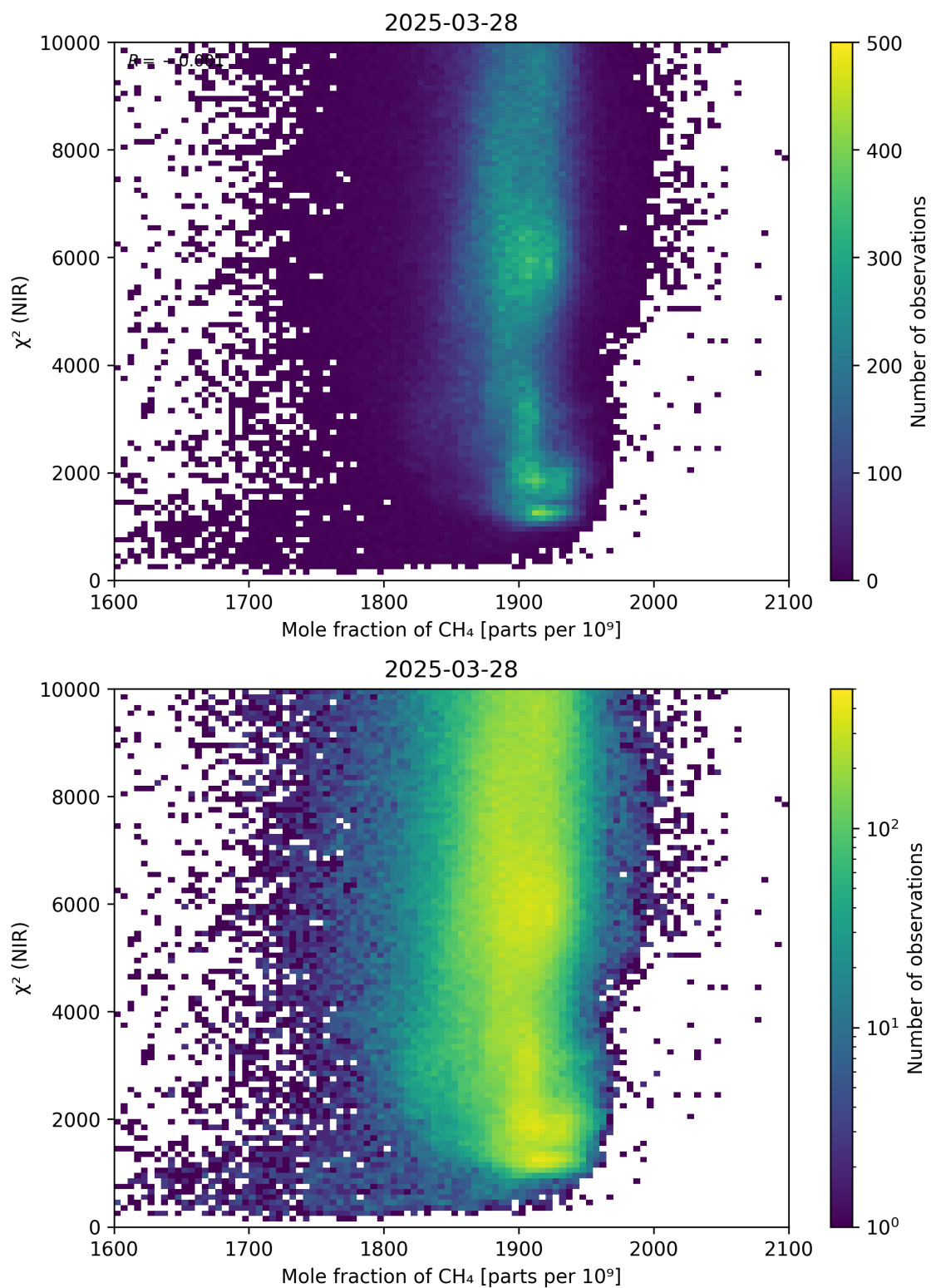
Figure 70: Scatter density plot of “Mole fraction of \text{CH}_4 ” against “ \chi^2 (NIR)” for 2025-03-28 to 2025-03-29.
