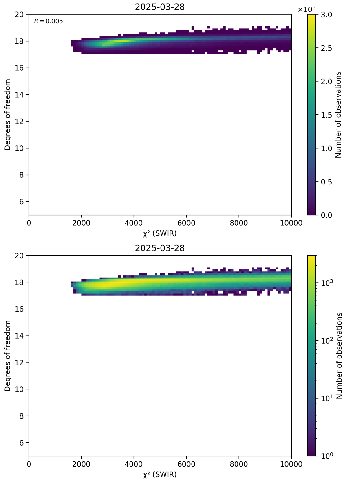
Figure 48: Scatter density plot of “ \chi^2 (SWIR)” against “Degrees of freedom” for 2025-03-28 to 2025-03-29.
