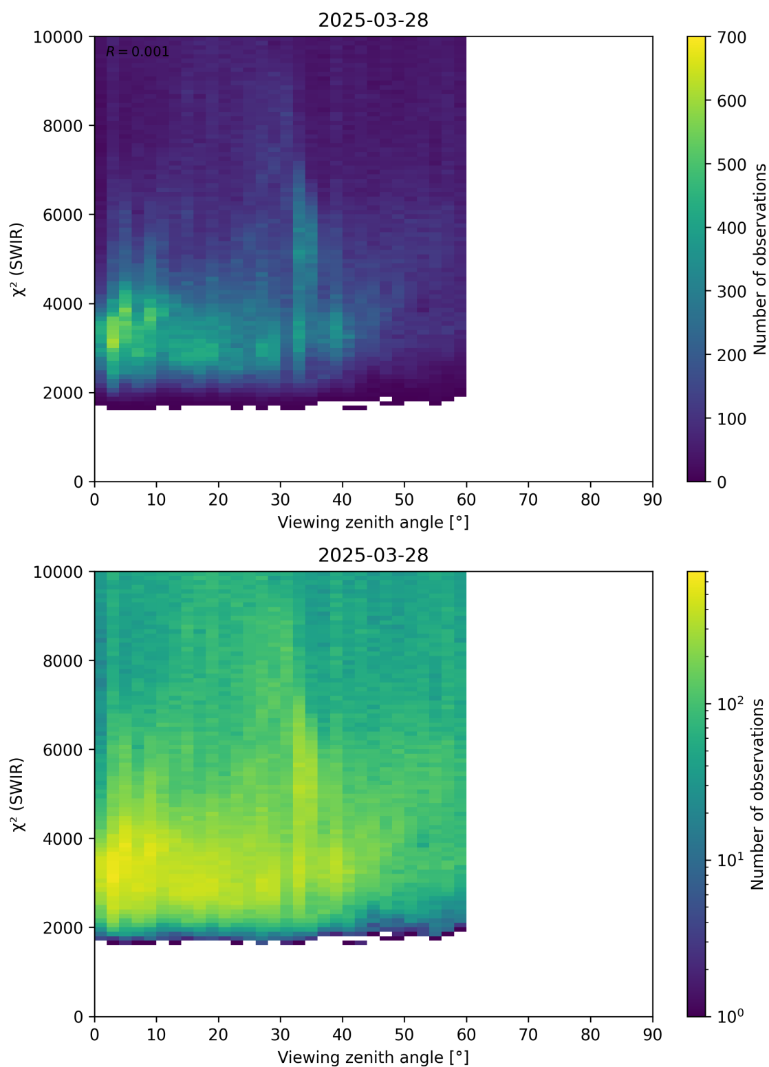
Figure 106: Scatter density plot of “Viewing zenith angle” against “ \chi^2 (SWIR)” for 2025-03-28 to 2025-03-29.
