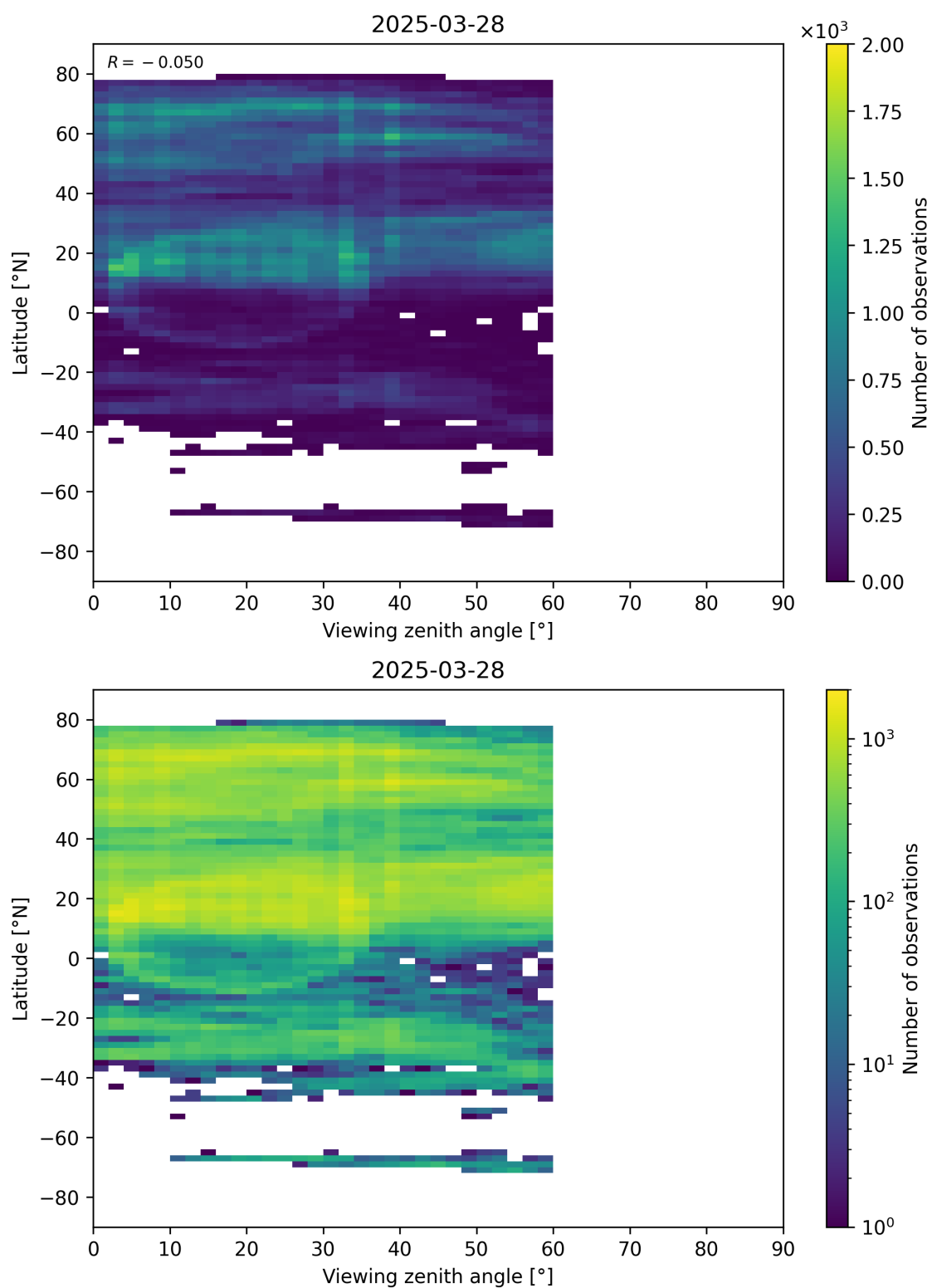
Figure 109: Scatter density plot of “Viewing zenith angle” against “Latitude” for 2025-03-28 to 2025-03-29.
