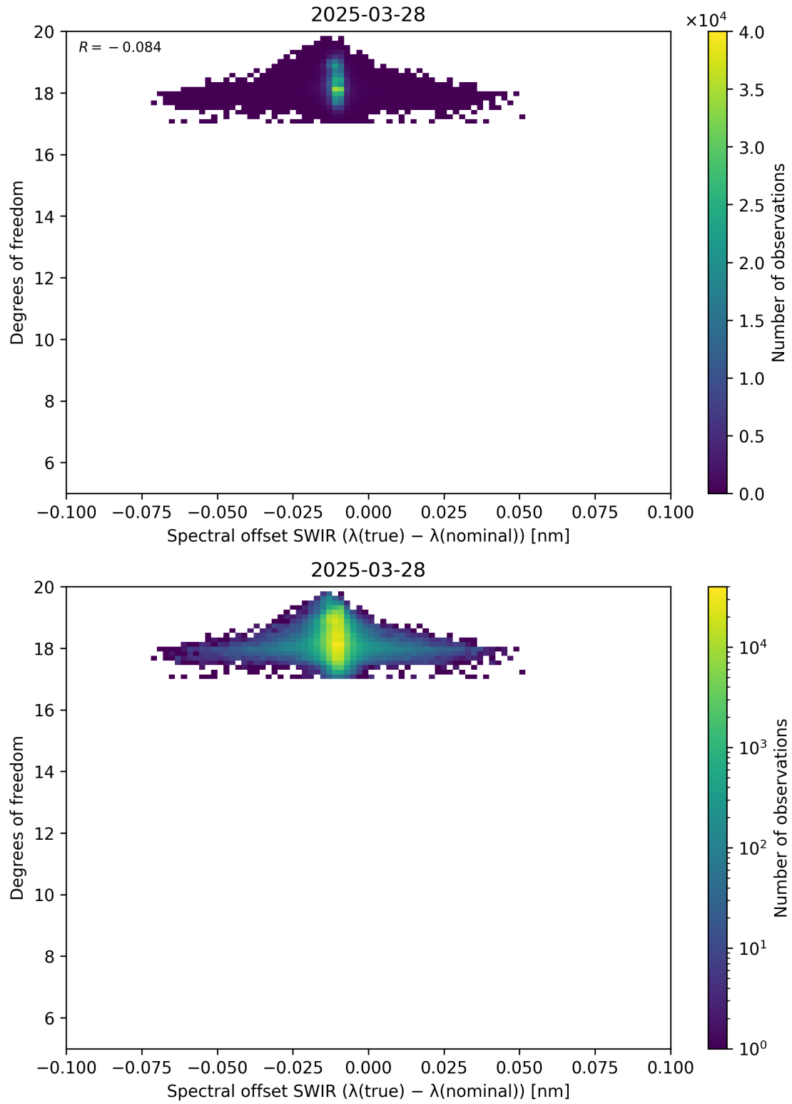
Figure 119: Scatter density plot of “Spectral offset SWIR ( \lambda_{\text{true}} - \lambda_{\text{nominal}} )” against “Degrees of freedom” for 2025-03-28 to 2025-03-29.
