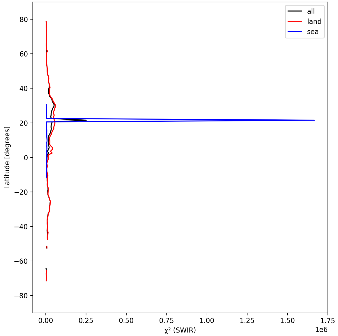
Figure 17: Zonal average of “ \chi^2 (SWIR)” for 2025-03-28 to 2025-03-29.
