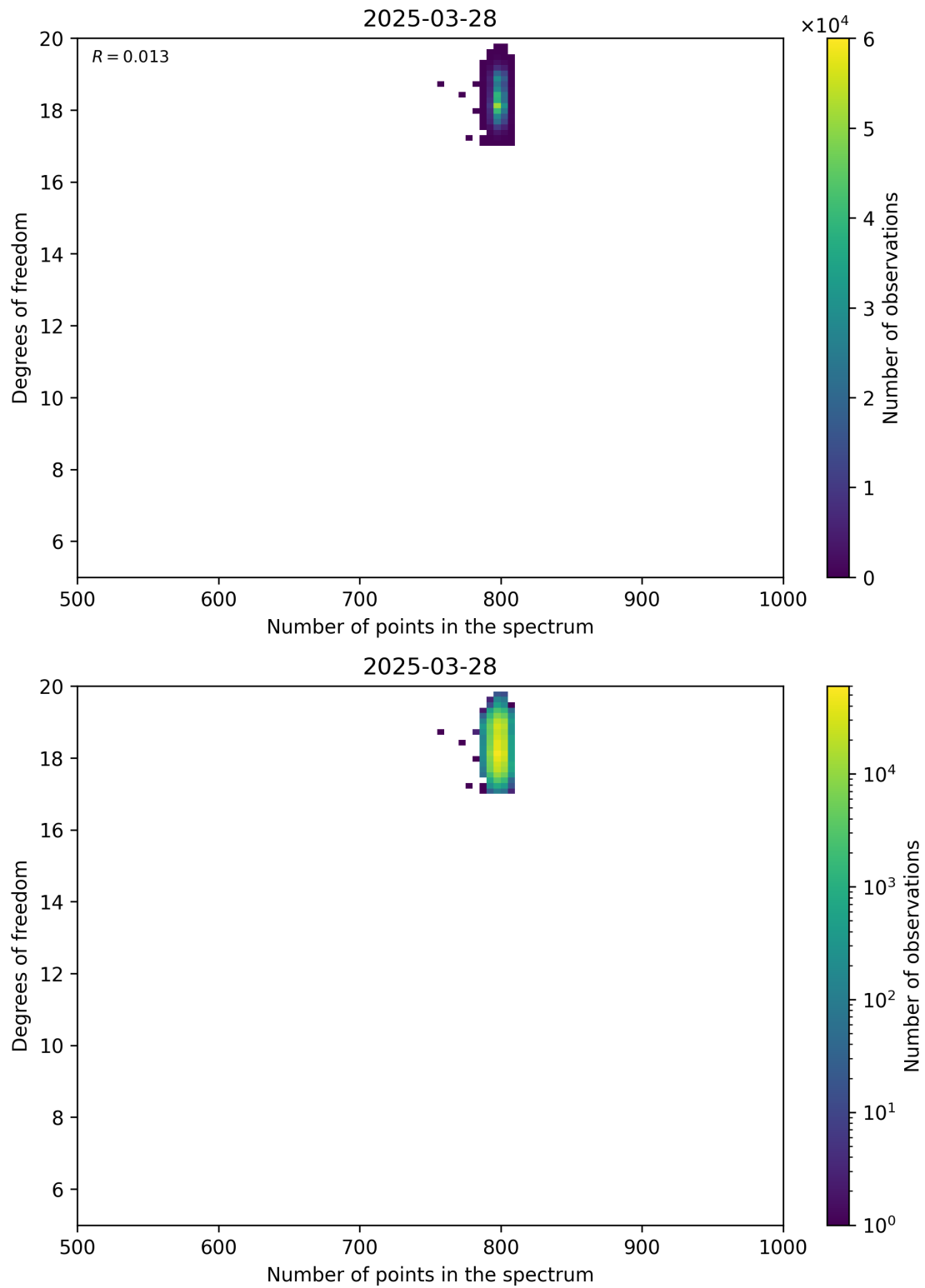
Figure 90: Scatter density plot of “Number of points in the spectrum” against “Degrees of freedom” for 2025-03-28 to 2025-03-29.
