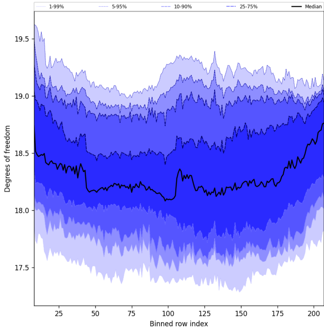
Figure 41: Along track statistics of “Degrees of freedom” for 2025-03-28 to 2025-03-29
