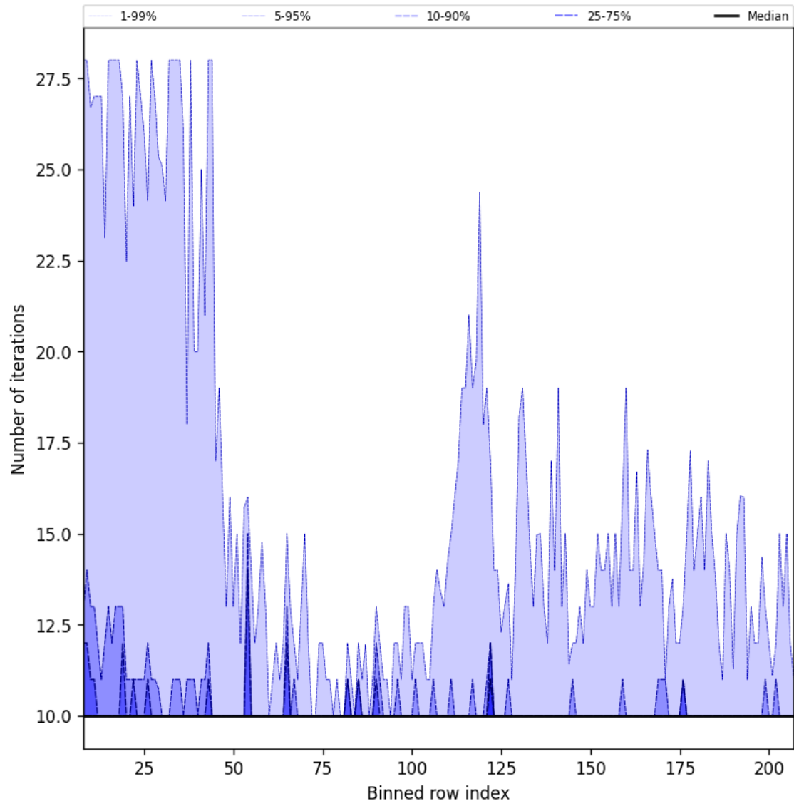
Figure 42: Along track statistics of “Number of iterations” for 2025-03-28 to 2025-03-29
