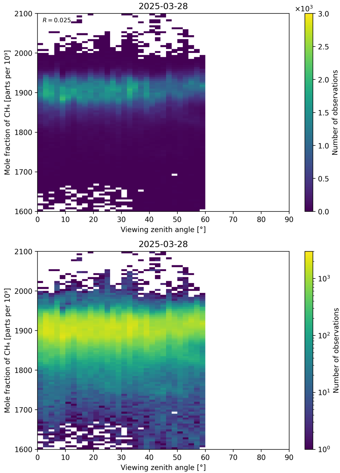
Figure 110: Scatter density plot of “Viewing zenith angle” against “Mole fraction of CH 4 ” for 2025-03-28 to 2025-03-29.
