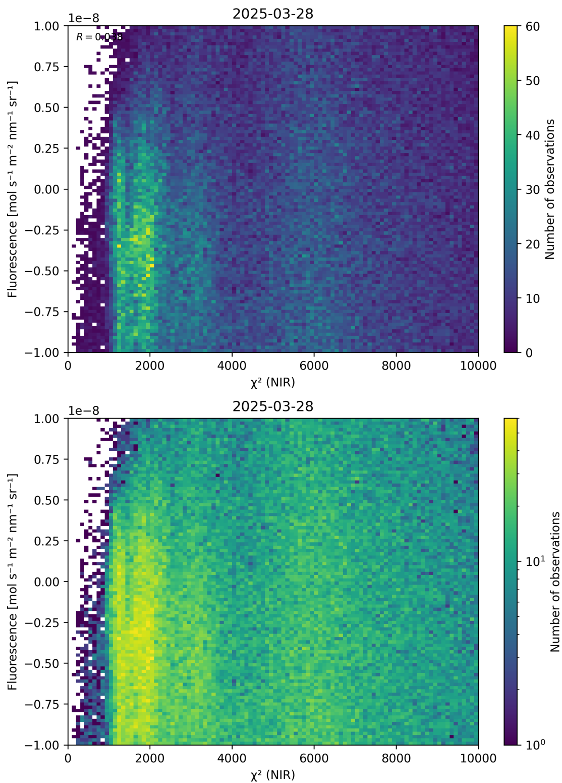
Figure 45: Scatter density plot of “ \chi^2 (NIR)” against “Fluorescence” for 2025-03-28 to 2025-03-29.
