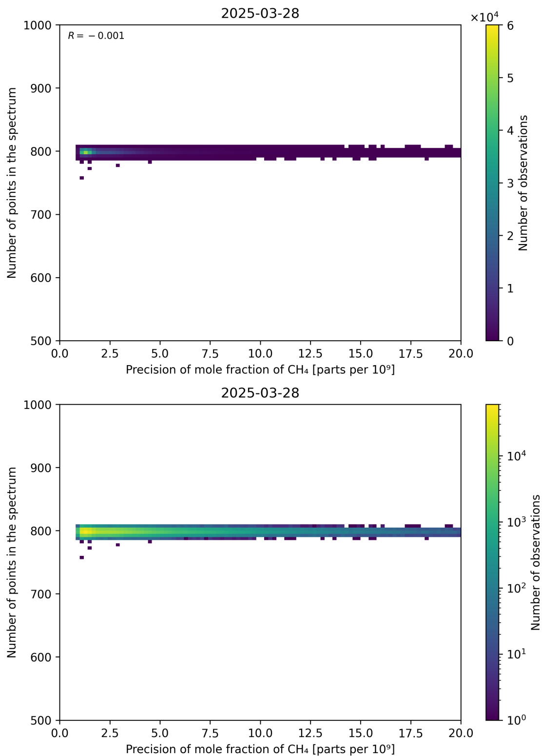
Figure 84: Scatter density plot of “Precision of mole fraction of CH 4 ” against “Number of points in the spectrum” for 2025-03-28 to 2025-03-29.
