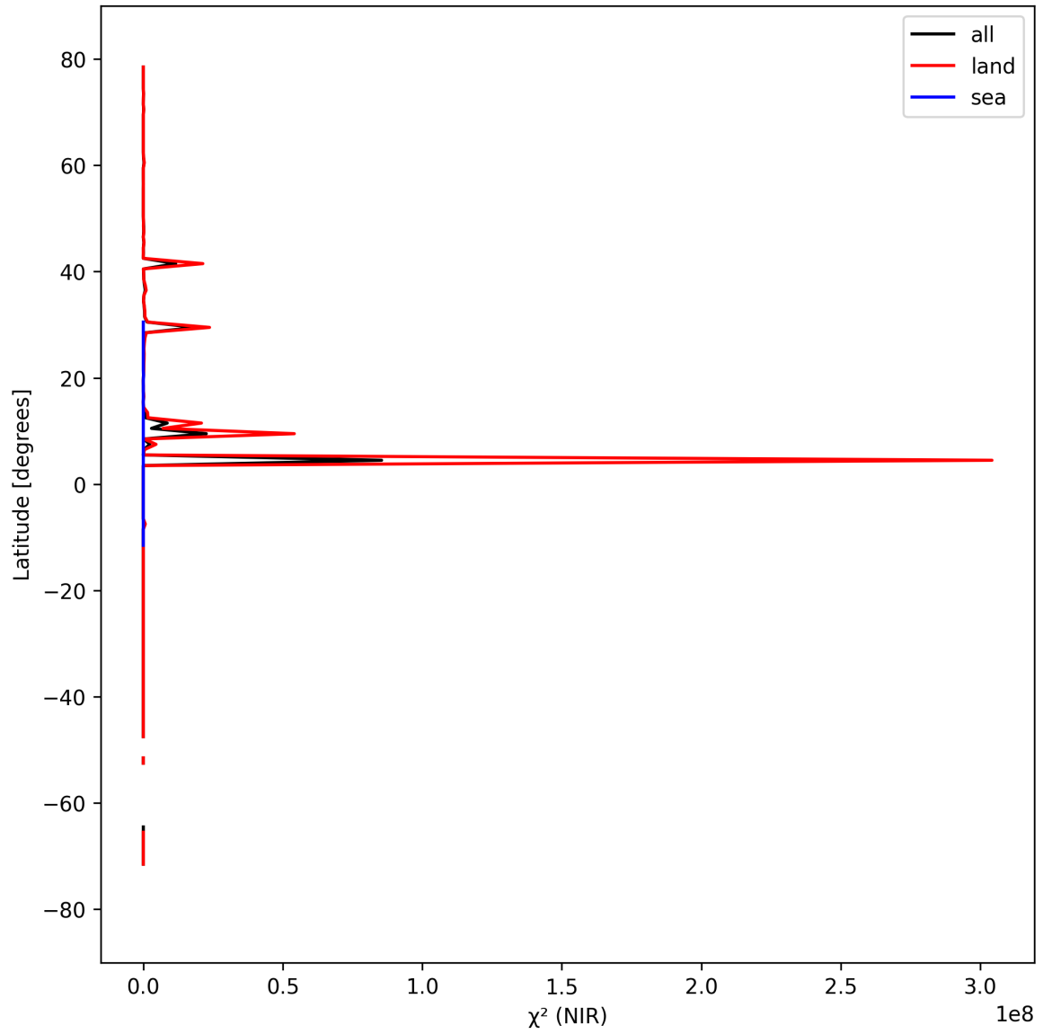
Figure 18: Zonal average of “ \chi^2 (NIR)” for 2025-03-28 to 2025-03-29.
