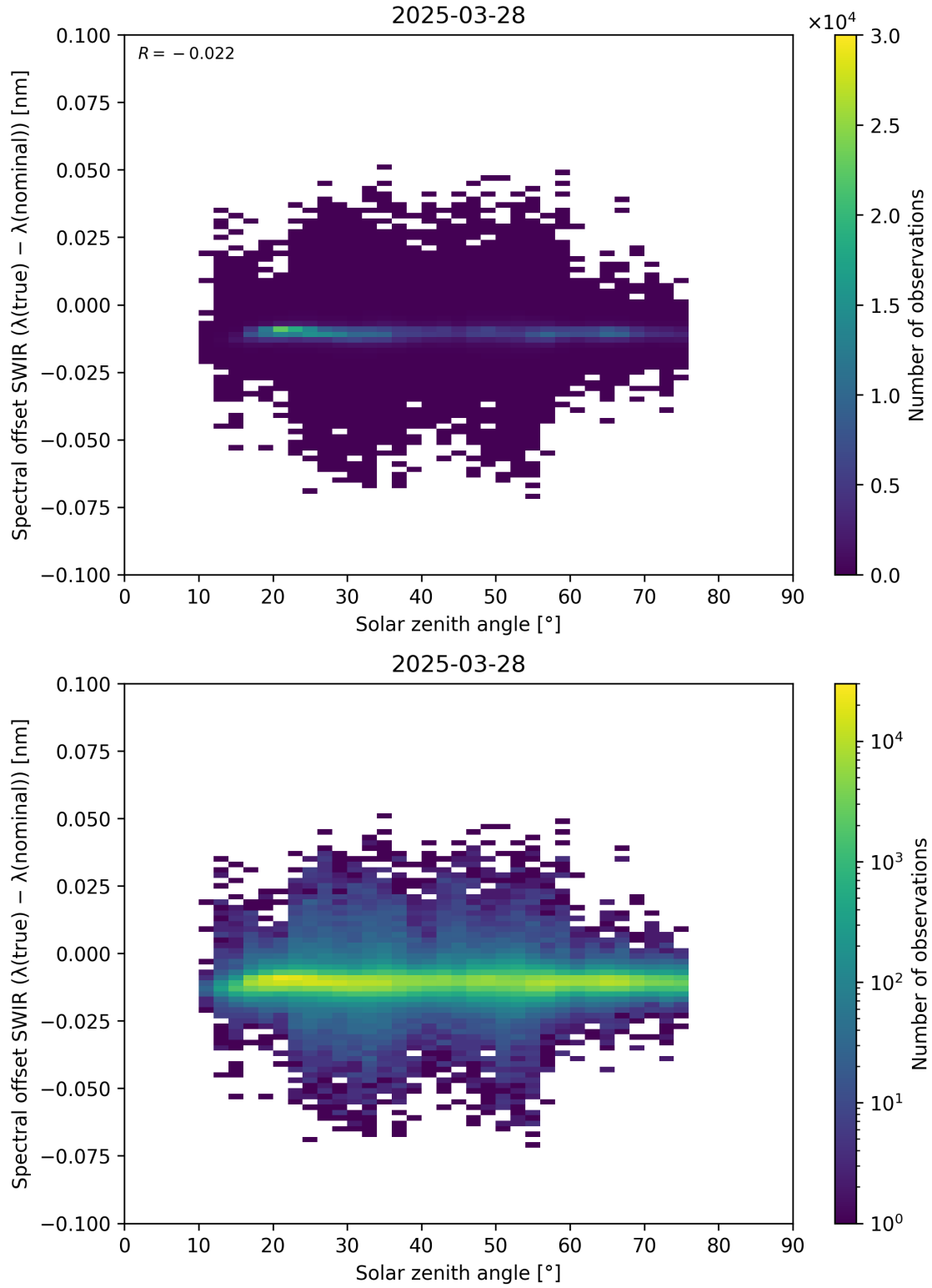
Figure 104: Scatter density plot of “Solar zenith angle” against “Spectral offset SWIR ( \lambda_{\text{true}} - \lambda_{\text{nominal}} )” for 2025-03-28 to 2025-03-29.
