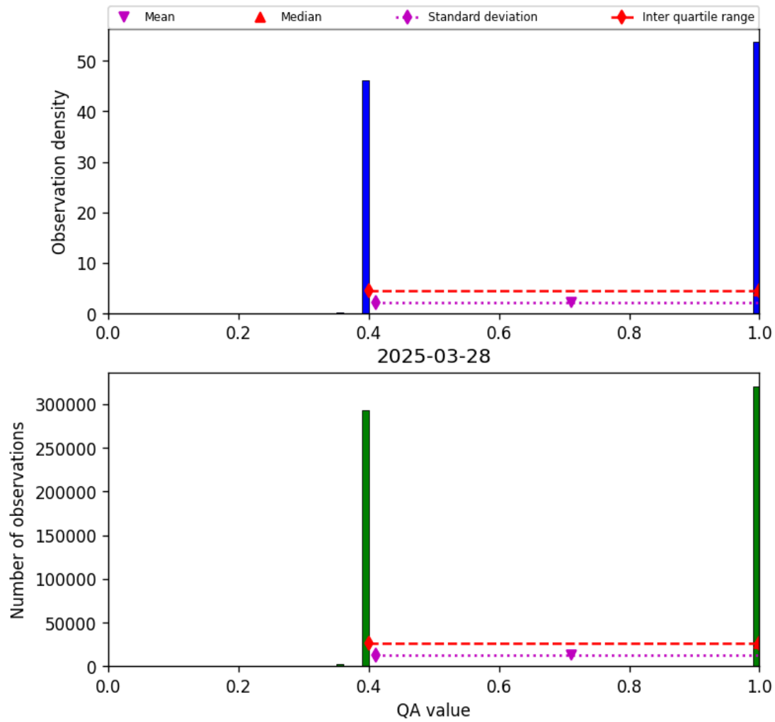
Figure 22: Histogram of “QA value” for 2025-03-28 to 2025-03-29
