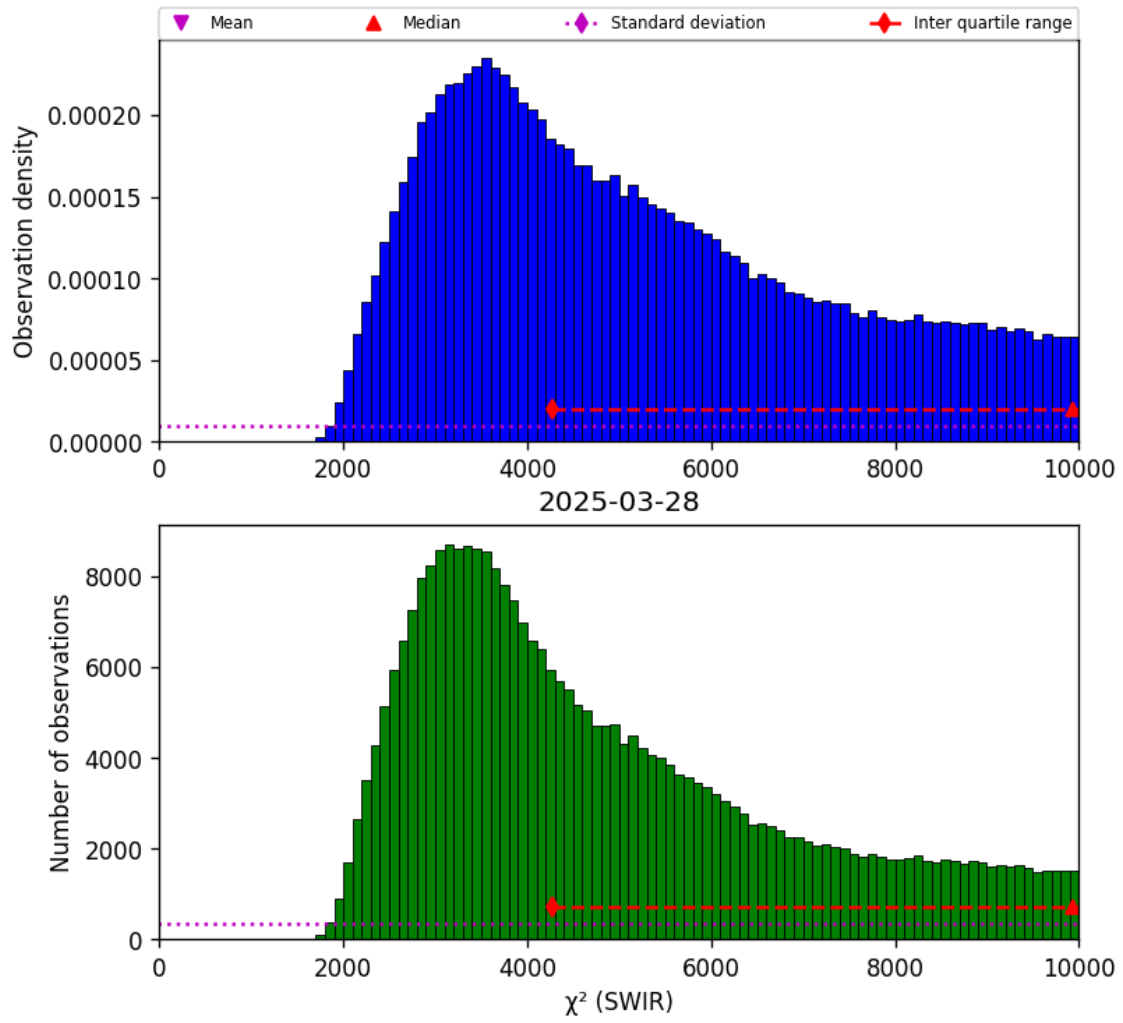
Figure 28: Histogram of “ \chi^2 (SWIR)” for 2025-03-28 to 2025-03-29
