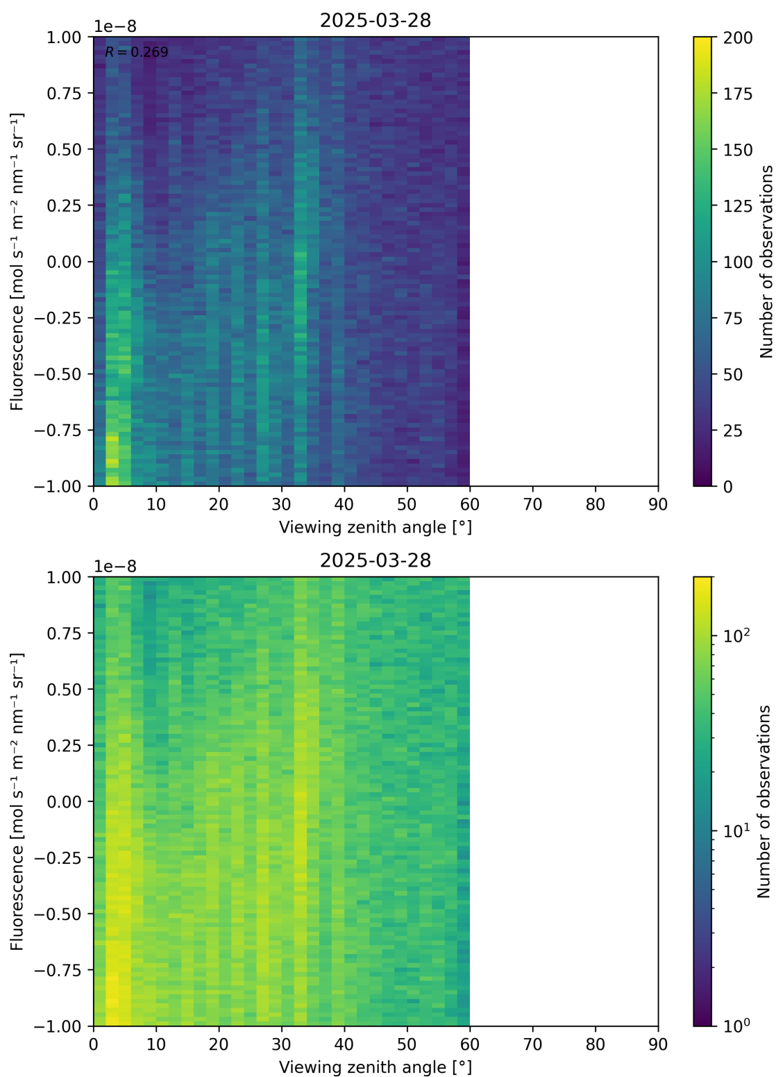
Figure 108: Scatter density plot of “Viewing zenith angle” against “Fluorescence” for 2025-03-28 to 2025-03-29.
