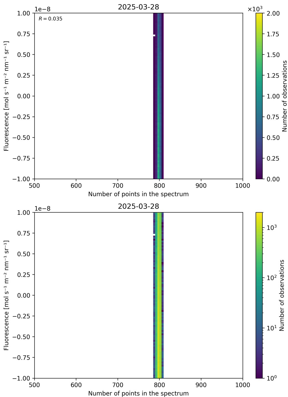
Figure 91: Scatter density plot of “Number of points in the spectrum” against “Fluorescence” for 2025-03-28 to 2025-03-29.
