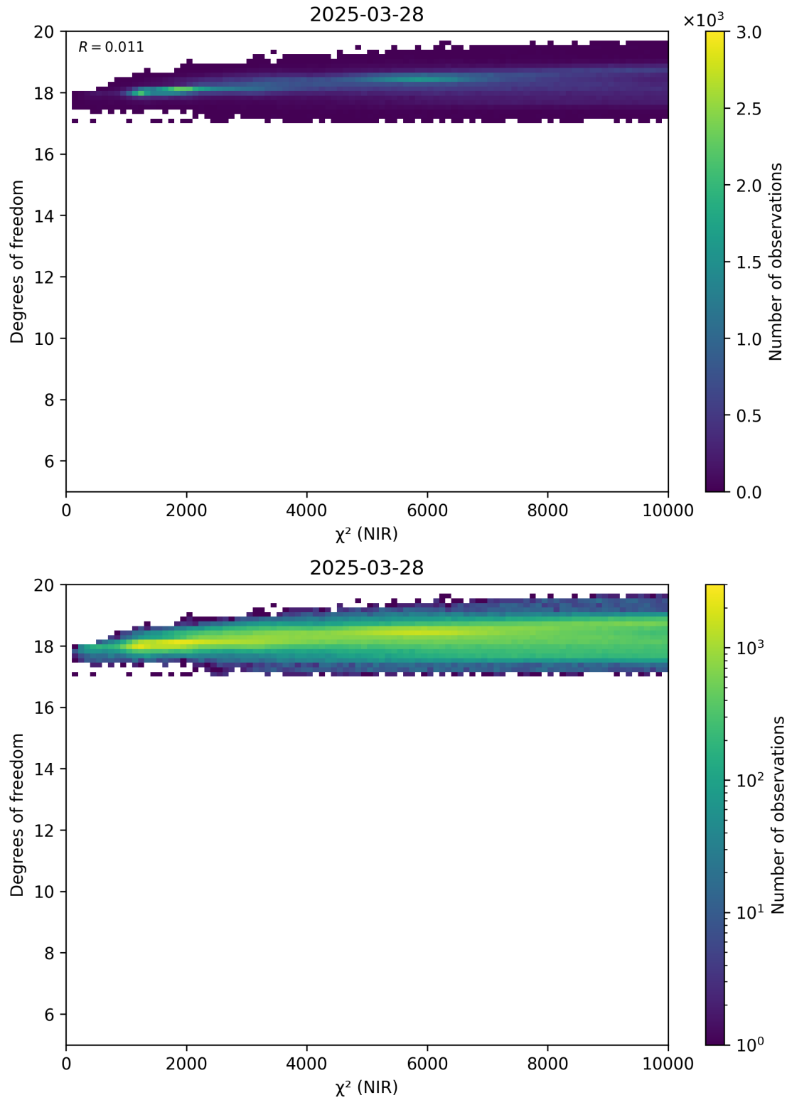
Figure 44: Scatter density plot of “ \chi^2 (NIR)” against “Degrees of freedom” for 2025-03-28 to 2025-03-29.
