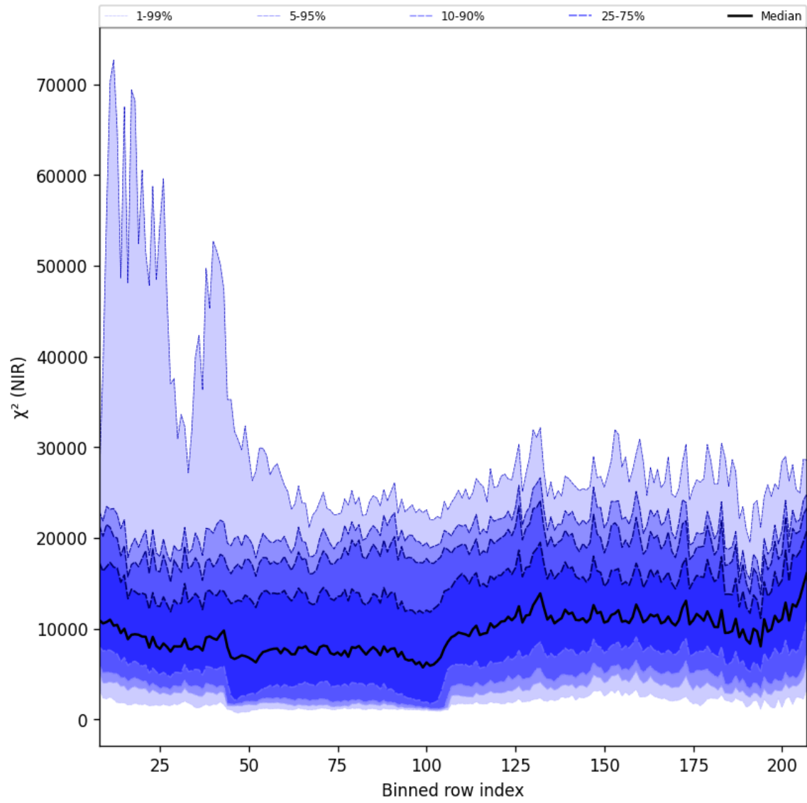
Figure 40: Along track statistics of “ \chi^2 (NIR)” for 2025-03-28 to 2025-03-29
