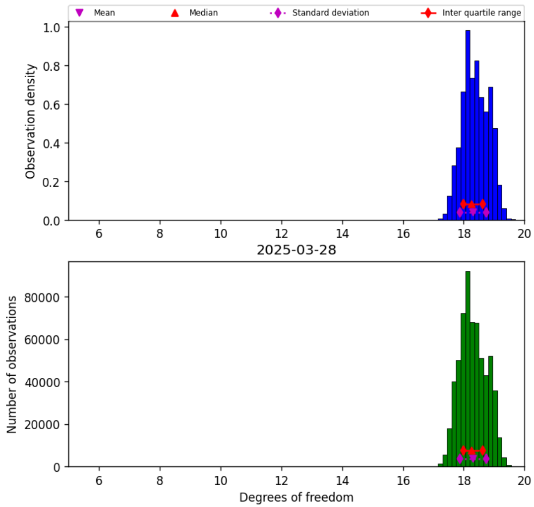
Figure 30: Histogram of “Degrees of freedom” for 2025-03-28 to 2025-03-29
