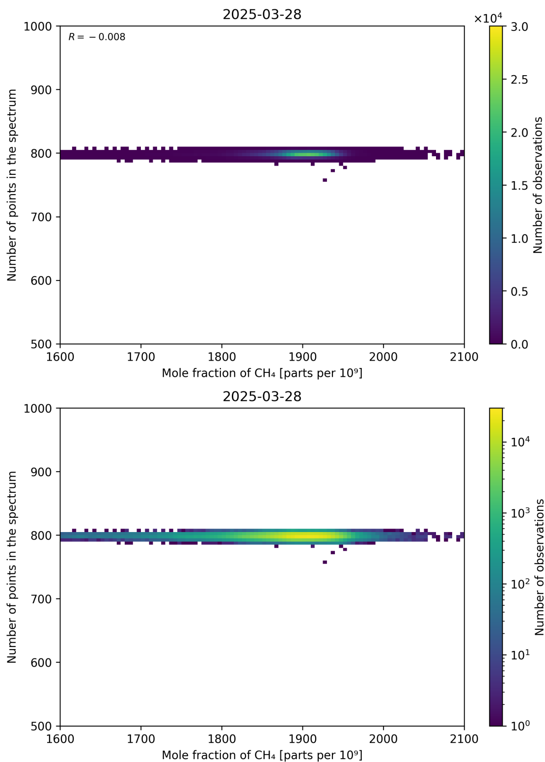
Figure 77: Scatter density plot of “Mole fraction of CH 4 ” against “Number of points in the spectrum” for 2025-03-28 to 2025-03-29.
