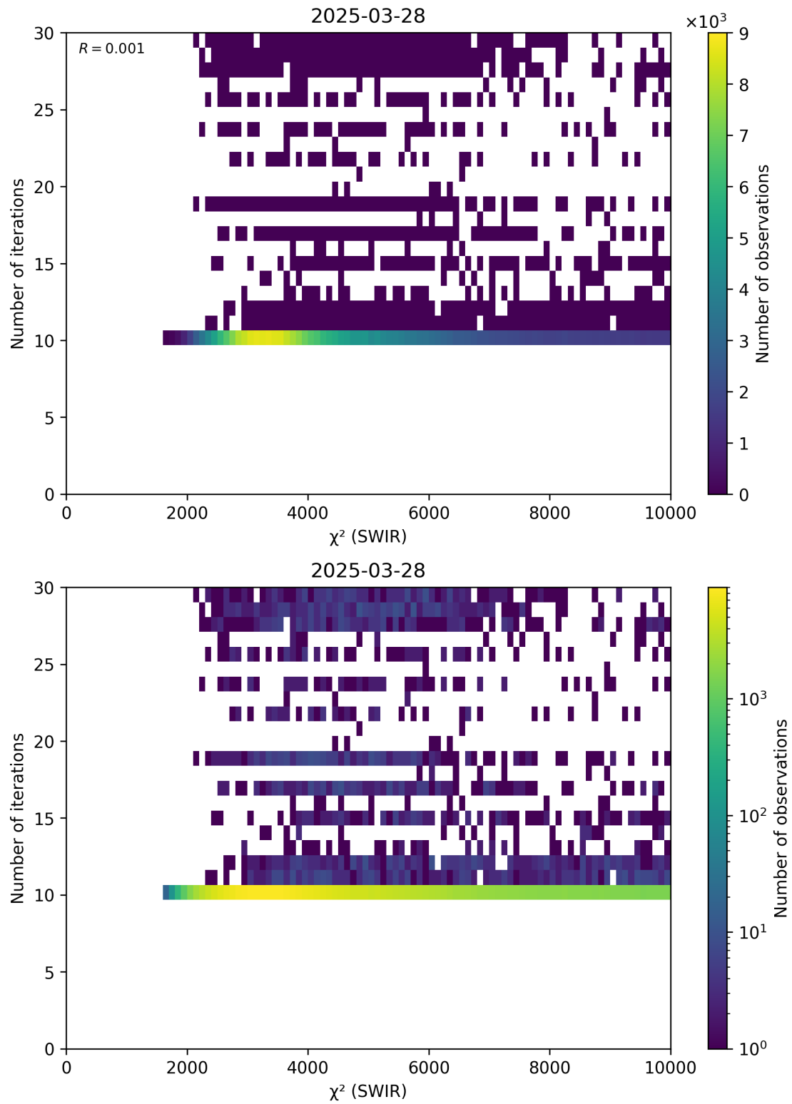
Figure 50: Scatter density plot of “ \chi^2 (SWIR)” against “Number of iterations” for 2025-03-28 to 2025-03-29.
