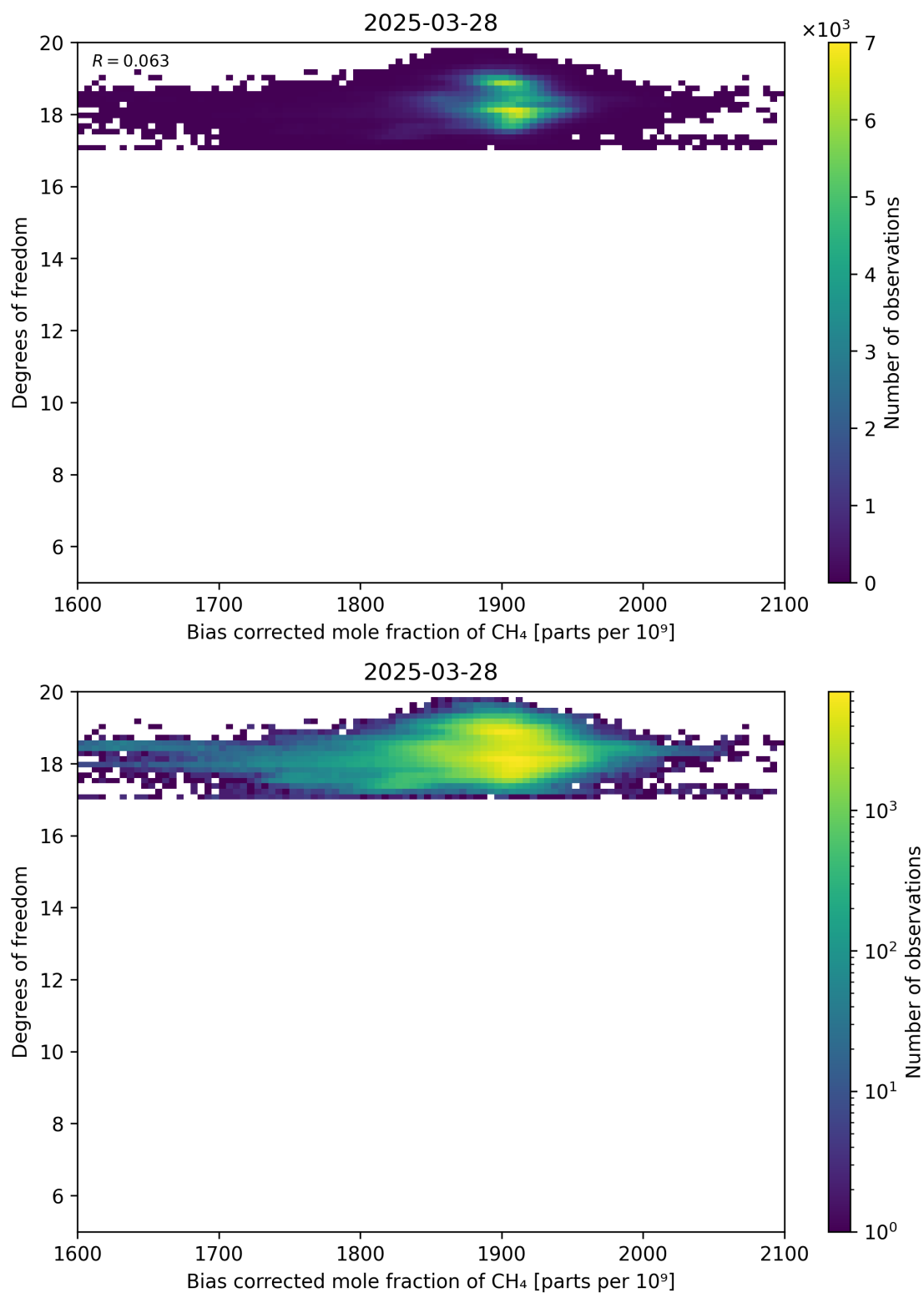
Figure 65: Scatter density plot of “Bias corrected mole fraction of CH 4 ” against “Degrees of freedom” for 2025-03-28 to 2025-03-29.
