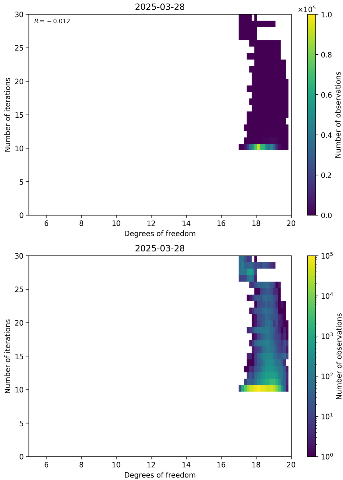
Figure 52: Scatter density plot of “Degrees of freedom” against “Number of iterations” for 2025-03-28 to 2025-03-29.
