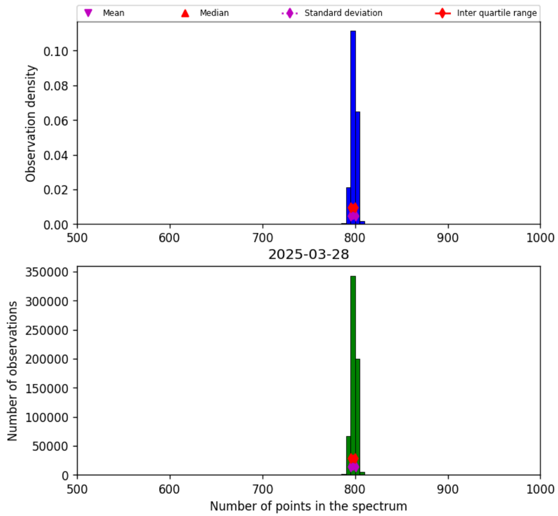
Figure 26: Histogram of “Number of points in the spectrum” for 2025-03-28 to 2025-03-29
