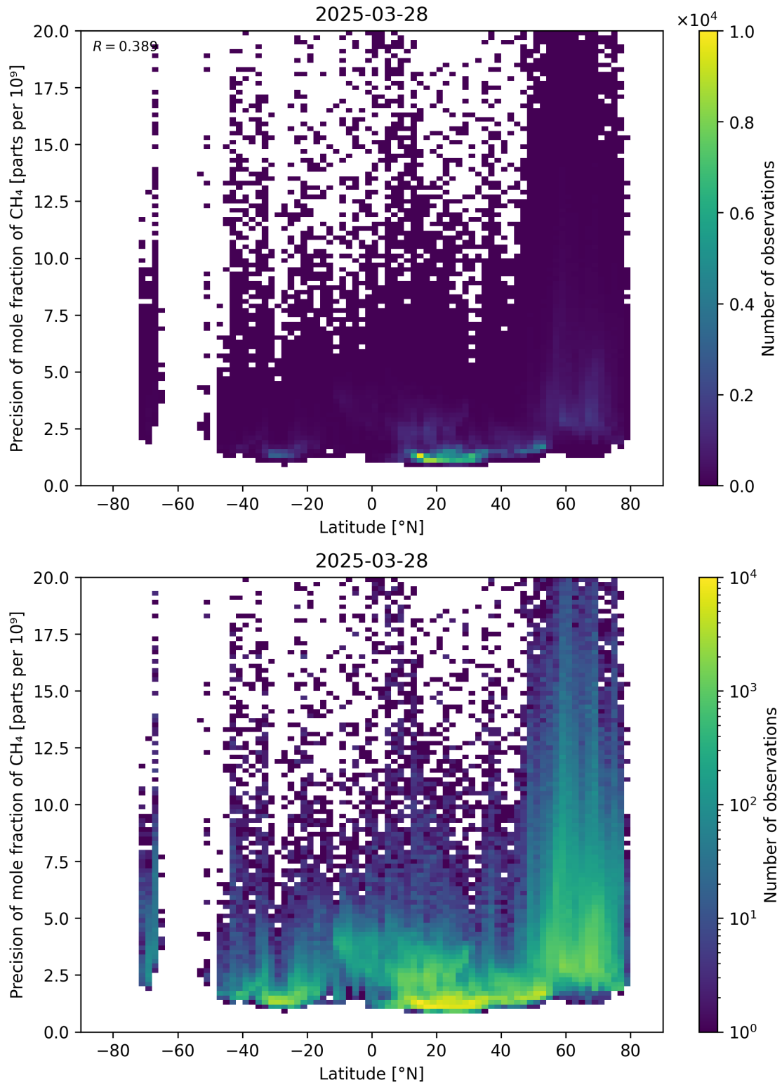
Figure 59: Scatter density plot of “Latitude” against “Precision of mole fraction of \text{CH}_4 ” for 2025-03-28 to 2025-03-29.
