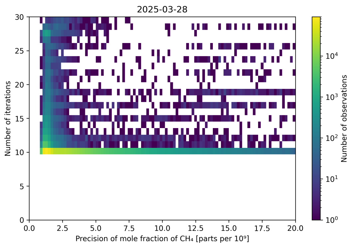
Figure 83: Scatter density plot of “Precision of mole fraction of CH 4 ” against “Number of iterations” for 2025-03-28 to 2025-03-29.
