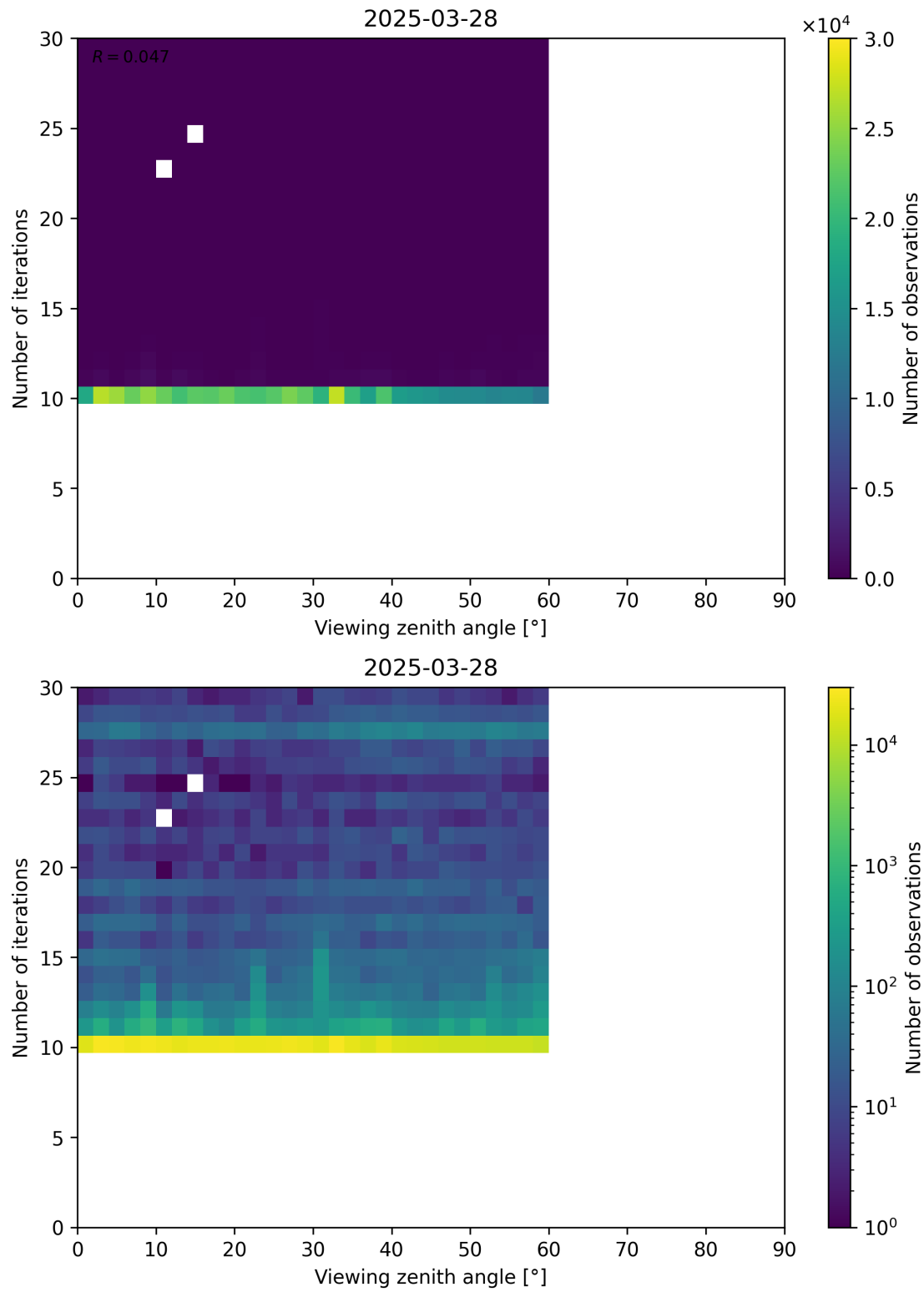
Figure 113: Scatter density plot of “Viewing zenith angle” against “Number of iterations” for 2025-03-28 to 2025-03-29.
