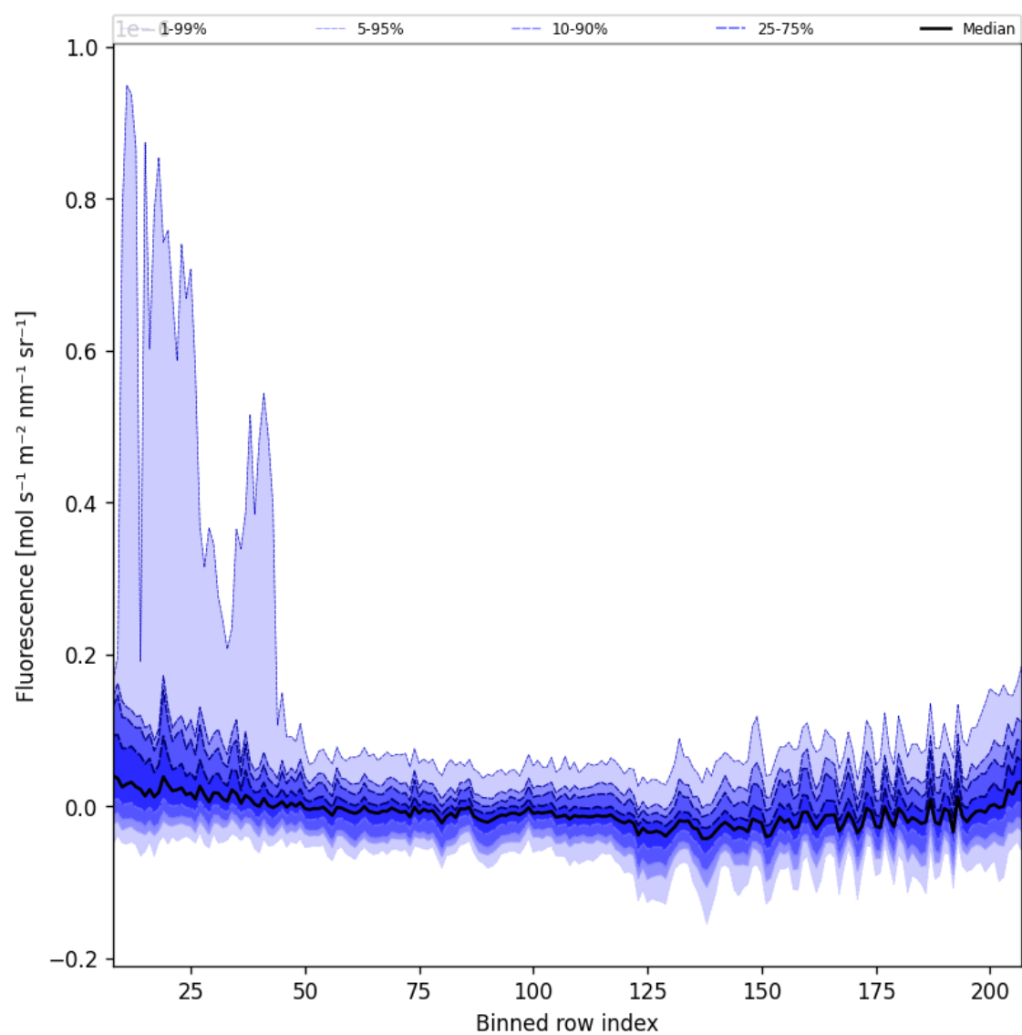
Figure 43: Along track statistics of “Fluorescence” for 2025-03-28 to 2025-03-29
