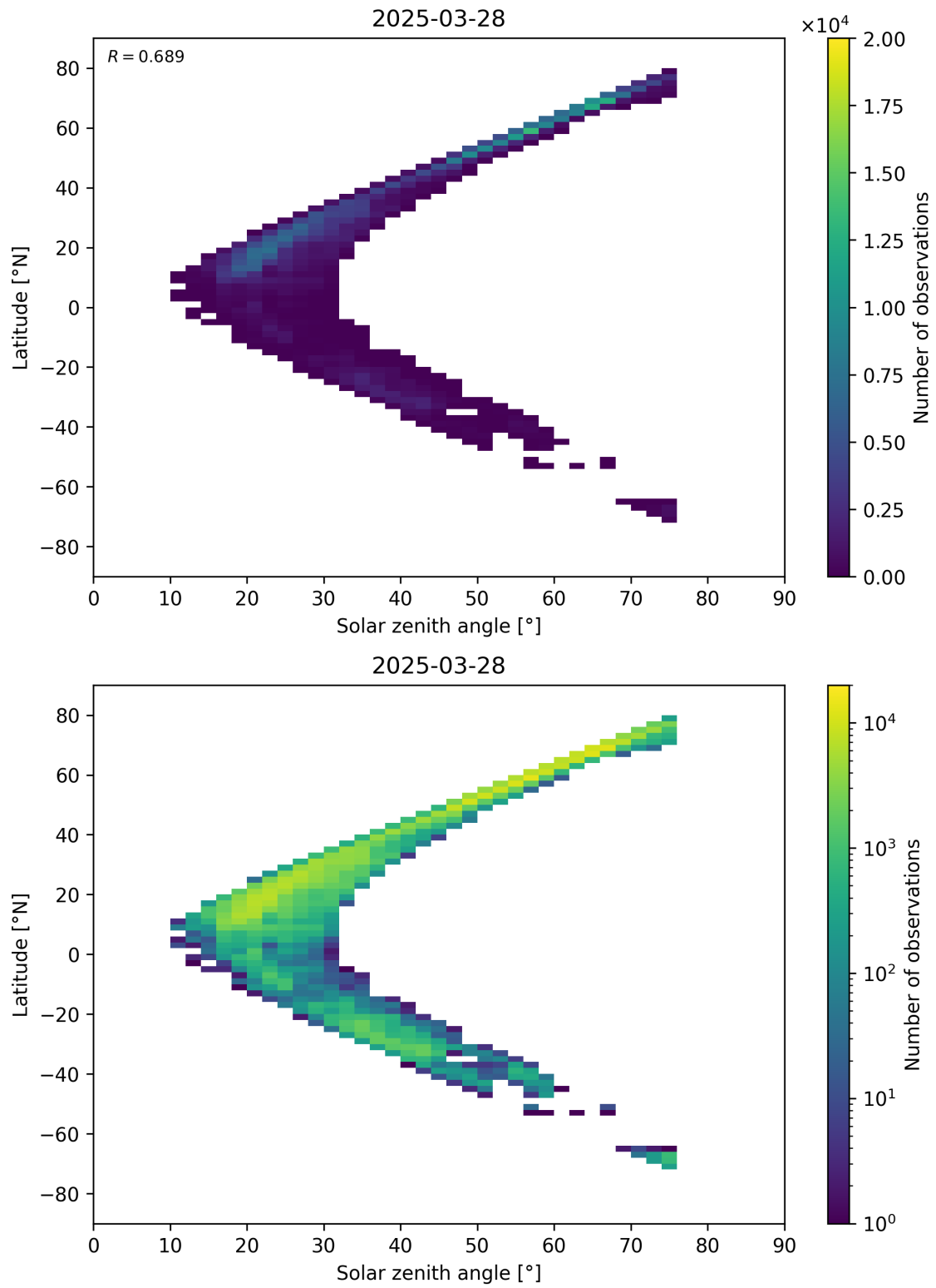
Figure 98: Scatter density plot of “Solar zenith angle” against “Latitude” for 2025-03-28 to 2025-03-29.
