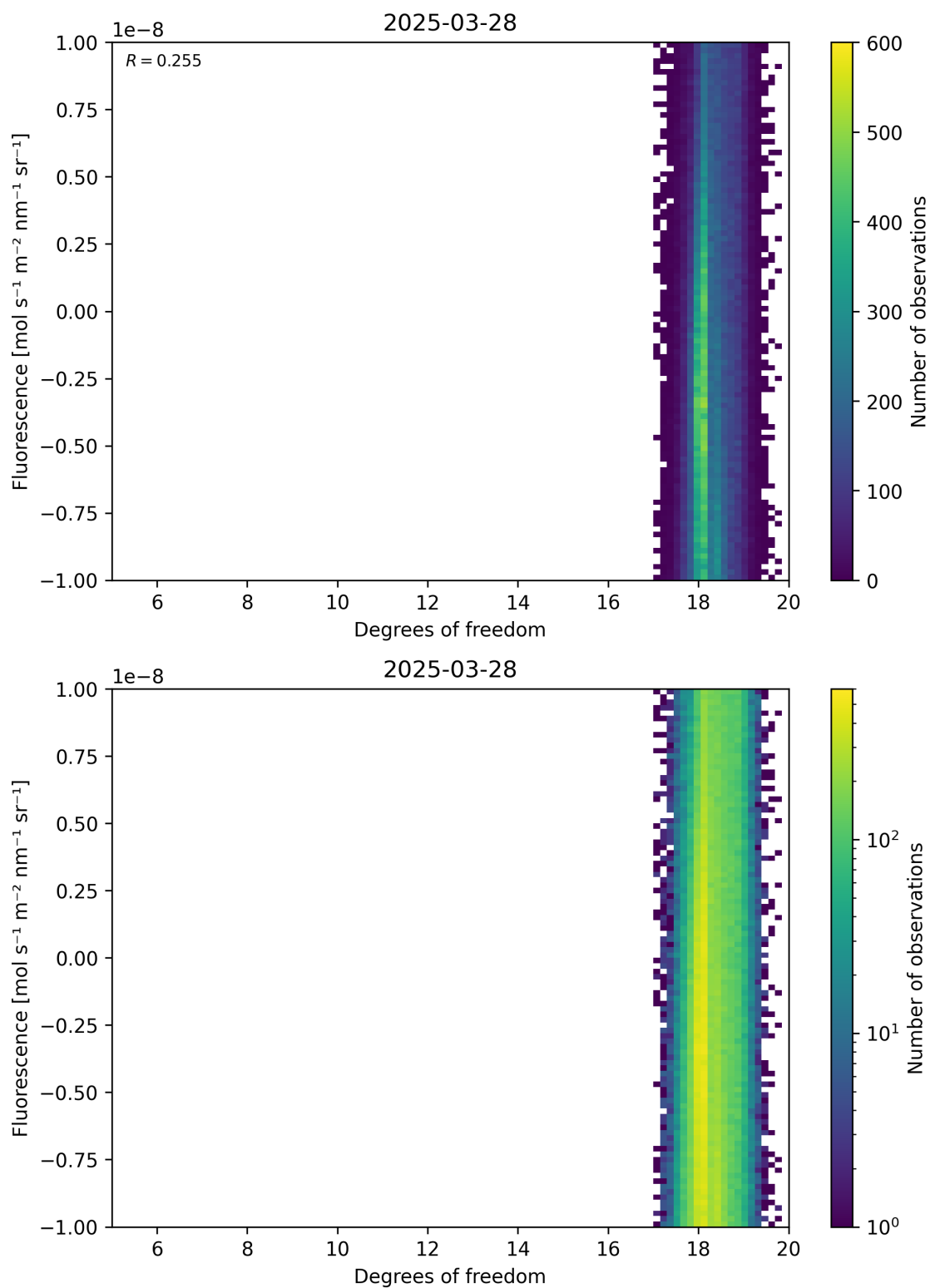
Figure 51: Scatter density plot of “Degrees of freedom” against “Fluorescence” for 2025-03-28 to 2025-03-29.
