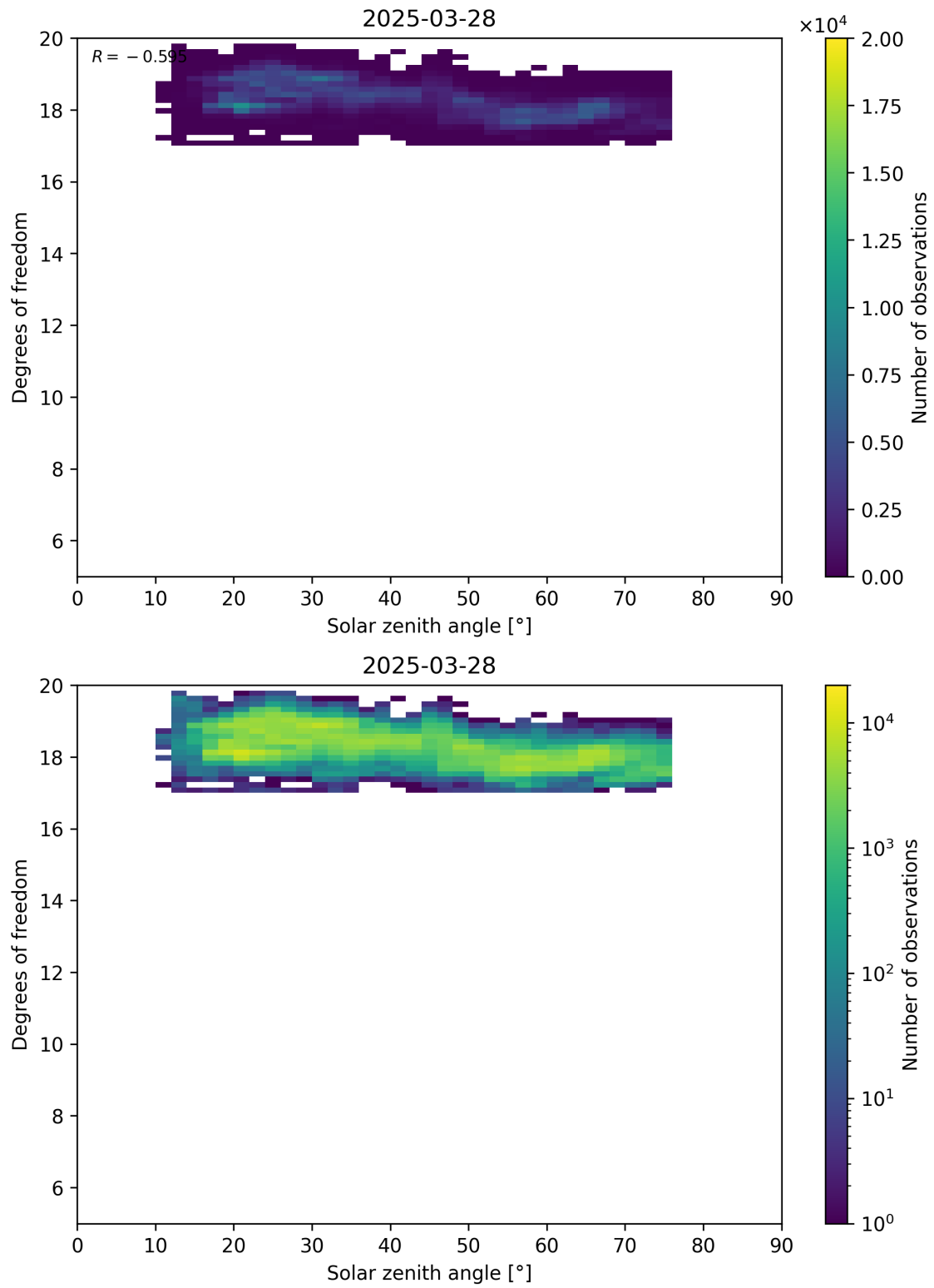
Figure 96: Scatter density plot of “Solar zenith angle” against “Degrees of freedom” for 2025-03-28 to 2025-03-29.
