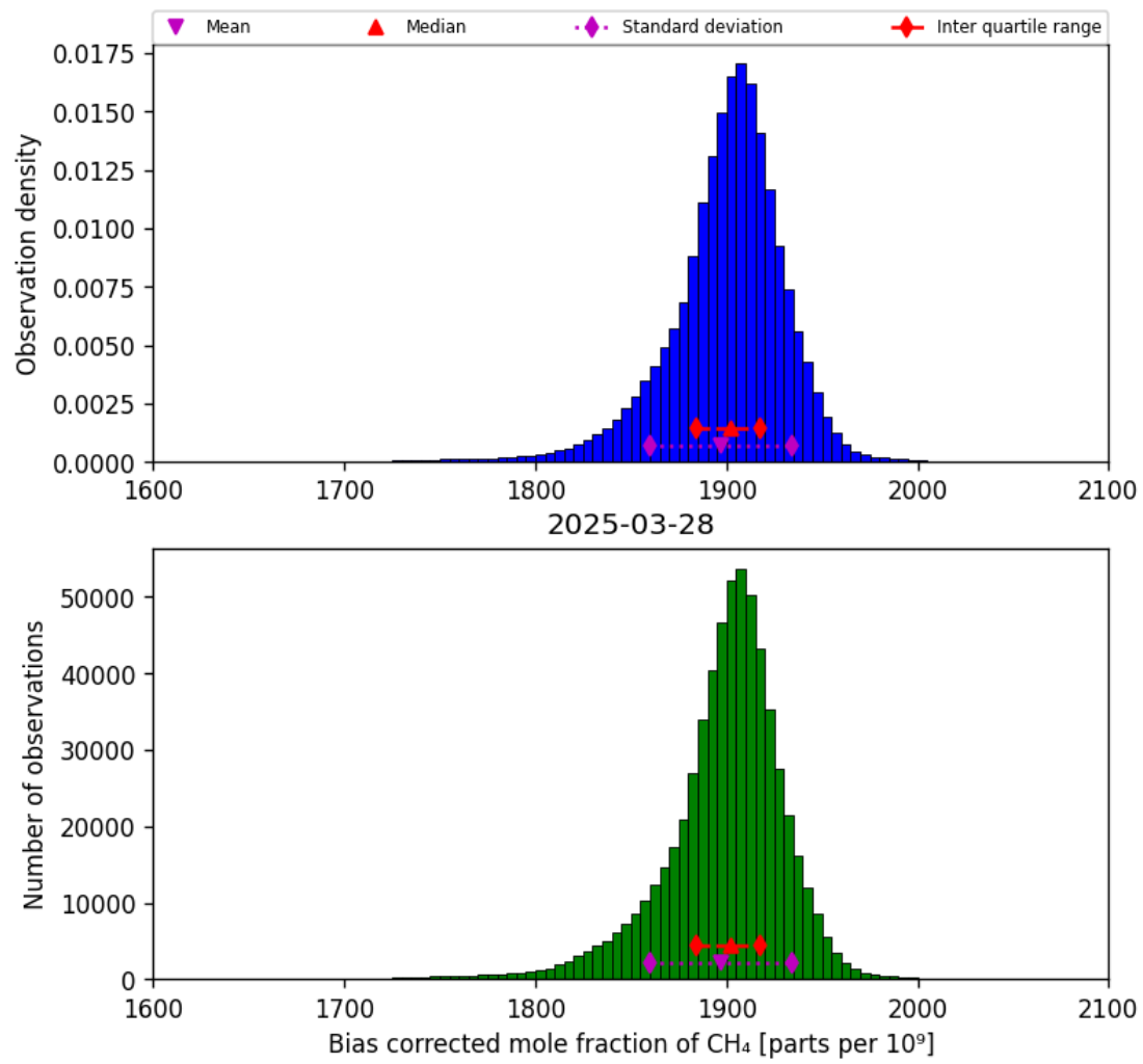
Figure 25: Histogram of “Bias corrected mole fraction of CH 4 ” for 2025-03-28 to 2025-03-29
