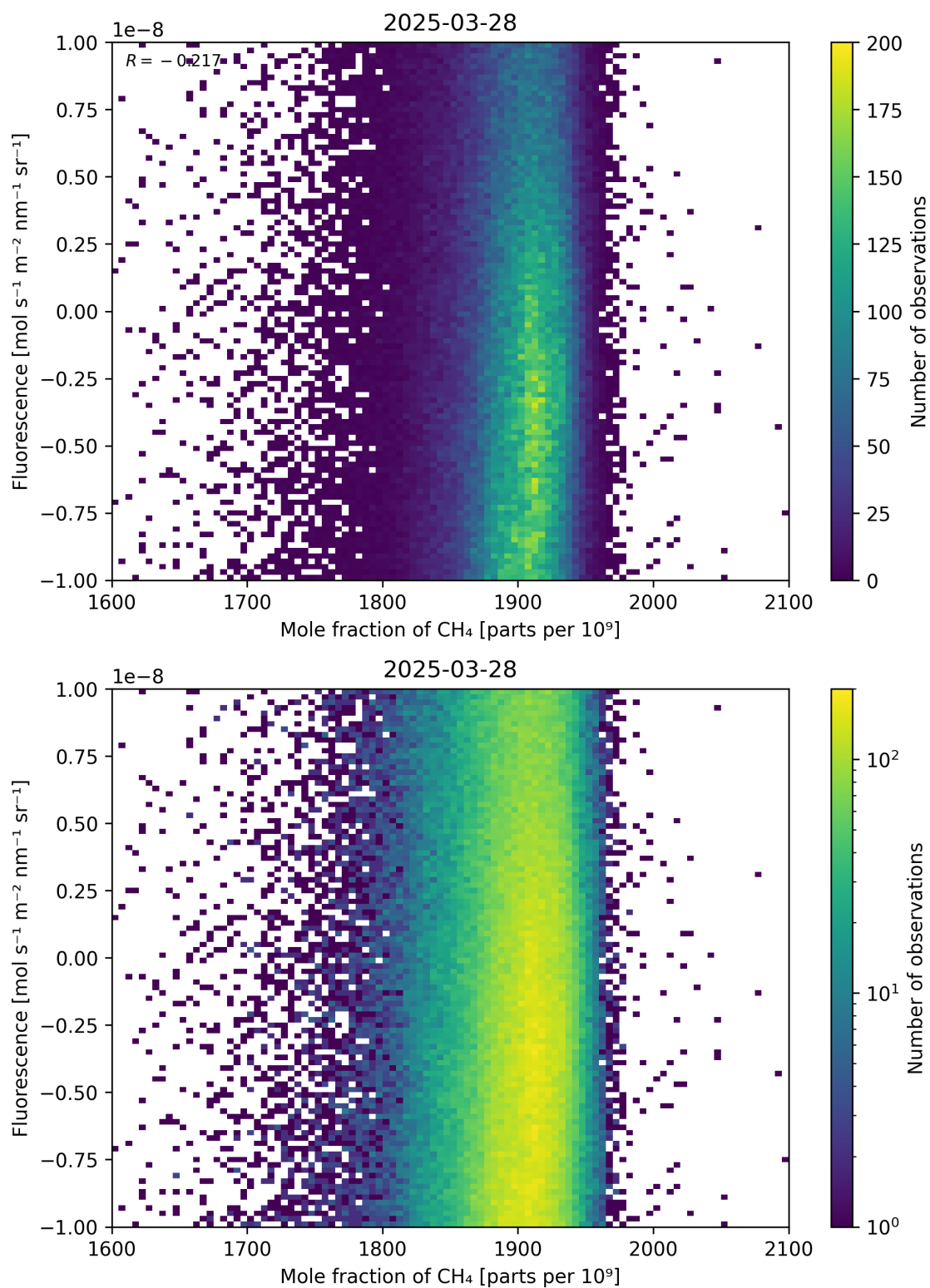
Figure 73: Scatter density plot of “Mole fraction of \text{CH}_4 ” against “Fluorescence” for 2025-03-28 to 2025-03-29.
