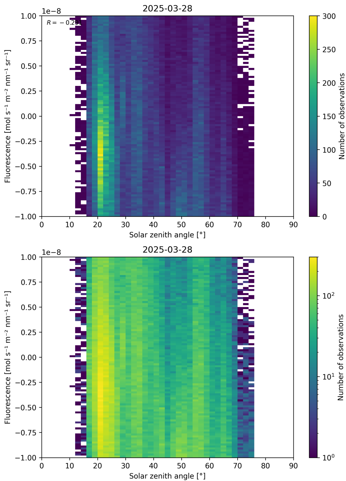
Figure 97: Scatter density plot of “Solar zenith angle” against “Fluorescence” for 2025-03-28 to 2025-03-29.
