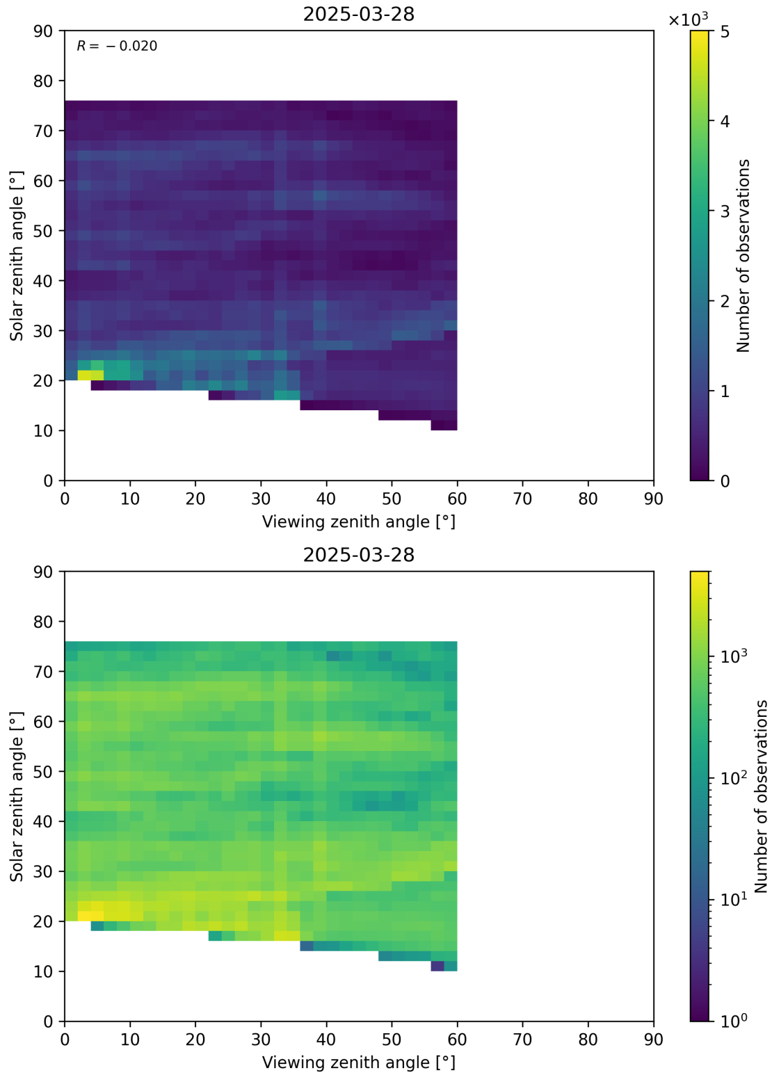
Figure 115: Scatter density plot of “Viewing zenith angle” against “Solar zenith angle” for 2025-03-28 to 2025-03-29.
