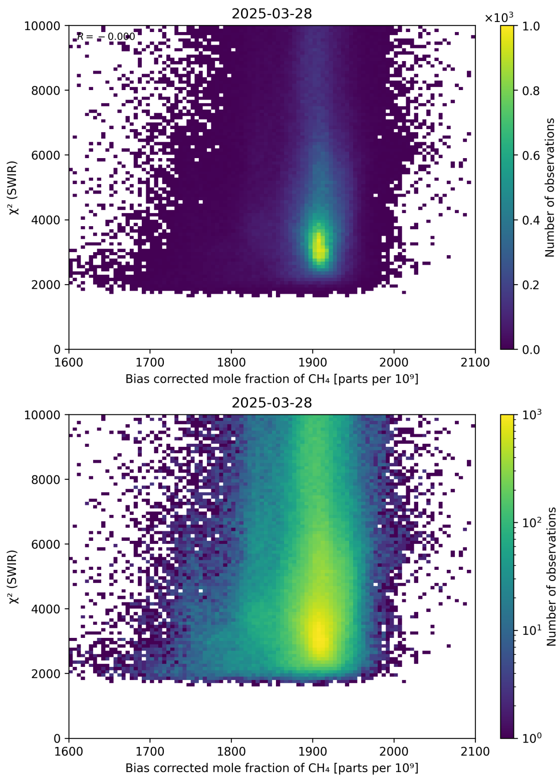
Figure 64: Scatter density plot of “Bias corrected mole fraction of \text{CH}_4 ” against “ \chi^2 (SWIR)” for 2025-03-28 to 2025-03-29.
