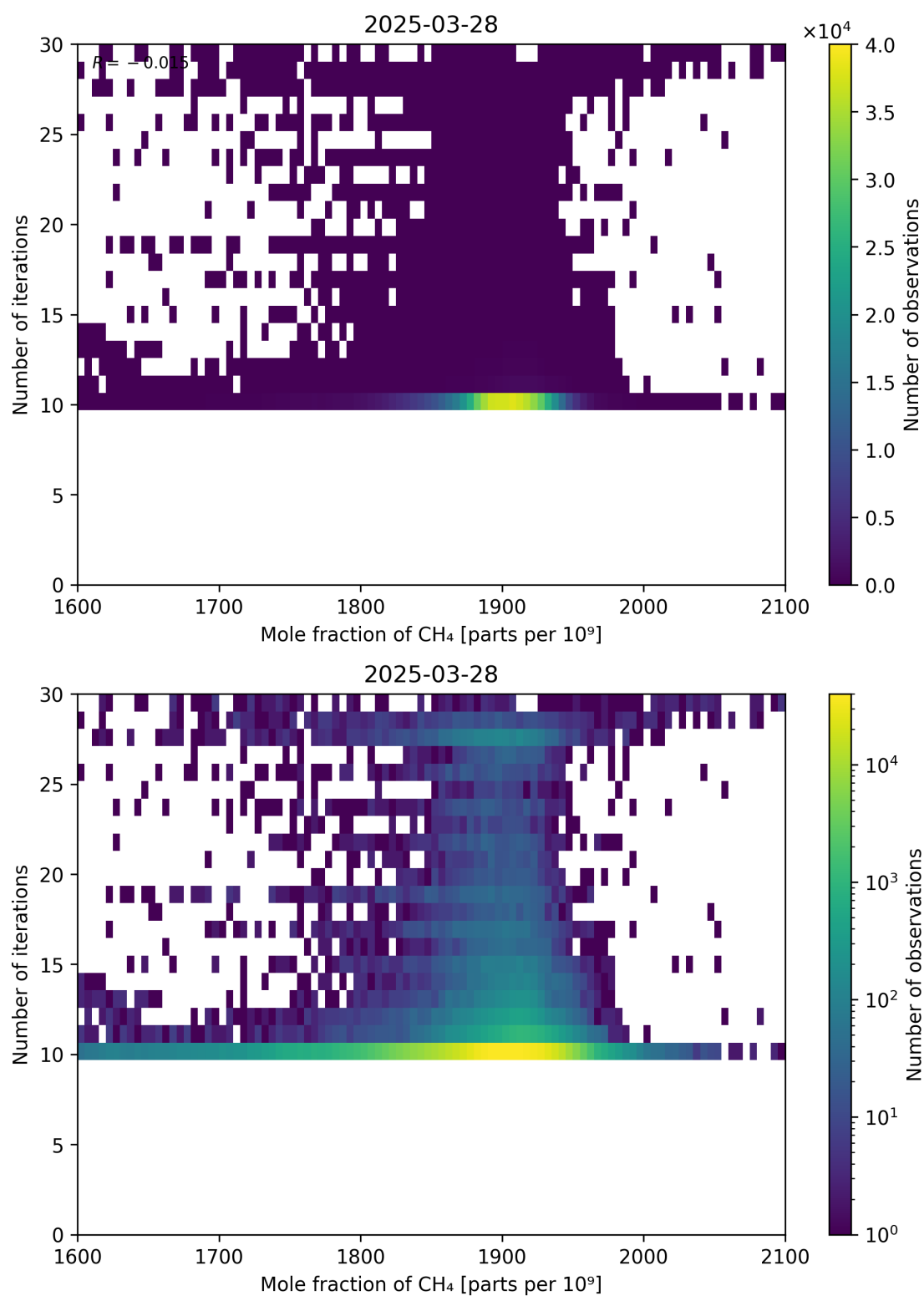
Figure 76: Scatter density plot of “Mole fraction of CH 4 ” against “Number of iterations” for 2025-03-28 to 2025-03-29.
