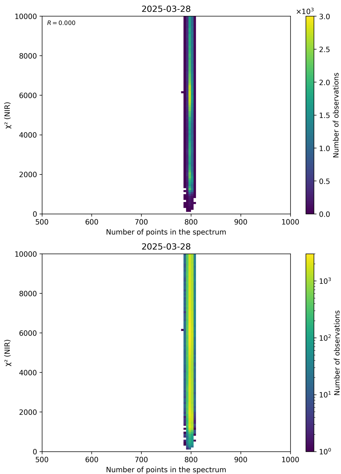
Figure 88: Scatter density plot of “Number of points in the spectrum” against “ \chi^2 (NIR)” for 2025-03-28 to 2025-03-29.
