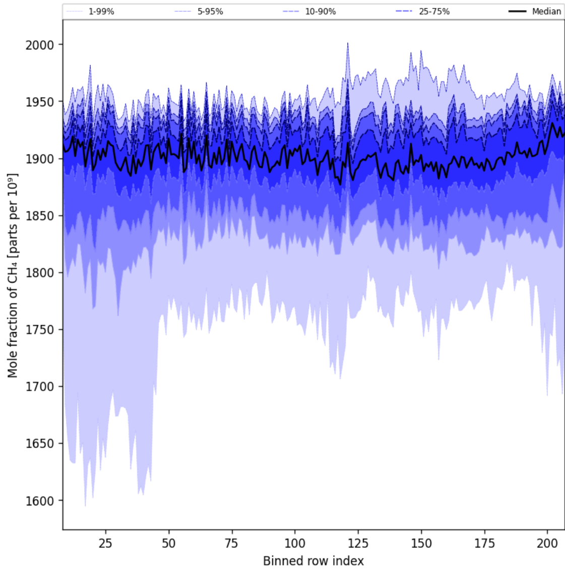
Figure 34: Along track statistics of “Mole fraction of CH 4 ” for 2025-03-28 to 2025-03-29
