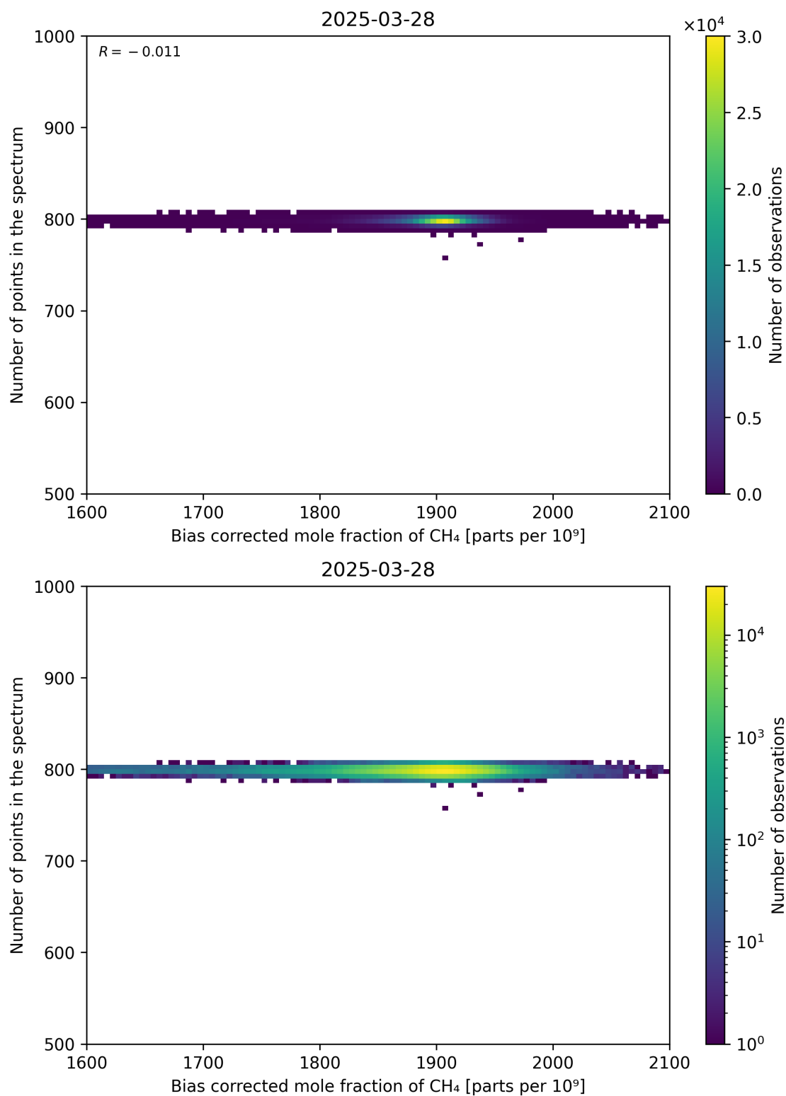
Figure 68: Scatter density plot of “Bias corrected mole fraction of CH 4 ” against “Number of points in the spectrum” for 2025-03-28 to 2025-03-29.
