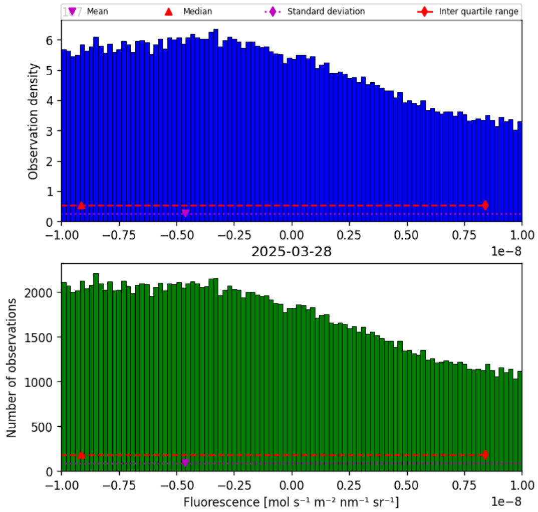
Figure 32: Histogram of “Fluorescence” for 2025-03-28 to 2025-03-29
