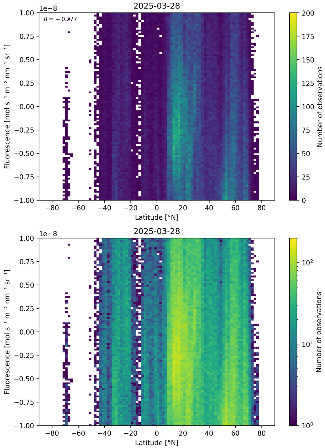
Figure 56: Scatter density plot of “Latitude” against “Fluorescence” for 2025-03-28 to 2025-03-29.
