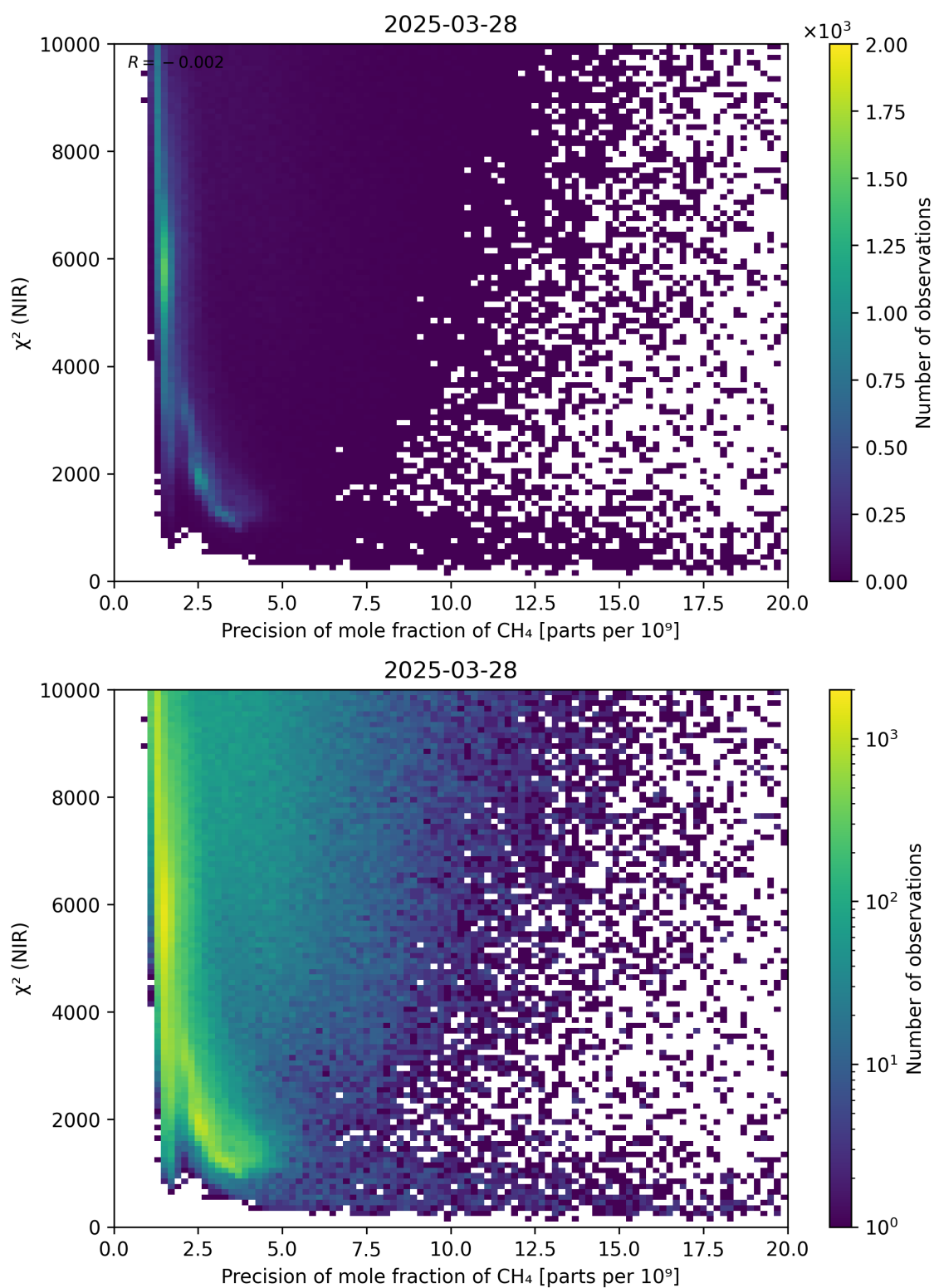
Figure 78: Scatter density plot of “Precision of mole fraction of CH 4 ” against “ \chi^2 (NIR)” for 2025-03-28 to 2025-03-29.
