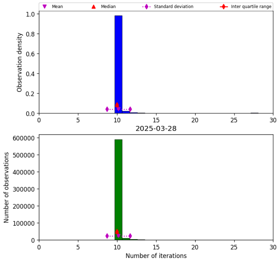
Figure 31: Histogram of “Number of iterations” for 2025-03-28 to 2025-03-29
