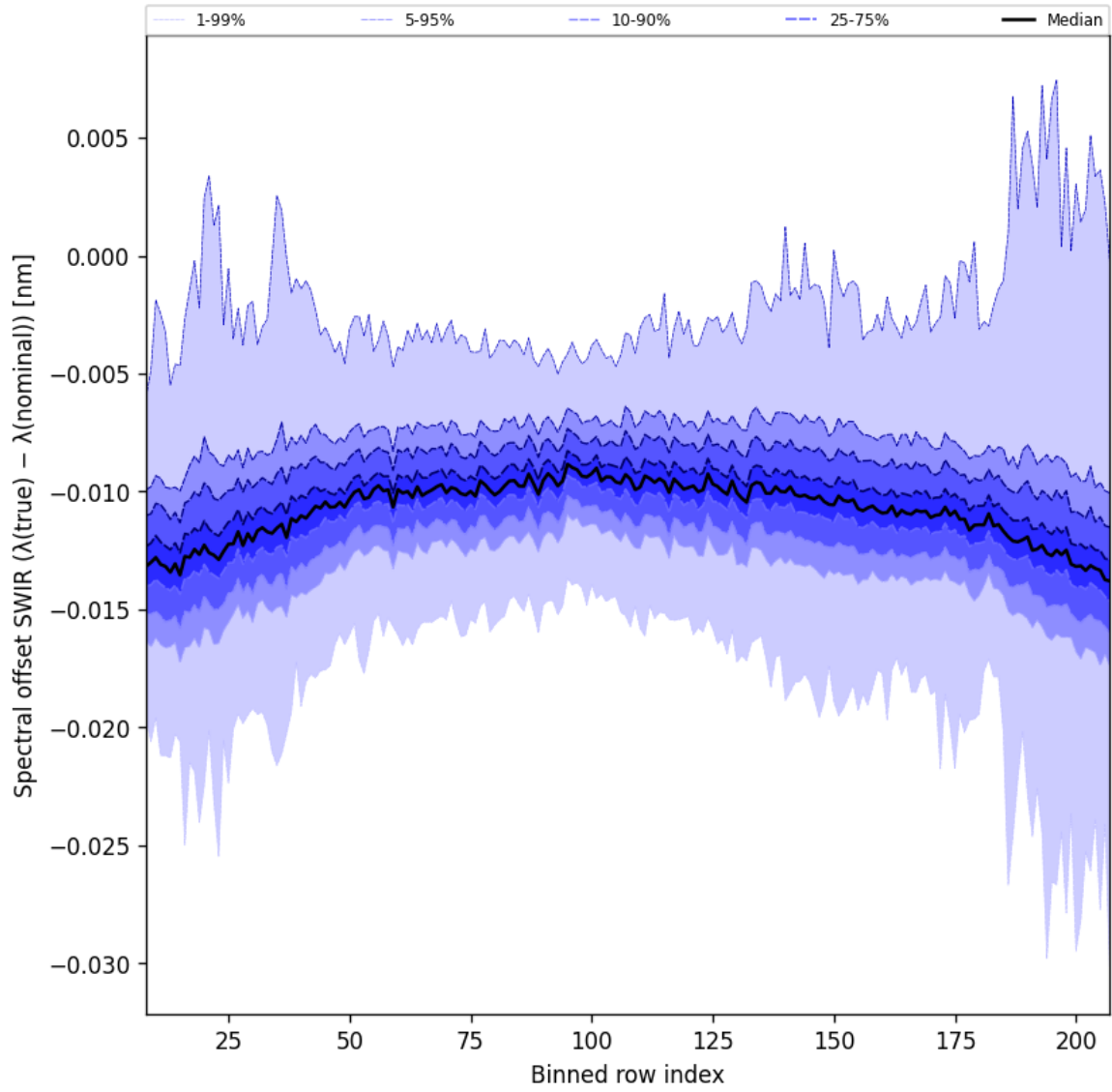
Figure 38: Along track statistics of “Spectral offset SWIR ( \lambda_{\text{true}} - \lambda_{\text{nominal}} )” for 2025-03-28 to 2025-03-29
