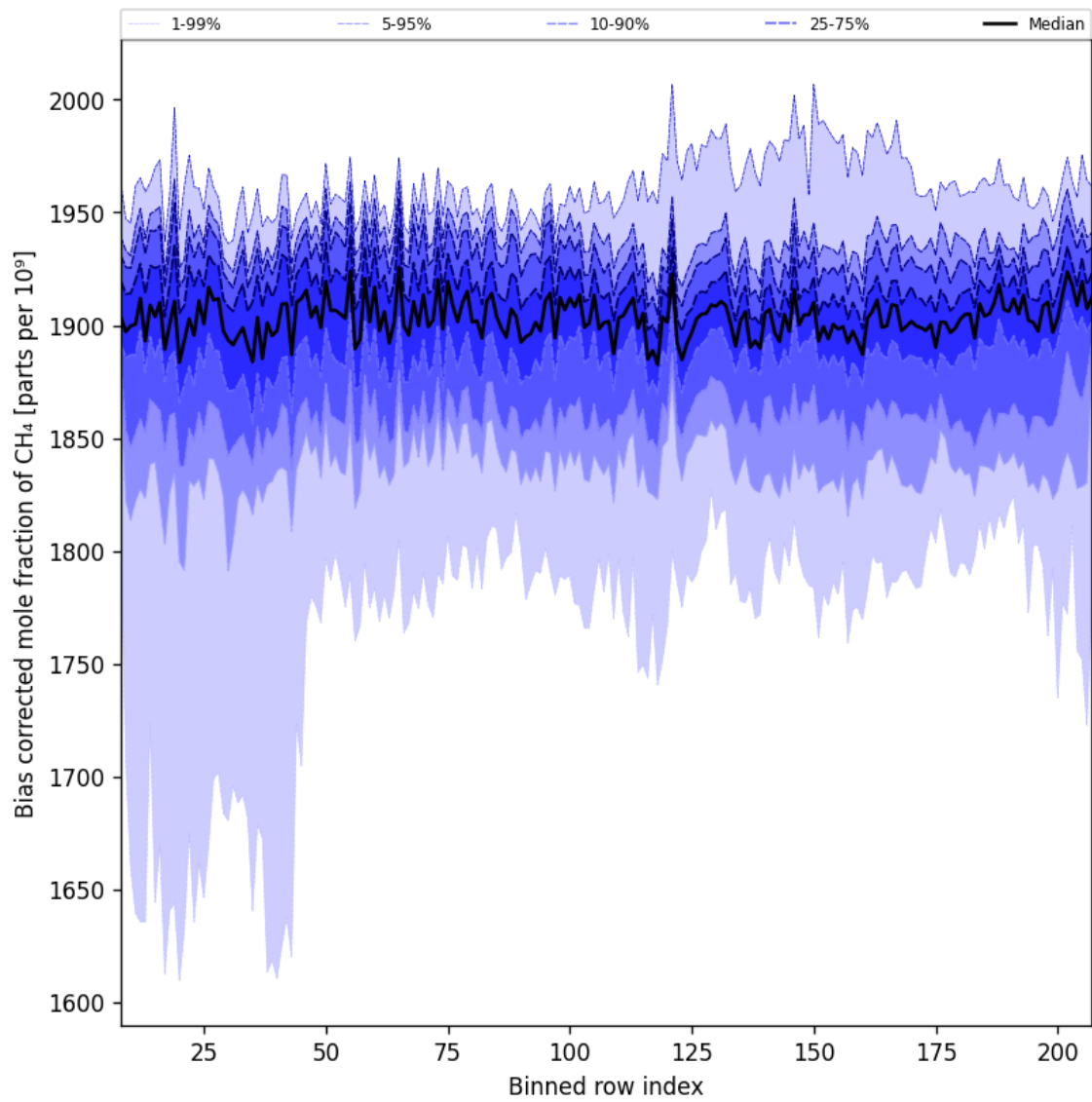
Figure 36: Along track statistics of “Bias corrected mole fraction of CH 4 ” for 2025-03-28 to 2025-03-29
