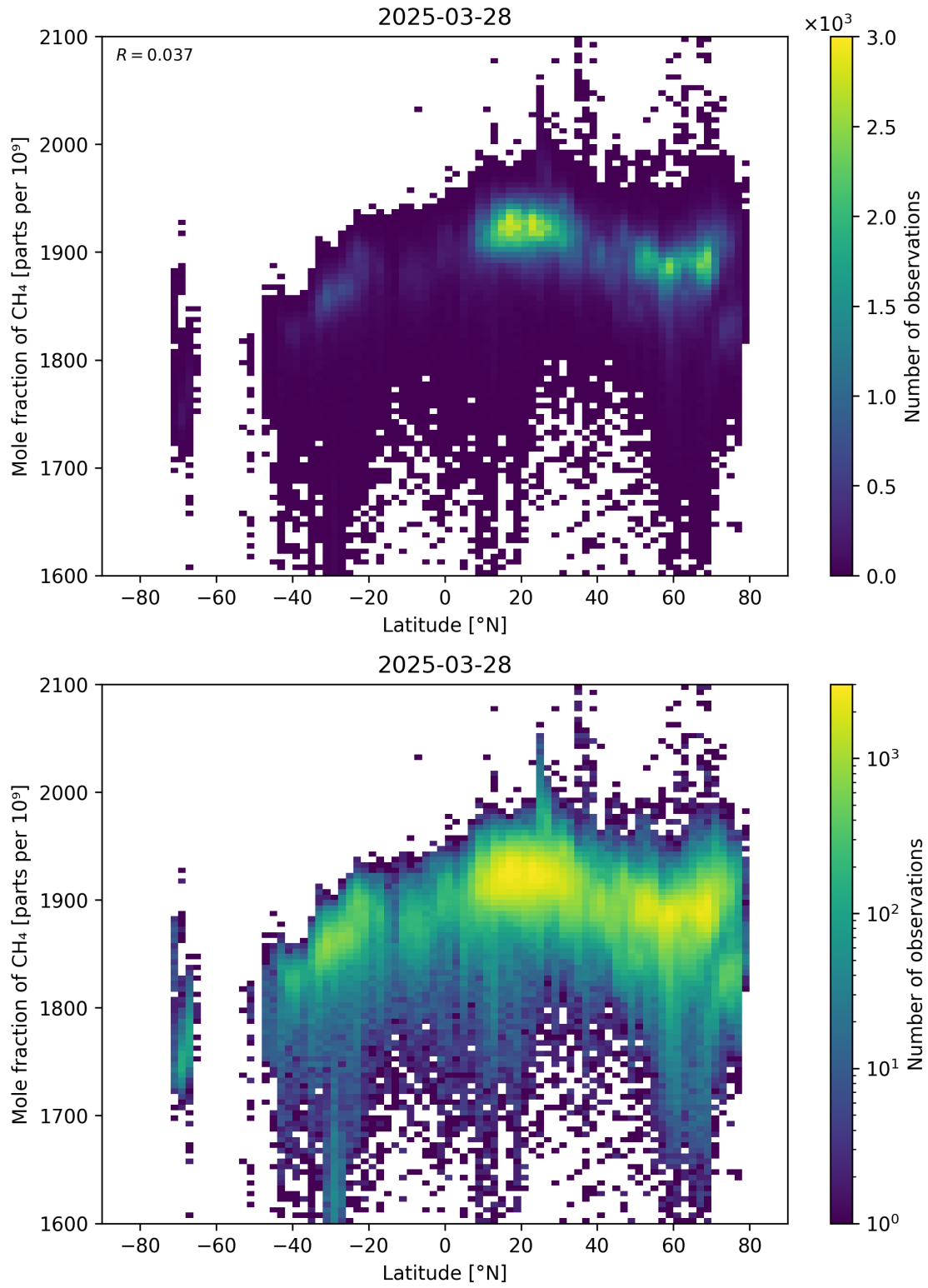
Figure 57: Scatter density plot of “Latitude” against “Mole fraction of \text{CH}_4 ” for 2025-03-28 to 2025-03-29.
