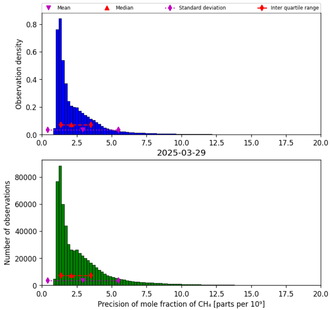
Figure 24: Histogram of “Precision of mole fraction of CH 4 ” for 2025-03-28 to 2025-03-30
