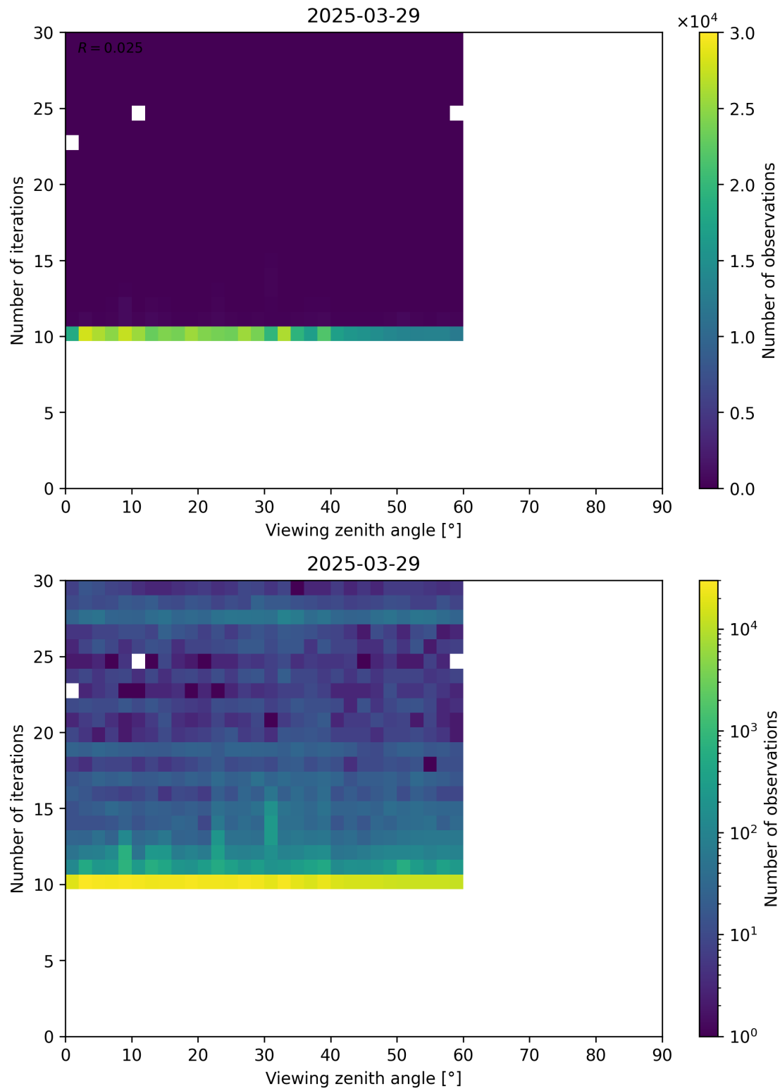
Figure 113: Scatter density plot of “Viewing zenith angle” against “Number of iterations” for 2025-03-28 to 2025-03-30.
