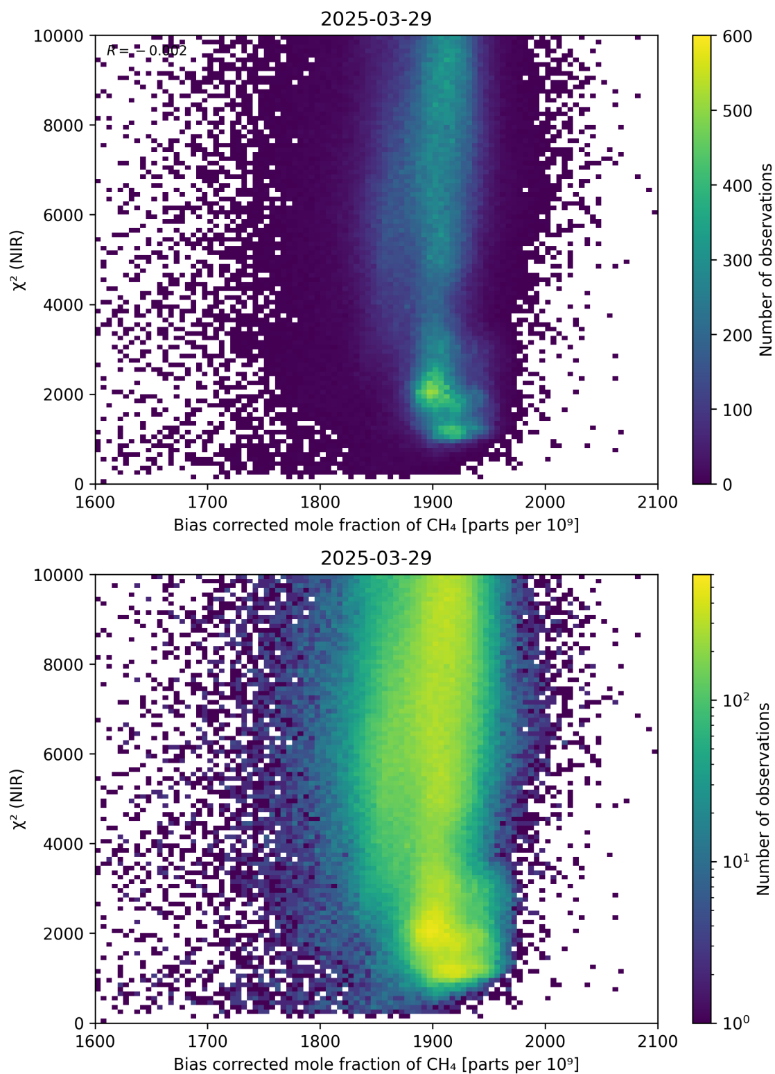
Figure 63: Scatter density plot of “Bias corrected mole fraction of \text{CH}_4 ” against “ \chi^2 (NIR)” for 2025-03-28 to 2025-03-30.
