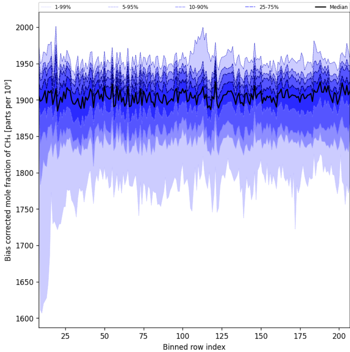
Figure 36: Along track statistics of “Bias corrected mole fraction of CH 4 ” for 2025-03-28 to 2025-03-30
