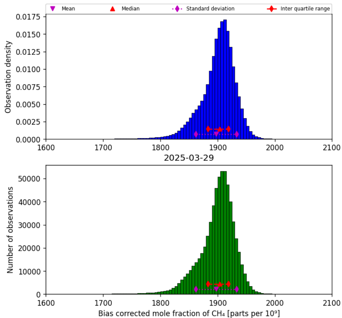
Figure 25: Histogram of “Bias corrected mole fraction of CH 4 ” for 2025-03-28 to 2025-03-30
