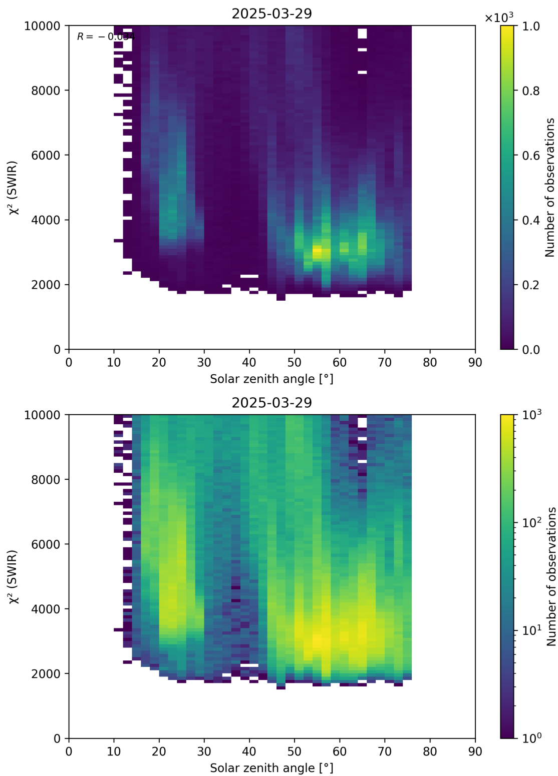
Figure 95: Scatter density plot of “Solar zenith angle” against “ \chi^2 (SWIR)” for 2025-03-28 to 2025-03-30.
