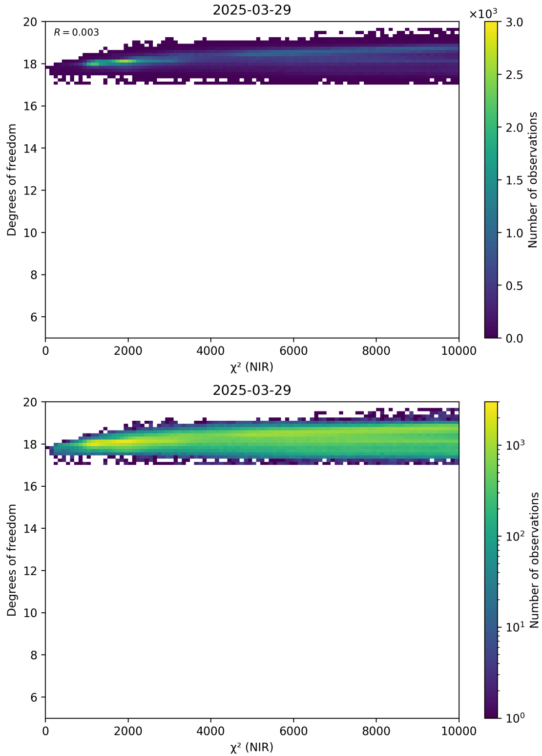
Figure 44: Scatter density plot of “ \chi^2 (NIR)” against “Degrees of freedom” for 2025-03-28 to 2025-03-30.
