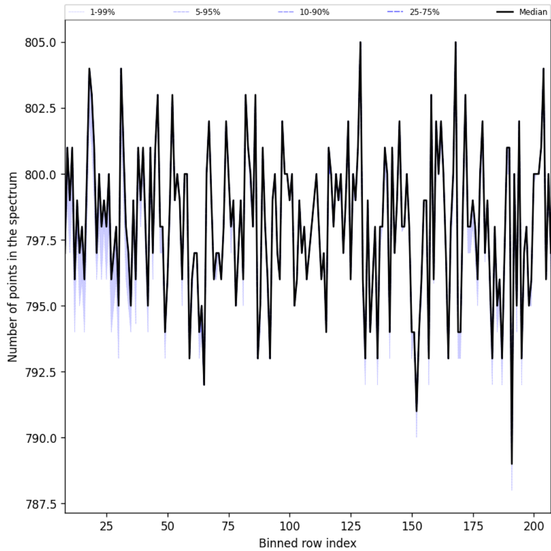
Figure 37: Along track statistics of “Number of points in the spectrum” for 2025-03-28 to 2025-03-30
