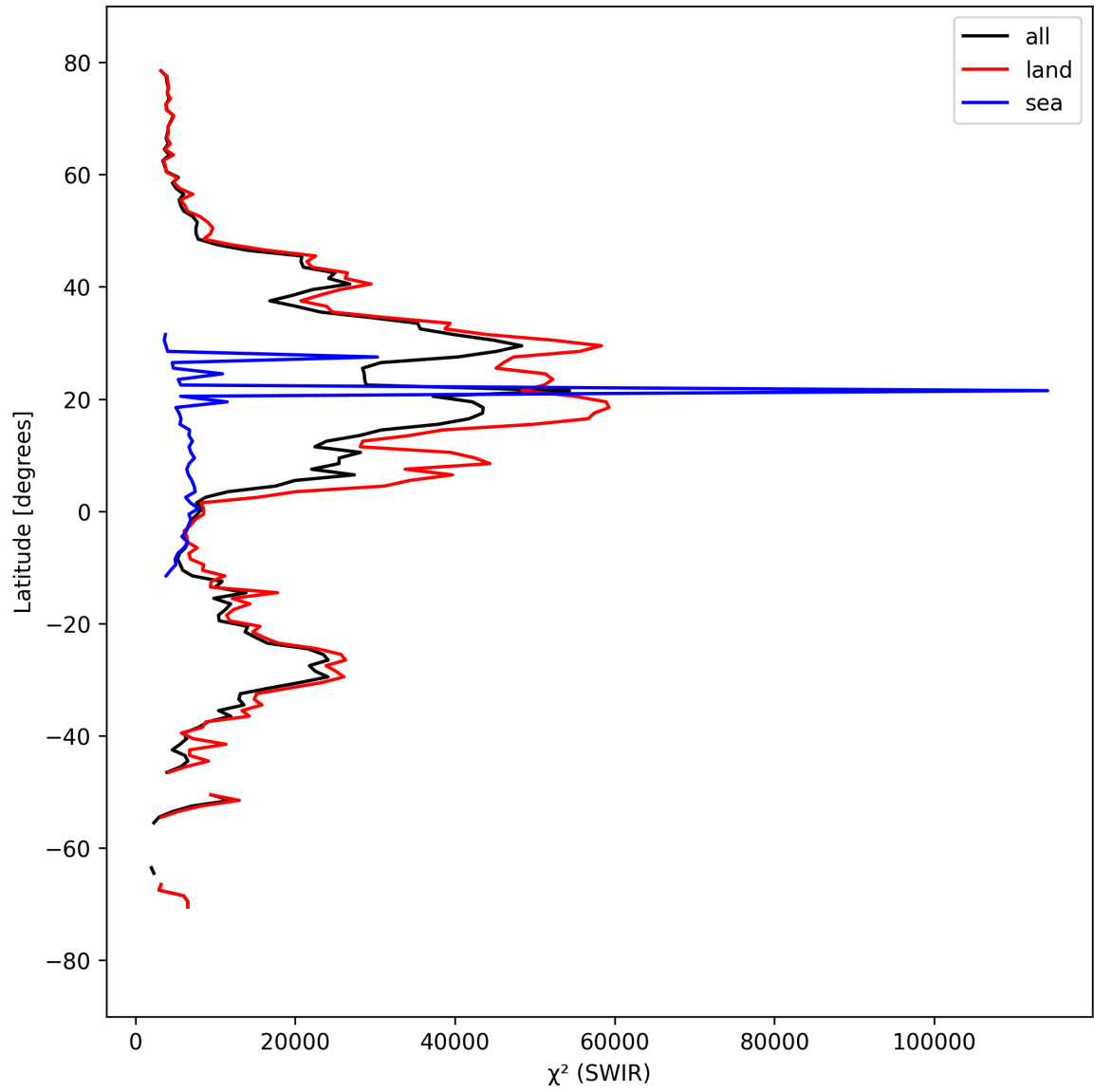
Figure 17: Zonal average of “ \chi^2 (SWIR)” for 2025-03-28 to 2025-03-30.
