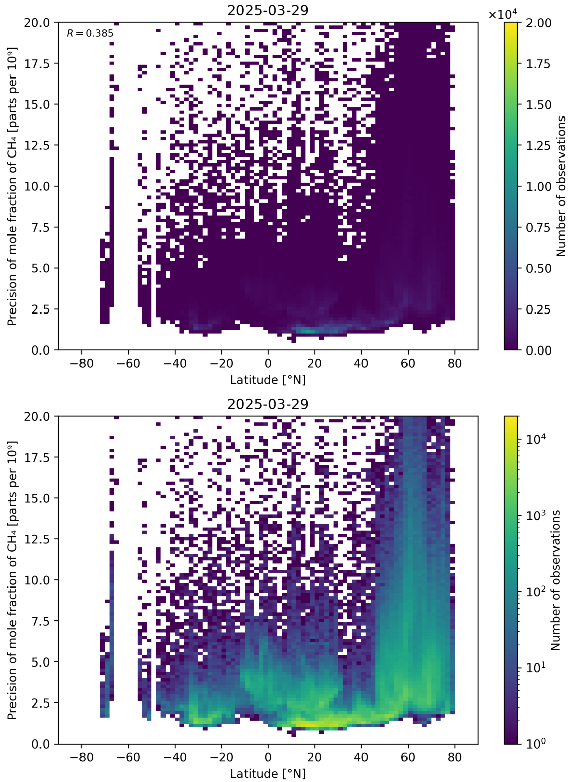
Figure 59: Scatter density plot of “Latitude” against “Precision of mole fraction of \text{CH}_4 ” for 2025-03-28 to 2025-03-30.
