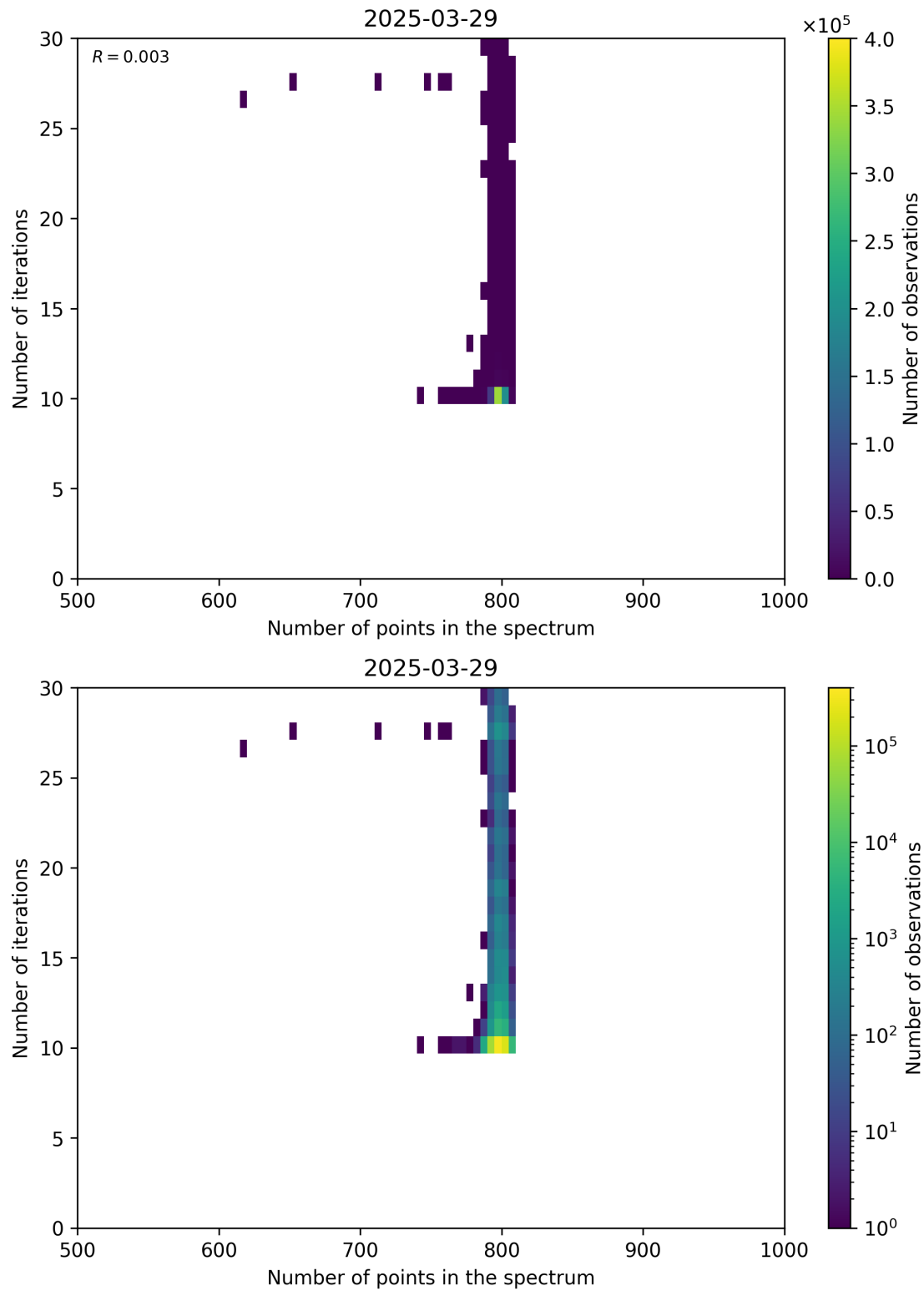
Figure 92: Scatter density plot of “Number of points in the spectrum” against “Number of iterations” for 2025-03-28 to 2025-03-30.
