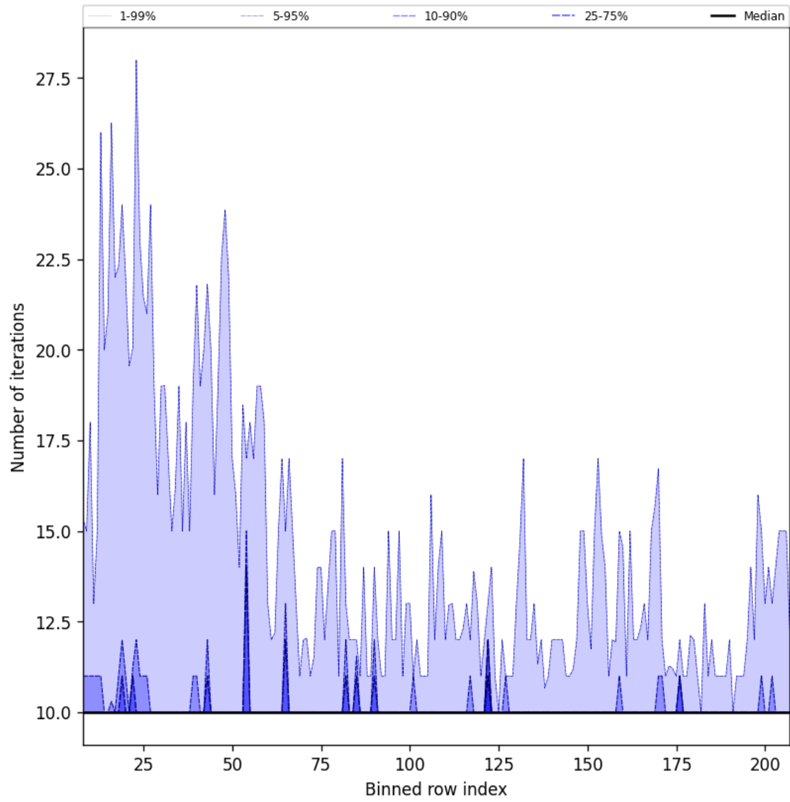
Figure 42: Along track statistics of “Number of iterations” for 2025-03-28 to 2025-03-30
