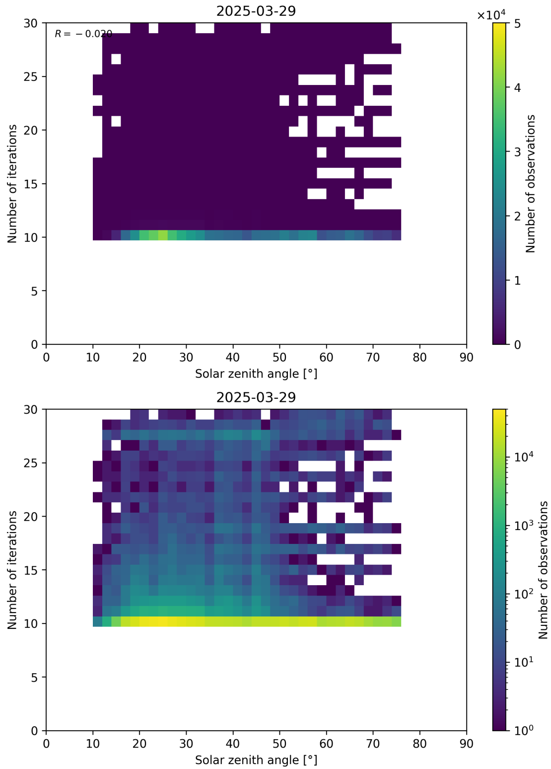
Figure 102: Scatter density plot of “Solar zenith angle” against “Number of iterations” for 2025-03-28 to 2025-03-30.
