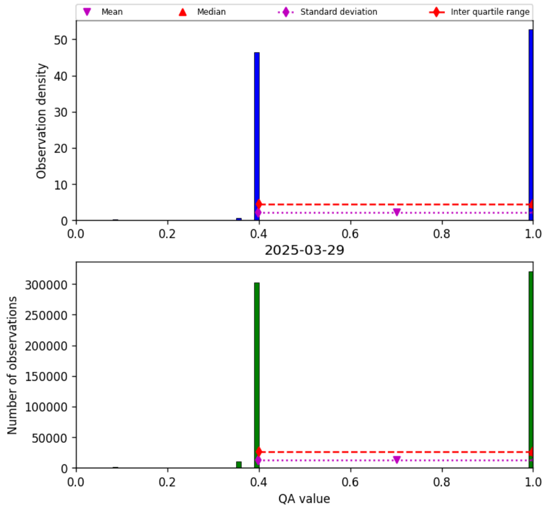
Figure 22: Histogram of “QA value” for 2025-03-28 to 2025-03-30
