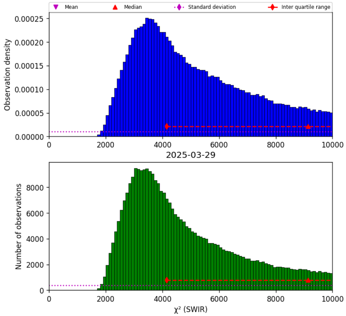
Figure 28: Histogram of “ \chi^2 (SWIR)” for 2025-03-28 to 2025-03-30
