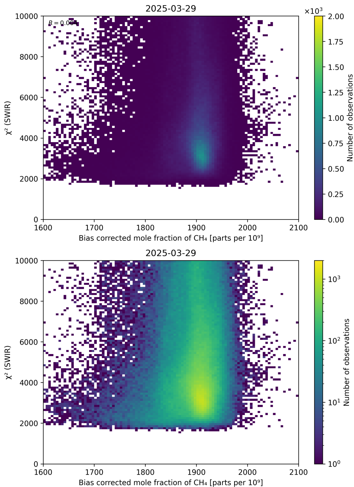
Figure 64: Scatter density plot of “Bias corrected mole fraction of \text{CH}_4 ” against “ \chi^2 (SWIR)” for 2025-03-28 to 2025-03-30.
