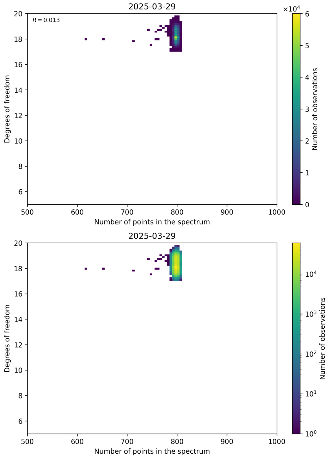
Figure 90: Scatter density plot of “Number of points in the spectrum” against “Degrees of freedom” for 2025-03-28 to 2025-03-30.
