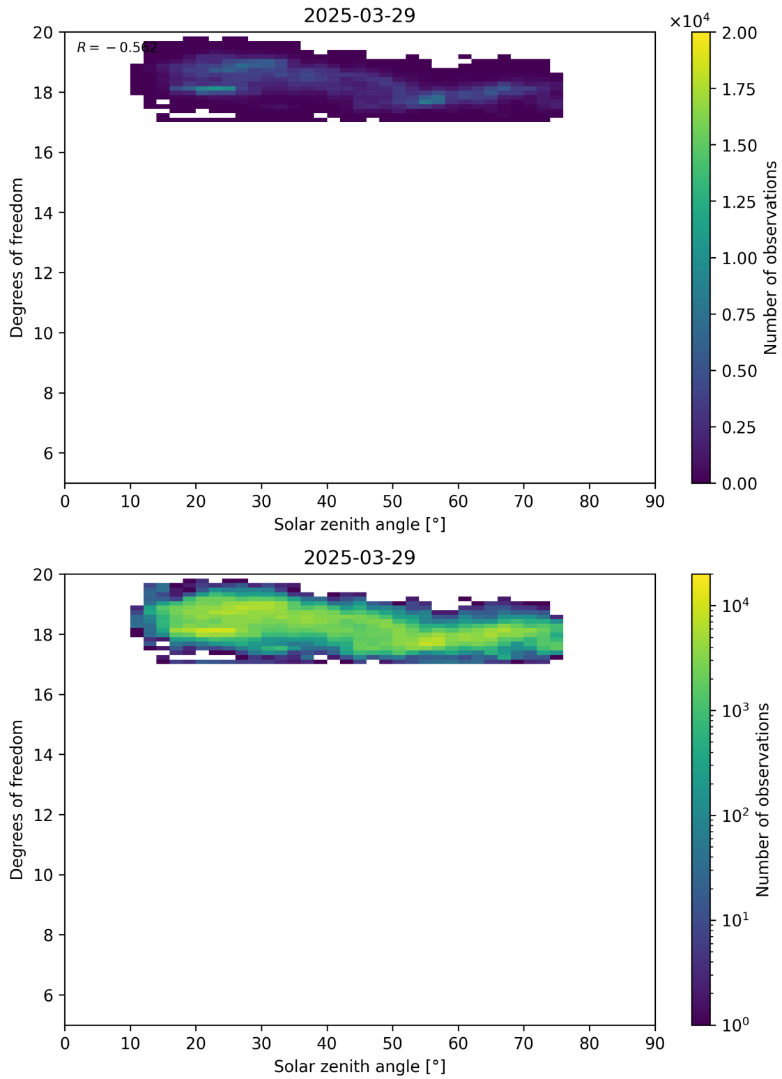
Figure 96: Scatter density plot of “Solar zenith angle” against “Degrees of freedom” for 2025-03-28 to 2025-03-30.
