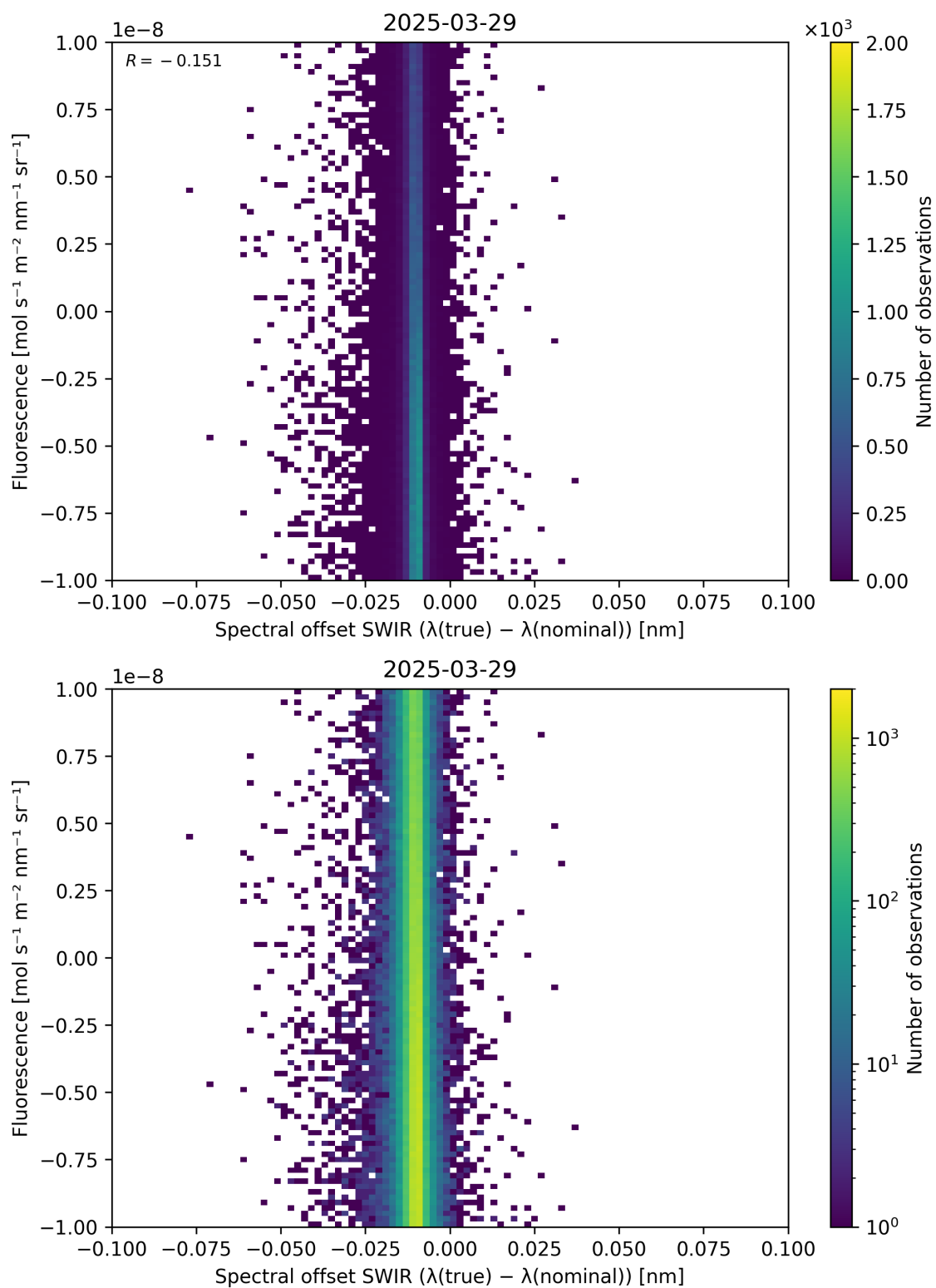
Figure 120: Scatter density plot of “Spectral offset SWIR ( \lambda_{\text{true}} - \lambda_{\text{nominal}} )” against “Fluorescence” for 2025-03-28 to 2025-03-30.
