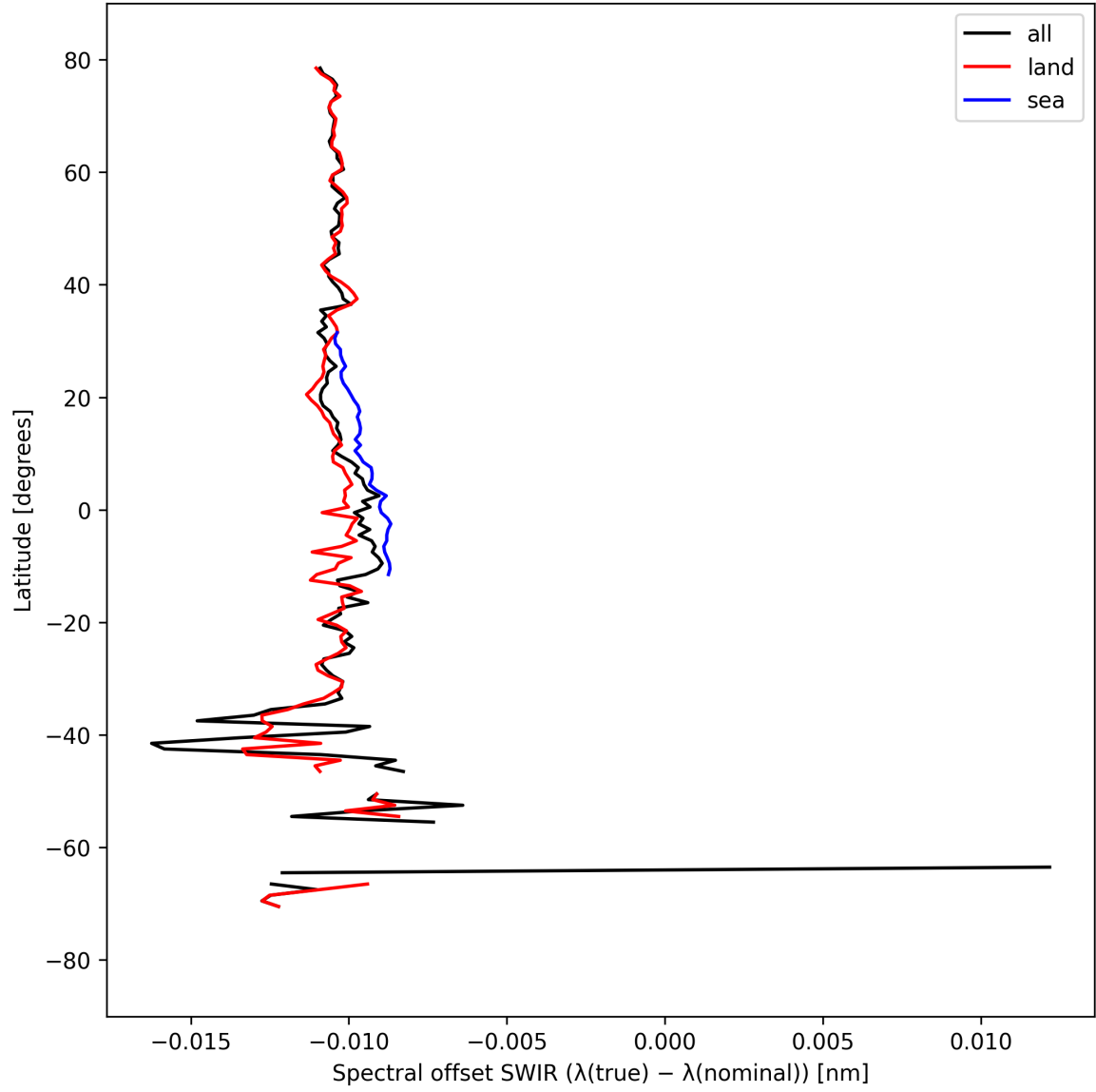
Figure 16: Zonal average of “Spectral offset SWIR ( \lambda_{\text{true}} - \lambda_{\text{nominal}} )” for 2025-03-28 to 2025-03-30.
