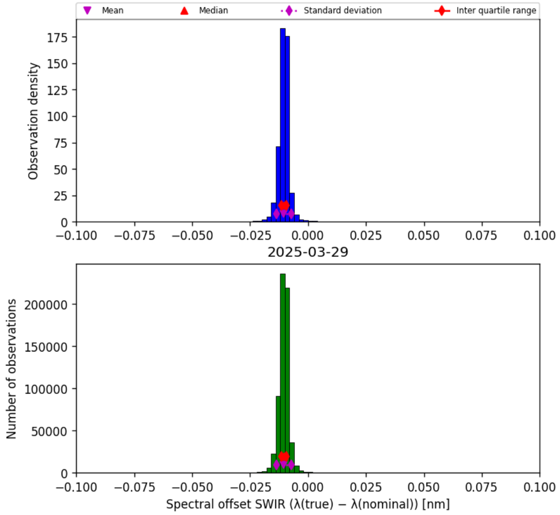
Figure 27: Histogram of “Spectral offset SWIR ( \lambda_{\text{true}} - \lambda_{\text{nominal}} )” for 2025-03-28 to 2025-03-30
