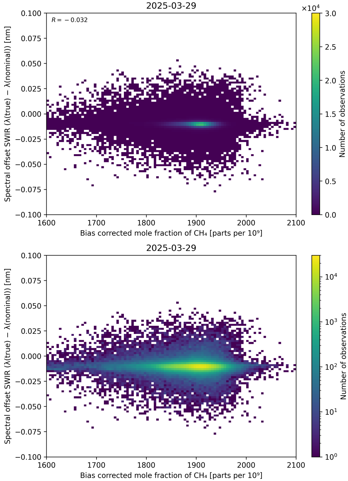
Figure 69: Scatter density plot of “Bias corrected mole fraction of \text{CH}_4 ” against “Spectral offset SWIR ( \lambda_{\text{true}} - \lambda_{\text{nominal}} )” for 2025-03-28 to 2025-03-30.
