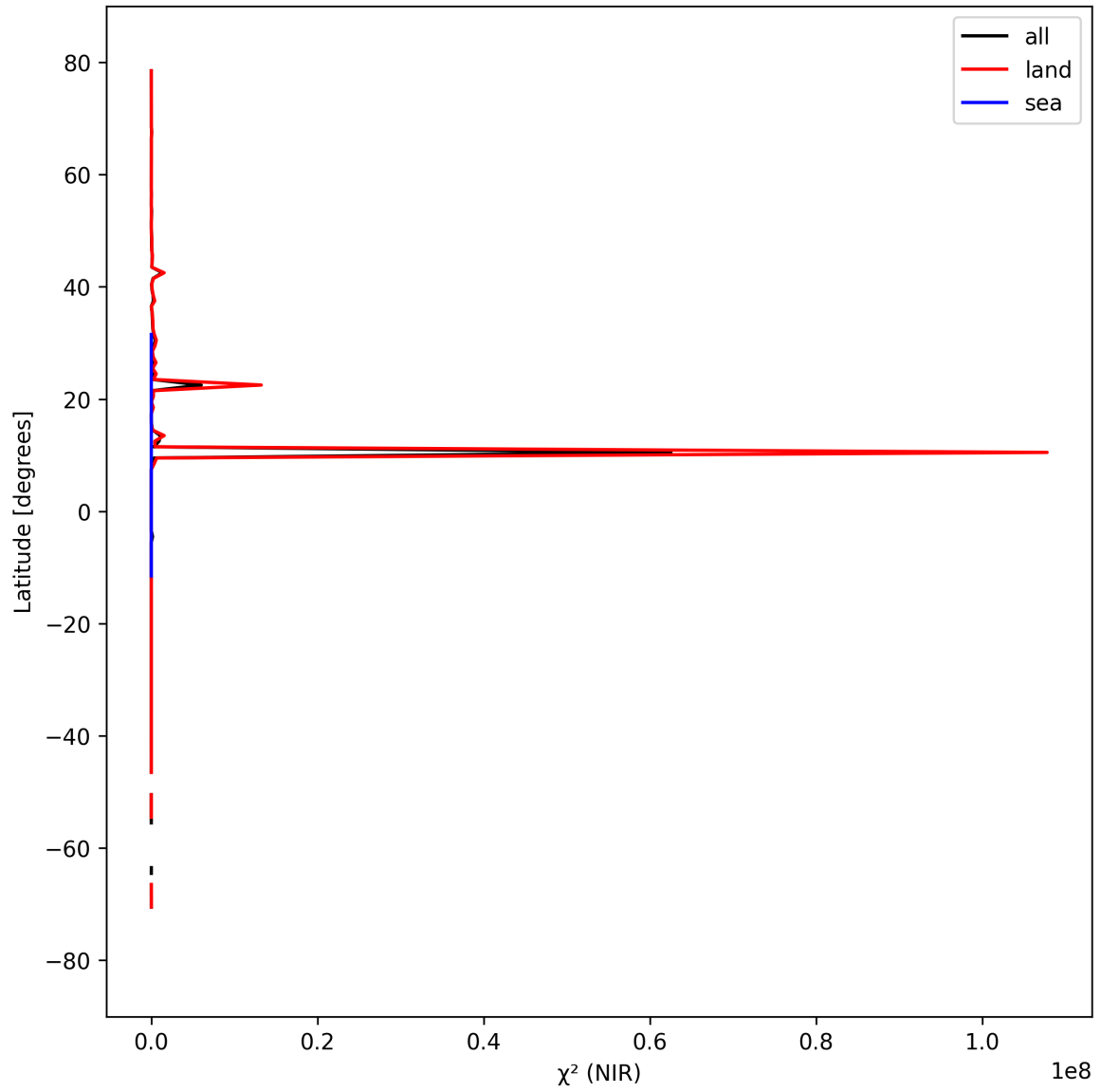
Figure 18: Zonal average of “ \chi^2 (NIR)” for 2025-03-28 to 2025-03-30.
