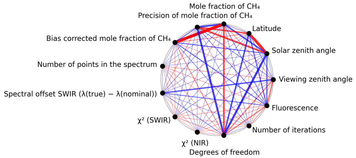
Figure 1: Map of correlation graph for 2025-03-28 to 2025-03-30.
