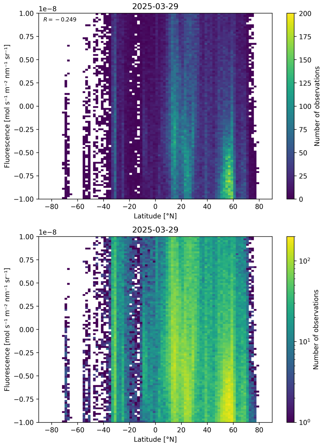
Figure 56: Scatter density plot of “Latitude” against “Fluorescence” for 2025-03-28 to 2025-03-30.
