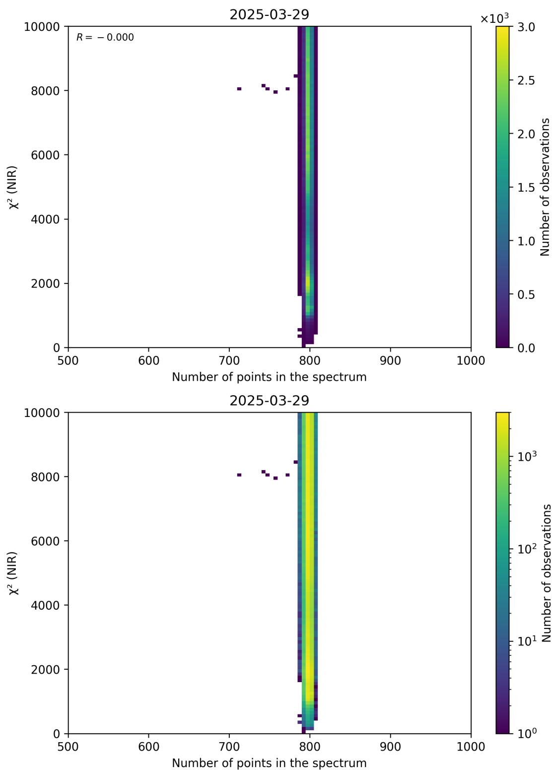
Figure 88: Scatter density plot of “Number of points in the spectrum” against “ \chi^2 (NIR)” for 2025-03-28 to 2025-03-30.
