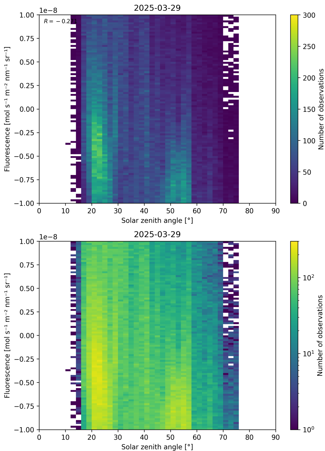
Figure 97: Scatter density plot of “Solar zenith angle” against “Fluorescence” for 2025-03-28 to 2025-03-30.
