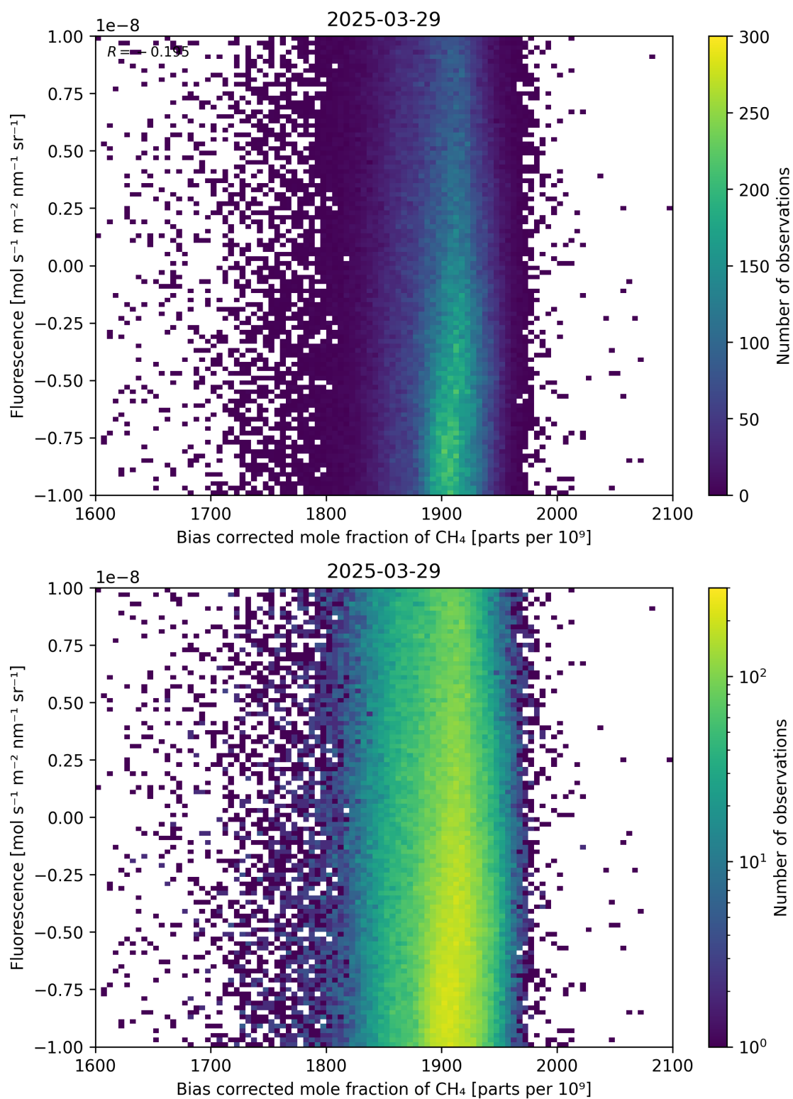
Figure 66: Scatter density plot of “Bias corrected mole fraction of \text{CH}_4 ” against “Fluorescence” for 2025-03-28 to 2025-03-30.
