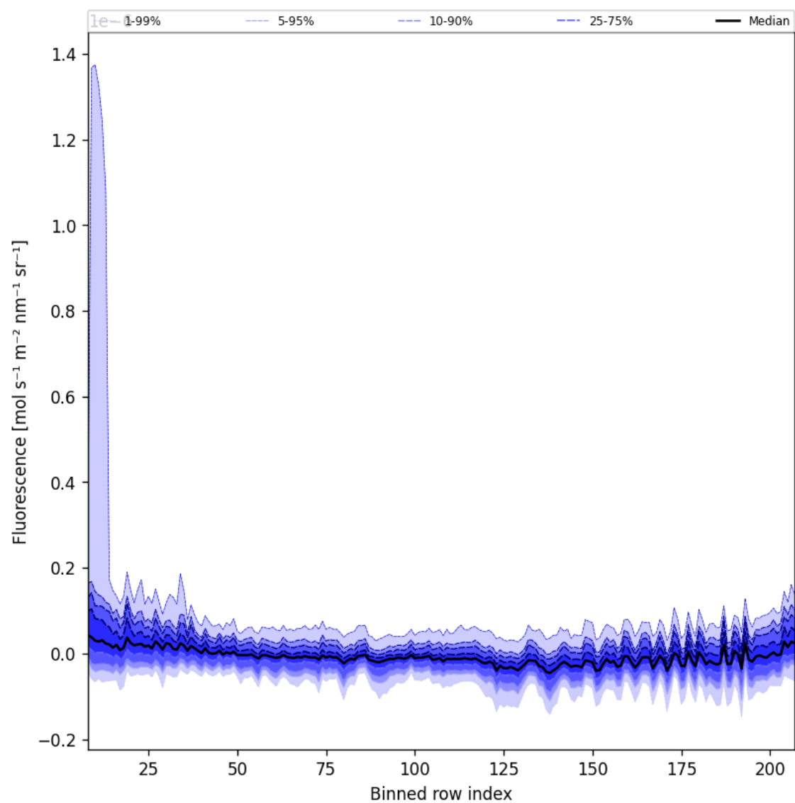
Figure 43: Along track statistics of “Fluorescence” for 2025-03-28 to 2025-03-30
