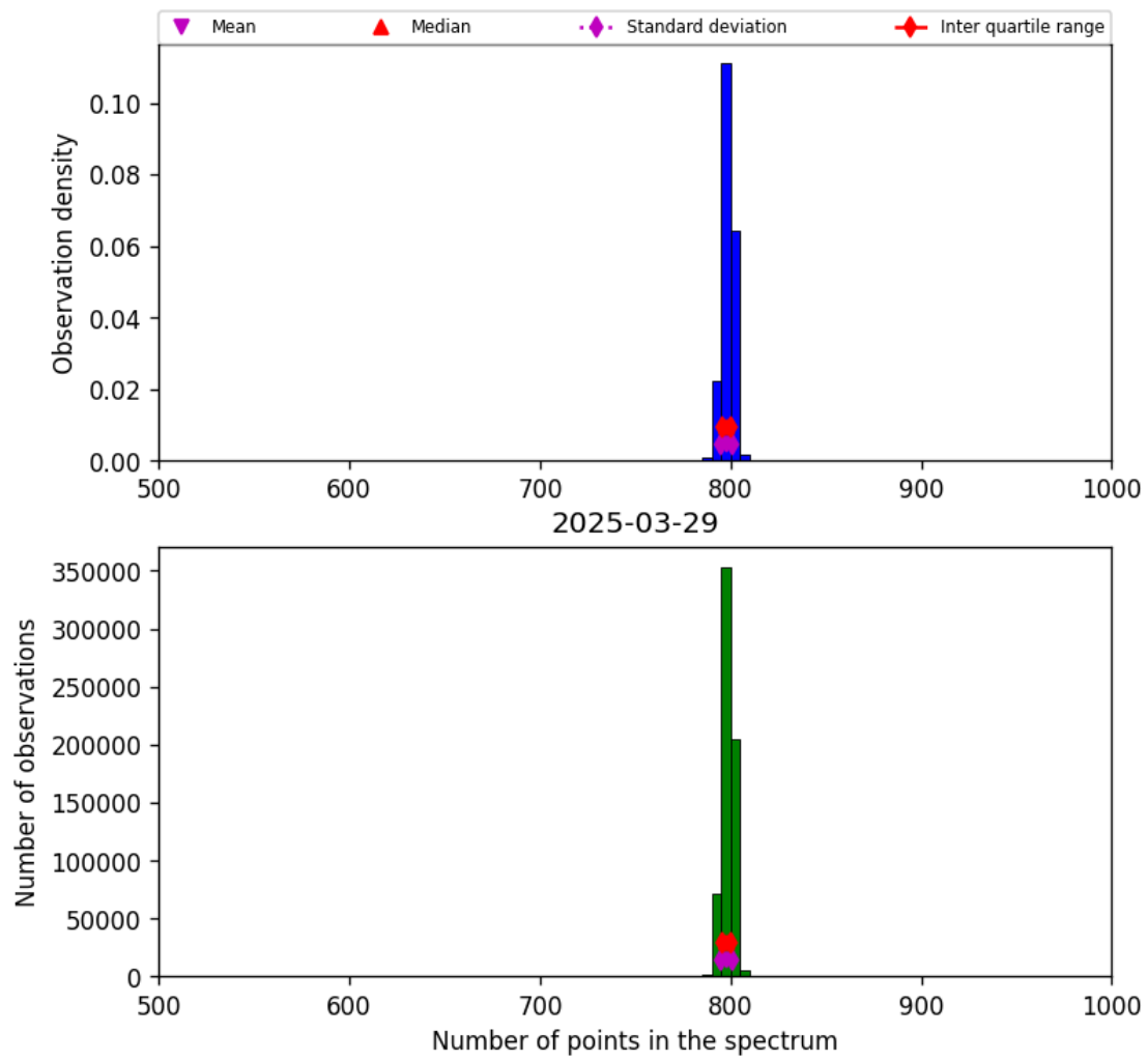
Figure 26: Histogram of “Number of points in the spectrum” for 2025-03-28 to 2025-03-30
