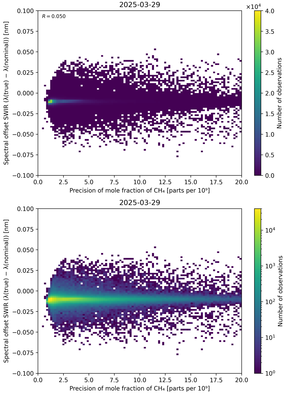
Figure 85: Scatter density plot of “Precision of mole fraction of CH 4 ” against “Spectral offset SWIR ( \lambda_{\text{true}} - \lambda_{\text{nominal}} )” for 2025-03-28 to 2025-03-30.
