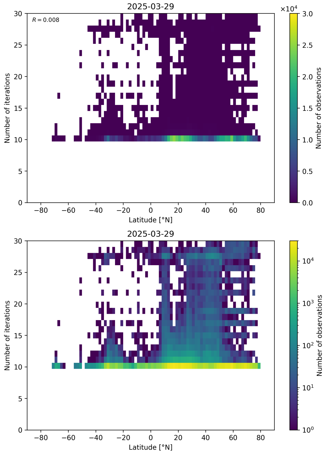
Figure 60: Scatter density plot of “Latitude” against “Number of iterations” for 2025-03-28 to 2025-03-30.
