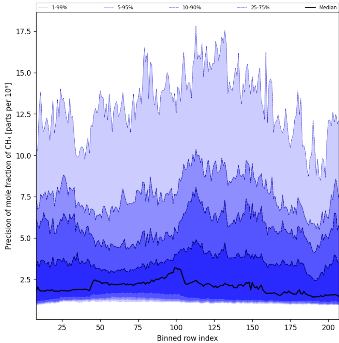
Figure 35: Along track statistics of “Precision of mole fraction of CH 4 ” for 2025-03-28 to 2025-03-30
