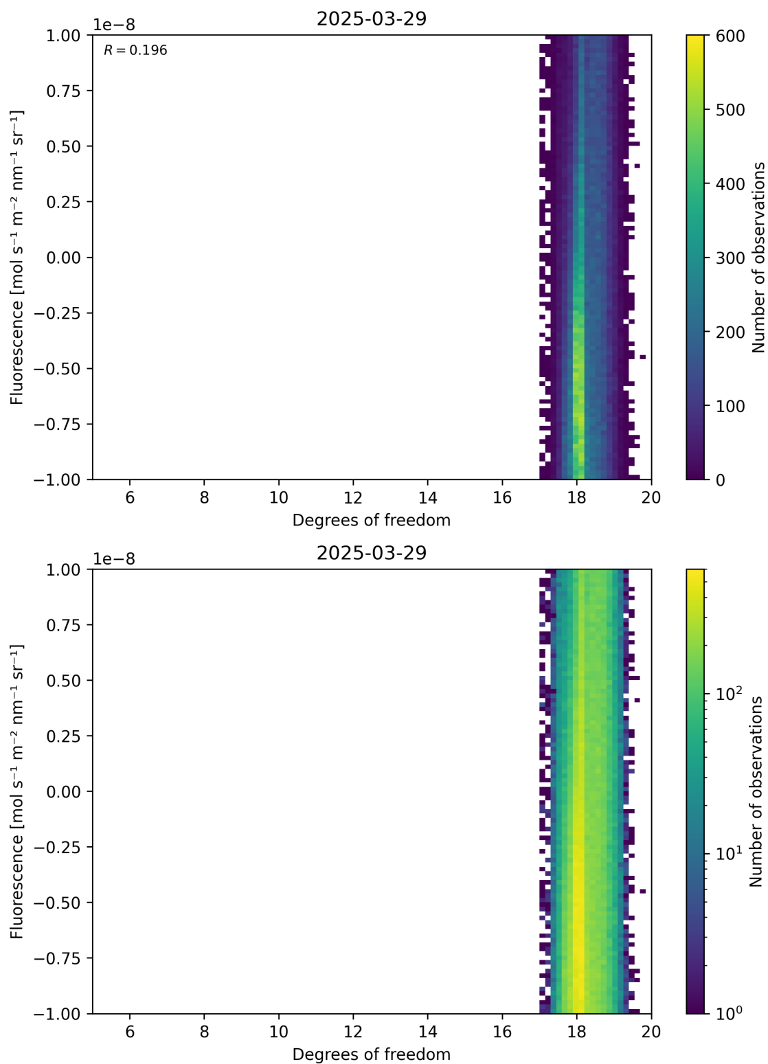
Figure 51: Scatter density plot of “Degrees of freedom” against “Fluorescence” for 2025-03-28 to 2025-03-30.
