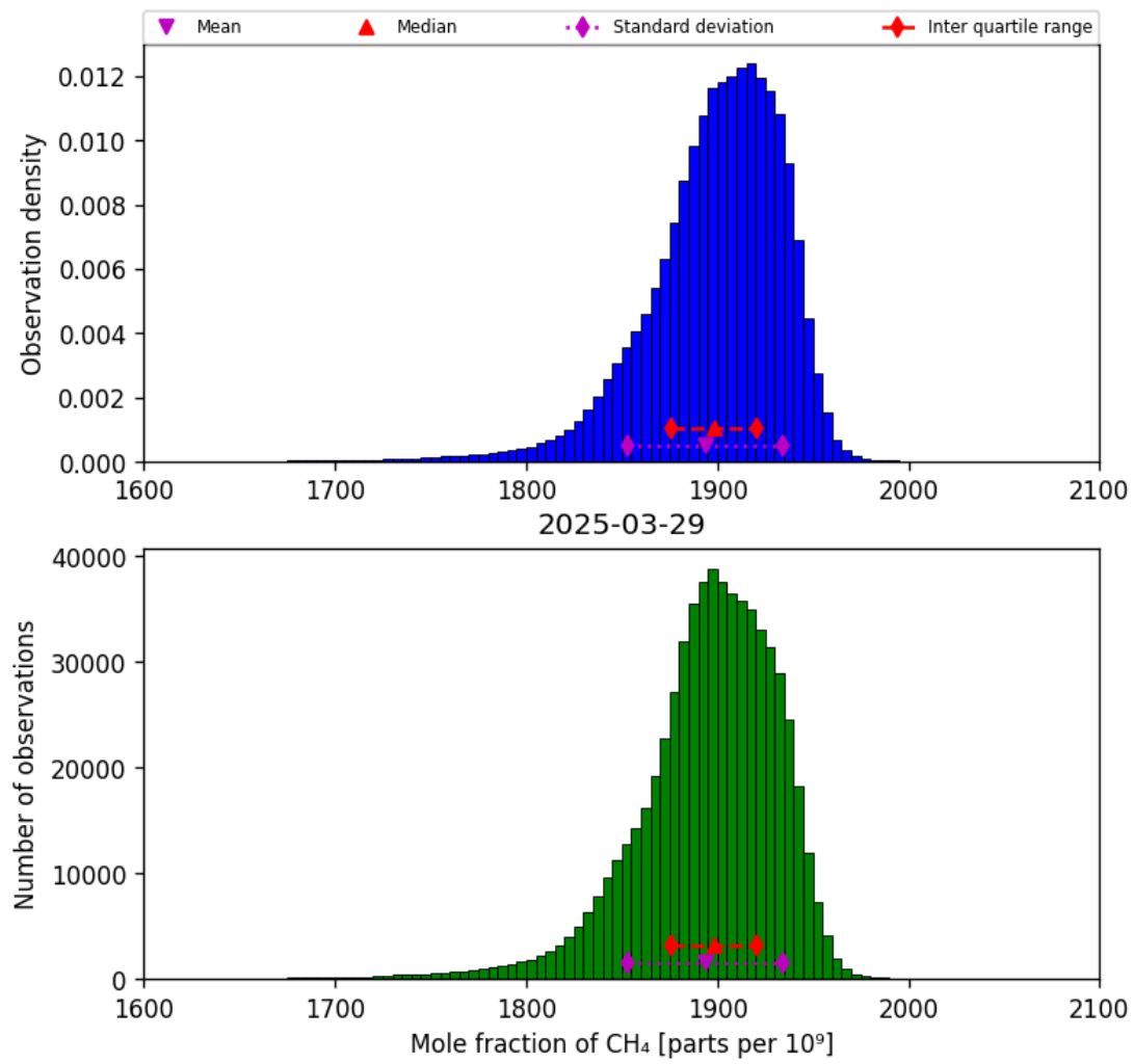
Figure 23: Histogram of “Mole fraction of CH 4 ” for 2025-03-28 to 2025-03-30
