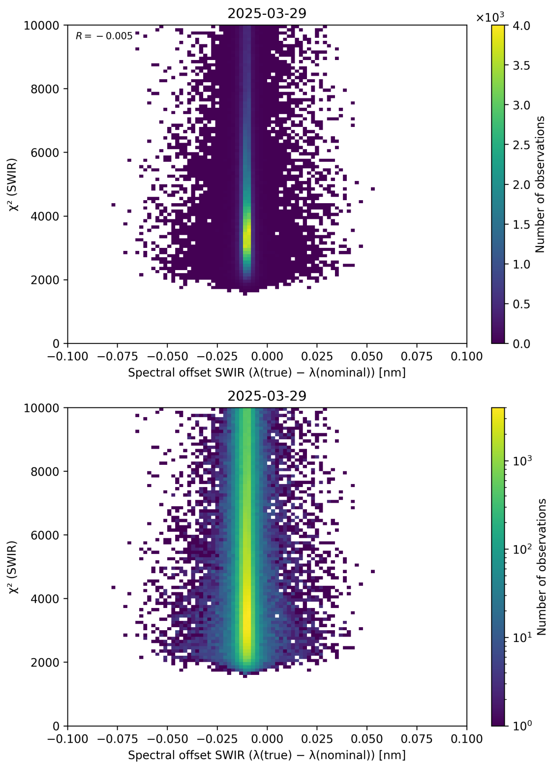
Figure 118: Scatter density plot of “Spectral offset SWIR ( \lambda_{\text{true}} - \lambda_{\text{nominal}} )” against “ \chi^2 (SWIR)” for 2025-03-28 to 2025-03-30.
