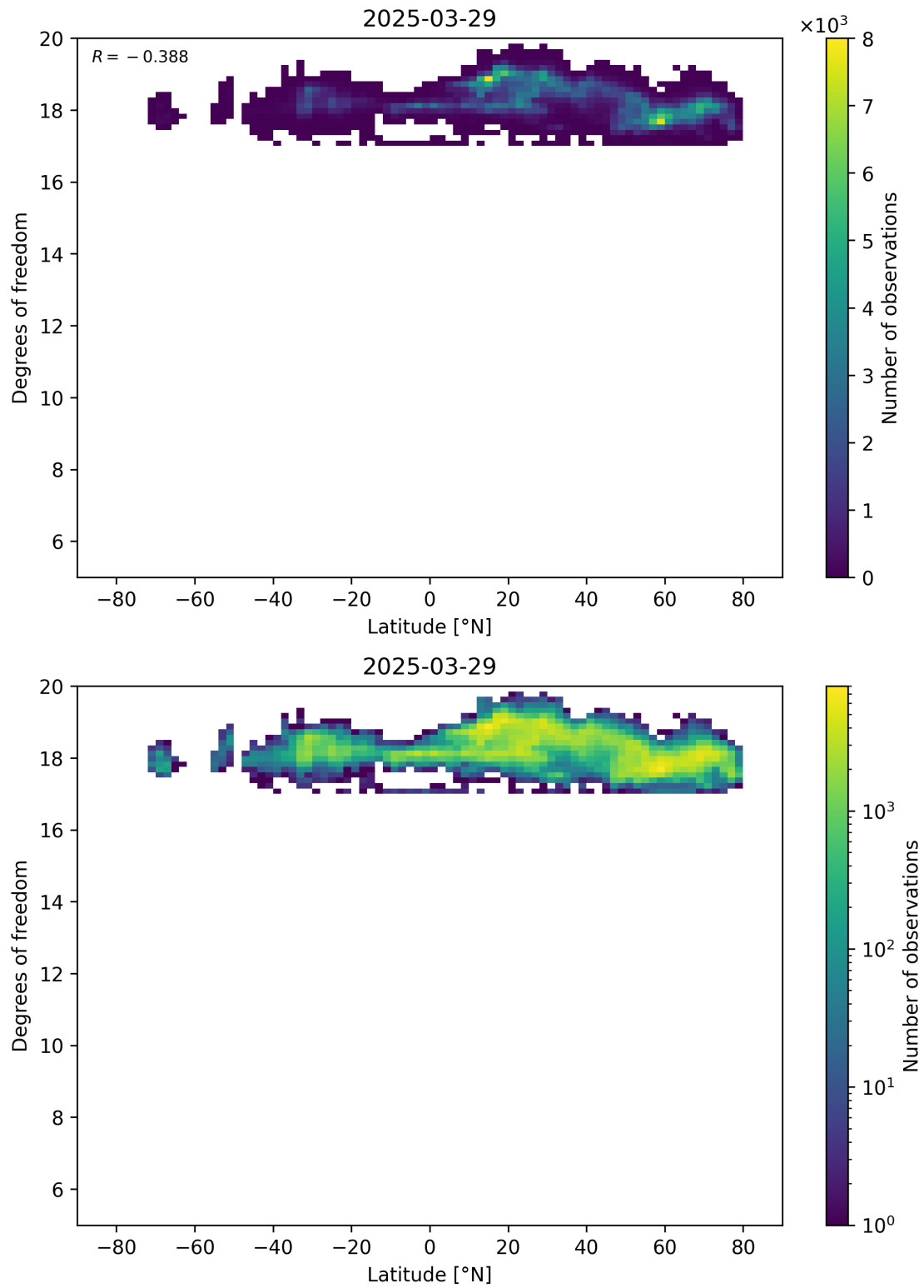
Figure 55: Scatter density plot of “Latitude” against “Degrees of freedom” for 2025-03-28 to 2025-03-30.
