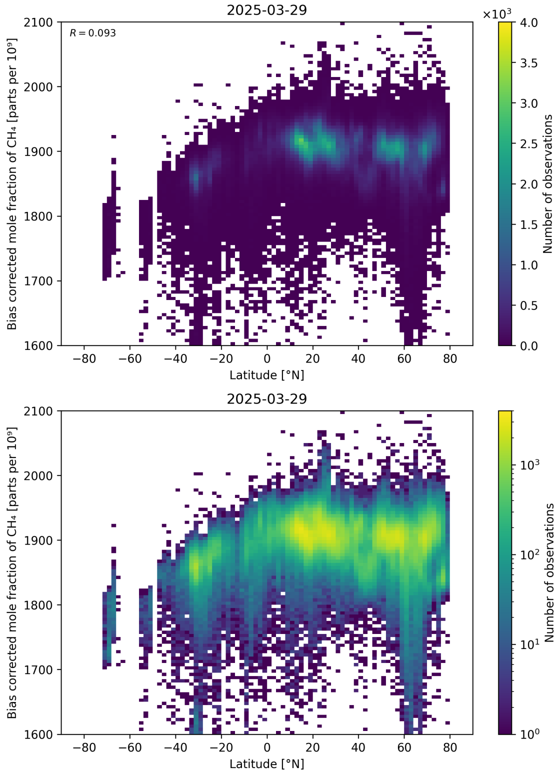
Figure 58: Scatter density plot of “Latitude” against “Bias corrected mole fraction of \text{CH}_4 ” for 2025-03-28 to 2025-03-30.
