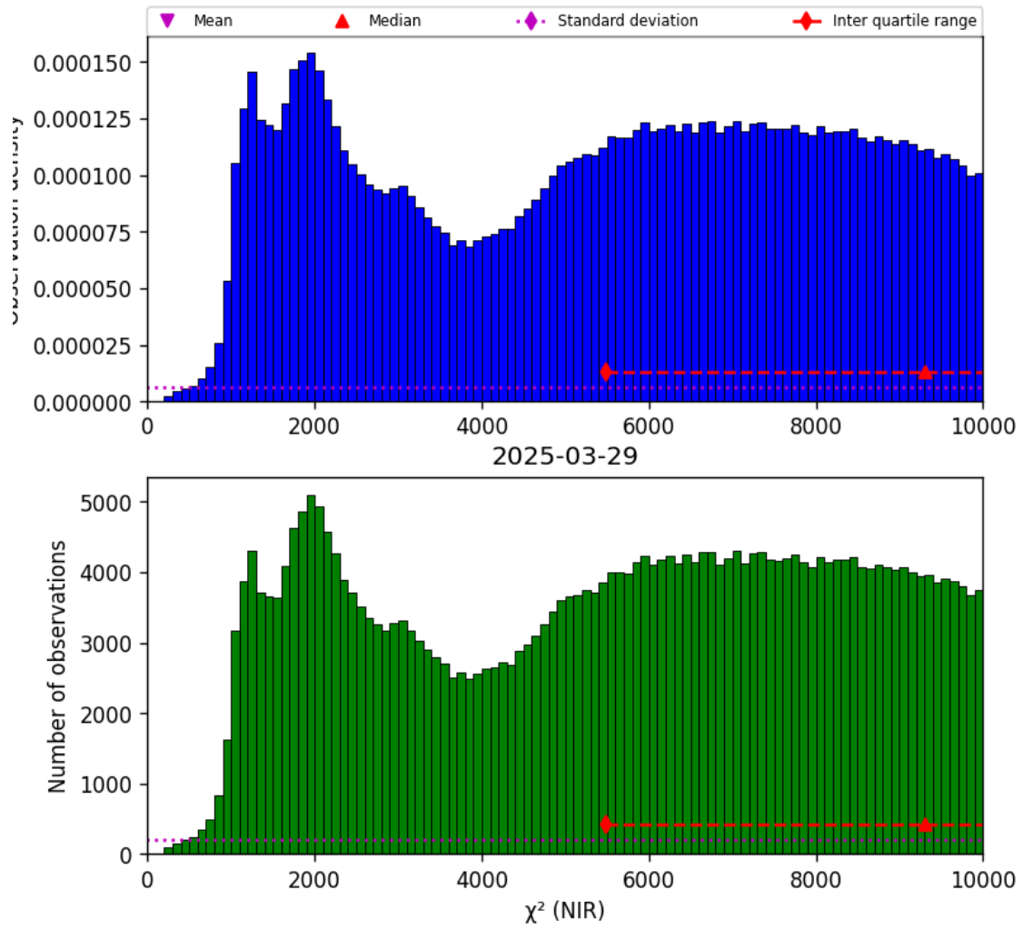
Figure 29: Histogram of “ \chi^2 (NIR)” for 2025-03-28 to 2025-03-30
