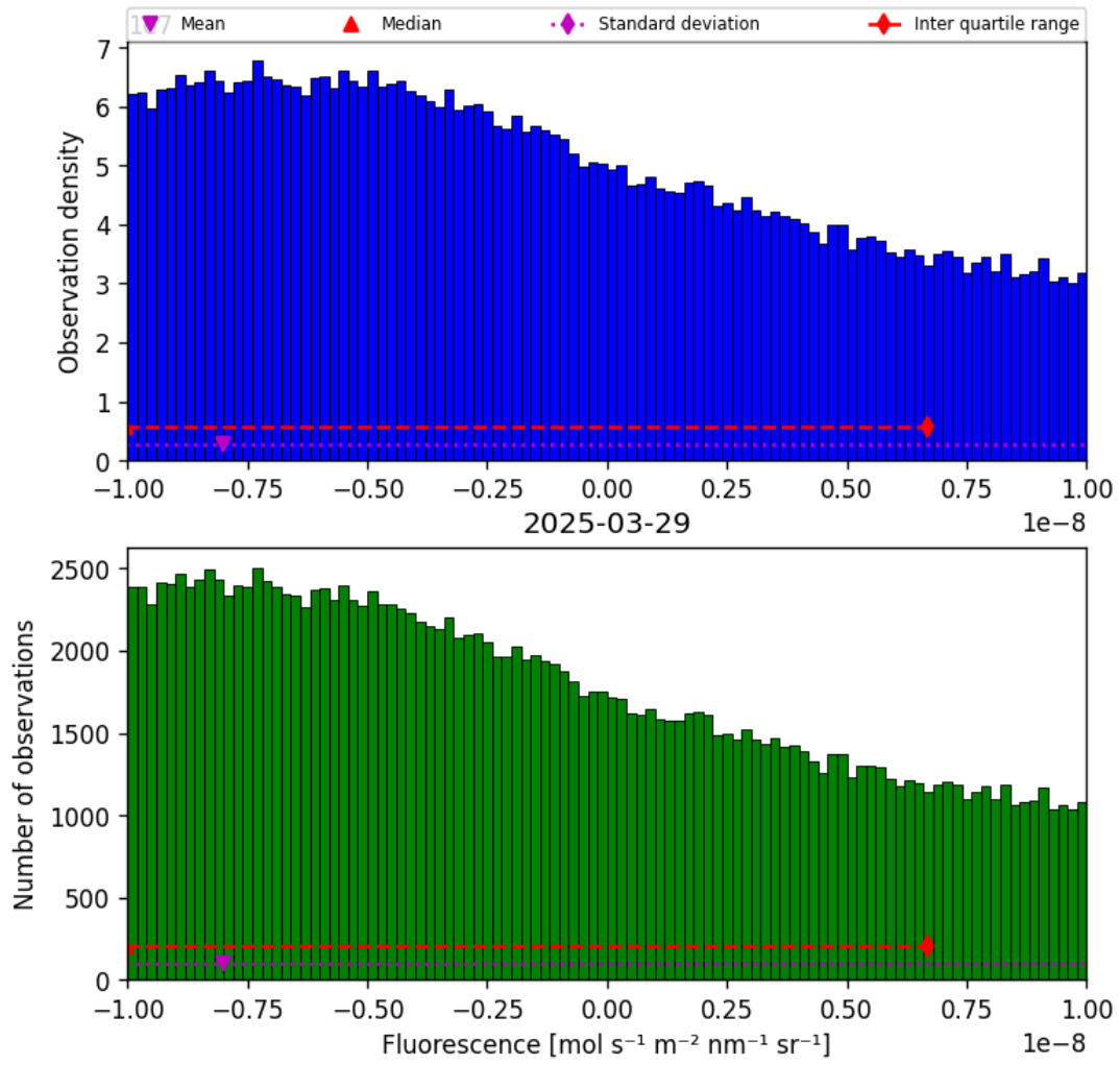
Figure 32: Histogram of “Fluorescence” for 2025-03-28 to 2025-03-30
