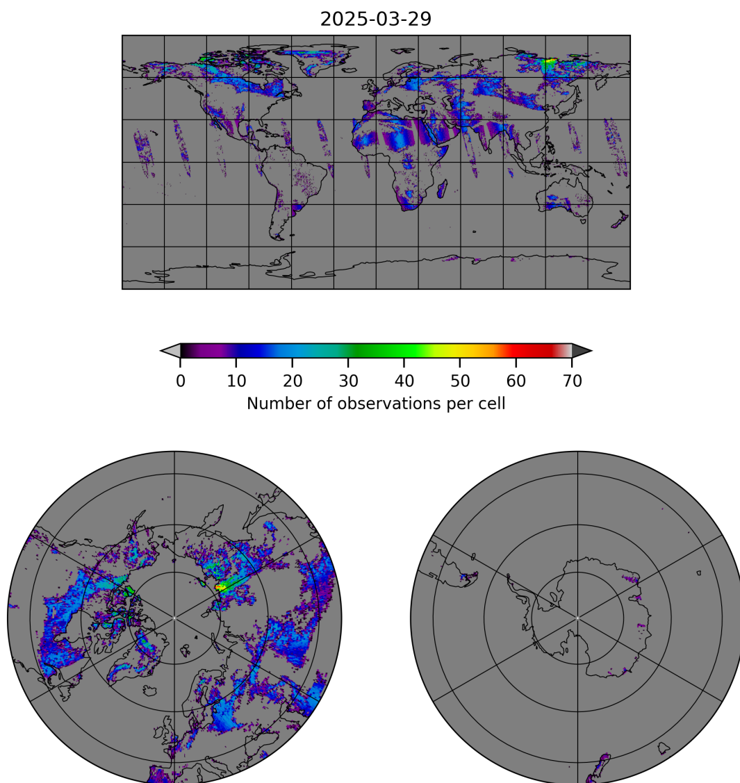
Figure 10: Map of the number of observations for 2025-03-28 to 2025-03-30
