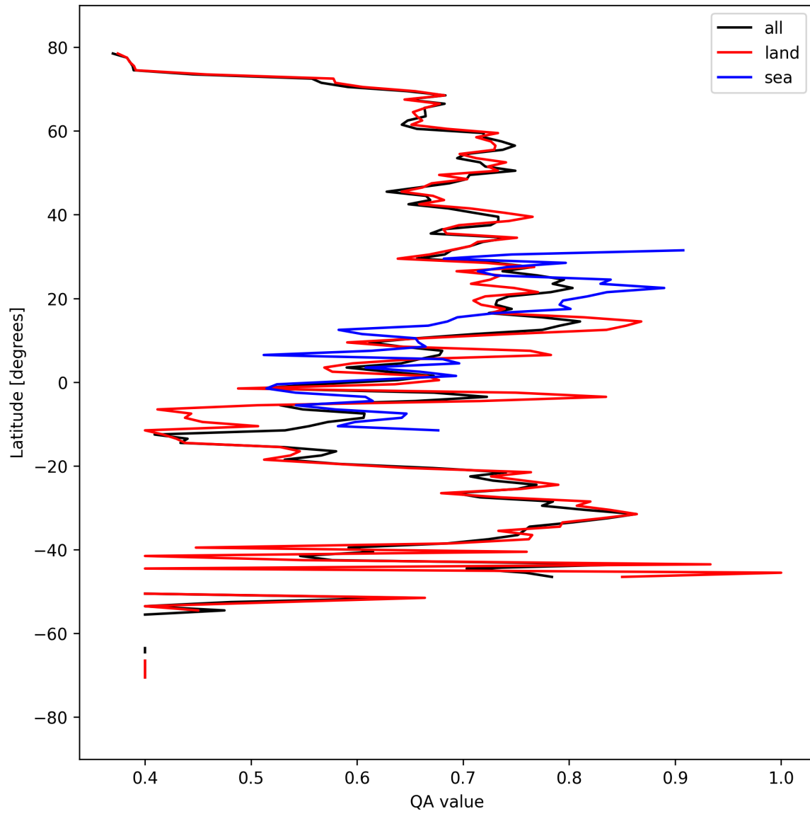
Figure 11: Zonal average of “QA value” for 2025-03-28 to 2025-03-30.
