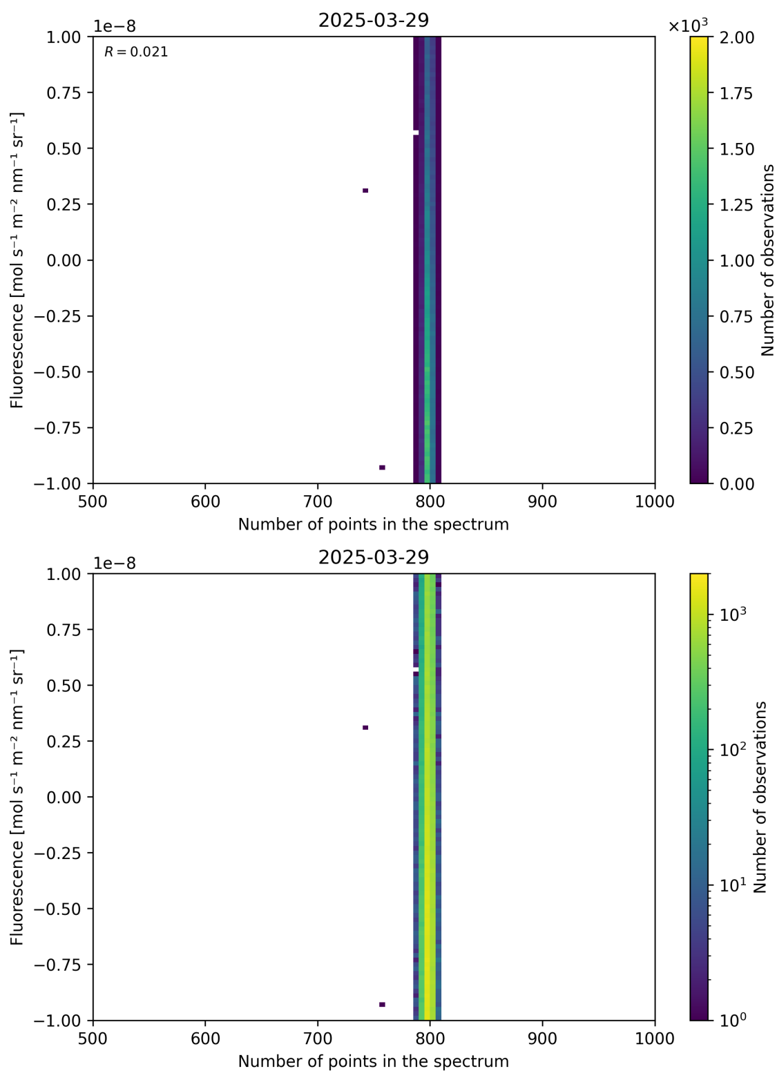
Figure 91: Scatter density plot of “Number of points in the spectrum” against “Fluorescence” for 2025-03-28 to 2025-03-30.
