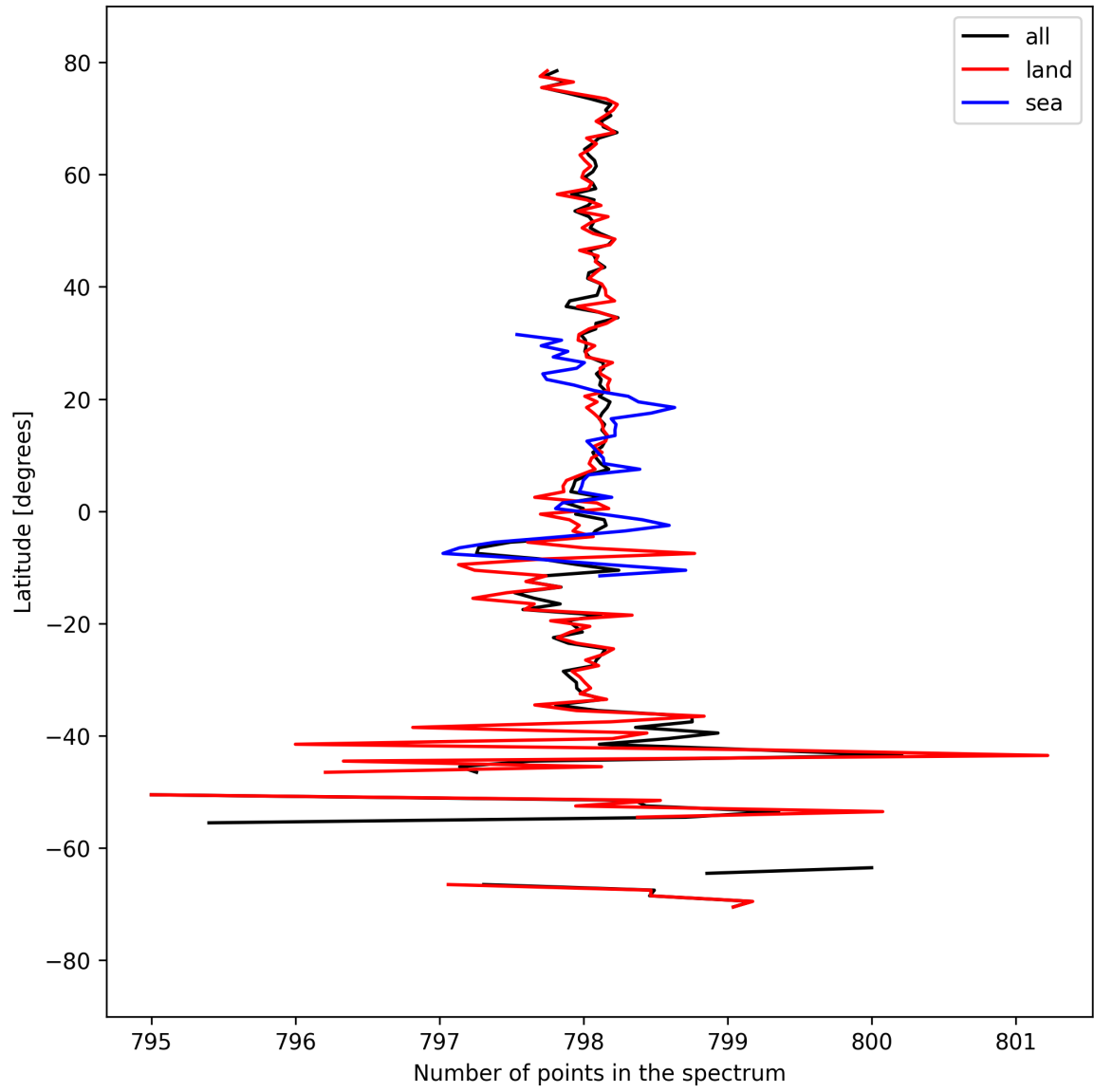
Figure 15: Zonal average of “Number of points in the spectrum” for 2025-03-28 to 2025-03-30.
