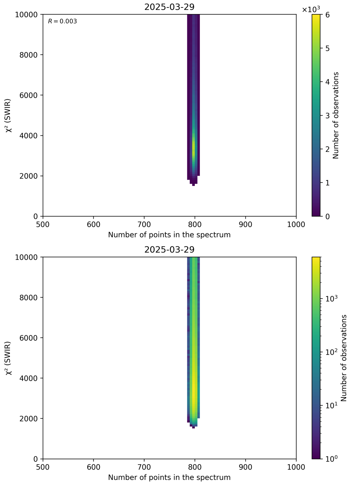
Figure 89: Scatter density plot of “Number of points in the spectrum” against “ \chi^2 (SWIR)” for 2025-03-28 to 2025-03-30.
