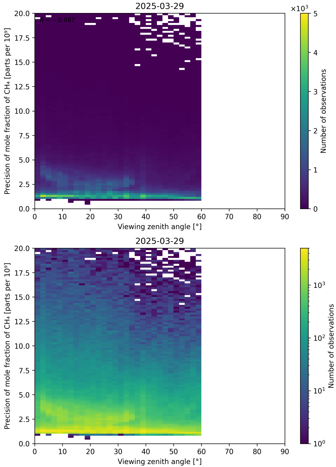
Figure 112: Scatter density plot of “Viewing zenith angle” against “Precision of mole fraction of CH 4 ” for 2025-03-28 to 2025-03-30.
