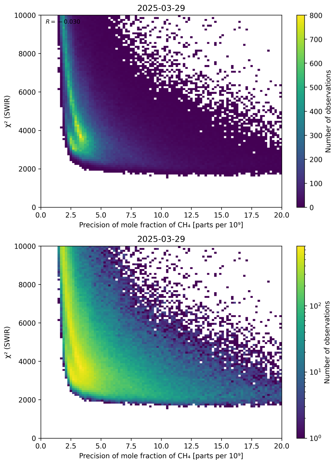
Figure 79: Scatter density plot of “Precision of mole fraction of \text{CH}_4 ” against “ \chi^2 (SWIR)” for 2025-03-28 to 2025-03-30.
