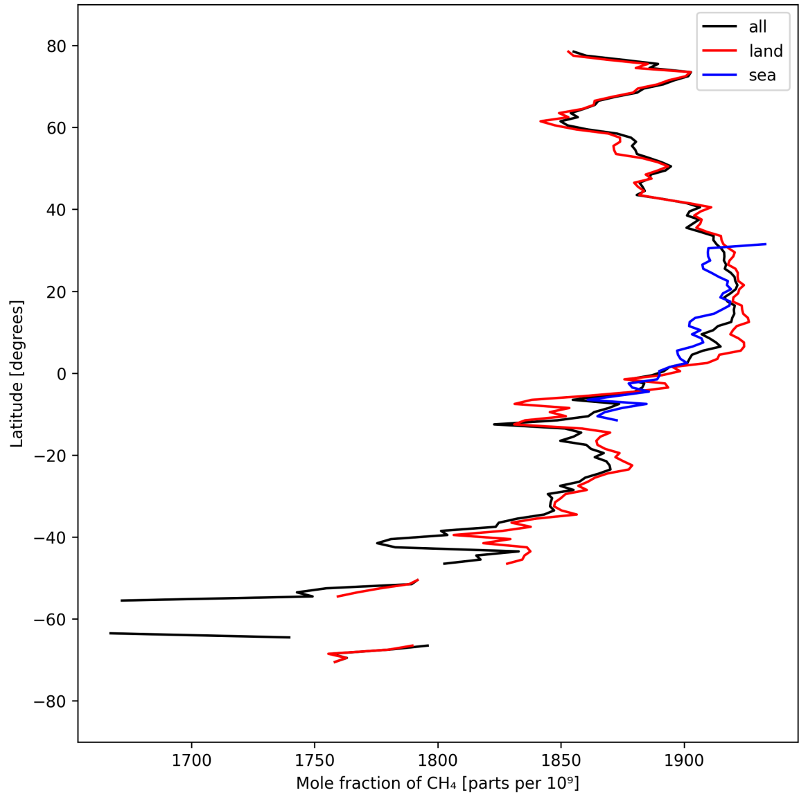
Figure 12: Zonal average of “Mole fraction of CH 4 ” for 2025-03-28 to 2025-03-30.
