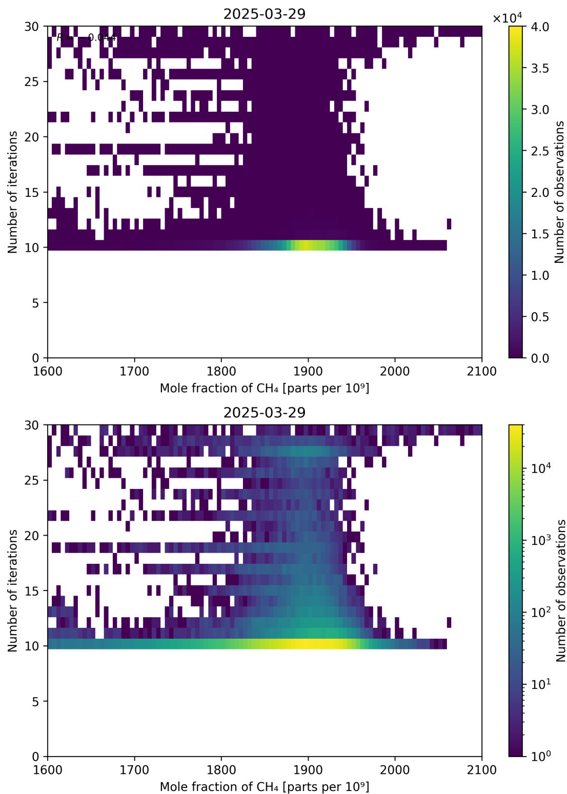
Figure 76: Scatter density plot of “Mole fraction of CH 4 ” against “Number of iterations” for 2025-03-28 to 2025-03-30.
