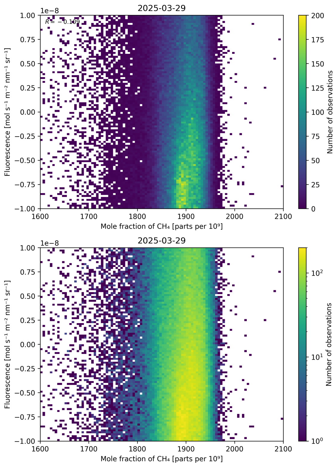
Figure 73: Scatter density plot of “Mole fraction of \text{CH}_4 ” against “Fluorescence” for 2025-03-28 to 2025-03-30.
