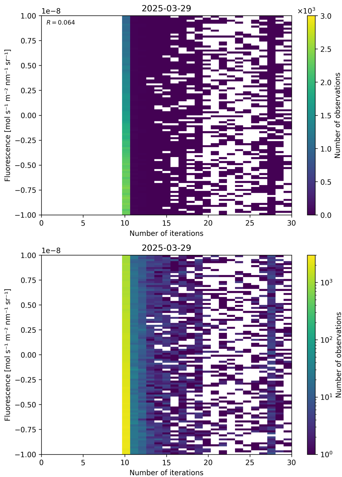
Figure 87: Scatter density plot of “Number of iterations” against “Fluorescence” for 2025-03-28 to 2025-03-30.
