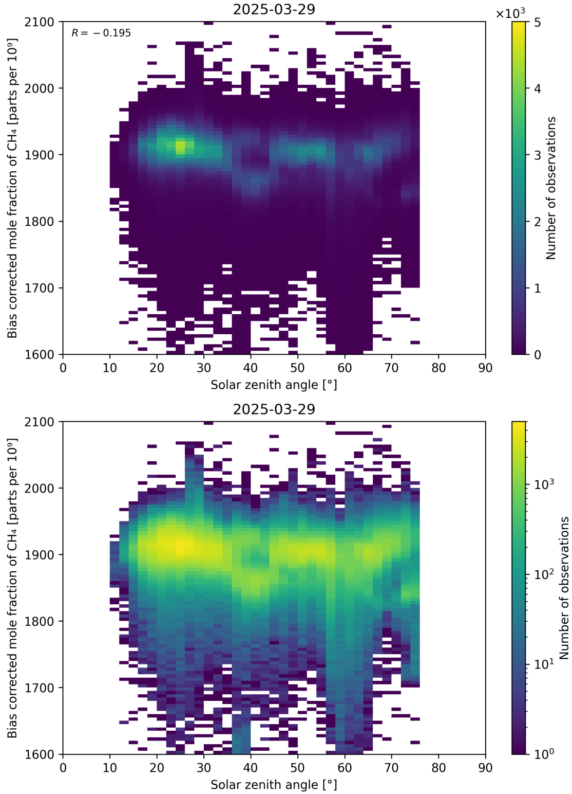
Figure 100: Scatter density plot of “Solar zenith angle” against “Bias corrected mole fraction of CH 4 ” for 2025-03-28 to 2025-03-30.
