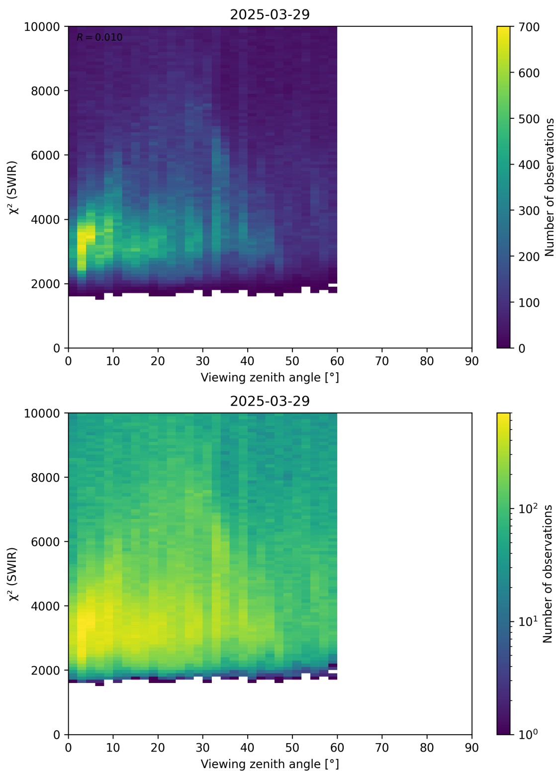
Figure 106: Scatter density plot of “Viewing zenith angle” against “ \chi^2 (SWIR)” for 2025-03-28 to 2025-03-30.
