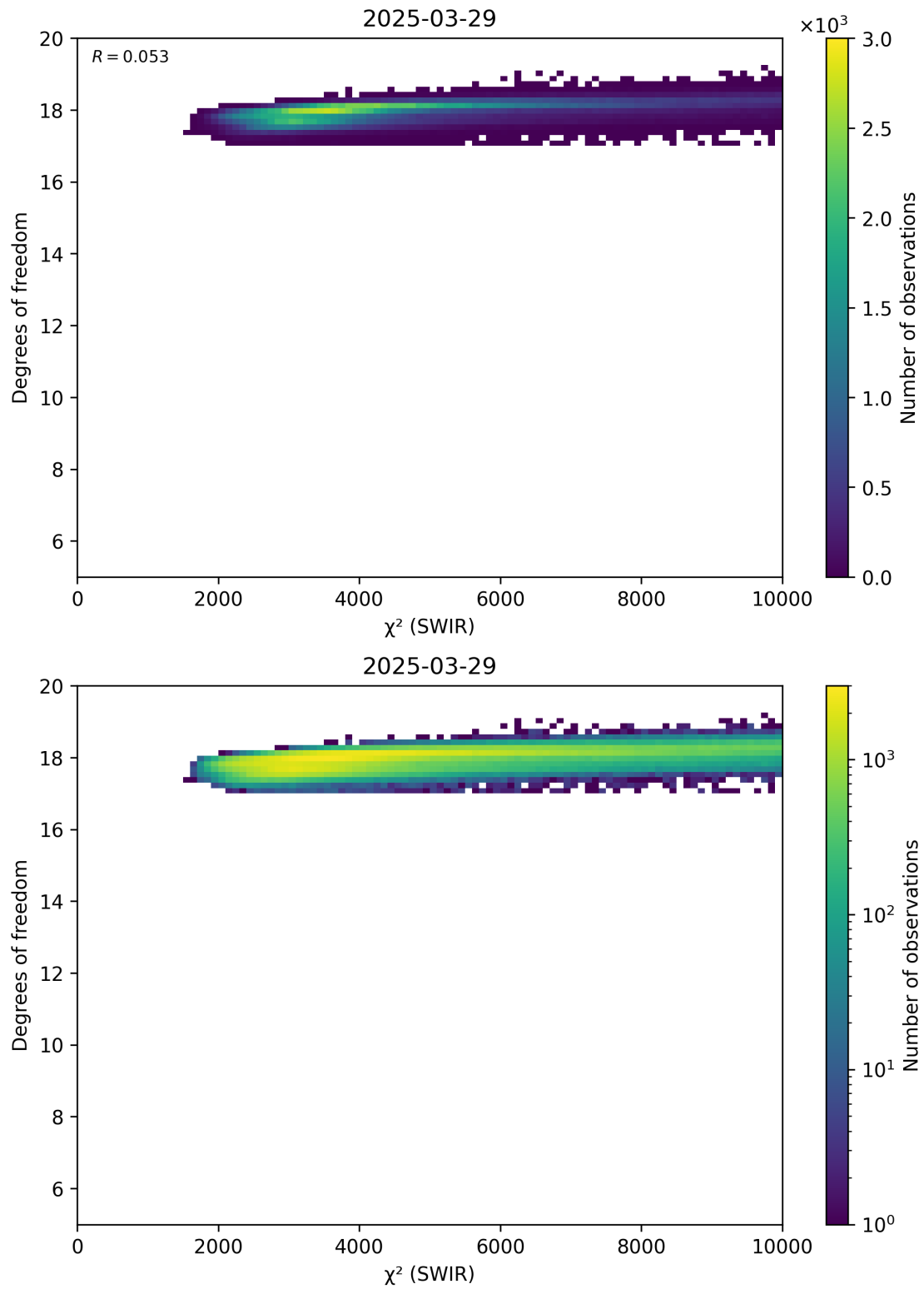
Figure 48: Scatter density plot of “ \chi^2 (SWIR)” against “Degrees of freedom” for 2025-03-28 to 2025-03-30.
