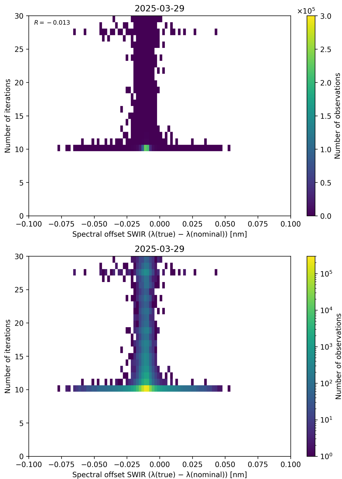
Figure 121: Scatter density plot of “Spectral offset SWIR ( \lambda_{\text{true}} - \lambda_{\text{nominal}} )” against “Number of iterations” for 2025-03-28 to 2025-03-30.
