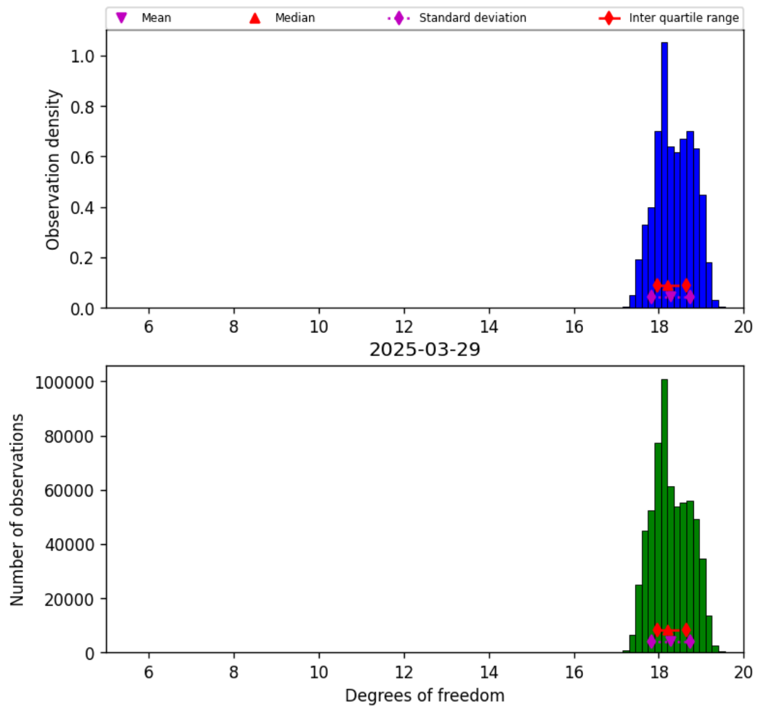
Figure 30: Histogram of “Degrees of freedom” for 2025-03-28 to 2025-03-30
