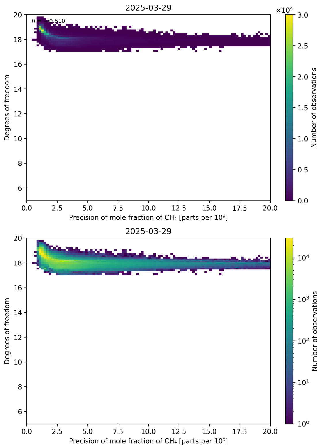
Figure 80: Scatter density plot of “Precision of mole fraction of CH 4 ” against “Degrees of freedom” for 2025-03-28 to 2025-03-30.
