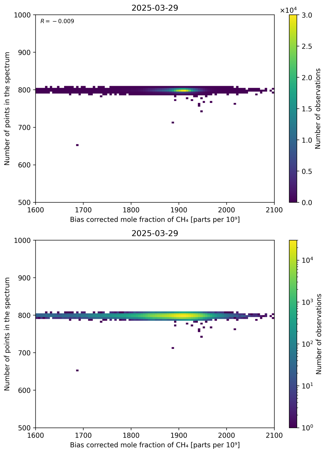
Figure 68: Scatter density plot of “Bias corrected mole fraction of CH 4 ” against “Number of points in the spectrum” for 2025-03-28 to 2025-03-30.
