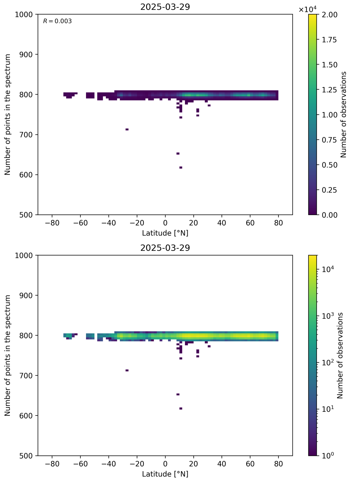
Figure 61: Scatter density plot of “Latitude” against “Number of points in the spectrum” for 2025-03-28 to 2025-03-30.
