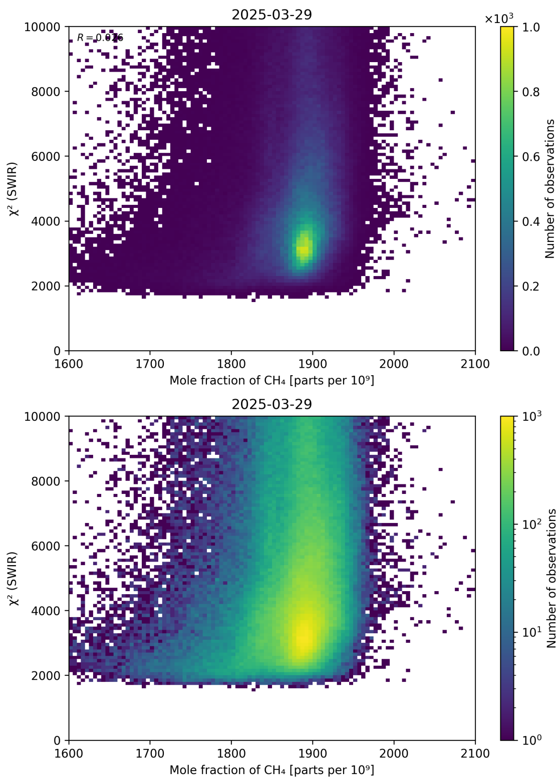
Figure 71: Scatter density plot of “Mole fraction of \text{CH}_4 ” against “ \chi^2 (SWIR)” for 2025-03-28 to 2025-03-30.
