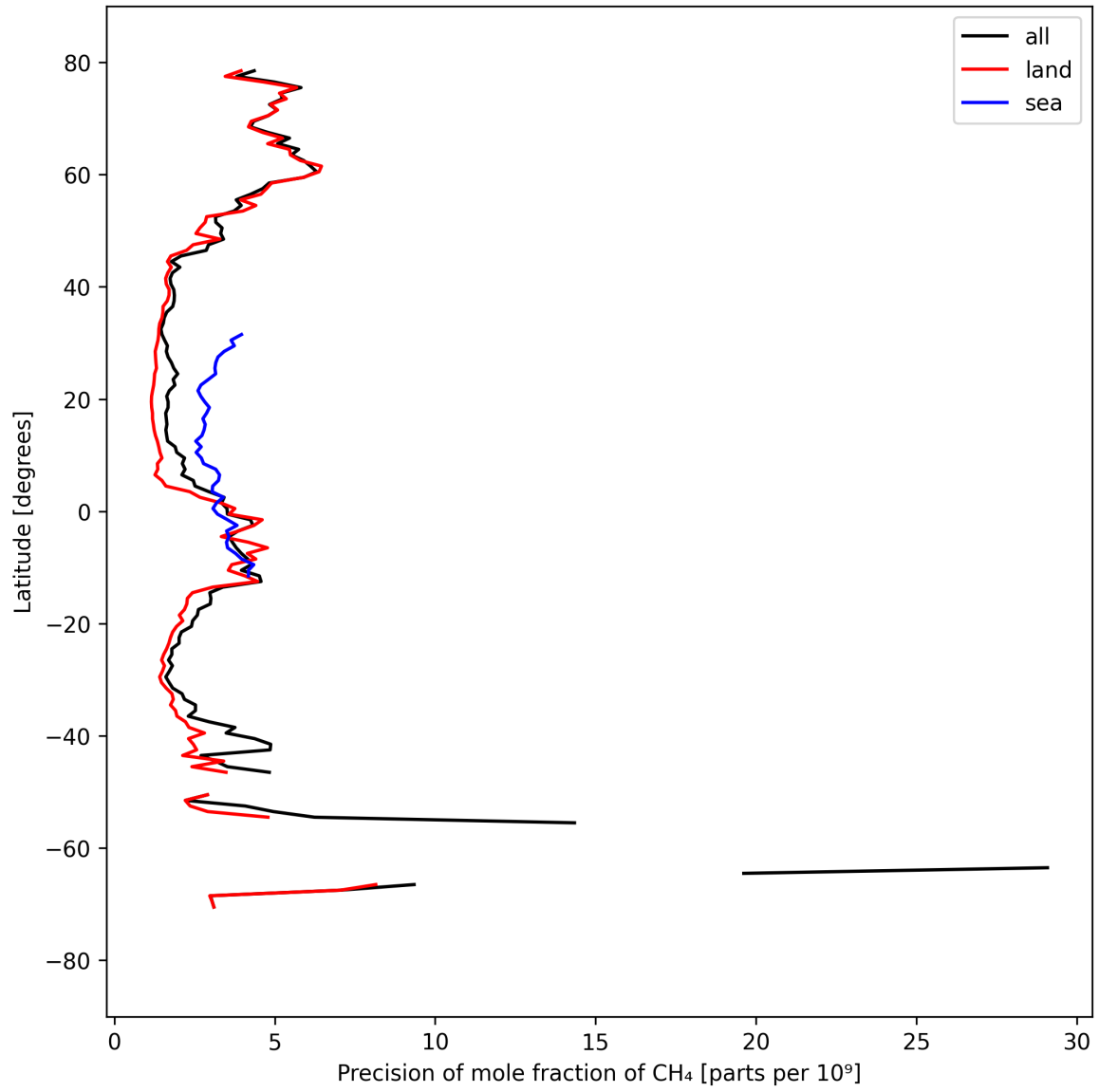
Figure 13: Zonal average of “Precision of mole fraction of CH 4 ” for 2025-03-28 to 2025-03-30.
