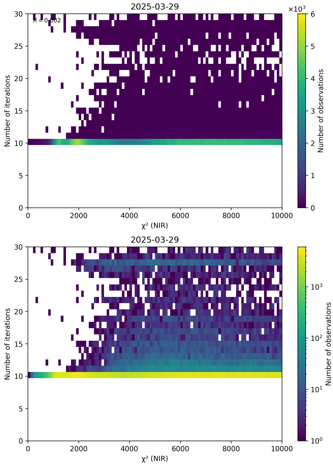
Figure 46: Scatter density plot of “ \chi^2 (NIR)” against “Number of iterations” for 2025-03-28 to 2025-03-30.
