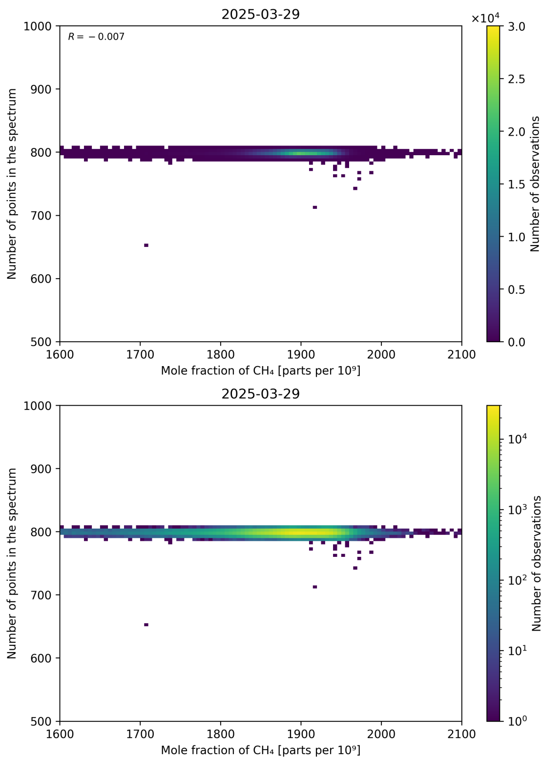
Figure 77: Scatter density plot of “Mole fraction of CH 4 ” against “Number of points in the spectrum” for 2025-03-28 to 2025-03-30.
