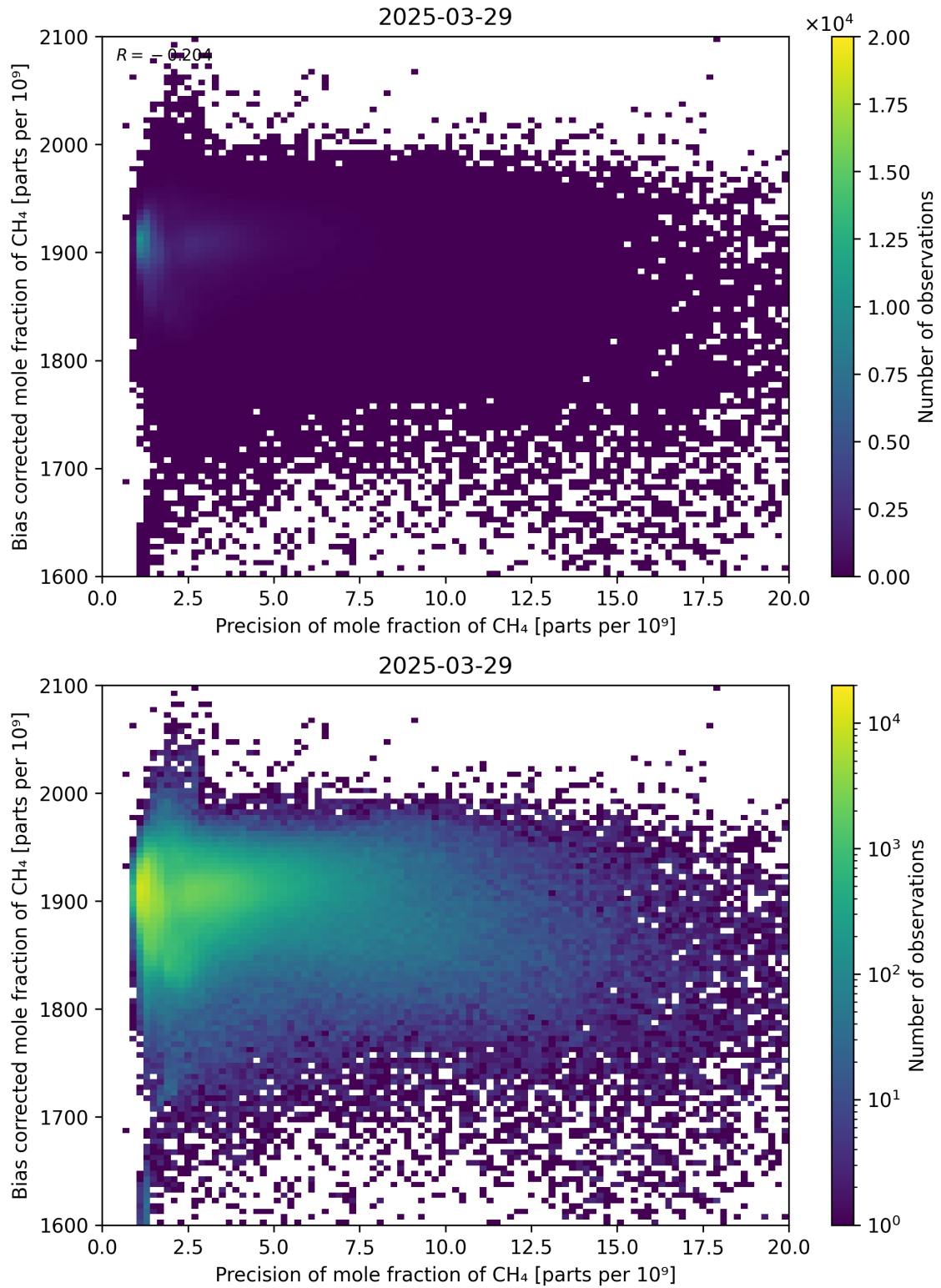
Figure 82: Scatter density plot of “Precision of mole fraction of CH 4 ” against “Bias corrected mole fraction of CH 4 ” for 2025-03-28 to 2025-03-30.
