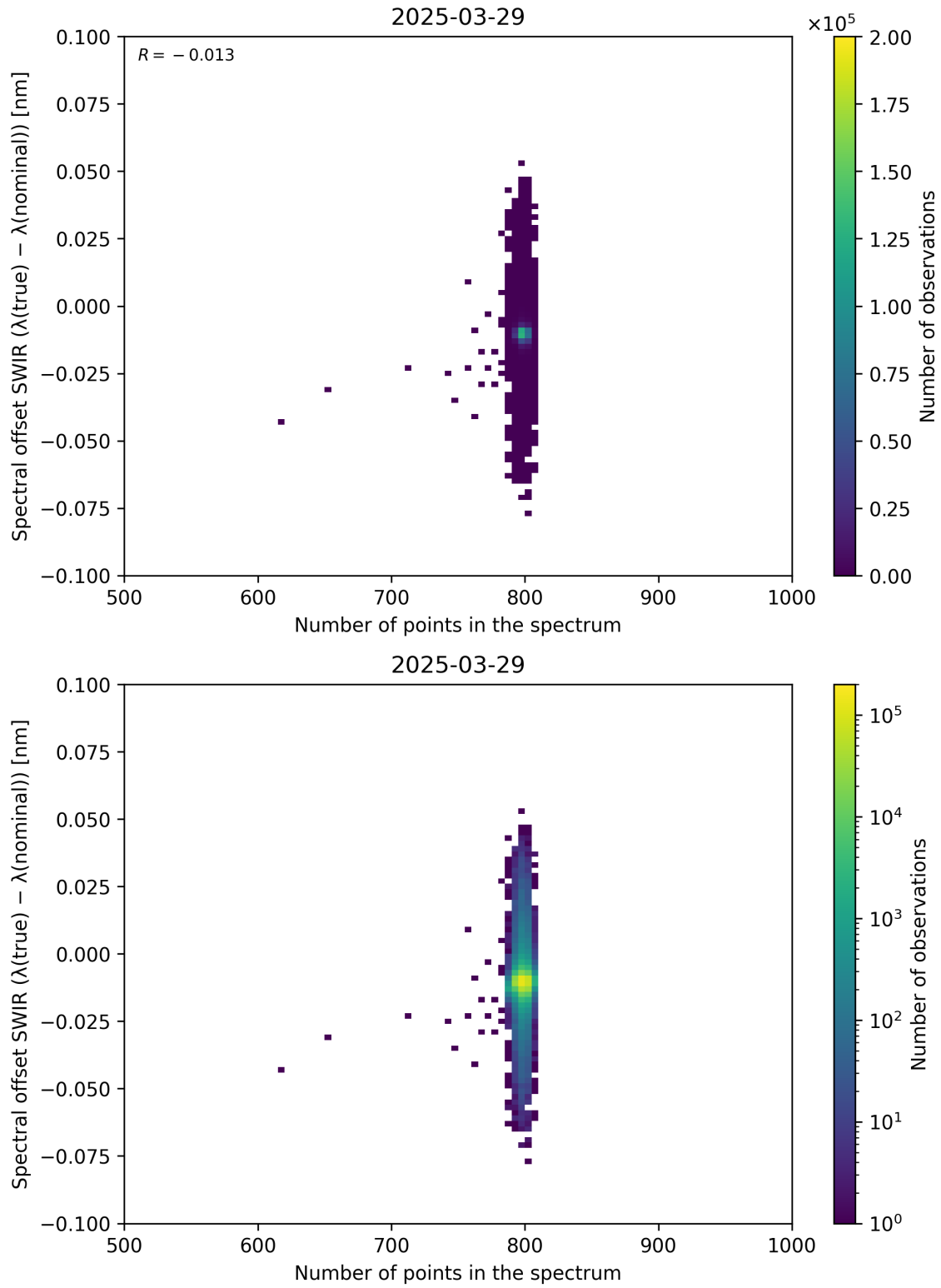
Figure 93: Scatter density plot of “Number of points in the spectrum” against “Spectral offset SWIR ( \lambda_{\text{true}} - \lambda_{\text{nominal}} )” for 2025-03-28 to 2025-03-30.
