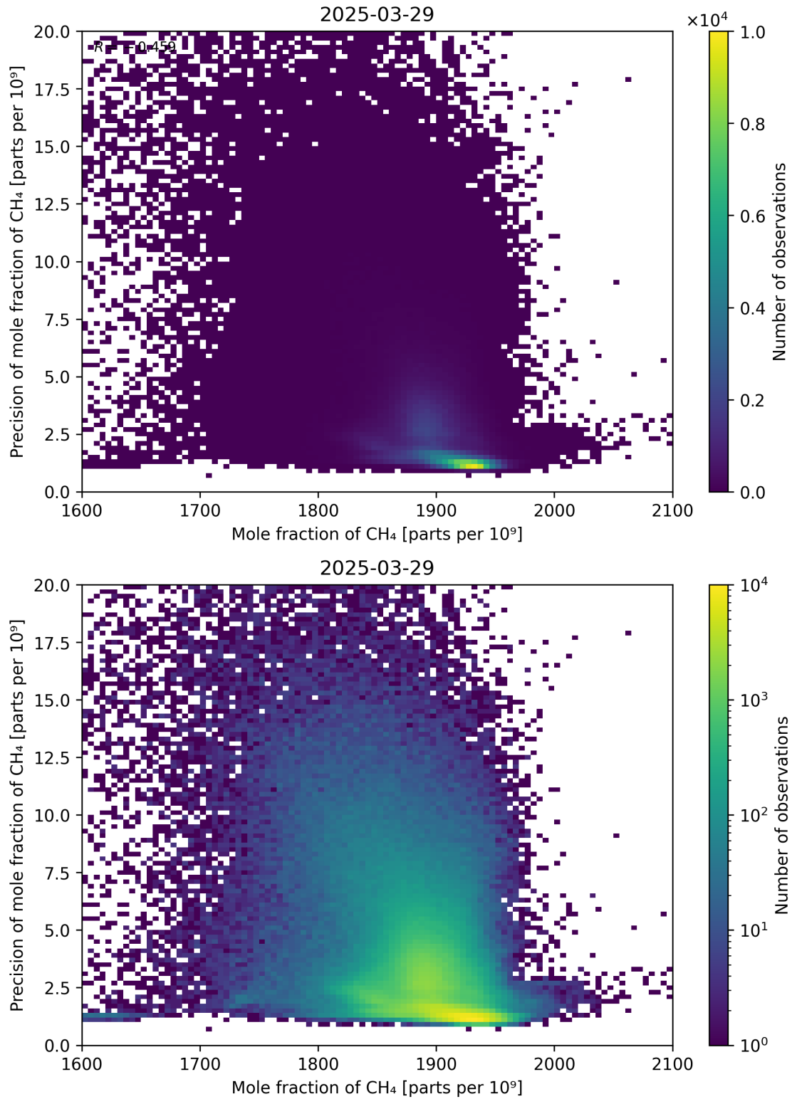
Figure 75: Scatter density plot of “Mole fraction of CH 4 ” against “Precision of mole fraction of CH 4 ” for 2025-03-28 to 2025-03-30.
