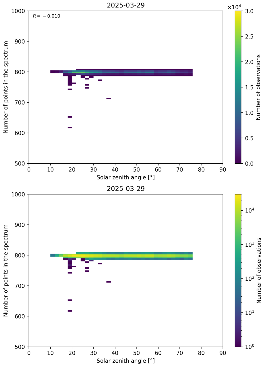
Figure 103: Scatter density plot of “Solar zenith angle” against “Number of points in the spectrum” for 2025-03-28 to 2025-03-30.
