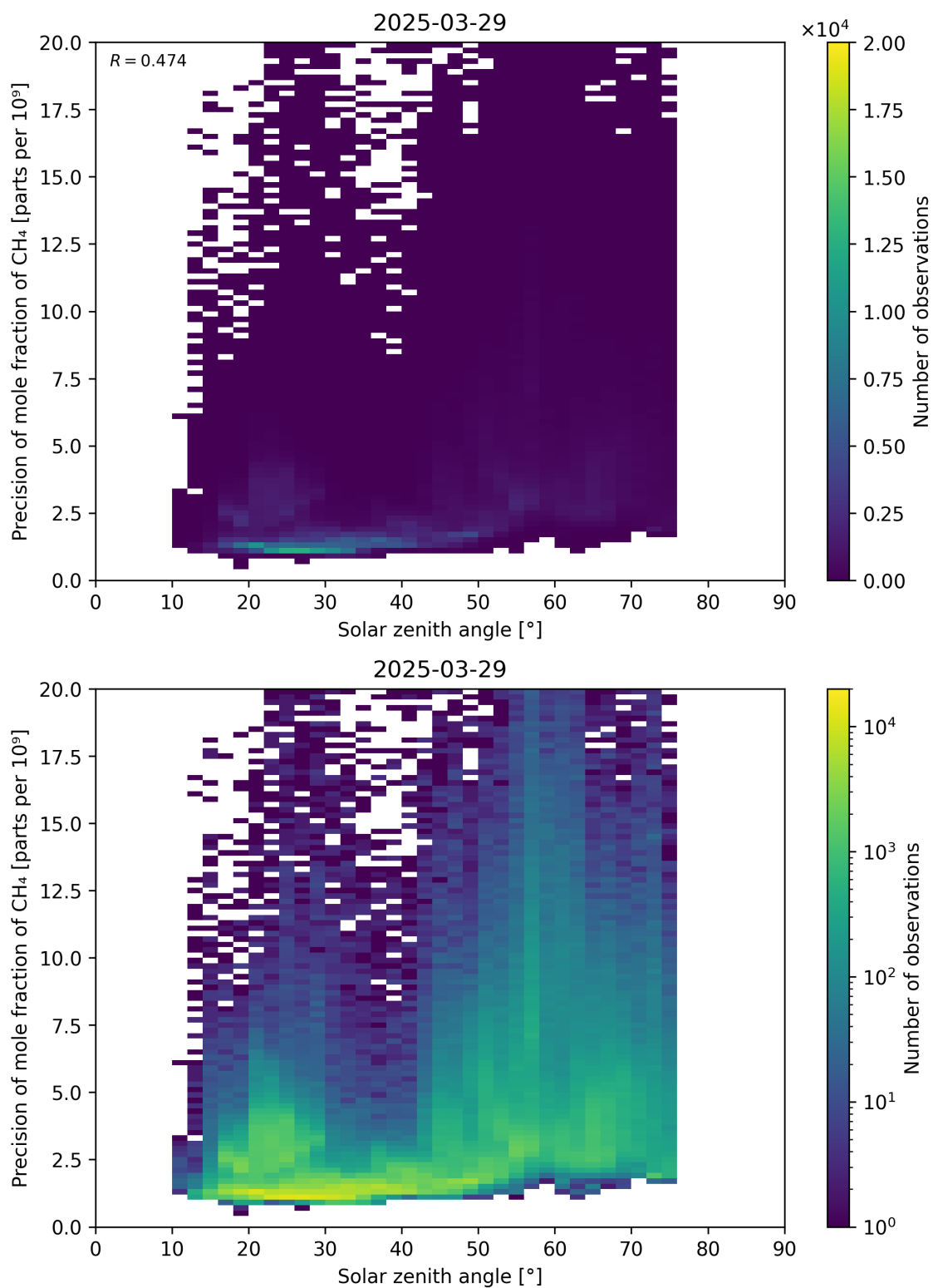
Figure 101: Scatter density plot of “Solar zenith angle” against “Precision of mole fraction of \text{CH}_4 ” for 2025-03-28 to 2025-03-30.
