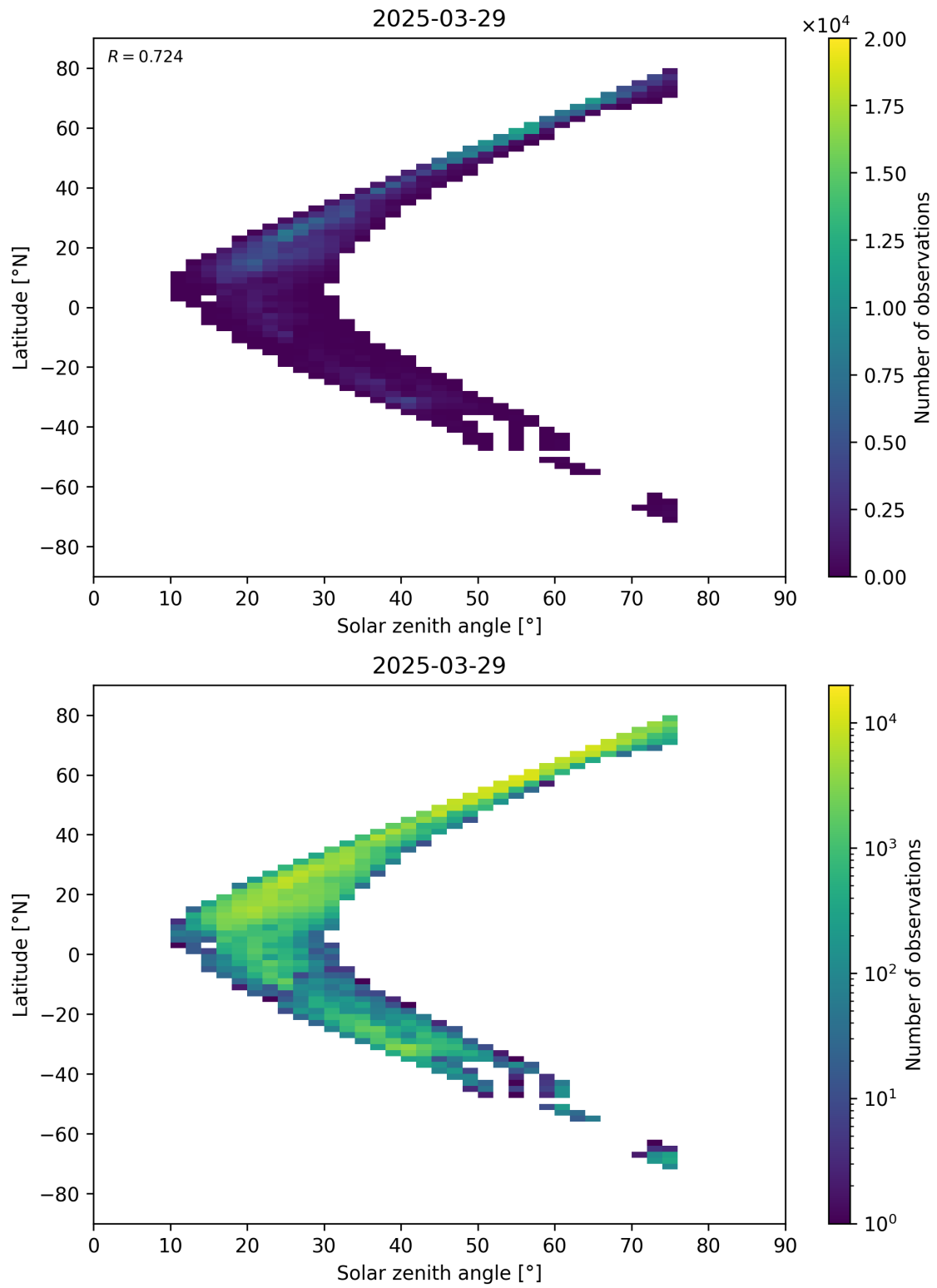
Figure 98: Scatter density plot of “Solar zenith angle” against “Latitude” for 2025-03-28 to 2025-03-30.
