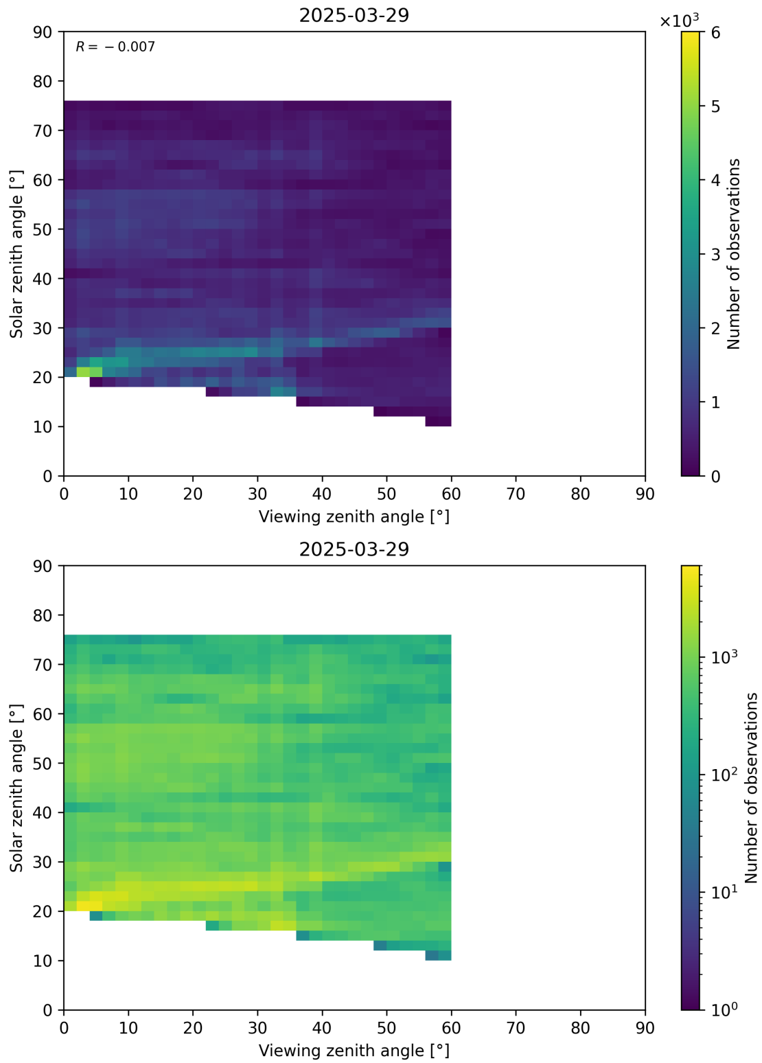
Figure 115: Scatter density plot of “Viewing zenith angle” against “Solar zenith angle” for 2025-03-28 to 2025-03-30.
