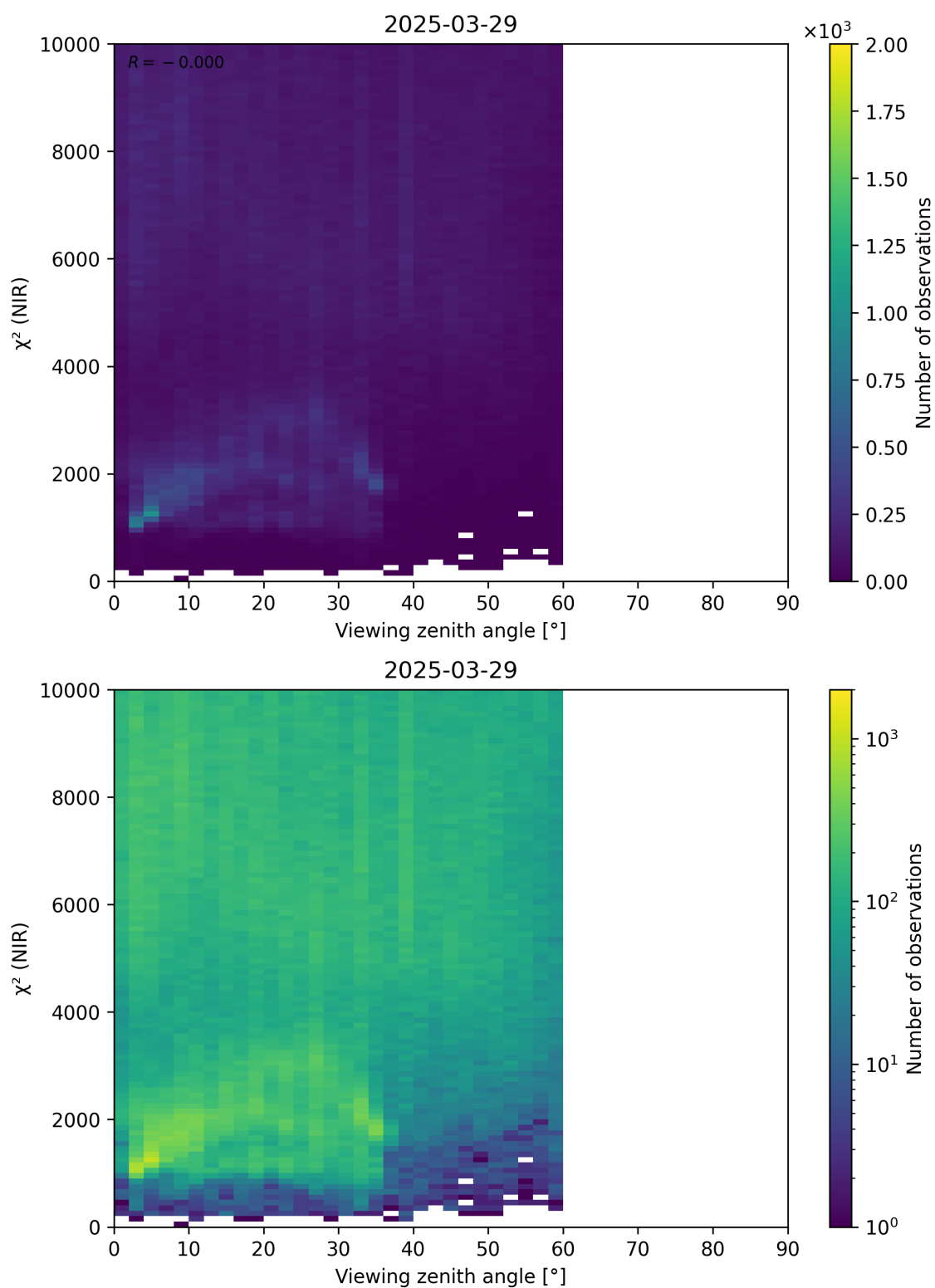
Figure 105: Scatter density plot of “Viewing zenith angle” against “ \chi^2 (NIR)” for 2025-03-28 to 2025-03-30.
