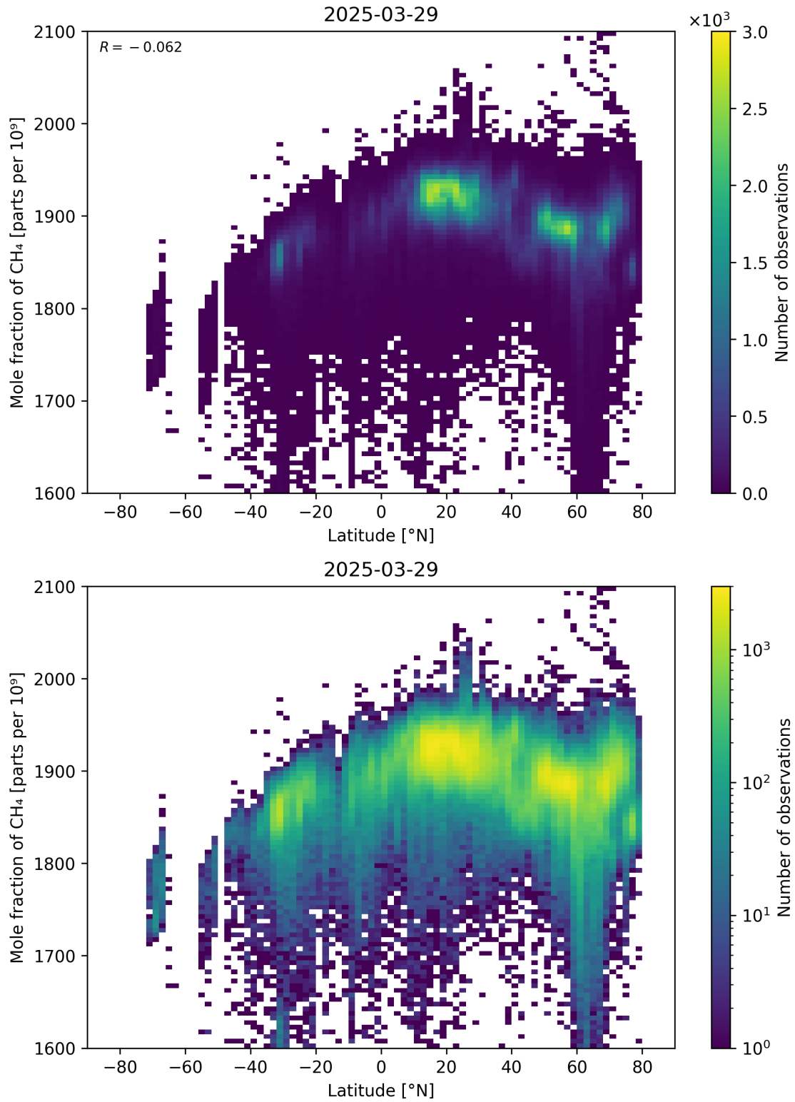
Figure 57: Scatter density plot of “Latitude” against “Mole fraction of CH 4 ” for 2025-03-28 to 2025-03-30.
