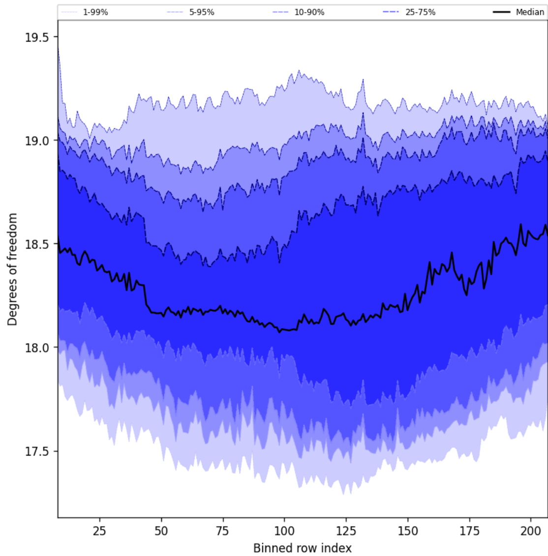
Figure 41: Along track statistics of “Degrees of freedom” for 2025-03-28 to 2025-03-30
