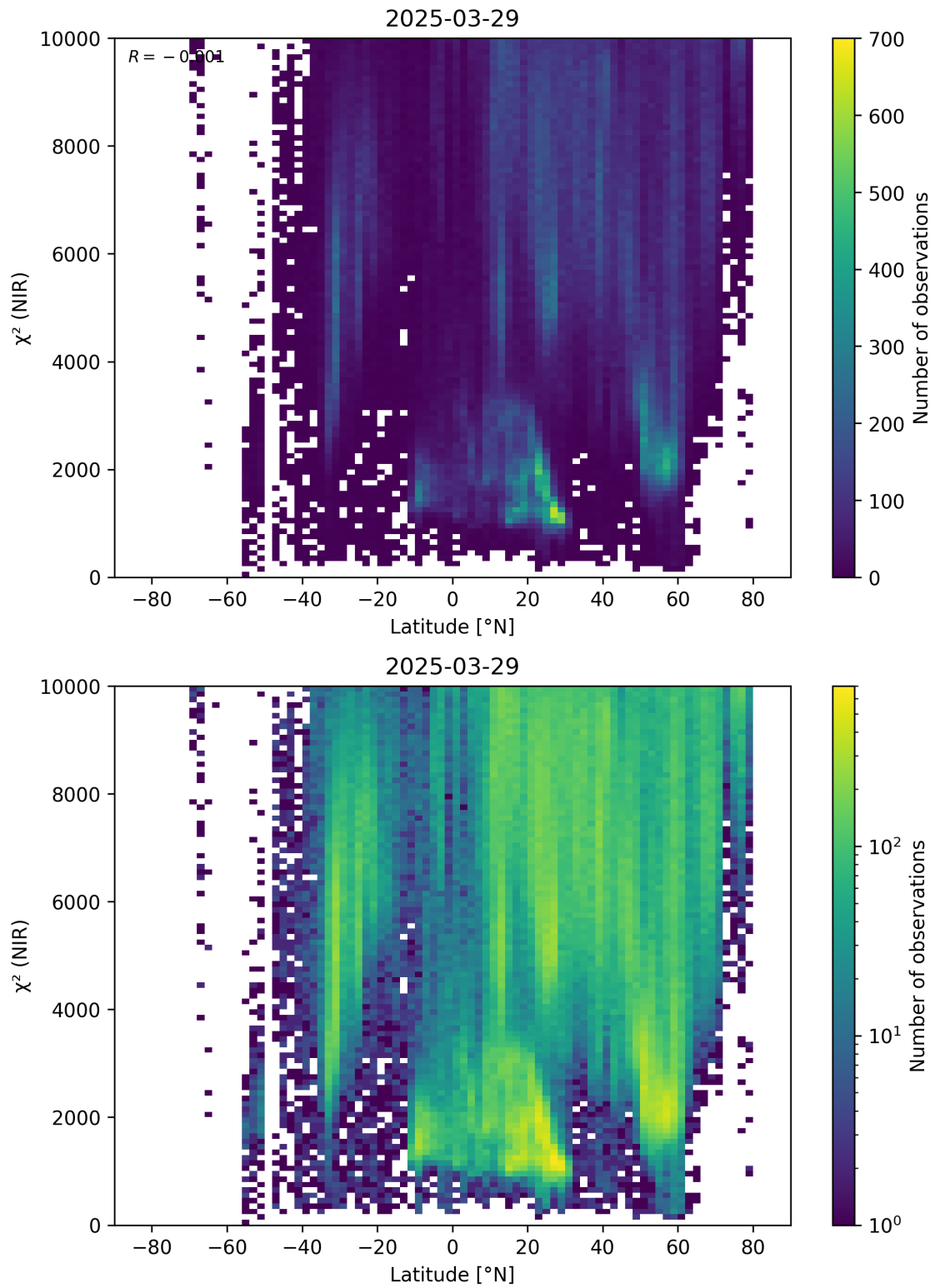
Figure 53: Scatter density plot of “Latitude” against “ \chi^2 (NIR)” for 2025-03-28 to 2025-03-30.
