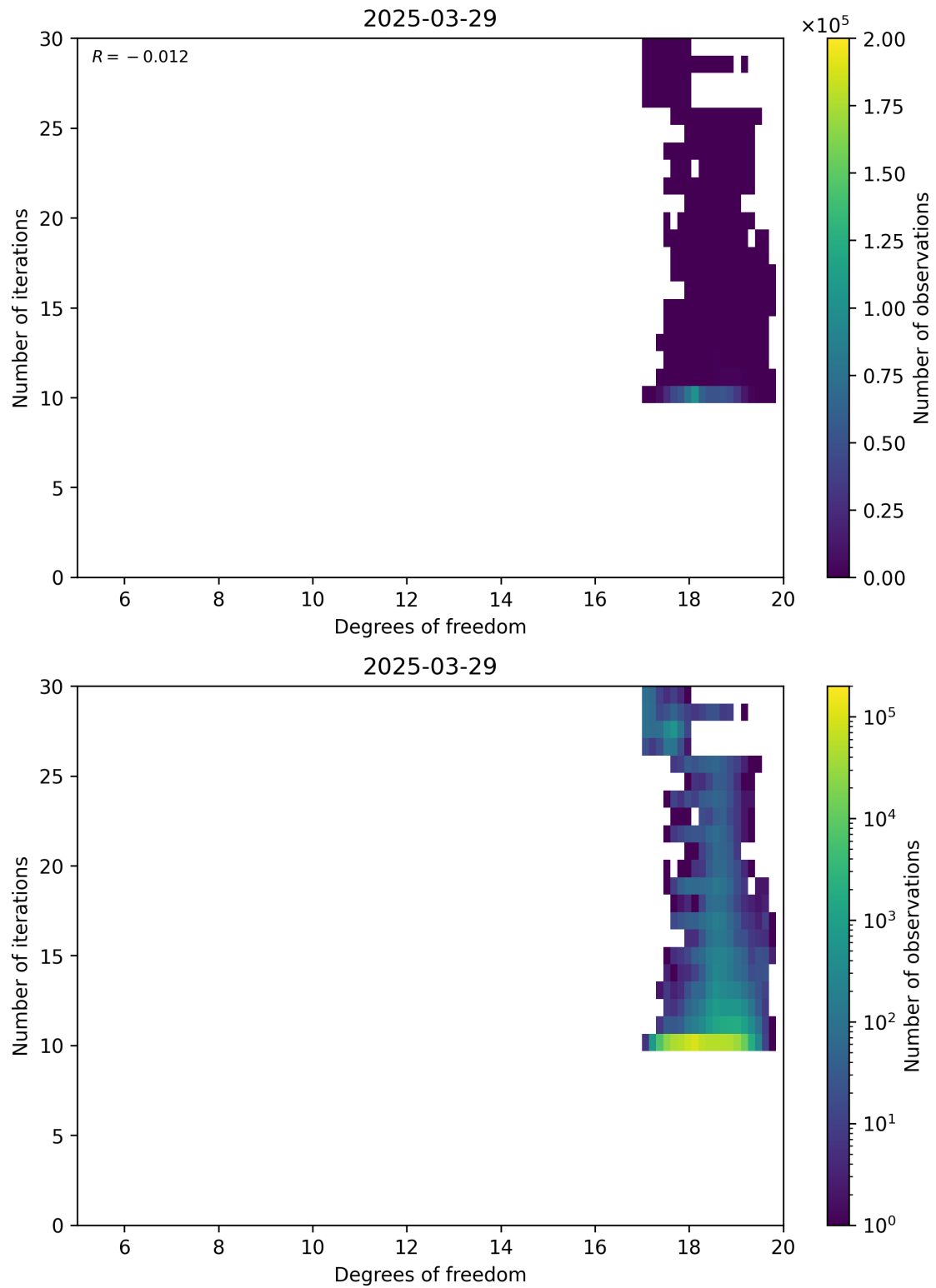
Figure 52: Scatter density plot of “Degrees of freedom” against “Number of iterations” for 2025-03-28 to 2025-03-30.
