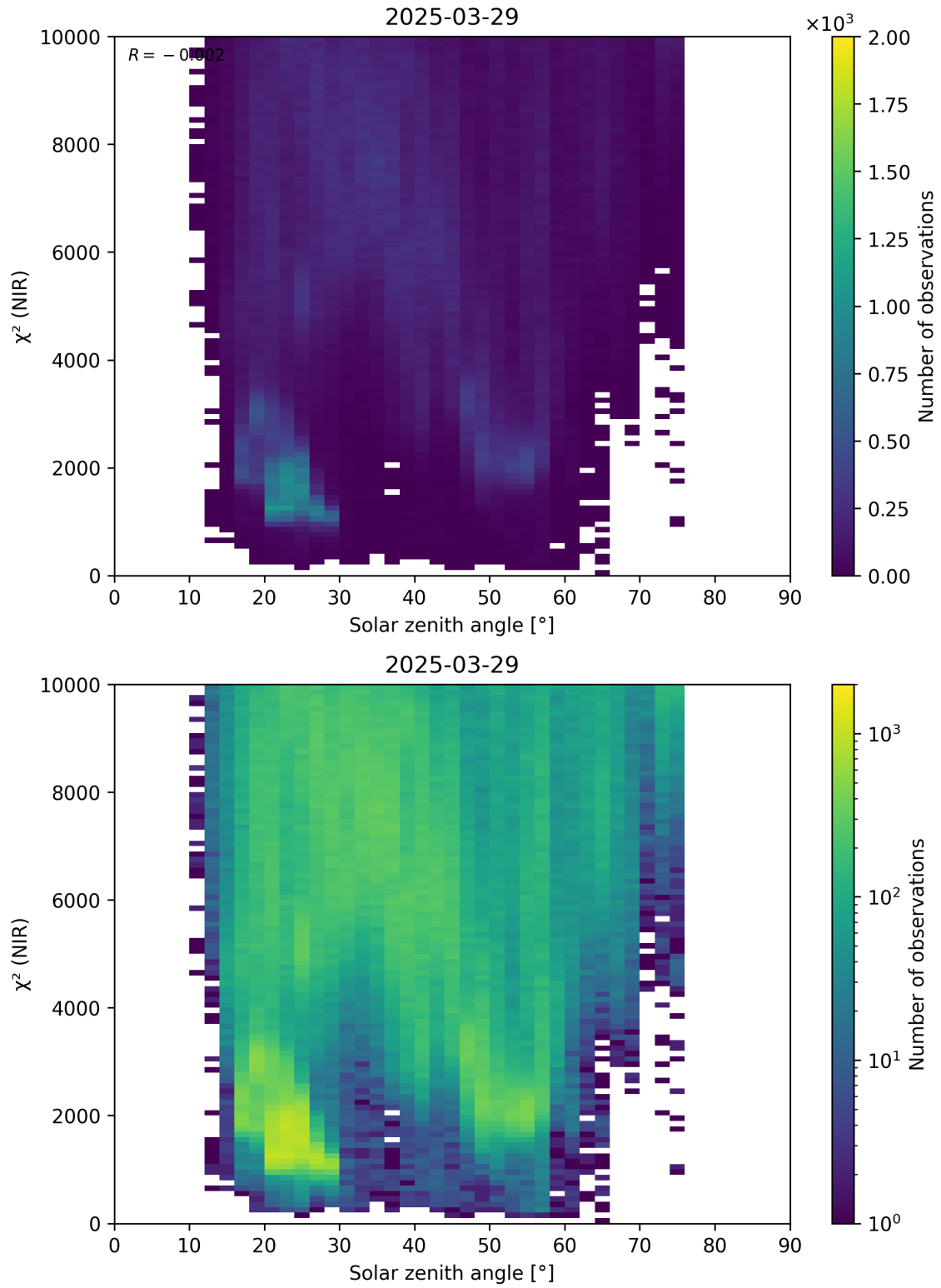
Figure 94: Scatter density plot of “Solar zenith angle” against “ \chi^2 (NIR)” for 2025-03-28 to 2025-03-30.
