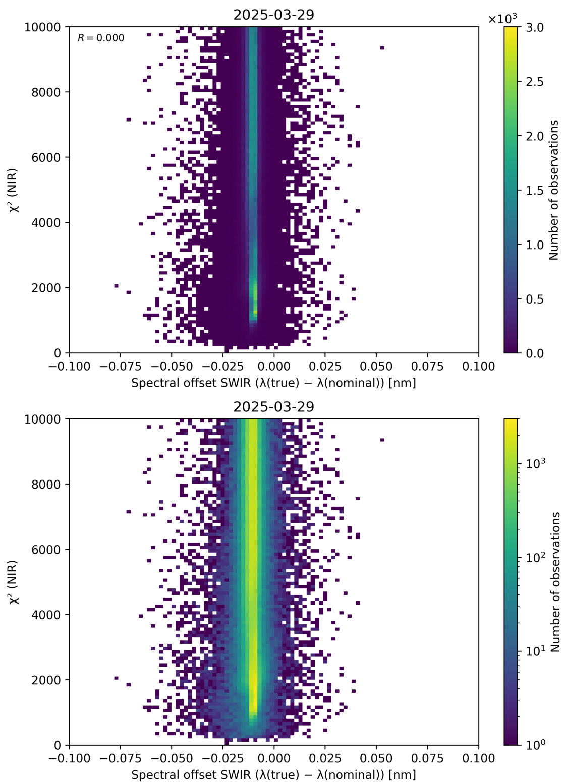
Figure 117: Scatter density plot of “Spectral offset SWIR ( \lambda_{\text{true}} - \lambda_{\text{nominal}} )” against “ \chi^2 (NIR)” for 2025-03-28 to 2025-03-30.
