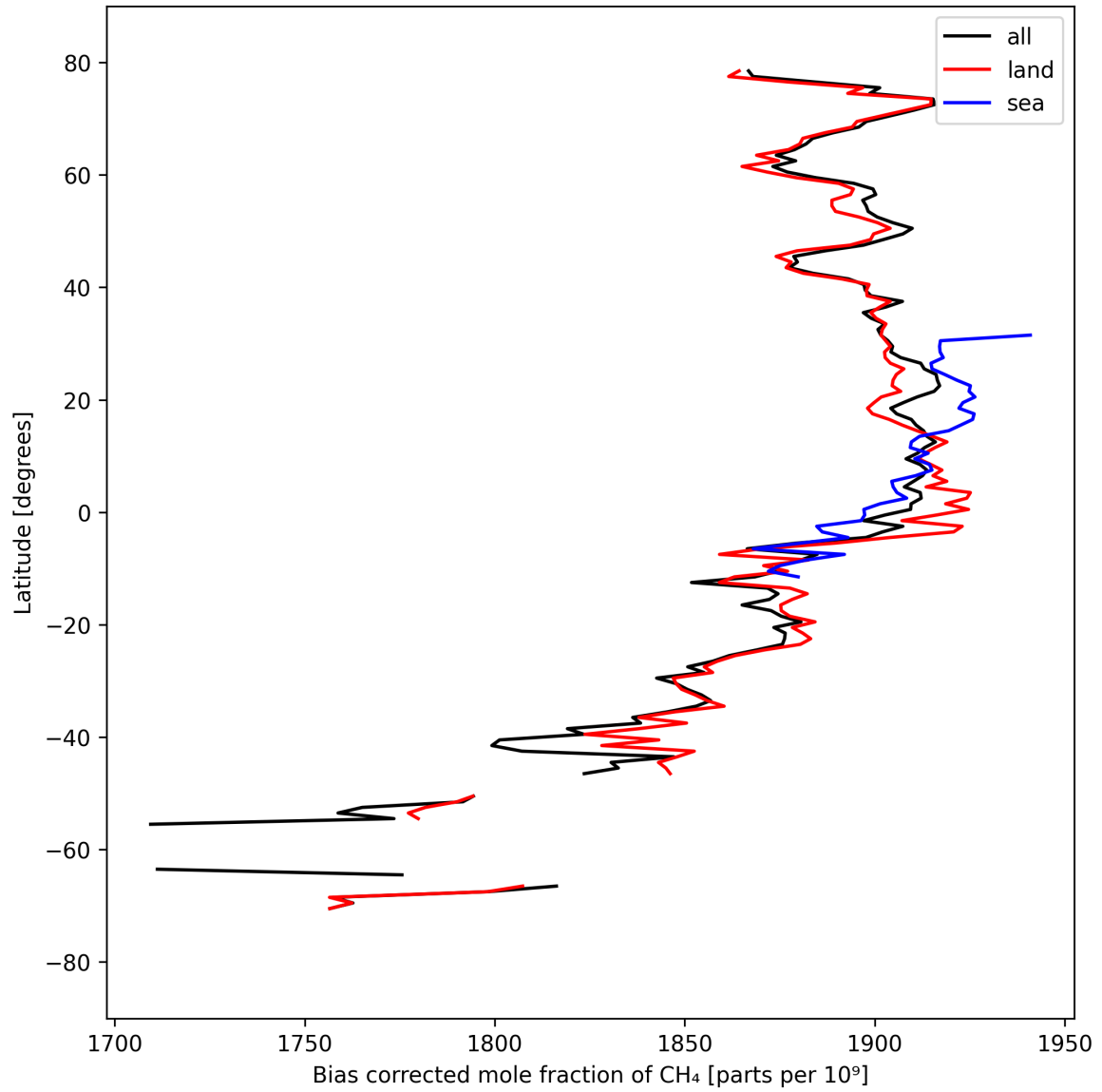
Figure 14: Zonal average of “Bias corrected mole fraction of \text{CH}_4 ” for 2025-03-28 to 2025-03-30.
