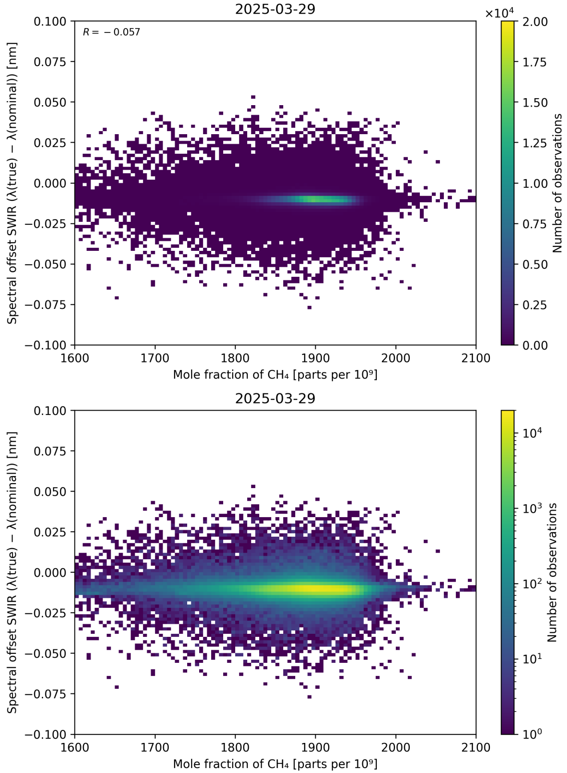
Figure 86: Scatter density plot of “Mole fraction of CH 4 ” against “Spectral offset SWIR ( \lambda_{\text{true}} - \lambda_{\text{nominal}} )” for 2025-03-28 to 2025-03-30.
