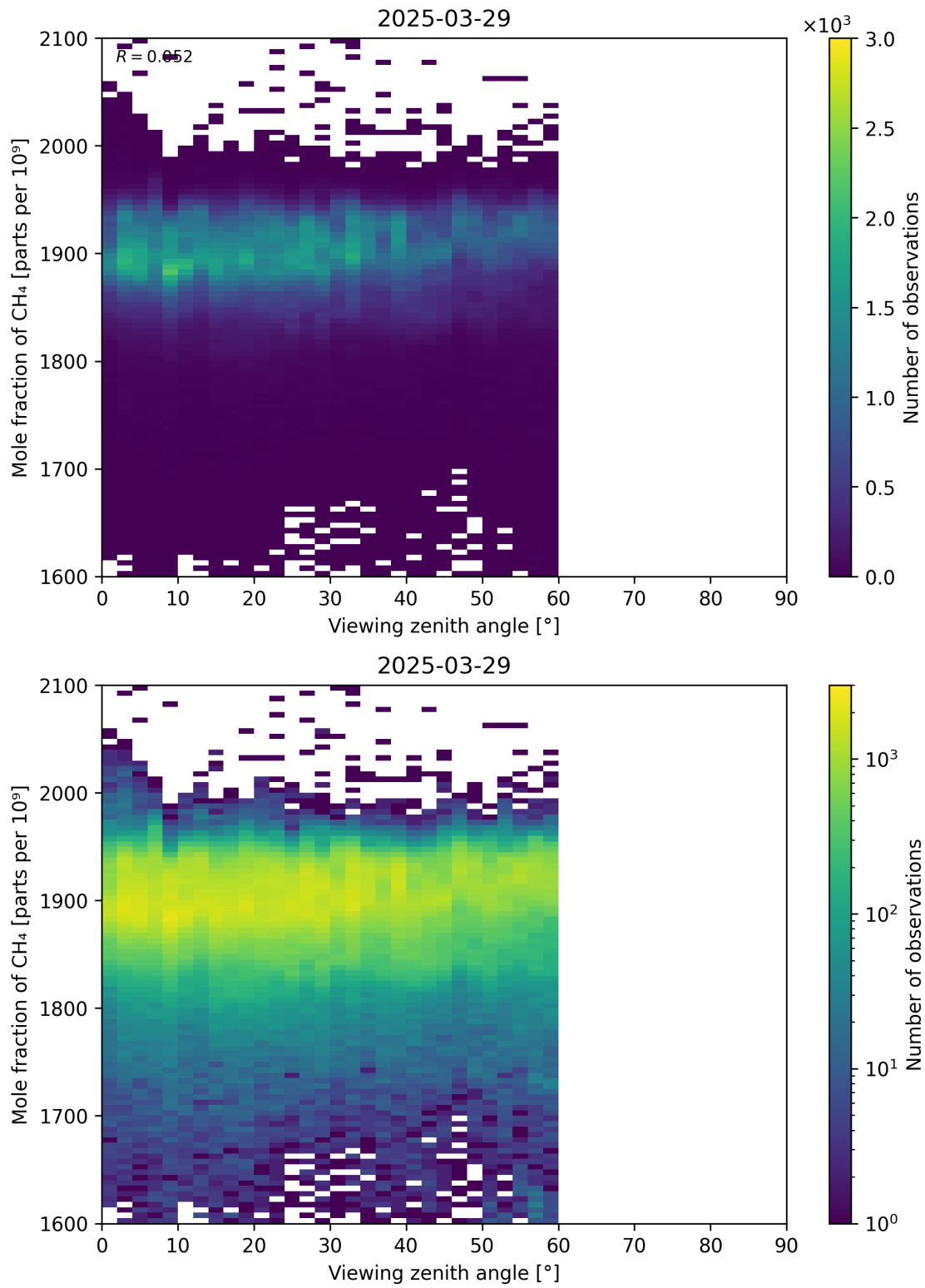
Figure 110: Scatter density plot of “Viewing zenith angle” against “Mole fraction of CH 4 ” for 2025-03-28 to 2025-03-30.
