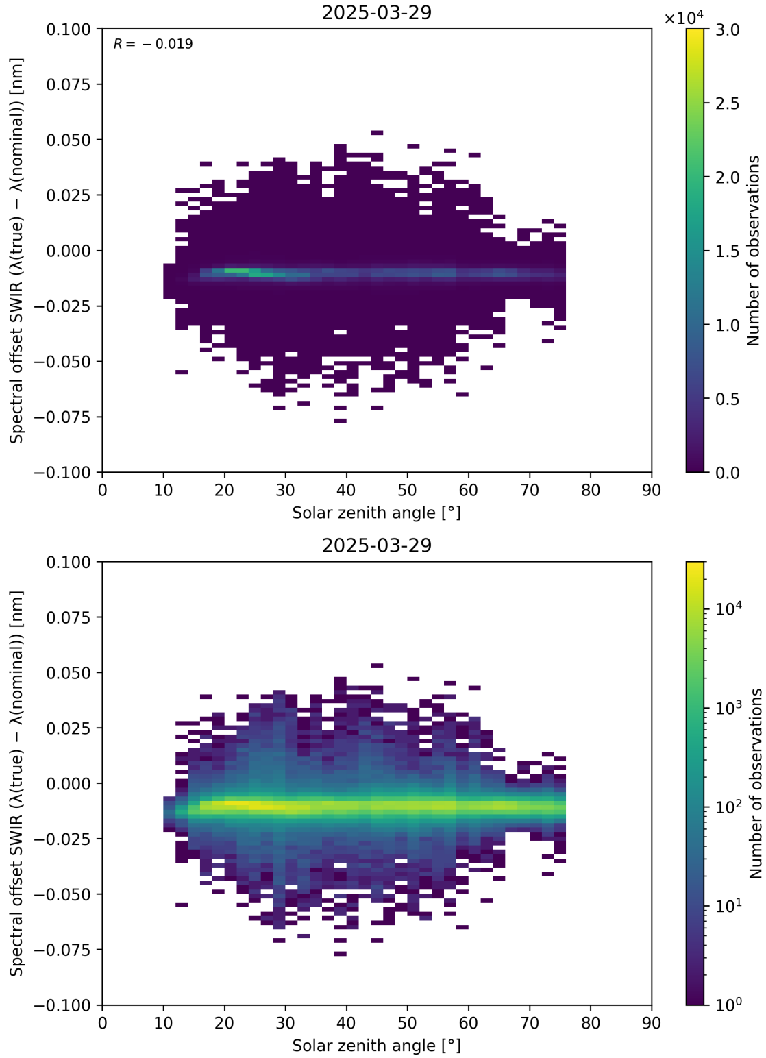
Figure 104: Scatter density plot of “Solar zenith angle” against “Spectral offset SWIR ( \lambda_{\text{true}} - \lambda_{\text{nominal}} )” for 2025-03-28 to 2025-03-30.
