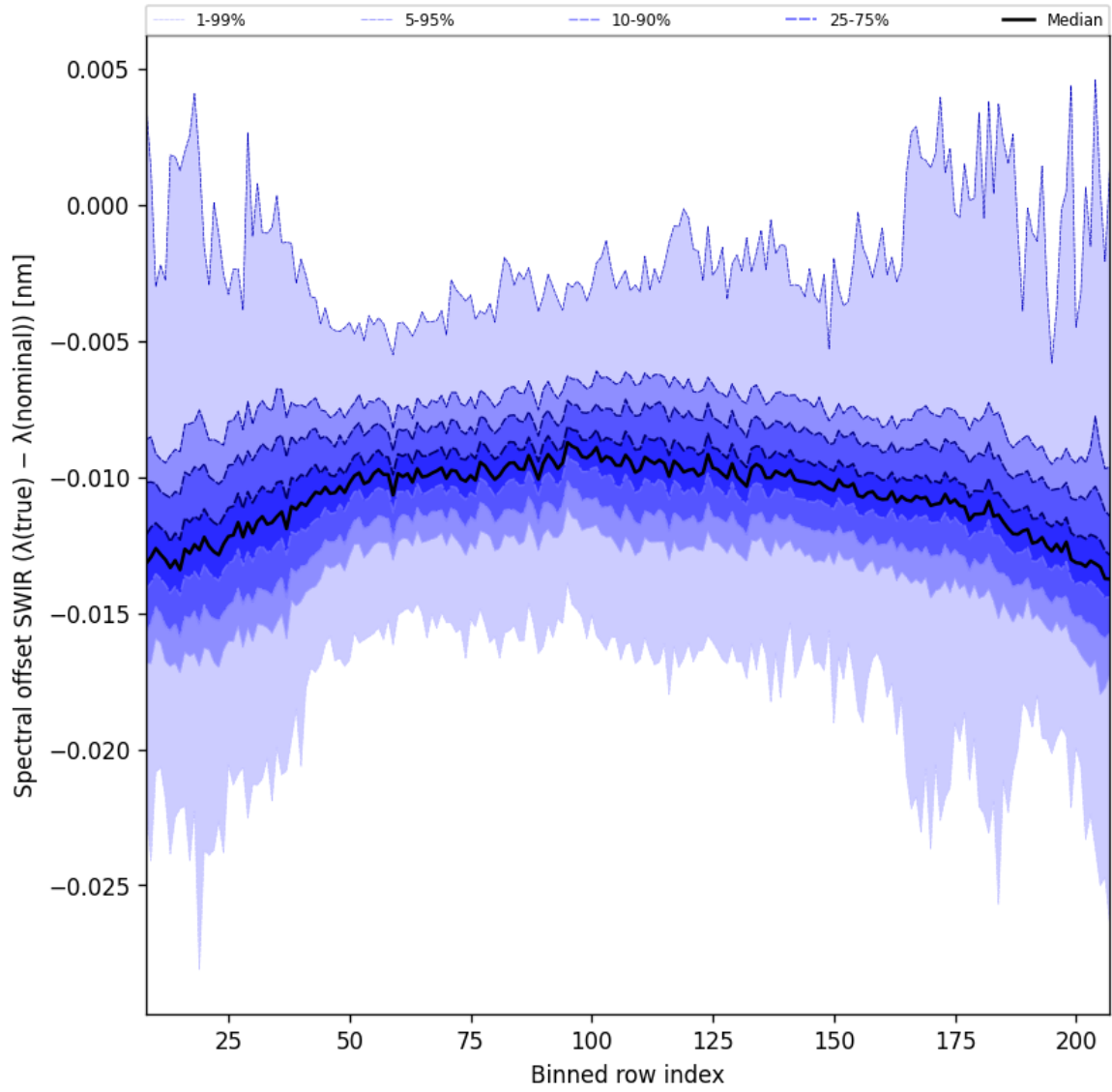
Figure 38: Along track statistics of “Spectral offset SWIR ( \lambda_{\text{true}} - \lambda_{\text{nominal}} )” for 2025-03-28 to 2025-03-30
