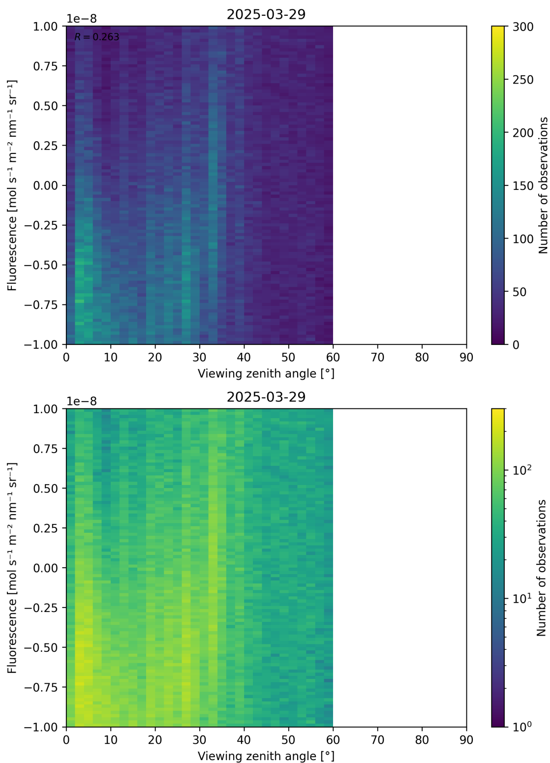
Figure 108: Scatter density plot of “Viewing zenith angle” against “Fluorescence” for 2025-03-28 to 2025-03-30.
