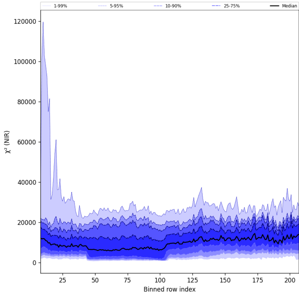
Figure 40: Along track statistics of “ \chi^2 (NIR)” for 2025-03-28 to 2025-03-30
