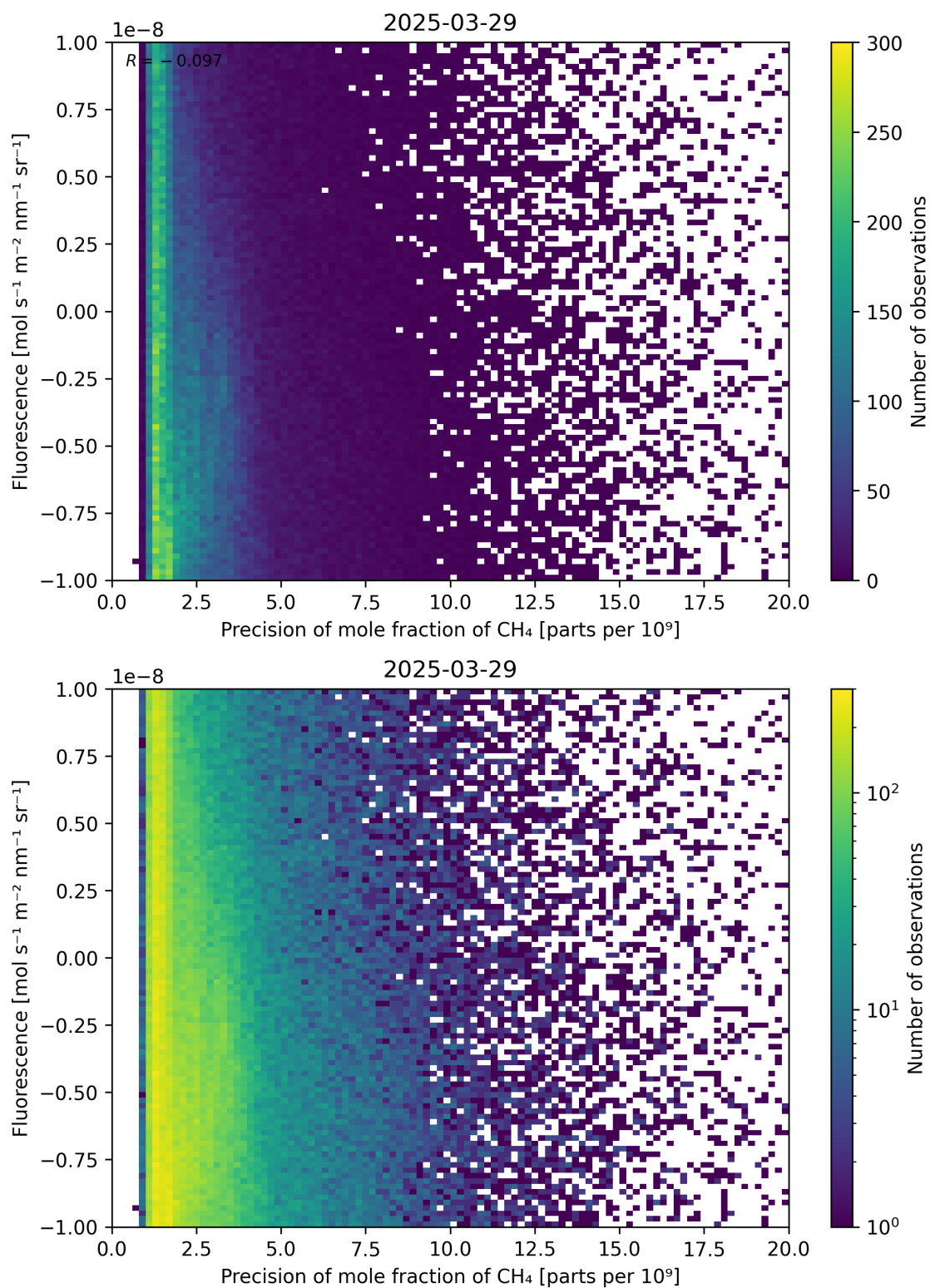
Figure 81: Scatter density plot of “Precision of mole fraction of CH 4 ” against “Fluorescence” for 2025-03-28 to 2025-03-30.
