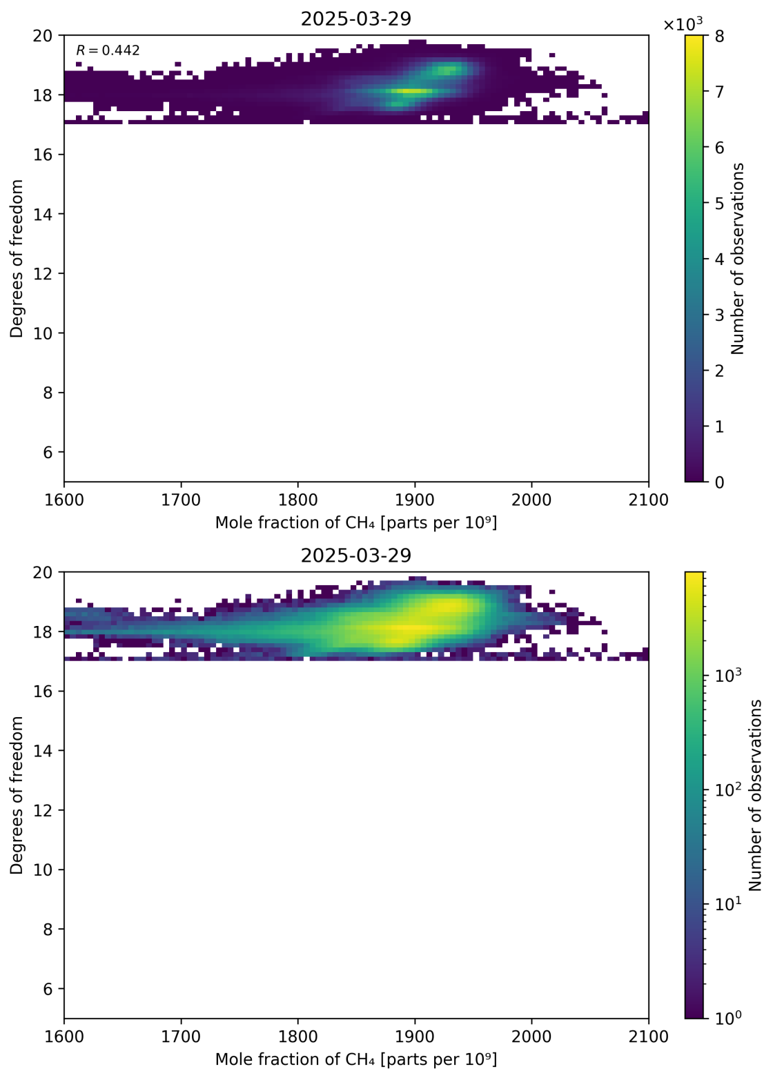
Figure 72: Scatter density plot of “Mole fraction of CH 4 ” against “Degrees of freedom” for 2025-03-28 to 2025-03-30.
