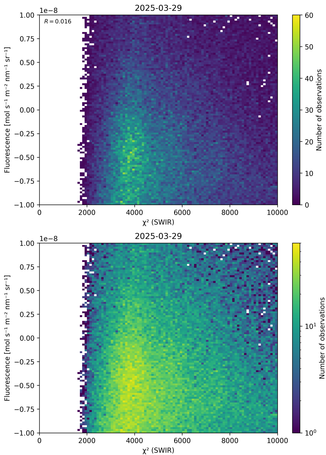
Figure 49: Scatter density plot of “ \chi^2 (SWIR)” against “Fluorescence” for 2025-03-28 to 2025-03-30.
