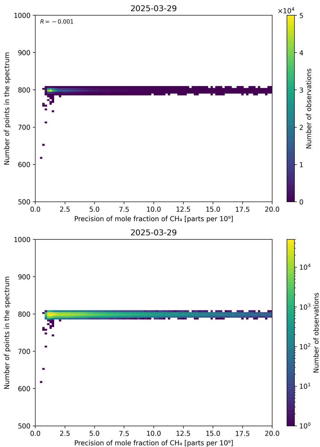
Figure 84: Scatter density plot of “Precision of mole fraction of CH 4 ” against “Number of points in the spectrum” for 2025-03-28 to 2025-03-30.
