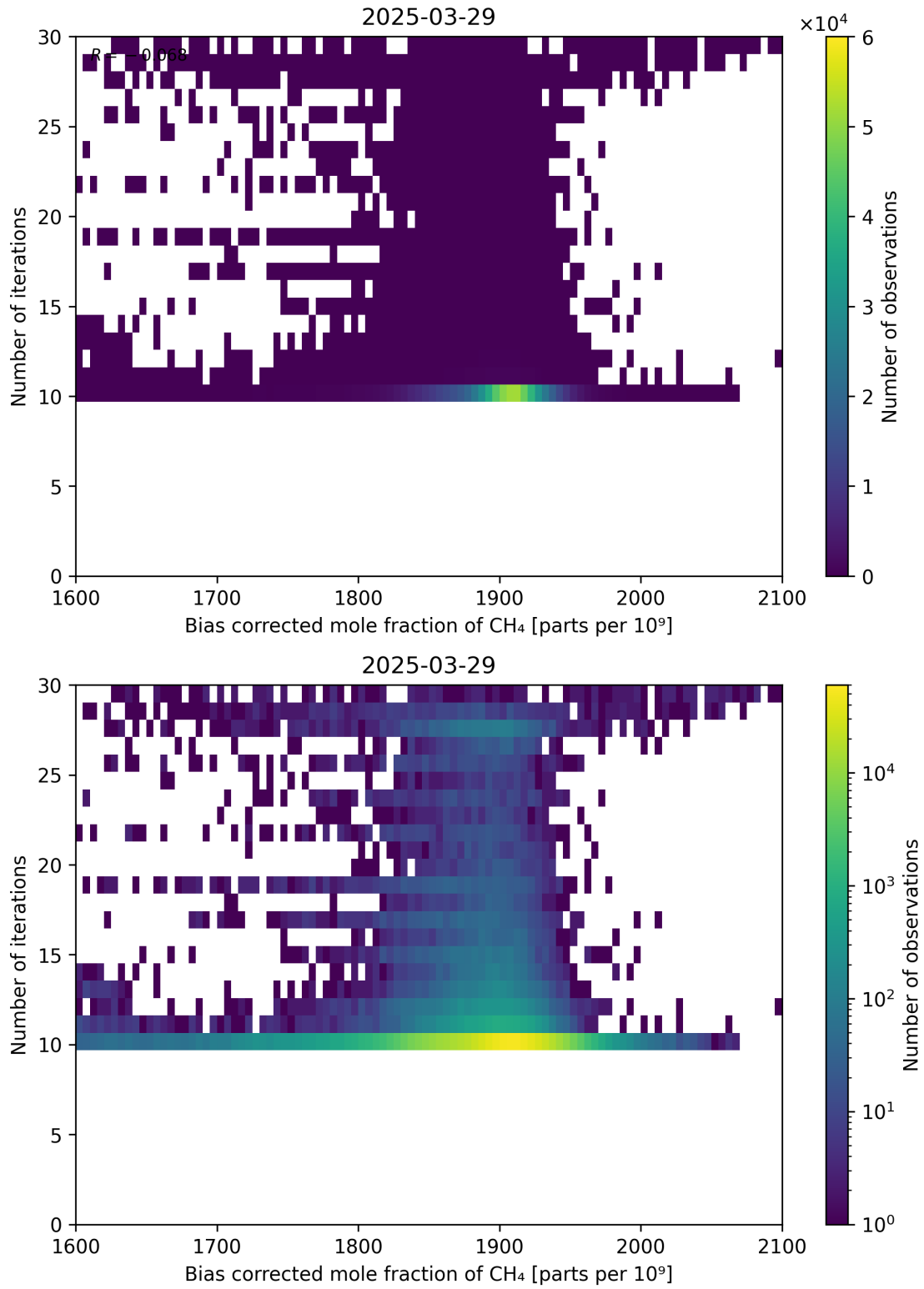
Figure 67: Scatter density plot of “Bias corrected mole fraction of \text{CH}_4 ” against “Number of iterations” for 2025-03-28 to 2025-03-30.
