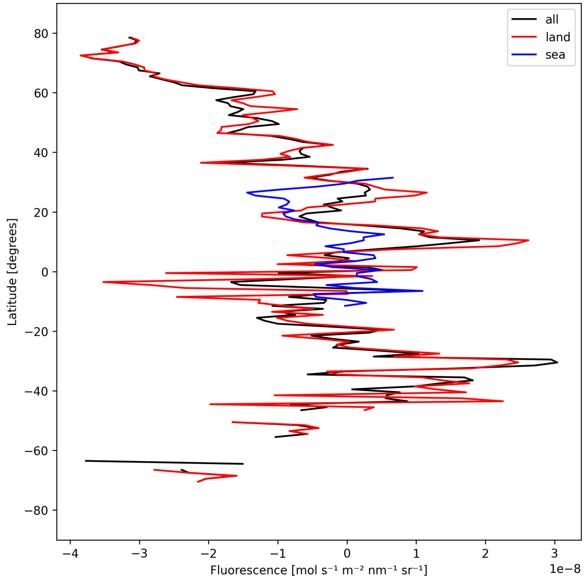
Figure 21: Zonal average of “Fluorescence” for 2025-03-28 to 2025-03-30.
