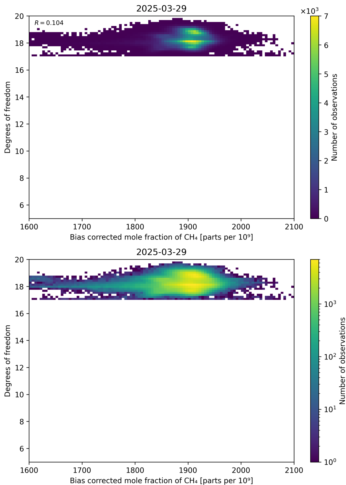
Figure 65: Scatter density plot of “Bias corrected mole fraction of CH 4 ” against “Degrees of freedom” for 2025-03-28 to 2025-03-30.
