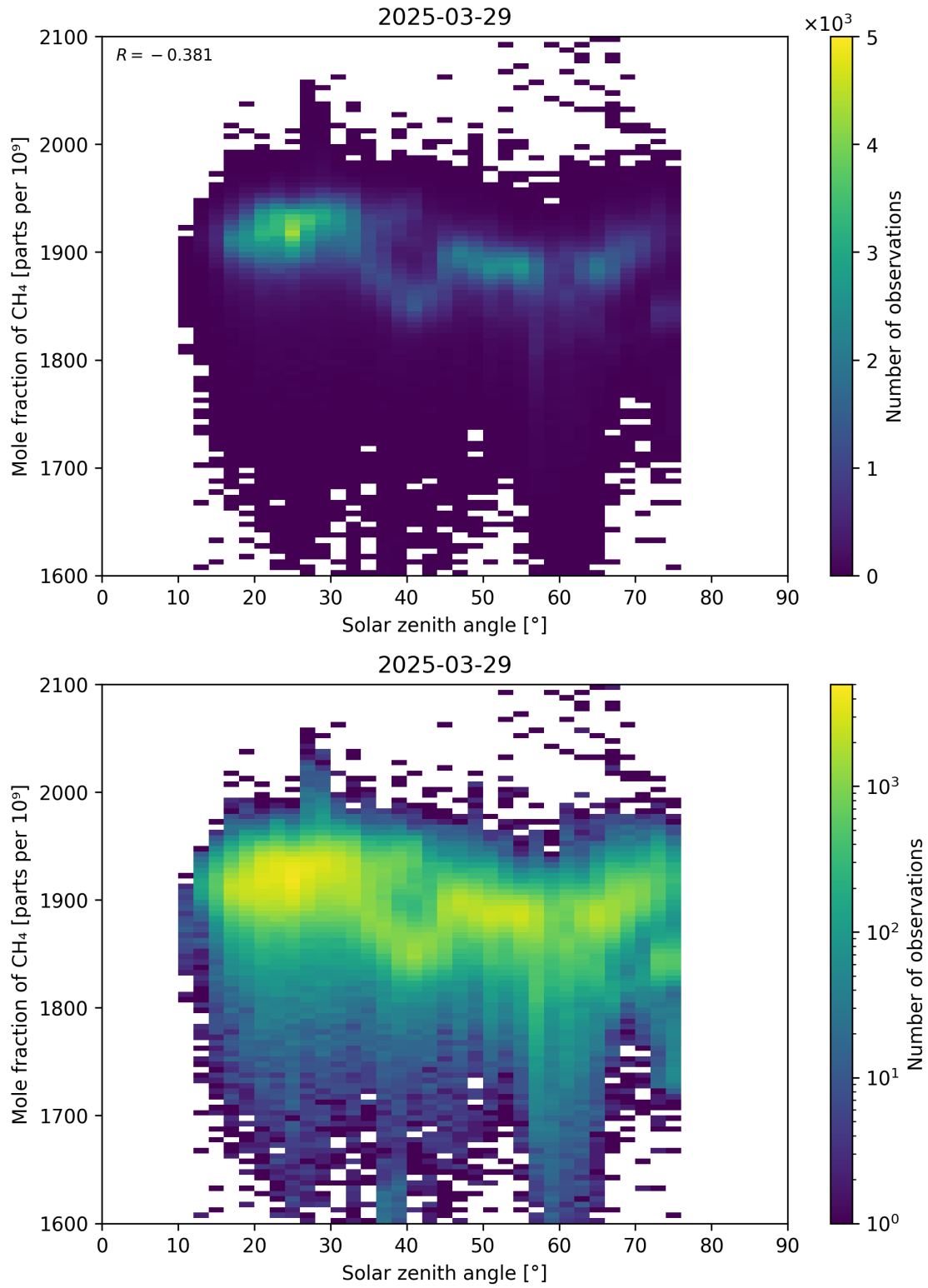
Figure 99: Scatter density plot of “Solar zenith angle” against “Mole fraction of CH 4 ” for 2025-03-28 to 2025-03-30.
