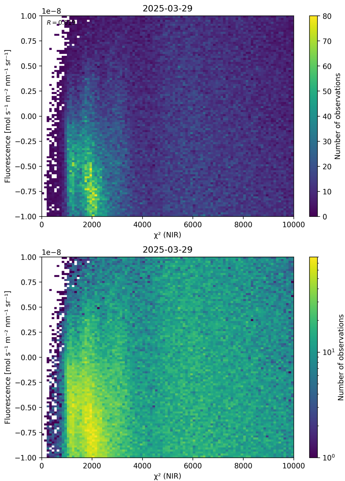
Figure 45: Scatter density plot of “ \chi^2 (NIR)” against “Fluorescence” for 2025-03-28 to 2025-03-30.
