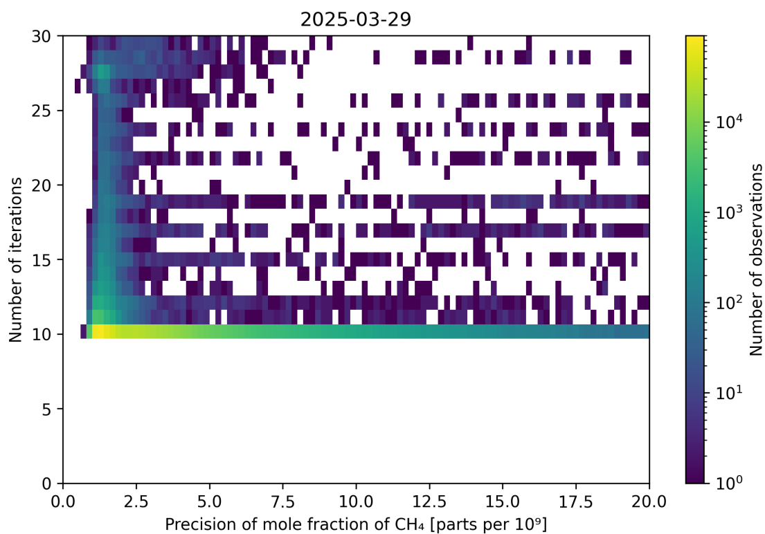
Figure 83: Scatter density plot of “Precision of mole fraction of CH 4 ” against “Number of iterations” for 2025-03-28 to 2025-03-30.
