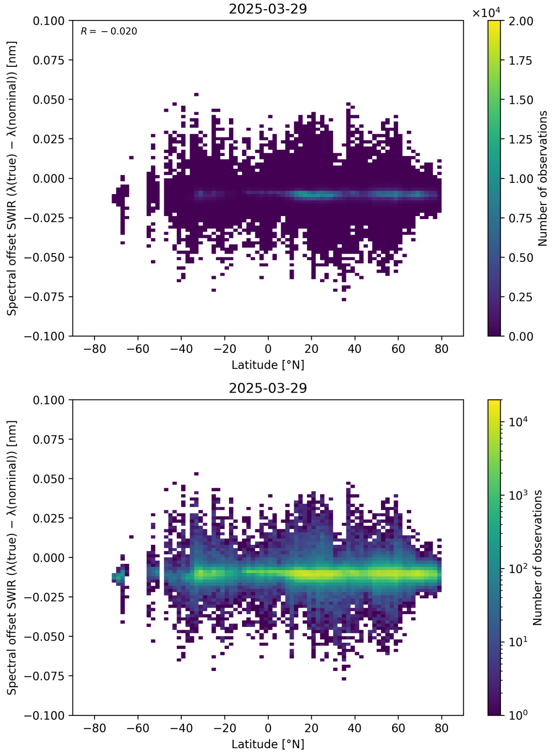
Figure 62: Scatter density plot of “Latitude” against “Spectral offset SWIR ( \lambda_{\text{true}} - \lambda_{\text{nominal}} )” for 2025-03-28 to 2025-03-30.
