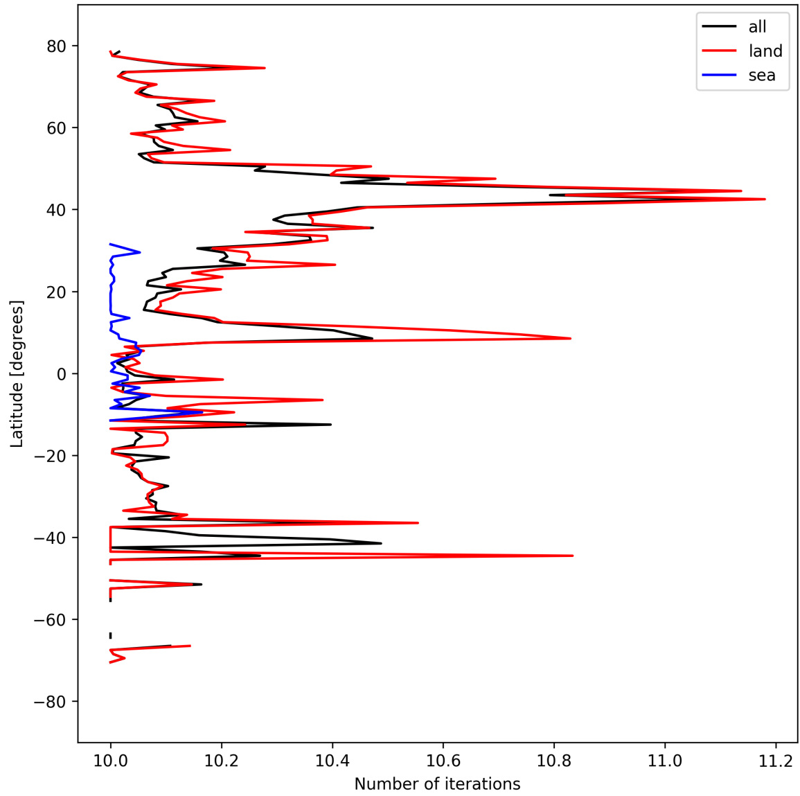
Figure 20: Zonal average of “Number of iterations” for 2025-03-28 to 2025-03-30.
