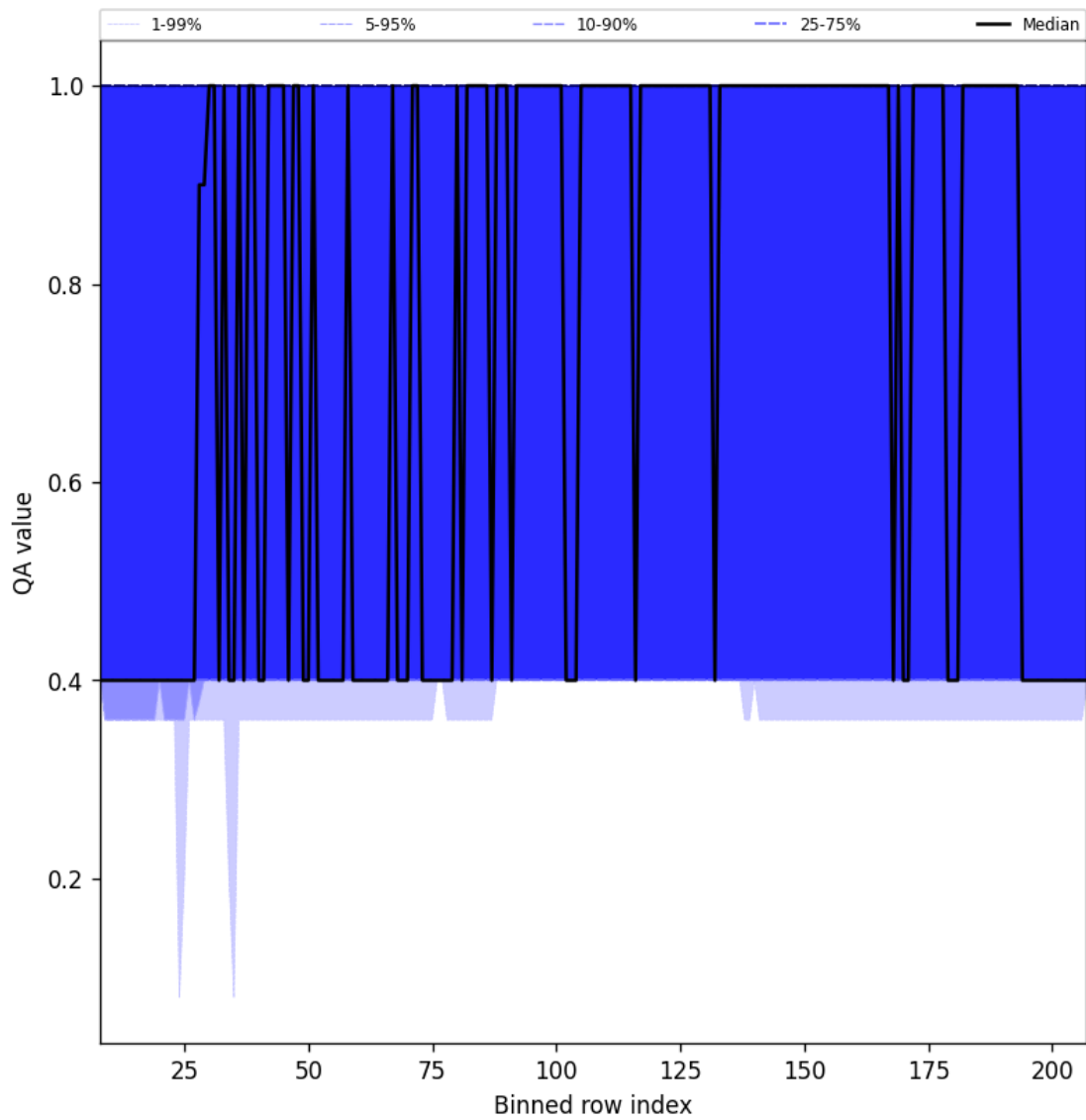
Figure 33: Along track statistics of “QA value” for 2025-03-28 to 2025-03-30
