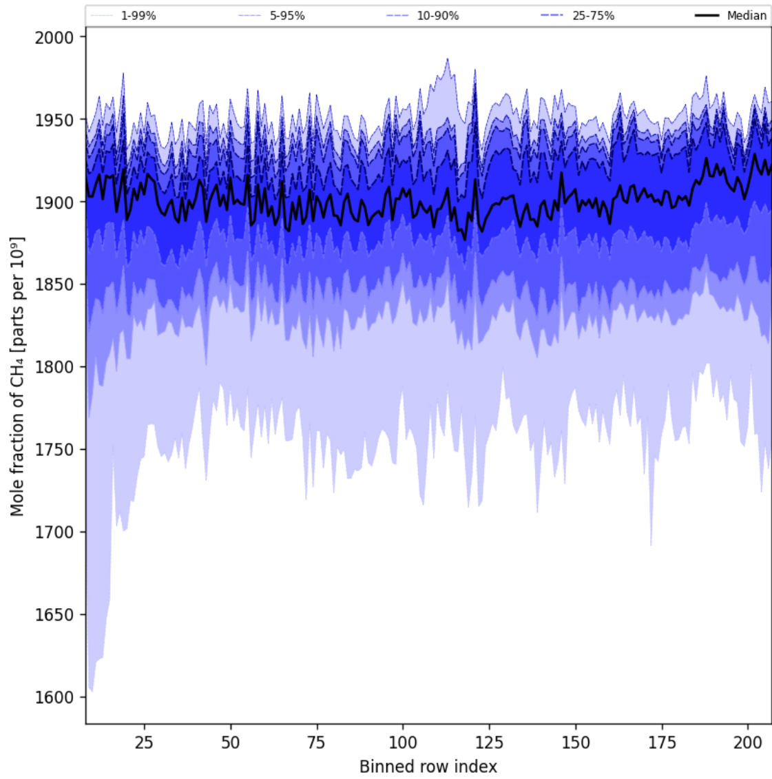
Figure 34: Along track statistics of “Mole fraction of CH 4 ” for 2025-03-28 to 2025-03-30
