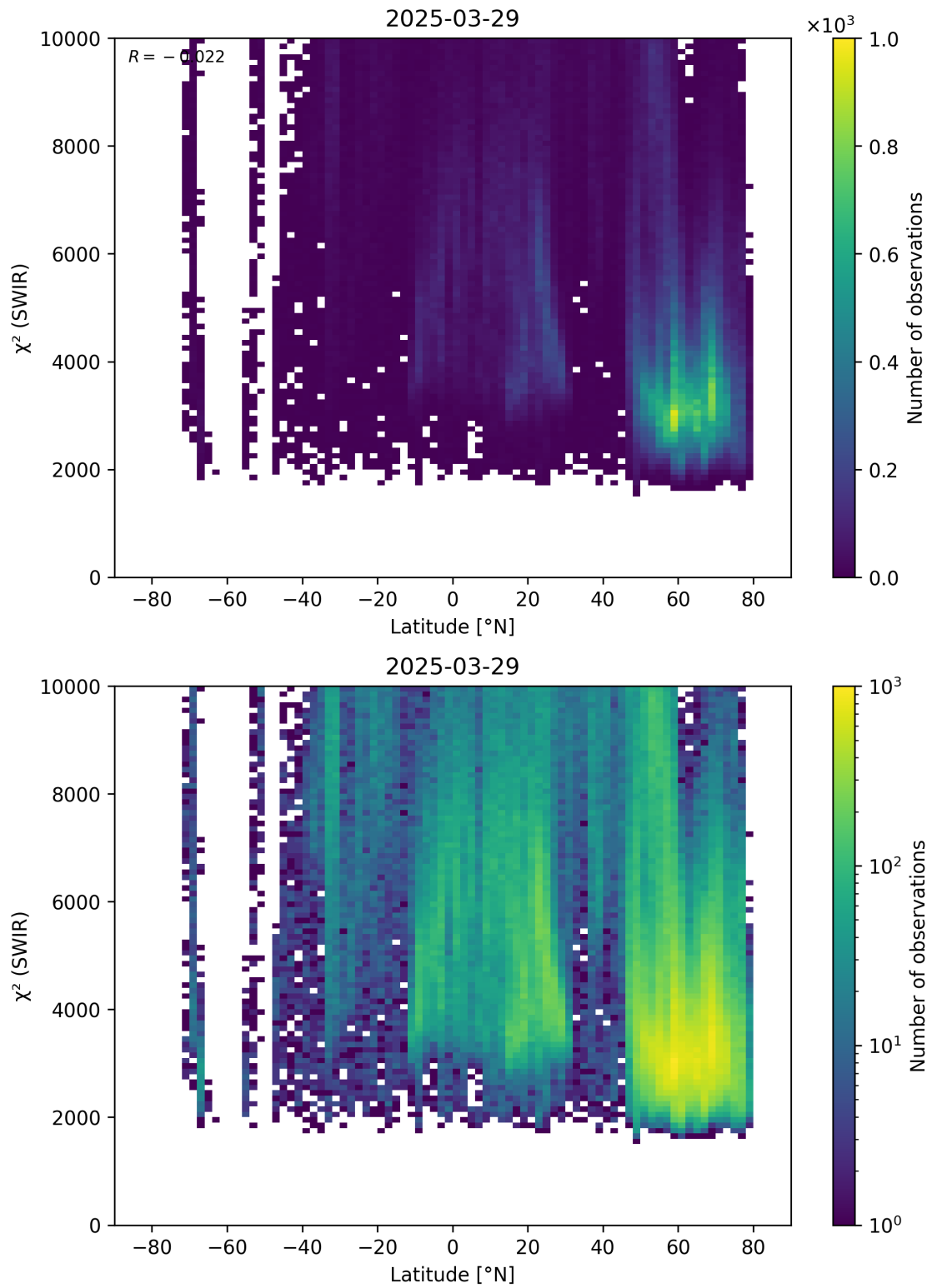
Figure 54: Scatter density plot of “Latitude” against “ \chi^2 (SWIR)” for 2025-03-28 to 2025-03-30.
