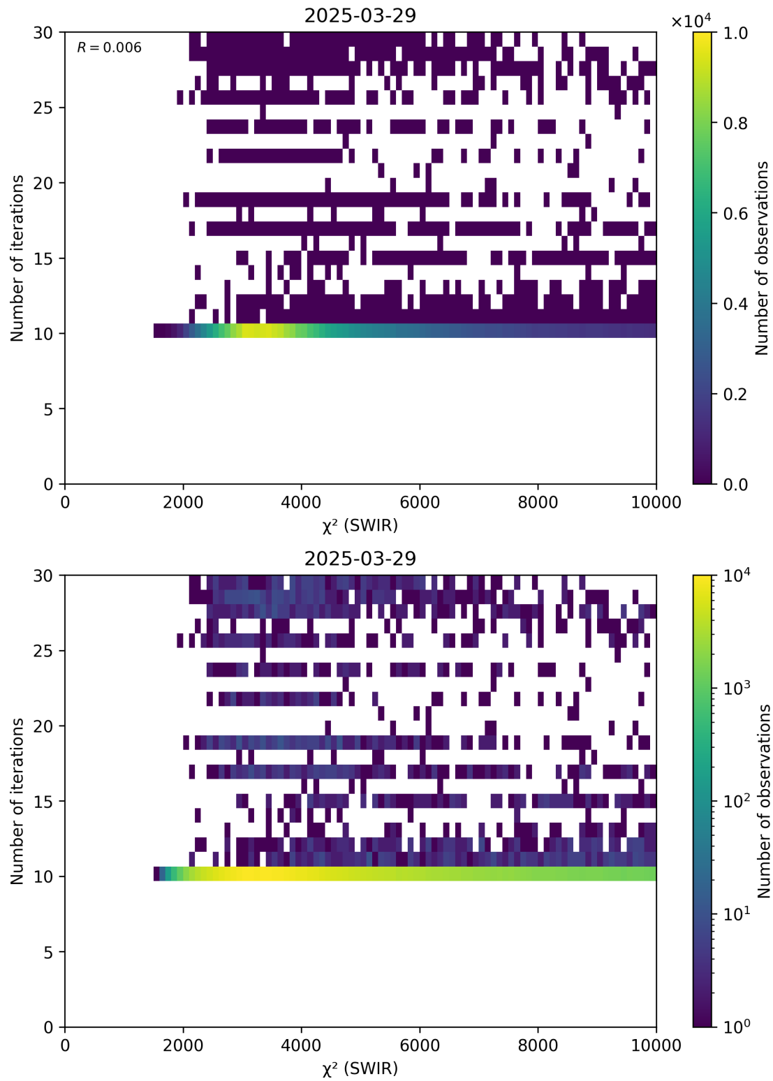
Figure 50: Scatter density plot of “ \chi^2 (SWIR)” against “Number of iterations” for 2025-03-28 to 2025-03-30.
