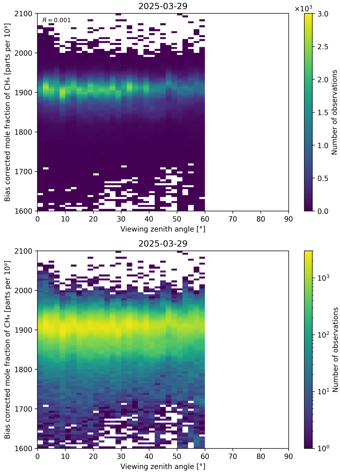
Figure 111: Scatter density plot of “Viewing zenith angle” against “Bias corrected mole fraction of \text{CH}_4 ” for 2025-03-28 to 2025-03-30.
