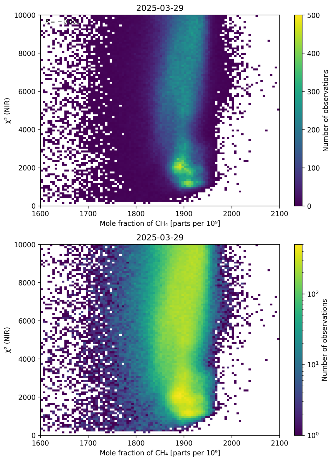
Figure 70: Scatter density plot of “Mole fraction of CH 4 ” against “ \chi^2 (NIR)” for 2025-03-28 to 2025-03-30.
