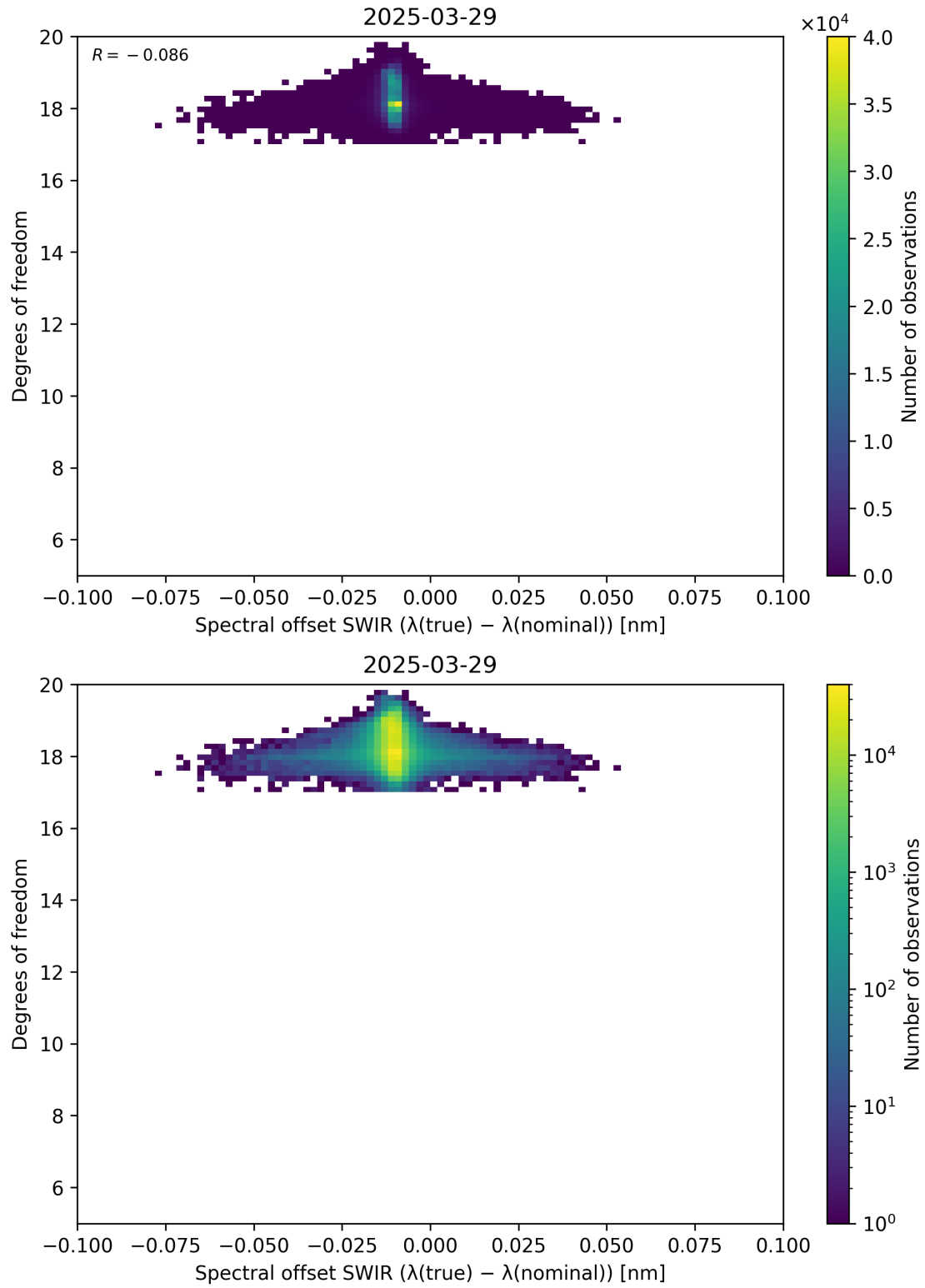
Figure 119: Scatter density plot of “Spectral offset SWIR ( \lambda_{\text{true}} - \lambda_{\text{nominal}} )” against “Degrees of freedom” for 2025-03-28 to 2025-03-30.
