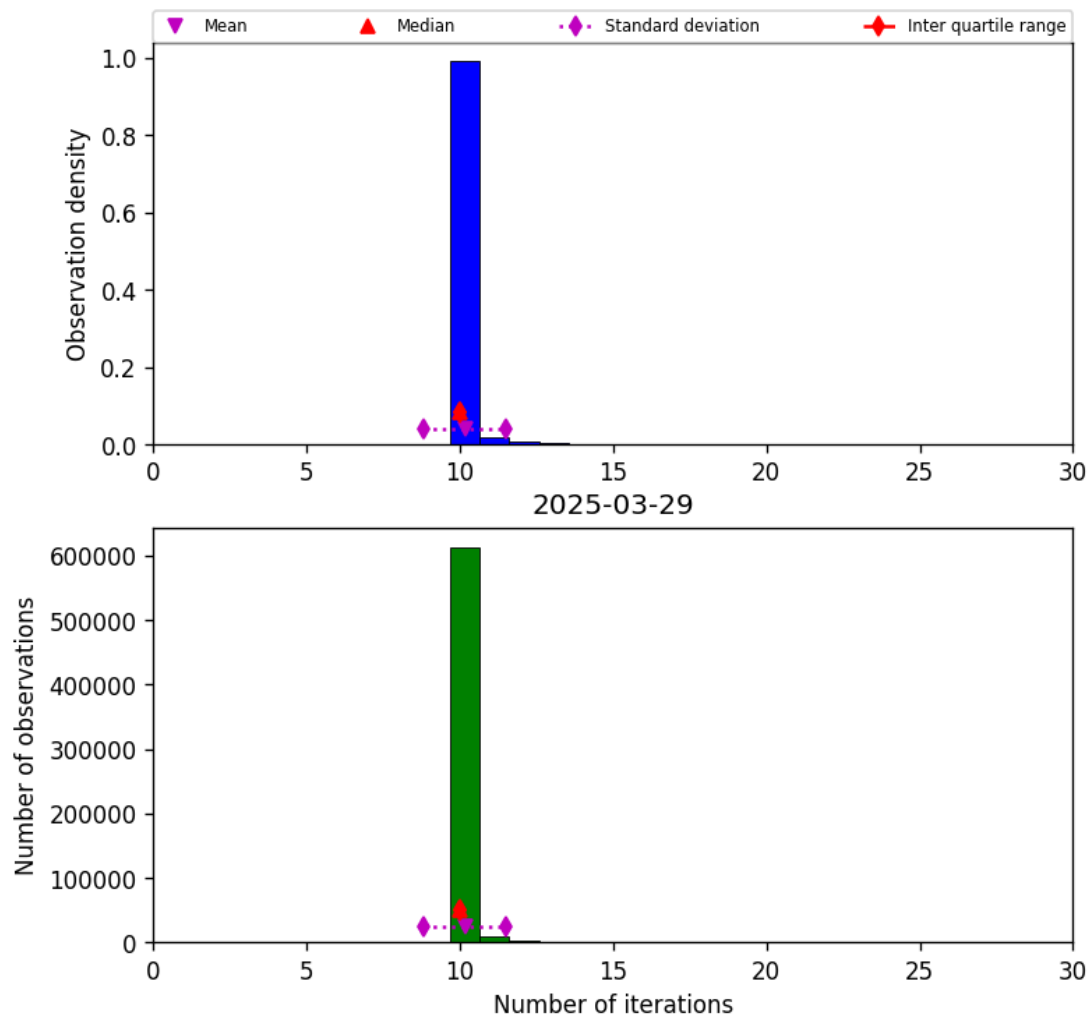
Figure 31: Histogram of “Number of iterations” for 2025-03-28 to 2025-03-30
