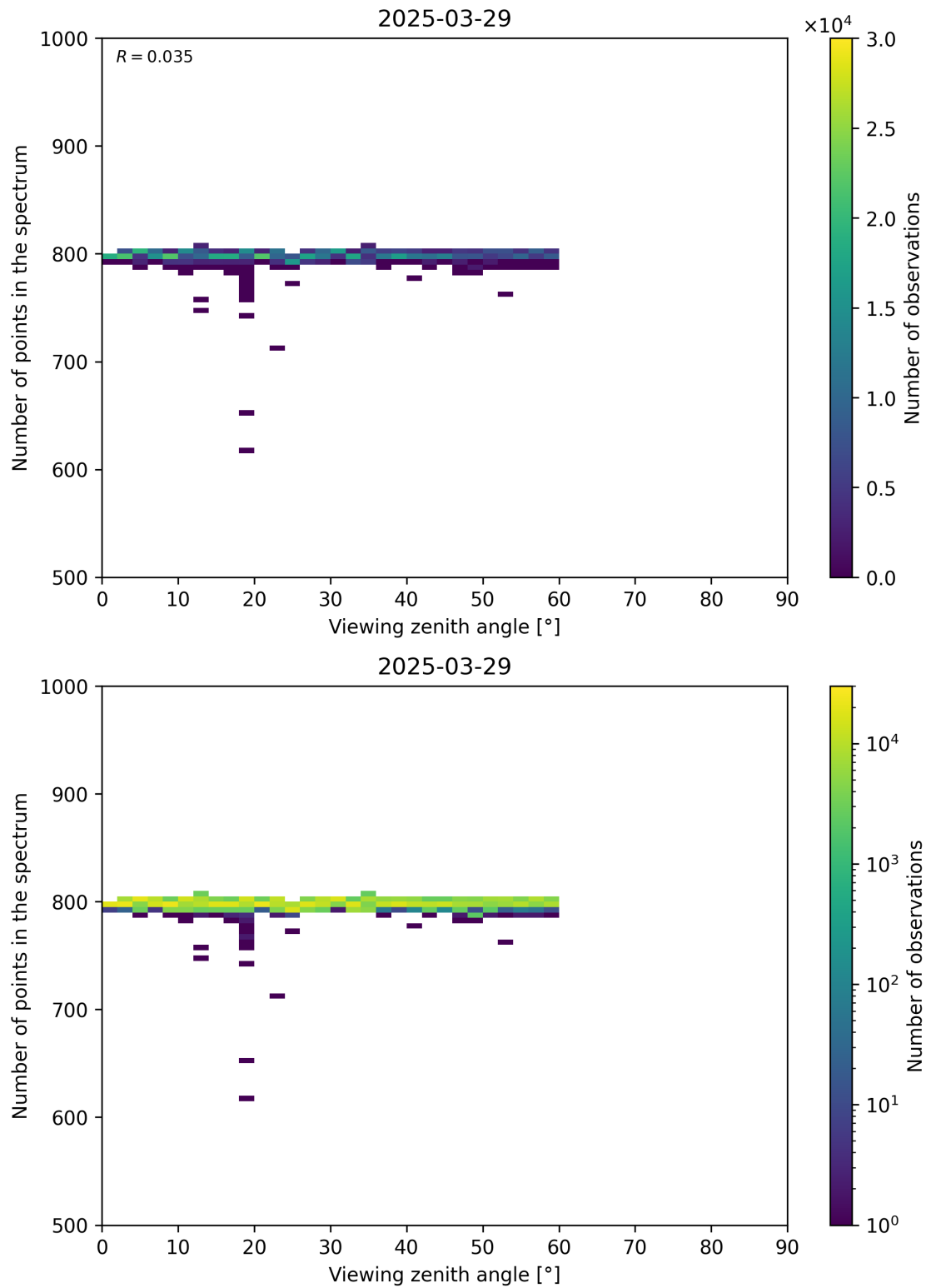
Figure 114: Scatter density plot of “Viewing zenith angle” against “Number of points in the spectrum” for 2025-03-28 to 2025-03-30.
