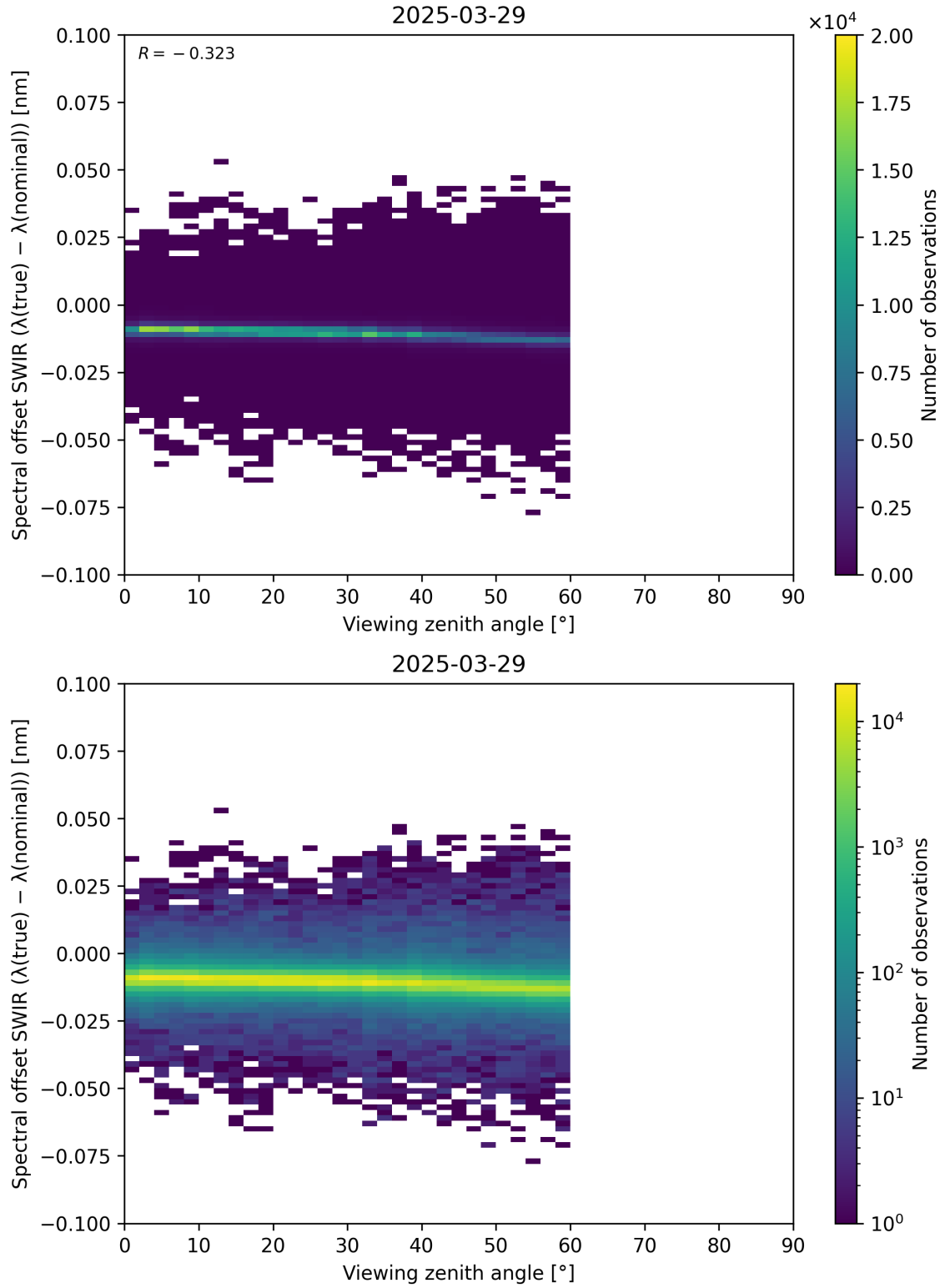
Figure 116: Scatter density plot of “Viewing zenith angle” against “Spectral offset SWIR ( \lambda_{\text{true}} - \lambda_{\text{nominal}} )” for 2025-03-28 to 2025-03-30.
