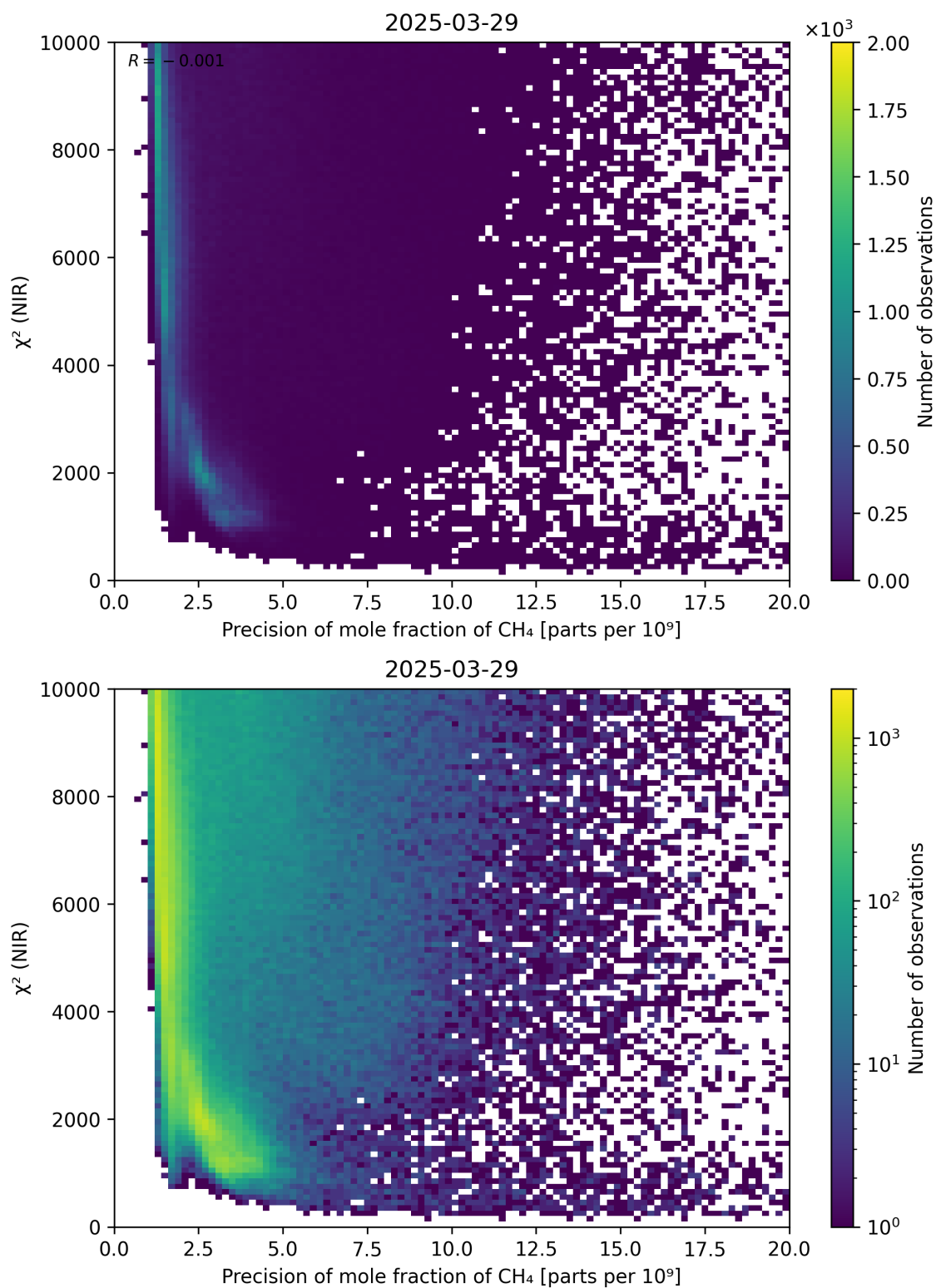
Figure 78: Scatter density plot of “Precision of mole fraction of CH 4 ” against “ \chi^2 (NIR)” for 2025-03-28 to 2025-03-30.
