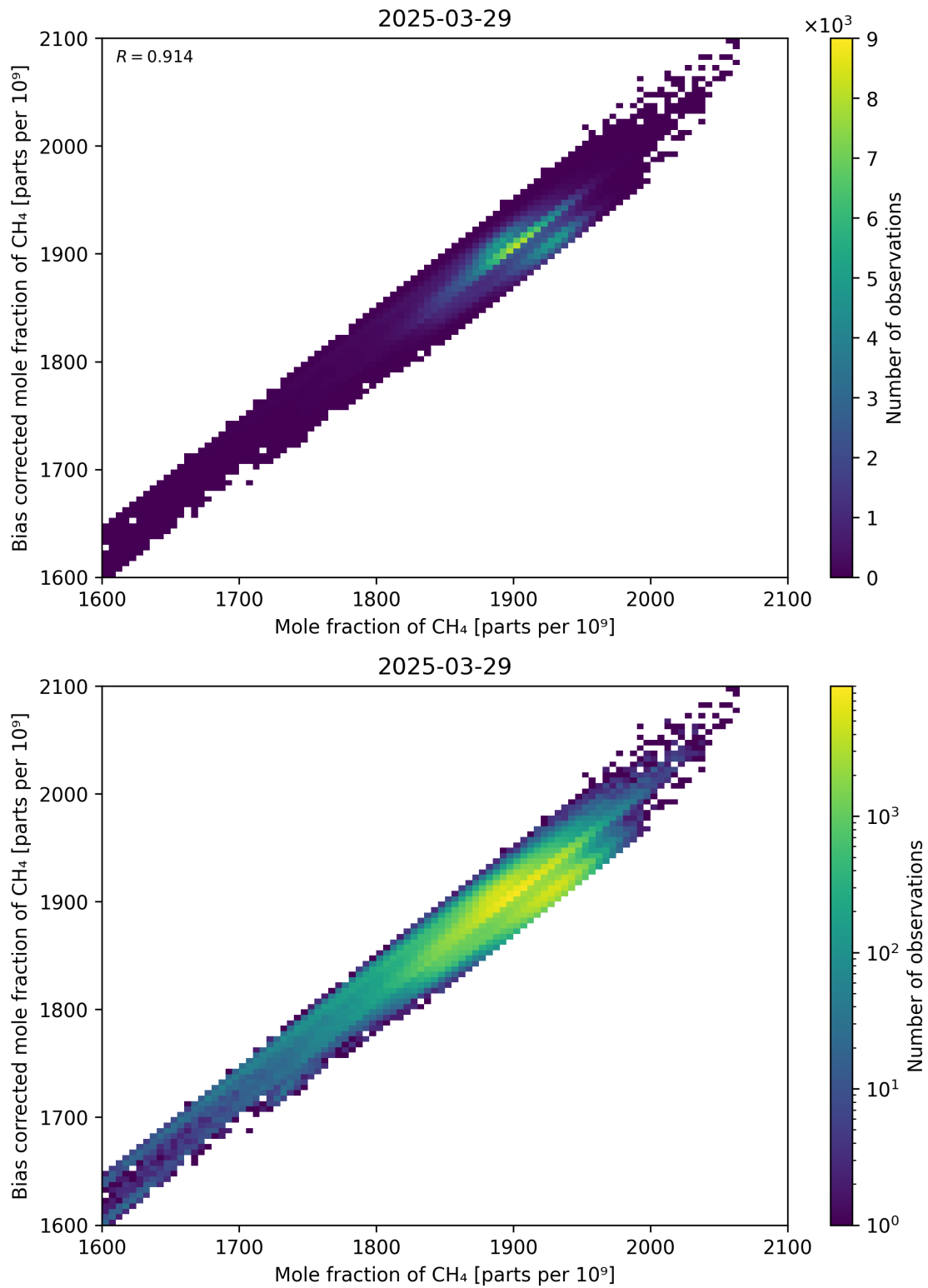
Figure 74: Scatter density plot of “Mole fraction of CH 4 ” against “Bias corrected mole fraction of CH 4 ” for 2025-03-28 to 2025-03-30.
