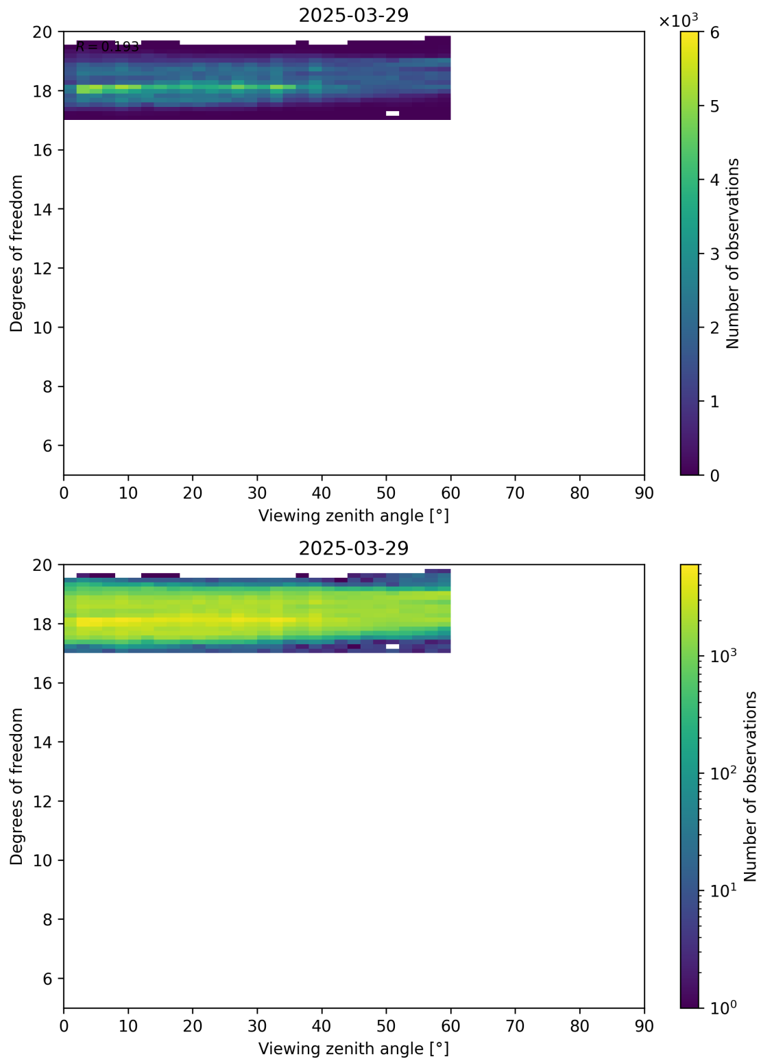
Figure 107: Scatter density plot of “Viewing zenith angle” against “Degrees of freedom” for 2025-03-28 to 2025-03-30.
