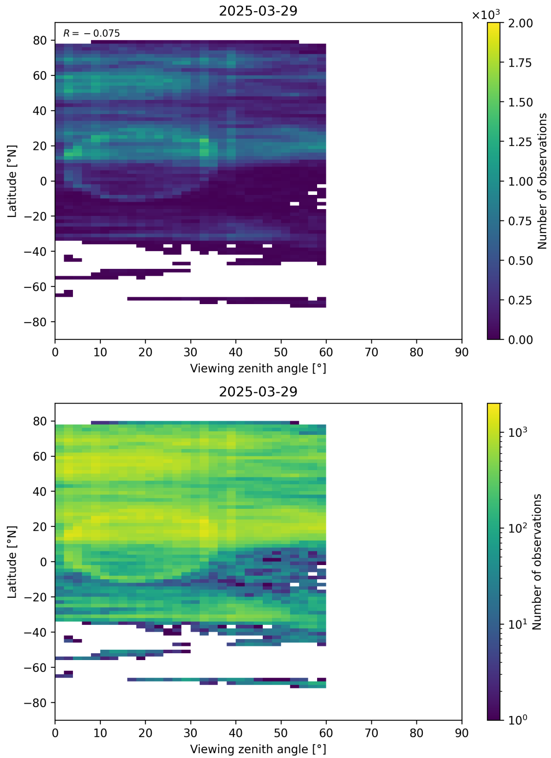
Figure 109: Scatter density plot of “Viewing zenith angle” against “Latitude” for 2025-03-28 to 2025-03-30.
