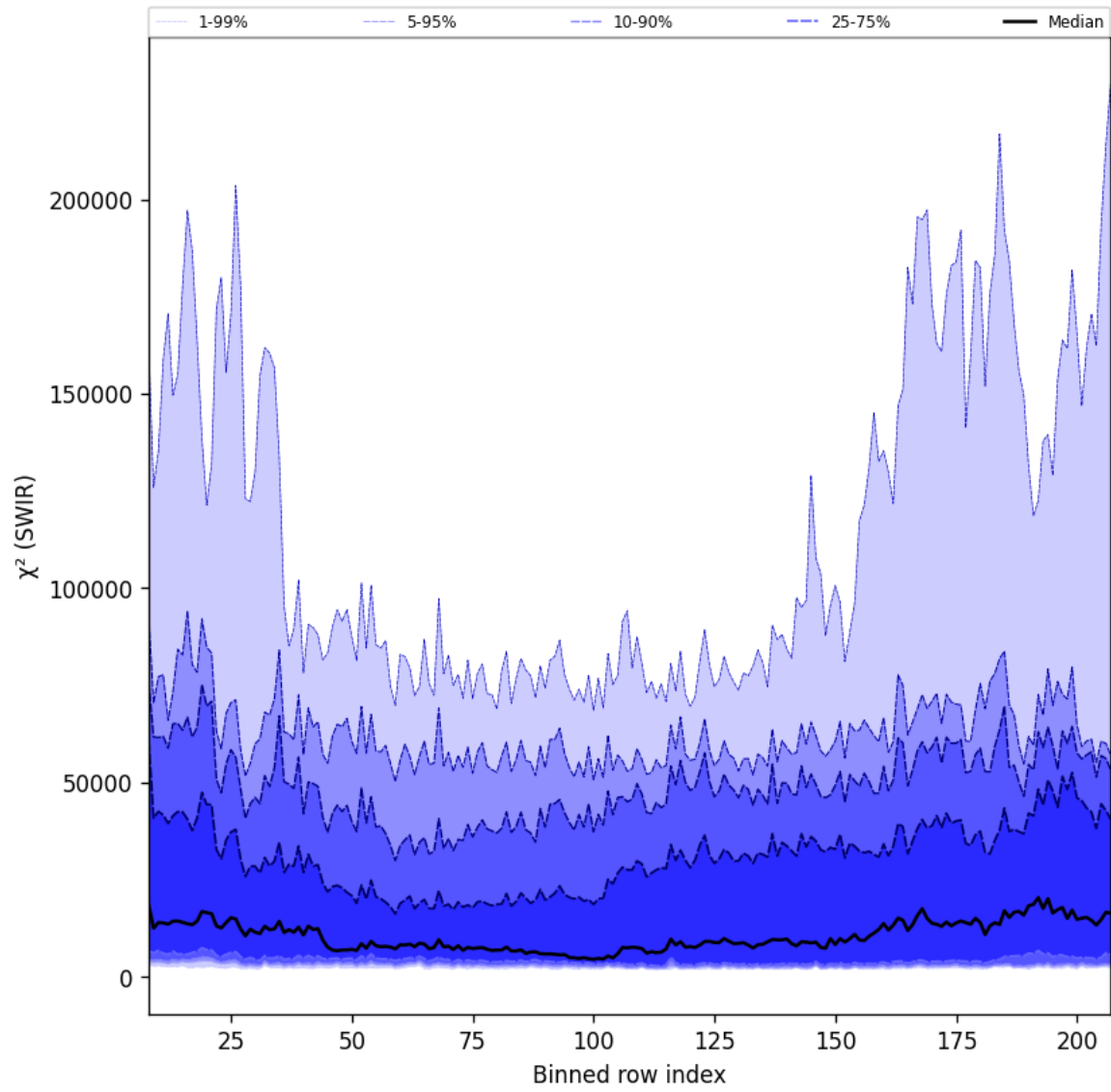
Figure 39: Along track statistics of “ \chi^2 (SWIR)” for 2025-03-28 to 2025-03-30
