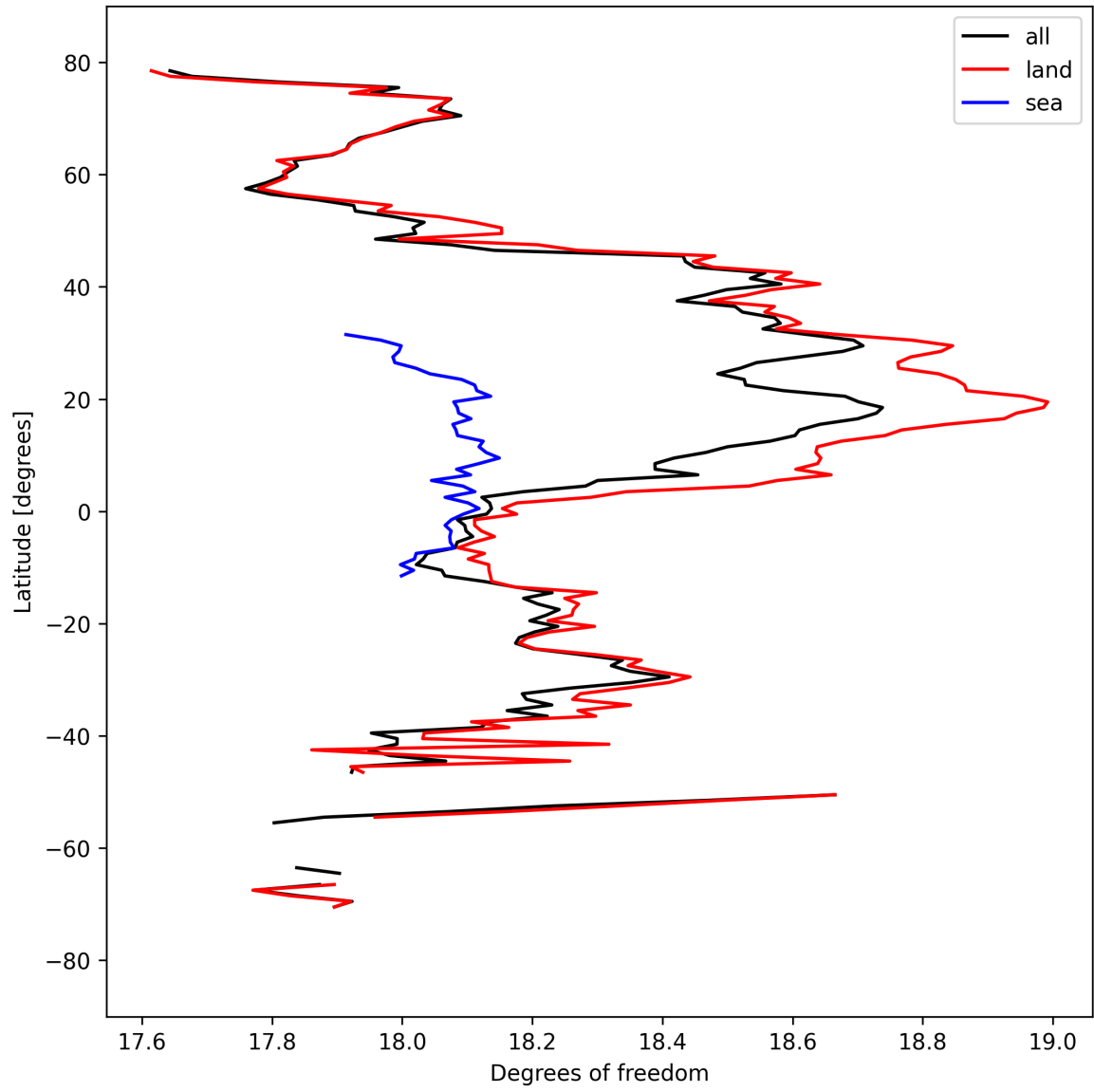
Figure 19: Zonal average of “Degrees of freedom” for 2025-03-28 to 2025-03-30.
