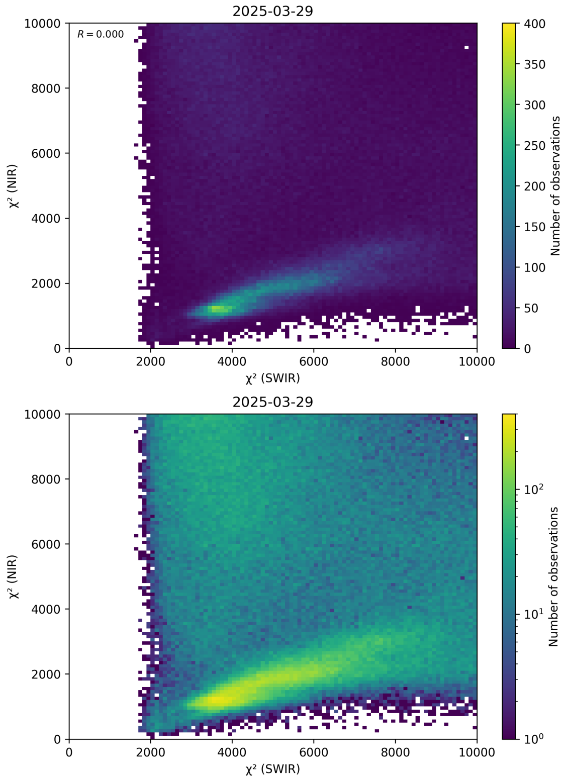
Figure 47: Scatter density plot of “ \chi^2 (SWIR)” against “ \chi^2 (NIR)” for 2025-03-28 to 2025-03-30.
