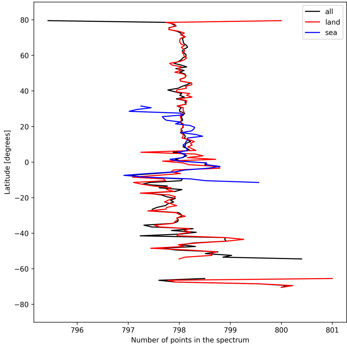
Figure 15: Zonal average of “Number of points in the spectrum” for 2025-03-29 to 2025-03-31.
