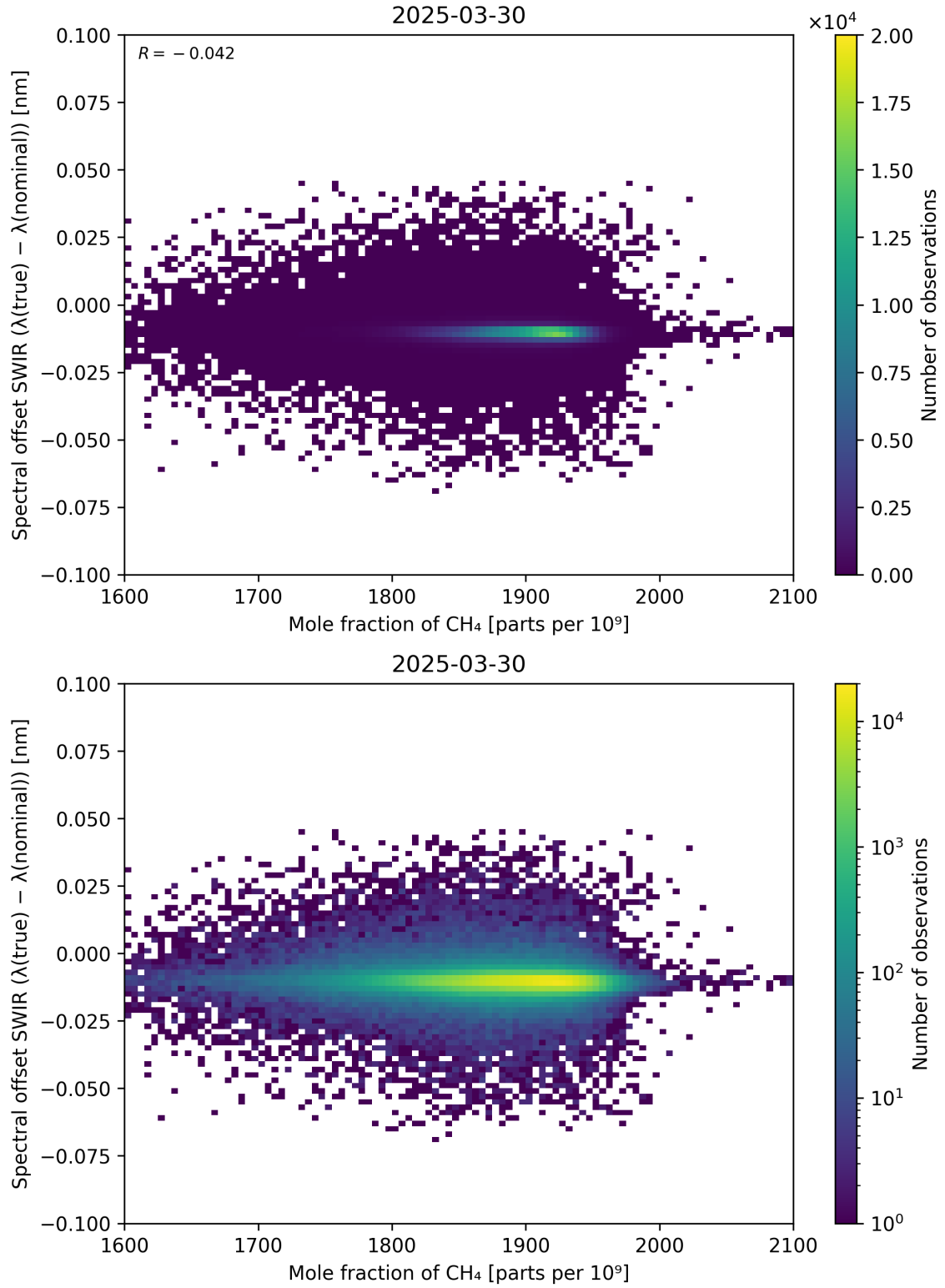
Figure 86: Scatter density plot of “Mole fraction of CH 4 ” against “Spectral offset SWIR ( \lambda_{\text{true}} - \lambda_{\text{nominal}} )” for 2025-03-29 to 2025-03-31.
