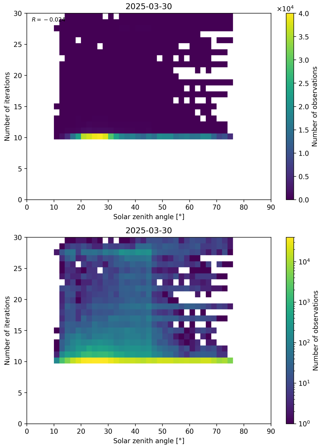
Figure 102: Scatter density plot of “Solar zenith angle” against “Number of iterations” for 2025-03-29 to 2025-03-31.
