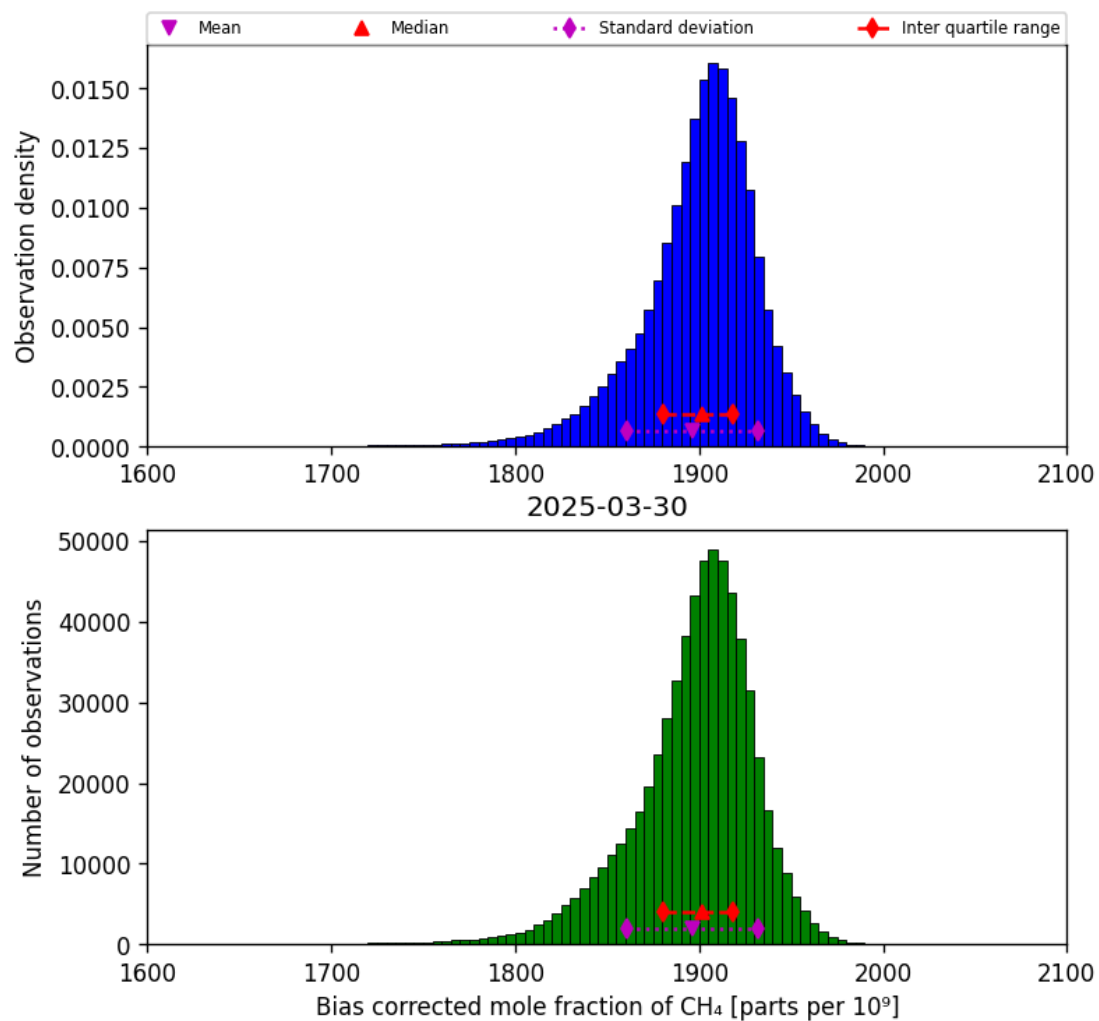
Figure 25: Histogram of “Bias corrected mole fraction of CH 4 ” for 2025-03-29 to 2025-03-31
