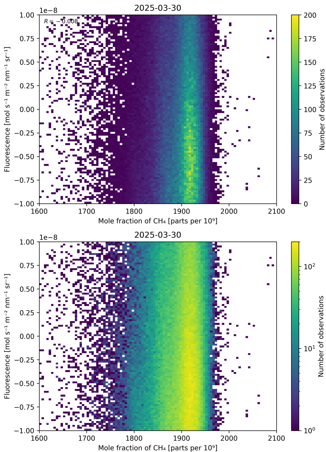
Figure 73: Scatter density plot of “Mole fraction of \text{CH}_4 ” against “Fluorescence” for 2025-03-29 to 2025-03-31.
