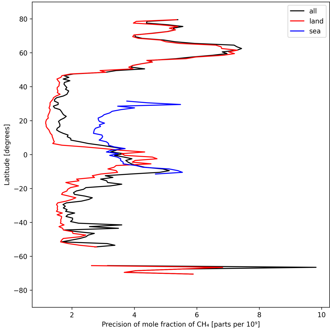
Figure 13: Zonal average of “Precision of mole fraction of CH 4 ” for 2025-03-29 to 2025-03-31.
