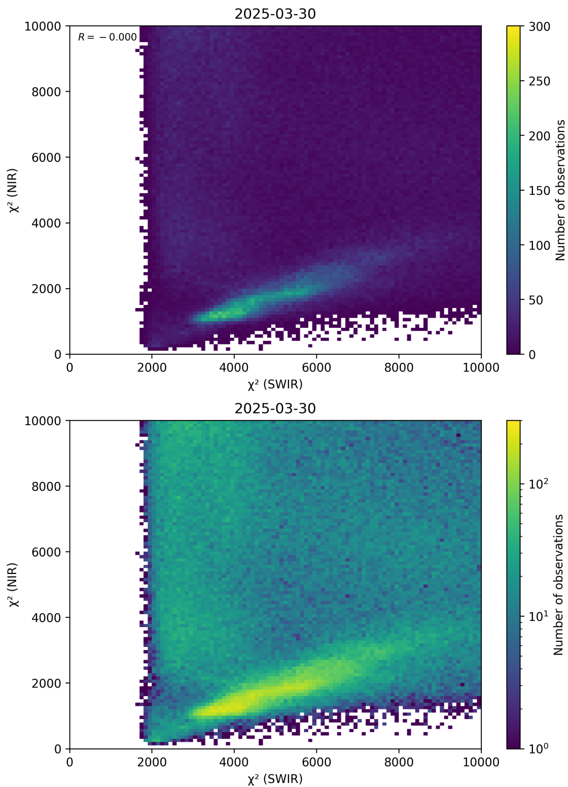
Figure 47: Scatter density plot of “ \chi^2 (SWIR)” against “ \chi^2 (NIR)” for 2025-03-29 to 2025-03-31.
