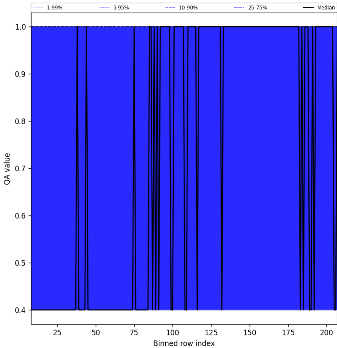
Figure 33: Along track statistics of “QA value” for 2025-03-29 to 2025-03-31
