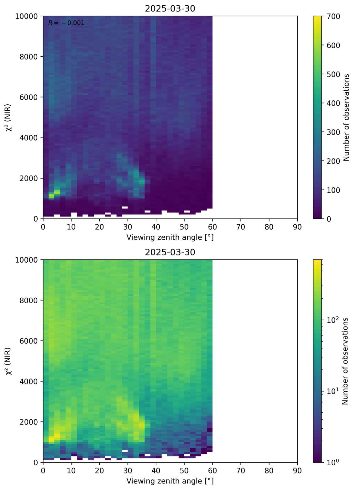
Figure 105: Scatter density plot of “Viewing zenith angle” against “ \chi^2 (NIR)” for 2025-03-29 to 2025-03-31.
