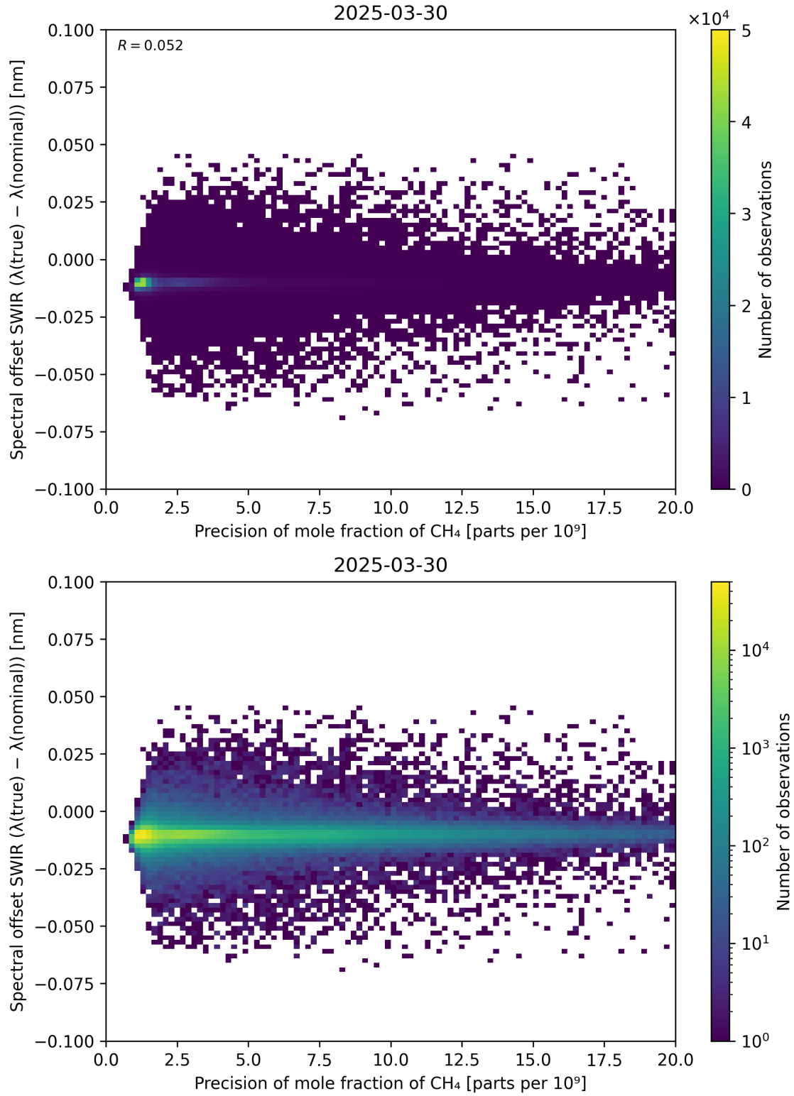
Figure 85: Scatter density plot of “Precision of mole fraction of \text{CH}_4 ” against “Spectral offset SWIR ( \lambda_{\text{true}} - \lambda_{\text{nominal}} )” for 2025-03-29 to 2025-03-31.
