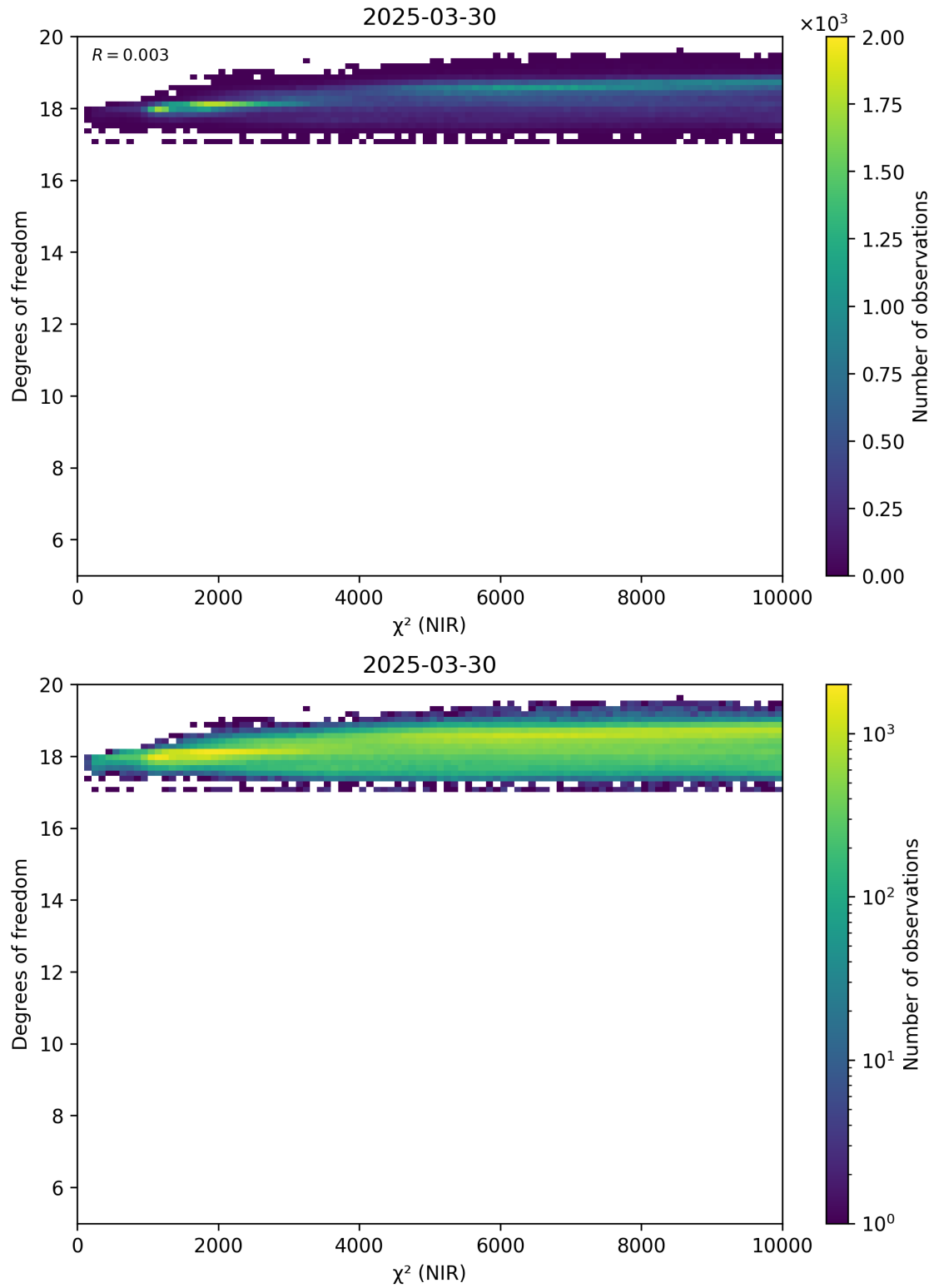
Figure 44: Scatter density plot of “ \chi^2 (NIR)” against “Degrees of freedom” for 2025-03-29 to 2025-03-31.
