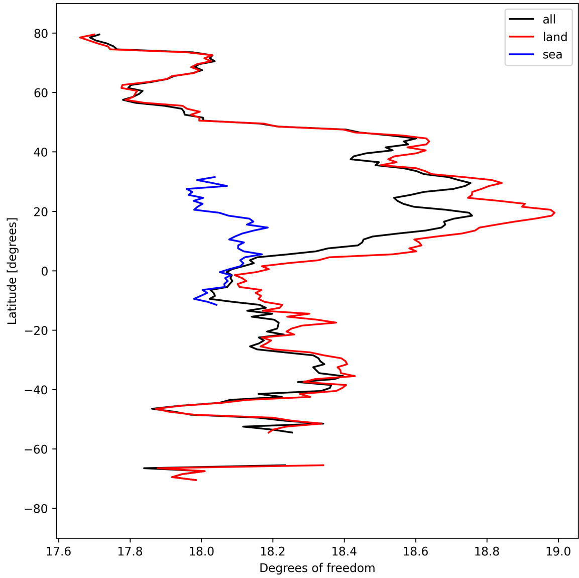
Figure 19: Zonal average of “Degrees of freedom” for 2025-03-29 to 2025-03-31.
