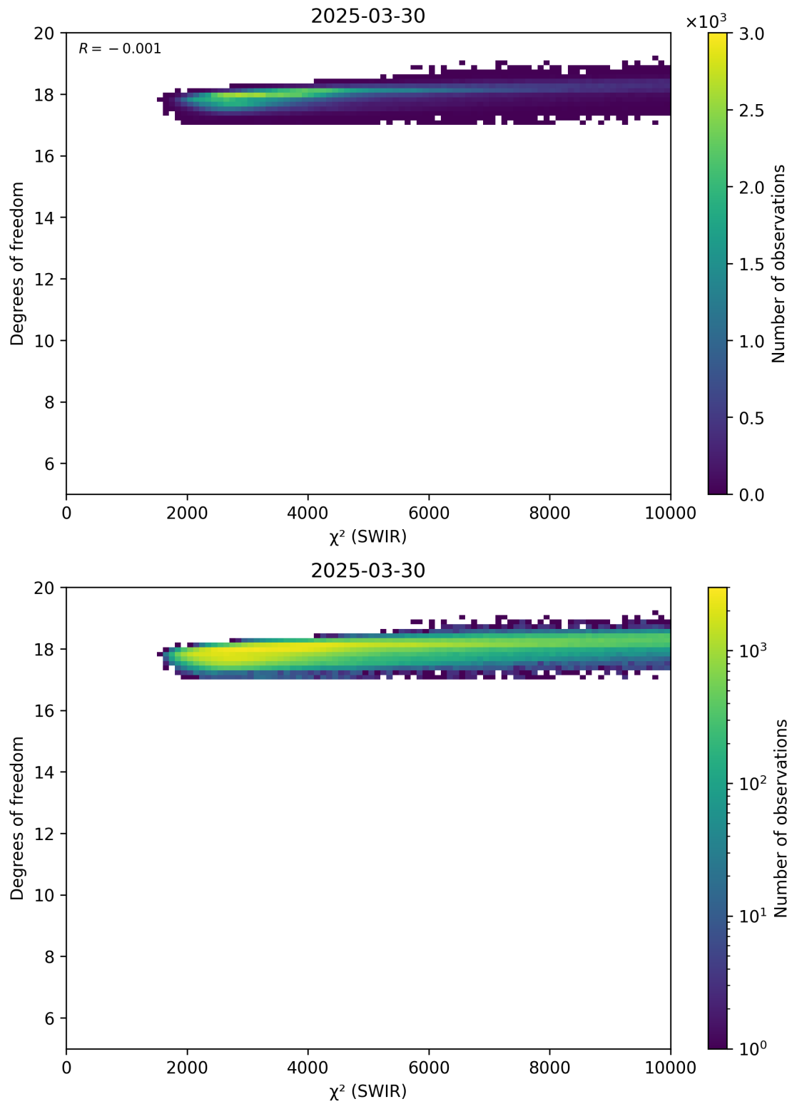
Figure 48: Scatter density plot of “ \chi^2 (SWIR)” against “Degrees of freedom” for 2025-03-29 to 2025-03-31.
