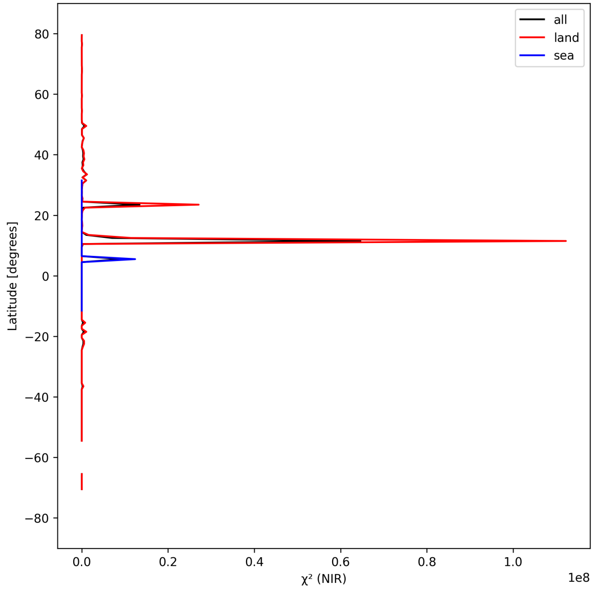
Figure 18: Zonal average of “ \chi^2 (NIR)” for 2025-03-29 to 2025-03-31.
