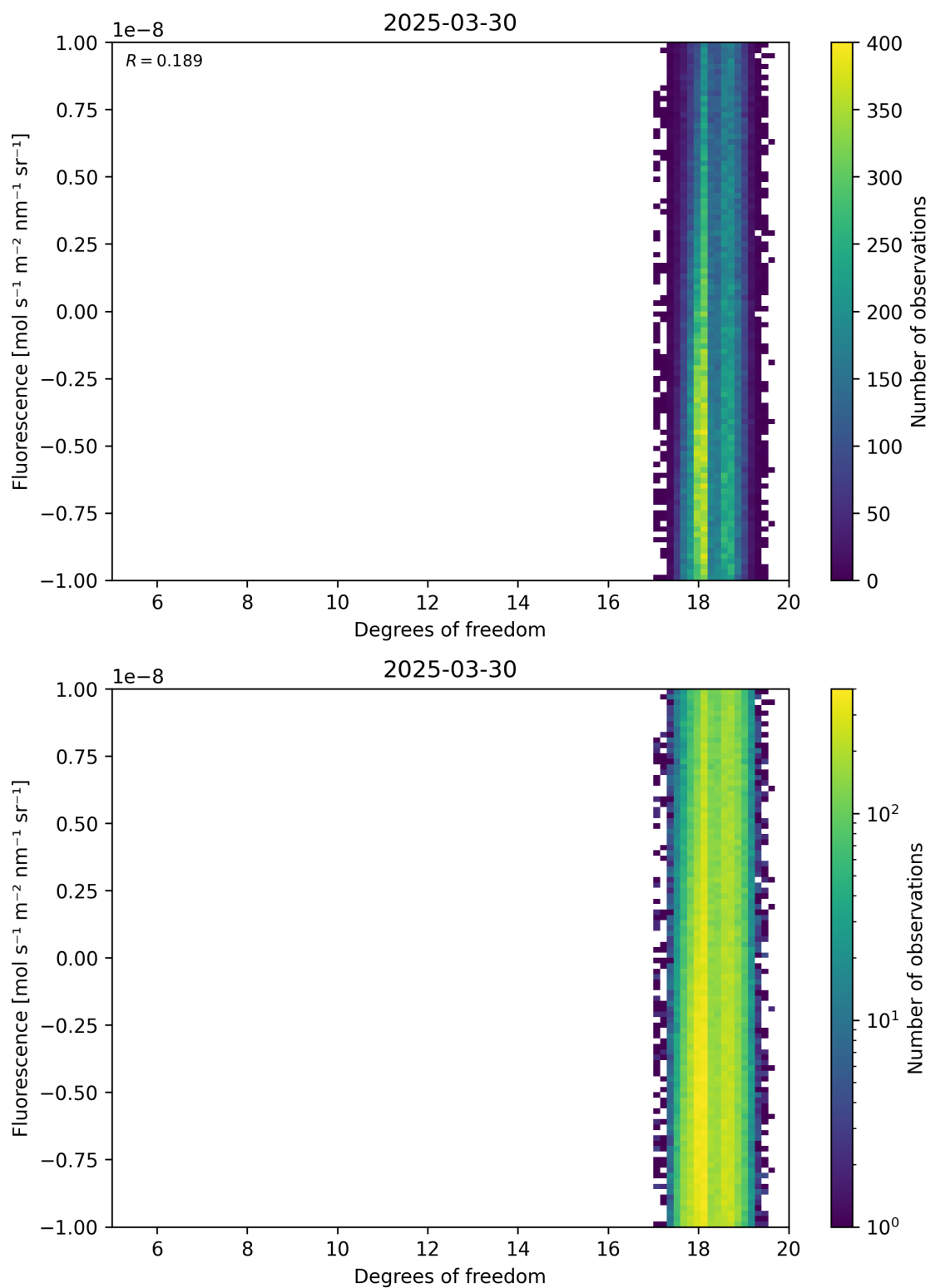
Figure 51: Scatter density plot of “Degrees of freedom” against “Fluorescence” for 2025-03-29 to 2025-03-31.
