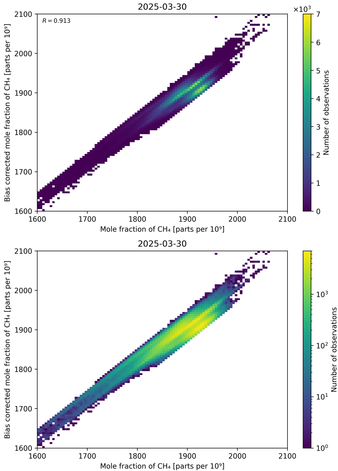
Figure 74: Scatter density plot of “Mole fraction of CH 4 ” against “Bias corrected mole fraction of CH 4 ” for 2025-03-29 to 2025-03-31.
