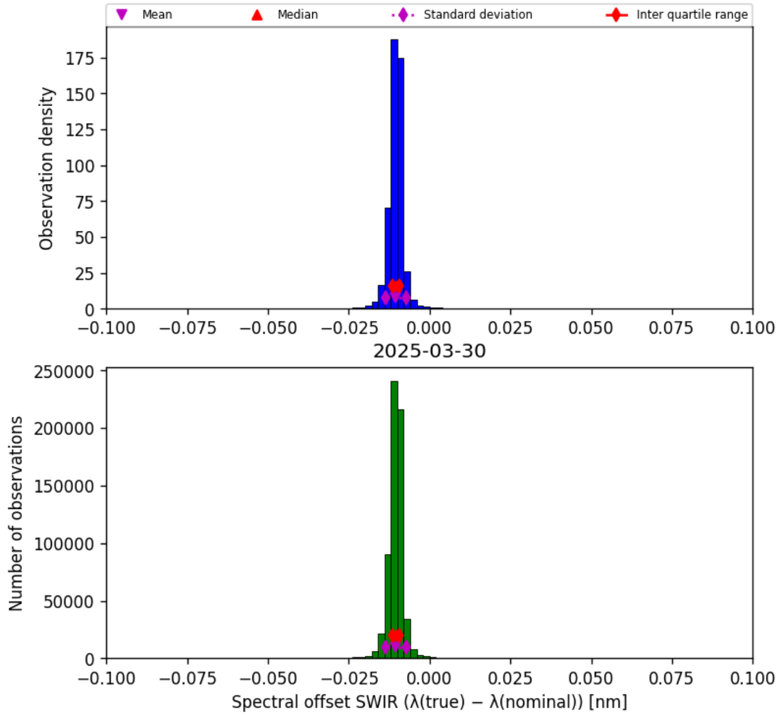
Figure 27: Histogram of “Spectral offset SWIR ( \lambda_{\text{true}} - \lambda_{\text{nominal}} )” for 2025-03-29 to 2025-03-31
