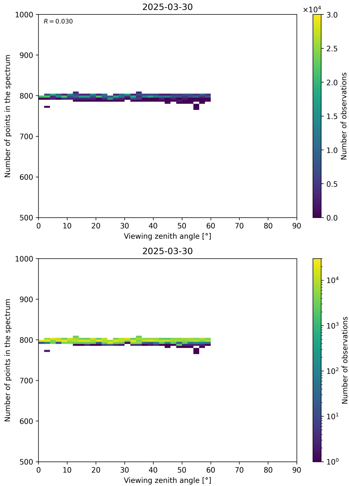
Figure 114: Scatter density plot of “Viewing zenith angle” against “Number of points in the spectrum” for 2025-03-29 to 2025-03-31.
