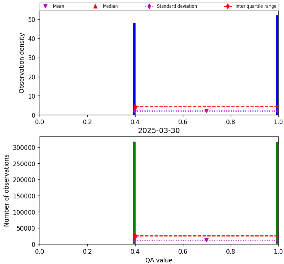
Figure 22: Histogram of “QA value” for 2025-03-29 to 2025-03-31
