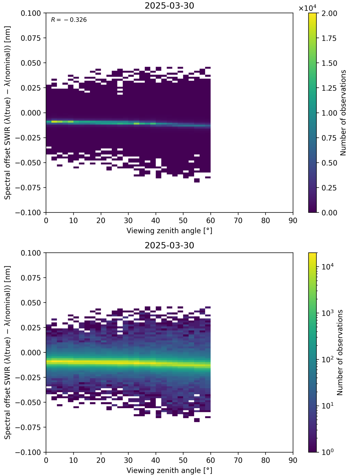
Figure 116: Scatter density plot of “Viewing zenith angle” against “Spectral offset SWIR ( \lambda_{\text{true}} - \lambda_{\text{nominal}} )” for 2025-03-29 to 2025-03-31.
