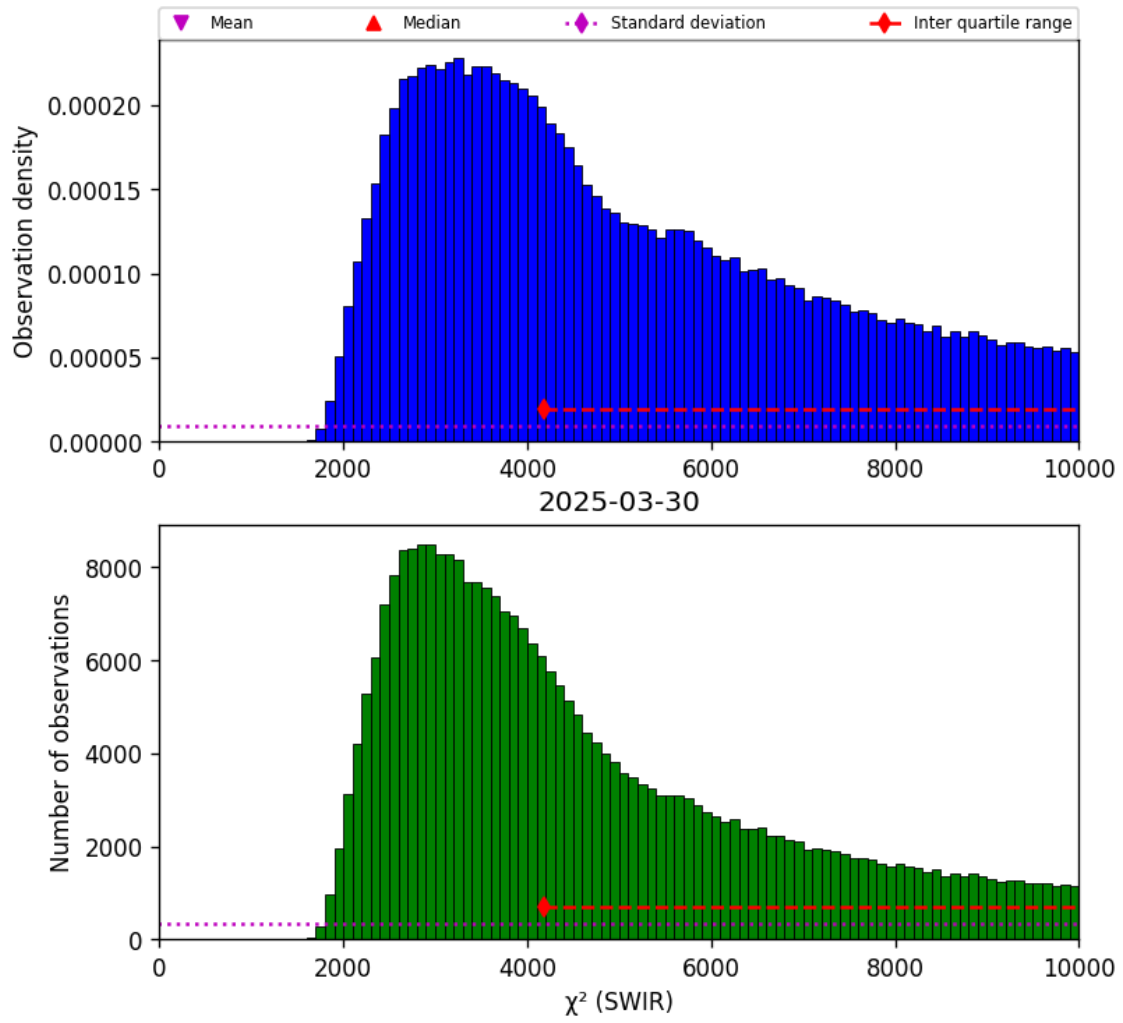
Figure 28: Histogram of “ \chi^2 (SWIR)” for 2025-03-29 to 2025-03-31
