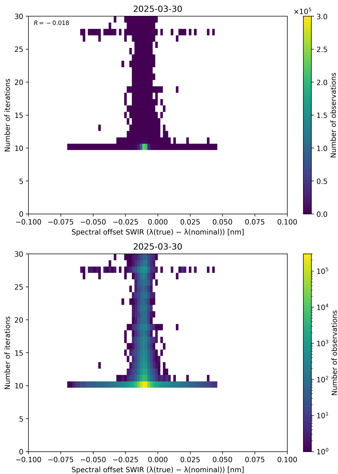
Figure 121: Scatter density plot of “Spectral offset SWIR ( \lambda_{\text{true}} - \lambda_{\text{nominal}} )” against “Number of iterations” for 2025-03-29 to 2025-03-31.
