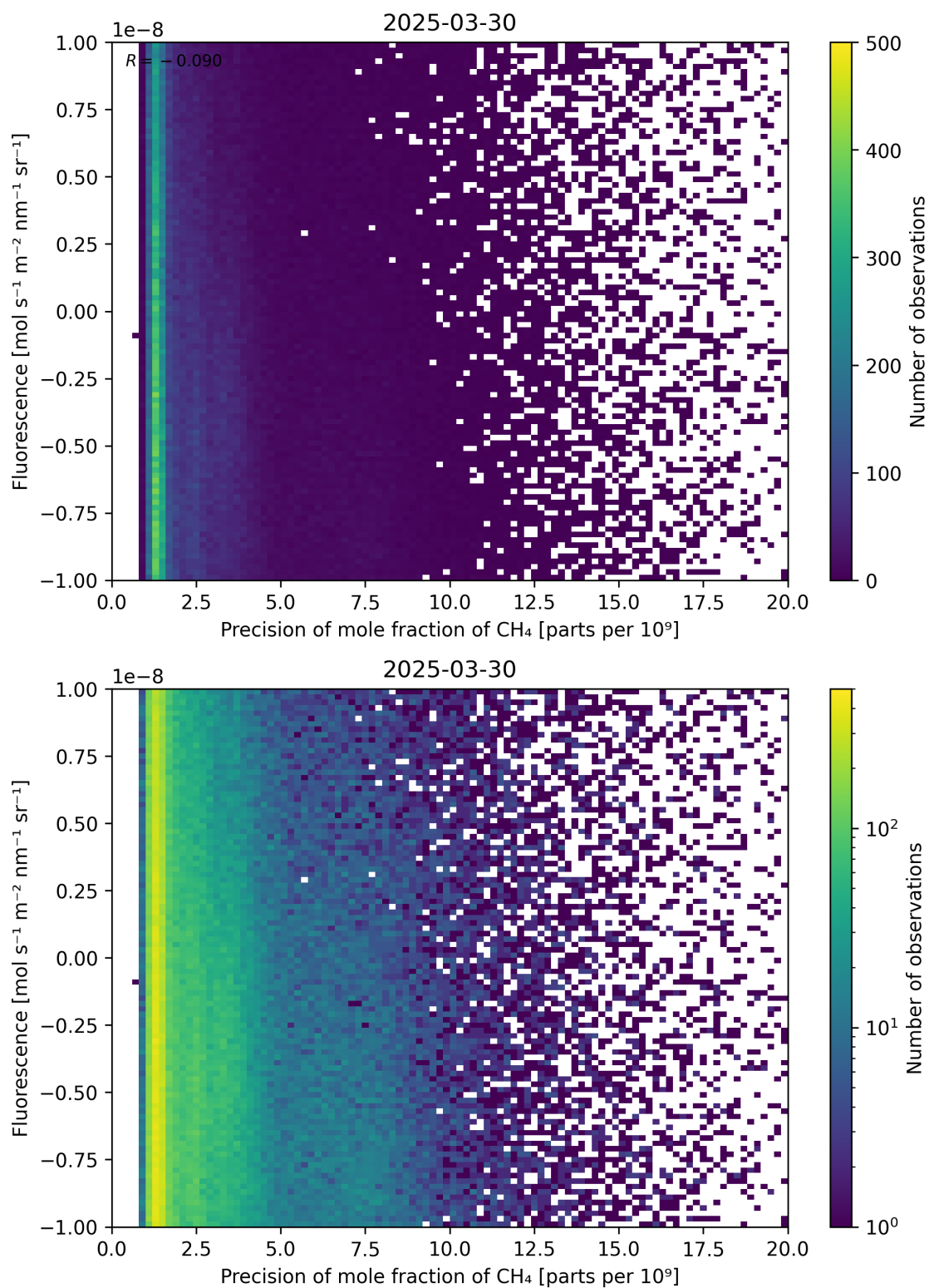
Figure 81: Scatter density plot of “Precision of mole fraction of \text{CH}_4 ” against “Fluorescence” for 2025-03-29 to 2025-03-31.
