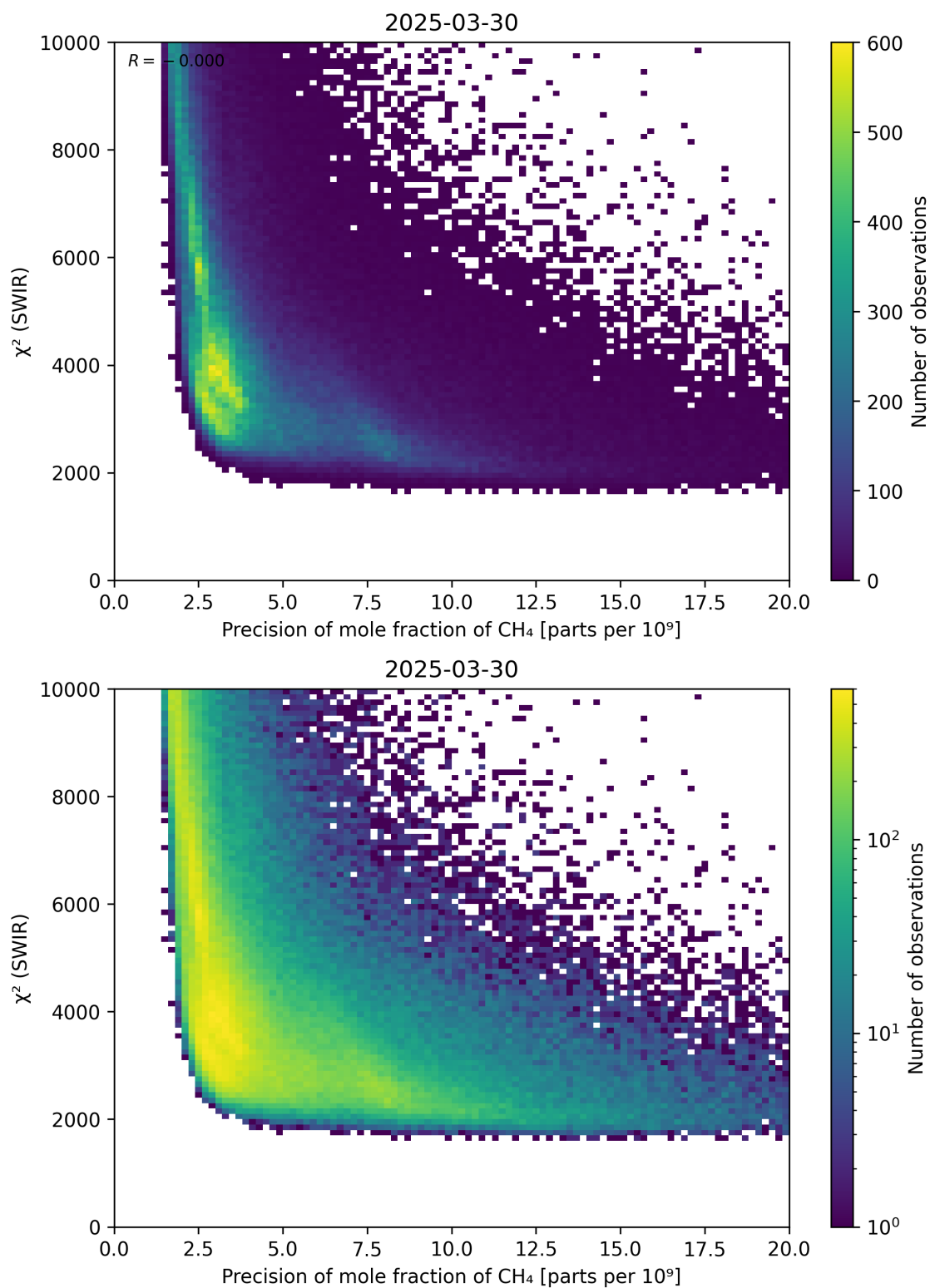
Figure 79: Scatter density plot of “Precision of mole fraction of CH 4 ” against “ \chi^2 (SWIR)” for 2025-03-29 to 2025-03-31.
