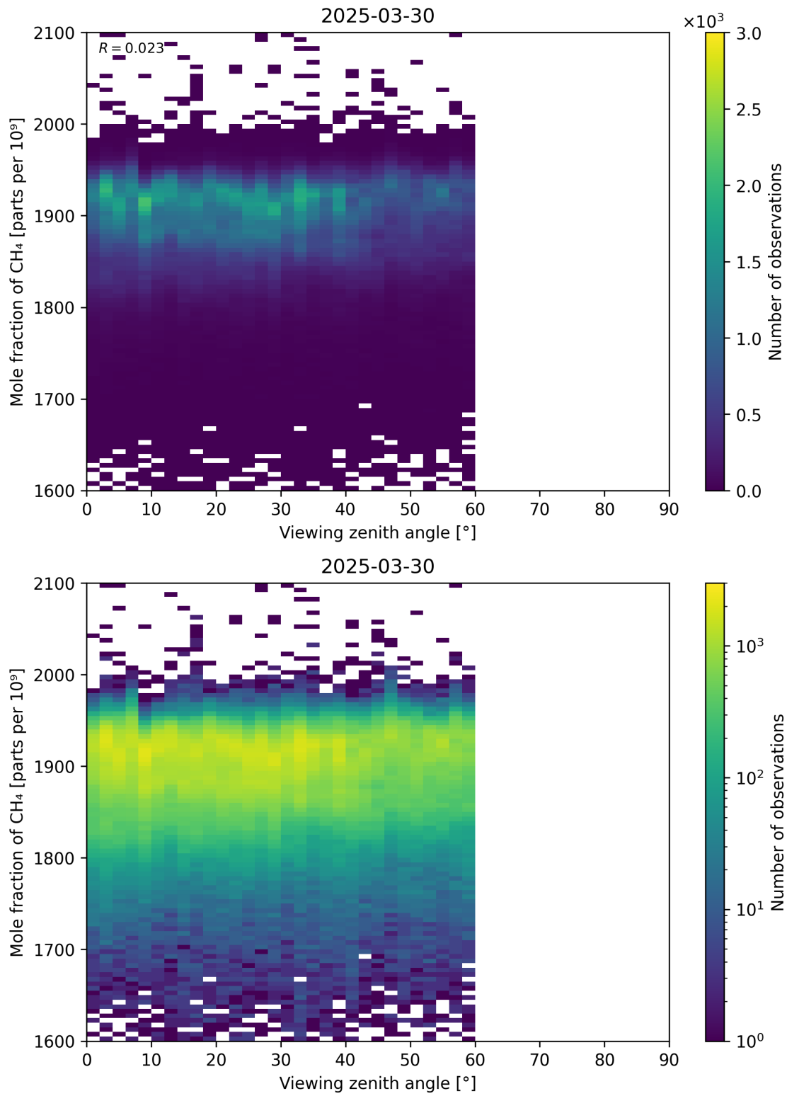
Figure 110: Scatter density plot of “Viewing zenith angle” against “Mole fraction of CH 4 ” for 2025-03-29 to 2025-03-31.
