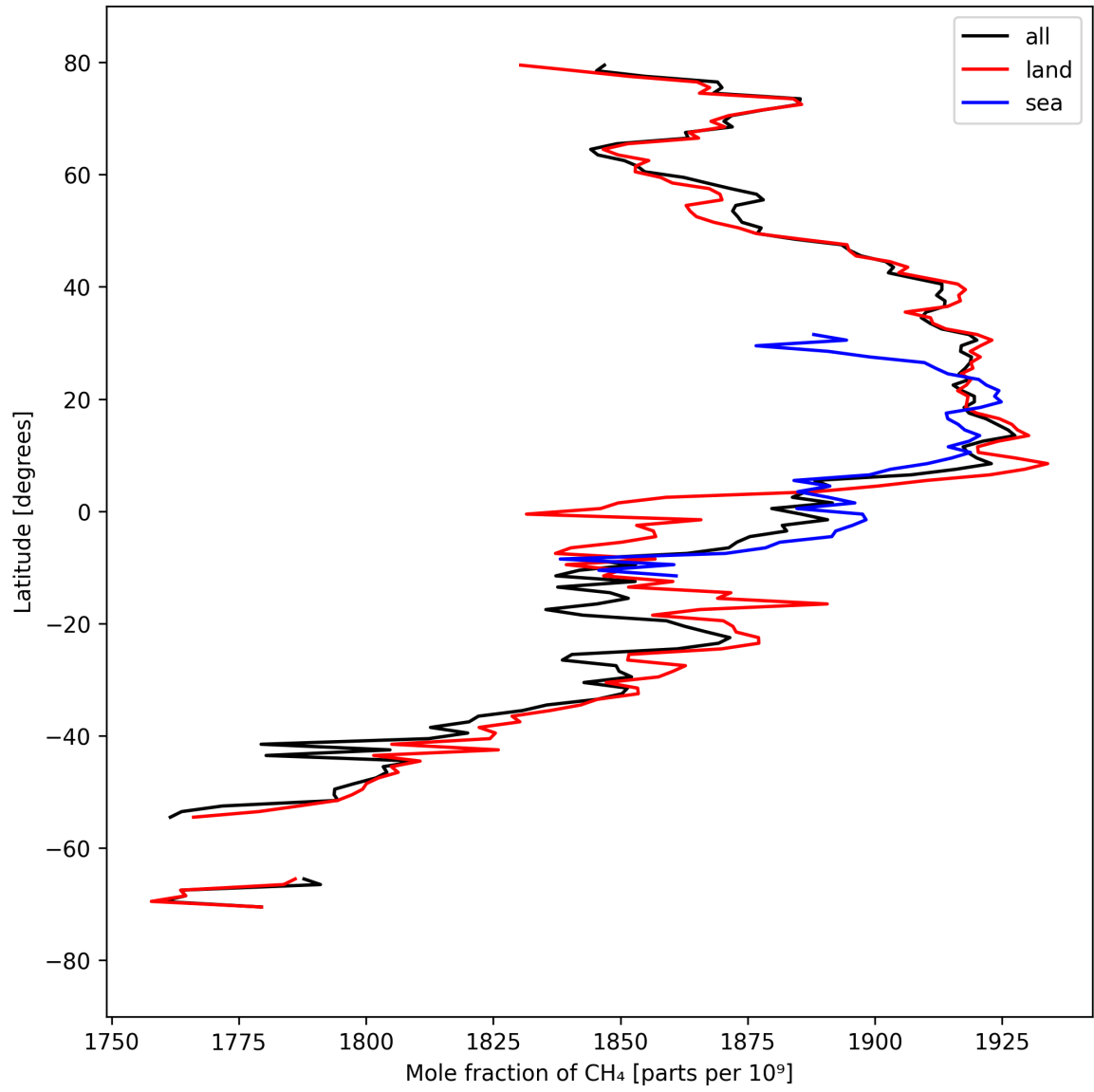
Figure 12: Zonal average of “Mole fraction of \text{CH}_4 ” for 2025-03-29 to 2025-03-31.
