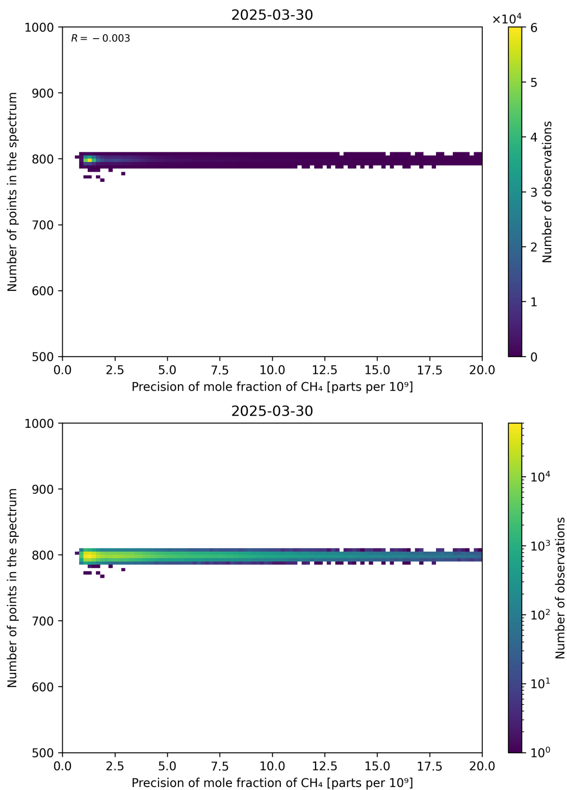
Figure 84: Scatter density plot of “Precision of mole fraction of CH 4 ” against “Number of points in the spectrum” for 2025-03-29 to 2025-03-31.
