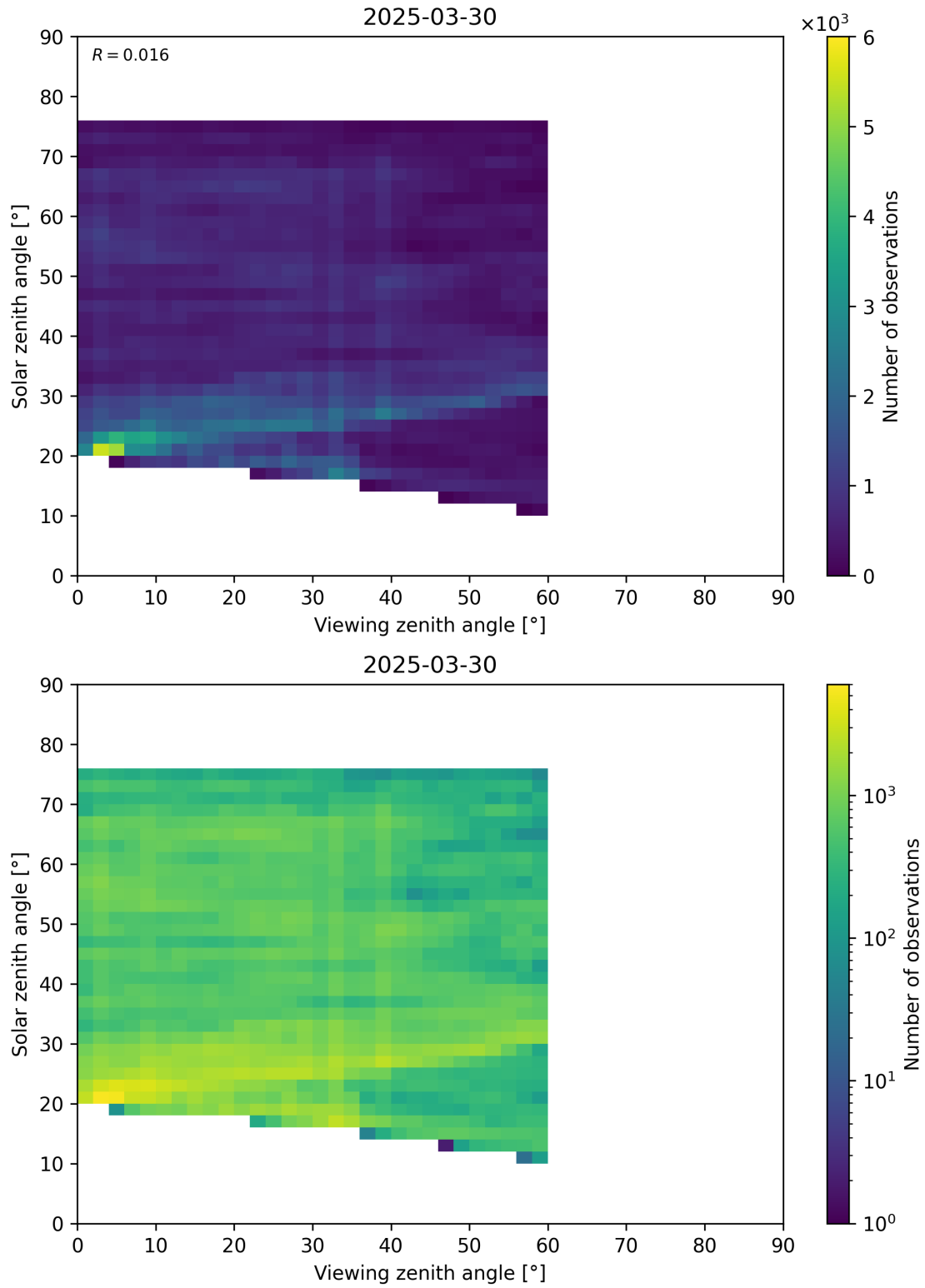
Figure 115: Scatter density plot of “Viewing zenith angle” against “Solar zenith angle” for 2025-03-29 to 2025-03-31.
