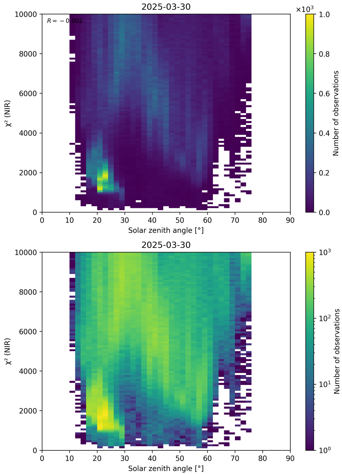
Figure 94: Scatter density plot of “Solar zenith angle” against “ \chi^2 (NIR)” for 2025-03-29 to 2025-03-31.
