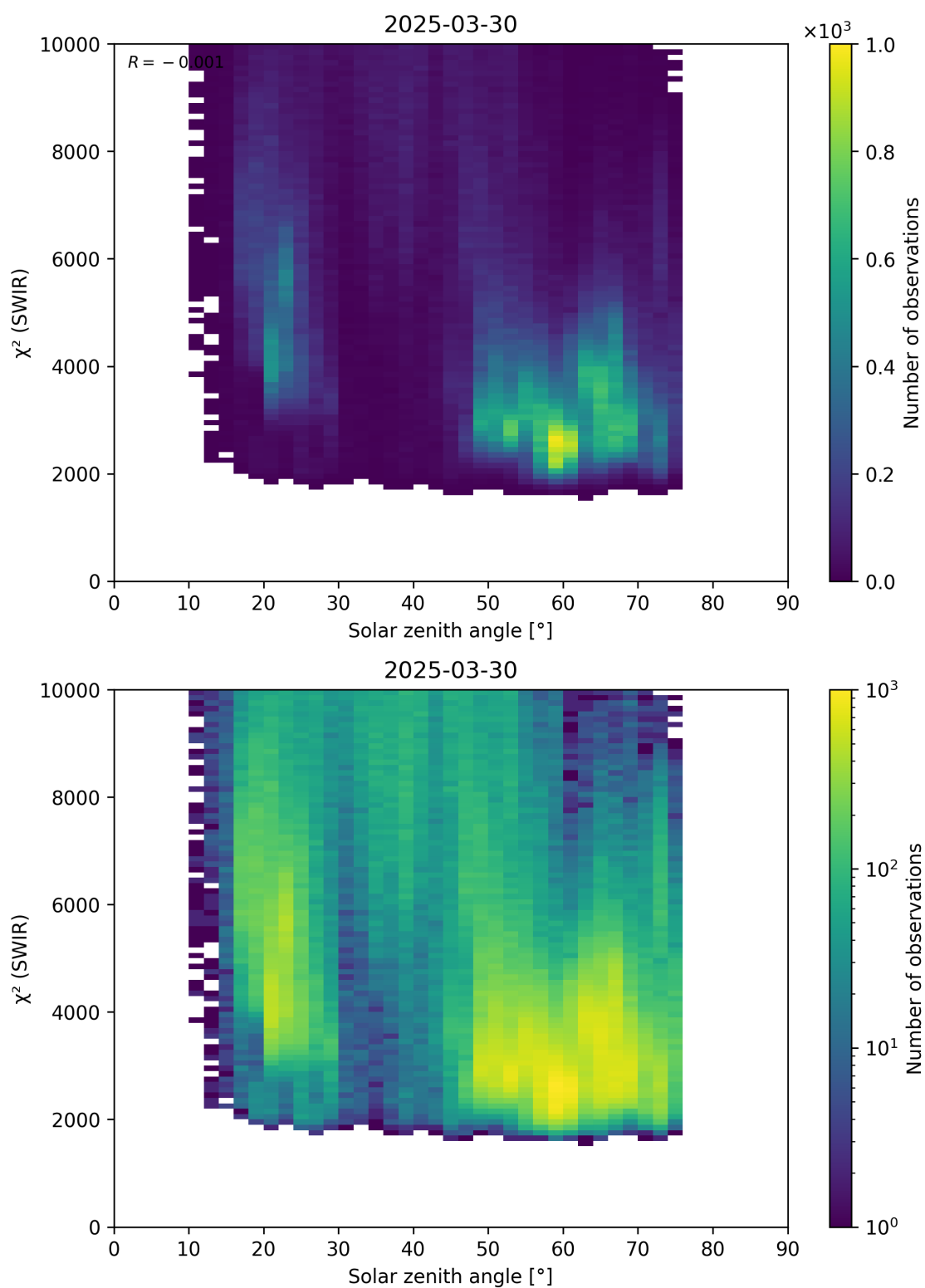
Figure 95: Scatter density plot of “Solar zenith angle” against “ \chi^2 (SWIR)” for 2025-03-29 to 2025-03-31.
