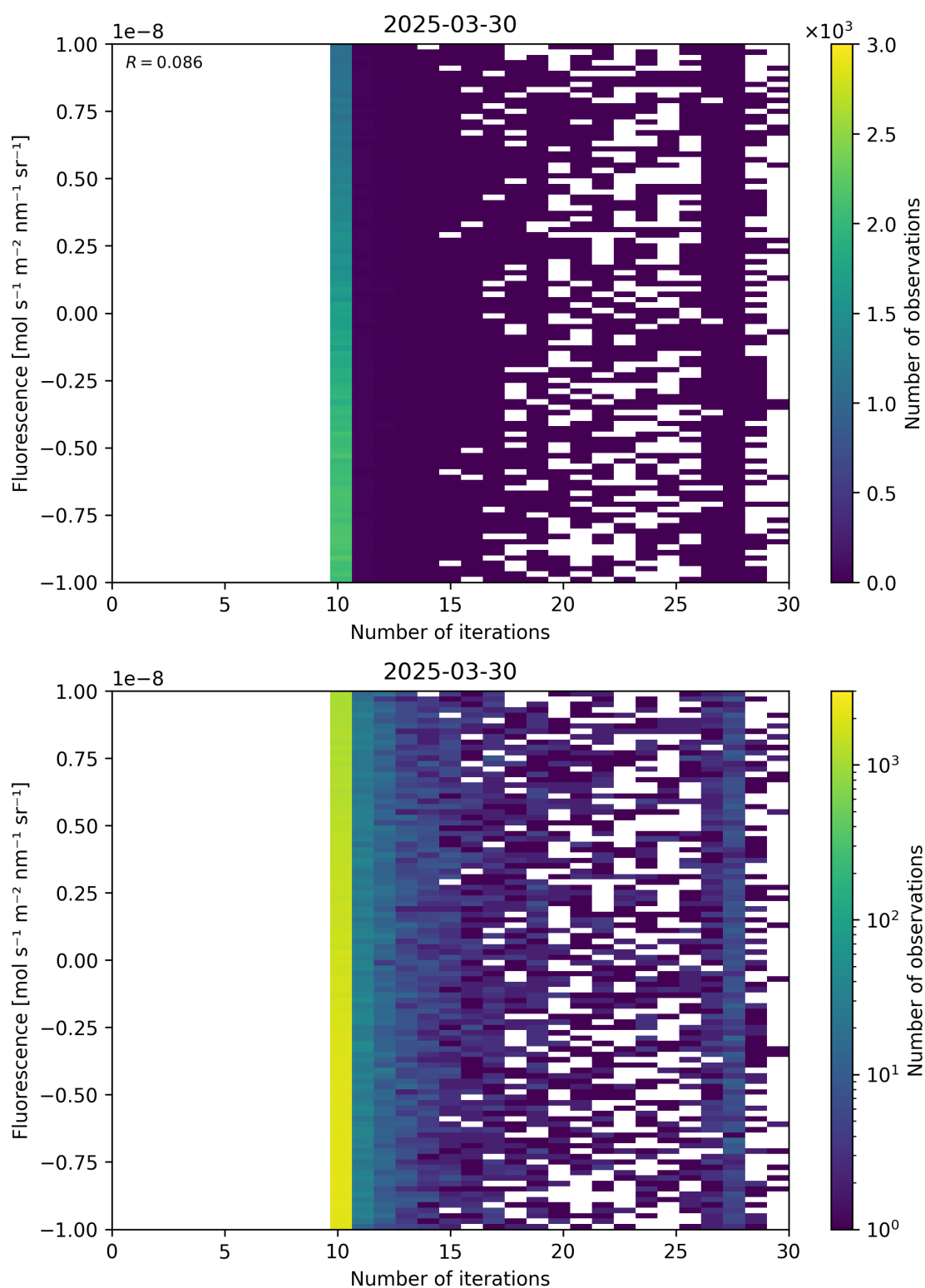
Figure 87: Scatter density plot of “Number of iterations” against “Fluorescence” for 2025-03-29 to 2025-03-31.
