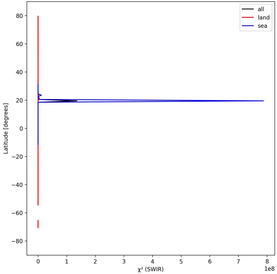
Figure 17: Zonal average of “ \chi^2 (SWIR)” for 2025-03-29 to 2025-03-31.
