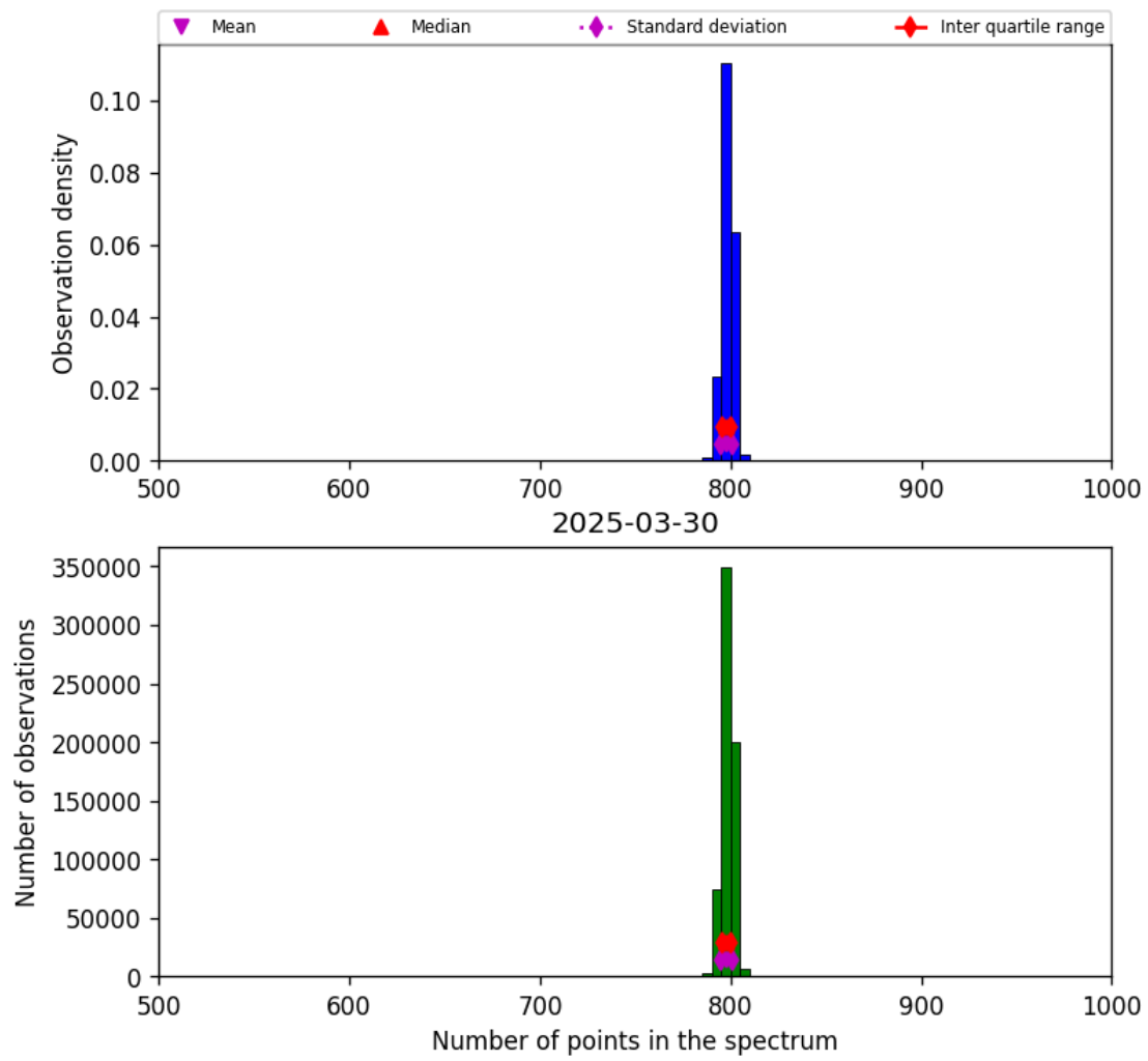
Figure 26: Histogram of “Number of points in the spectrum” for 2025-03-29 to 2025-03-31
