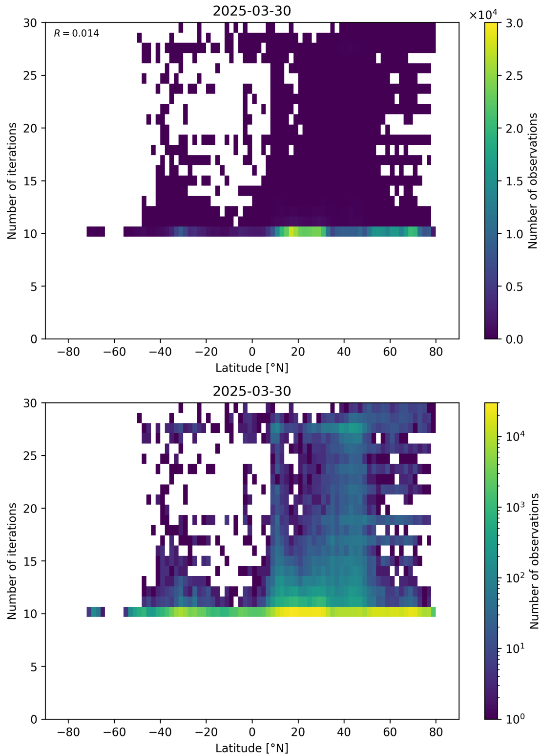
Figure 60: Scatter density plot of “Latitude” against “Number of iterations” for 2025-03-29 to 2025-03-31.
