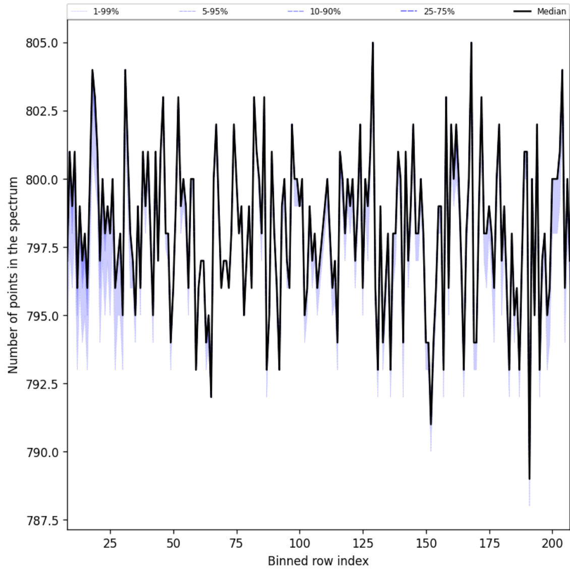
Figure 37: Along track statistics of “Number of points in the spectrum” for 2025-03-29 to 2025-03-31
