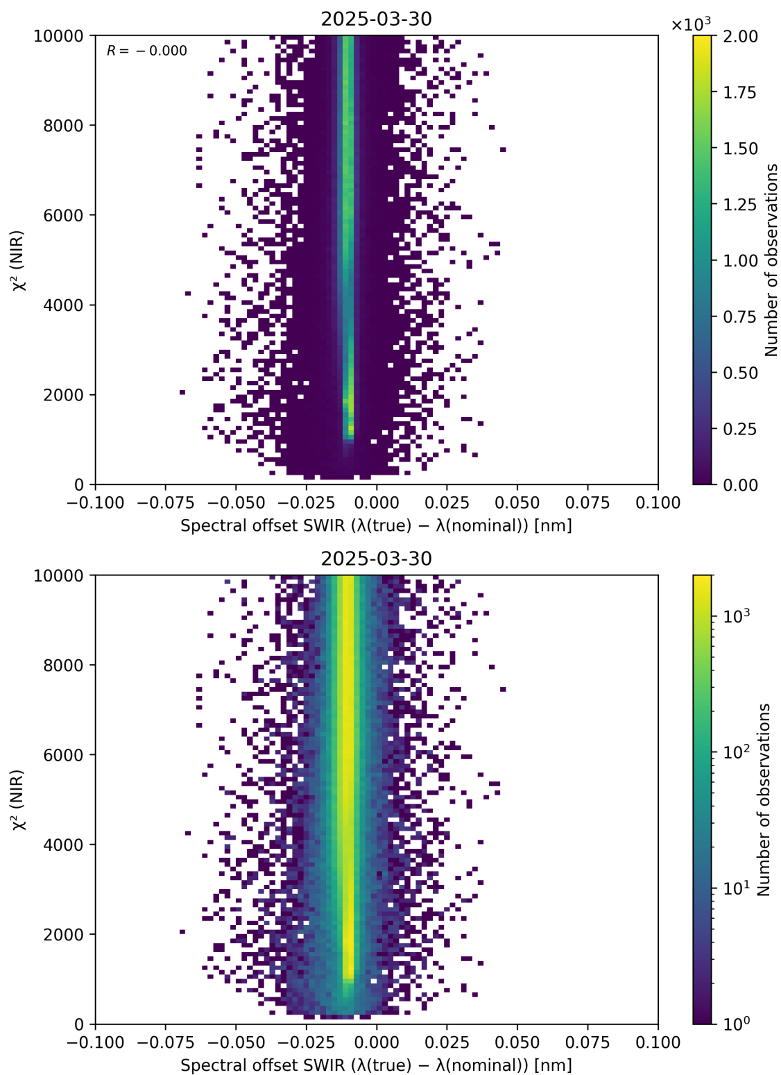
Figure 117: Scatter density plot of “Spectral offset SWIR ( \lambda_{\text{true}} - \lambda_{\text{nominal}} )” against “ \chi^2 (NIR)” for 2025-03-29 to 2025-03-31.
