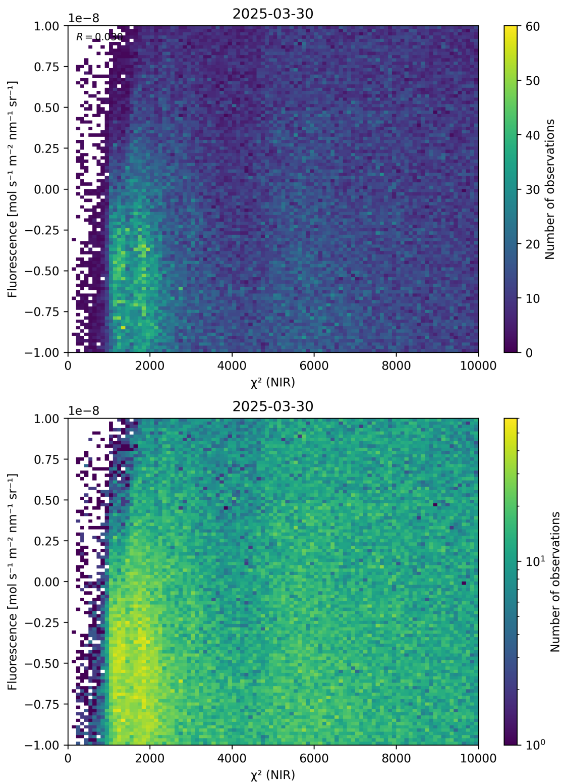
Figure 45: Scatter density plot of “ \chi^2 (NIR)” against “Fluorescence” for 2025-03-29 to 2025-03-31.
