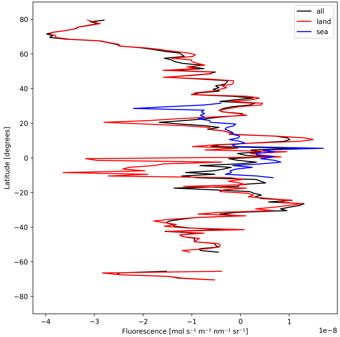
Figure 21: Zonal average of “Fluorescence” for 2025-03-29 to 2025-03-31.
