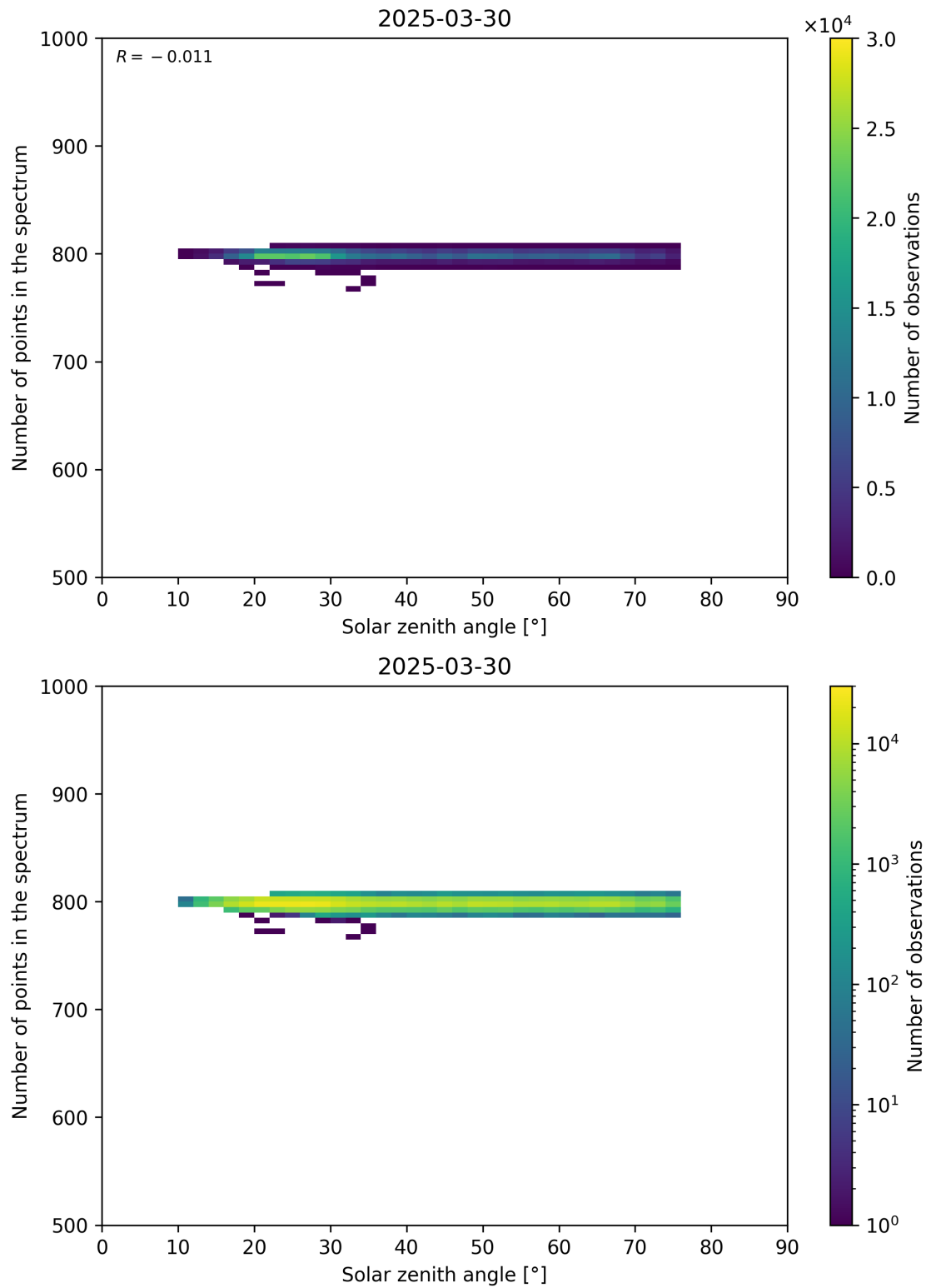
Figure 103: Scatter density plot of “Solar zenith angle” against “Number of points in the spectrum” for 2025-03-29 to 2025-03-31.
