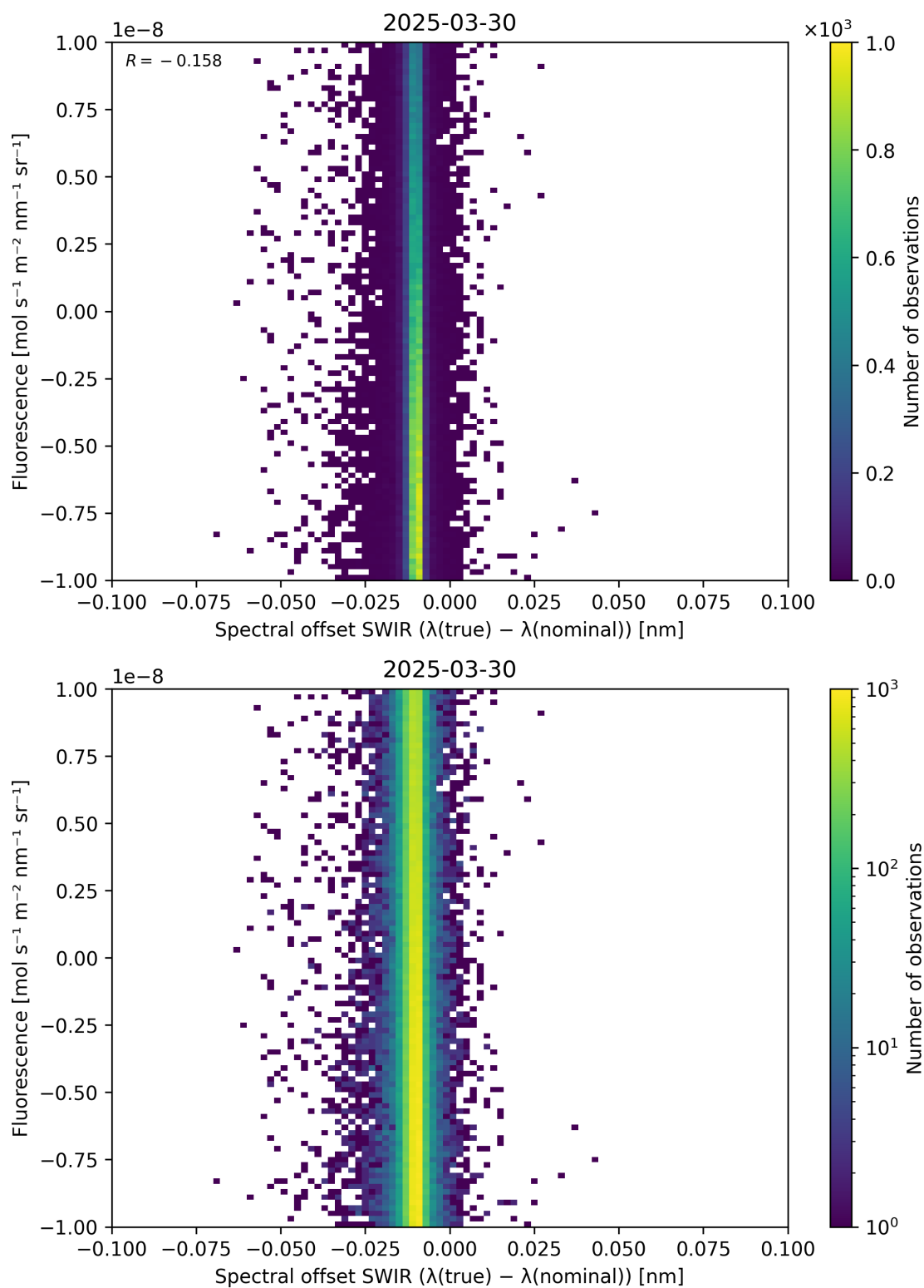
Figure 120: Scatter density plot of “Spectral offset SWIR ( \lambda_{\text{true}} - \lambda_{\text{nominal}} )” against “Fluorescence” for 2025-03-29 to 2025-03-31.
