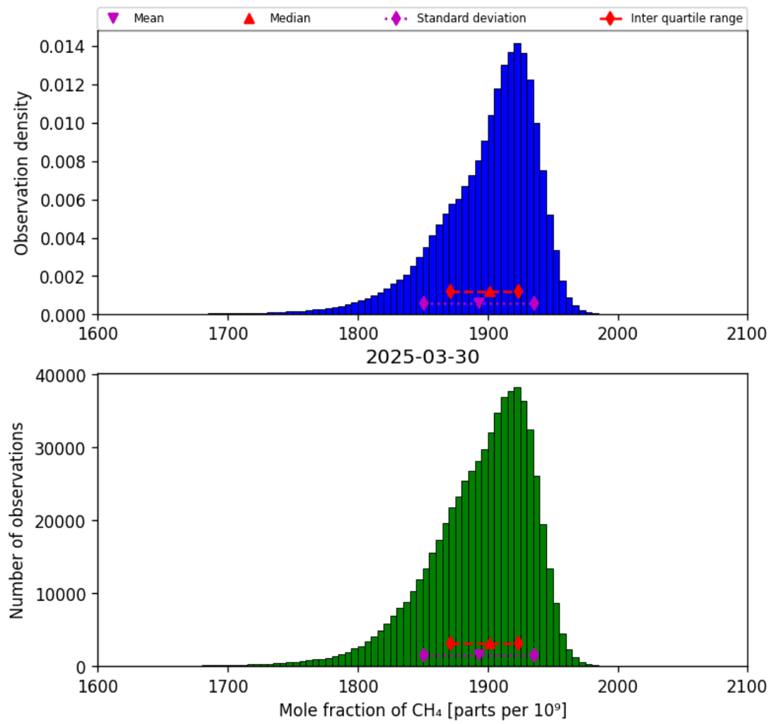
Figure 23: Histogram of “Mole fraction of CH 4 ” for 2025-03-29 to 2025-03-31
