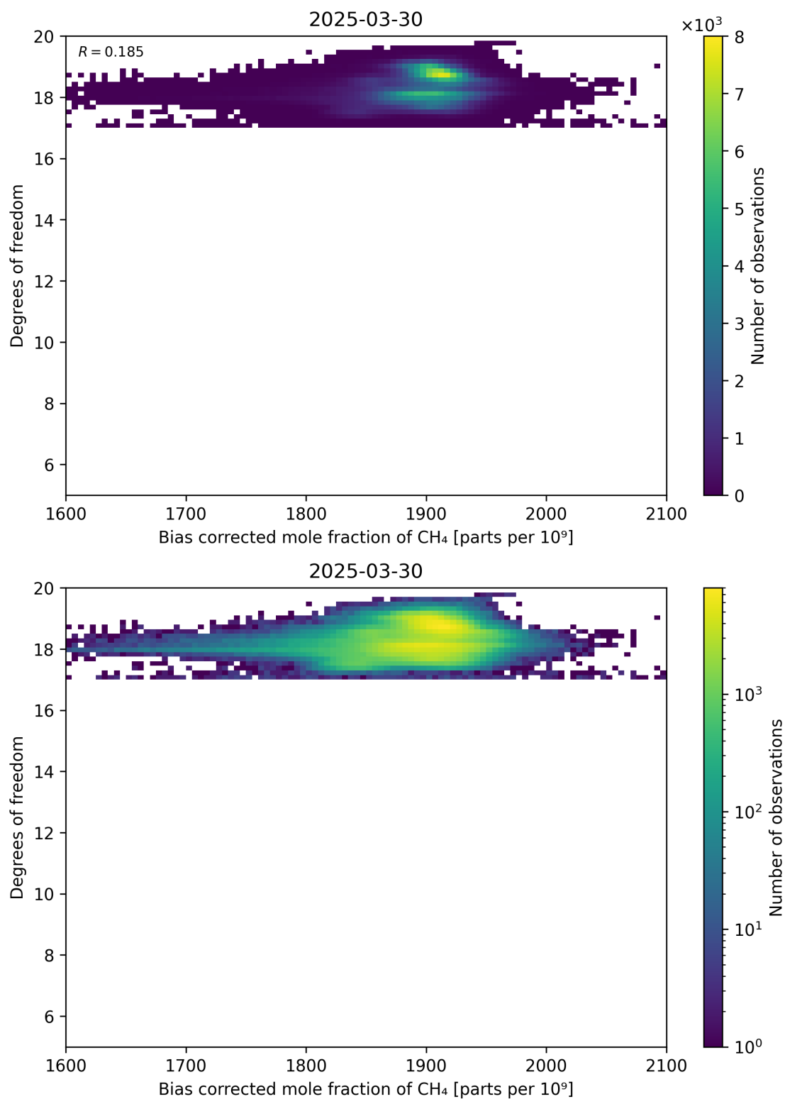
Figure 65: Scatter density plot of “Bias corrected mole fraction of CH 4 ” against “Degrees of freedom” for 2025-03-29 to 2025-03-31.
