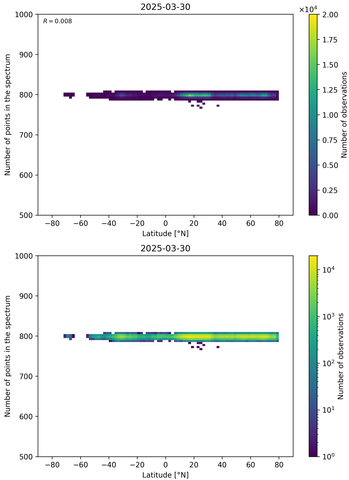
Figure 61: Scatter density plot of “Latitude” against “Number of points in the spectrum” for 2025-03-29 to 2025-03-31.
