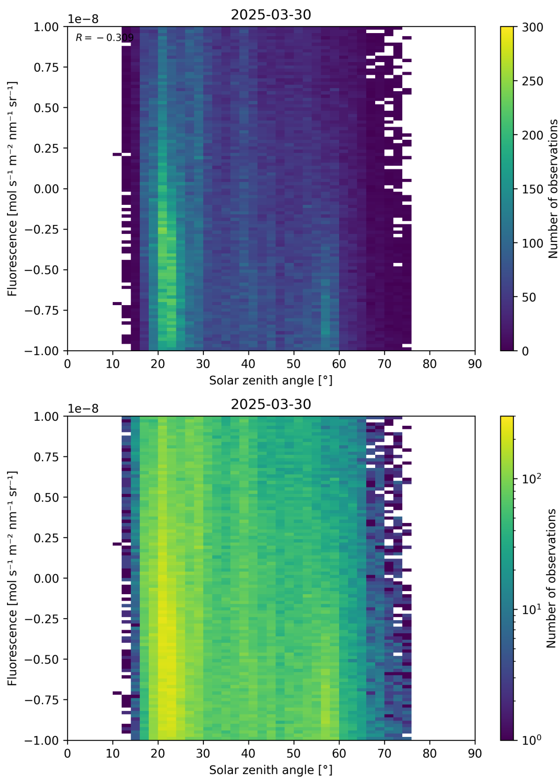
Figure 97: Scatter density plot of “Solar zenith angle” against “Fluorescence” for 2025-03-29 to 2025-03-31.
