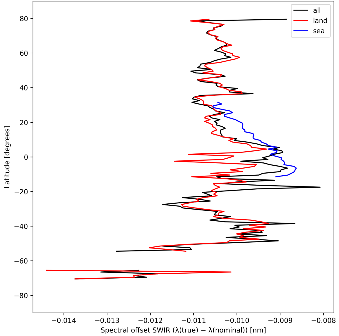
Figure 16: Zonal average of “Spectral offset SWIR ( \lambda_{\text{true}} - \lambda_{\text{nominal}} )” for 2025-03-29 to 2025-03-31.
