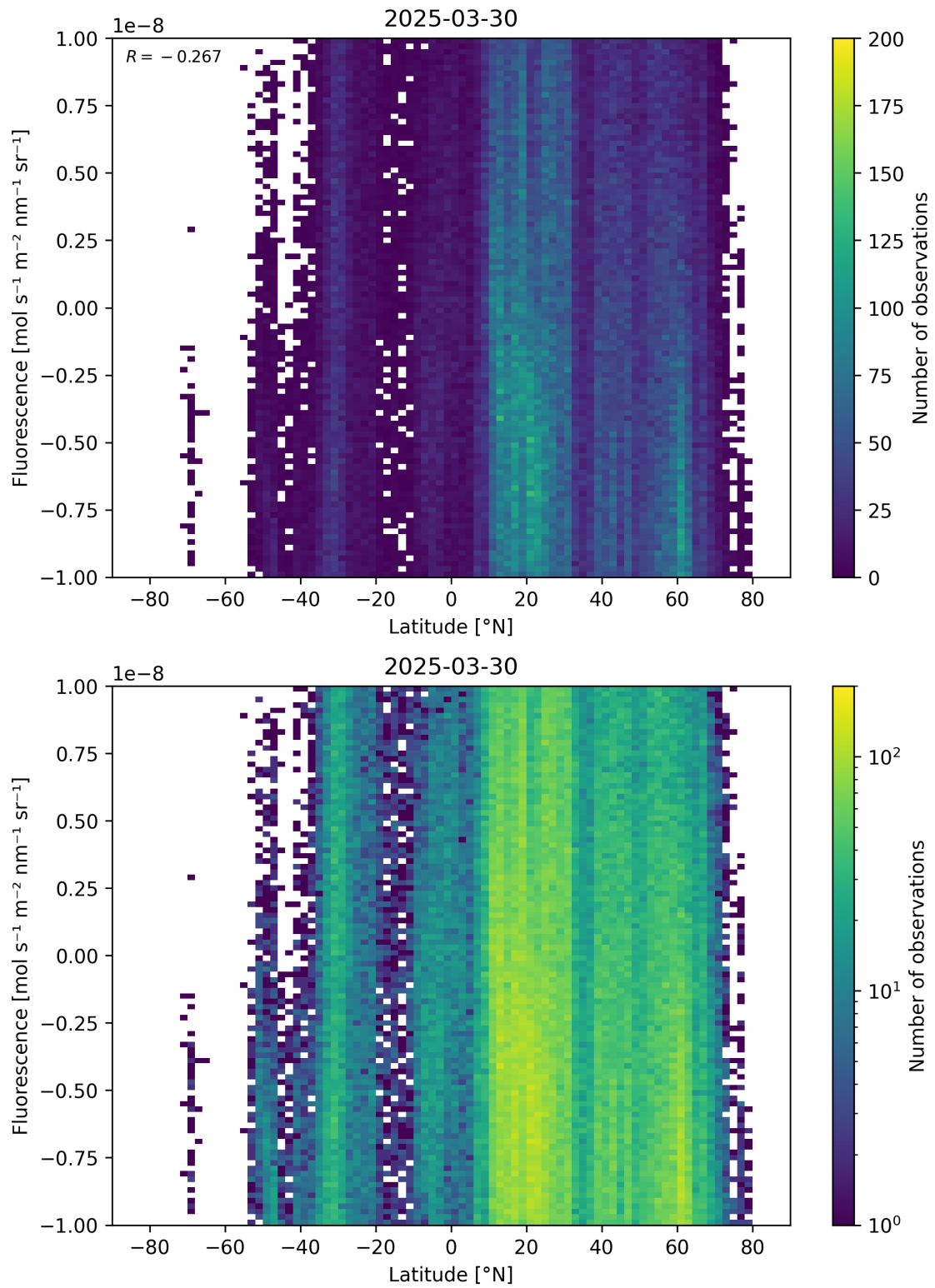
Figure 56: Scatter density plot of “Latitude” against “Fluorescence” for 2025-03-29 to 2025-03-31.
