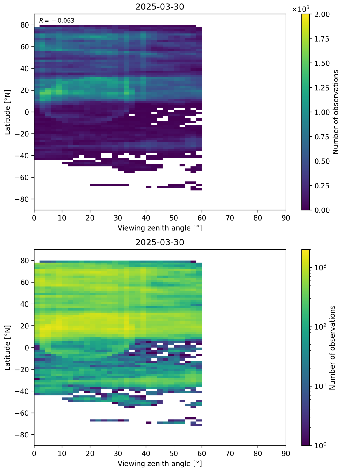
Figure 109: Scatter density plot of “Viewing zenith angle” against “Latitude” for 2025-03-29 to 2025-03-31.
