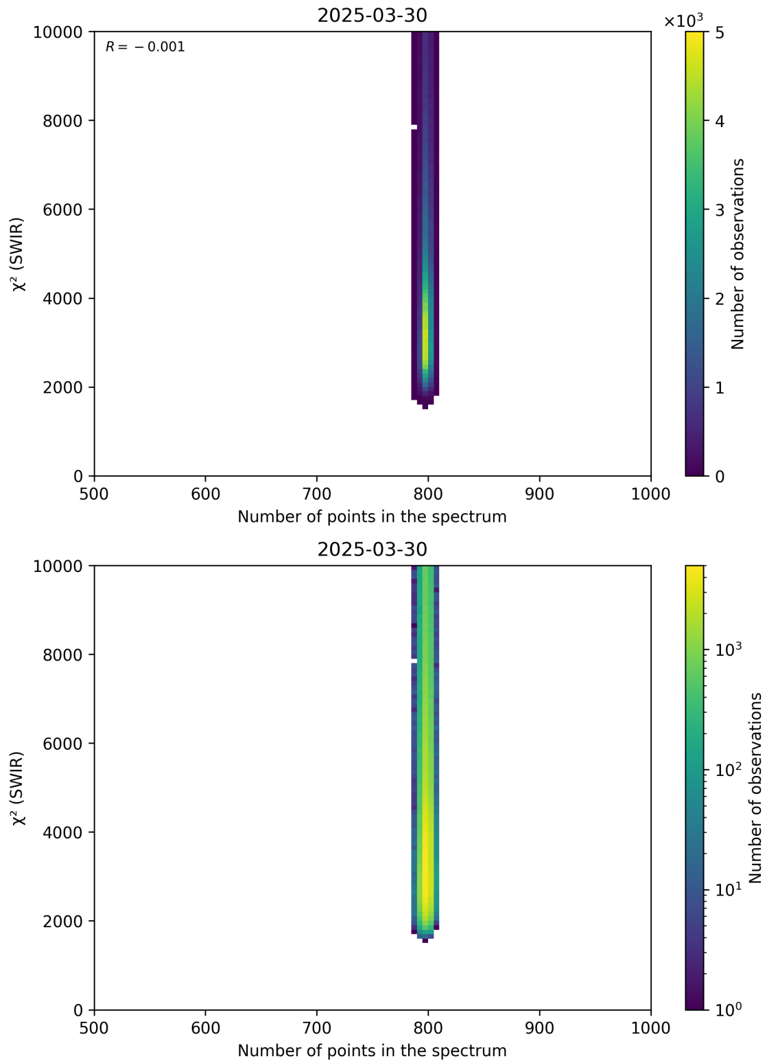
Figure 89: Scatter density plot of “Number of points in the spectrum” against “ \chi^2 (SWIR)” for 2025-03-29 to 2025-03-31.
