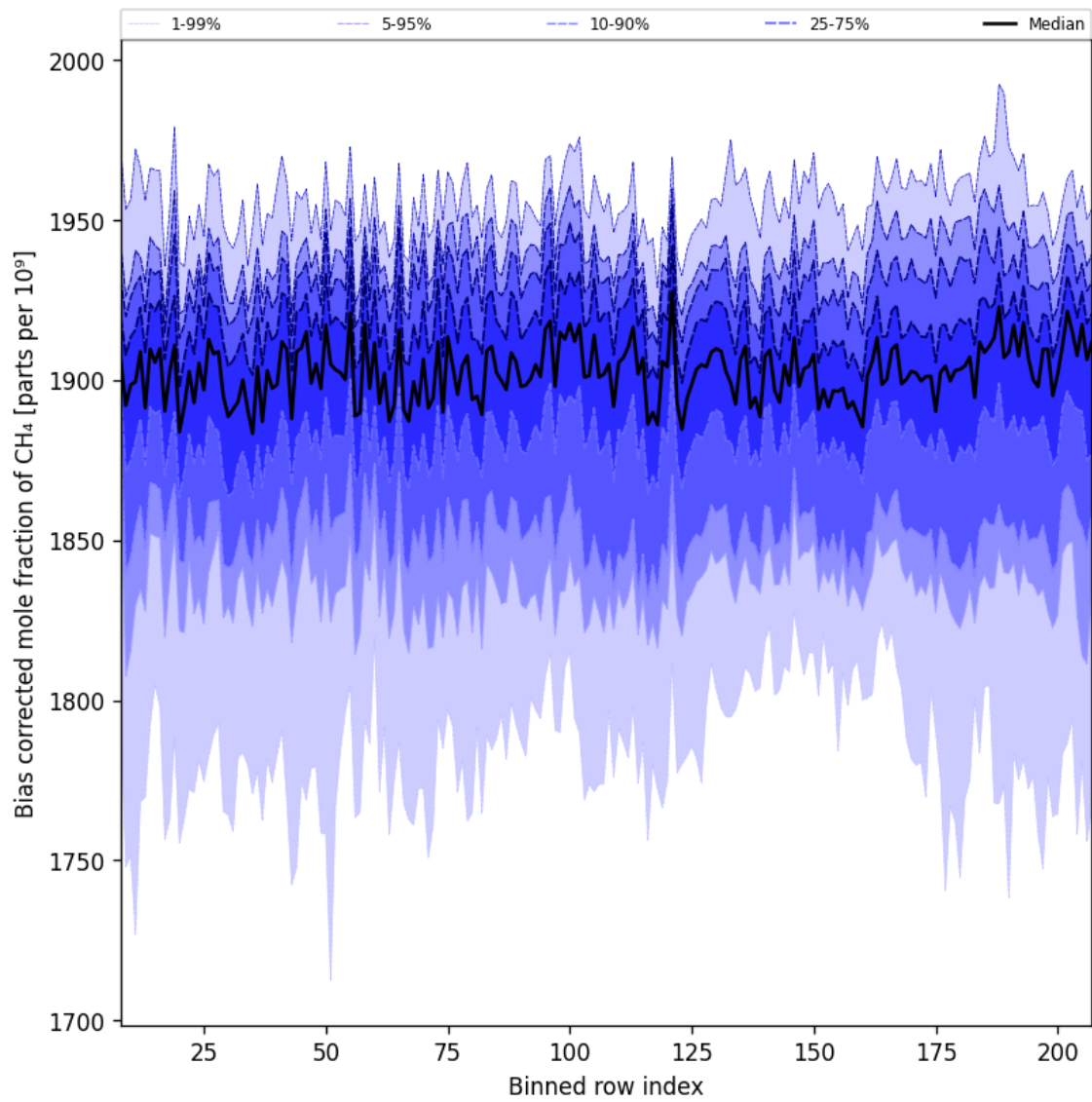
Figure 36: Along track statistics of “Bias corrected mole fraction of CH 4 ” for 2025-03-29 to 2025-03-31
