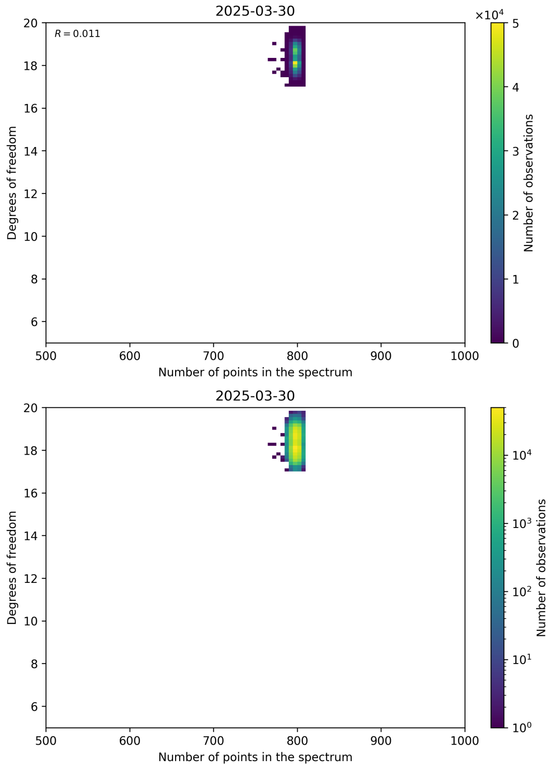
Figure 90: Scatter density plot of “Number of points in the spectrum” against “Degrees of freedom” for 2025-03-29 to 2025-03-31.
