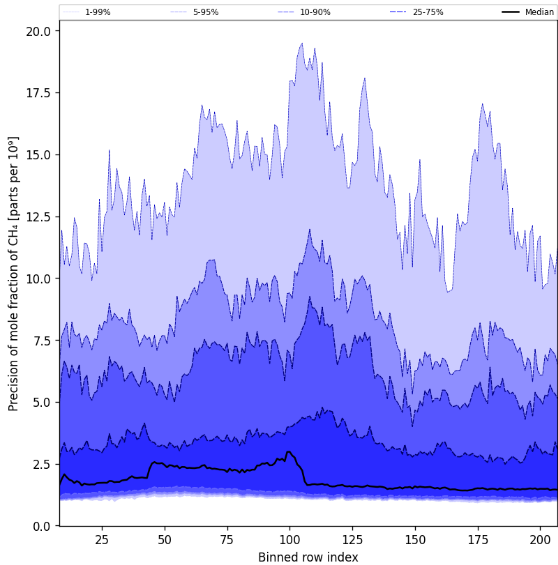
Figure 35: Along track statistics of “Precision of mole fraction of CH 4 ” for 2025-03-29 to 2025-03-31
