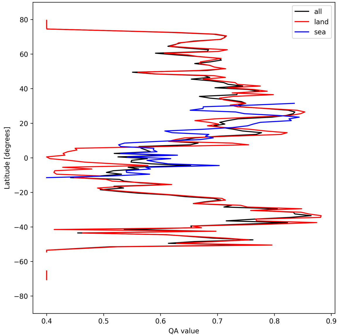
Figure 11: Zonal average of “QA value” for 2025-03-29 to 2025-03-31.
