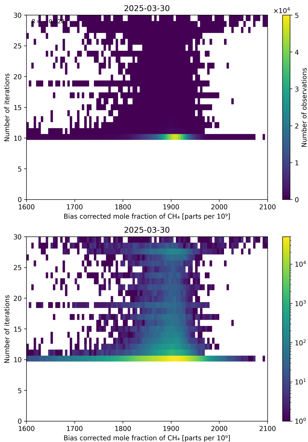
Figure 67: Scatter density plot of “Bias corrected mole fraction of \text{CH}_4 ” against “Number of iterations” for 2025-03-29 to 2025-03-31.
