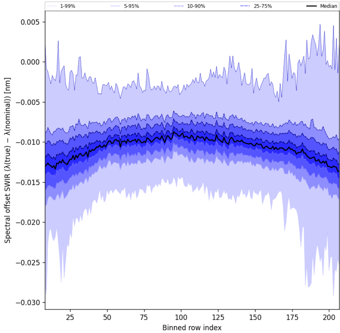
Figure 38: Along track statistics of “Spectral offset SWIR ( \lambda_{\text{true}} - \lambda_{\text{nominal}} )” for 2025-03-29 to 2025-03-31
