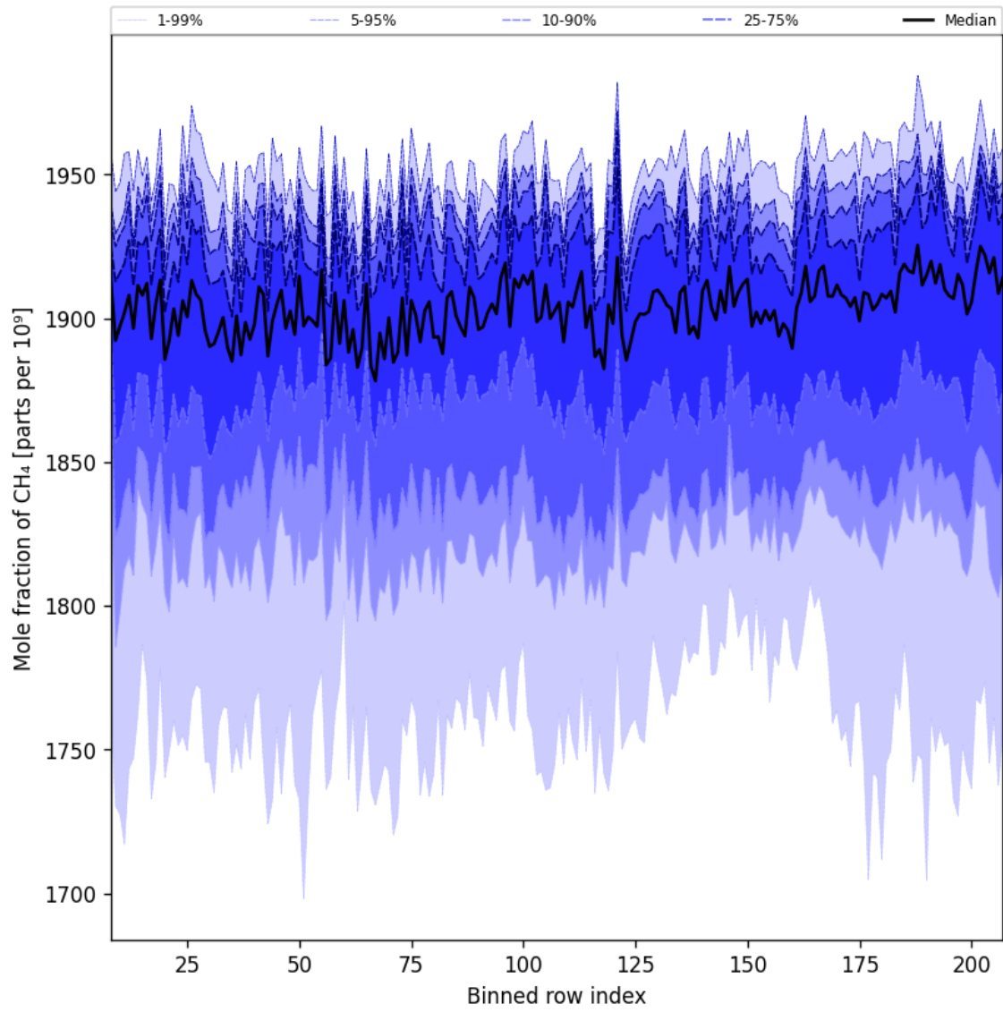
Figure 34: Along track statistics of “Mole fraction of CH 4 ” for 2025-03-29 to 2025-03-31
