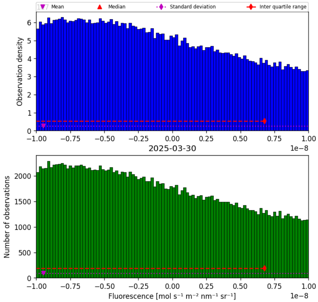
Figure 32: Histogram of “Fluorescence” for 2025-03-29 to 2025-03-31
