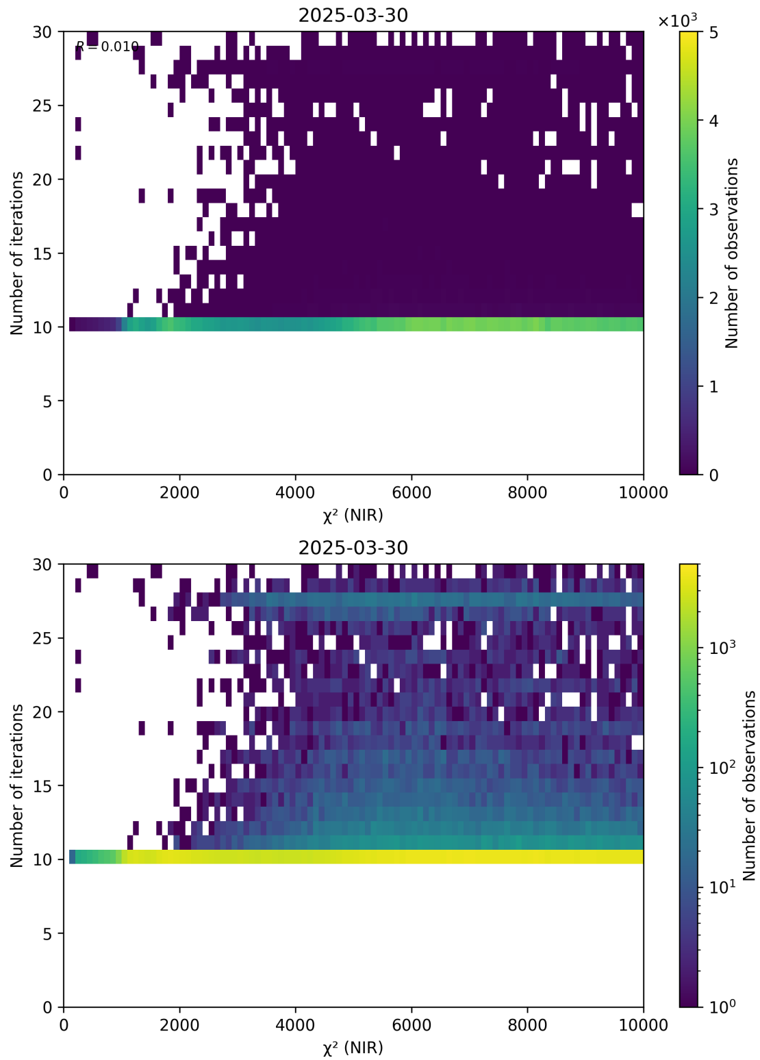
Figure 46: Scatter density plot of “ \chi^2 (NIR)” against “Number of iterations” for 2025-03-29 to 2025-03-31.
