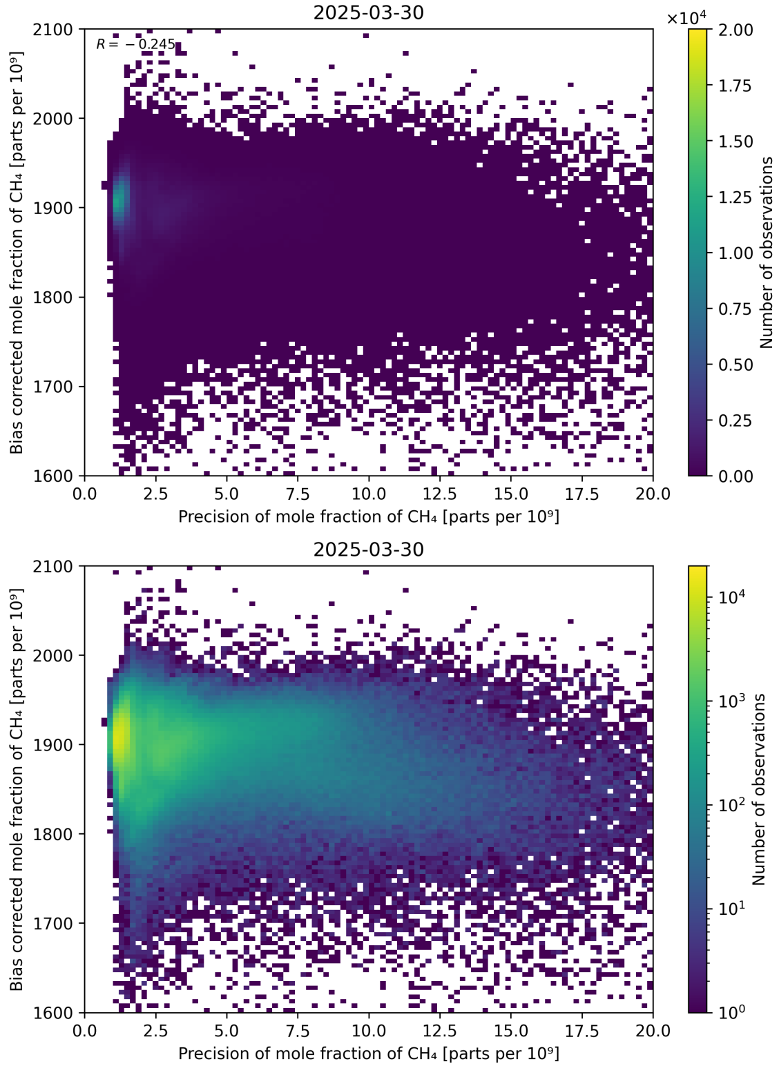
Figure 82: Scatter density plot of “Precision of mole fraction of CH 4 ” against “Bias corrected mole fraction of CH 4 ” for 2025-03-29 to 2025-03-31.
