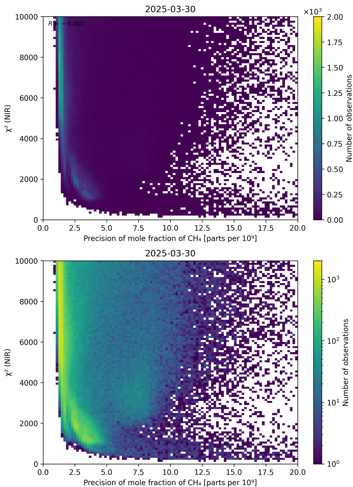
Figure 78: Scatter density plot of “Precision of mole fraction of CH 4 ” against “ \chi^2 (NIR)” for 2025-03-29 to 2025-03-31.
