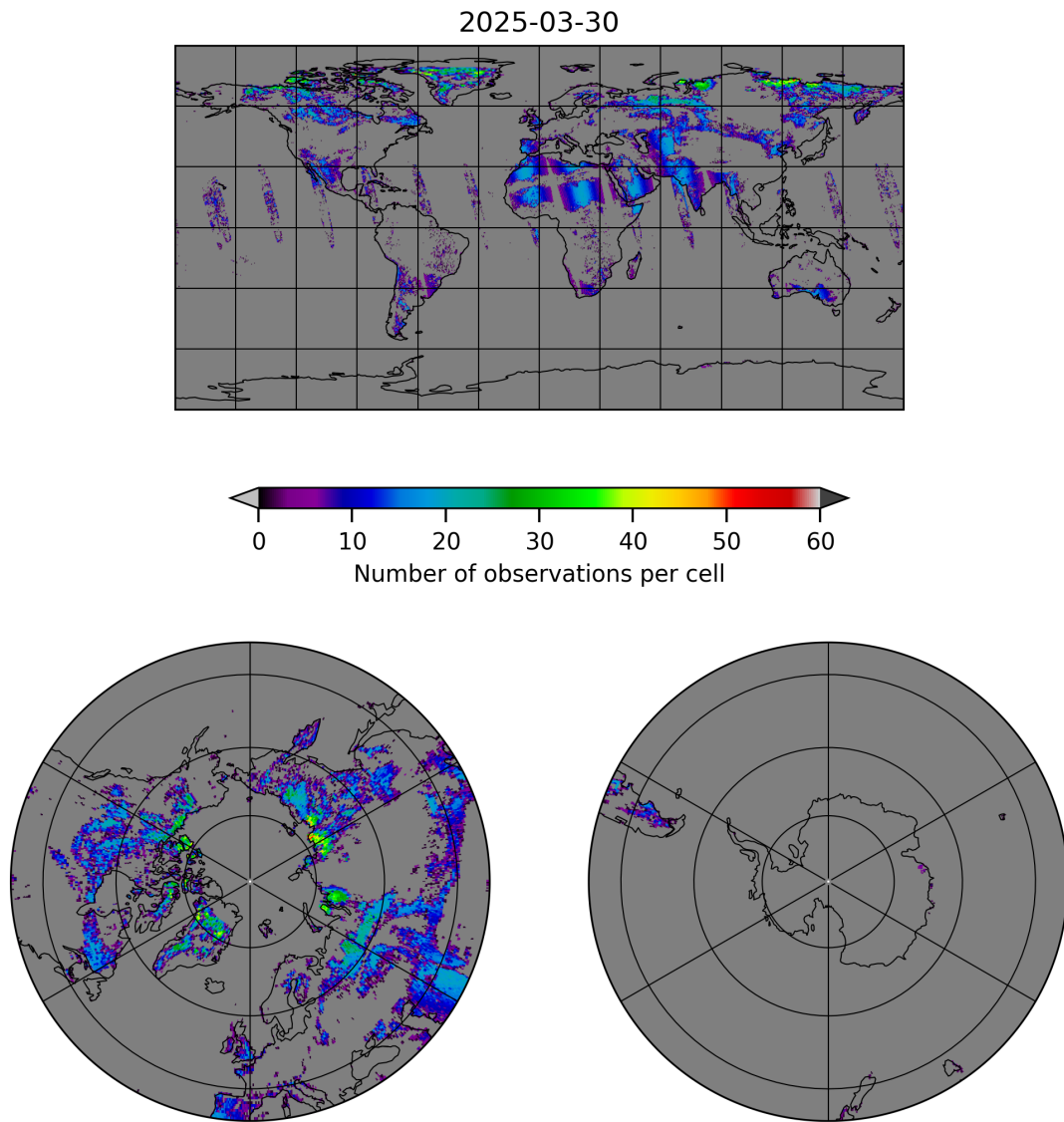
Figure 10: Map of the number of observations for 2025-03-29 to 2025-03-31
