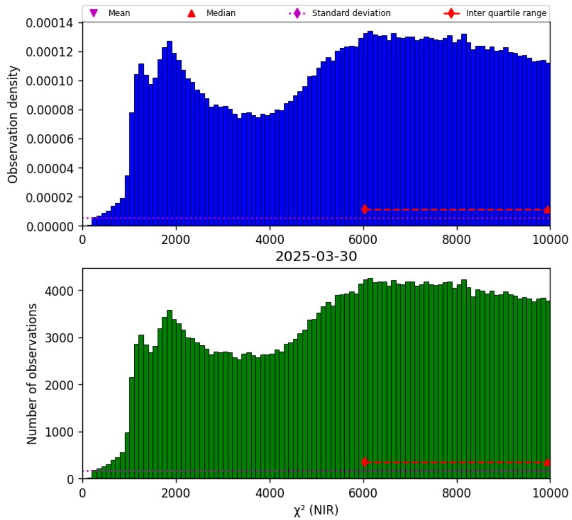
Figure 29: Histogram of “ \chi^2 (NIR)” for 2025-03-29 to 2025-03-31
