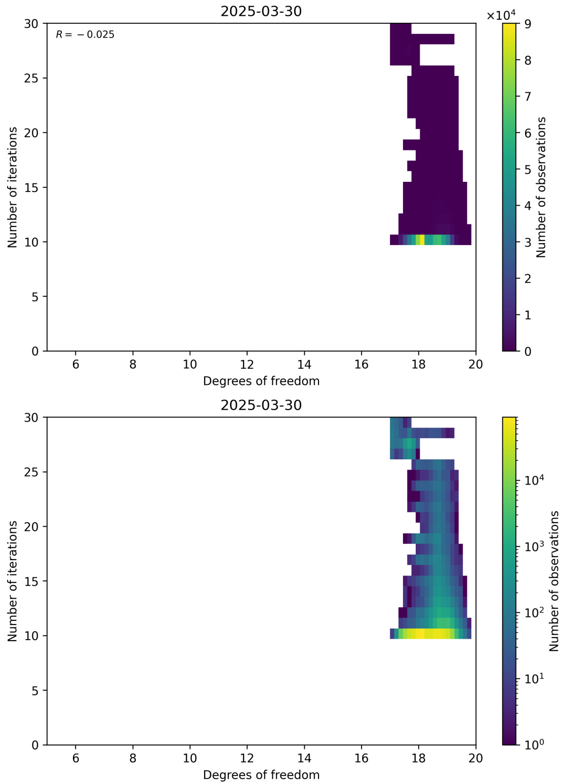
Figure 52: Scatter density plot of “Degrees of freedom” against “Number of iterations” for 2025-03-29 to 2025-03-31.
