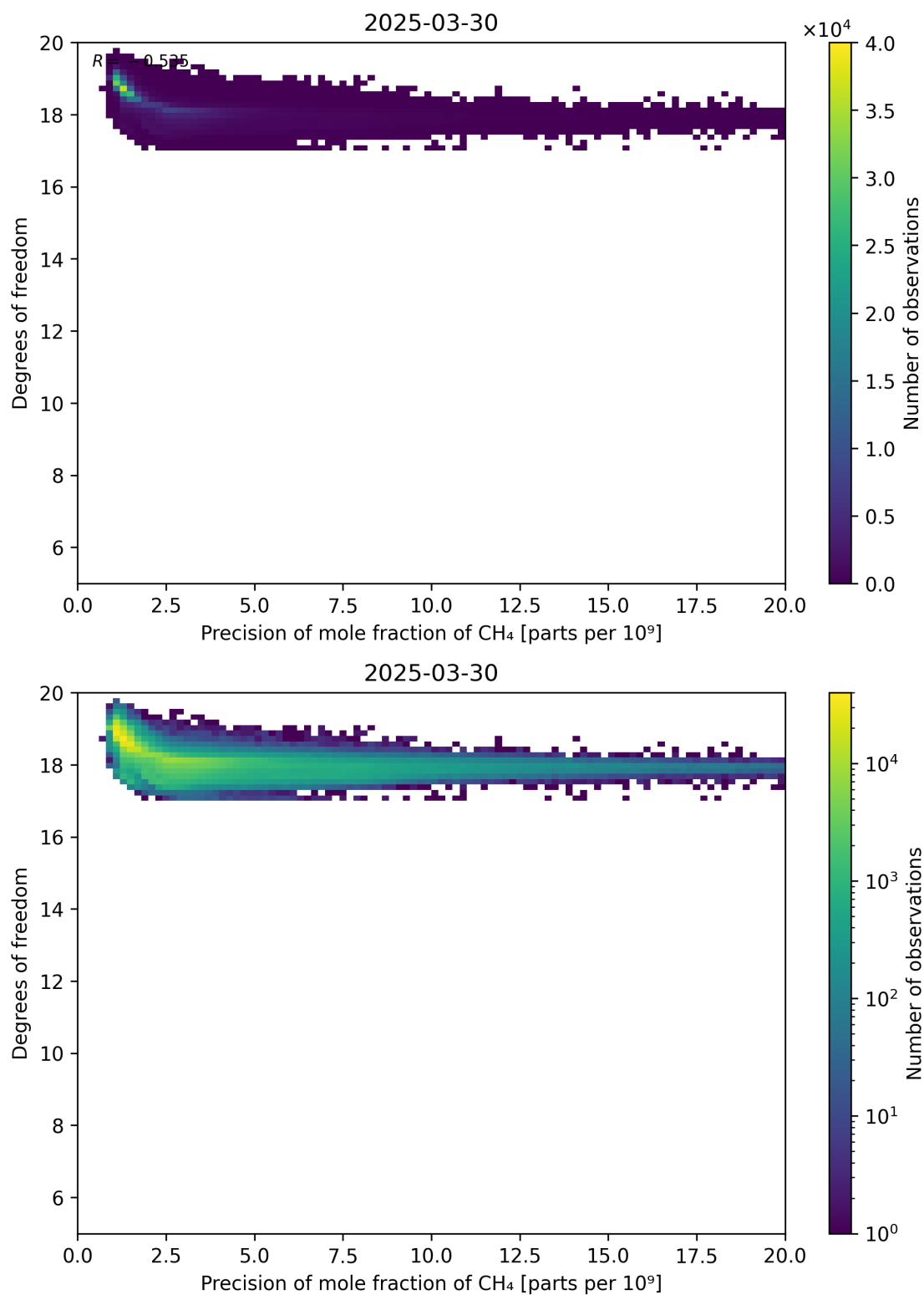
Figure 80: Scatter density plot of “Precision of mole fraction of CH 4 ” against “Degrees of freedom” for 2025-03-29 to 2025-03-31.
