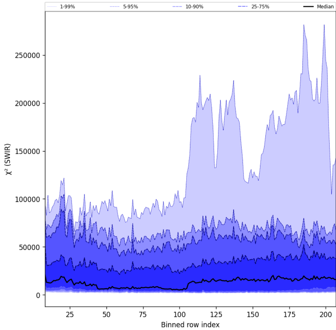
Figure 39: Along track statistics of “ \chi^2 (SWIR)” for 2025-03-29 to 2025-03-31
