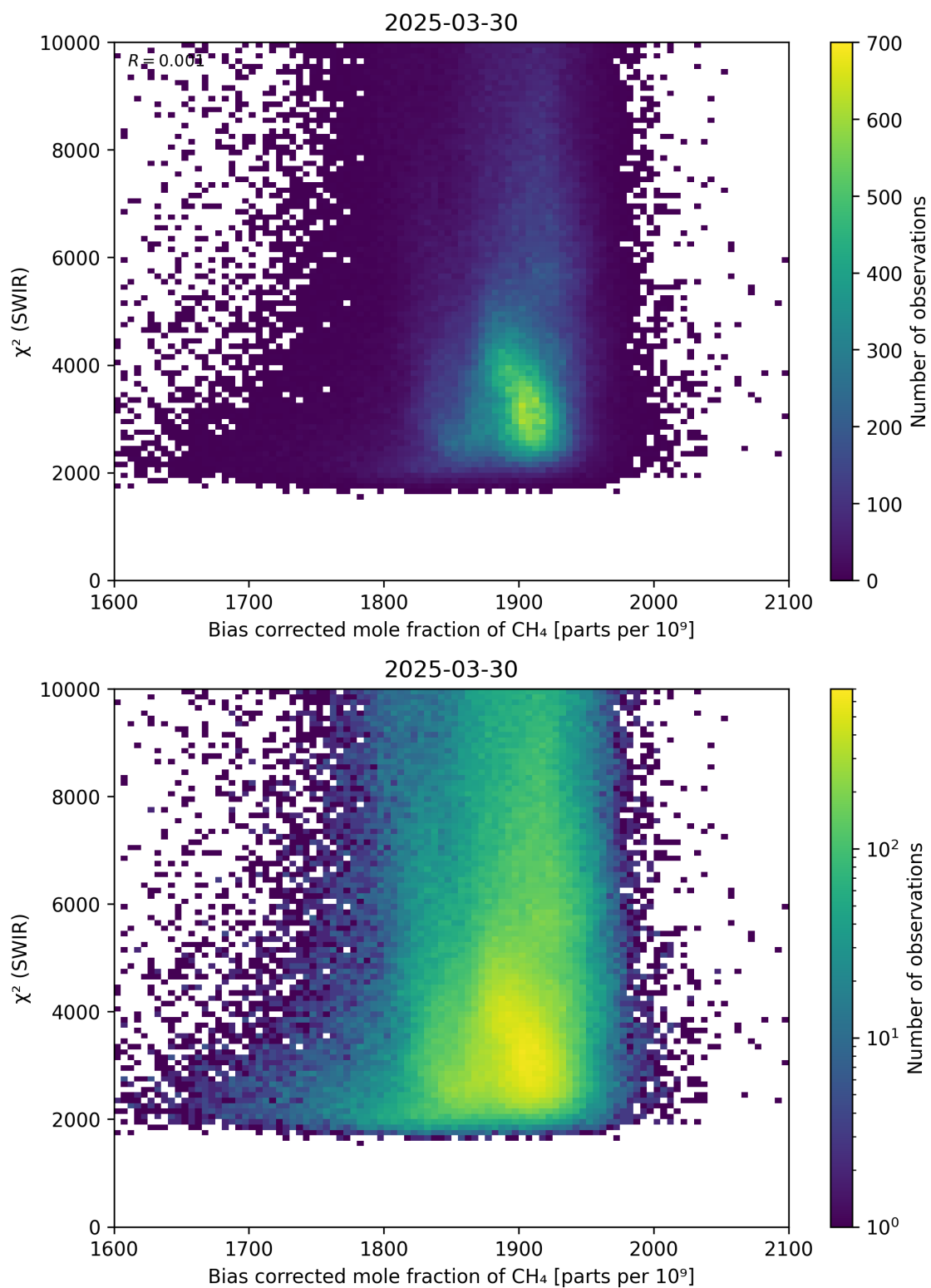
Figure 64: Scatter density plot of “Bias corrected mole fraction of \text{CH}_4 ” against “ \chi^2 (SWIR)” for 2025-03-29 to 2025-03-31.
