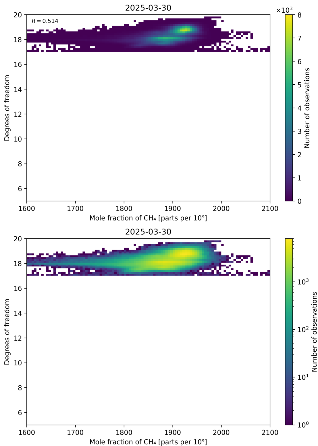
Figure 72: Scatter density plot of “Mole fraction of CH 4 ” against “Degrees of freedom” for 2025-03-29 to 2025-03-31.
