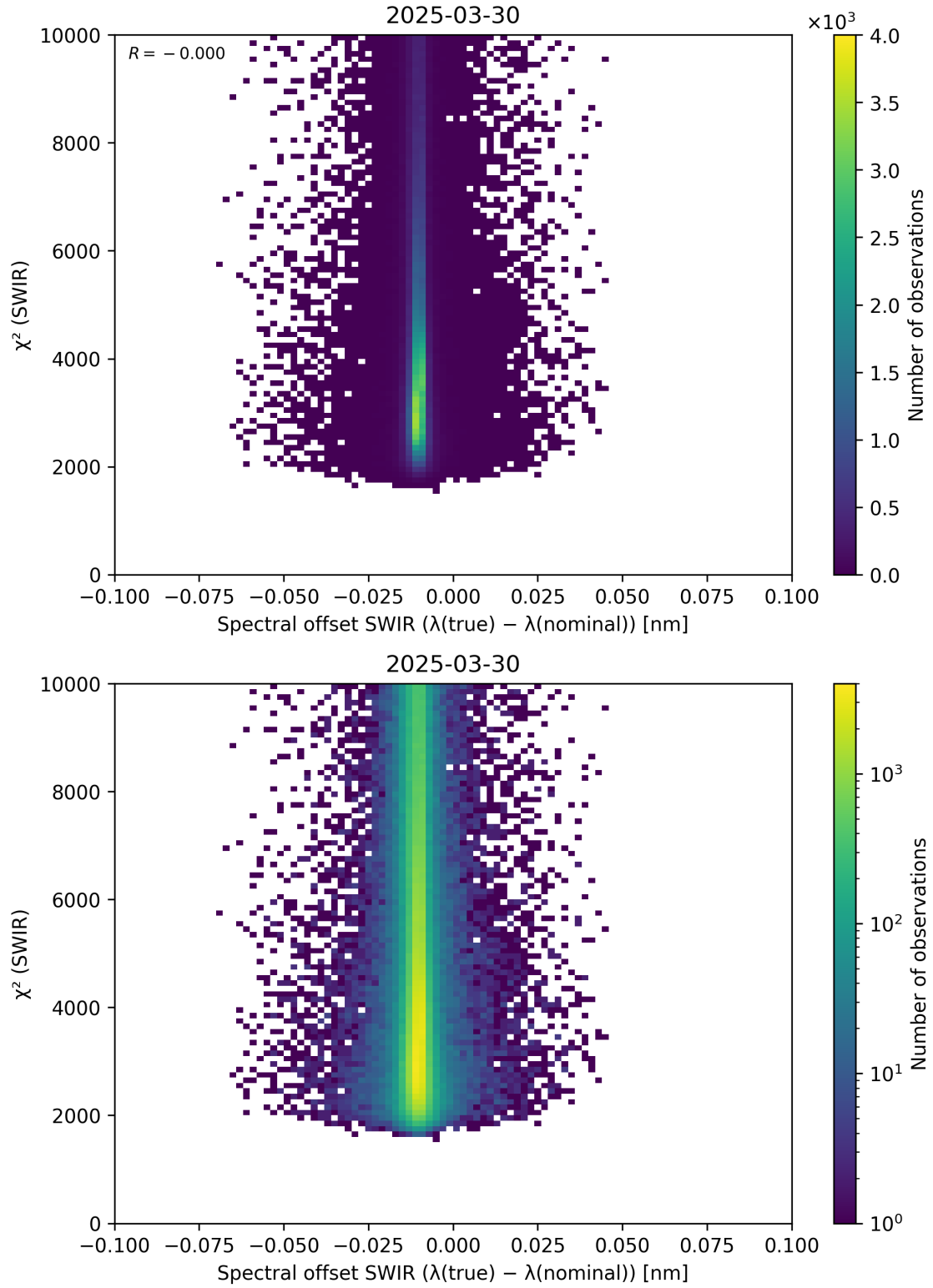
Figure 118: Scatter density plot of “Spectral offset SWIR ( \lambda_{\text{true}} - \lambda_{\text{nominal}} )” against “ \chi^2 (SWIR)” for 2025-03-29 to 2025-03-31.
