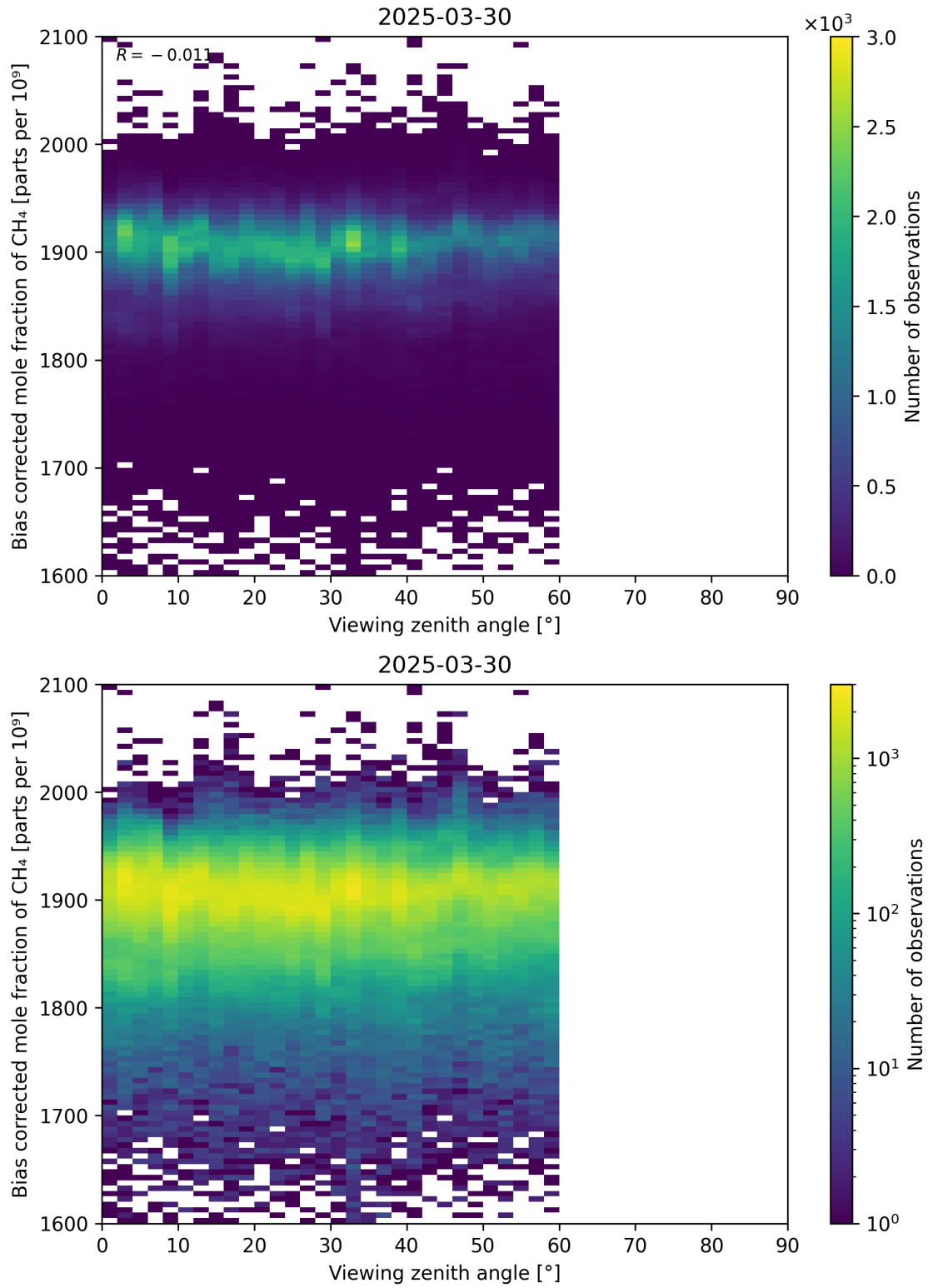
Figure 111: Scatter density plot of “Viewing zenith angle” against “Bias corrected mole fraction of CH 4 ” for 2025-03-29 to 2025-03-31.
