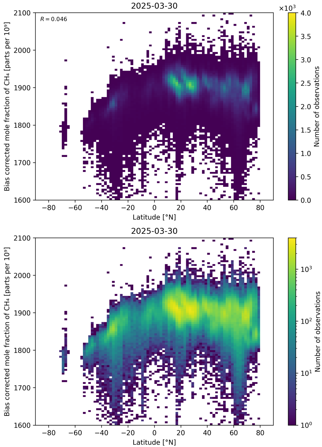
Figure 58: Scatter density plot of “Latitude” against “Bias corrected mole fraction of CH 4 ” for 2025-03-29 to 2025-03-31.
