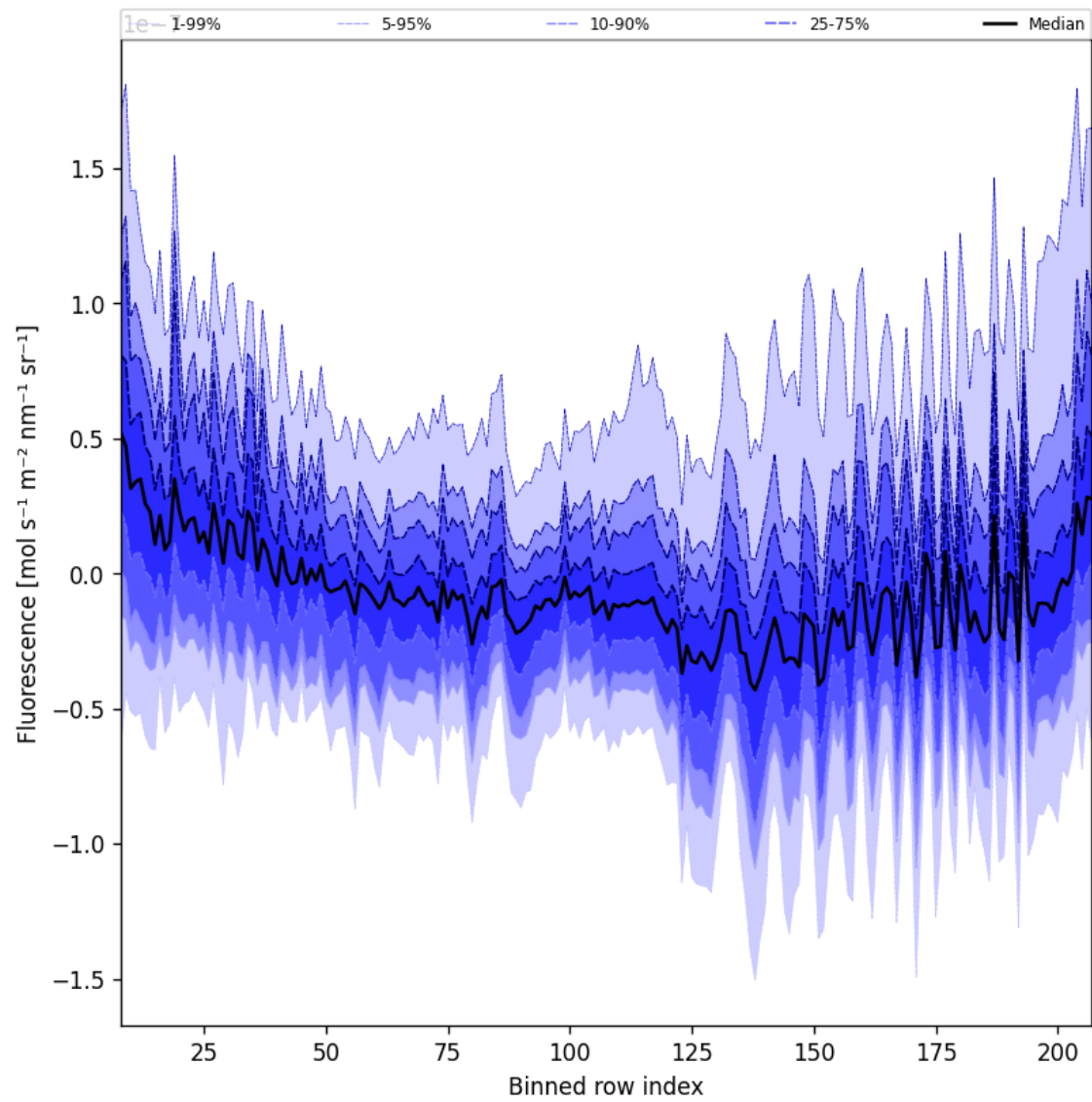
Figure 43: Along track statistics of “Fluorescence” for 2025-03-29 to 2025-03-31
