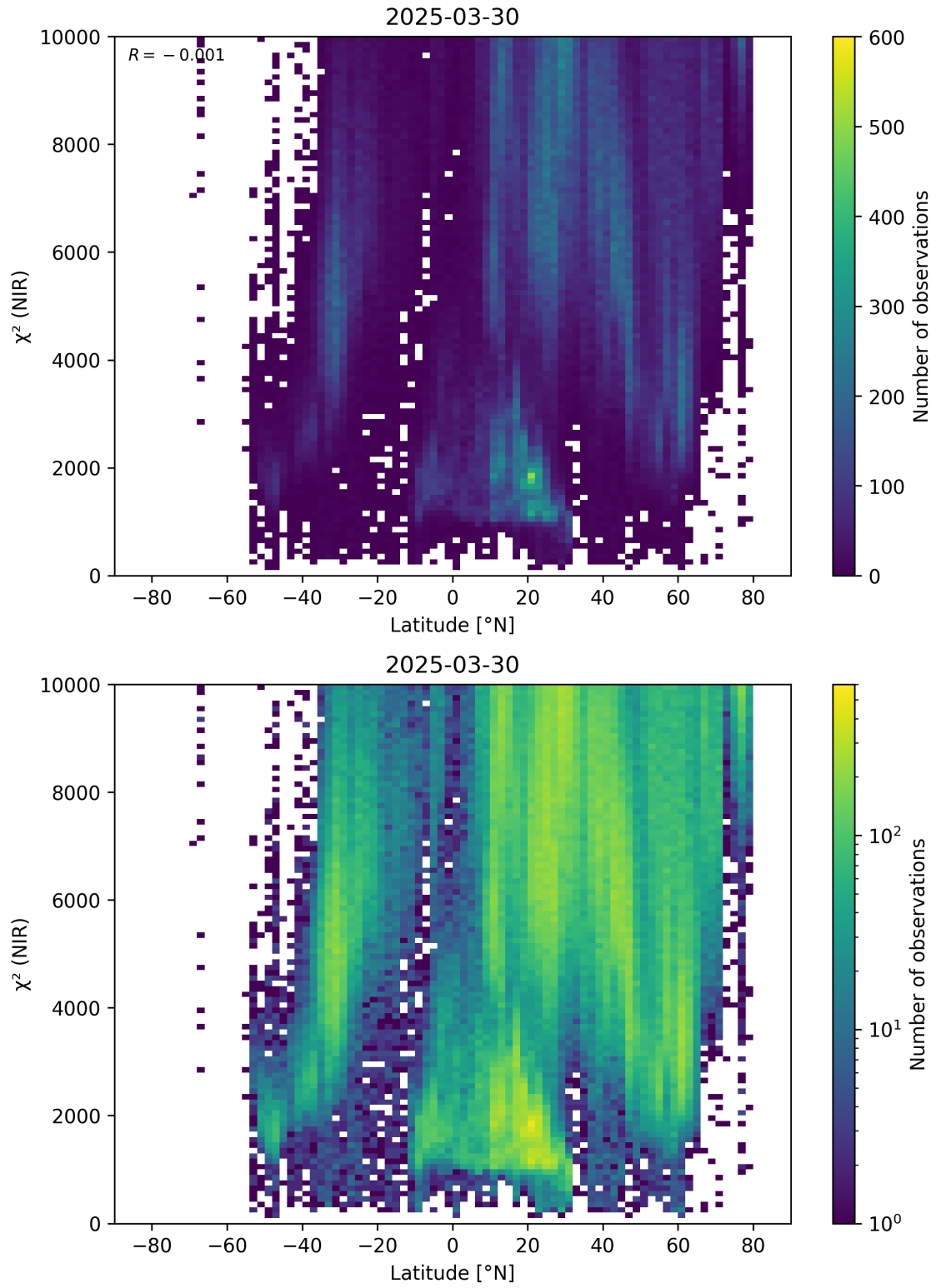
Figure 53: Scatter density plot of “Latitude” against “ \chi^2 (NIR)” for 2025-03-29 to 2025-03-31.
