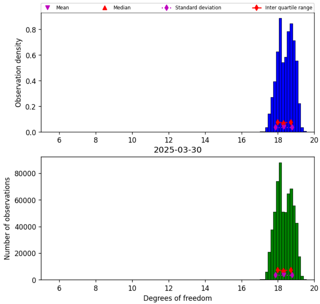
Figure 30: Histogram of “Degrees of freedom” for 2025-03-29 to 2025-03-31
