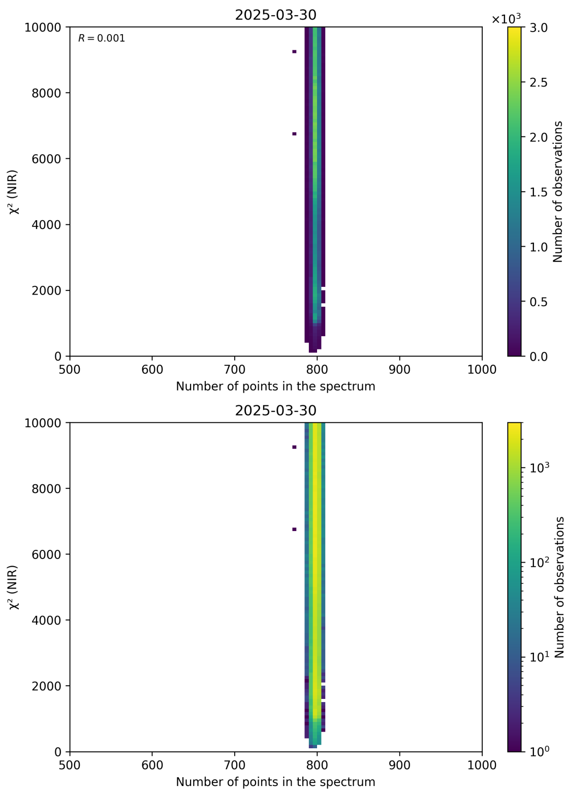
Figure 88: Scatter density plot of “Number of points in the spectrum” against “ \chi^2 (NIR)” for 2025-03-29 to 2025-03-31.
