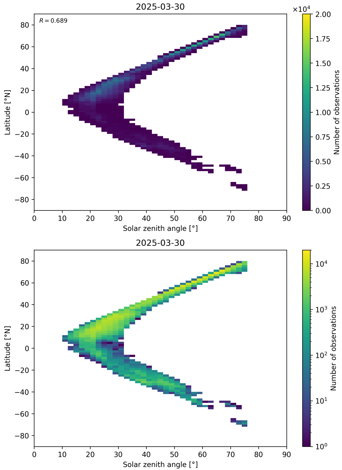
Figure 98: Scatter density plot of “Solar zenith angle” against “Latitude” for 2025-03-29 to 2025-03-31.
