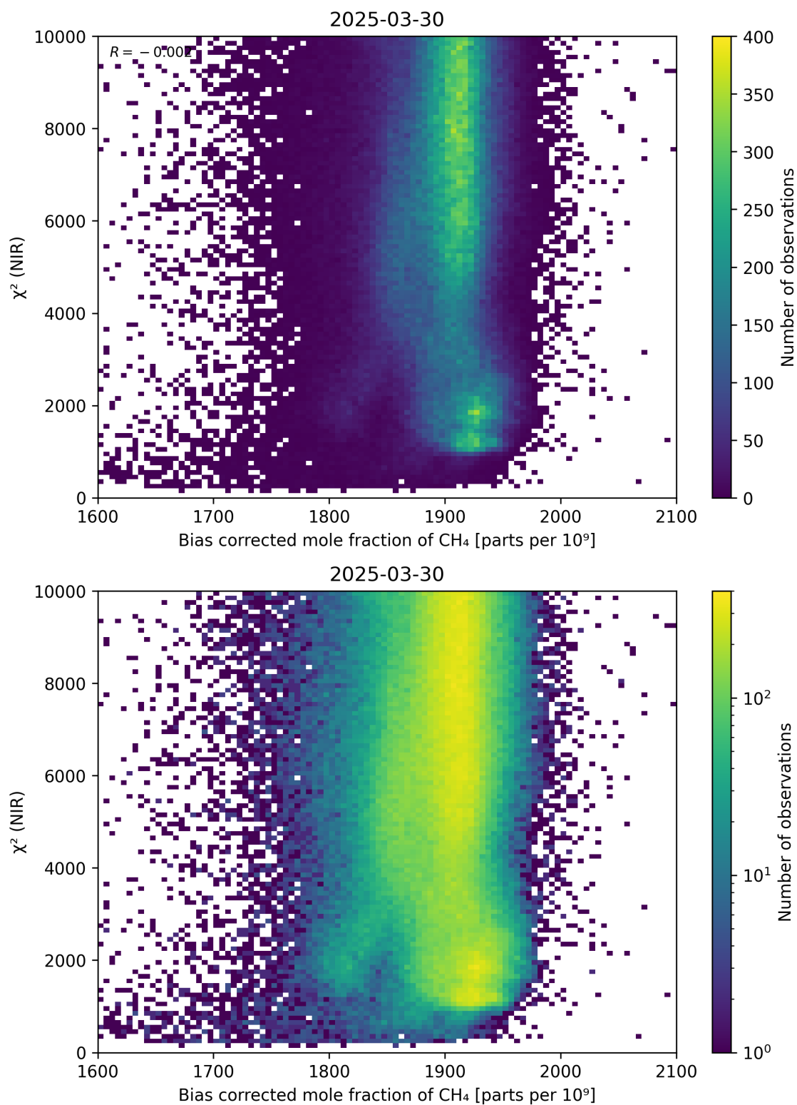
Figure 63: Scatter density plot of “Bias corrected mole fraction of \text{CH}_4 ” against “ \chi^2 (NIR)” for 2025-03-29 to 2025-03-31.
