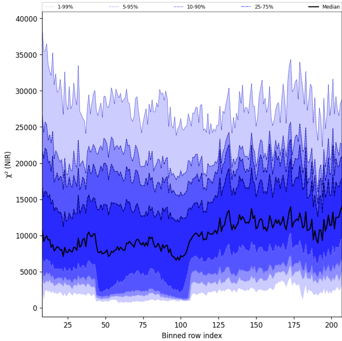
Figure 40: Along track statistics of “ \chi^2 (NIR)” for 2025-03-29 to 2025-03-31
