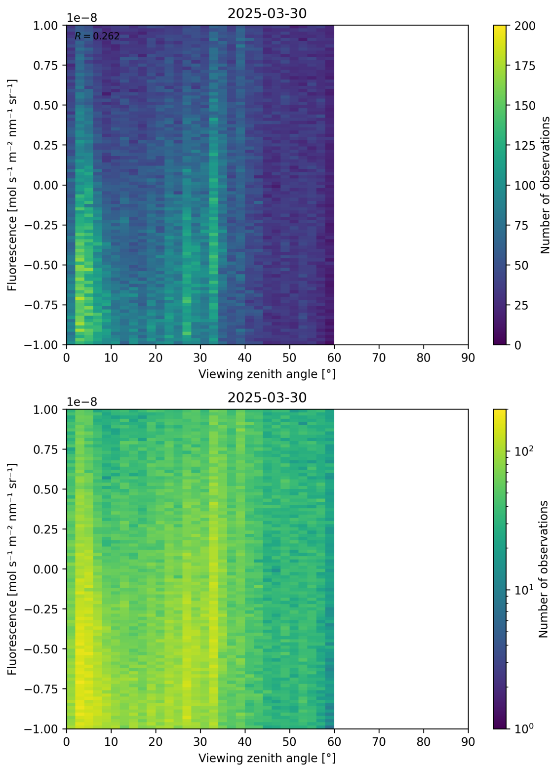
Figure 108: Scatter density plot of “Viewing zenith angle” against “Fluorescence” for 2025-03-29 to 2025-03-31.
