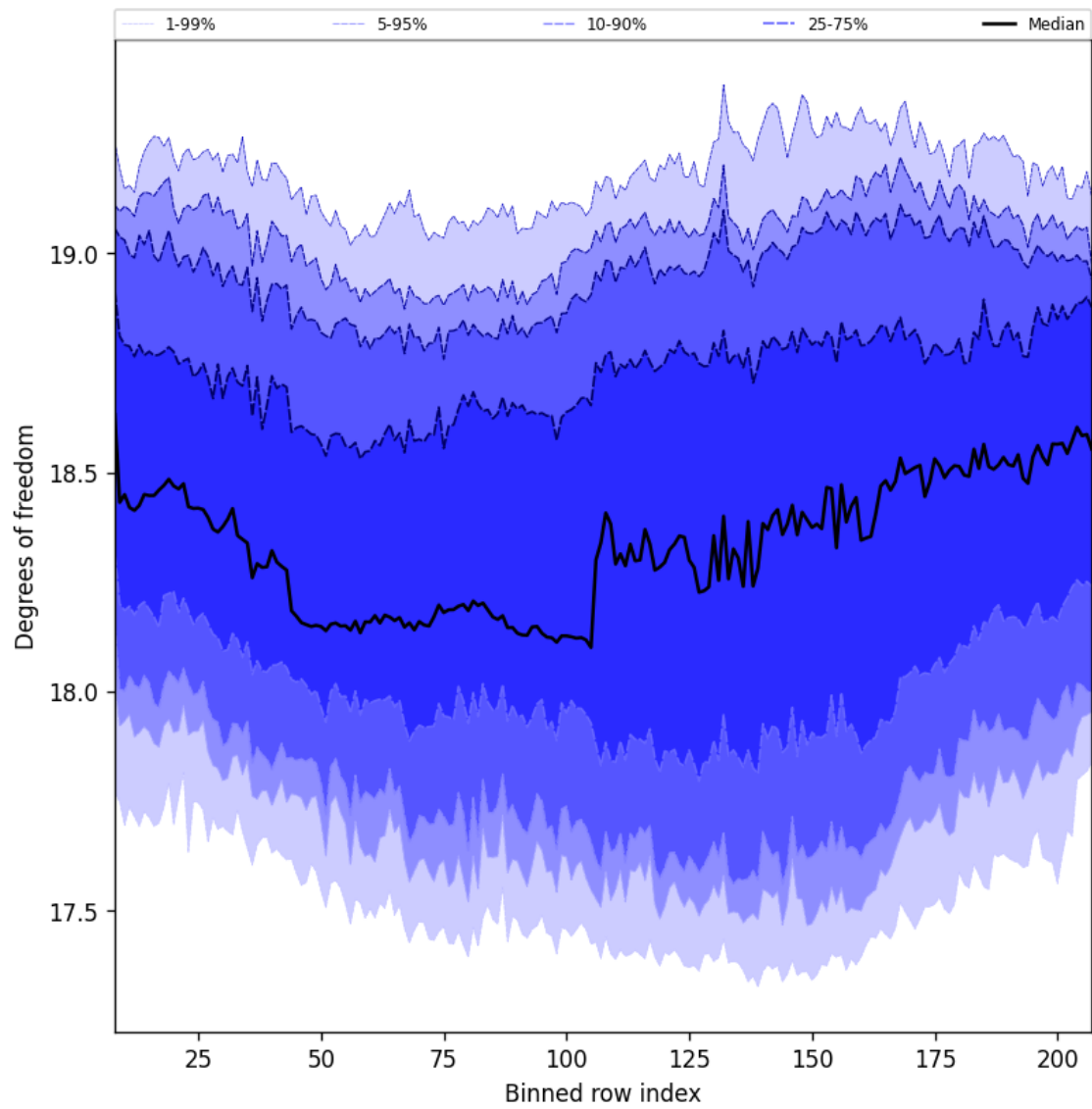
Figure 41: Along track statistics of “Degrees of freedom” for 2025-03-29 to 2025-03-31
