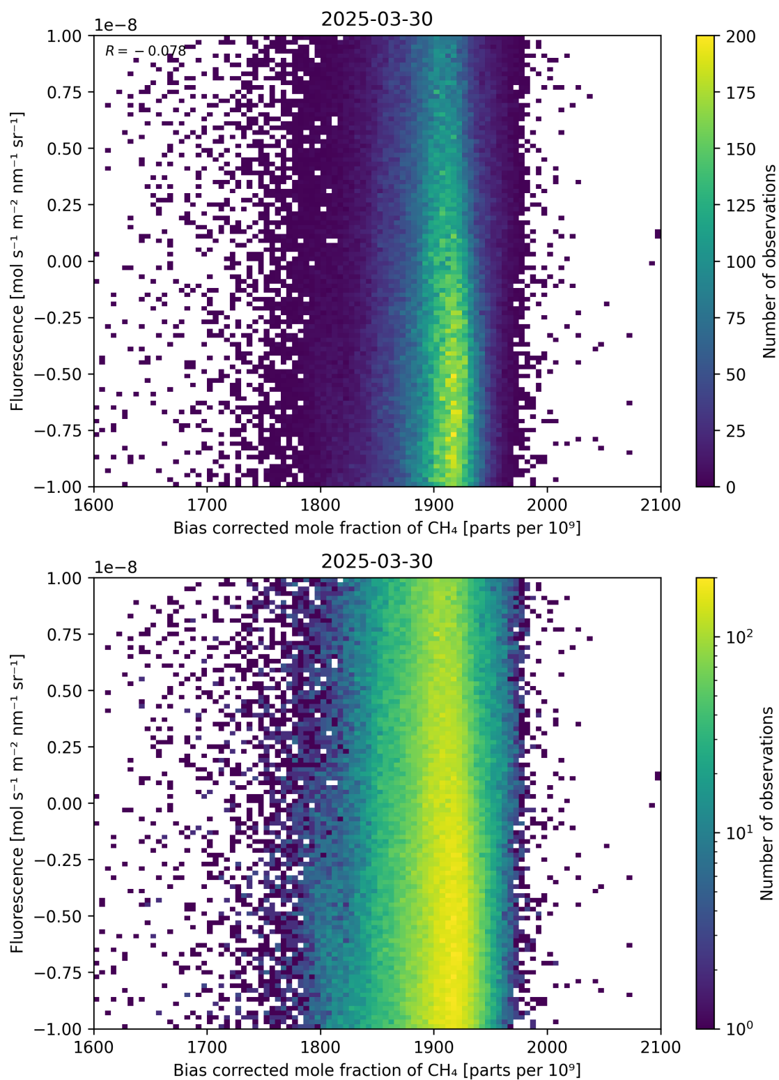
Figure 66: Scatter density plot of “Bias corrected mole fraction of \text{CH}_4 ” against “Fluorescence” for 2025-03-29 to 2025-03-31.
