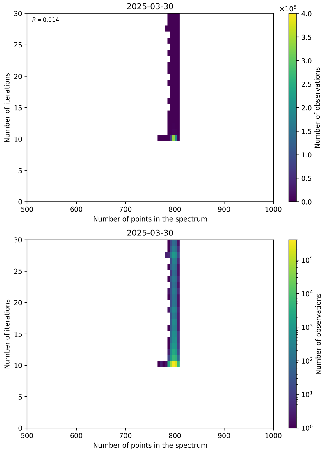
Figure 92: Scatter density plot of “Number of points in the spectrum” against “Number of iterations” for 2025-03-29 to 2025-03-31.
