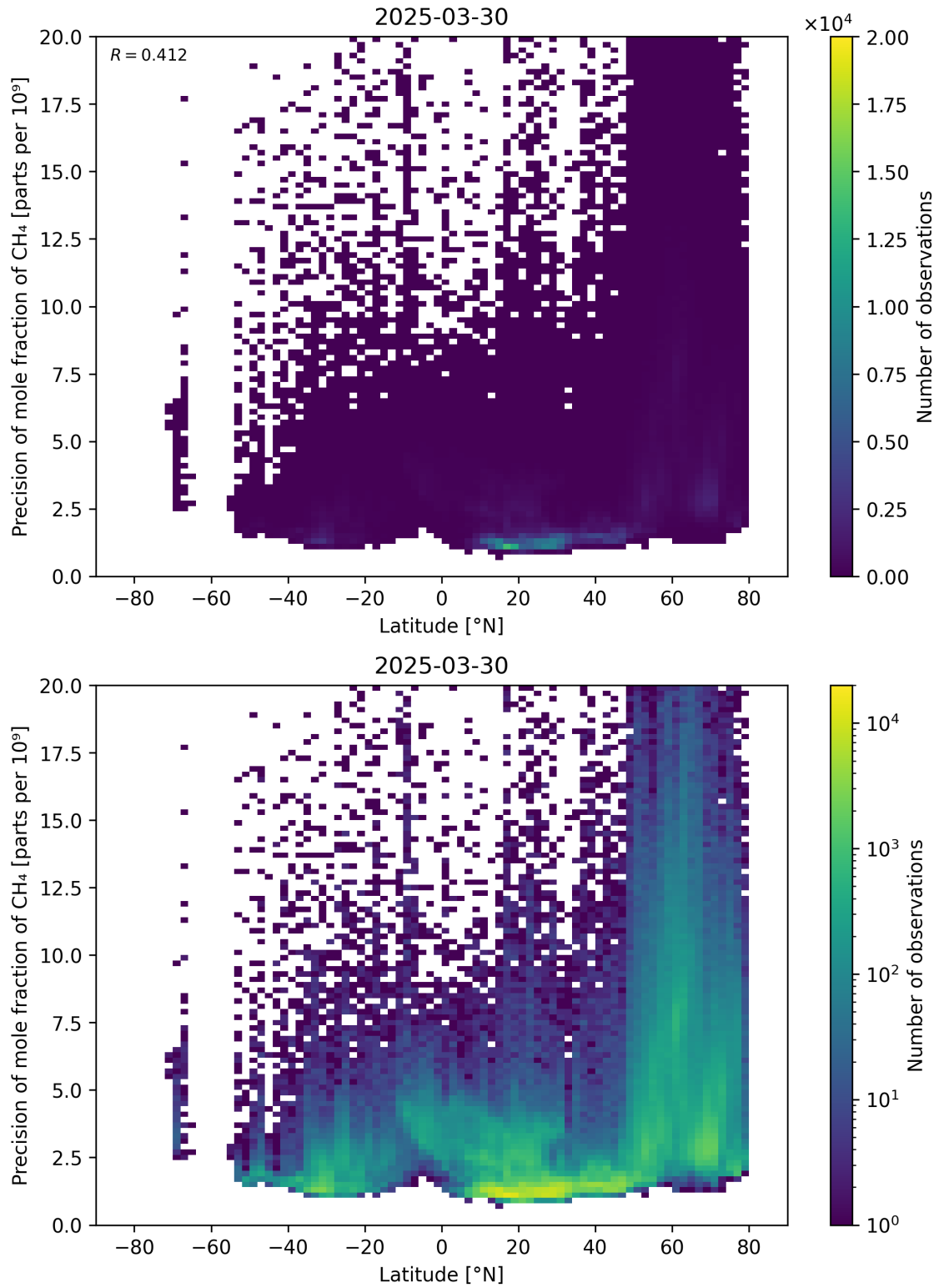
Figure 59: Scatter density plot of “Latitude” against “Precision of mole fraction of \text{CH}_4 ” for 2025-03-29 to 2025-03-31.
