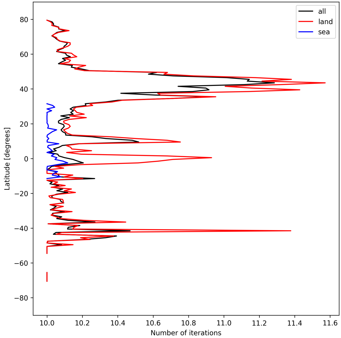
Figure 20: Zonal average of “Number of iterations” for 2025-03-29 to 2025-03-31.
