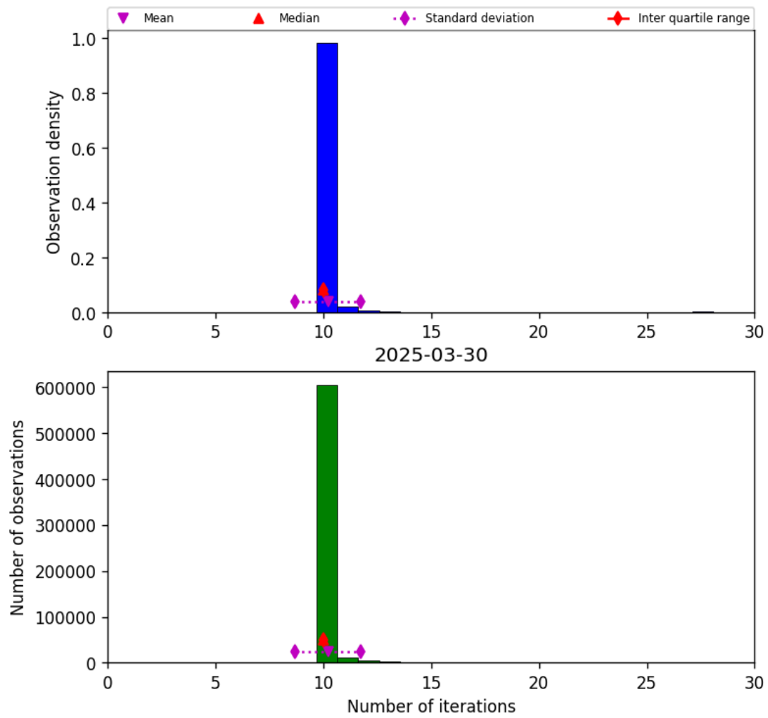
Figure 31: Histogram of “Number of iterations” for 2025-03-29 to 2025-03-31
