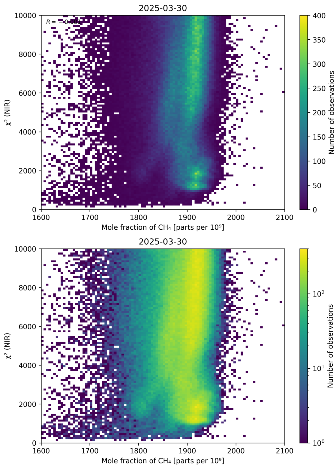
Figure 70: Scatter density plot of “Mole fraction of \text{CH}_4 ” against “ \chi^2 (NIR)” for 2025-03-29 to 2025-03-31.
