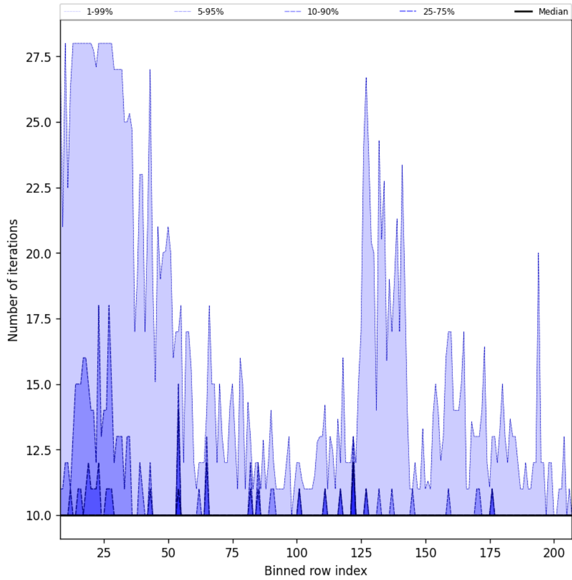
Figure 42: Along track statistics of “Number of iterations” for 2025-03-29 to 2025-03-31
