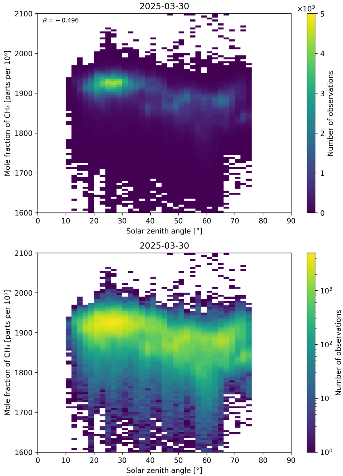
Figure 99: Scatter density plot of “Solar zenith angle” against “Mole fraction of CH 4 ” for 2025-03-29 to 2025-03-31.
