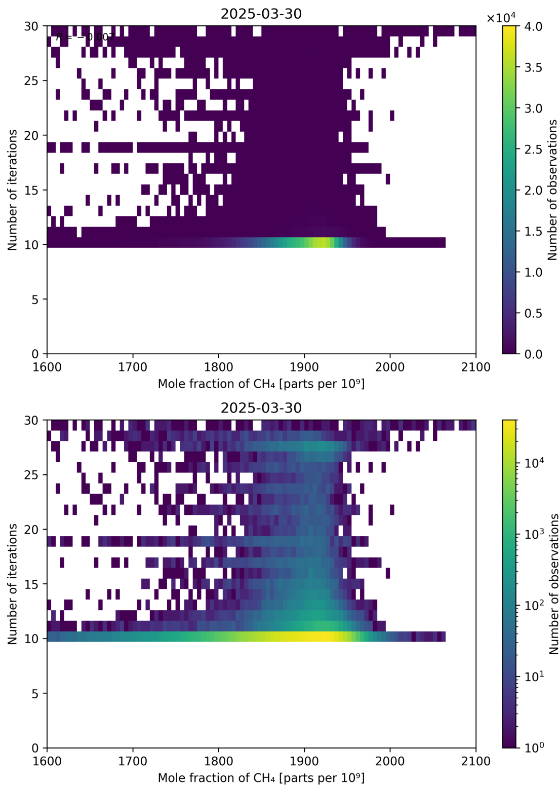
Figure 76: Scatter density plot of “Mole fraction of CH 4 ” against “Number of iterations” for 2025-03-29 to 2025-03-31.
