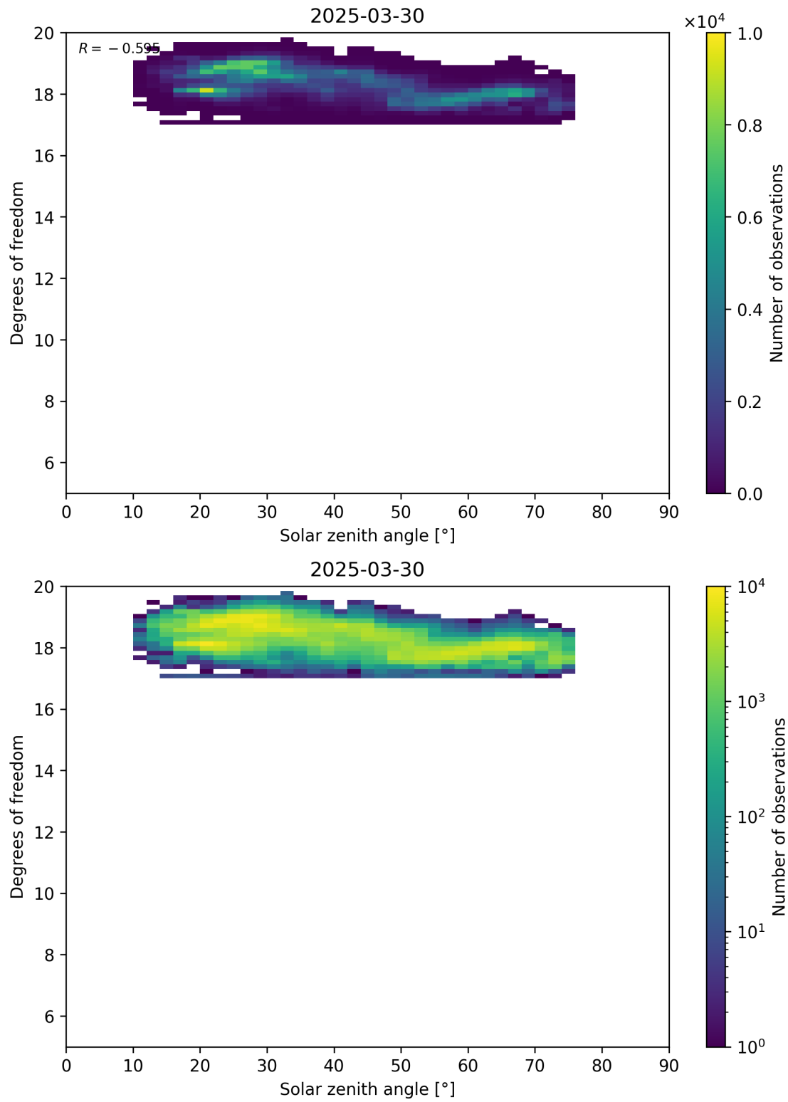
Figure 96: Scatter density plot of “Solar zenith angle” against “Degrees of freedom” for 2025-03-29 to 2025-03-31.
