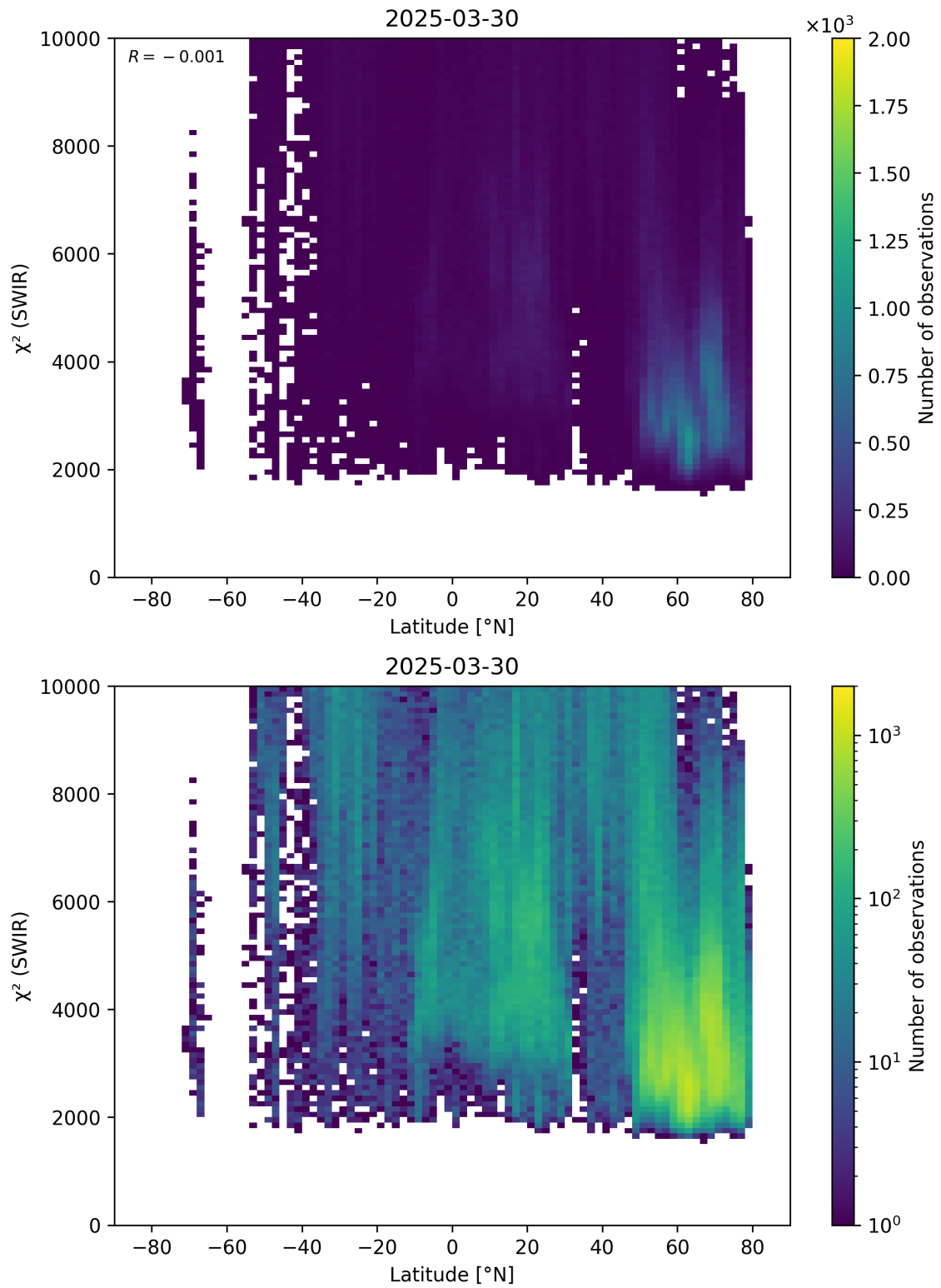
Figure 54: Scatter density plot of “Latitude” against “ \chi^2 (SWIR)” for 2025-03-29 to 2025-03-31.
