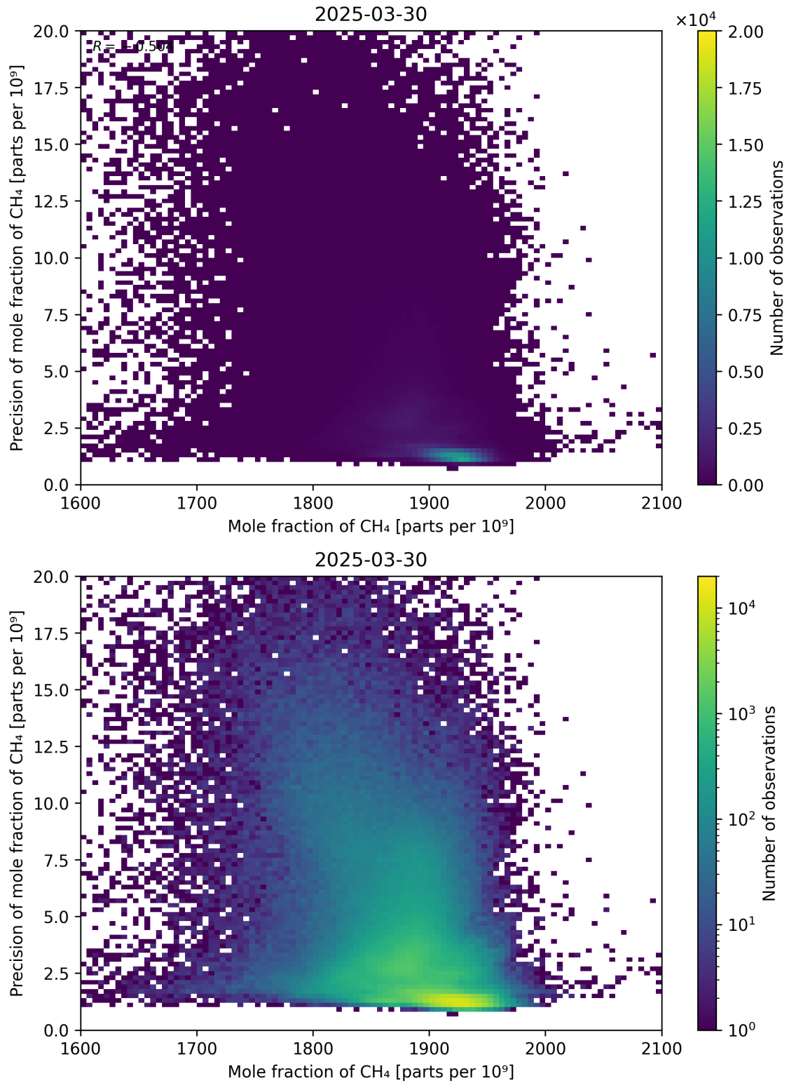
Figure 75: Scatter density plot of “Mole fraction of CH 4 ” against “Precision of mole fraction of CH 4 ” for 2025-03-29 to 2025-03-31.
