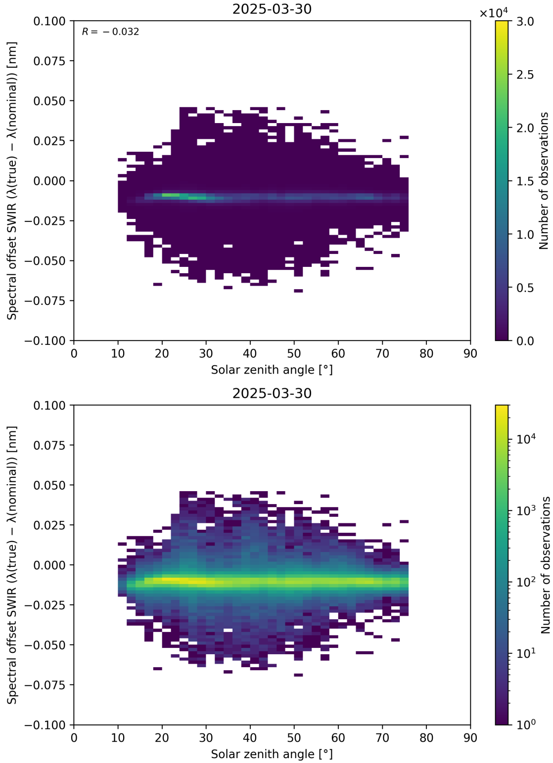
Figure 104: Scatter density plot of “Solar zenith angle” against “Spectral offset SWIR ( \lambda_{\text{true}} - \lambda_{\text{nominal}} )” for 2025-03-29 to 2025-03-31.
