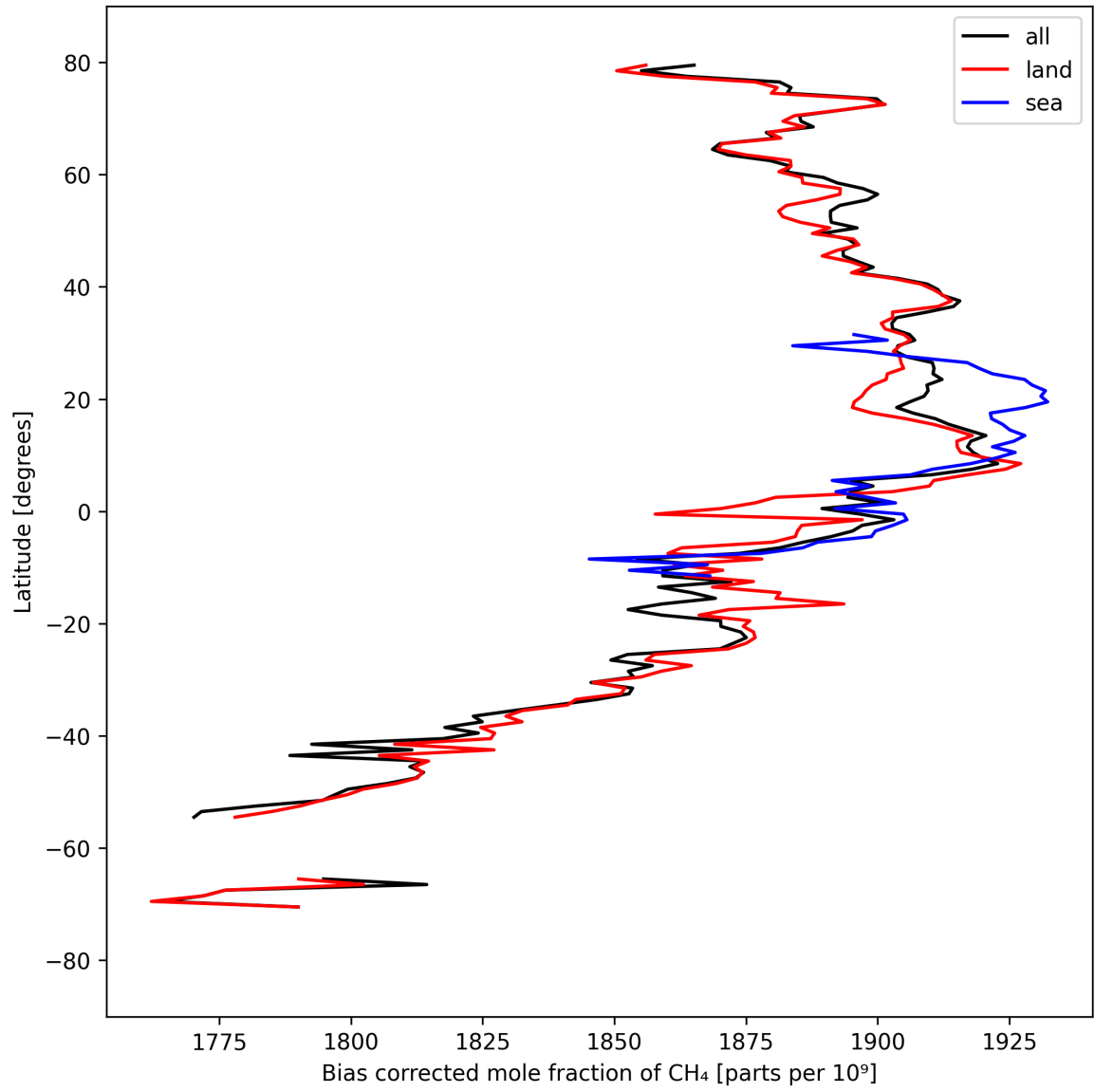
Figure 14: Zonal average of “Bias corrected mole fraction of CH 4 ” for 2025-03-29 to 2025-03-31.
