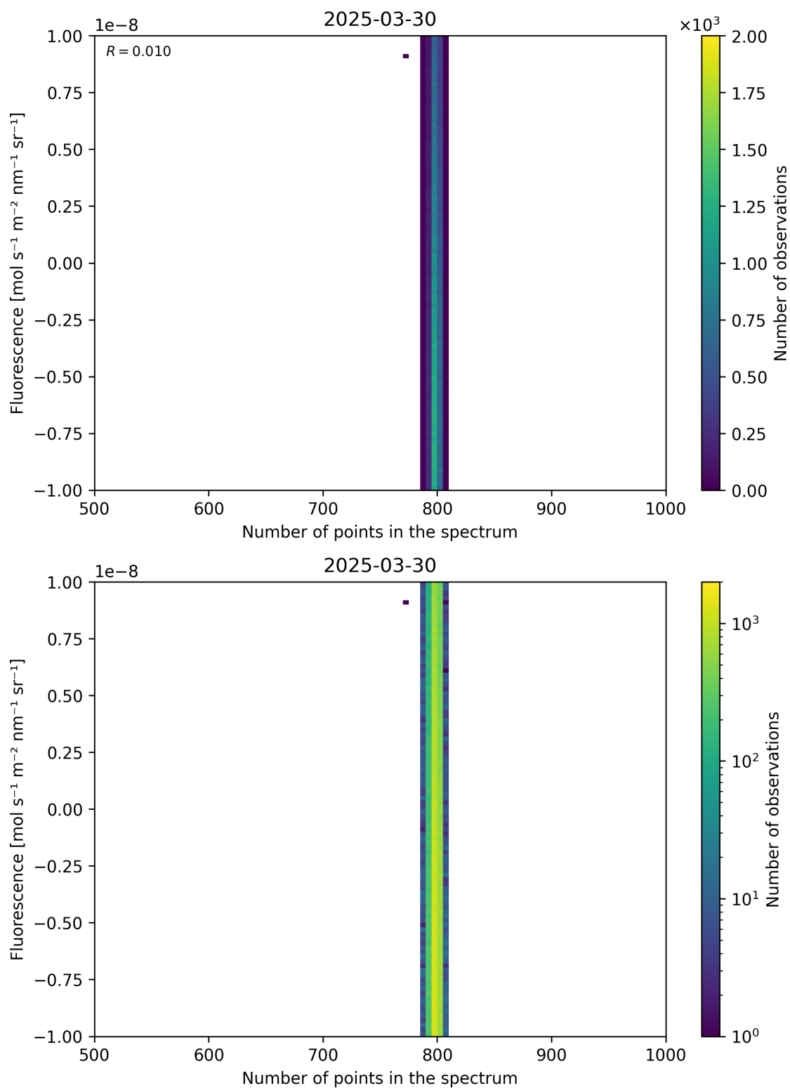
Figure 91: Scatter density plot of “Number of points in the spectrum” against “Fluorescence” for 2025-03-29 to 2025-03-31.
