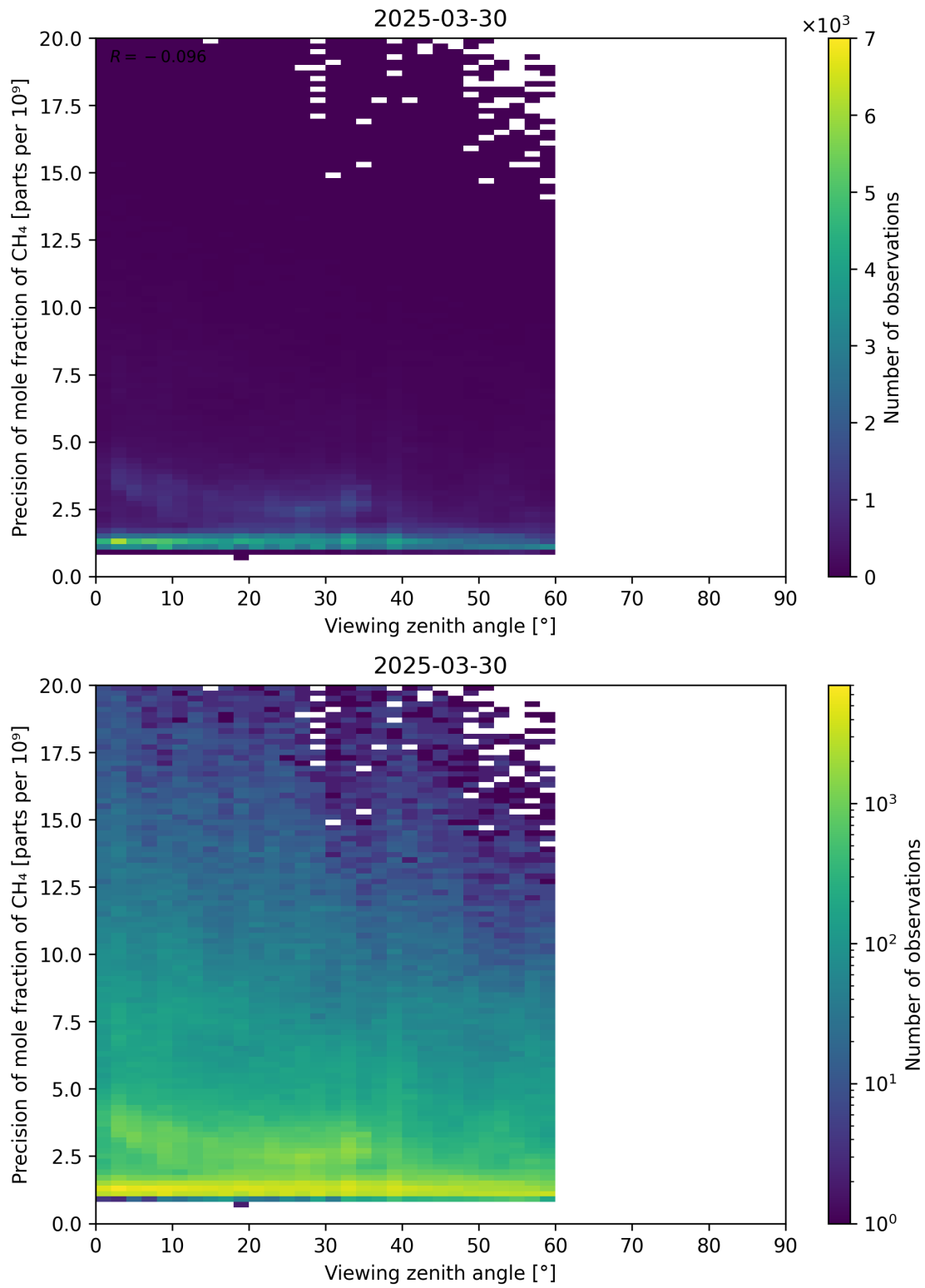
Figure 112: Scatter density plot of “Viewing zenith angle” against “Precision of mole fraction of \text{CH}_4 ” for 2025-03-29 to 2025-03-31.
