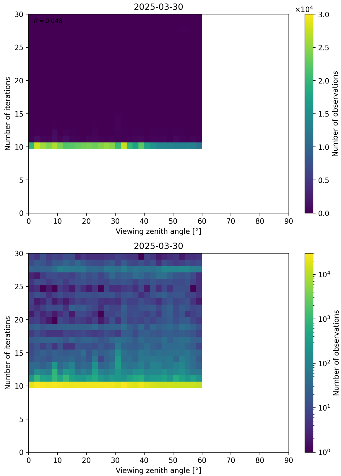
Figure 113: Scatter density plot of “Viewing zenith angle” against “Number of iterations” for 2025-03-29 to 2025-03-31.
