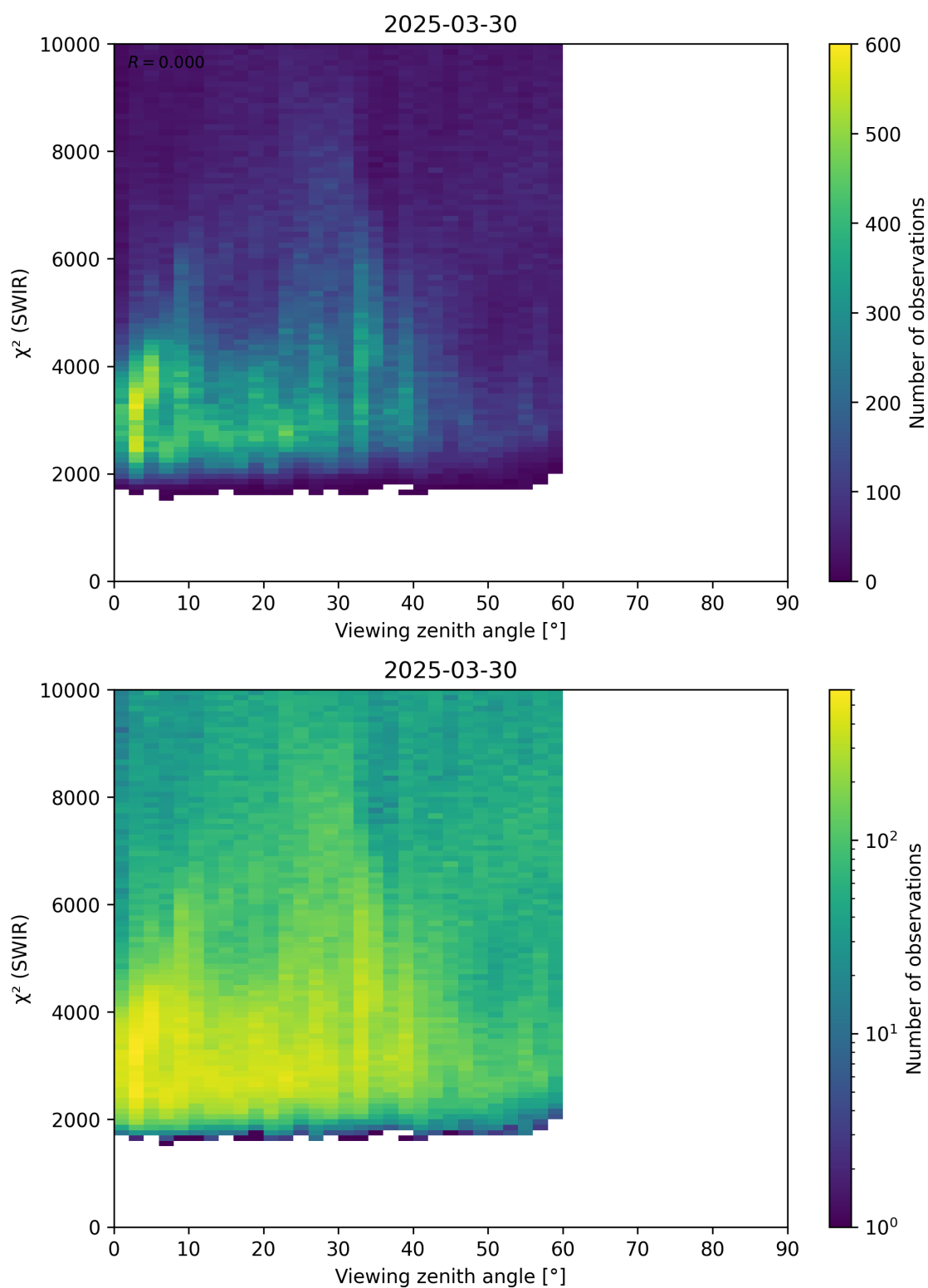
Figure 106: Scatter density plot of “Viewing zenith angle” against “ \chi^2 (SWIR)” for 2025-03-29 to 2025-03-31.
