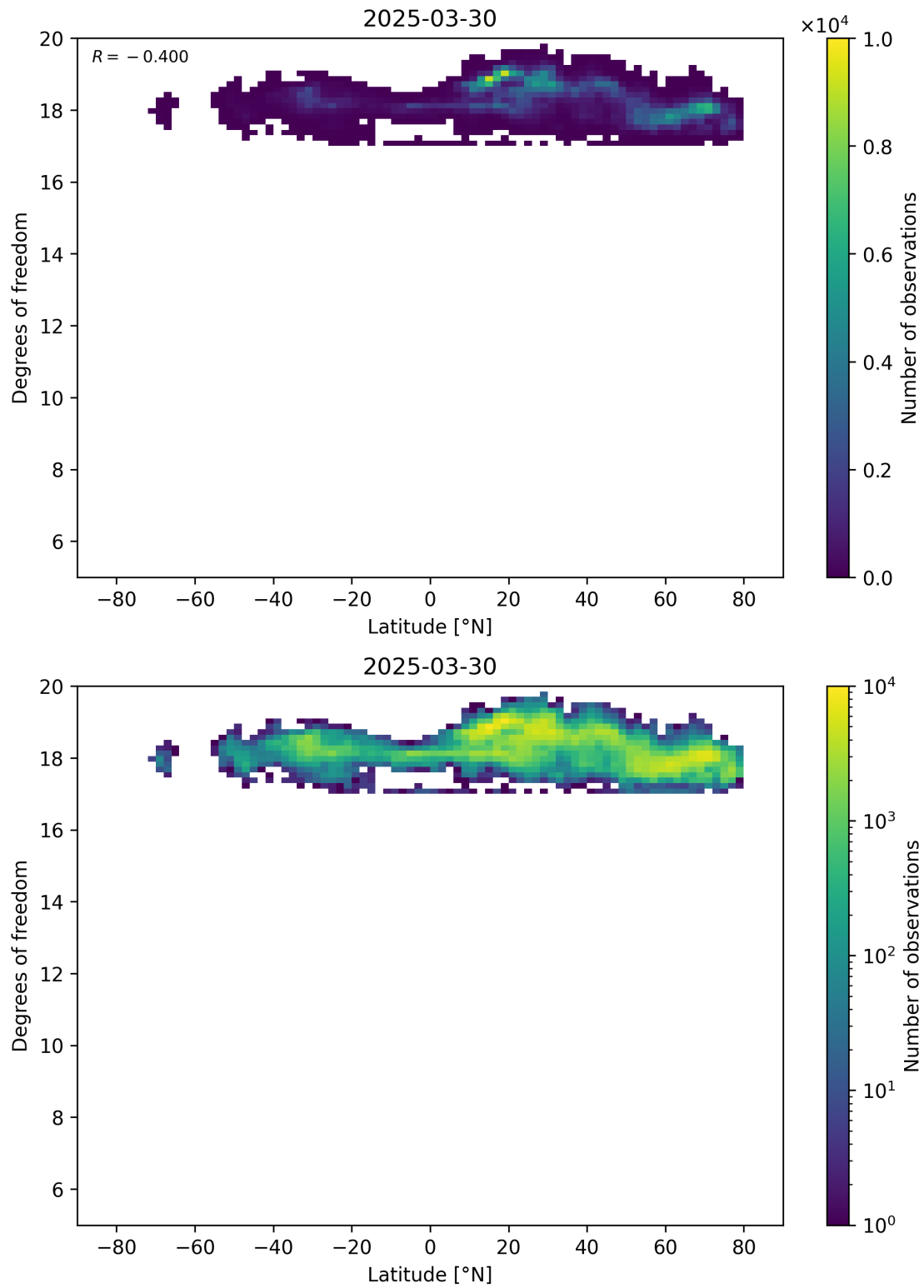
Figure 55: Scatter density plot of “Latitude” against “Degrees of freedom” for 2025-03-29 to 2025-03-31.
