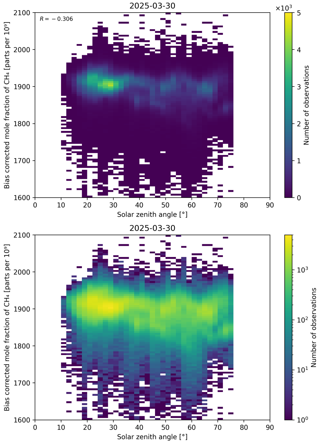
Figure 100: Scatter density plot of “Solar zenith angle” against “Bias corrected mole fraction of CH 4 ” for 2025-03-29 to 2025-03-31.
