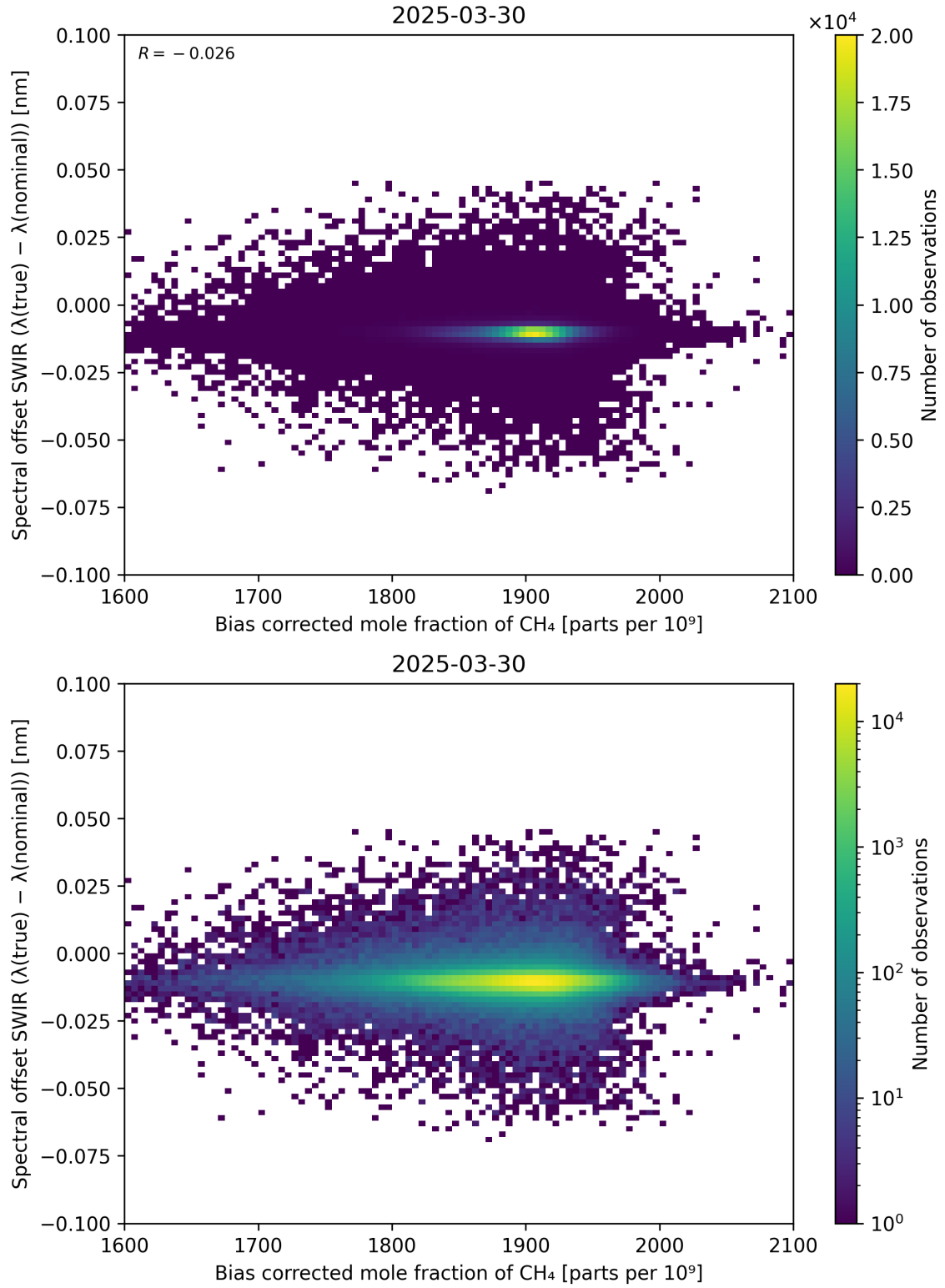
Figure 69: Scatter density plot of “Bias corrected mole fraction of \text{CH}_4 ” against “Spectral offset SWIR ( \lambda_{\text{true}} - \lambda_{\text{nominal}} )” for 2025-03-29 to 2025-03-31.
