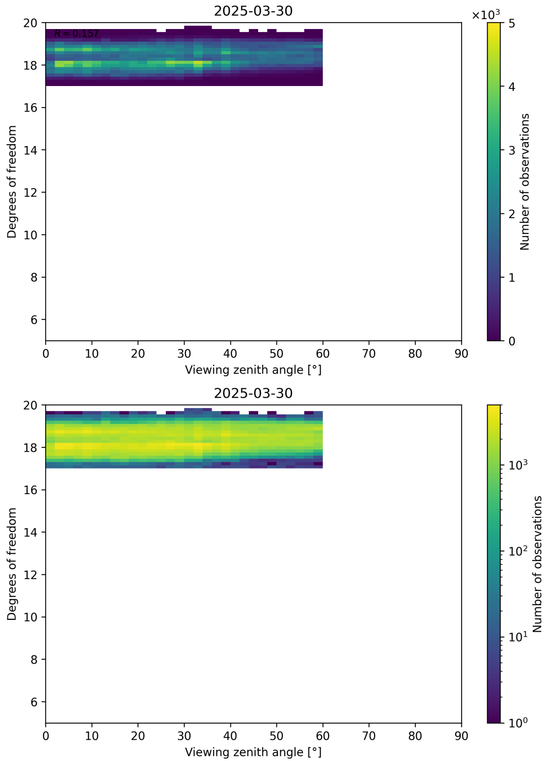
Figure 107: Scatter density plot of “Viewing zenith angle” against “Degrees of freedom” for 2025-03-29 to 2025-03-31.
