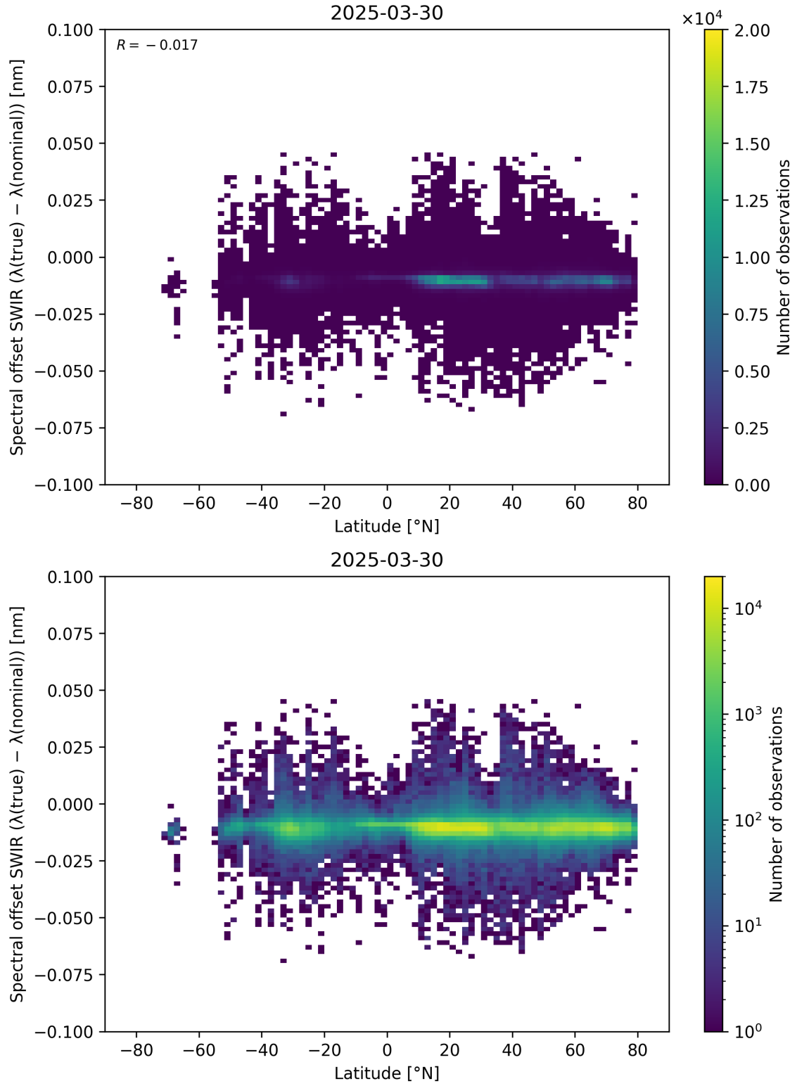
Figure 62: Scatter density plot of “Latitude” against “Spectral offset SWIR ( \lambda_{\text{true}} - \lambda_{\text{nominal}} )” for 2025-03-29 to 2025-03-31.
