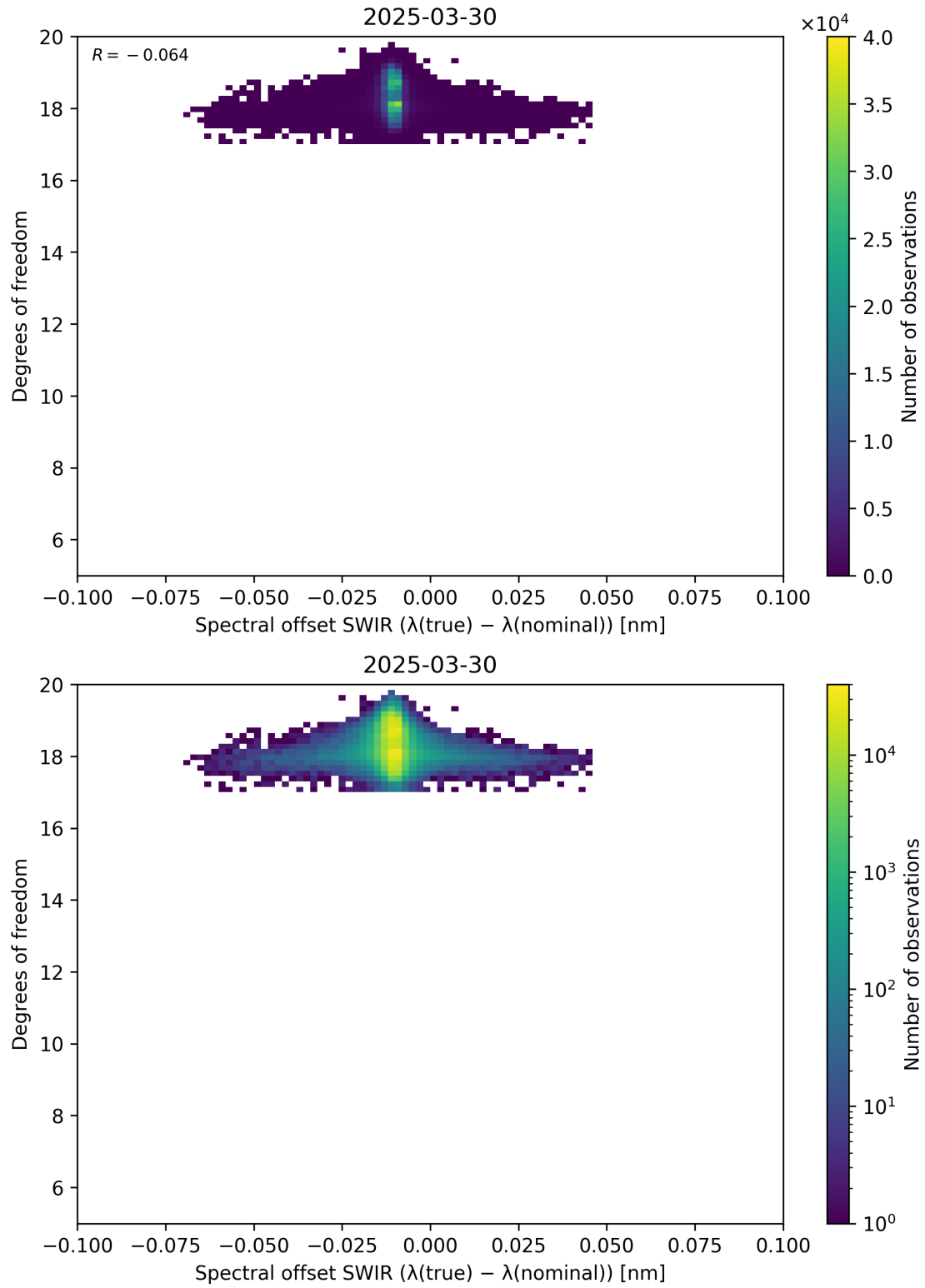
Figure 119: Scatter density plot of “Spectral offset SWIR ( \lambda_{\text{true}} - \lambda_{\text{nominal}} )” against “Degrees of freedom” for 2025-03-29 to 2025-03-31.
