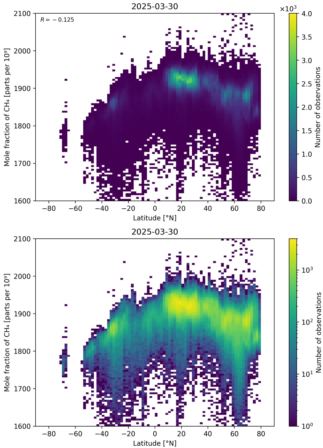
Figure 57: Scatter density plot of “Latitude” against “Mole fraction of CH 4 ” for 2025-03-29 to 2025-03-31.
