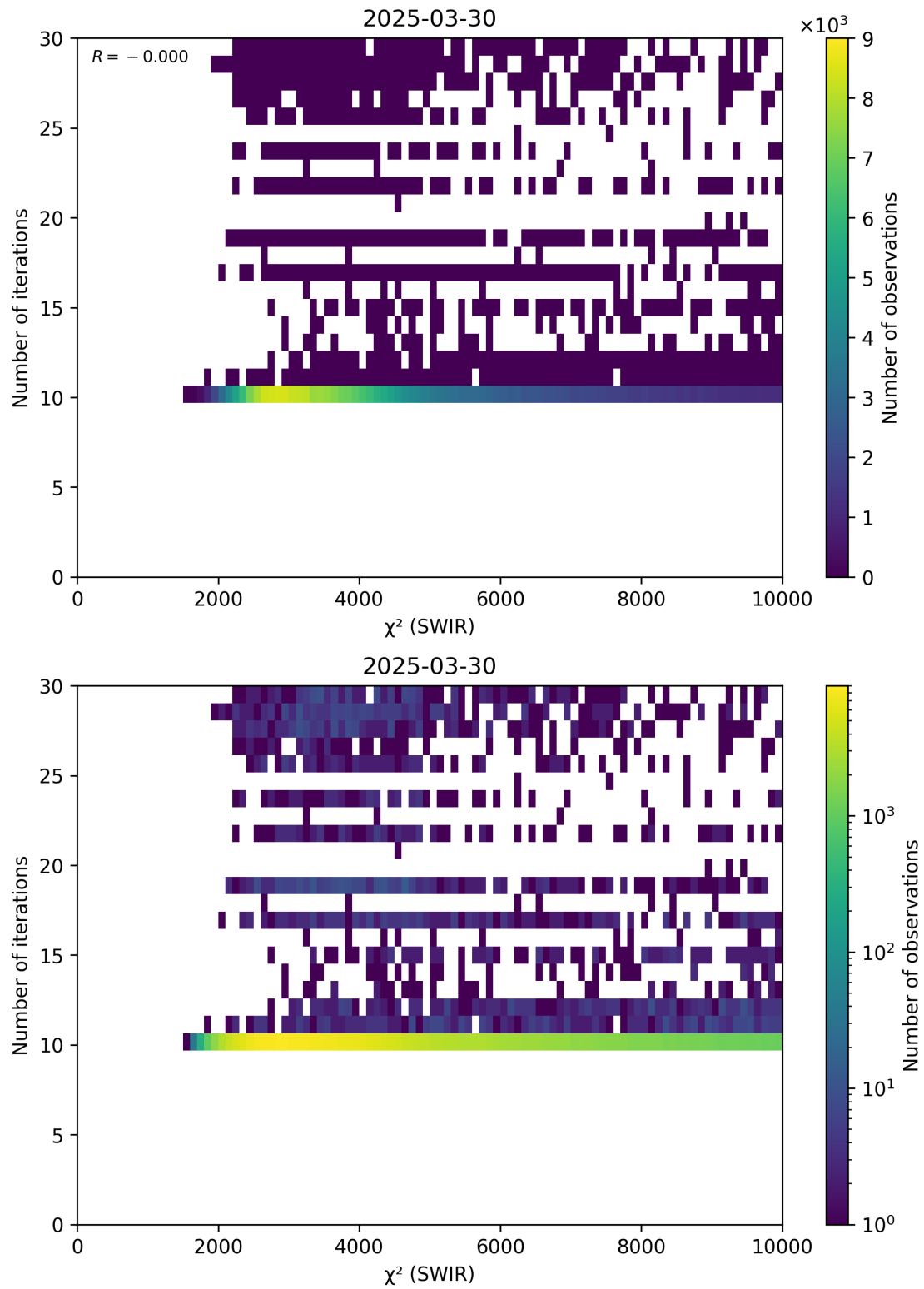
Figure 50: Scatter density plot of “ \chi^2 (SWIR)” against “Number of iterations” for 2025-03-29 to 2025-03-31.
