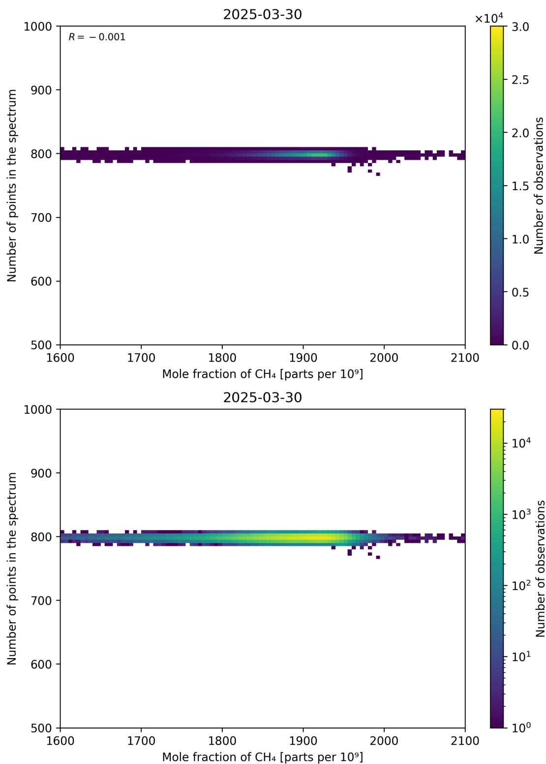
Figure 77: Scatter density plot of “Mole fraction of CH 4 ” against “Number of points in the spectrum” for 2025-03-29 to 2025-03-31.
