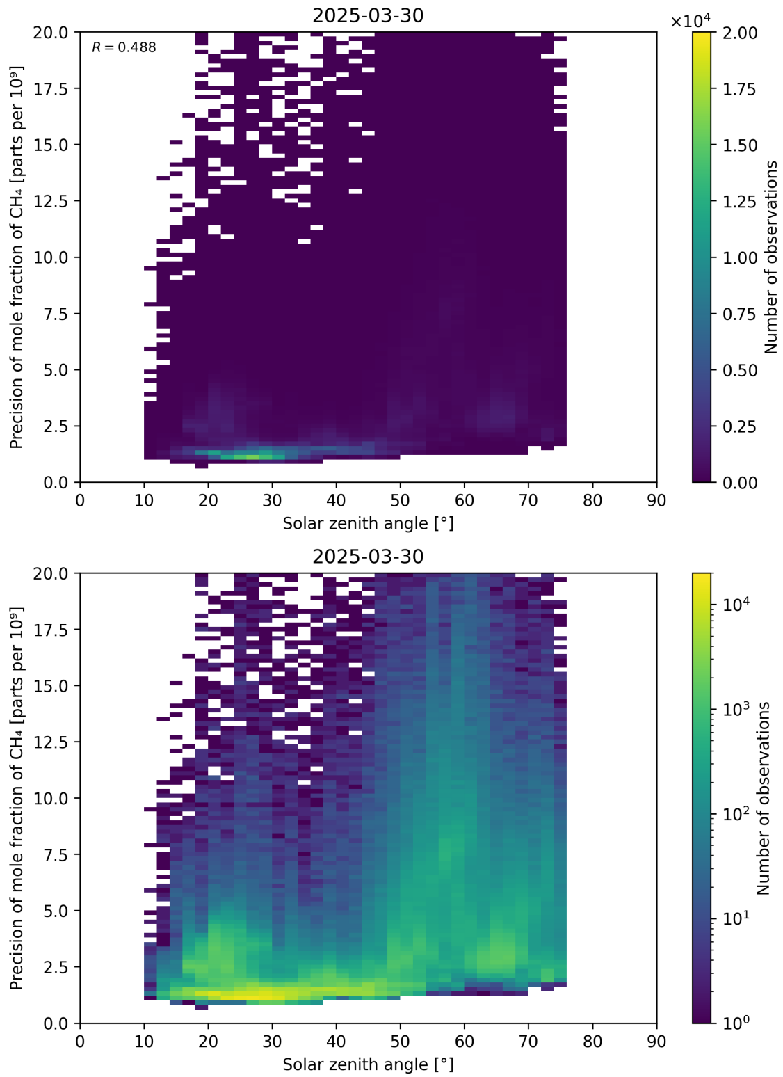
Figure 101: Scatter density plot of “Solar zenith angle” against “Precision of mole fraction of CH 4 ” for 2025-03-29 to 2025-03-31.
