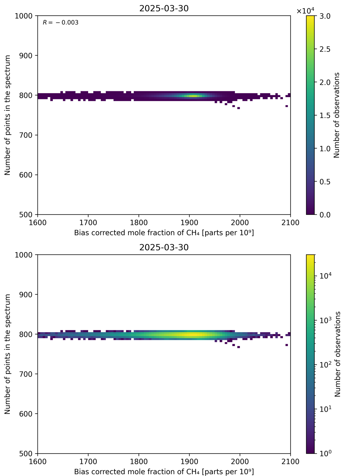
Figure 68: Scatter density plot of “Bias corrected mole fraction of CH 4 ” against “Number of points in the spectrum” for 2025-03-29 to 2025-03-31.
