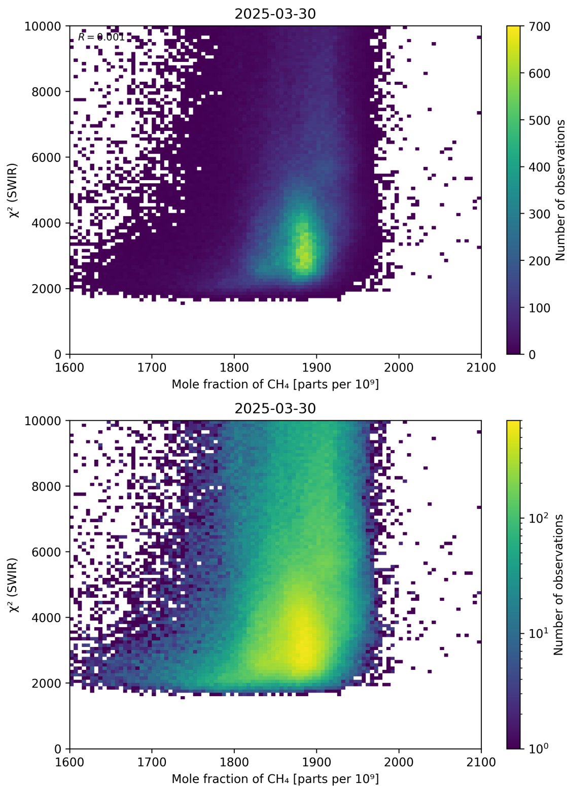
Figure 71: Scatter density plot of “Mole fraction of CH 4 ” against “ \chi^2 (SWIR)” for 2025-03-29 to 2025-03-31.
