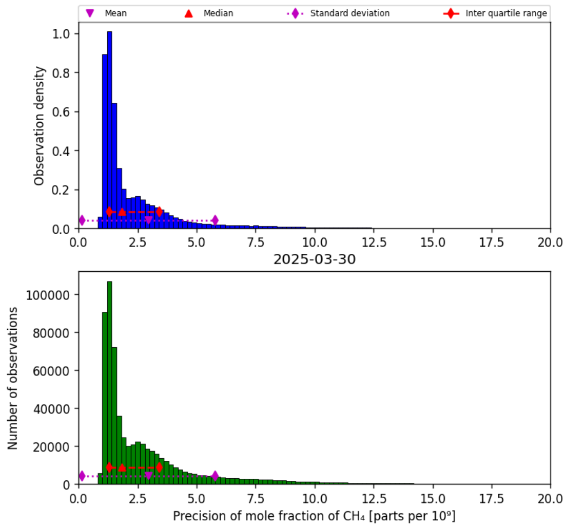
Figure 24: Histogram of “Precision of mole fraction of CH 4 ” for 2025-03-29 to 2025-03-31
