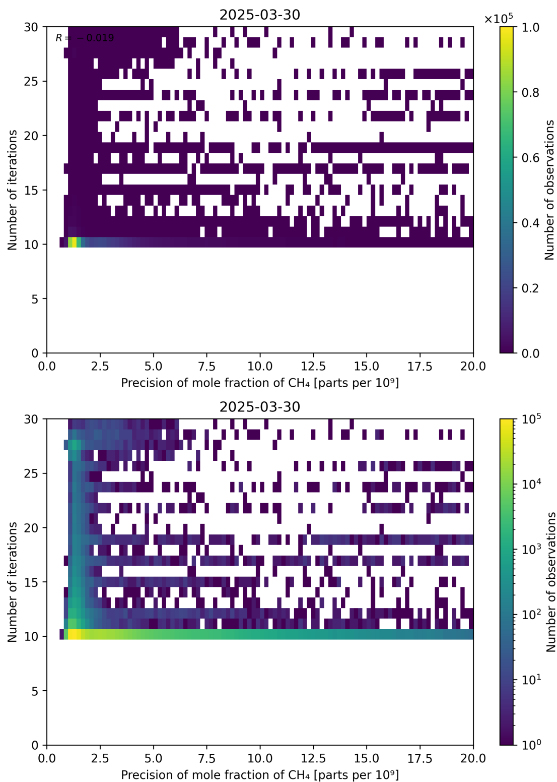
Figure 83: Scatter density plot of “Precision of mole fraction of CH 4 ” against “Number of iterations” for 2025-03-29 to 2025-03-31.
