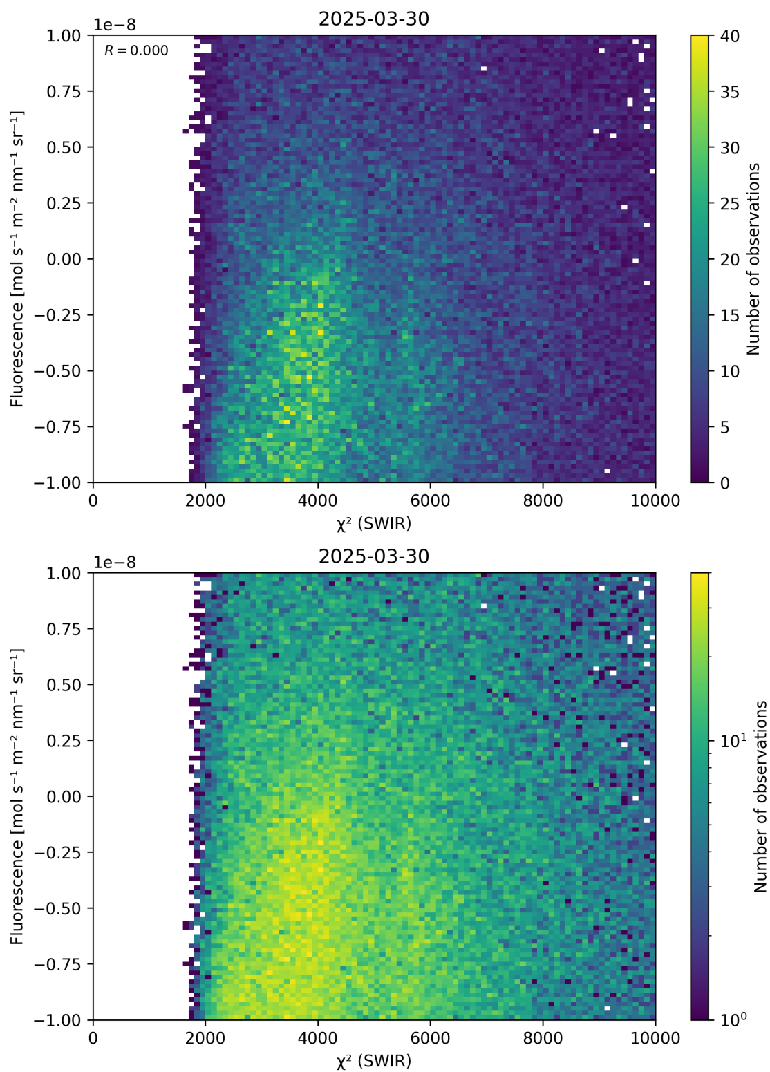
Figure 49: Scatter density plot of “ \chi^2 (SWIR)” against “Fluorescence” for 2025-03-29 to 2025-03-31.
