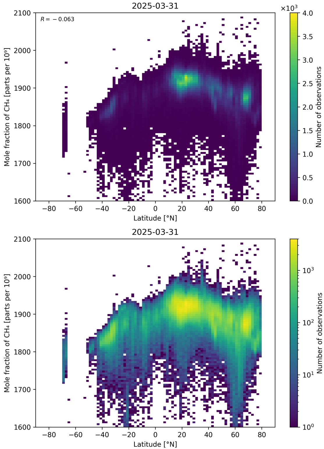
Figure 57: Scatter density plot of “Latitude” against “Mole fraction of CH 4 ” for 2025-03-30 to 2025-04-01.
