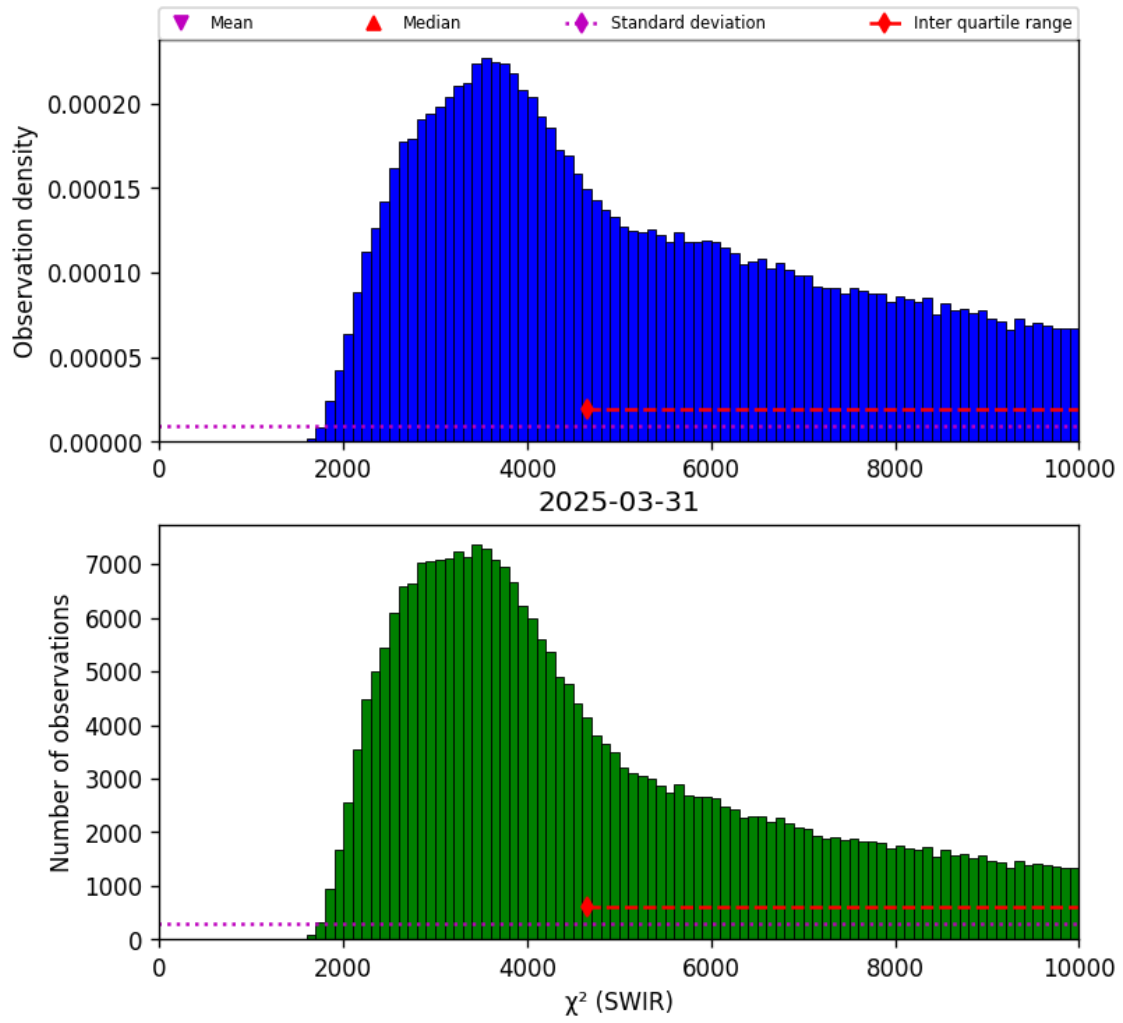
Figure 28: Histogram of " \chi^2 (SWIR)" for 2025-03-30 to 2025-04-01
