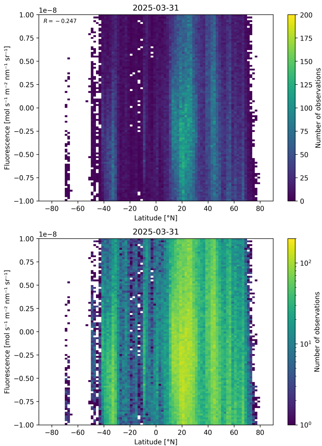
Figure 56: Scatter density plot of “Latitude” against “Fluorescence” for 2025-03-30 to 2025-04-01.
