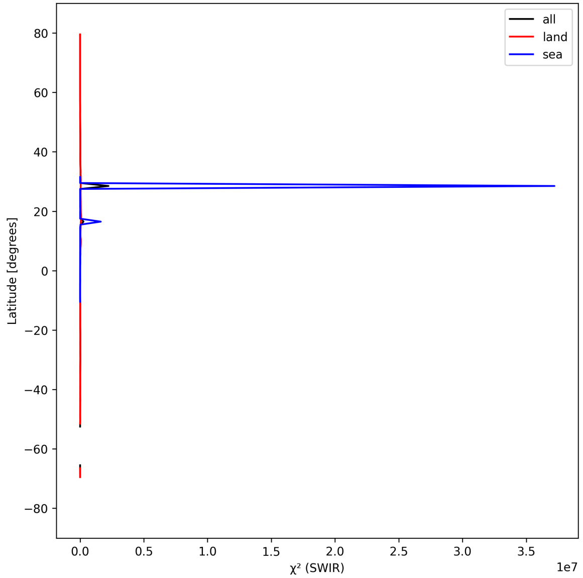
Figure 17: Zonal average of “ \chi^2 (SWIR)” for 2025-03-30 to 2025-04-01.
