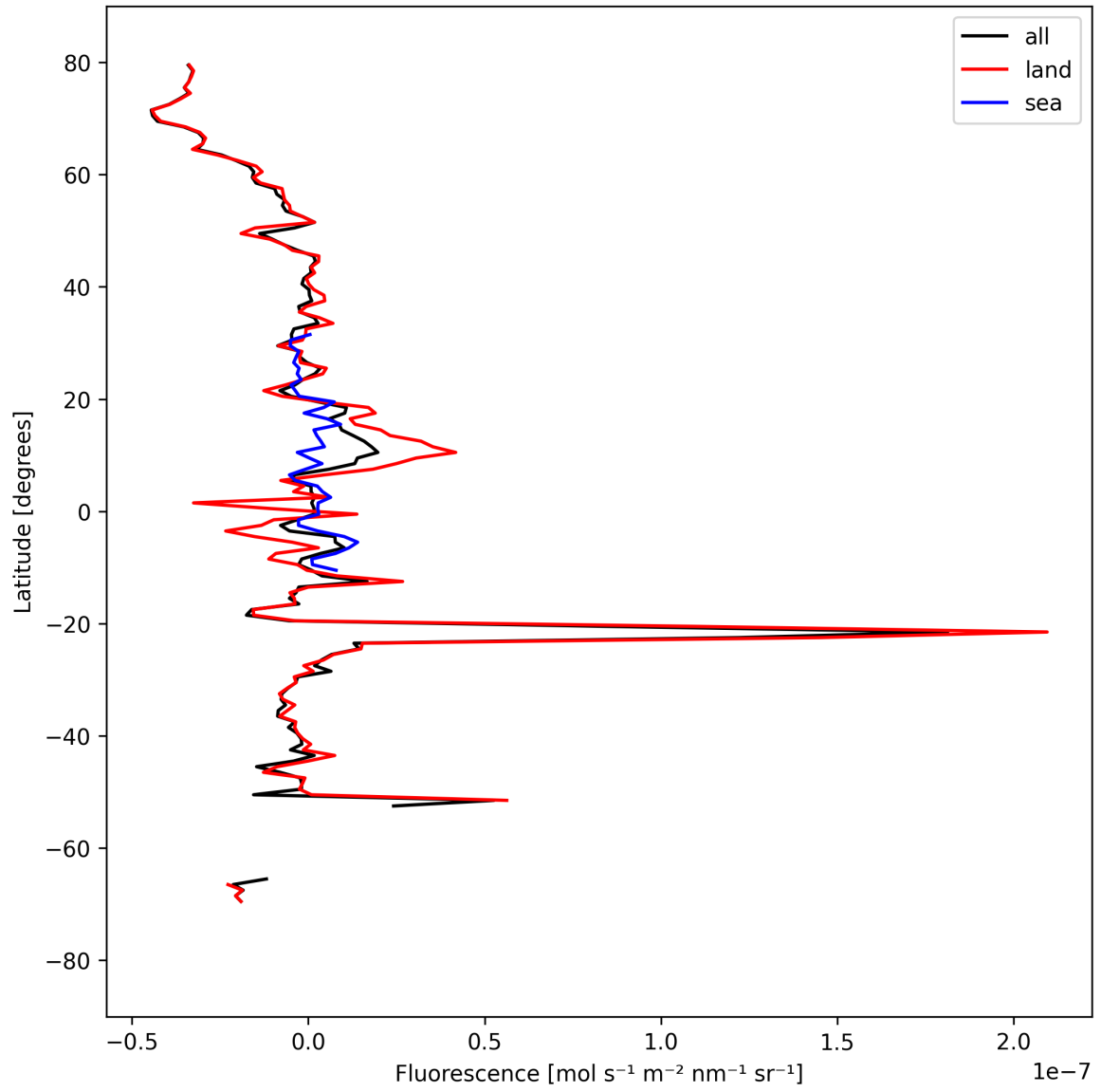
Figure 21: Zonal average of “Fluorescence” for 2025-03-30 to 2025-04-01.
