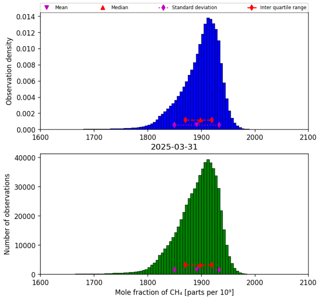
Figure 23: Histogram of “Mole fraction of CH 4 ” for 2025-03-30 to 2025-04-01
