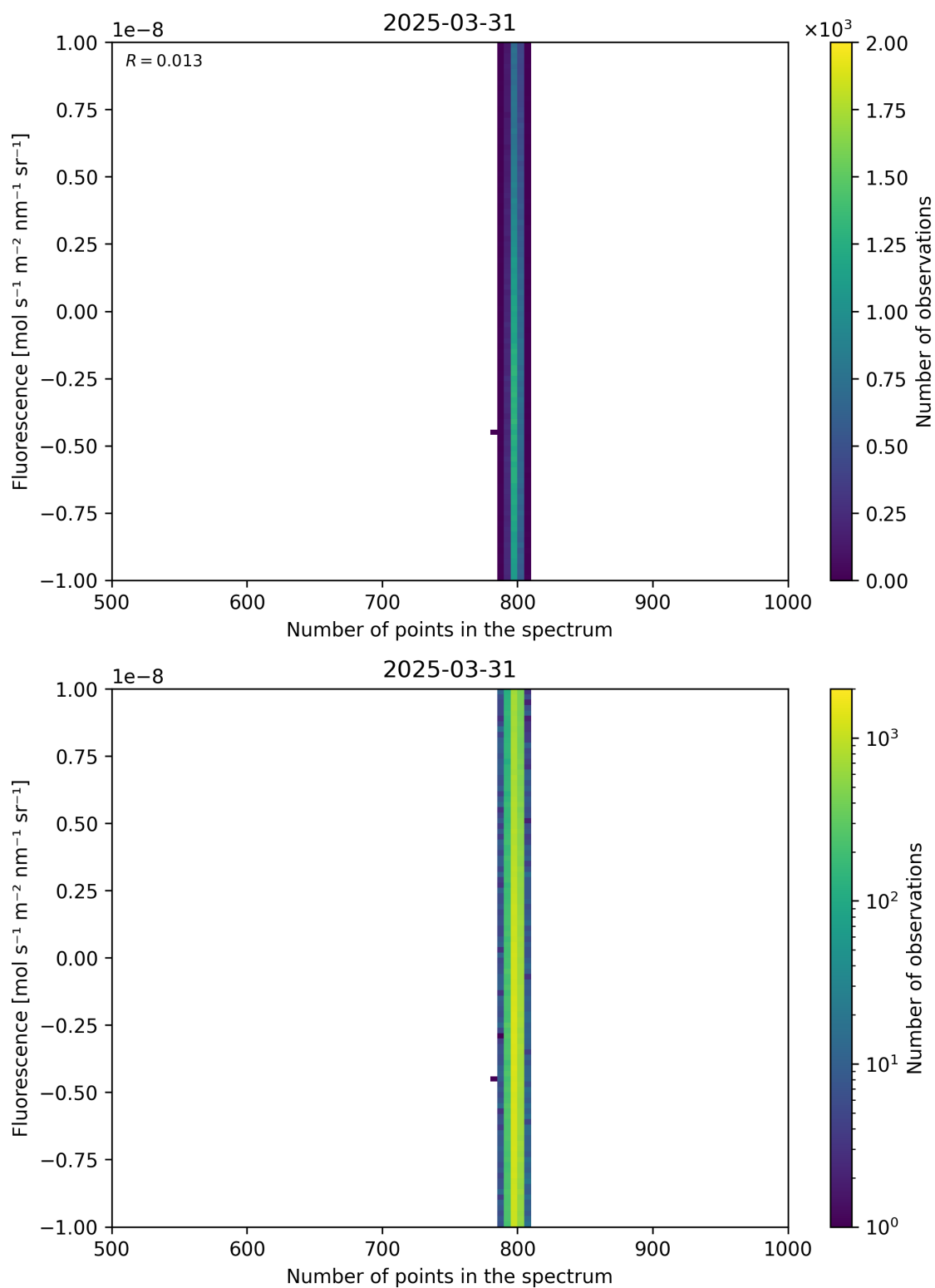
Figure 91: Scatter density plot of “Number of points in the spectrum” against “Fluorescence” for 2025-03-30 to 2025-04-01.
