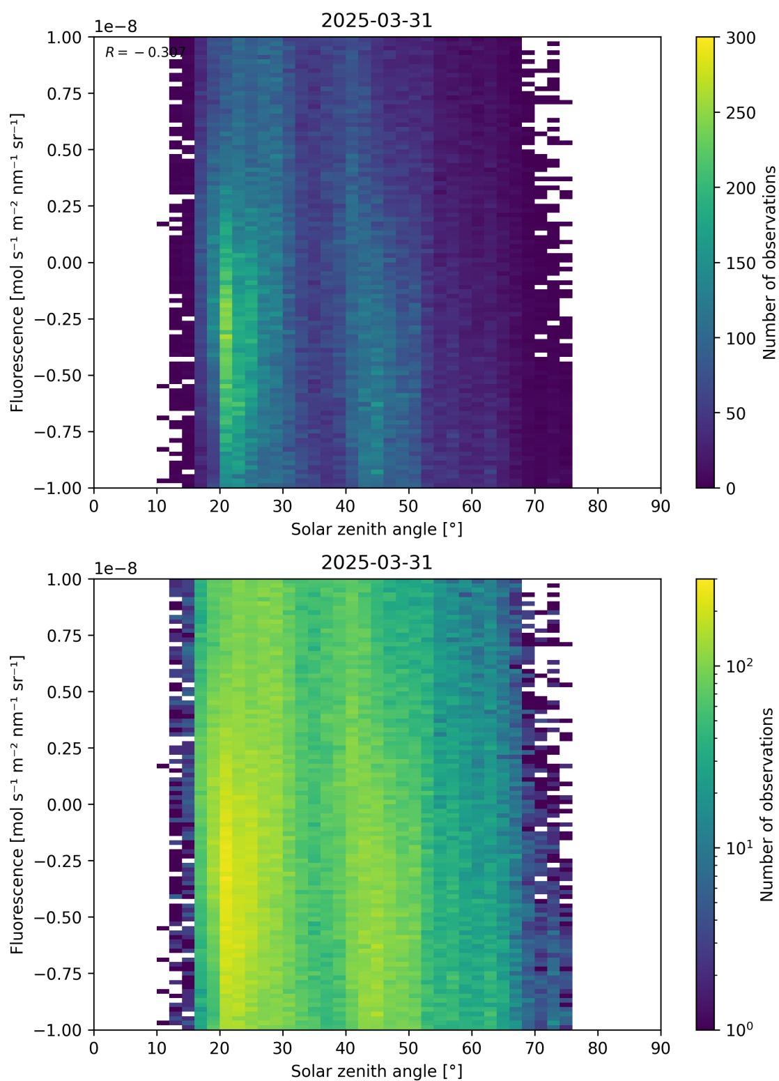
Figure 97: Scatter density plot of “Solar zenith angle” against “Fluorescence” for 2025-03-30 to 2025-04-01.
