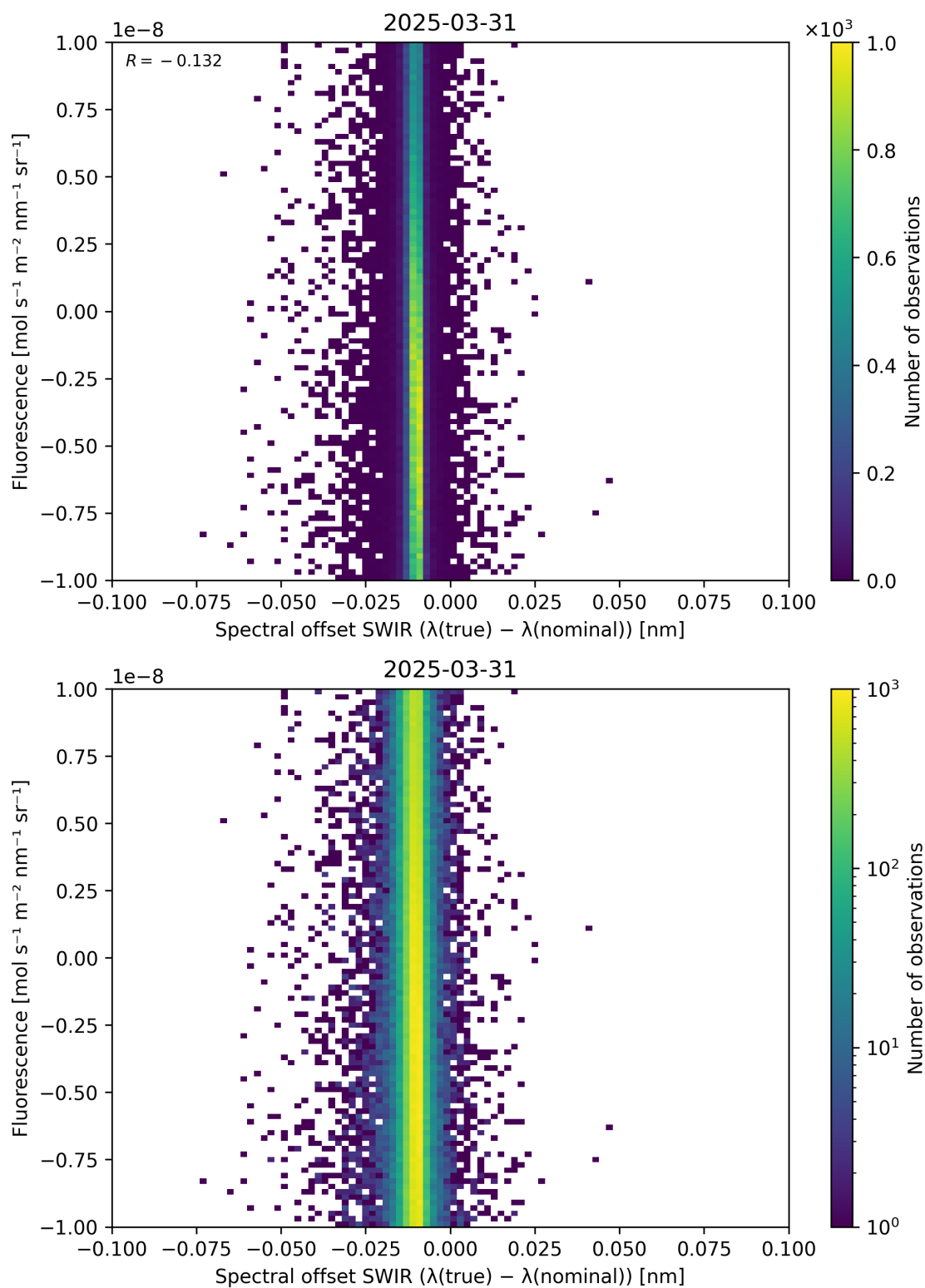
Figure 120: Scatter density plot of “Spectral offset SWIR ( \lambda_{\text{true}} - \lambda_{\text{nominal}} )” against “Fluorescence” for 2025-03-30 to 2025-04-01.
