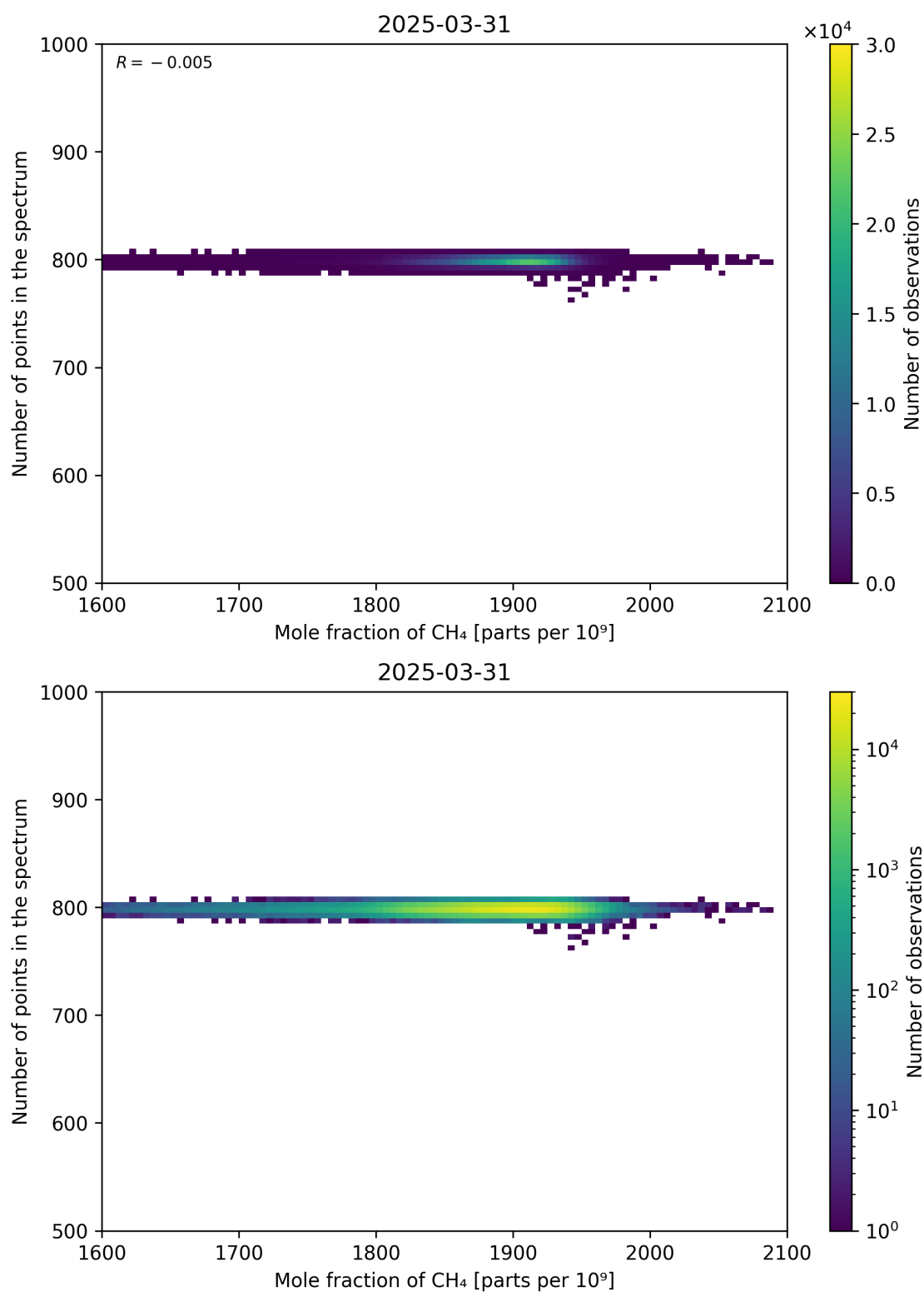
Figure 77: Scatter density plot of “Mole fraction of CH 4 ” against “Number of points in the spectrum” for 2025-03-30 to 2025-04-01.
