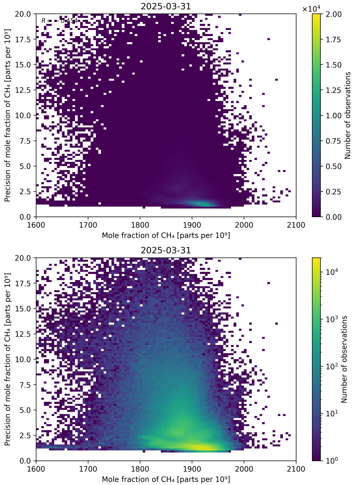
Figure 75: Scatter density plot of “Mole fraction of CH 4 ” against “Precision of mole fraction of CH 4 ” for 2025-03-30 to 2025-04-01.
