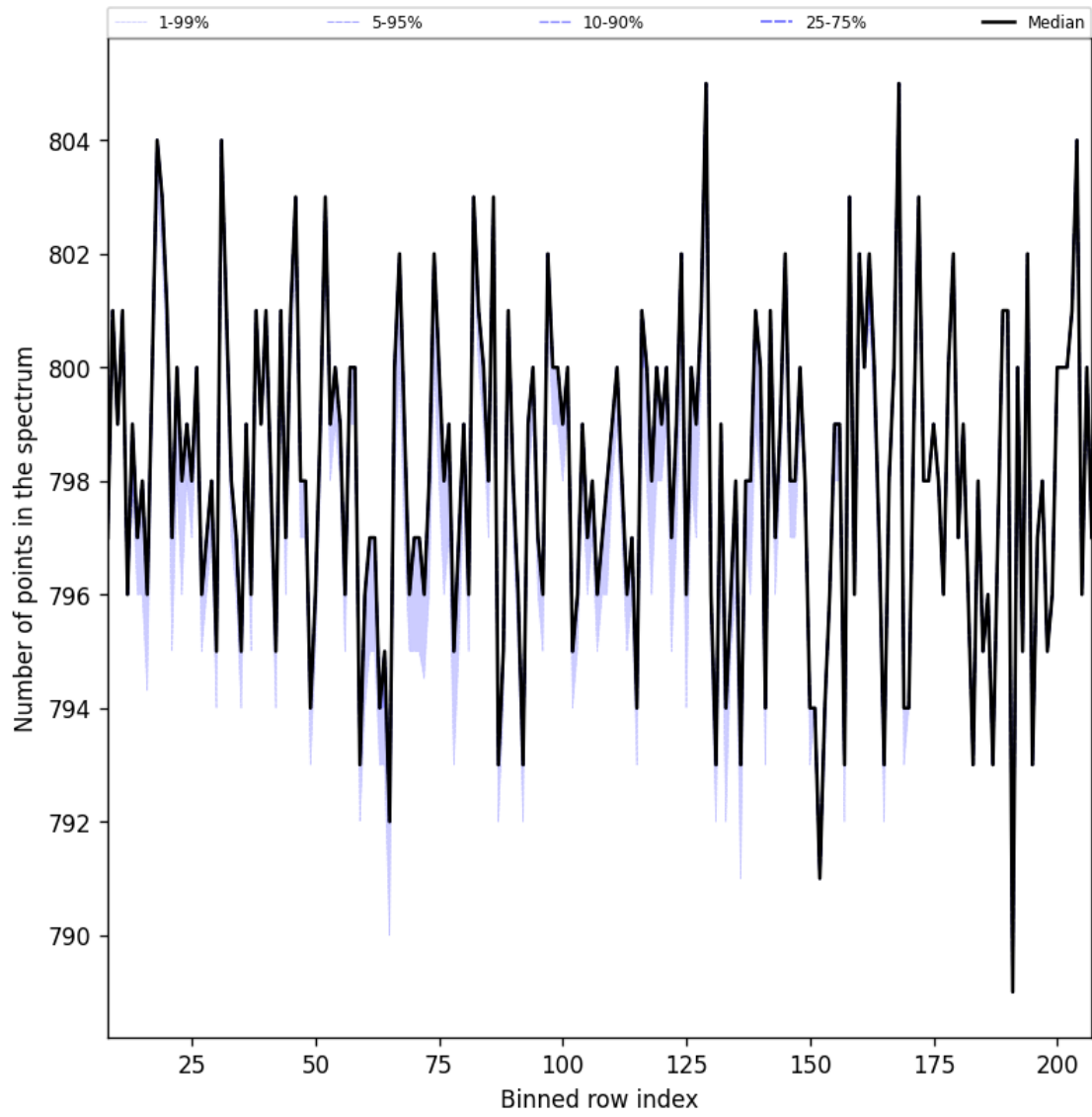
Figure 37: Along track statistics of “Number of points in the spectrum” for 2025-03-30 to 2025-04-01
