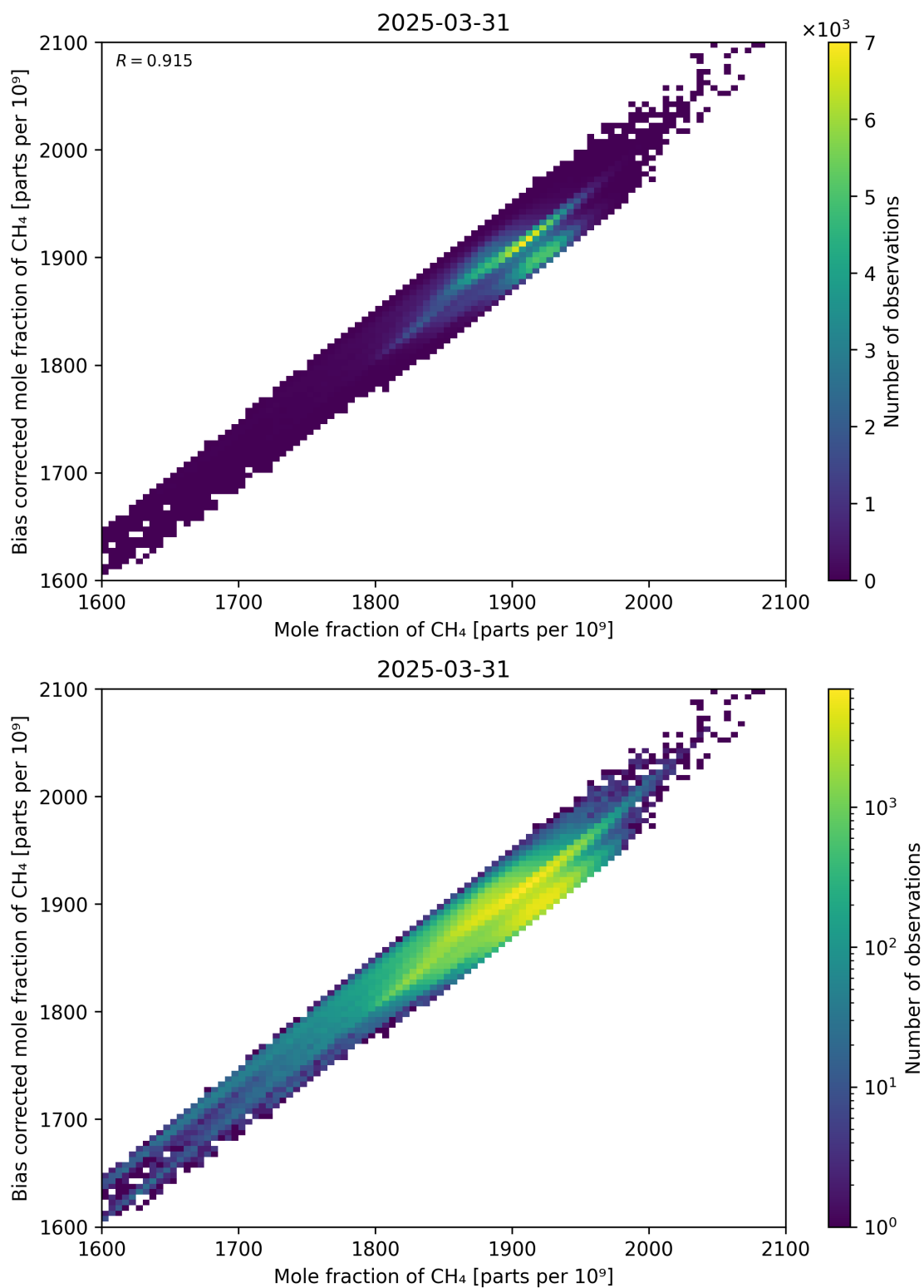
Figure 74: Scatter density plot of “Mole fraction of CH 4 ” against “Bias corrected mole fraction of CH 4 ” for 2025-03-30 to 2025-04-01.
