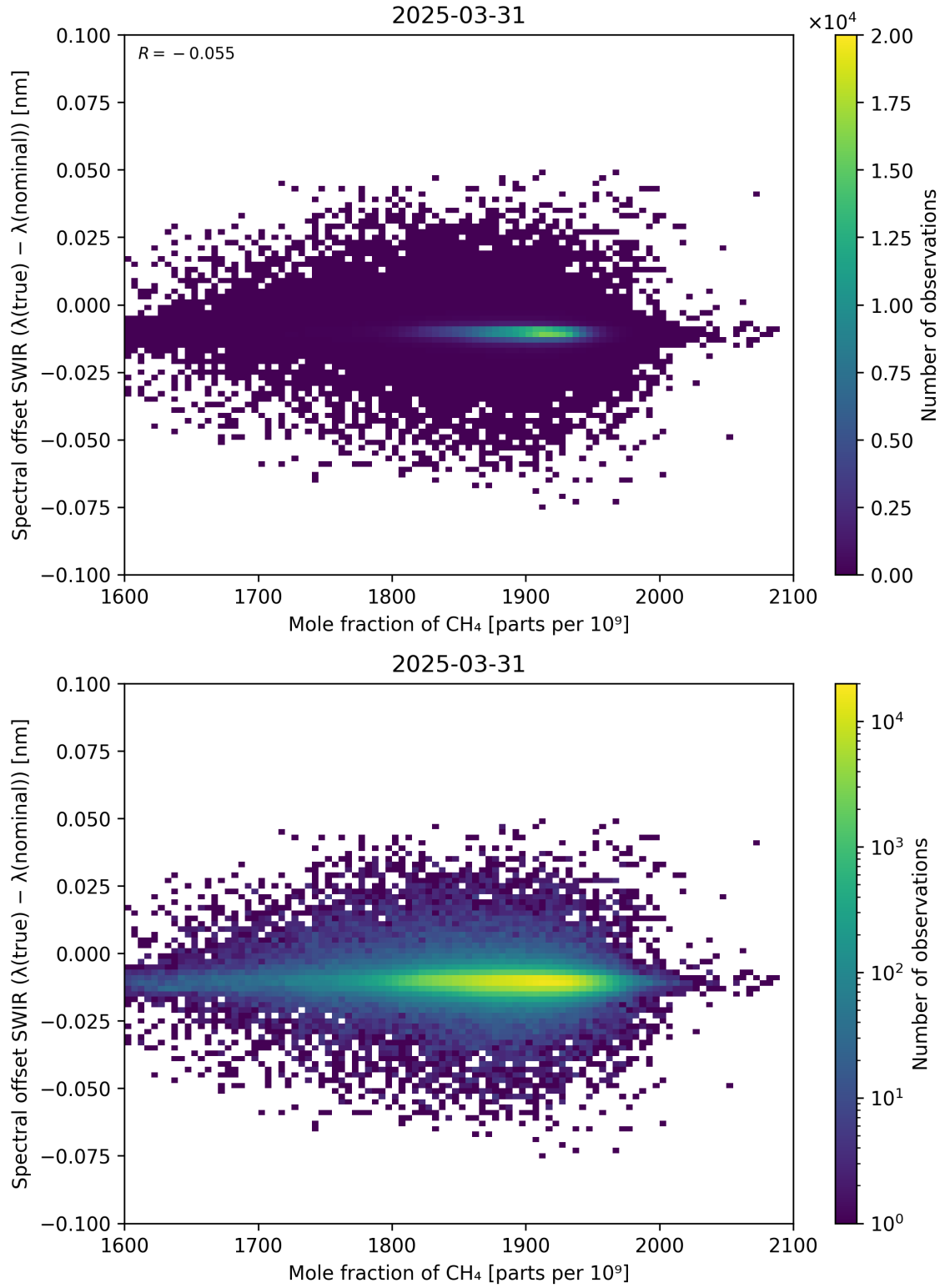
Figure 86: Scatter density plot of “Mole fraction of \text{CH}_4 ” against “Spectral offset SWIR ( \lambda_{\text{true}} - \lambda_{\text{nominal}} )” for 2025-03-30 to 2025-04-01.
