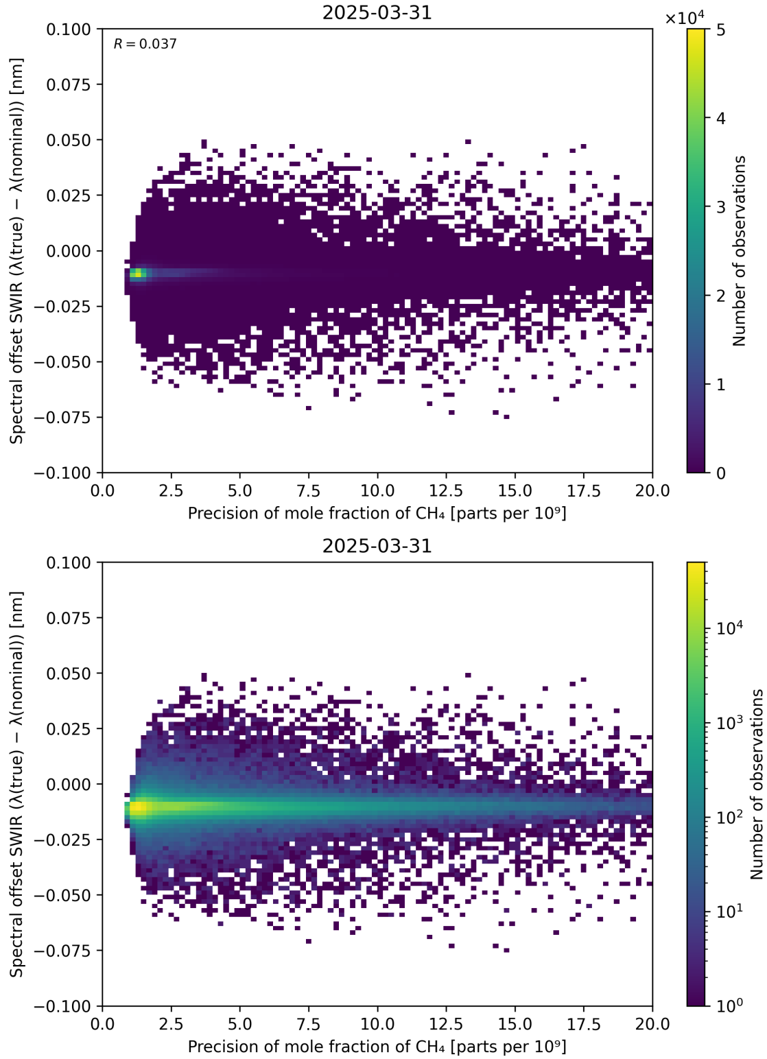
Figure 85: Scatter density plot of “Precision of mole fraction of \text{CH}_4 ” against “Spectral offset SWIR ( \lambda_{\text{true}} - \lambda_{\text{nominal}} )” for 2025-03-30 to 2025-04-01.
