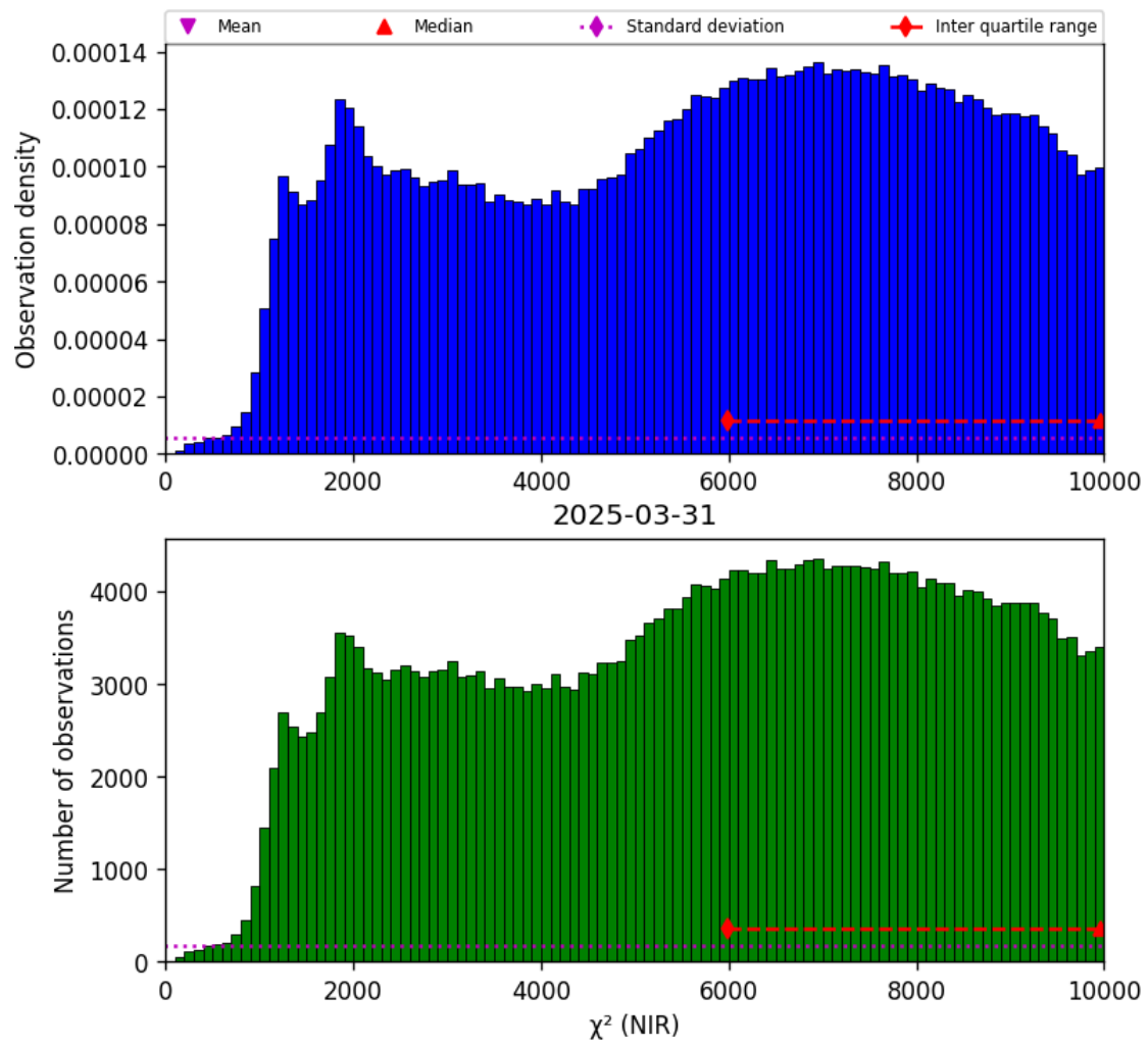
Figure 29: Histogram of “ \chi^2 (NIR)” for 2025-03-30 to 2025-04-01
