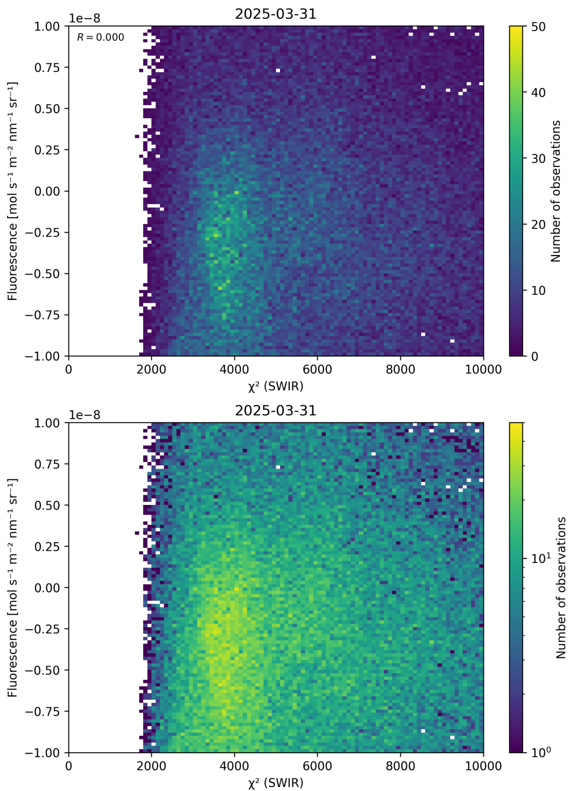
Figure 49: Scatter density plot of “ \chi^2 (SWIR)” against “Fluorescence” for 2025-03-30 to 2025-04-01.
