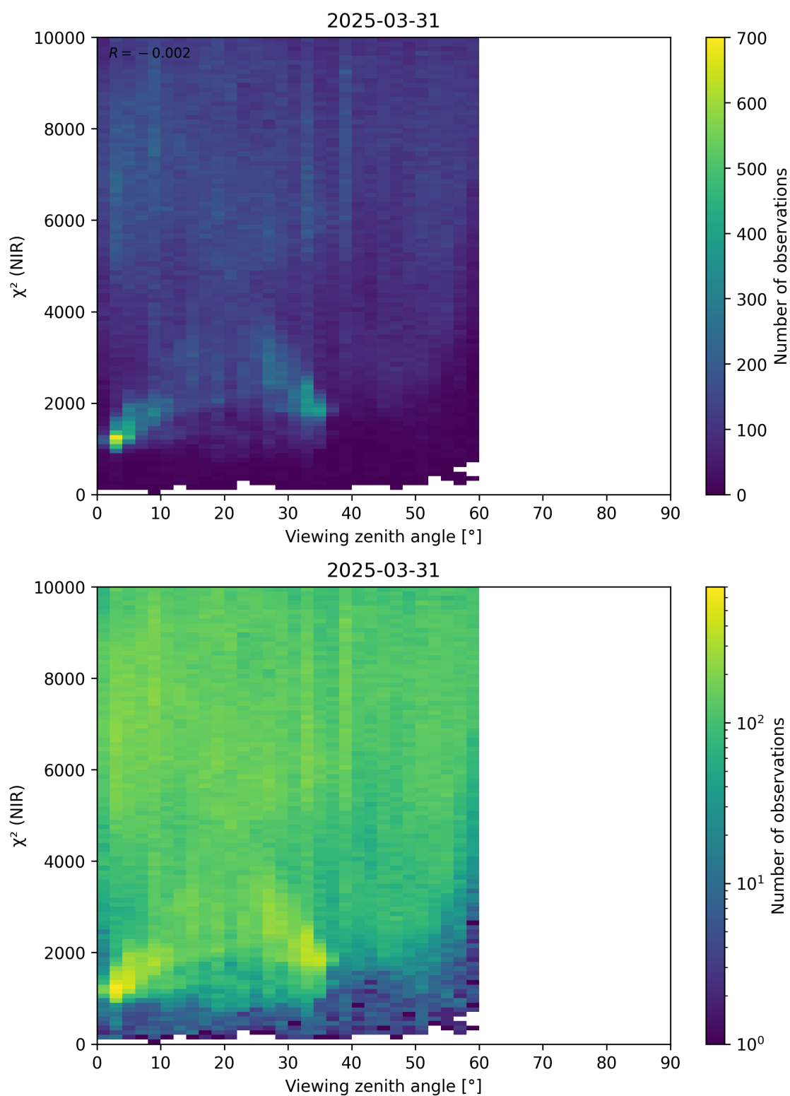
Figure 105: Scatter density plot of “Viewing zenith angle” against “ \chi^2 (NIR)” for 2025-03-30 to 2025-04-01.
