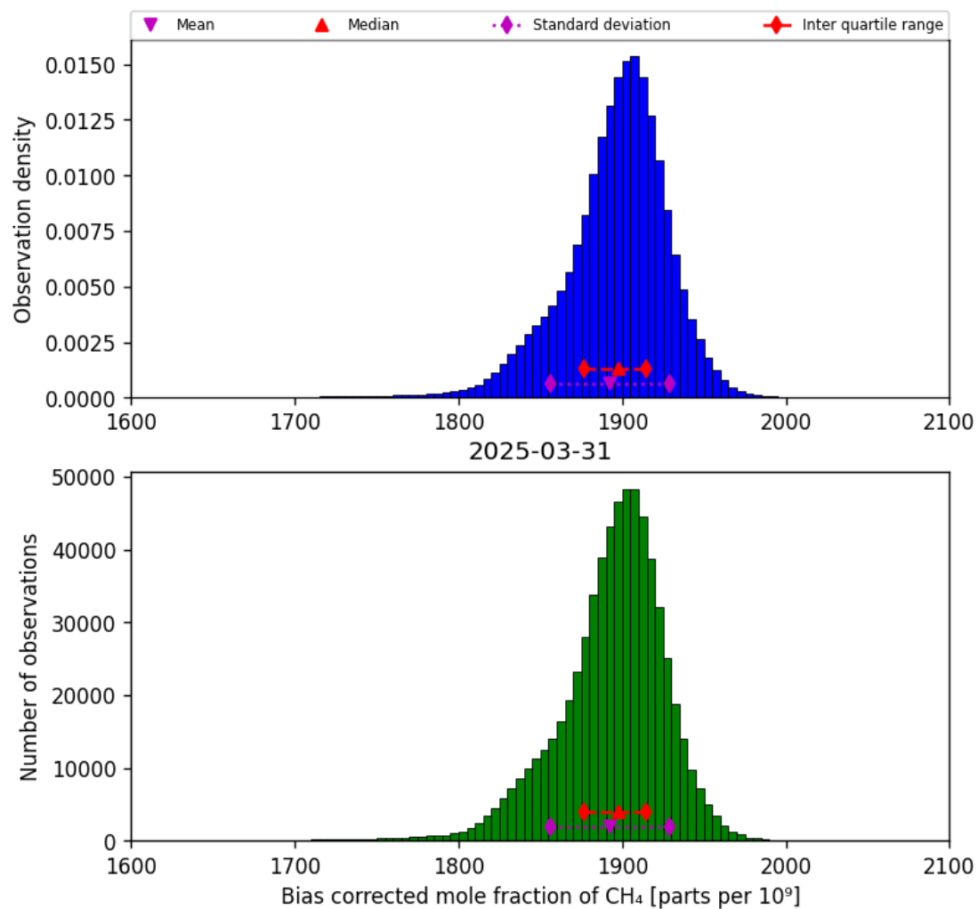
Figure 25: Histogram of “Bias corrected mole fraction of CH 4 ” for 2025-03-30 to 2025-04-01
