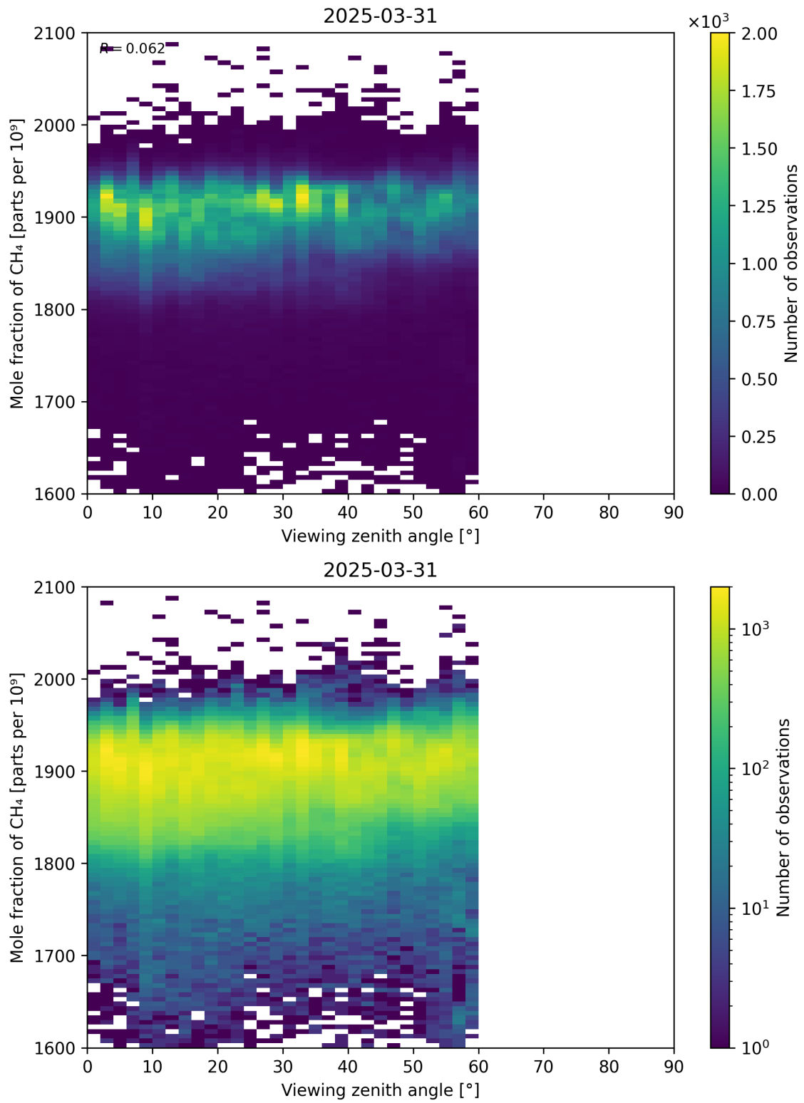
Figure 110: Scatter density plot of “Viewing zenith angle” against “Mole fraction of CH 4 ” for 2025-03-30 to 2025-04-01.
