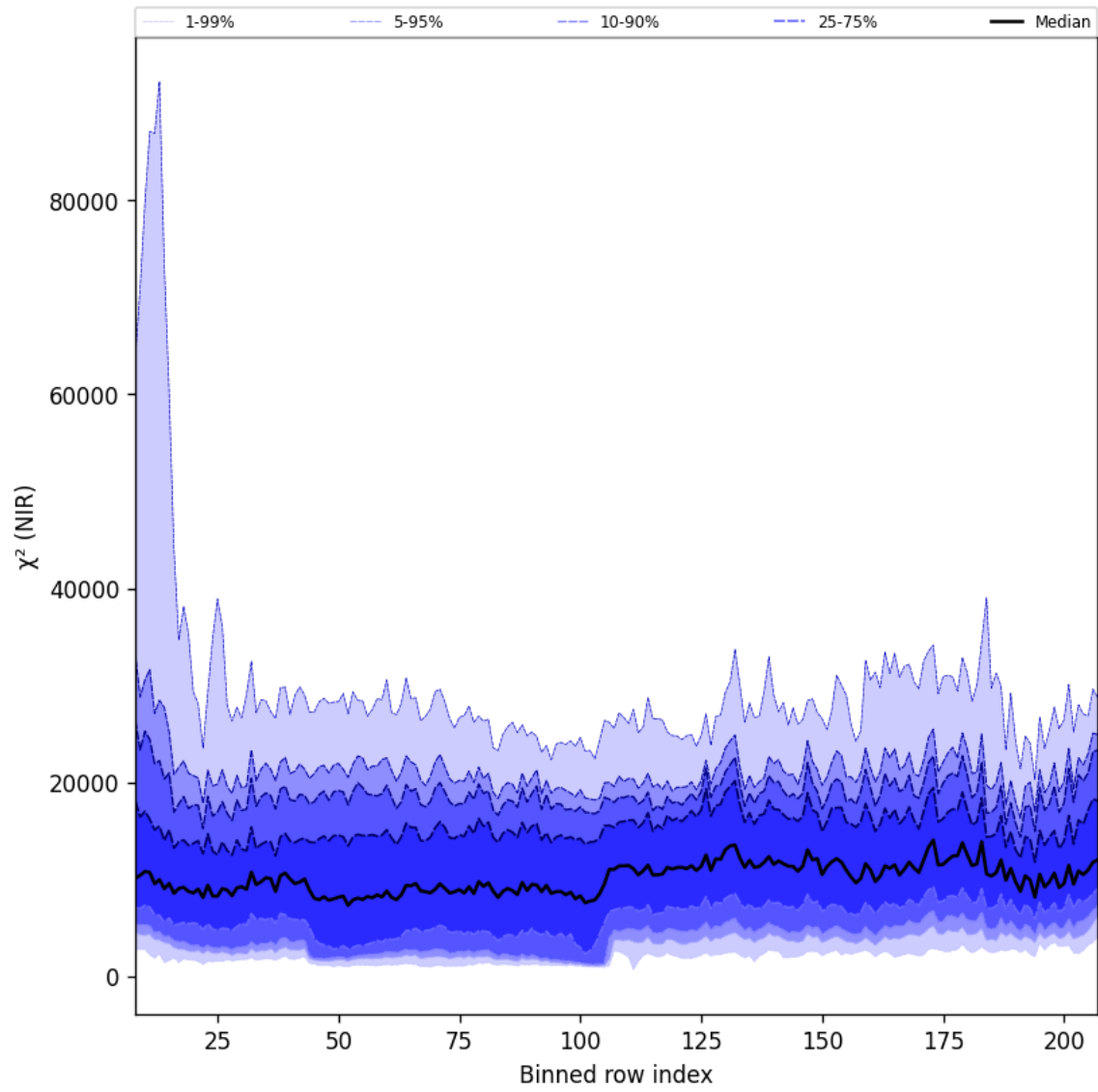
Figure 40: Along track statistics of “ \chi^2 (NIR)” for 2025-03-30 to 2025-04-01
