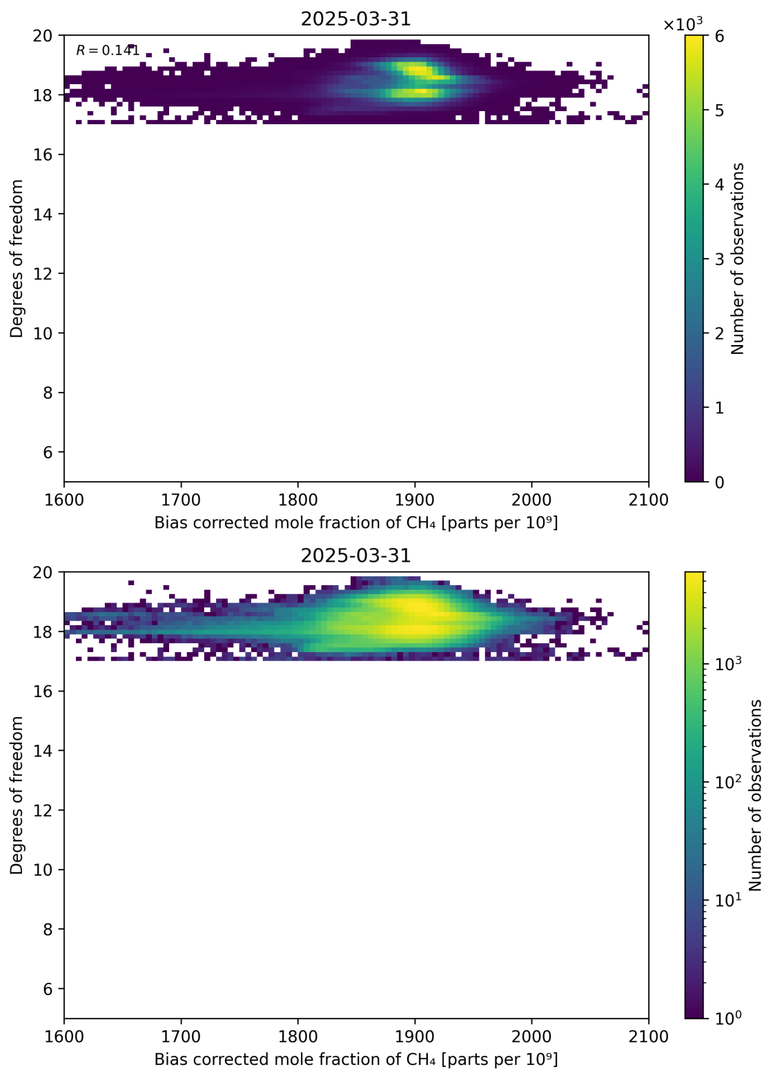
Figure 65: Scatter density plot of “Bias corrected mole fraction of CH 4 ” against “Degrees of freedom” for 2025-03-30 to 2025-04-01.
