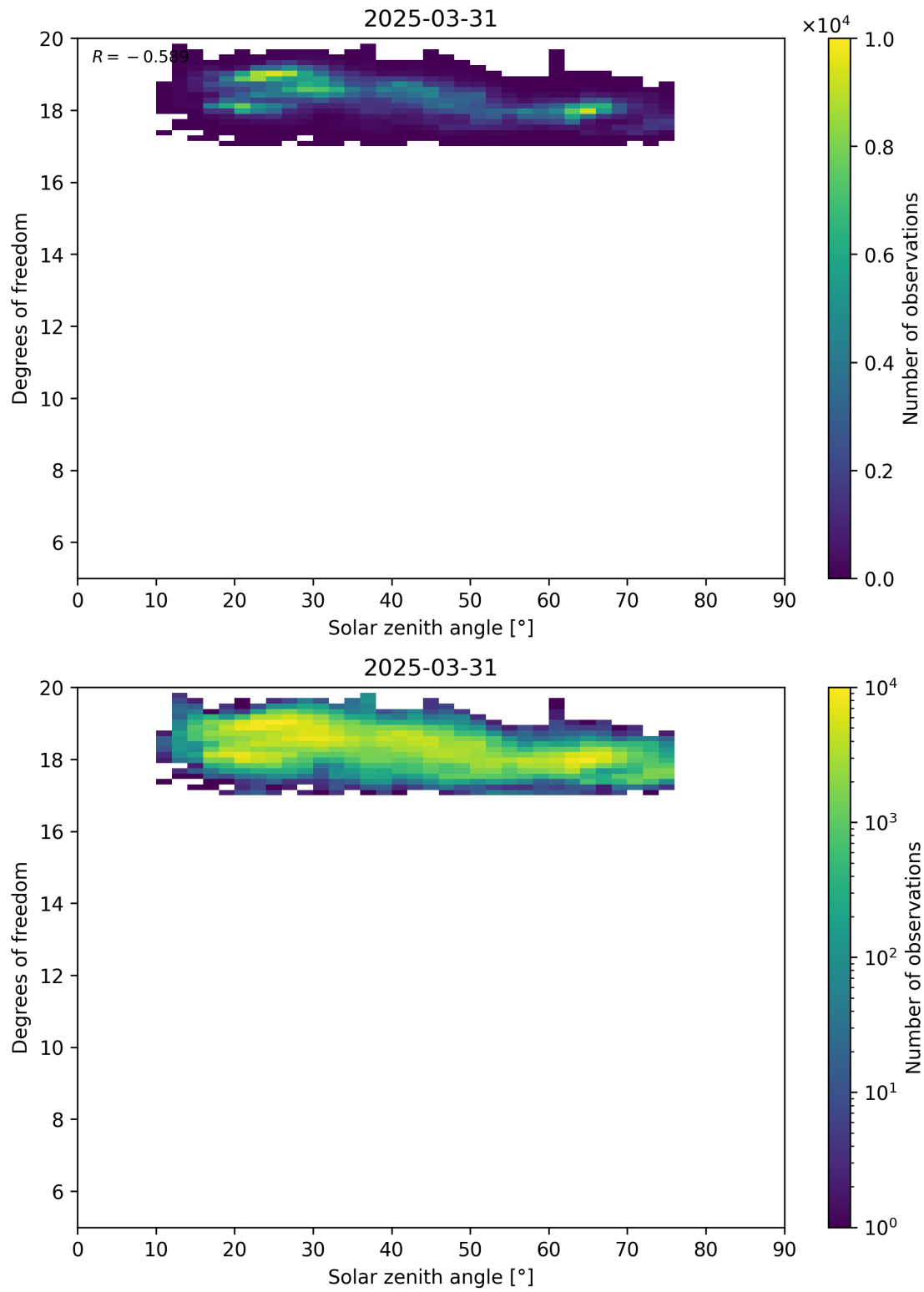
Figure 96: Scatter density plot of “Solar zenith angle” against “Degrees of freedom” for 2025-03-30 to 2025-04-01.
