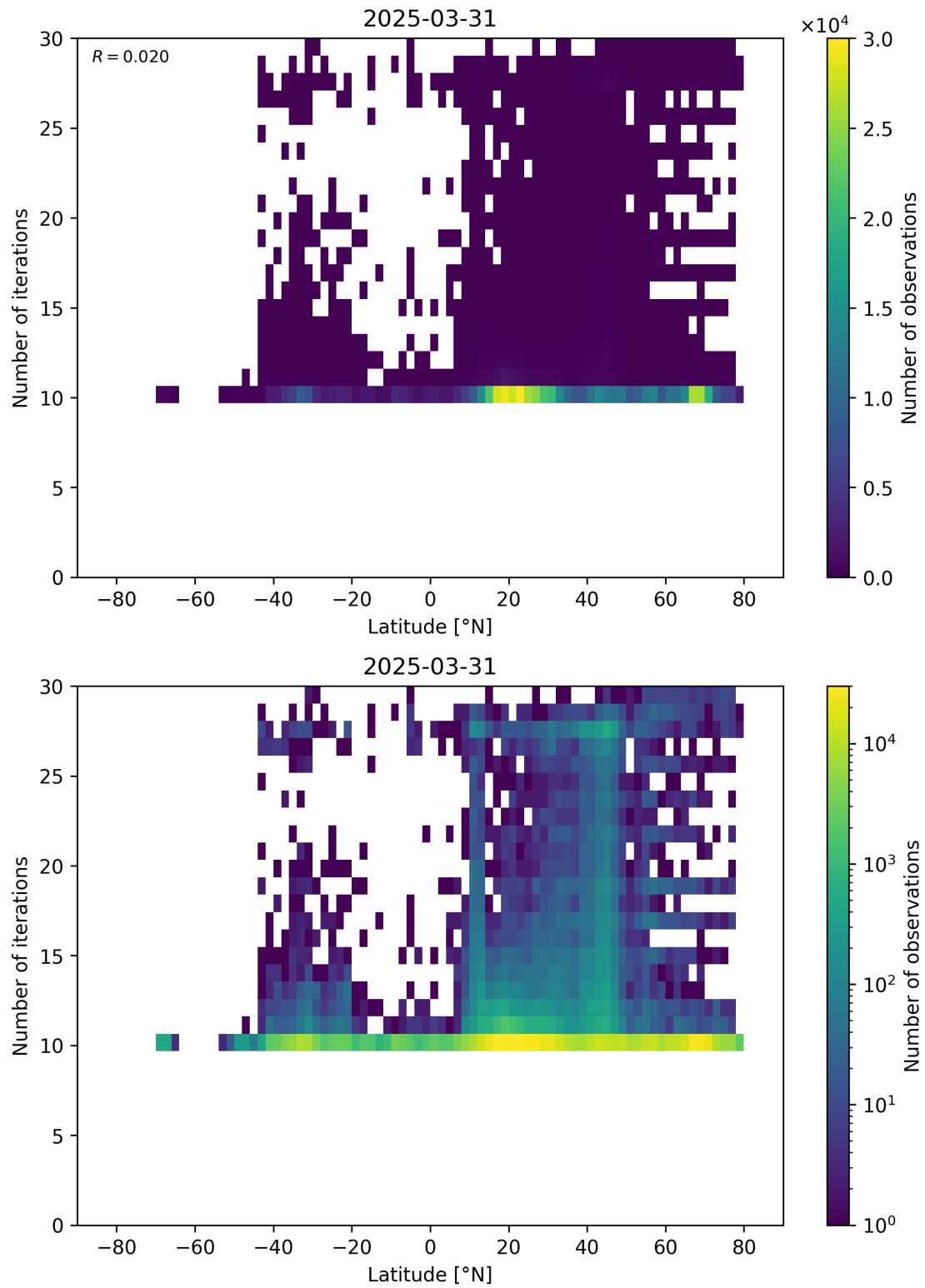
Figure 60: Scatter density plot of “Latitude” against “Number of iterations” for 2025-03-30 to 2025-04-01.
