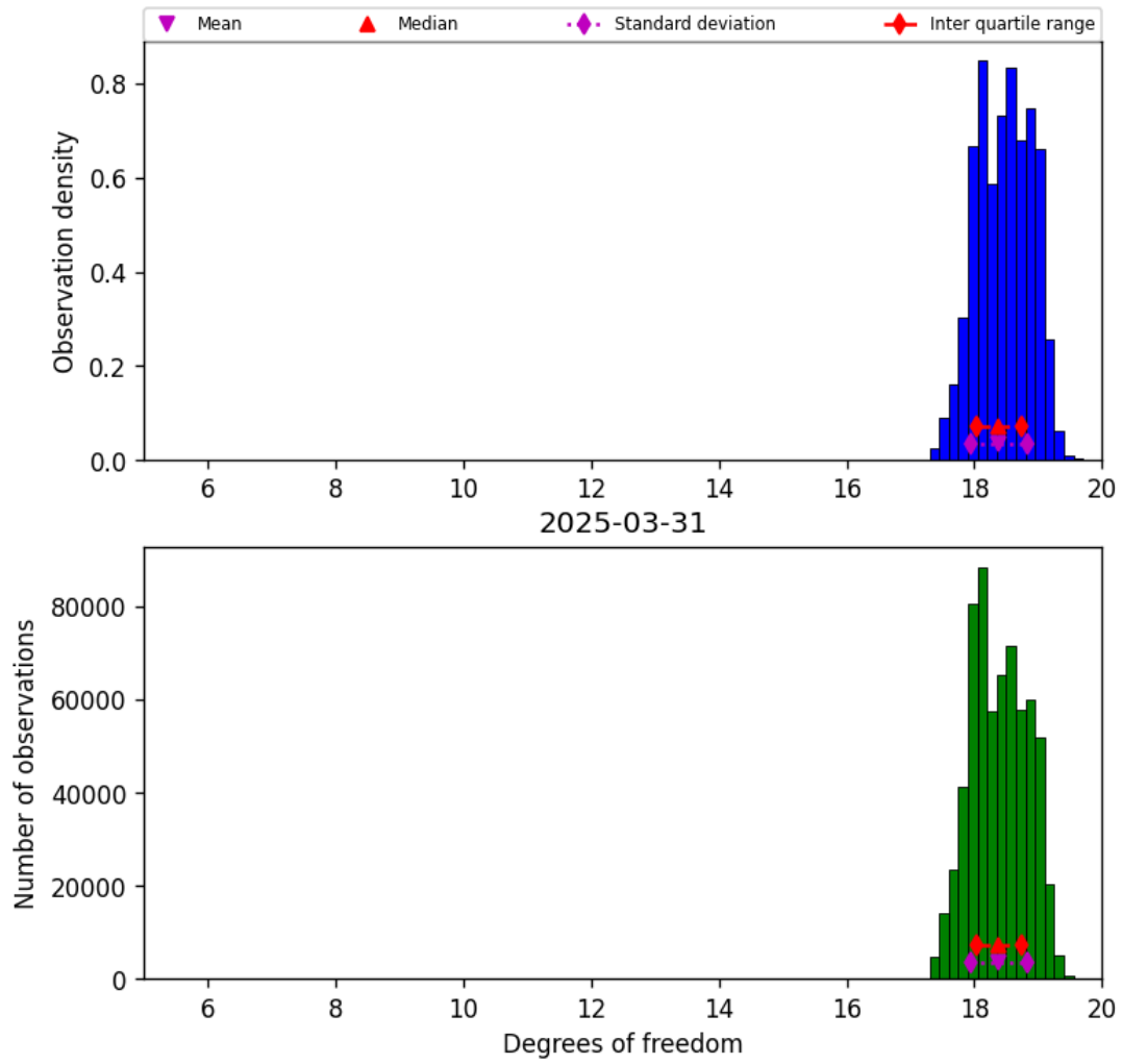
Figure 30: Histogram of “Degrees of freedom” for 2025-03-30 to 2025-04-01
