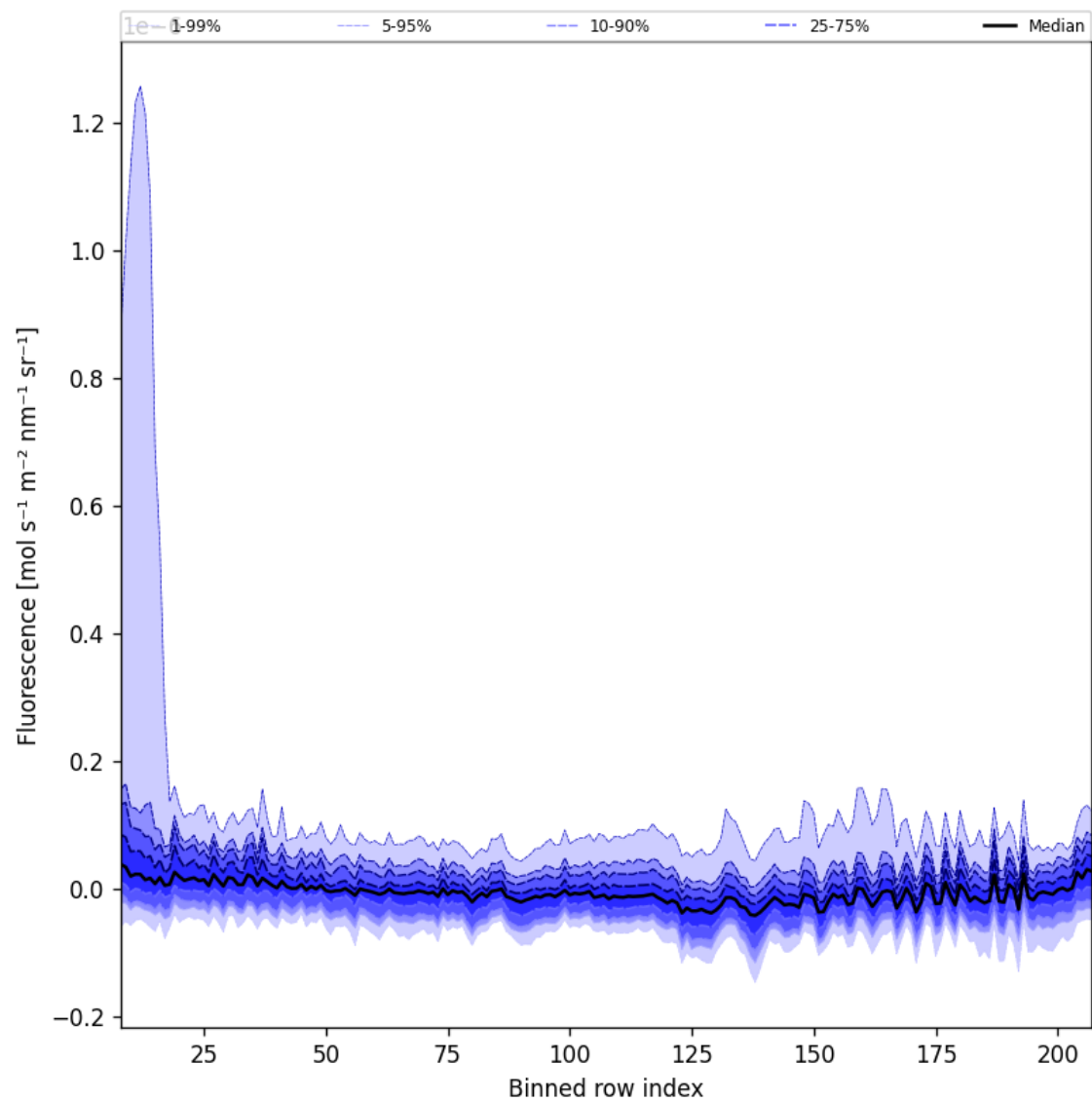
Figure 43: Along track statistics of “Fluorescence” for 2025-03-30 to 2025-04-01
