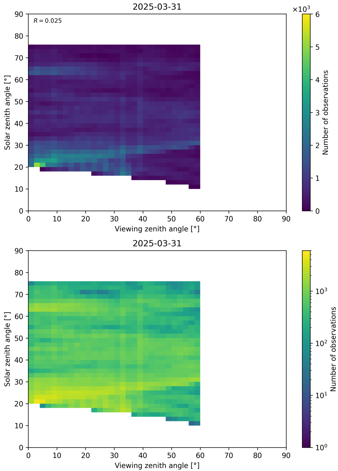
Figure 115: Scatter density plot of “Viewing zenith angle” against “Solar zenith angle” for 2025-03-30 to 2025-04-01.
