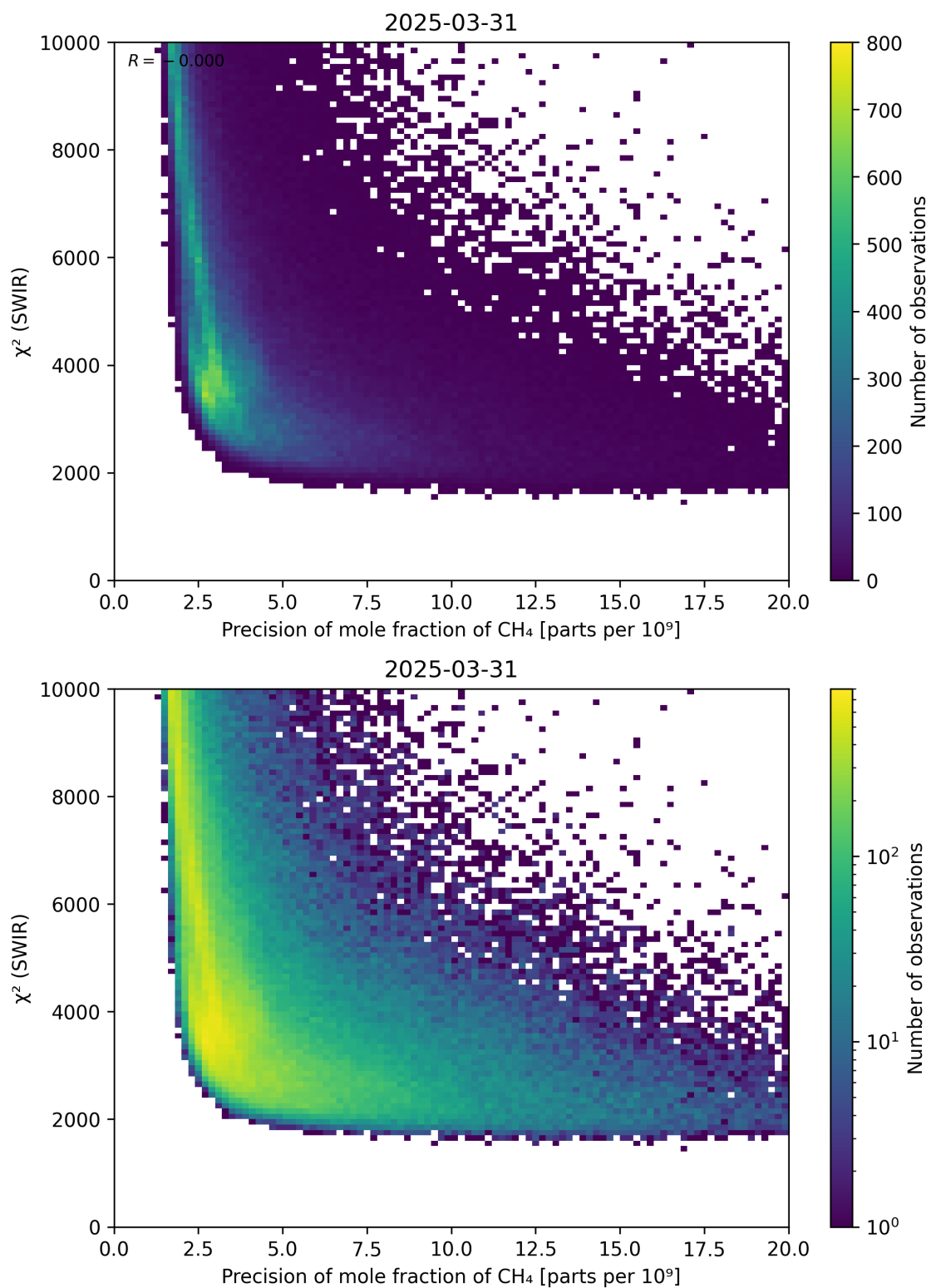
Figure 79: Scatter density plot of “Precision of mole fraction of \text{CH}_4 ” against “ \chi^2 (SWIR)” for 2025-03-30 to 2025-04-01.
