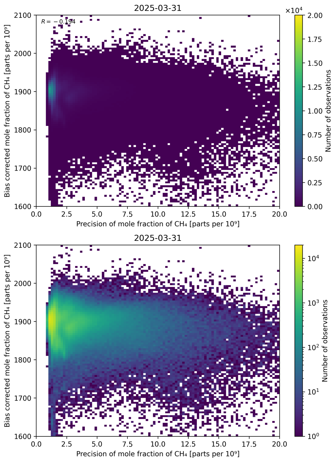
Figure 82: Scatter density plot of “Precision of mole fraction of CH 4 ” against “Bias corrected mole fraction of CH 4 ” for 2025-03-30 to 2025-04-01.
