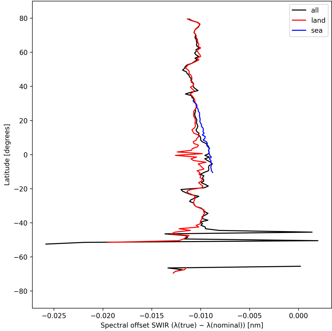
Figure 16: Zonal average of “Spectral offset SWIR ( \lambda_{\text{true}} - \lambda_{\text{nominal}} )” for 2025-03-30 to 2025-04-01.
