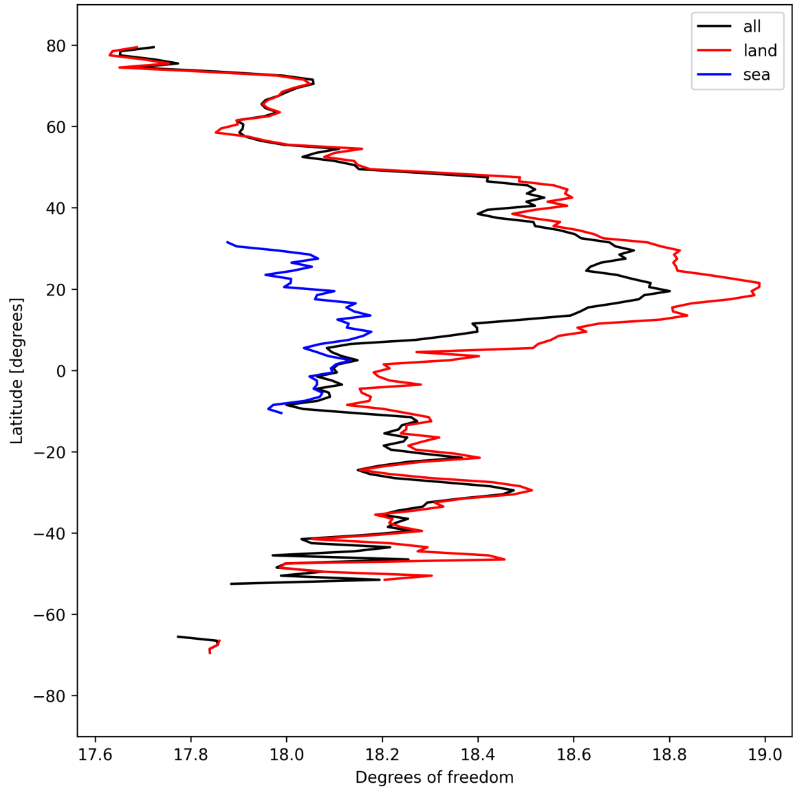
Figure 19: Zonal average of “Degrees of freedom” for 2025-03-30 to 2025-04-01.
