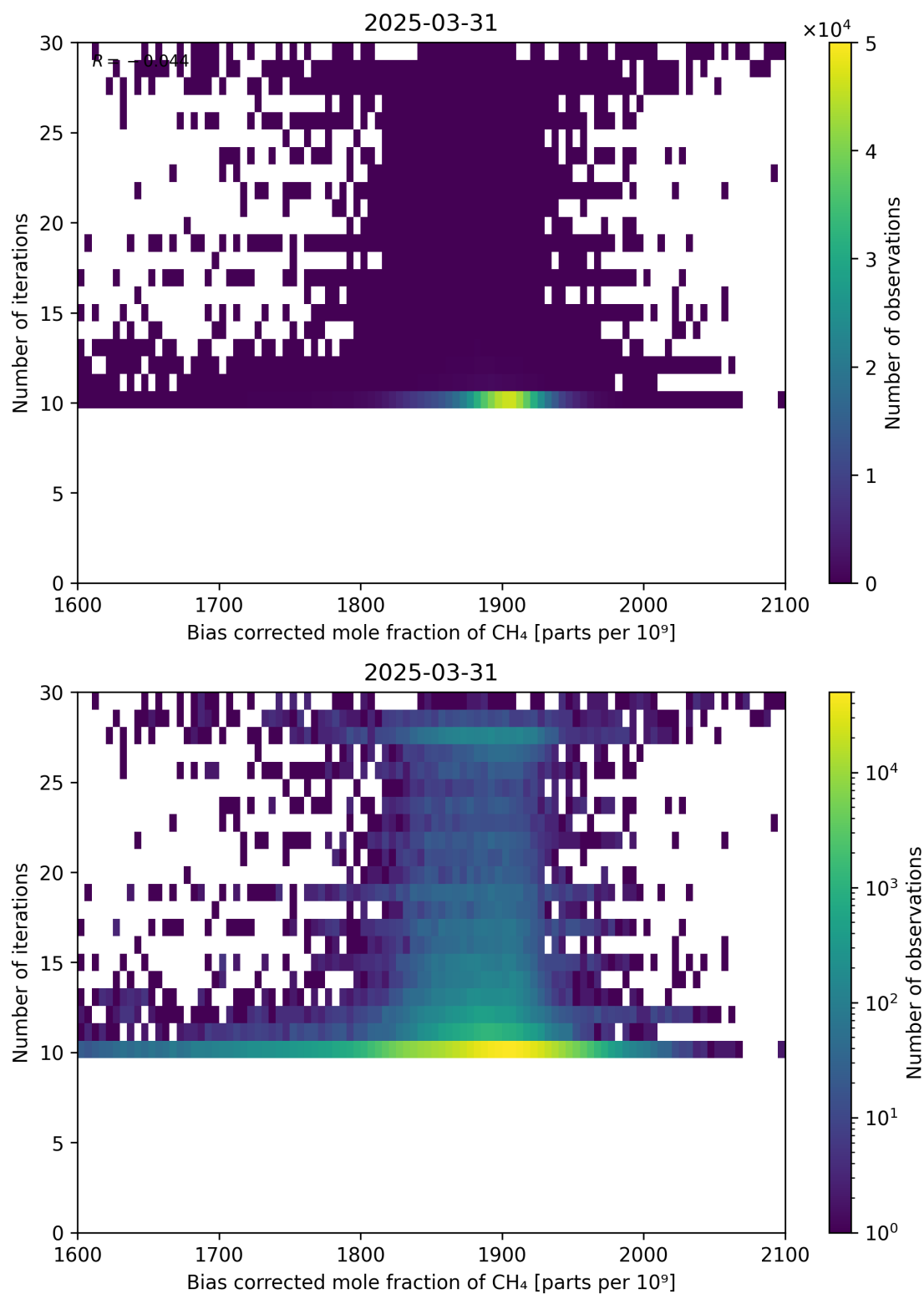
Figure 67: Scatter density plot of “Bias corrected mole fraction of \text{CH}_4 ” against “Number of iterations” for 2025-03-30 to 2025-04-01.
