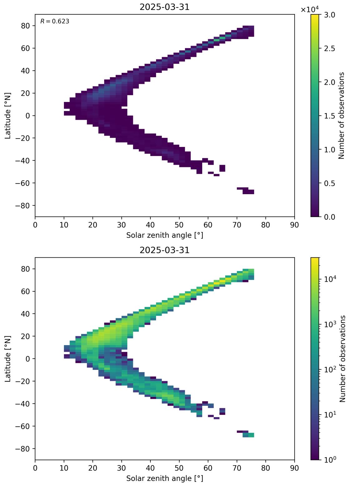
Figure 98: Scatter density plot of “Solar zenith angle” against “Latitude” for 2025-03-30 to 2025-04-01.
