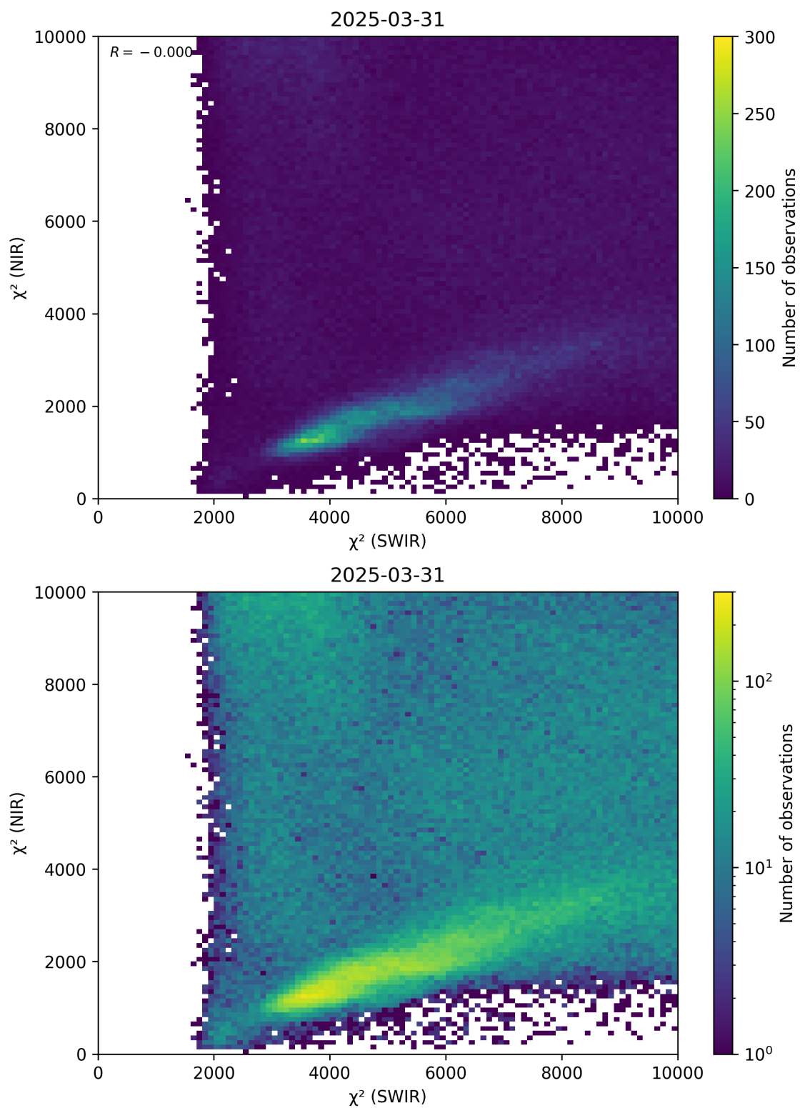
Figure 47: Scatter density plot of “ \chi^2 (SWIR)” against “ \chi^2 (NIR)” for 2025-03-30 to 2025-04-01.
