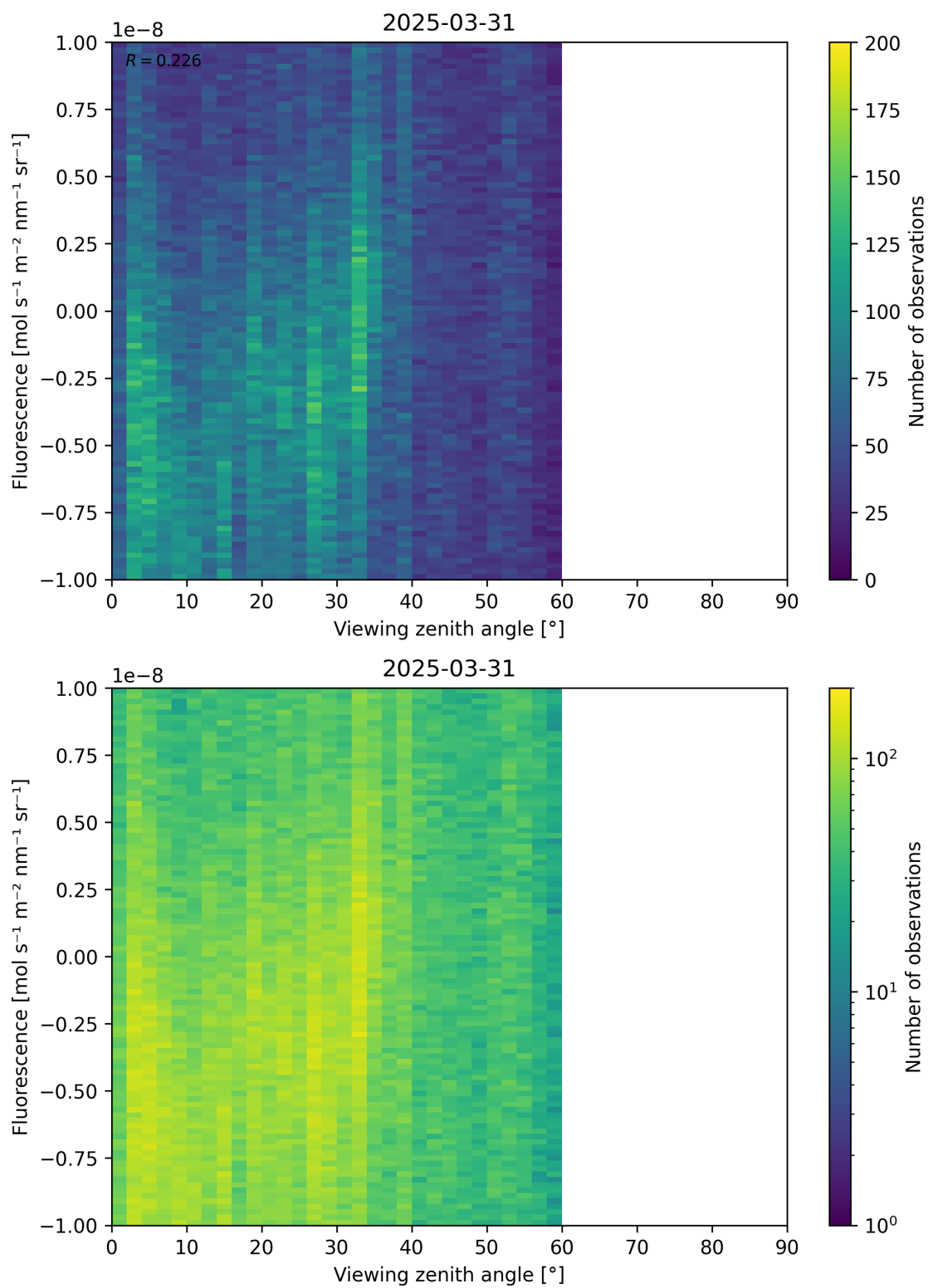
Figure 108: Scatter density plot of “Viewing zenith angle” against “Fluorescence” for 2025-03-30 to 2025-04-01.
