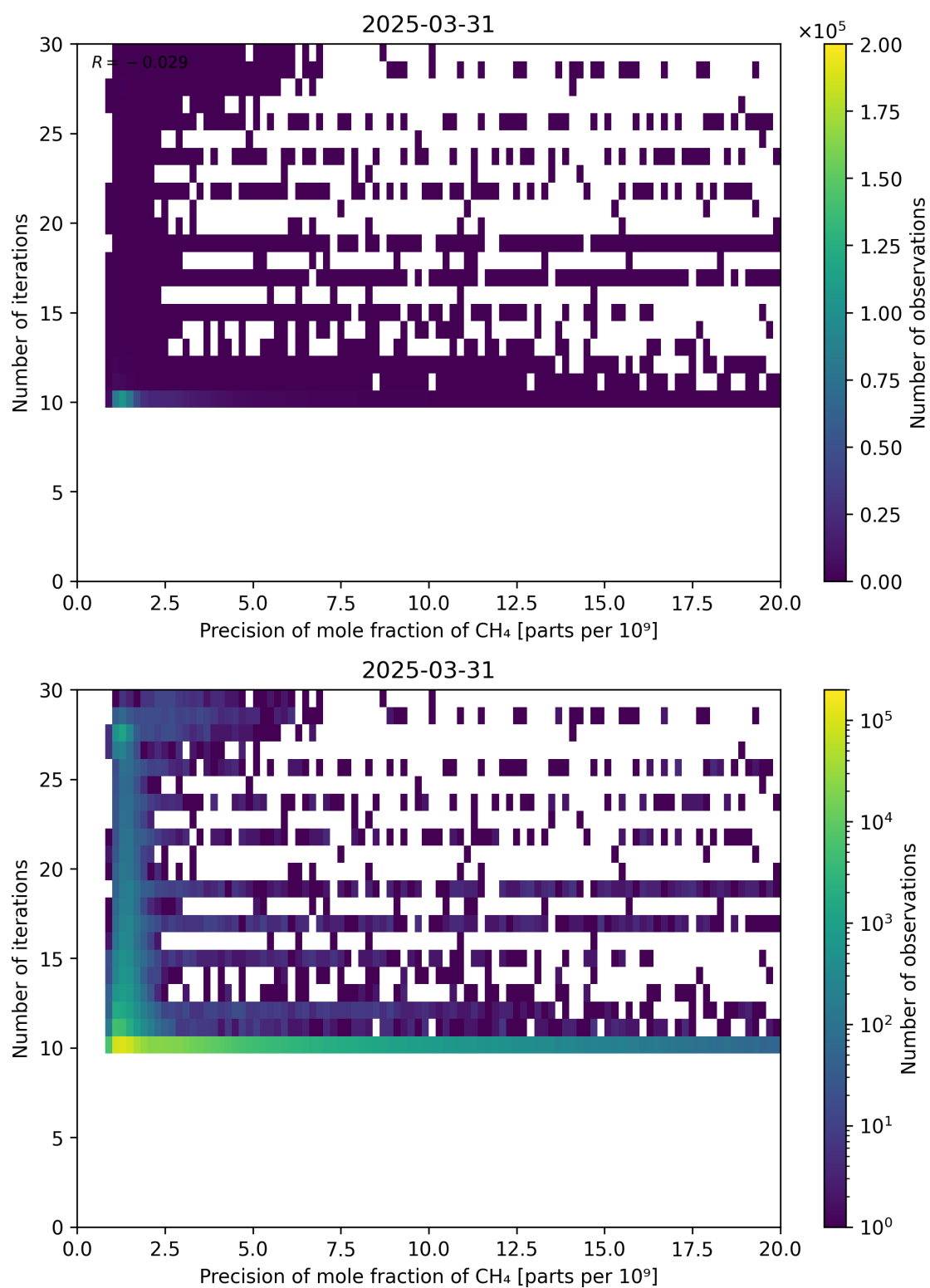
Figure 83: Scatter density plot of “Precision of mole fraction of CH 4 ” against “Number of iterations” for 2025-03-30 to 2025-04-01.
