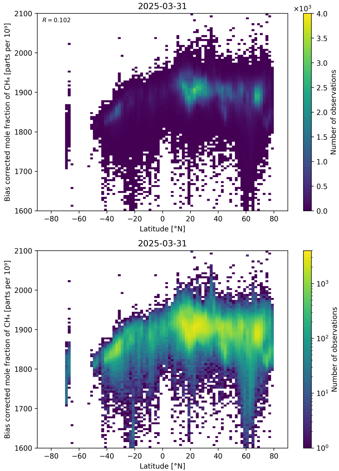
Figure 58: Scatter density plot of “Latitude” against “Bias corrected mole fraction of CH 4 ” for 2025-03-30 to 2025-04-01.
