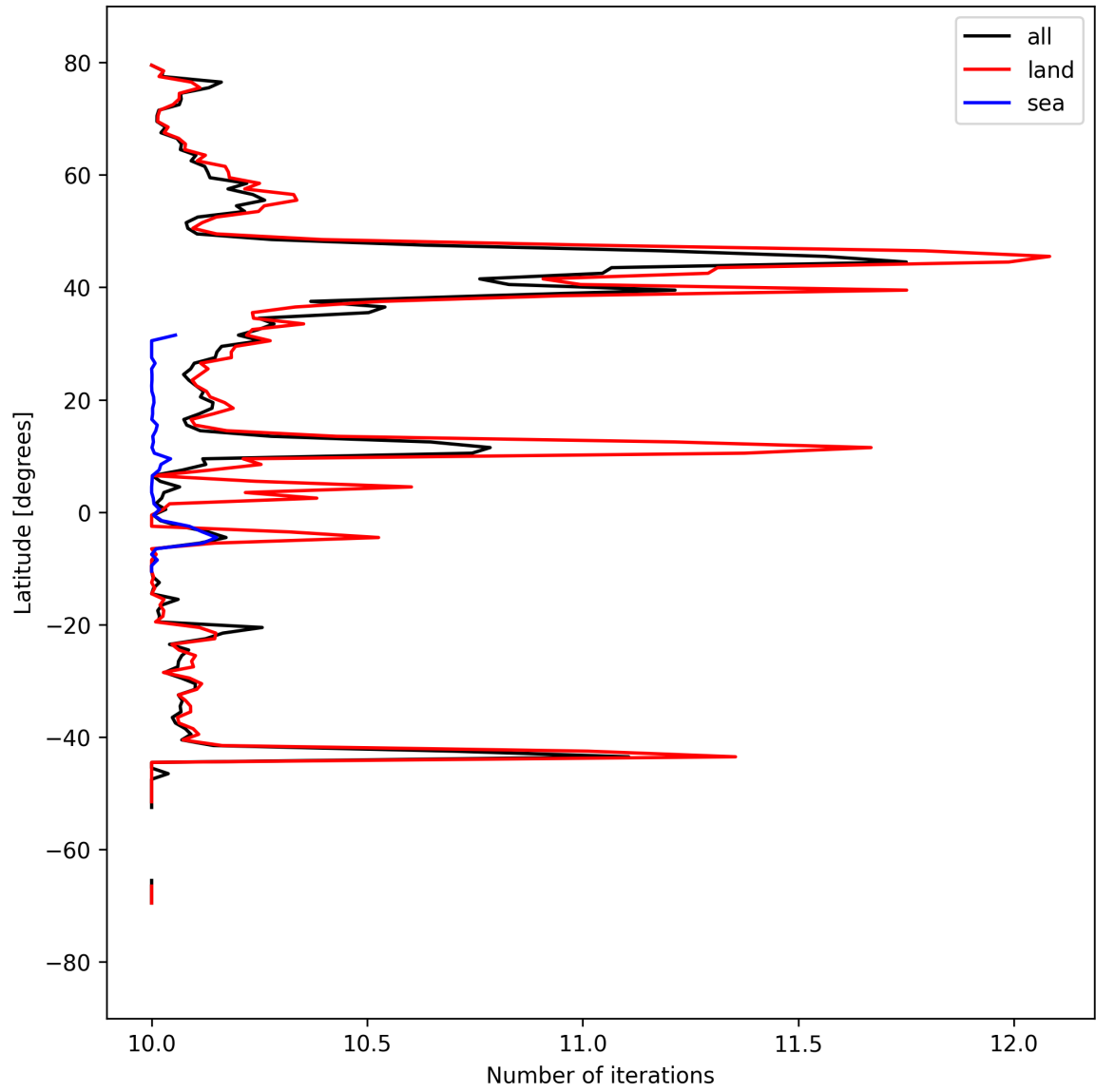
Figure 20: Zonal average of “Number of iterations” for 2025-03-30 to 2025-04-01.
