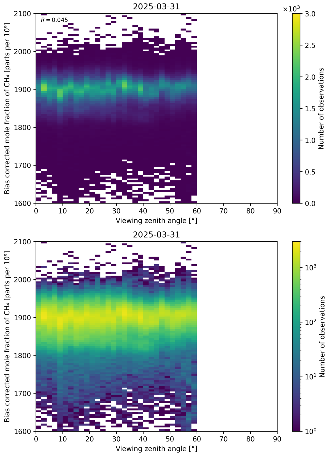
Figure 111: Scatter density plot of “Viewing zenith angle” against “Bias corrected mole fraction of CH 4 ” for 2025-03-30 to 2025-04-01.
