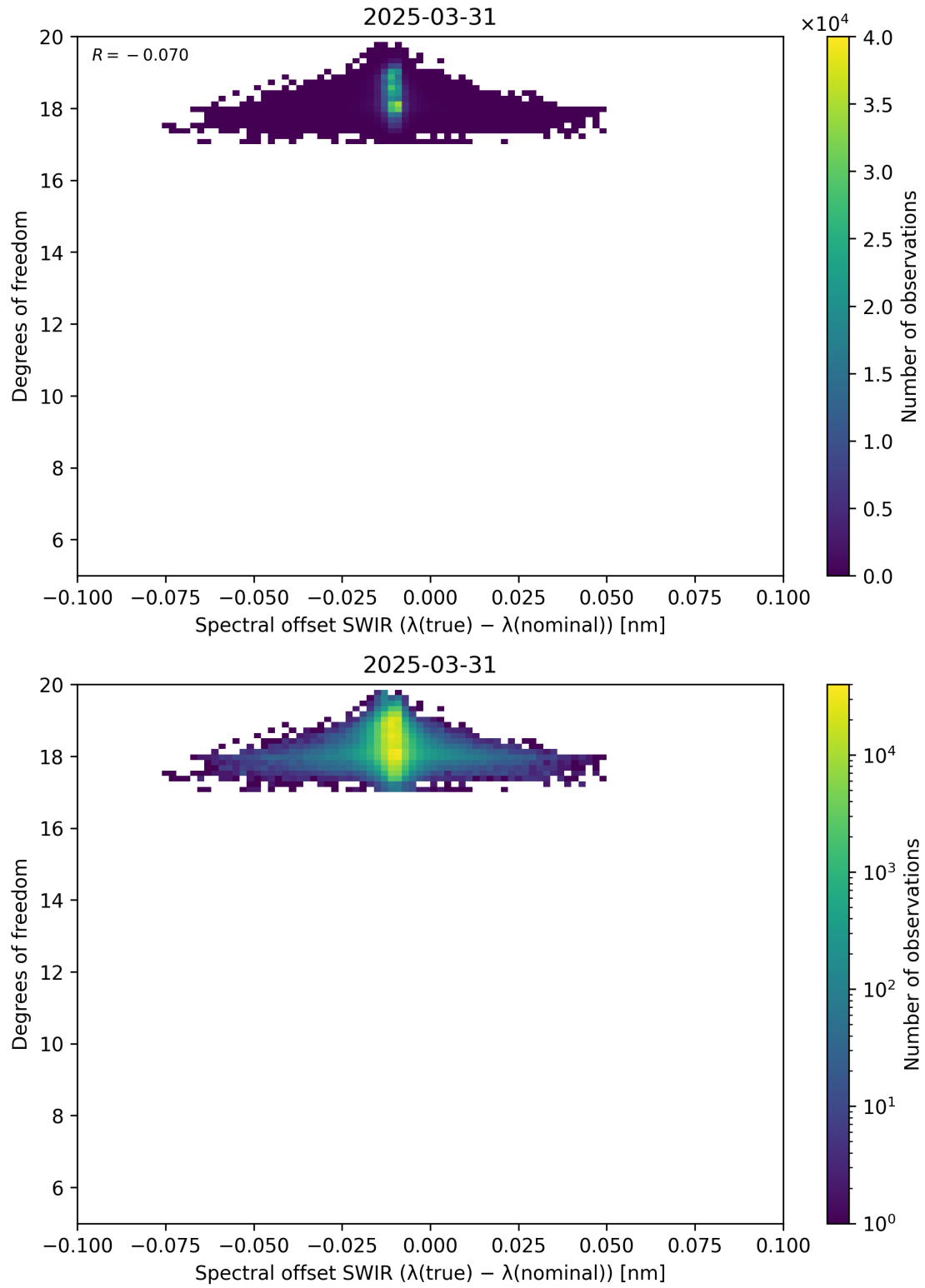
Figure 119: Scatter density plot of “Spectral offset SWIR ( \lambda_{\text{true}} - \lambda_{\text{nominal}} )” against “Degrees of freedom” for 2025-03-30 to 2025-04-01.
