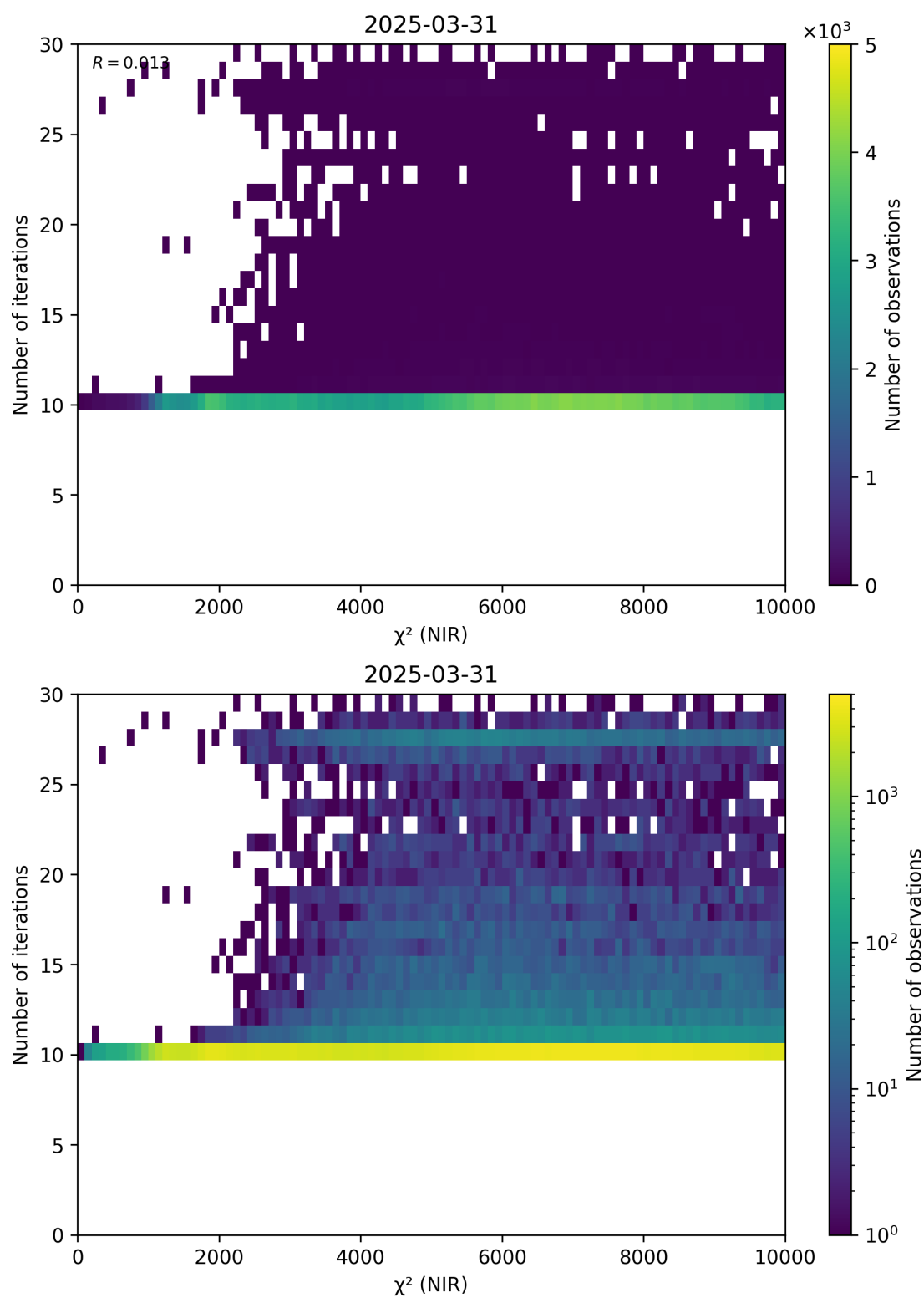
Figure 46: Scatter density plot of “ \chi^2 (NIR)” against “Number of iterations” for 2025-03-30 to 2025-04-01.
