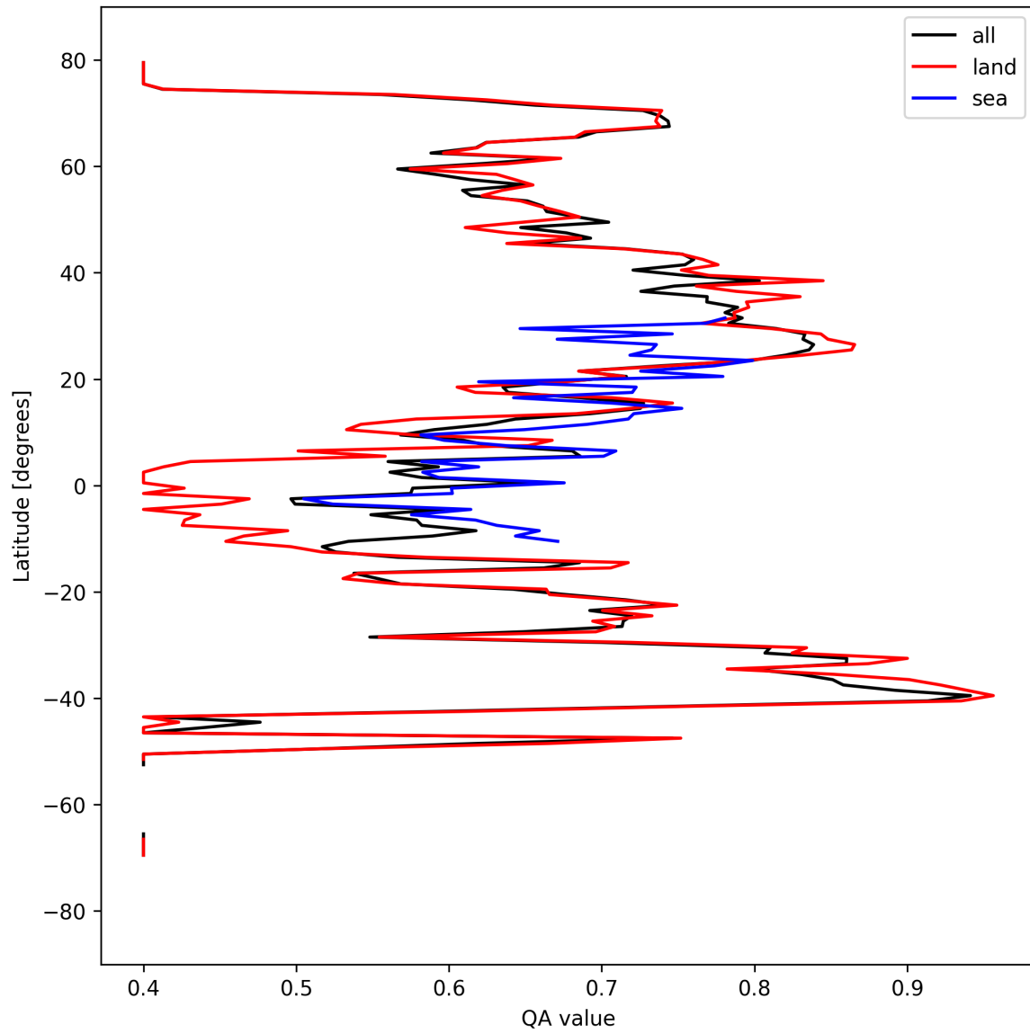
Figure 11: Zonal average of “QA value” for 2025-03-30 to 2025-04-01.
