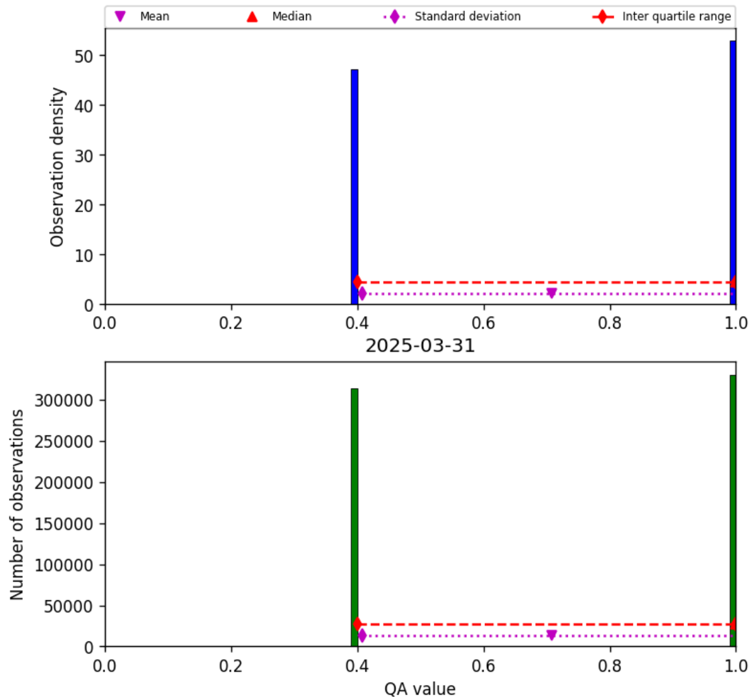
Figure 22: Histogram of “QA value” for 2025-03-30 to 2025-04-01
