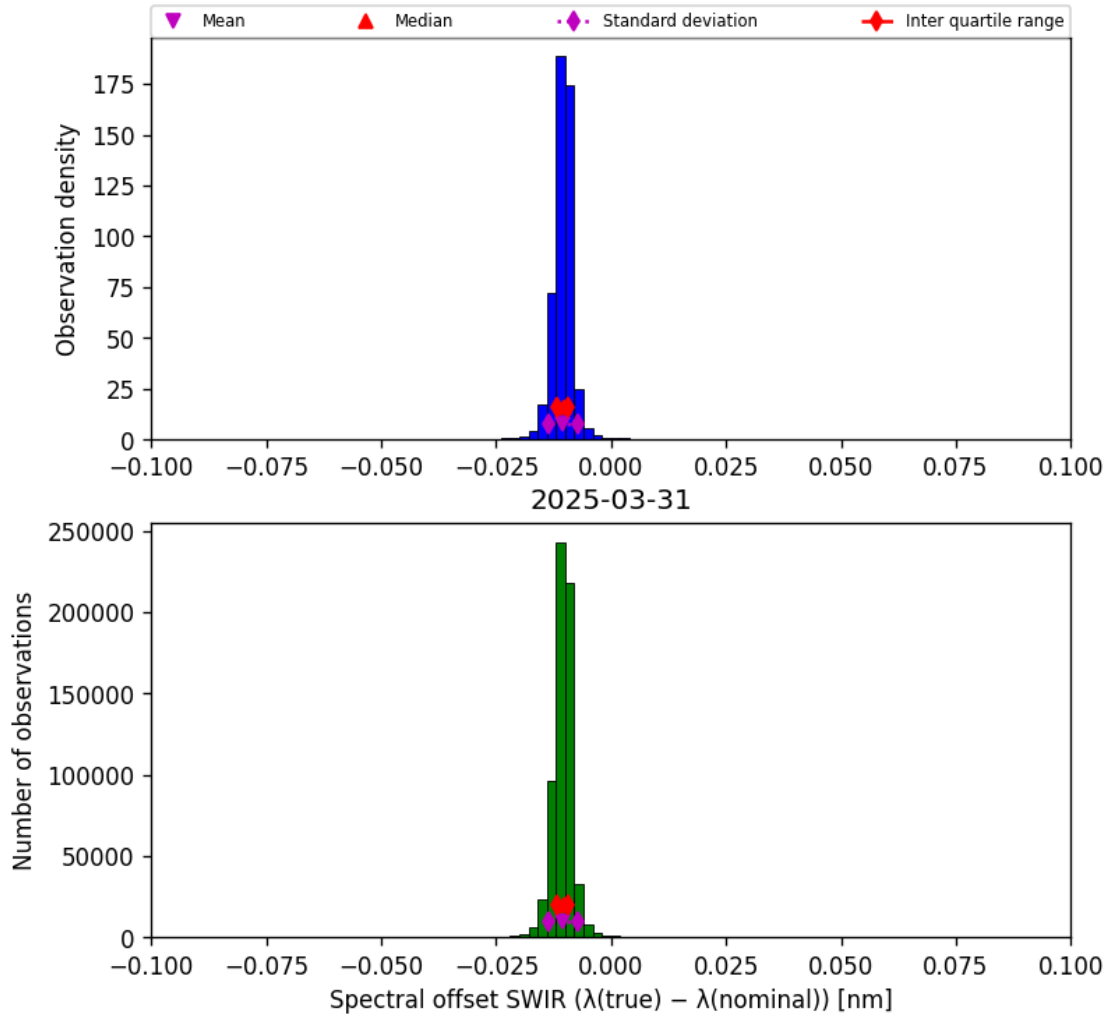
Figure 27: Histogram of “Spectral offset SWIR ( \lambda_{\text{true}} - \lambda_{\text{nominal}} )” for 2025-03-30 to 2025-04-01
