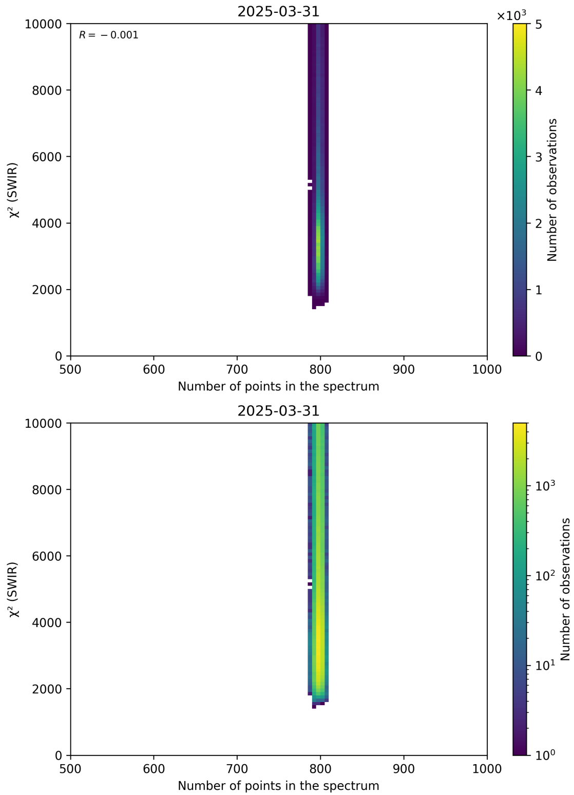
Figure 89: Scatter density plot of “Number of points in the spectrum” against “ \chi^2 (SWIR)” for 2025-03-30 to 2025-04-01.
