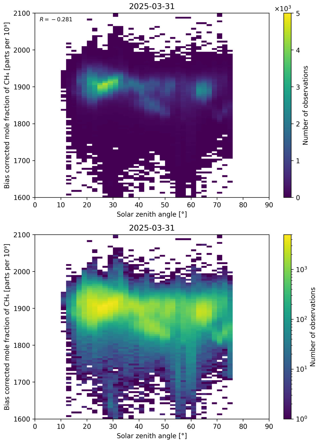
Figure 100: Scatter density plot of “Solar zenith angle” against “Bias corrected mole fraction of CH 4 ” for 2025-03-30 to 2025-04-01.
