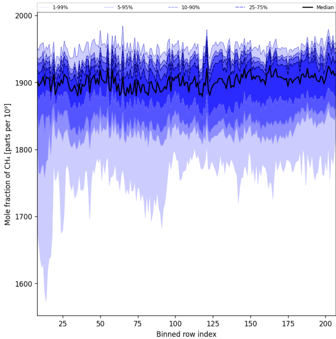
Figure 34: Along track statistics of “Mole fraction of CH 4 ” for 2025-03-30 to 2025-04-01
