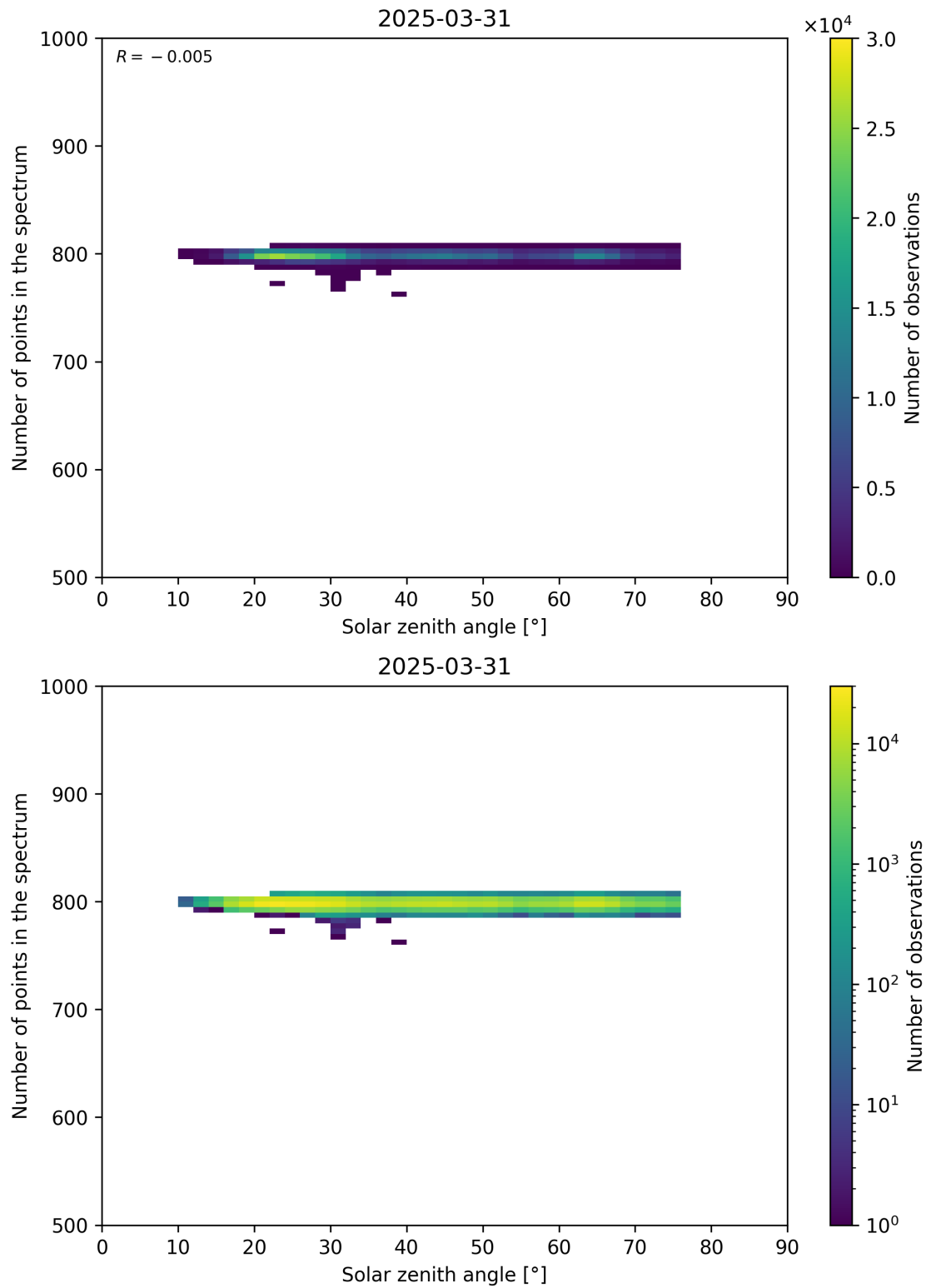
Figure 103: Scatter density plot of “Solar zenith angle” against “Number of points in the spectrum” for 2025-03-30 to 2025-04-01.
