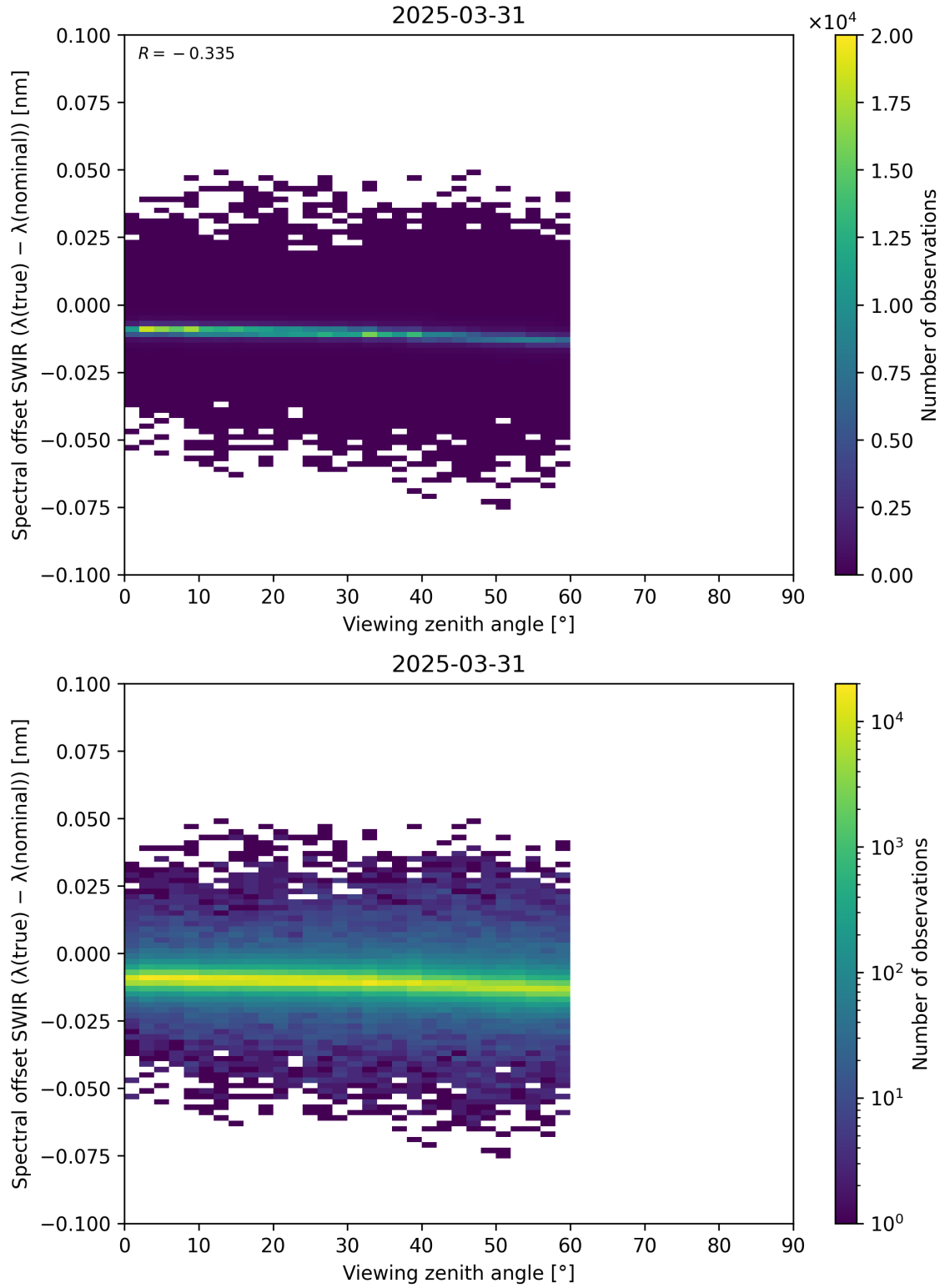
Figure 116: Scatter density plot of “Viewing zenith angle” against “Spectral offset SWIR ( \lambda_{\text{true}} - \lambda_{\text{nominal}} )” for 2025-03-30 to 2025-04-01.
