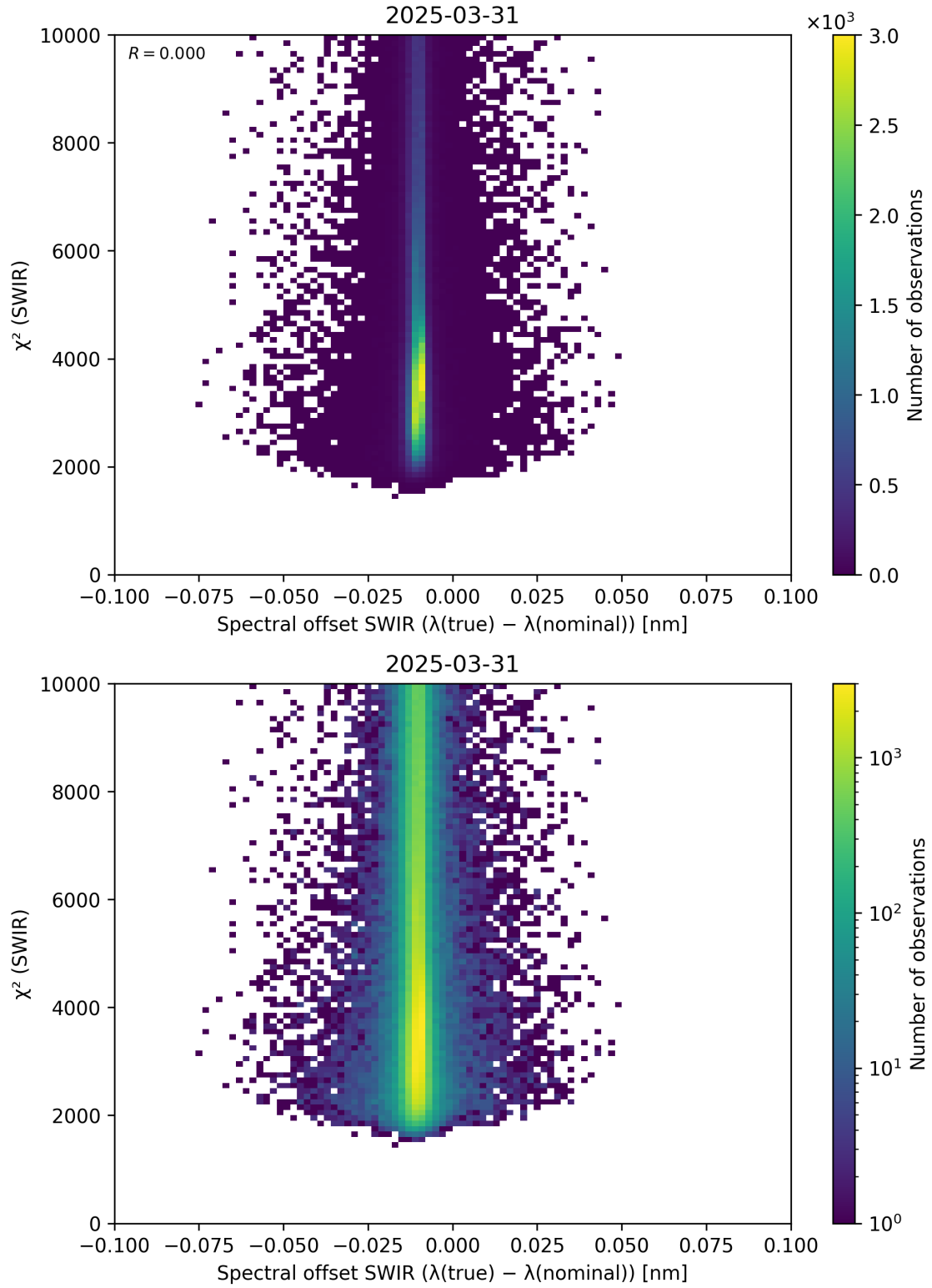
Figure 118: Scatter density plot of “Spectral offset SWIR ( \lambda_{\text{true}} - \lambda_{\text{nominal}} )” against “ \chi^2 (SWIR)” for 2025-03-30 to 2025-04-01.
