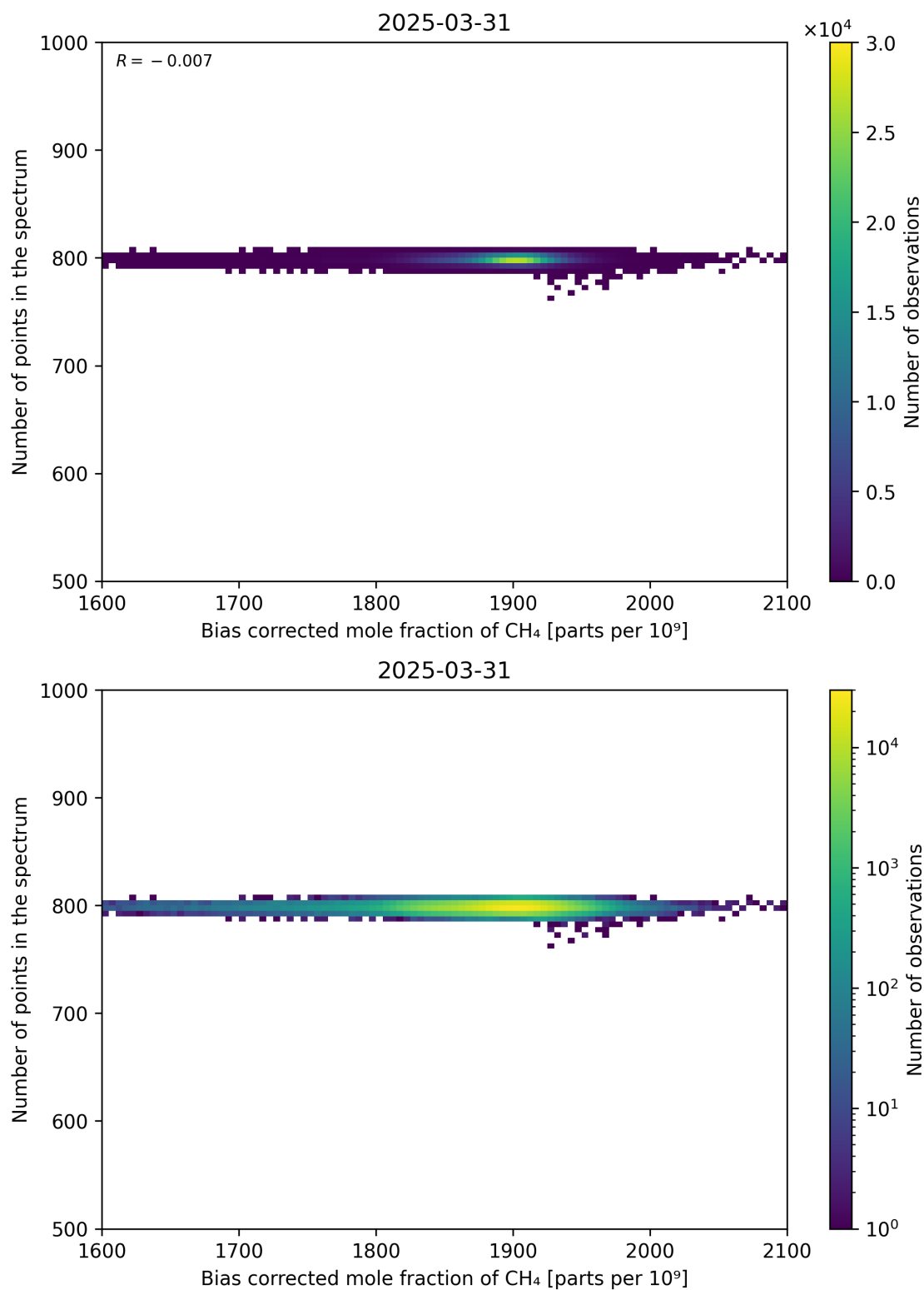
Figure 68: Scatter density plot of “Bias corrected mole fraction of CH 4 ” against “Number of points in the spectrum” for 2025-03-30 to 2025-04-01.
