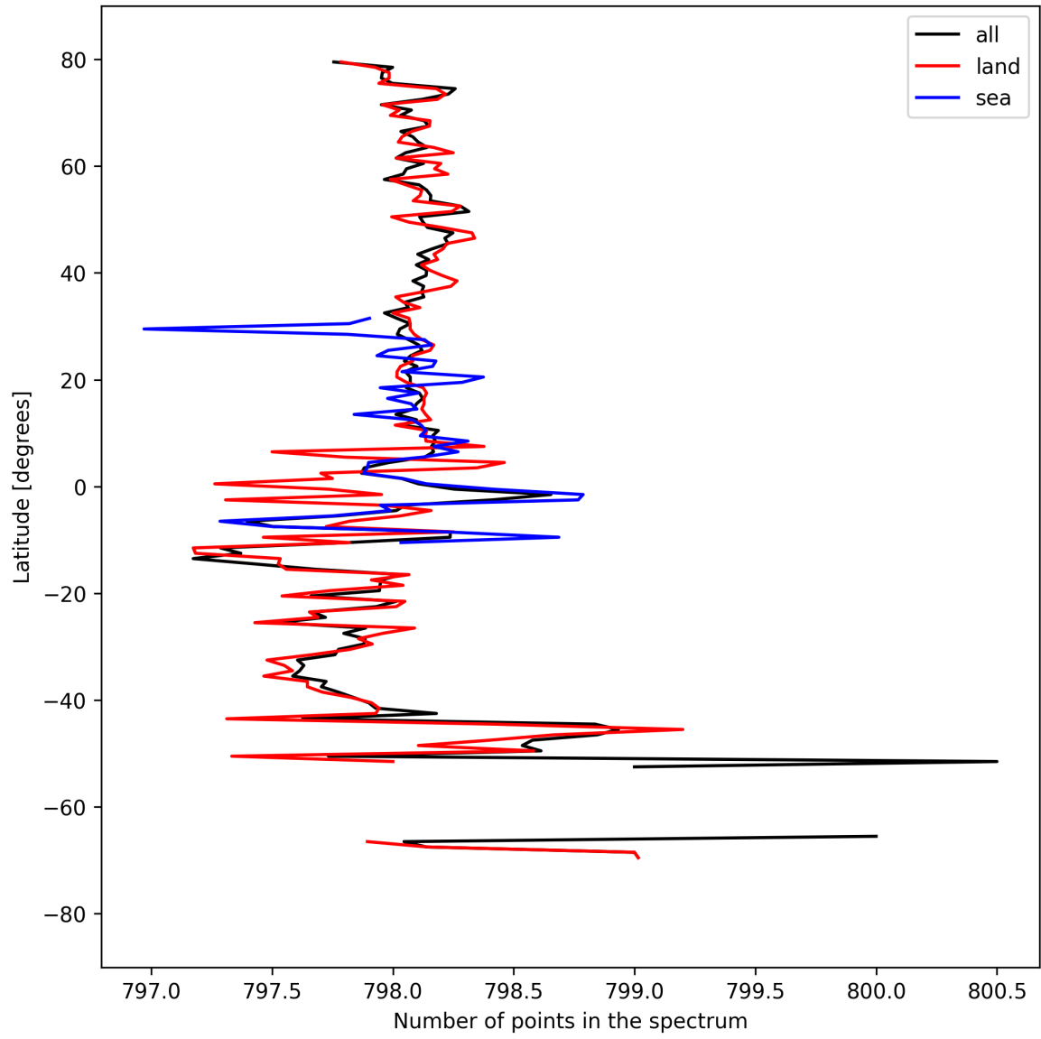
Figure 15: Zonal average of “Number of points in the spectrum” for 2025-03-30 to 2025-04-01.
