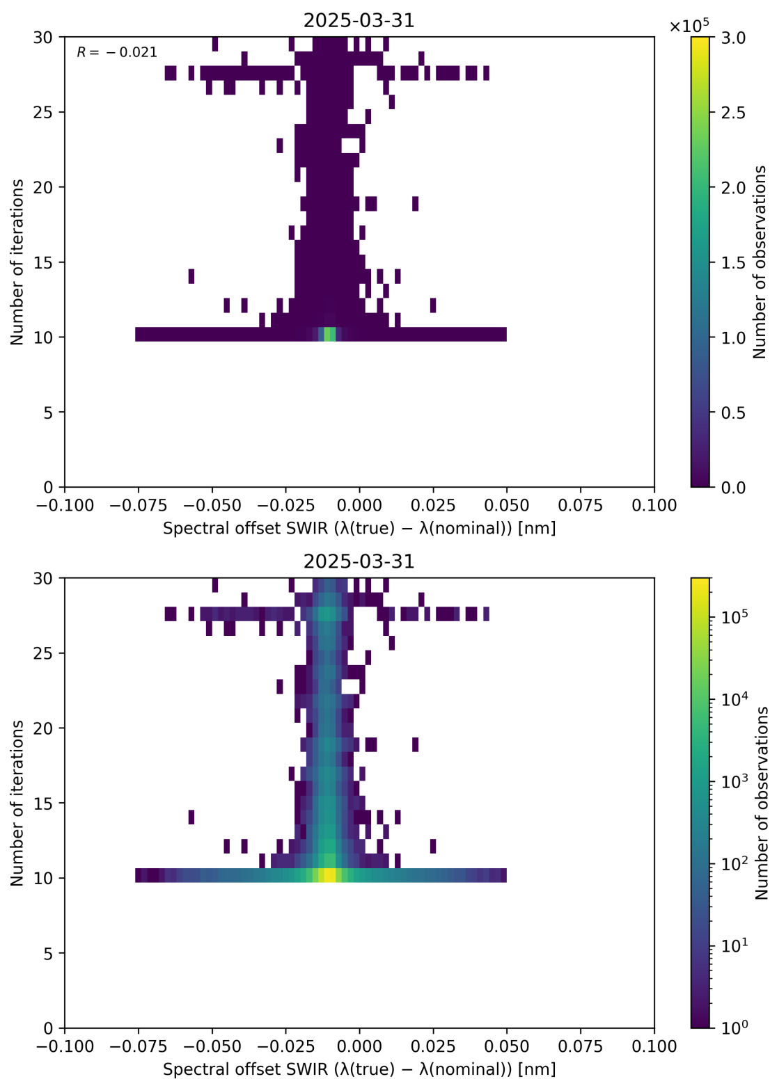
Figure 121: Scatter density plot of “Spectral offset SWIR ( \lambda_{\text{true}} - \lambda_{\text{nominal}} )” against “Number of iterations” for 2025-03-30 to 2025-04-01.
