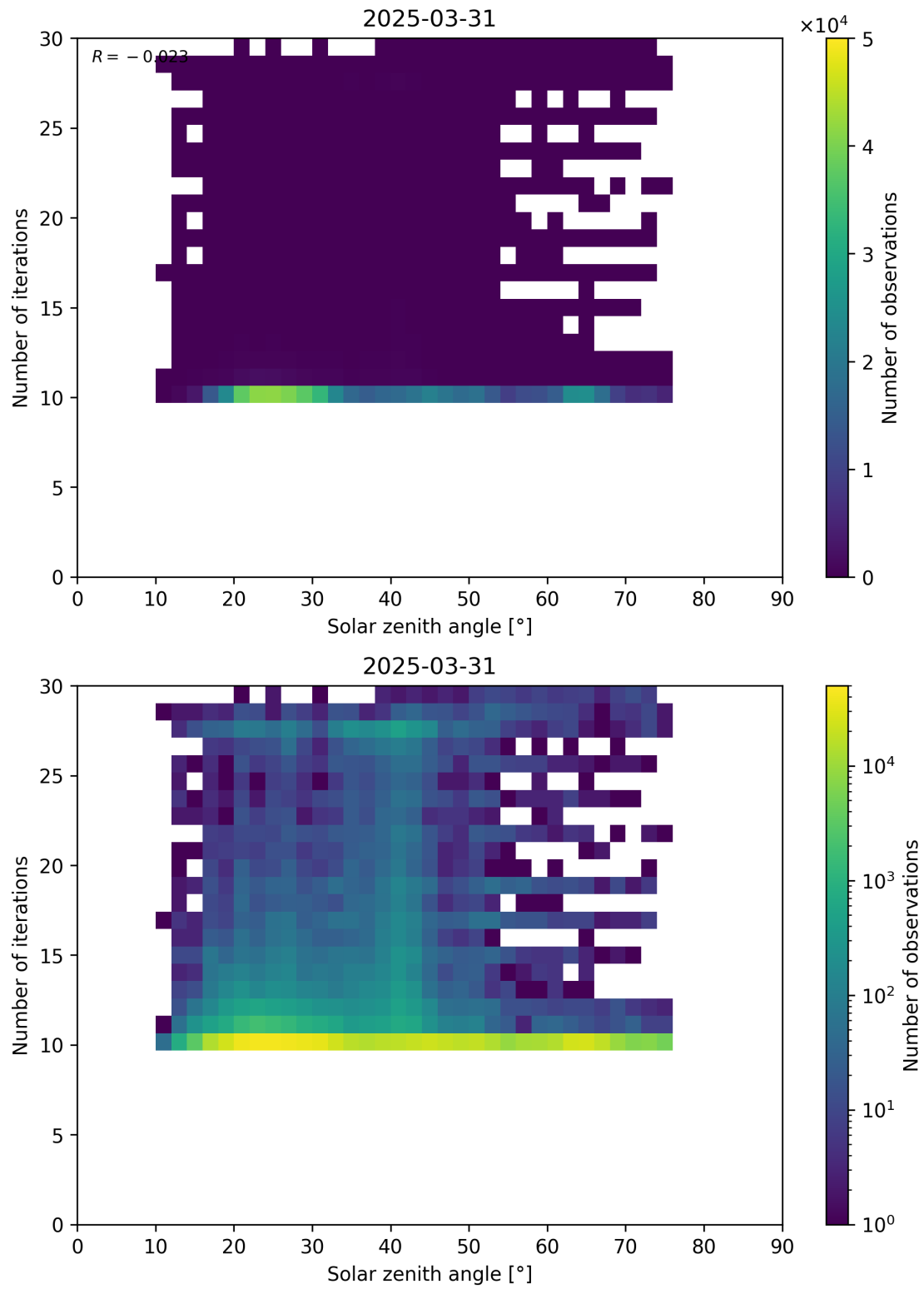
Figure 102: Scatter density plot of “Solar zenith angle” against “Number of iterations” for 2025-03-30 to 2025-04-01.
