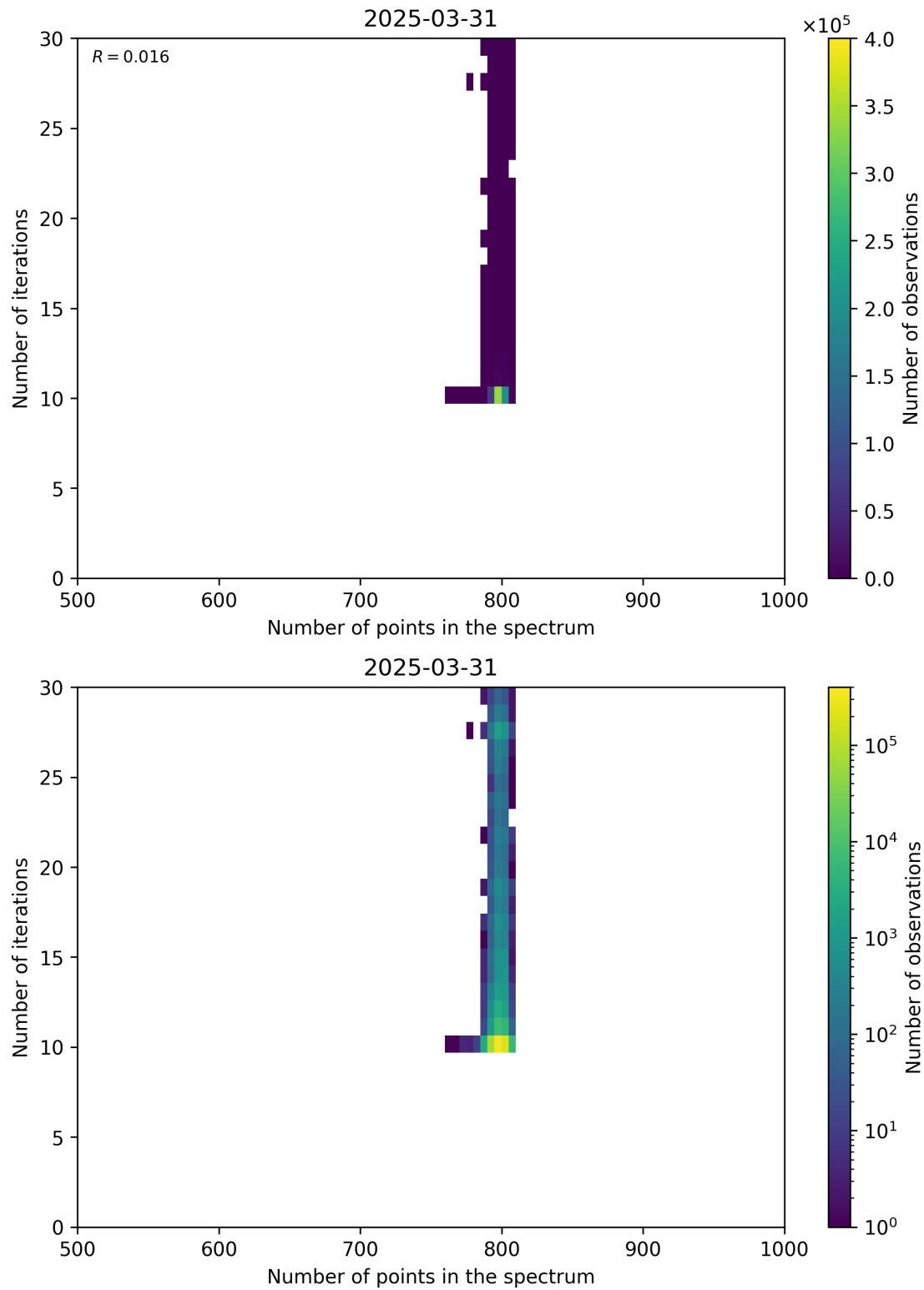
Figure 92: Scatter density plot of “Number of points in the spectrum” against “Number of iterations” for 2025-03-30 to 2025-04-01.
