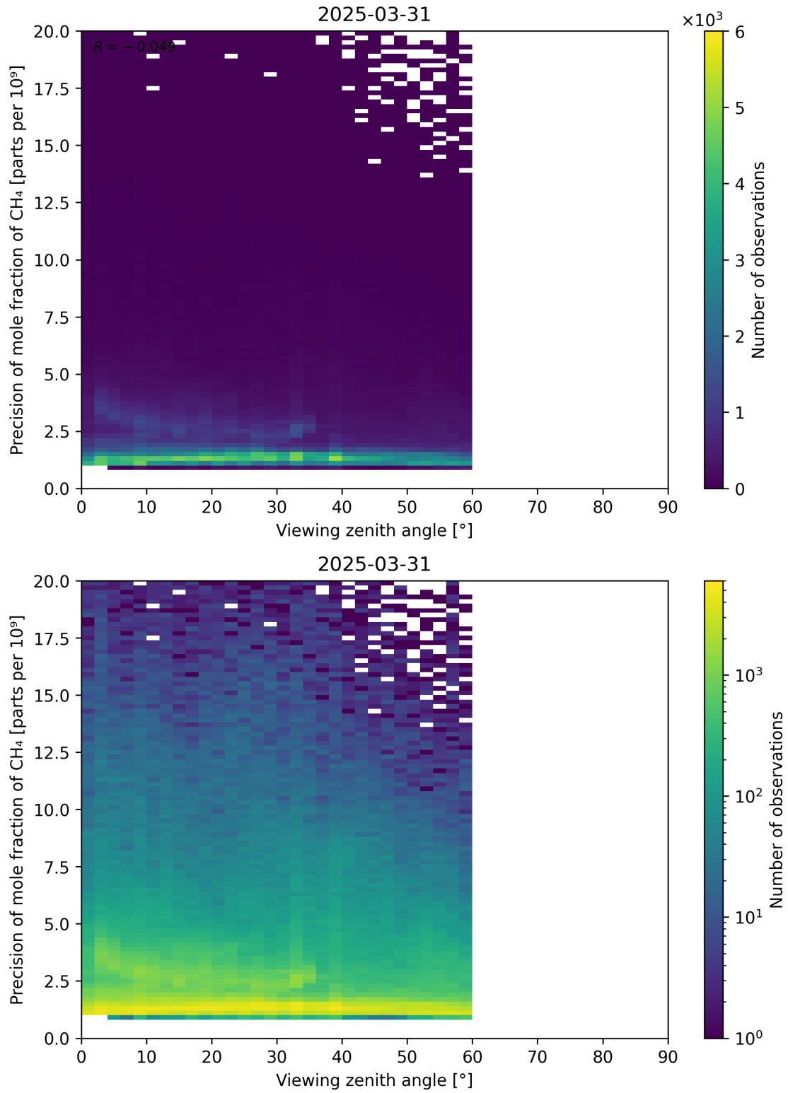
Figure 112: Scatter density plot of “Viewing zenith angle” against “Precision of mole fraction of CH 4 ” for 2025-03-30 to 2025-04-01.
