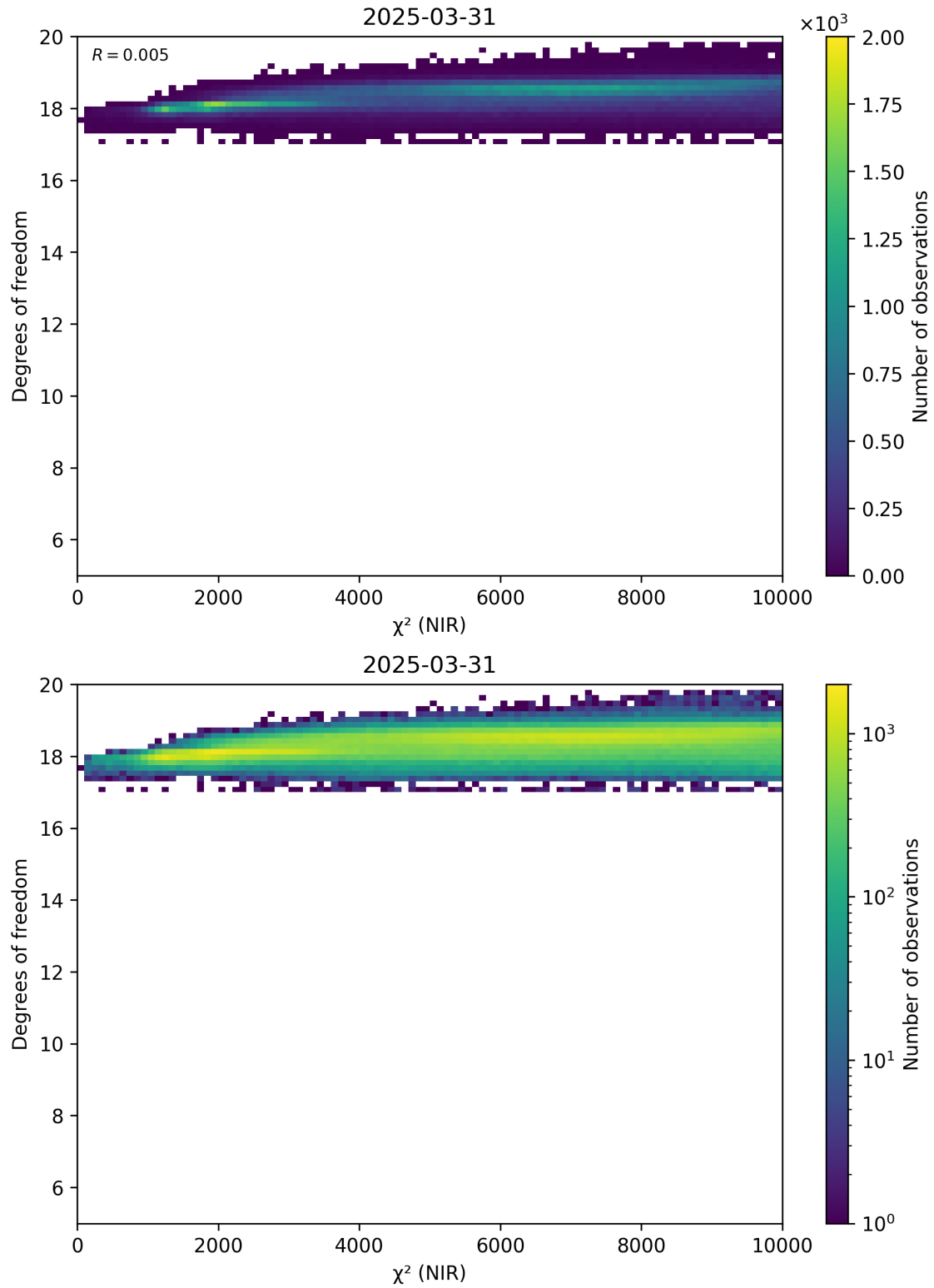
Figure 44: Scatter density plot of “ \chi^2 (NIR)” against “Degrees of freedom” for 2025-03-30 to 2025-04-01.
