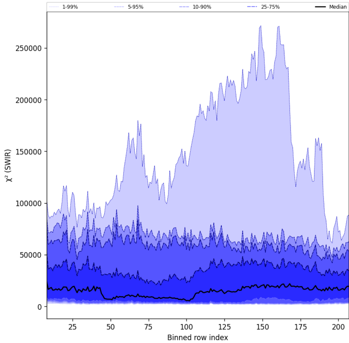
Figure 39: Along track statistics of " \chi^2 (SWIR)" for 2025-03-30 to 2025-04-01
