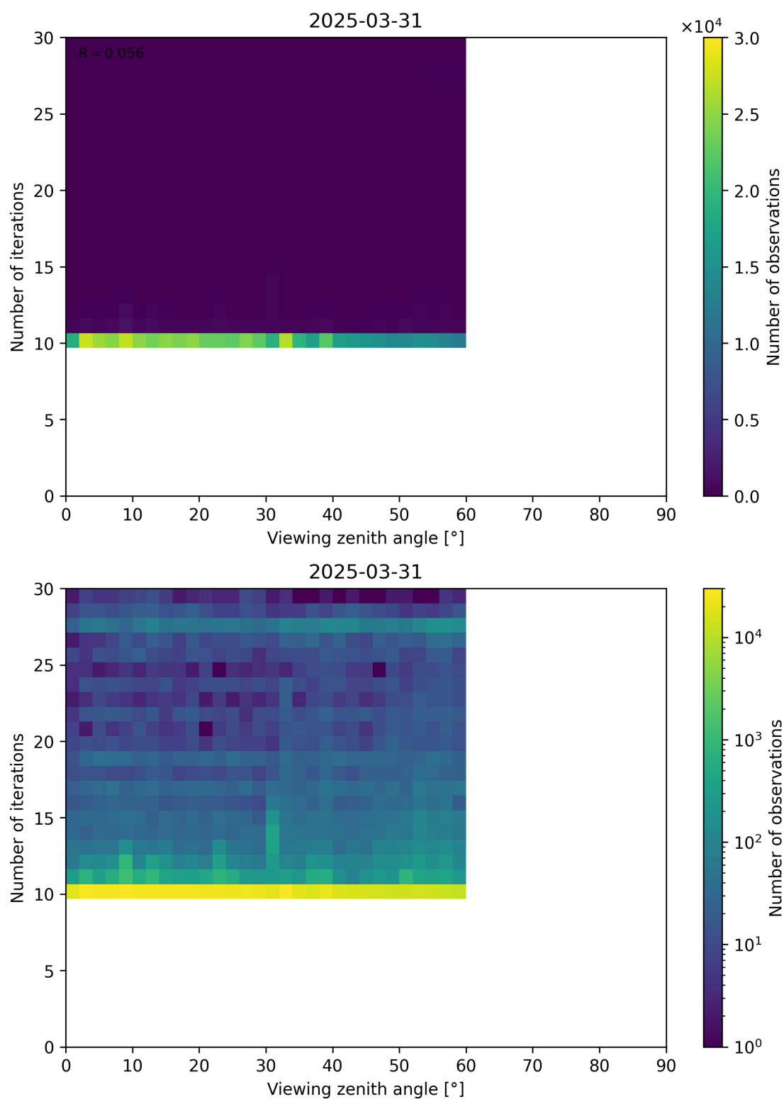
Figure 113: Scatter density plot of “Viewing zenith angle” against “Number of iterations” for 2025-03-30 to 2025-04-01.
