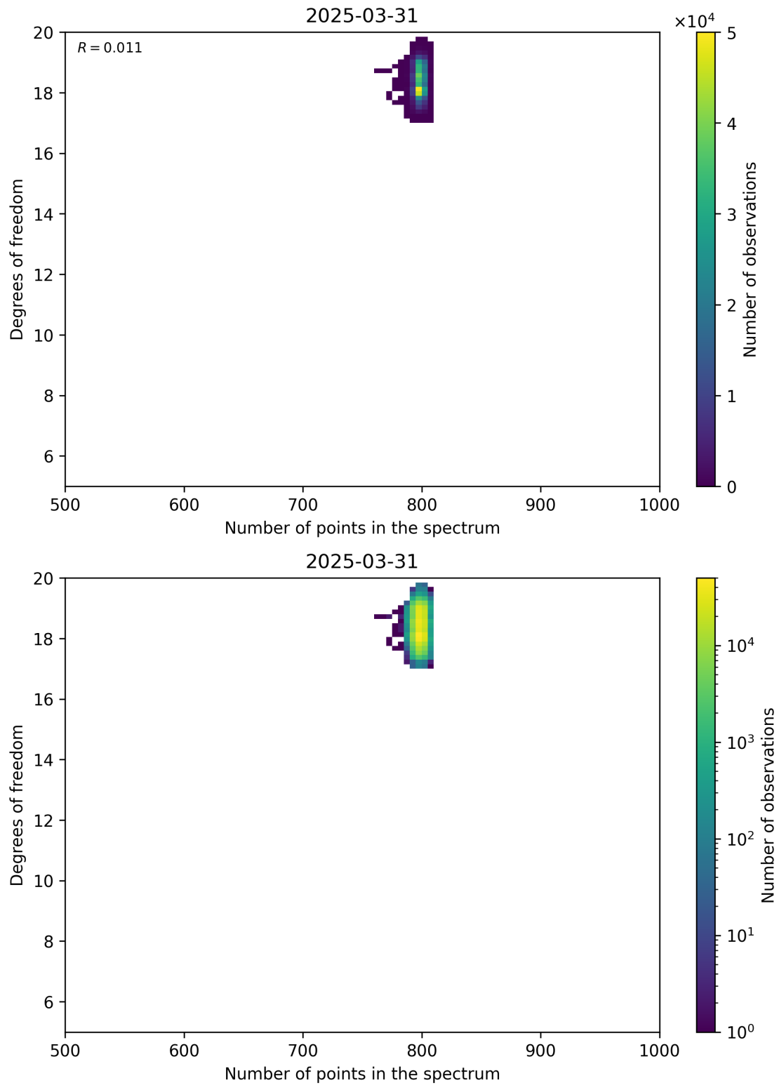
Figure 90: Scatter density plot of “Number of points in the spectrum” against “Degrees of freedom” for 2025-03-30 to 2025-04-01.
