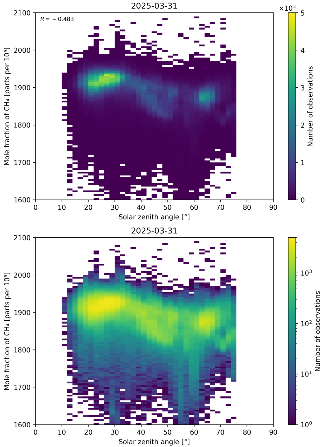
Figure 99: Scatter density plot of “Solar zenith angle” against “Mole fraction of CH 4 ” for 2025-03-30 to 2025-04-01.
