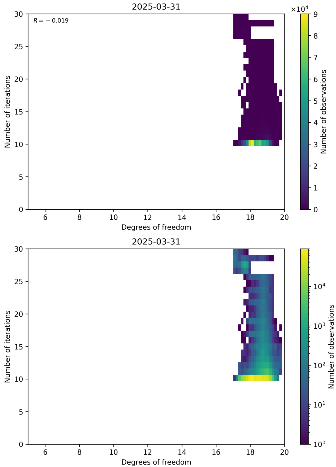
Figure 52: Scatter density plot of “Degrees of freedom” against “Number of iterations” for 2025-03-30 to 2025-04-01.
