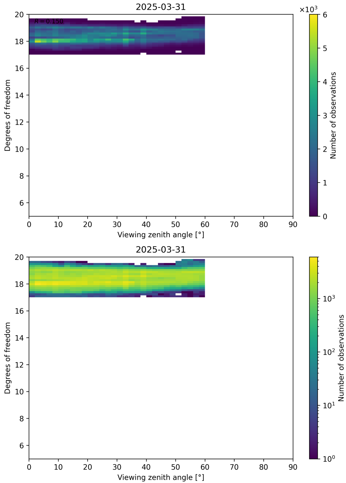
Figure 107: Scatter density plot of “Viewing zenith angle” against “Degrees of freedom” for 2025-03-30 to 2025-04-01.
