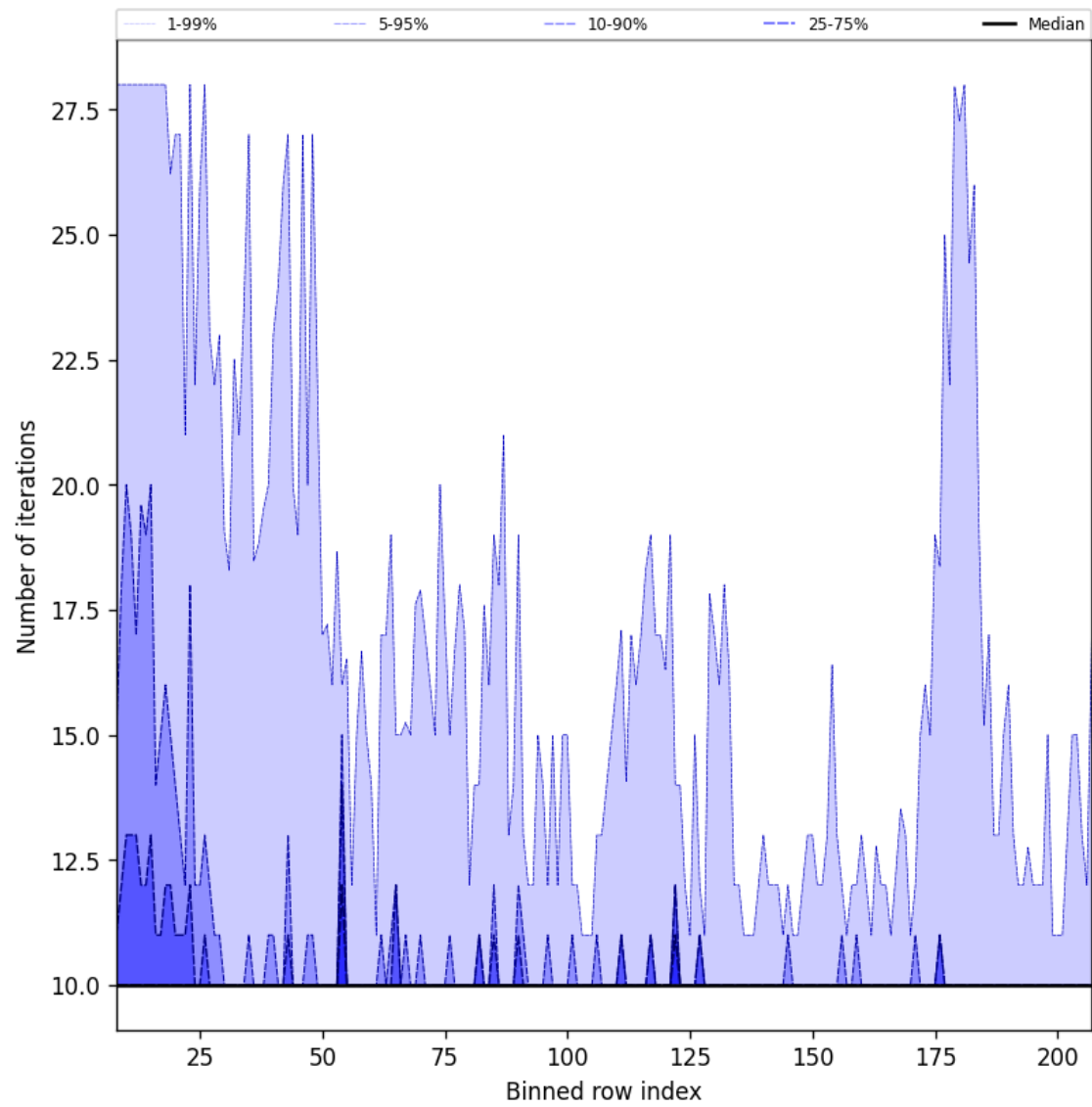
Figure 42: Along track statistics of “Number of iterations” for 2025-03-30 to 2025-04-01
