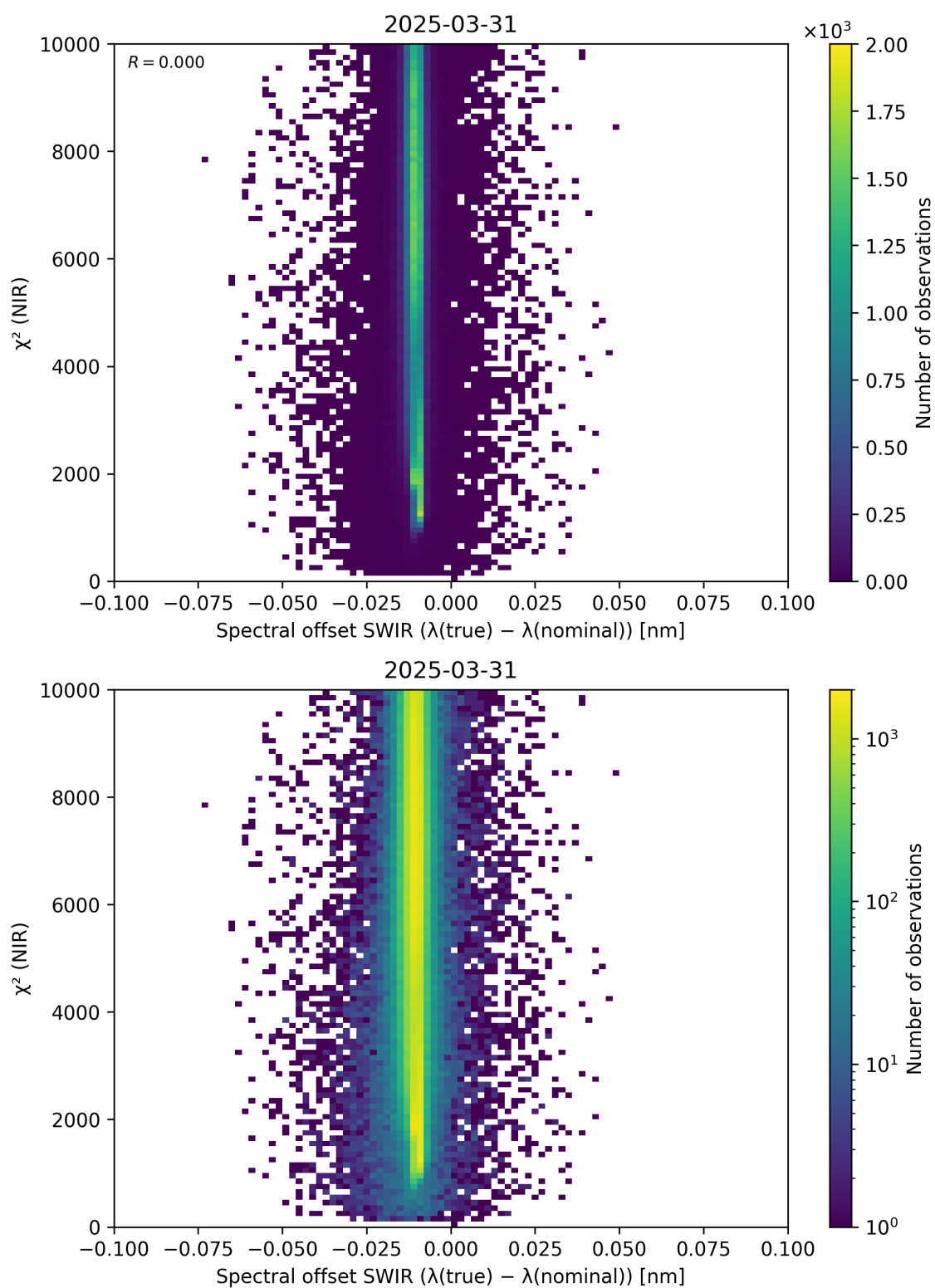
Figure 117: Scatter density plot of “Spectral offset SWIR ( \lambda_{\text{true}} - \lambda_{\text{nominal}} )” against “ \chi^2 (NIR)” for 2025-03-30 to 2025-04-01.
