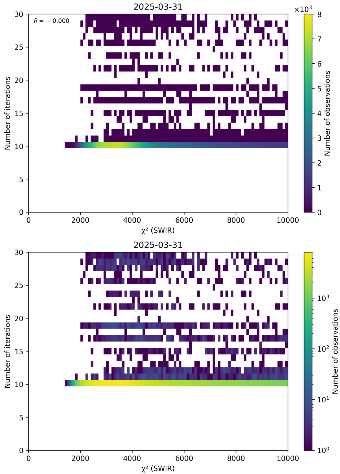
Figure 50: Scatter density plot of “ \chi^2 (SWIR)” against “Number of iterations” for 2025-03-30 to 2025-04-01.
