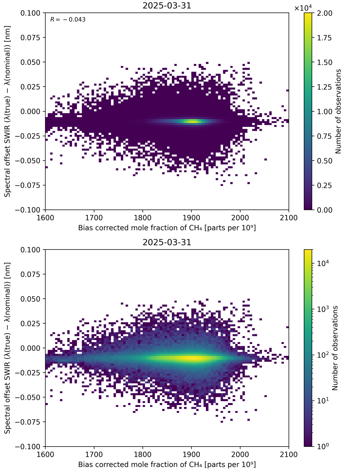
Figure 69: Scatter density plot of “Bias corrected mole fraction of \text{CH}_4 ” against “Spectral offset SWIR ( \lambda_{\text{true}} - \lambda_{\text{nominal}} )” for 2025-03-30 to 2025-04-01.
