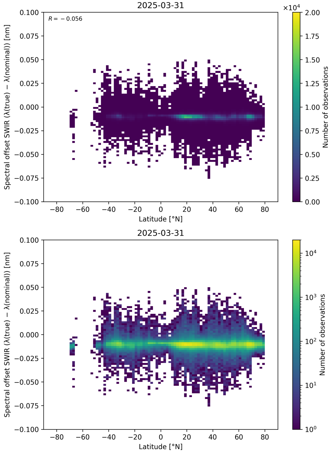
Figure 62: Scatter density plot of “Latitude” against “Spectral offset SWIR ( \lambda_{\text{true}} - \lambda_{\text{nominal}} )” for 2025-03-30 to 2025-04-01.
