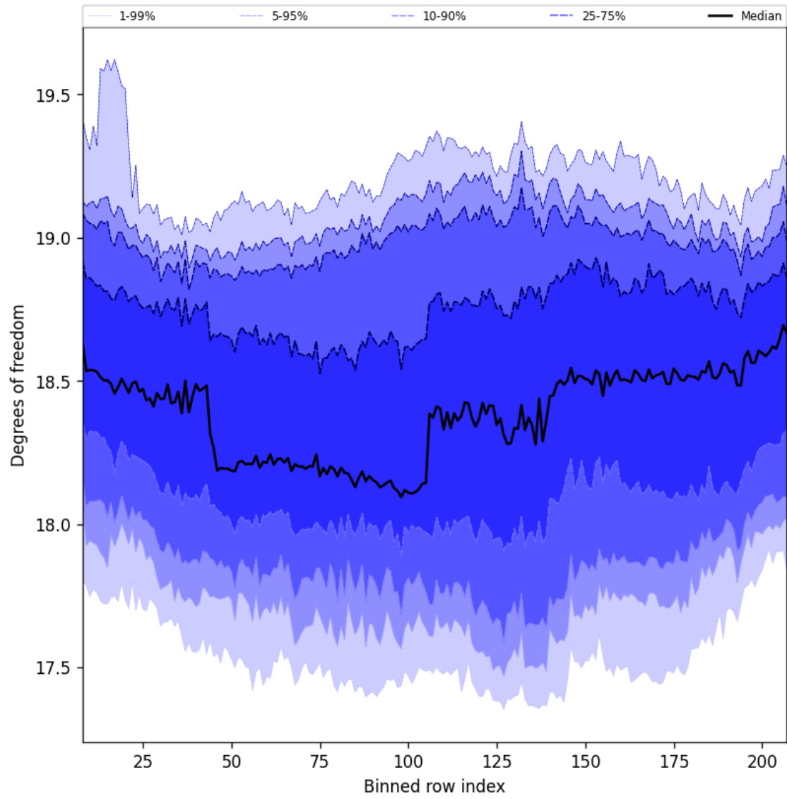
Figure 41: Along track statistics of “Degrees of freedom” for 2025-03-30 to 2025-04-01
