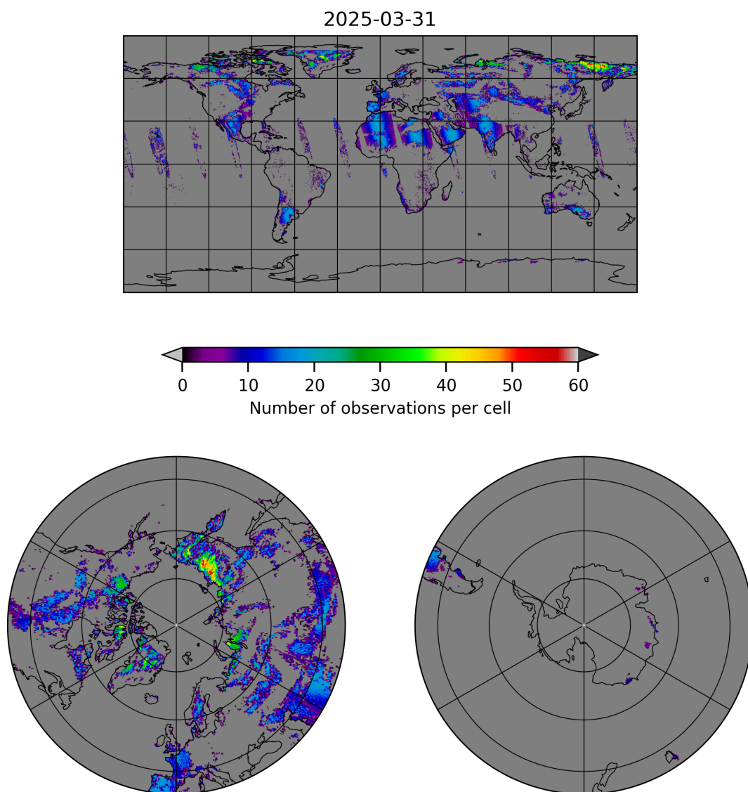
Figure 10: Map of the number of observations for 2025-03-30 to 2025-04-01
