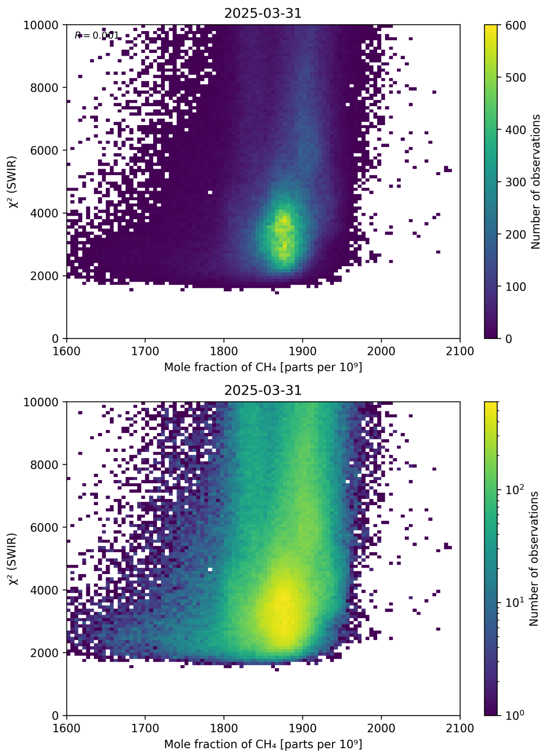
Figure 71: Scatter density plot of “Mole fraction of CH 4 ” against “ \chi^2 (SWIR)” for 2025-03-30 to 2025-04-01.
