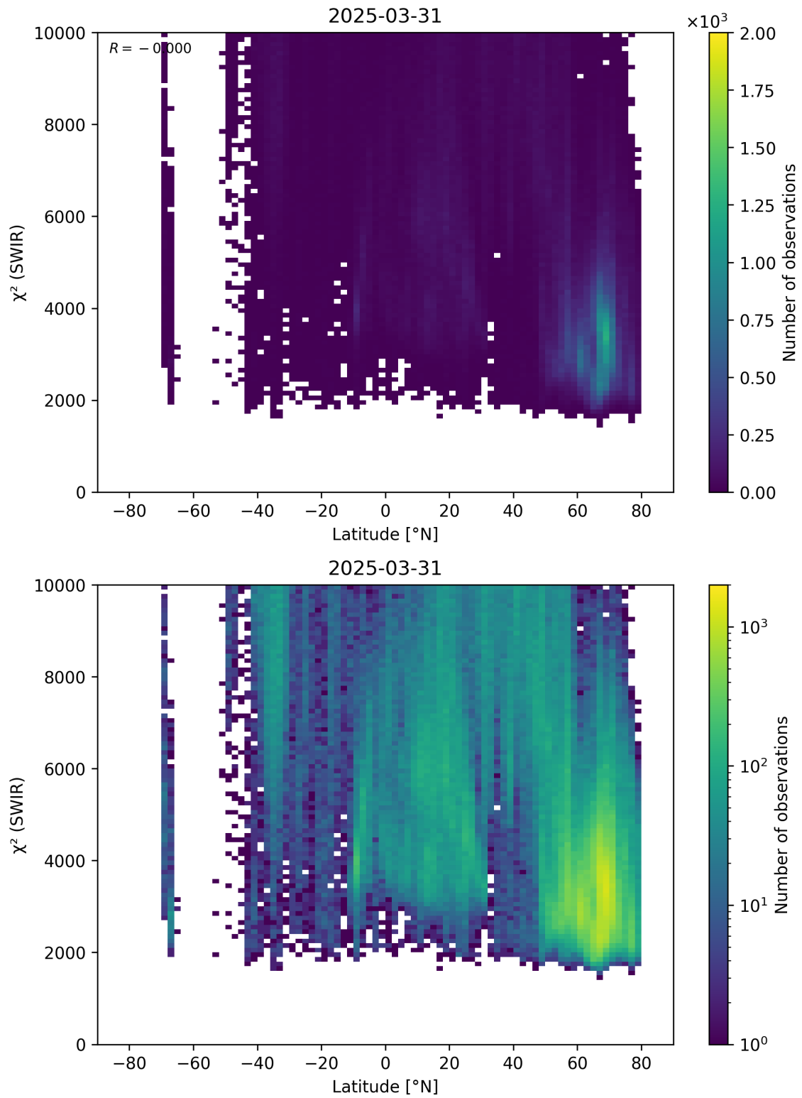
Figure 54: Scatter density plot of “Latitude” against “ \chi^2 (SWIR)” for 2025-03-30 to 2025-04-01.
