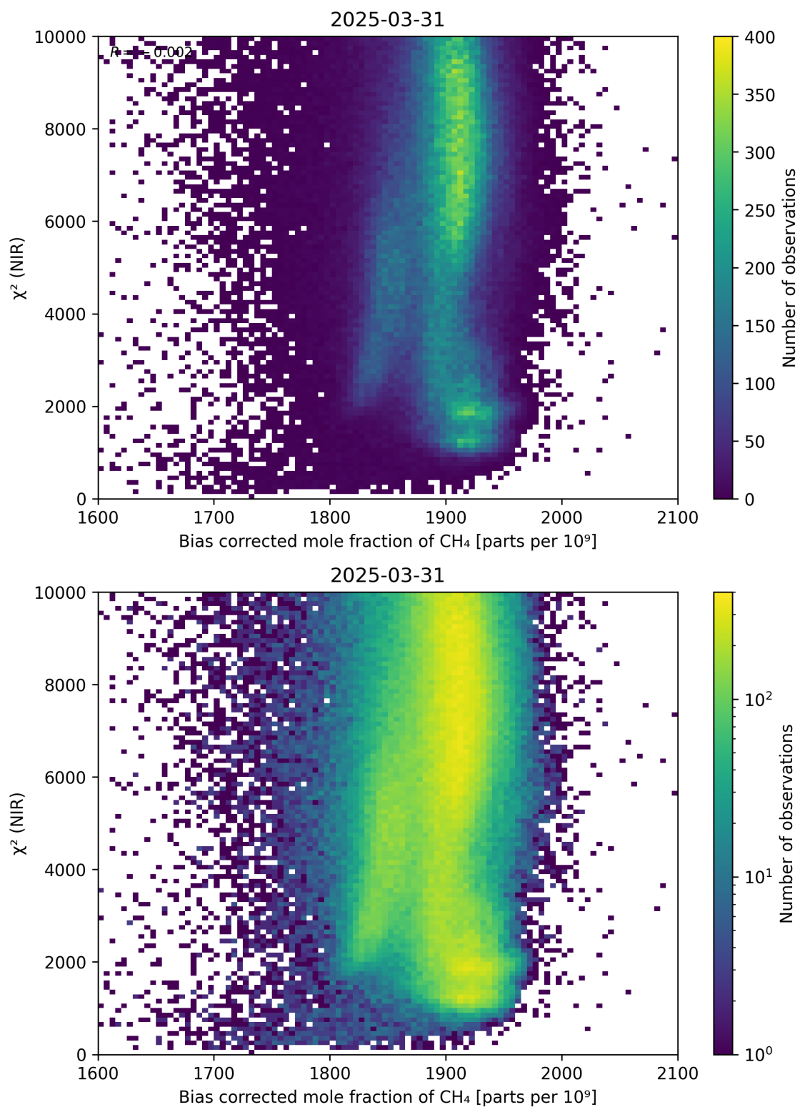
Figure 63: Scatter density plot of “Bias corrected mole fraction of CH 4 ” against “ \chi^2 (NIR)” for 2025-03-30 to 2025-04-01.
