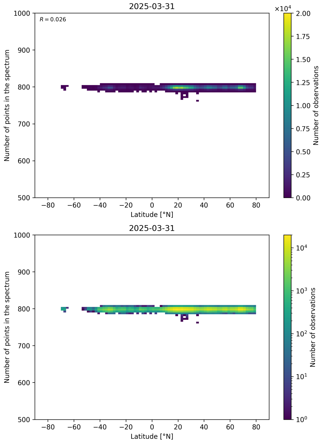
Figure 61: Scatter density plot of “Latitude” against “Number of points in the spectrum” for 2025-03-30 to 2025-04-01.
