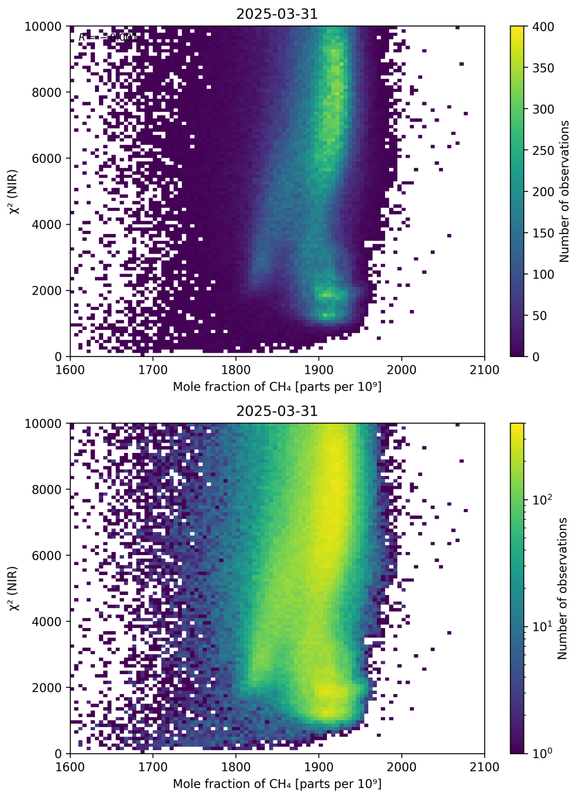
Figure 70: Scatter density plot of “Mole fraction of CH 4 ” against “ \chi^2 (NIR)” for 2025-03-30 to 2025-04-01.
