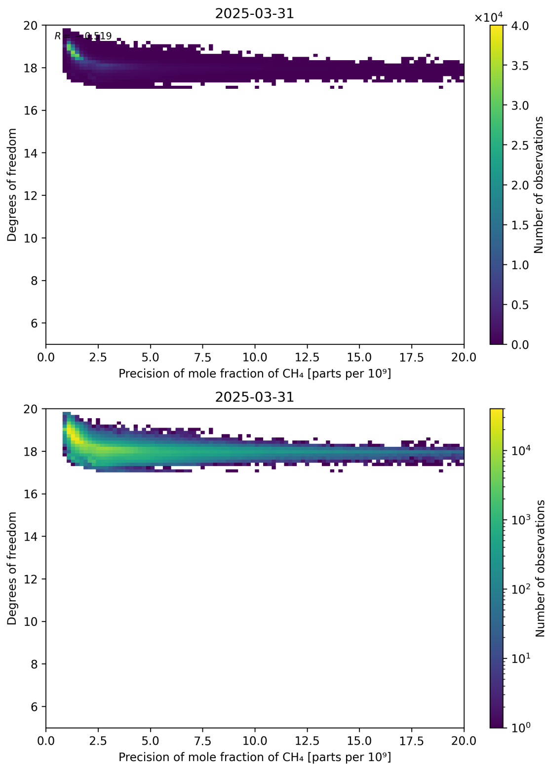
Figure 80: Scatter density plot of “Precision of mole fraction of CH 4 ” against “Degrees of freedom” for 2025-03-30 to 2025-04-01.
