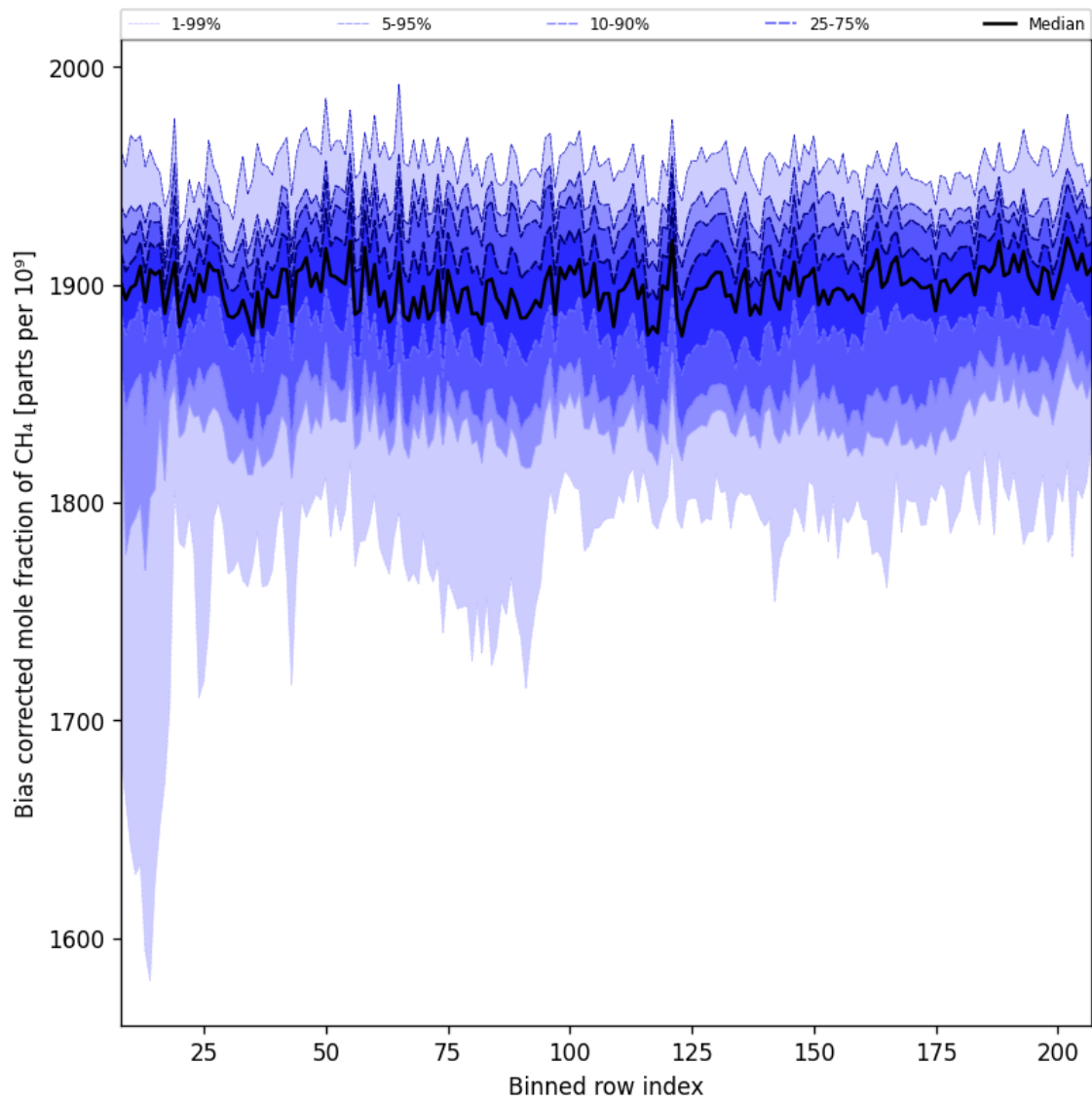
Figure 36: Along track statistics of “Bias corrected mole fraction of CH 4 ” for 2025-03-30 to 2025-04-01
