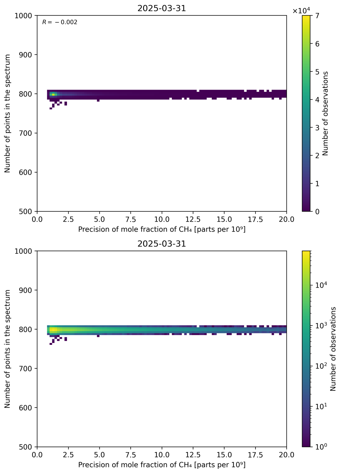
Figure 84: Scatter density plot of “Precision of mole fraction of CH 4 ” against “Number of points in the spectrum” for 2025-03-30 to 2025-04-01.
