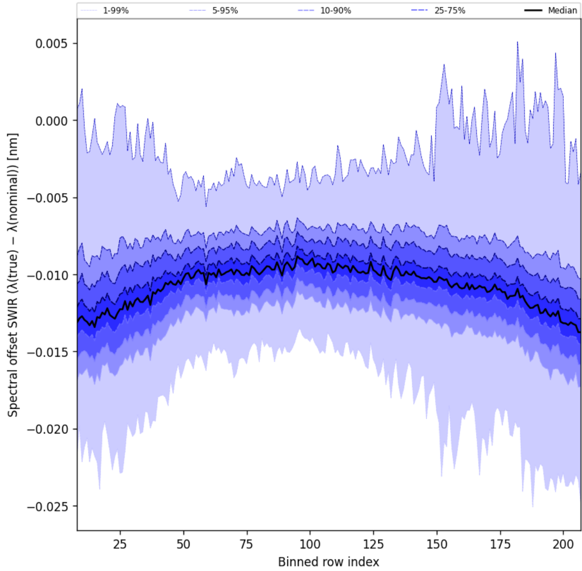
Figure 38: Along track statistics of “Spectral offset SWIR ( \lambda_{\text{true}} - \lambda_{\text{nominal}} )” for 2025-03-30 to 2025-04-01
