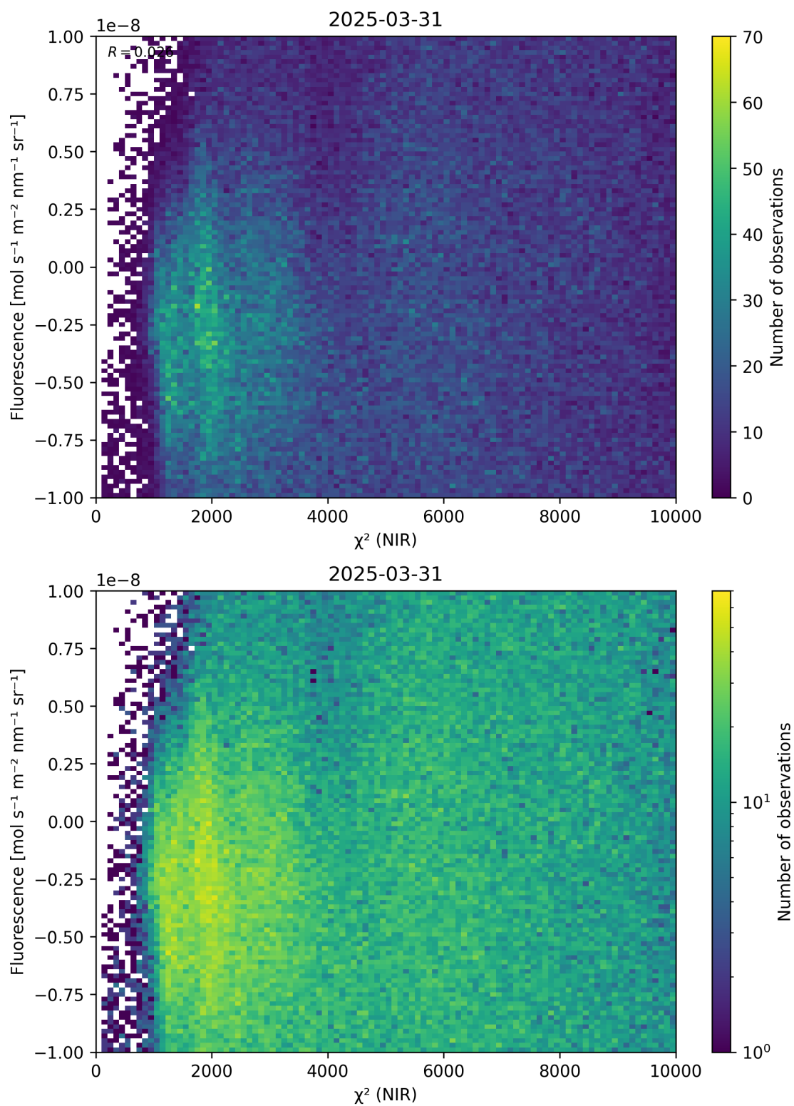
Figure 45: Scatter density plot of “ \chi^2 (NIR)” against “Fluorescence” for 2025-03-30 to 2025-04-01.
