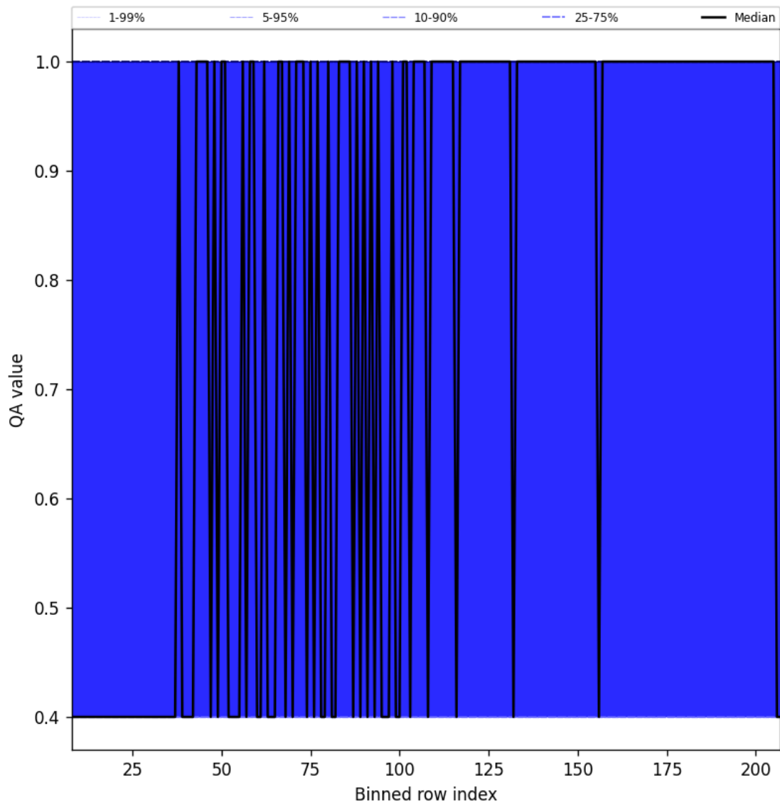
Figure 33: Along track statistics of “QA value” for 2025-03-30 to 2025-04-01
