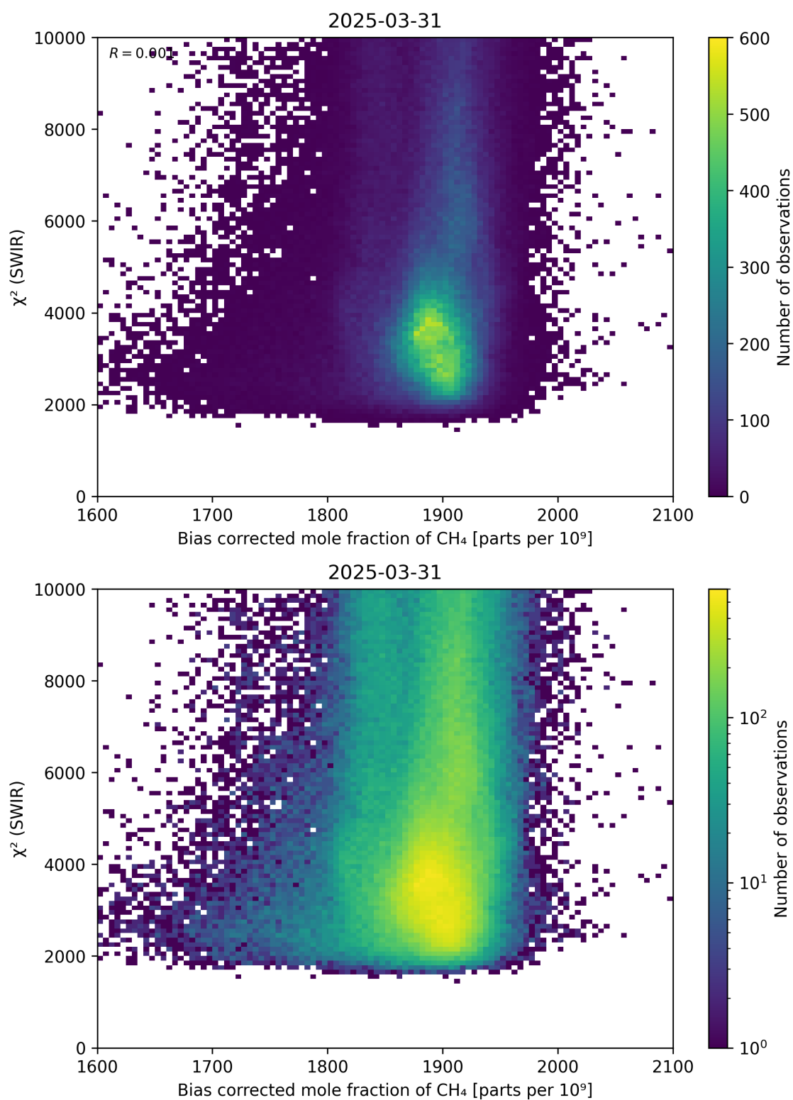
Figure 64: Scatter density plot of “Bias corrected mole fraction of CH 4 ” against “ \chi^2 (SWIR)” for 2025-03-30 to 2025-04-01.
