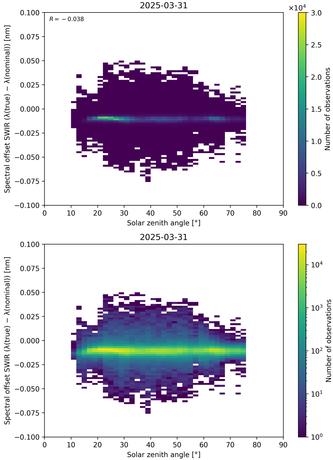
Figure 104: Scatter density plot of “Solar zenith angle” against “Spectral offset SWIR ( \lambda_{\text{true}} - \lambda_{\text{nominal}} )” for 2025-03-30 to 2025-04-01.
