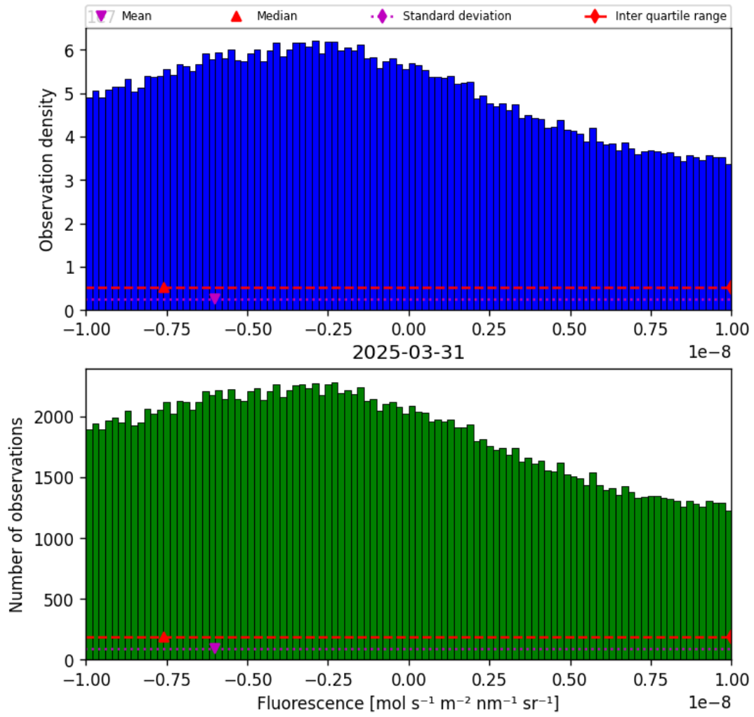
Figure 32: Histogram of “Fluorescence” for 2025-03-30 to 2025-04-01
