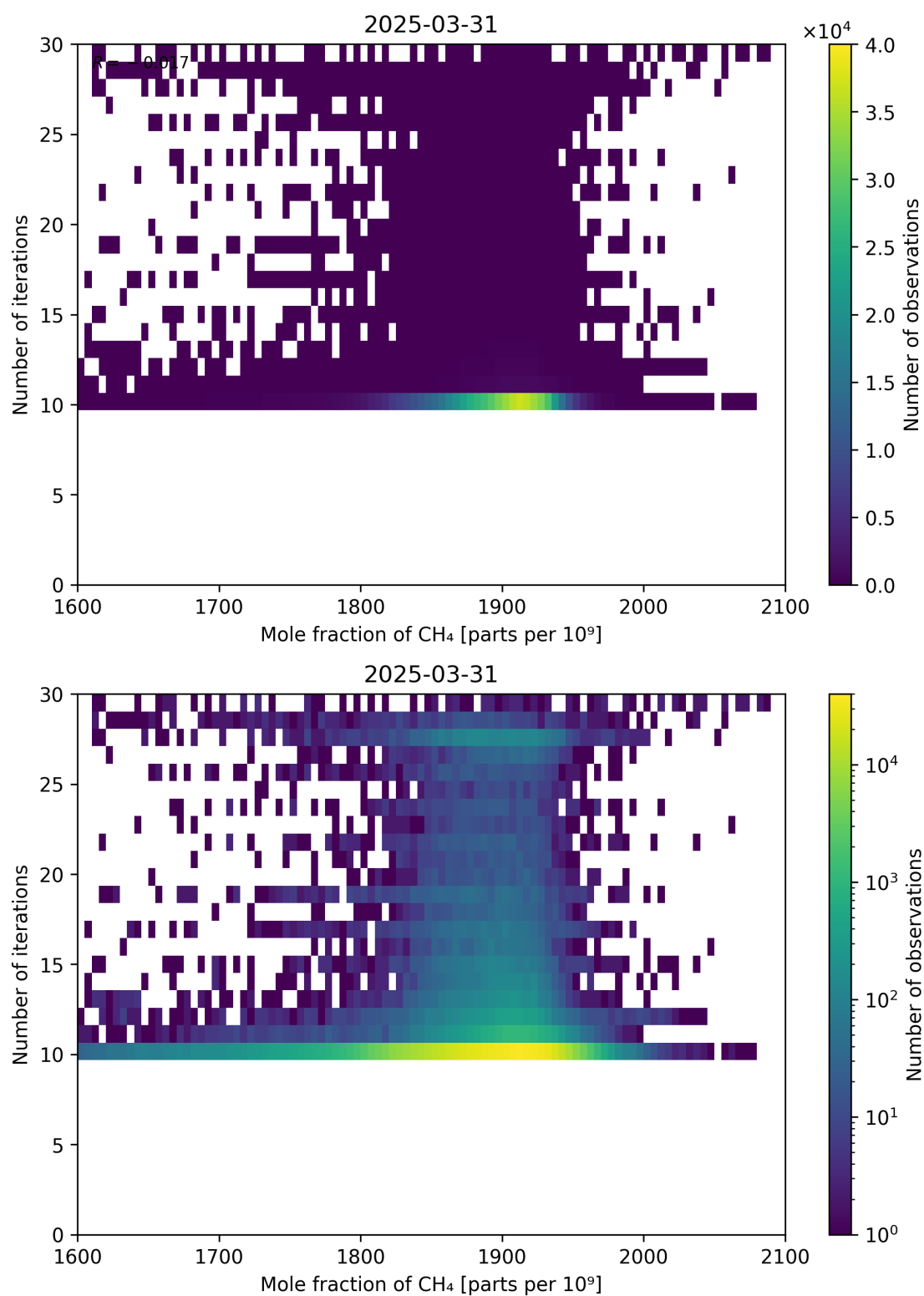
Figure 76: Scatter density plot of “Mole fraction of CH 4 ” against “Number of iterations” for 2025-03-30 to 2025-04-01.
