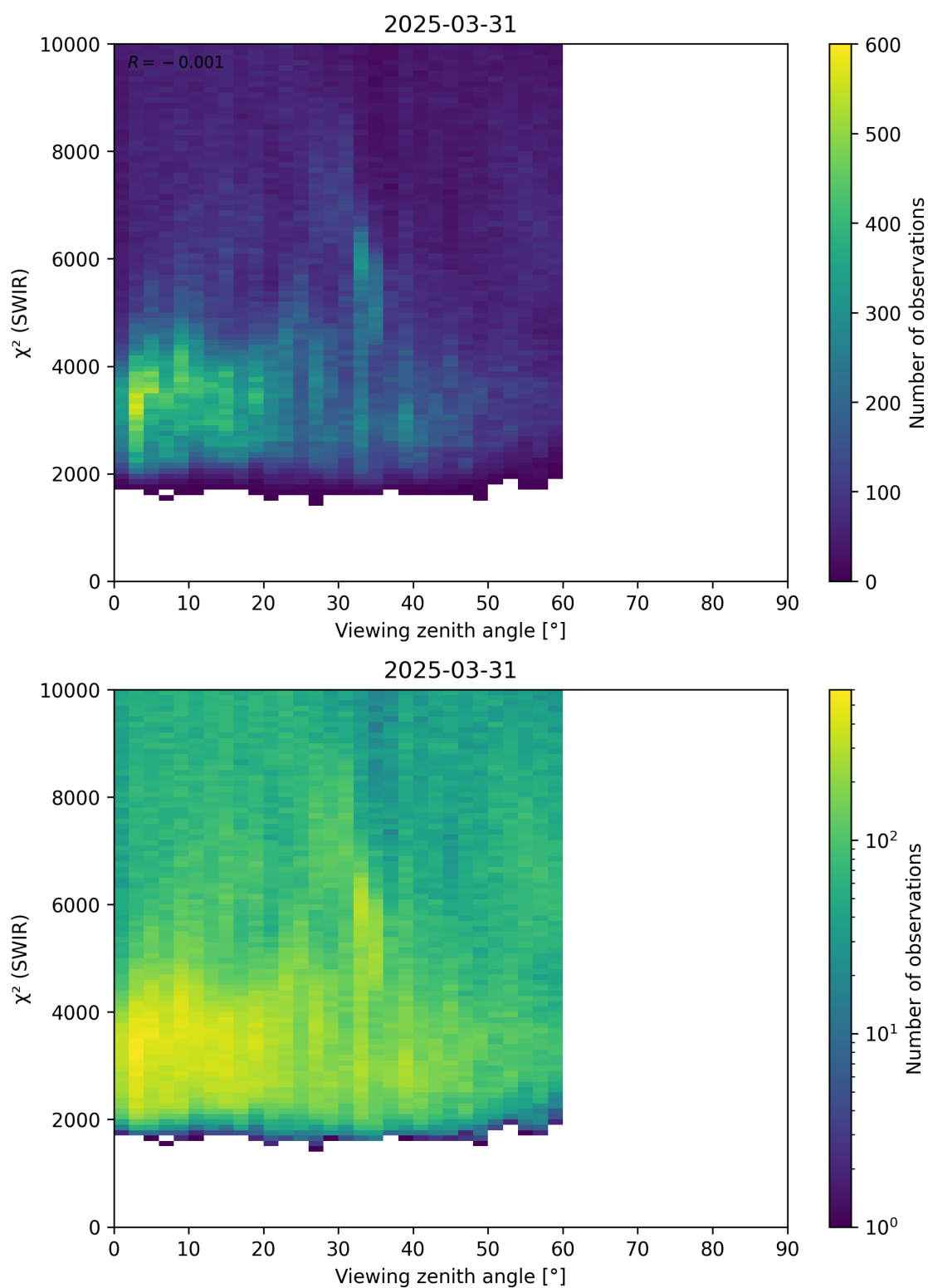
Figure 106: Scatter density plot of “Viewing zenith angle” against “ \chi^2 (SWIR)” for 2025-03-30 to 2025-04-01.
