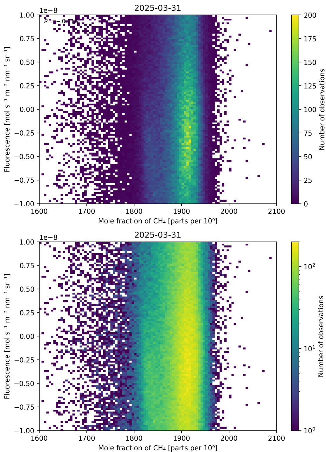
Figure 73: Scatter density plot of “Mole fraction of CH 4 ” against “Fluorescence” for 2025-03-30 to 2025-04-01.
