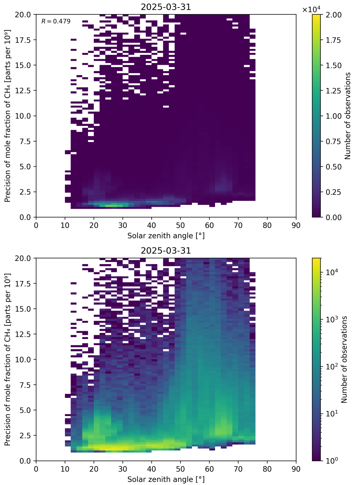
Figure 101: Scatter density plot of “Solar zenith angle” against “Precision of mole fraction of CH 4 ” for 2025-03-30 to 2025-04-01.
