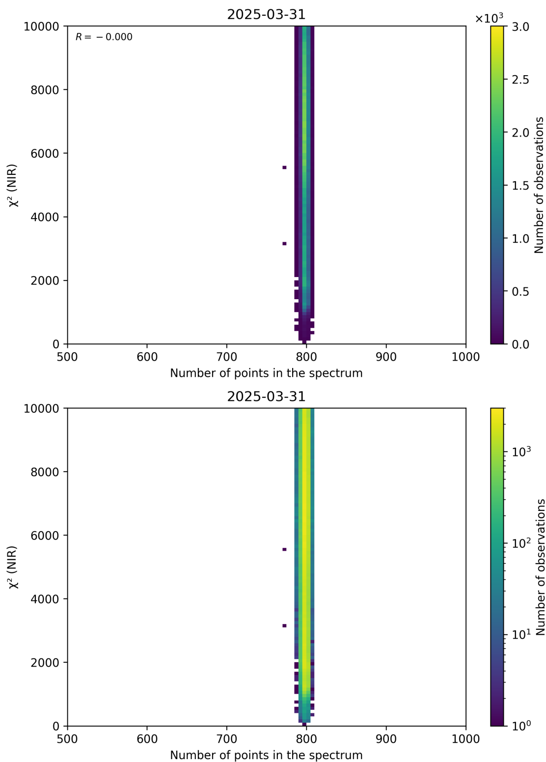
Figure 88: Scatter density plot of “Number of points in the spectrum” against “ \chi^2 (NIR)” for 2025-03-30 to 2025-04-01.
