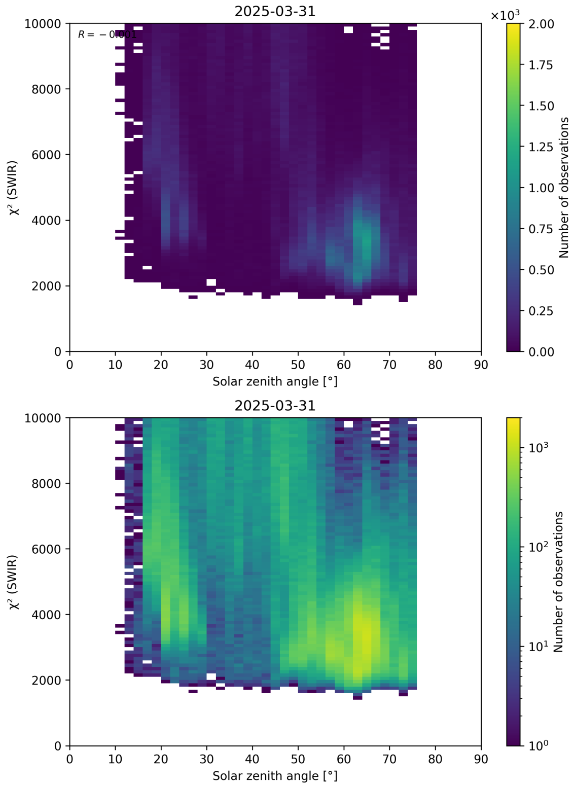
Figure 95: Scatter density plot of “Solar zenith angle” against “ \chi^2 (SWIR)” for 2025-03-30 to 2025-04-01.
