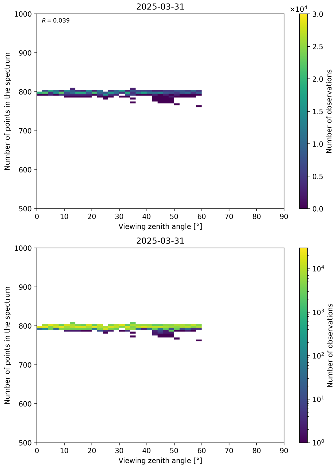
Figure 114: Scatter density plot of “Viewing zenith angle” against “Number of points in the spectrum” for 2025-03-30 to 2025-04-01.
