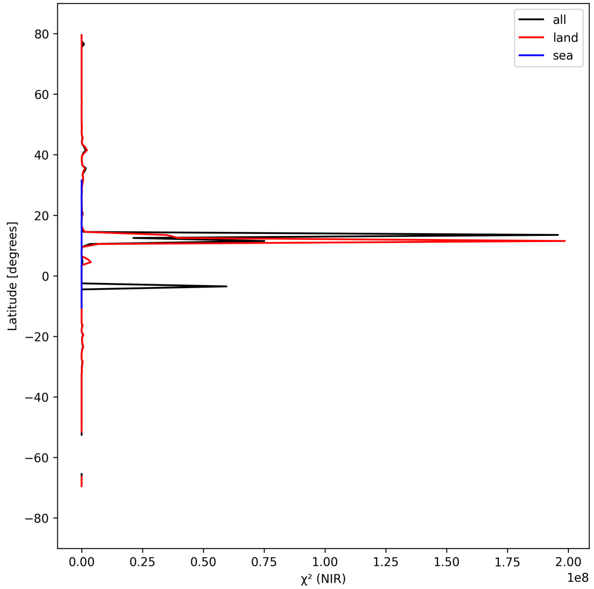
Figure 18: Zonal average of “ \chi^2 (NIR)” for 2025-03-30 to 2025-04-01.
