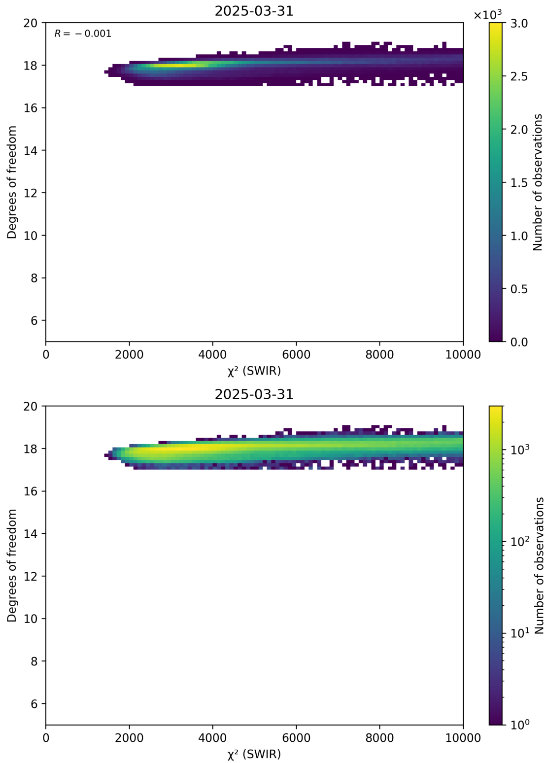
Figure 48: Scatter density plot of “ \chi^2 (SWIR)” against “Degrees of freedom” for 2025-03-30 to 2025-04-01.
