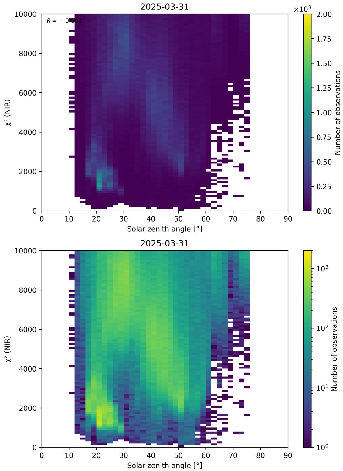
Figure 94: Scatter density plot of “Solar zenith angle” against “ \chi^2 (NIR)” for 2025-03-30 to 2025-04-01.
