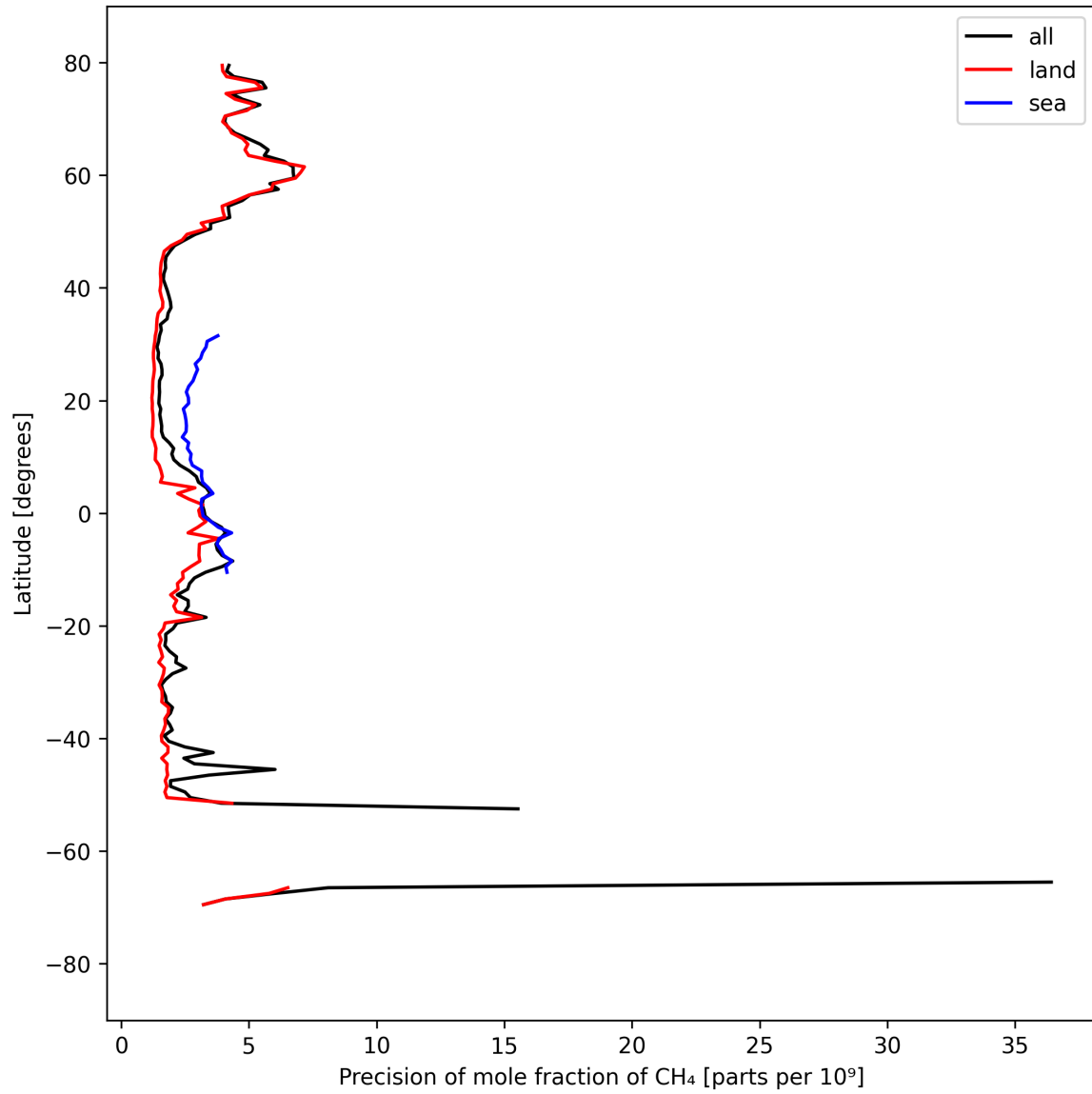
Figure 13: Zonal average of “Precision of mole fraction of CH 4 ” for 2025-03-30 to 2025-04-01.
