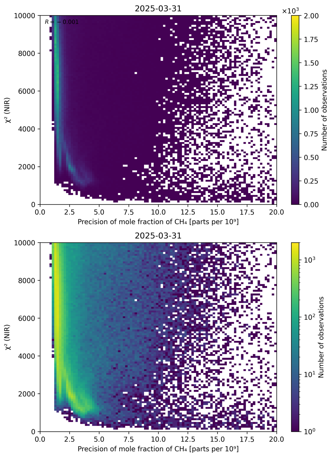
Figure 78: Scatter density plot of “Precision of mole fraction of CH 4 ” against “ \chi^2 (NIR)” for 2025-03-30 to 2025-04-01.
