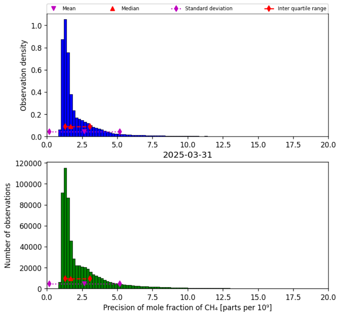
Figure 24: Histogram of “Precision of mole fraction of CH 4 ” for 2025-03-30 to 2025-04-01
