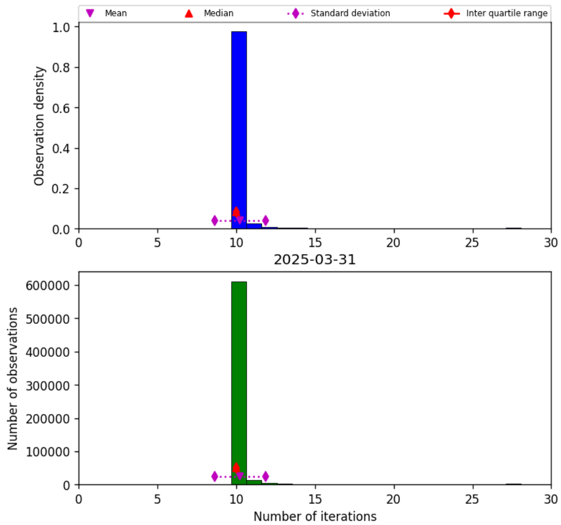
Figure 31: Histogram of “Number of iterations” for 2025-03-30 to 2025-04-01
