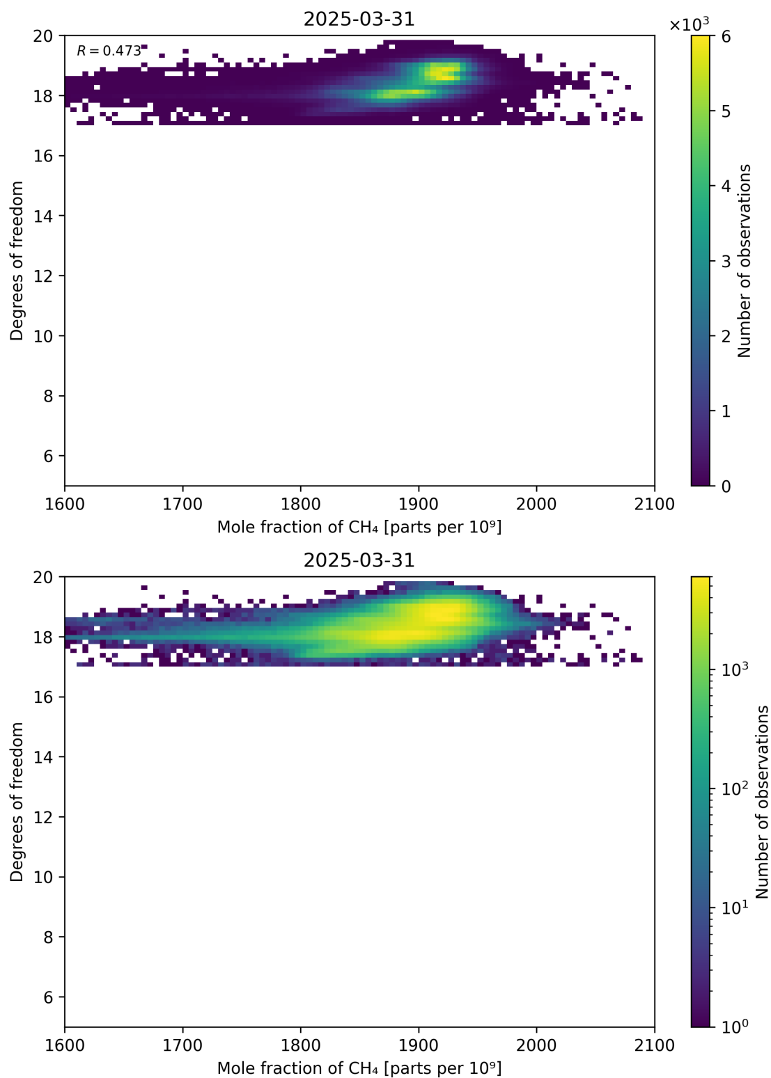
Figure 72: Scatter density plot of “Mole fraction of CH 4 ” against “Degrees of freedom” for 2025-03-30 to 2025-04-01.
