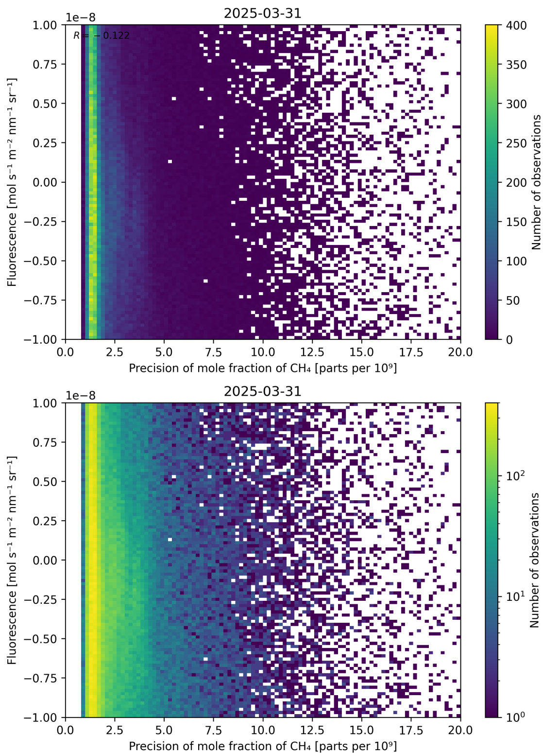
Figure 81: Scatter density plot of “Precision of mole fraction of CH 4 ” against “Fluorescence” for 2025-03-30 to 2025-04-01.
