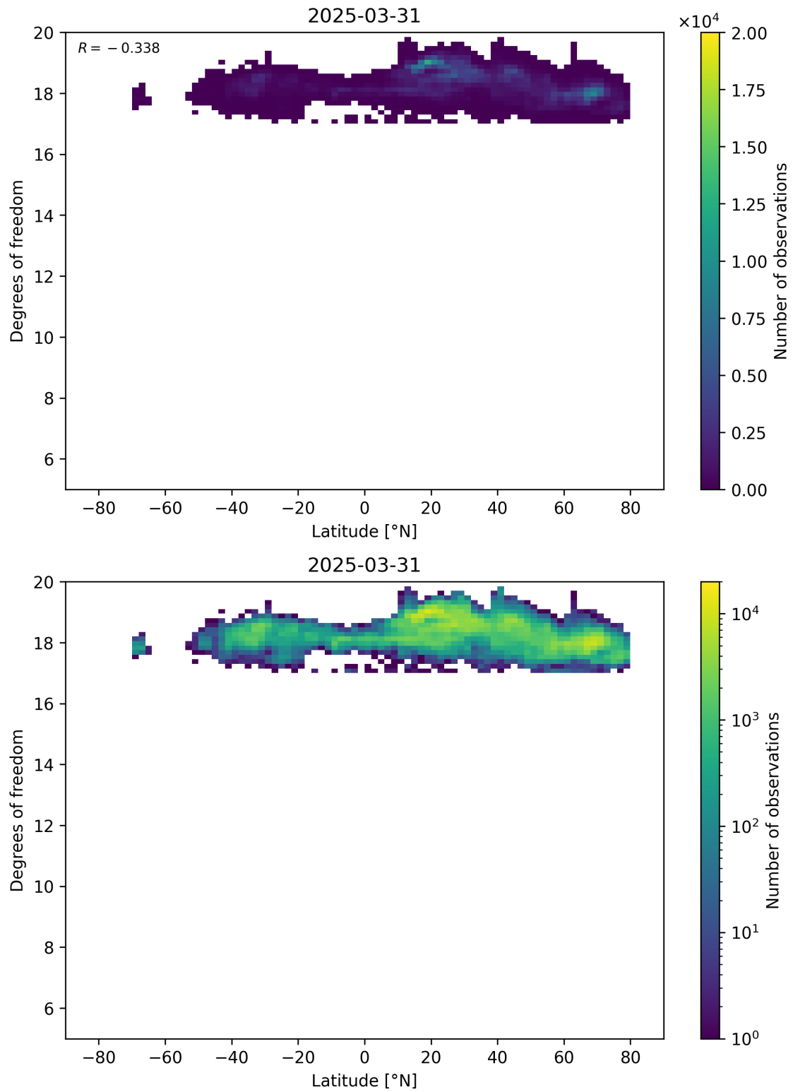
Figure 55: Scatter density plot of “Latitude” against “Degrees of freedom” for 2025-03-30 to 2025-04-01.
