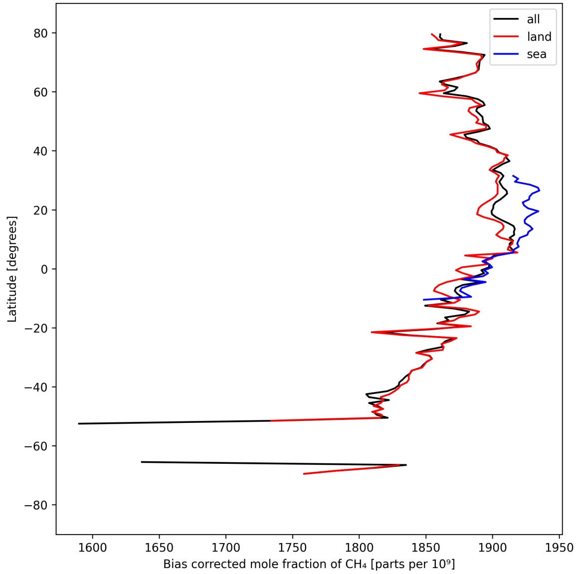
Figure 14: Zonal average of “Bias corrected mole fraction of CH 4 ” for 2025-03-30 to 2025-04-01.
