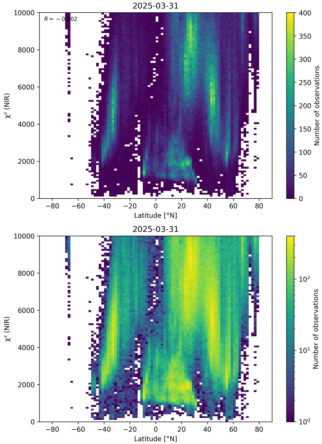
Figure 53: Scatter density plot of “Latitude” against “ \chi^2 (NIR)” for 2025-03-30 to 2025-04-01.
