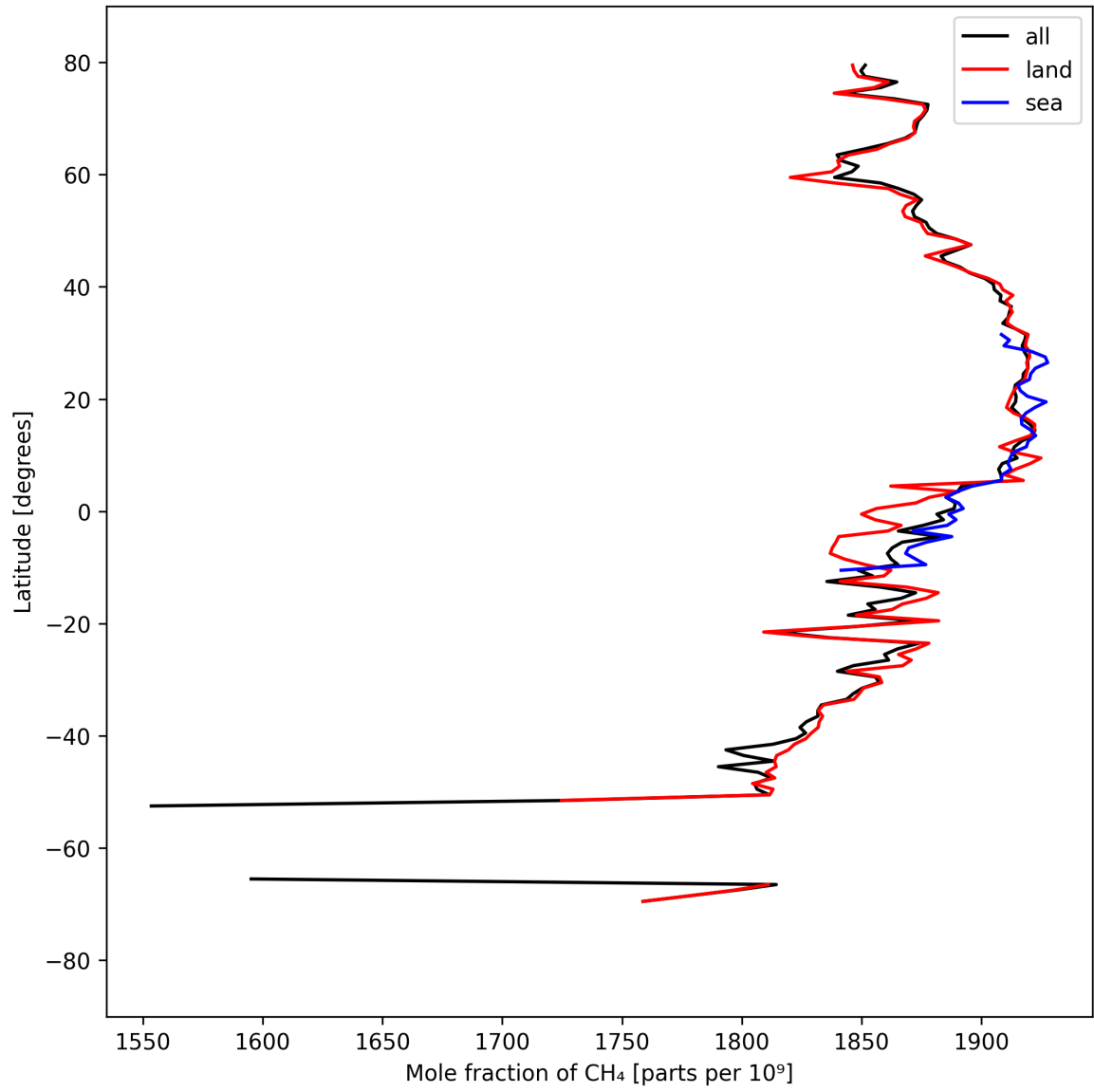
Figure 12: Zonal average of “Mole fraction of CH 4 ” for 2025-03-30 to 2025-04-01.
