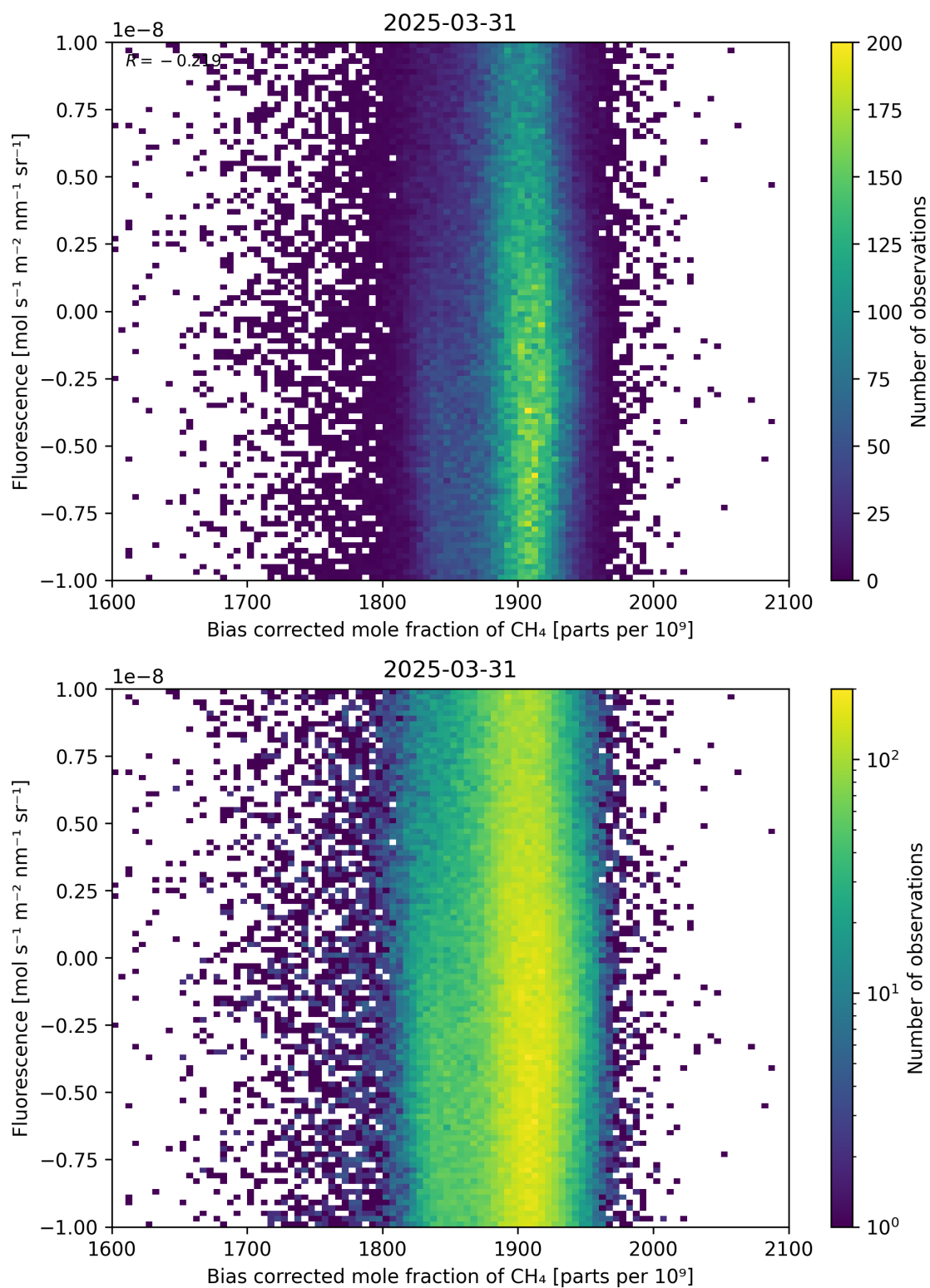
Figure 66: Scatter density plot of “Bias corrected mole fraction of \text{CH}_4 ” against “Fluorescence” for 2025-03-30 to 2025-04-01.
