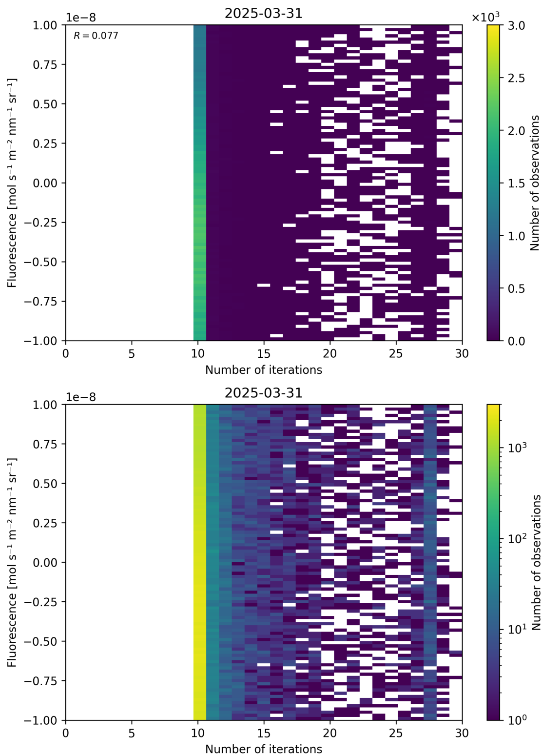
Figure 87: Scatter density plot of “Number of iterations” against “Fluorescence” for 2025-03-30 to 2025-04-01.
