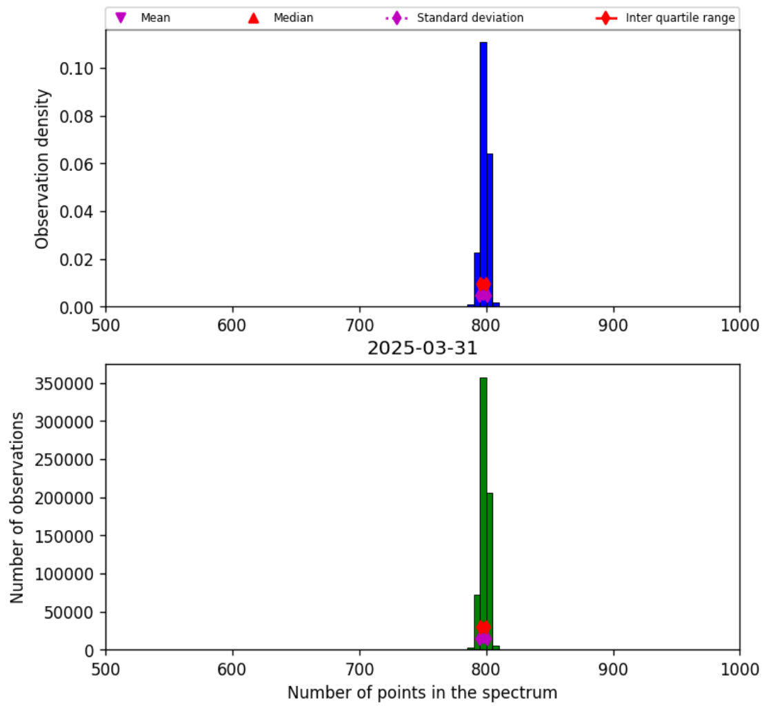
Figure 26: Histogram of “Number of points in the spectrum” for 2025-03-30 to 2025-04-01
