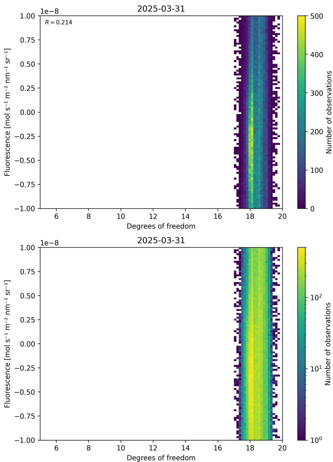
Figure 51: Scatter density plot of “Degrees of freedom” against “Fluorescence” for 2025-03-30 to 2025-04-01.
