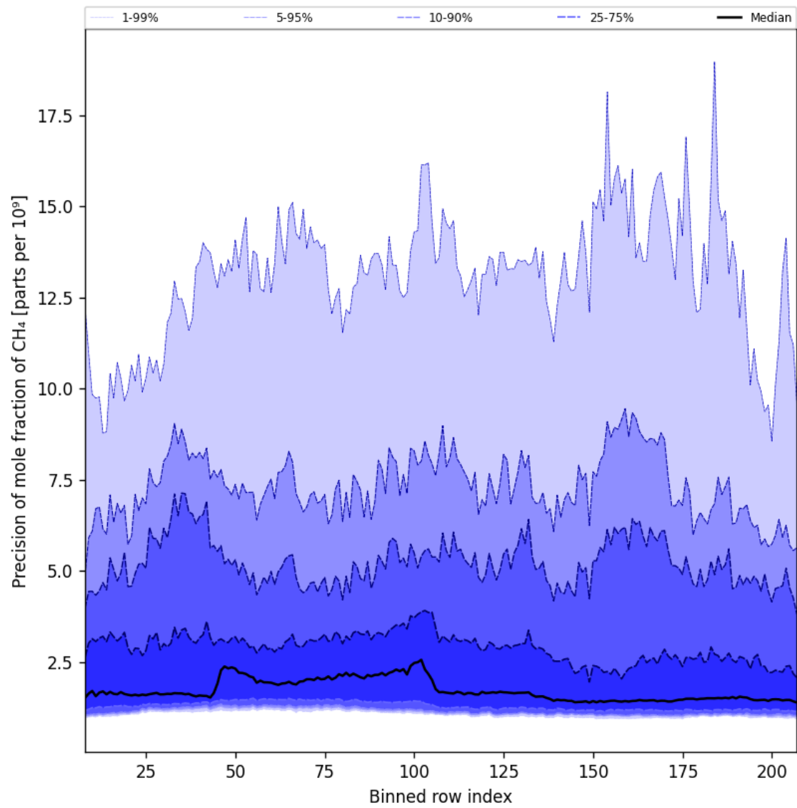
Figure 35: Along track statistics of “Precision of mole fraction of CH 4 ” for 2025-03-30 to 2025-04-01
