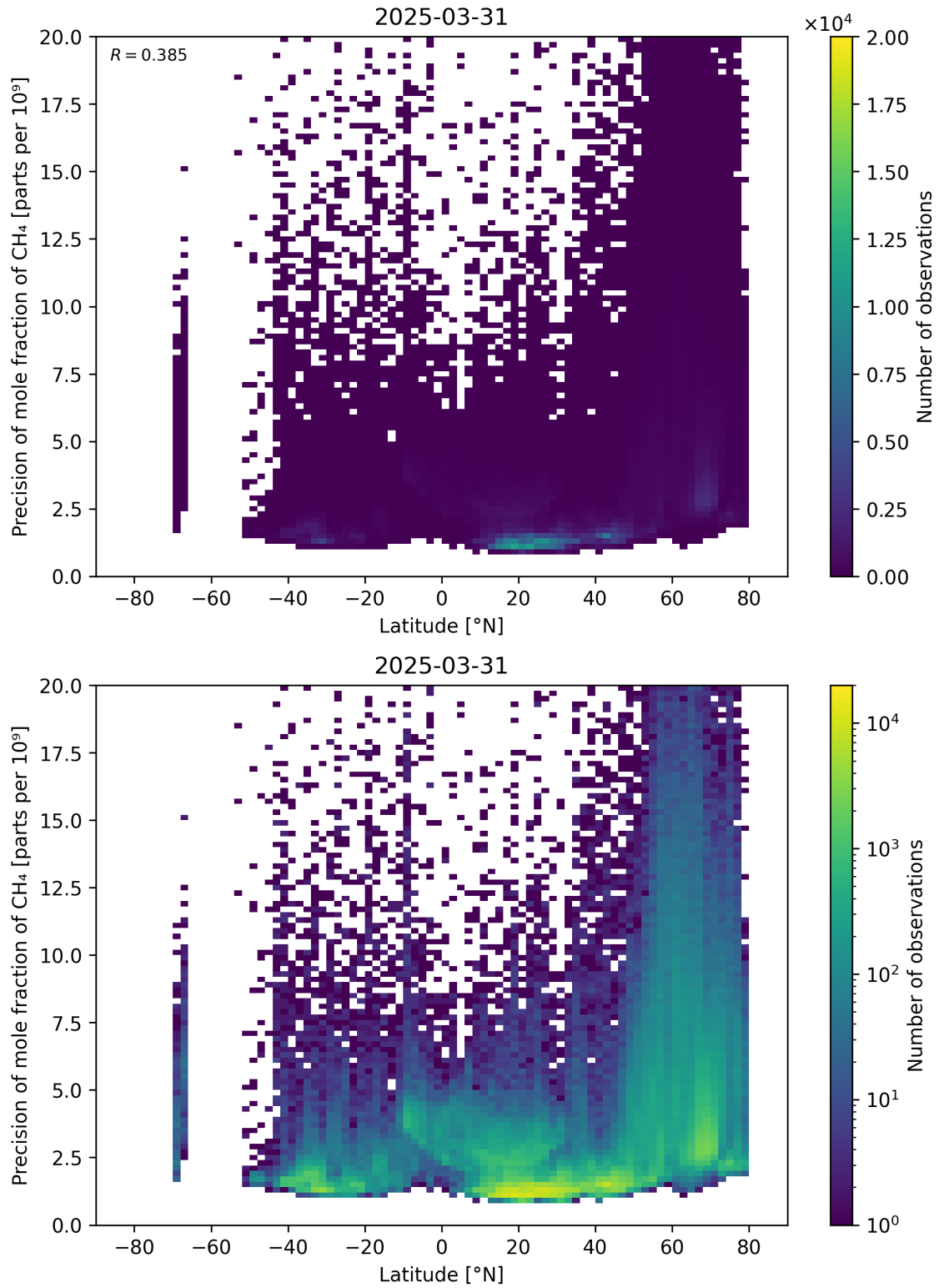
Figure 59: Scatter density plot of “Latitude” against “Precision of mole fraction of \text{CH}_4 ” for 2025-03-30 to 2025-04-01.
