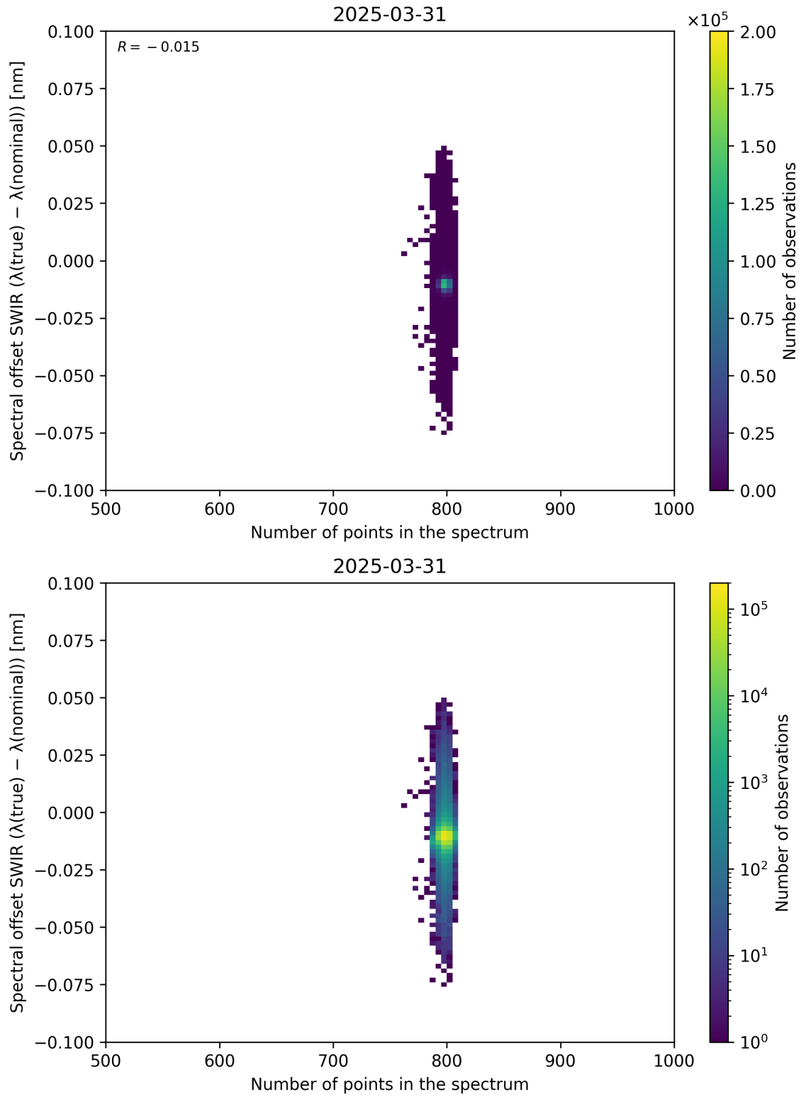
Figure 93: Scatter density plot of “Number of points in the spectrum” against “Spectral offset SWIR ( \lambda_{\text{true}} - \lambda_{\text{nominal}} )” for 2025-03-30 to 2025-04-01.
