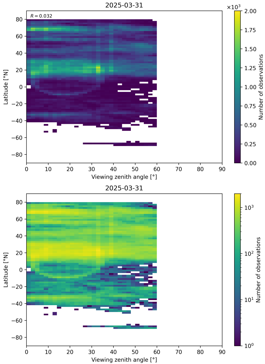
Figure 109: Scatter density plot of “Viewing zenith angle” against “Latitude” for 2025-03-30 to 2025-04-01.
