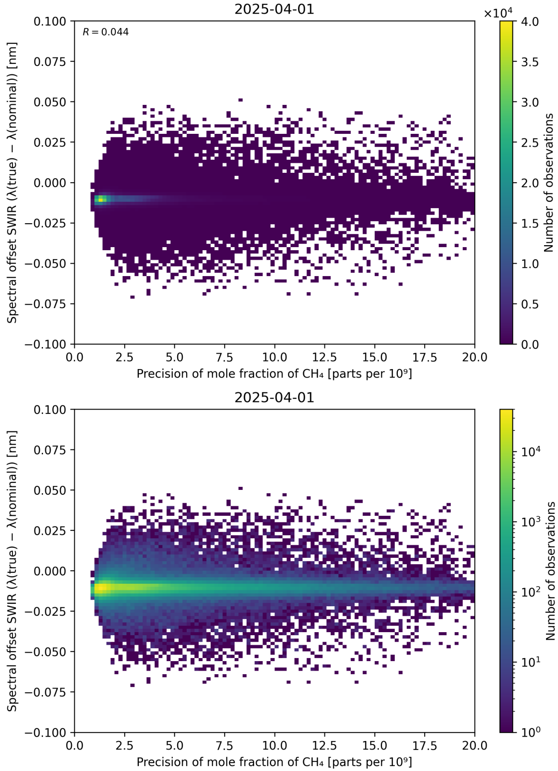
Figure 85: Scatter density plot of “Precision of mole fraction of \text{CH}_4 ” against “Spectral offset SWIR ( \lambda_{\text{true}} - \lambda_{\text{nominal}} )” for 2025-03-31 to 2025-04-02.
