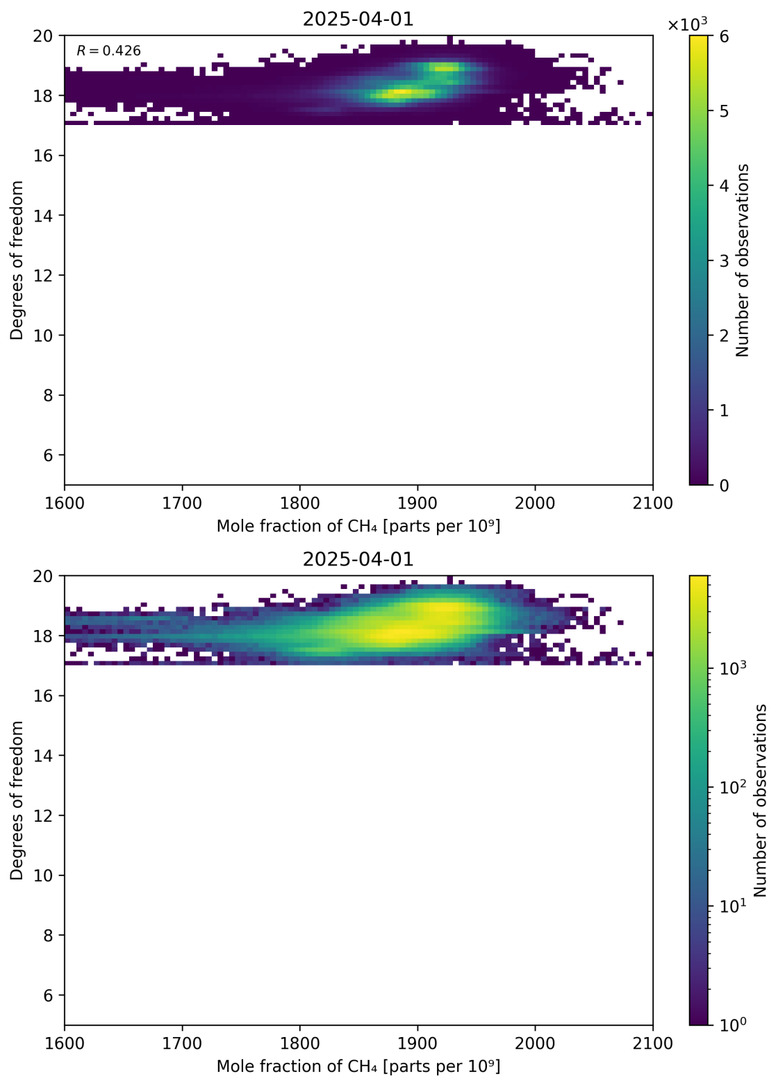
Figure 72: Scatter density plot of “Mole fraction of CH 4 ” against “Degrees of freedom” for 2025-03-31 to 2025-04-02.
