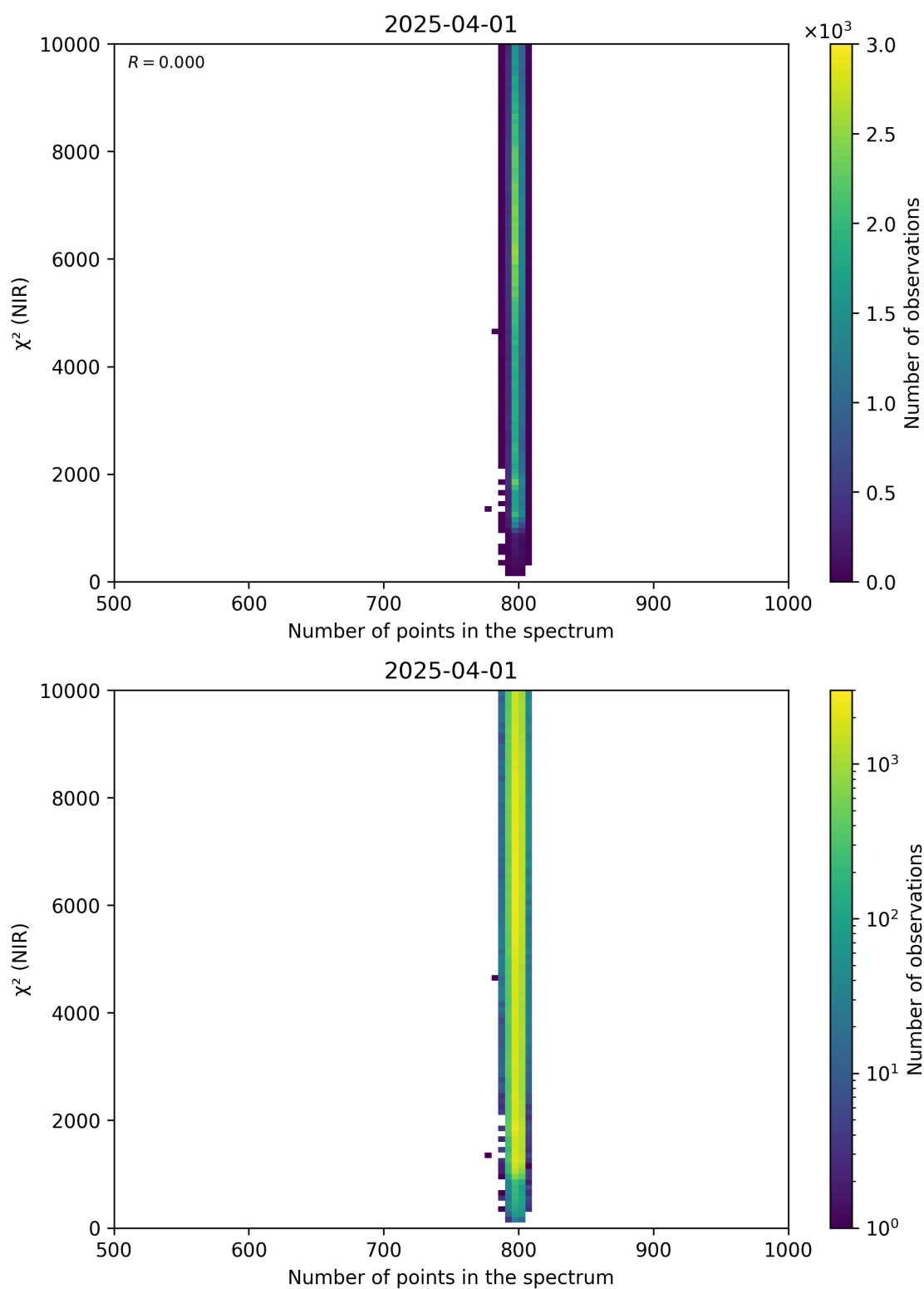
Figure 88: Scatter density plot of “Number of points in the spectrum” against “ \chi^2 (NIR)” for 2025-03-31 to 2025-04-02.
