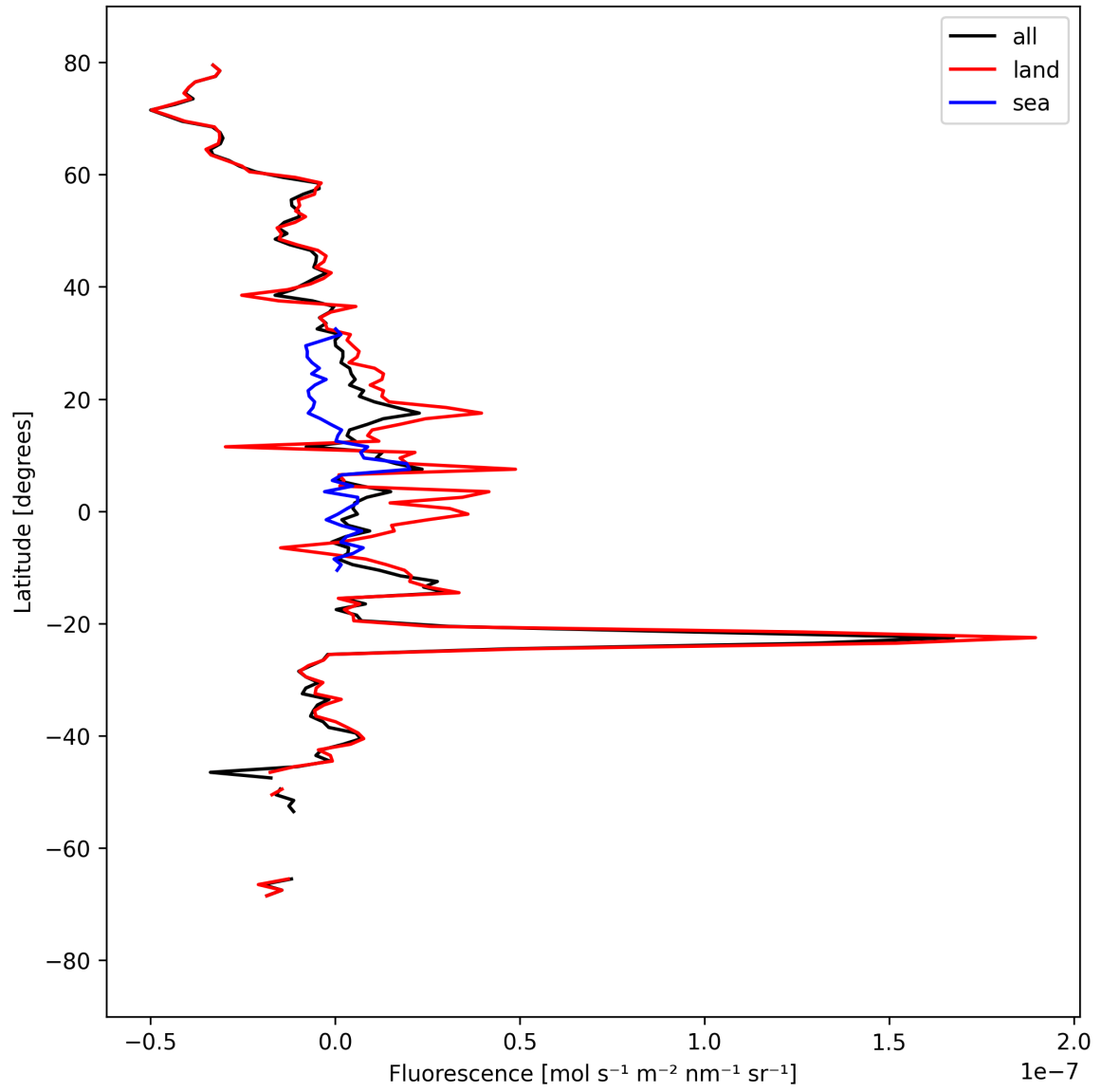
Figure 21: Zonal average of “Fluorescence” for 2025-03-31 to 2025-04-02.
