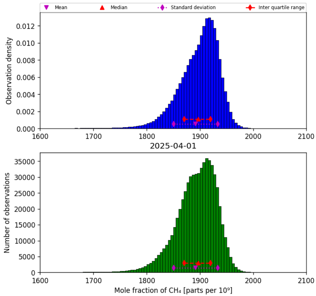
Figure 23: Histogram of “Mole fraction of CH 4 ” for 2025-03-31 to 2025-04-02
