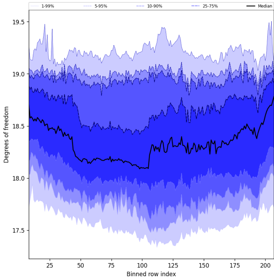
Figure 41: Along track statistics of “Degrees of freedom” for 2025-03-31 to 2025-04-02
