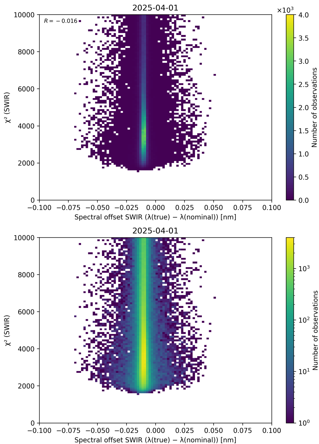
Figure 118: Scatter density plot of “Spectral offset SWIR ( \lambda_{\text{true}} - \lambda_{\text{nominal}} )” against “ \chi^2 (SWIR)” for 2025-03-31 to 2025-04-02.
