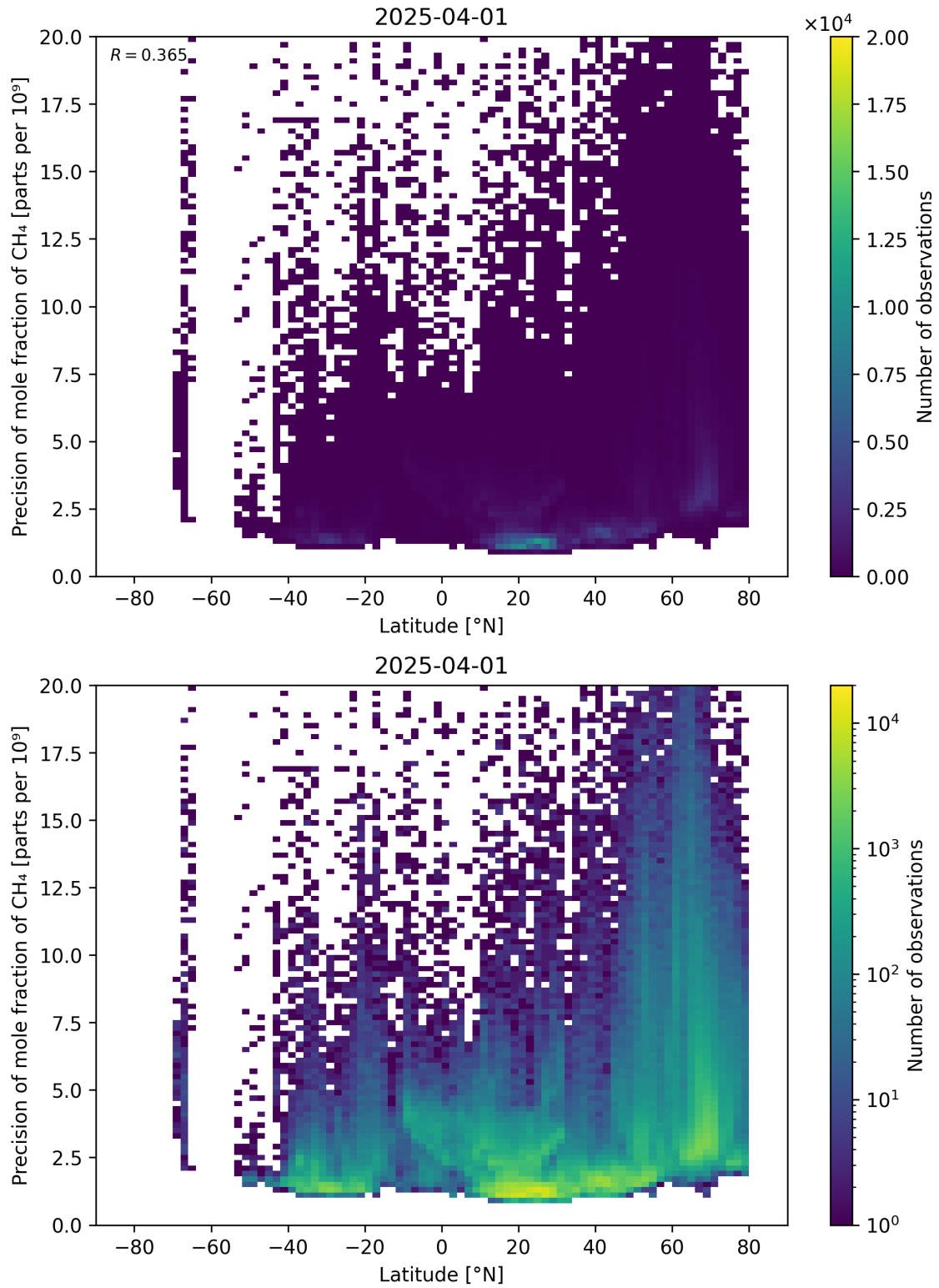
Figure 59: Scatter density plot of “Latitude” against “Precision of mole fraction of \text{CH}_4 ” for 2025-03-31 to 2025-04-02.
