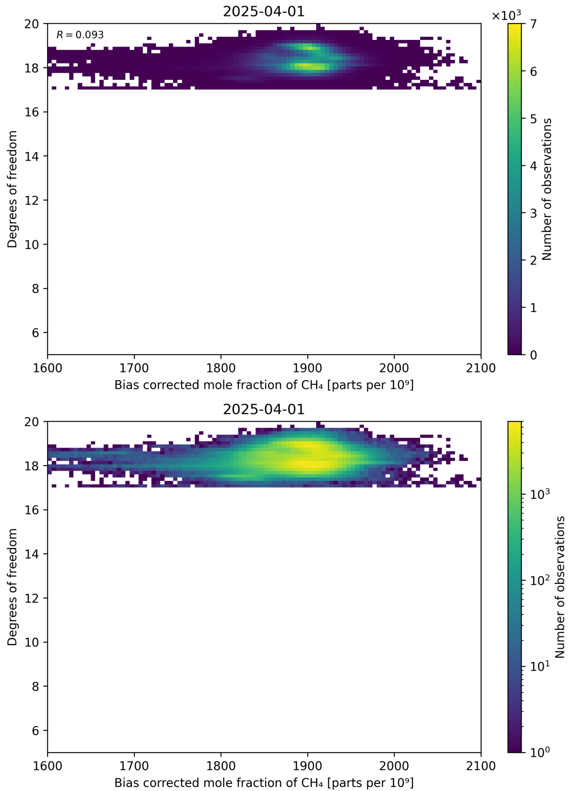
Figure 65: Scatter density plot of “Bias corrected mole fraction of CH 4 ” against “Degrees of freedom” for 2025-03-31 to 2025-04-02.
