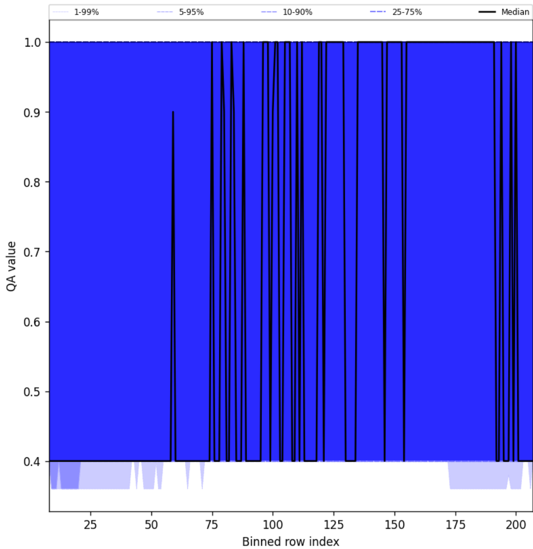
Figure 33: Along track statistics of “QA value” for 2025-03-31 to 2025-04-02
