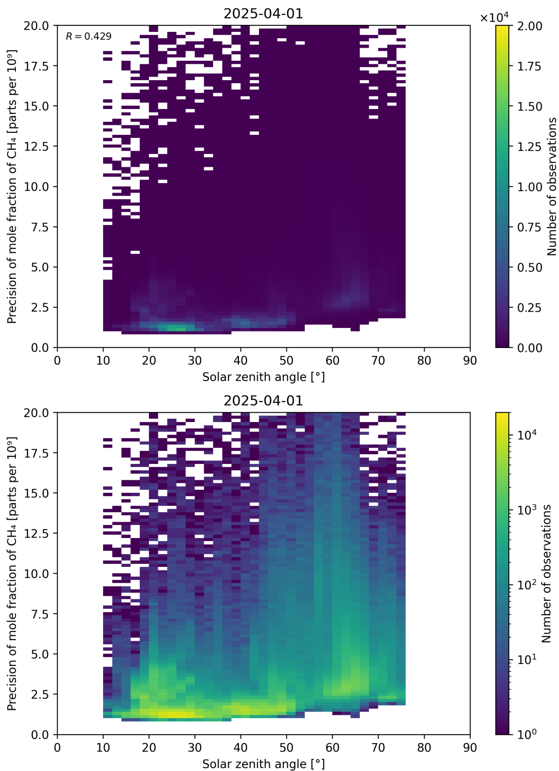
Figure 101: Scatter density plot of “Solar zenith angle” against “Precision of mole fraction of \text{CH}_4 ” for 2025-03-31 to 2025-04-02.
