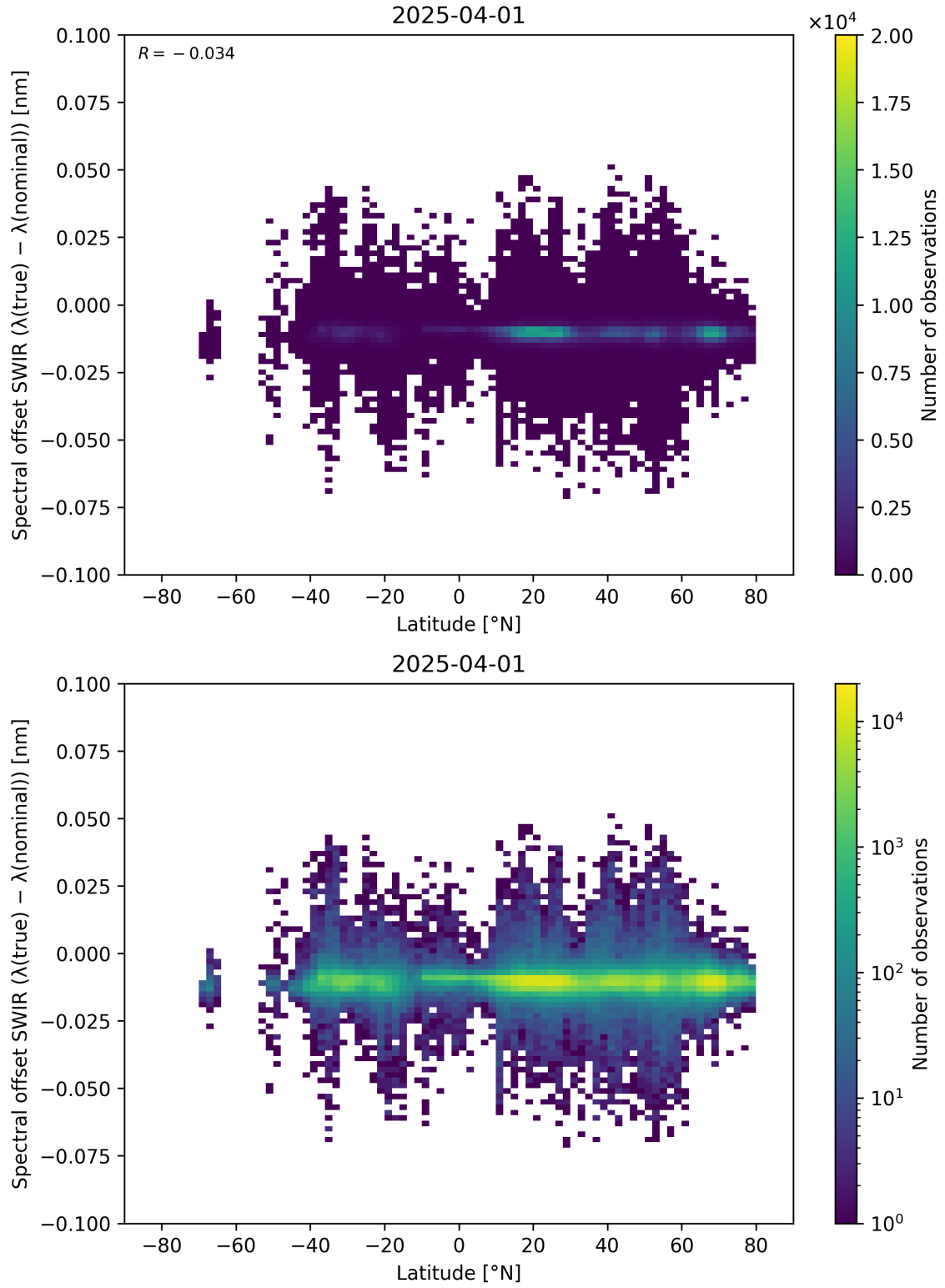
Figure 62: Scatter density plot of “Latitude” against “Spectral offset SWIR ( \lambda_{\text{true}} - \lambda_{\text{nominal}} )” for 2025-03-31 to 2025-04-02.
