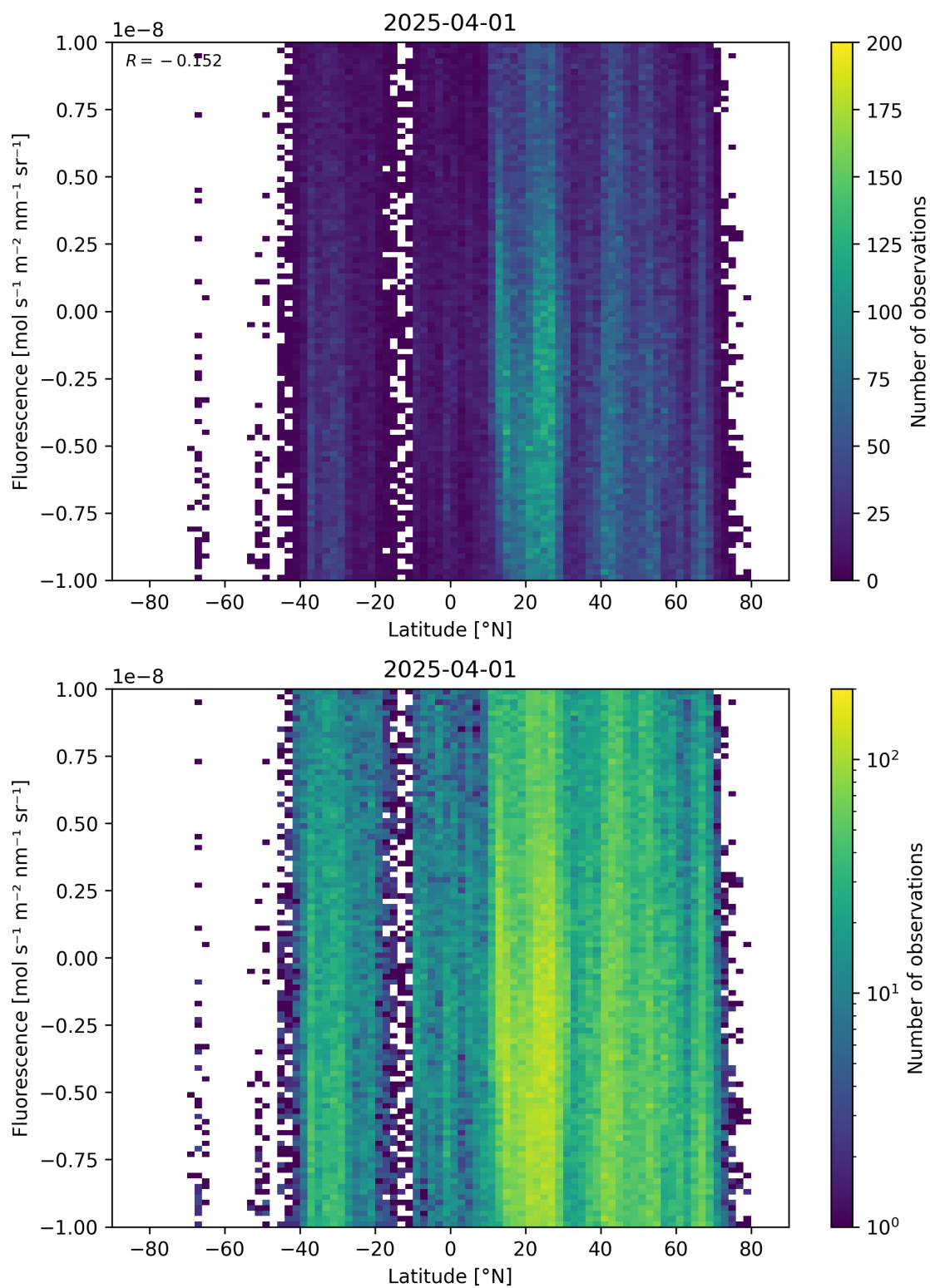
Figure 56: Scatter density plot of “Latitude” against “Fluorescence” for 2025-03-31 to 2025-04-02.
