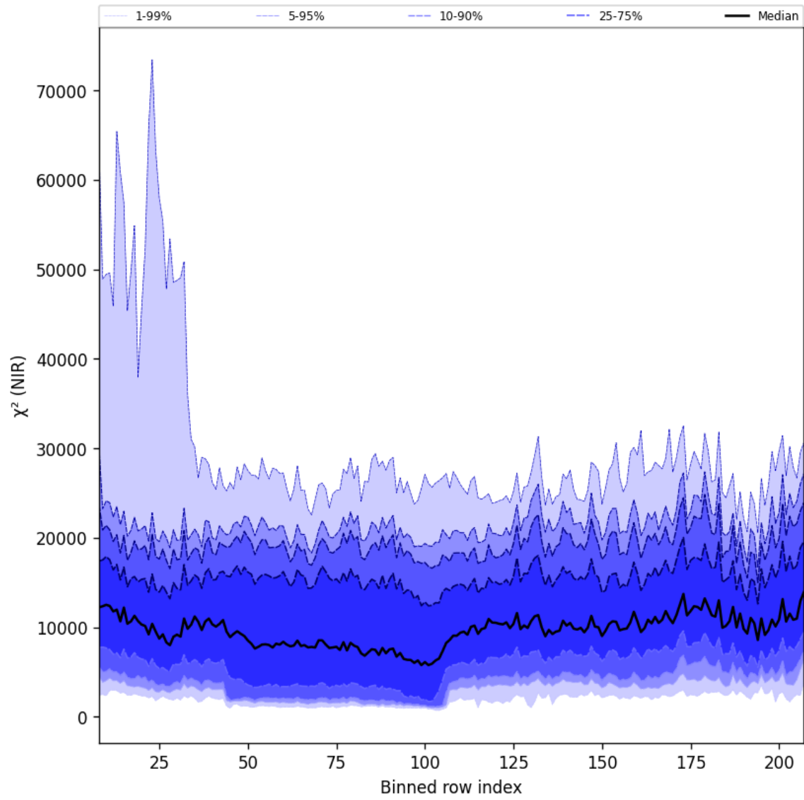
Figure 40: Along track statistics of " \chi^2 (NIR)" for 2025-03-31 to 2025-04-02
