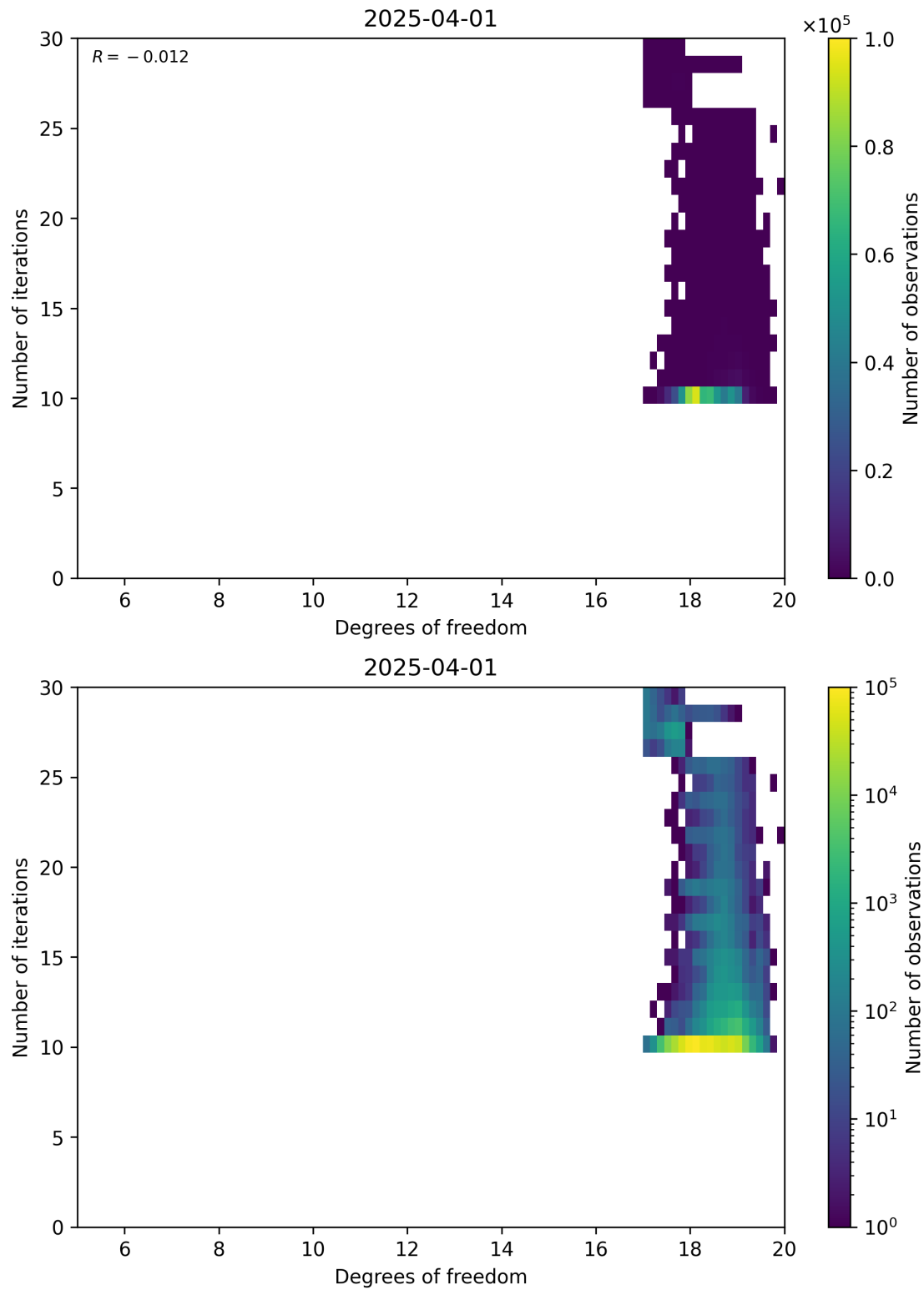
Figure 52: Scatter density plot of “Degrees of freedom” against “Number of iterations” for 2025-03-31 to 2025-04-02.
