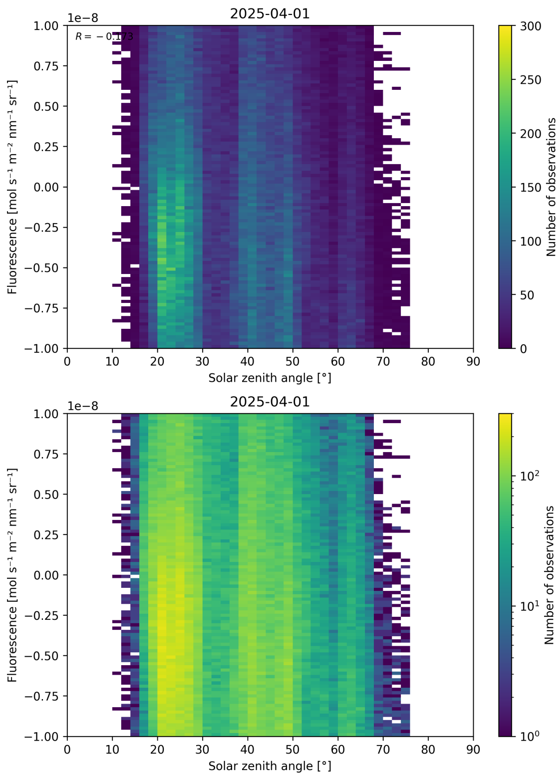
Figure 97: Scatter density plot of “Solar zenith angle” against “Fluorescence” for 2025-03-31 to 2025-04-02.
