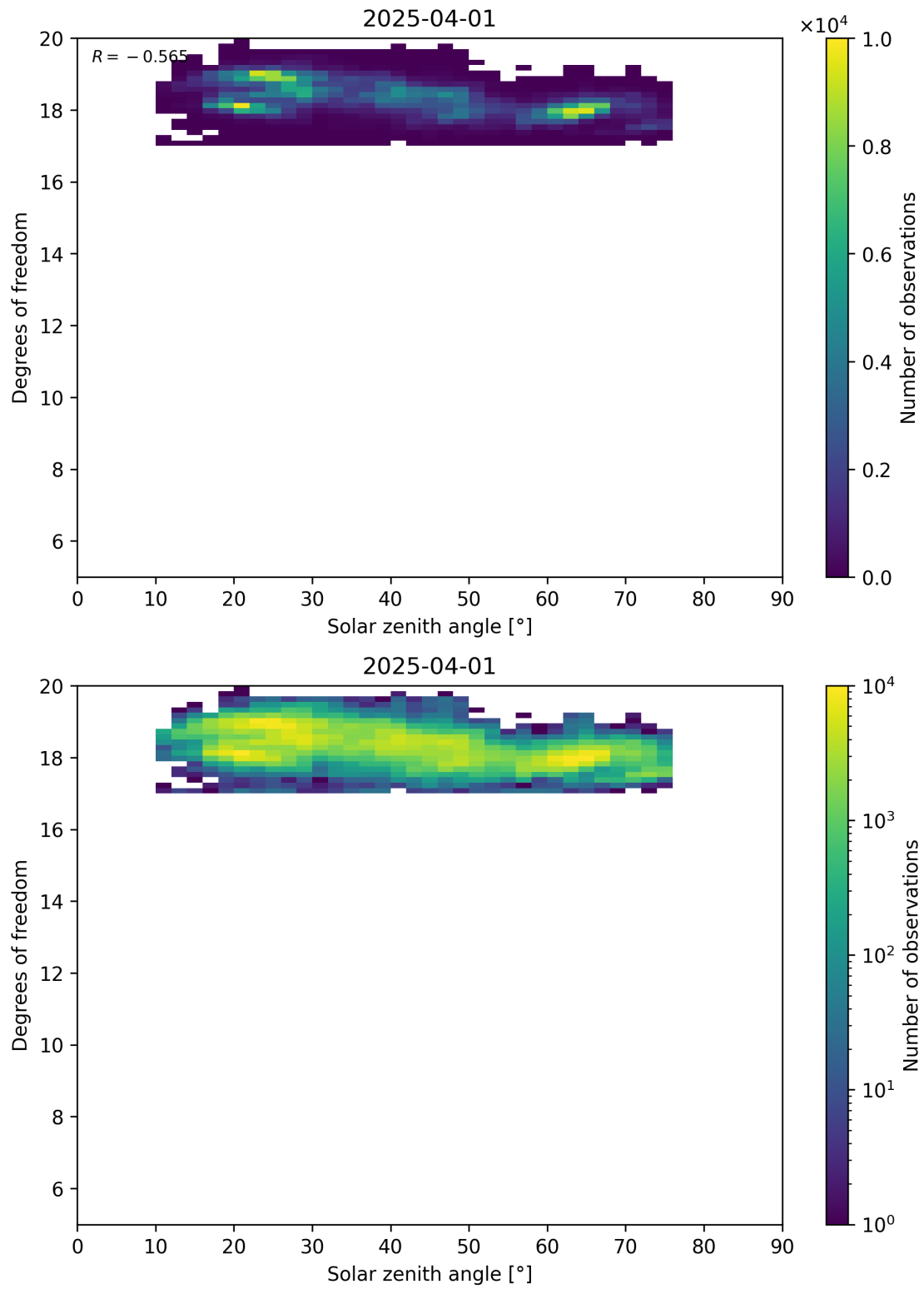
Figure 96: Scatter density plot of “Solar zenith angle” against “Degrees of freedom” for 2025-03-31 to 2025-04-02.
