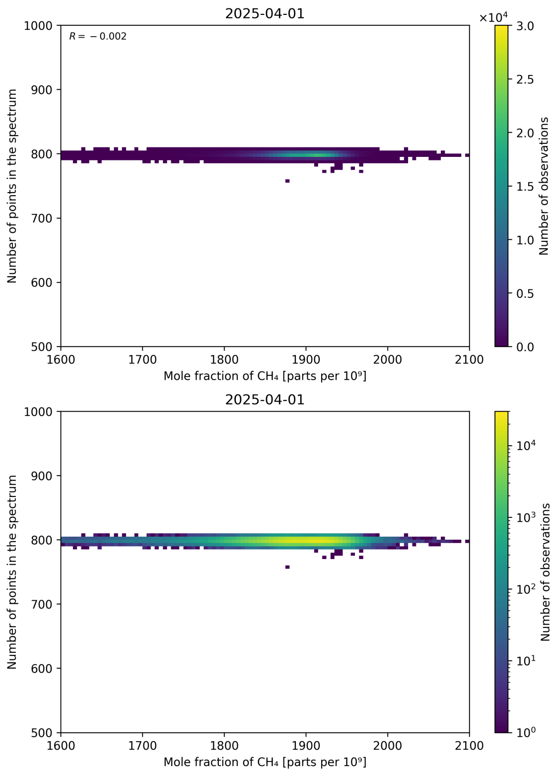
Figure 77: Scatter density plot of “Mole fraction of CH 4 ” against “Number of points in the spectrum” for 2025-03-31 to 2025-04-02.
