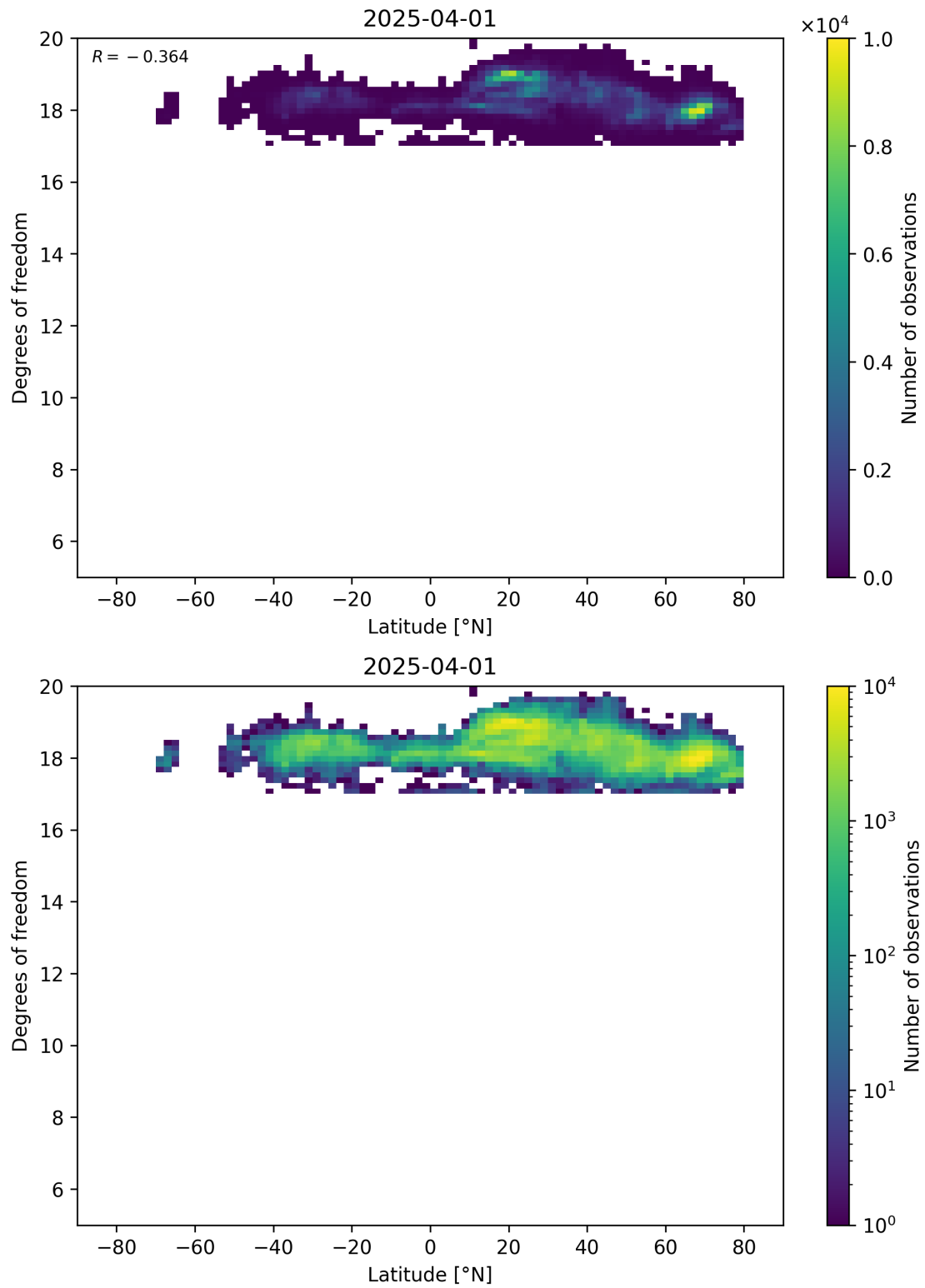
Figure 55: Scatter density plot of “Latitude” against “Degrees of freedom” for 2025-03-31 to 2025-04-02.
