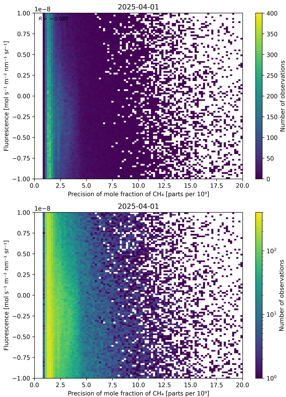
Figure 81: Scatter density plot of “Precision of mole fraction of \text{CH}_4 ” against “Fluorescence” for 2025-03-31 to 2025-04-02.
