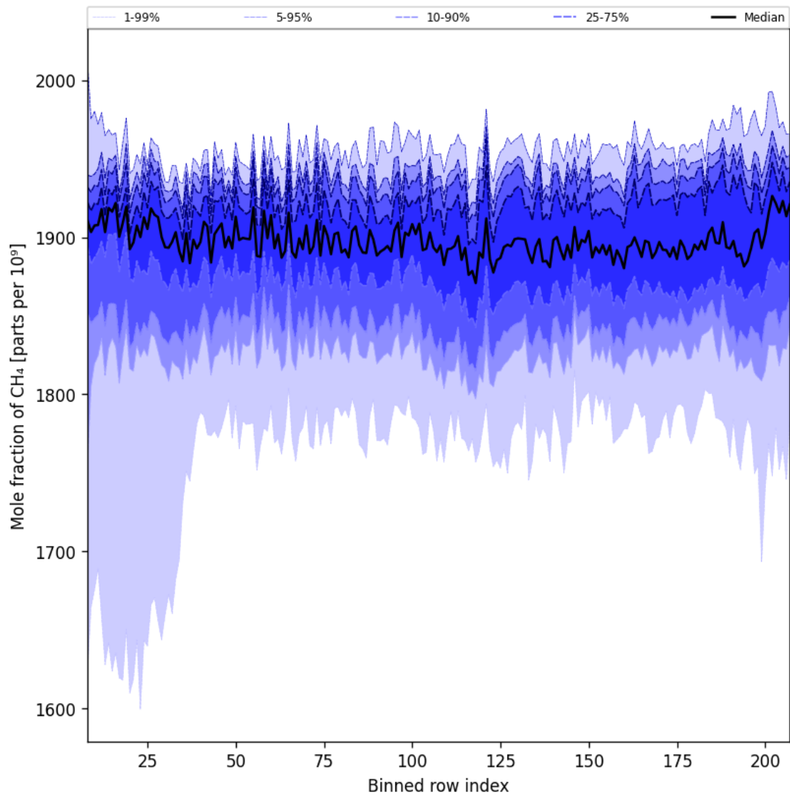
Figure 34: Along track statistics of “Mole fraction of CH 4 ” for 2025-03-31 to 2025-04-02
