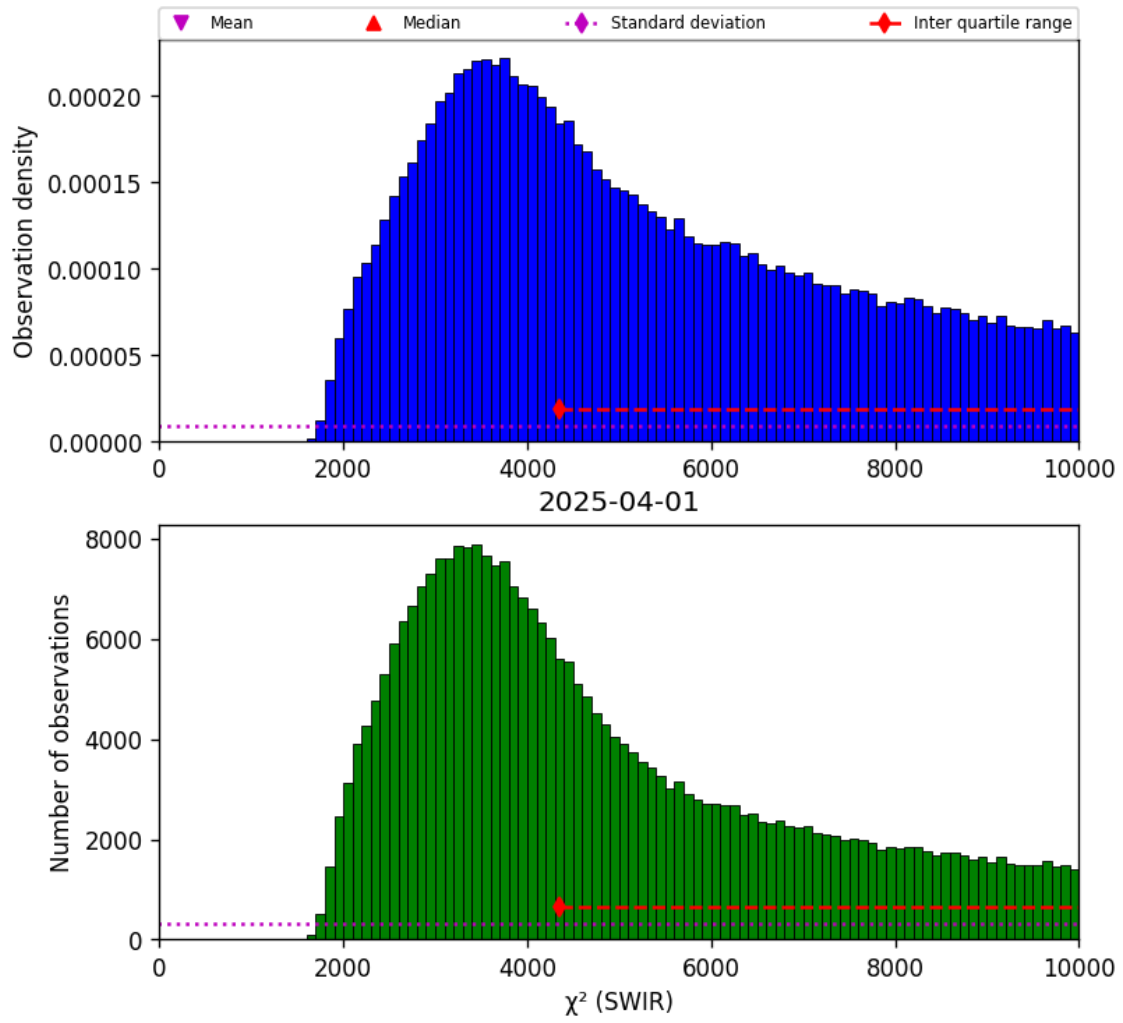
Figure 28: Histogram of “ \chi^2 (SWIR)” for 2025-03-31 to 2025-04-02
