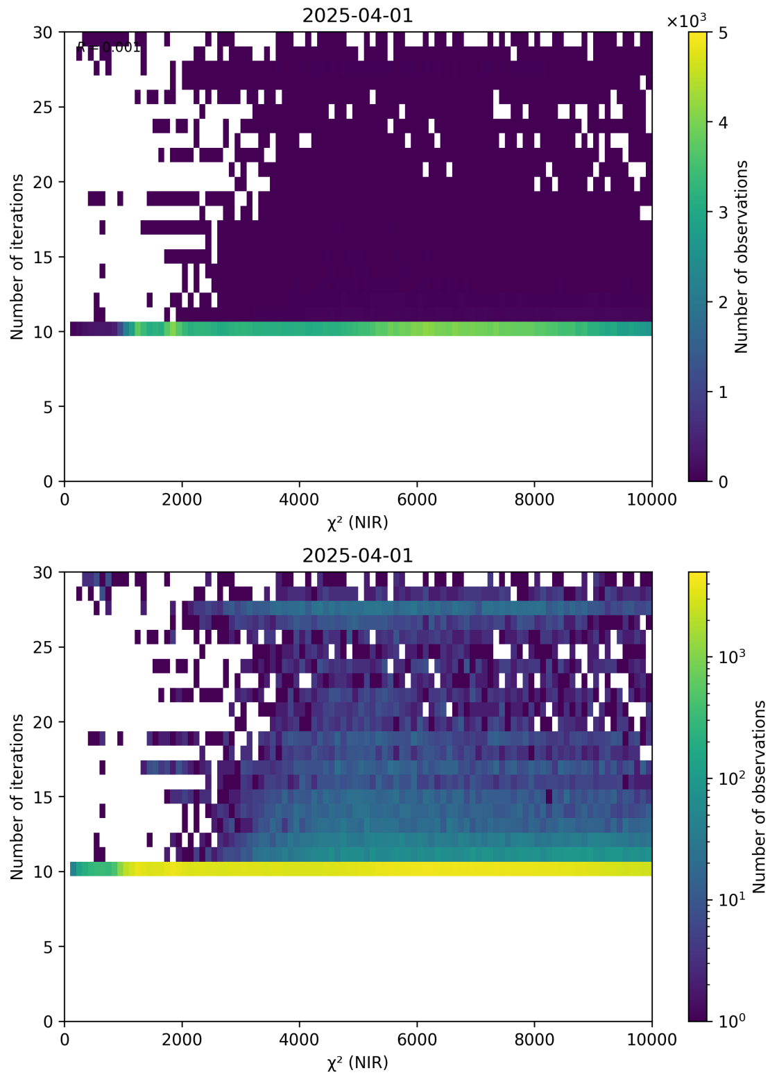
Figure 46: Scatter density plot of “ \chi^2 (NIR)” against “Number of iterations” for 2025-03-31 to 2025-04-02.
