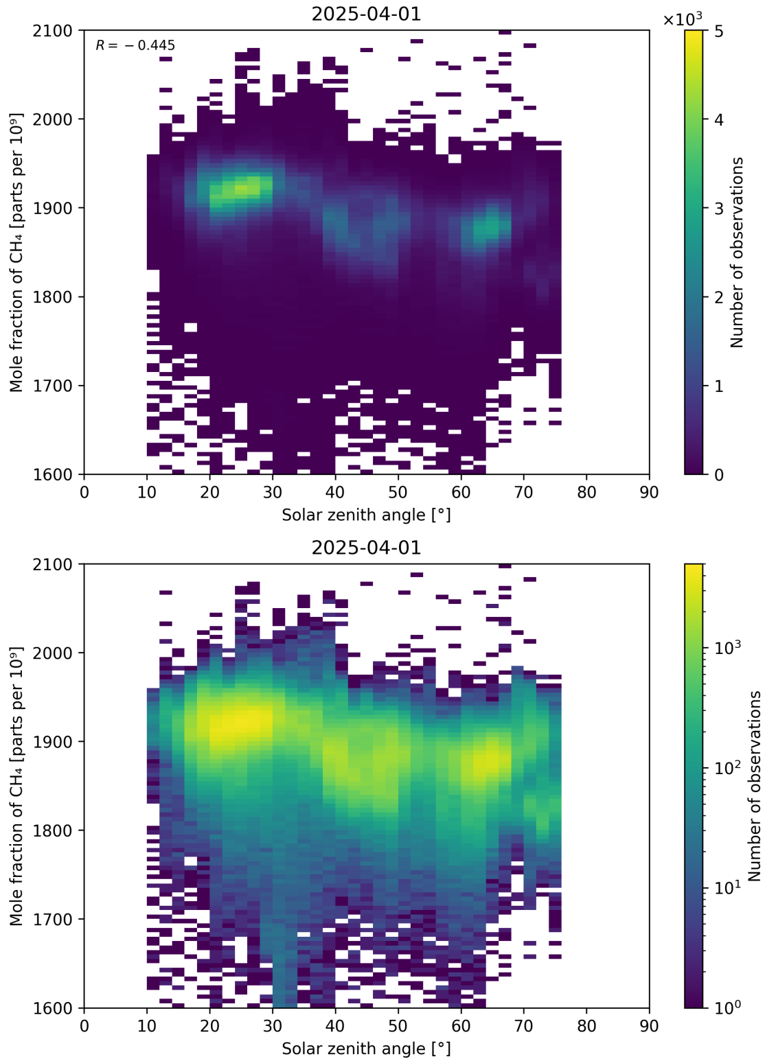
Figure 99: Scatter density plot of “Solar zenith angle” against “Mole fraction of CH 4 ” for 2025-03-31 to 2025-04-02.
