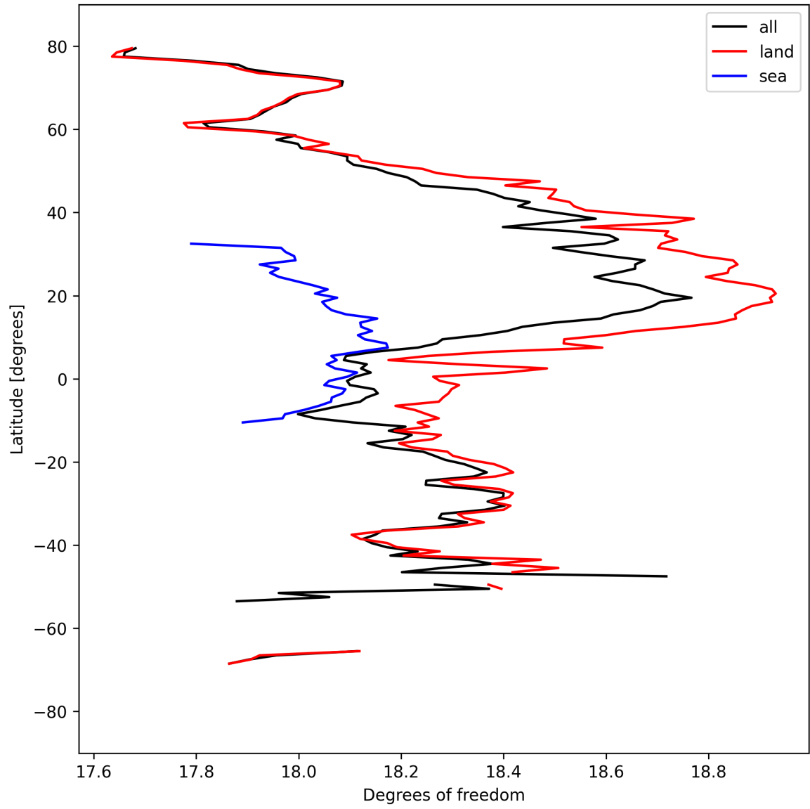
Figure 19: Zonal average of “Degrees of freedom” for 2025-03-31 to 2025-04-02.
