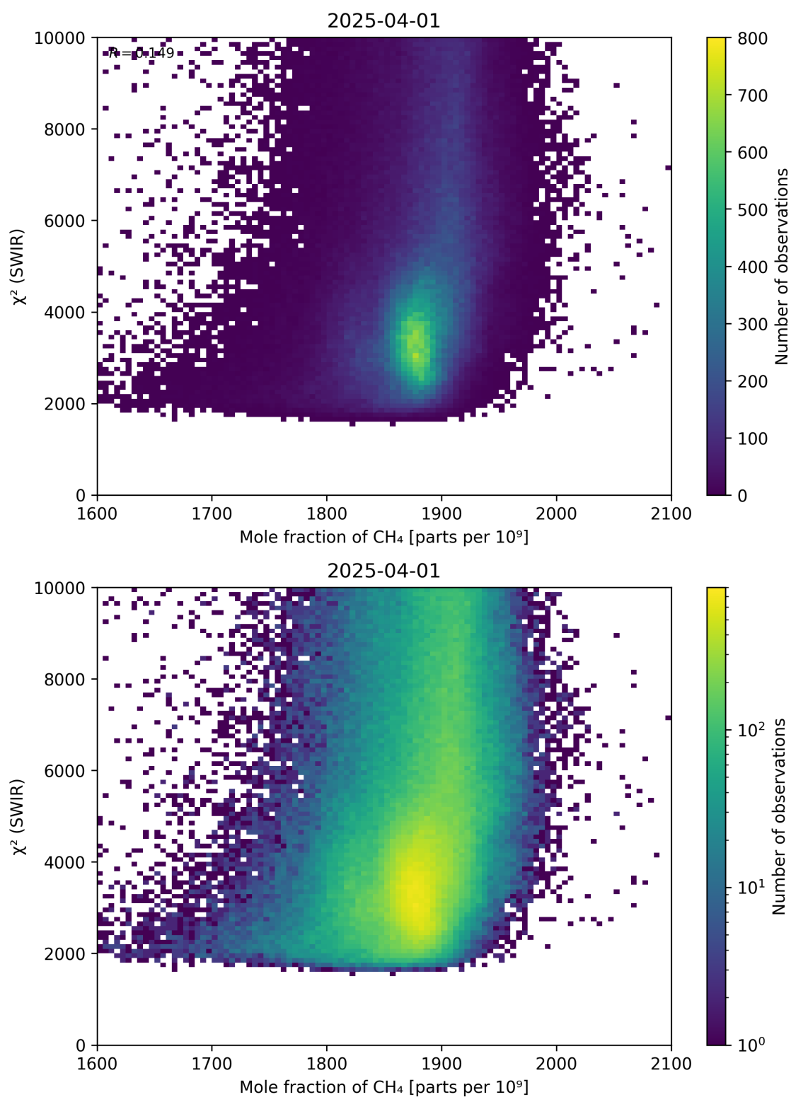
Figure 71: Scatter density plot of “Mole fraction of CH 4 ” against “ \chi^2 (SWIR)” for 2025-03-31 to 2025-04-02.
