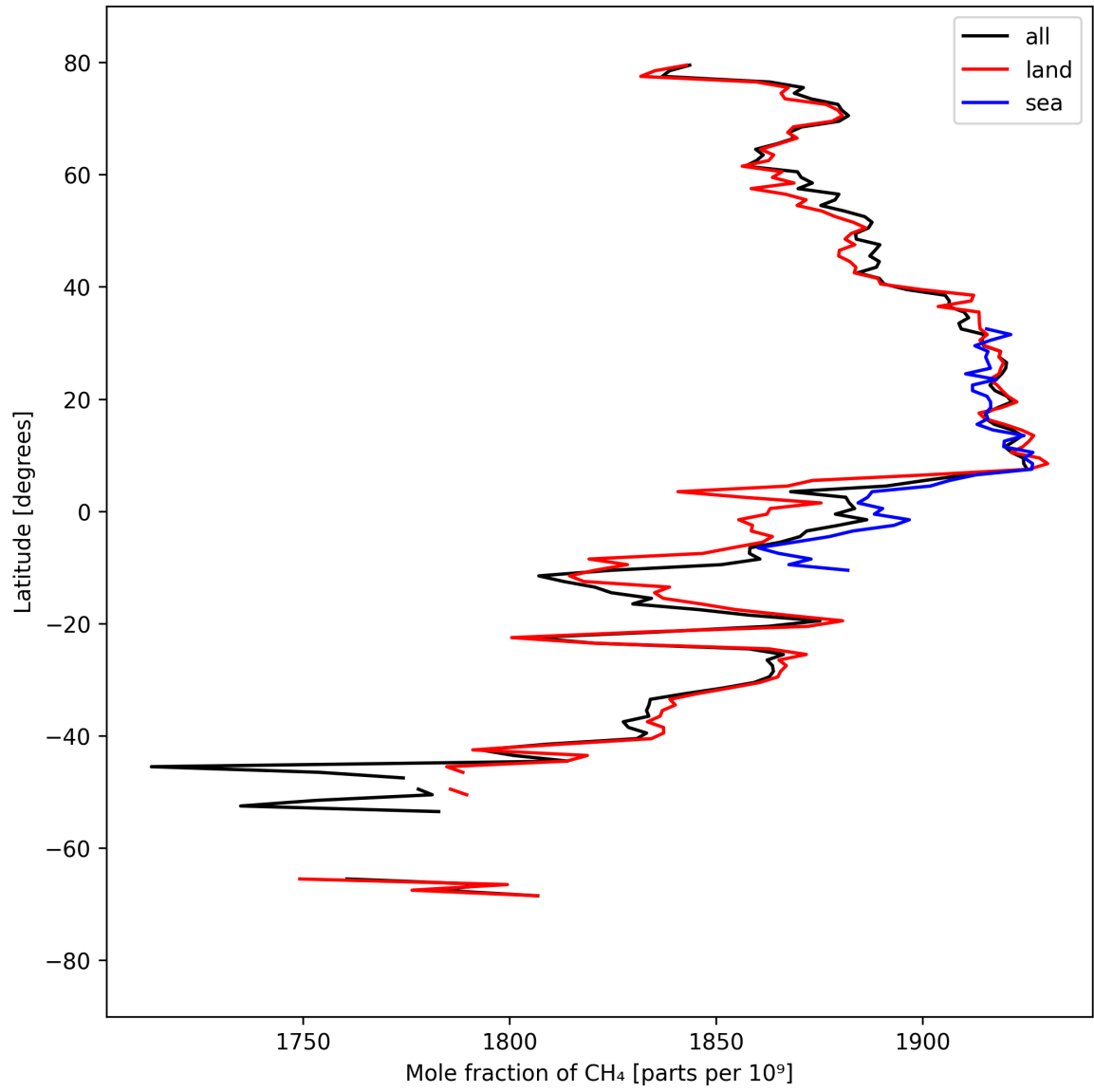
Figure 12: Zonal average of “Mole fraction of CH 4 ” for 2025-03-31 to 2025-04-02.
