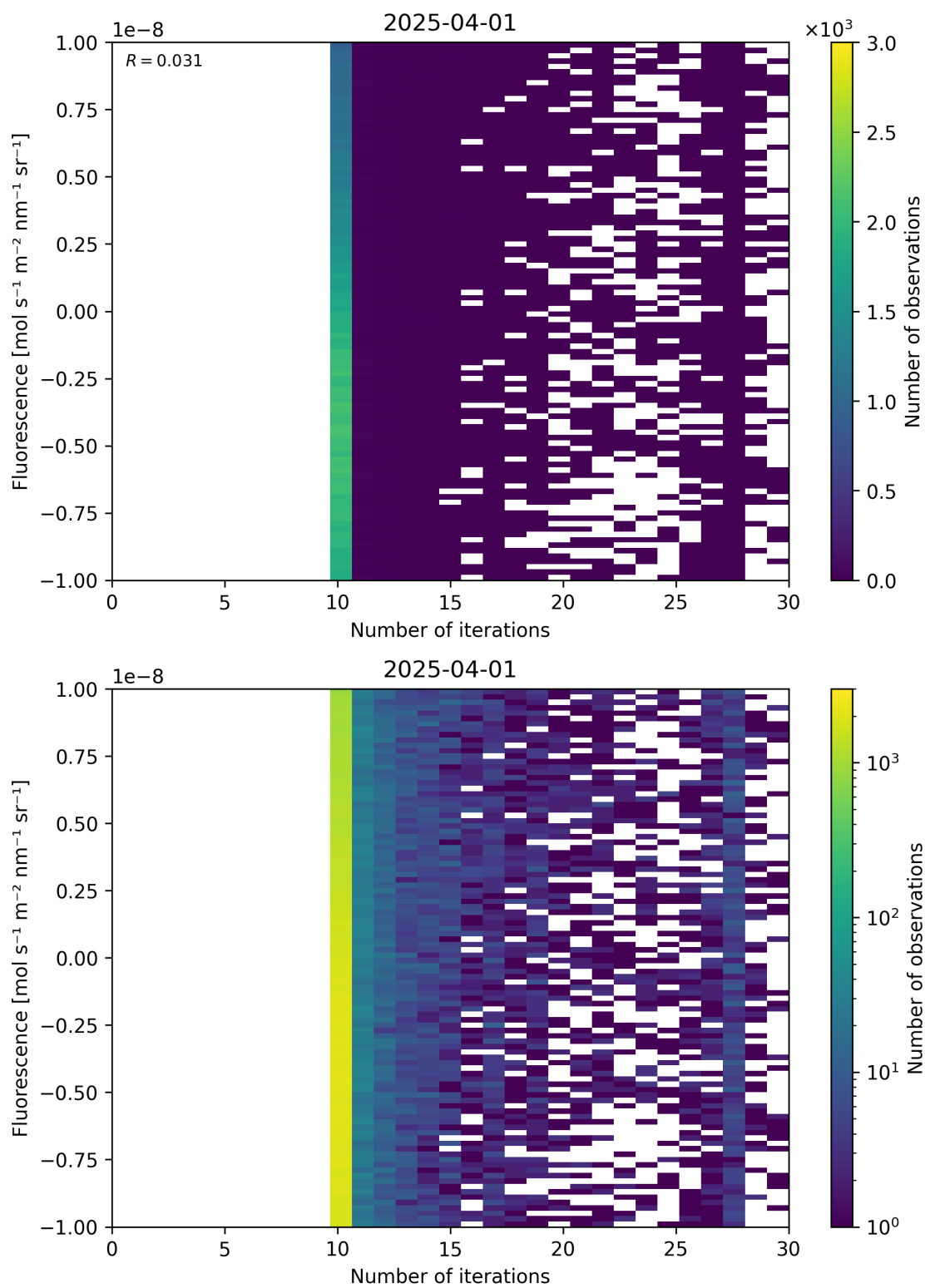
Figure 87: Scatter density plot of “Number of iterations” against “Fluorescence” for 2025-03-31 to 2025-04-02.
