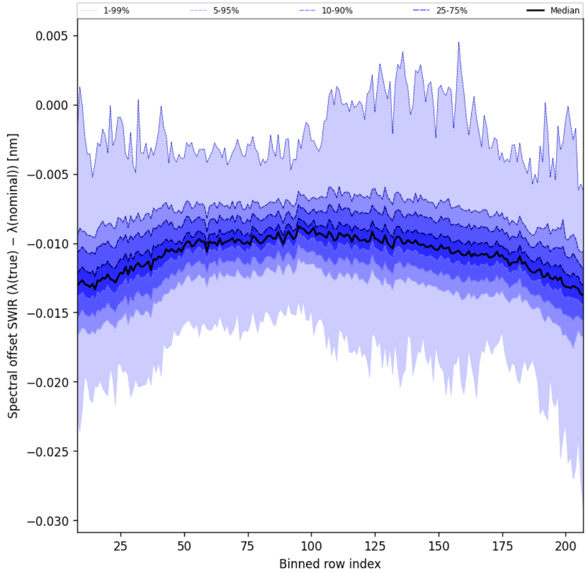
Figure 38: Along track statistics of “Spectral offset SWIR ( \lambda_{\text{true}} - \lambda_{\text{nominal}} )” for 2025-03-31 to 2025-04-02
