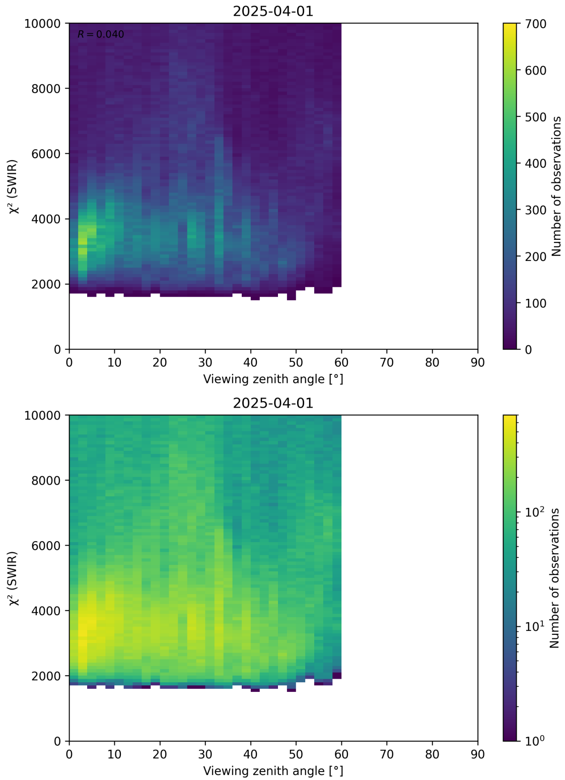
Figure 106: Scatter density plot of “Viewing zenith angle” against “ \chi^2 (SWIR)” for 2025-03-31 to 2025-04-02.
