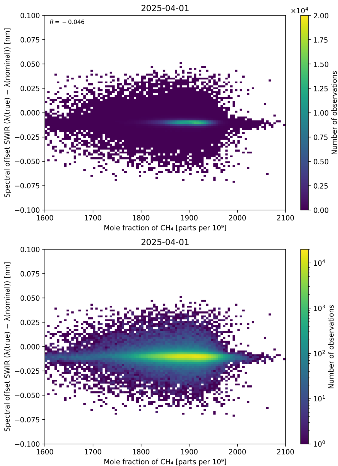
Figure 86: Scatter density plot of “Mole fraction of \text{CH}_4 ” against “Spectral offset SWIR ( \lambda_{\text{true}} - \lambda_{\text{nominal}} )” for 2025-03-31 to 2025-04-02.
