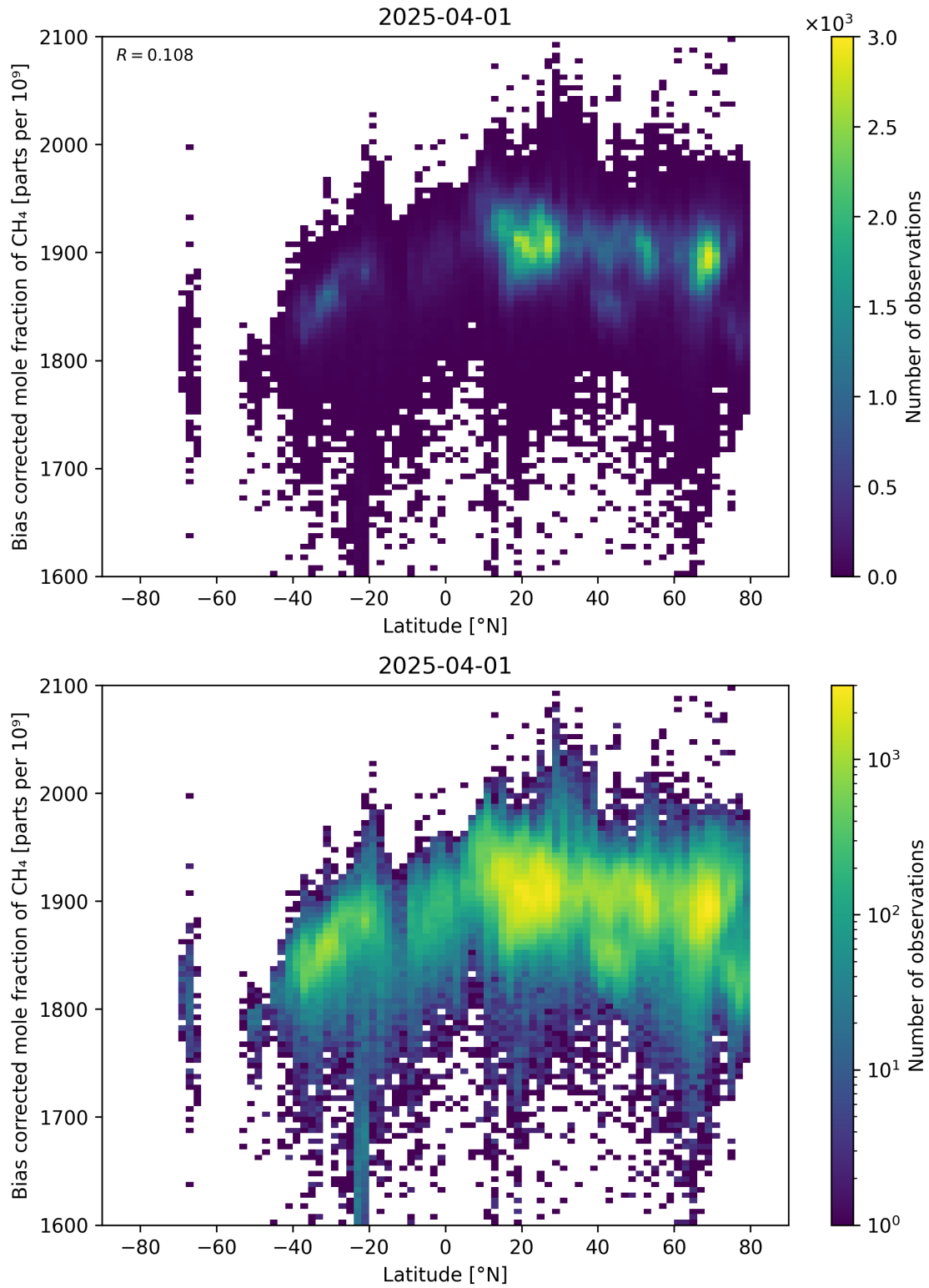
Figure 58: Scatter density plot of “Latitude” against “Bias corrected mole fraction of CH 4 ” for 2025-03-31 to 2025-04-02.
