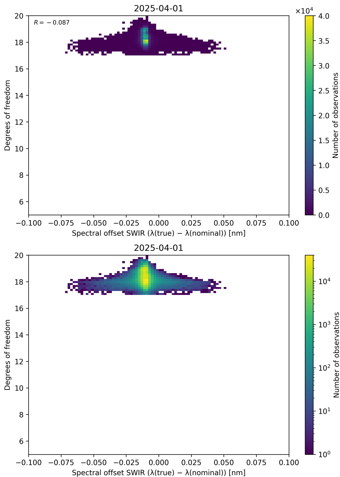
Figure 119: Scatter density plot of “Spectral offset SWIR ( \lambda_{\text{true}} - \lambda_{\text{nominal}} )” against “Degrees of freedom” for 2025-03-31 to 2025-04-02.
