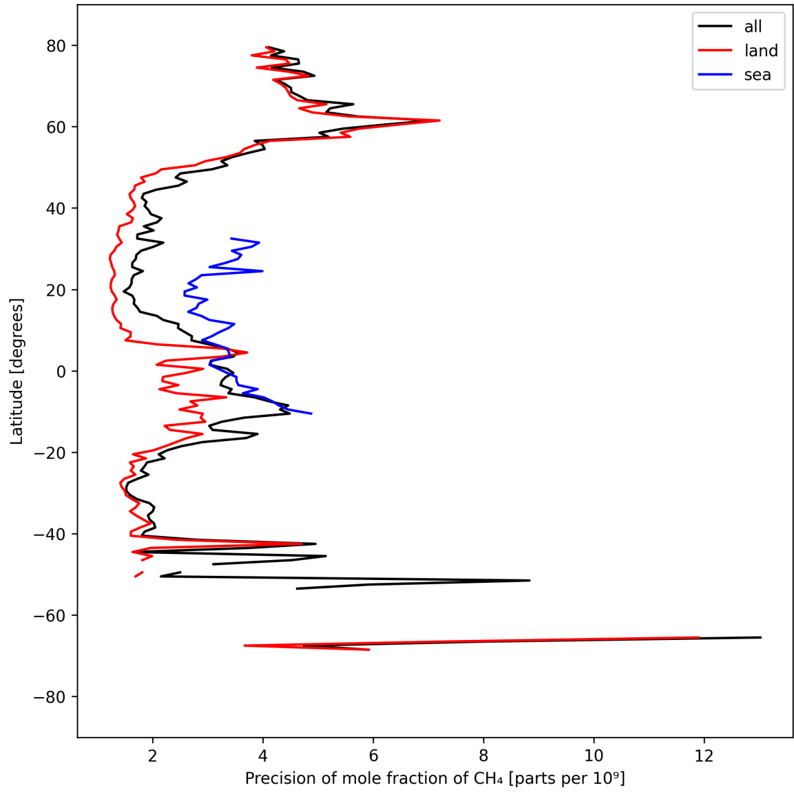
Figure 13: Zonal average of “Precision of mole fraction of CH 4 ” for 2025-03-31 to 2025-04-02.
