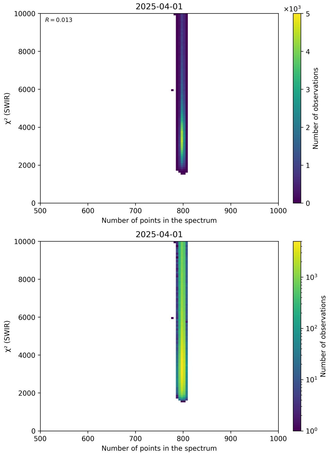
Figure 89: Scatter density plot of “Number of points in the spectrum” against “ \chi^2 (SWIR)” for 2025-03-31 to 2025-04-02.
