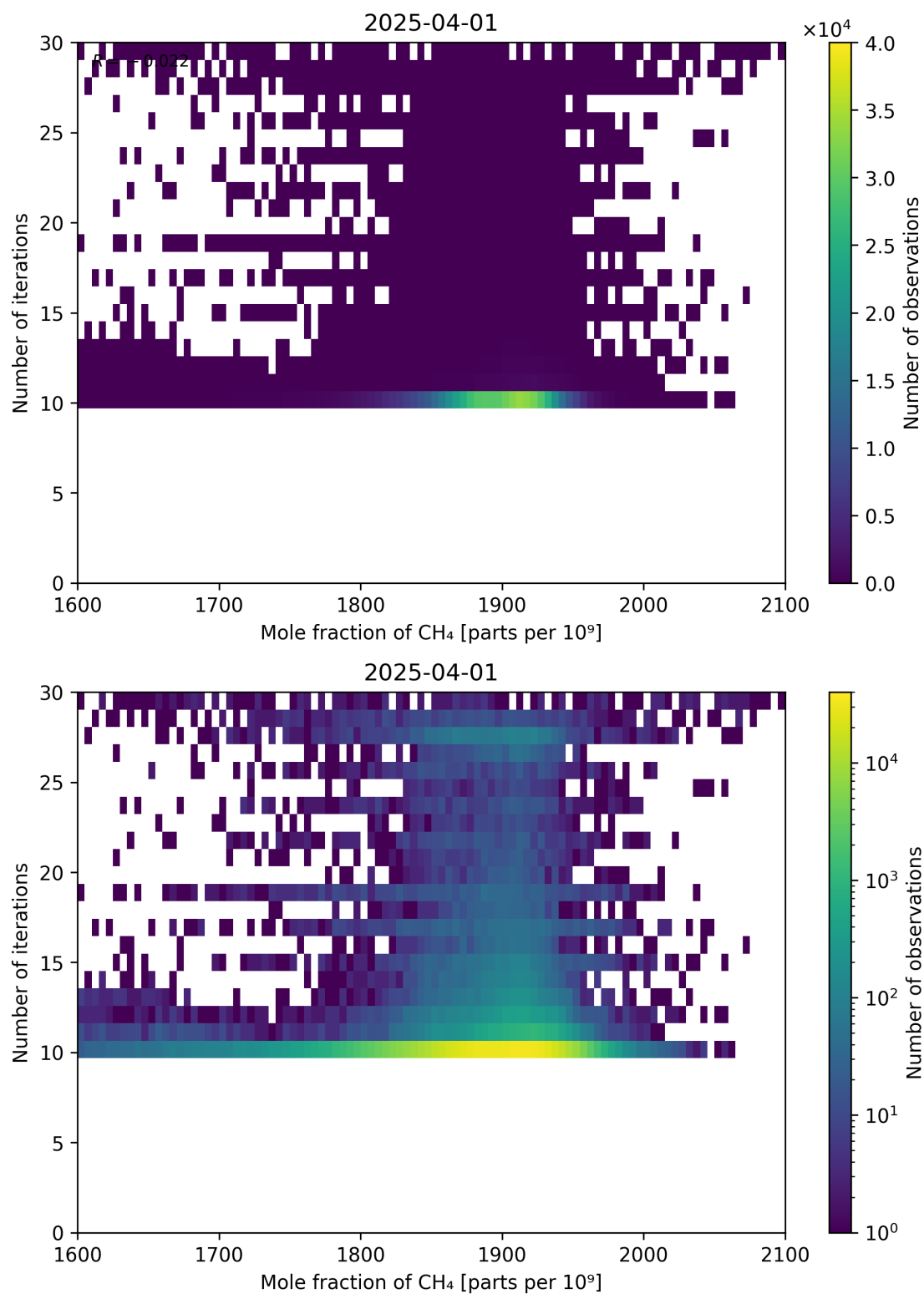
Figure 76: Scatter density plot of “Mole fraction of CH 4 ” against “Number of iterations” for 2025-03-31 to 2025-04-02.
