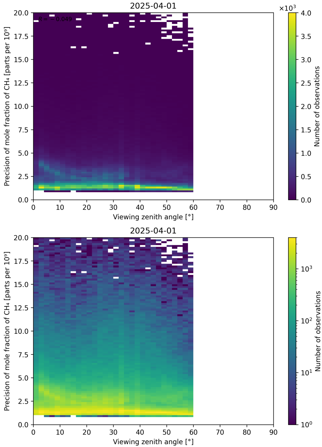
Figure 112: Scatter density plot of “Viewing zenith angle” against “Precision of mole fraction of CH 4 ” for 2025-03-31 to 2025-04-02.
