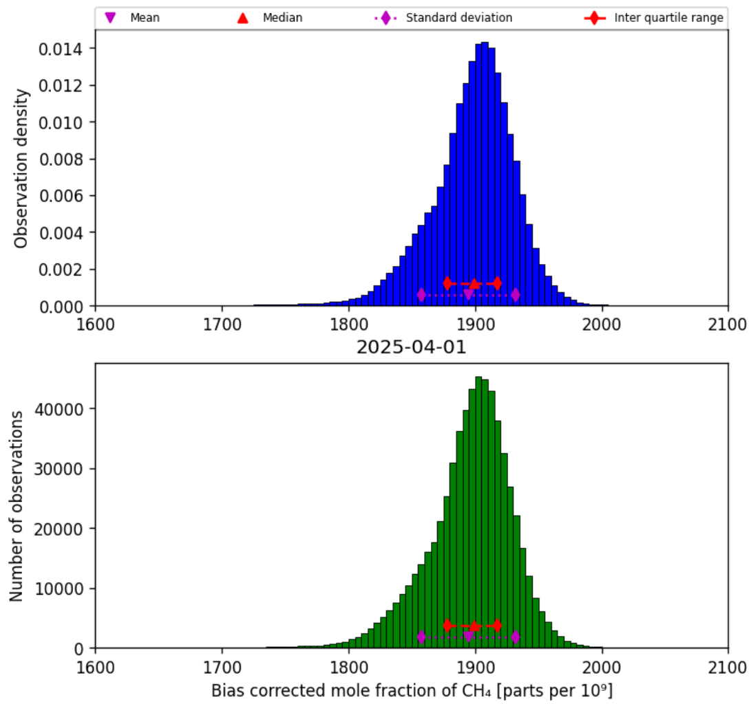
Figure 25: Histogram of “Bias corrected mole fraction of CH 4 ” for 2025-03-31 to 2025-04-02
