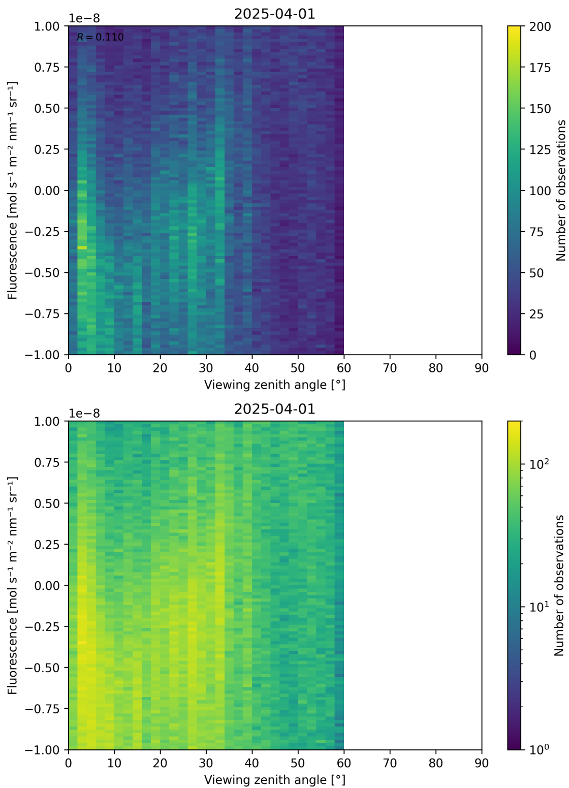
Figure 108: Scatter density plot of “Viewing zenith angle” against “Fluorescence” for 2025-03-31 to 2025-04-02.
