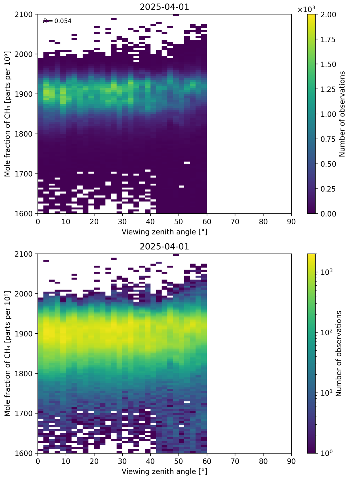
Figure 110: Scatter density plot of “Viewing zenith angle” against “Mole fraction of CH 4 ” for 2025-03-31 to 2025-04-02.
