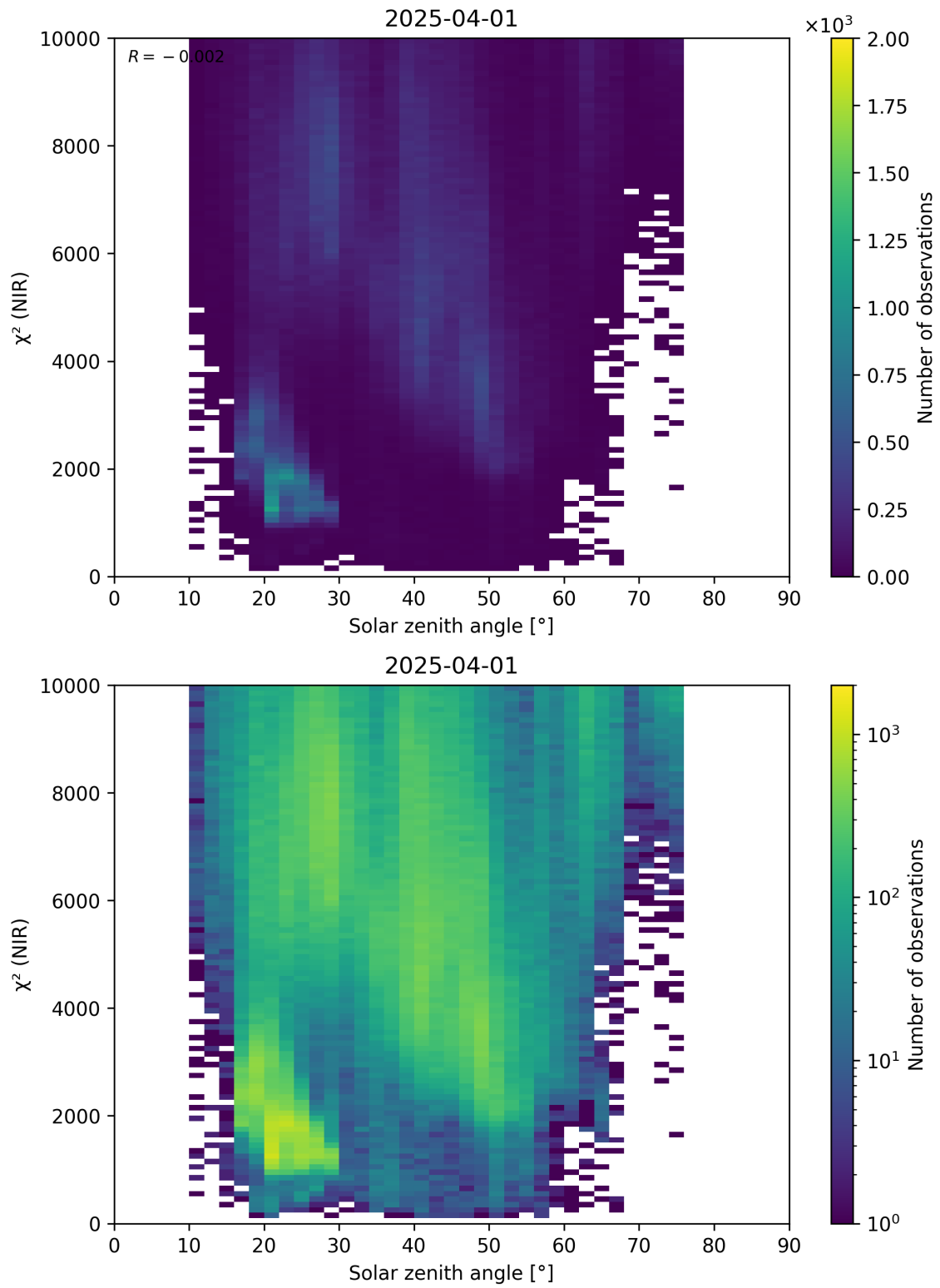
Figure 94: Scatter density plot of “Solar zenith angle” against “ \chi^2 (NIR)” for 2025-03-31 to 2025-04-02.
