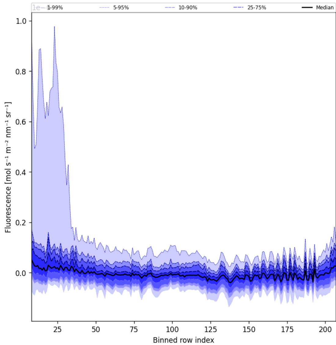
Figure 43: Along track statistics of “Fluorescence” for 2025-03-31 to 2025-04-02
