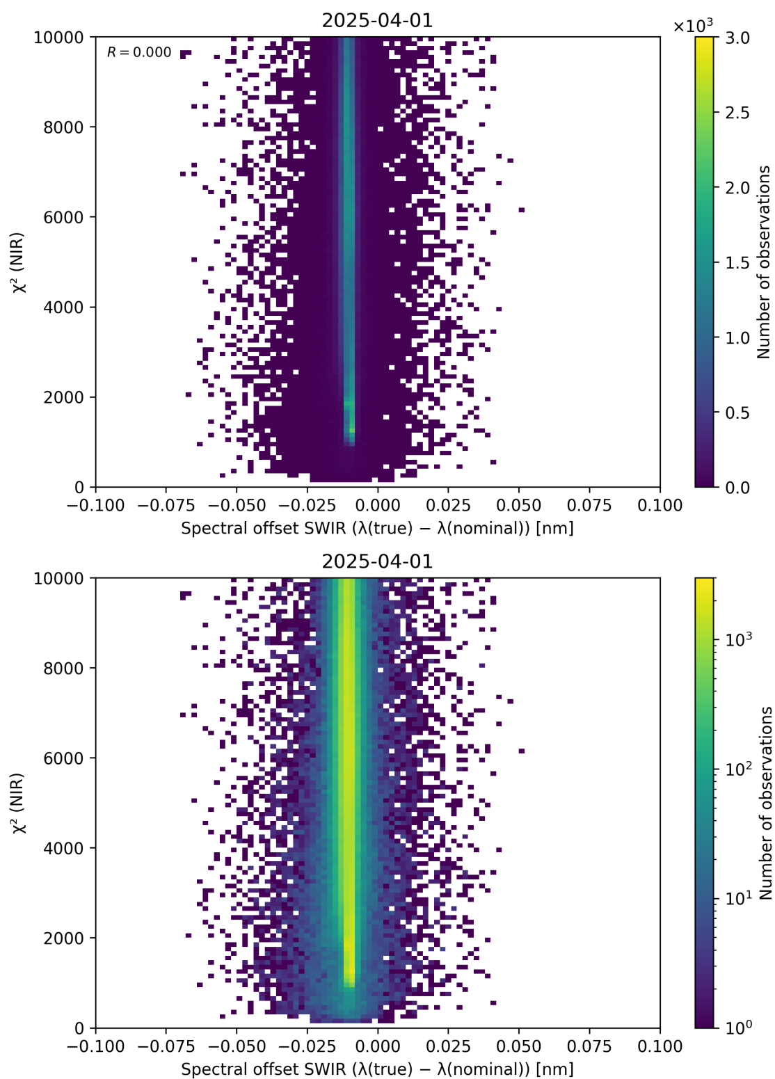
Figure 117: Scatter density plot of “Spectral offset SWIR ( \lambda_{\text{true}} - \lambda_{\text{nominal}} )” against “ \chi^2 (NIR)” for 2025-03-31 to 2025-04-02.
