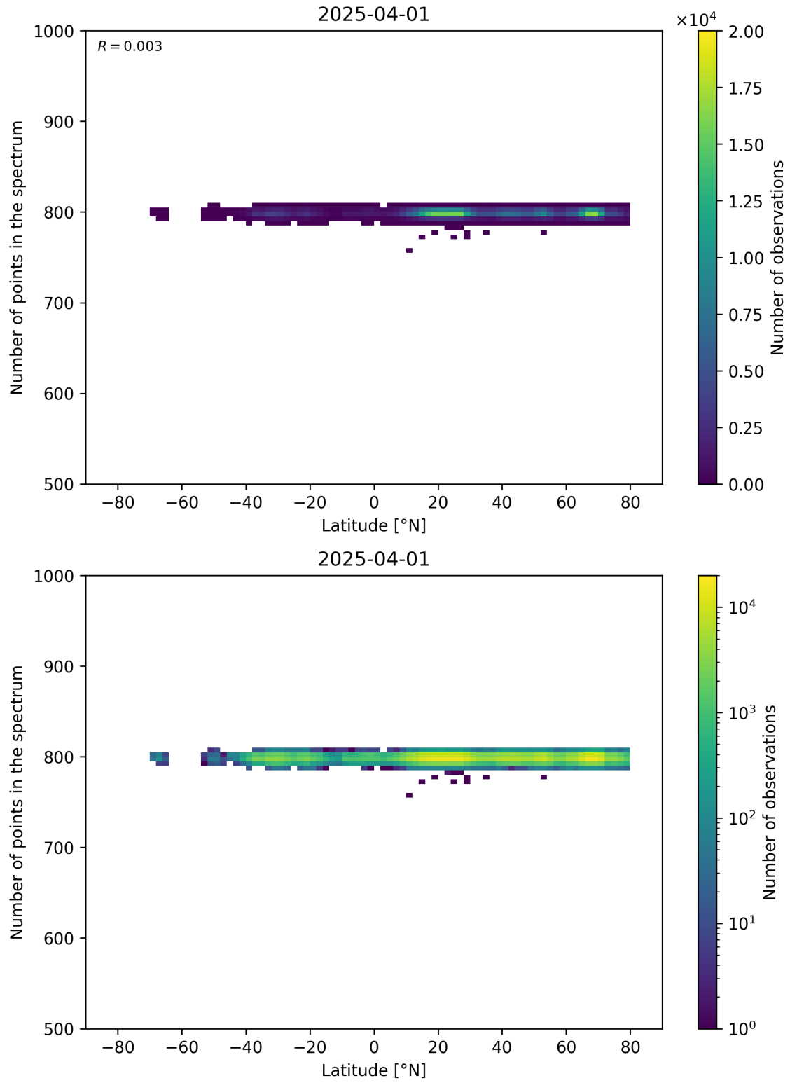
Figure 61: Scatter density plot of “Latitude” against “Number of points in the spectrum” for 2025-03-31 to 2025-04-02.
