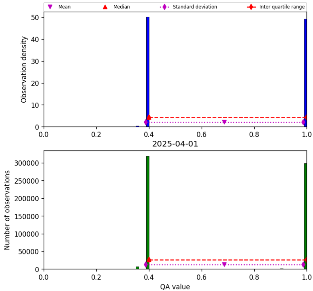
Figure 22: Histogram of “QA value” for 2025-03-31 to 2025-04-02
