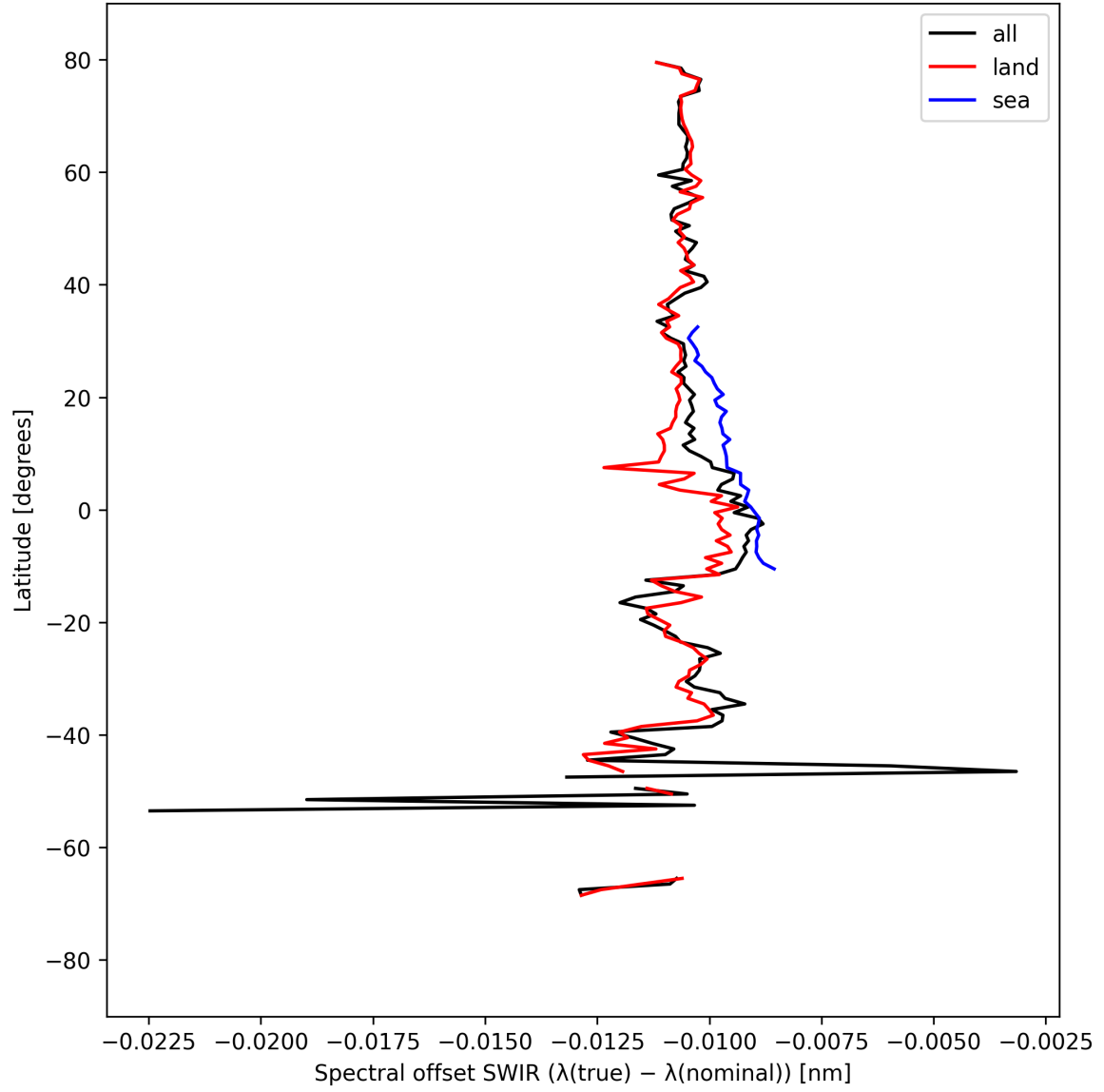
Figure 16: Zonal average of “Spectral offset SWIR ( \lambda_{\text{true}} - \lambda_{\text{nominal}} )” for 2025-03-31 to 2025-04-02.
