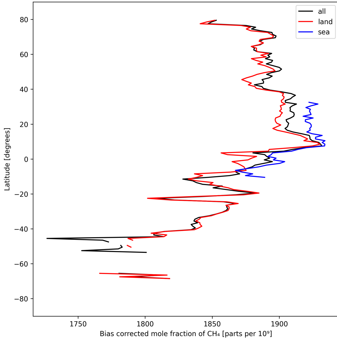
Figure 14: Zonal average of “Bias corrected mole fraction of \text{CH}_4 ” for 2025-03-31 to 2025-04-02.
