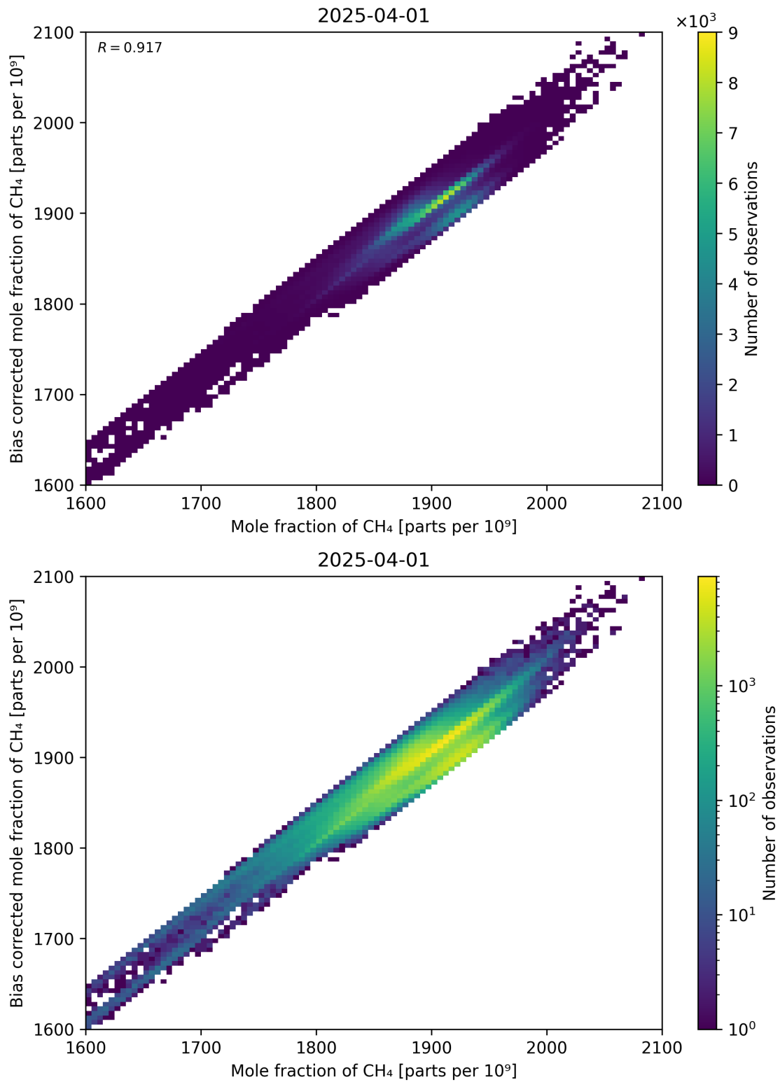
Figure 74: Scatter density plot of “Mole fraction of CH 4 ” against “Bias corrected mole fraction of CH 4 ” for 2025-03-31 to 2025-04-02.
