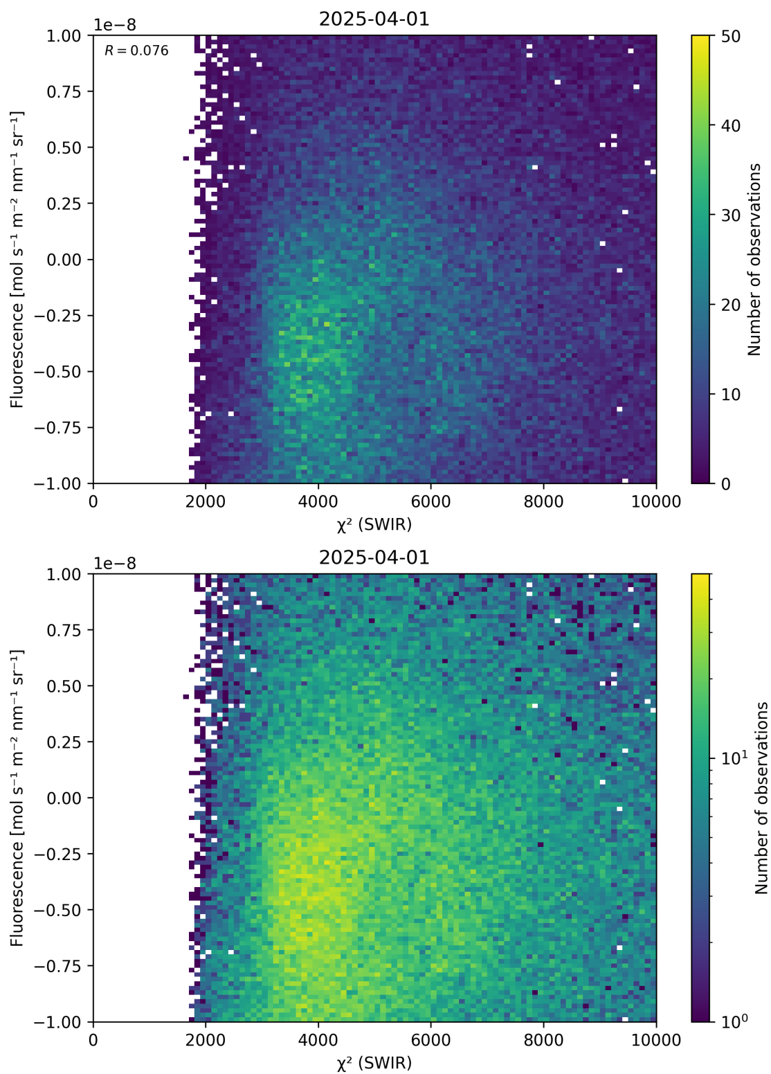
Figure 49: Scatter density plot of “ \chi^2 (SWIR)” against “Fluorescence” for 2025-03-31 to 2025-04-02.
