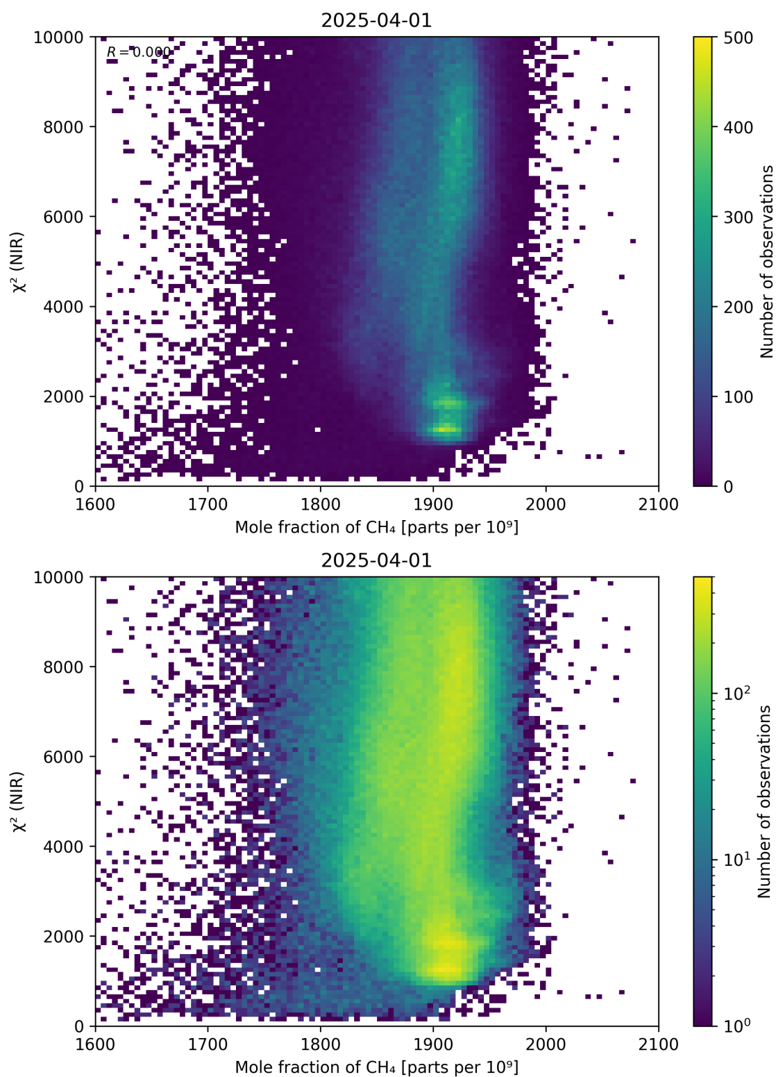
Figure 70: Scatter density plot of “Mole fraction of CH 4 ” against “ \chi^2 (NIR)” for 2025-03-31 to 2025-04-02.
