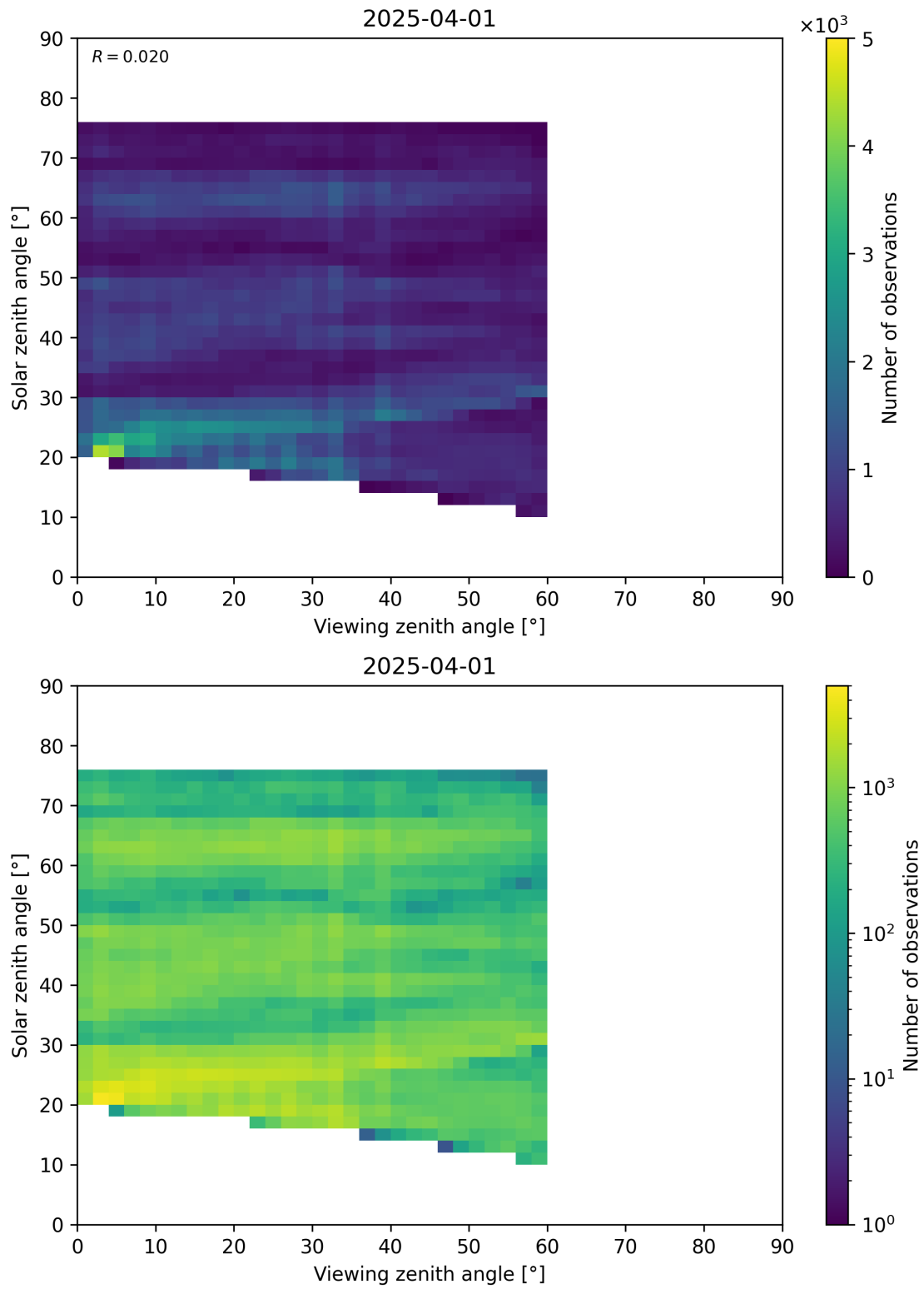
Figure 115: Scatter density plot of “Viewing zenith angle” against “Solar zenith angle” for 2025-03-31 to 2025-04-02.
