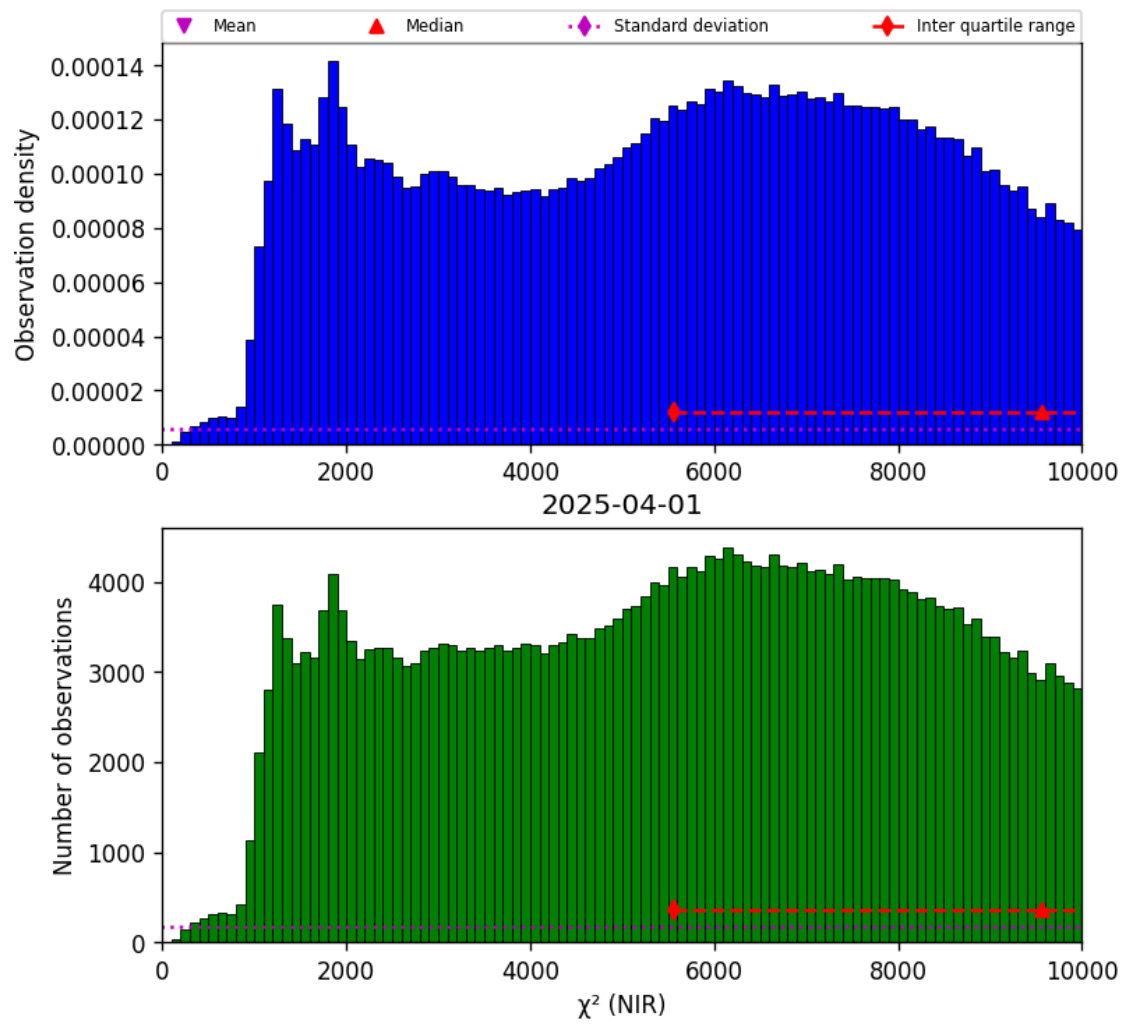
Figure 29: Histogram of " \chi^2 (NIR)" for 2025-03-31 to 2025-04-02
