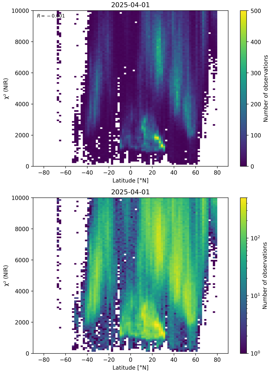
Figure 53: Scatter density plot of “Latitude” against “ \chi^2 (NIR)” for 2025-03-31 to 2025-04-02.
