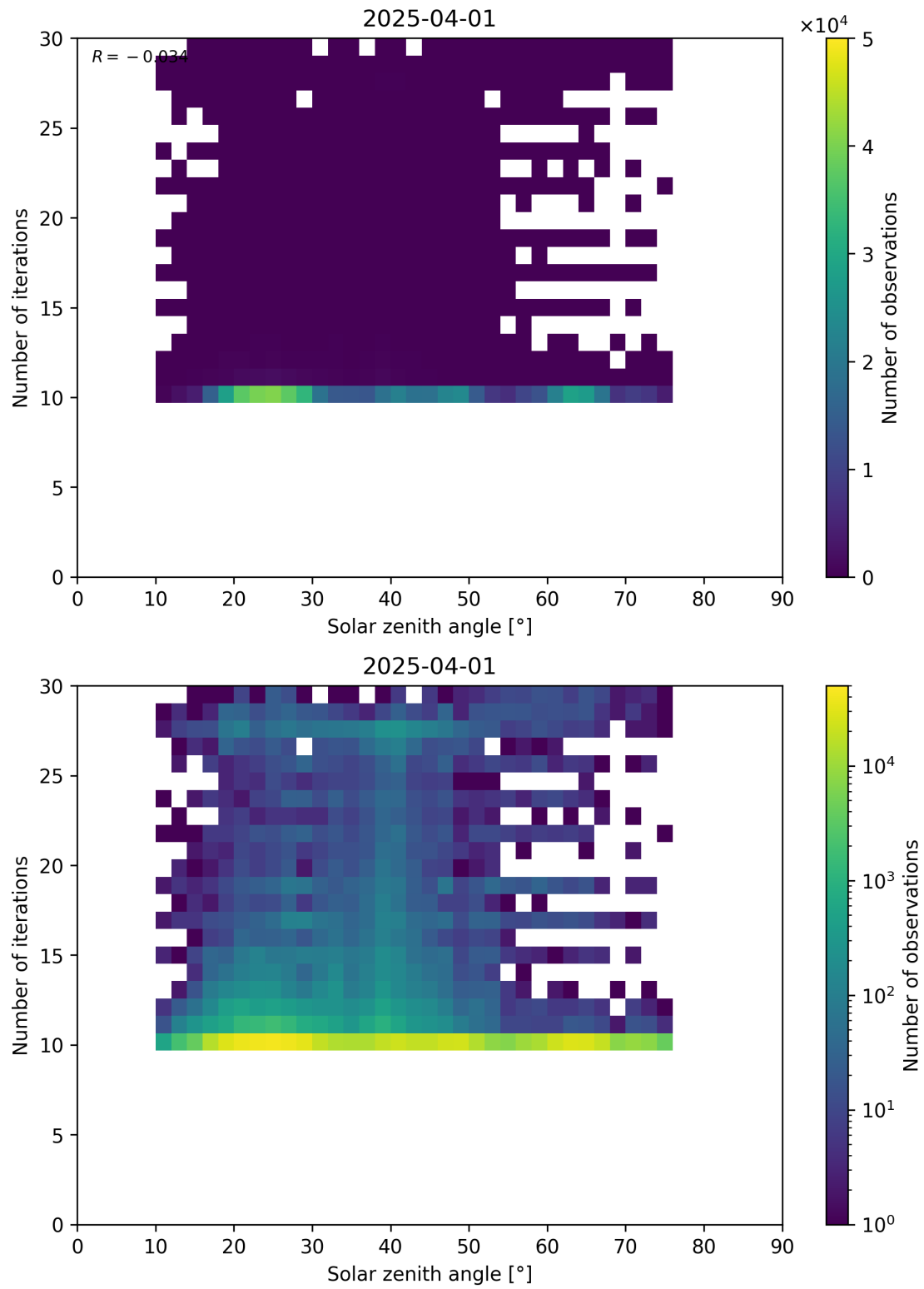
Figure 102: Scatter density plot of “Solar zenith angle” against “Number of iterations” for 2025-03-31 to 2025-04-02.
