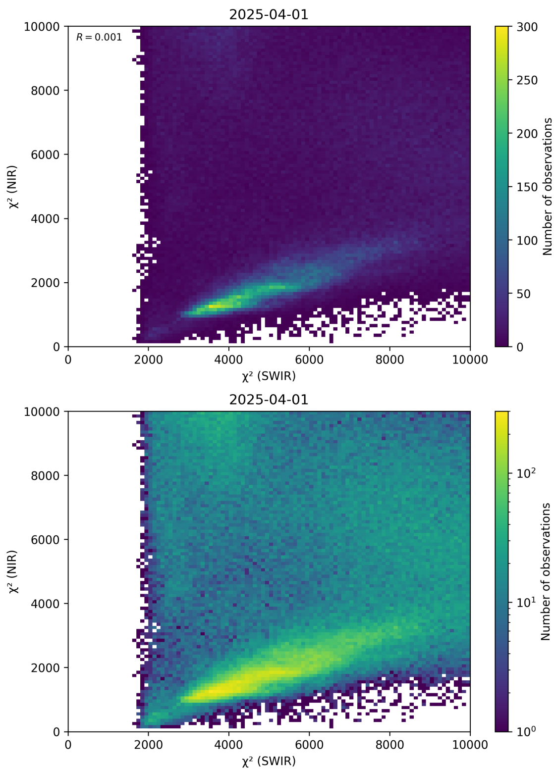
Figure 47: Scatter density plot of “ \chi^2 (SWIR)” against “ \chi^2 (NIR)” for 2025-03-31 to 2025-04-02.
