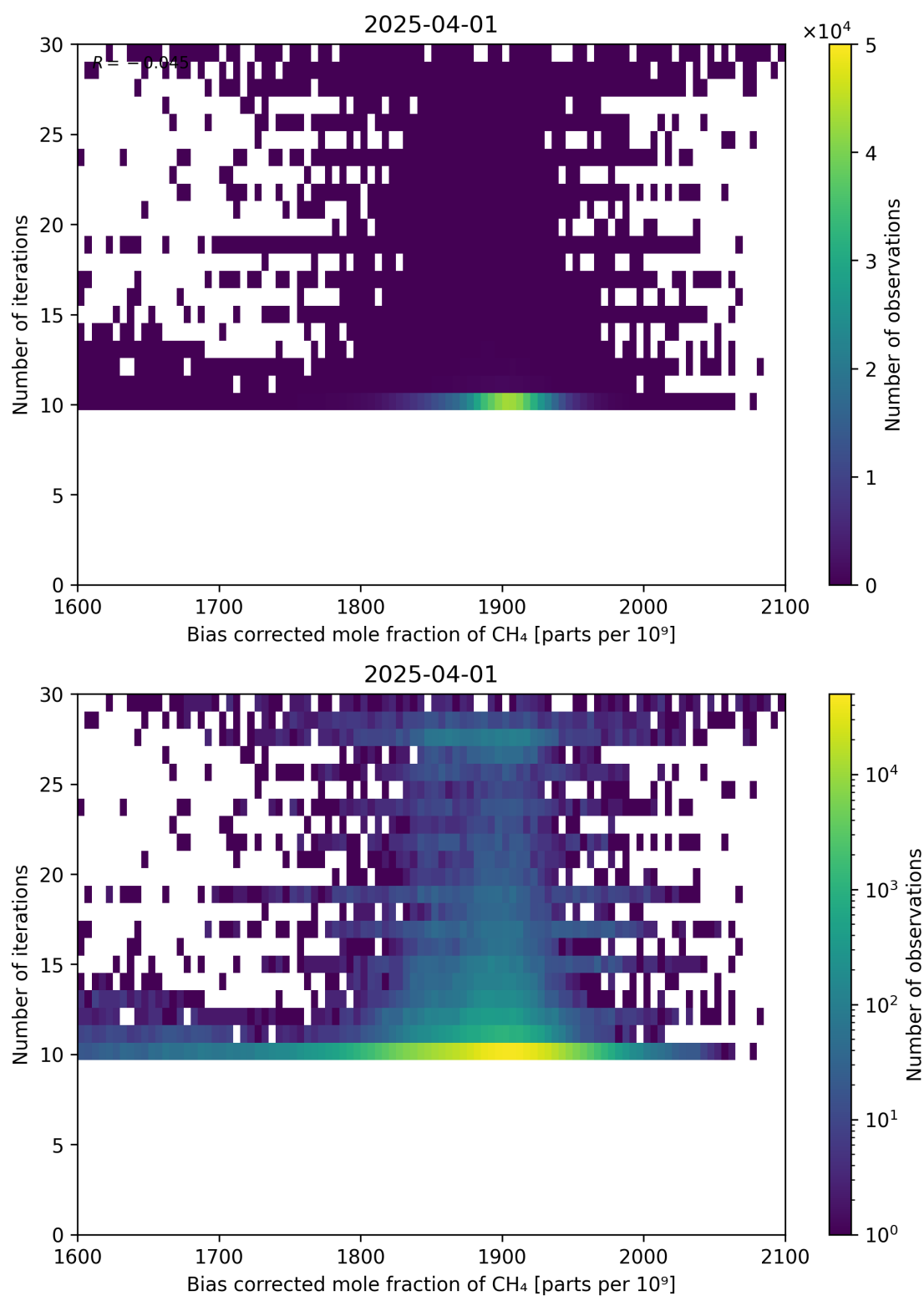
Figure 67: Scatter density plot of “Bias corrected mole fraction of CH 4 ” against “Number of iterations” for 2025-03-31 to 2025-04-02.
