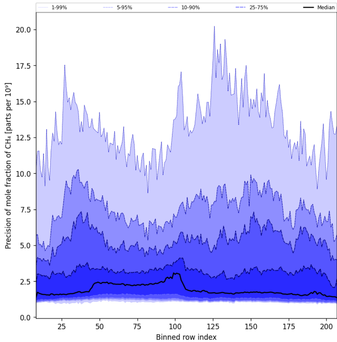
Figure 35: Along track statistics of “Precision of mole fraction of CH 4 ” for 2025-03-31 to 2025-04-02
