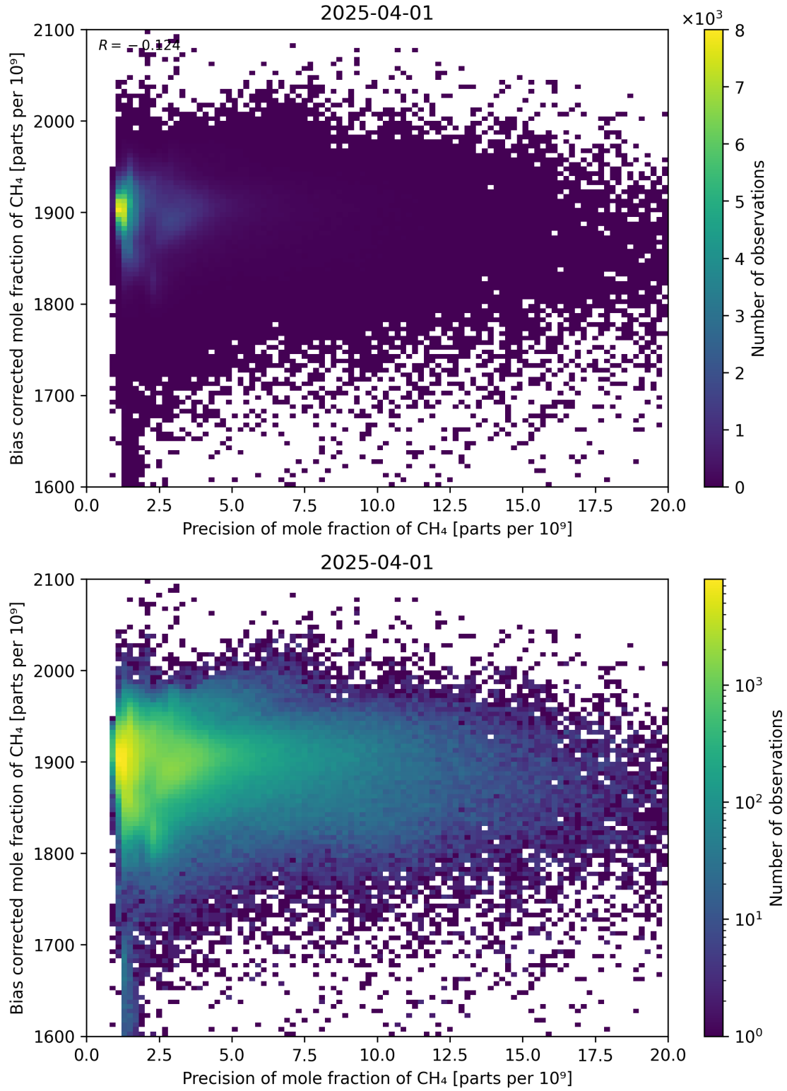
Figure 82: Scatter density plot of “Precision of mole fraction of CH 4 ” against “Bias corrected mole fraction of CH 4 ” for 2025-03-31 to 2025-04-02.
