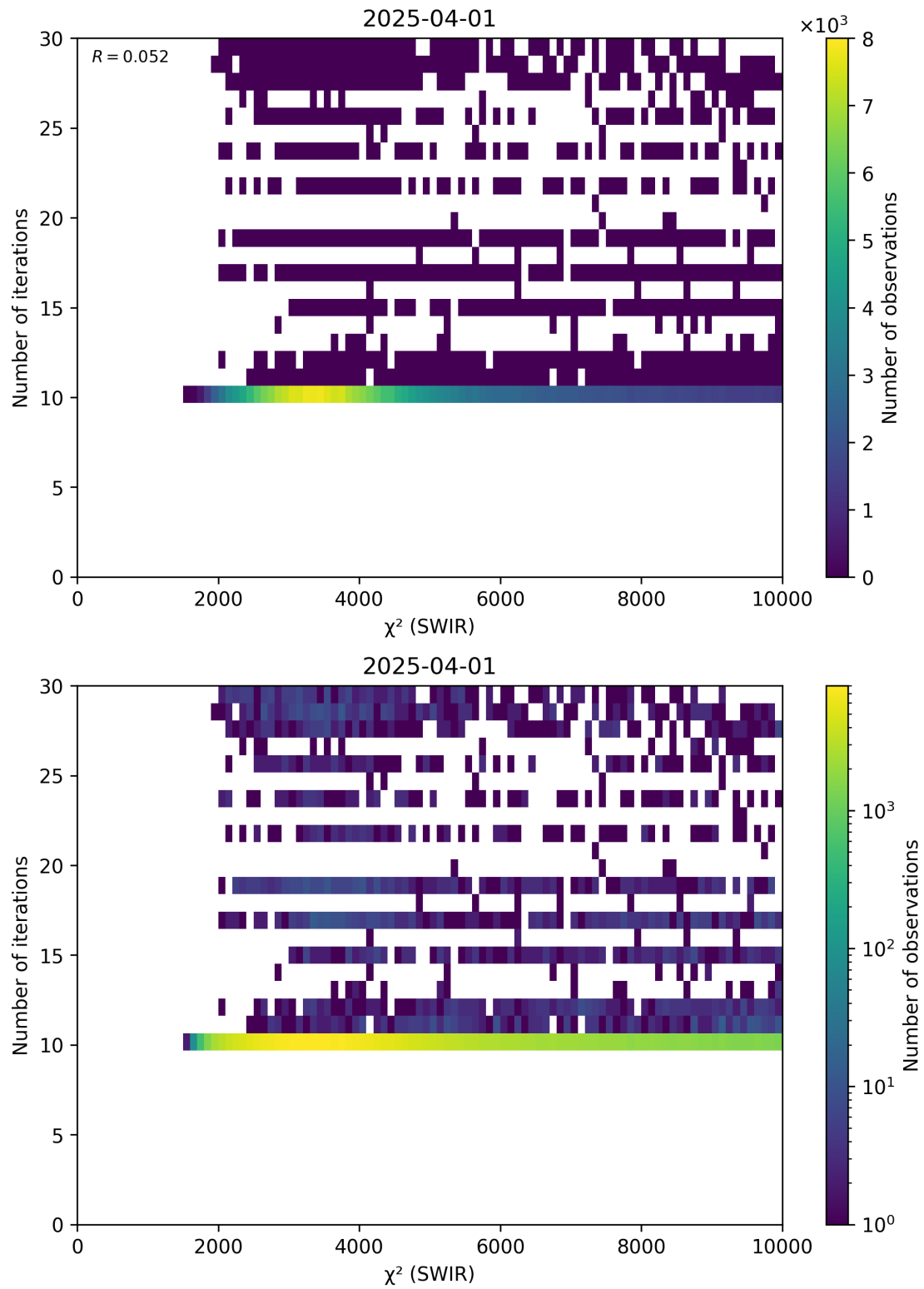
Figure 50: Scatter density plot of “ \chi^2 (SWIR)” against “Number of iterations” for 2025-03-31 to 2025-04-02.
