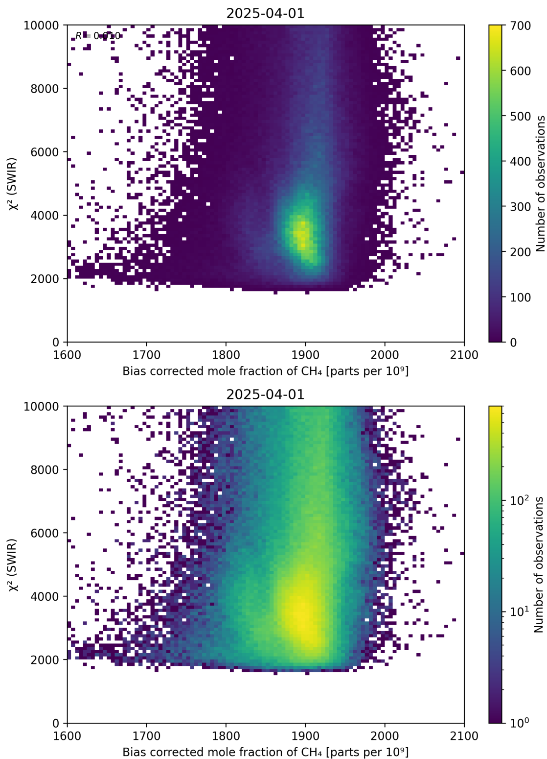
Figure 64: Scatter density plot of “Bias corrected mole fraction of \text{CH}_4 ” against “ \chi^2 (SWIR)” for 2025-03-31 to 2025-04-02.
