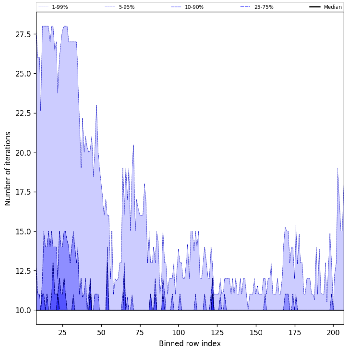
Figure 42: Along track statistics of “Number of iterations” for 2025-03-31 to 2025-04-02
