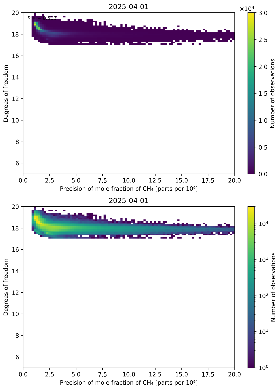
Figure 80: Scatter density plot of “Precision of mole fraction of CH 4 ” against “Degrees of freedom” for 2025-03-31 to 2025-04-02.
