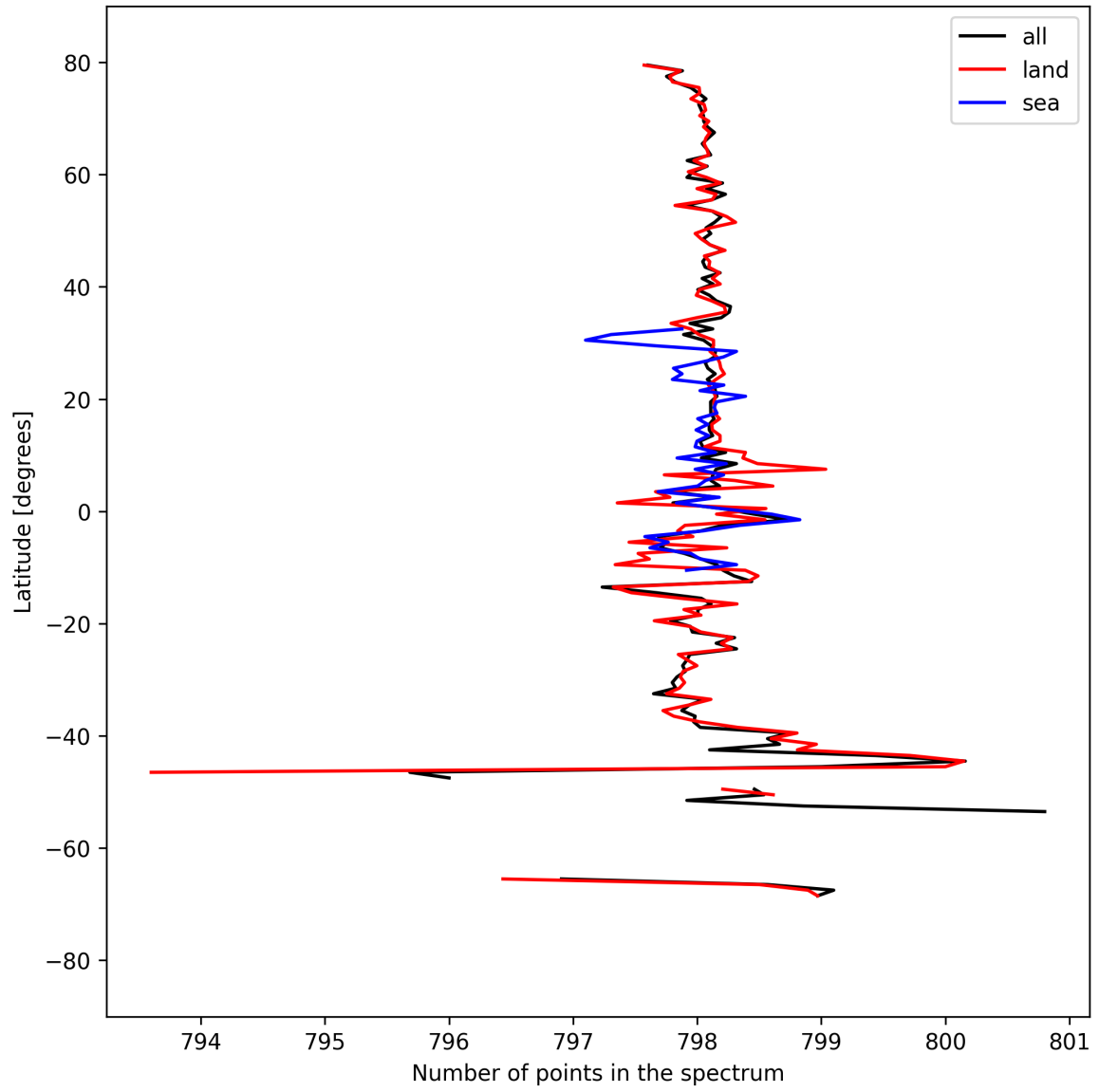
Figure 15: Zonal average of “Number of points in the spectrum” for 2025-03-31 to 2025-04-02.
