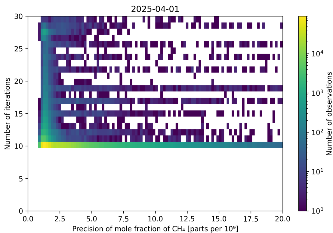
Figure 83: Scatter density plot of “Precision of mole fraction of CH 4 ” against “Number of iterations” for 2025-03-31 to 2025-04-02.
