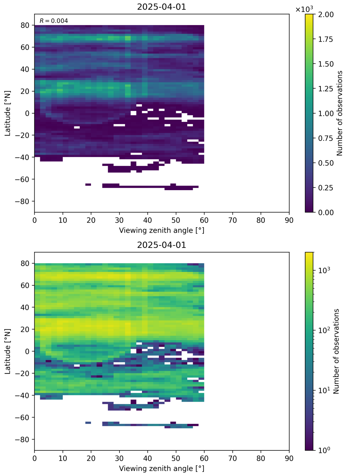
Figure 109: Scatter density plot of “Viewing zenith angle” against “Latitude” for 2025-03-31 to 2025-04-02.
