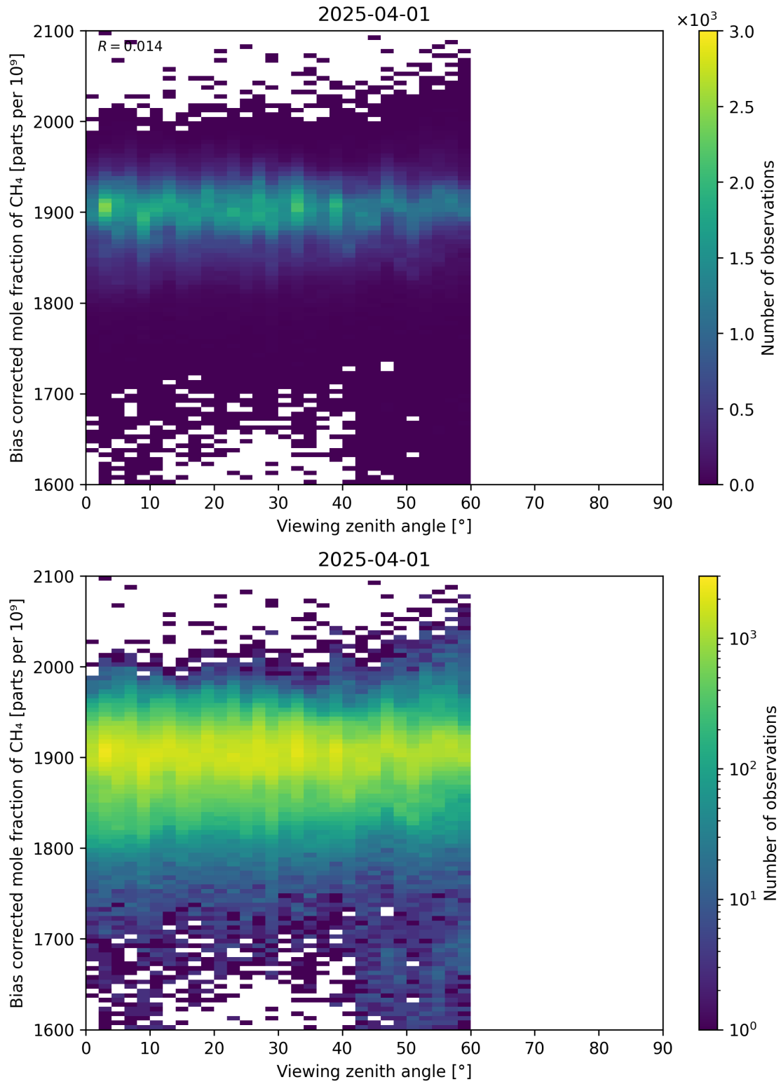
Figure 111: Scatter density plot of “Viewing zenith angle” against “Bias corrected mole fraction of CH 4 ” for 2025-03-31 to 2025-04-02.
