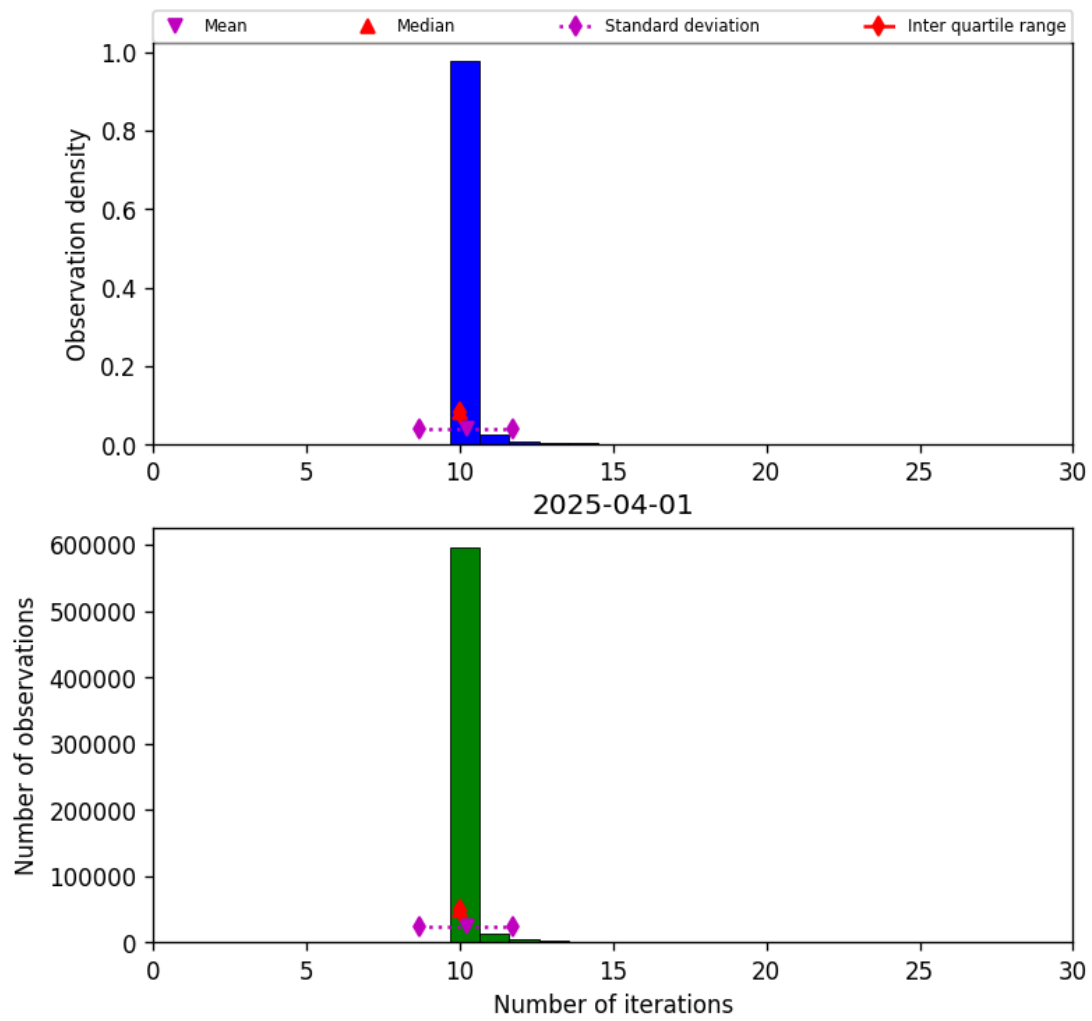
Figure 31: Histogram of “Number of iterations” for 2025-03-31 to 2025-04-02
