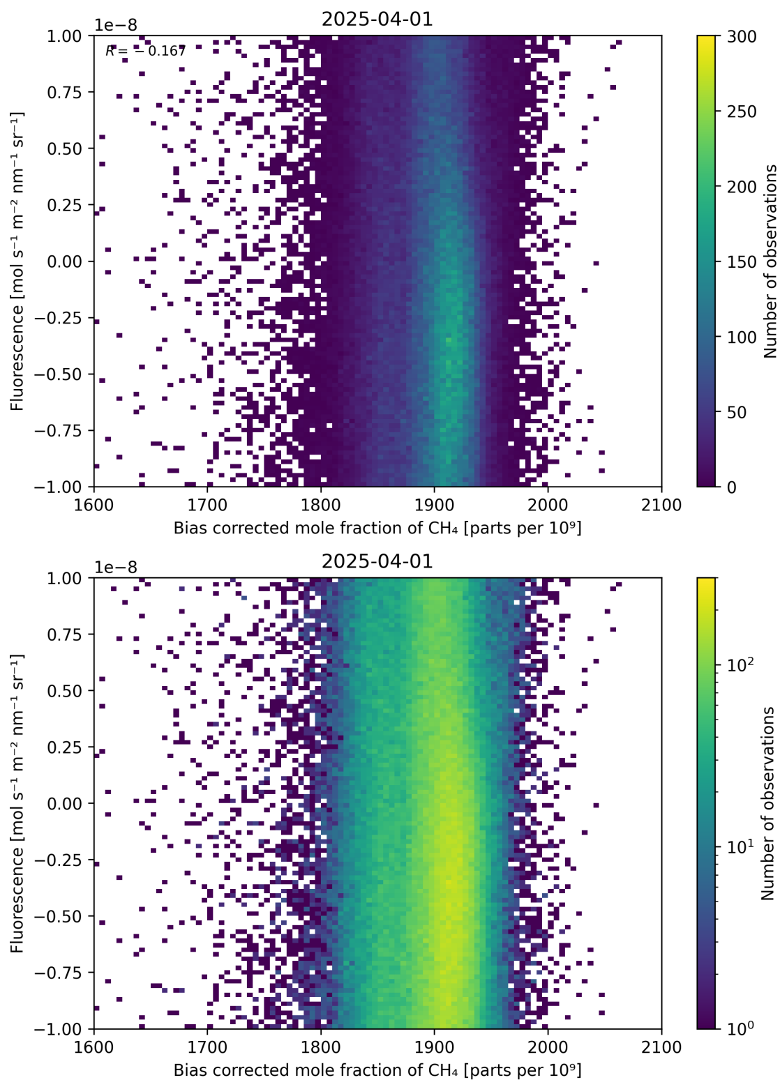
Figure 66: Scatter density plot of “Bias corrected mole fraction of CH 4 ” against “Fluorescence” for 2025-03-31 to 2025-04-02.
