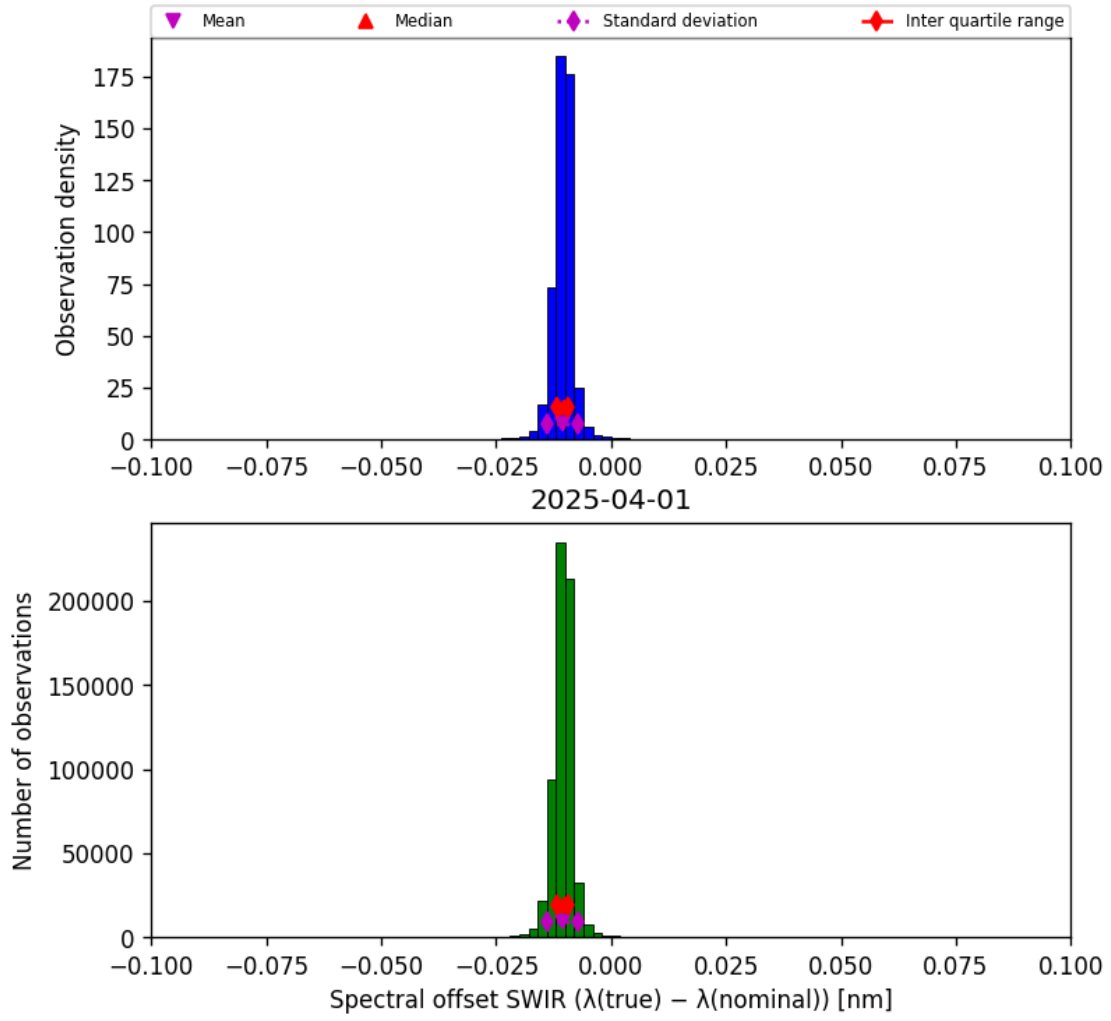
Figure 27: Histogram of “Spectral offset SWIR ( \lambda_{\text{true}} - \lambda_{\text{nominal}} )” for 2025-03-31 to 2025-04-02
