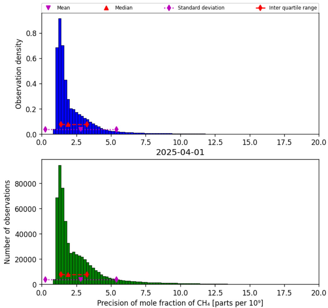
Figure 24: Histogram of “Precision of mole fraction of CH 4 ” for 2025-03-31 to 2025-04-02
