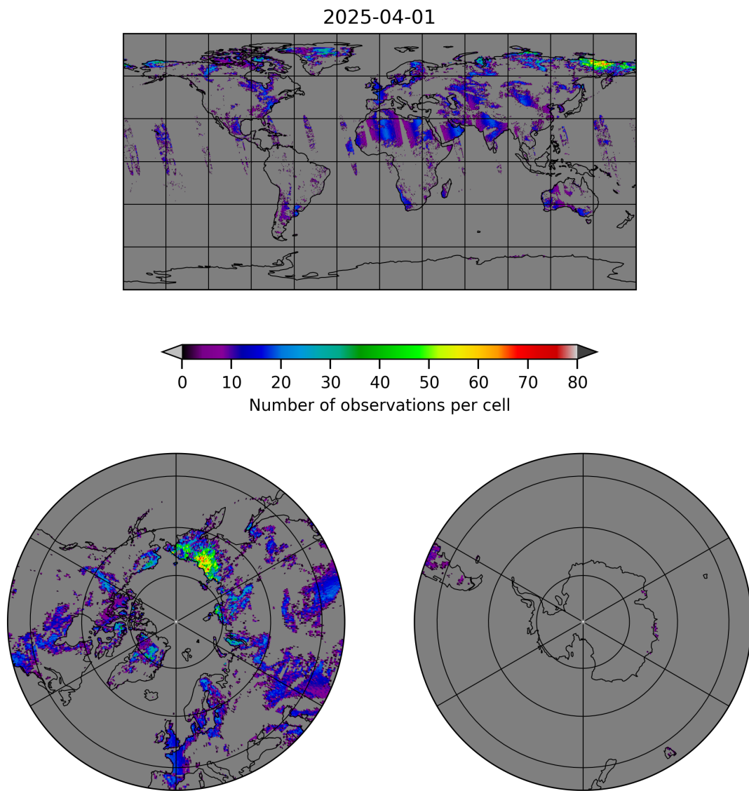
Figure 10: Map of the number of observations for 2025-03-31 to 2025-04-02
