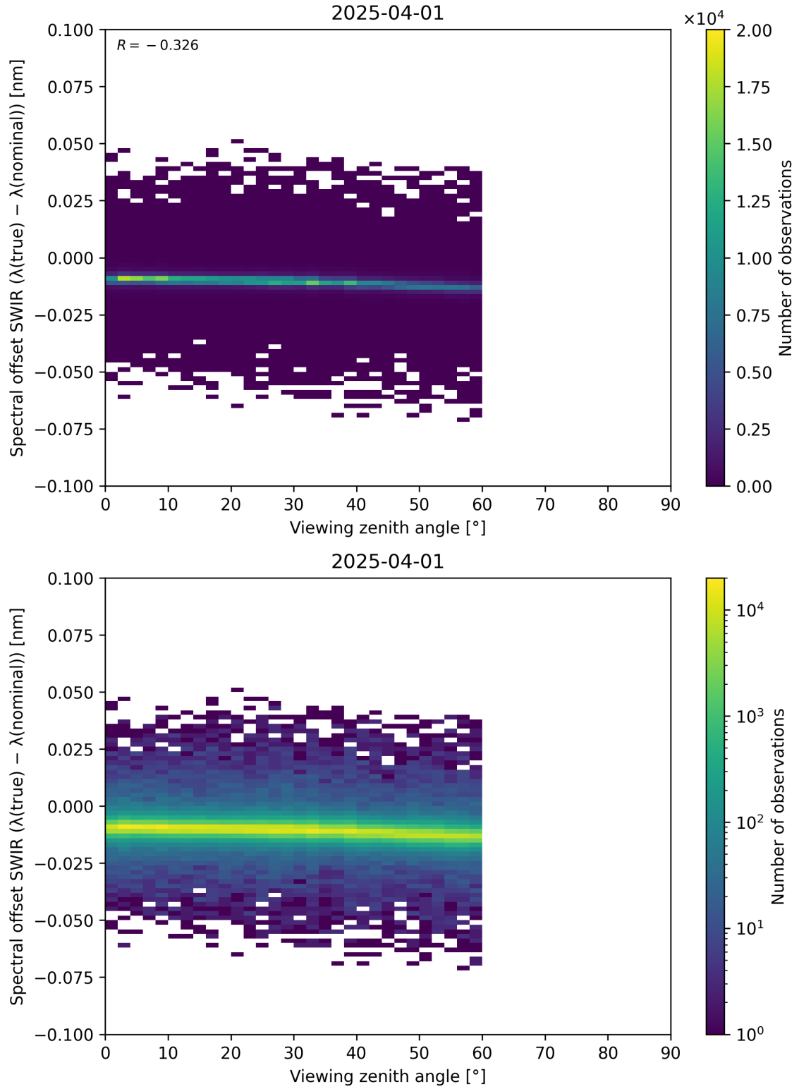
Figure 116: Scatter density plot of “Viewing zenith angle” against “Spectral offset SWIR ( \lambda_{\text{true}} - \lambda_{\text{nominal}} )” for 2025-03-31 to 2025-04-02.
