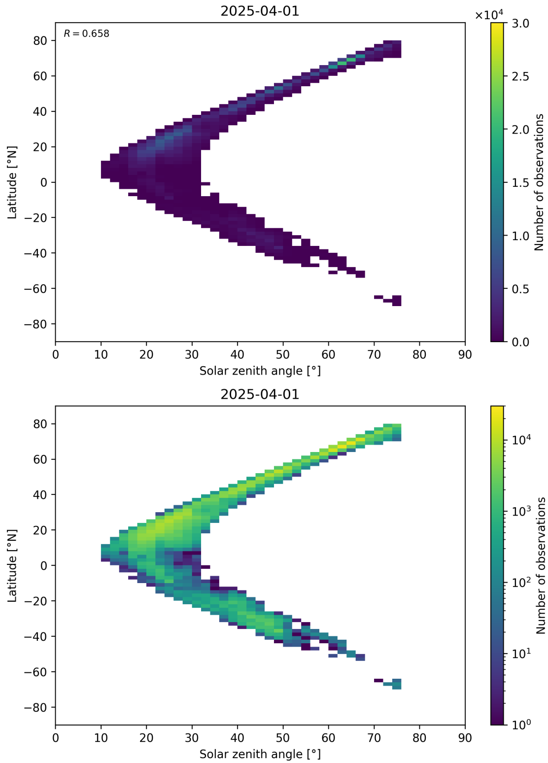
Figure 98: Scatter density plot of “Solar zenith angle” against “Latitude” for 2025-03-31 to 2025-04-02.
