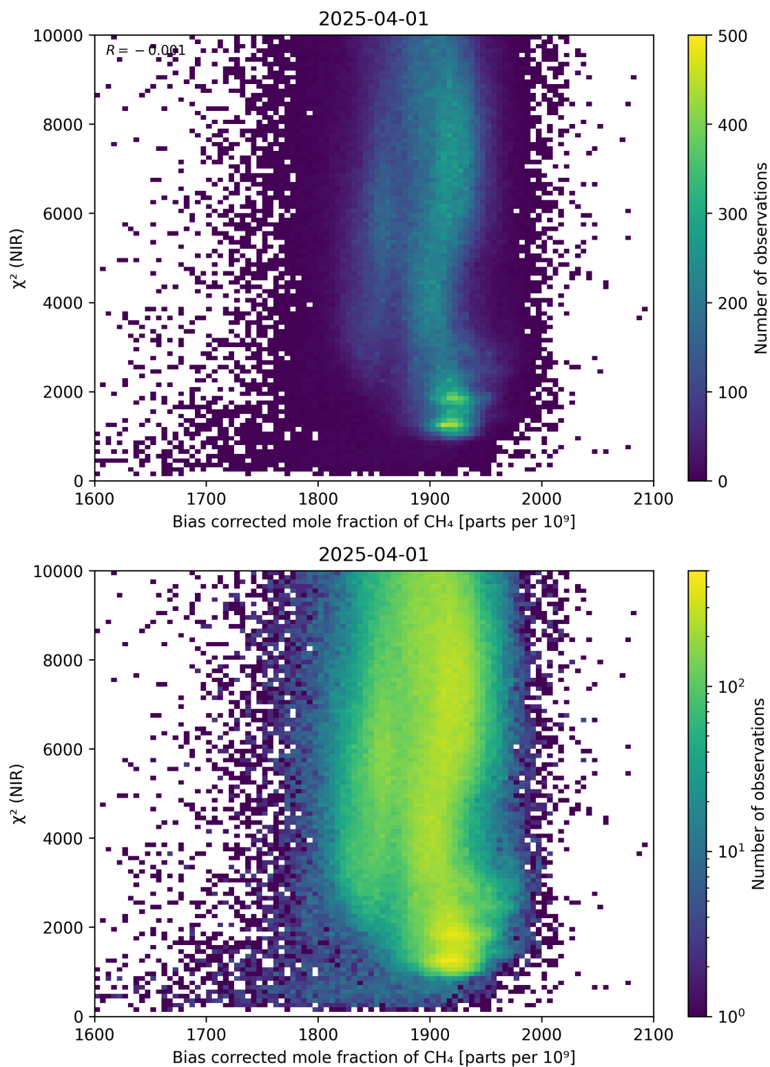
Figure 63: Scatter density plot of “Bias corrected mole fraction of \text{CH}_4 ” against “ \chi^2 (NIR)” for 2025-03-31 to 2025-04-02.
