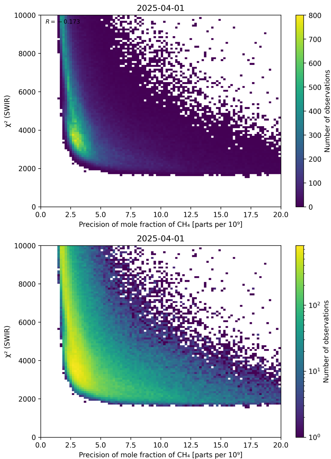
Figure 79: Scatter density plot of “Precision of mole fraction of \text{CH}_4 ” against “ \chi^2 (SWIR)” for 2025-03-31 to 2025-04-02.
