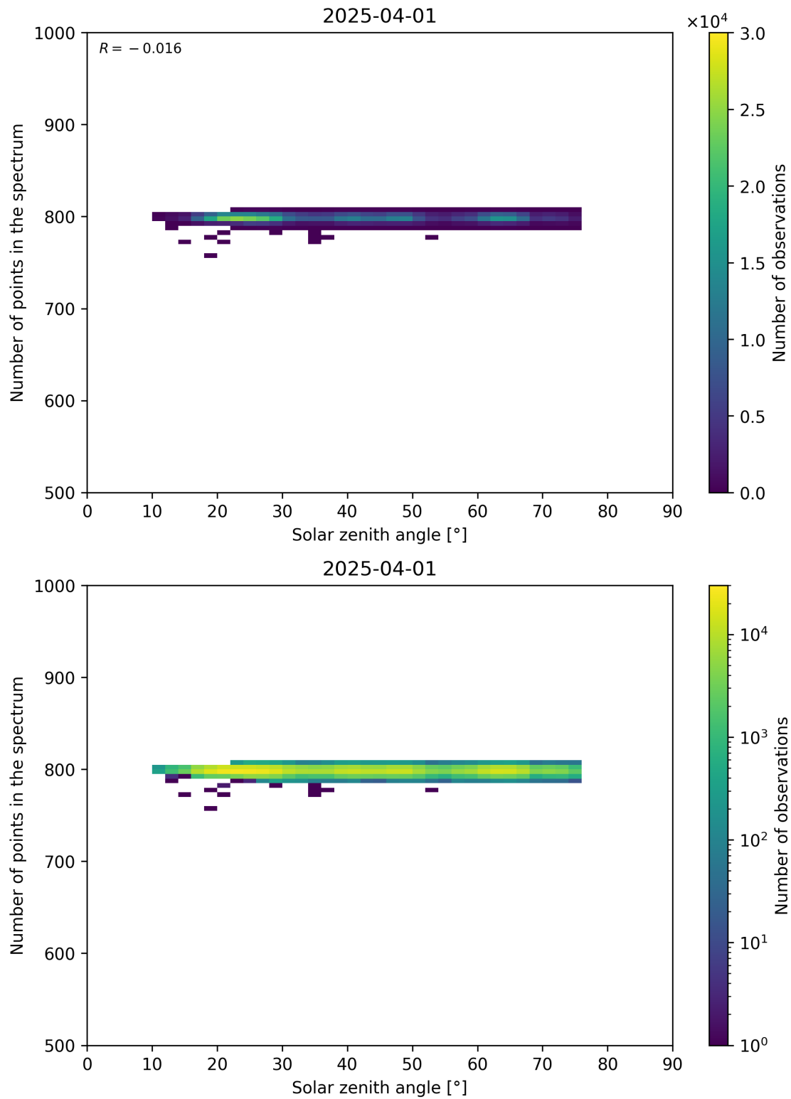
Figure 103: Scatter density plot of “Solar zenith angle” against “Number of points in the spectrum” for 2025-03-31 to 2025-04-02.
