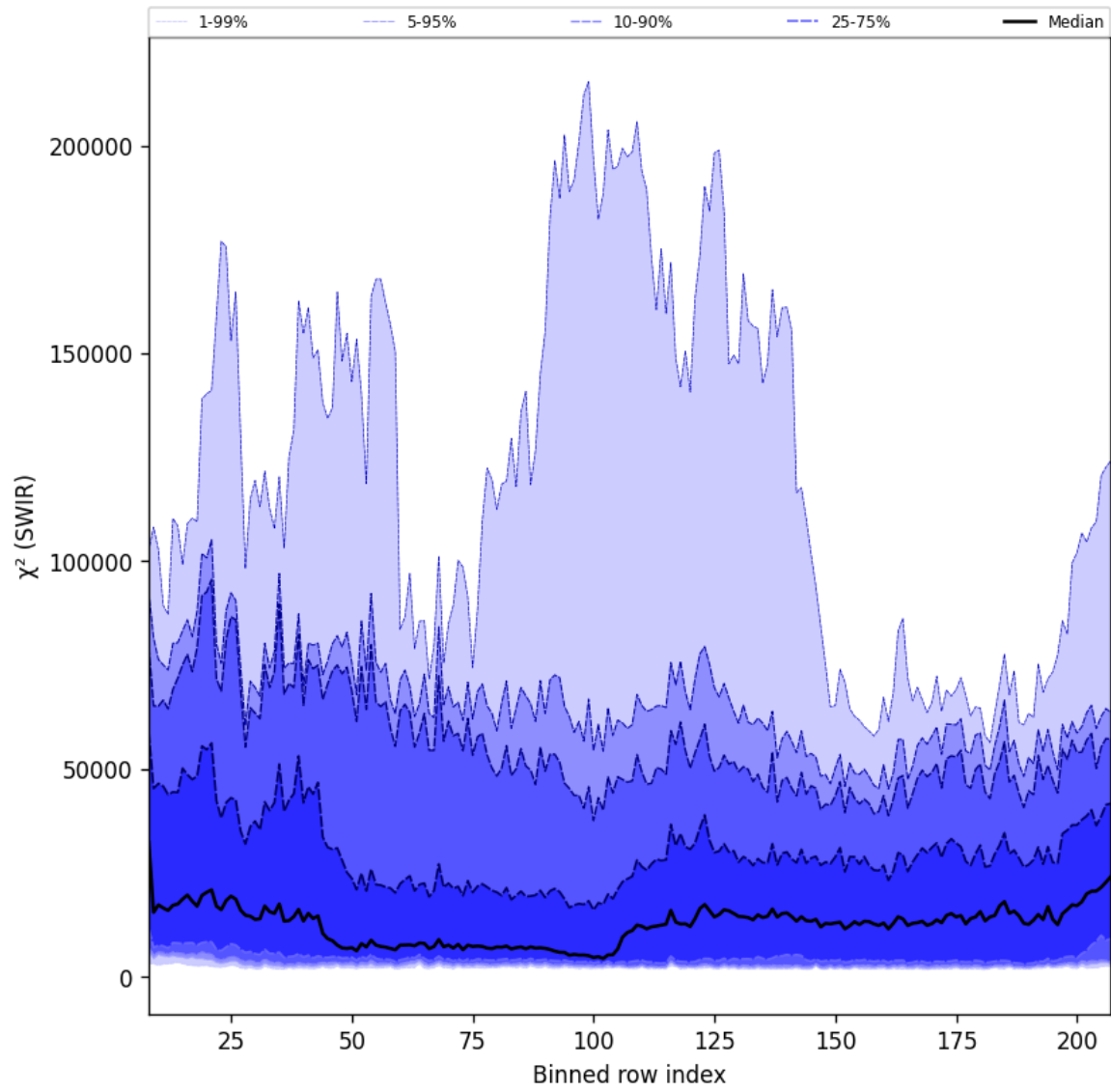
Figure 39: Along track statistics of “ \chi^2 (SWIR)” for 2025-03-31 to 2025-04-02
