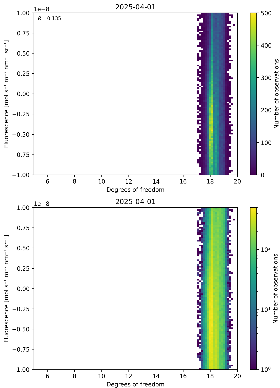
Figure 51: Scatter density plot of “Degrees of freedom” against “Fluorescence” for 2025-03-31 to 2025-04-02.
