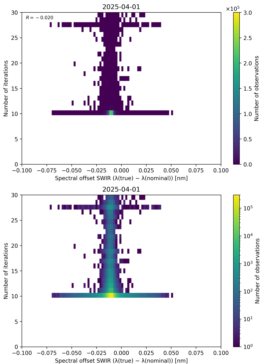
Figure 121: Scatter density plot of “Spectral offset SWIR ( \lambda_{\text{true}} - \lambda_{\text{nominal}} )” against “Number of iterations” for 2025-03-31 to 2025-04-02.
