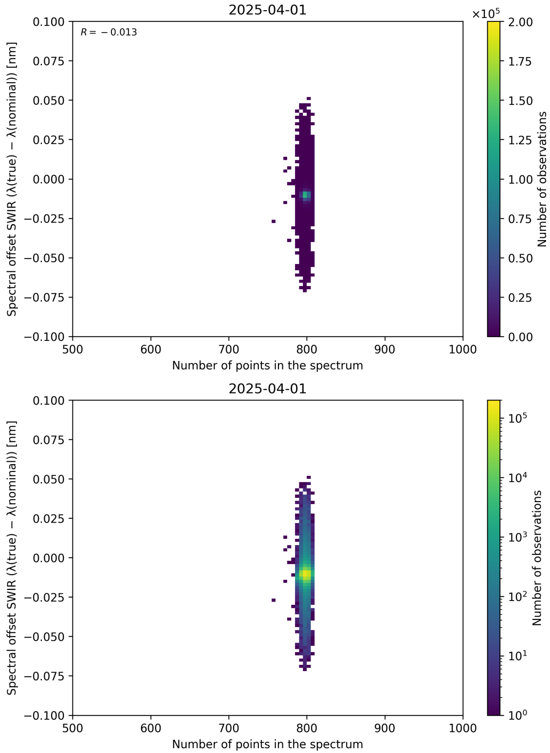
Figure 93: Scatter density plot of “Number of points in the spectrum” against “Spectral offset SWIR ( \lambda_{\text{true}} - \lambda_{\text{nominal}} )” for 2025-03-31 to 2025-04-02.
