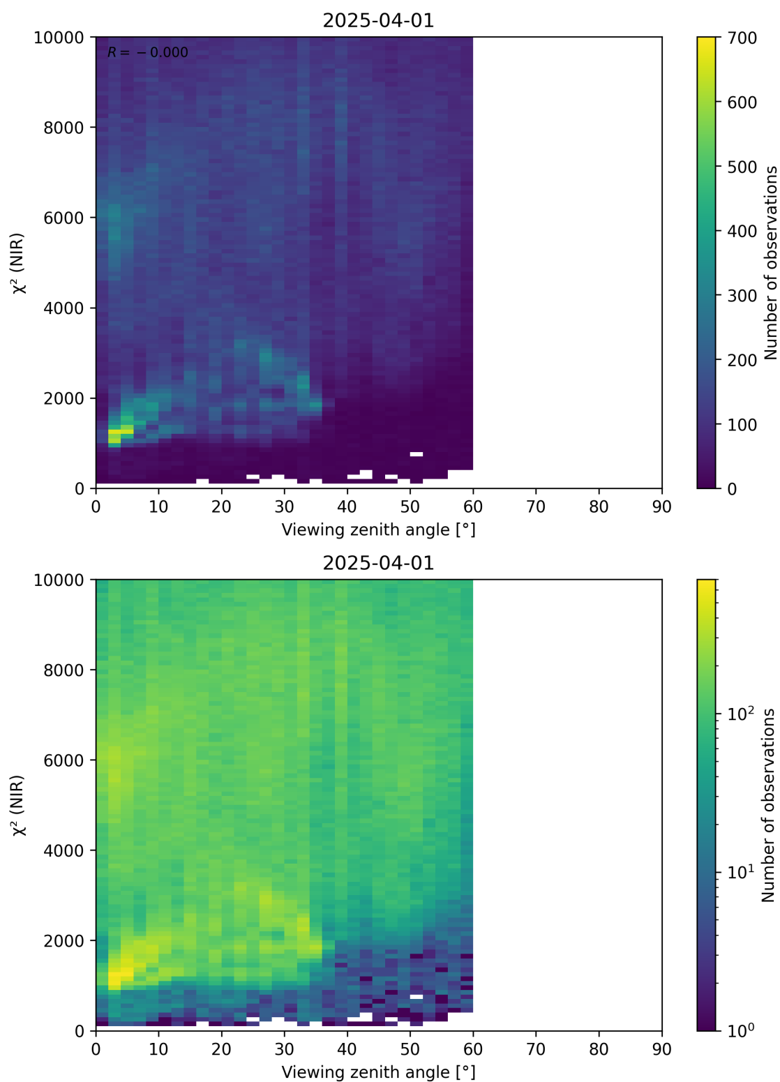
Figure 105: Scatter density plot of “Viewing zenith angle” against “ \chi^2 (NIR)” for 2025-03-31 to 2025-04-02.
