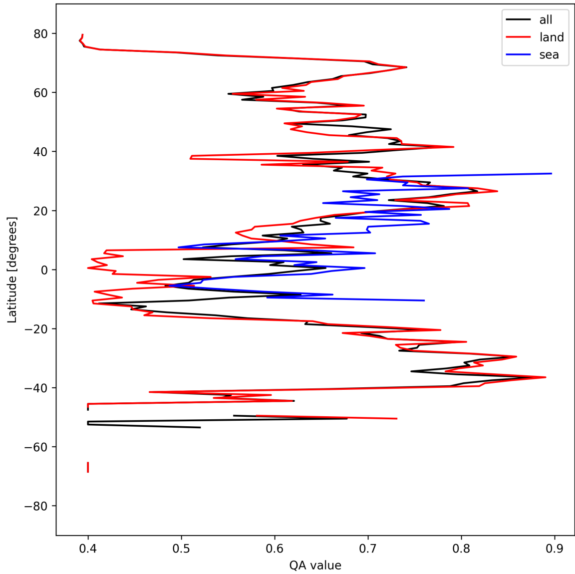
Figure 11: Zonal average of “QA value” for 2025-03-31 to 2025-04-02.
