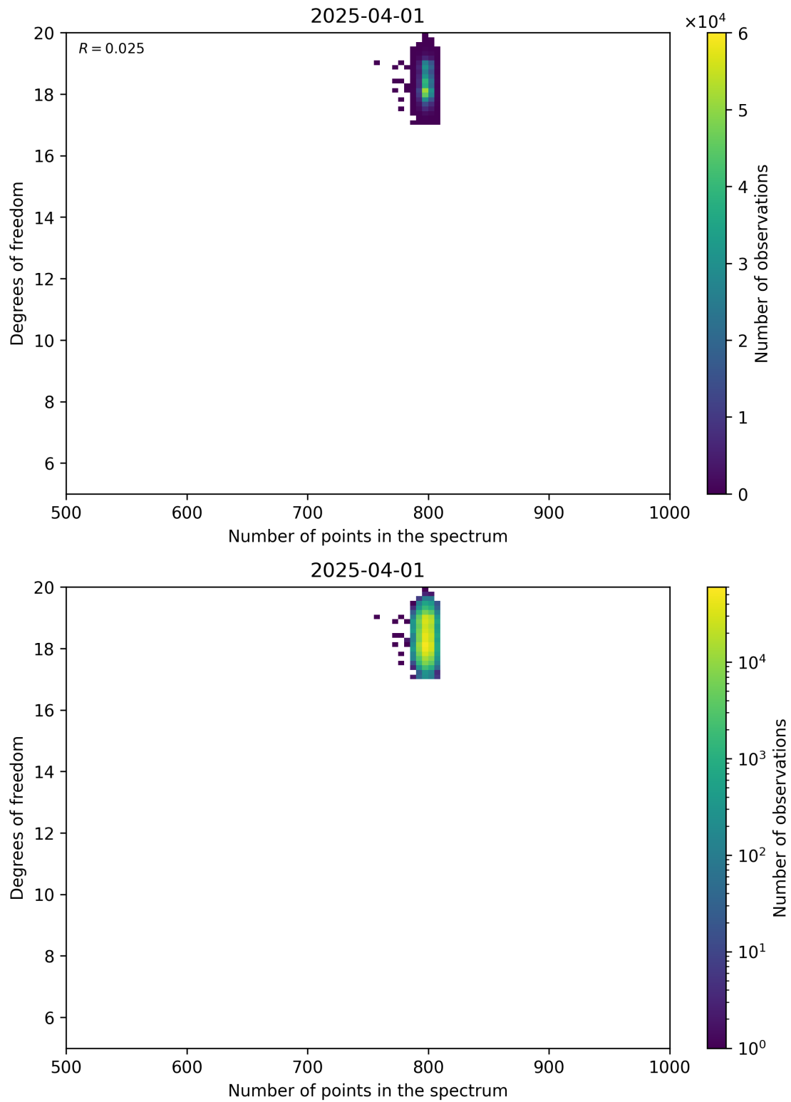
Figure 90: Scatter density plot of “Number of points in the spectrum” against “Degrees of freedom” for 2025-03-31 to 2025-04-02.
