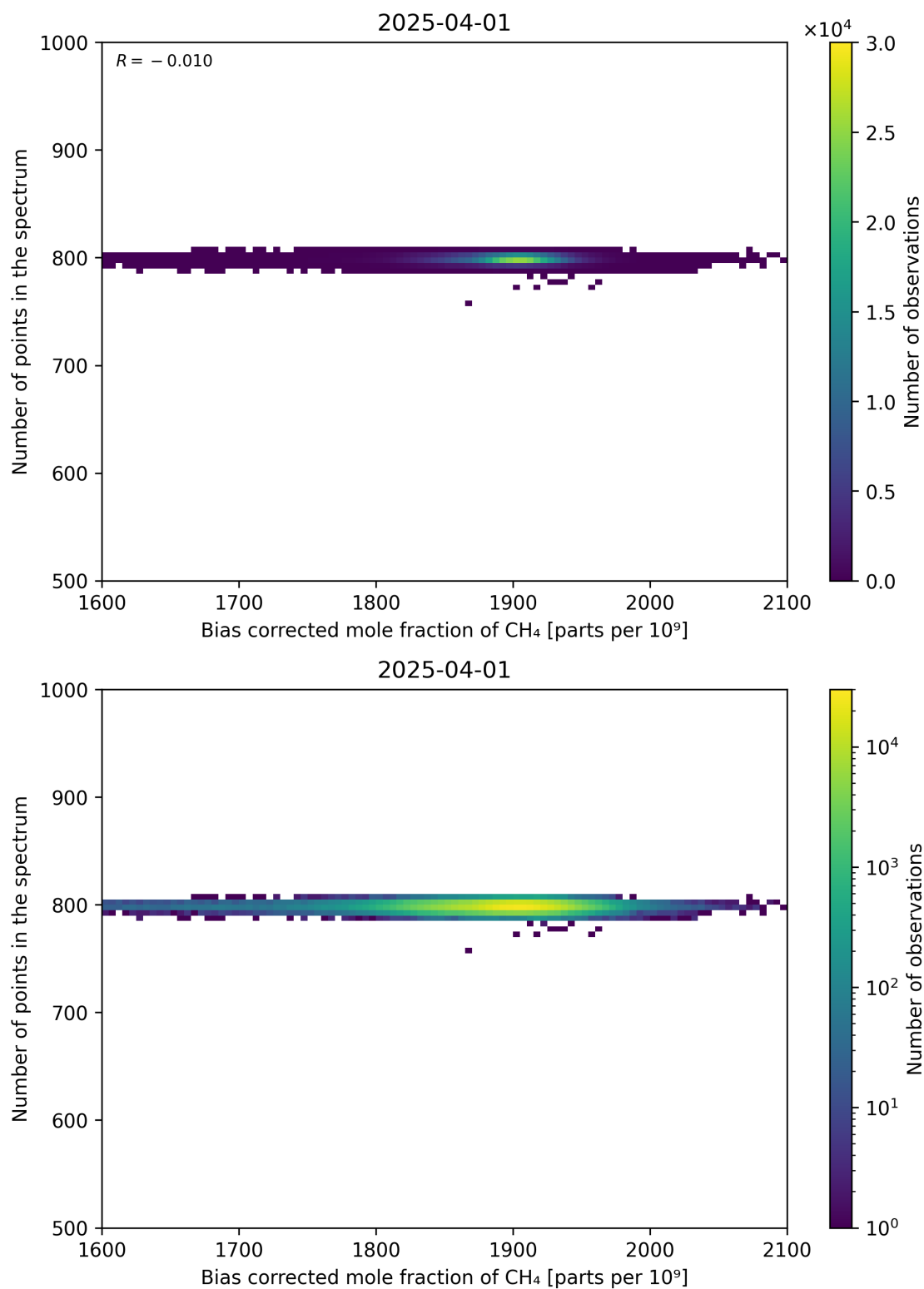
Figure 68: Scatter density plot of “Bias corrected mole fraction of CH 4 ” against “Number of points in the spectrum” for 2025-03-31 to 2025-04-02.
