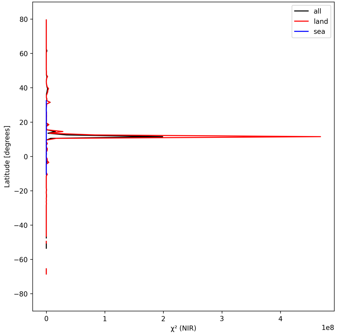
Figure 18: Zonal average of “ \chi^2 (NIR)” for 2025-03-31 to 2025-04-02.
