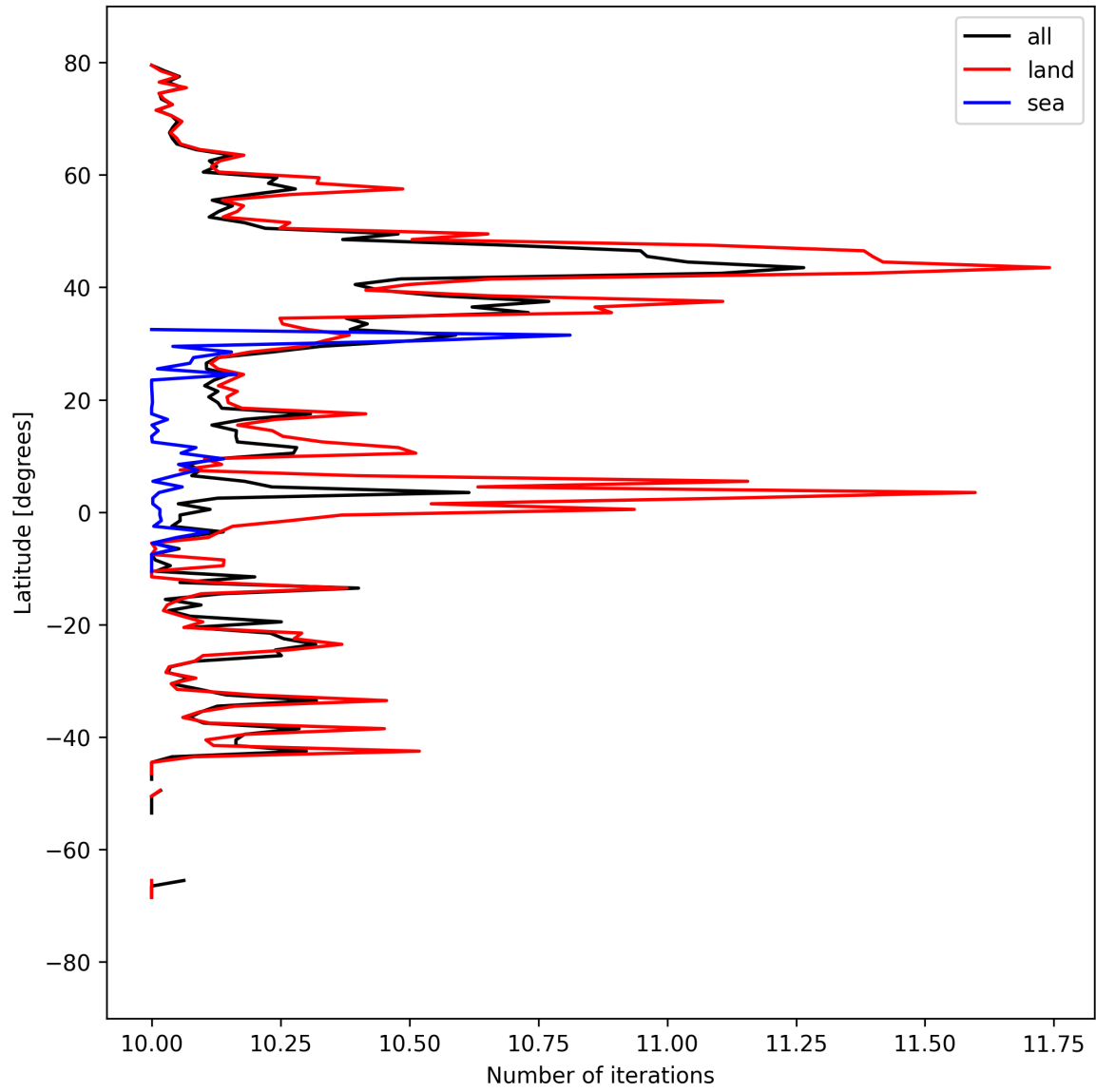
Figure 20: Zonal average of “Number of iterations” for 2025-03-31 to 2025-04-02.
