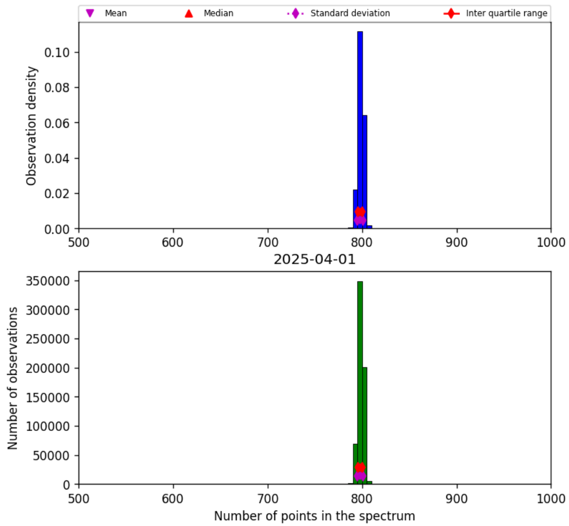
Figure 26: Histogram of “Number of points in the spectrum” for 2025-03-31 to 2025-04-02
