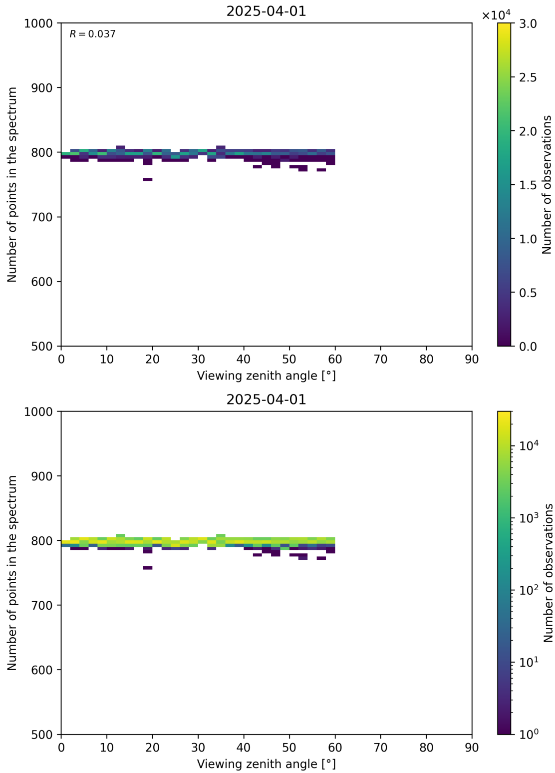
Figure 114: Scatter density plot of “Viewing zenith angle” against “Number of points in the spectrum” for 2025-03-31 to 2025-04-02.
