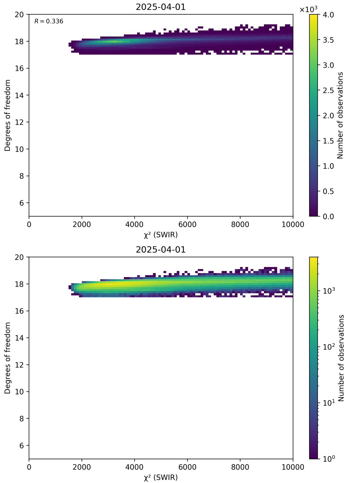
Figure 48: Scatter density plot of “ \chi^2 (SWIR)” against “Degrees of freedom” for 2025-03-31 to 2025-04-02.
