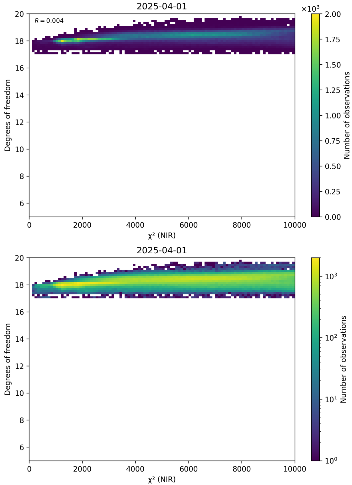
Figure 44: Scatter density plot of “ \chi^2 (NIR)” against “Degrees of freedom” for 2025-03-31 to 2025-04-02.
