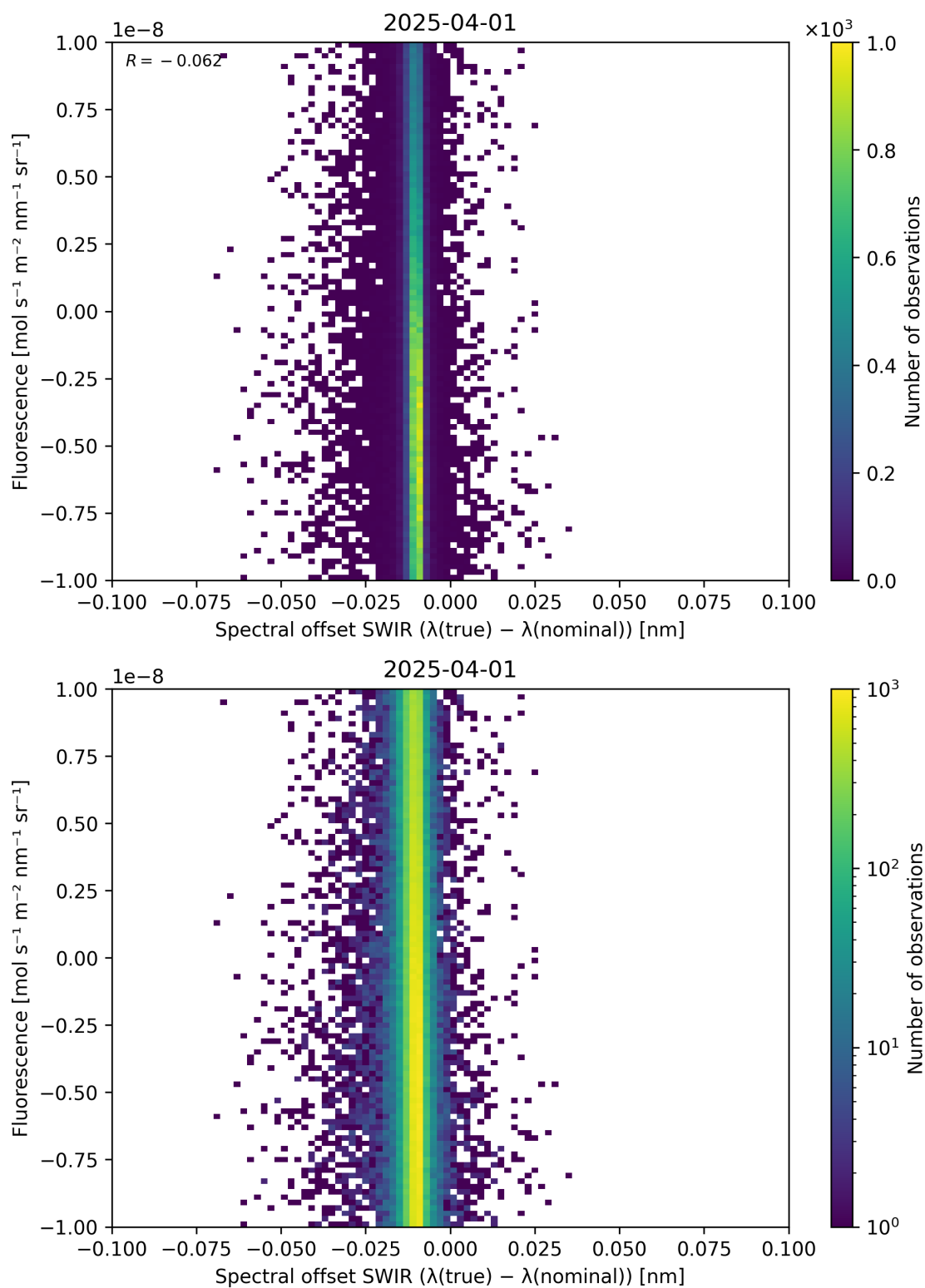
Figure 120: Scatter density plot of “Spectral offset SWIR ( \lambda_{\text{true}} - \lambda_{\text{nominal}} )” against “Fluorescence” for 2025-03-31 to 2025-04-02.
