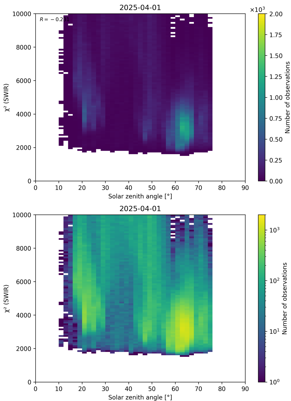
Figure 95: Scatter density plot of “Solar zenith angle” against “ \chi^2 (SWIR)” for 2025-03-31 to 2025-04-02.
