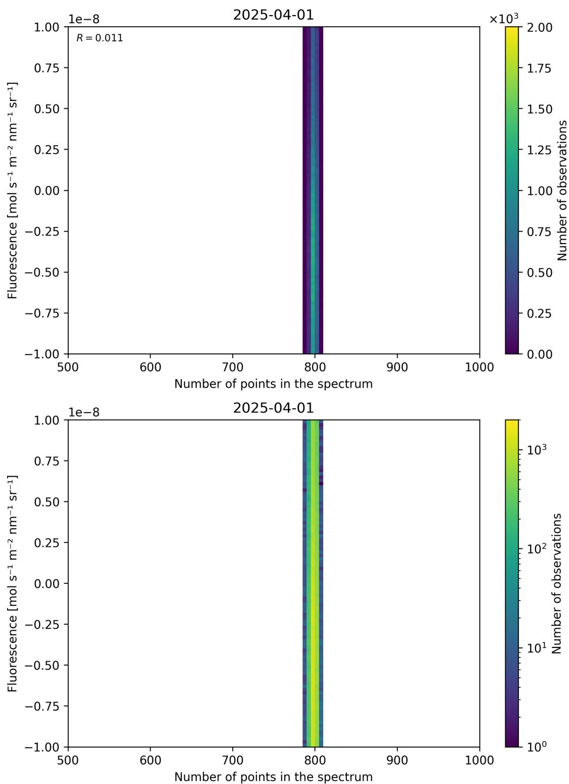
Figure 91: Scatter density plot of “Number of points in the spectrum” against “Fluorescence” for 2025-03-31 to 2025-04-02.
