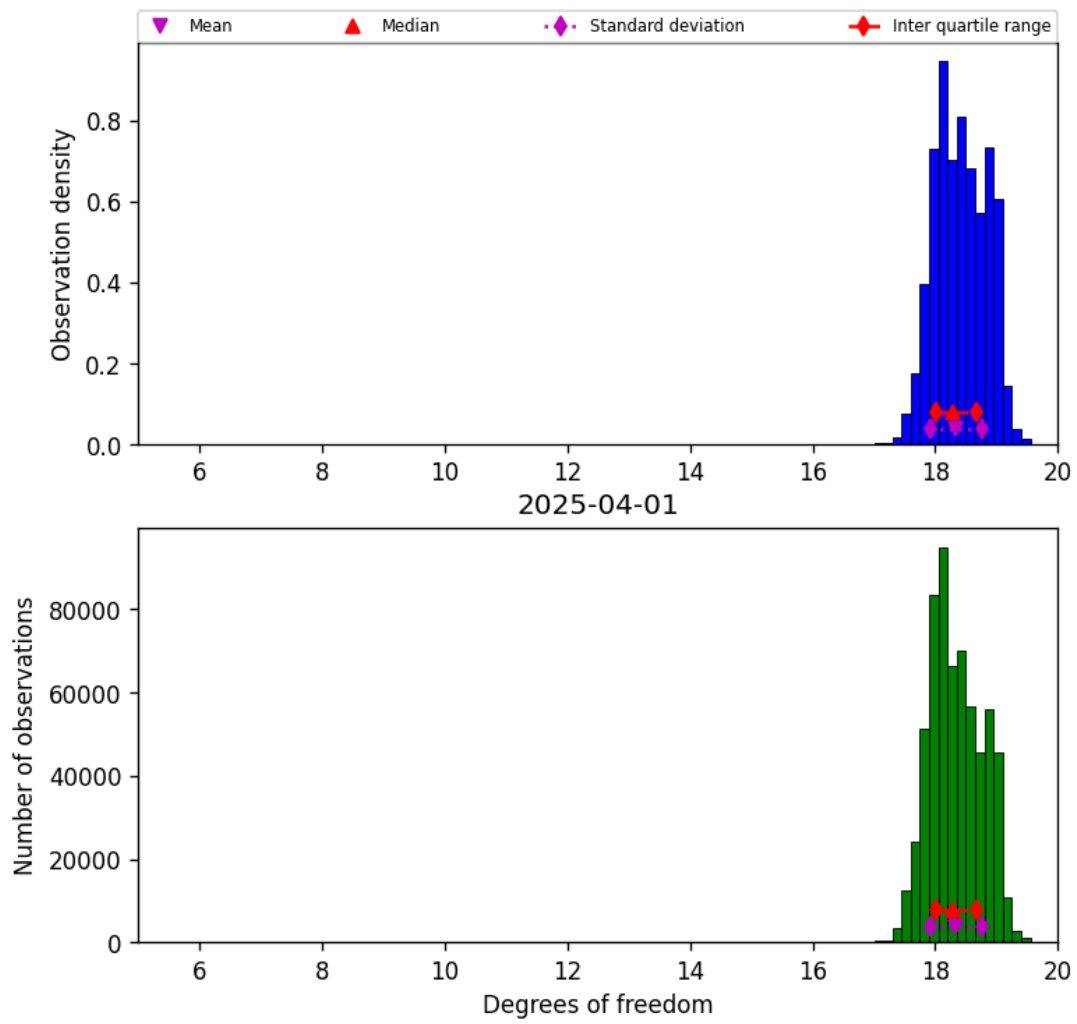
Figure 30: Histogram of “Degrees of freedom” for 2025-03-31 to 2025-04-02
