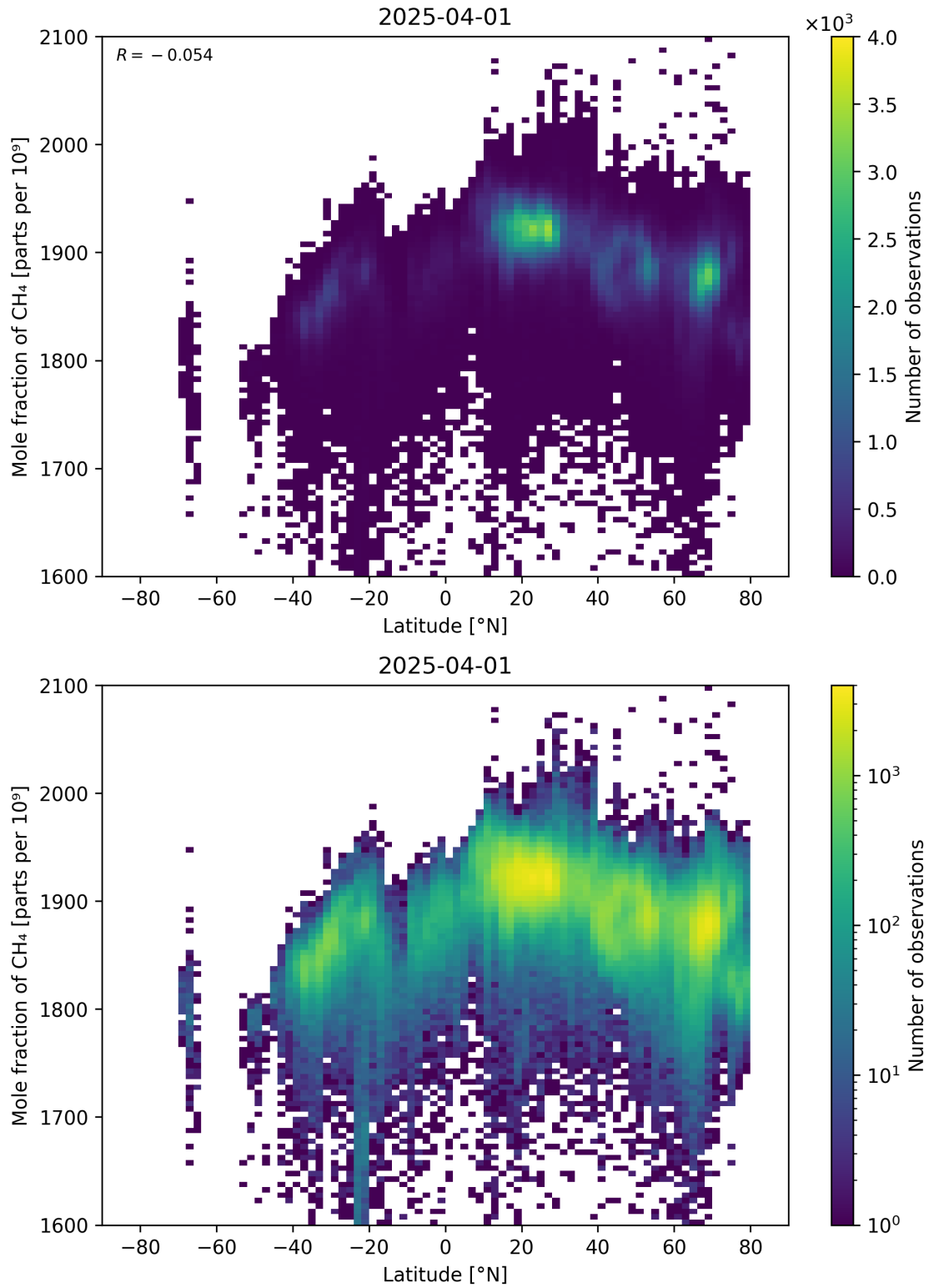
Figure 57: Scatter density plot of “Latitude” against “Mole fraction of CH 4 ” for 2025-03-31 to 2025-04-02.
