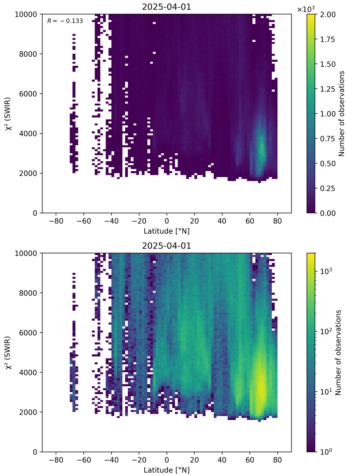
Figure 54: Scatter density plot of “Latitude” against “ \chi^2 (SWIR)” for 2025-03-31 to 2025-04-02.
