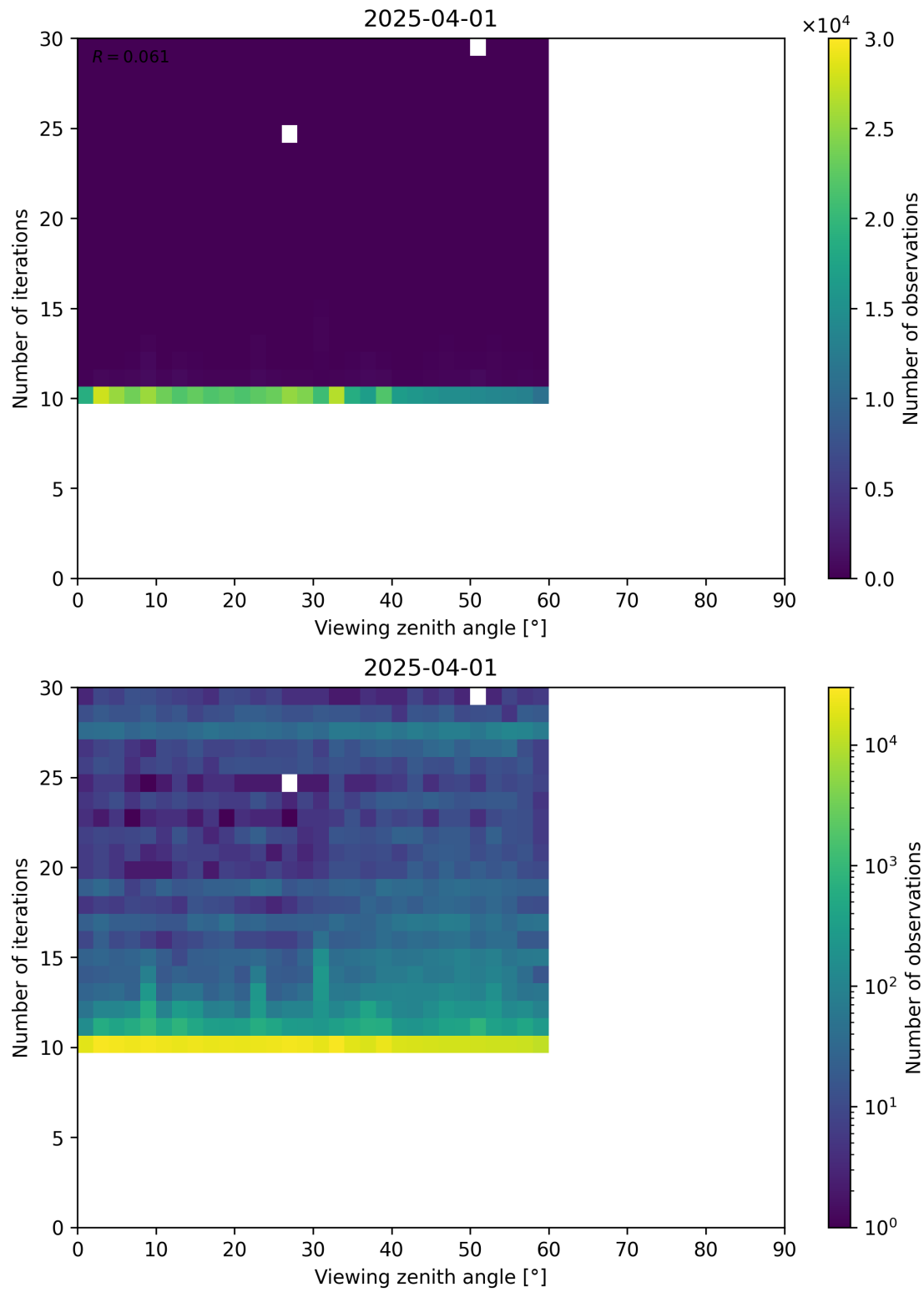
Figure 113: Scatter density plot of “Viewing zenith angle” against “Number of iterations” for 2025-03-31 to 2025-04-02.
