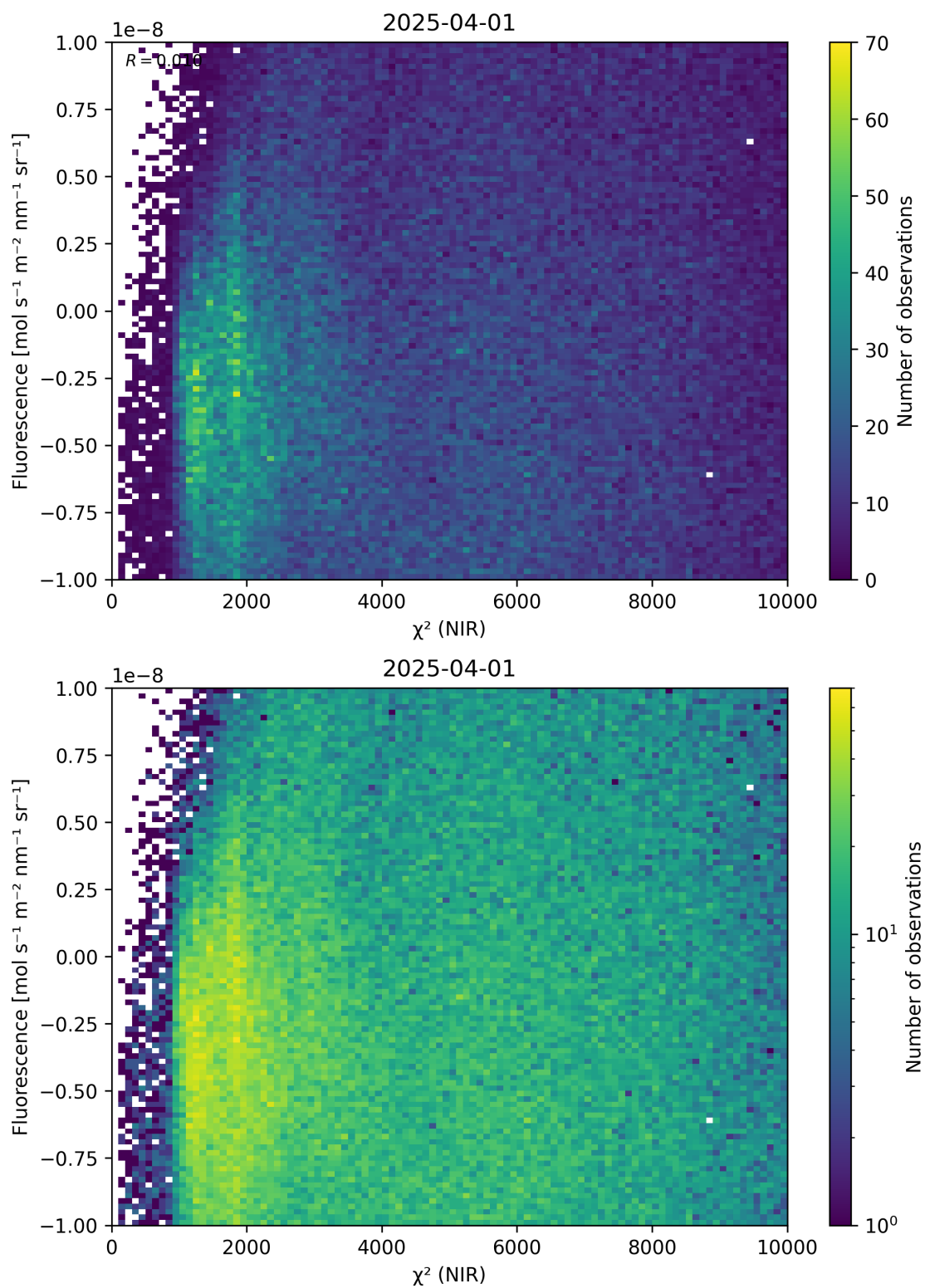
Figure 45: Scatter density plot of “ \chi^2 (NIR)” against “Fluorescence” for 2025-03-31 to 2025-04-02.
