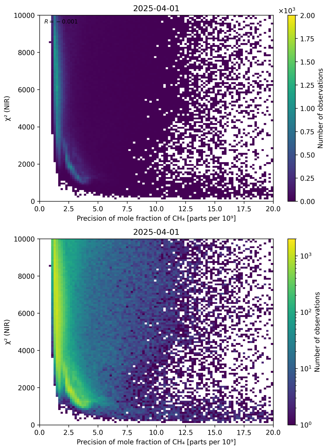
Figure 78: Scatter density plot of “Precision of mole fraction of CH 4 ” against “ \chi^2 (NIR)” for 2025-03-31 to 2025-04-02.
