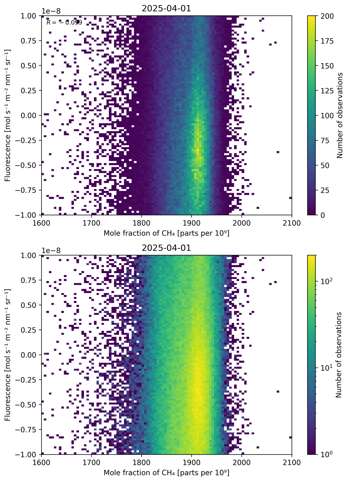
Figure 73: Scatter density plot of “Mole fraction of CH 4 ” against “Fluorescence” for 2025-03-31 to 2025-04-02.
