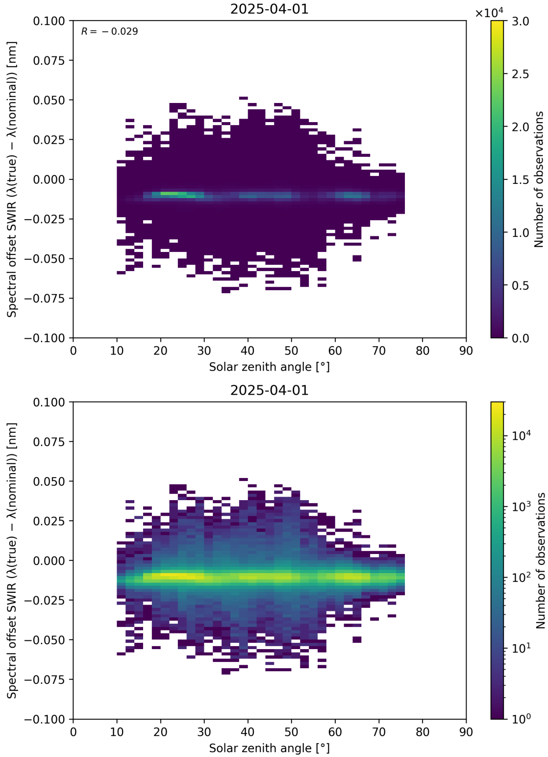
Figure 104: Scatter density plot of “Solar zenith angle” against “Spectral offset SWIR ( \lambda_{\text{true}} - \lambda_{\text{nominal}} )” for 2025-03-31 to 2025-04-02.
