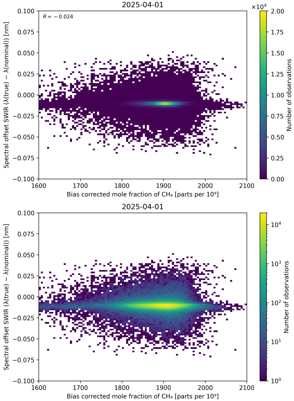
Figure 69: Scatter density plot of “Bias corrected mole fraction of CH 4 ” against “Spectral offset SWIR ( \lambda_{\text{true}} - \lambda_{\text{nominal}} )” for 2025-03-31 to 2025-04-02.
