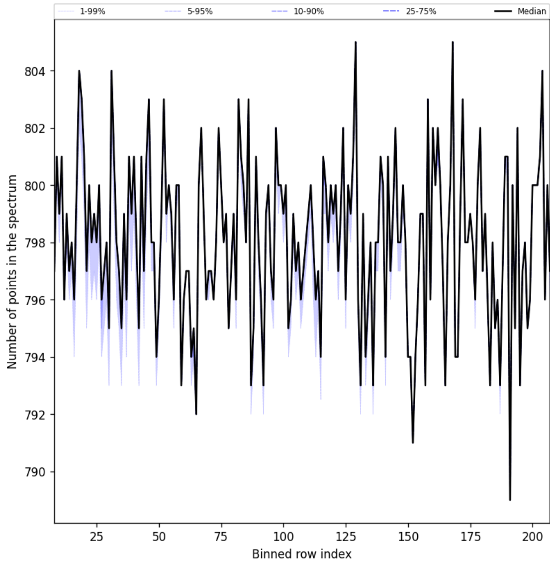
Figure 37: Along track statistics of “Number of points in the spectrum” for 2025-03-31 to 2025-04-02
