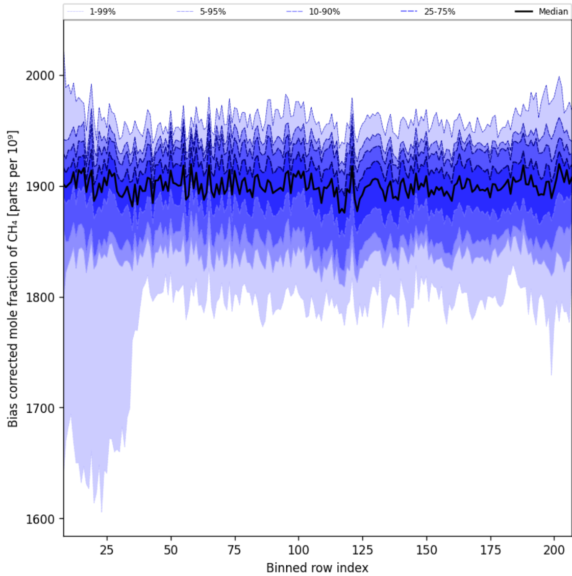
Figure 36: Along track statistics of “Bias corrected mole fraction of CH 4 ” for 2025-03-31 to 2025-04-02
