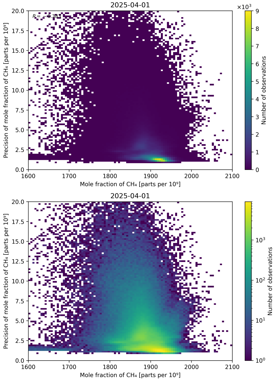
Figure 75: Scatter density plot of “Mole fraction of CH 4 ” against “Precision of mole fraction of CH 4 ” for 2025-03-31 to 2025-04-02.
