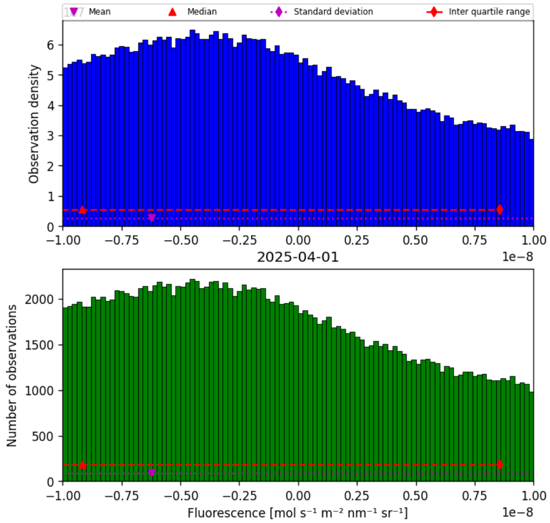
Figure 32: Histogram of “Fluorescence” for 2025-03-31 to 2025-04-02
