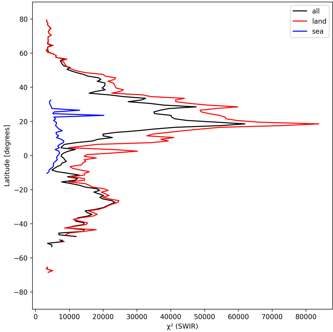
Figure 17: Zonal average of “ \chi^2 (SWIR)” for 2025-03-31 to 2025-04-02.
