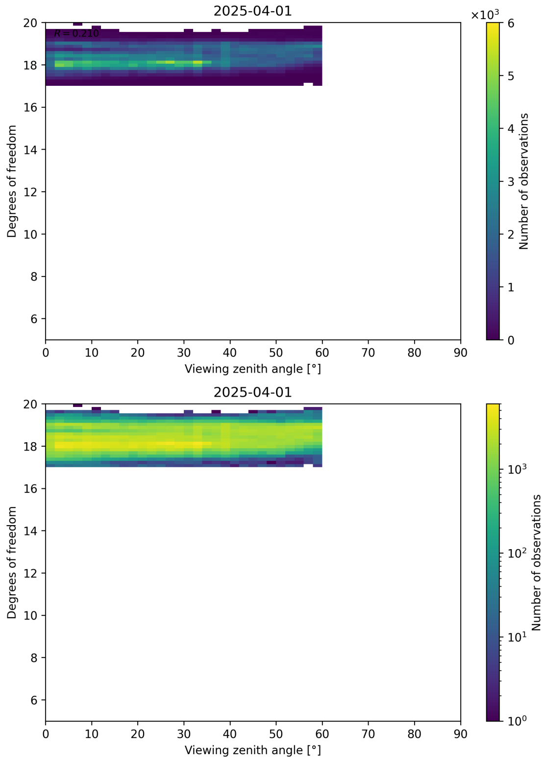
Figure 107: Scatter density plot of “Viewing zenith angle” against “Degrees of freedom” for 2025-03-31 to 2025-04-02.
