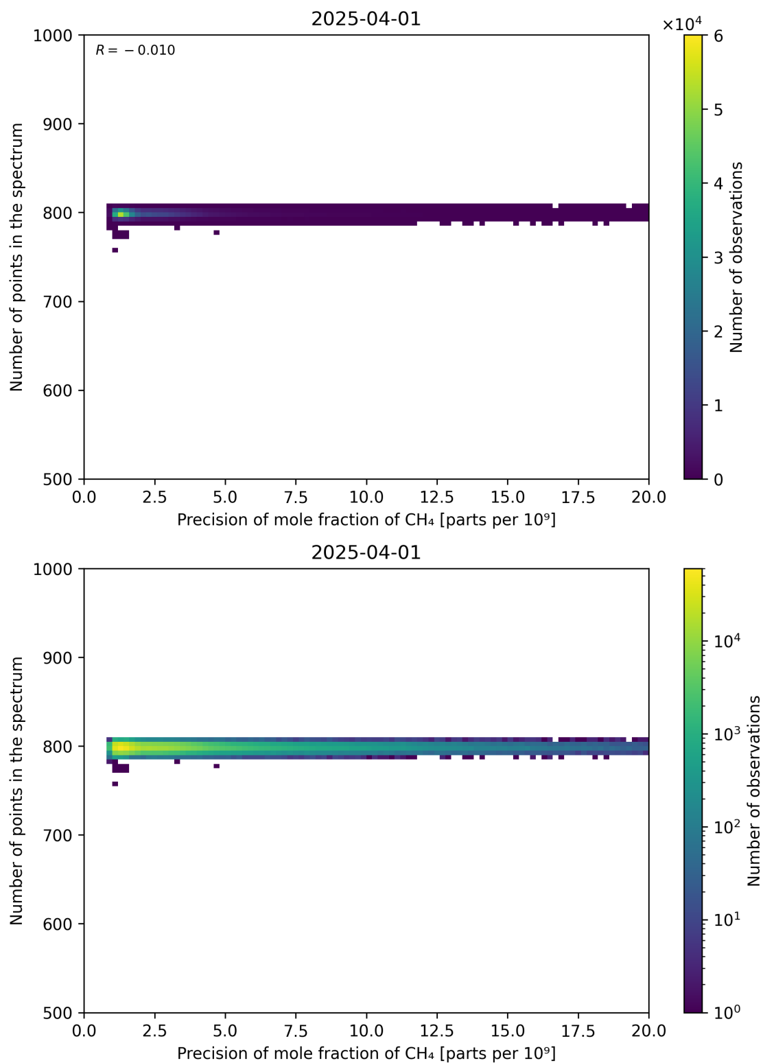
Figure 84: Scatter density plot of “Precision of mole fraction of CH 4 ” against “Number of points in the spectrum” for 2025-03-31 to 2025-04-02.
