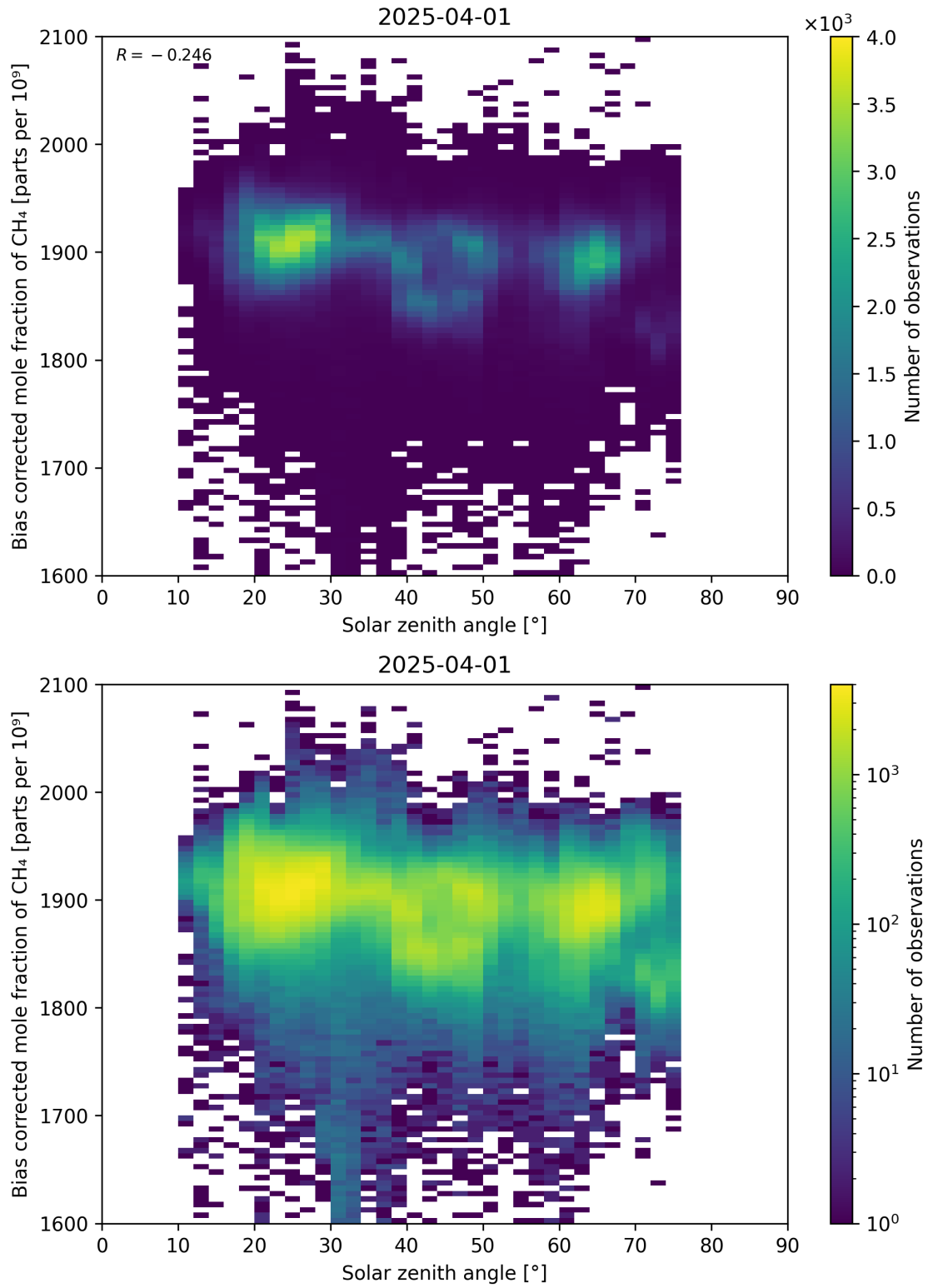
Figure 100: Scatter density plot of “Solar zenith angle” against “Bias corrected mole fraction of \text{CH}_4 ” for 2025-03-31 to 2025-04-02.
