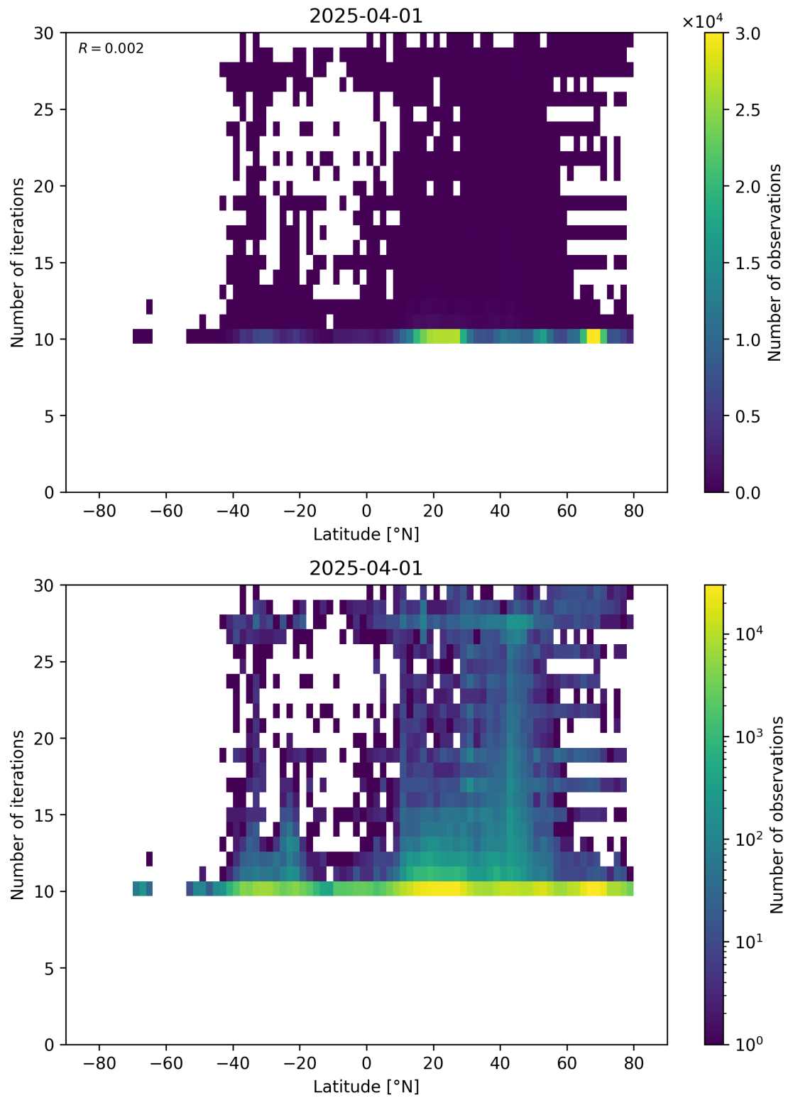
Figure 60: Scatter density plot of “Latitude” against “Number of iterations” for 2025-03-31 to 2025-04-02.
