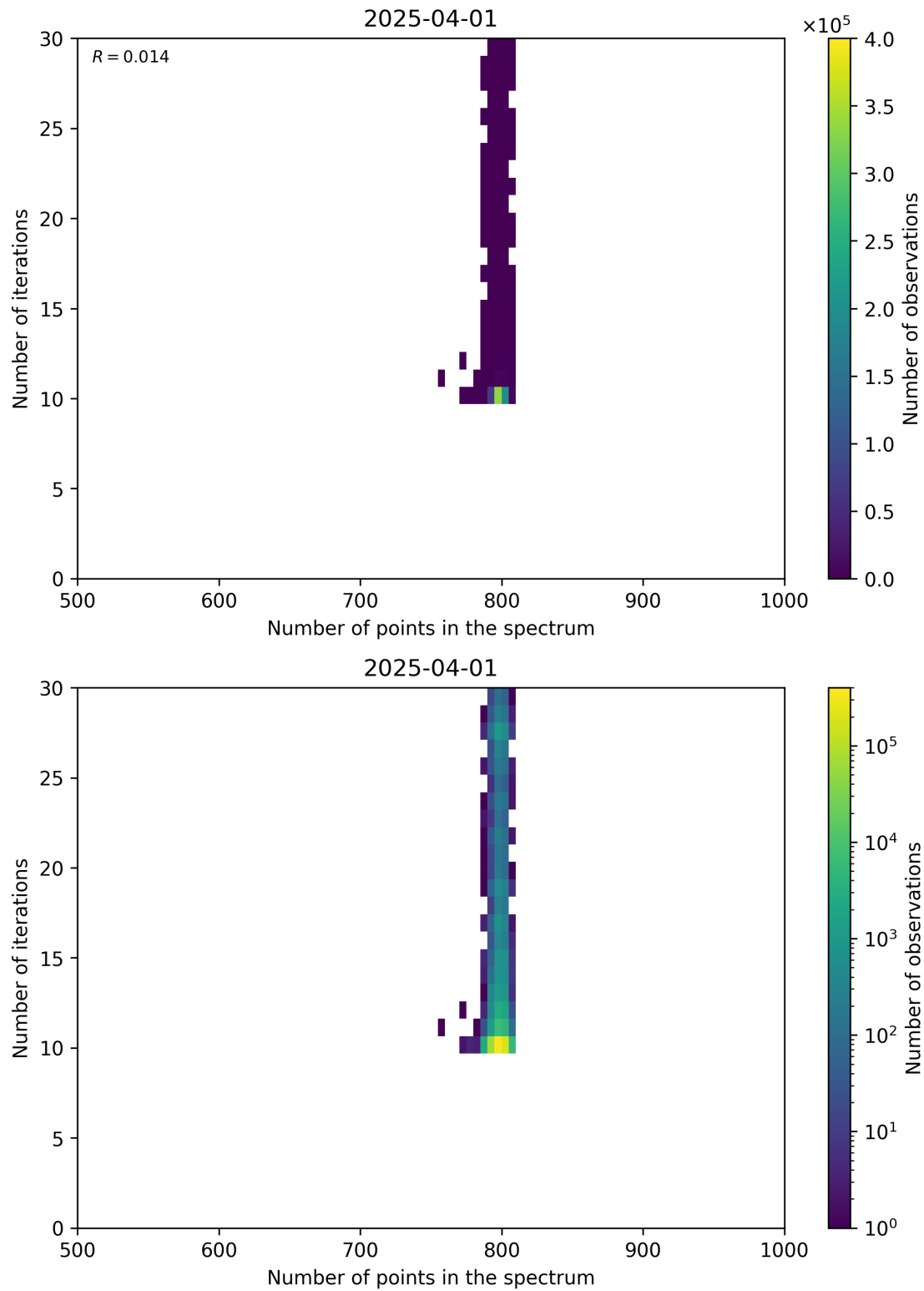
Figure 92: Scatter density plot of “Number of points in the spectrum” against “Number of iterations” for 2025-03-31 to 2025-04-02.
