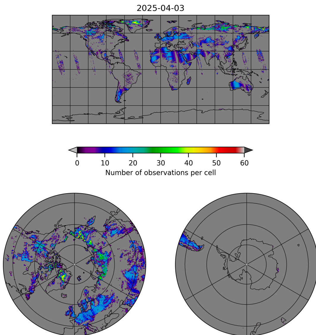
Figure 10: Map of the number of observations for 2025-04-03 to 2025-04-04
