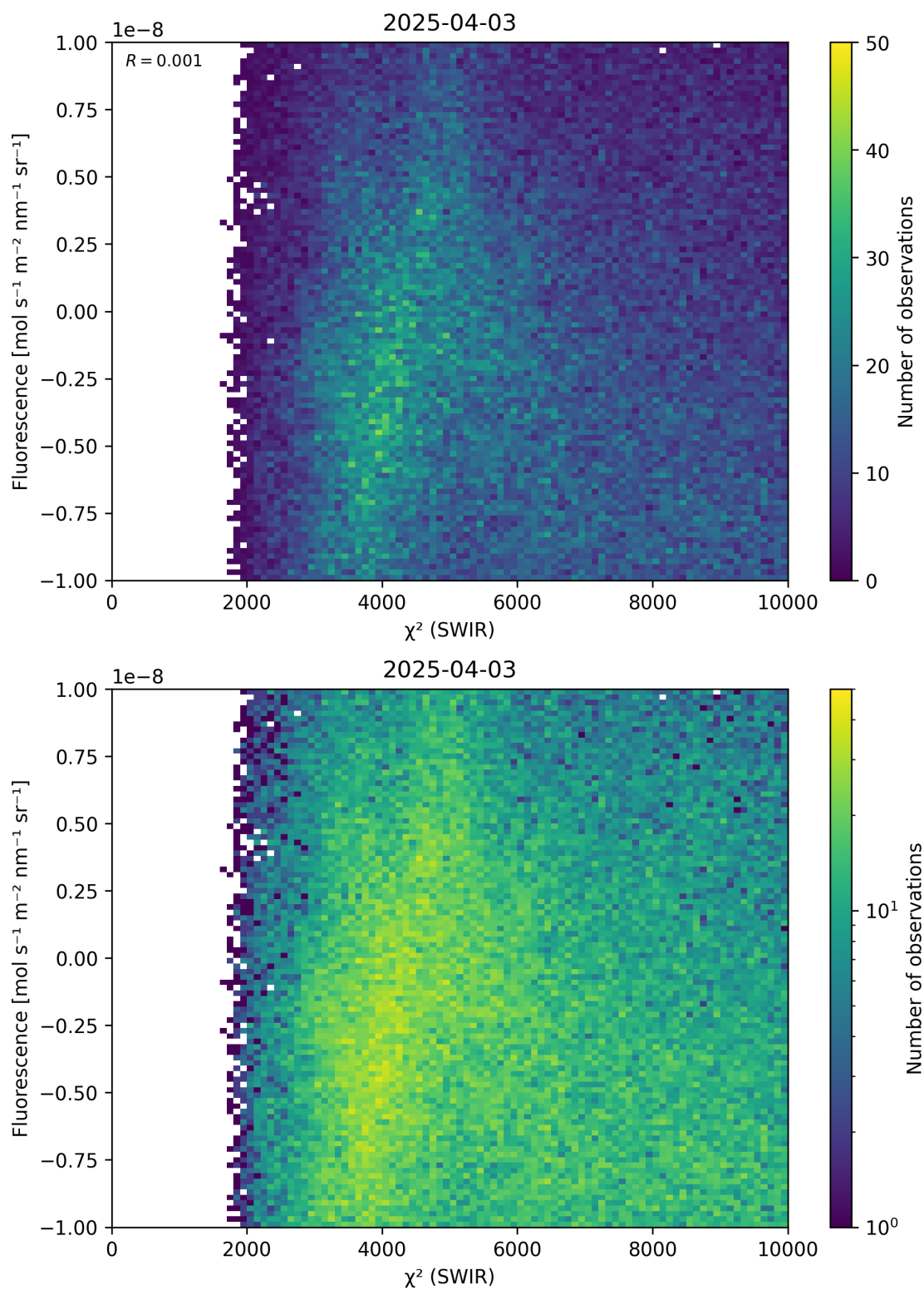
Figure 49: Scatter density plot of “ \chi^2 (SWIR)” against “Fluorescence” for 2025-04-03 to 2025-04-04.
