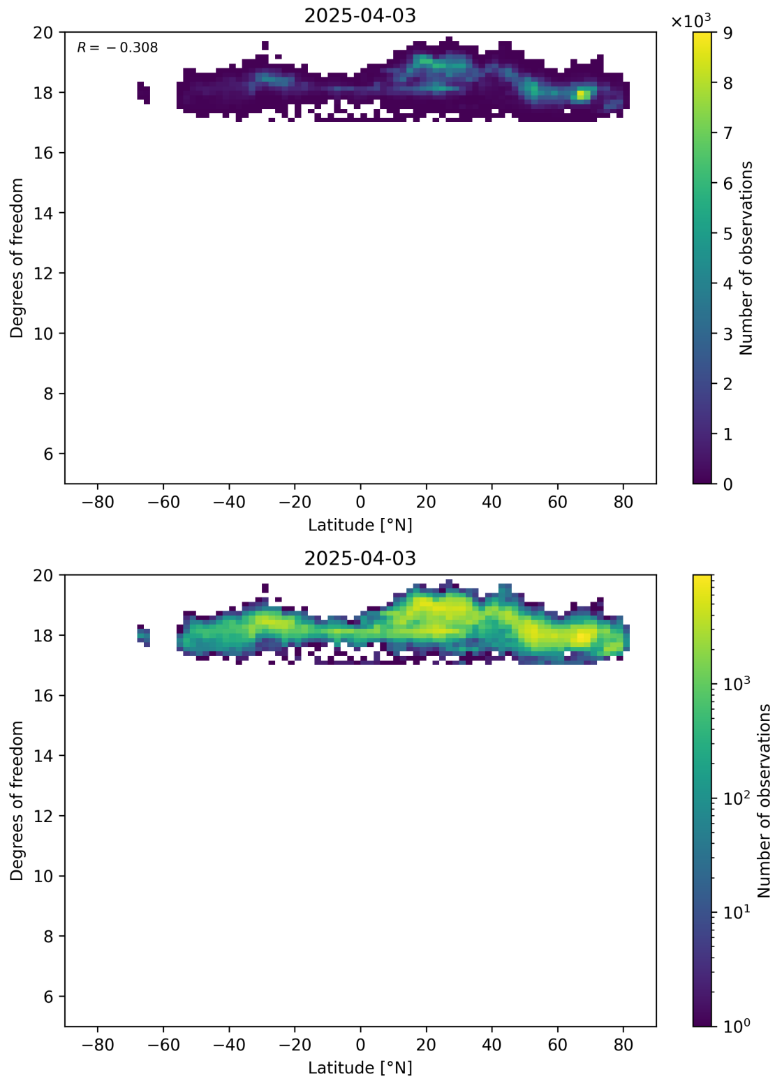
Figure 55: Scatter density plot of “Latitude” against “Degrees of freedom” for 2025-04-03 to 2025-04-04.
