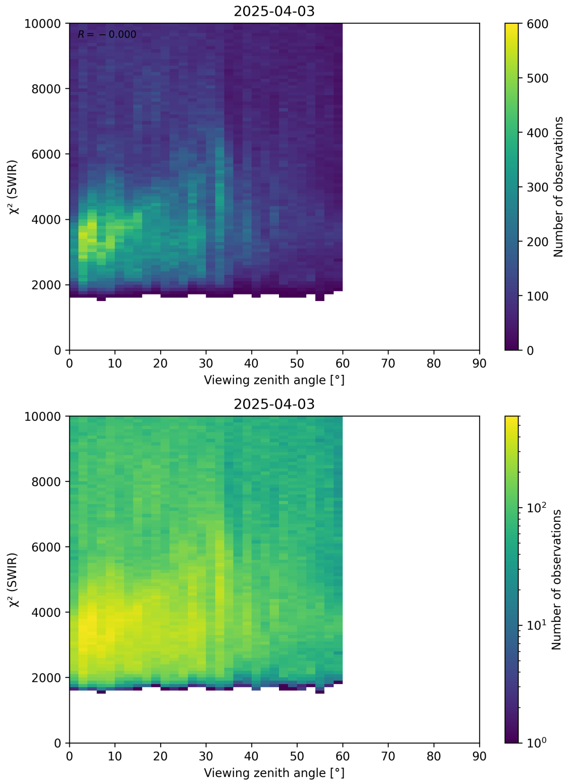
Figure 106: Scatter density plot of “Viewing zenith angle” against “ \chi^2 (SWIR)” for 2025-04-03 to 2025-04-04.
