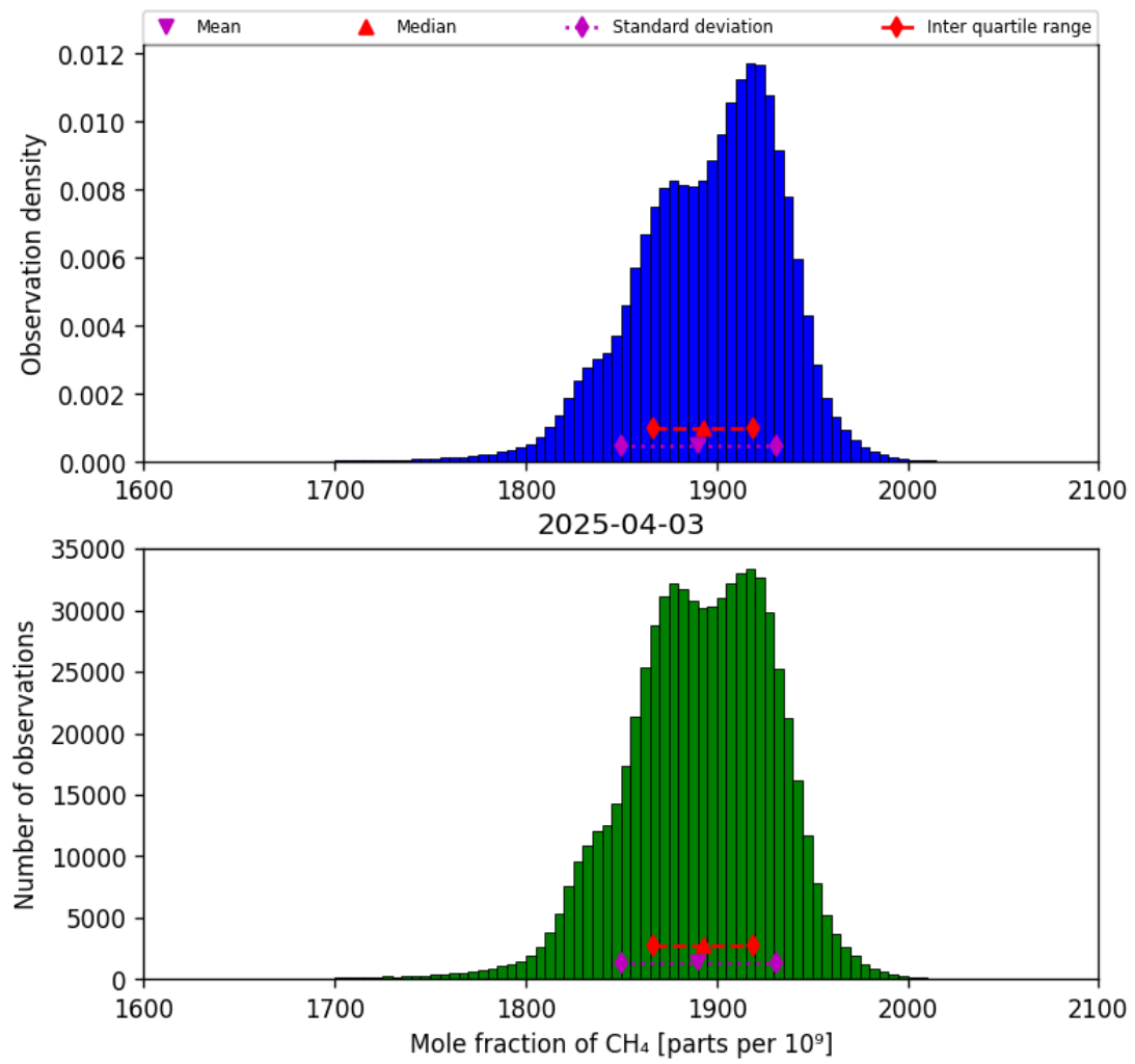
Figure 23: Histogram of “Mole fraction of CH 4 ” for 2025-04-03 to 2025-04-04
