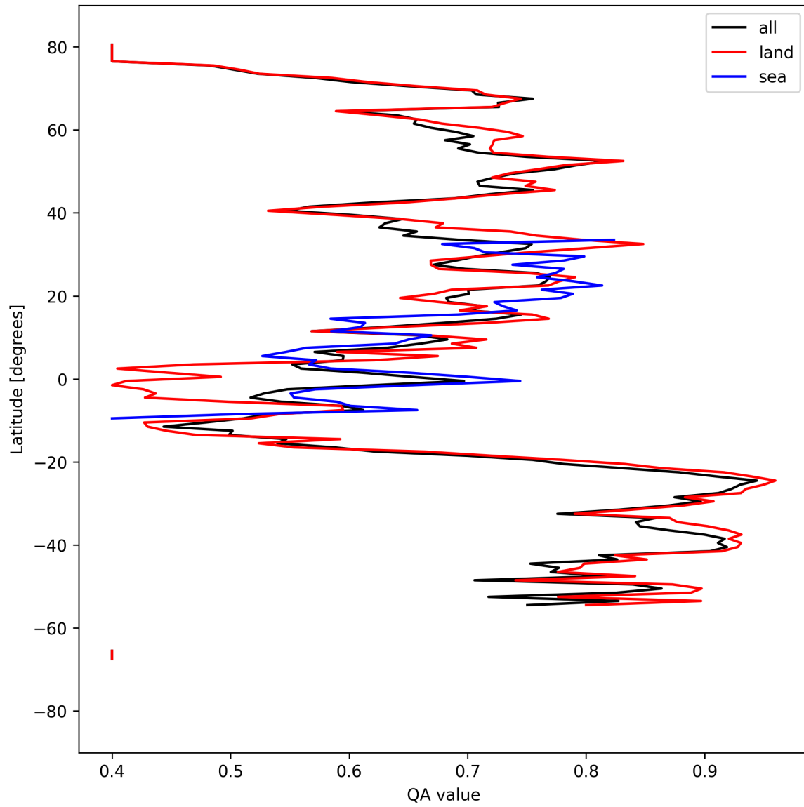
Figure 11: Zonal average of “QA value” for 2025-04-03 to 2025-04-04.
