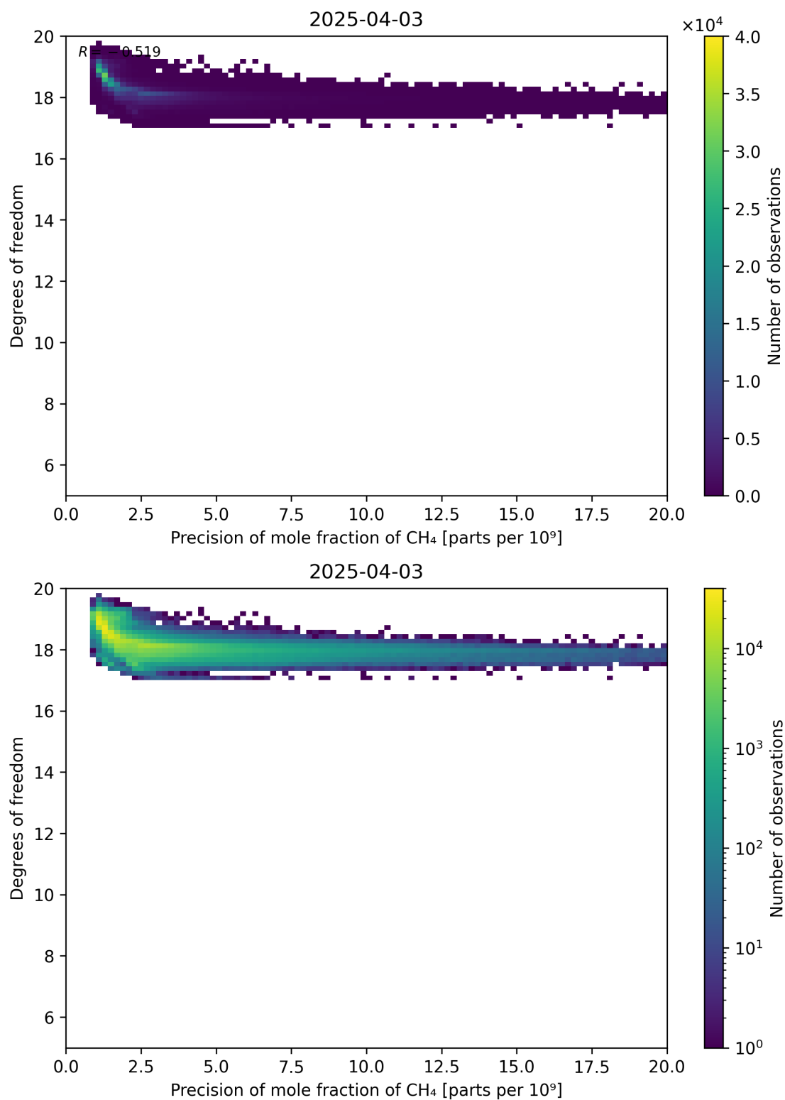
Figure 80: Scatter density plot of “Precision of mole fraction of CH 4 ” against “Degrees of freedom” for 2025-04-03 to 2025-04-04.
