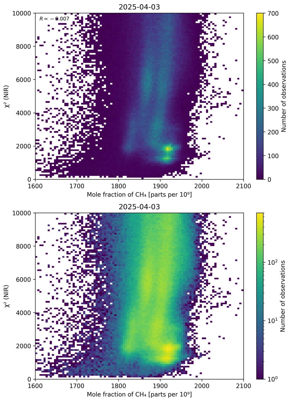
Figure 70: Scatter density plot of “Mole fraction of CH 4 ” against “ \chi^2 (NIR)” for 2025-04-03 to 2025-04-04.
