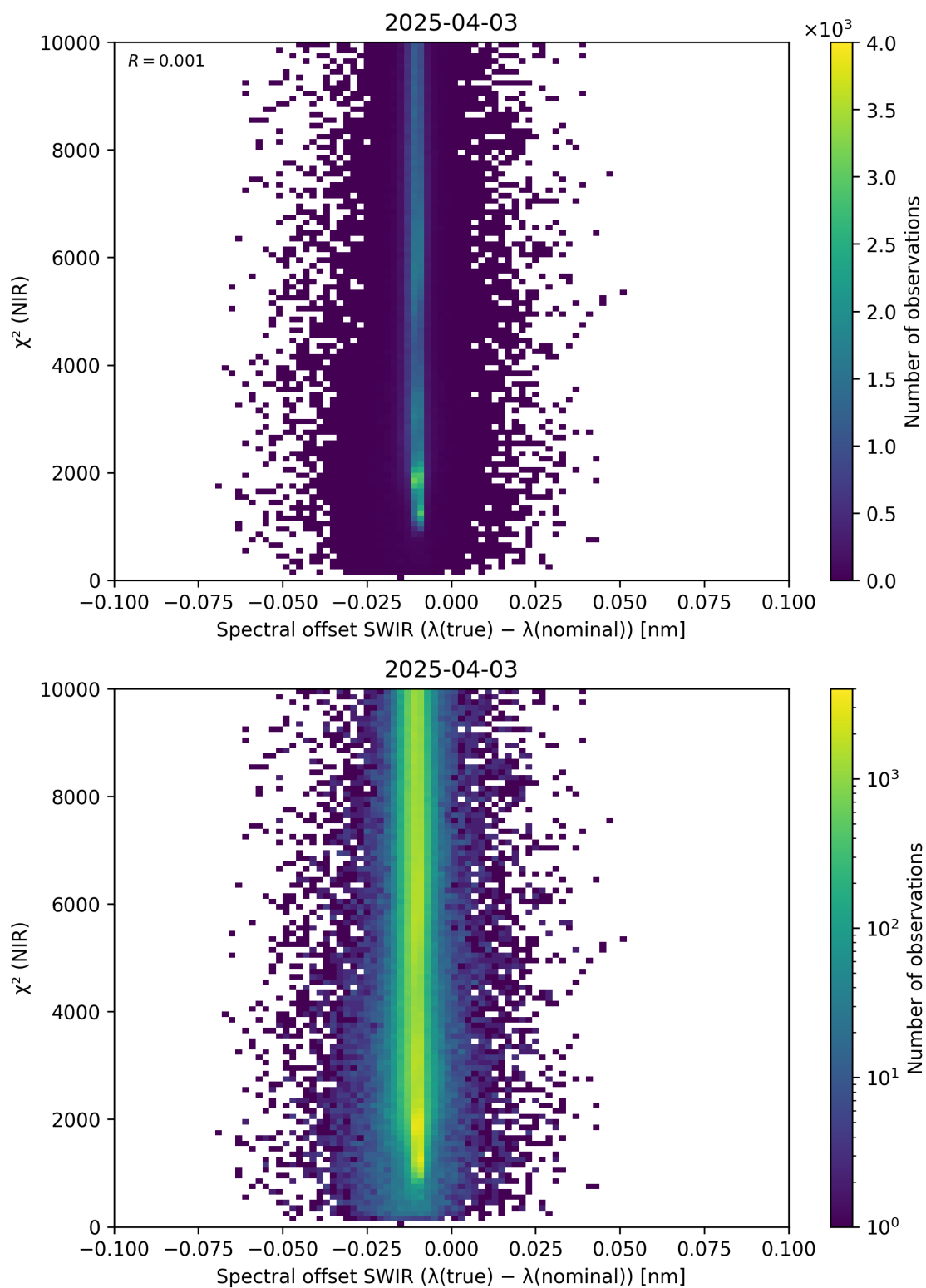
Figure 117: Scatter density plot of “Spectral offset SWIR ( \lambda_{\text{true}} - \lambda_{\text{nominal}} )” against “ \chi^2 (NIR)” for 2025-04-03 to 2025-04-04.
