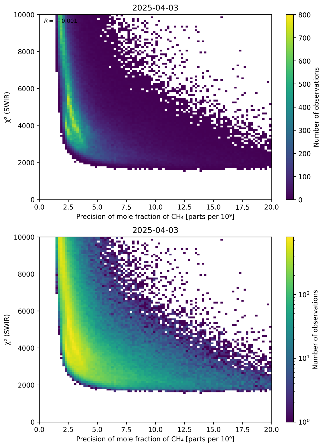
Figure 79: Scatter density plot of “Precision of mole fraction of CH 4 ” against “ \chi^2 (SWIR)” for 2025-04-03 to 2025-04-04.
