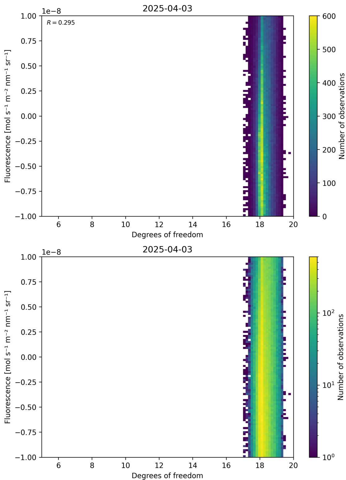
Figure 51: Scatter density plot of “Degrees of freedom” against “Fluorescence” for 2025-04-03 to 2025-04-04.
