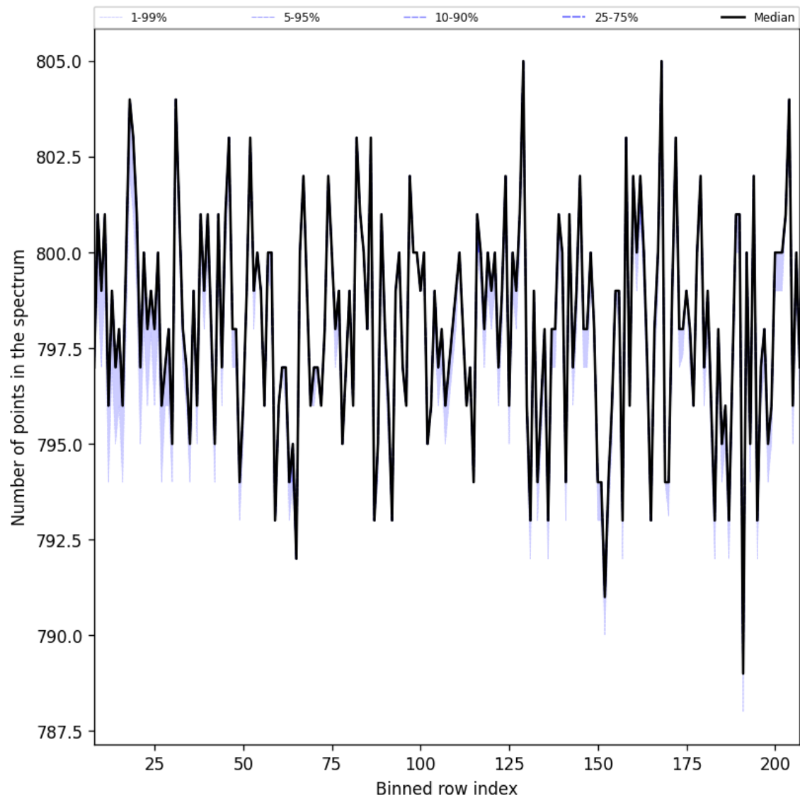
Figure 37: Along track statistics of “Number of points in the spectrum” for 2025-04-03 to 2025-04-04
