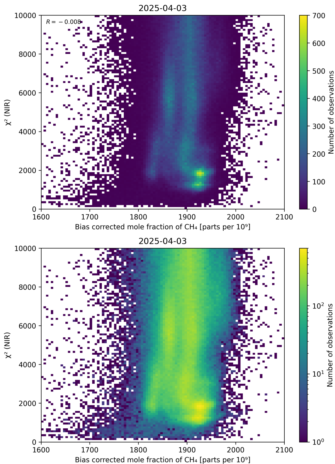
Figure 63: Scatter density plot of “Bias corrected mole fraction of CH 4 ” against “ \chi^2 (NIR)” for 2025-04-03 to 2025-04-04.
