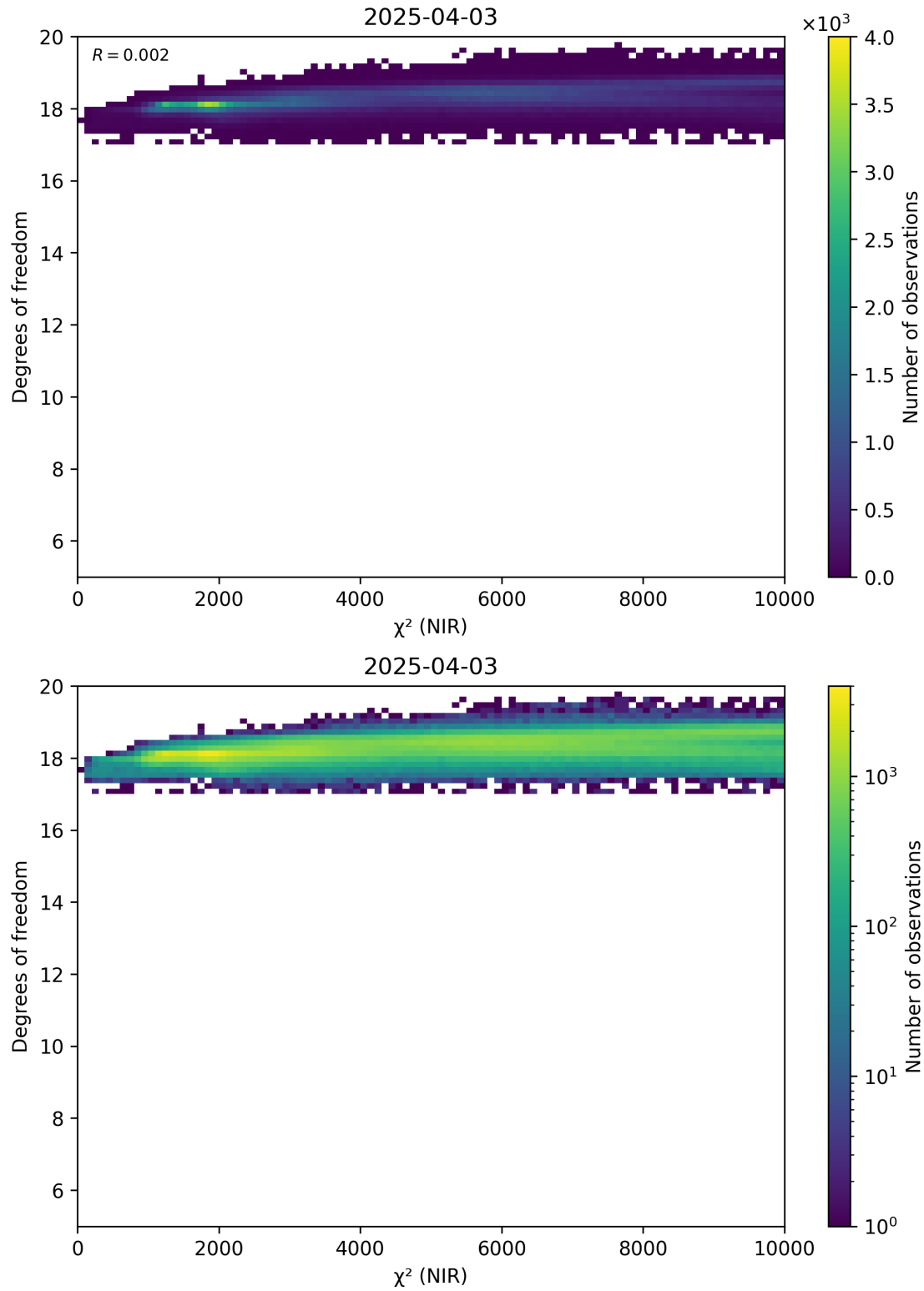
Figure 44: Scatter density plot of “ \chi^2 (NIR)” against “Degrees of freedom” for 2025-04-03 to 2025-04-04.
