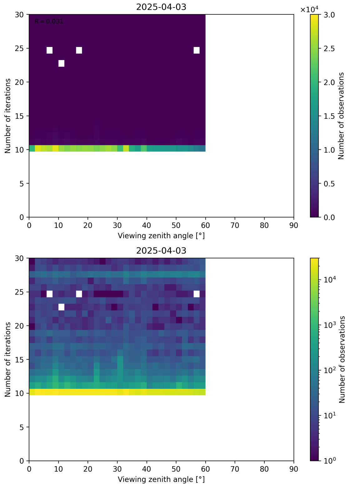
Figure 113: Scatter density plot of “Viewing zenith angle” against “Number of iterations” for 2025-04-03 to 2025-04-04.
