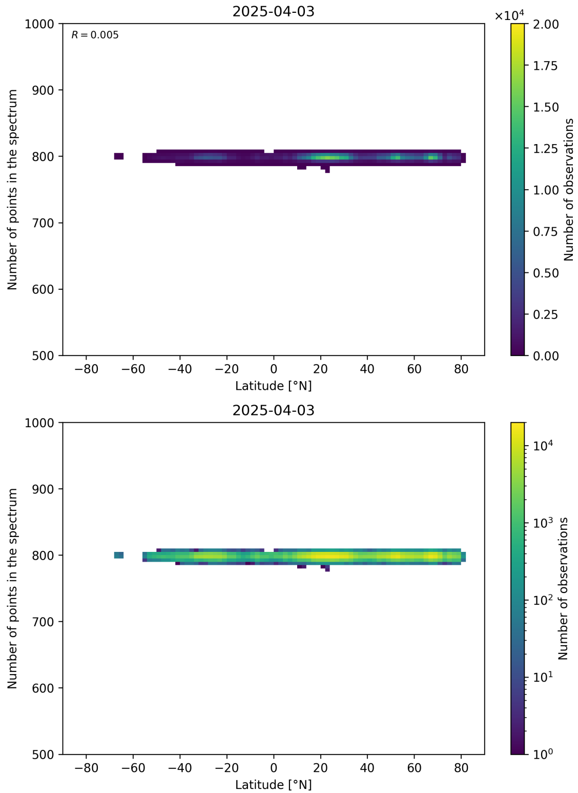
Figure 61: Scatter density plot of “Latitude” against “Number of points in the spectrum” for 2025-04-03 to 2025-04-04.
