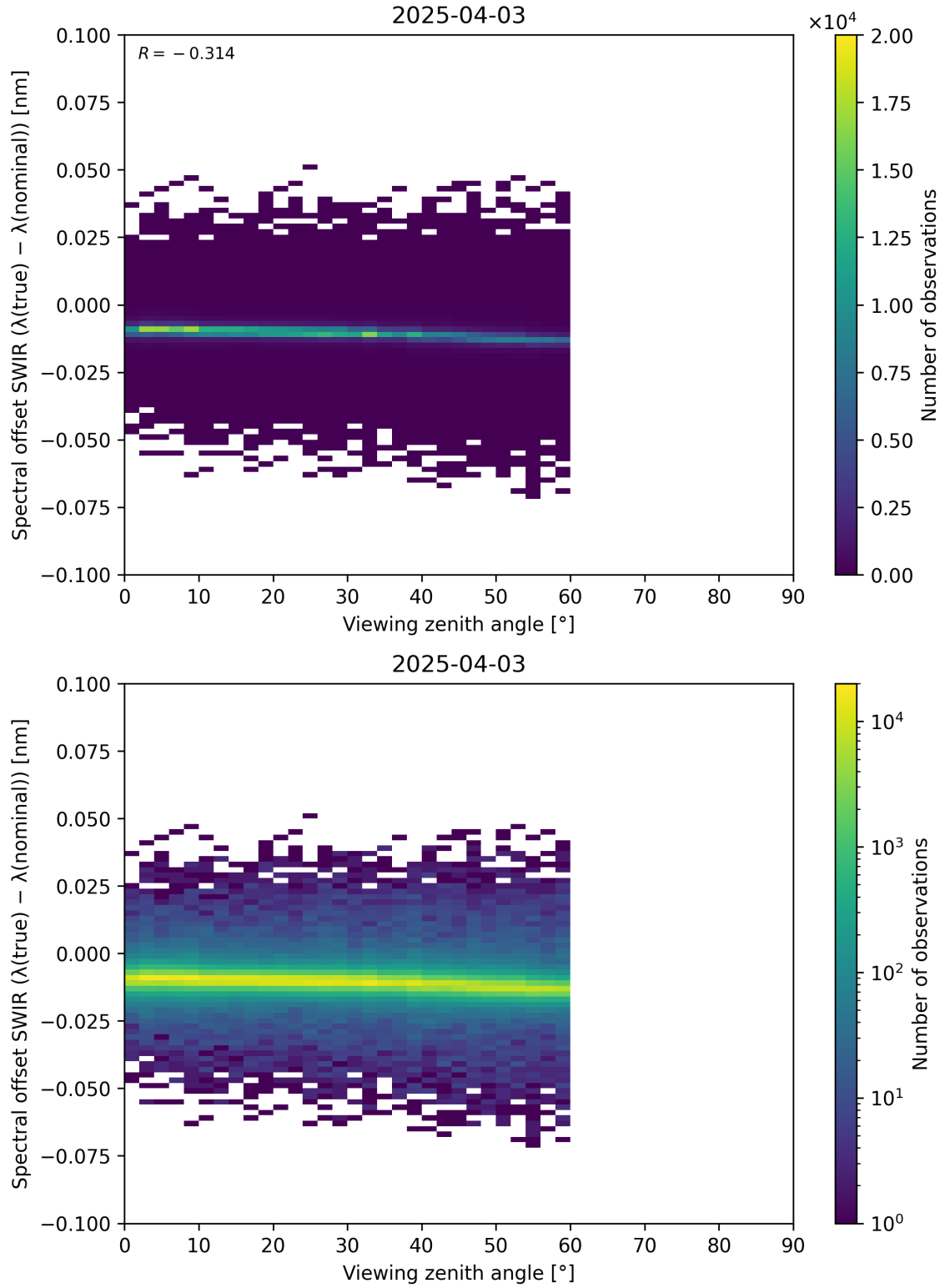
Figure 116: Scatter density plot of “Viewing zenith angle” against “Spectral offset SWIR ( \lambda_{\text{true}} - \lambda_{\text{nominal}} )” for 2025-04-03 to 2025-04-04.
