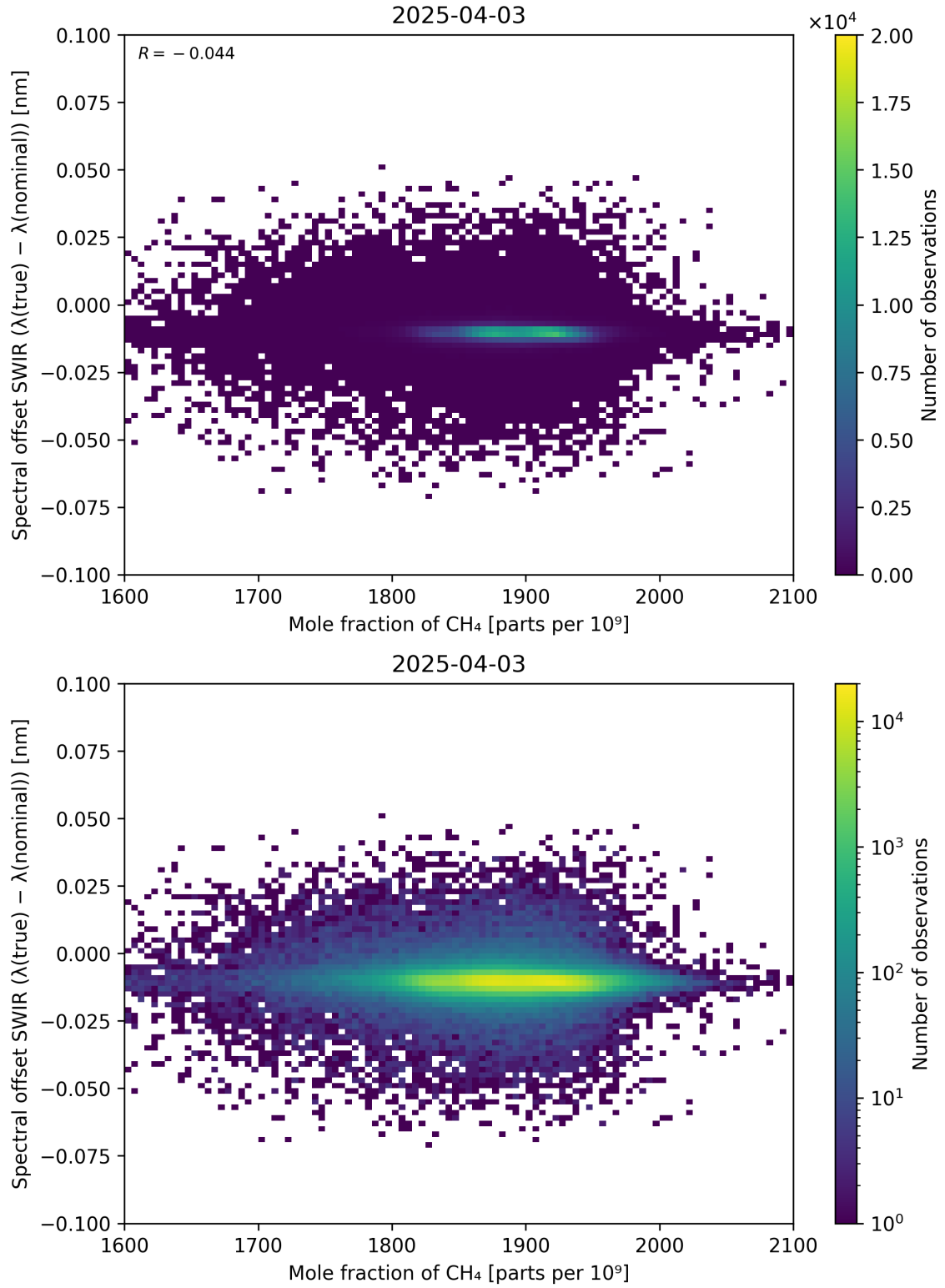
Figure 86: Scatter density plot of “Mole fraction of CH 4 ” against “Spectral offset SWIR ( \lambda_{\text{true}} - \lambda_{\text{nominal}} )” for 2025-04-03 to 2025-04-04.
