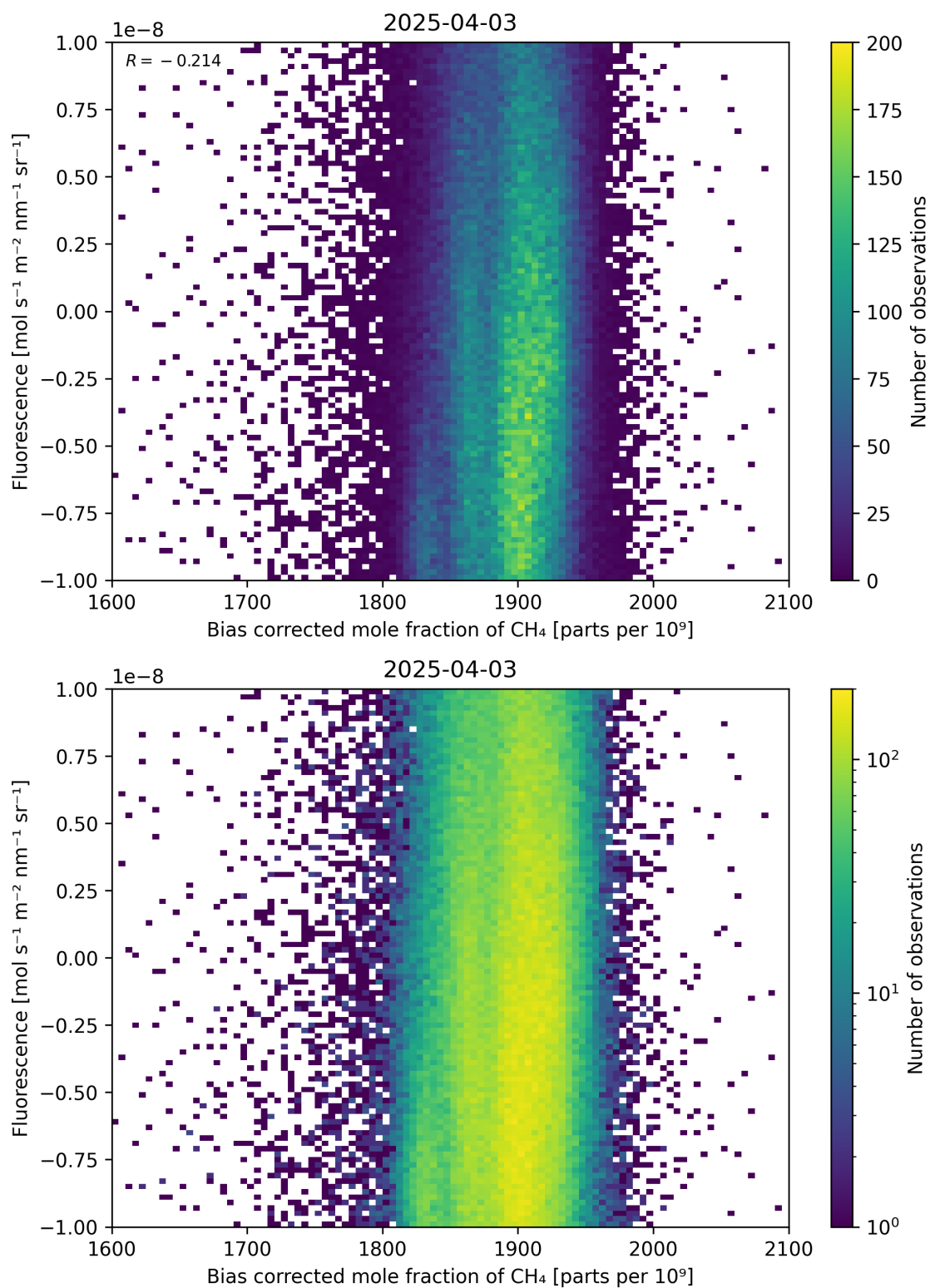
Figure 66: Scatter density plot of “Bias corrected mole fraction of \text{CH}_4 ” against “Fluorescence” for 2025-04-03 to 2025-04-04.
