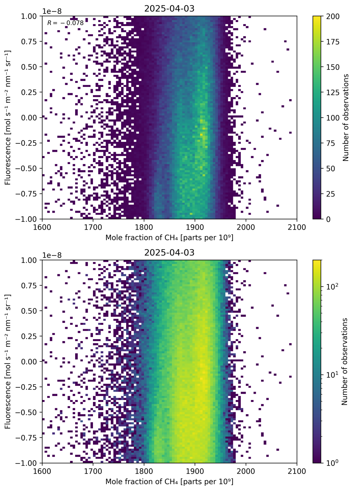
Figure 73: Scatter density plot of “Mole fraction of \text{CH}_4 ” against “Fluorescence” for 2025-04-03 to 2025-04-04.
