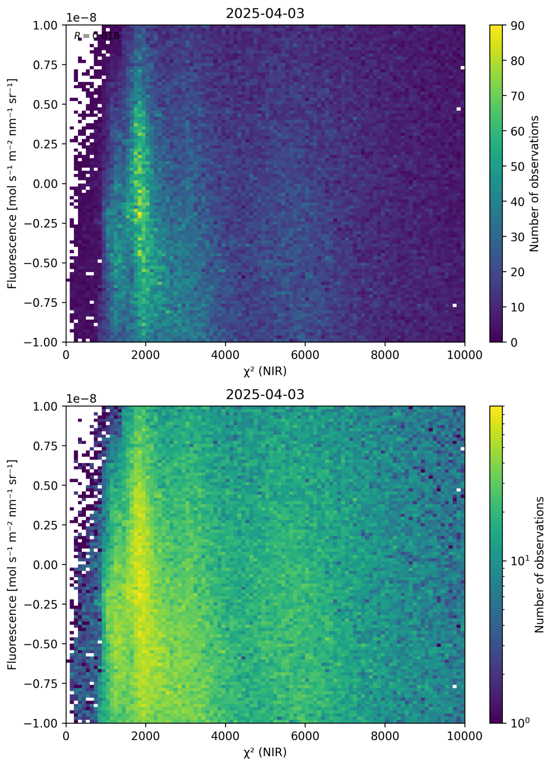
Figure 45: Scatter density plot of “ \chi^2 (NIR)” against “Fluorescence” for 2025-04-03 to 2025-04-04.
