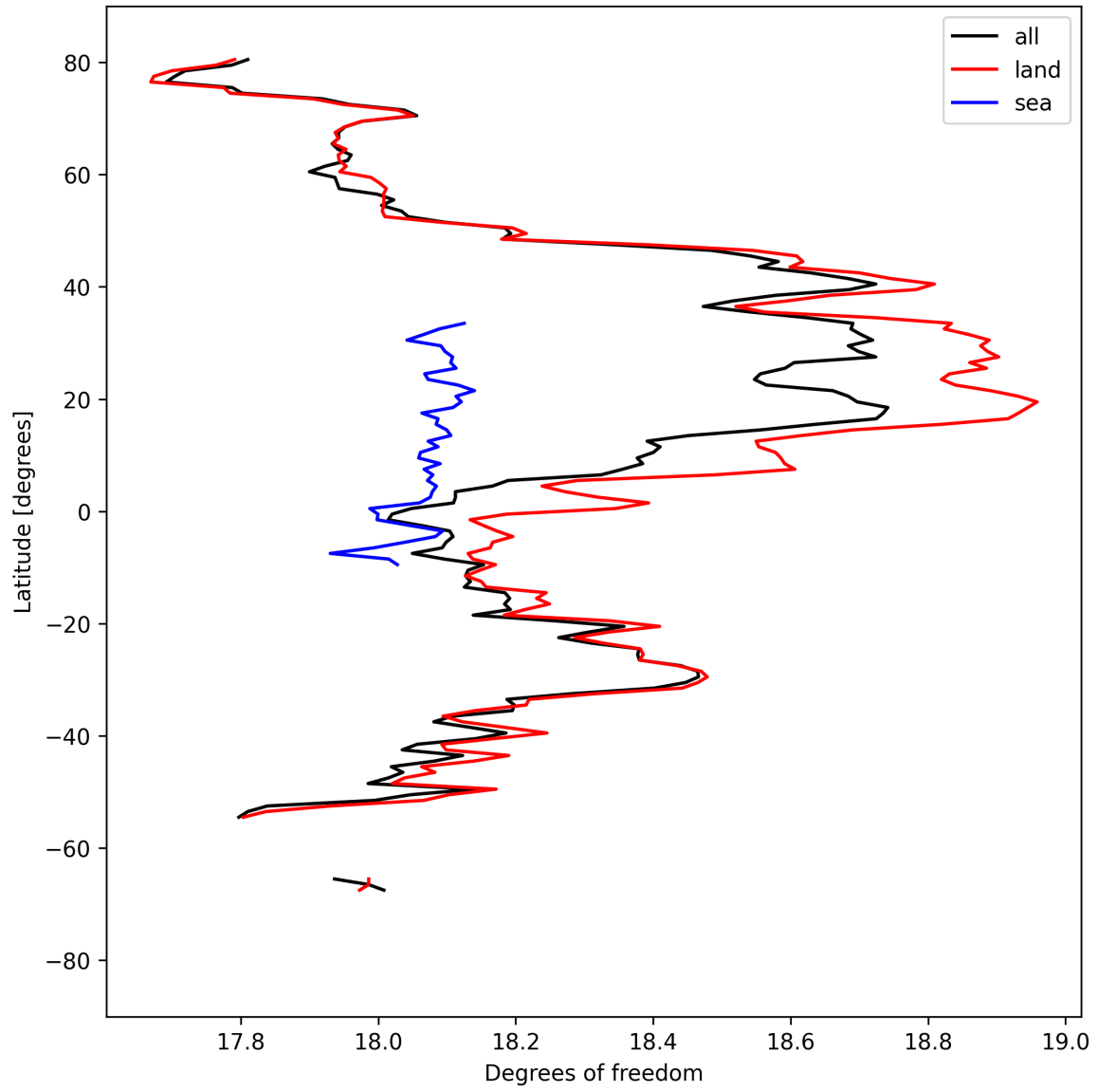
Figure 19: Zonal average of "Degrees of freedom" for 2025-04-03 to 2025-04-04.
