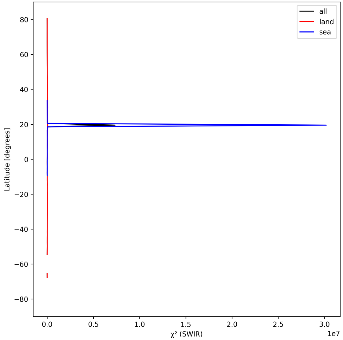
Figure 17: Zonal average of “ \chi^2 (SWIR)” for 2025-04-03 to 2025-04-04.
