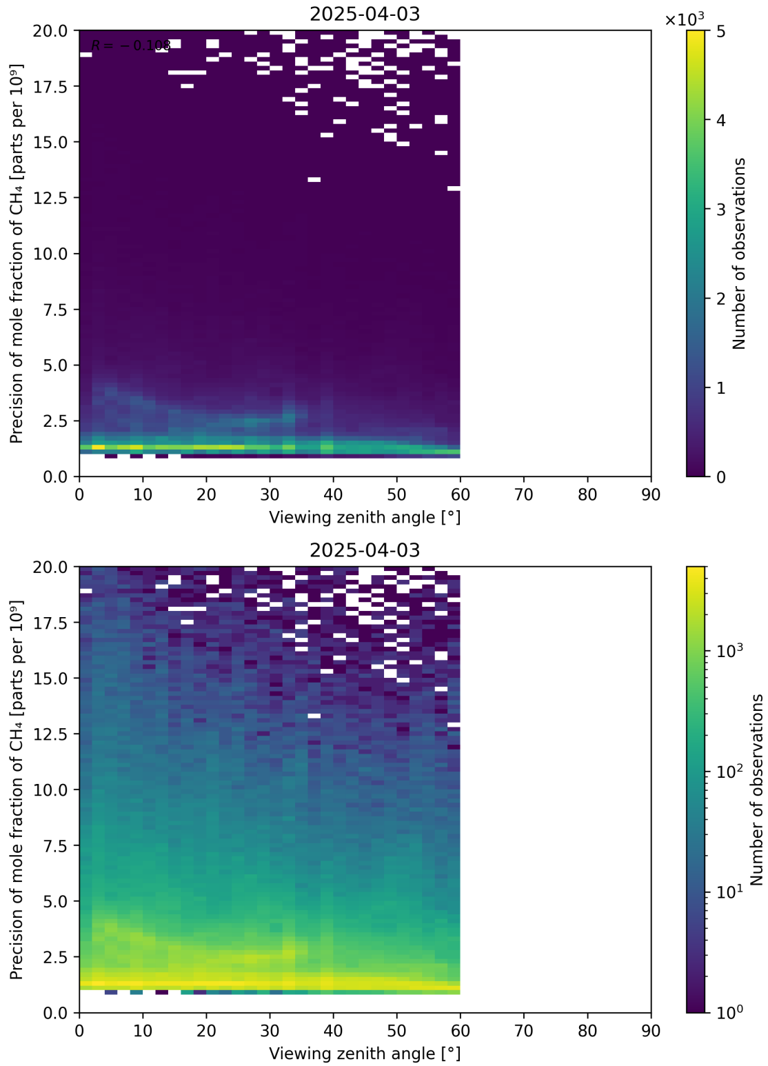
Figure 112: Scatter density plot of “Viewing zenith angle” against “Precision of mole fraction of CH 4 ” for 2025-04-03 to 2025-04-04.
