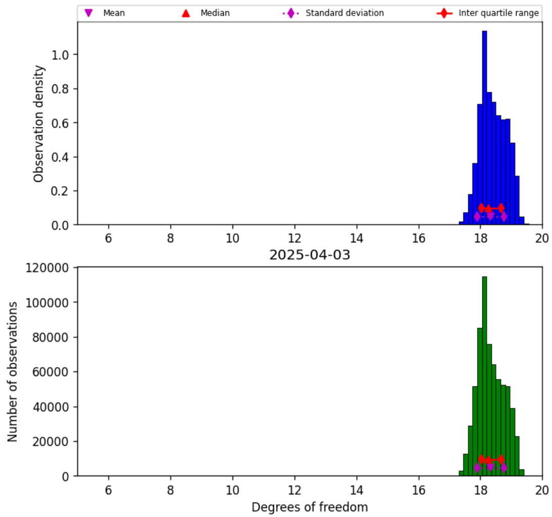
Figure 30: Histogram of “Degrees of freedom” for 2025-04-03 to 2025-04-04
