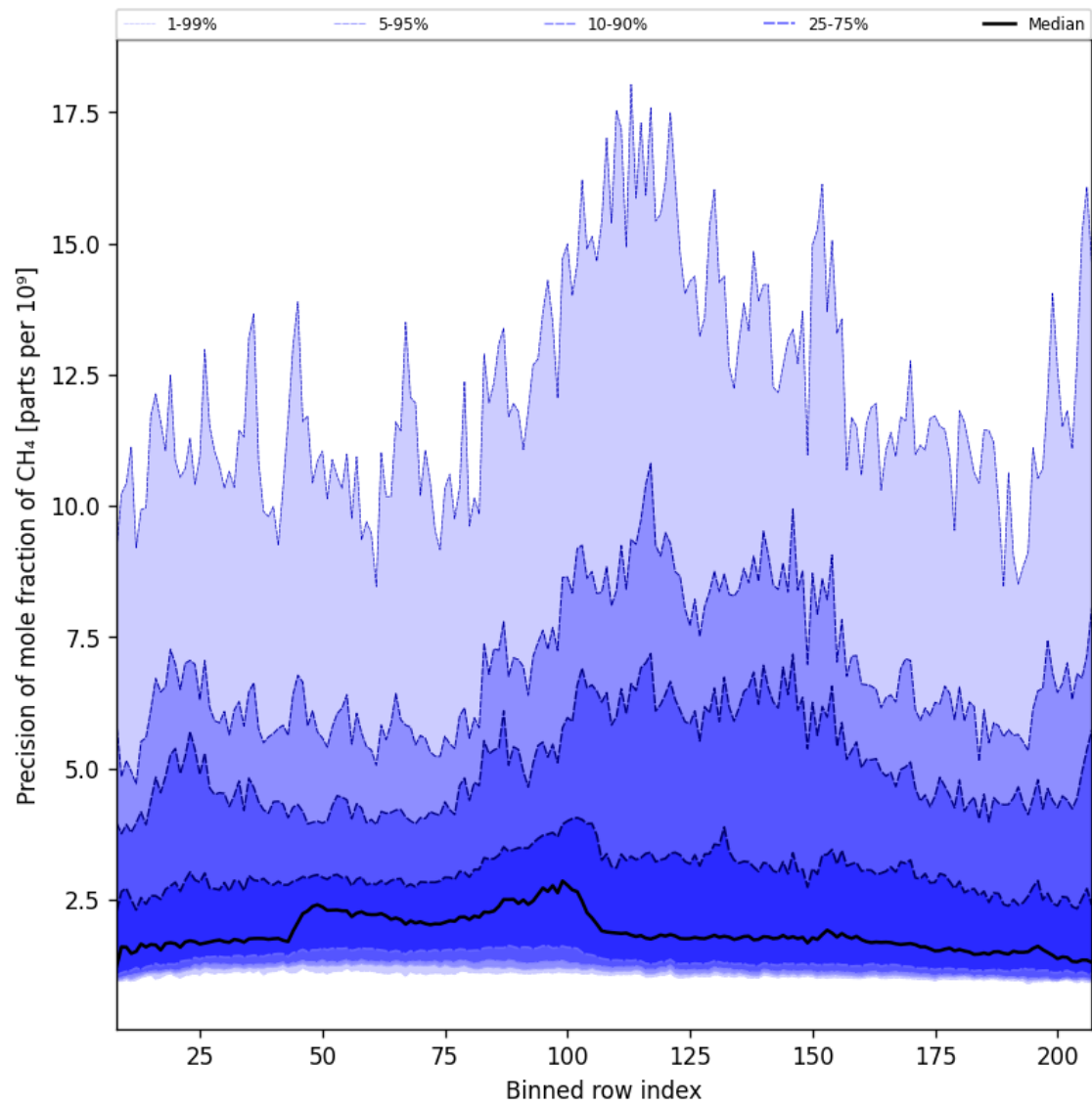
Figure 35: Along track statistics of “Precision of mole fraction of CH 4 ” for 2025-04-03 to 2025-04-04
