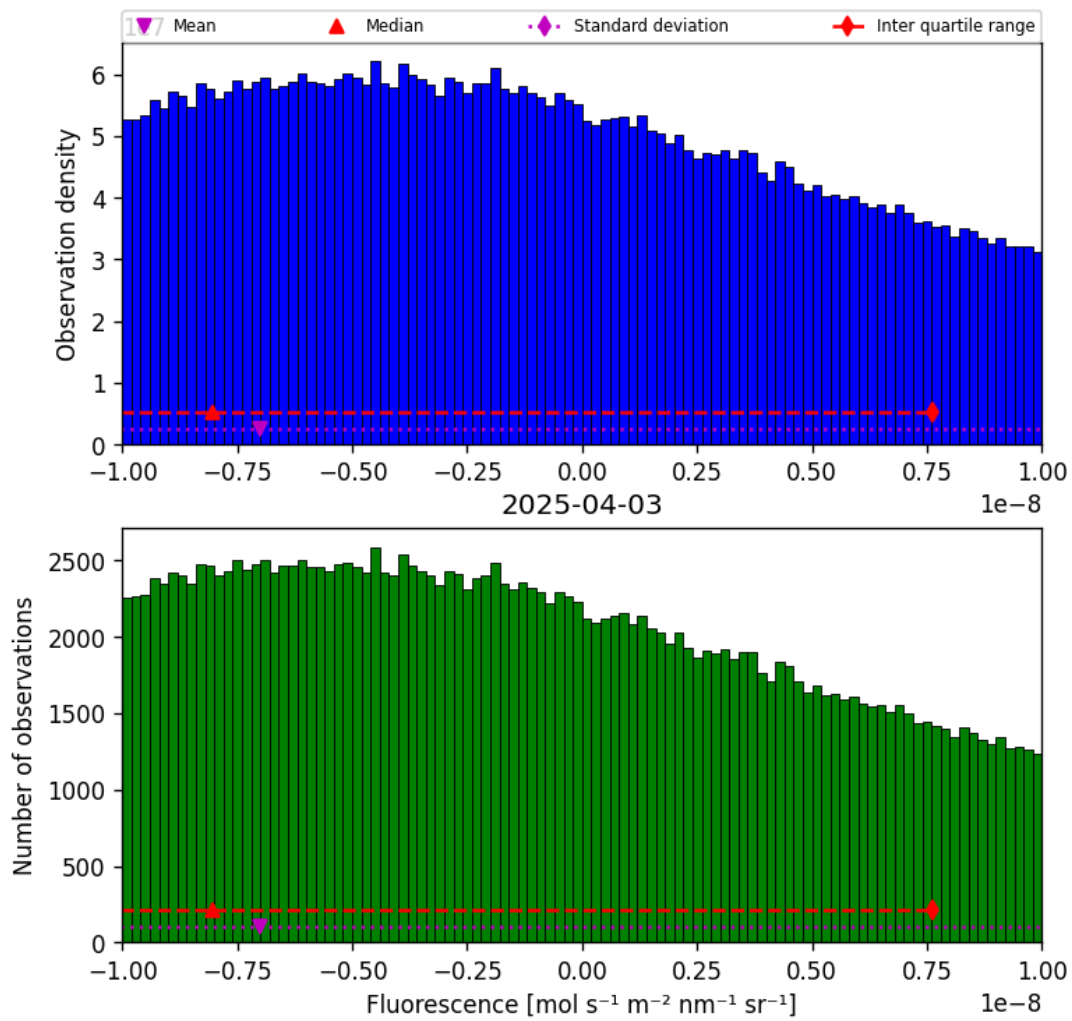
Figure 32: Histogram of “Fluorescence” for 2025-04-03 to 2025-04-04
