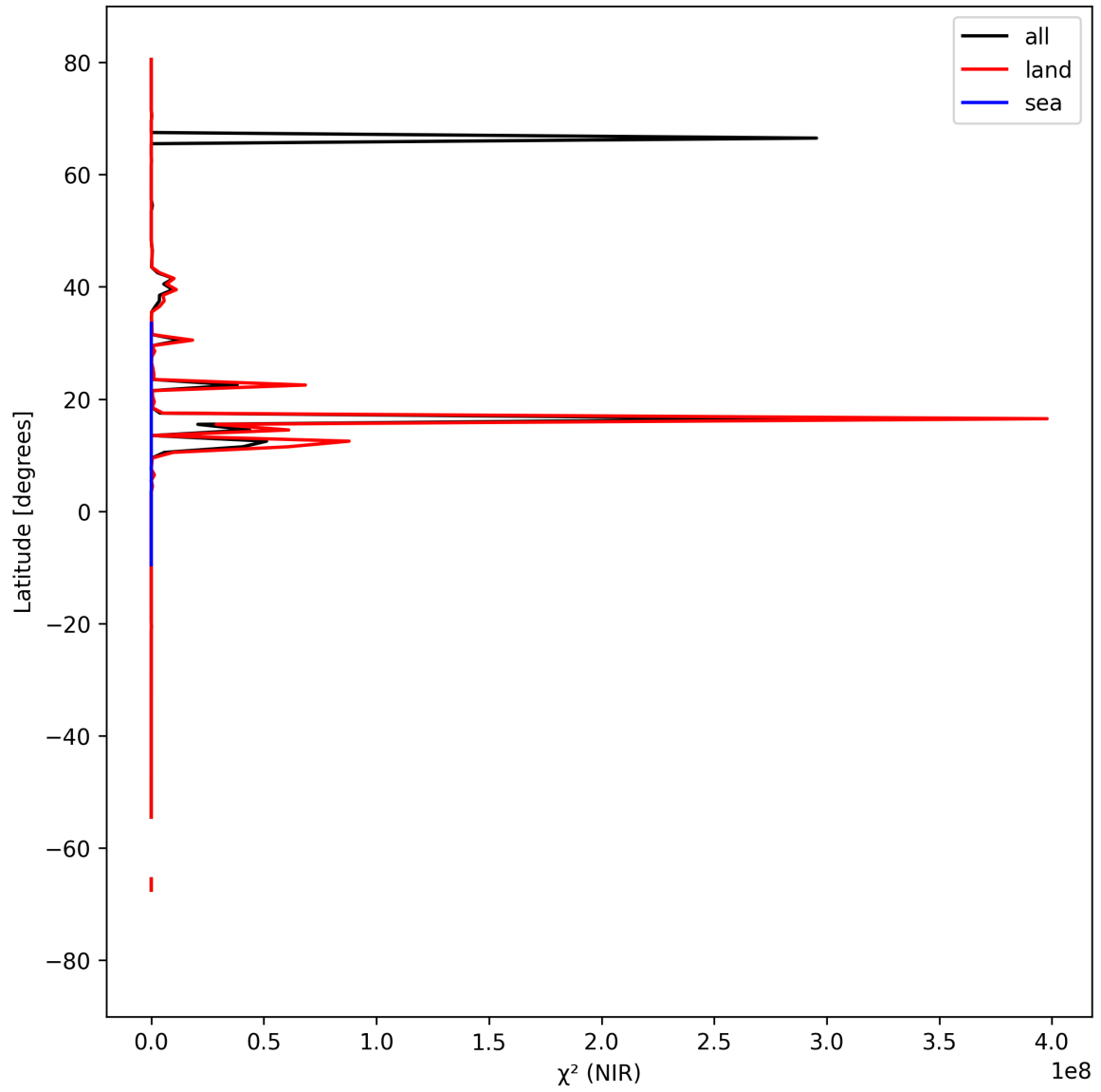
Figure 18: Zonal average of “ \chi^2 (NIR)” for 2025-04-03 to 2025-04-04.
