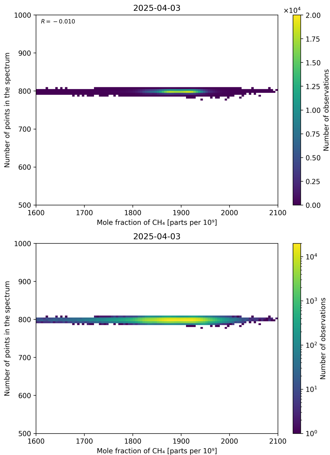
Figure 77: Scatter density plot of “Mole fraction of CH 4 ” against “Number of points in the spectrum” for 2025-04-03 to 2025-04-04.
