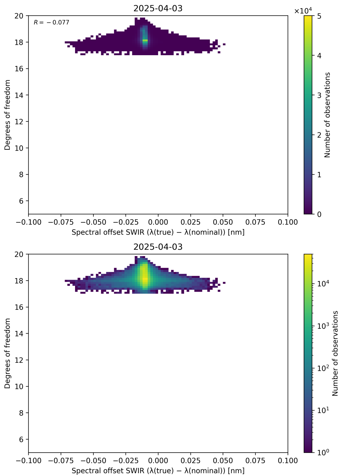
Figure 119: Scatter density plot of “Spectral offset SWIR ( \lambda_{\text{true}} - \lambda_{\text{nominal}} )” against “Degrees of freedom” for 2025-04-03 to 2025-04-04.
