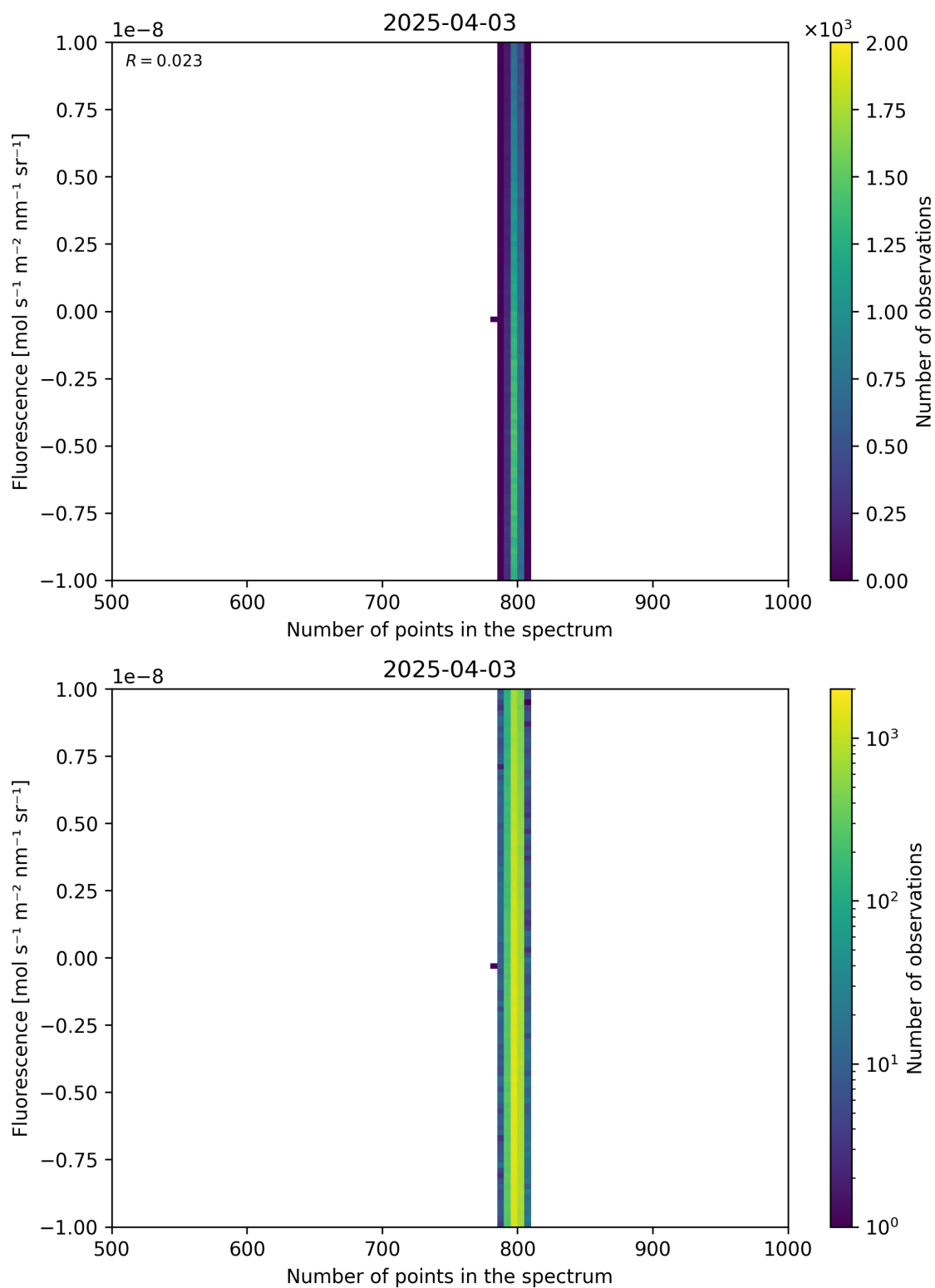
Figure 91: Scatter density plot of “Number of points in the spectrum” against “Fluorescence” for 2025-04-03 to 2025-04-04.
