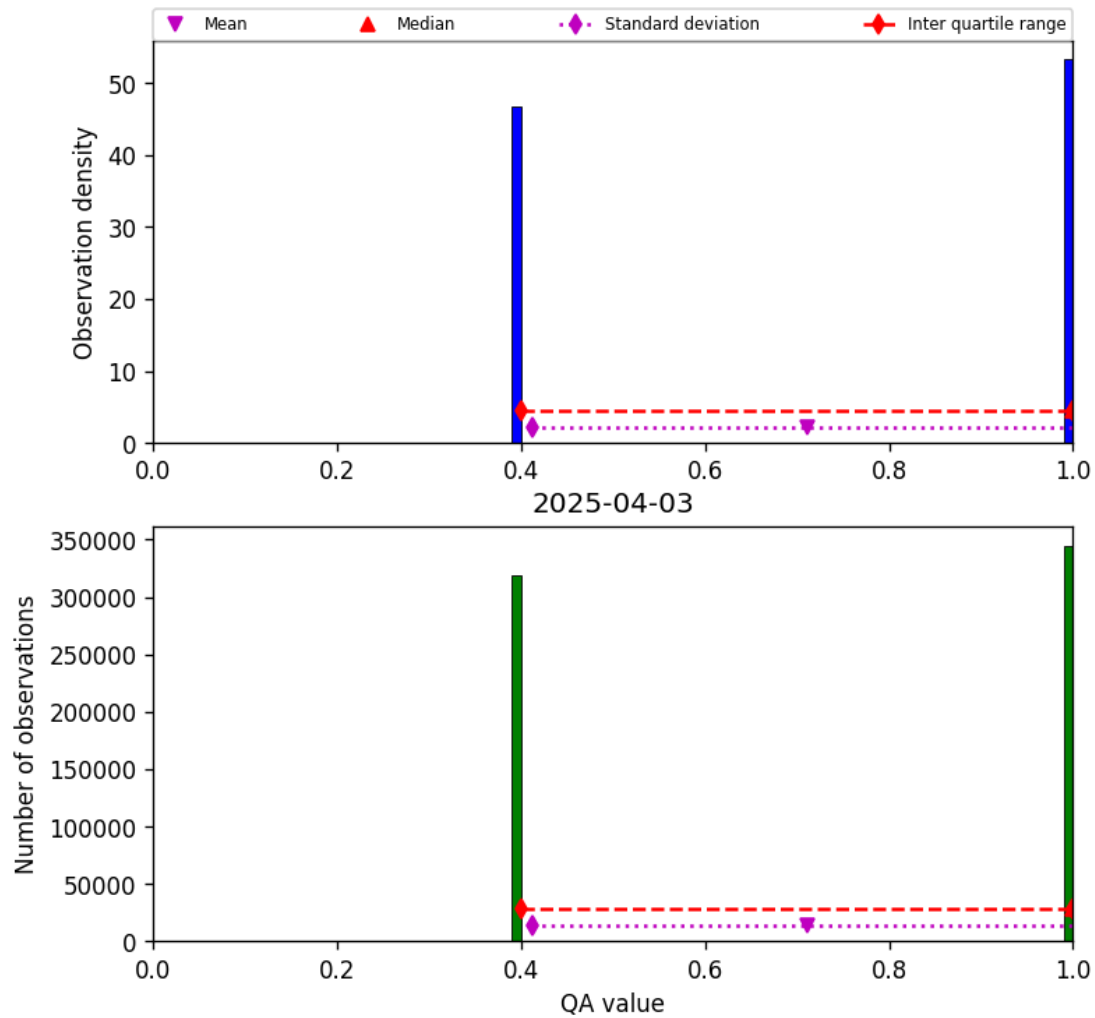
Figure 22: Histogram of “QA value” for 2025-04-03 to 2025-04-04
