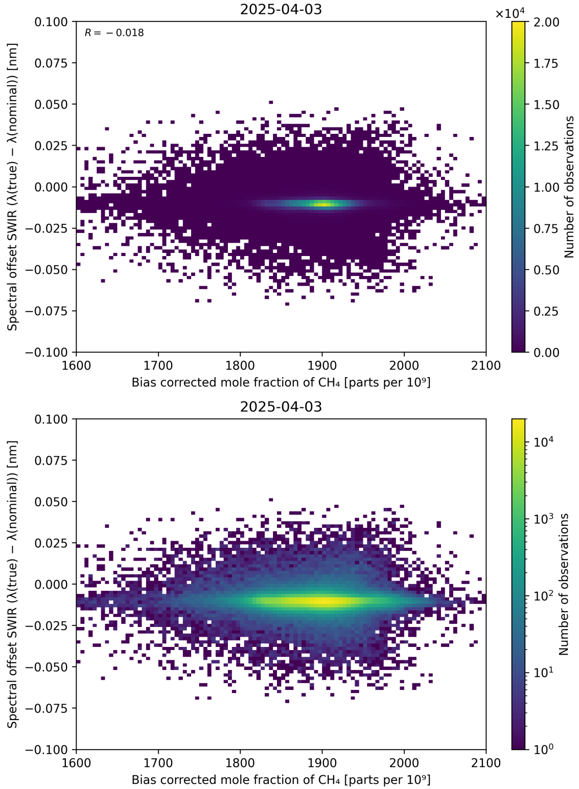
Figure 69: Scatter density plot of “Bias corrected mole fraction of \text{CH}_4 ” against “Spectral offset SWIR ( \lambda_{\text{true}} - \lambda_{\text{nominal}} )” for 2025-04-03 to 2025-04-04.
