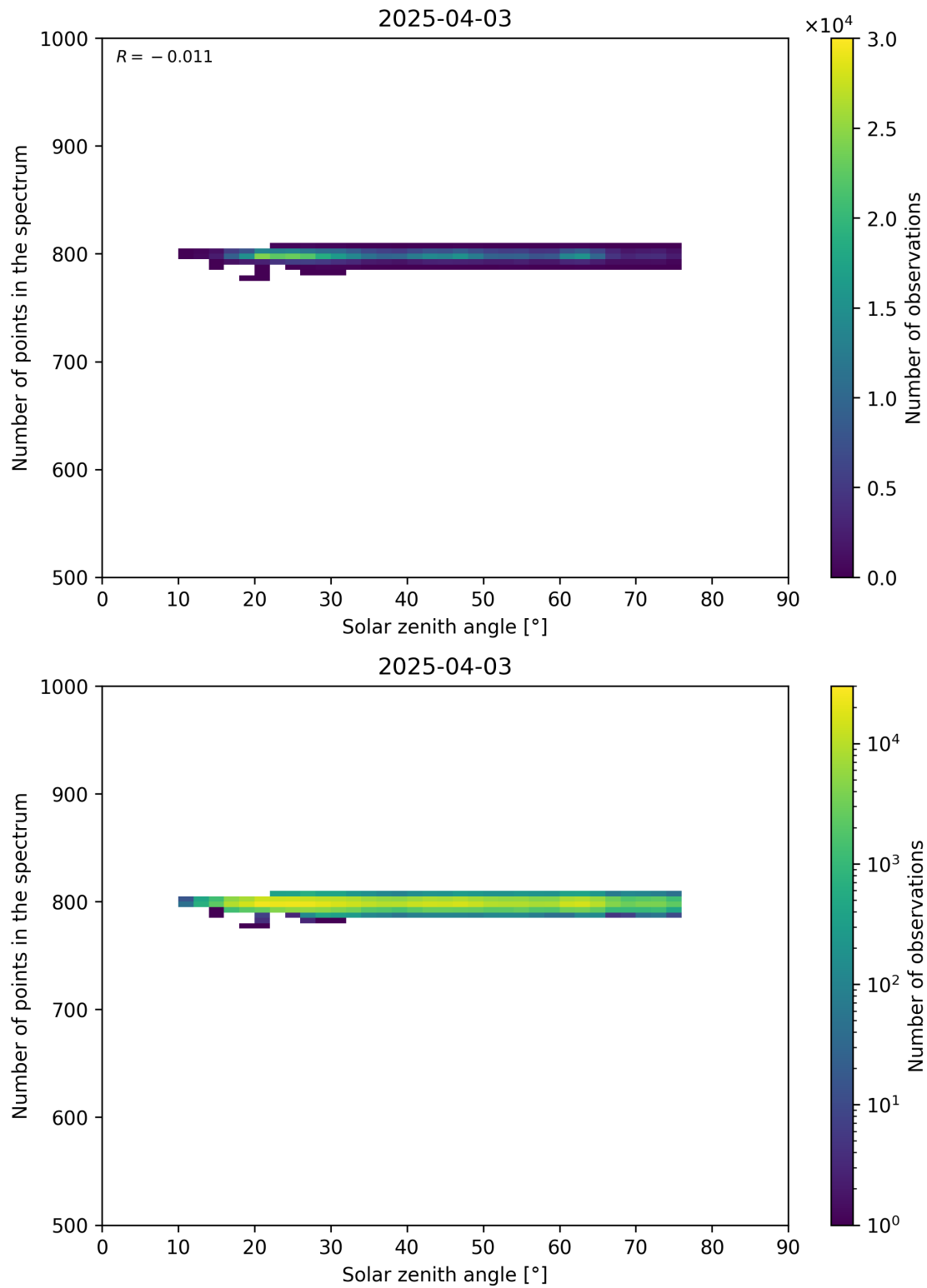
Figure 103: Scatter density plot of “Solar zenith angle” against “Number of points in the spectrum” for 2025-04-03 to 2025-04-04.
