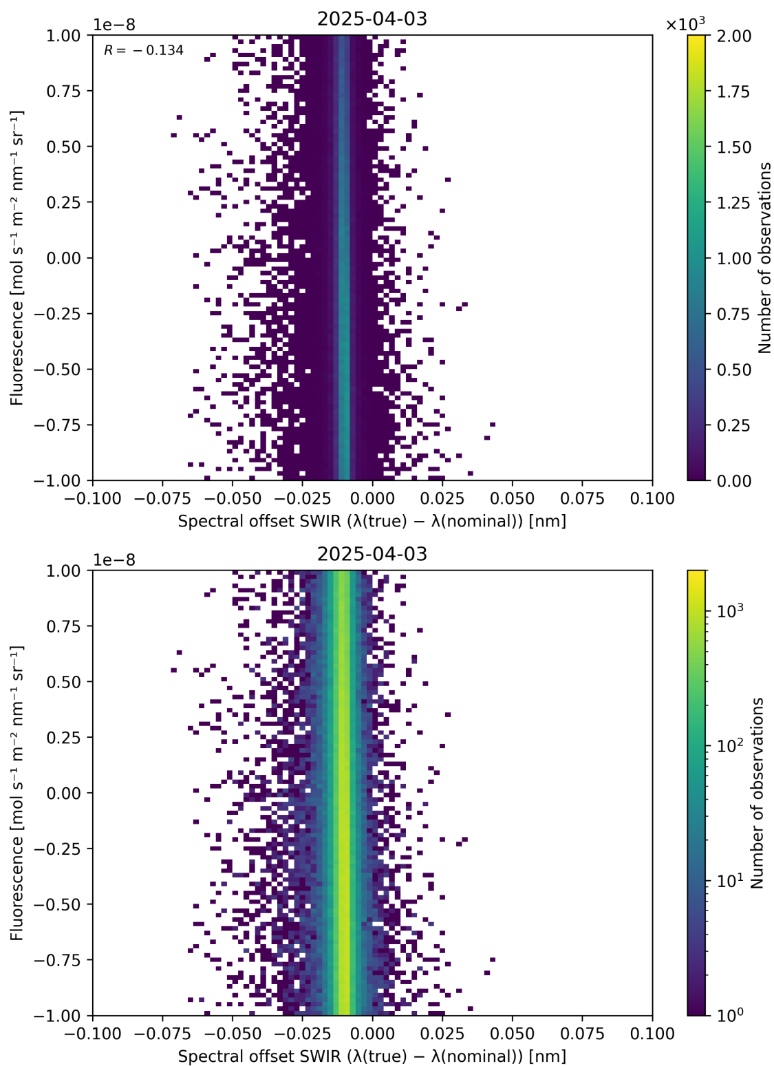
Figure 120: Scatter density plot of “Spectral offset SWIR ( \lambda_{\text{true}} - \lambda_{\text{nominal}} )” against “Fluorescence” for 2025-04-03 to 2025-04-04.
