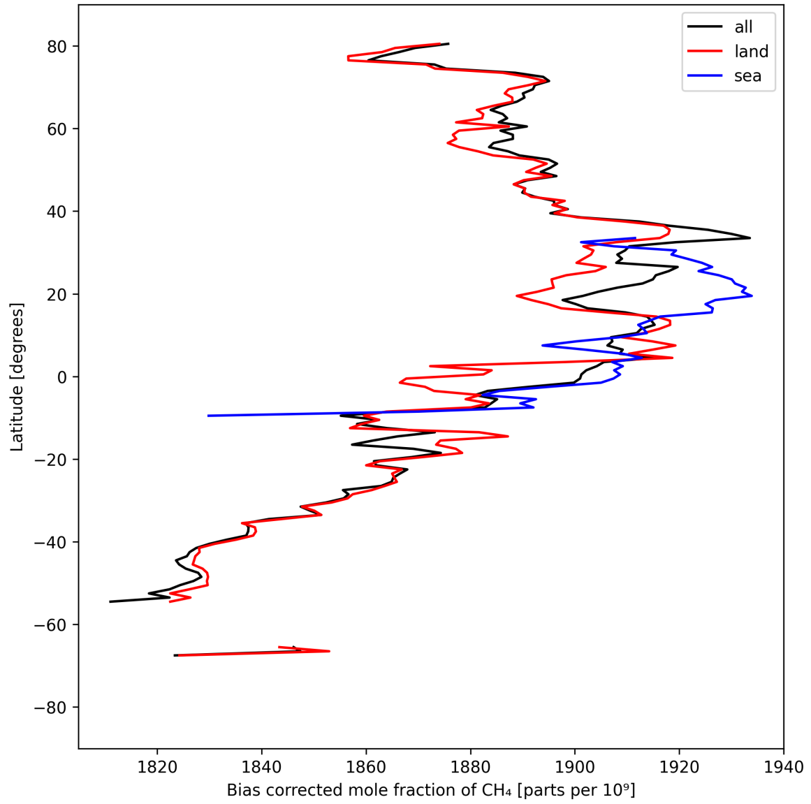
Figure 14: Zonal average of “Bias corrected mole fraction of CH 4 ” for 2025-04-03 to 2025-04-04.
