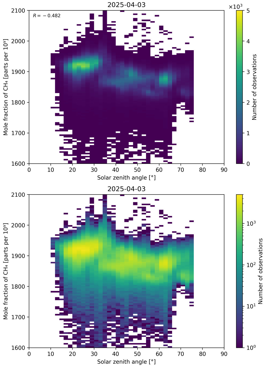
Figure 99: Scatter density plot of “Solar zenith angle” against “Mole fraction of CH 4 ” for 2025-04-03 to 2025-04-04.
