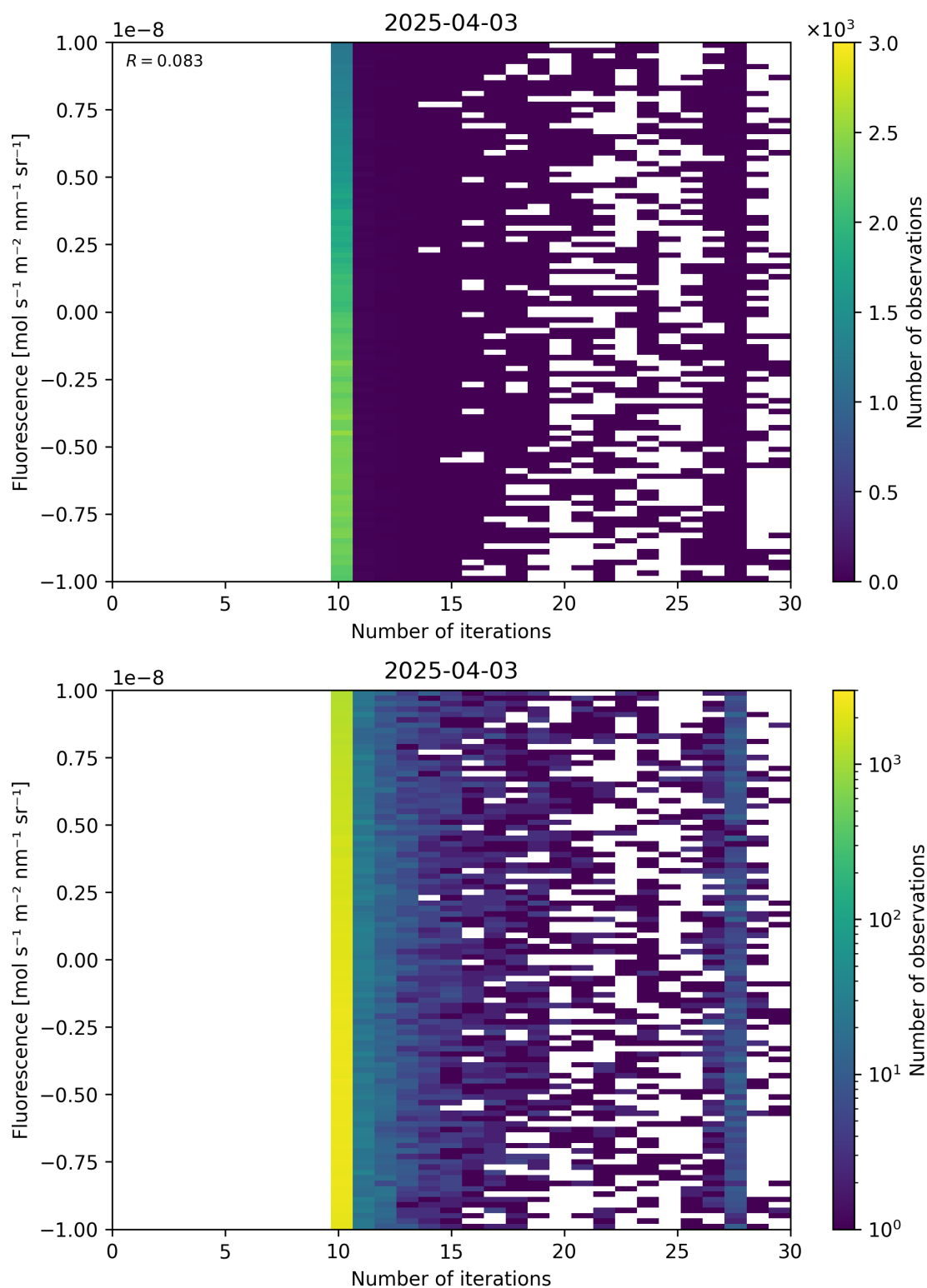
Figure 87: Scatter density plot of "Number of iterations" against "Fluorescence" for 2025-04-03 to 2025-04-04.
