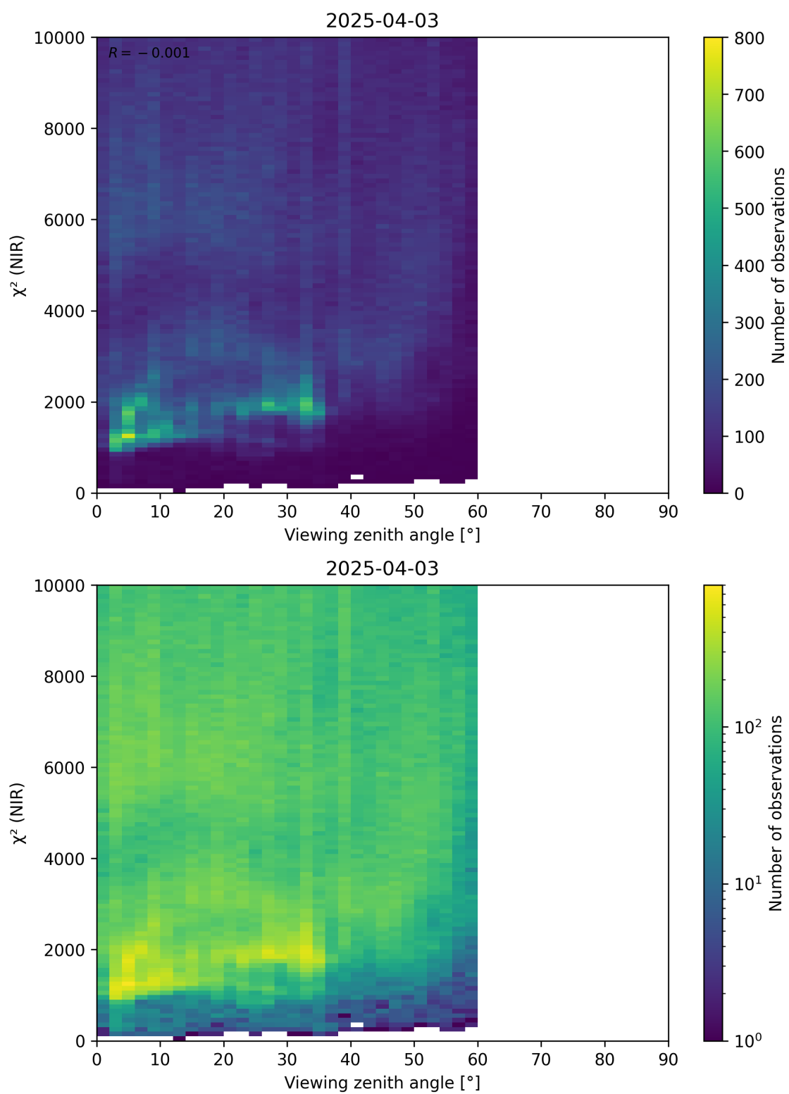
Figure 105: Scatter density plot of “Viewing zenith angle” against “ \chi^2 (NIR)” for 2025-04-03 to 2025-04-04.
