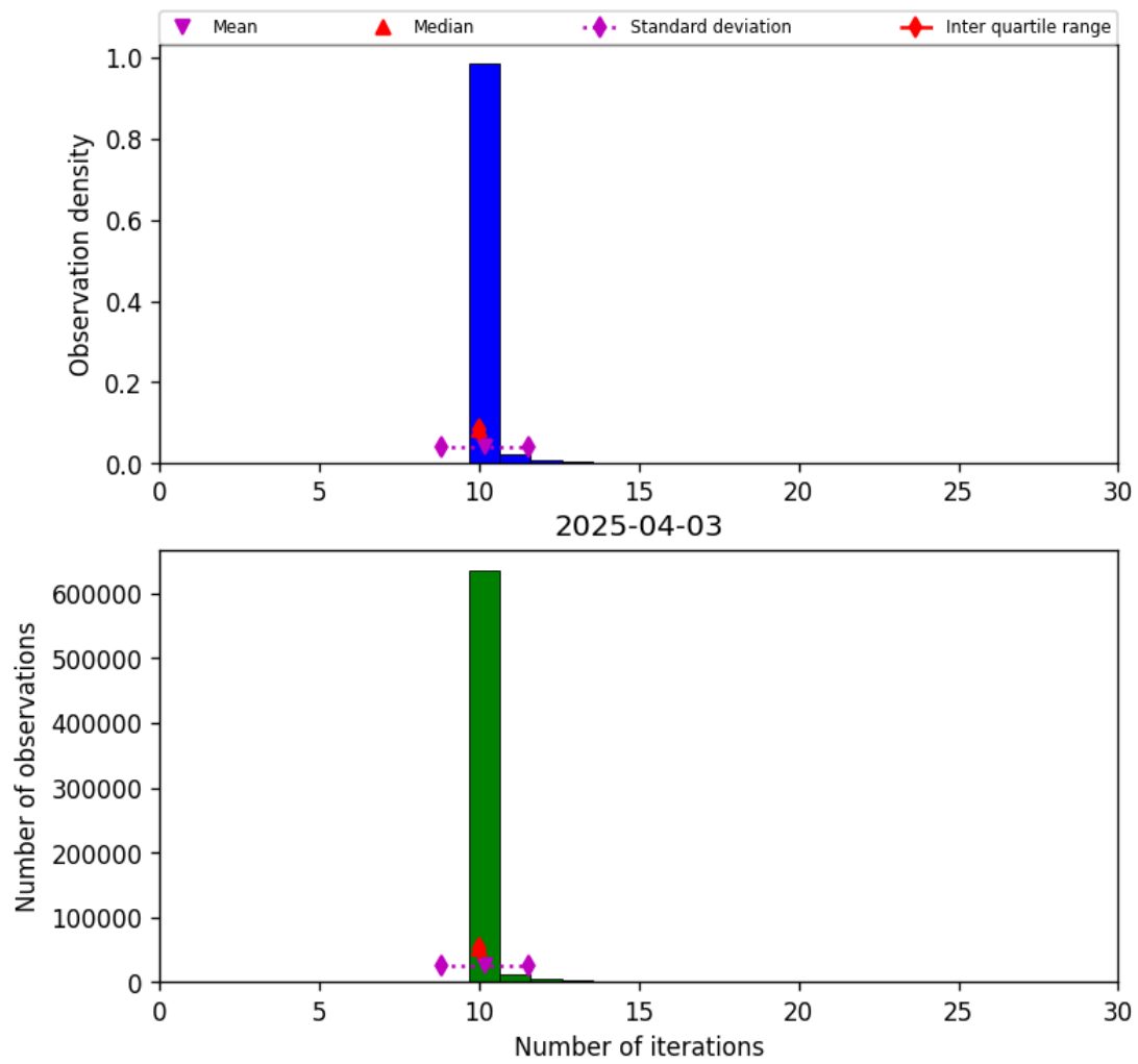
Figure 31: Histogram of “Number of iterations” for 2025-04-03 to 2025-04-04
