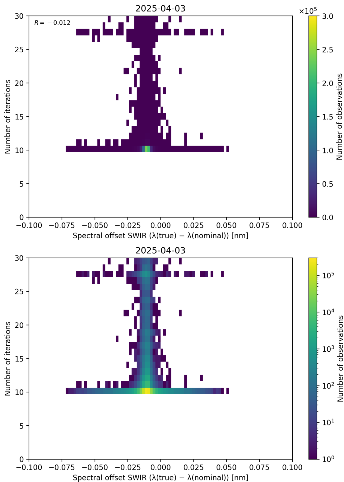
Figure 121: Scatter density plot of “Spectral offset SWIR ( \lambda_{\text{true}} - \lambda_{\text{nominal}} )” against “Number of iterations” for 2025-04-03 to 2025-04-04.
