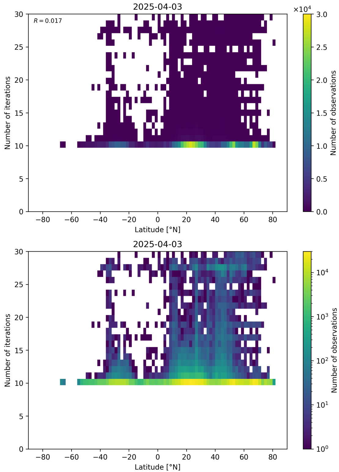
Figure 60: Scatter density plot of “Latitude” against “Number of iterations” for 2025-04-03 to 2025-04-04.
