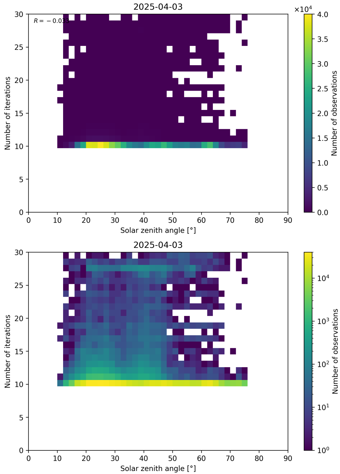
Figure 102: Scatter density plot of “Solar zenith angle” against “Number of iterations” for 2025-04-03 to 2025-04-04.
