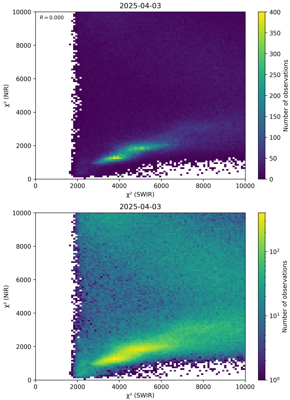
Figure 47: Scatter density plot of “ \chi^2 (SWIR)” against “ \chi^2 (NIR)” for 2025-04-03 to 2025-04-04.
