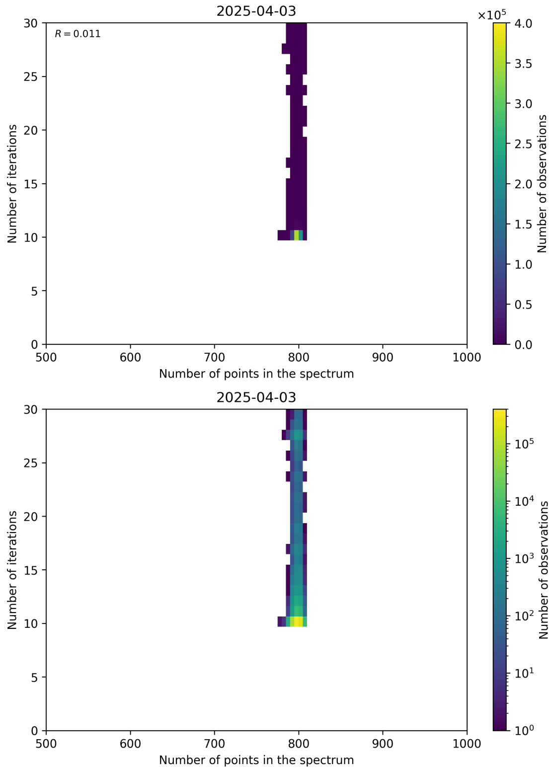
Figure 92: Scatter density plot of “Number of points in the spectrum” against “Number of iterations” for 2025-04-03 to 2025-04-04.
