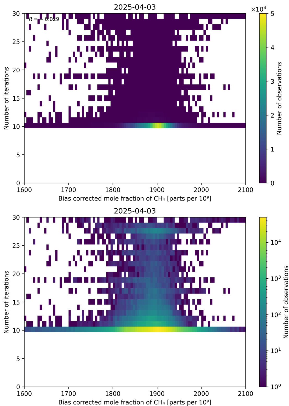
Figure 67: Scatter density plot of “Bias corrected mole fraction of CH 4 ” against “Number of iterations” for 2025-04-03 to 2025-04-04.
