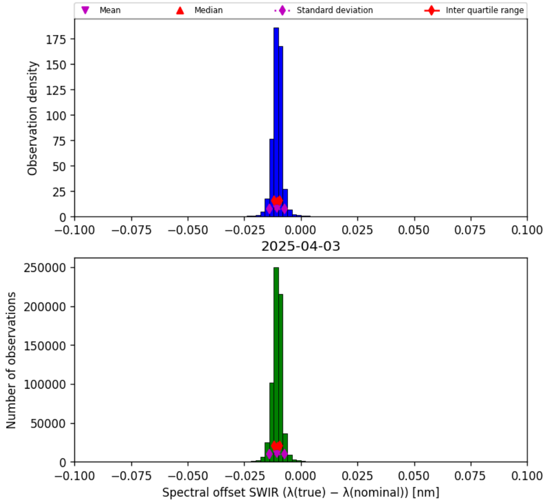
Figure 27: Histogram of “Spectral offset SWIR ( \lambda_{\text{true}} - \lambda_{\text{nominal}} )” for 2025-04-03 to 2025-04-04
