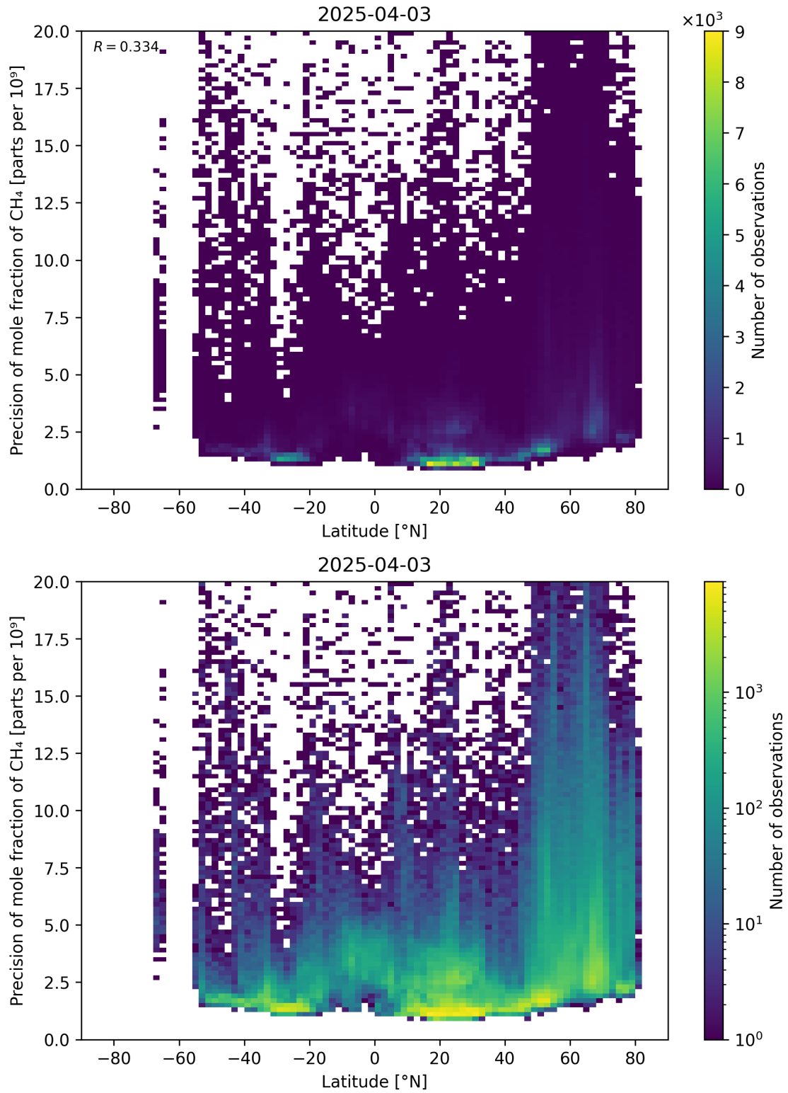
Figure 59: Scatter density plot of “Latitude” against “Precision of mole fraction of CH 4 ” for 2025-04-03 to 2025-04-04.
