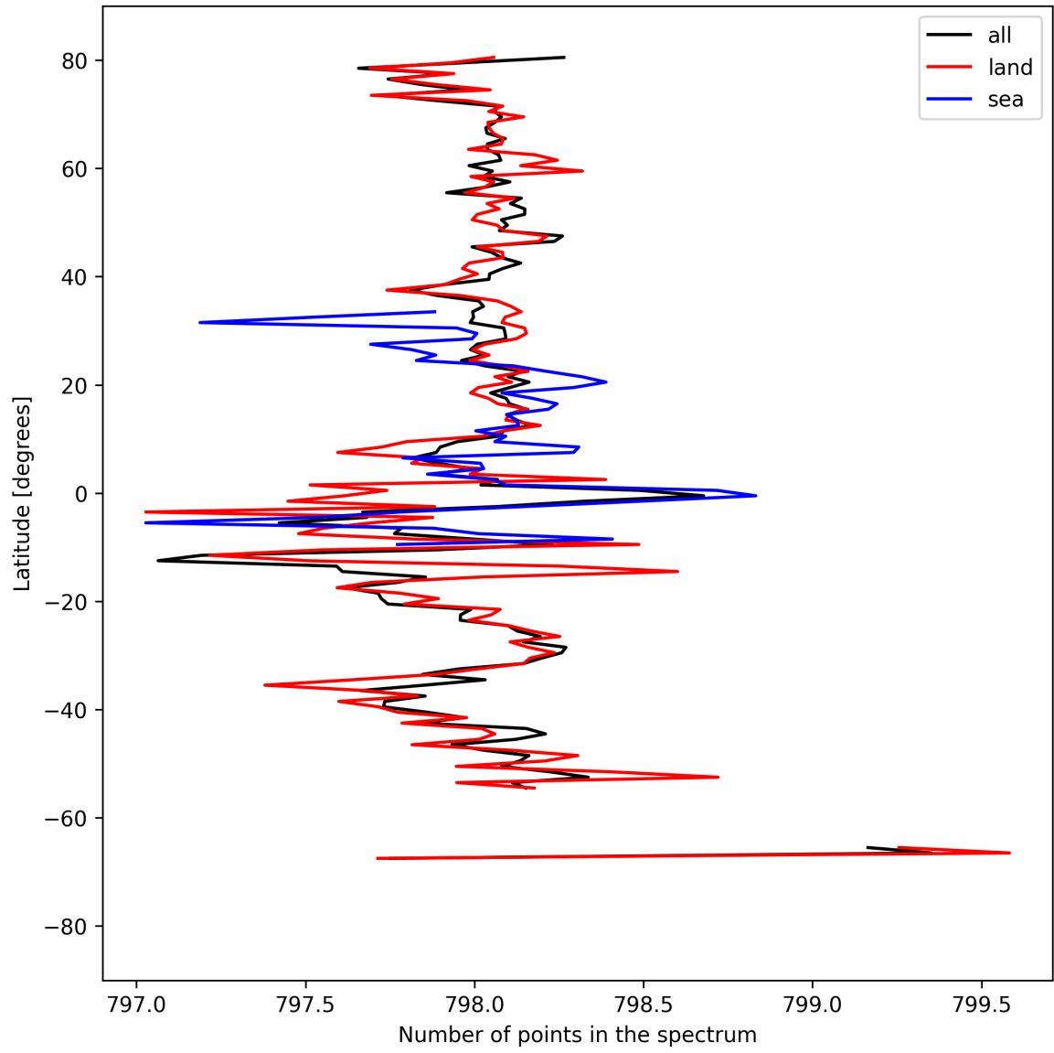
Figure 15: Zonal average of “Number of points in the spectrum” for 2025-04-03 to 2025-04-04.
