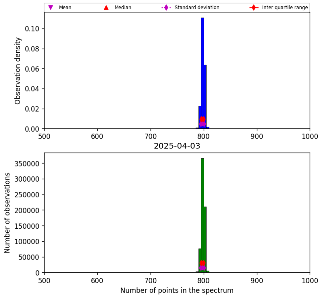
Figure 26: Histogram of “Number of points in the spectrum” for 2025-04-03 to 2025-04-04
