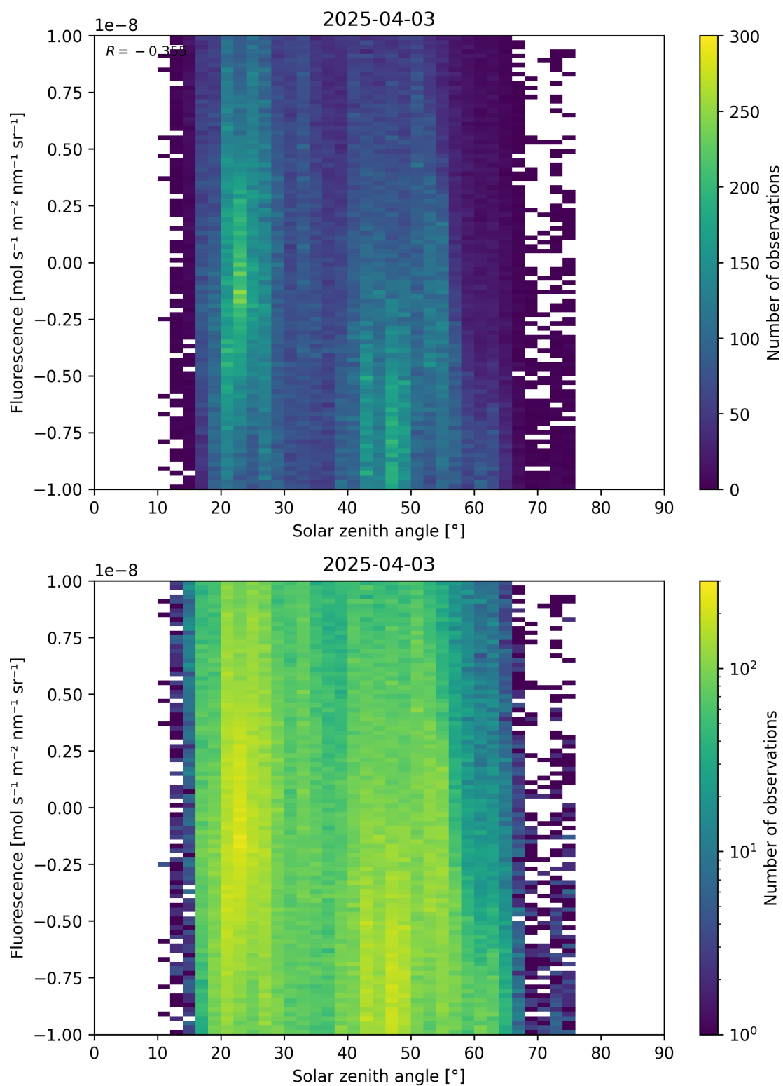
Figure 97: Scatter density plot of “Solar zenith angle” against “Fluorescence” for 2025-04-03 to 2025-04-04.
