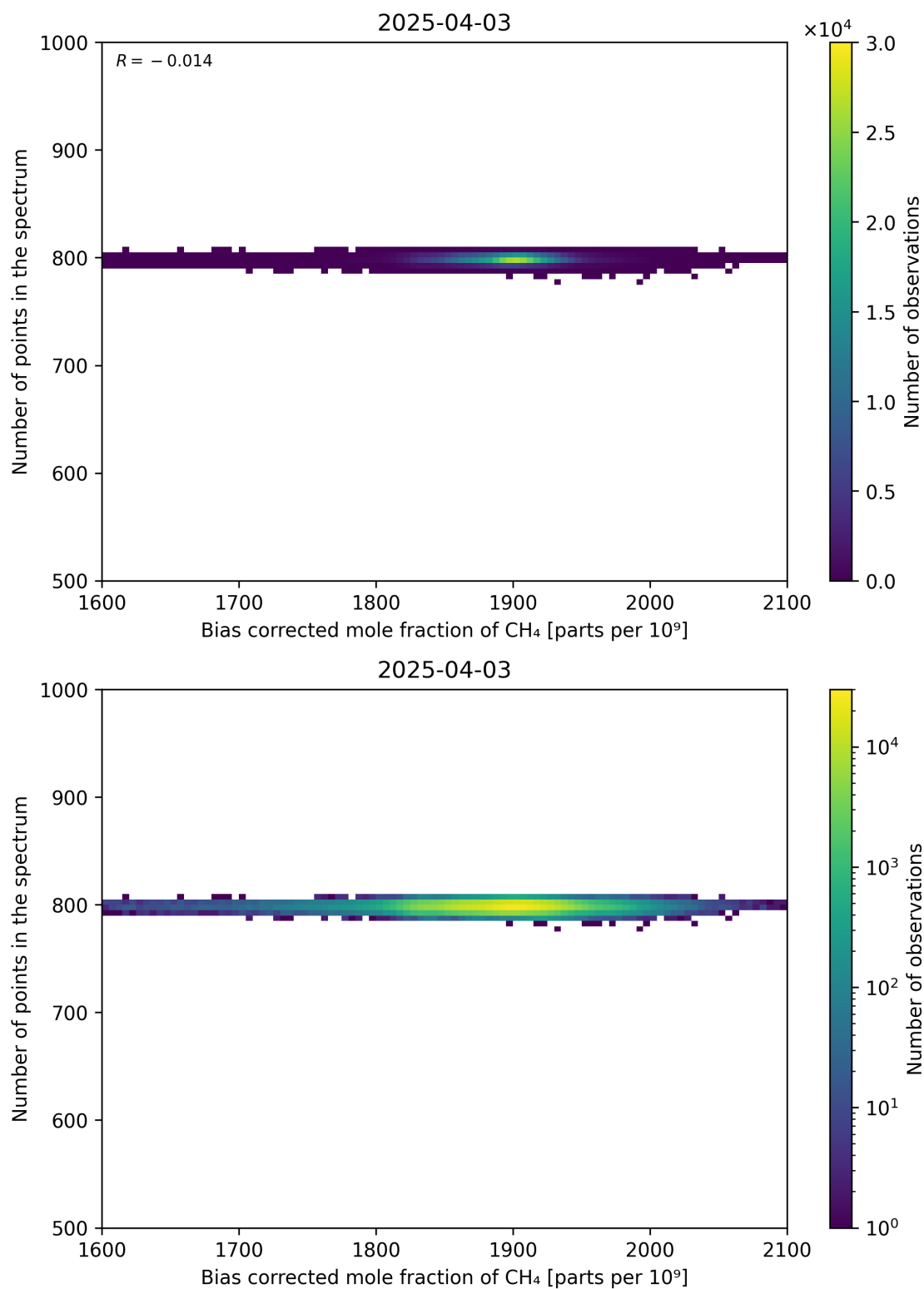
Figure 68: Scatter density plot of “Bias corrected mole fraction of CH 4 ” against “Number of points in the spectrum” for 2025-04-03 to 2025-04-04.
