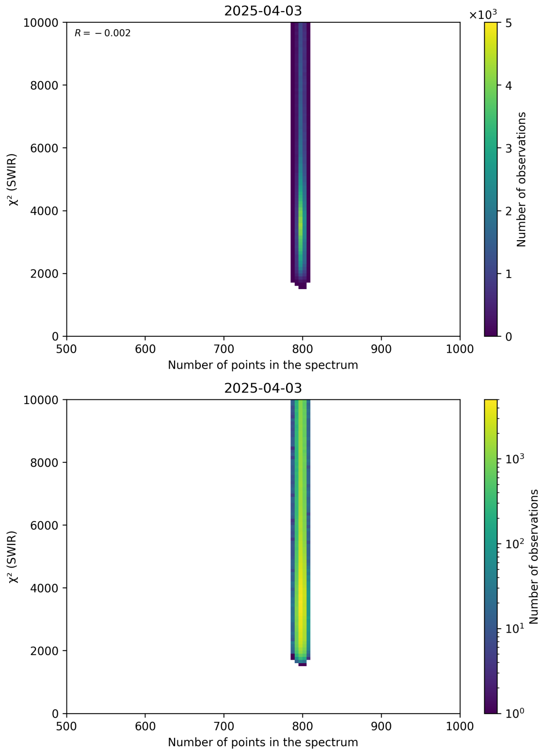
Figure 89: Scatter density plot of “Number of points in the spectrum” against “ \chi^2 (SWIR)” for 2025-04-03 to 2025-04-04.
