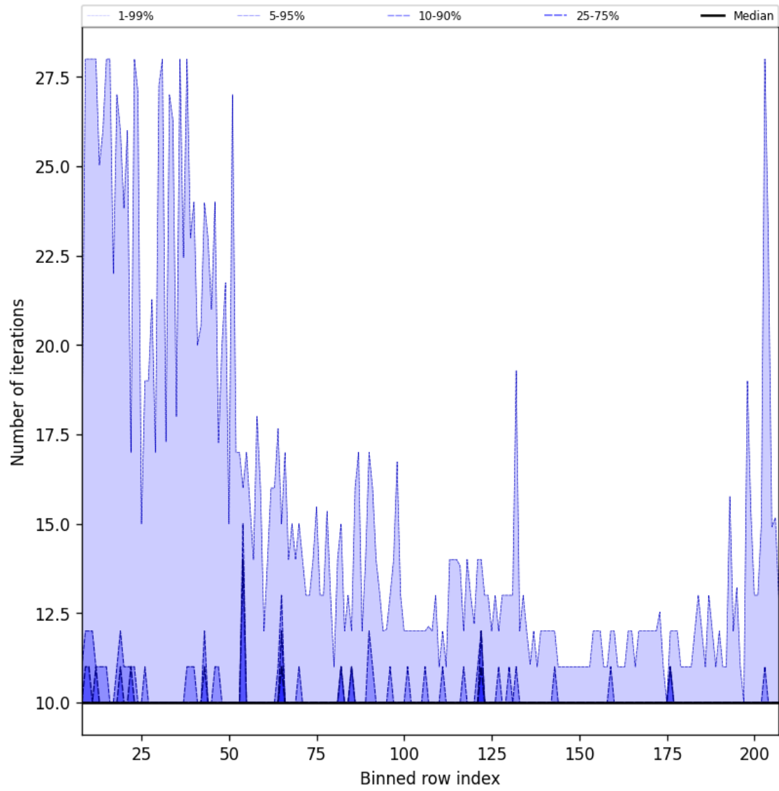
Figure 42: Along track statistics of “Number of iterations” for 2025-04-03 to 2025-04-04
