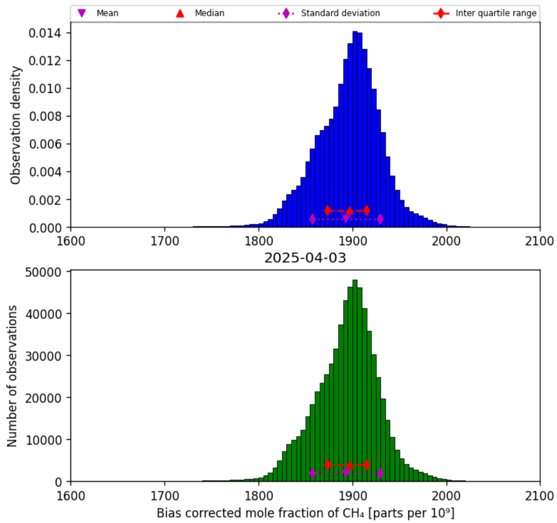
Figure 25: Histogram of “Bias corrected mole fraction of CH 4 ” for 2025-04-03 to 2025-04-04
