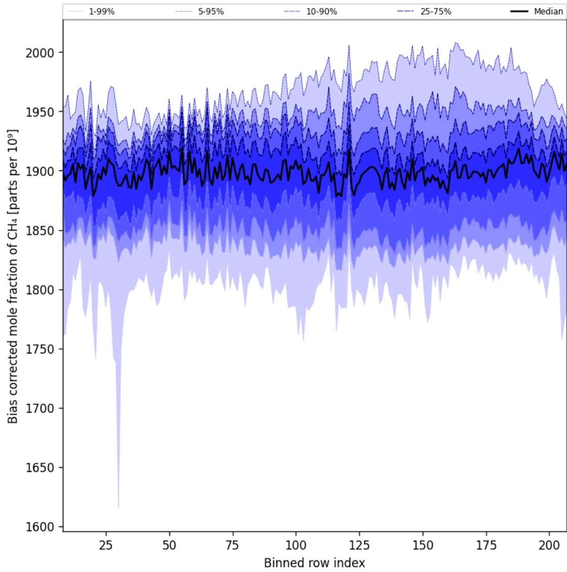
Figure 36: Along track statistics of “Bias corrected mole fraction of CH 4 ” for 2025-04-03 to 2025-04-04
