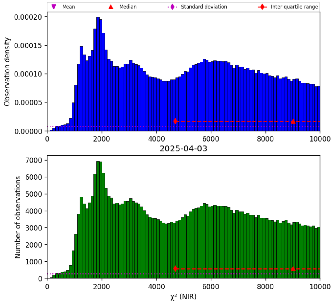
Figure 29: Histogram of “ \chi^2 (NIR)” for 2025-04-03 to 2025-04-04
