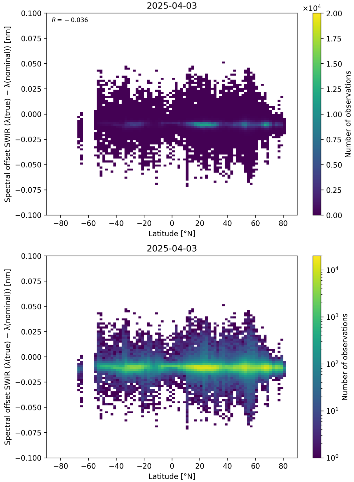
Figure 62: Scatter density plot of “Latitude” against “Spectral offset SWIR ( \lambda_{\text{true}} - \lambda_{\text{nominal}} )” for 2025-04-03 to 2025-04-04.
