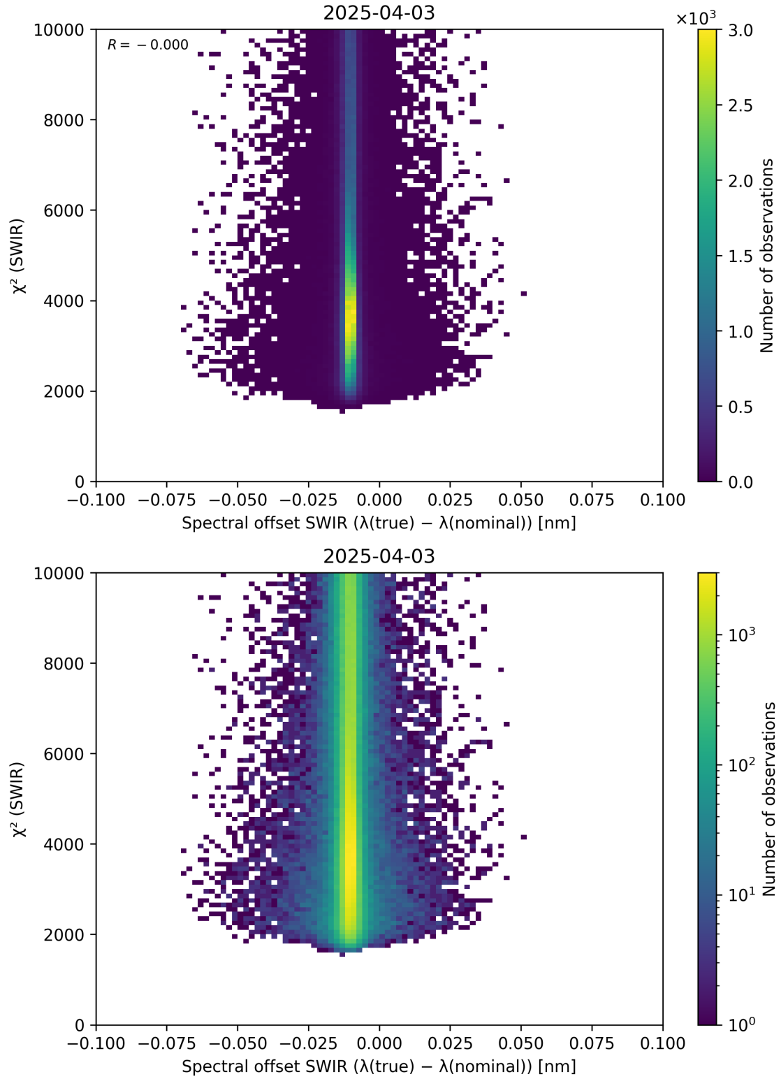
Figure 118: Scatter density plot of “Spectral offset SWIR ( \lambda_{\text{true}} - \lambda_{\text{nominal}} )” against “ \chi^2 (SWIR)” for 2025-04-03 to 2025-04-04.
