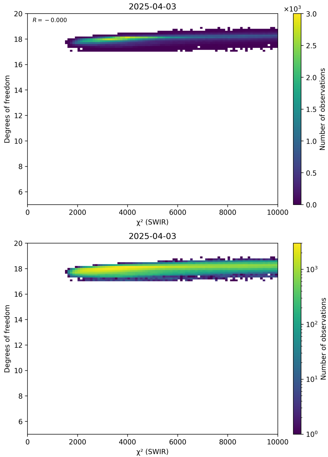
Figure 48: Scatter density plot of “ \chi^2 (SWIR)” against “Degrees of freedom” for 2025-04-03 to 2025-04-04.
