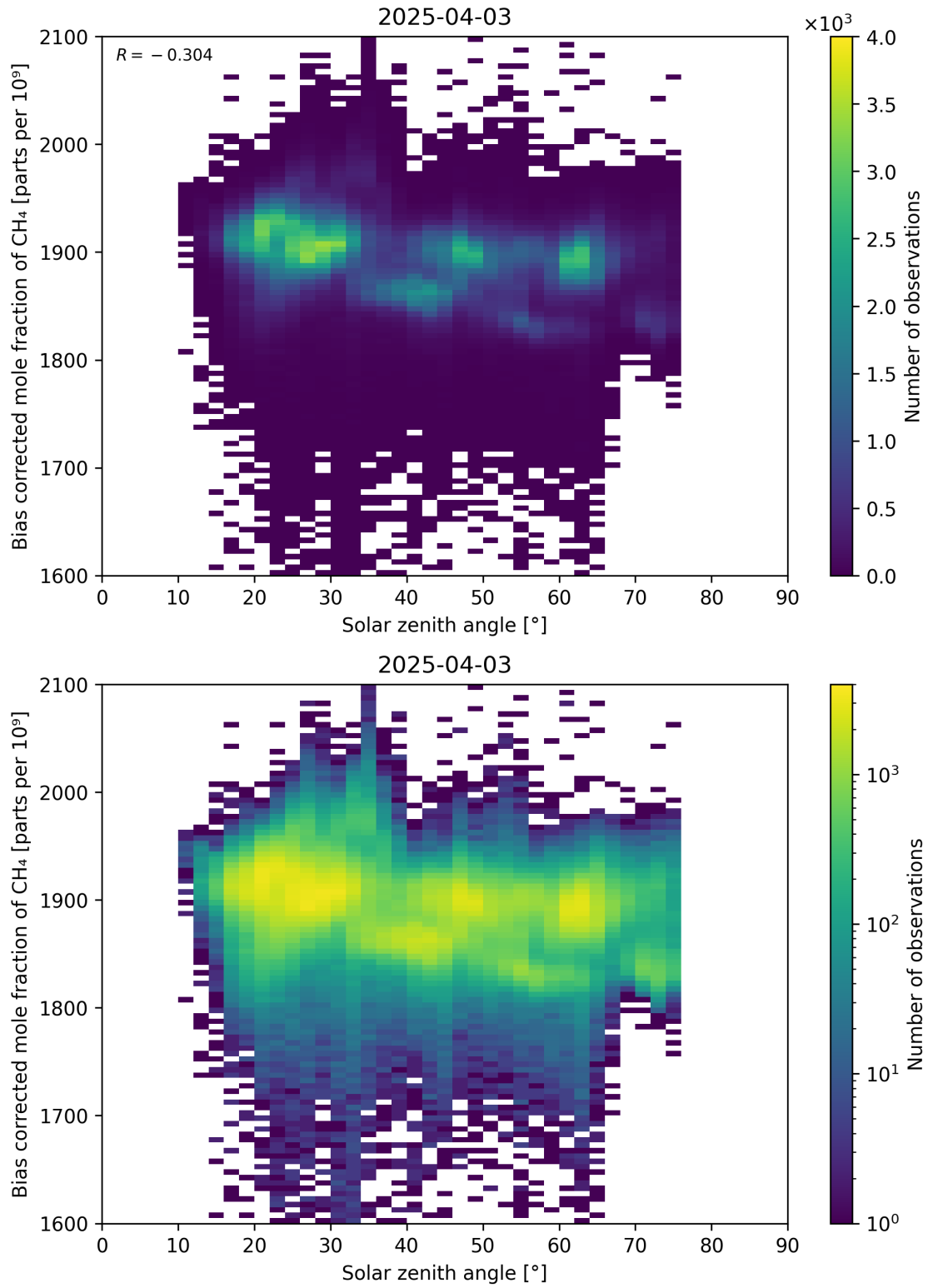
Figure 100: Scatter density plot of “Solar zenith angle” against “Bias corrected mole fraction of CH 4 ” for 2025-04-03 to 2025-04-04.
