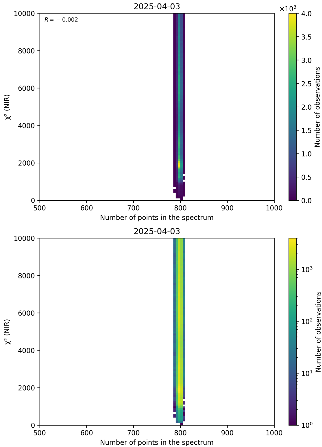
Figure 88: Scatter density plot of “Number of points in the spectrum” against “ \chi^2 (NIR)” for 2025-04-03 to 2025-04-04.
