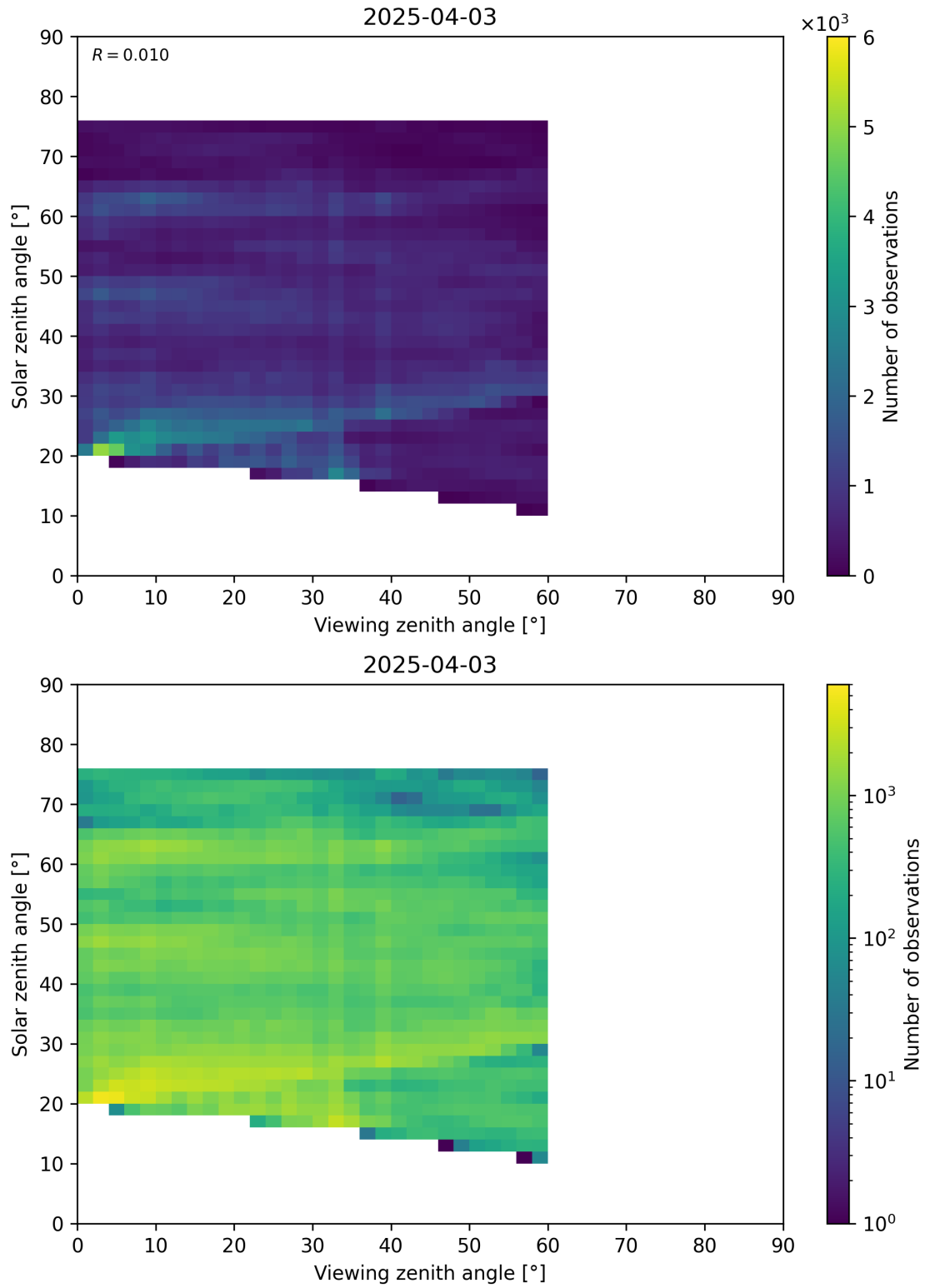
Figure 115: Scatter density plot of “Viewing zenith angle” against “Solar zenith angle” for 2025-04-03 to 2025-04-04.
