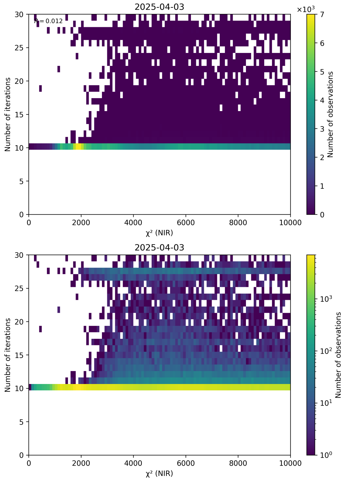
Figure 46: Scatter density plot of “ \chi^2 (NIR)” against “Number of iterations” for 2025-04-03 to 2025-04-04.
