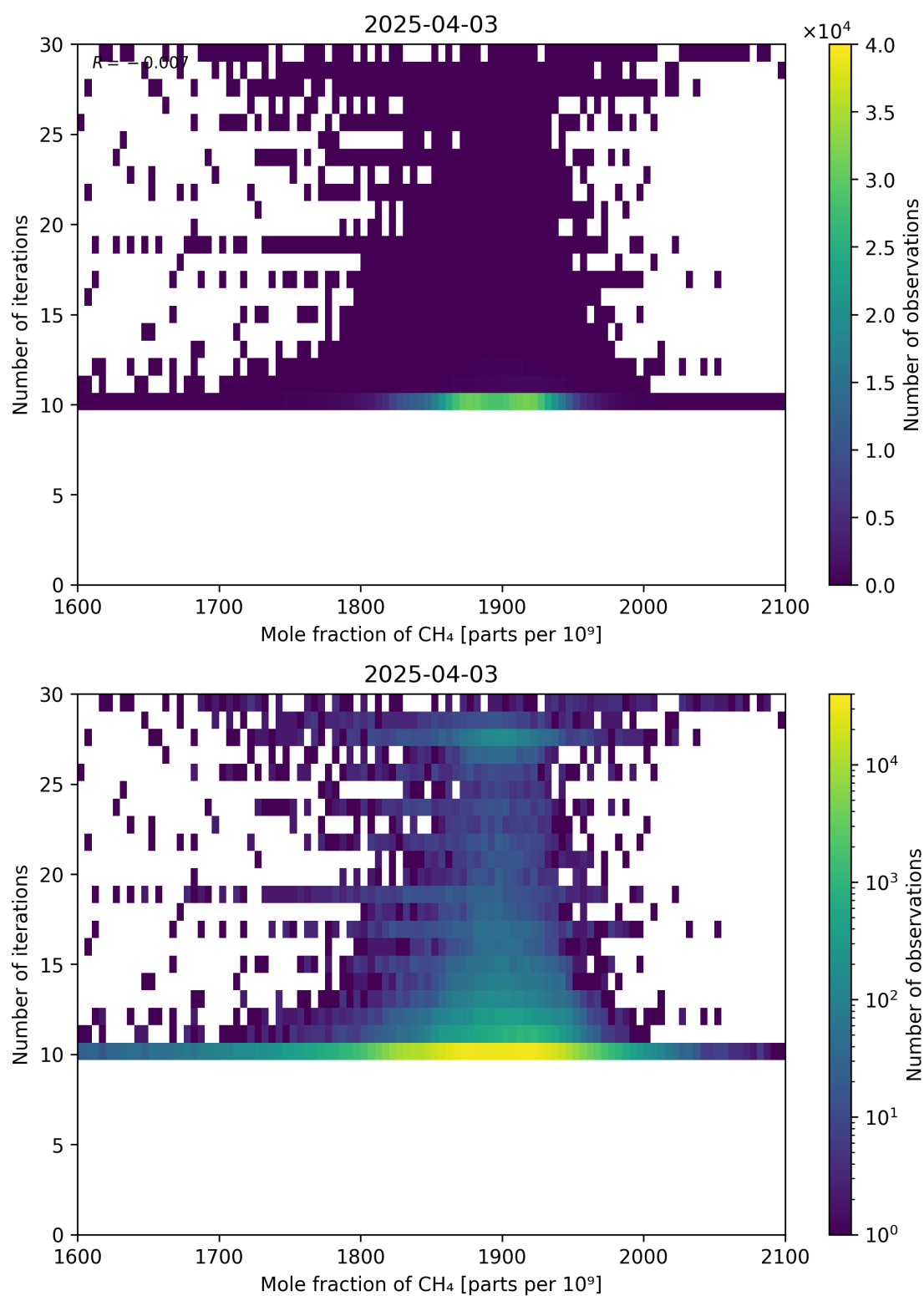
Figure 76: Scatter density plot of “Mole fraction of CH 4 ” against “Number of iterations” for 2025-04-03 to 2025-04-04.
