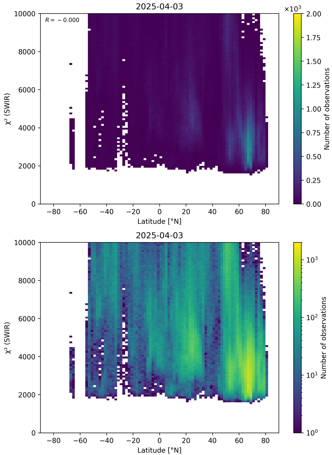
Figure 54: Scatter density plot of “Latitude” against “ \chi^2 (SWIR)” for 2025-04-03 to 2025-04-04.
