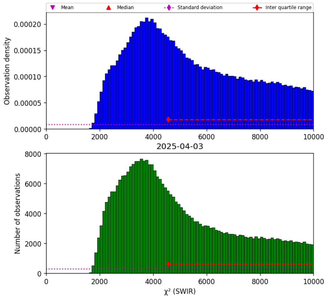
Figure 28: Histogram of “ \chi^2 (SWIR)” for 2025-04-03 to 2025-04-04
