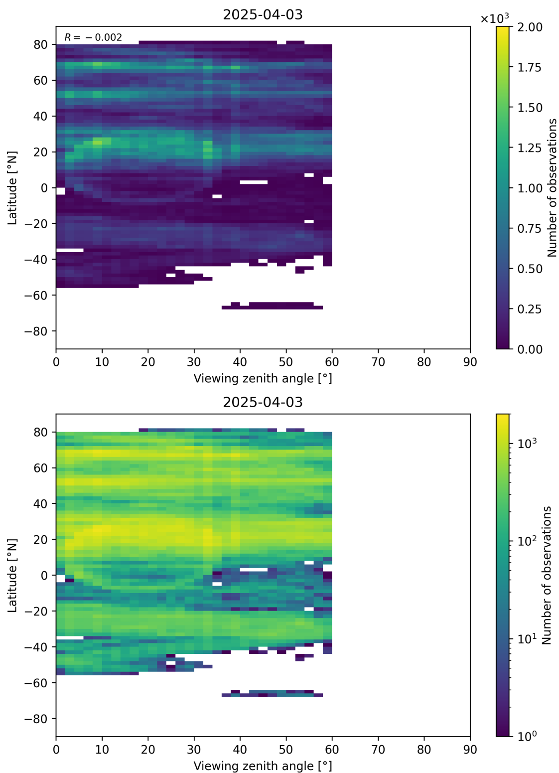
Figure 109: Scatter density plot of “Viewing zenith angle” against “Latitude” for 2025-04-03 to 2025-04-04.
