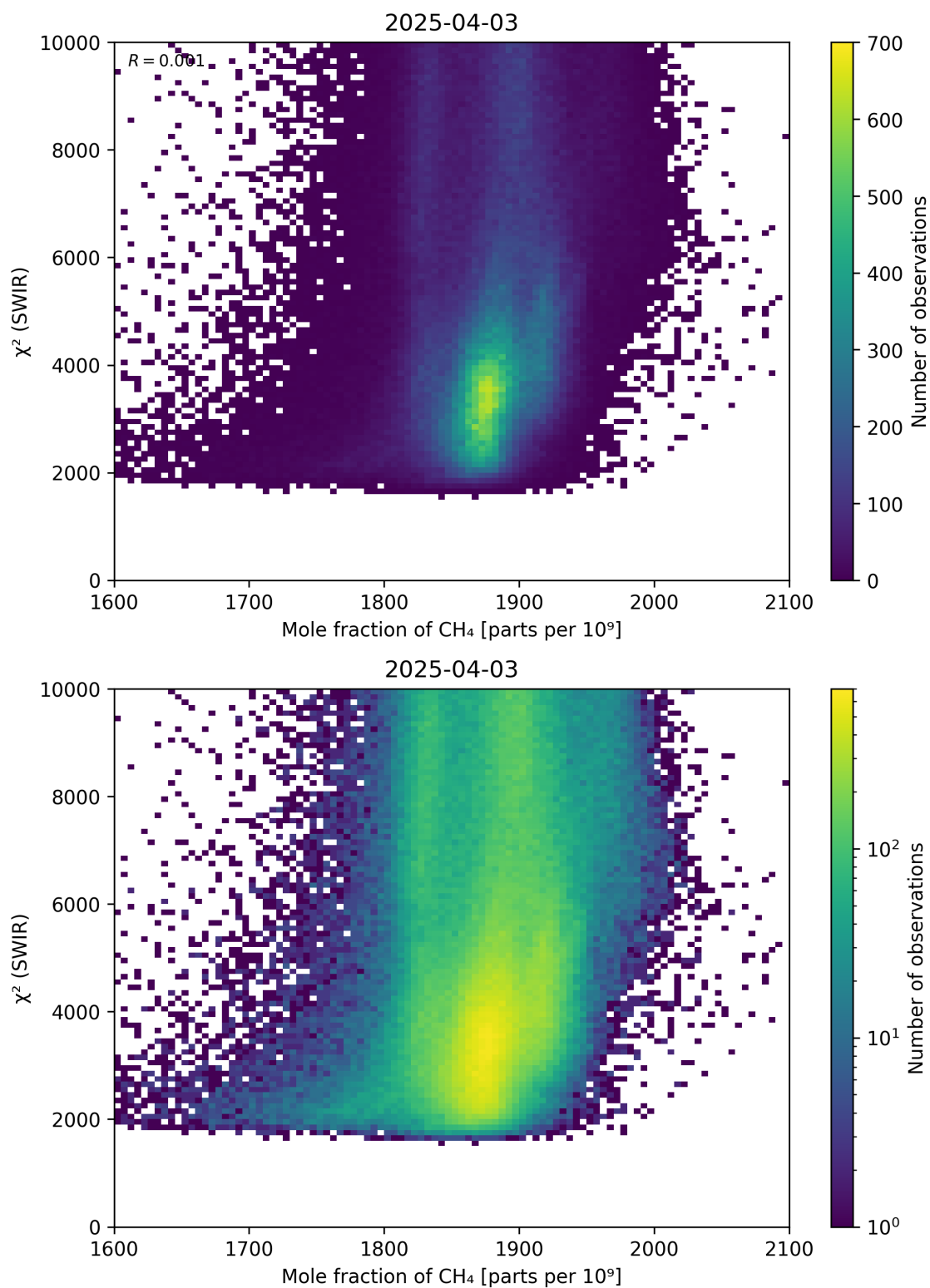
Figure 71: Scatter density plot of “Mole fraction of \text{CH}_4 ” against “ \chi^2 (SWIR)” for 2025-04-03 to 2025-04-04.
