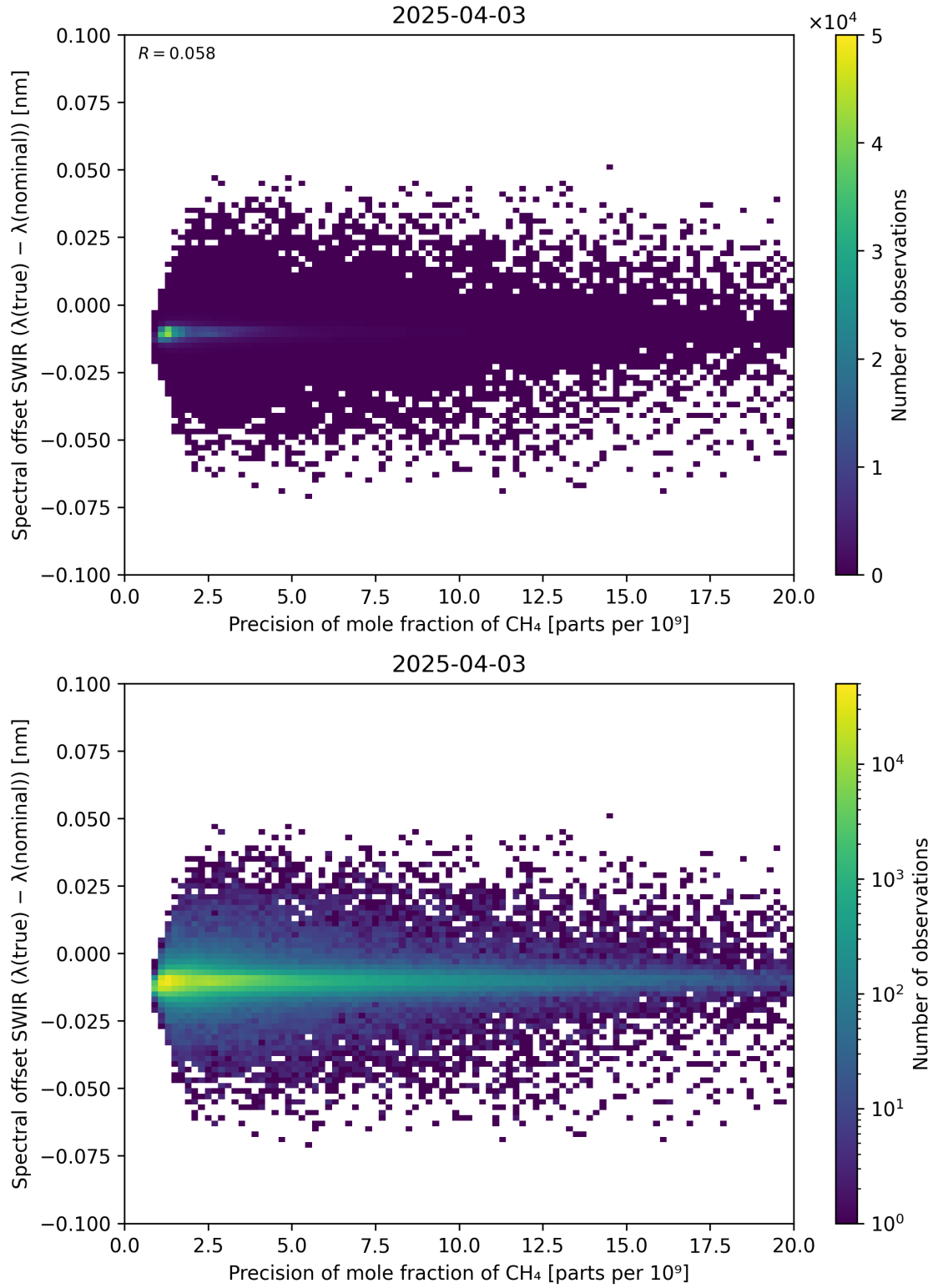
Figure 85: Scatter density plot of “Precision of mole fraction of CH 4 ” against “Spectral offset SWIR ( \lambda_{\text{true}} - \lambda_{\text{nominal}} )” for 2025-04-03 to 2025-04-04.
