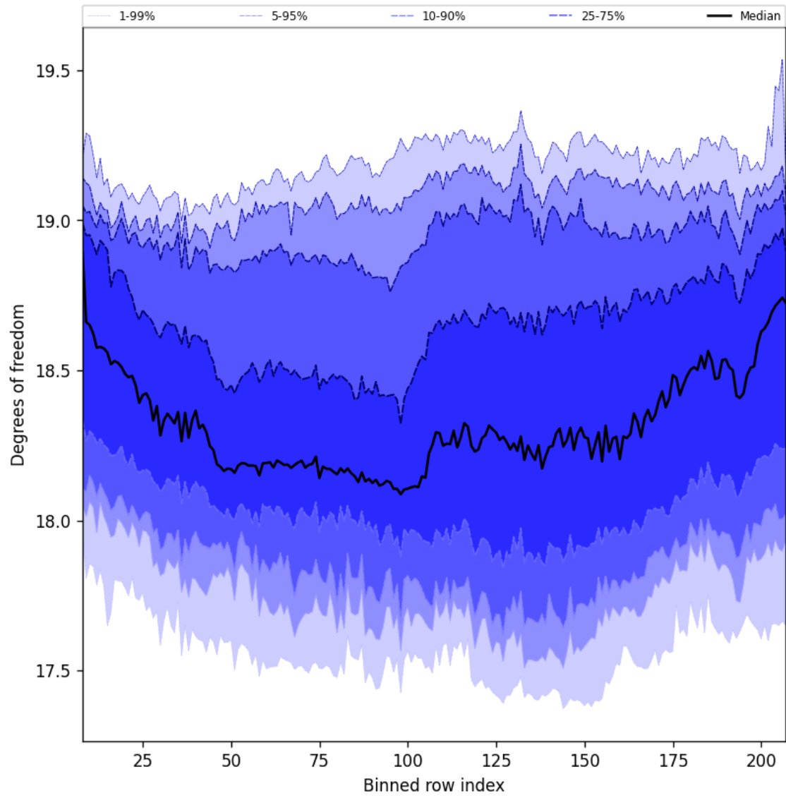
Figure 41: Along track statistics of “Degrees of freedom” for 2025-04-03 to 2025-04-04
