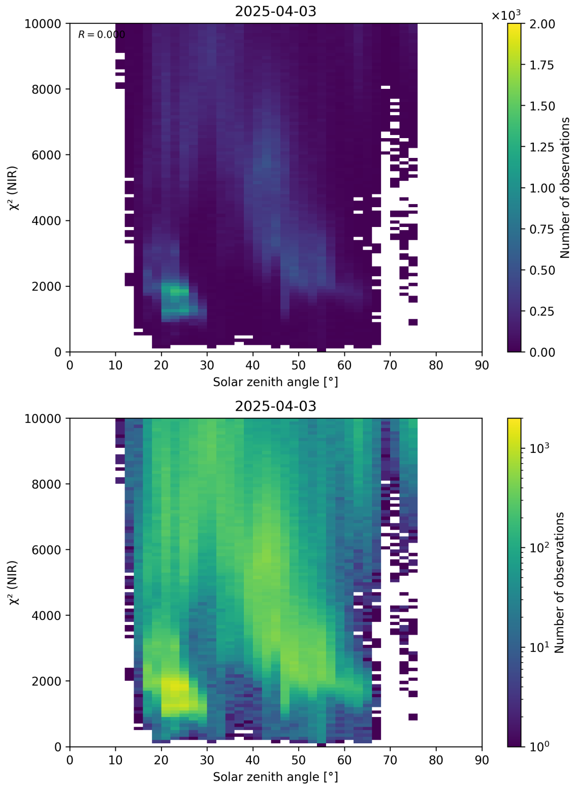
Figure 94: Scatter density plot of “Solar zenith angle” against “ \chi^2 (NIR)” for 2025-04-03 to 2025-04-04.
