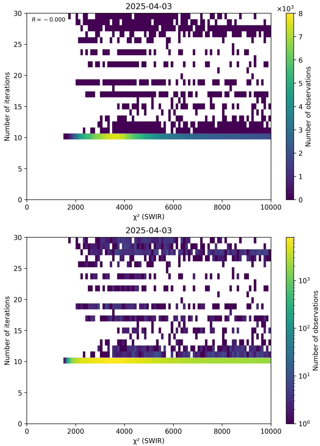
Figure 50: Scatter density plot of “ \chi^2 (SWIR)” against “Number of iterations” for 2025-04-03 to 2025-04-04.
