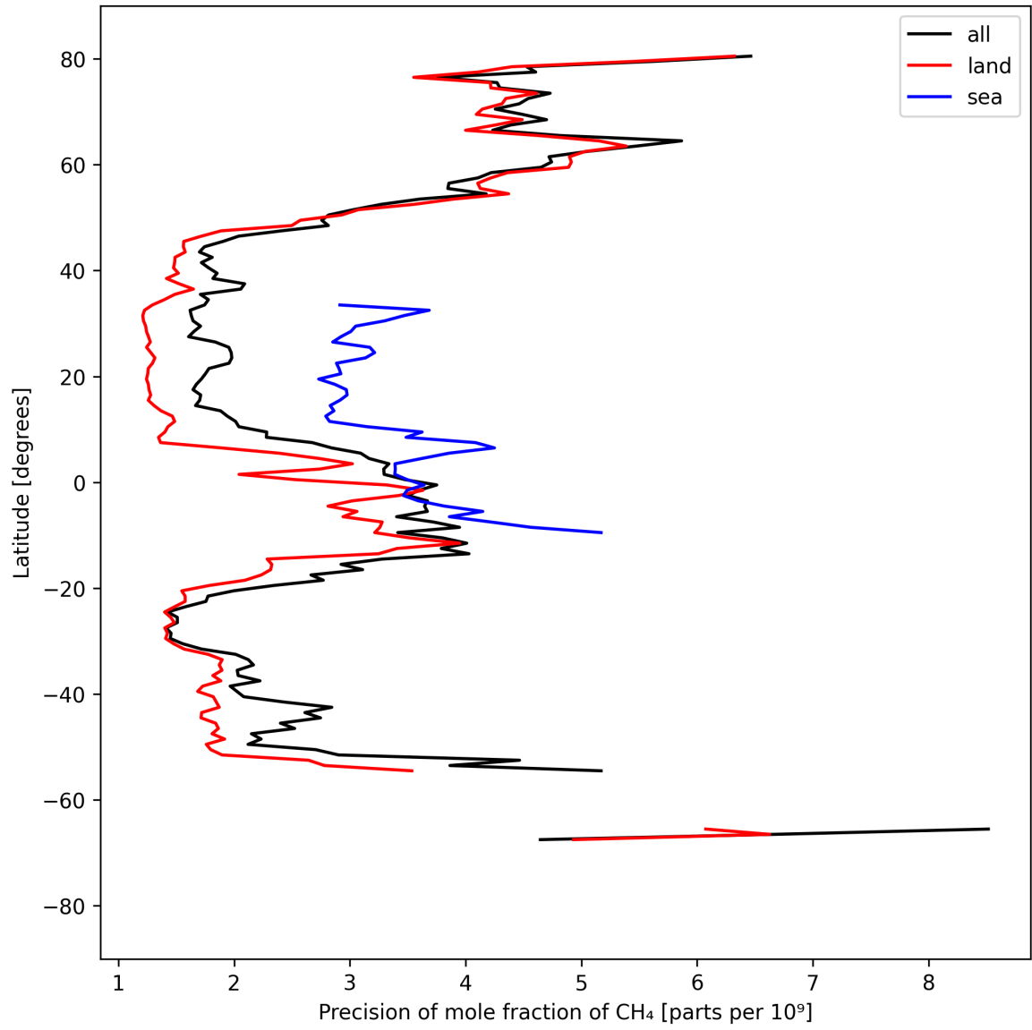
Figure 13: Zonal average of “Precision of mole fraction of CH 4 ” for 2025-04-03 to 2025-04-04.
