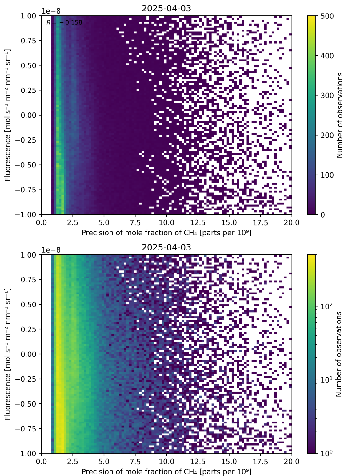
Figure 81: Scatter density plot of “Precision of mole fraction of CH 4 ” against “Fluorescence” for 2025-04-03 to 2025-04-04.
