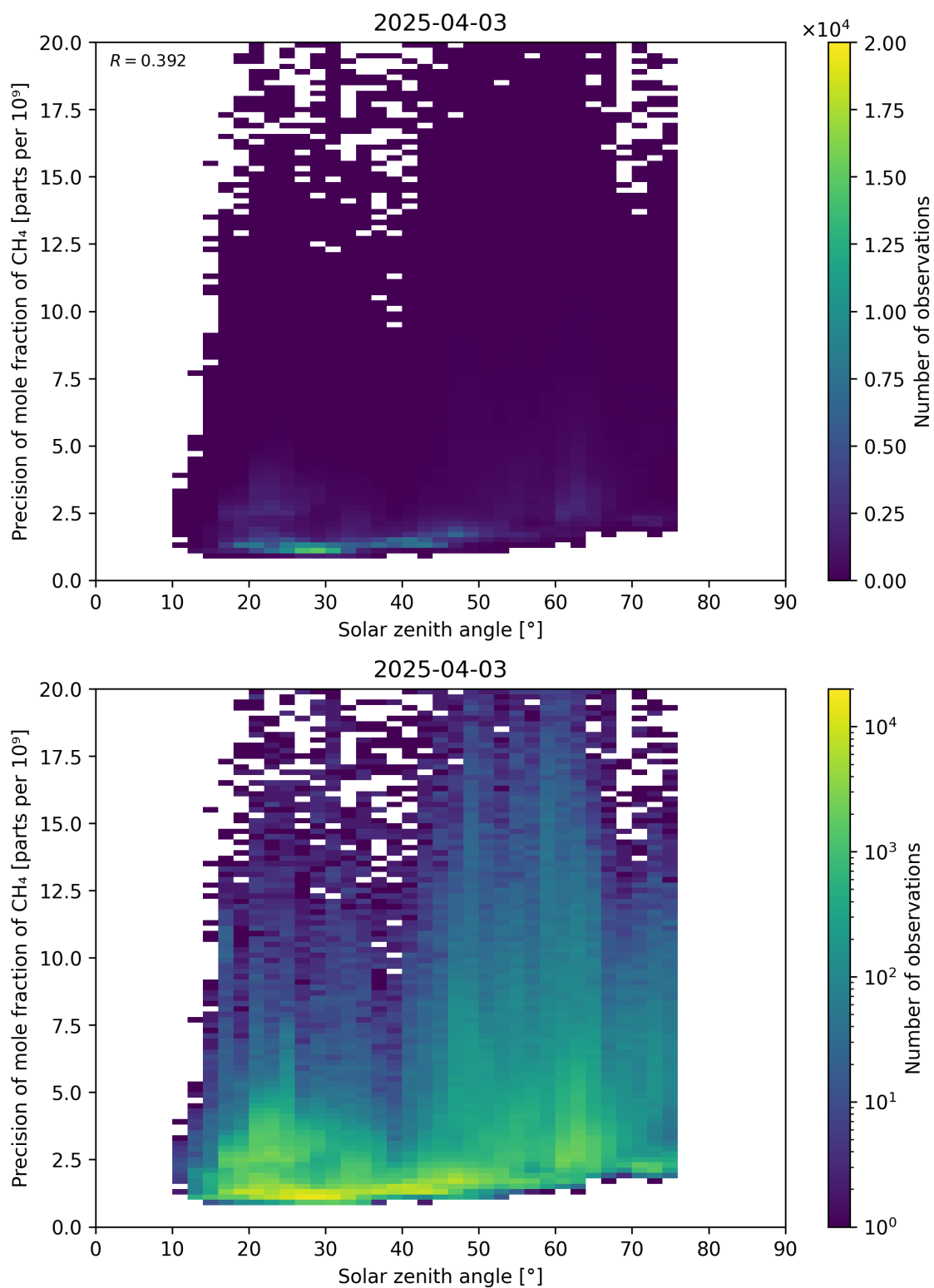
Figure 101: Scatter density plot of “Solar zenith angle” against “Precision of mole fraction of CH 4 ” for 2025-04-03 to 2025-04-04.
