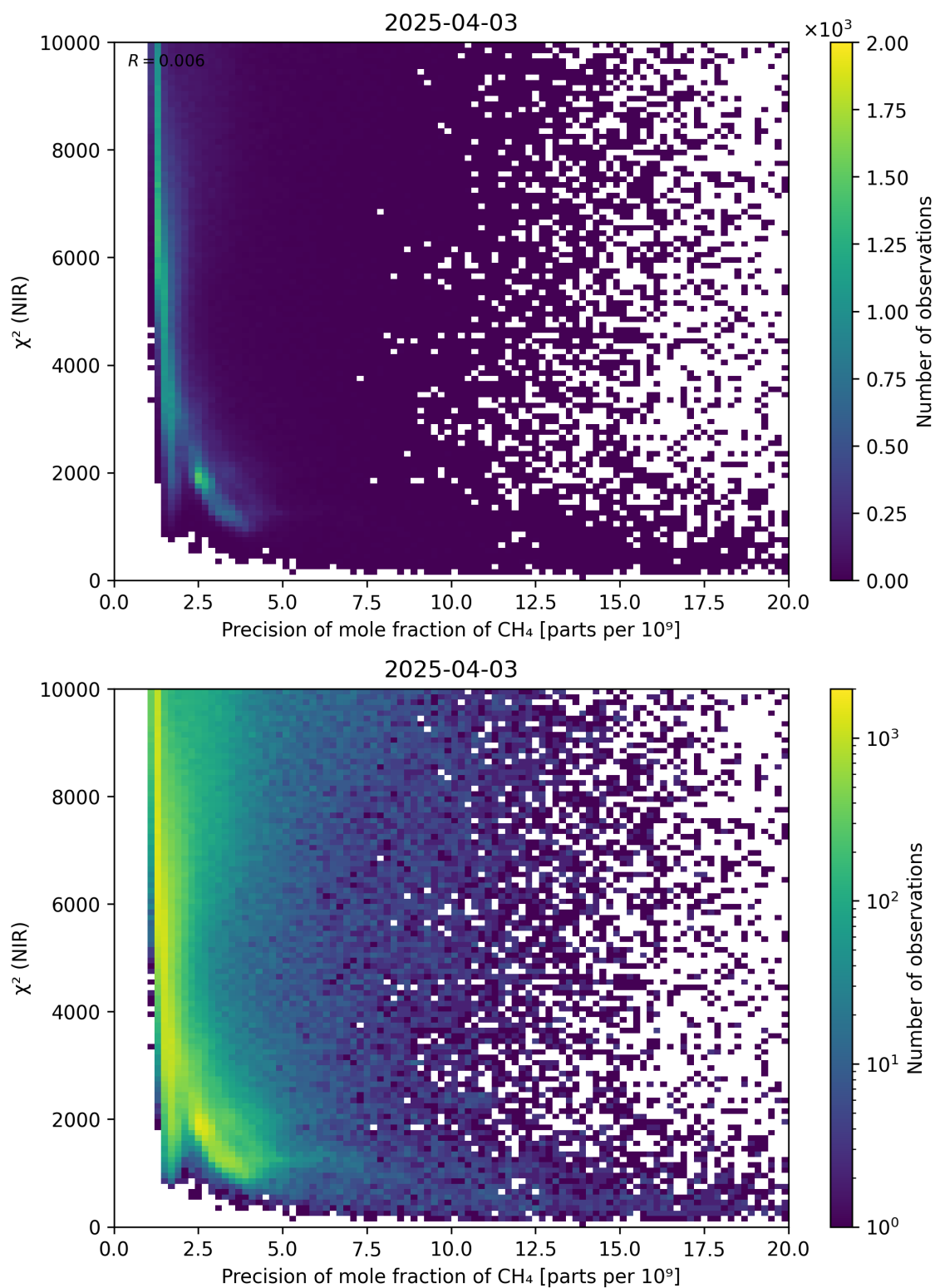
Figure 78: Scatter density plot of “Precision of mole fraction of \text{CH}_4 ” against “ \chi^2 (NIR)” for 2025-04-03 to 2025-04-04.
