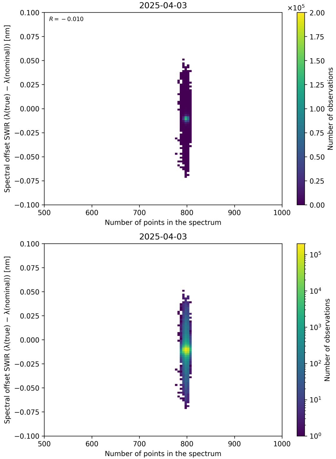
Figure 93: Scatter density plot of “Number of points in the spectrum” against “Spectral offset SWIR ( \lambda_{\text{true}} - \lambda_{\text{nominal}} )” for 2025-04-03 to 2025-04-04.
