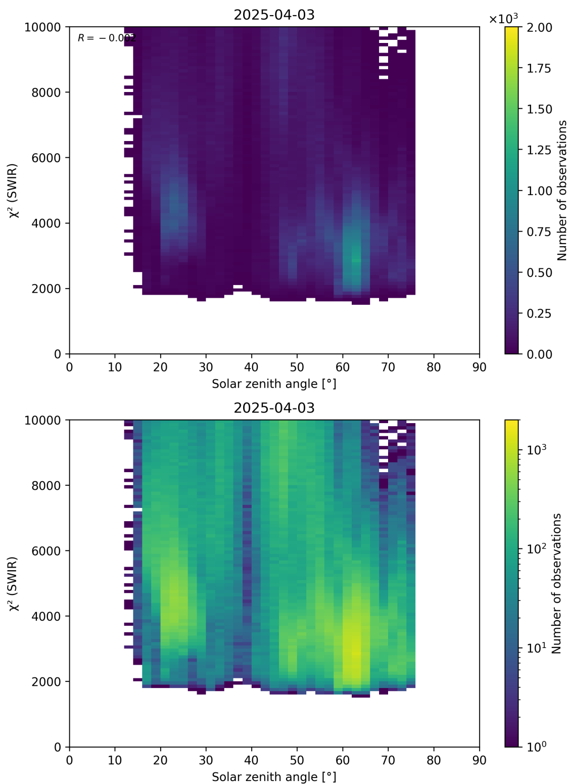
Figure 95: Scatter density plot of “Solar zenith angle” against “ \chi^2 (SWIR)” for 2025-04-03 to 2025-04-04.
