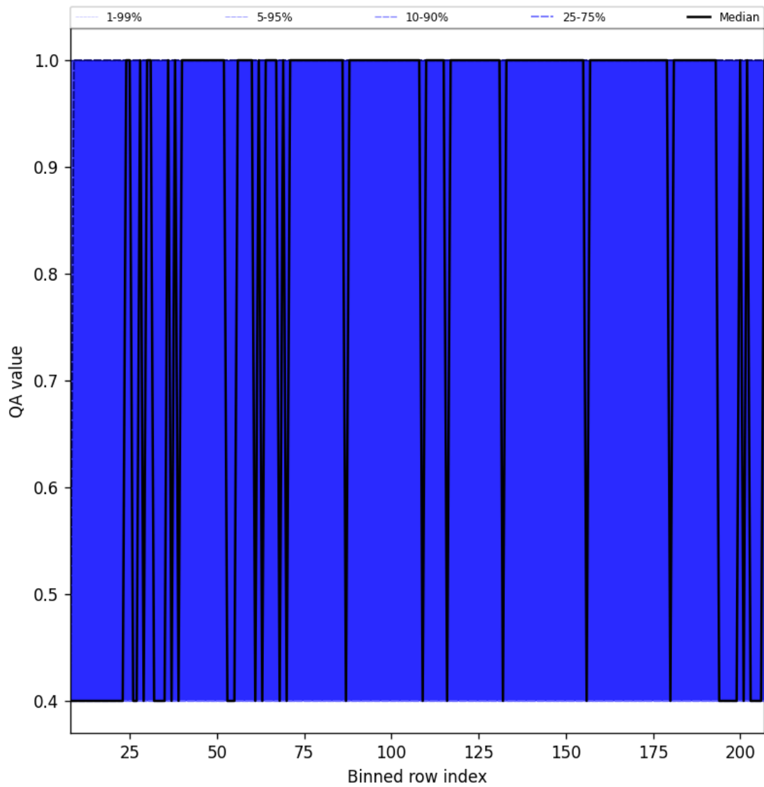
Figure 33: Along track statistics of “QA value” for 2025-04-03 to 2025-04-04
