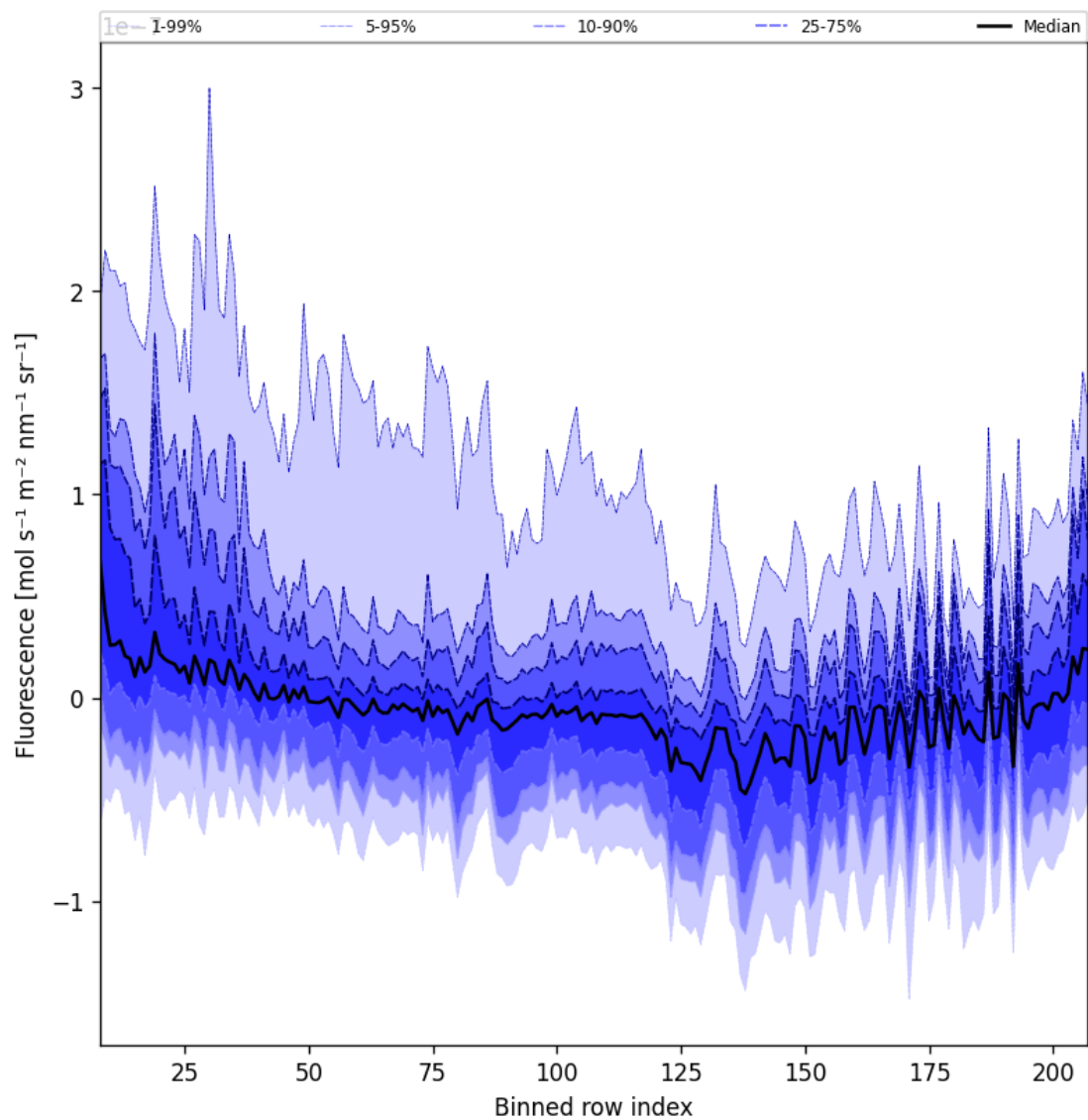
Figure 43: Along track statistics of “Fluorescence” for 2025-04-03 to 2025-04-04
