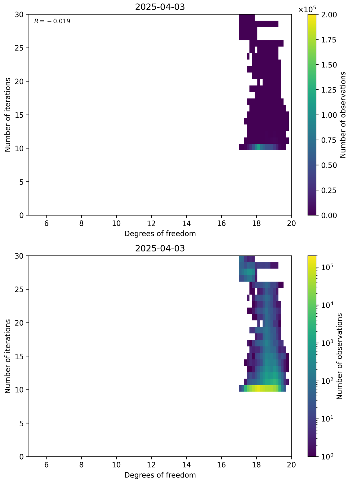
Figure 52: Scatter density plot of “Degrees of freedom” against “Number of iterations” for 2025-04-03 to 2025-04-04.
