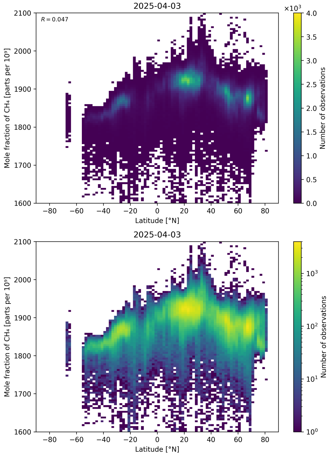
Figure 57: Scatter density plot of “Latitude” against “Mole fraction of CH 4 ” for 2025-04-03 to 2025-04-04.
