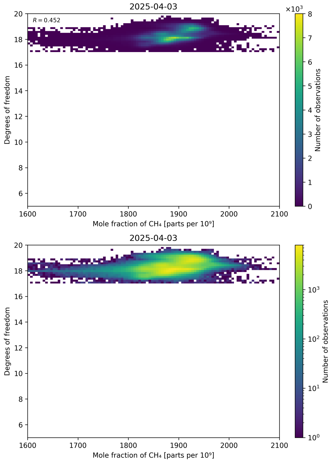
Figure 72: Scatter density plot of “Mole fraction of CH 4 ” against “Degrees of freedom” for 2025-04-03 to 2025-04-04.
