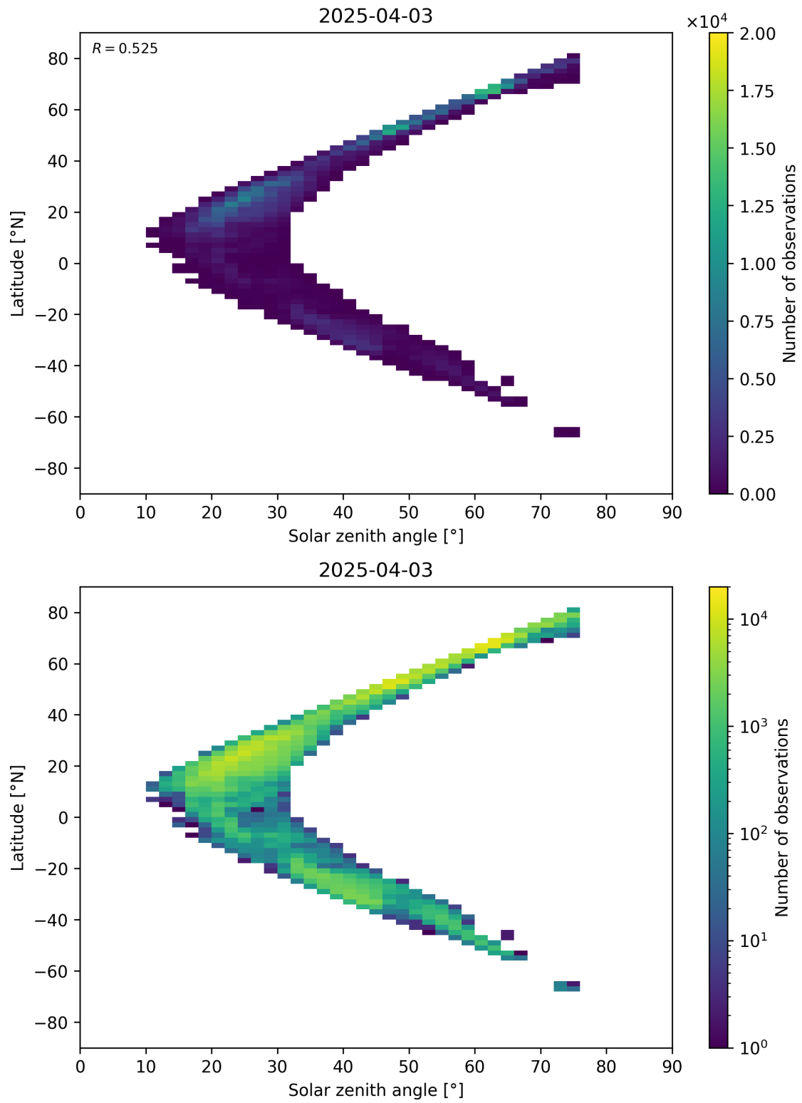
Figure 98: Scatter density plot of “Solar zenith angle” against “Latitude” for 2025-04-03 to 2025-04-04.
