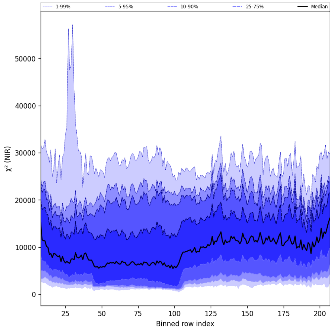
Figure 40: Along track statistics of “ \chi^2 (NIR)” for 2025-04-03 to 2025-04-04
