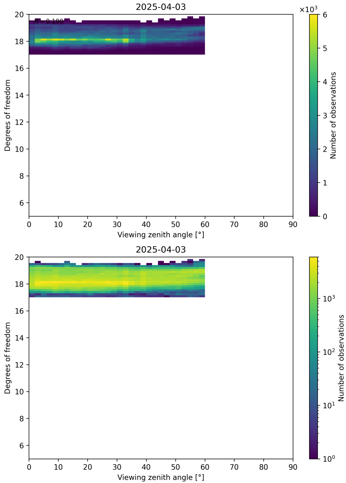
Figure 107: Scatter density plot of “Viewing zenith angle” against “Degrees of freedom” for 2025-04-03 to 2025-04-04.
