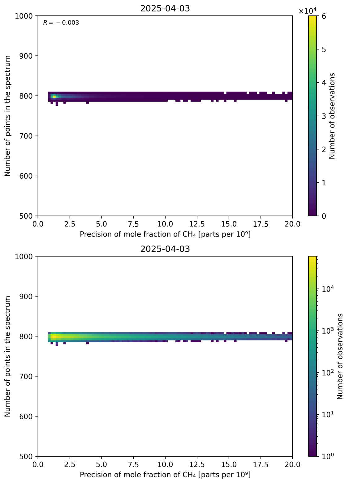
Figure 84: Scatter density plot of “Precision of mole fraction of CH 4 ” against “Number of points in the spectrum” for 2025-04-03 to 2025-04-04.
