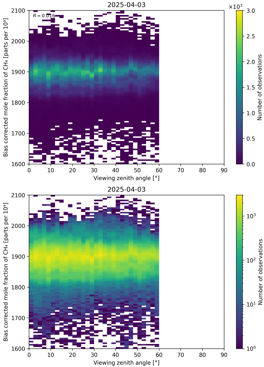
Figure 111: Scatter density plot of “Viewing zenith angle” against “Bias corrected mole fraction of CH 4 ” for 2025-04-03 to 2025-04-04.
