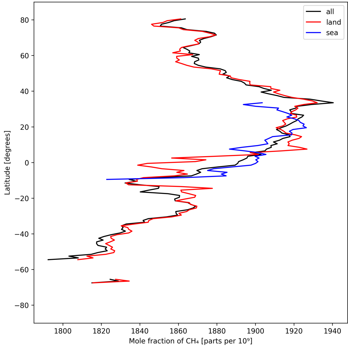
Figure 12: Zonal average of “Mole fraction of \text{CH}_4 ” for 2025-04-03 to 2025-04-04.
