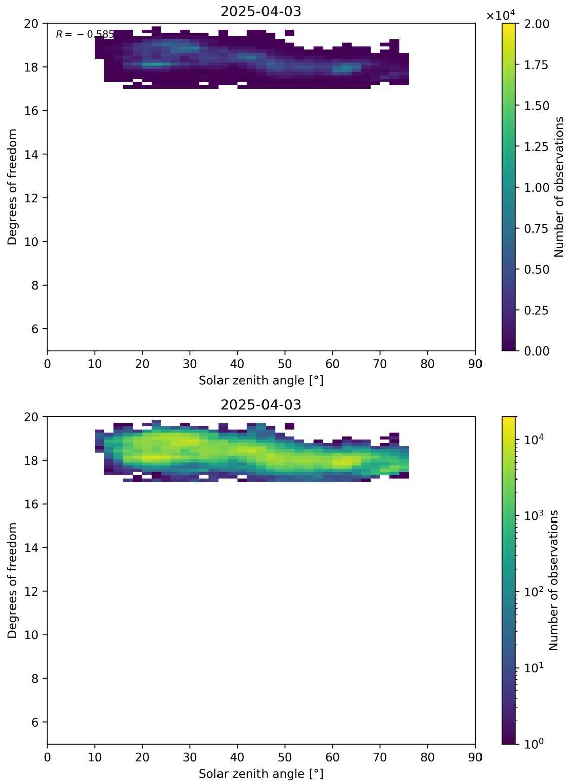
Figure 96: Scatter density plot of “Solar zenith angle” against “Degrees of freedom” for 2025-04-03 to 2025-04-04.
