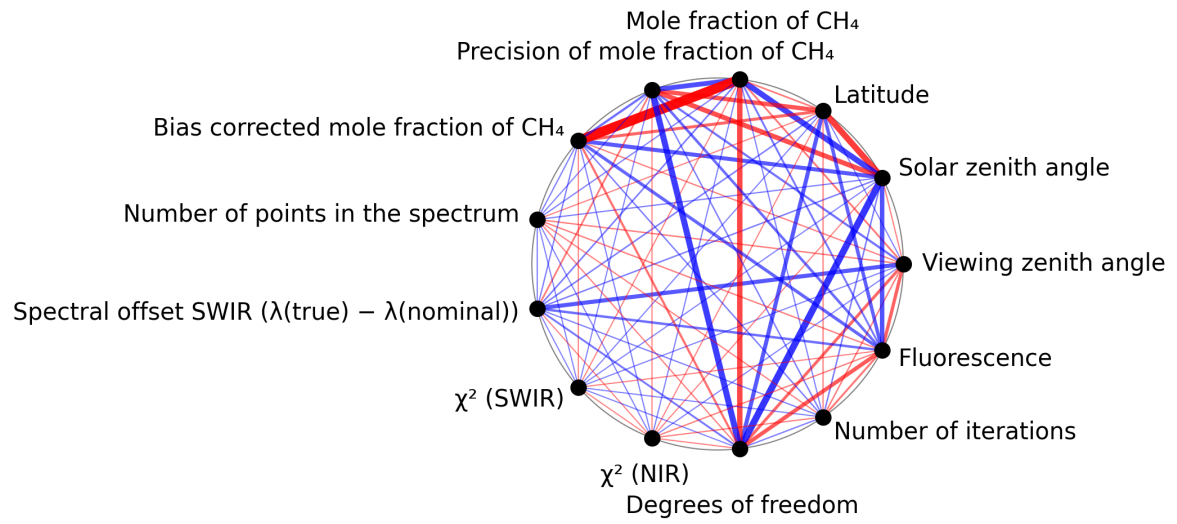
Figure 1: Map of correlation graph for 2025-04-03 to 2025-04-04.
