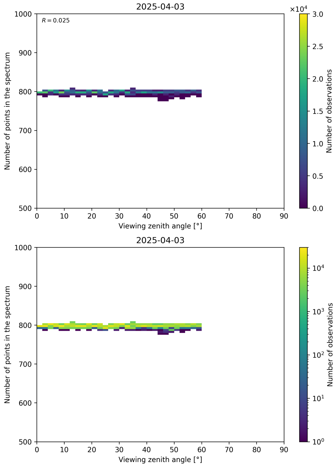
Figure 114: Scatter density plot of “Viewing zenith angle” against “Number of points in the spectrum” for 2025-04-03 to 2025-04-04.
