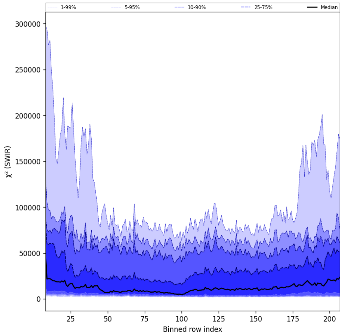
Figure 39: Along track statistics of " \chi^2 (SWIR)" for 2025-04-03 to 2025-04-04
