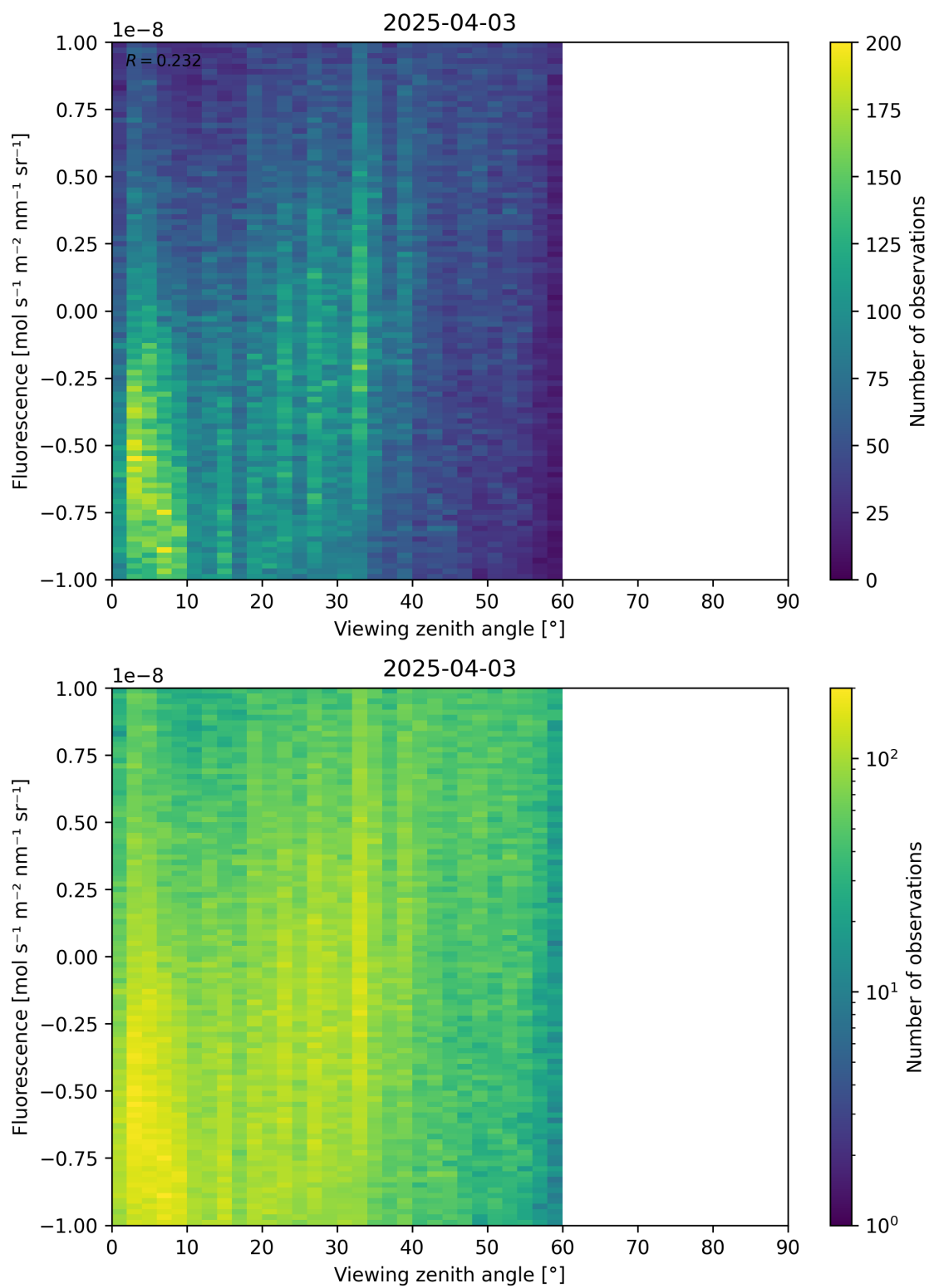
Figure 108: Scatter density plot of “Viewing zenith angle” against “Fluorescence” for 2025-04-03 to 2025-04-04.
