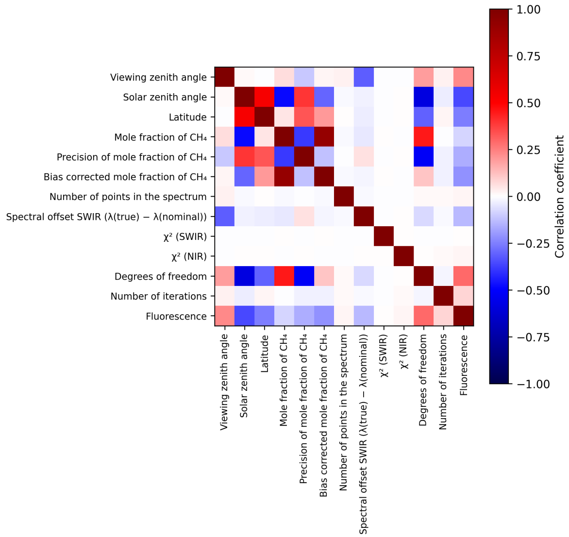
Figure 2: Map of correlation matrix for 2025-04-03 to 2025-04-04.
