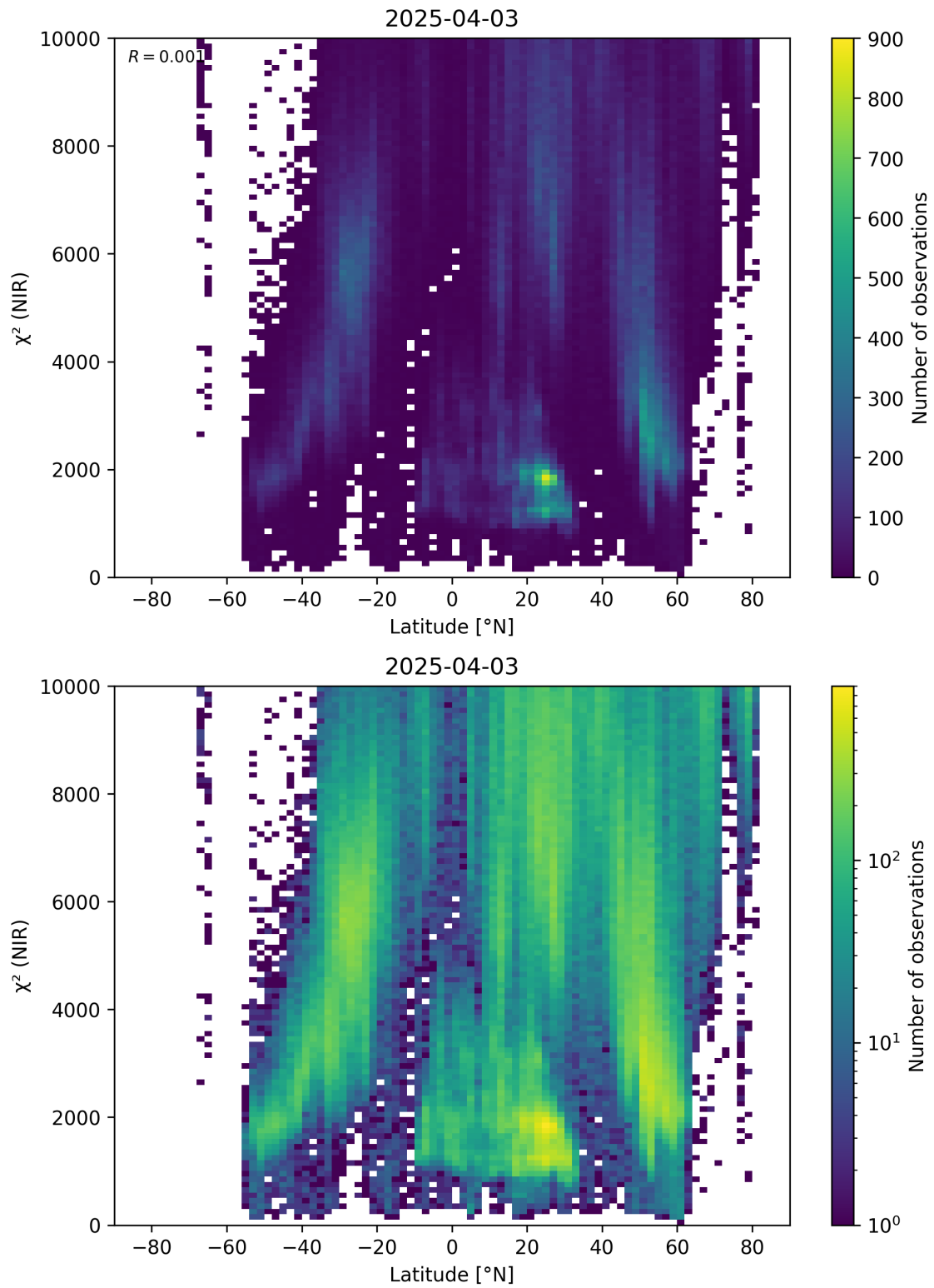
Figure 53: Scatter density plot of “Latitude” against “ \chi^2 (NIR)” for 2025-04-03 to 2025-04-04.
