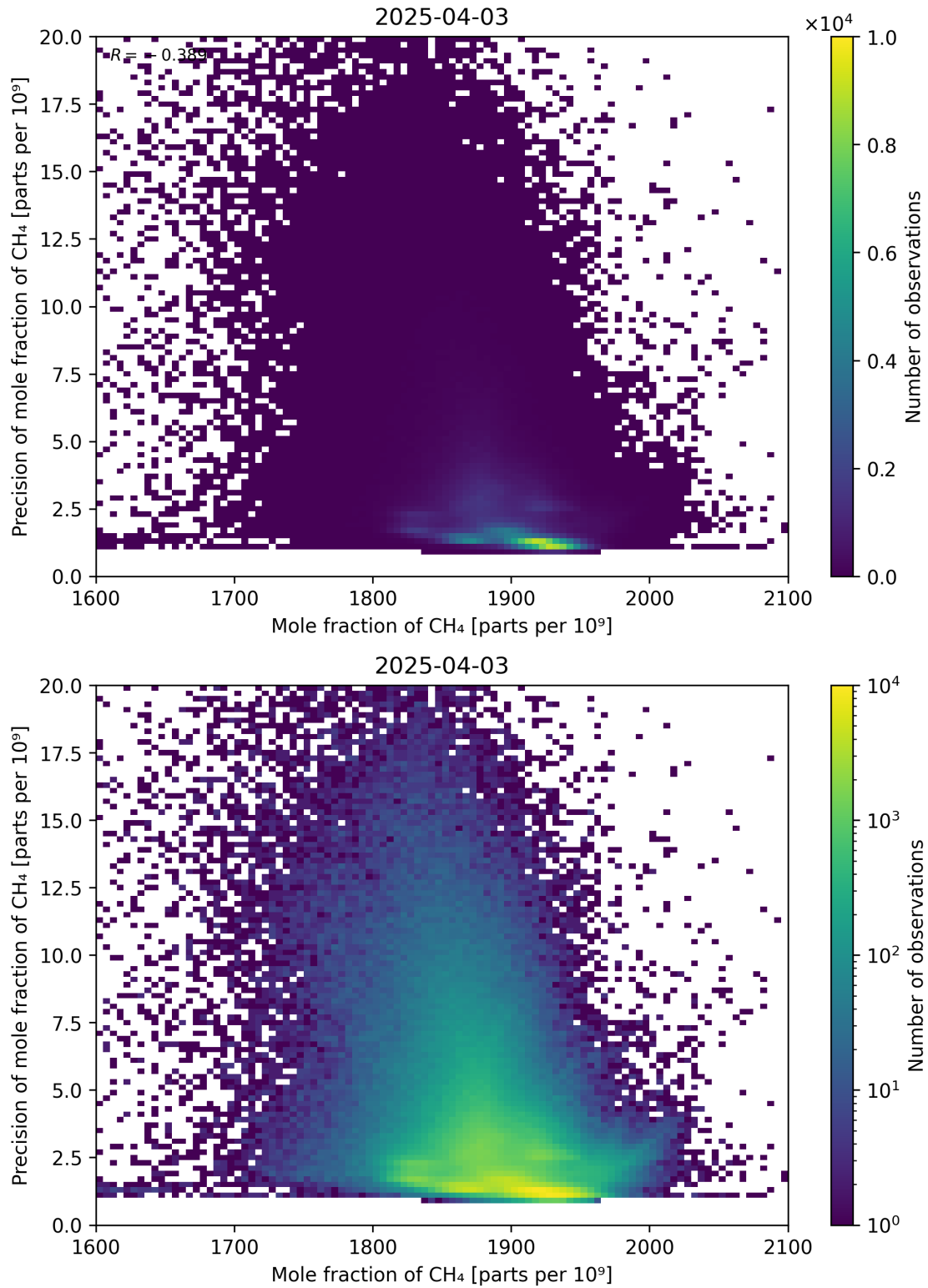
Figure 75: Scatter density plot of “Mole fraction of CH 4 ” against “Precision of mole fraction of CH 4 ” for 2025-04-03 to 2025-04-04.
