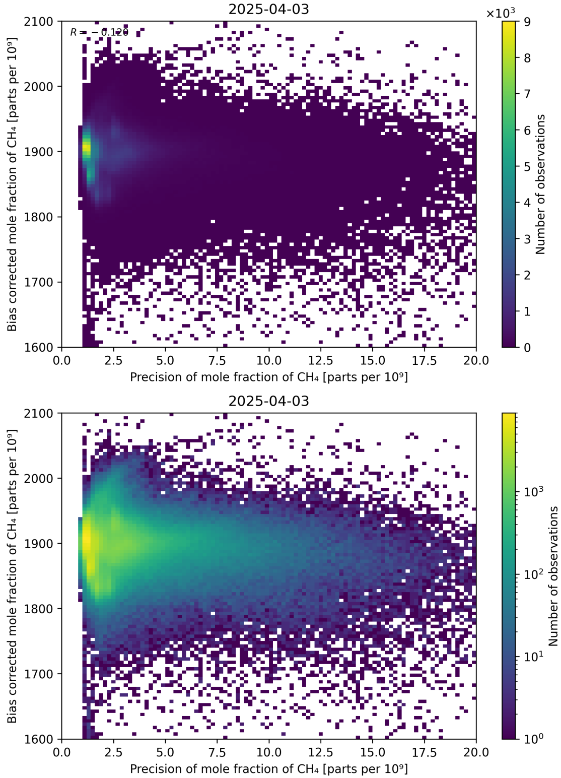
Figure 82: Scatter density plot of “Precision of mole fraction of CH 4 ” against “Bias corrected mole fraction of CH 4 ” for 2025-04-03 to 2025-04-04.
