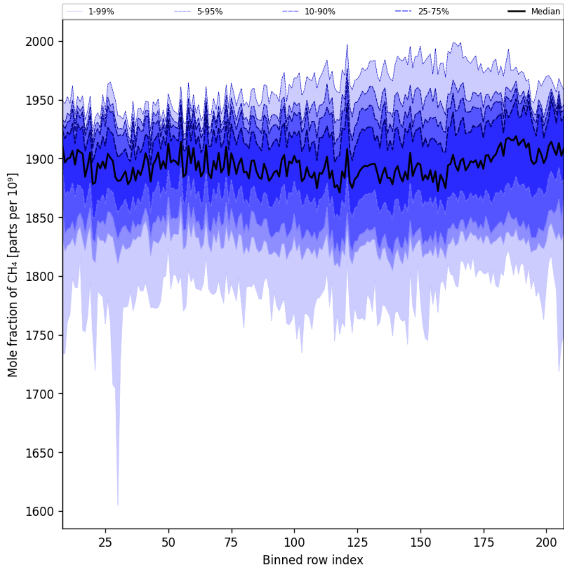
Figure 34: Along track statistics of “Mole fraction of CH 4 ” for 2025-04-03 to 2025-04-04
