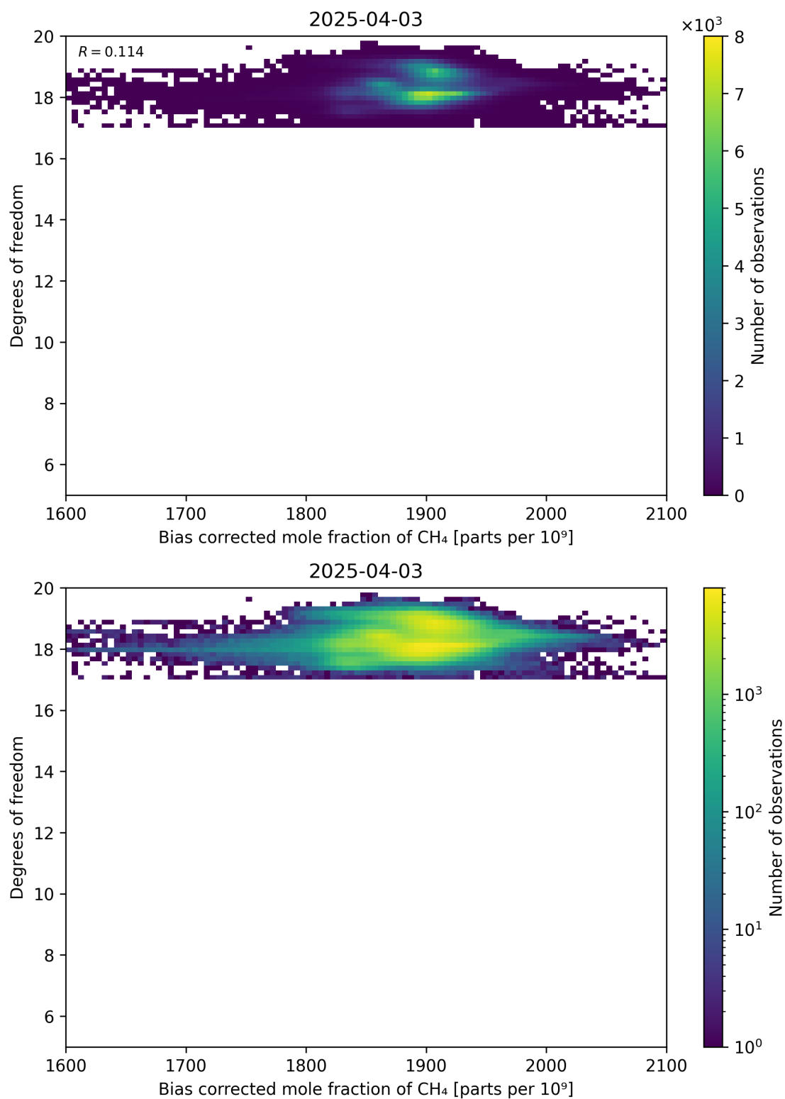
Figure 65: Scatter density plot of “Bias corrected mole fraction of CH 4 ” against “Degrees of freedom” for 2025-04-03 to 2025-04-04.
