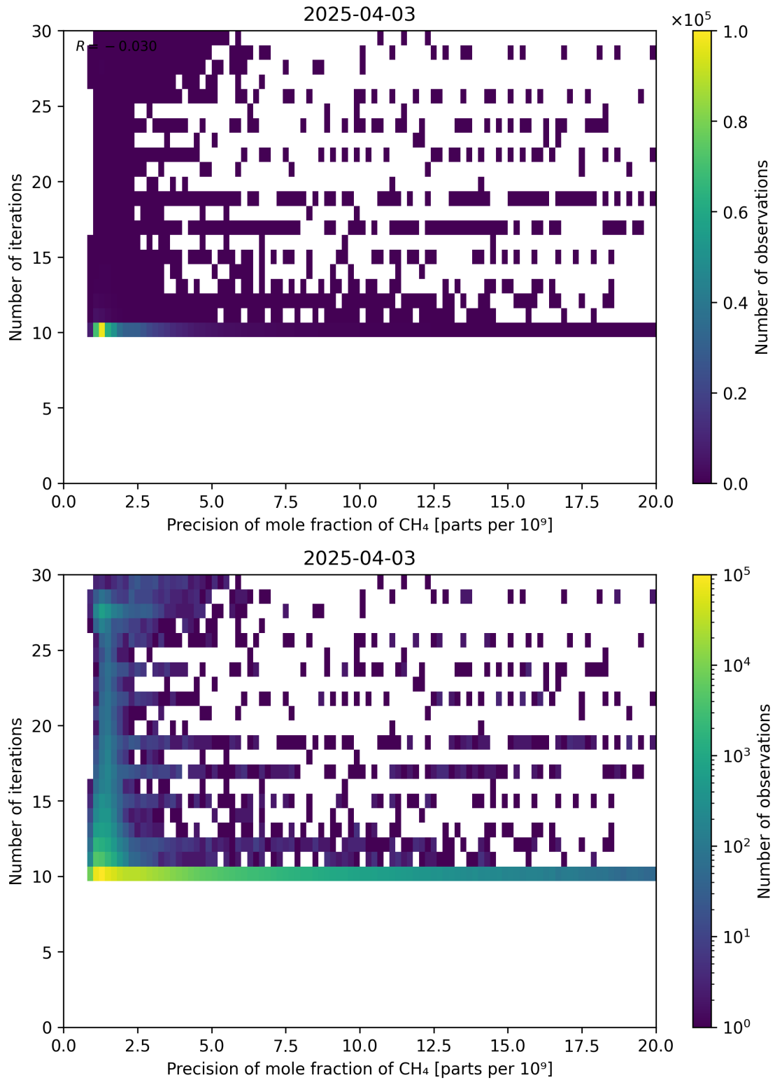
Figure 83: Scatter density plot of “Precision of mole fraction of CH 4 ” against “Number of iterations” for 2025-04-03 to 2025-04-04.
