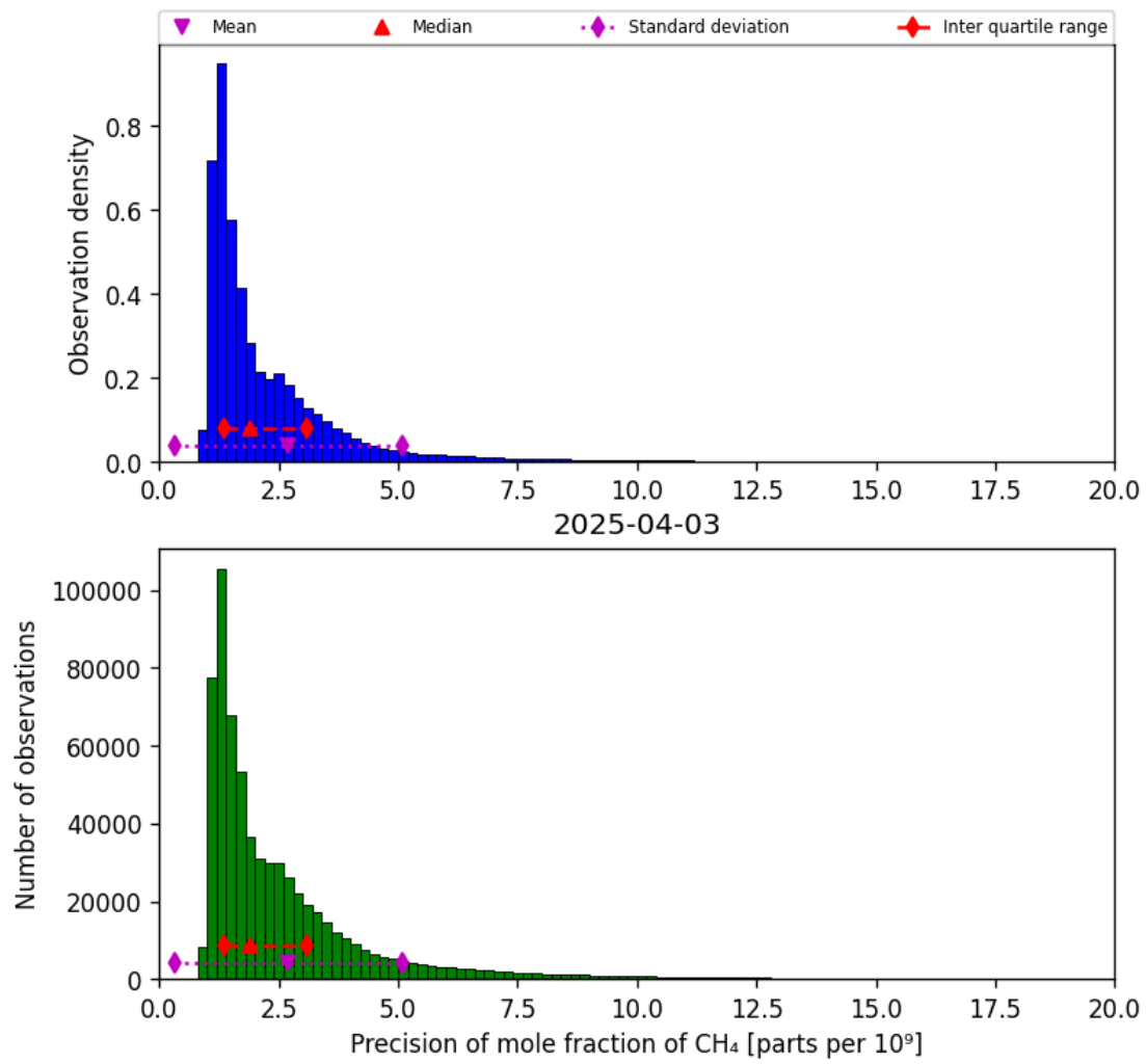
Figure 24: Histogram of “Precision of mole fraction of CH 4 ” for 2025-04-03 to 2025-04-04
