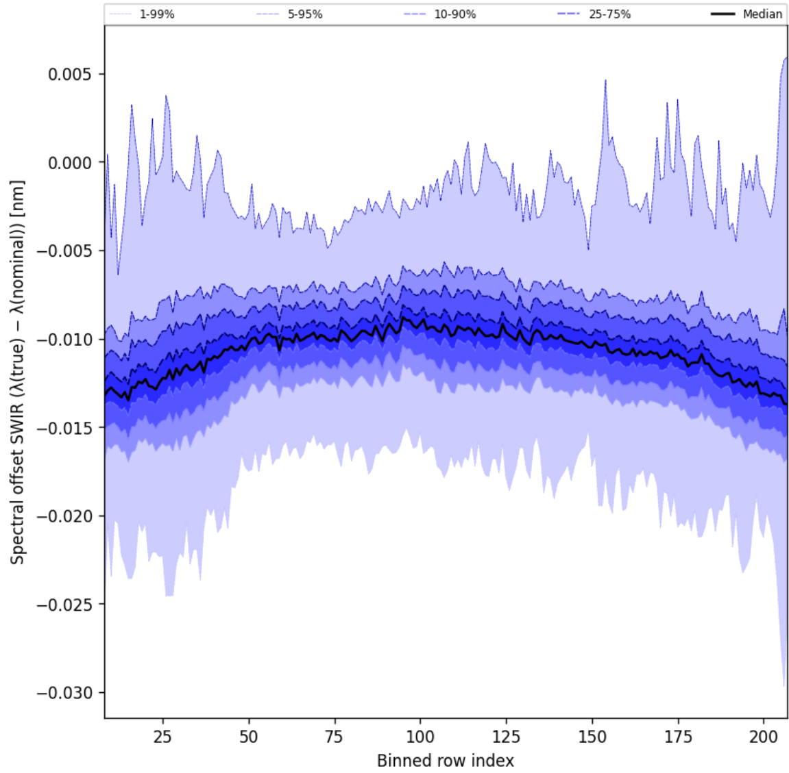
Figure 38: Along track statistics of “Spectral offset SWIR ( \lambda_{\text{true}} - \lambda_{\text{nominal}} )” for 2025-04-03 to 2025-04-04
