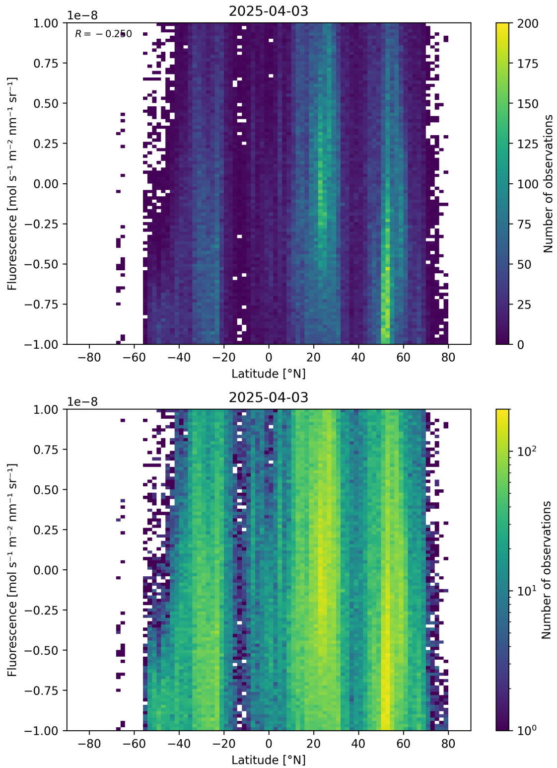
Figure 56: Scatter density plot of “Latitude” against “Fluorescence” for 2025-04-03 to 2025-04-04.
