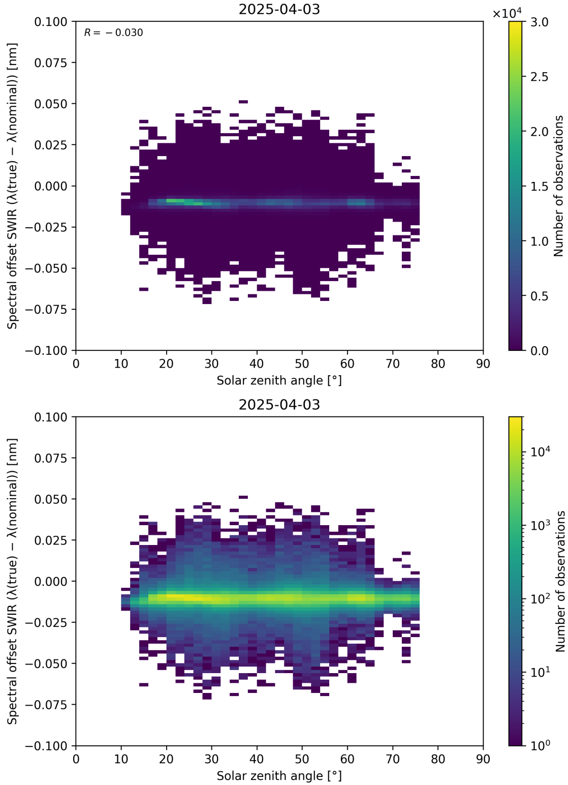
Figure 104: Scatter density plot of “Solar zenith angle” against “Spectral offset SWIR ( \lambda_{\text{true}} - \lambda_{\text{nominal}} )” for 2025-04-03 to 2025-04-04.
