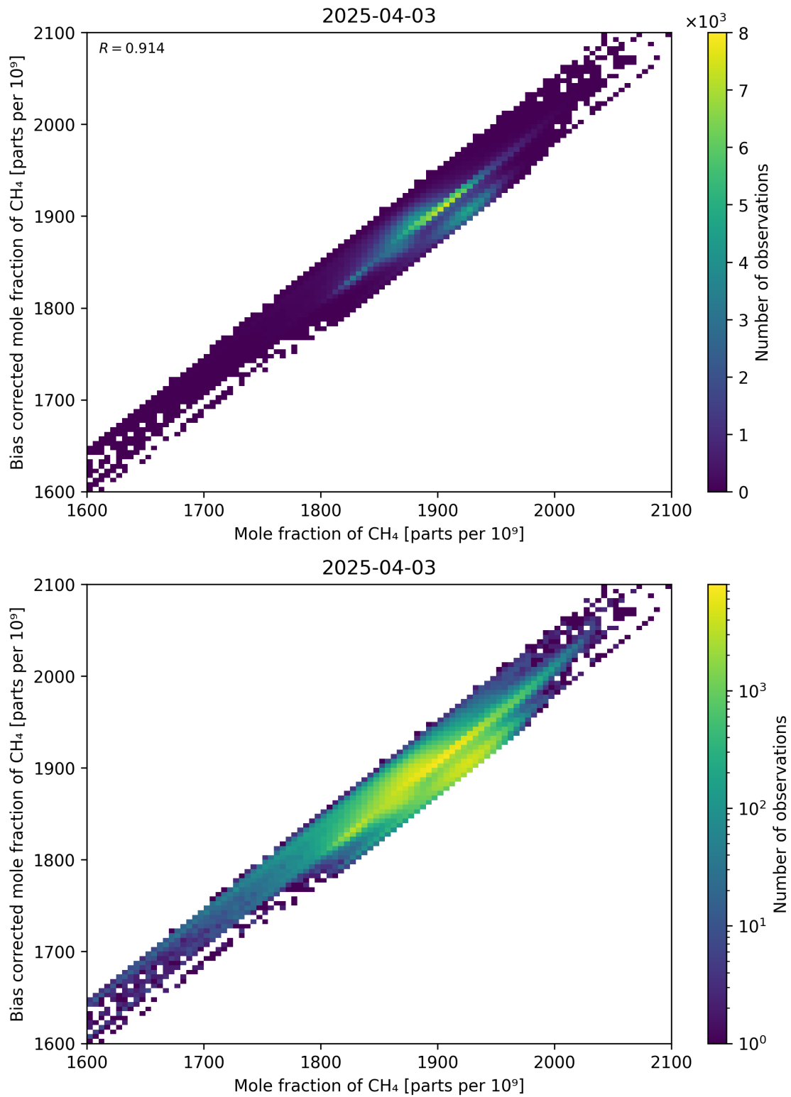
Figure 74: Scatter density plot of “Mole fraction of CH 4 ” against “Bias corrected mole fraction of CH 4 ” for 2025-04-03 to 2025-04-04.
