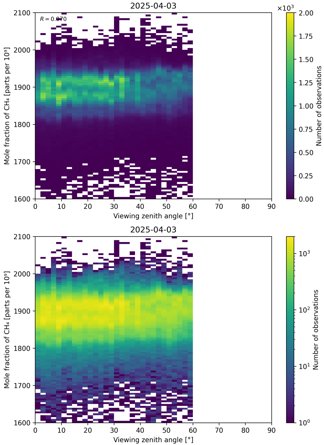
Figure 110: Scatter density plot of “Viewing zenith angle” against “Mole fraction of CH 4 ” for 2025-04-03 to 2025-04-04.
