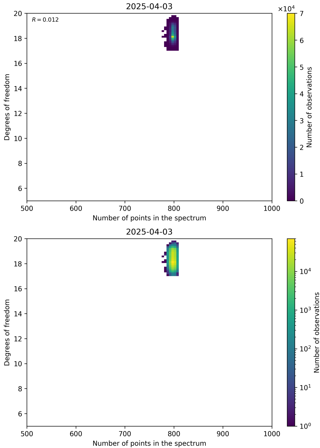
Figure 90: Scatter density plot of “Number of points in the spectrum” against “Degrees of freedom” for 2025-04-03 to 2025-04-04.
