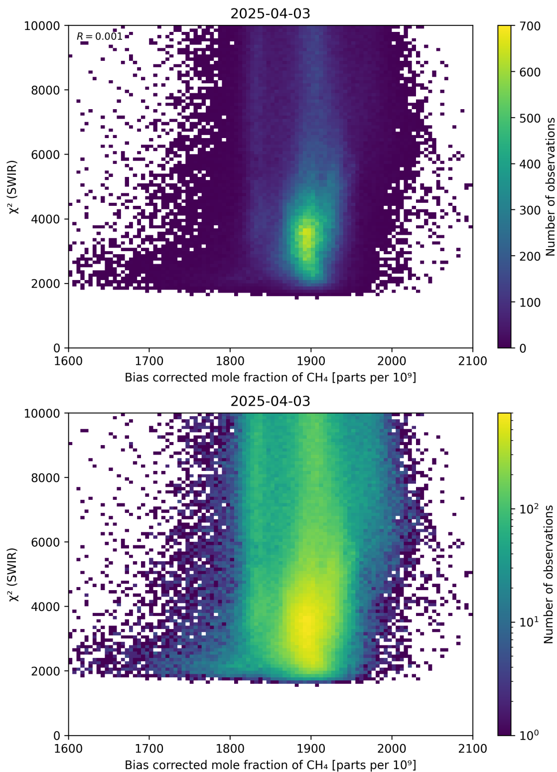
Figure 64: Scatter density plot of “Bias corrected mole fraction of \text{CH}_4 ” against “ \chi^2 (SWIR)” for 2025-04-03 to 2025-04-04.
