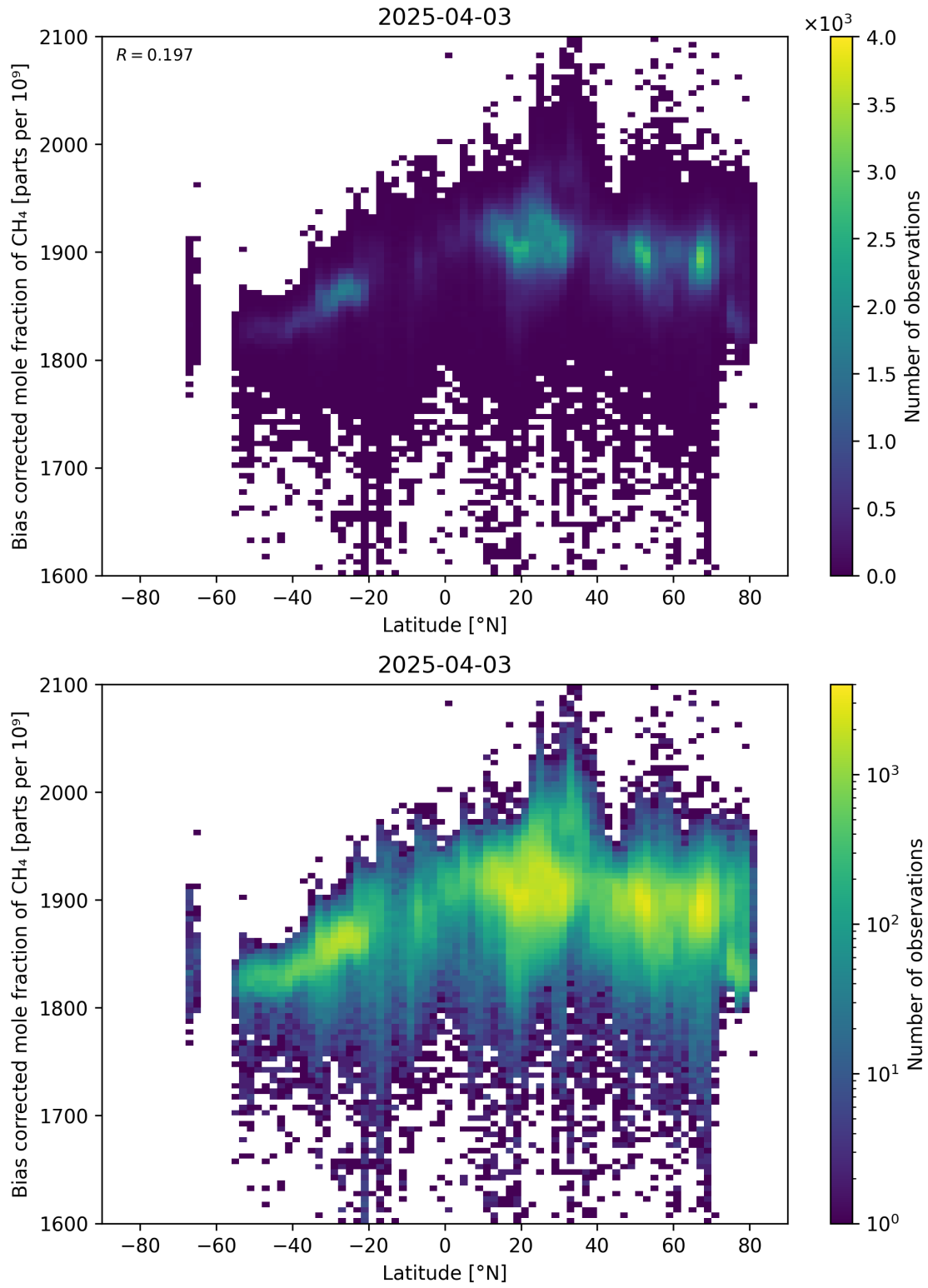
Figure 58: Scatter density plot of “Latitude” against “Bias corrected mole fraction of CH 4 ” for 2025-04-03 to 2025-04-04.
