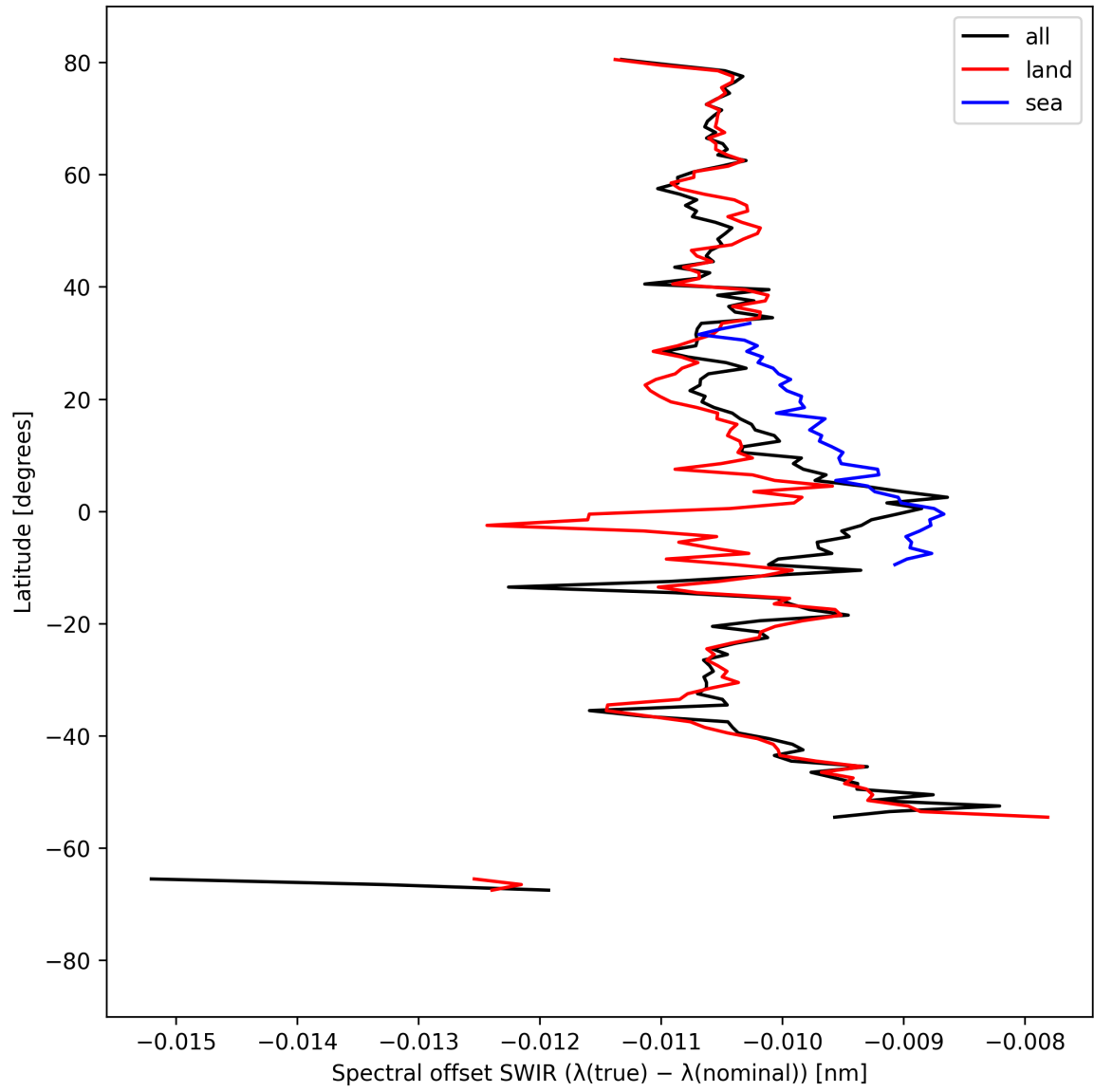
Figure 16: Zonal average of “Spectral offset SWIR ( \lambda_{\text{true}} - \lambda_{\text{nominal}} )” for 2025-04-03 to 2025-04-04.
