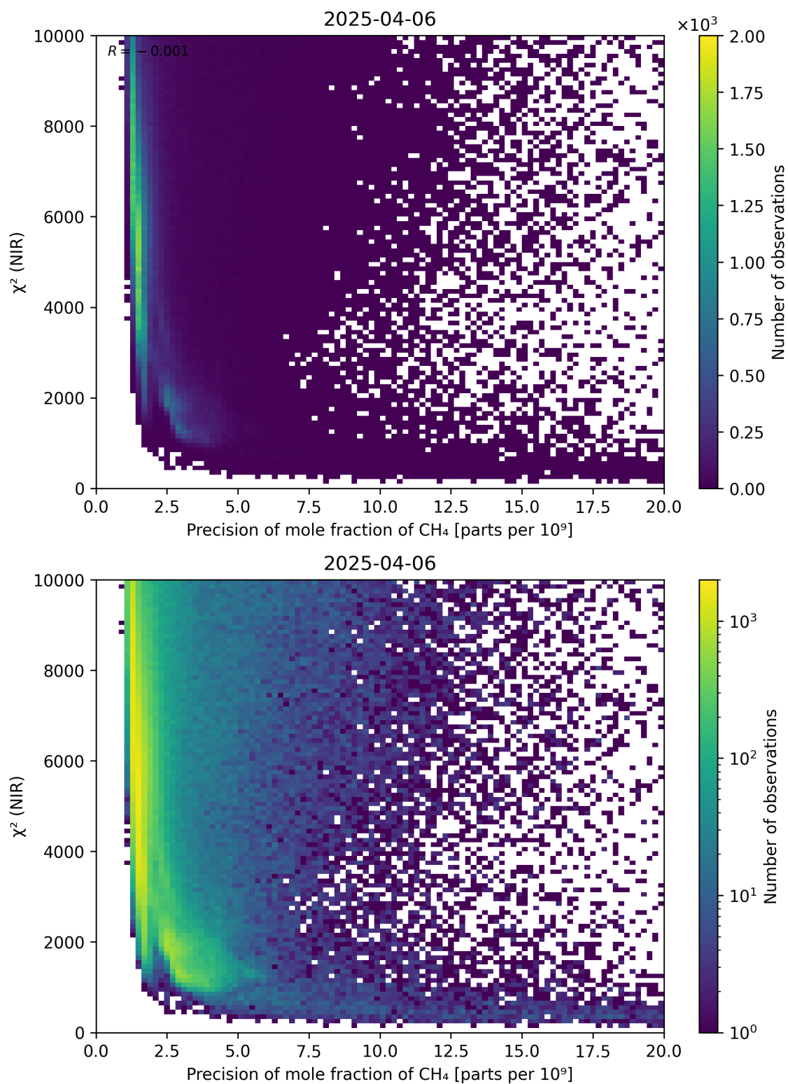
Figure 78: Scatter density plot of “Precision of mole fraction of CH 4 ” against “ \chi^2 (NIR)” for 2025-04-05 to 2025-04-07.
