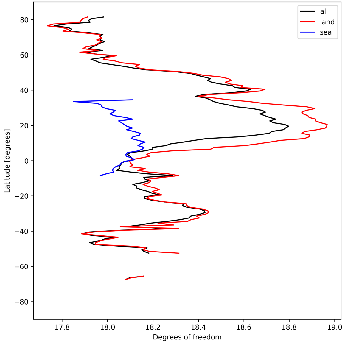
Figure 19: Zonal average of “Degrees of freedom” for 2025-04-05 to 2025-04-07.
