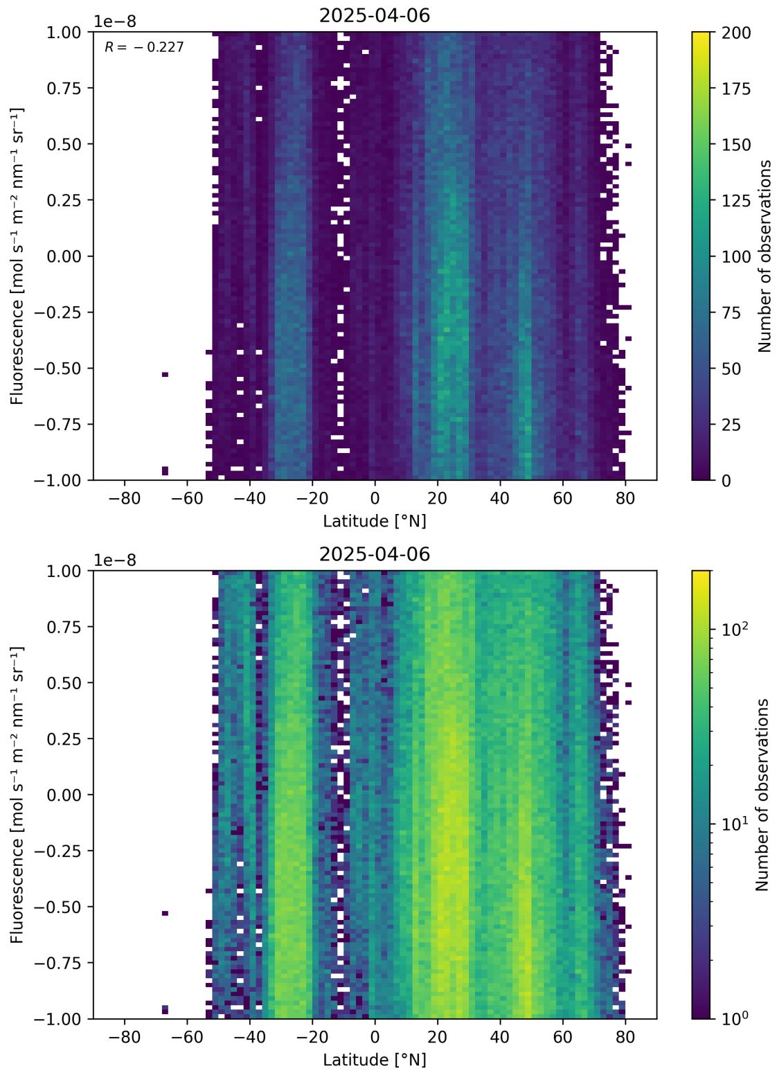
Figure 56: Scatter density plot of “Latitude” against “Fluorescence” for 2025-04-05 to 2025-04-07.
