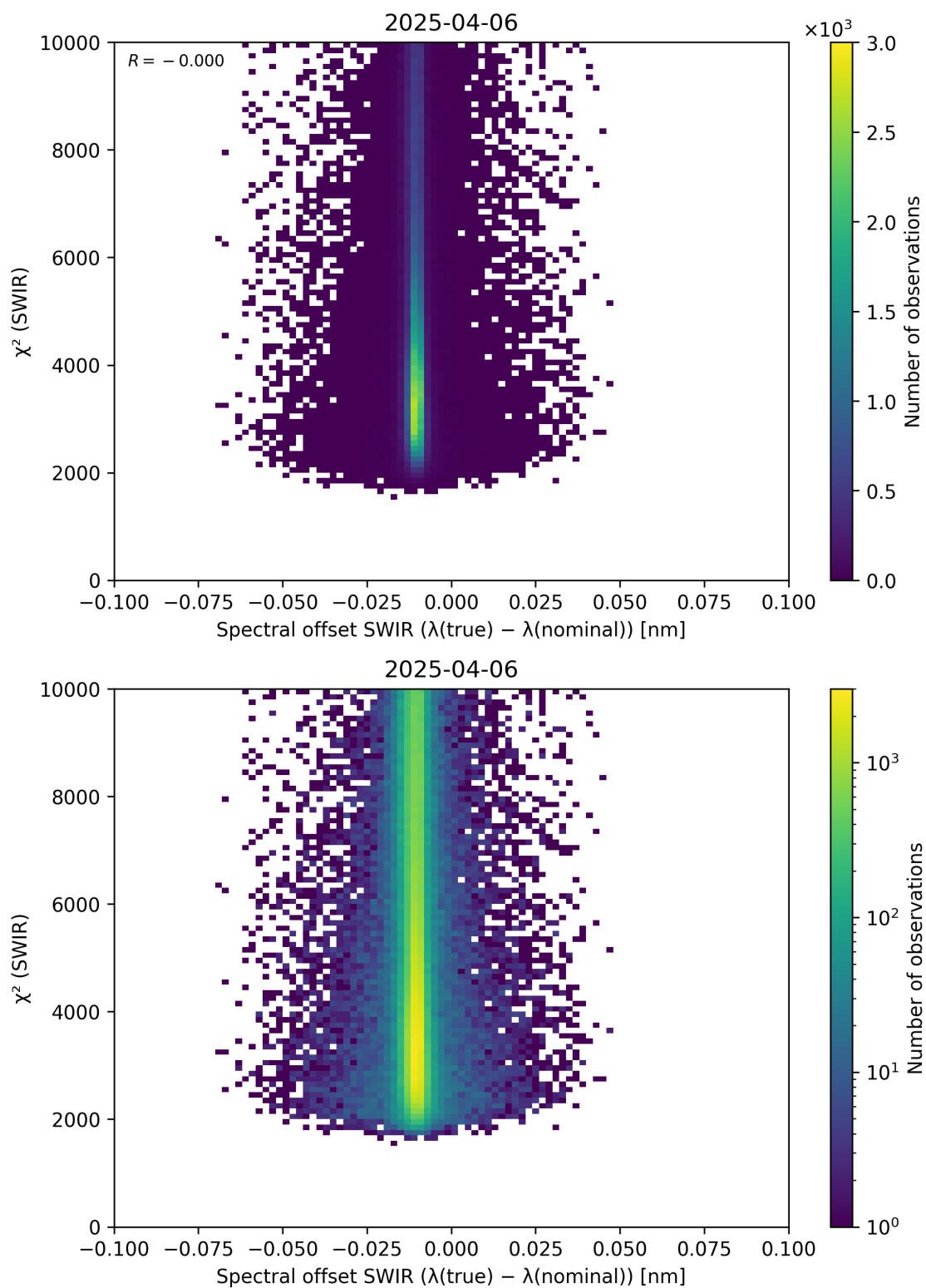
Figure 118: Scatter density plot of “Spectral offset SWIR ( \lambda_{\text{true}} - \lambda_{\text{nominal}} )” against “ \chi^2 (SWIR)” for 2025-04-05 to 2025-04-07.
