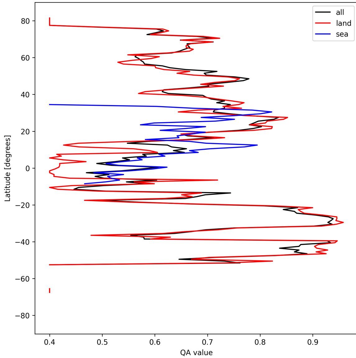
Figure 11: Zonal average of “QA value” for 2025-04-05 to 2025-04-07.
