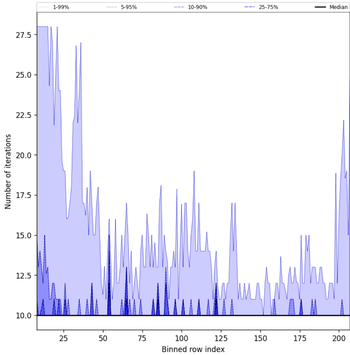
Figure 42: Along track statistics of “Number of iterations” for 2025-04-05 to 2025-04-07
