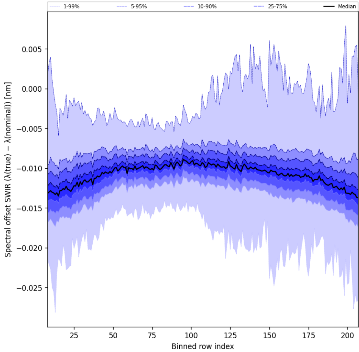
Figure 38: Along track statistics of “Spectral offset SWIR ( \lambda_{\text{true}} - \lambda_{\text{nominal}} )” for 2025-04-05 to 2025-04-07
