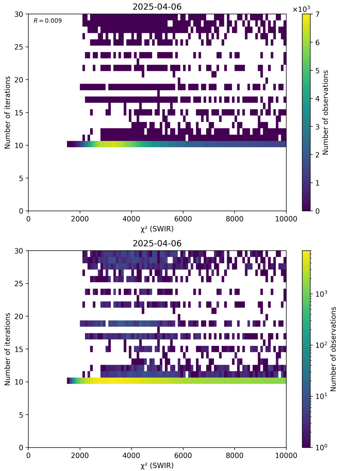
Figure 50: Scatter density plot of “ \chi^2 (SWIR)” against “Number of iterations” for 2025-04-05 to 2025-04-07.
