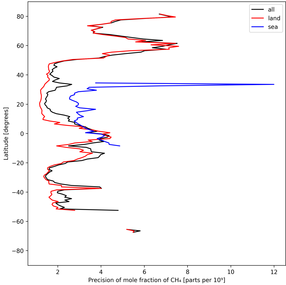
Figure 13: Zonal average of “Precision of mole fraction of CH 4 ” for 2025-04-05 to 2025-04-07.
