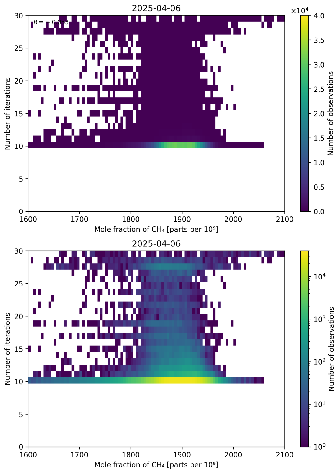
Figure 76: Scatter density plot of “Mole fraction of CH 4 ” against “Number of iterations” for 2025-04-05 to 2025-04-07.
