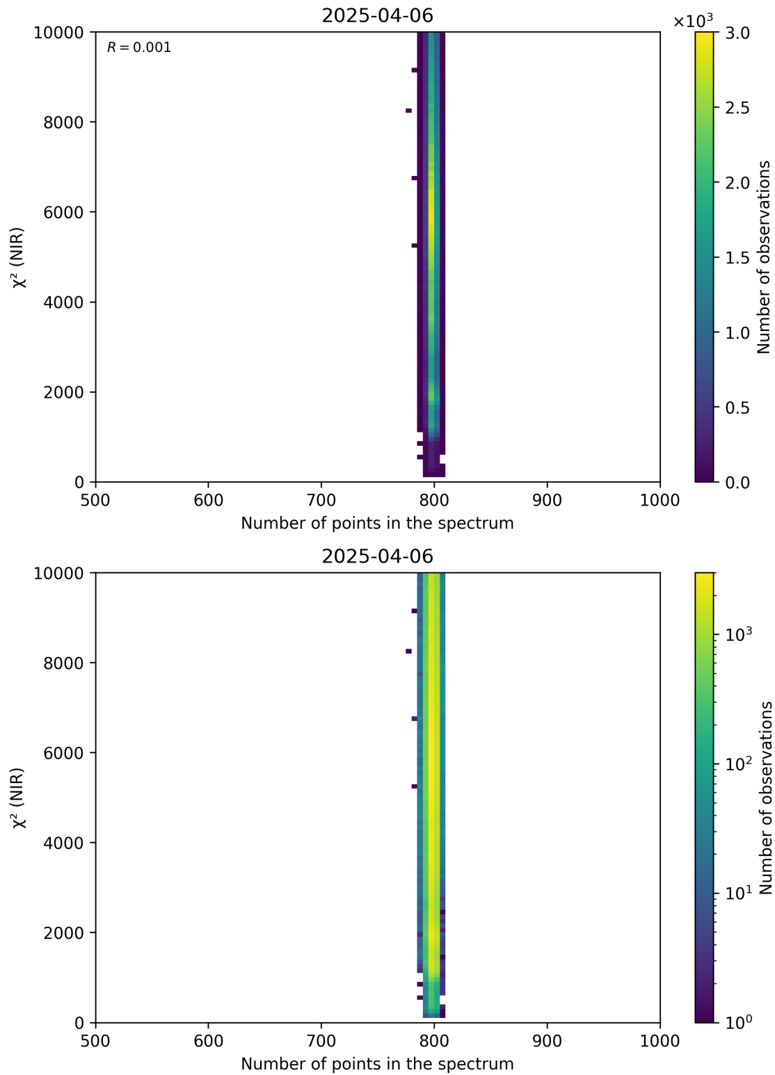
Figure 88: Scatter density plot of “Number of points in the spectrum” against “ \chi^2 (NIR)” for 2025-04-05 to 2025-04-07.
