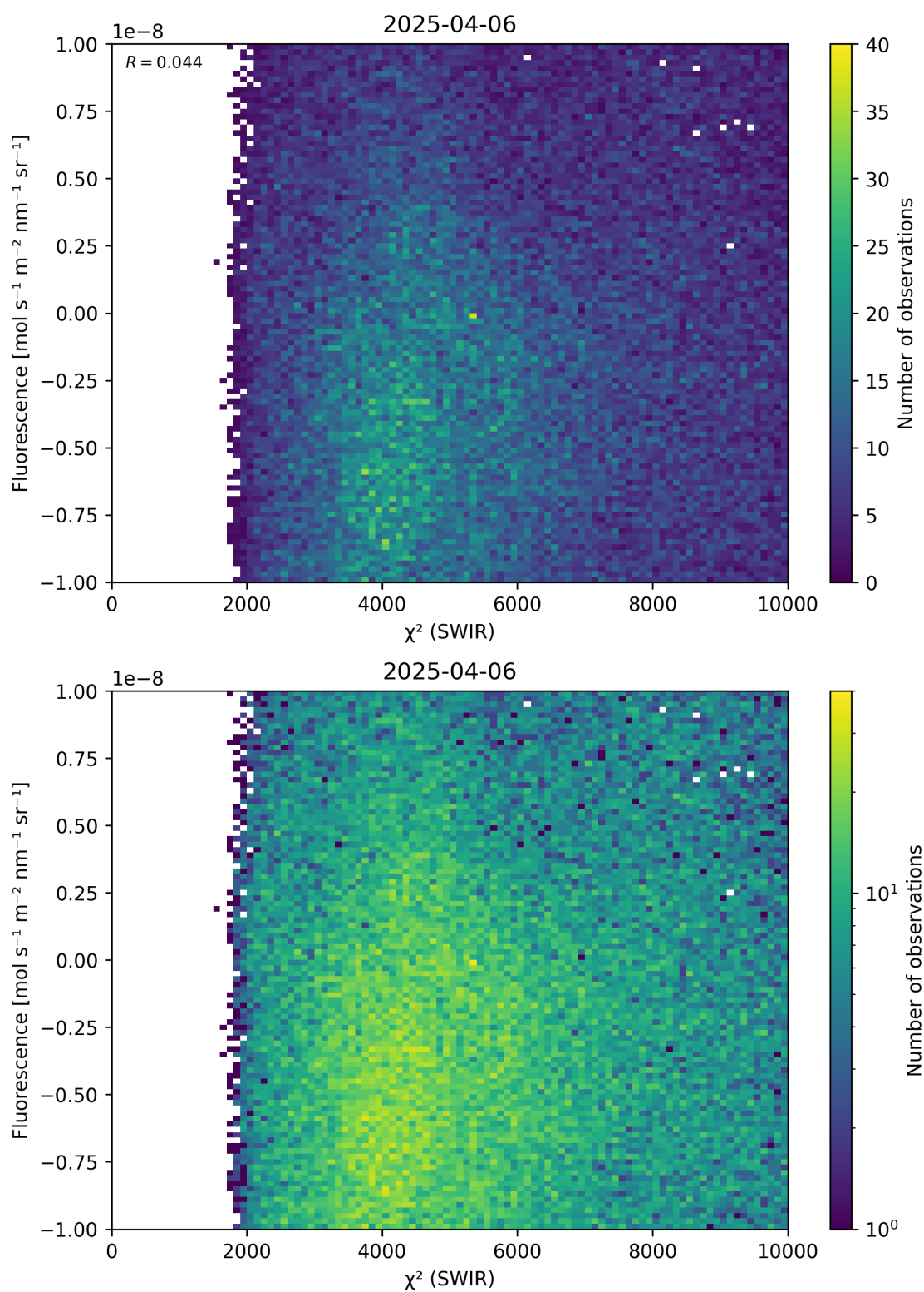
Figure 49: Scatter density plot of “ \chi^2 (SWIR)” against “Fluorescence” for 2025-04-05 to 2025-04-07.
