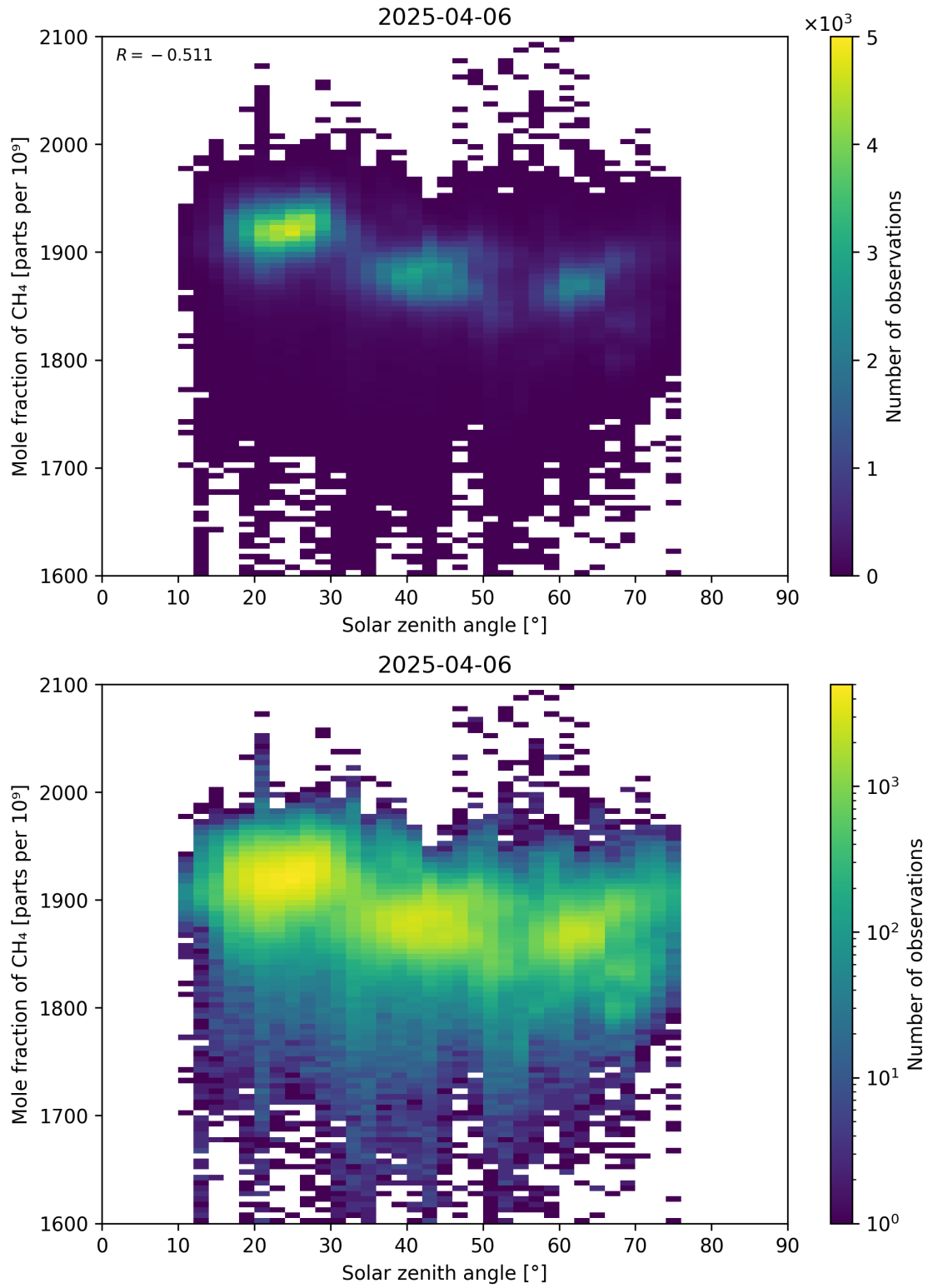
Figure 99: Scatter density plot of “Solar zenith angle” against “Mole fraction of \text{CH}_4 ” for 2025-04-05 to 2025-04-07.
