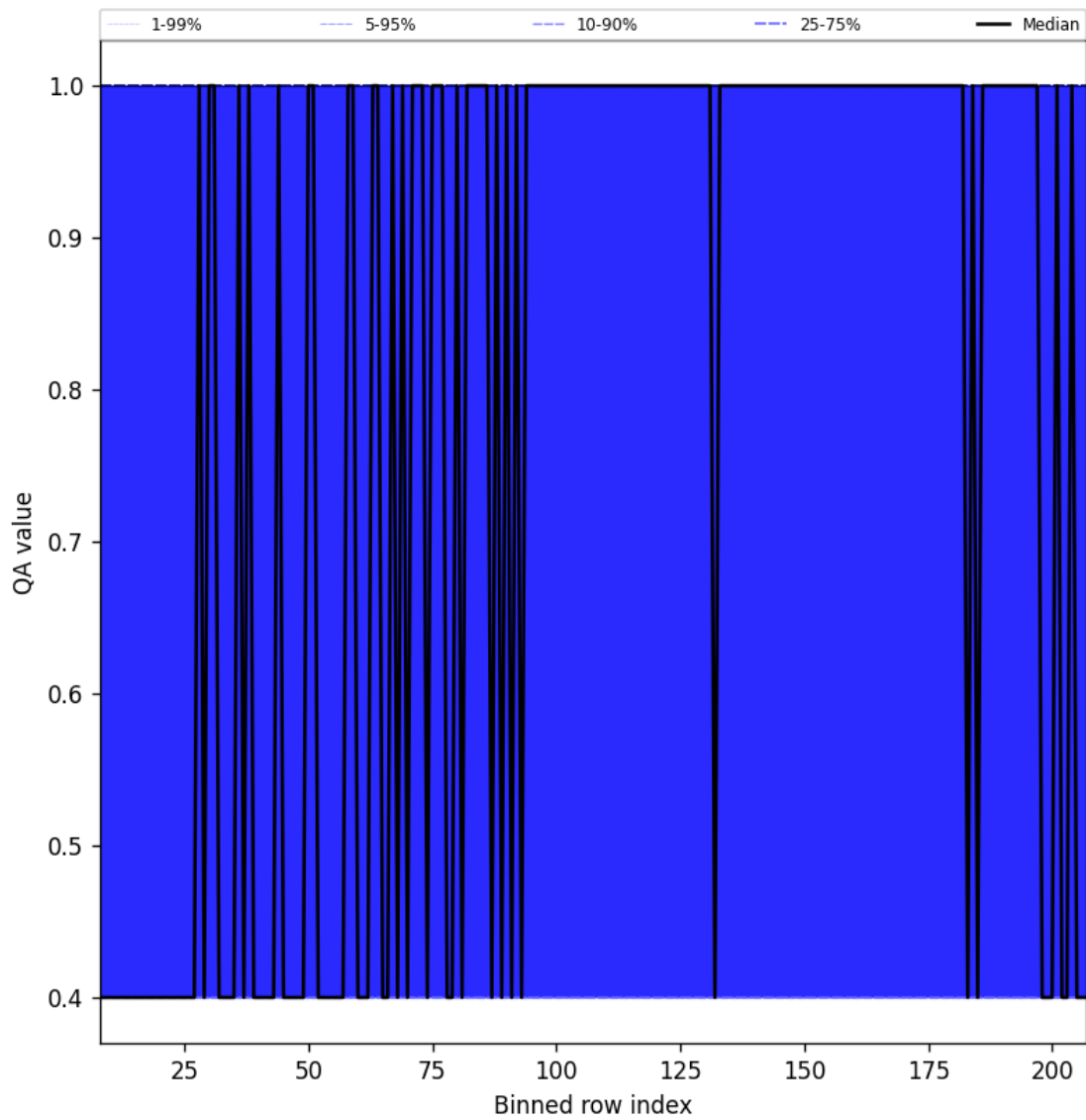
Figure 33: Along track statistics of “QA value” for 2025-04-05 to 2025-04-07
