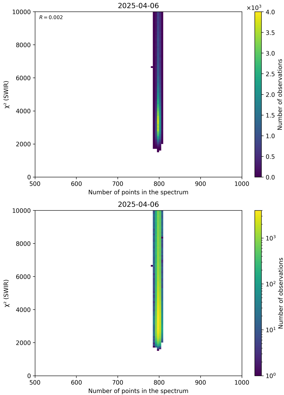
Figure 89: Scatter density plot of “Number of points in the spectrum” against “ \chi^2 (SWIR)” for 2025-04-05 to 2025-04-07.
