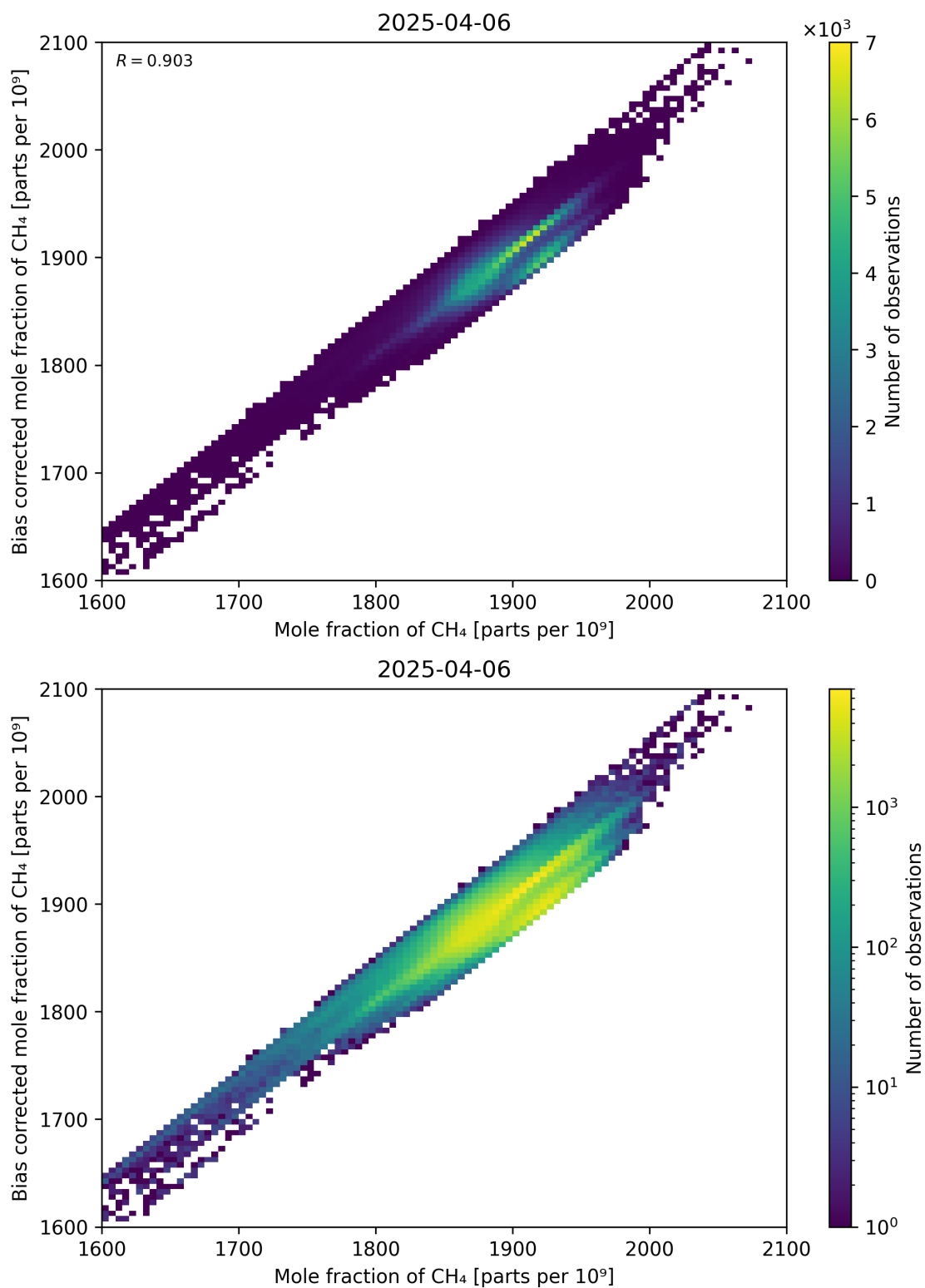
Figure 74: Scatter density plot of “Mole fraction of CH 4 ” against “Bias corrected mole fraction of CH 4 ” for 2025-04-05 to 2025-04-07.
