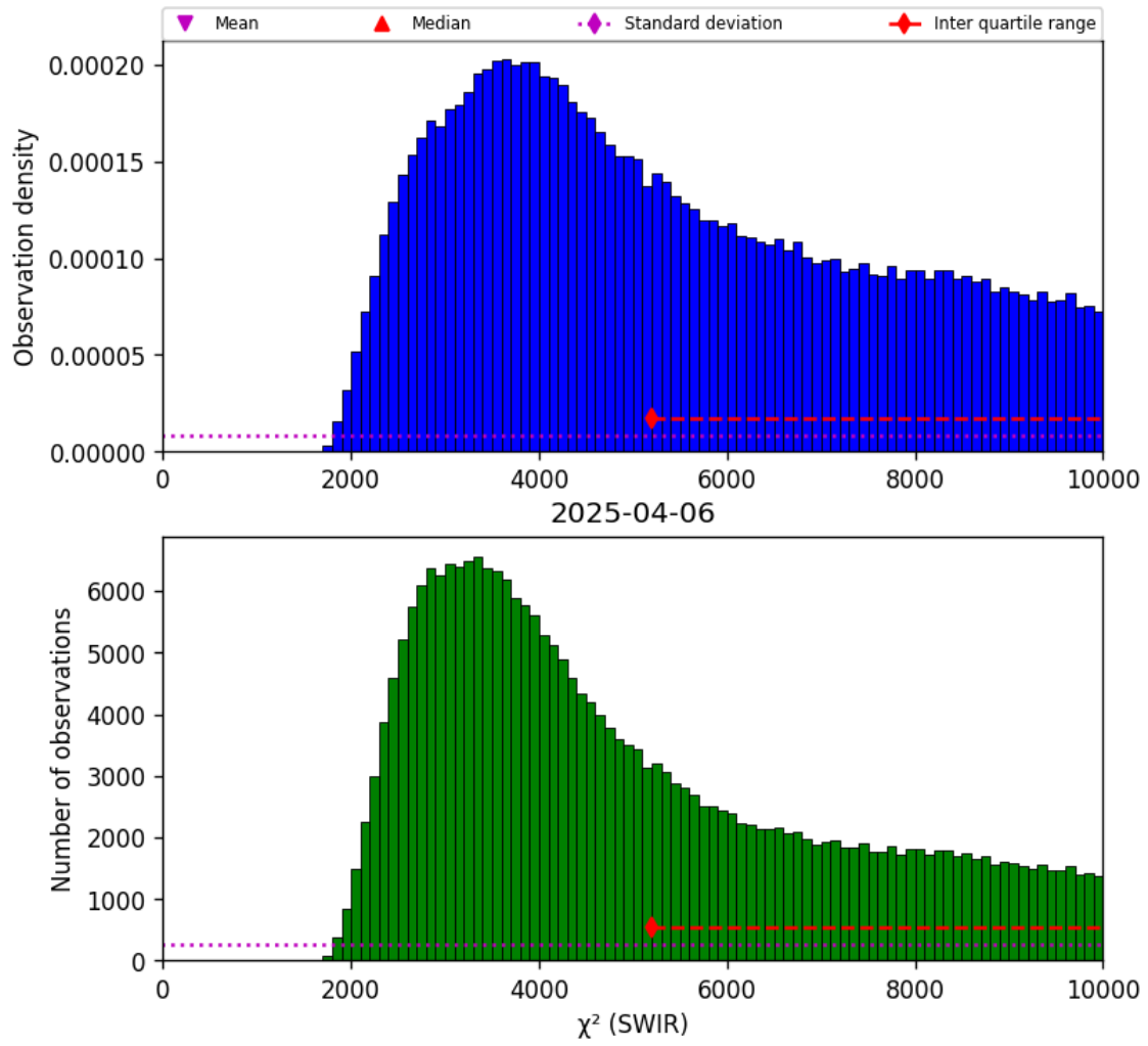
Figure 28: Histogram of “ \chi^2 (SWIR)” for 2025-04-05 to 2025-04-07
