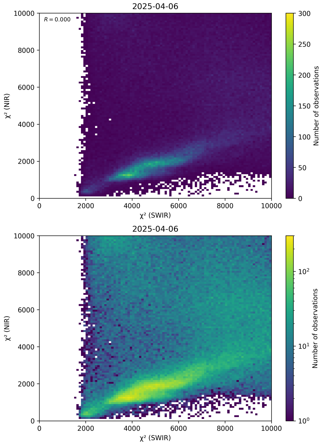
Figure 47: Scatter density plot of “ \chi^2 (SWIR)” against “ \chi^2 (NIR)” for 2025-04-05 to 2025-04-07.
