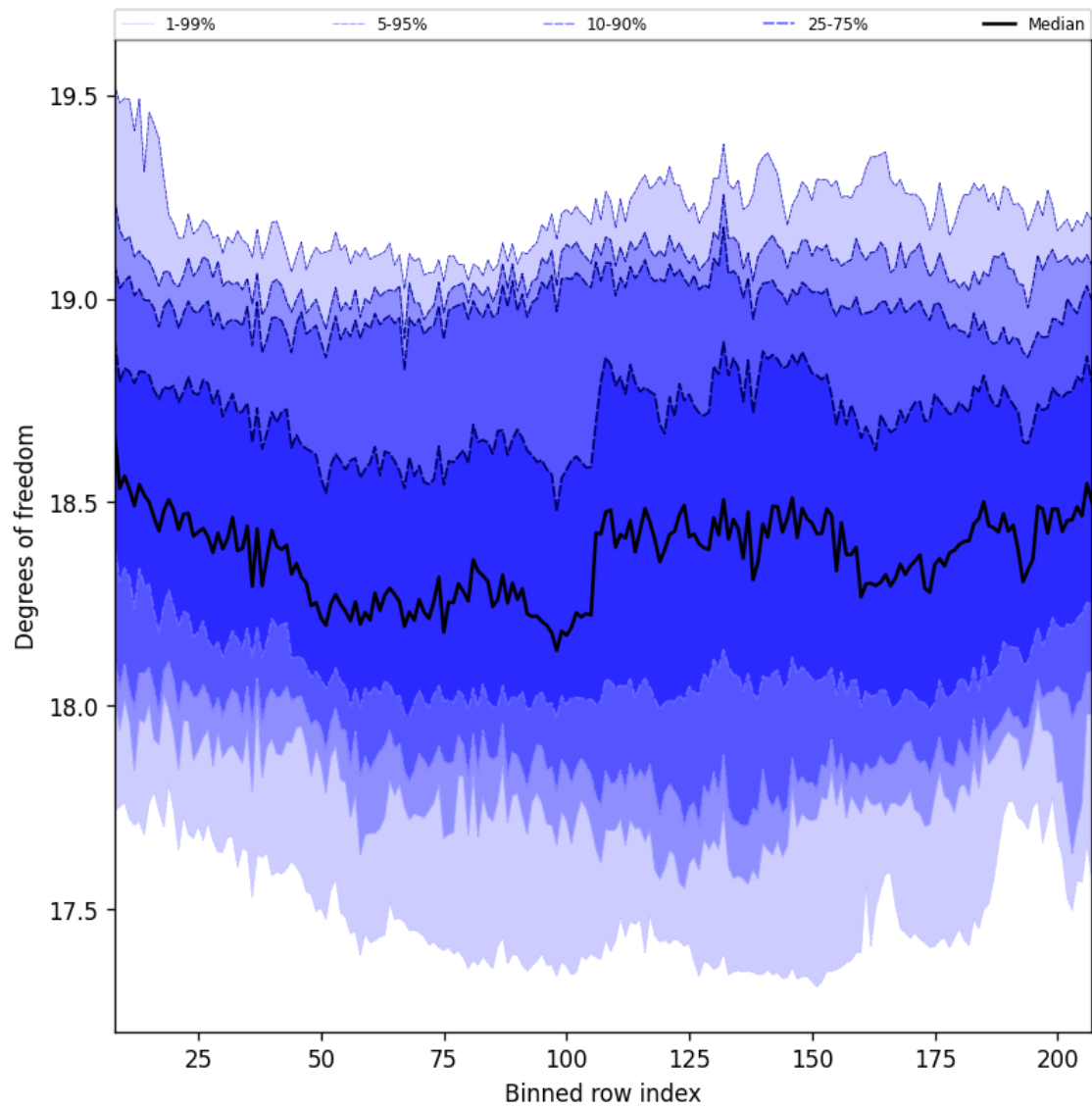
Figure 41: Along track statistics of “Degrees of freedom” for 2025-04-05 to 2025-04-07
