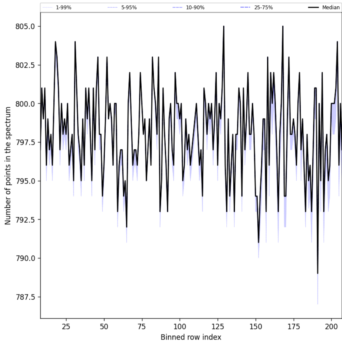
Figure 37: Along track statistics of “Number of points in the spectrum” for 2025-04-05 to 2025-04-07
