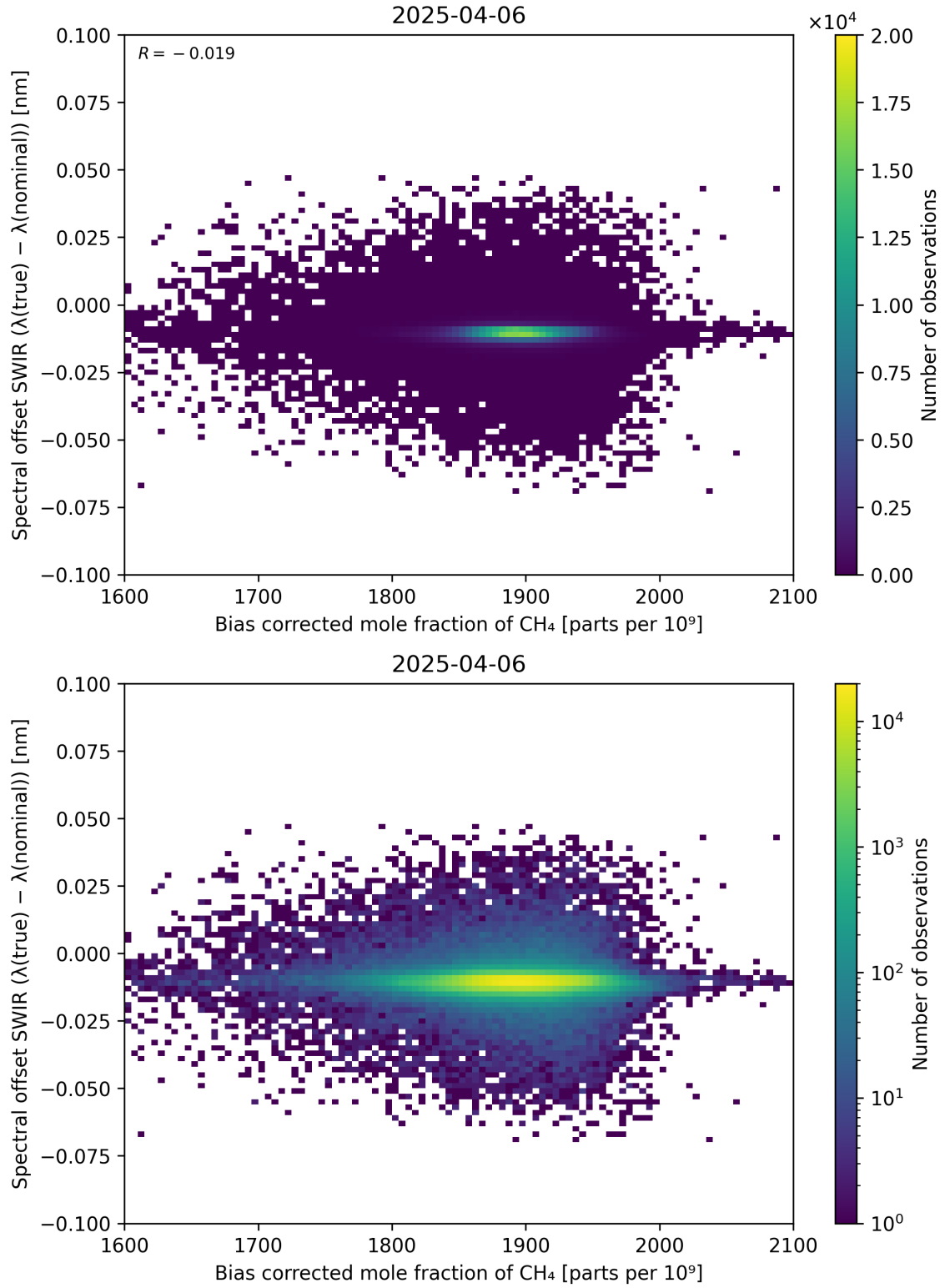
Figure 69: Scatter density plot of “Bias corrected mole fraction of CH 4 ” against “Spectral offset SWIR ( \lambda_{\text{true}} - \lambda_{\text{nominal}} )” for 2025-04-05 to 2025-04-07.
