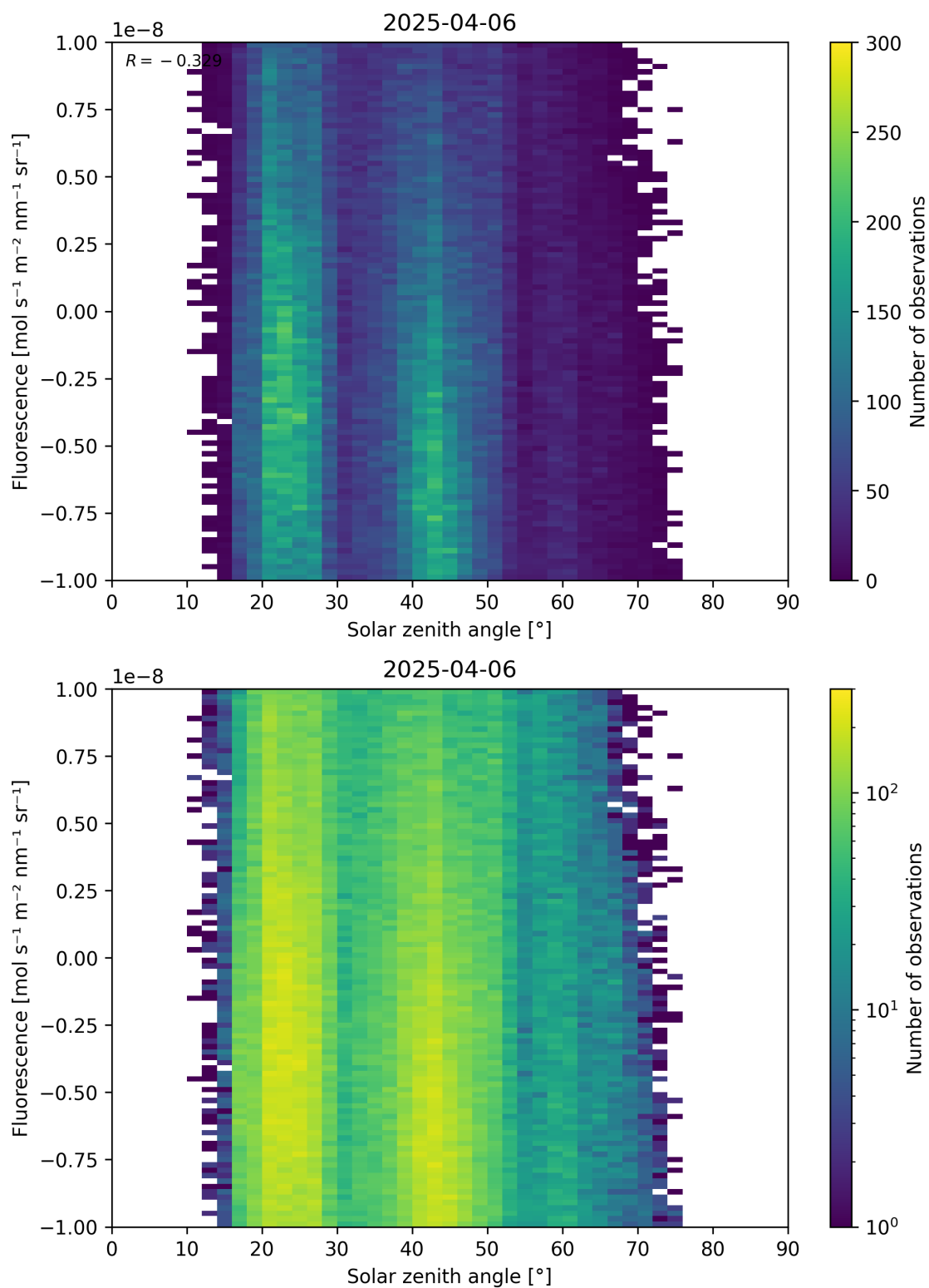
Figure 97: Scatter density plot of “Solar zenith angle” against “Fluorescence” for 2025-04-05 to 2025-04-07.
