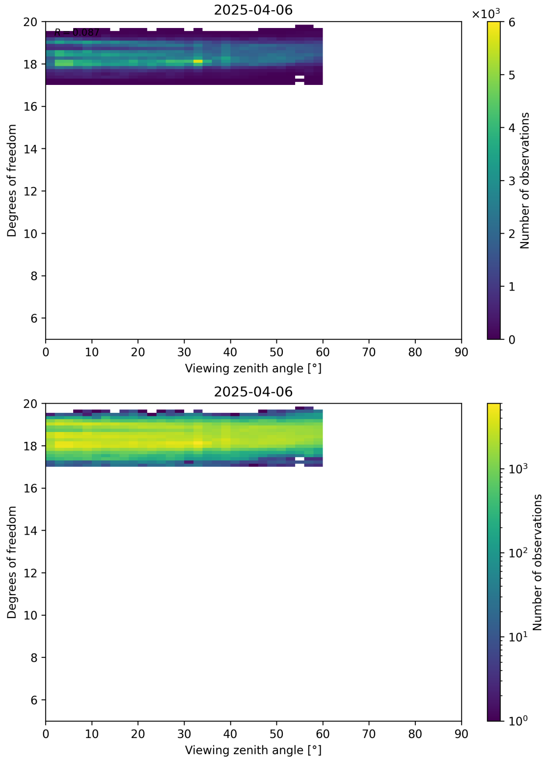
Figure 107: Scatter density plot of “Viewing zenith angle” against “Degrees of freedom” for 2025-04-05 to 2025-04-07.
