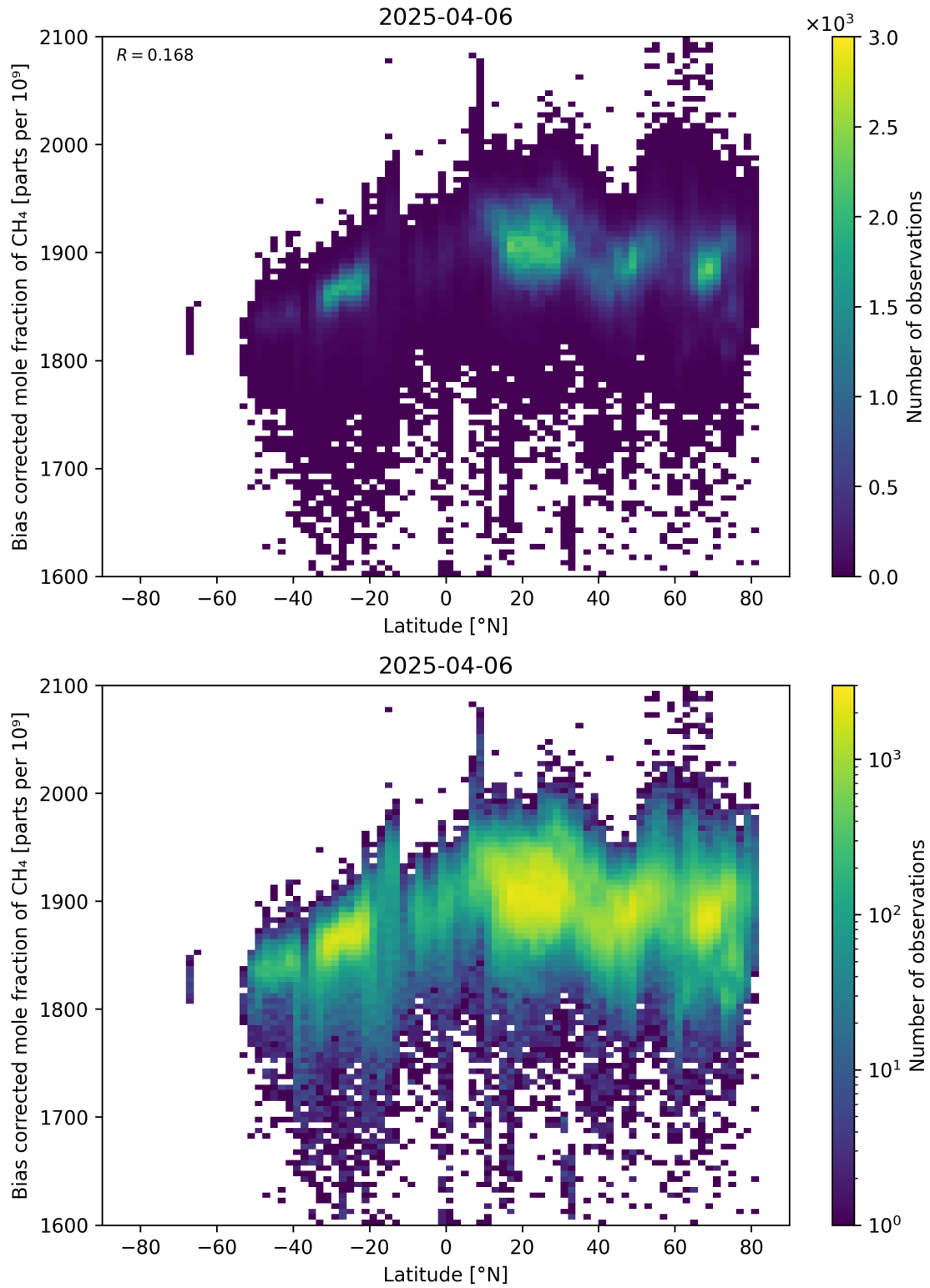
Figure 58: Scatter density plot of “Latitude” against “Bias corrected mole fraction of CH 4 ” for 2025-04-05 to 2025-04-07.
