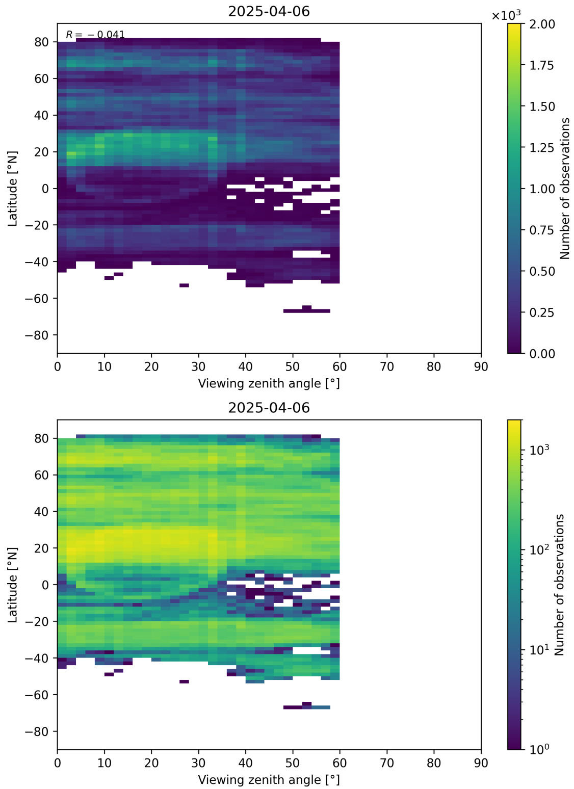
Figure 109: Scatter density plot of “Viewing zenith angle” against “Latitude” for 2025-04-05 to 2025-04-07.
