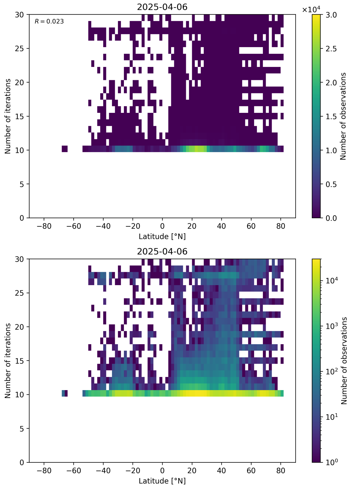
Figure 60: Scatter density plot of “Latitude” against “Number of iterations” for 2025-04-05 to 2025-04-07.
