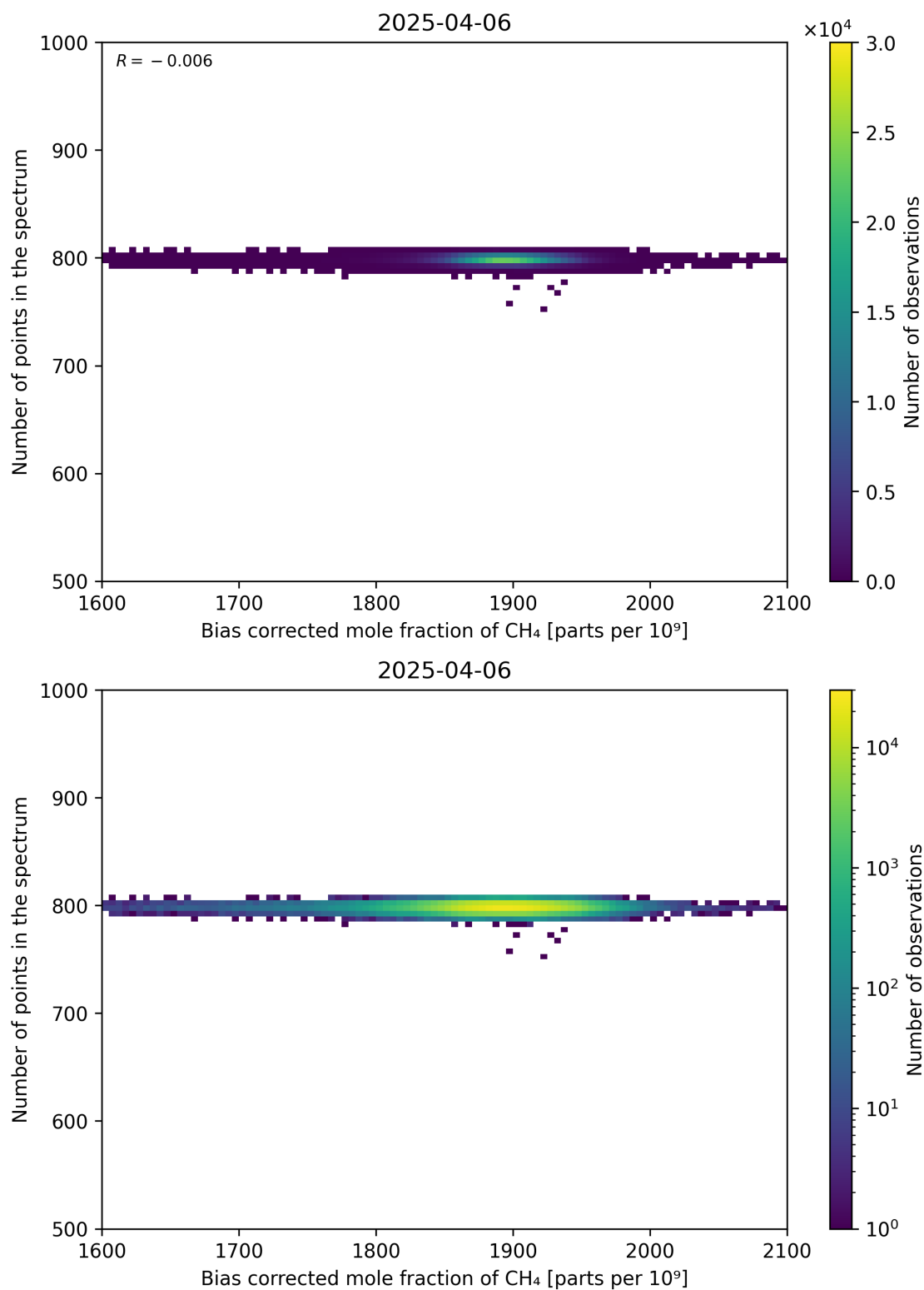
Figure 68: Scatter density plot of “Bias corrected mole fraction of CH 4 ” against “Number of points in the spectrum” for 2025-04-05 to 2025-04-07.
