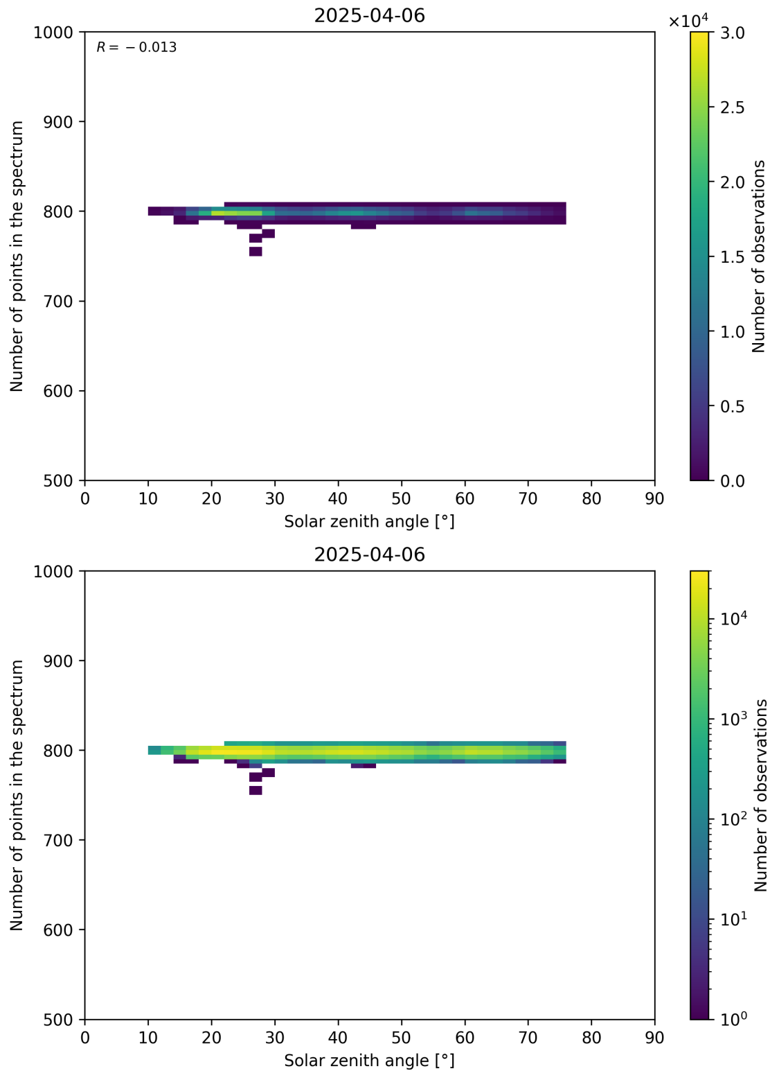
Figure 103: Scatter density plot of “Solar zenith angle” against “Number of points in the spectrum” for 2025-04-05 to 2025-04-07.
