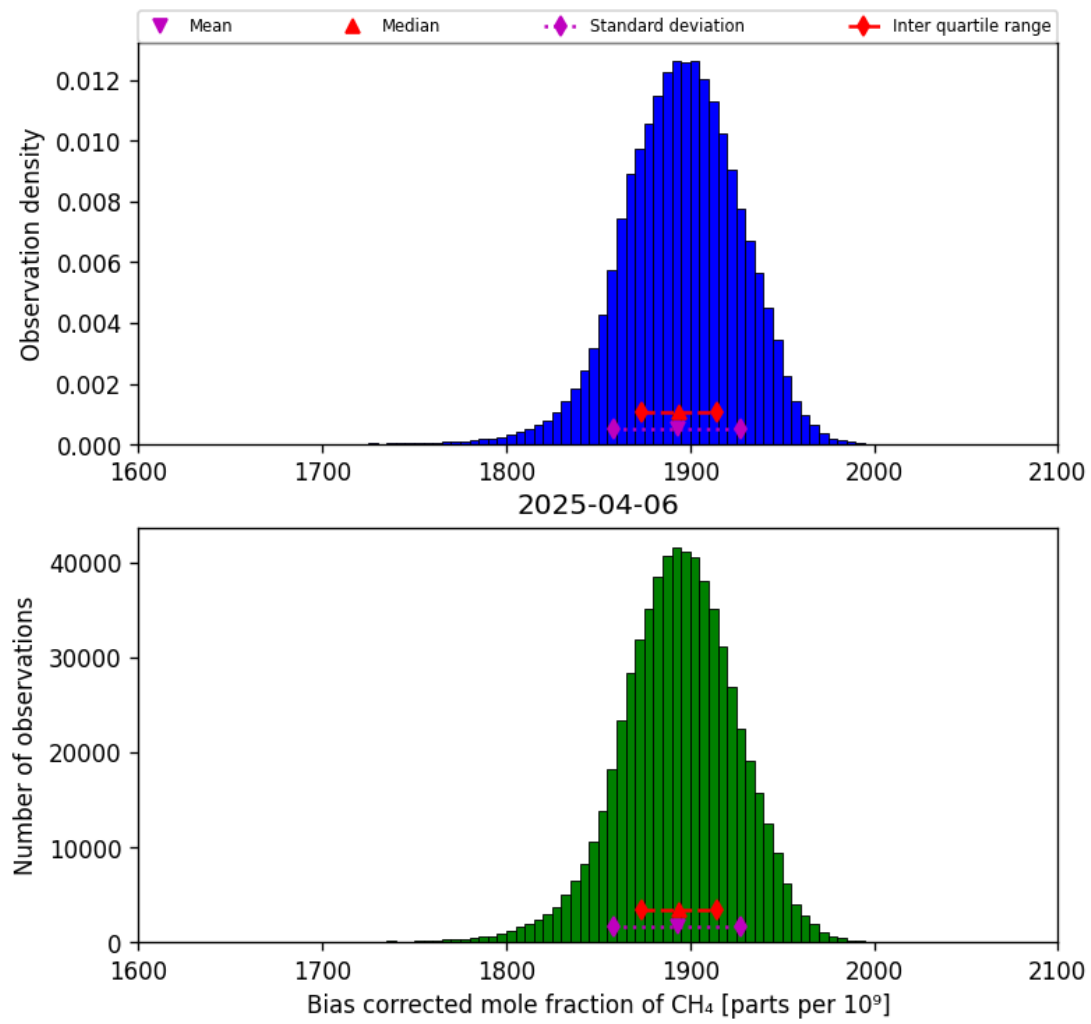
Figure 25: Histogram of “Bias corrected mole fraction of CH 4 ” for 2025-04-05 to 2025-04-07
