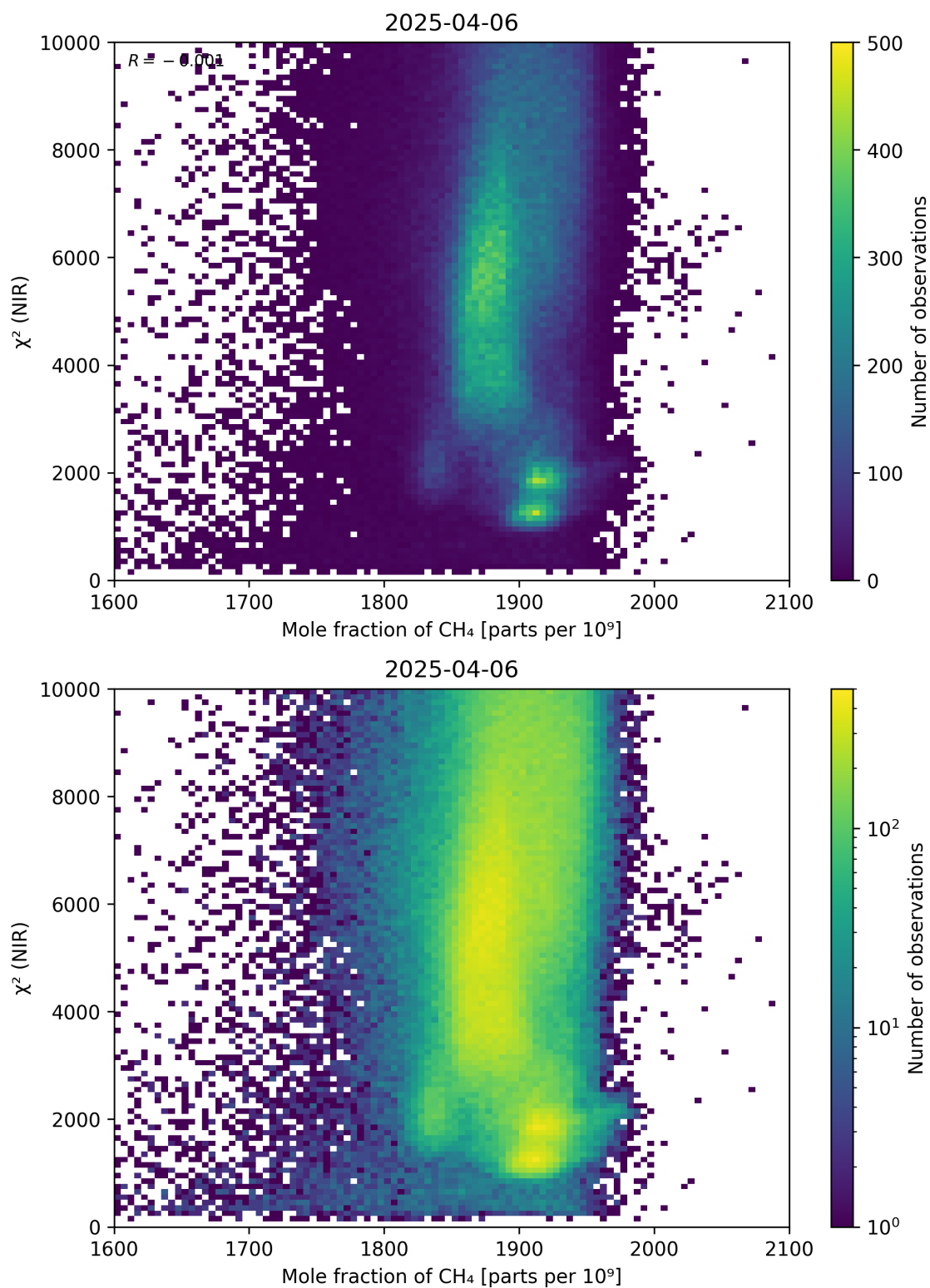
Figure 70: Scatter density plot of “Mole fraction of CH 4 ” against “ \chi^2 (NIR)” for 2025-04-05 to 2025-04-07.
