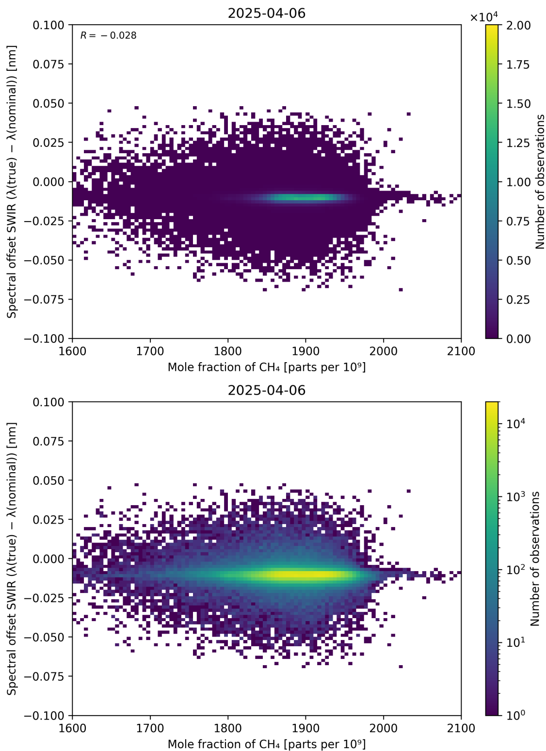
Figure 86: Scatter density plot of “Mole fraction of \text{CH}_4 ” against “Spectral offset SWIR ( \lambda_{\text{true}} - \lambda_{\text{nominal}} )” for 2025-04-05 to 2025-04-07.
