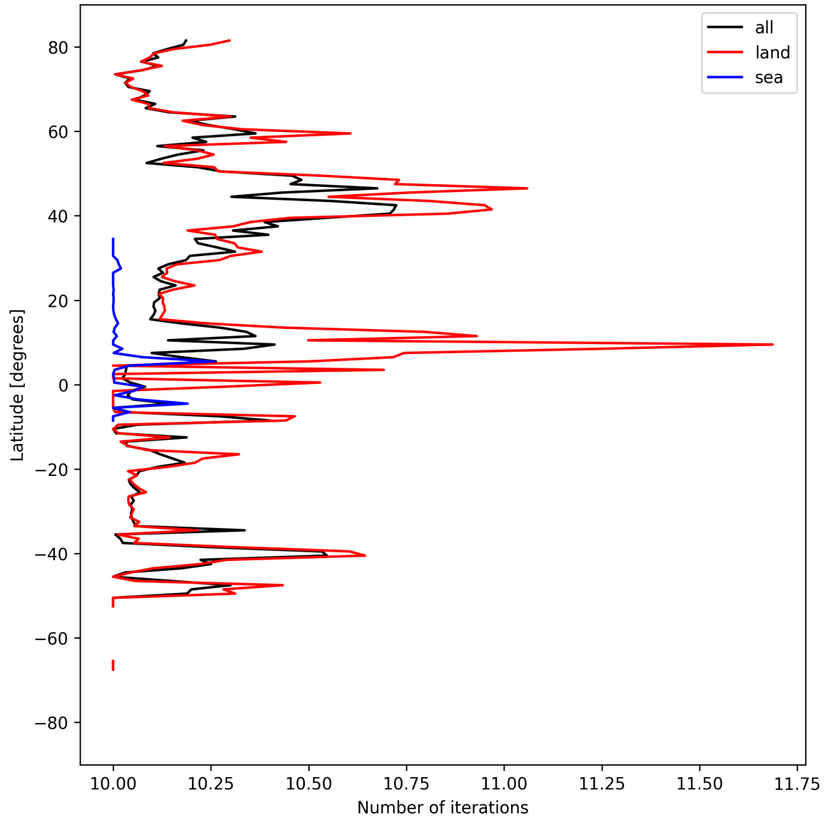
Figure 20: Zonal average of “Number of iterations” for 2025-04-05 to 2025-04-07.
