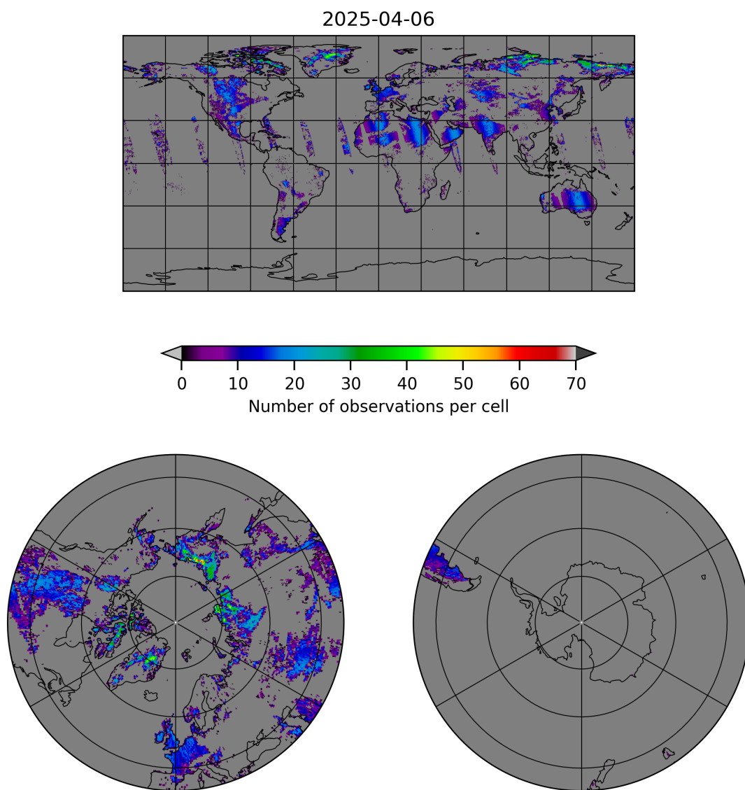
Figure 10: Map of the number of observations for 2025-04-05 to 2025-04-07
