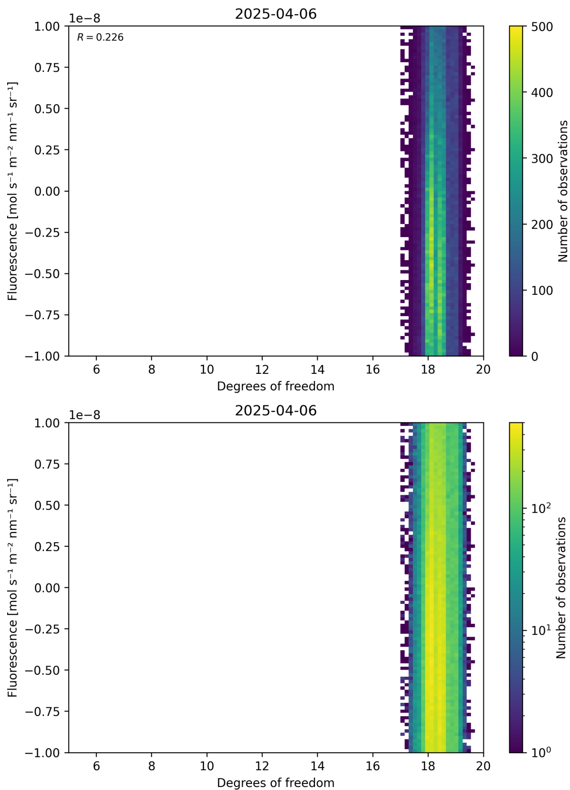
Figure 51: Scatter density plot of “Degrees of freedom” against “Fluorescence” for 2025-04-05 to 2025-04-07.
