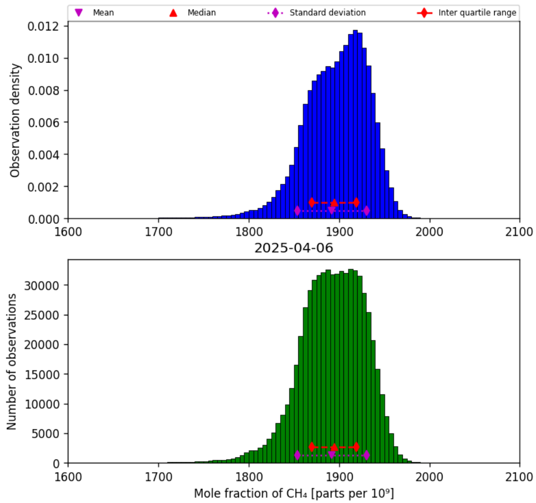
Figure 23: Histogram of “Mole fraction of CH 4 ” for 2025-04-05 to 2025-04-07
