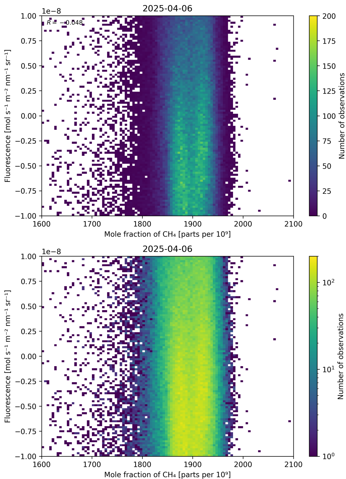
Figure 73: Scatter density plot of “Mole fraction of \text{CH}_4 ” against “Fluorescence” for 2025-04-05 to 2025-04-07.
