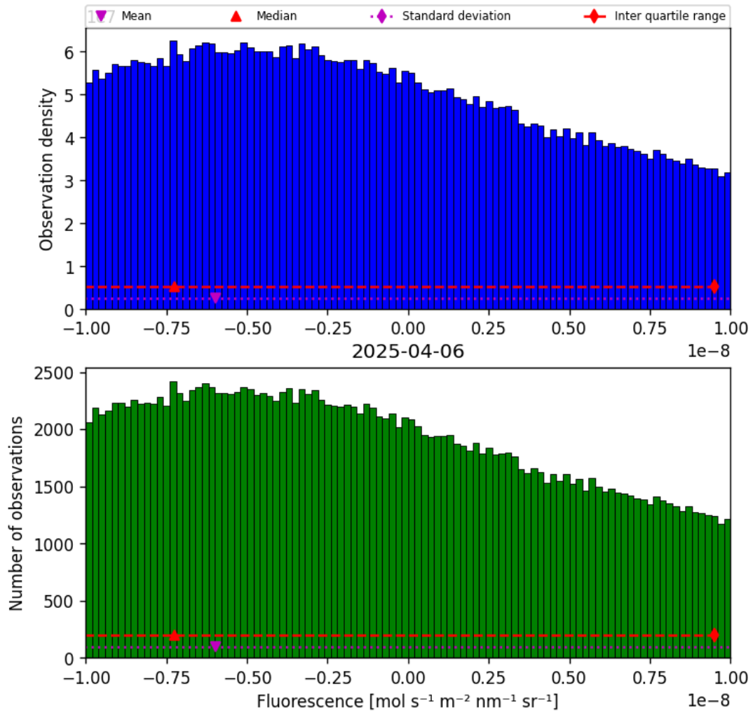
Figure 32: Histogram of “Fluorescence” for 2025-04-05 to 2025-04-07
