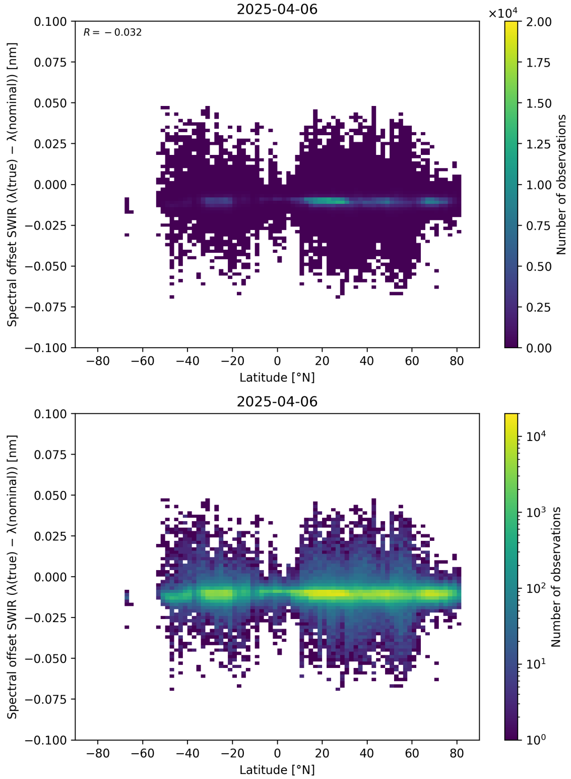
Figure 62: Scatter density plot of “Latitude” against “Spectral offset SWIR ( \lambda_{\text{true}} - \lambda_{\text{nominal}} )” for 2025-04-05 to 2025-04-07.
