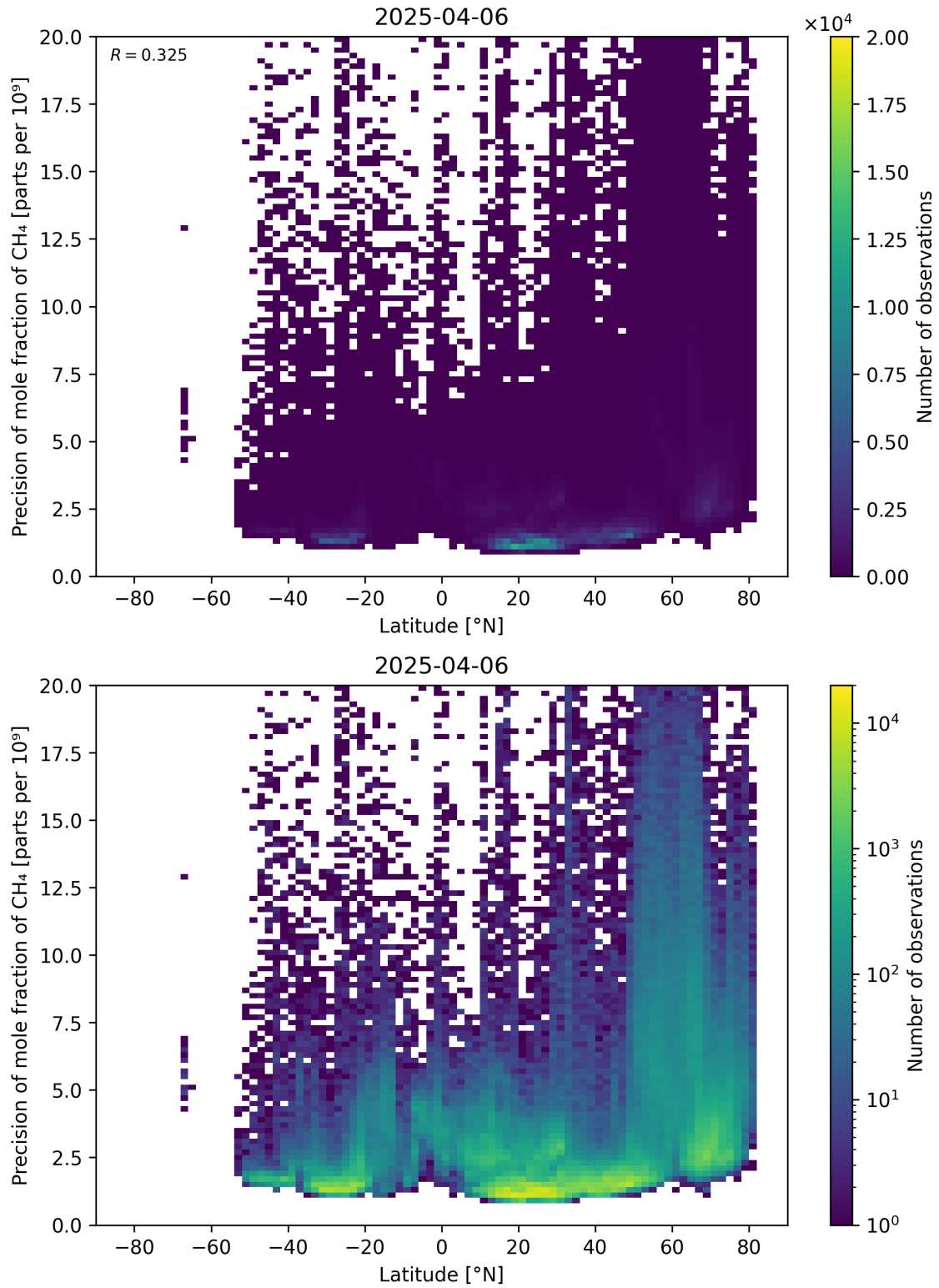
Figure 59: Scatter density plot of “Latitude” against “Precision of mole fraction of \text{CH}_4 ” for 2025-04-05 to 2025-04-07.
