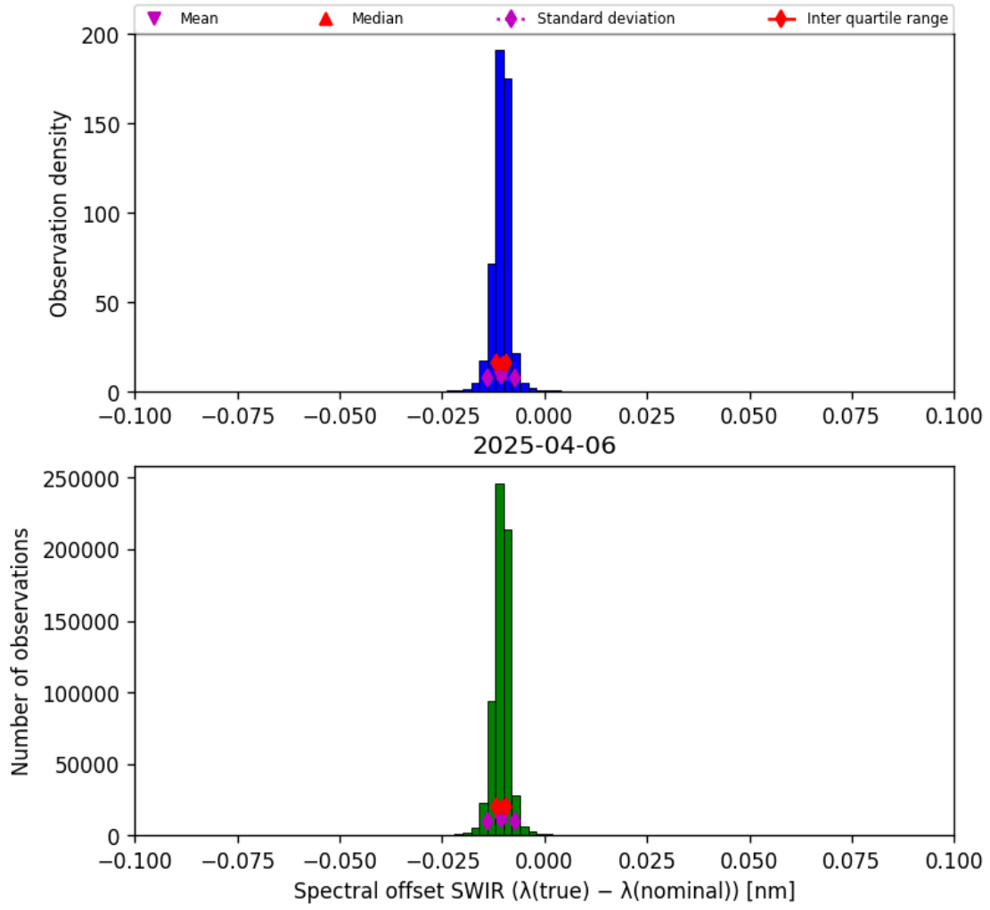
Figure 27: Histogram of “Spectral offset SWIR ( \lambda_{\text{true}} - \lambda_{\text{nominal}} )” for 2025-04-05 to 2025-04-07
