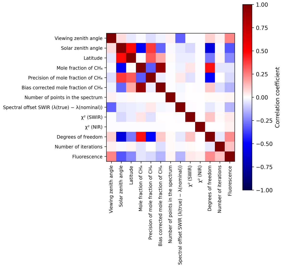
Figure 2: Map of correlation matrix for 2025-04-05 to 2025-04-07.
