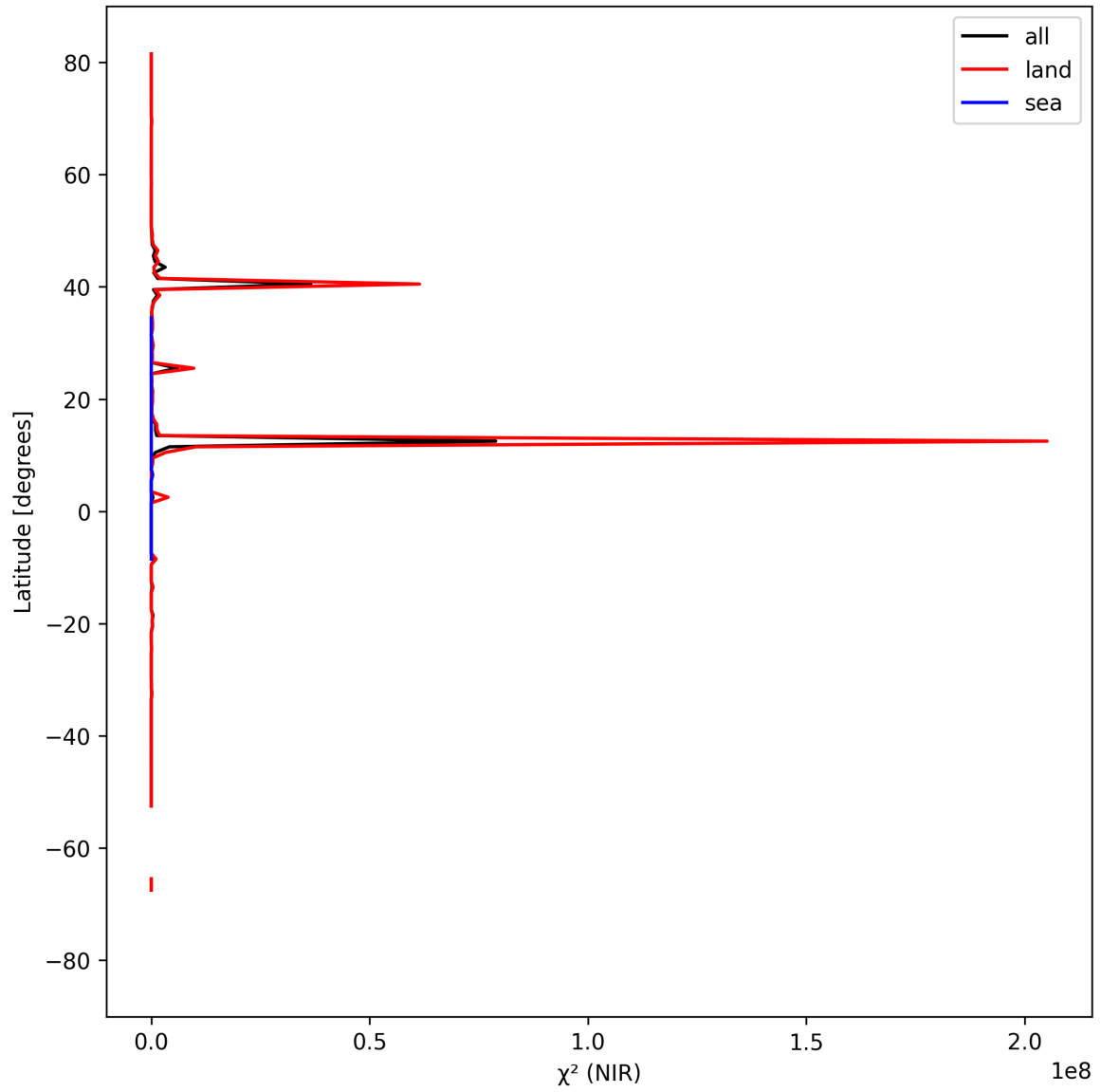
Figure 18: Zonal average of “ \chi^2 (NIR)” for 2025-04-05 to 2025-04-07.
