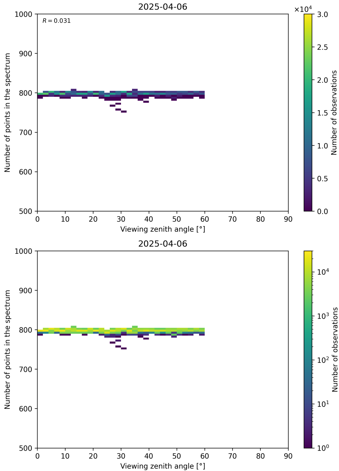
Figure 114: Scatter density plot of “Viewing zenith angle” against “Number of points in the spectrum” for 2025-04-05 to 2025-04-07.
