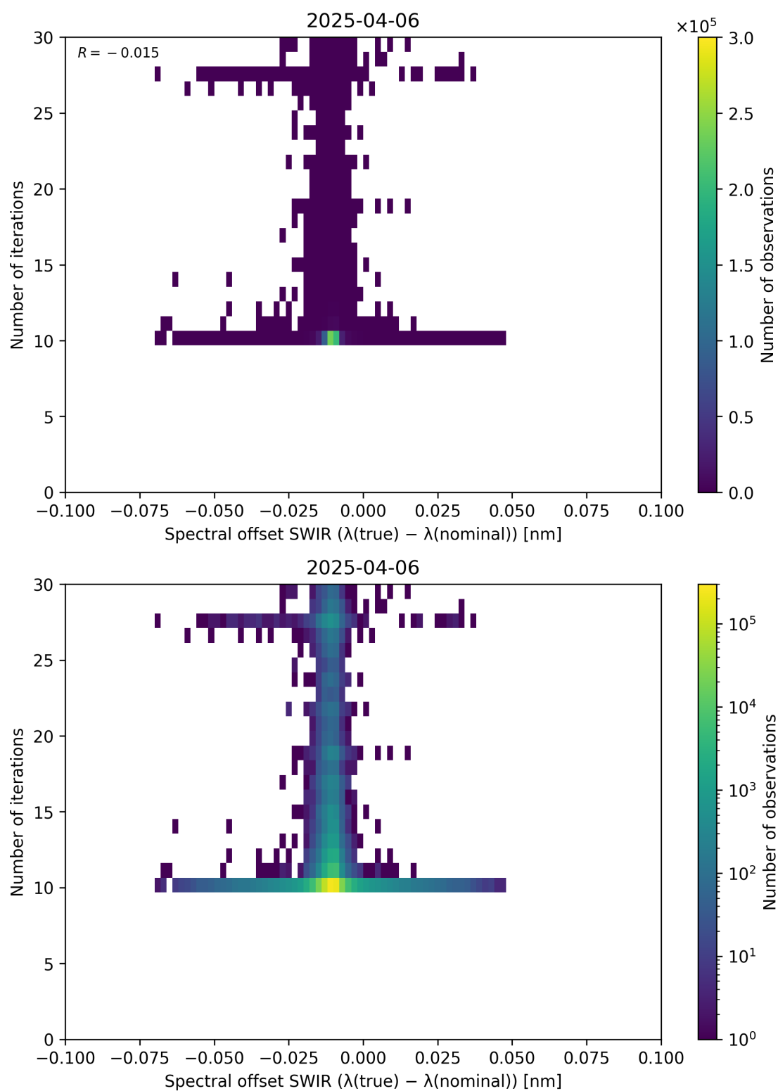
Figure 121: Scatter density plot of “Spectral offset SWIR ( \lambda_{\text{true}} - \lambda_{\text{nominal}} )” against “Number of iterations” for 2025-04-05 to 2025-04-07.
