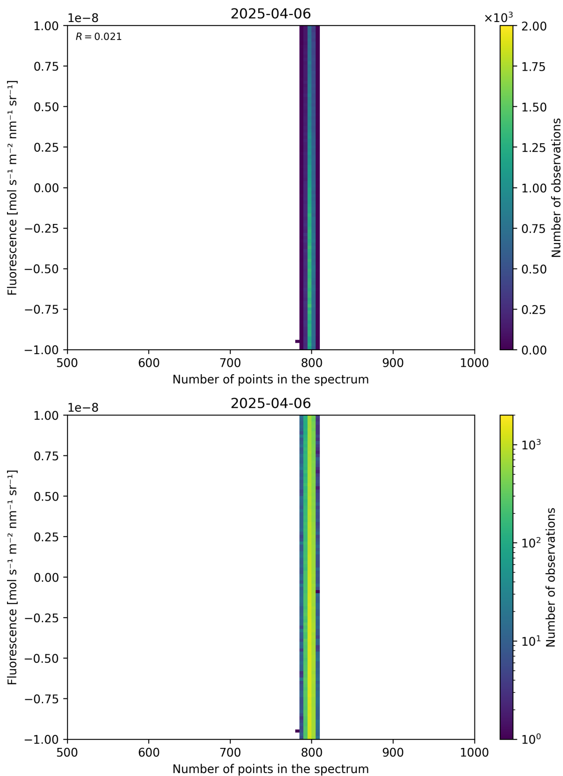
Figure 91: Scatter density plot of “Number of points in the spectrum” against “Fluorescence” for 2025-04-05 to 2025-04-07.
