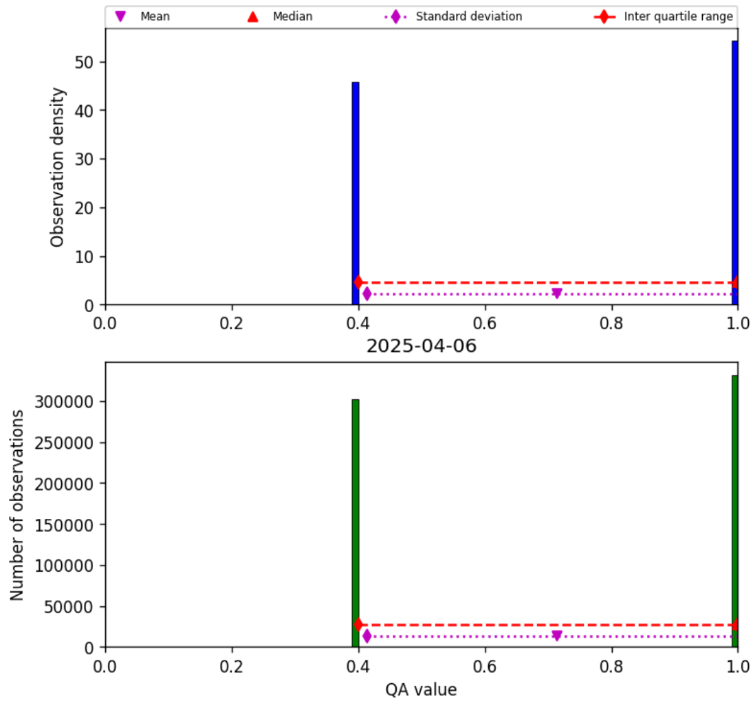
Figure 22: Histogram of “QA value” for 2025-04-05 to 2025-04-07
