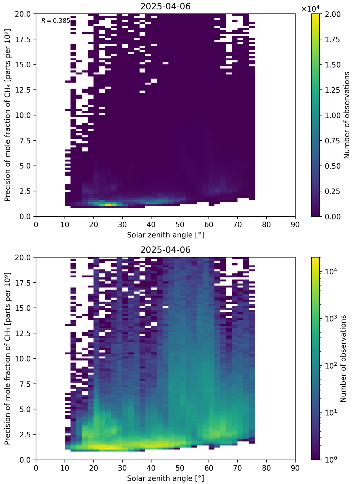
Figure 101: Scatter density plot of “Solar zenith angle” against “Precision of mole fraction of \text{CH}_4 ” for 2025-04-05 to 2025-04-07.
