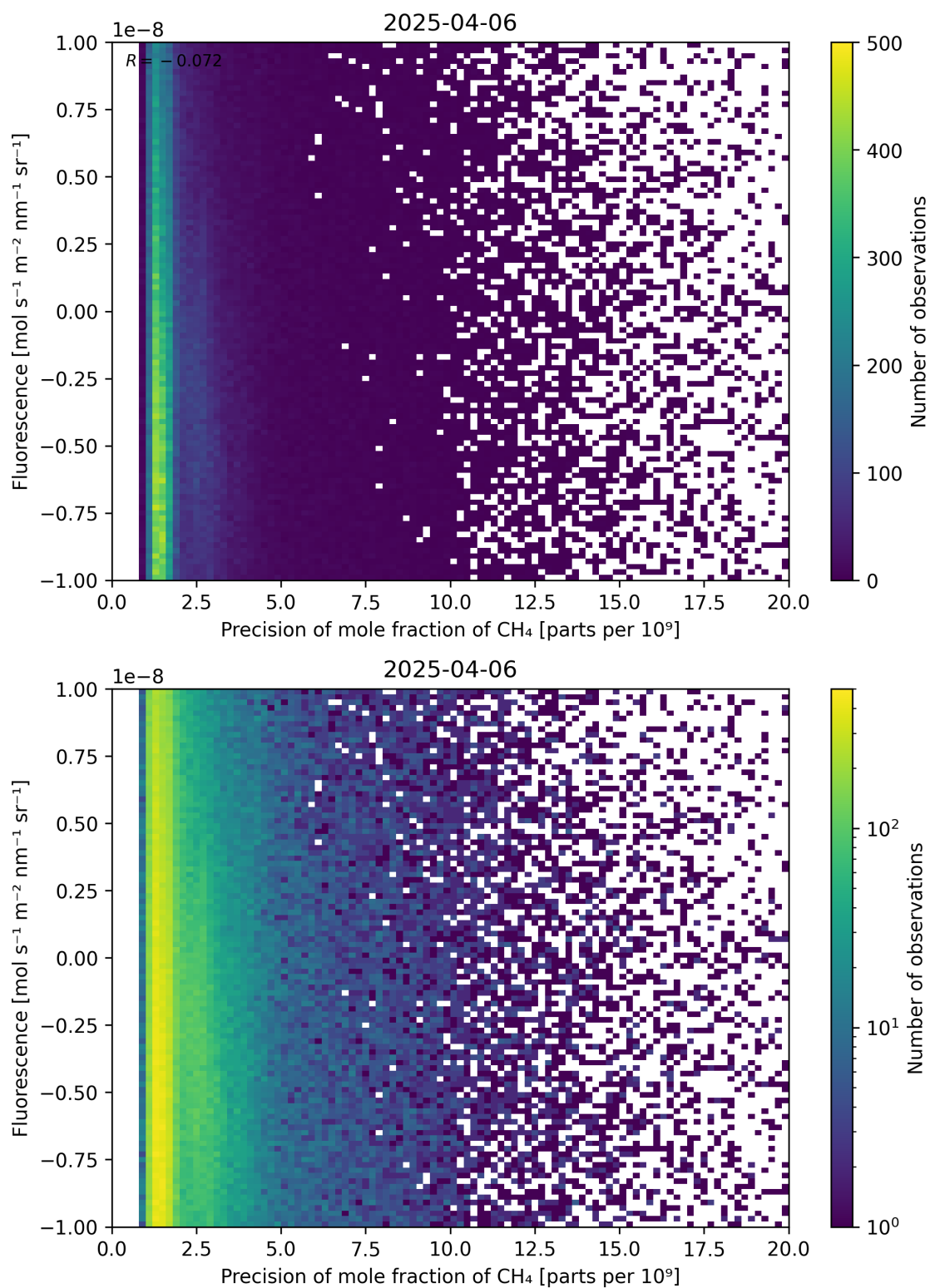
Figure 81: Scatter density plot of “Precision of mole fraction of CH 4 ” against “Fluorescence” for 2025-04-05 to 2025-04-07.
