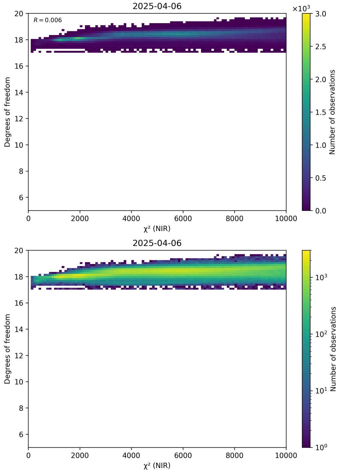
Figure 44: Scatter density plot of “ \chi^2 (NIR)” against “Degrees of freedom” for 2025-04-05 to 2025-04-07.
