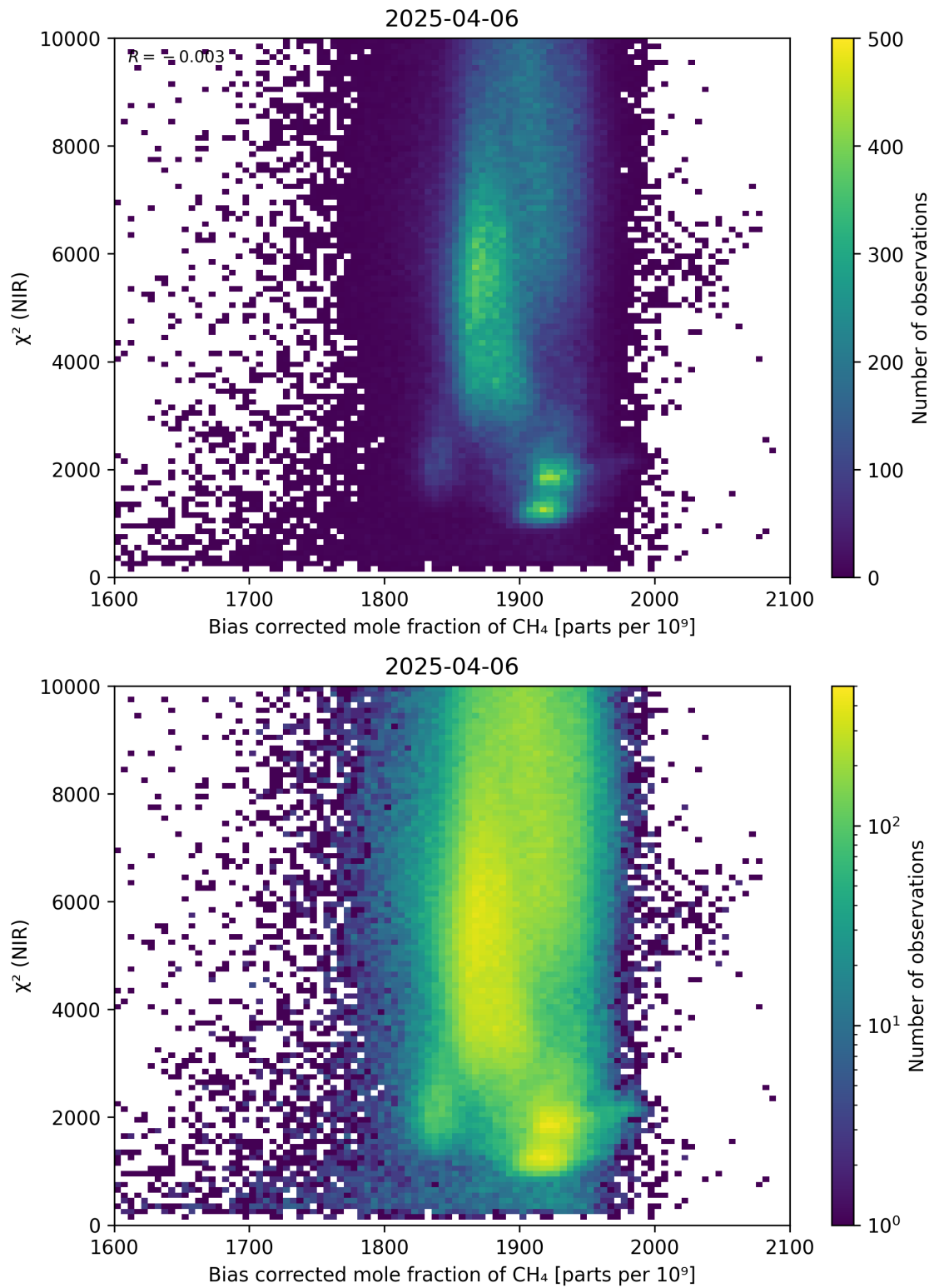
Figure 63: Scatter density plot of “Bias corrected mole fraction of CH 4 ” against “ \chi^2 (NIR)” for 2025-04-05 to 2025-04-07.
