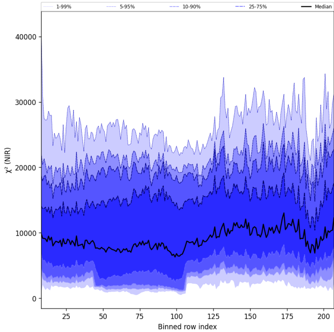
Figure 40: Along track statistics of “ \chi^2 (NIR)” for 2025-04-05 to 2025-04-07
