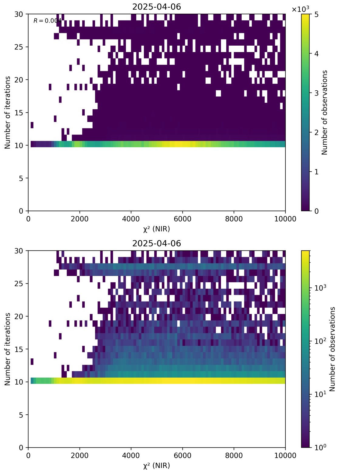
Figure 46: Scatter density plot of “ \chi^2 (NIR)” against “Number of iterations” for 2025-04-05 to 2025-04-07.
