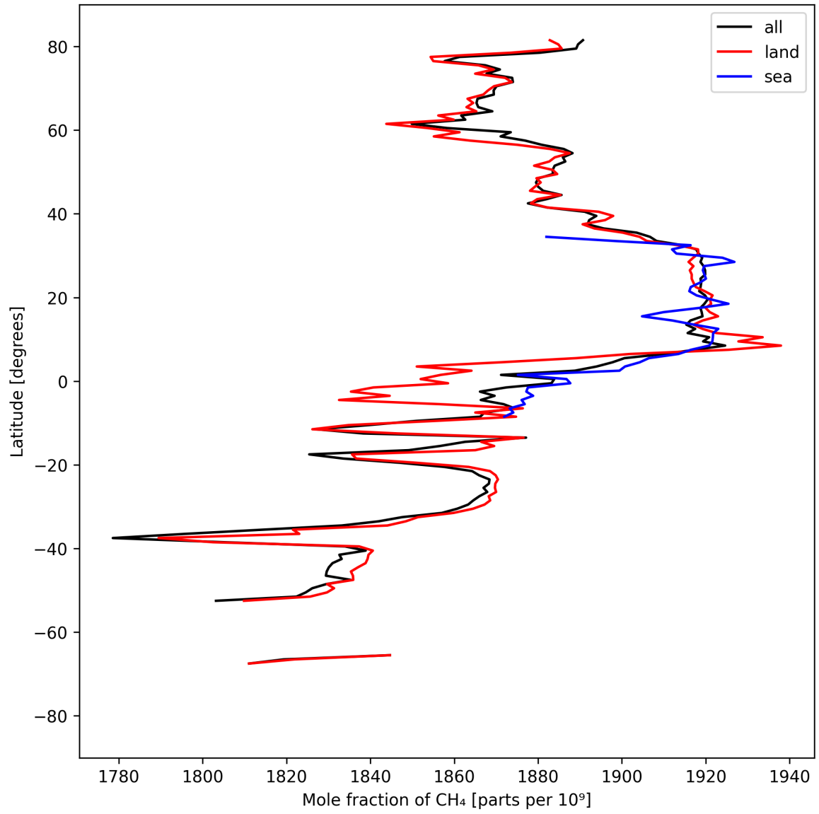
Figure 12: Zonal average of “Mole fraction of \text{CH}_4 ” for 2025-04-05 to 2025-04-07.
