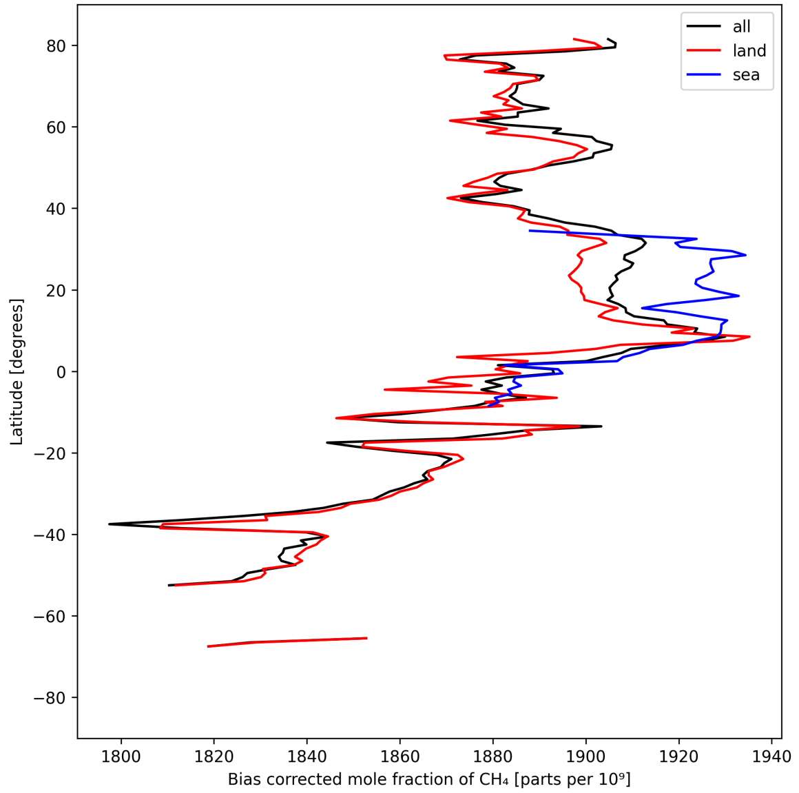
Figure 14: Zonal average of “Bias corrected mole fraction of CH 4 ” for 2025-04-05 to 2025-04-07.
