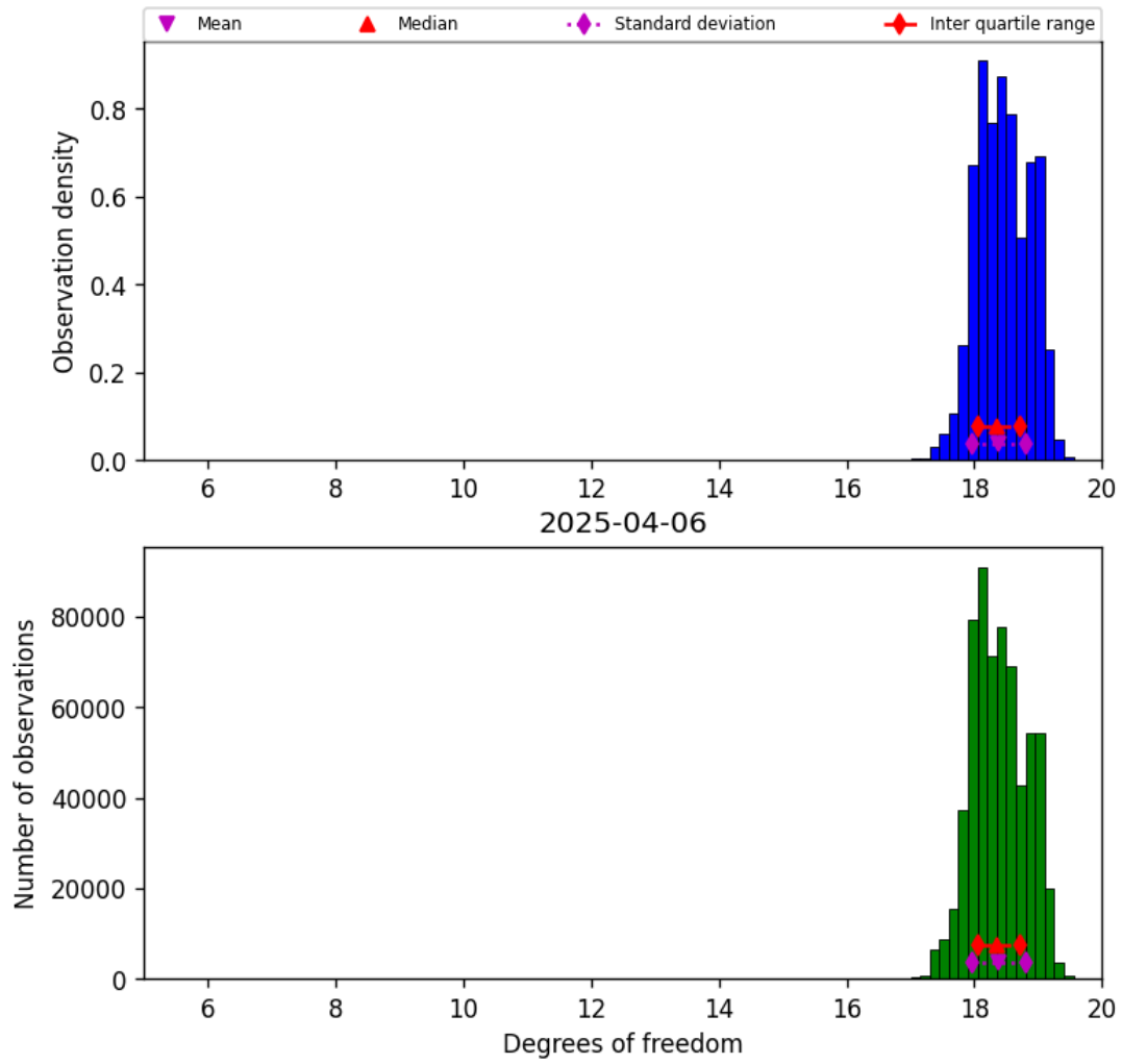
Figure 30: Histogram of “Degrees of freedom” for 2025-04-05 to 2025-04-07
