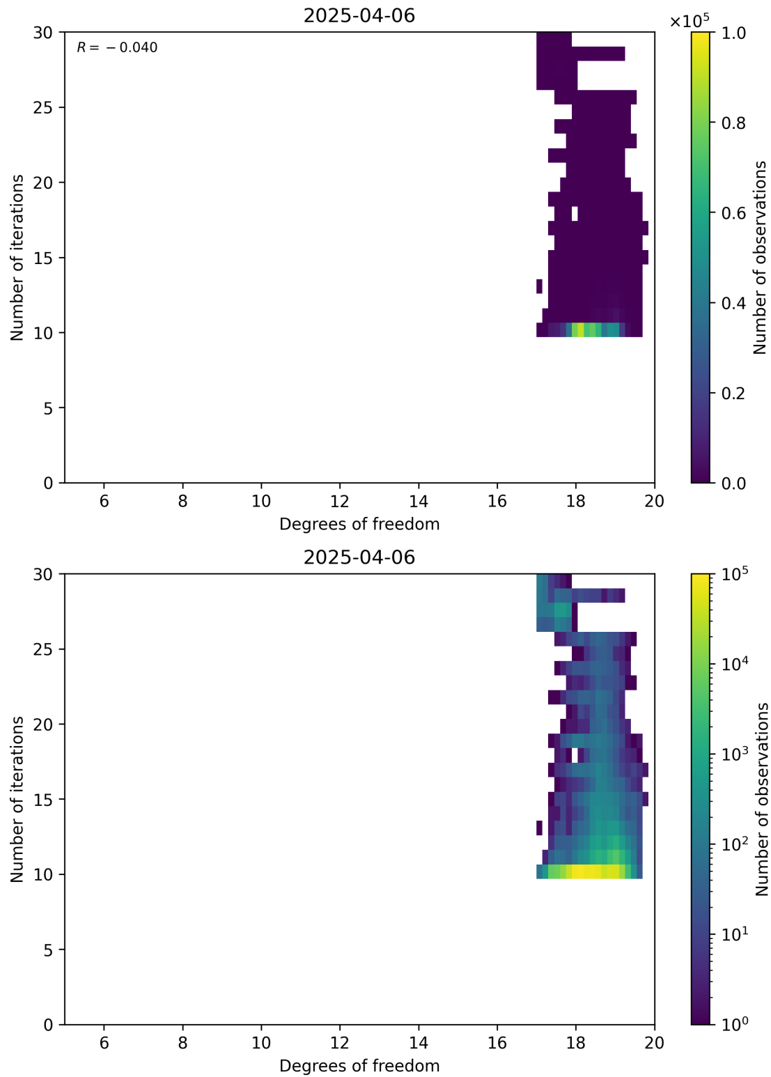
Figure 52: Scatter density plot of “Degrees of freedom” against “Number of iterations” for 2025-04-05 to 2025-04-07.
