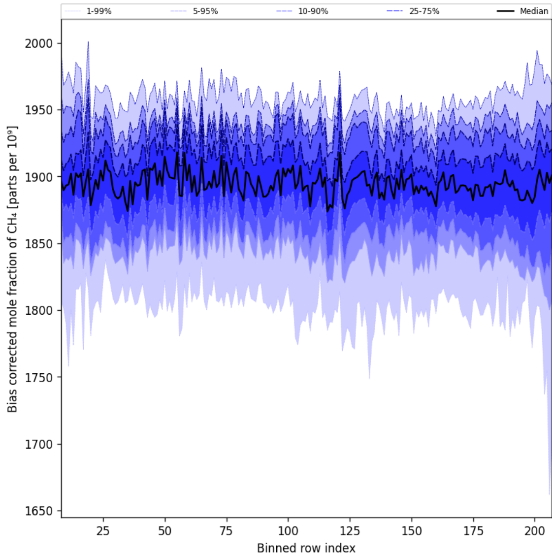
Figure 36: Along track statistics of “Bias corrected mole fraction of CH 4 ” for 2025-04-05 to 2025-04-07
