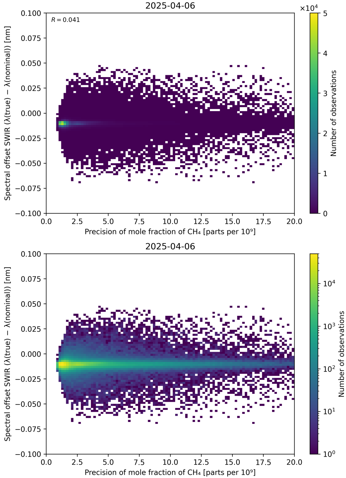
Figure 85: Scatter density plot of “Precision of mole fraction of CH 4 ” against “Spectral offset SWIR ( \lambda_{\text{true}} - \lambda_{\text{nominal}} )” for 2025-04-05 to 2025-04-07.
