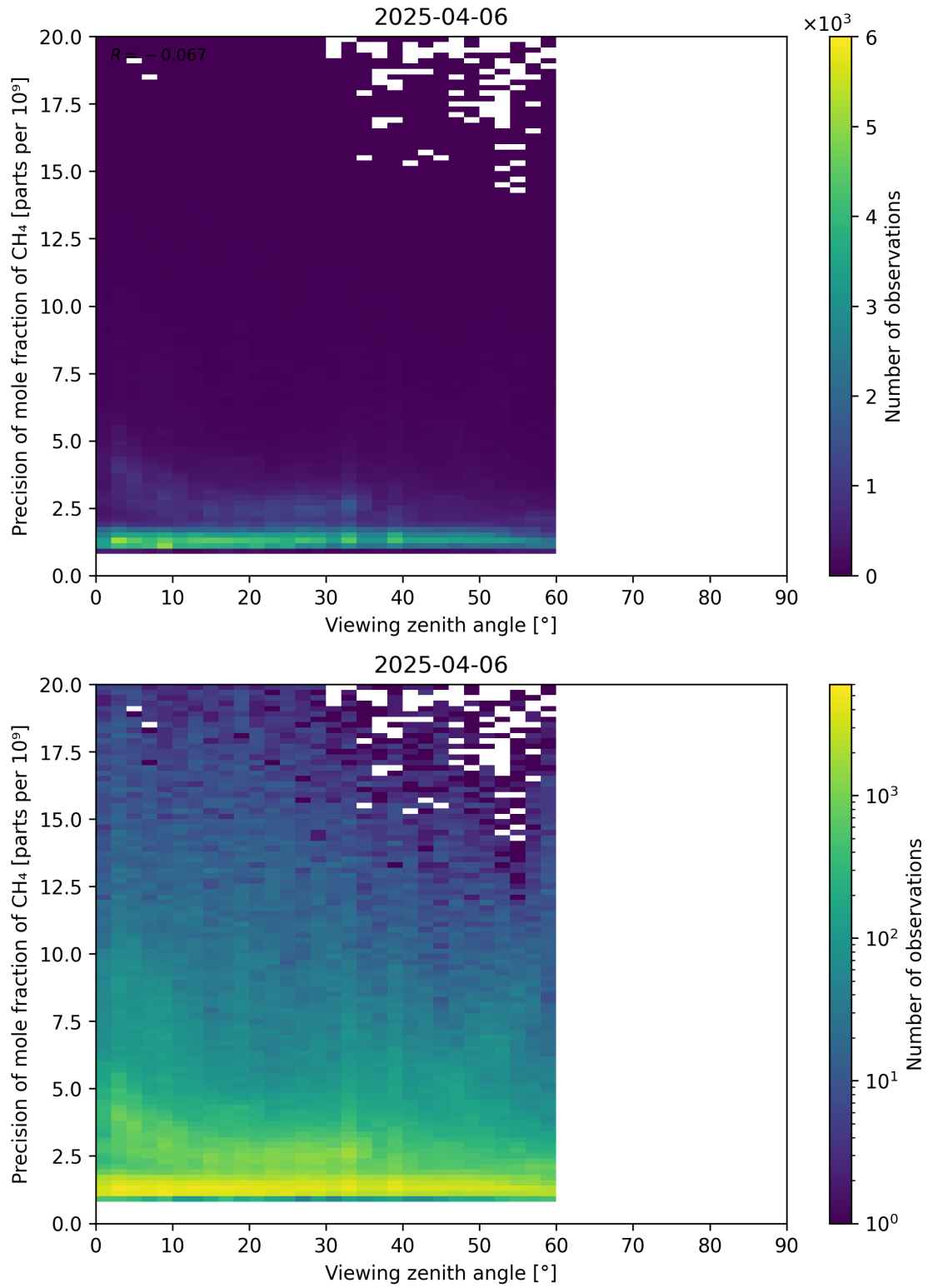
Figure 112: Scatter density plot of “Viewing zenith angle” against “Precision of mole fraction of CH 4 ” for 2025-04-05 to 2025-04-07.
