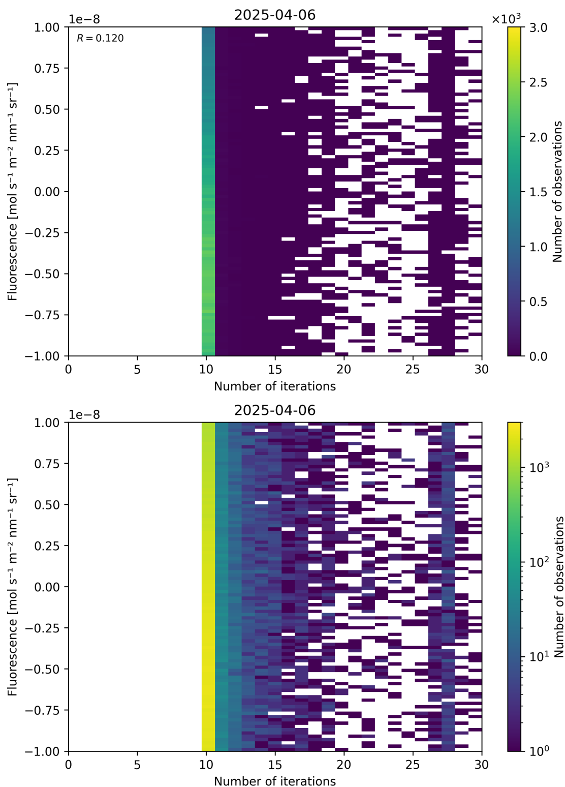
Figure 87: Scatter density plot of “Number of iterations” against “Fluorescence” for 2025-04-05 to 2025-04-07.
