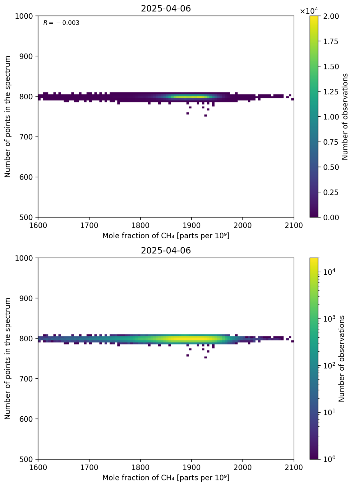
Figure 77: Scatter density plot of “Mole fraction of CH 4 ” against “Number of points in the spectrum” for 2025-04-05 to 2025-04-07.
