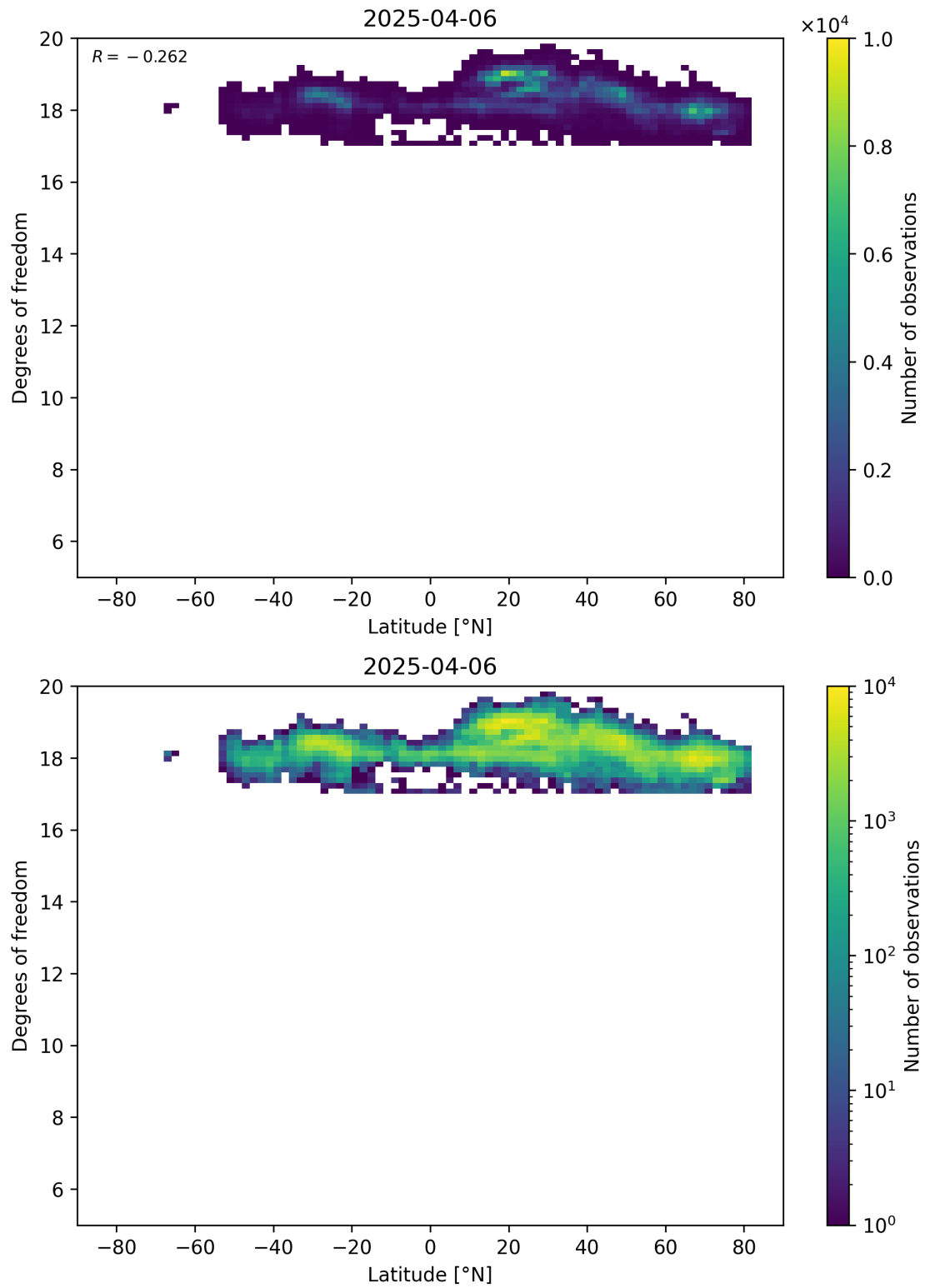
Figure 55: Scatter density plot of “Latitude” against “Degrees of freedom” for 2025-04-05 to 2025-04-07.
