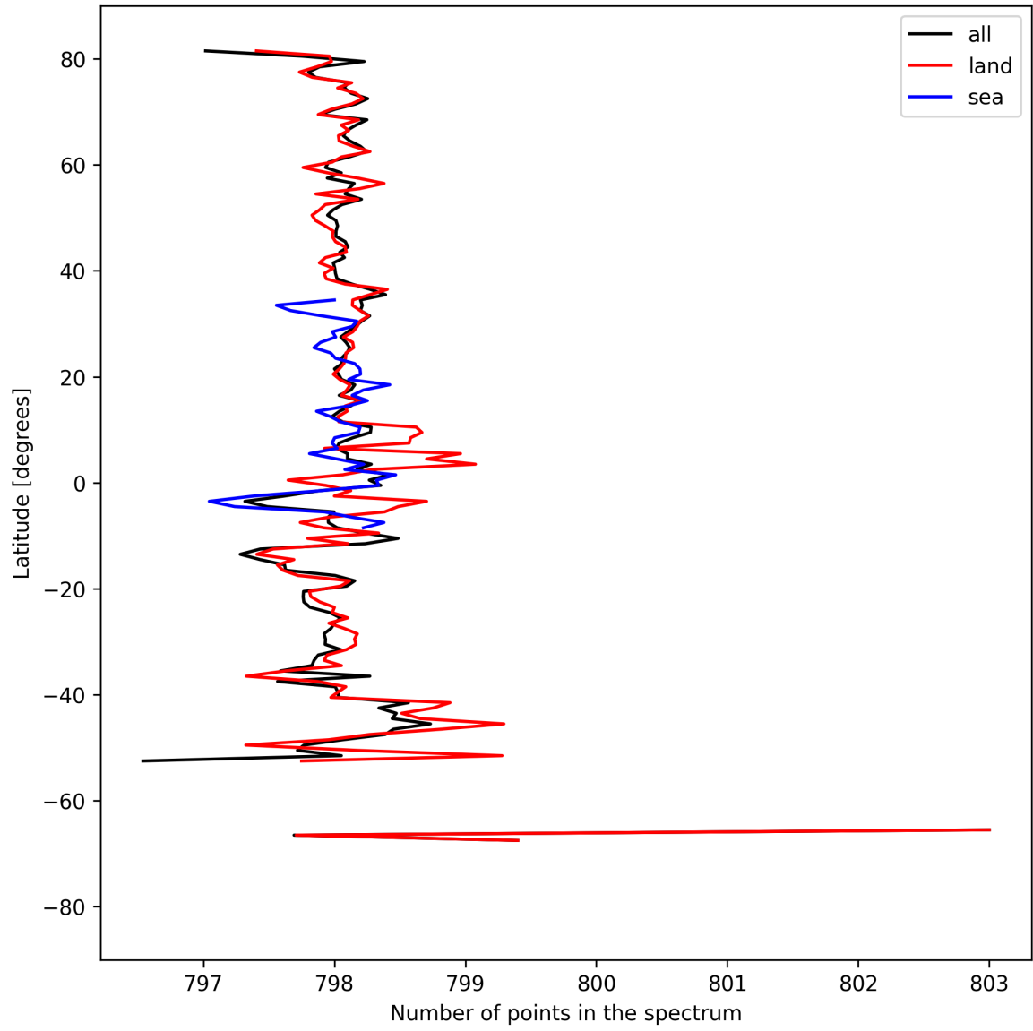
Figure 15: Zonal average of “Number of points in the spectrum” for 2025-04-05 to 2025-04-07.
