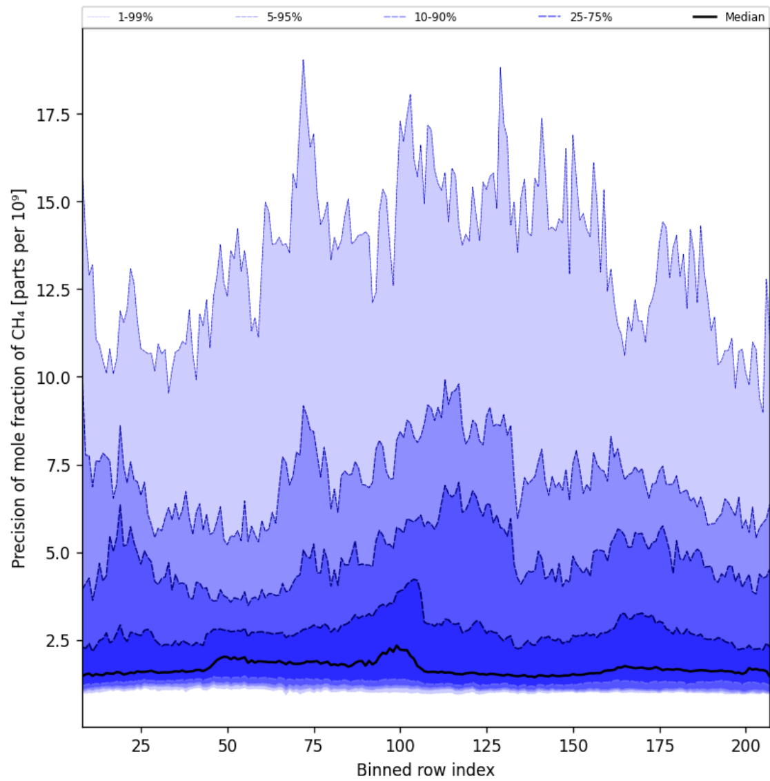
Figure 35: Along track statistics of “Precision of mole fraction of CH 4 ” for 2025-04-05 to 2025-04-07
