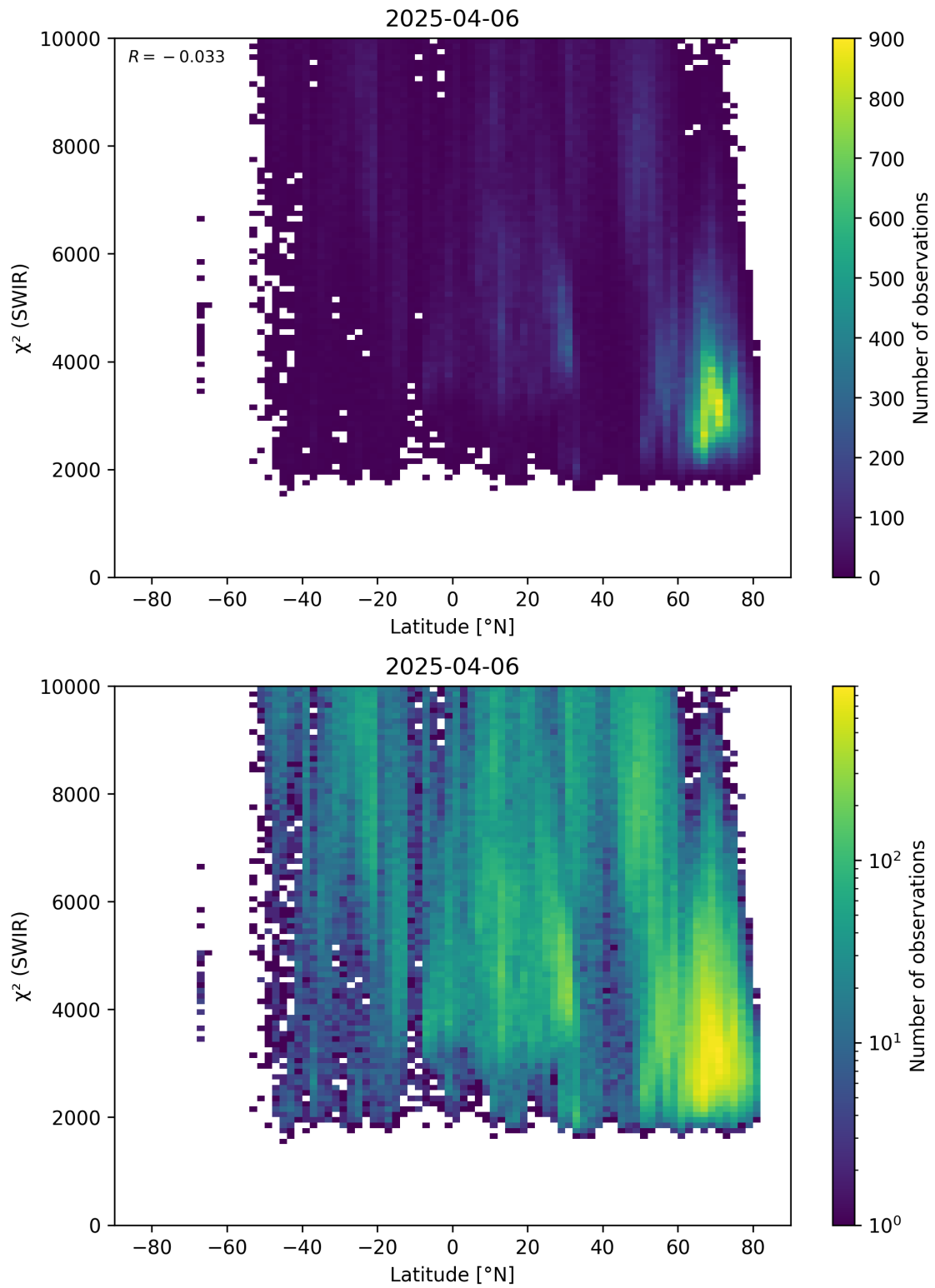
Figure 54: Scatter density plot of “Latitude” against “ \chi^2 (SWIR)” for 2025-04-05 to 2025-04-07.
