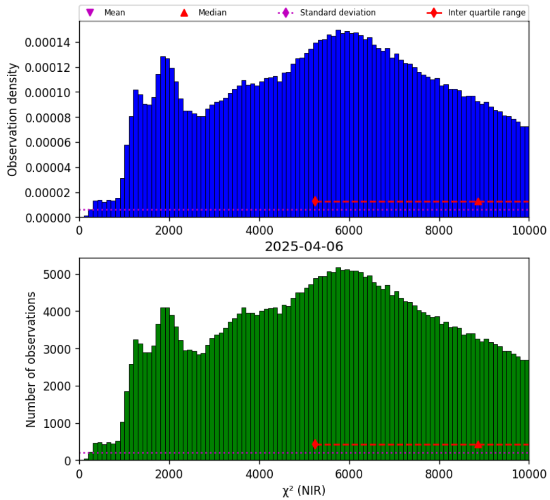
Figure 29: Histogram of " \chi^2 (NIR)" for 2025-04-05 to 2025-04-07
