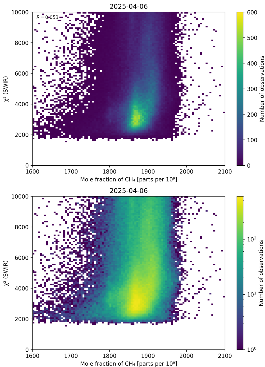
Figure 71: Scatter density plot of “Mole fraction of \text{CH}_4 ” against “ \chi^2 (SWIR)” for 2025-04-05 to 2025-04-07.
