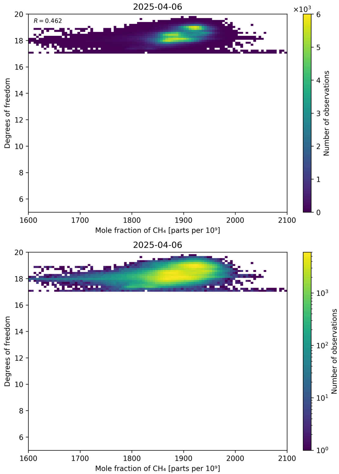
Figure 72: Scatter density plot of “Mole fraction of CH 4 ” against “Degrees of freedom” for 2025-04-05 to 2025-04-07.
