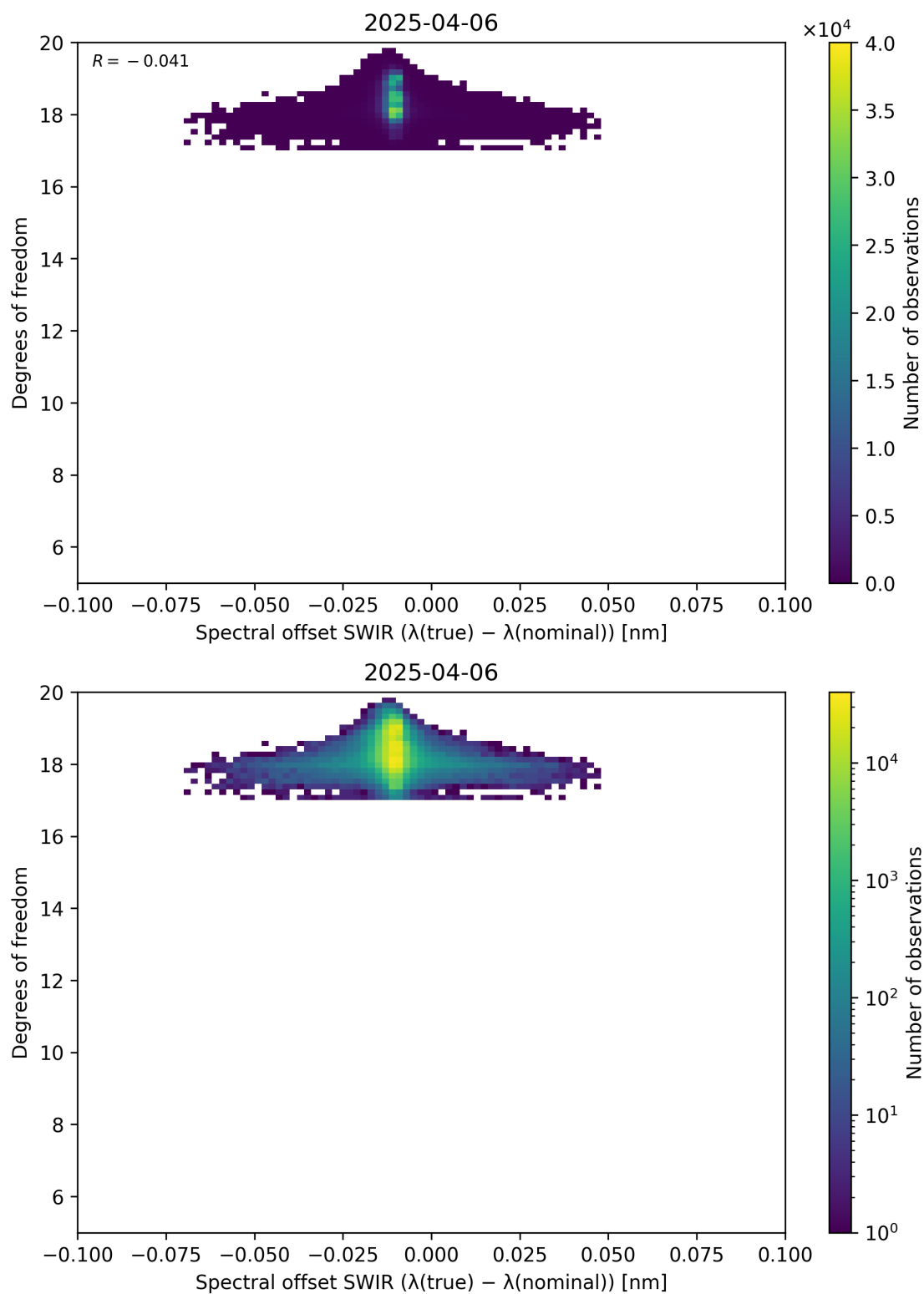
Figure 119: Scatter density plot of “Spectral offset SWIR ( \lambda_{\text{true}} - \lambda_{\text{nominal}} )” against “Degrees of freedom” for 2025-04-05 to 2025-04-07.
