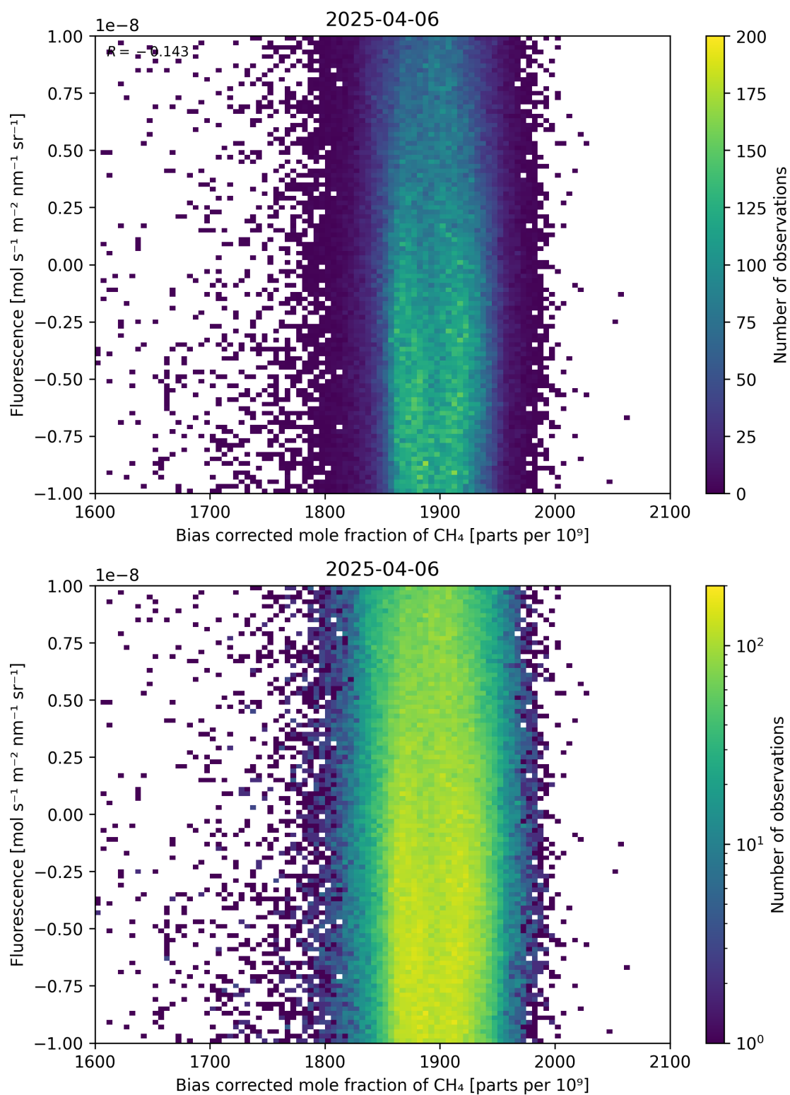
Figure 66: Scatter density plot of “Bias corrected mole fraction of \text{CH}_4 ” against “Fluorescence” for 2025-04-05 to 2025-04-07.
