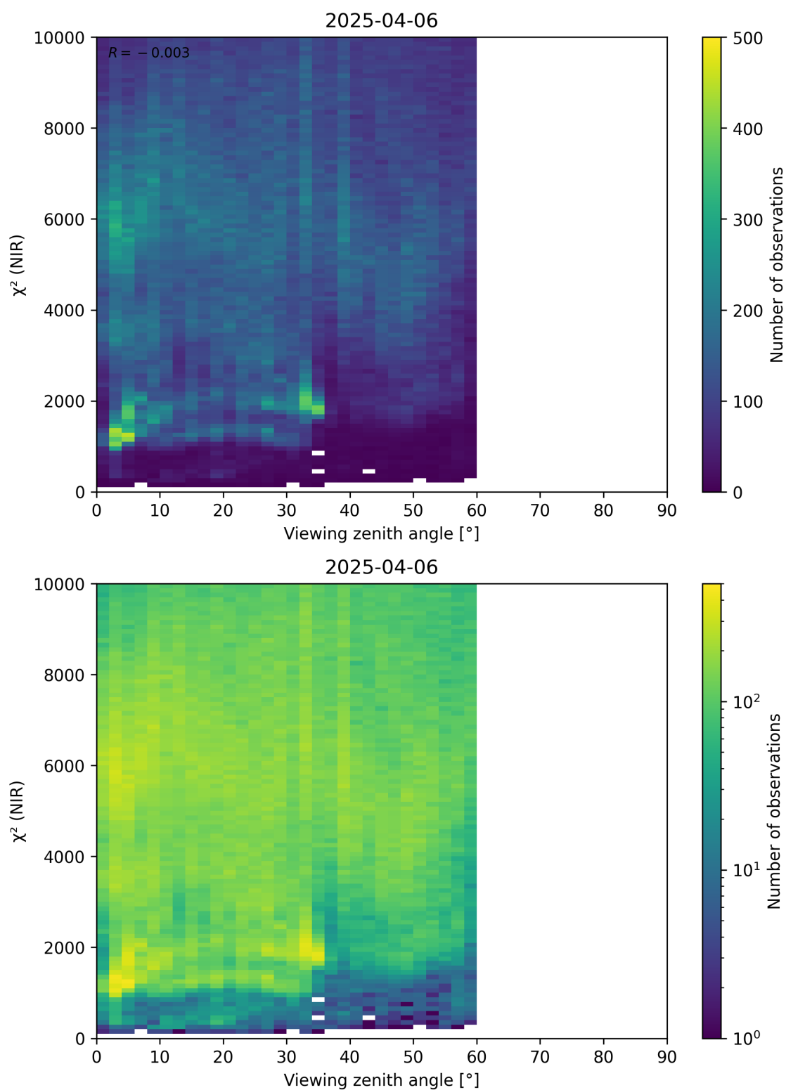
Figure 105: Scatter density plot of “Viewing zenith angle” against “ \chi^2 (NIR)” for 2025-04-05 to 2025-04-07.
