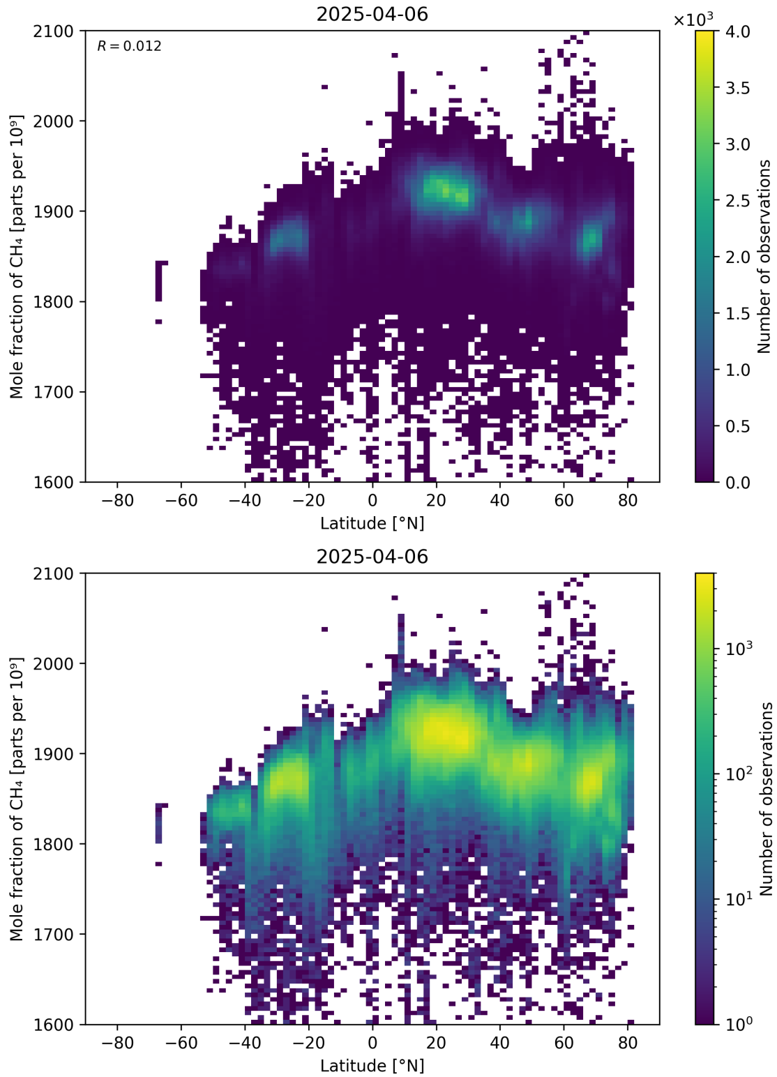
Figure 57: Scatter density plot of “Latitude” against “Mole fraction of \text{CH}_4 ” for 2025-04-05 to 2025-04-07.
