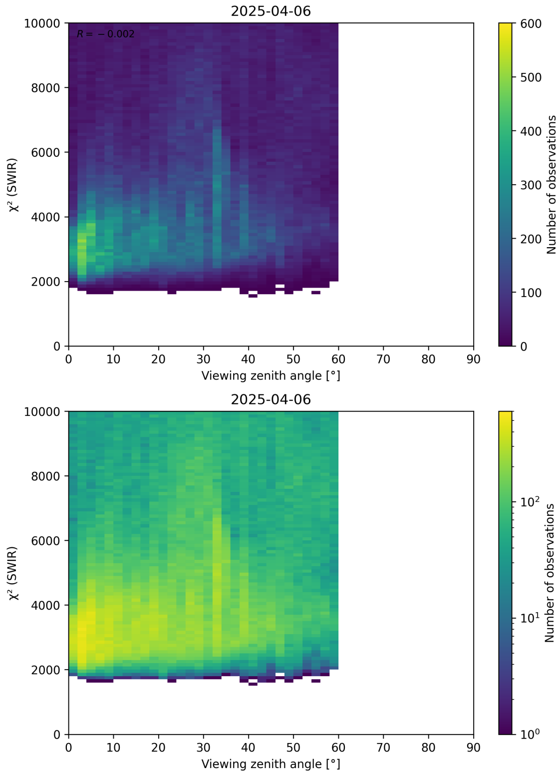
Figure 106: Scatter density plot of “Viewing zenith angle” against “ \chi^2 (SWIR)” for 2025-04-05 to 2025-04-07.
