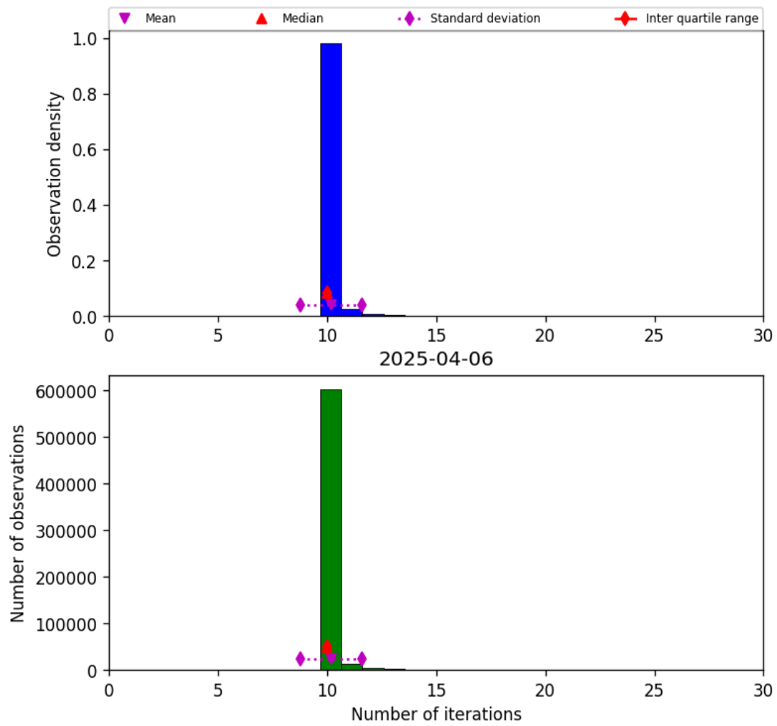
Figure 31: Histogram of “Number of iterations” for 2025-04-05 to 2025-04-07
