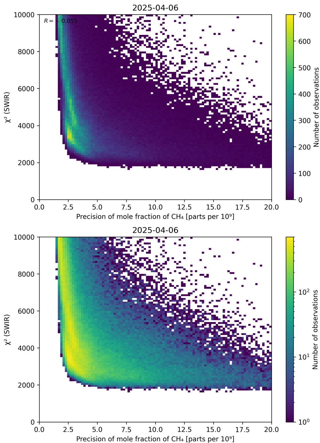
Figure 79: Scatter density plot of “Precision of mole fraction of CH 4 ” against “ \chi^2 (SWIR)” for 2025-04-05 to 2025-04-07.
