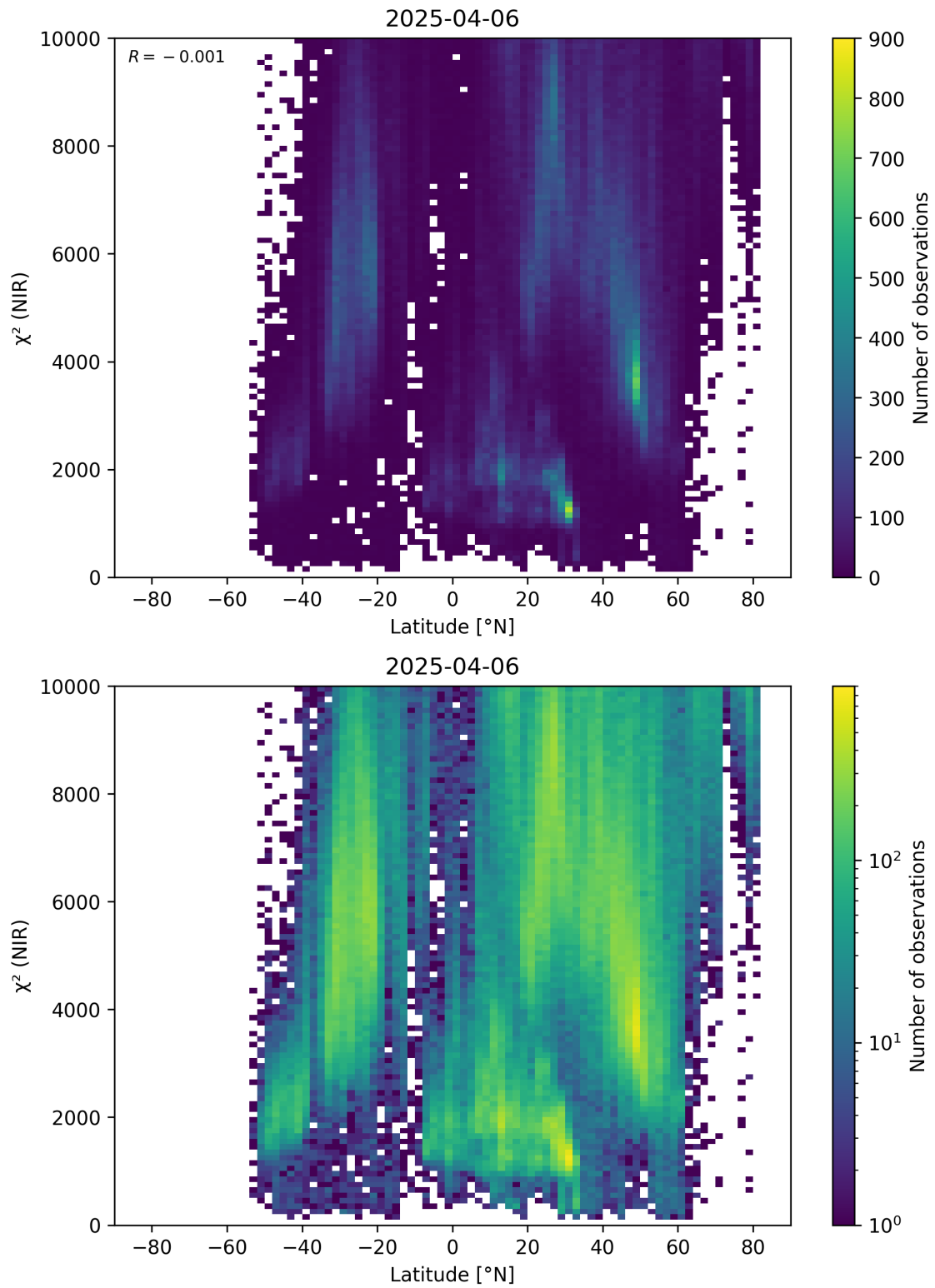
Figure 53: Scatter density plot of “Latitude” against “ \chi^2 (NIR)” for 2025-04-05 to 2025-04-07.
