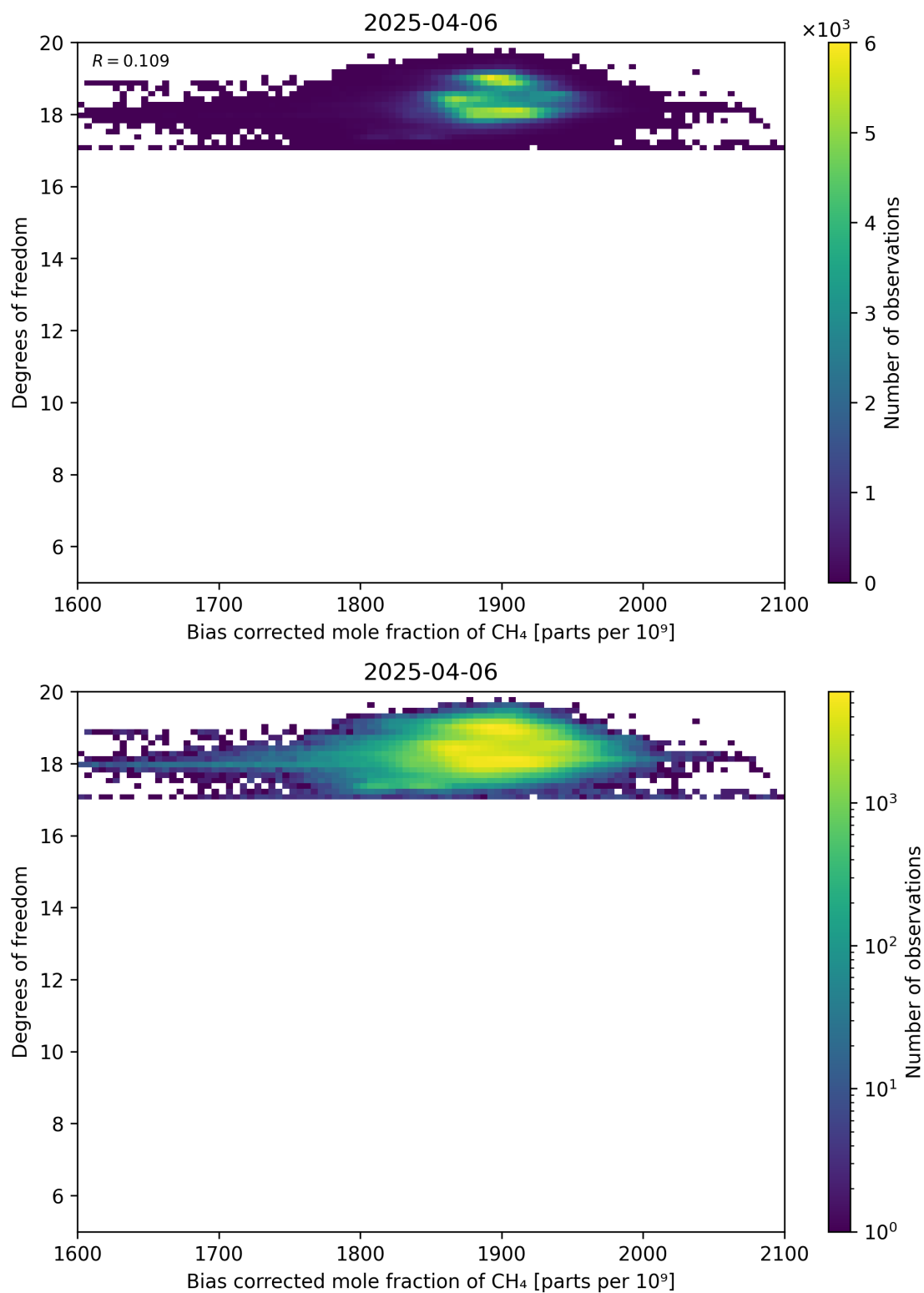
Figure 65: Scatter density plot of “Bias corrected mole fraction of CH 4 ” against “Degrees of freedom” for 2025-04-05 to 2025-04-07.
