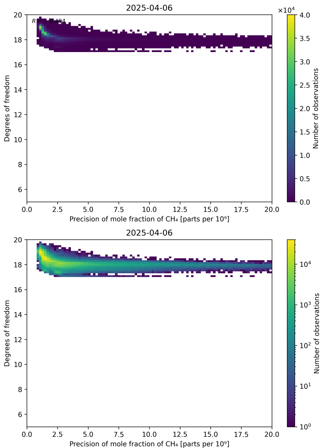
Figure 80: Scatter density plot of “Precision of mole fraction of CH 4 ” against “Degrees of freedom” for 2025-04-05 to 2025-04-07.
