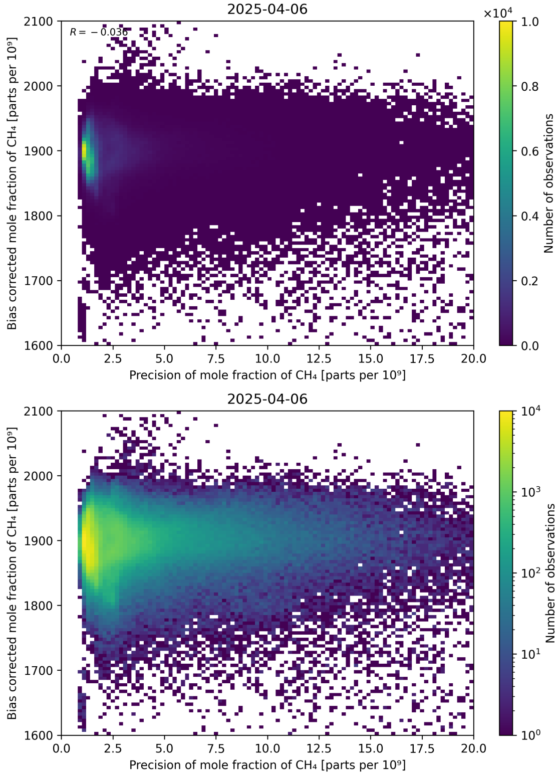
Figure 82: Scatter density plot of “Precision of mole fraction of CH 4 ” against “Bias corrected mole fraction of CH 4 ” for 2025-04-05 to 2025-04-07.
