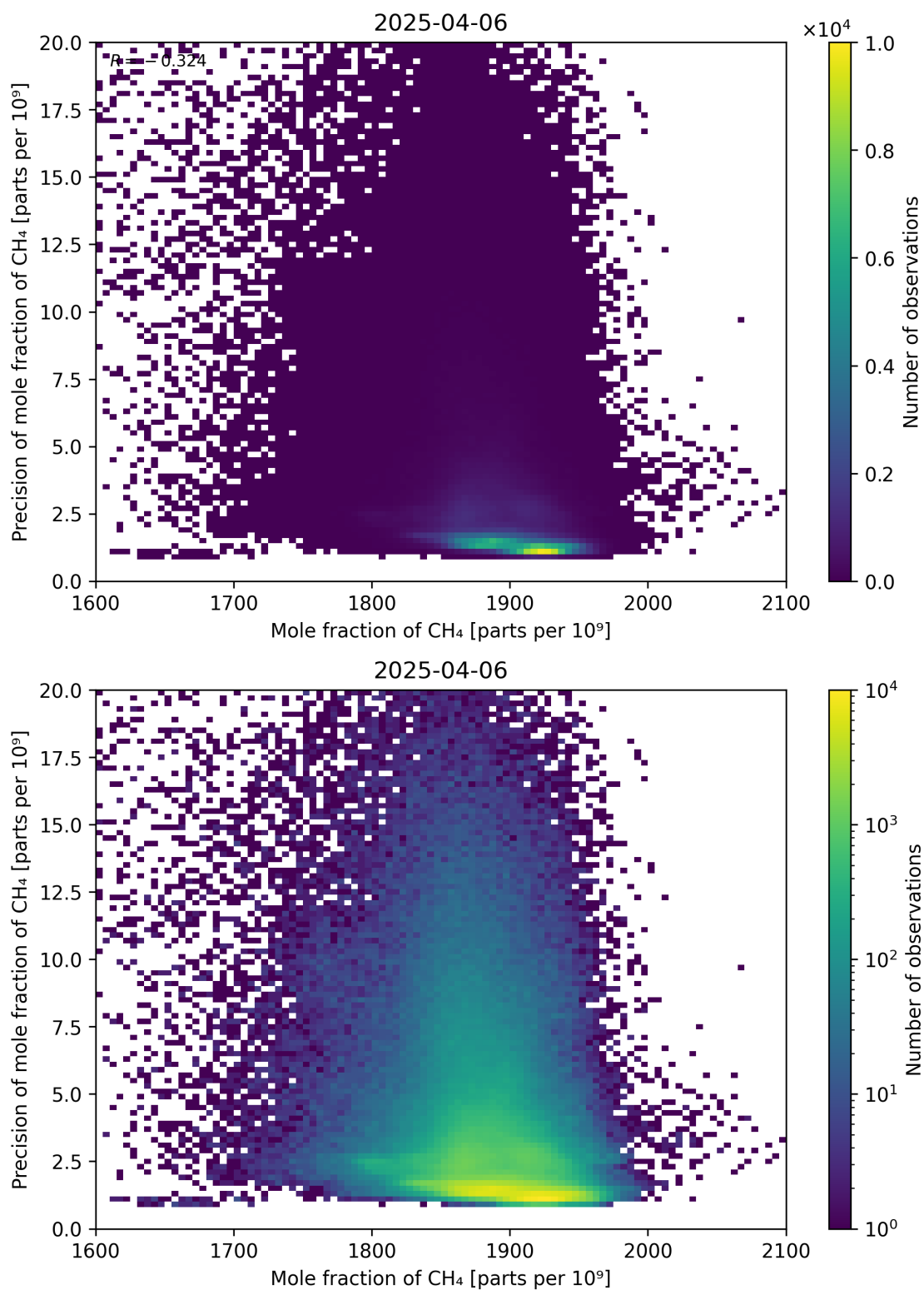
Figure 75: Scatter density plot of “Mole fraction of CH 4 ” against “Precision of mole fraction of CH 4 ” for 2025-04-05 to 2025-04-07.
