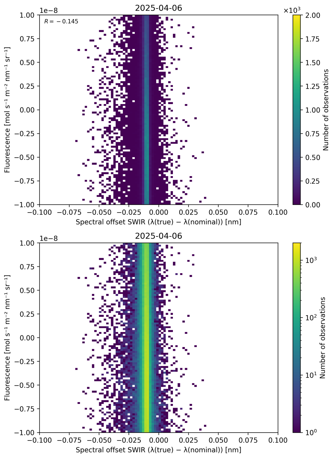
Figure 120: Scatter density plot of “Spectral offset SWIR ( \lambda_{\text{true}} - \lambda_{\text{nominal}} )” against “Fluorescence” for 2025-04-05 to 2025-04-07.
