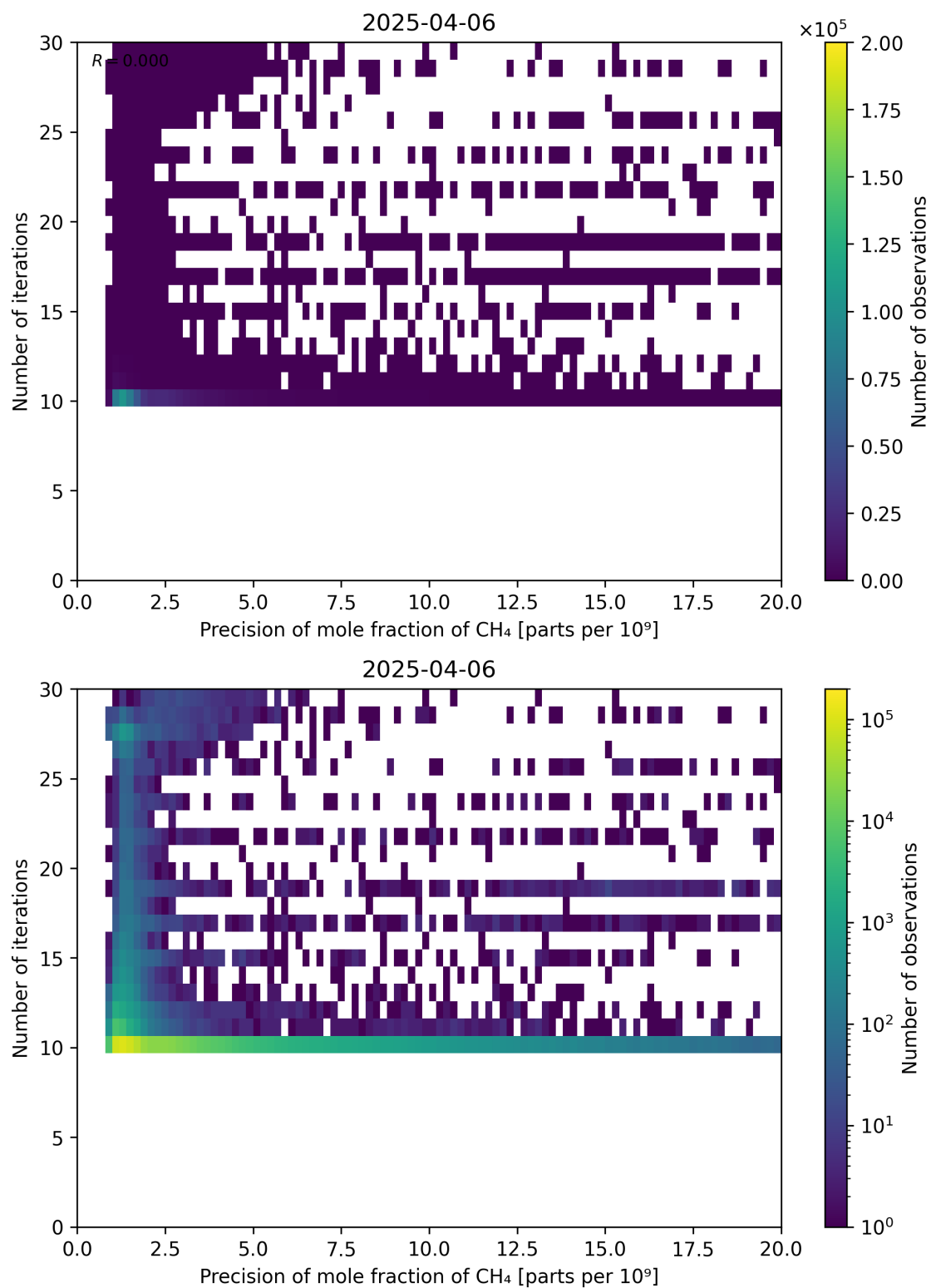
Figure 83: Scatter density plot of “Precision of mole fraction of CH 4 ” against “Number of iterations” for 2025-04-05 to 2025-04-07.
