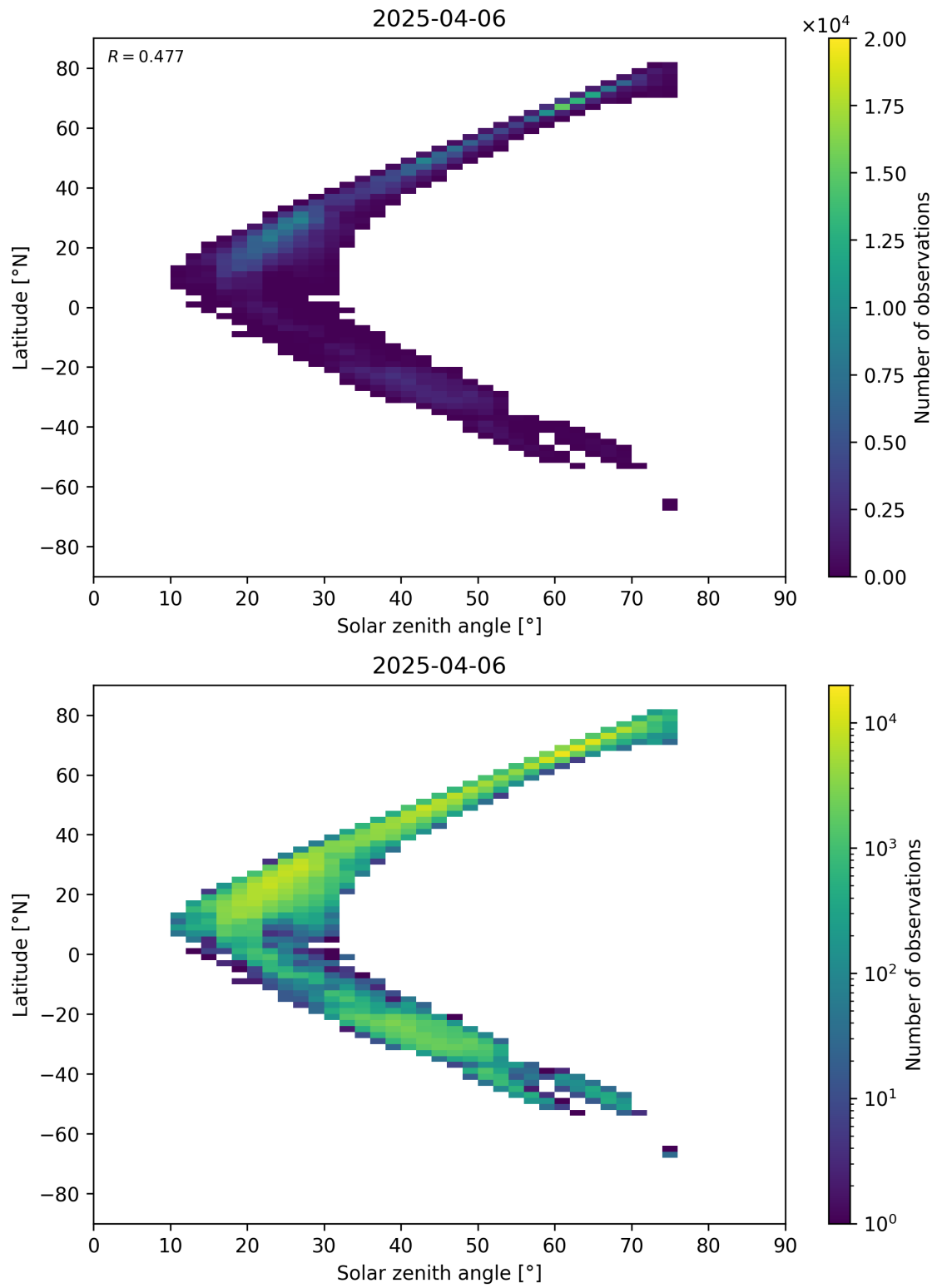
Figure 98: Scatter density plot of “Solar zenith angle” against “Latitude” for 2025-04-05 to 2025-04-07.
