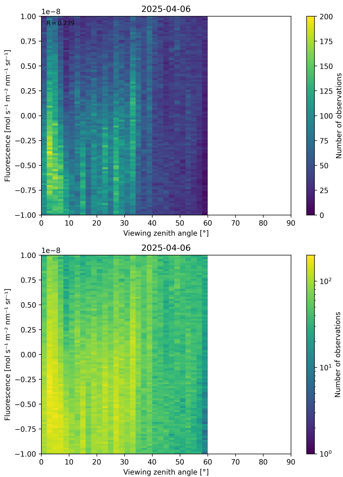
Figure 108: Scatter density plot of “Viewing zenith angle” against “Fluorescence” for 2025-04-05 to 2025-04-07.
