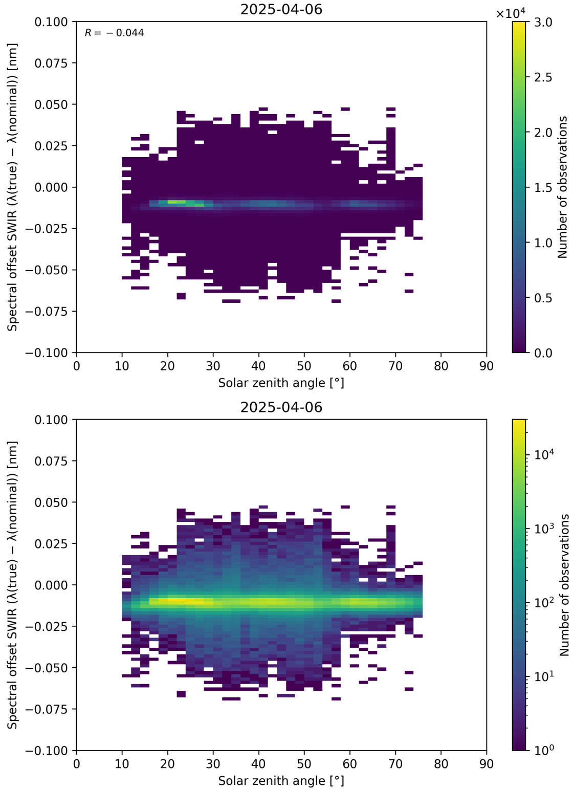
Figure 104: Scatter density plot of “Solar zenith angle” against “Spectral offset SWIR ( \lambda_{\text{true}} - \lambda_{\text{nominal}} )” for 2025-04-05 to 2025-04-07.
