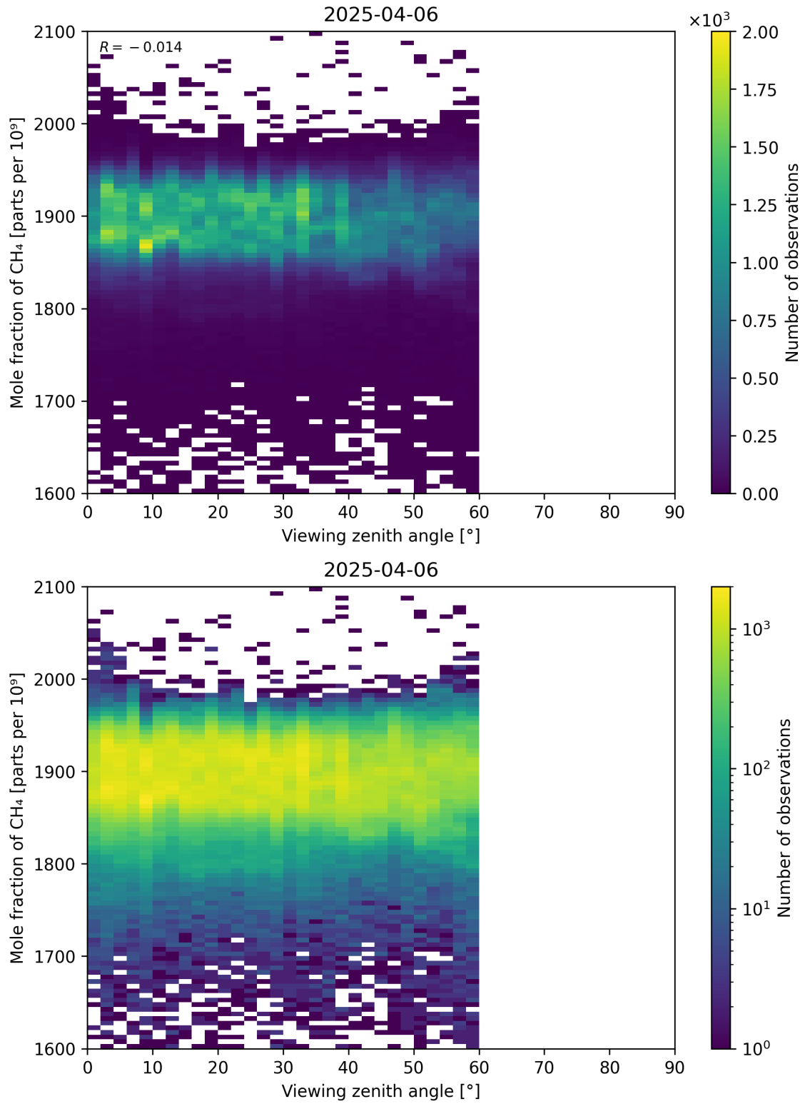
Figure 110: Scatter density plot of “Viewing zenith angle” against “Mole fraction of CH 4 ” for 2025-04-05 to 2025-04-07.
