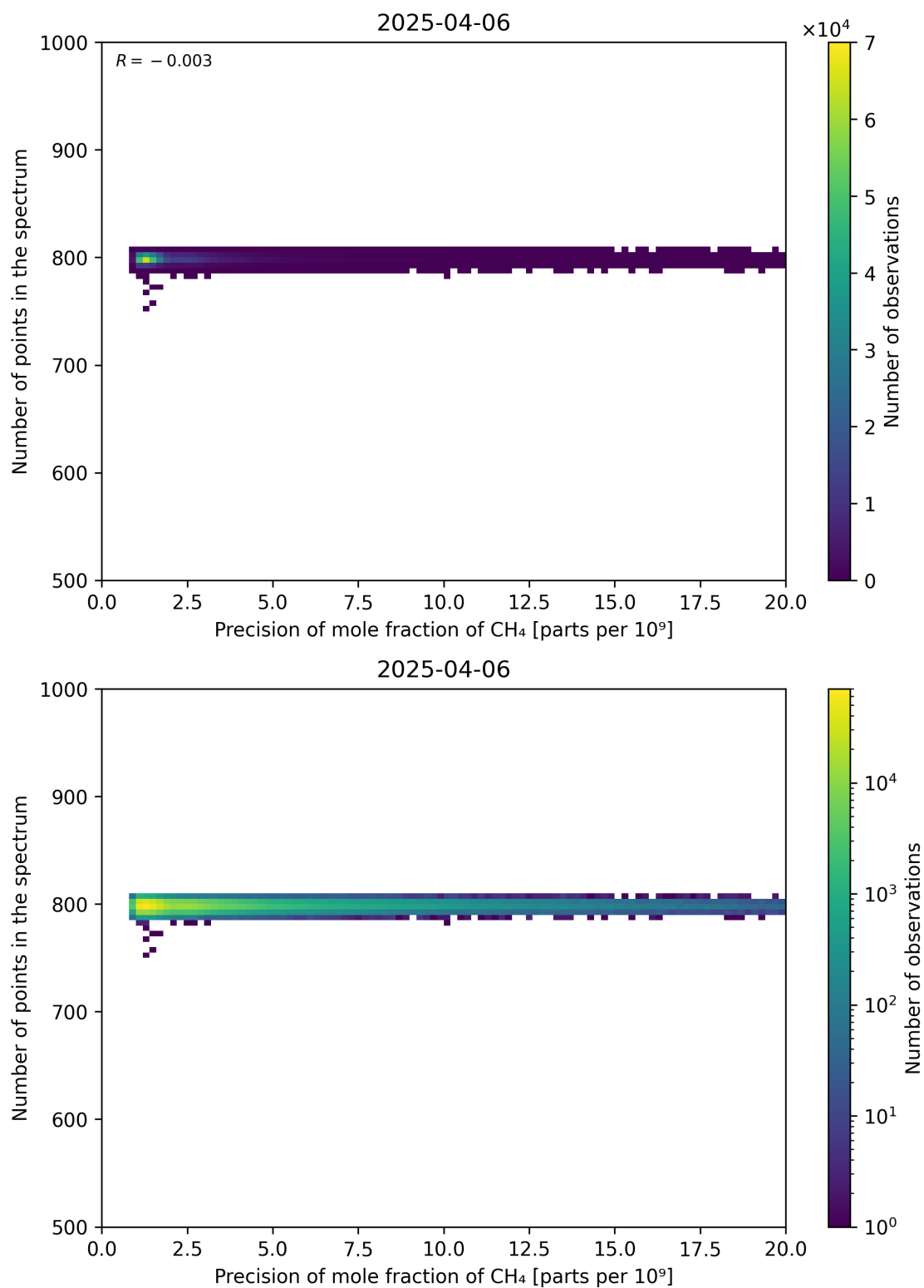
Figure 84: Scatter density plot of “Precision of mole fraction of CH 4 ” against “Number of points in the spectrum” for 2025-04-05 to 2025-04-07.
