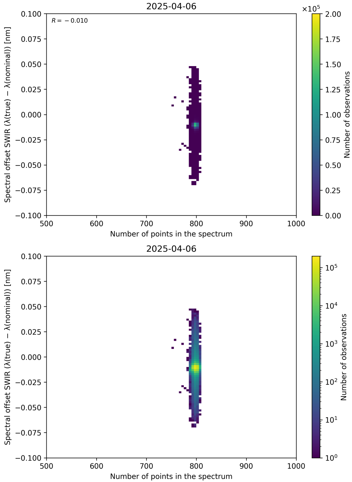
Figure 93: Scatter density plot of “Number of points in the spectrum” against “Spectral offset SWIR ( \lambda_{\text{true}} - \lambda_{\text{nominal}} )” for 2025-04-05 to 2025-04-07.
