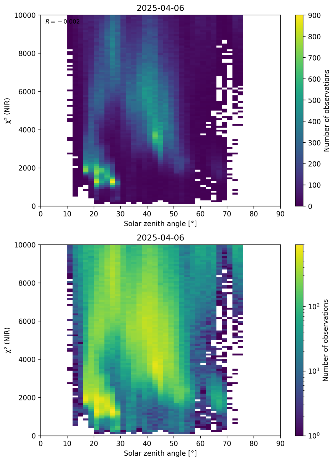
Figure 94: Scatter density plot of “Solar zenith angle” against “ \chi^2 (NIR)” for 2025-04-05 to 2025-04-07.
