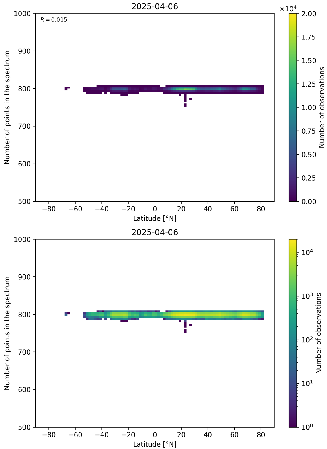
Figure 61: Scatter density plot of “Latitude” against “Number of points in the spectrum” for 2025-04-05 to 2025-04-07.
