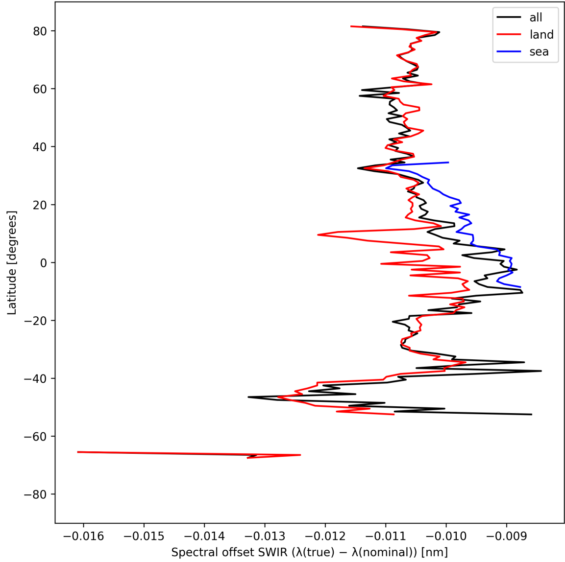
Figure 16: Zonal average of “Spectral offset SWIR ( \lambda_{\text{true}} - \lambda_{\text{nominal}} )” for 2025-04-05 to 2025-04-07.
