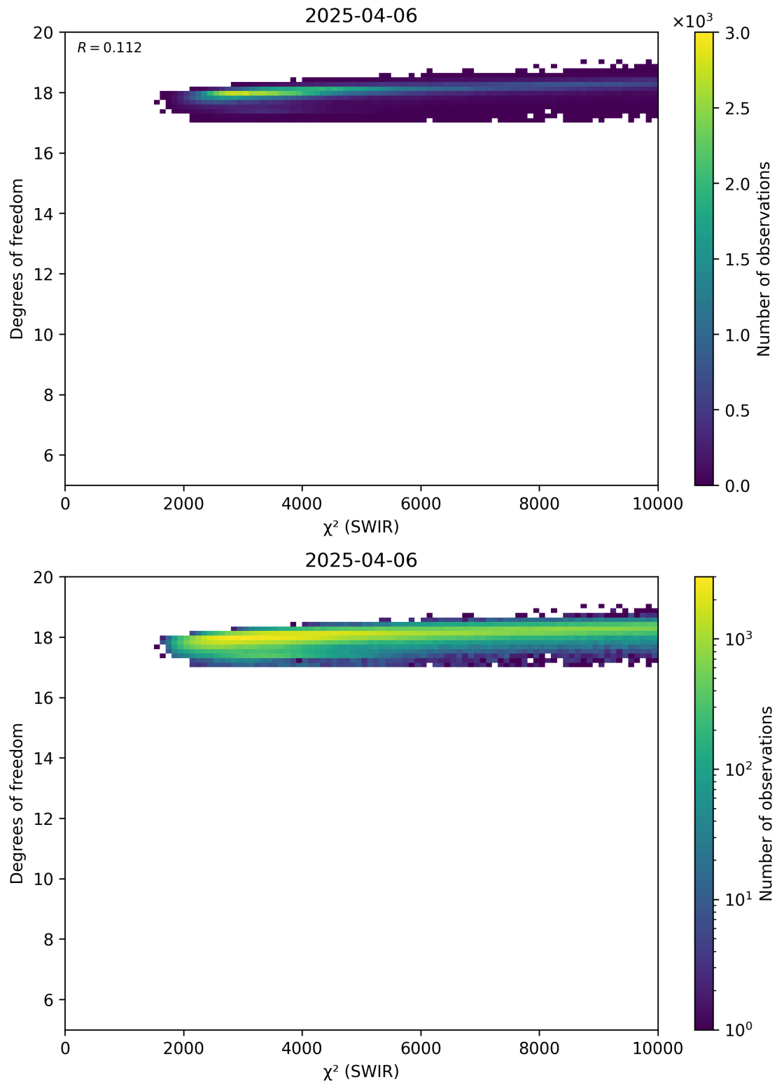
Figure 48: Scatter density plot of “ \chi^2 (SWIR)” against “Degrees of freedom” for 2025-04-05 to 2025-04-07.
