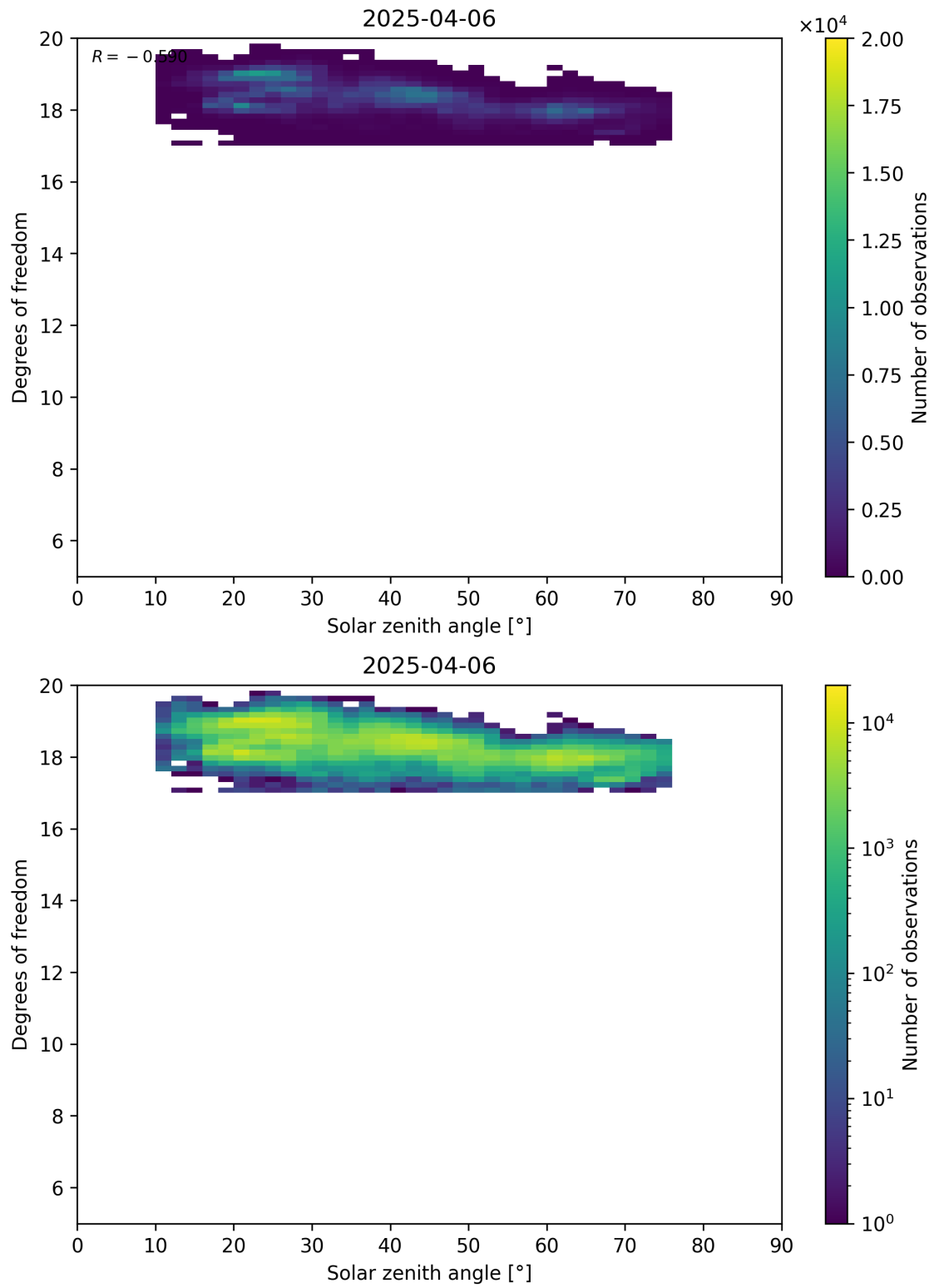
Figure 96: Scatter density plot of “Solar zenith angle” against “Degrees of freedom” for 2025-04-05 to 2025-04-07.
