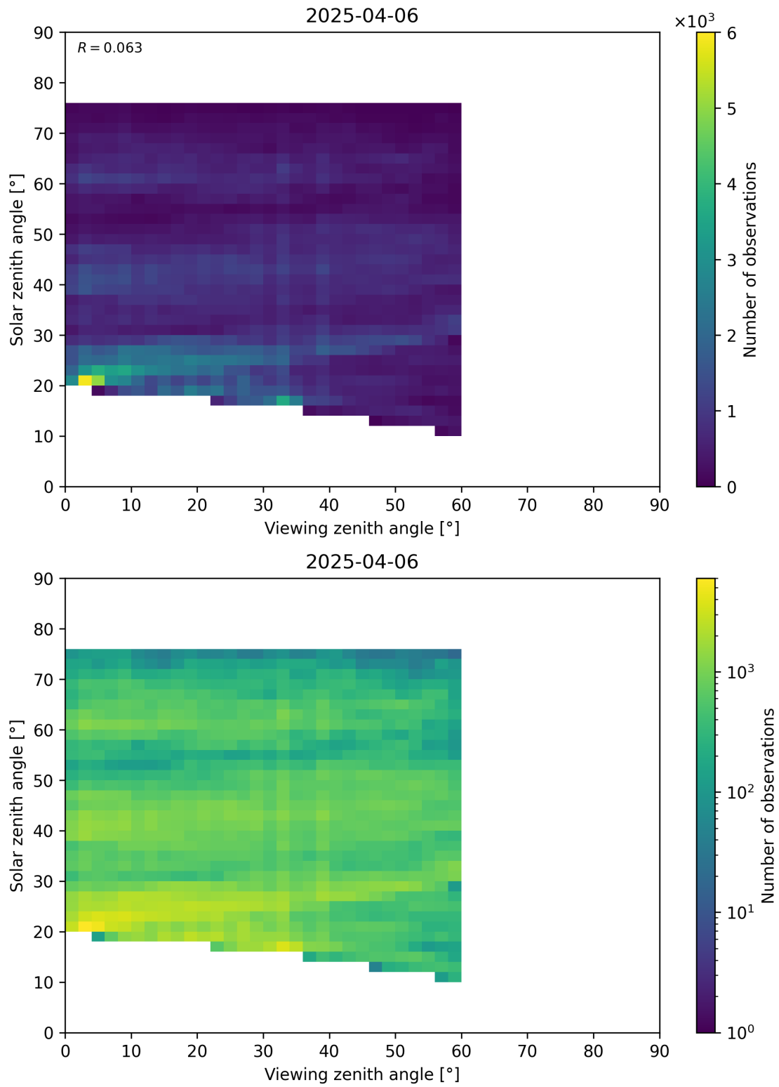
Figure 115: Scatter density plot of “Viewing zenith angle” against “Solar zenith angle” for 2025-04-05 to 2025-04-07.
