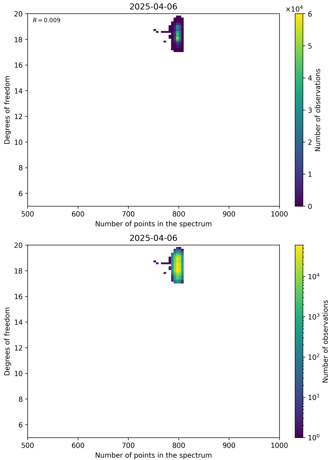
Figure 90: Scatter density plot of “Number of points in the spectrum” against “Degrees of freedom” for 2025-04-05 to 2025-04-07.
