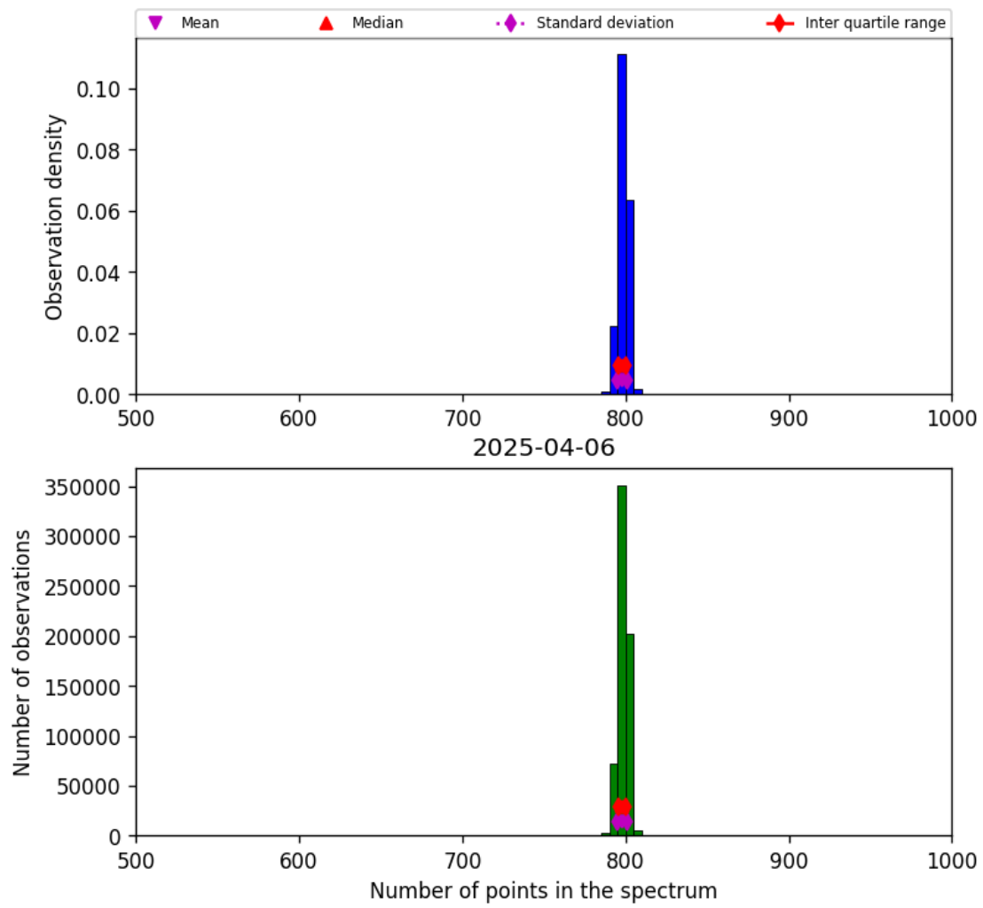
Figure 26: Histogram of “Number of points in the spectrum” for 2025-04-05 to 2025-04-07
