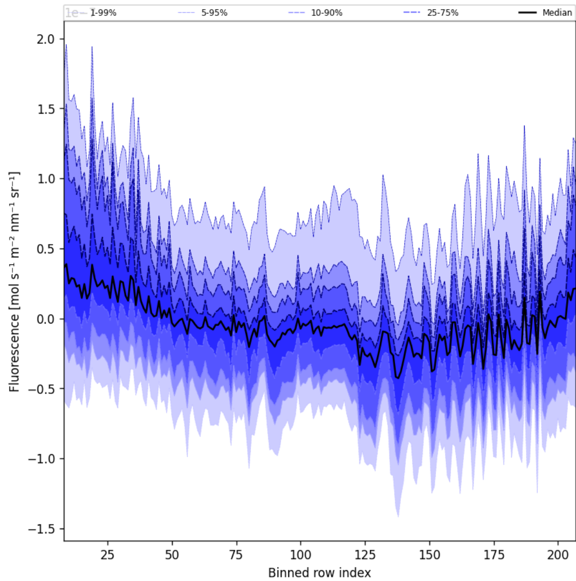
Figure 43: Along track statistics of “Fluorescence” for 2025-04-05 to 2025-04-07
