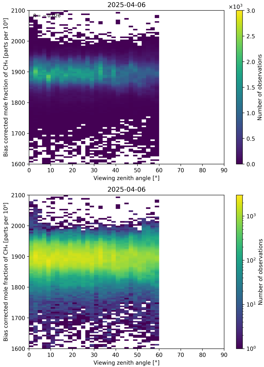
Figure 111: Scatter density plot of “Viewing zenith angle” against “Bias corrected mole fraction of CH 4 ” for 2025-04-05 to 2025-04-07.
