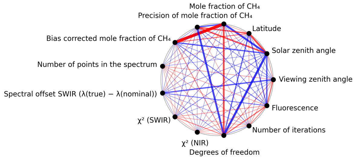
Figure 1: Map of correlation graph for 2025-04-05 to 2025-04-07.
