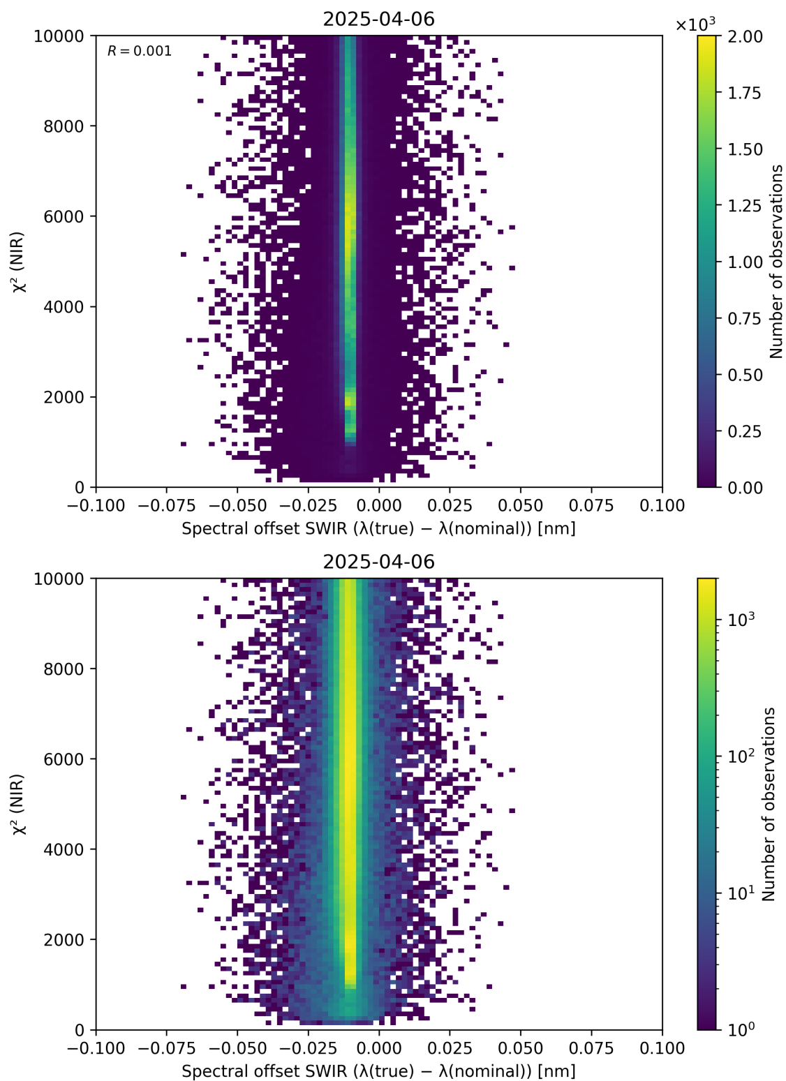
Figure 117: Scatter density plot of “Spectral offset SWIR ( \lambda_{\text{true}} - \lambda_{\text{nominal}} )” against “ \chi^2 (NIR)” for 2025-04-05 to 2025-04-07.
