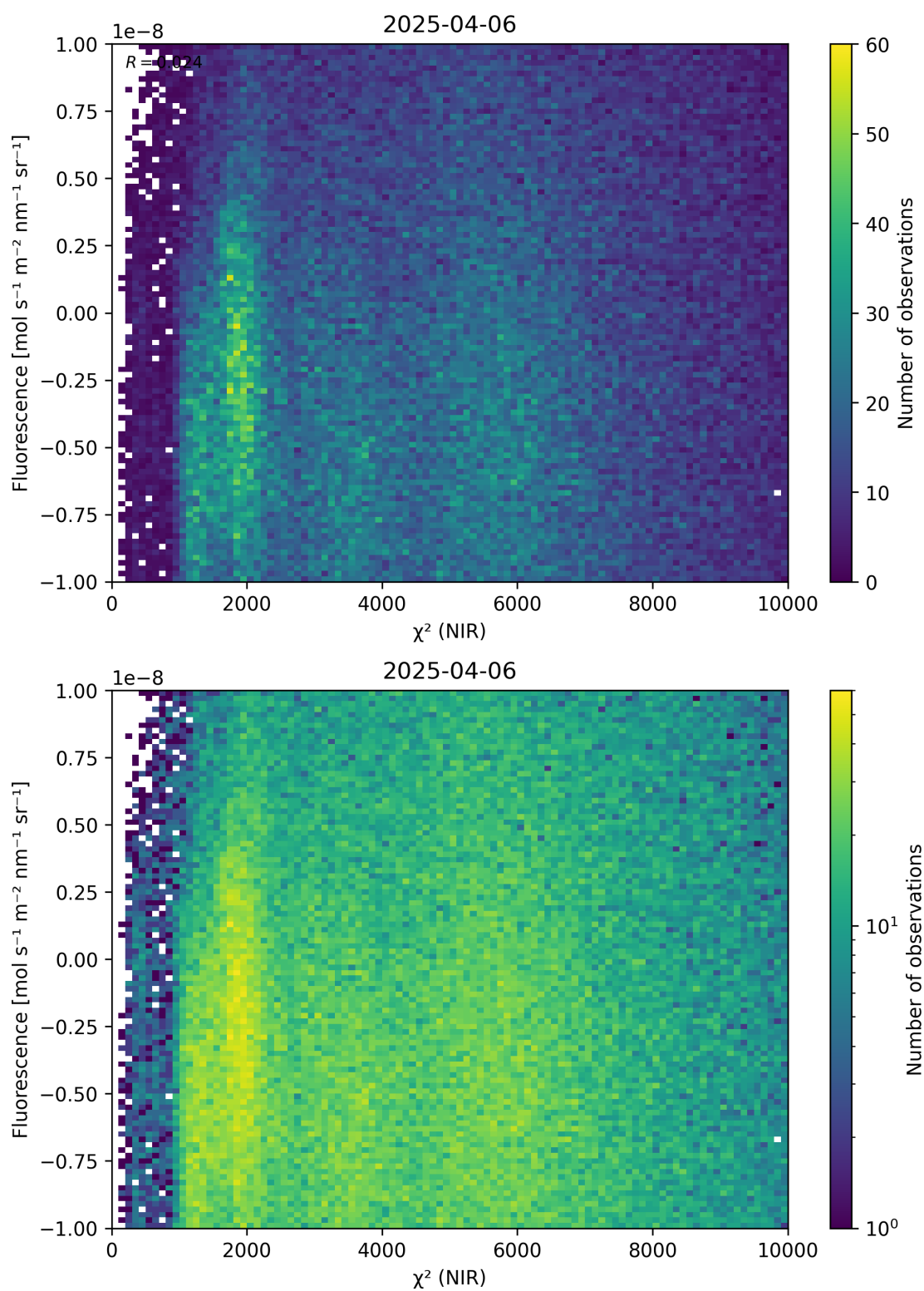
Figure 45: Scatter density plot of “ \chi^2 (NIR)” against “Fluorescence” for 2025-04-05 to 2025-04-07.
