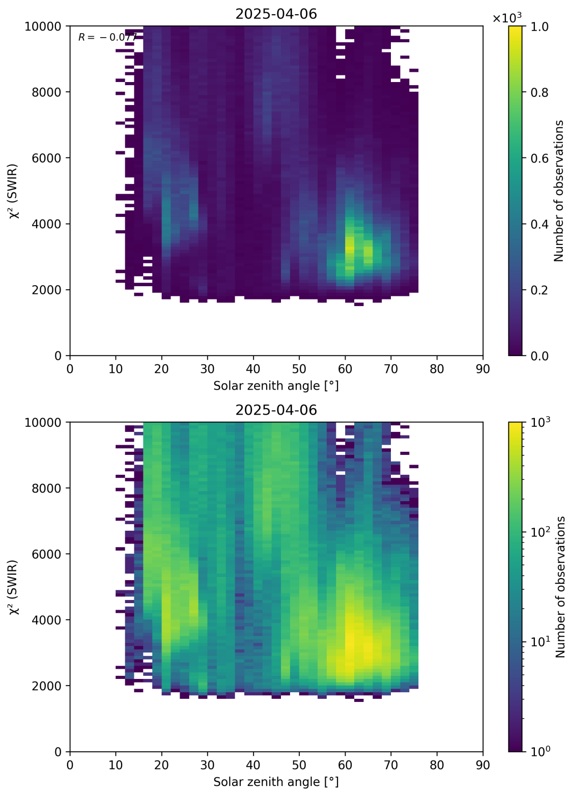
Figure 95: Scatter density plot of “Solar zenith angle” against “ \chi^2 (SWIR)” for 2025-04-05 to 2025-04-07.
