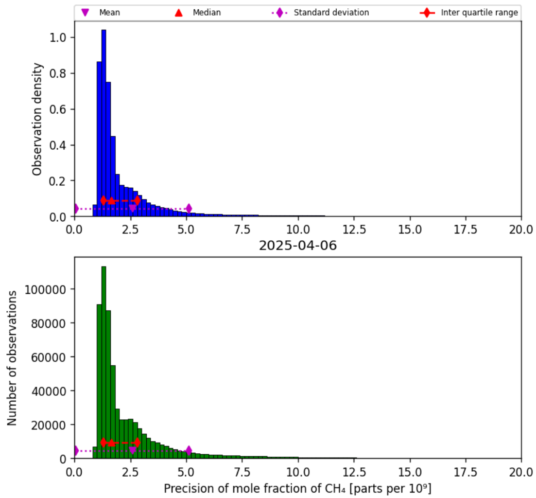
Figure 24: Histogram of "Precision of mole fraction of CH 4 " for 2025-04-05 to 2025-04-07
