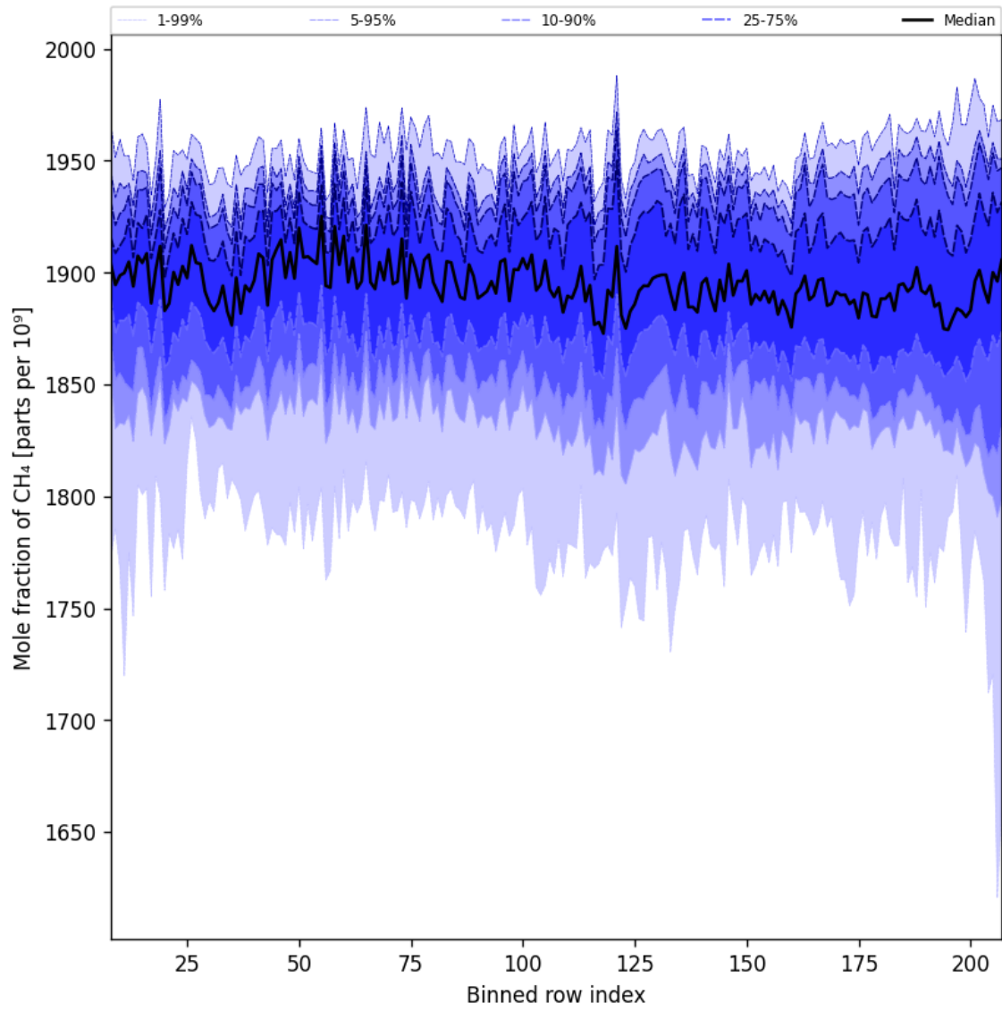
Figure 34: Along track statistics of “Mole fraction of CH 4 ” for 2025-04-05 to 2025-04-07
