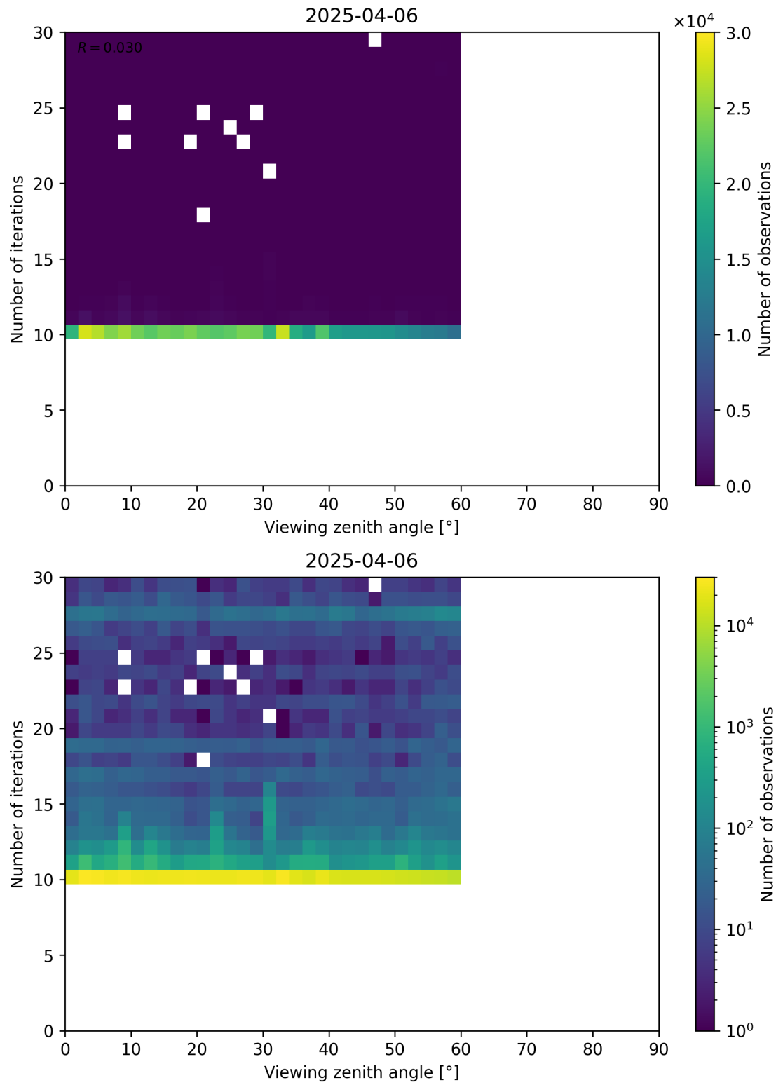
Figure 113: Scatter density plot of “Viewing zenith angle” against “Number of iterations” for 2025-04-05 to 2025-04-07.
