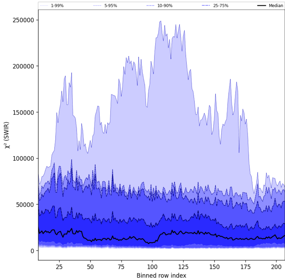
Figure 39: Along track statistics of “ \chi^2 (SWIR)” for 2025-04-05 to 2025-04-07
