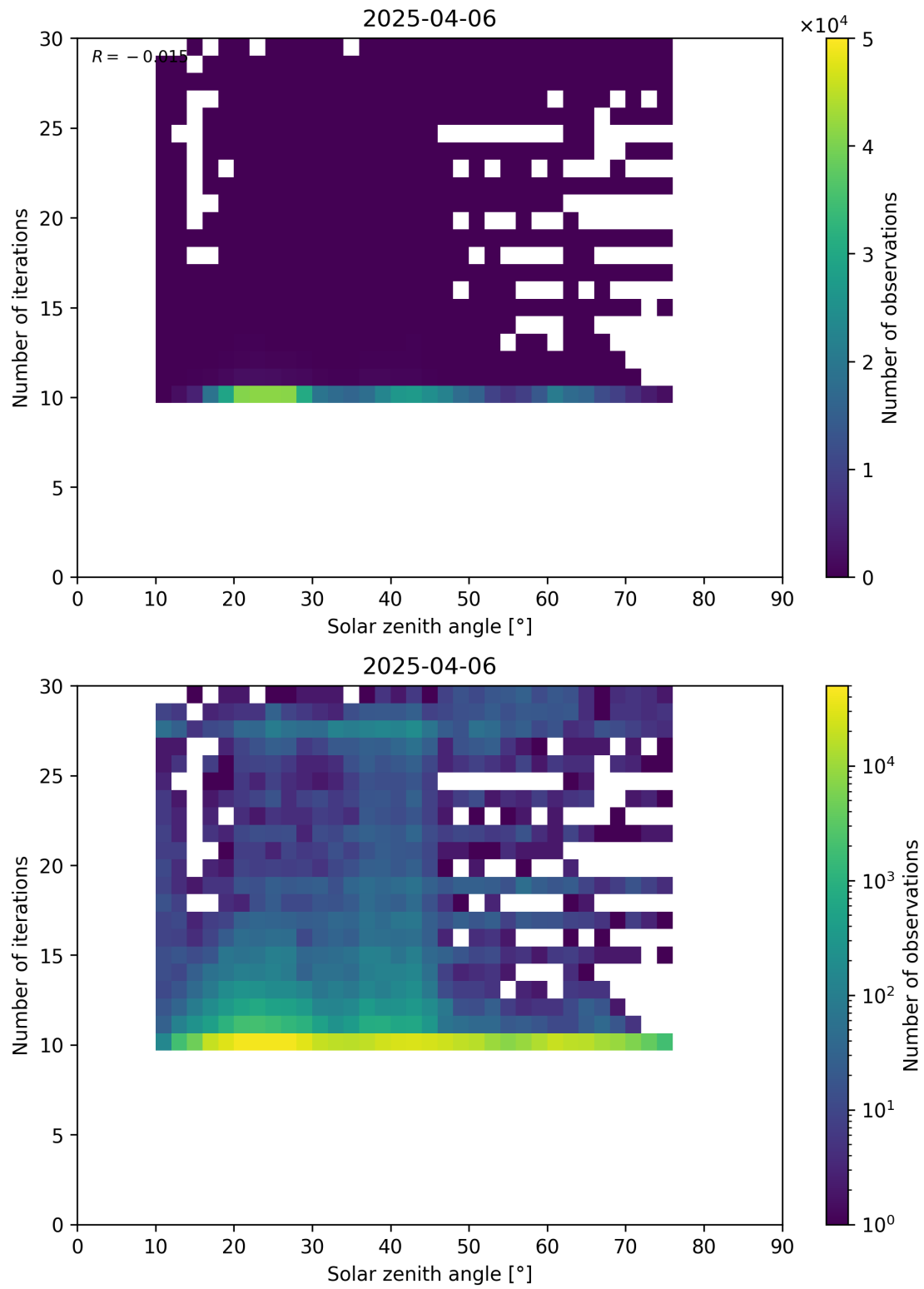
Figure 102: Scatter density plot of “Solar zenith angle” against “Number of iterations” for 2025-04-05 to 2025-04-07.
