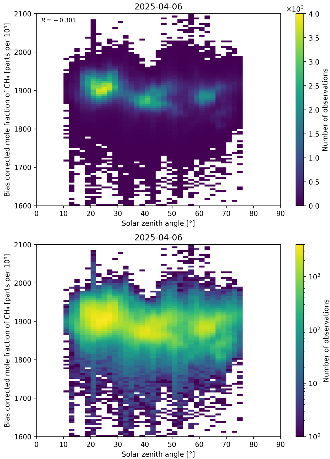
Figure 100: Scatter density plot of “Solar zenith angle” against “Bias corrected mole fraction of CH 4 ” for 2025-04-05 to 2025-04-07.
