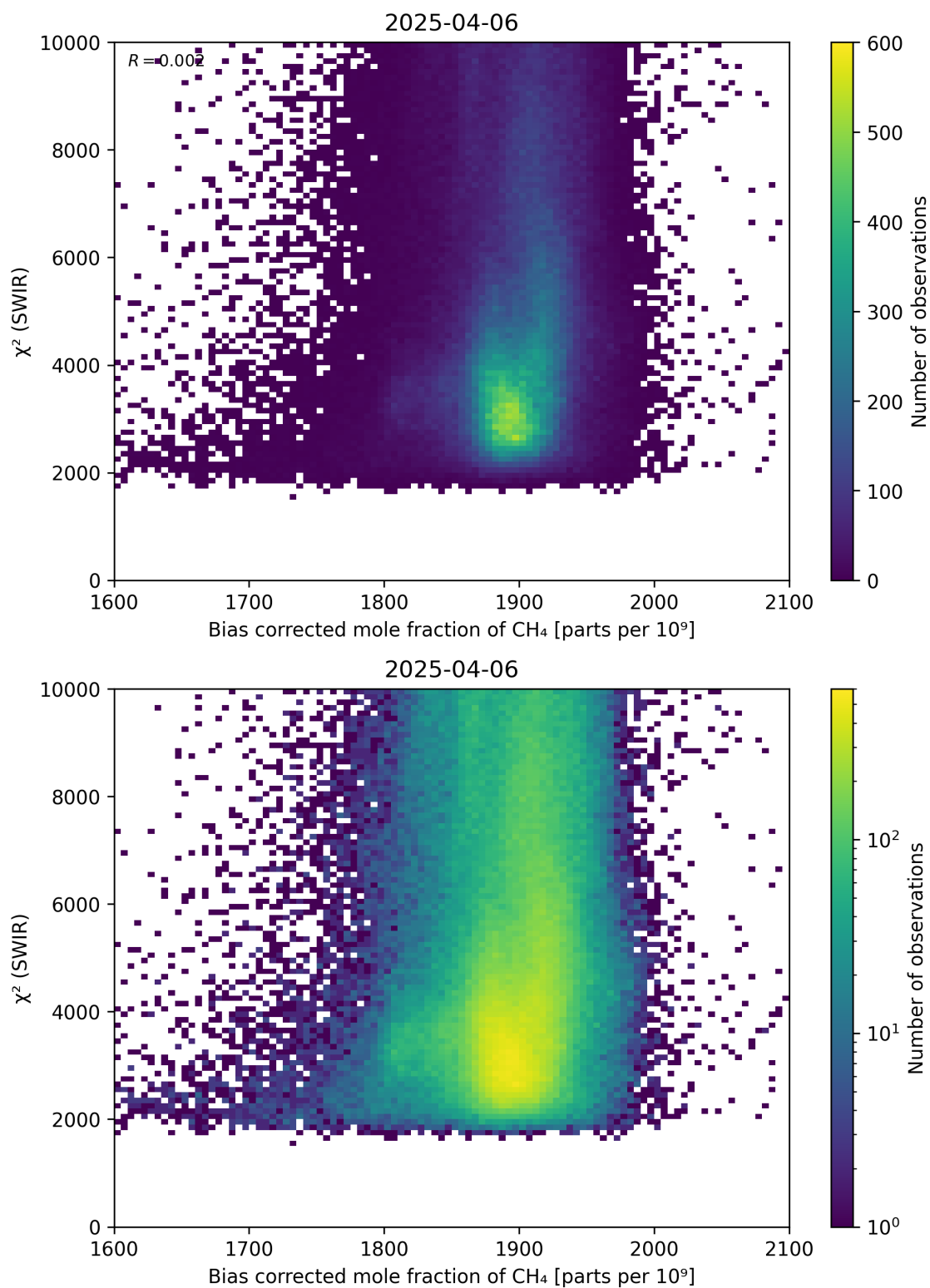
Figure 64: Scatter density plot of “Bias corrected mole fraction of CH 4 ” against “ \chi^2 (SWIR)” for 2025-04-05 to 2025-04-07.
