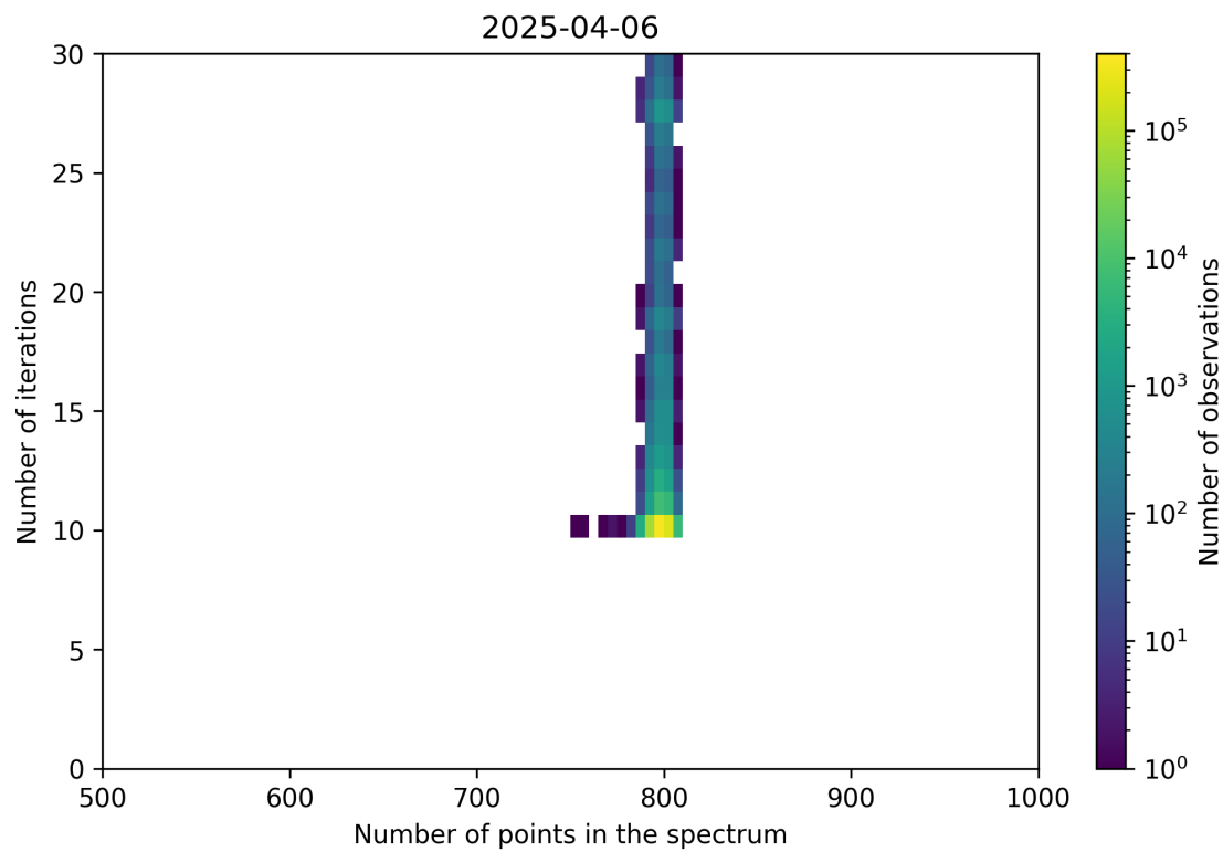
Figure 92: Scatter density plot of “Number of points in the spectrum” against “Number of iterations” for 2025-04-05 to 2025-04-07.
