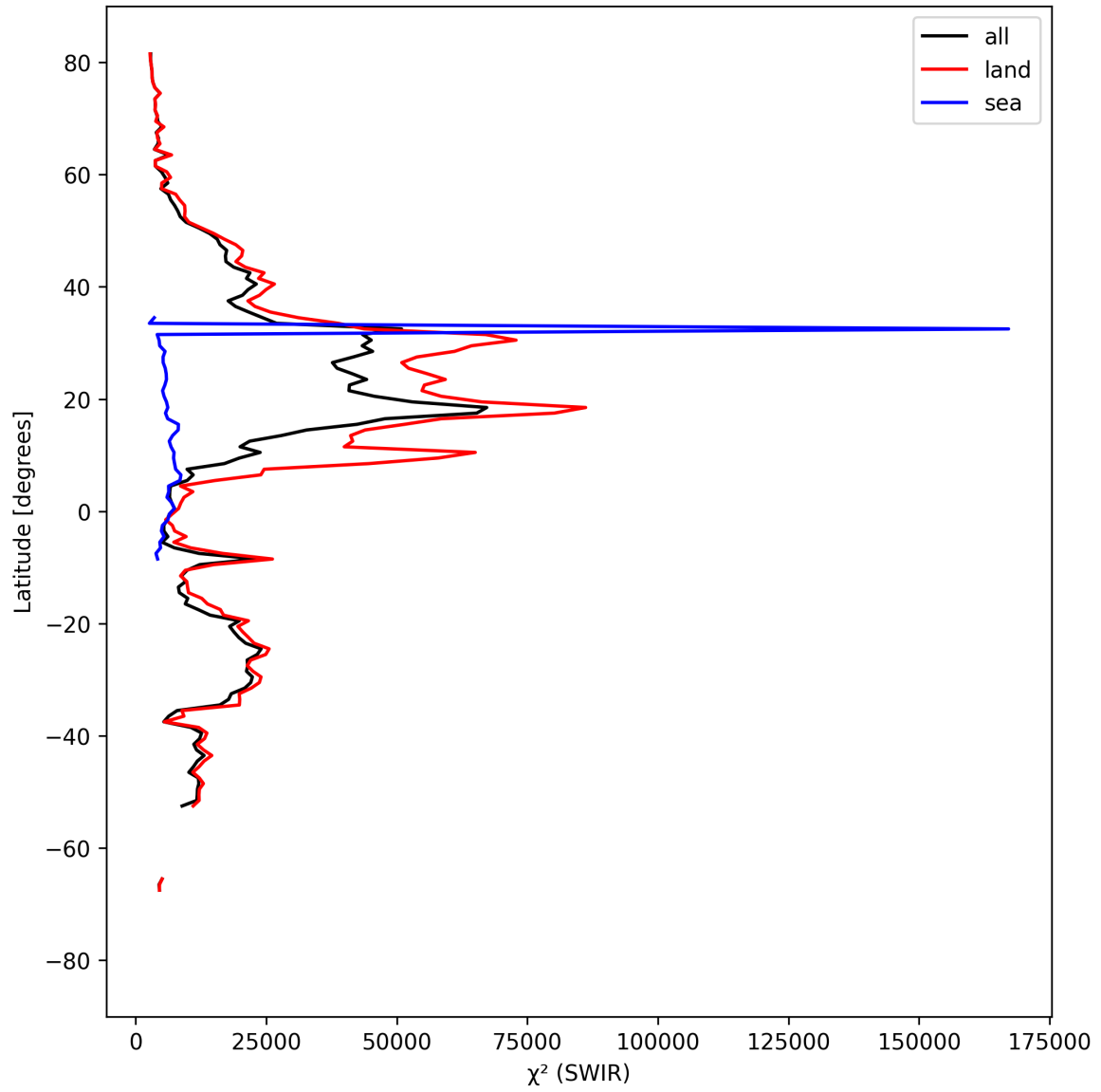
Figure 17: Zonal average of “ \chi^2 (SWIR)” for 2025-04-05 to 2025-04-07.
