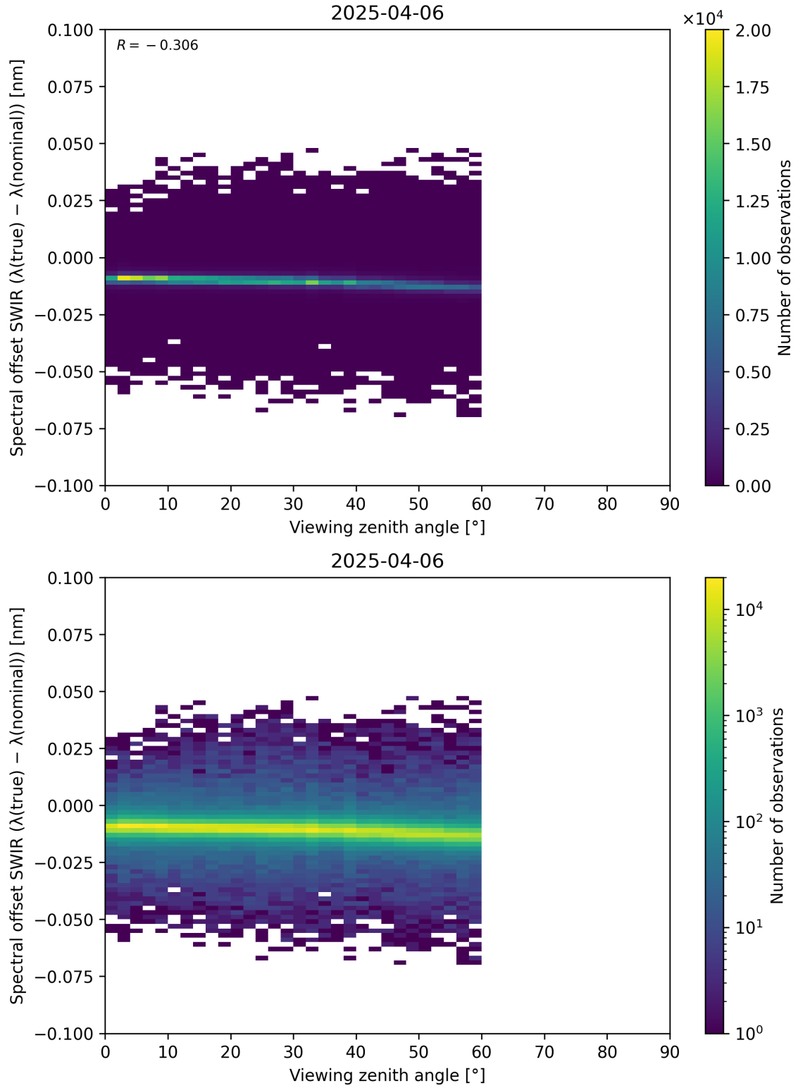
Figure 116: Scatter density plot of “Viewing zenith angle” against “Spectral offset SWIR ( \lambda_{\text{true}} - \lambda_{\text{nominal}} )” for 2025-04-05 to 2025-04-07.
