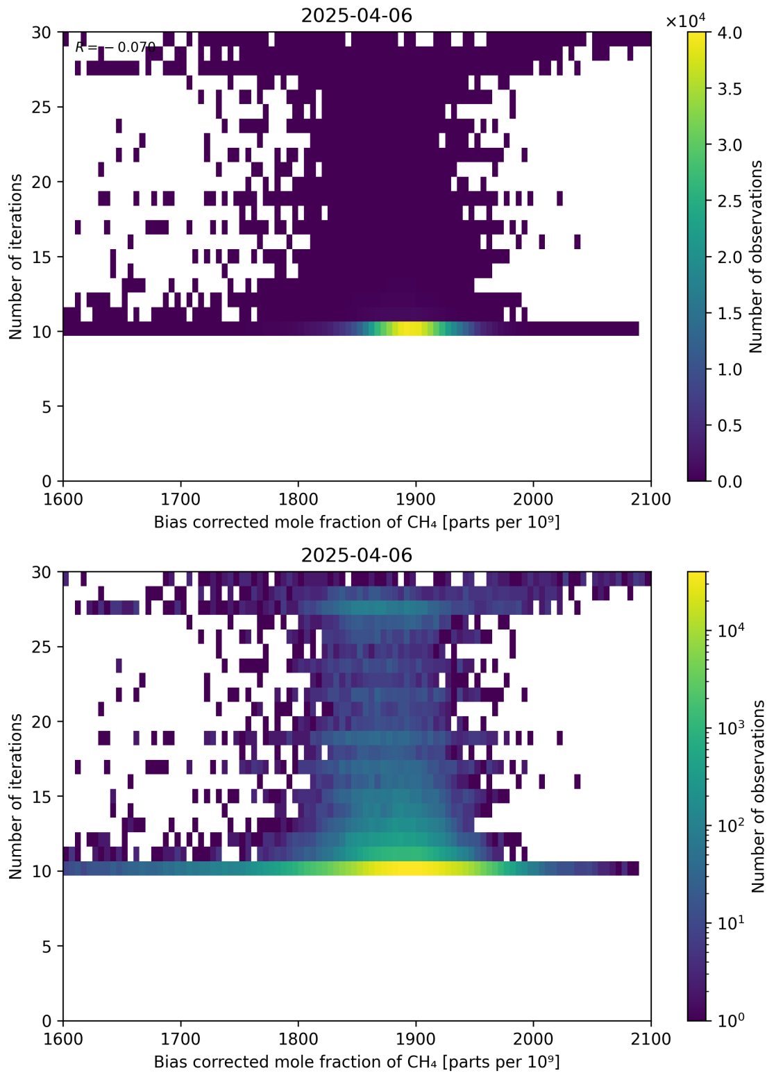
Figure 67: Scatter density plot of “Bias corrected mole fraction of CH 4 ” against “Number of iterations” for 2025-04-05 to 2025-04-07.
