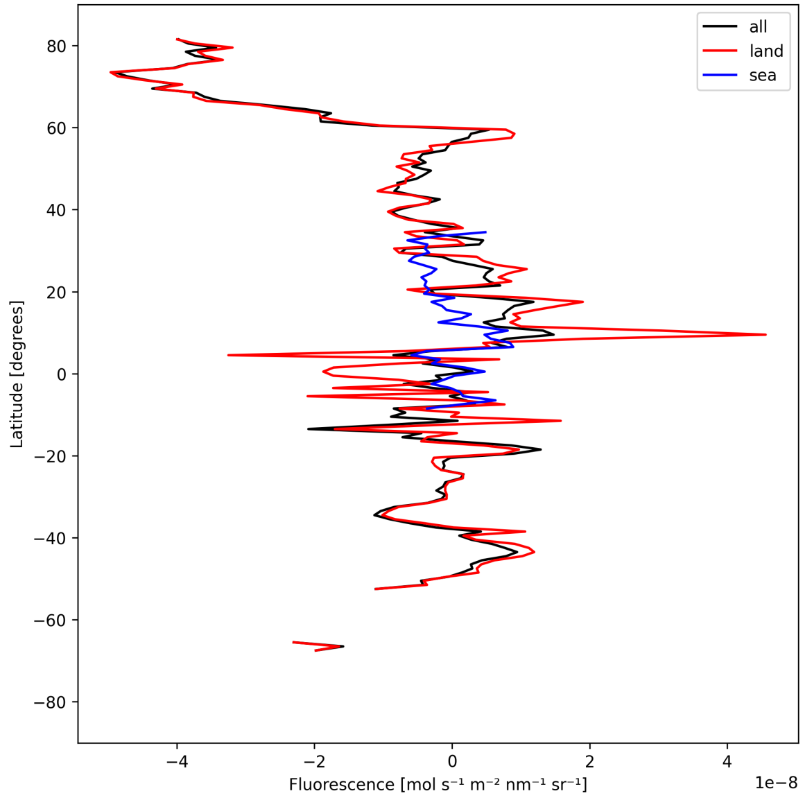
Figure 21: Zonal average of “Fluorescence” for 2025-04-05 to 2025-04-07.
