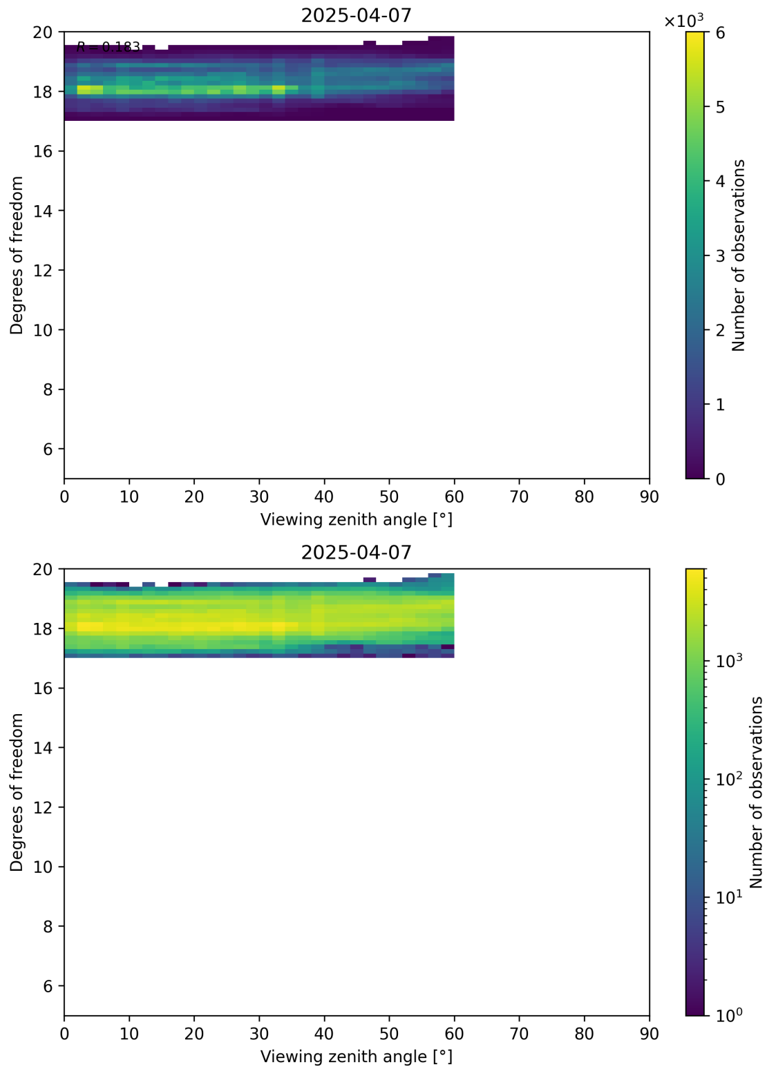
Figure 107: Scatter density plot of “Viewing zenith angle” against “Degrees of freedom” for 2025-04-06 to 2025-04-08.
