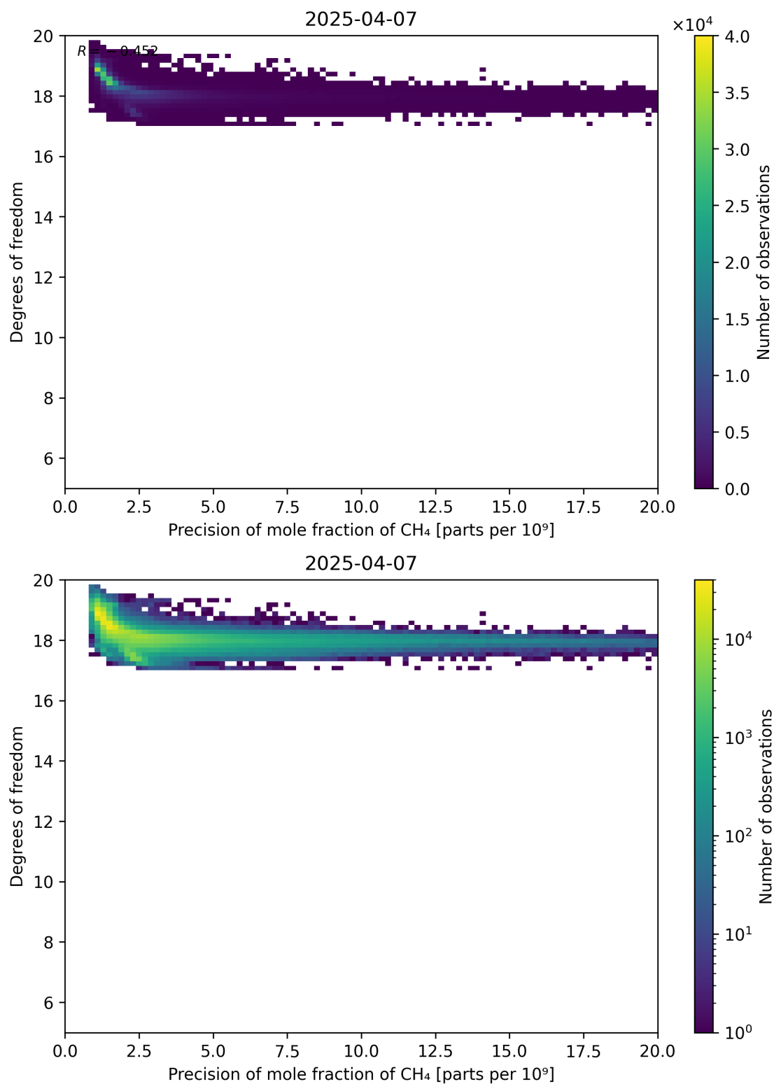
Figure 80: Scatter density plot of “Precision of mole fraction of CH 4 ” against “Degrees of freedom” for 2025-04-06 to 2025-04-08.
