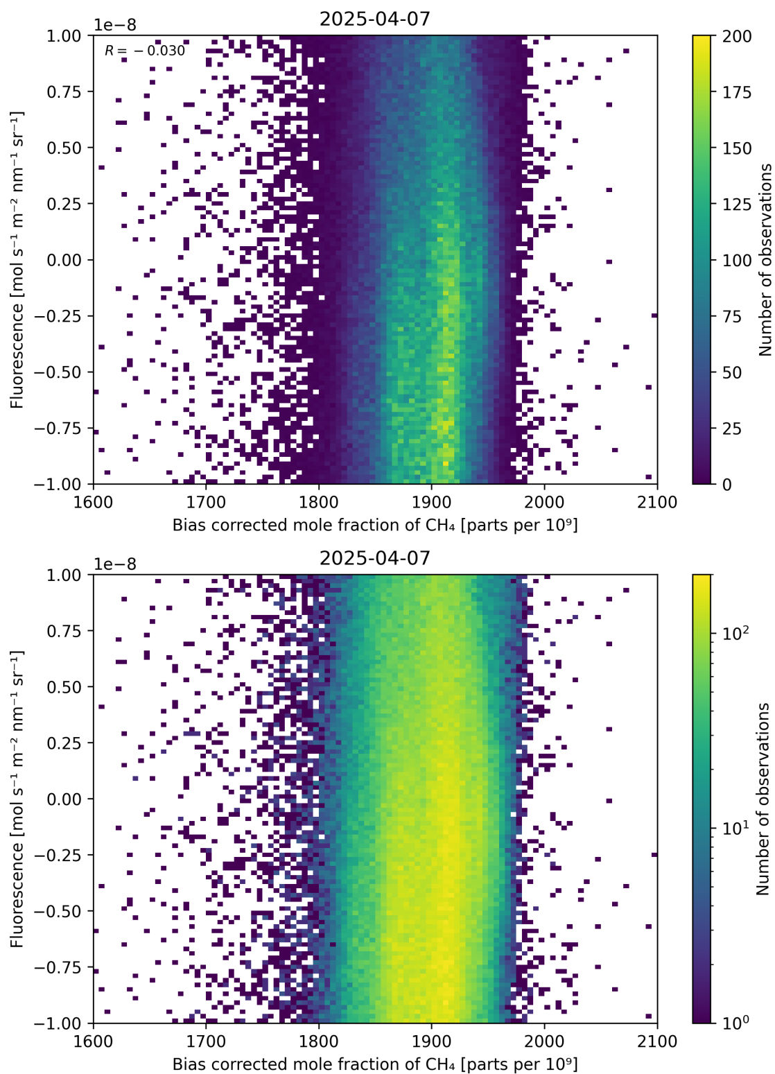
Figure 66: Scatter density plot of “Bias corrected mole fraction of \text{CH}_4 ” against “Fluorescence” for 2025-04-06 to 2025-04-08.
