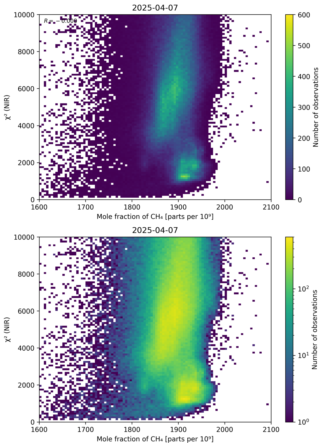
Figure 70: Scatter density plot of “Mole fraction of \text{CH}_4 ” against “ \chi^2 (NIR)” for 2025-04-06 to 2025-04-08.
