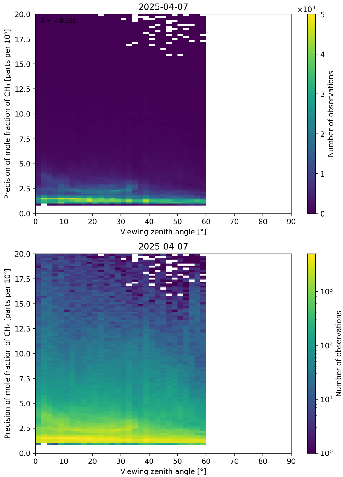
Figure 112: Scatter density plot of “Viewing zenith angle” against “Precision of mole fraction of CH 4 ” for 2025-04-06 to 2025-04-08.
