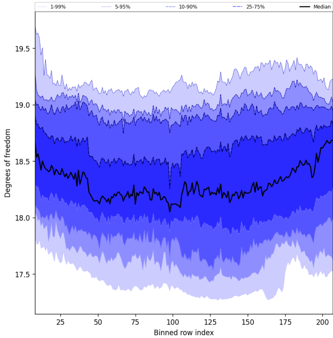
Figure 41: Along track statistics of “Degrees of freedom” for 2025-04-06 to 2025-04-08
