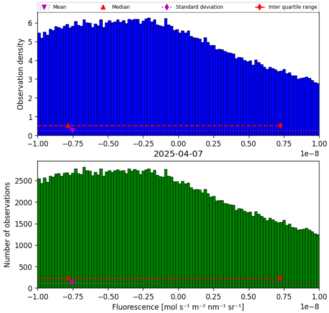
Figure 32: Histogram of “Fluorescence” for 2025-04-06 to 2025-04-08
