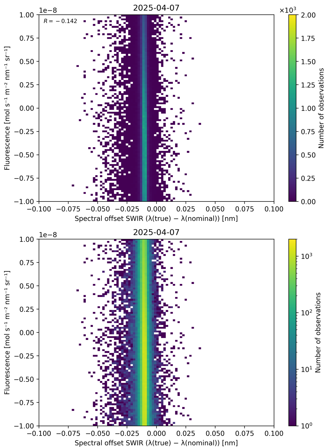
Figure 120: Scatter density plot of “Spectral offset SWIR ( \lambda_{\text{true}} - \lambda_{\text{nominal}} )” against “Fluorescence” for 2025-04-06 to 2025-04-08.
