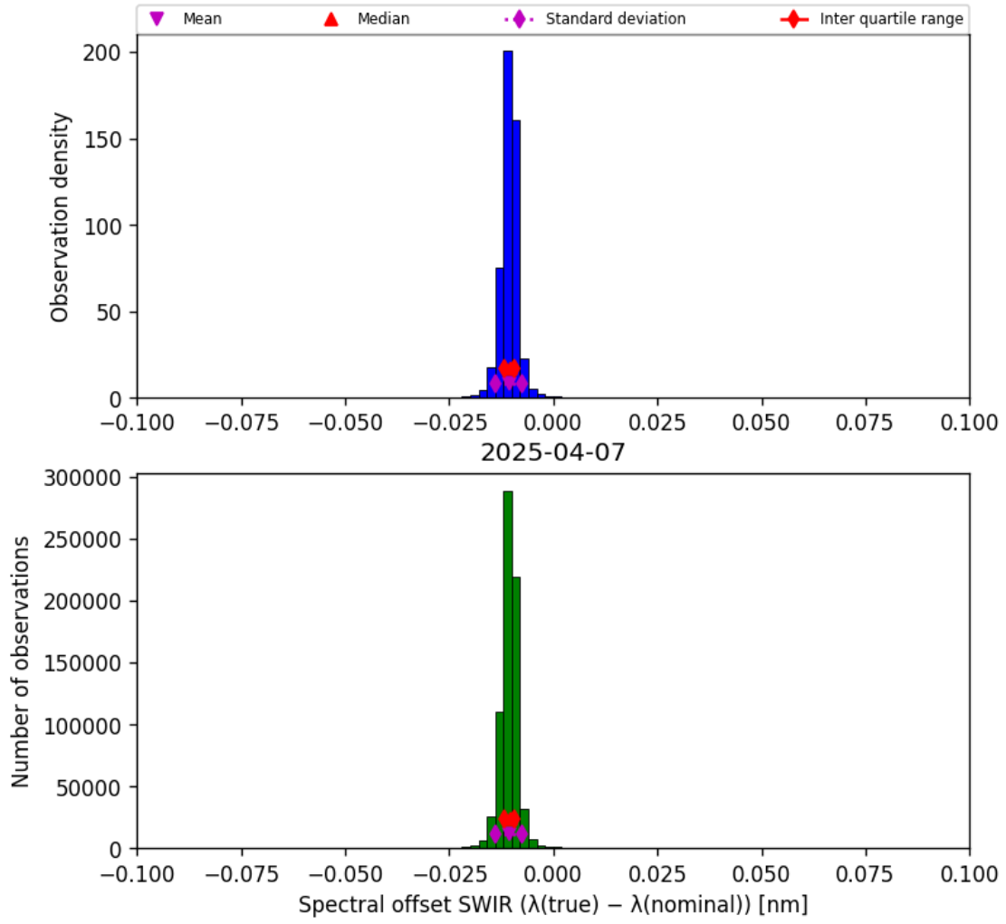
Figure 27: Histogram of “Spectral offset SWIR ( \lambda_{\text{true}} - \lambda_{\text{nominal}} )” for 2025-04-06 to 2025-04-08
