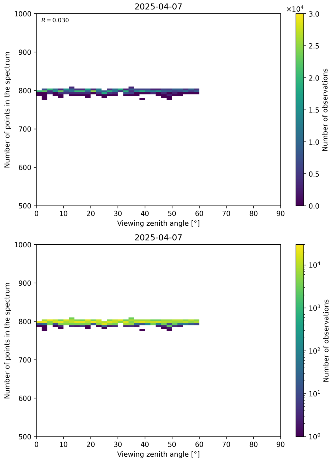
Figure 114: Scatter density plot of “Viewing zenith angle” against “Number of points in the spectrum” for 2025-04-06 to 2025-04-08.
