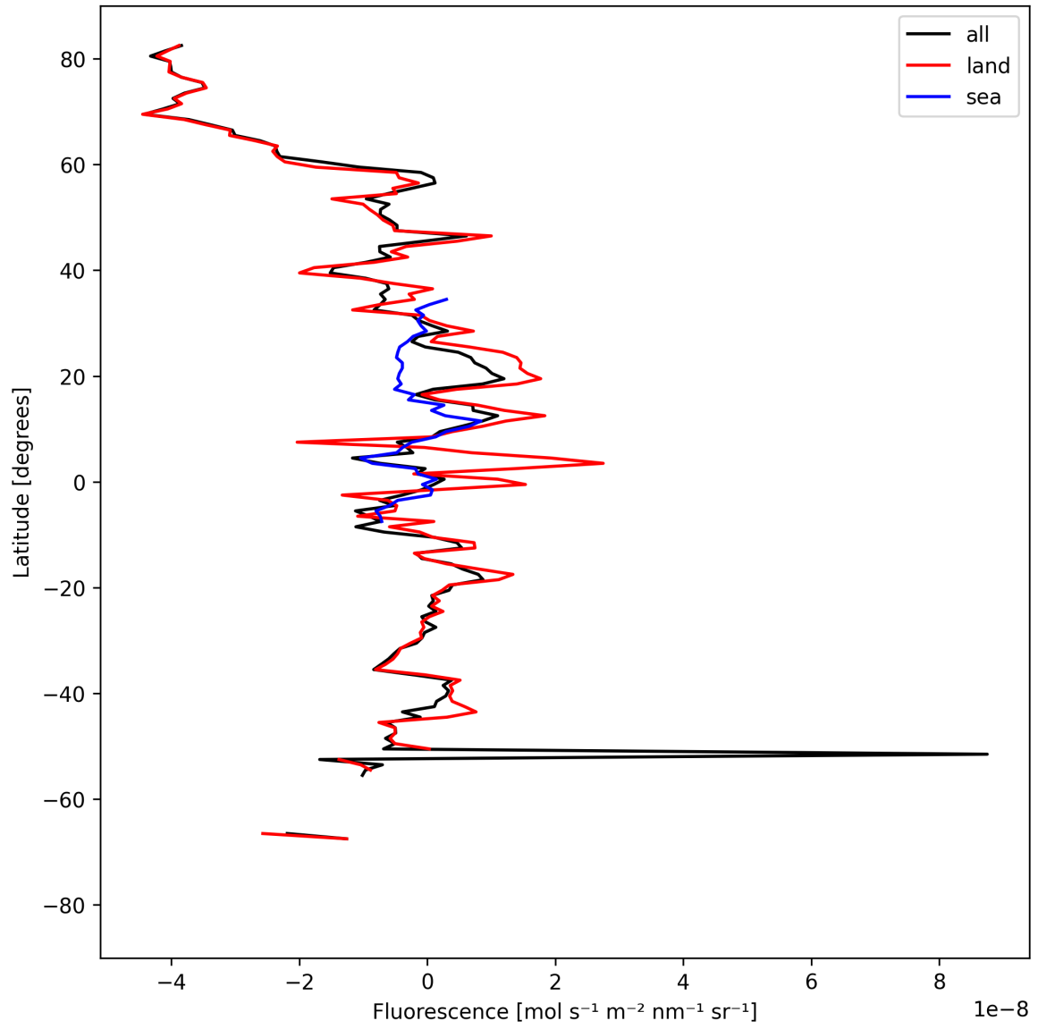
Figure 21: Zonal average of “Fluorescence” for 2025-04-06 to 2025-04-08.
