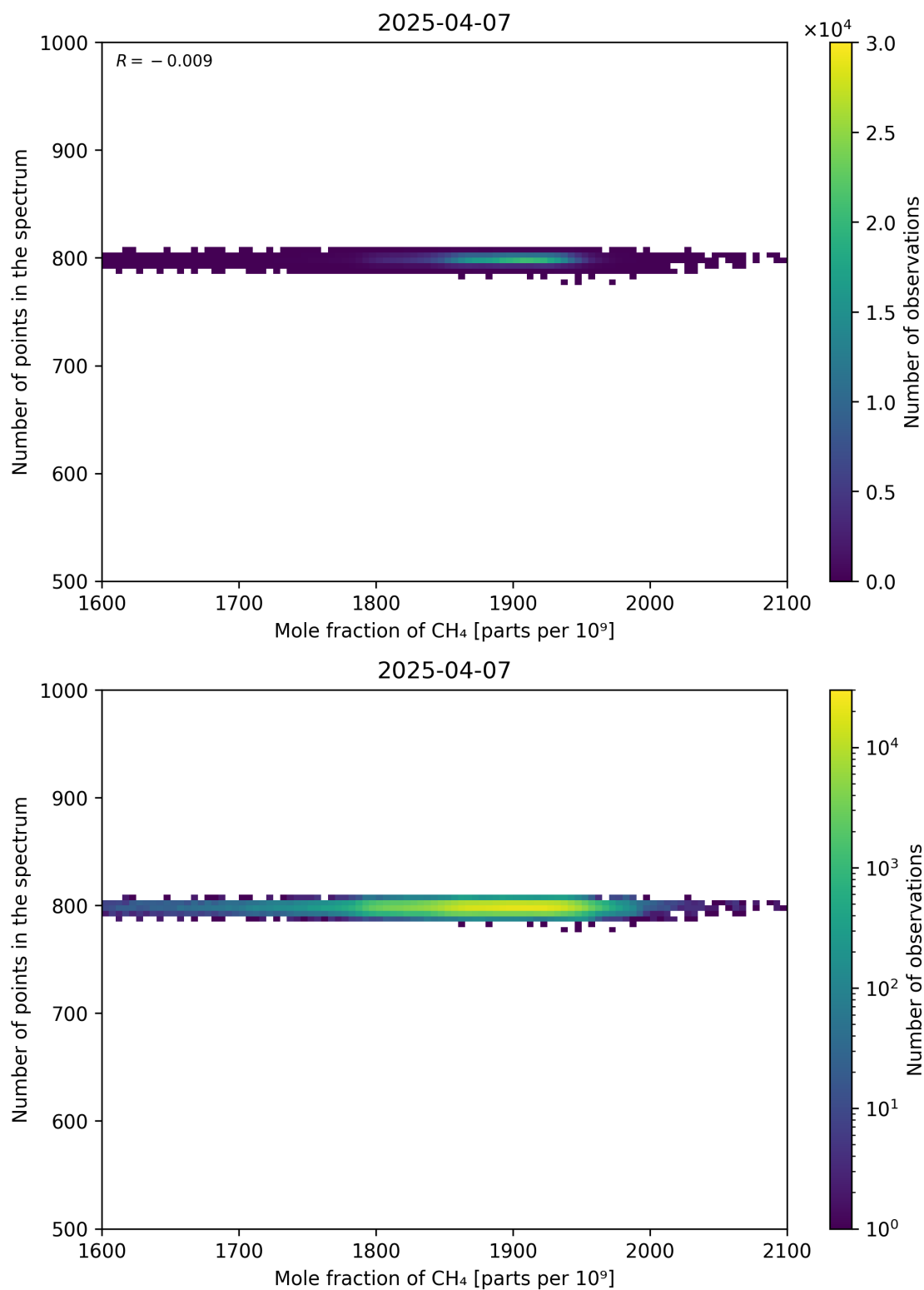
Figure 77: Scatter density plot of “Mole fraction of CH 4 ” against “Number of points in the spectrum” for 2025-04-06 to 2025-04-08.
