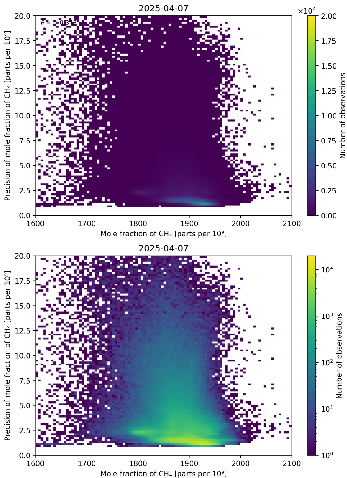
Figure 75: Scatter density plot of “Mole fraction of CH 4 ” against “Precision of mole fraction of CH 4 ” for 2025-04-06 to 2025-04-08.
