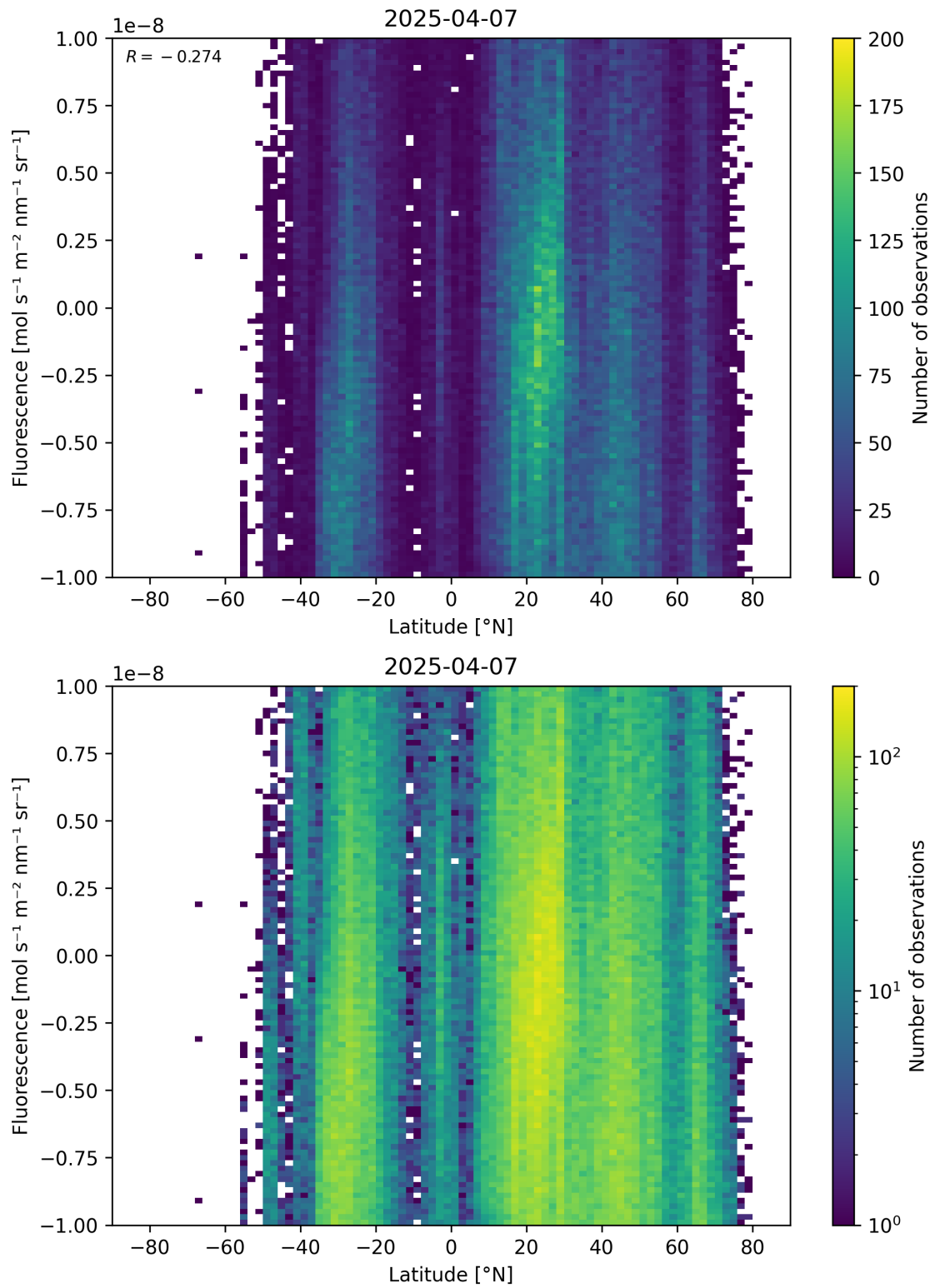
Figure 56: Scatter density plot of “Latitude” against “Fluorescence” for 2025-04-06 to 2025-04-08.
