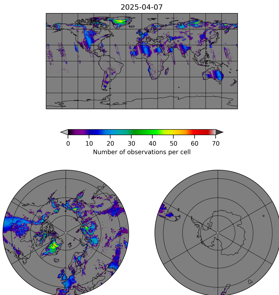
Figure 10: Map of the number of observations for 2025-04-06 to 2025-04-08
