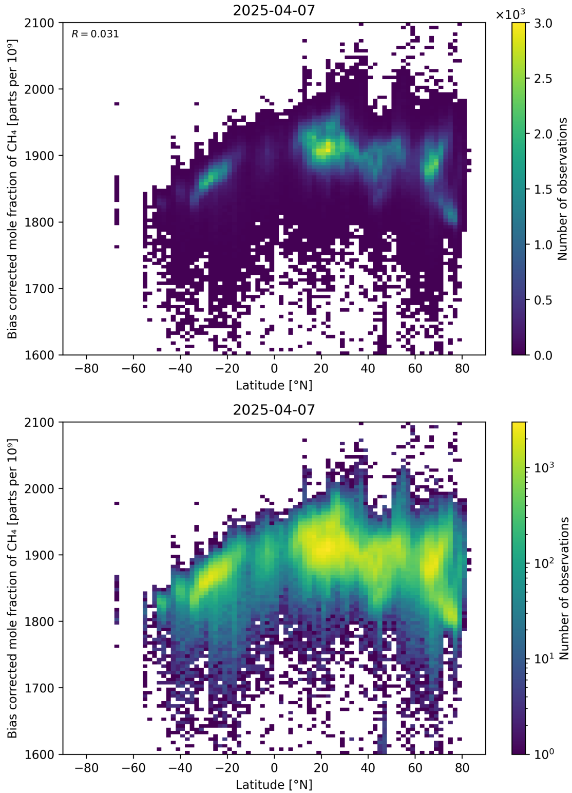
Figure 58: Scatter density plot of “Latitude” against “Bias corrected mole fraction of CH 4 ” for 2025-04-06 to 2025-04-08.
