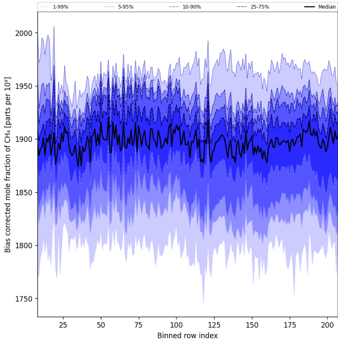
Figure 36: Along track statistics of “Bias corrected mole fraction of CH 4 ” for 2025-04-06 to 2025-04-08
