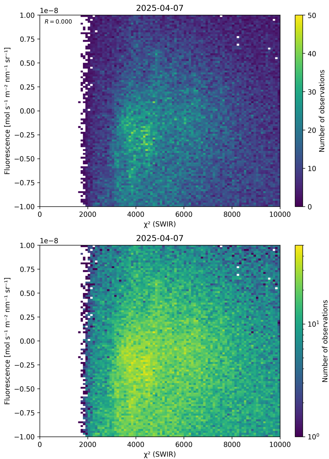
Figure 49: Scatter density plot of “ \chi^2 (SWIR)” against “Fluorescence” for 2025-04-06 to 2025-04-08.
