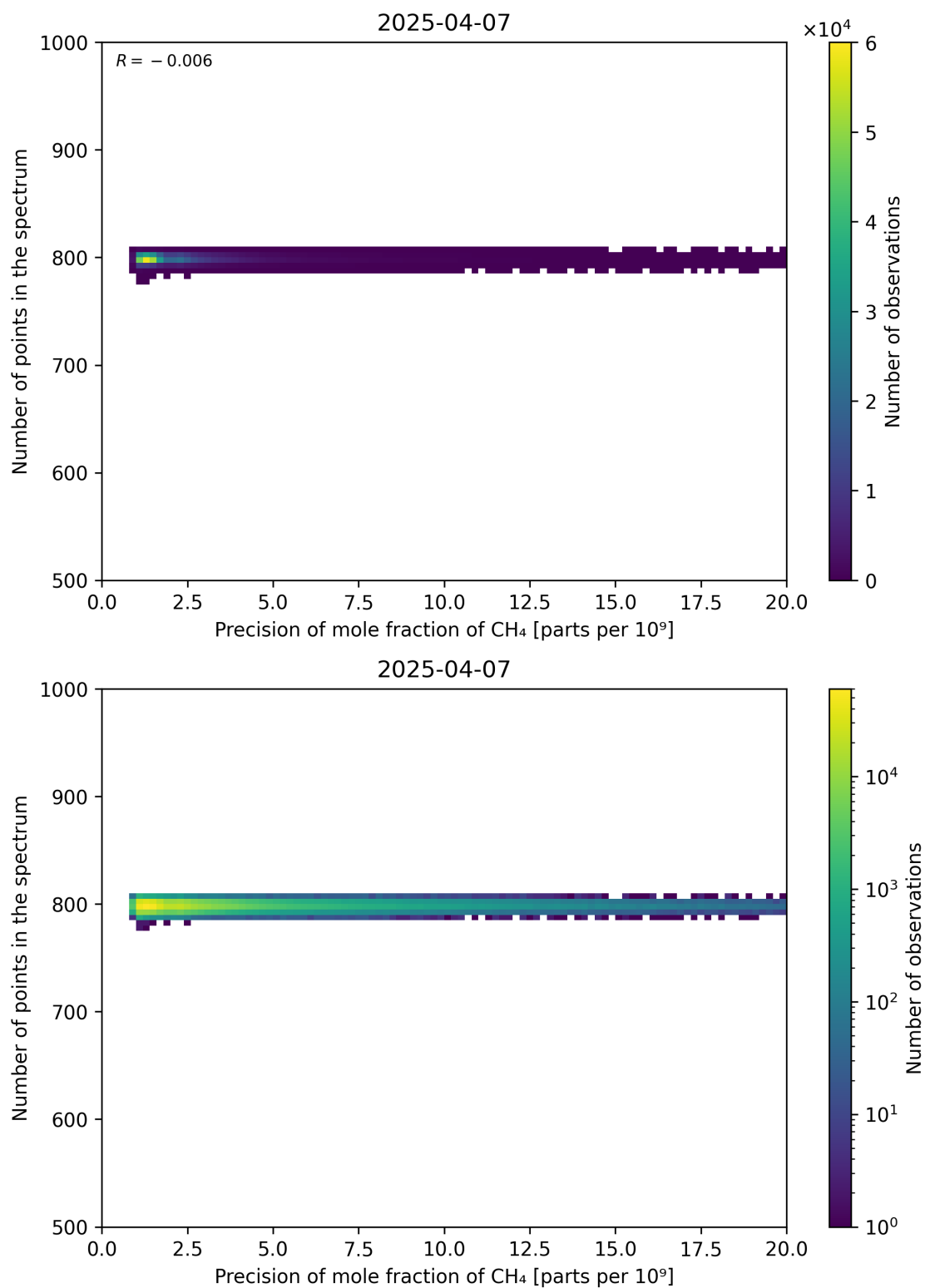
Figure 84: Scatter density plot of “Precision of mole fraction of CH 4 ” against “Number of points in the spectrum” for 2025-04-06 to 2025-04-08.
