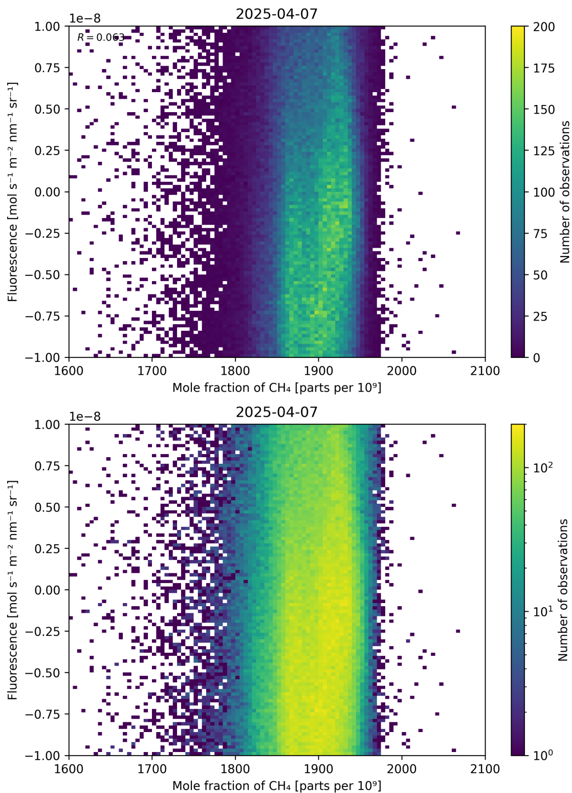
Figure 73: Scatter density plot of “Mole fraction of \text{CH}_4 ” against “Fluorescence” for 2025-04-06 to 2025-04-08.
