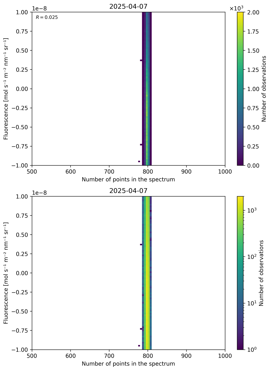
Figure 91: Scatter density plot of “Number of points in the spectrum” against “Fluorescence” for 2025-04-06 to 2025-04-08.
