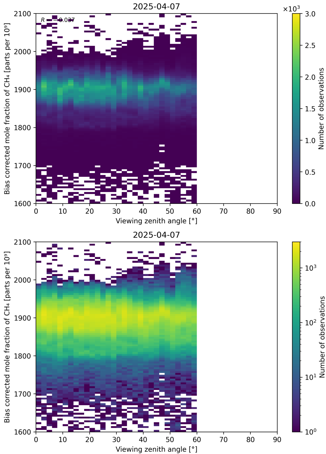
Figure 111: Scatter density plot of “Viewing zenith angle” against “Bias corrected mole fraction of CH 4 ” for 2025-04-06 to 2025-04-08.
