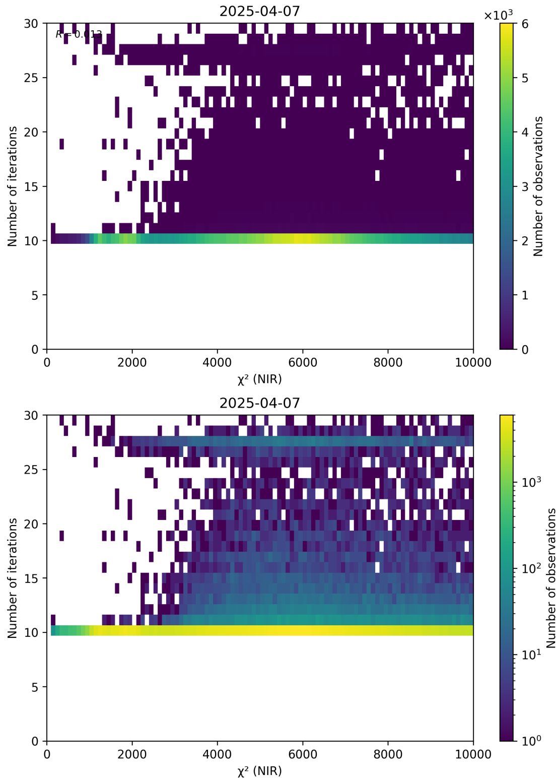
Figure 46: Scatter density plot of “ \chi^2 (NIR)” against “Number of iterations” for 2025-04-06 to 2025-04-08.
