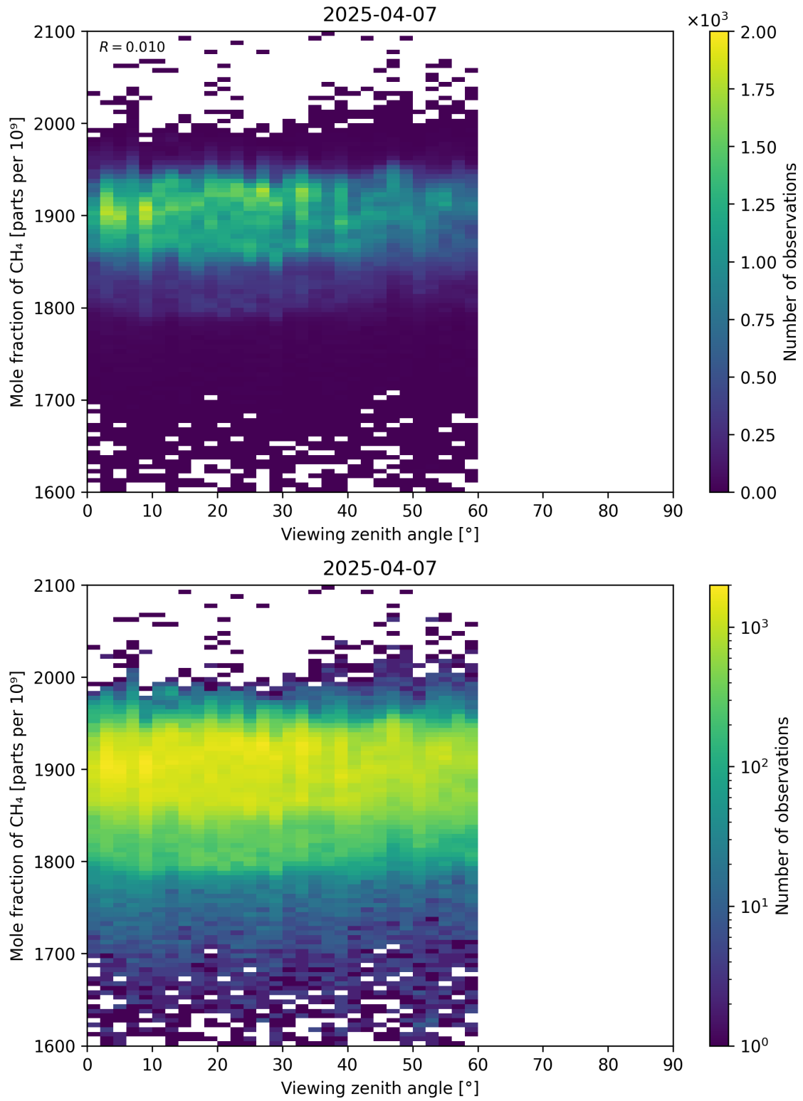
Figure 110: Scatter density plot of “Viewing zenith angle” against “Mole fraction of CH 4 ” for 2025-04-06 to 2025-04-08.
