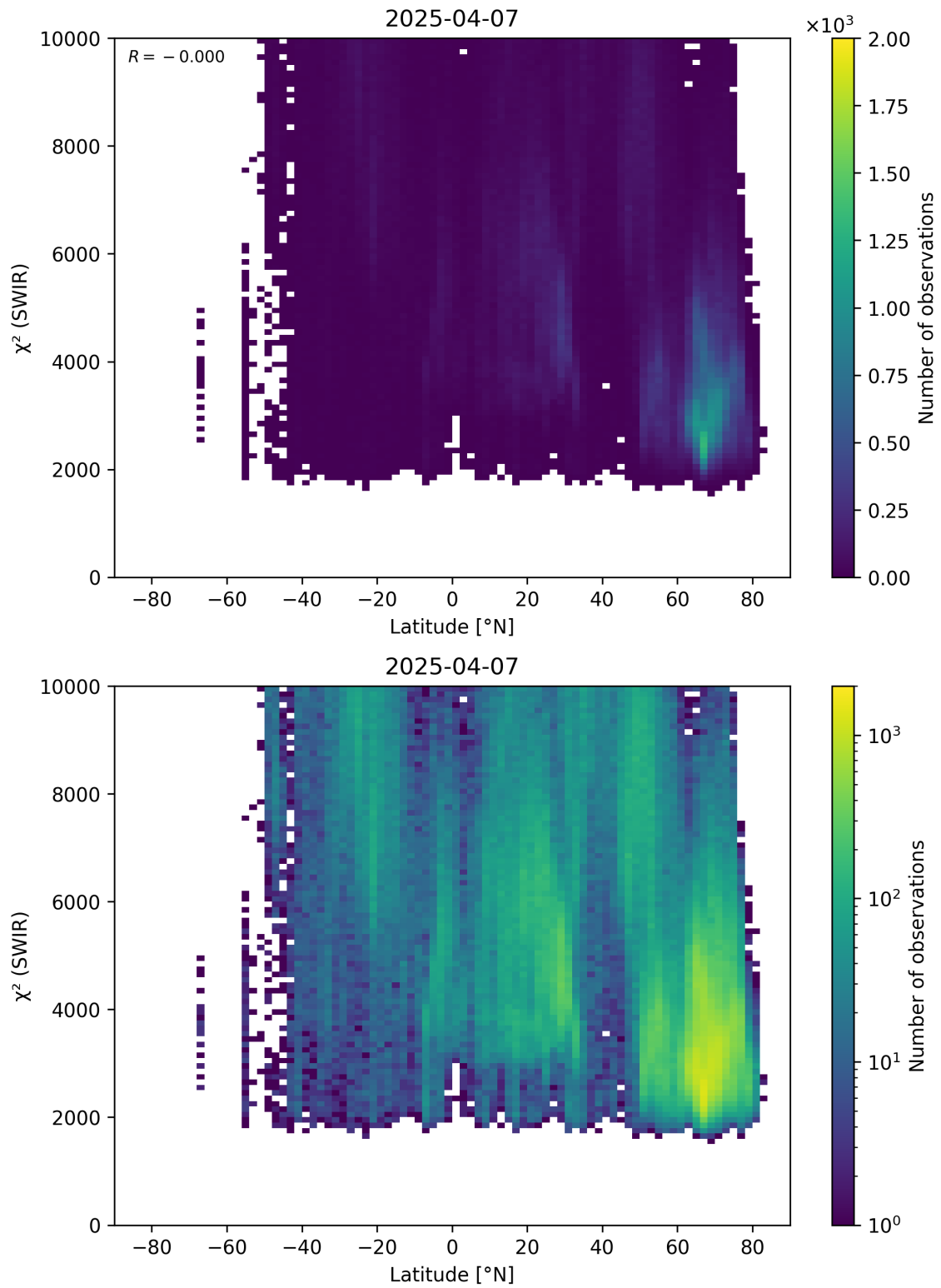
Figure 54: Scatter density plot of “Latitude” against “ \chi^2 (SWIR)” for 2025-04-06 to 2025-04-08.
