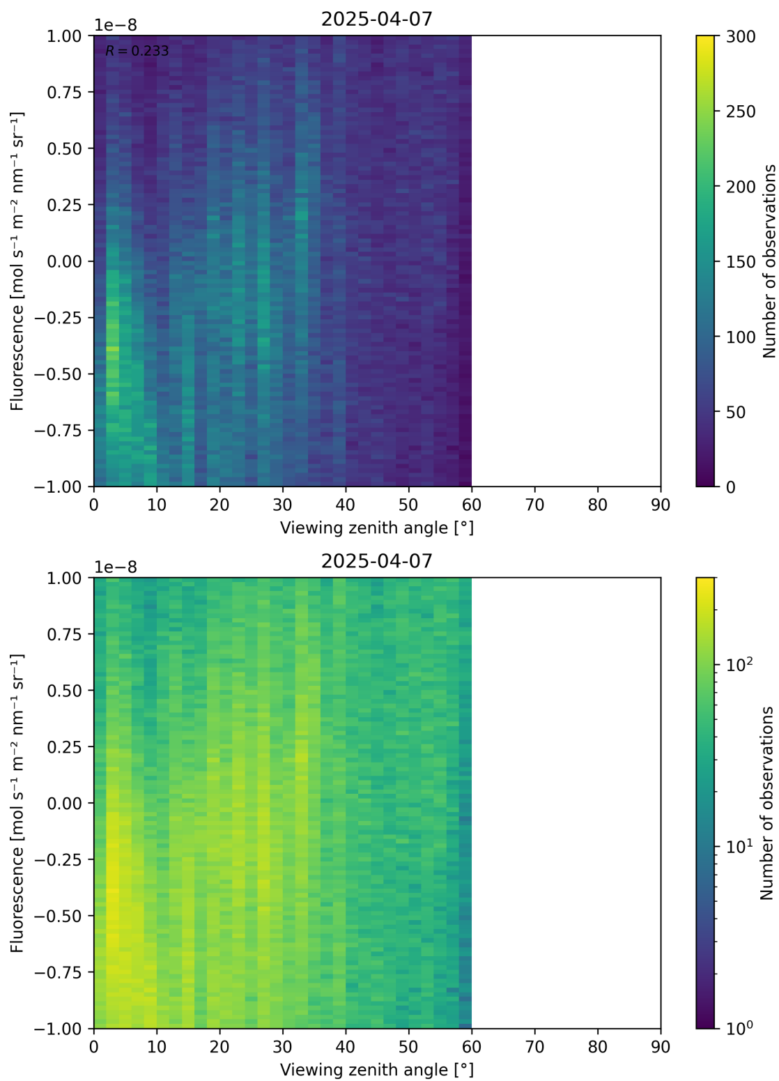
Figure 108: Scatter density plot of “Viewing zenith angle” against “Fluorescence” for 2025-04-06 to 2025-04-08.
