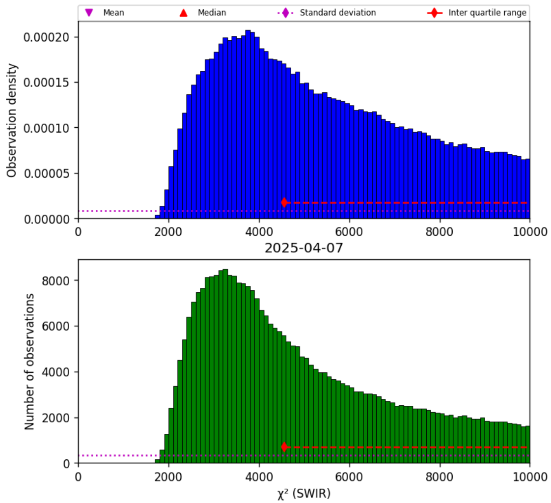
Figure 28: Histogram of “ \chi^2 (SWIR)” for 2025-04-06 to 2025-04-08
