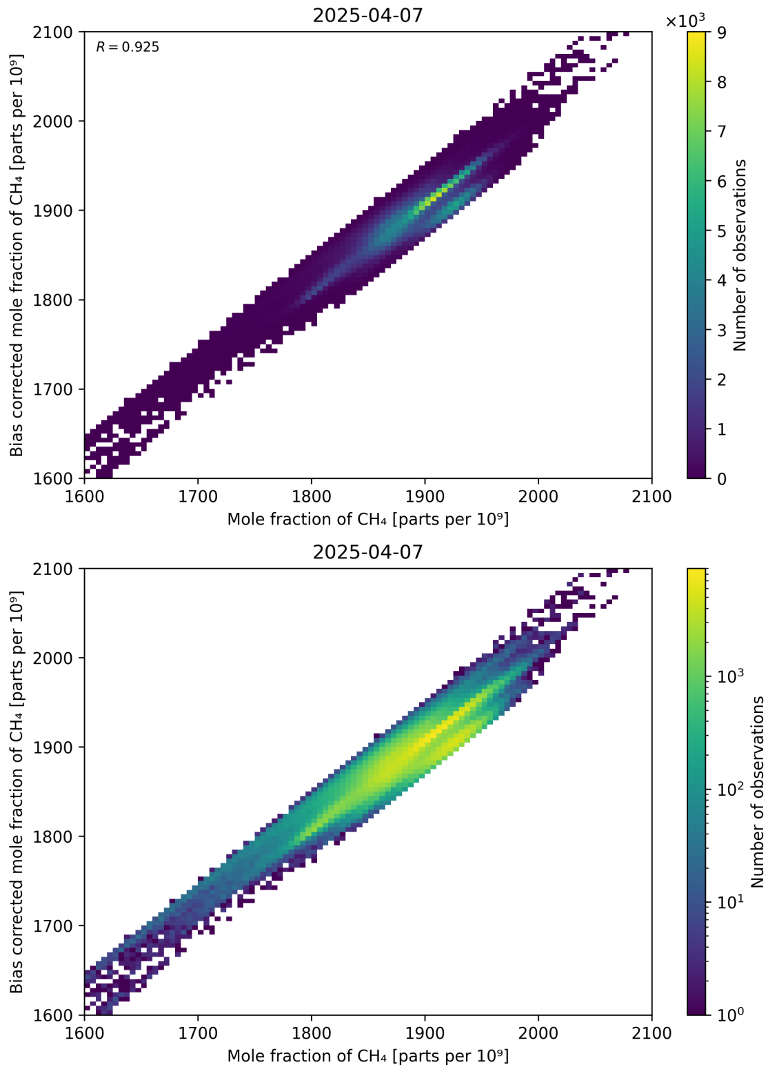
Figure 74: Scatter density plot of “Mole fraction of CH 4 ” against “Bias corrected mole fraction of CH 4 ” for 2025-04-06 to 2025-04-08.
