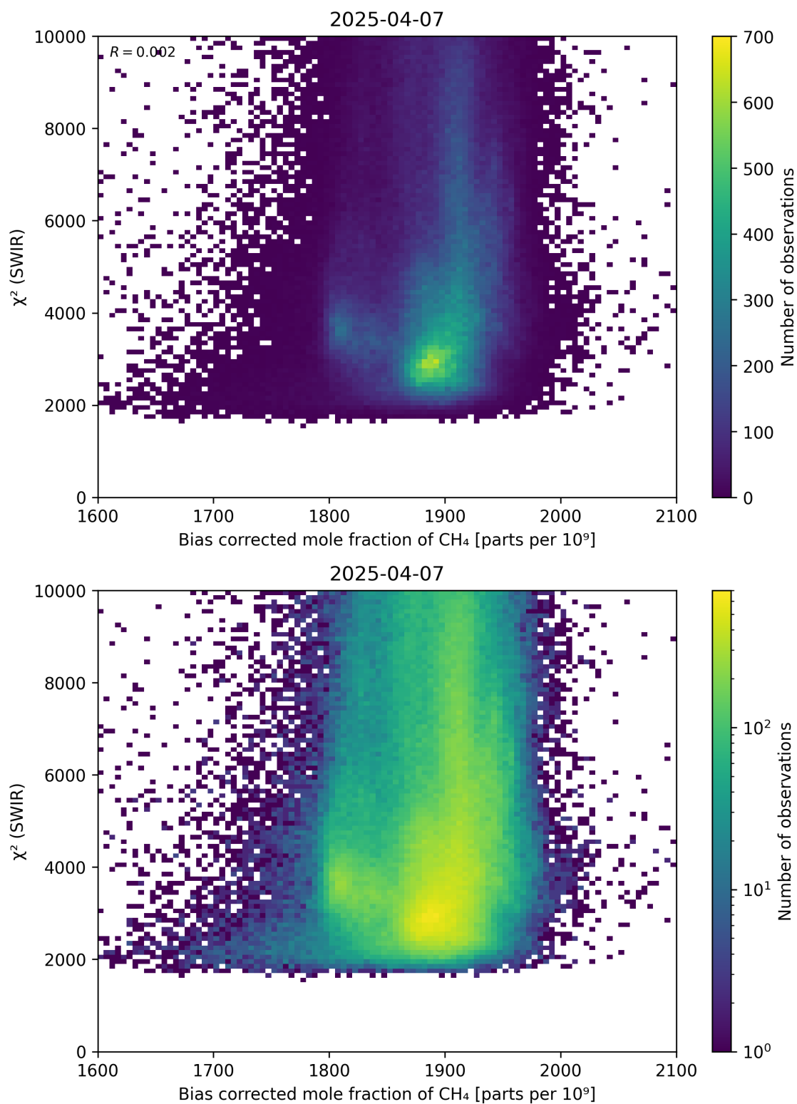
Figure 64: Scatter density plot of “Bias corrected mole fraction of \text{CH}_4 ” against “ \chi^2 (SWIR)” for 2025-04-06 to 2025-04-08.
