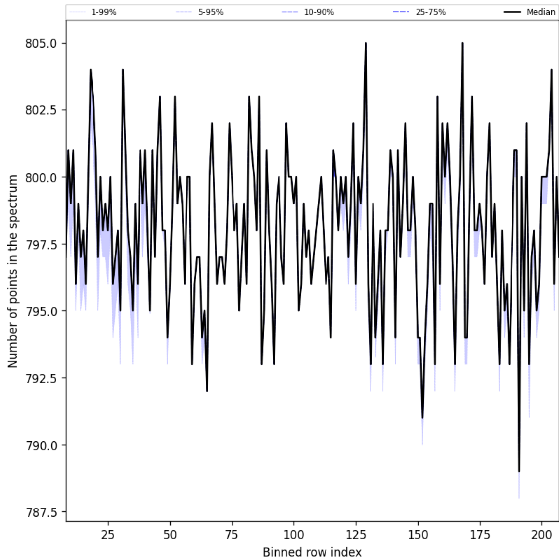
Figure 37: Along track statistics of “Number of points in the spectrum” for 2025-04-06 to 2025-04-08
