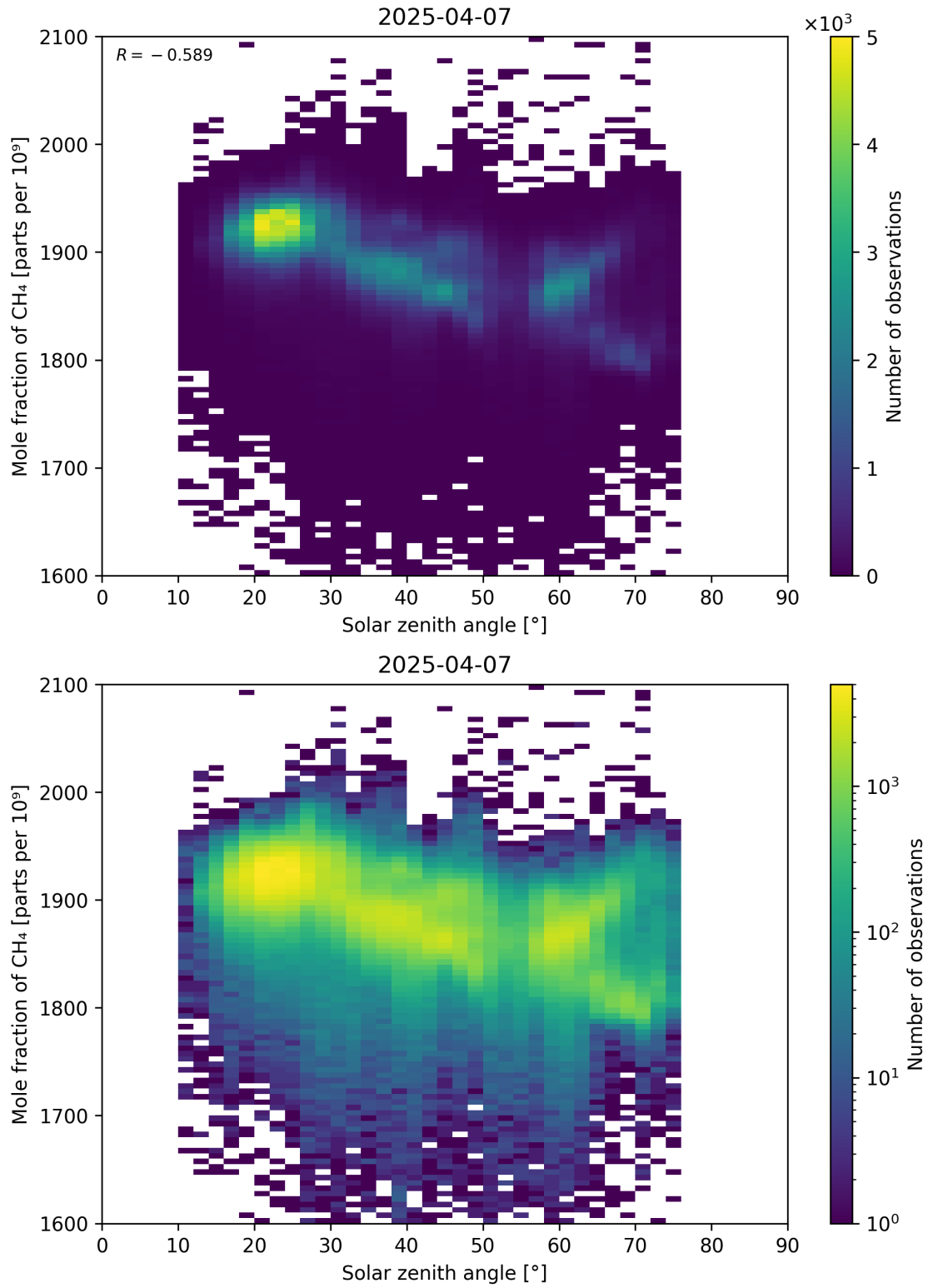
Figure 99: Scatter density plot of “Solar zenith angle” against “Mole fraction of \text{CH}_4 ” for 2025-04-06 to 2025-04-08.
