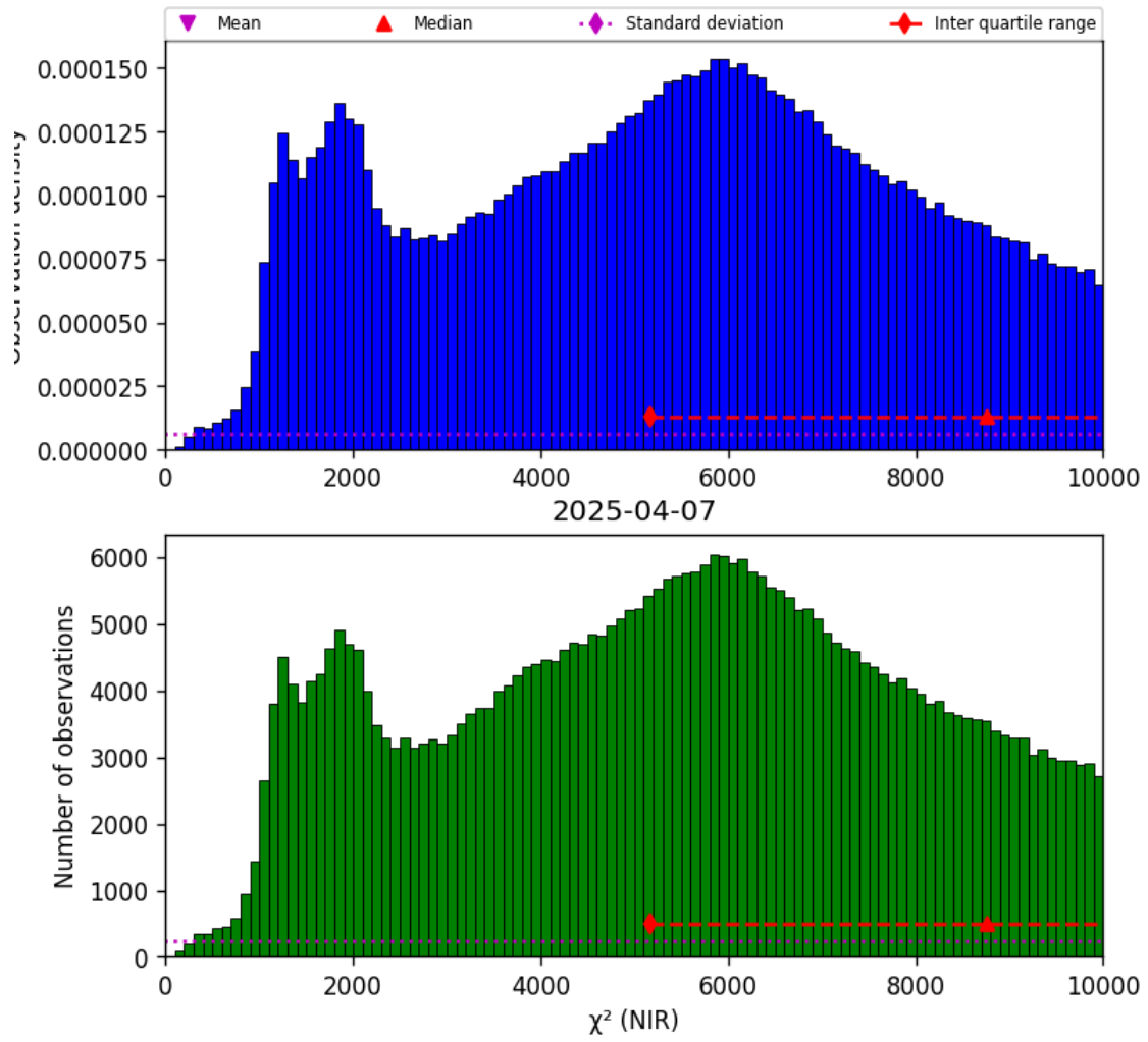
Figure 29: Histogram of “ \chi^2 (NIR)” for 2025-04-06 to 2025-04-08
