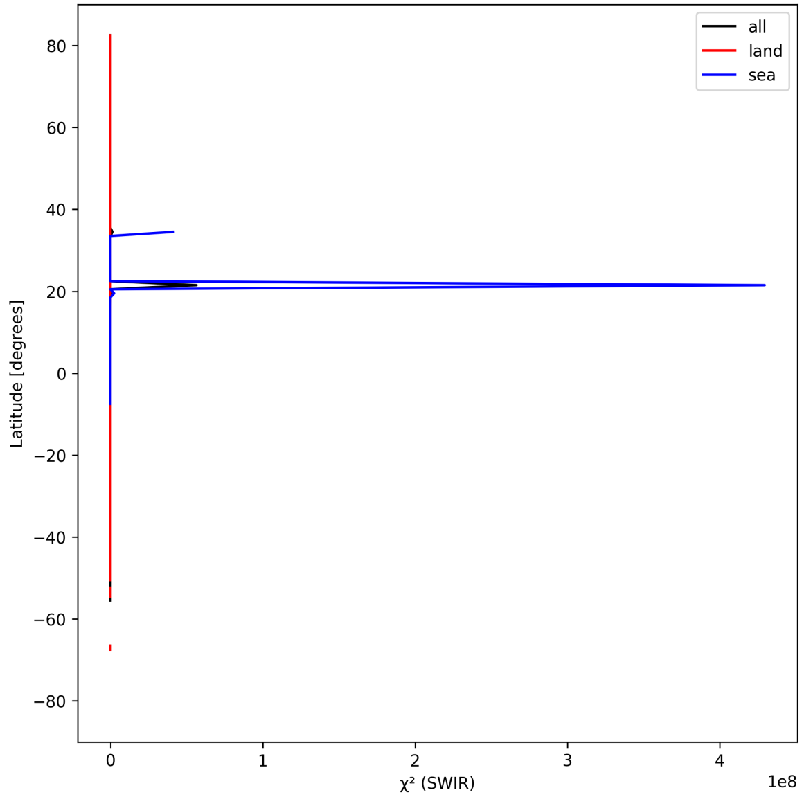
Figure 17: Zonal average of “ \chi^2 (SWIR)” for 2025-04-06 to 2025-04-08.
