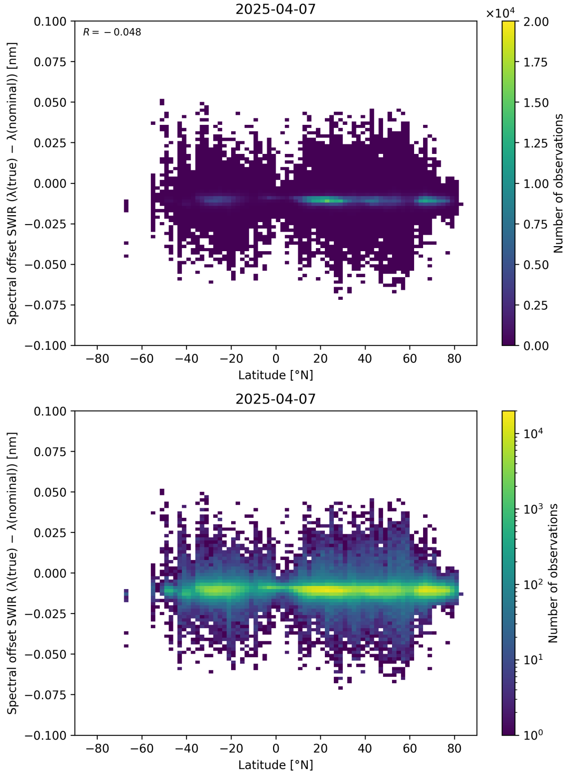
Figure 62: Scatter density plot of “Latitude” against “Spectral offset SWIR ( \lambda_{\text{true}} - \lambda_{\text{nominal}} )” for 2025-04-06 to 2025-04-08.
