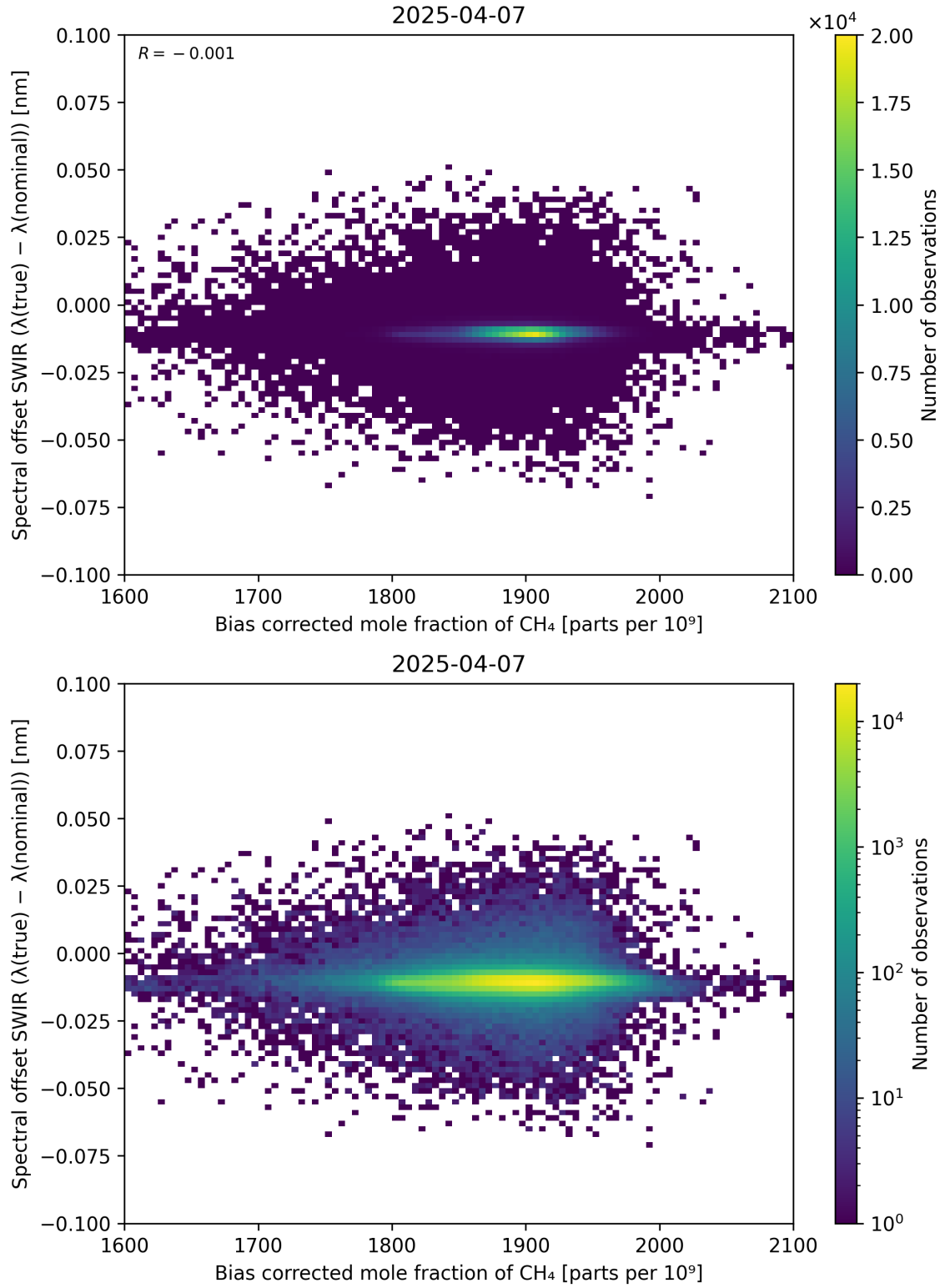
Figure 69: Scatter density plot of “Bias corrected mole fraction of \text{CH}_4 ” against “Spectral offset SWIR ( \lambda_{\text{true}} - \lambda_{\text{nominal}} )” for 2025-04-06 to 2025-04-08.
