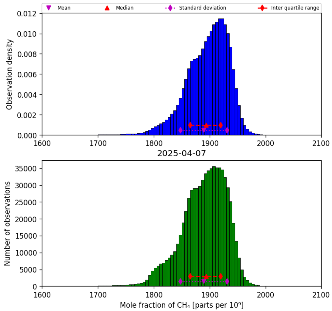
Figure 23: Histogram of “Mole fraction of CH 4 ” for 2025-04-06 to 2025-04-08
