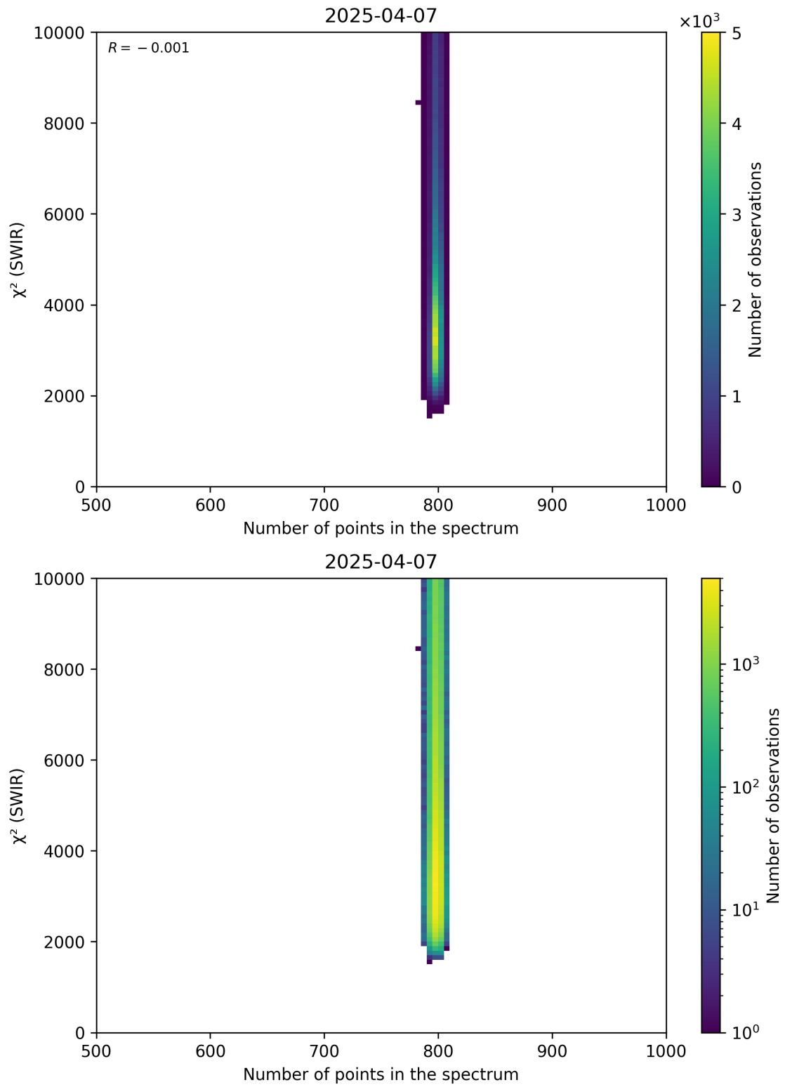
Figure 89: Scatter density plot of “Number of points in the spectrum” against “ \chi^2 (SWIR)” for 2025-04-06 to 2025-04-08.
