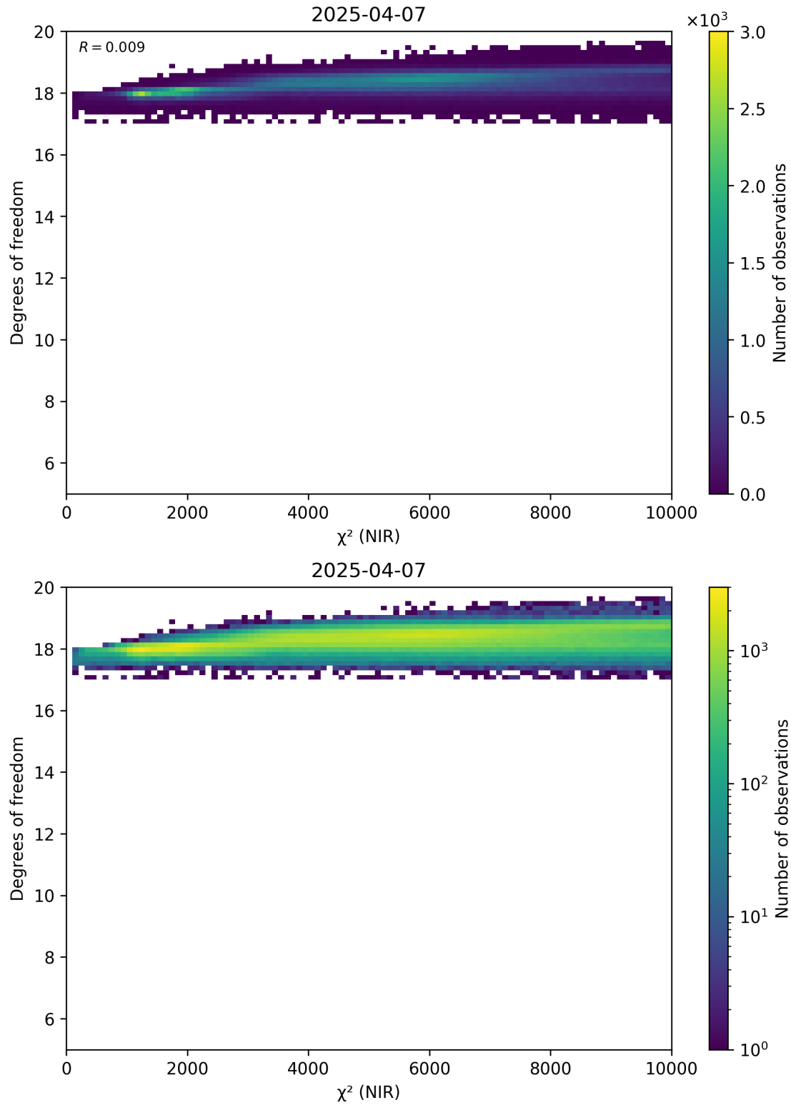
Figure 44: Scatter density plot of “ \chi^2 (NIR)” against “Degrees of freedom” for 2025-04-06 to 2025-04-08.
