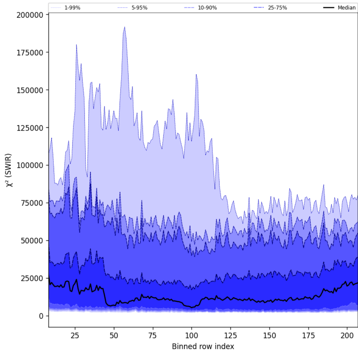
Figure 39: Along track statistics of “ \chi^2 (SWIR)” for 2025-04-06 to 2025-04-08
