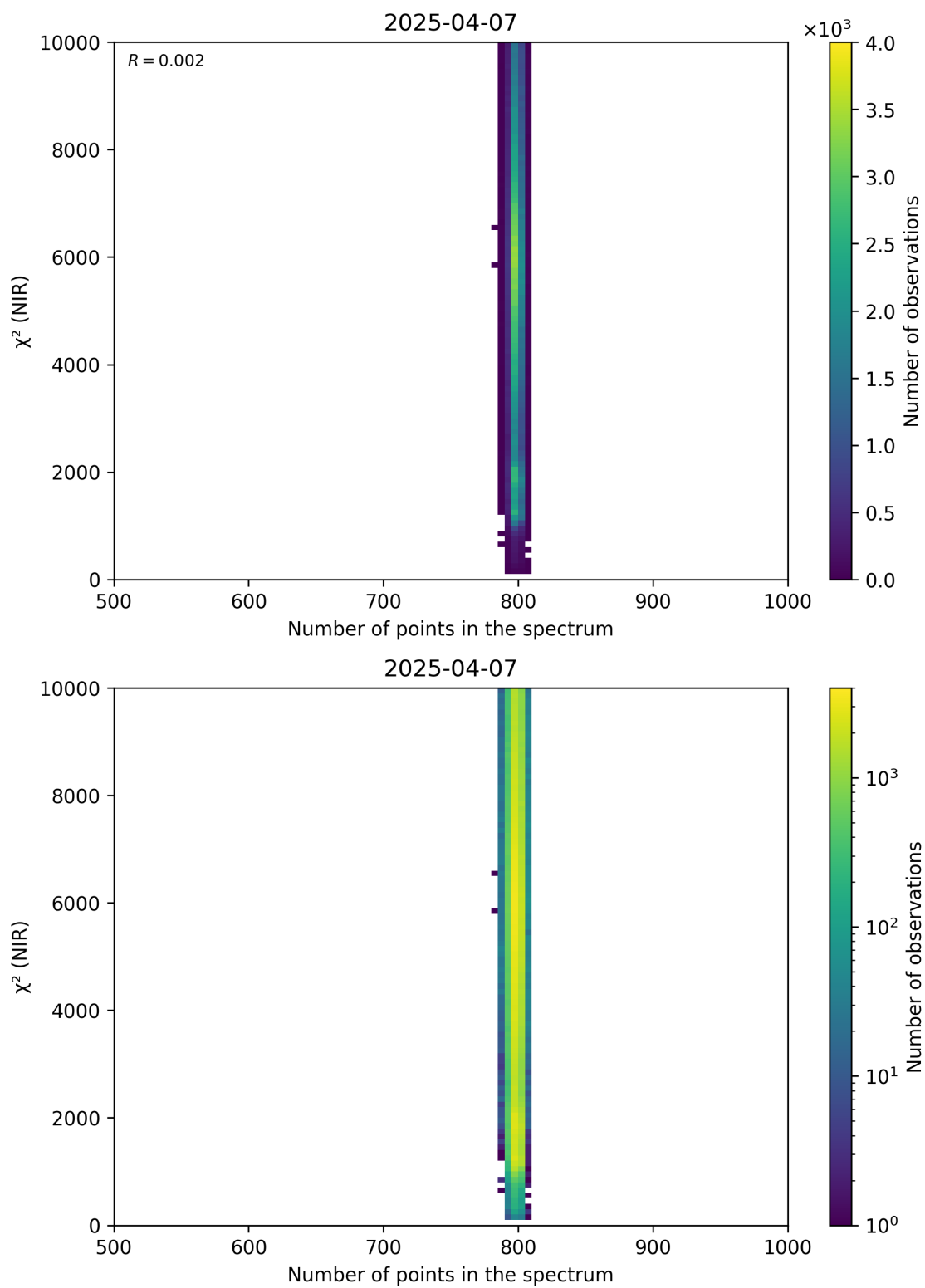
Figure 88: Scatter density plot of “Number of points in the spectrum” against “ \chi^2 (NIR)” for 2025-04-06 to 2025-04-08.
