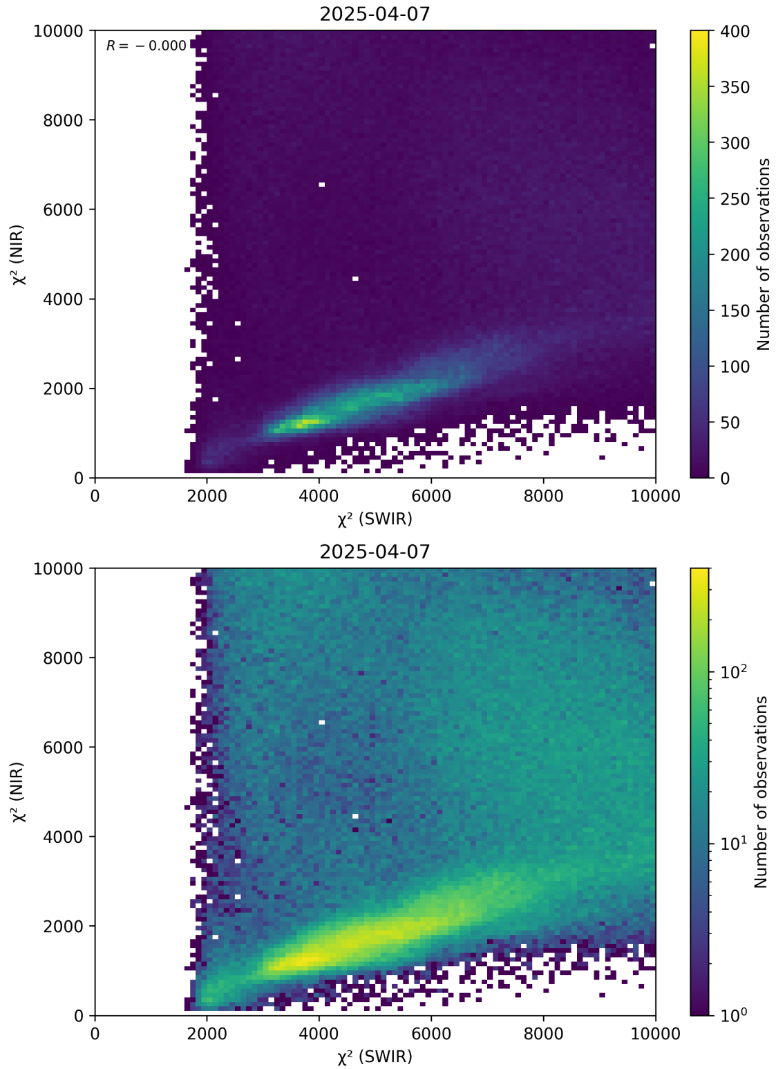
Figure 47: Scatter density plot of “ \chi^2 (SWIR)” against “ \chi^2 (NIR)” for 2025-04-06 to 2025-04-08.
