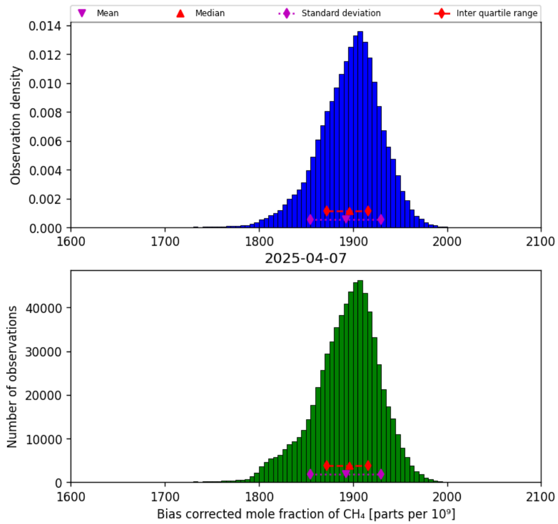
Figure 25: Histogram of “Bias corrected mole fraction of CH 4 ” for 2025-04-06 to 2025-04-08
