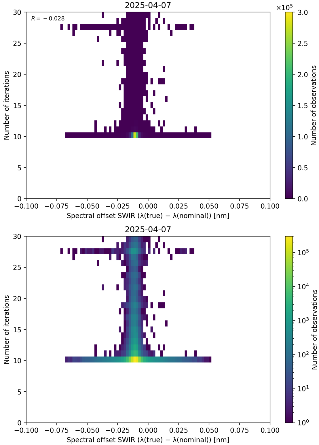
Figure 121: Scatter density plot of “Spectral offset SWIR ( \lambda_{\text{true}} - \lambda_{\text{nominal}} )” against “Number of iterations” for 2025-04-06 to 2025-04-08.
