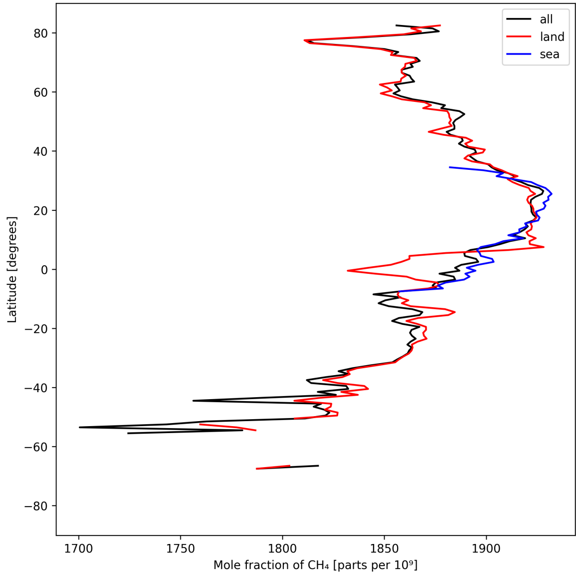
Figure 12: Zonal average of “Mole fraction of \text{CH}_4 ” for 2025-04-06 to 2025-04-08.
