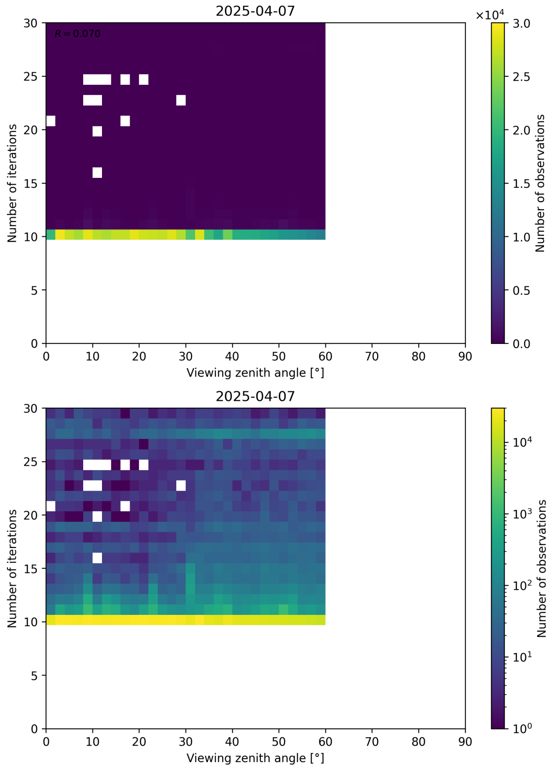
Figure 113: Scatter density plot of “Viewing zenith angle” against “Number of iterations” for 2025-04-06 to 2025-04-08.
