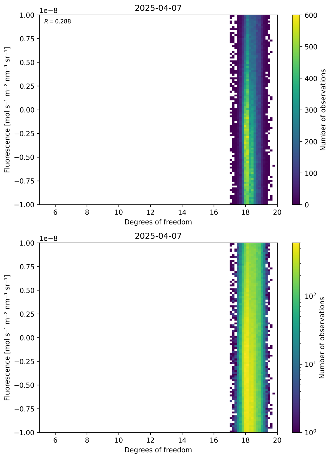
Figure 51: Scatter density plot of “Degrees of freedom” against “Fluorescence” for 2025-04-06 to 2025-04-08.
