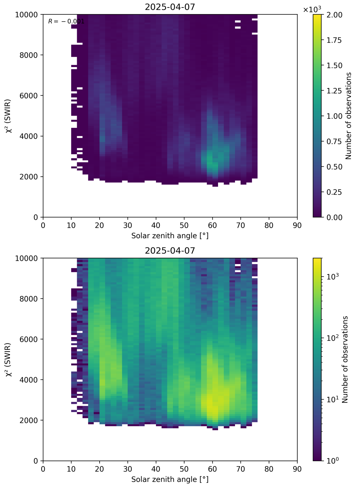
Figure 95: Scatter density plot of “Solar zenith angle” against “ \chi^2 (SWIR)” for 2025-04-06 to 2025-04-08.
