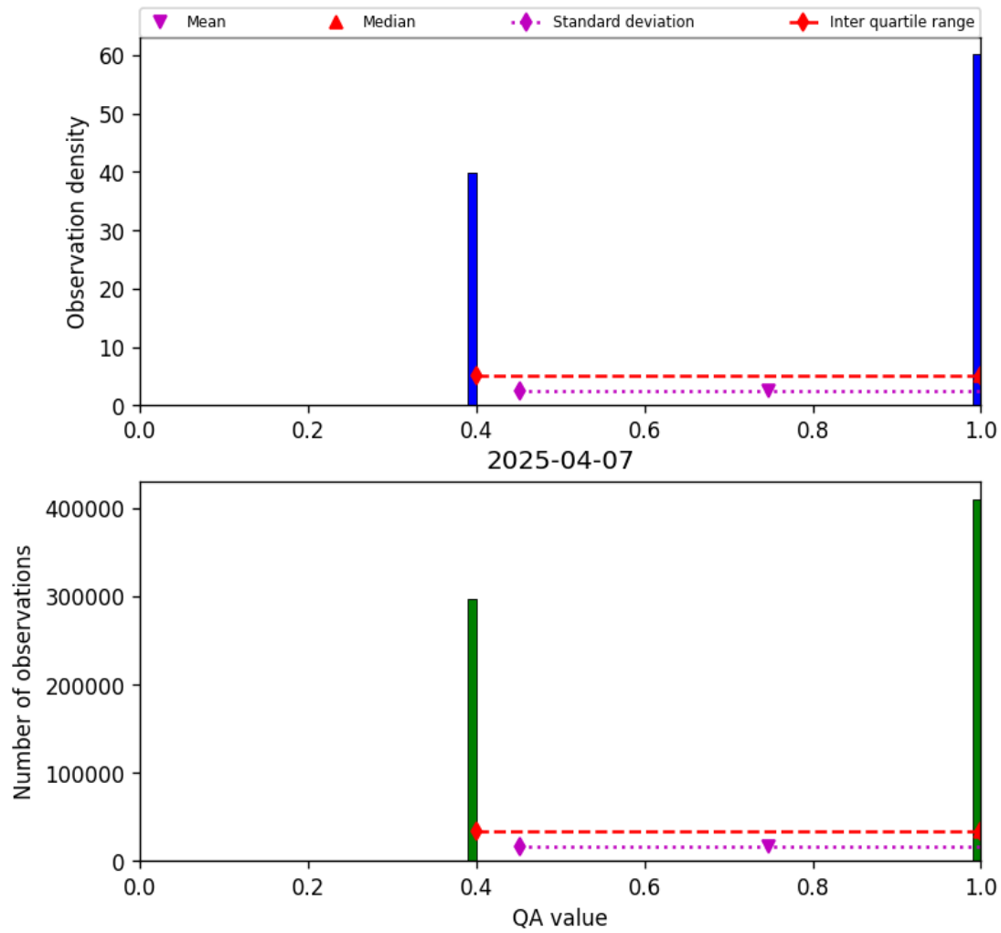
Figure 22: Histogram of “QA value” for 2025-04-06 to 2025-04-08
