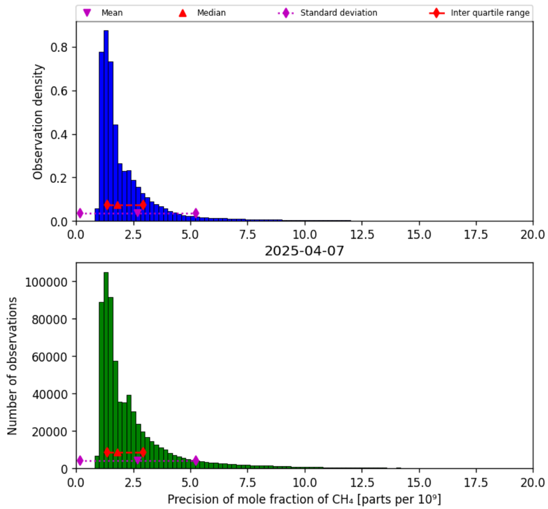
Figure 24: Histogram of “Precision of mole fraction of CH 4 ” for 2025-04-06 to 2025-04-08
