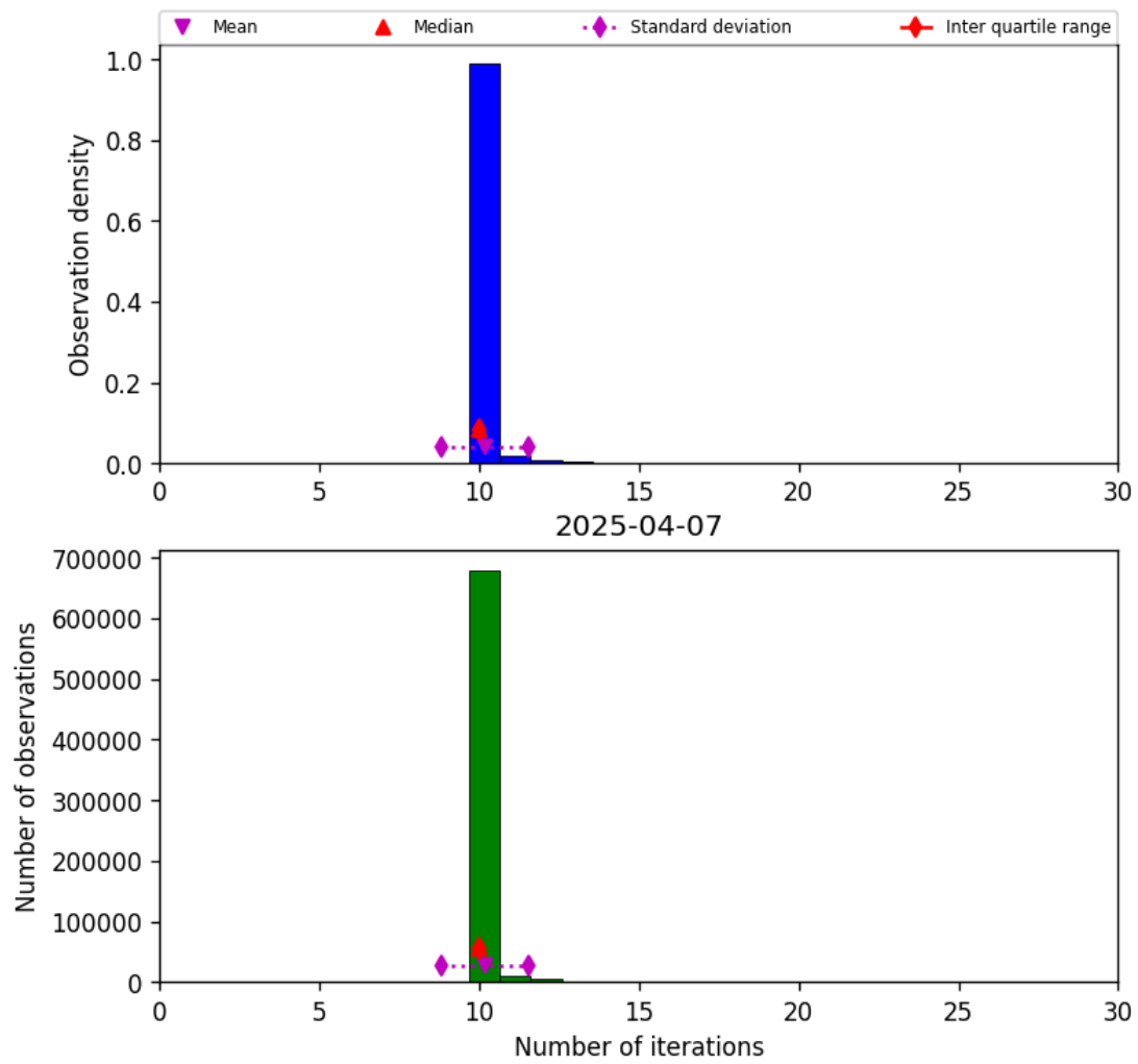
Figure 31: Histogram of “Number of iterations” for 2025-04-06 to 2025-04-08
