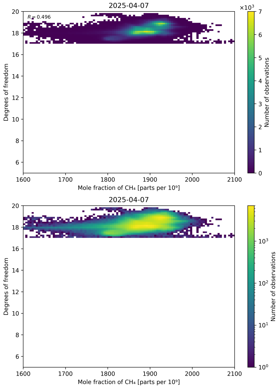
Figure 72: Scatter density plot of “Mole fraction of CH 4 ” against “Degrees of freedom” for 2025-04-06 to 2025-04-08.
