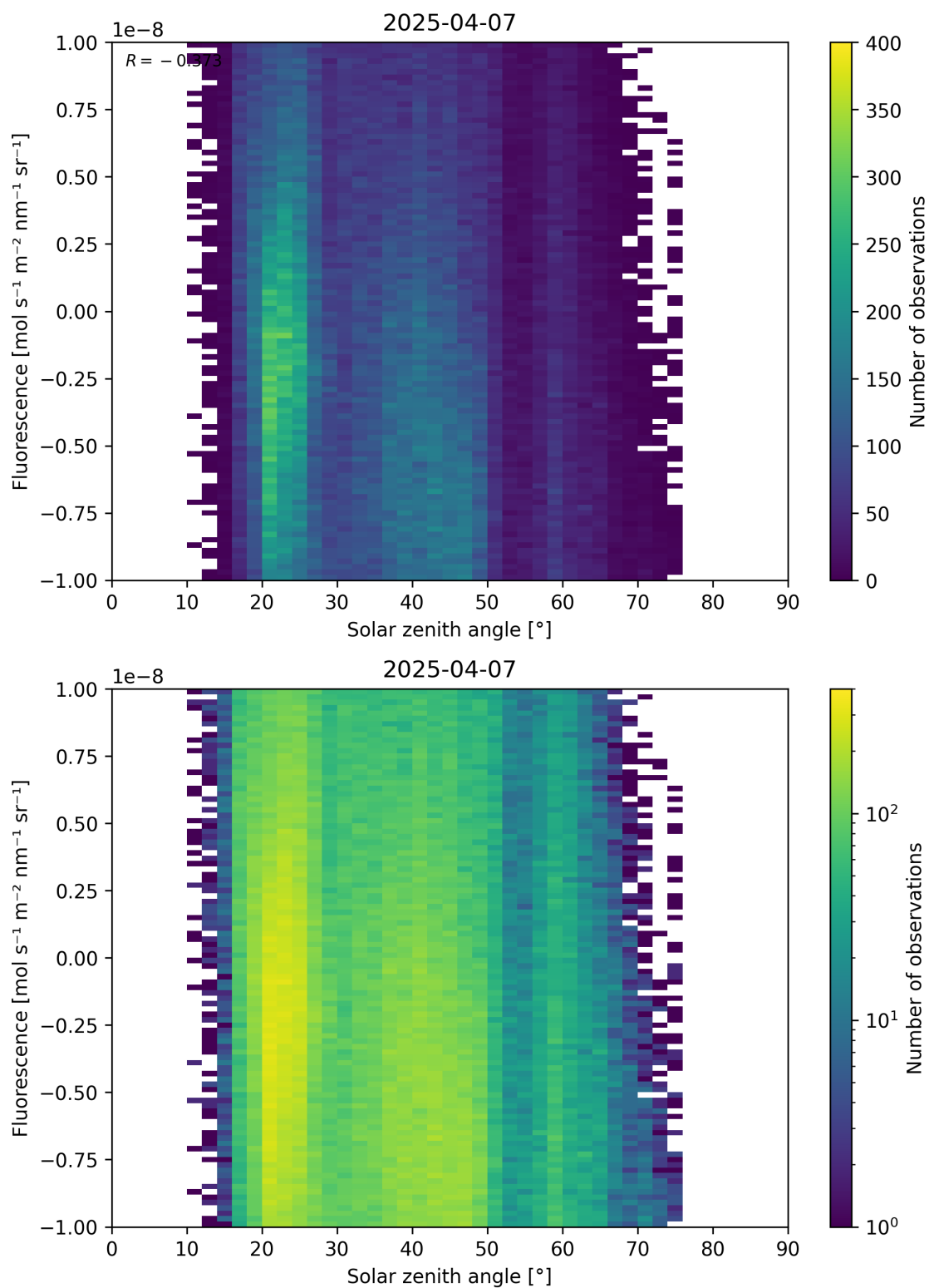
Figure 97: Scatter density plot of “Solar zenith angle” against “Fluorescence” for 2025-04-06 to 2025-04-08.
