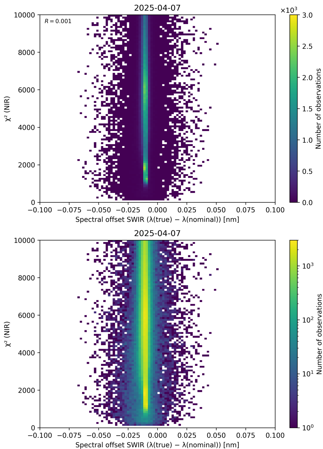
Figure 117: Scatter density plot of “Spectral offset SWIR ( \lambda_{\text{true}} - \lambda_{\text{nominal}} )” against “ \chi^2 (NIR)” for 2025-04-06 to 2025-04-08.
