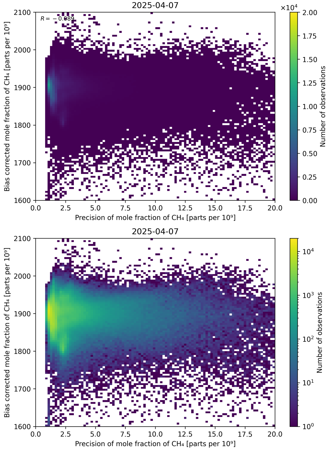
Figure 82: Scatter density plot of “Precision of mole fraction of CH 4 ” against “Bias corrected mole fraction of CH 4 ” for 2025-04-06 to 2025-04-08.
