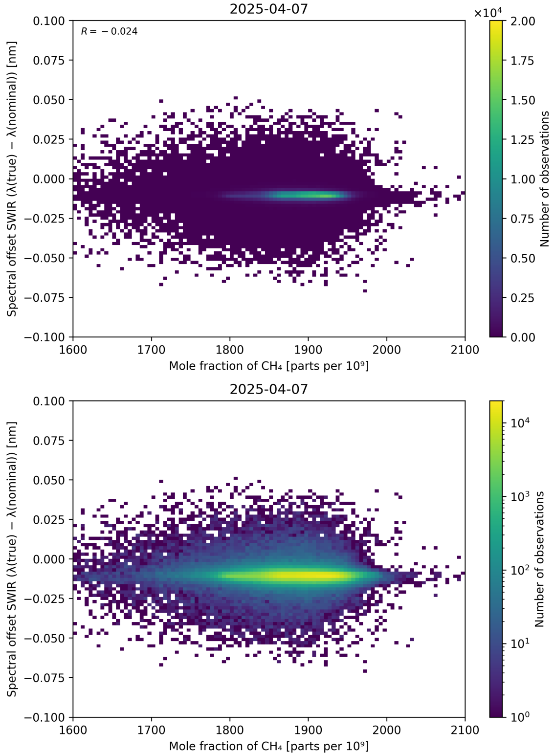
Figure 86: Scatter density plot of “Mole fraction of CH 4 ” against “Spectral offset SWIR ( \lambda_{\text{true}} - \lambda_{\text{nominal}} )” for 2025-04-06 to 2025-04-08.
