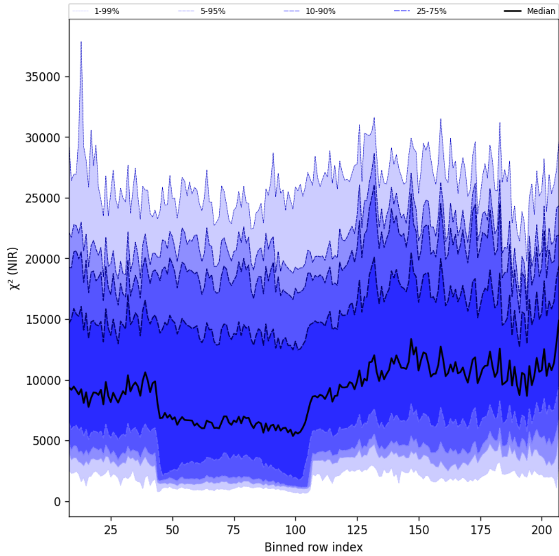
Figure 40: Along track statistics of “ \chi^2 (NIR)” for 2025-04-06 to 2025-04-08
