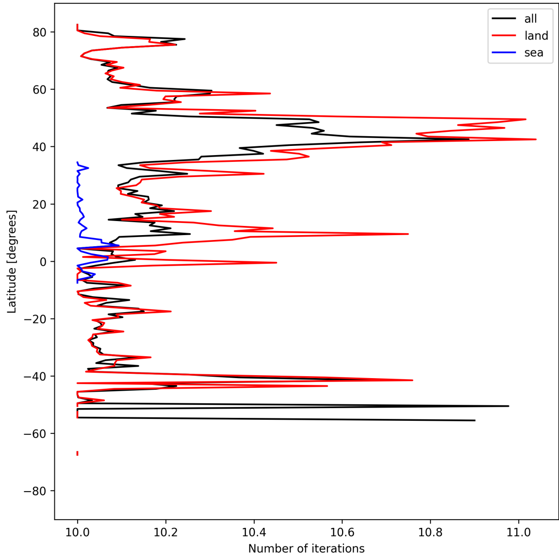
Figure 20: Zonal average of “Number of iterations” for 2025-04-06 to 2025-04-08.
