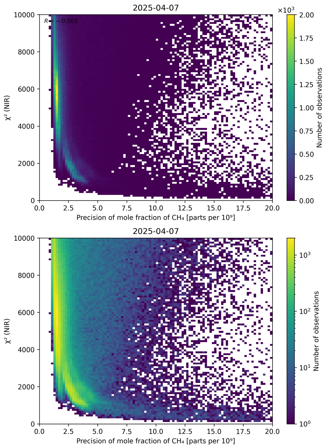
Figure 78: Scatter density plot of “Precision of mole fraction of CH 4 ” against “ \chi^2 (NIR)” for 2025-04-06 to 2025-04-08.
