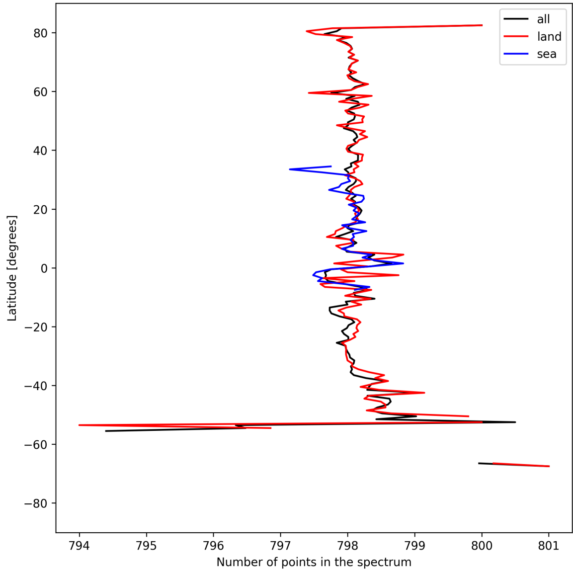
Figure 15: Zonal average of “Number of points in the spectrum” for 2025-04-06 to 2025-04-08.
