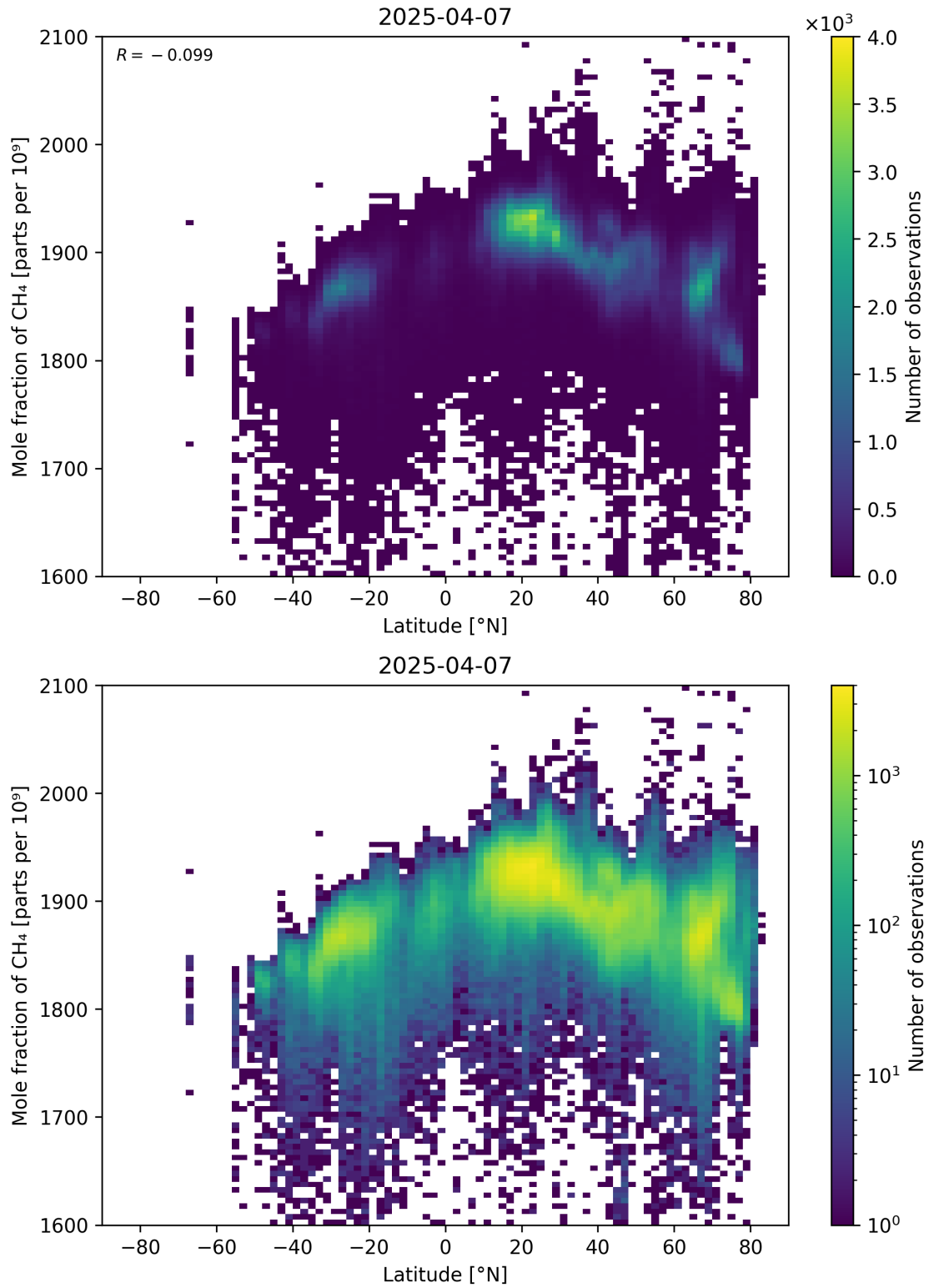
Figure 57: Scatter density plot of “Latitude” against “Mole fraction of CH 4 ” for 2025-04-06 to 2025-04-08.
