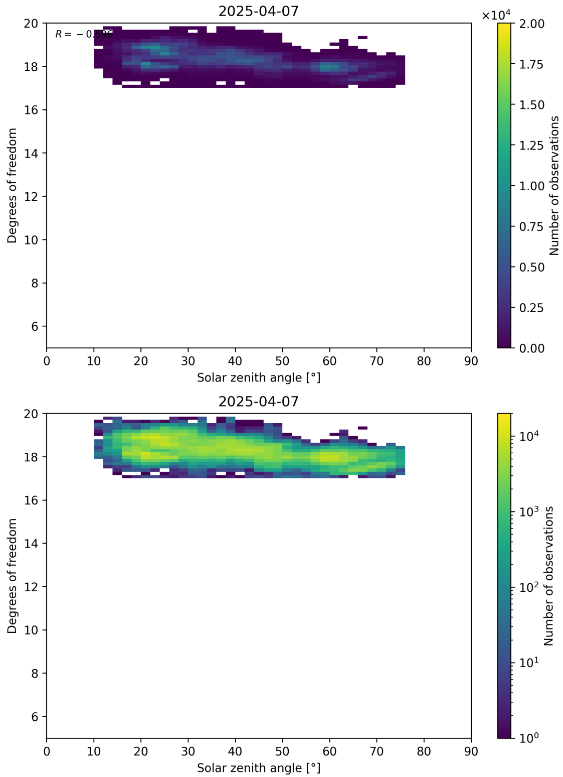
Figure 96: Scatter density plot of “Solar zenith angle” against “Degrees of freedom” for 2025-04-06 to 2025-04-08.
