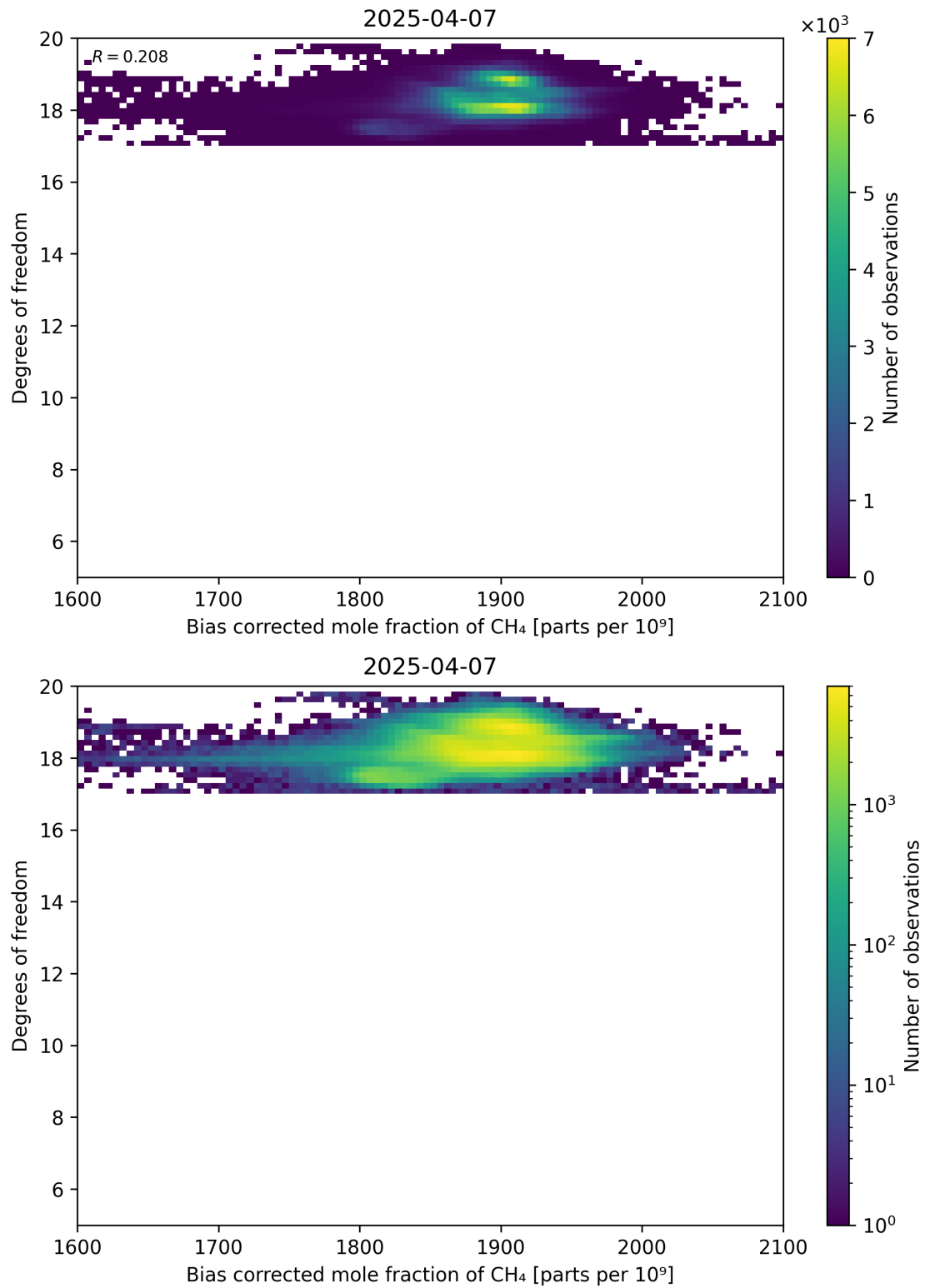
Figure 65: Scatter density plot of “Bias corrected mole fraction of CH 4 ” against “Degrees of freedom” for 2025-04-06 to 2025-04-08.
