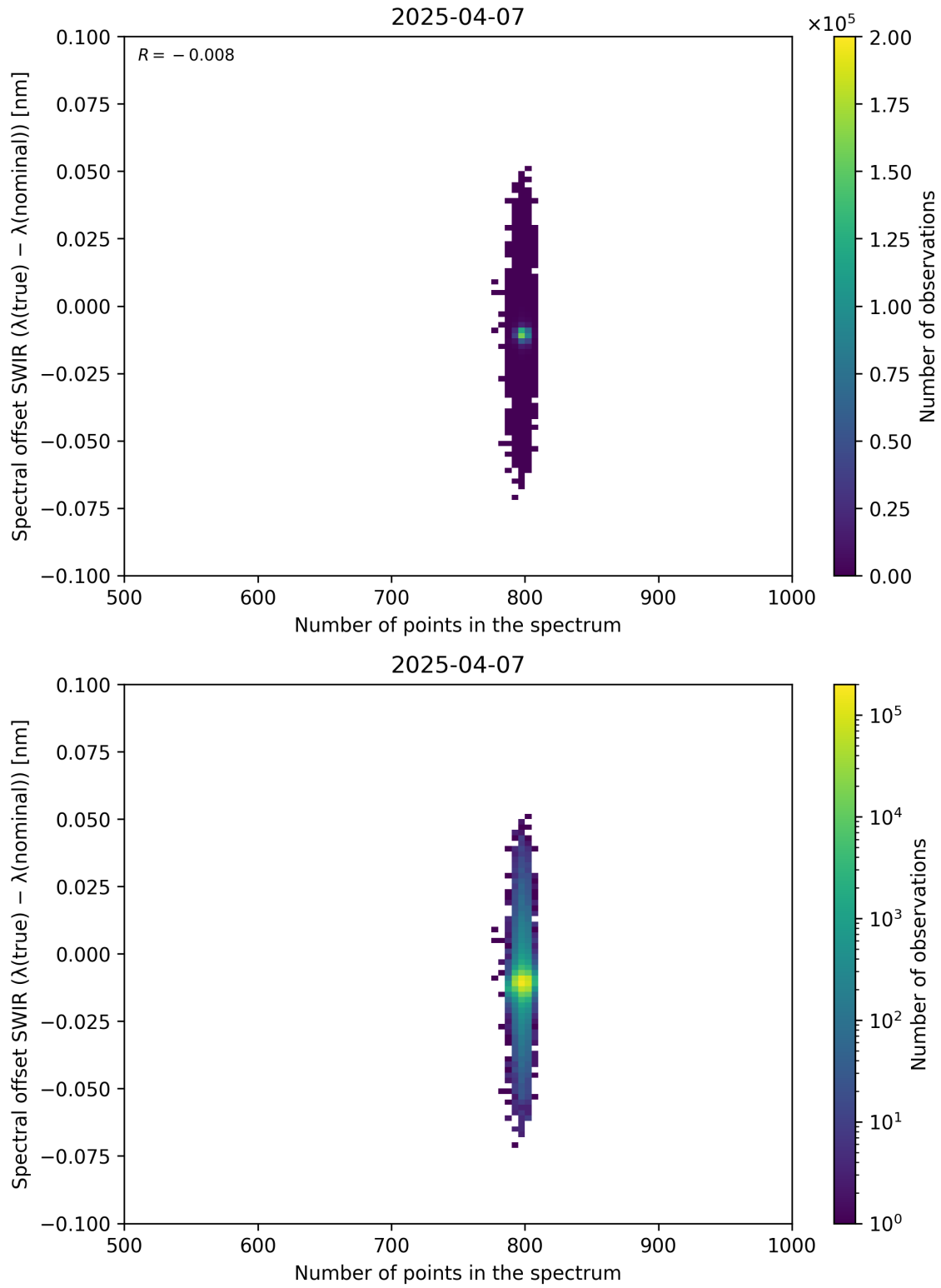
Figure 93: Scatter density plot of “Number of points in the spectrum” against “Spectral offset SWIR ( \lambda_{\text{true}} - \lambda_{\text{nominal}} )” for 2025-04-06 to 2025-04-08.
