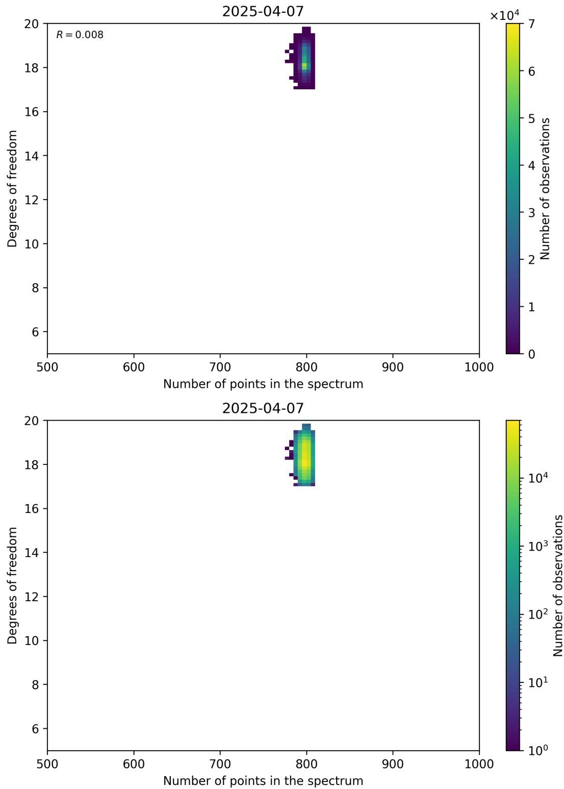
Figure 90: Scatter density plot of “Number of points in the spectrum” against “Degrees of freedom” for 2025-04-06 to 2025-04-08.
