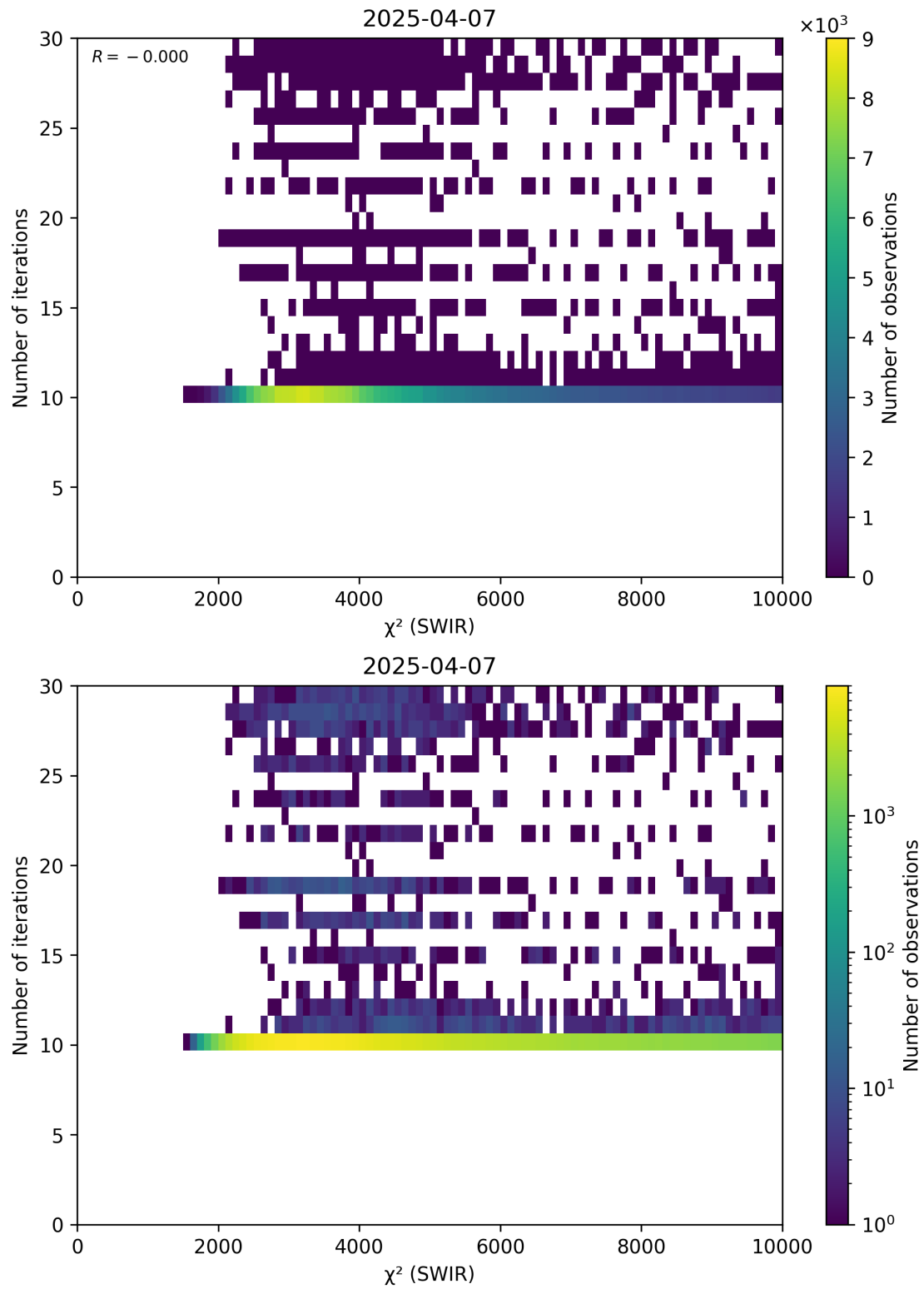
Figure 50: Scatter density plot of “ \chi^2 (SWIR)” against “Number of iterations” for 2025-04-06 to 2025-04-08.
