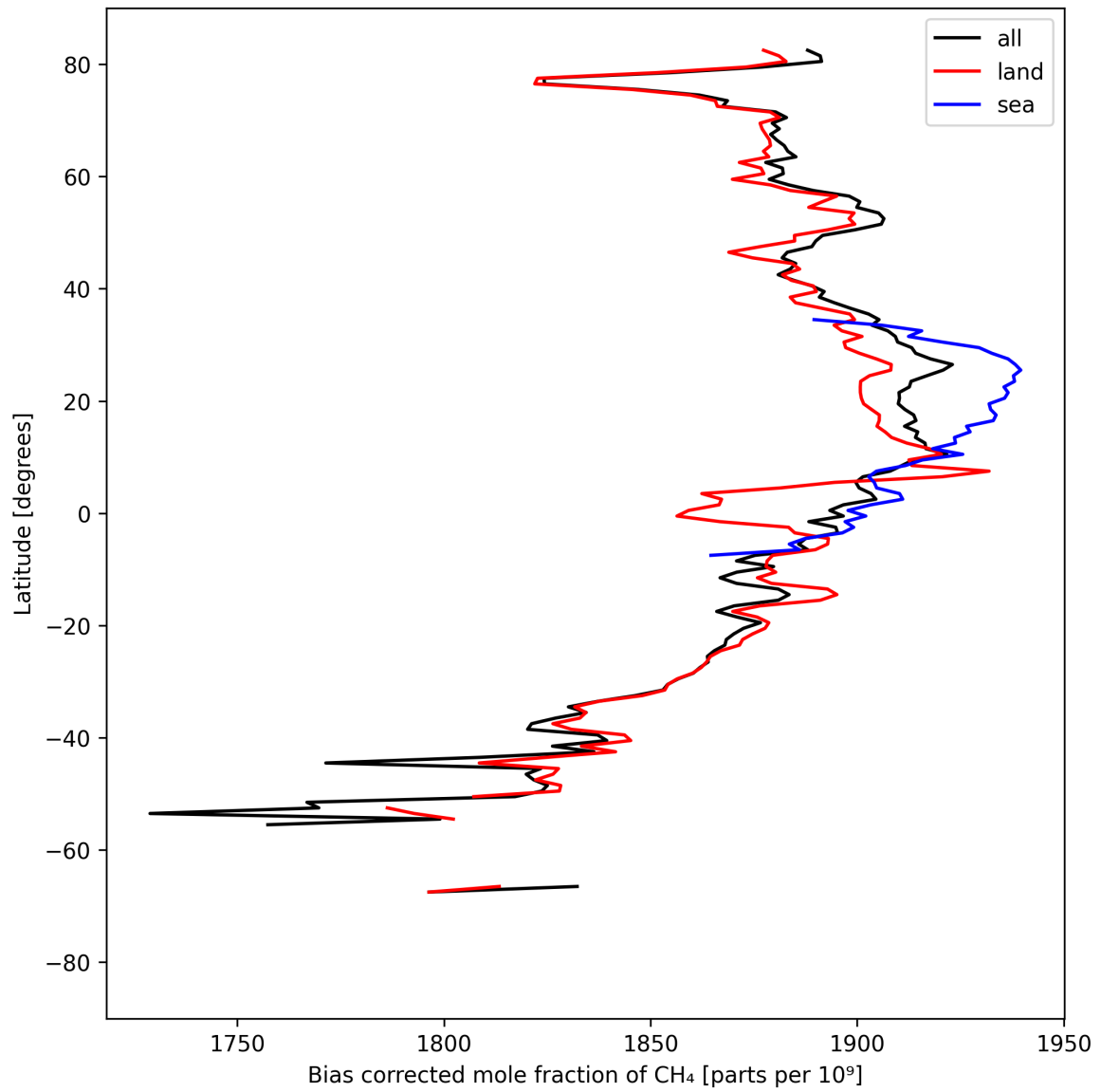
Figure 14: Zonal average of “Bias corrected mole fraction of CH 4 ” for 2025-04-06 to 2025-04-08.
