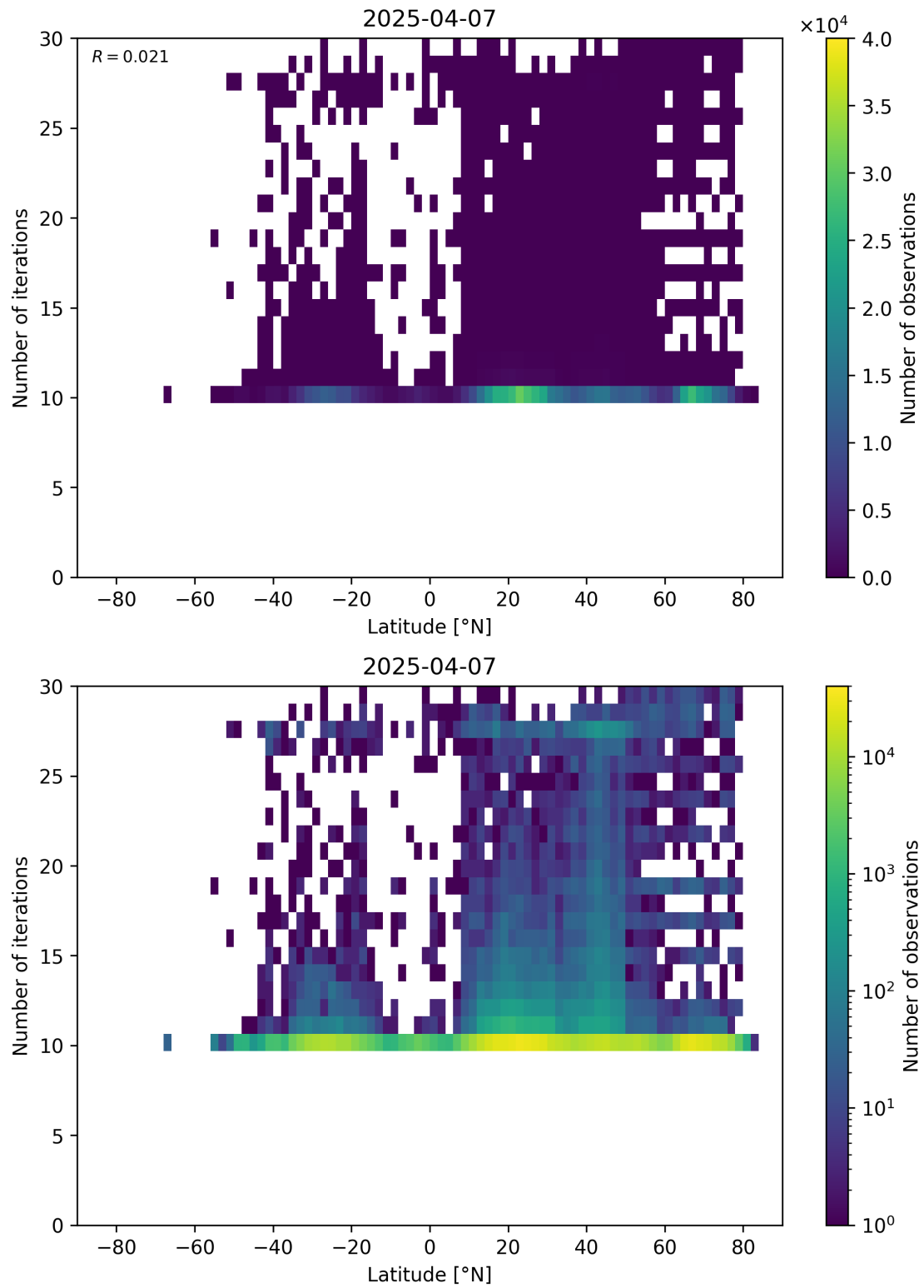
Figure 60: Scatter density plot of “Latitude” against “Number of iterations” for 2025-04-06 to 2025-04-08.
