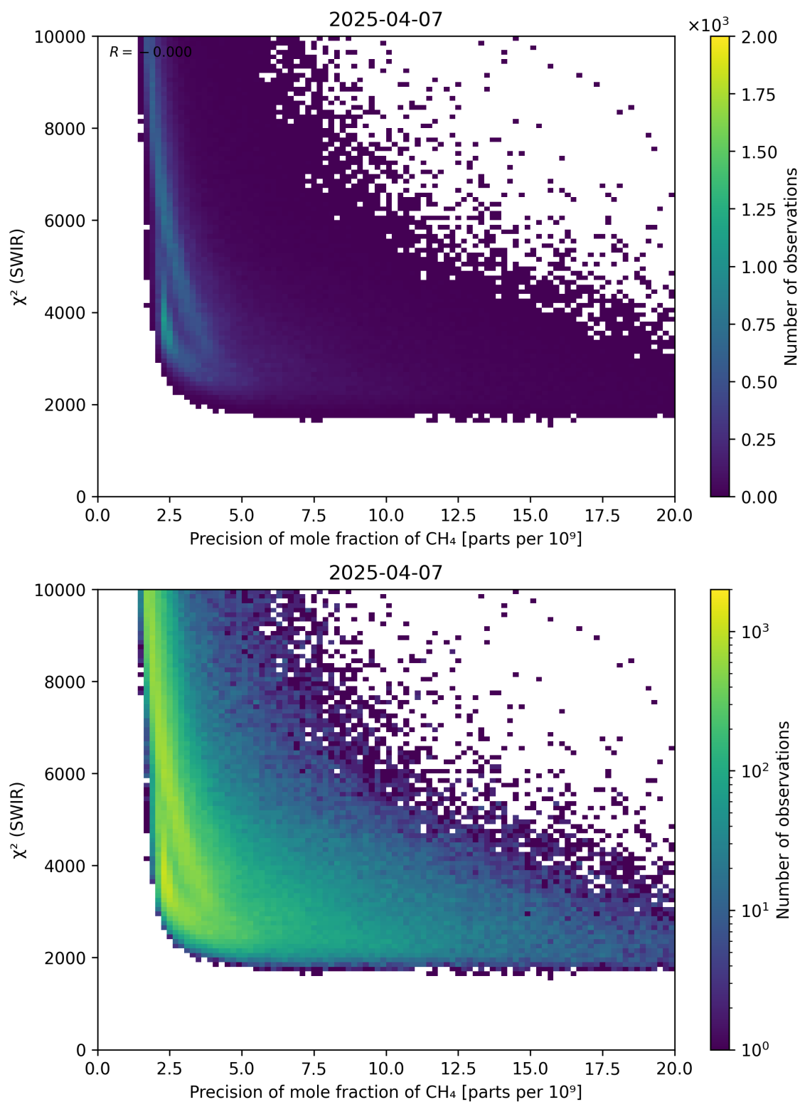
Figure 79: Scatter density plot of “Precision of mole fraction of \text{CH}_4 ” against “ \chi^2 (SWIR)” for 2025-04-06 to 2025-04-08.
