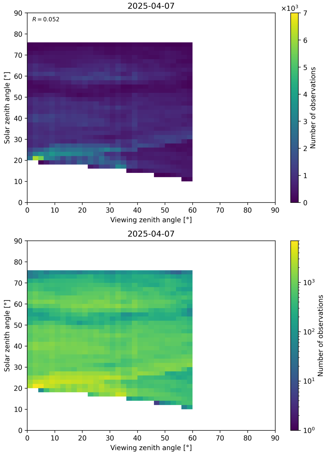
Figure 115: Scatter density plot of “Viewing zenith angle” against “Solar zenith angle” for 2025-04-06 to 2025-04-08.
