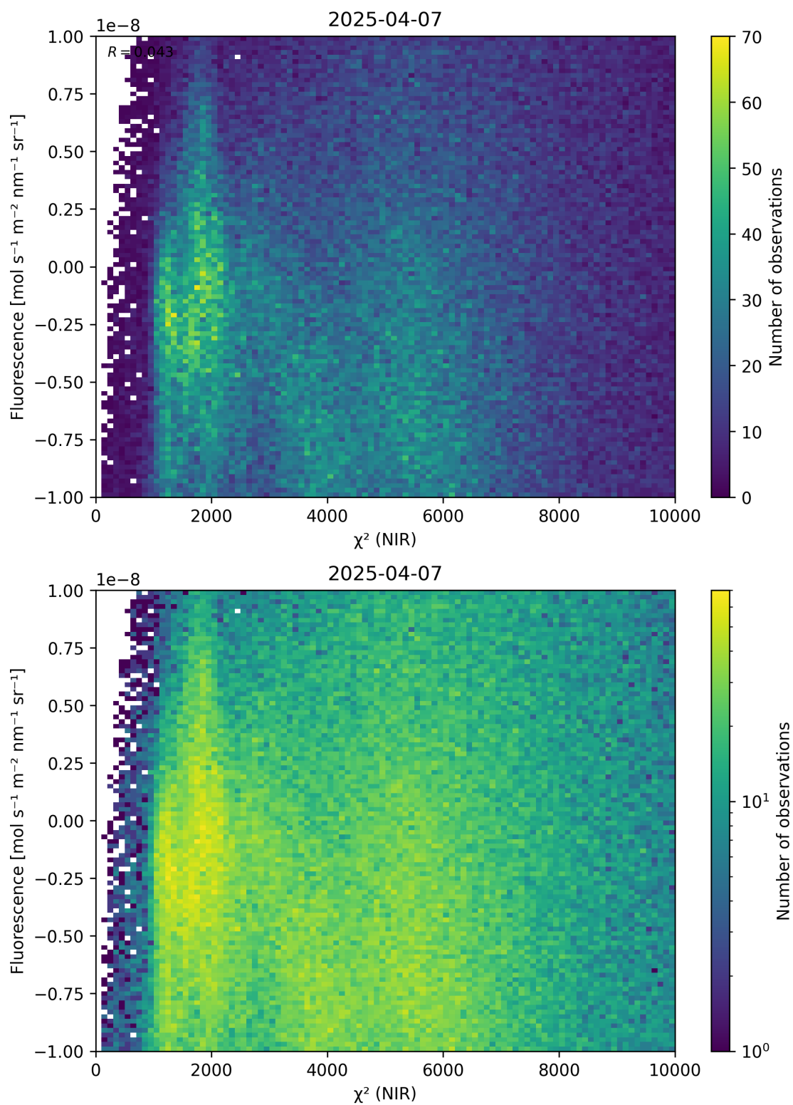
Figure 45: Scatter density plot of “ \chi^2 (NIR)” against “Fluorescence” for 2025-04-06 to 2025-04-08.
