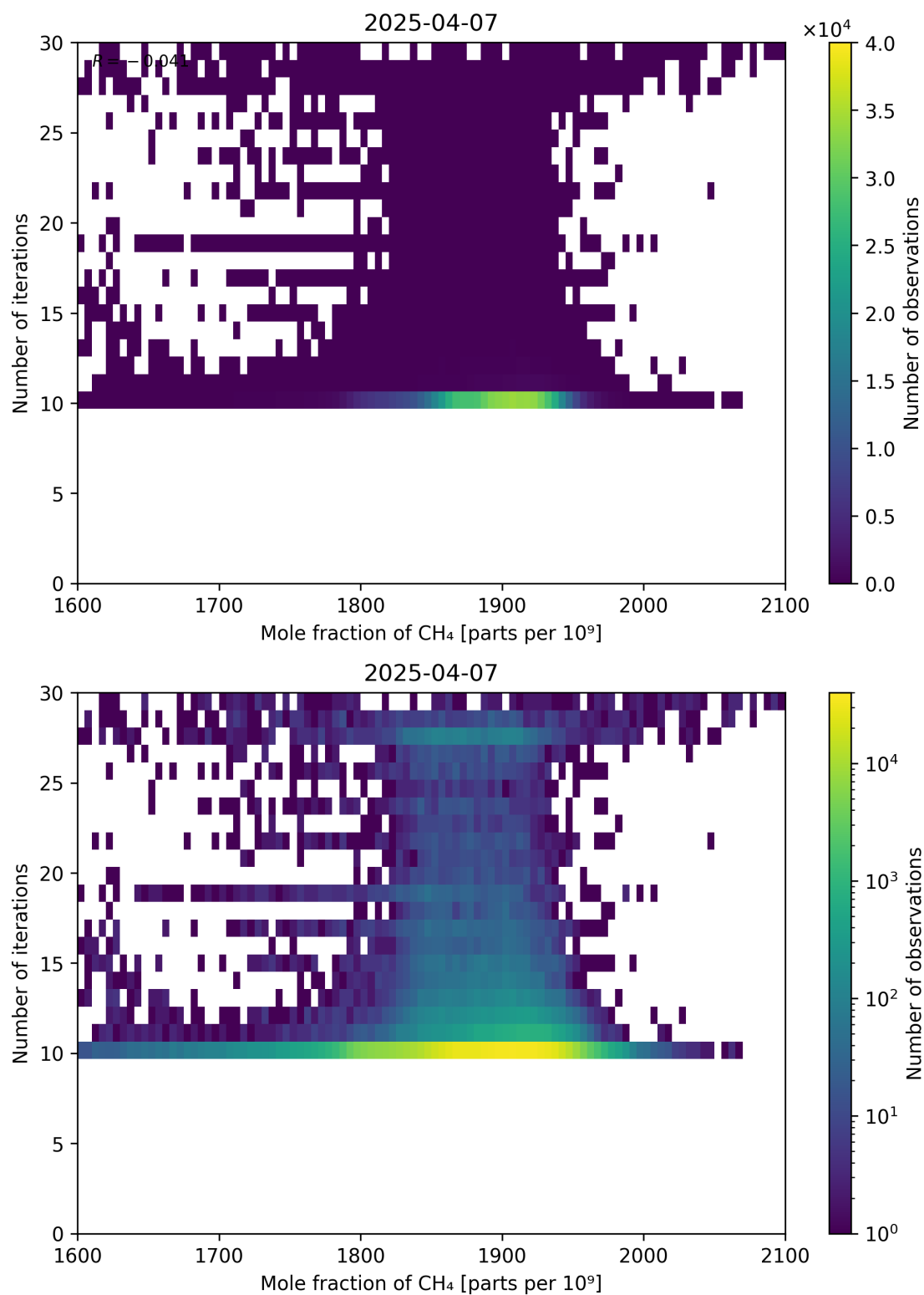
Figure 76: Scatter density plot of “Mole fraction of CH 4 ” against “Number of iterations” for 2025-04-06 to 2025-04-08.
