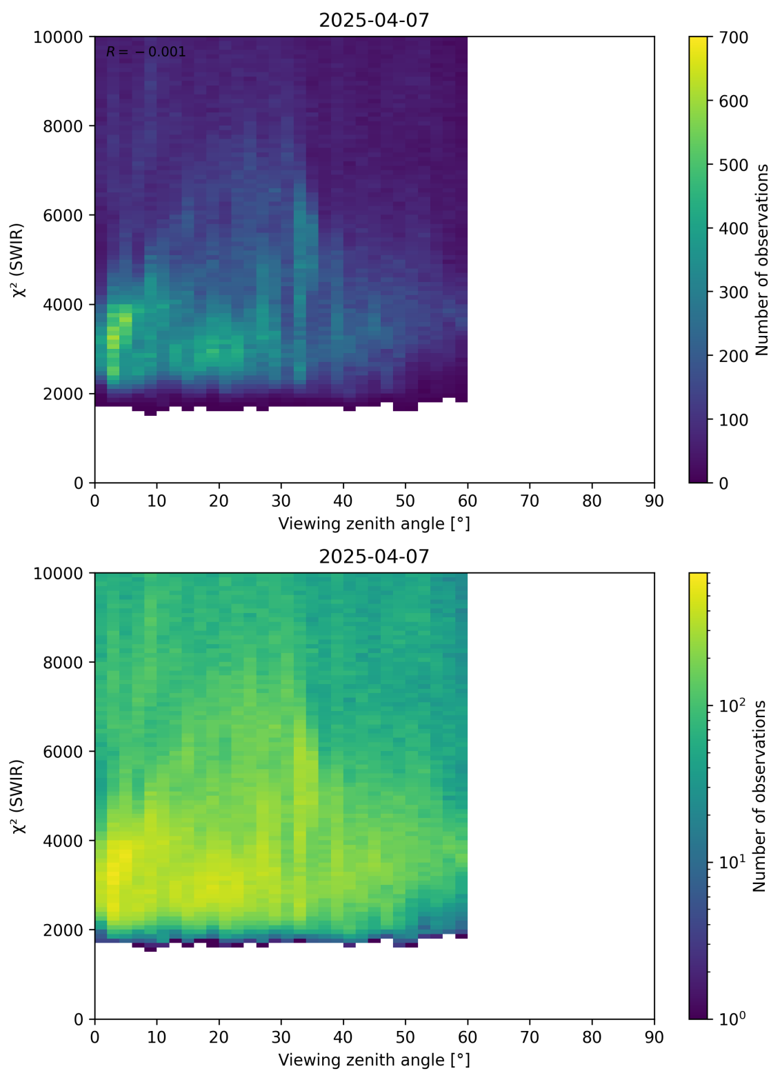
Figure 106: Scatter density plot of “Viewing zenith angle” against “ \chi^2 (SWIR)” for 2025-04-06 to 2025-04-08.
