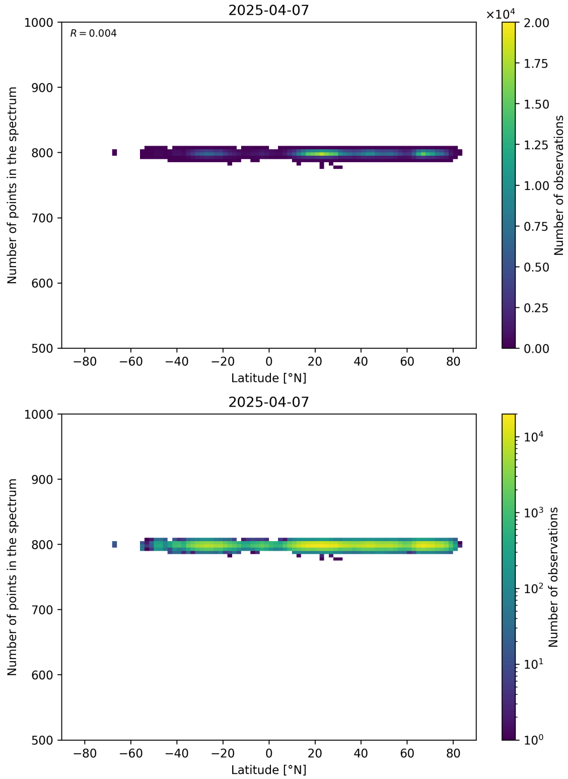
Figure 61: Scatter density plot of “Latitude” against “Number of points in the spectrum” for 2025-04-06 to 2025-04-08.
