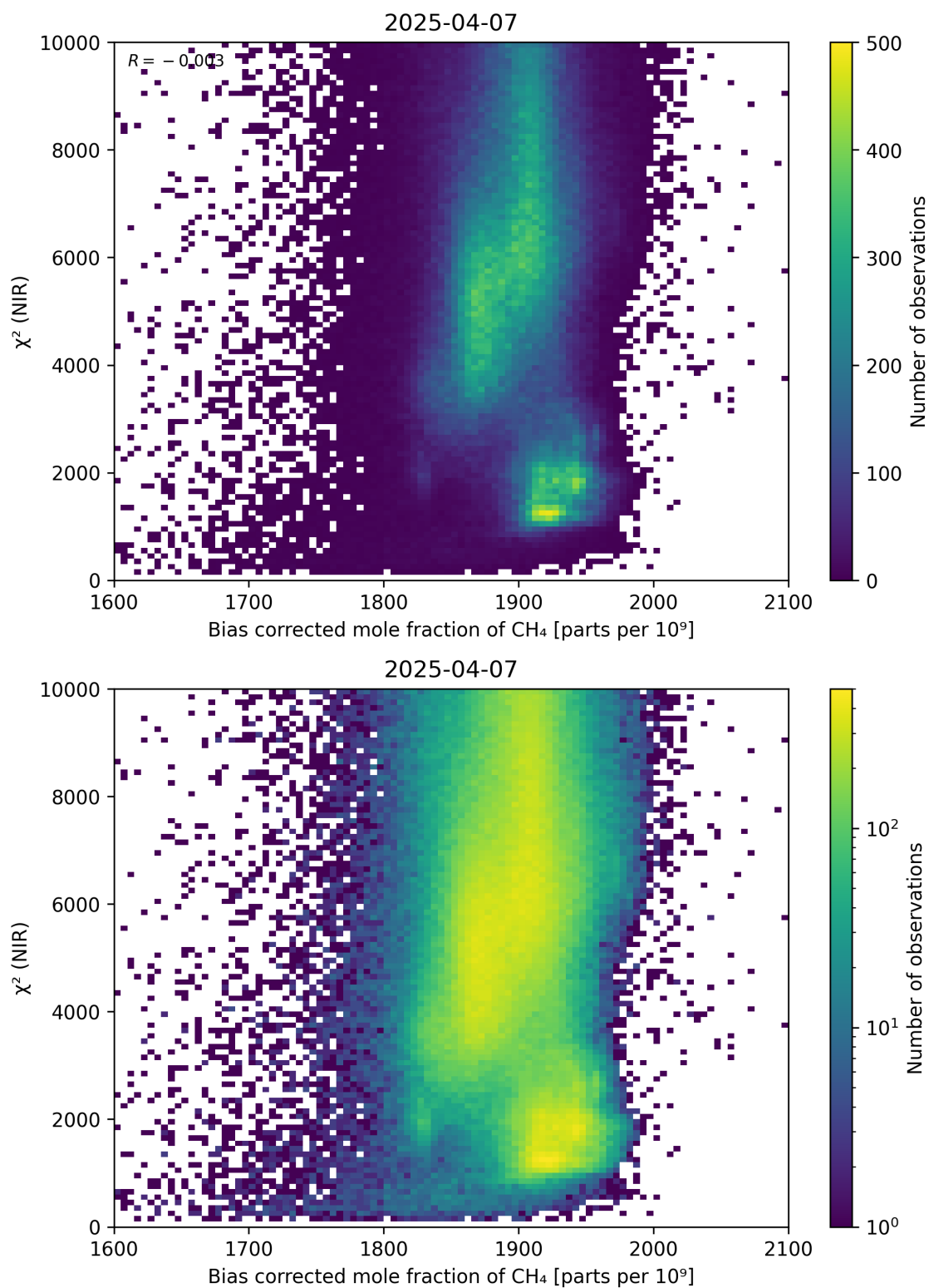
Figure 63: Scatter density plot of “Bias corrected mole fraction of \text{CH}_4 ” against “ \chi^2 (NIR)” for 2025-04-06 to 2025-04-08.
