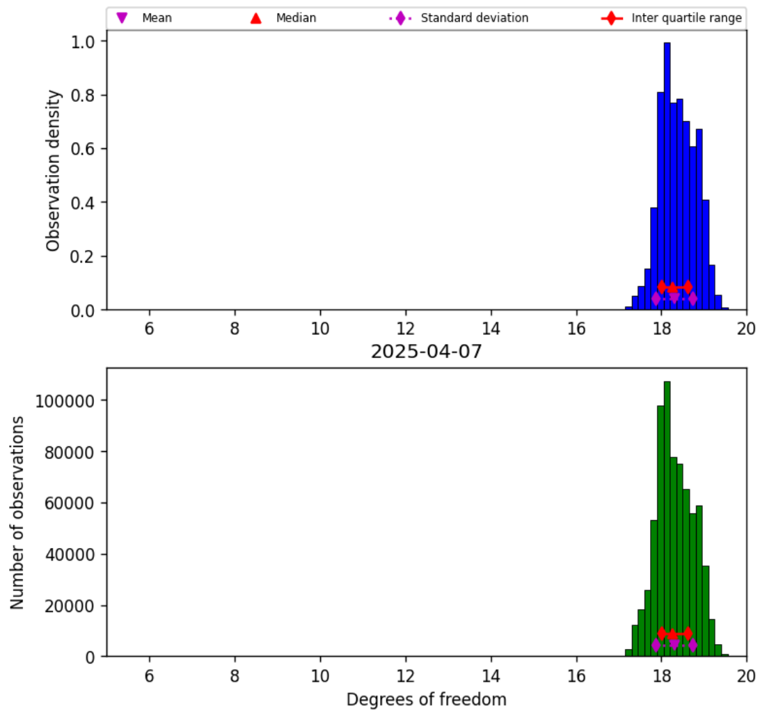
Figure 30: Histogram of “Degrees of freedom” for 2025-04-06 to 2025-04-08
