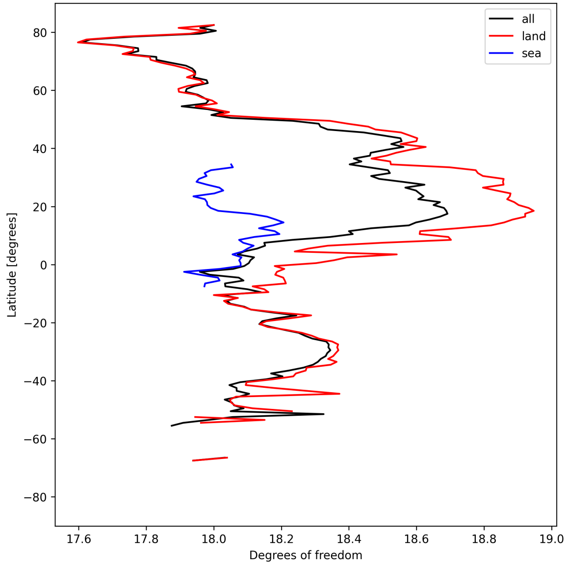
Figure 19: Zonal average of “Degrees of freedom” for 2025-04-06 to 2025-04-08.
