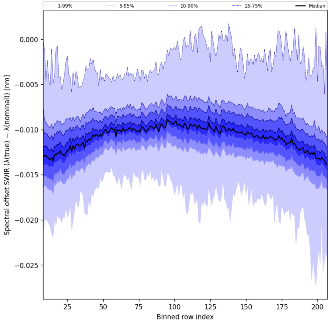
Figure 38: Along track statistics of “Spectral offset SWIR ( \lambda_{\text{true}} - \lambda_{\text{nominal}} )” for 2025-04-06 to 2025-04-08
