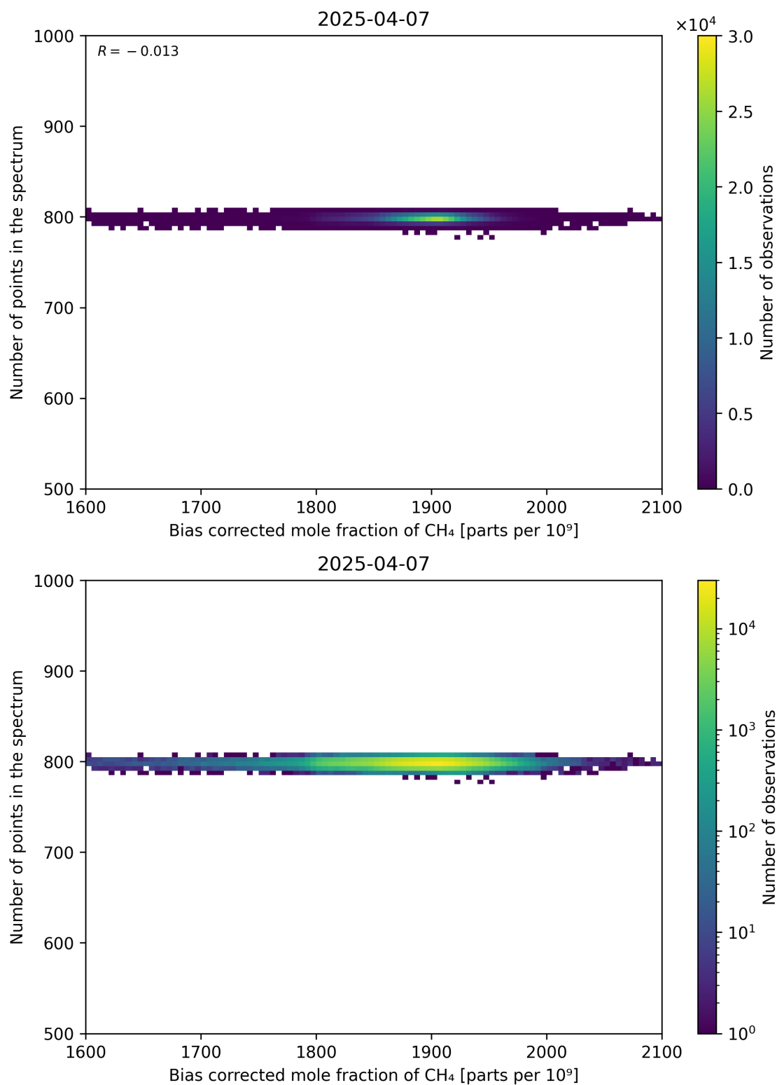
Figure 68: Scatter density plot of “Bias corrected mole fraction of CH 4 ” against “Number of points in the spectrum” for 2025-04-06 to 2025-04-08.
