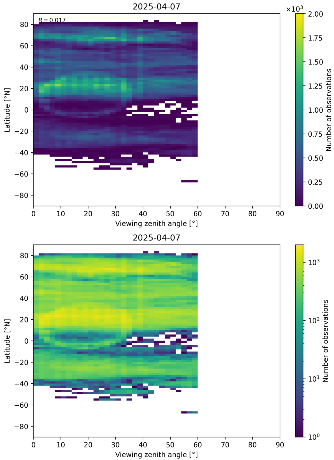
Figure 109: Scatter density plot of “Viewing zenith angle” against “Latitude” for 2025-04-06 to 2025-04-08.
