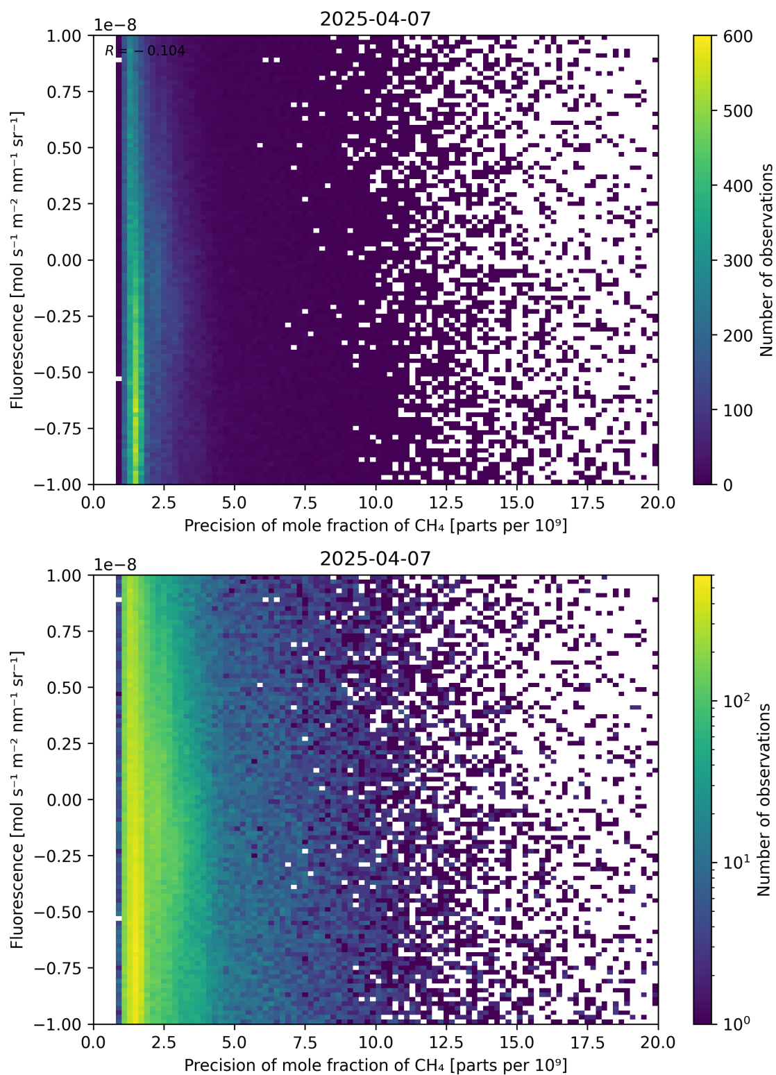
Figure 81: Scatter density plot of “Precision of mole fraction of CH 4 ” against “Fluorescence” for 2025-04-06 to 2025-04-08.
