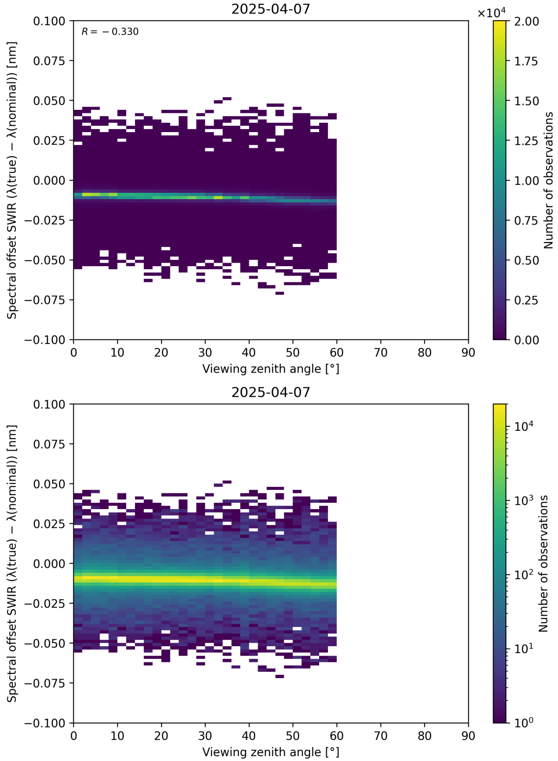
Figure 116: Scatter density plot of “Viewing zenith angle” against “Spectral offset SWIR ( \lambda_{\text{true}} - \lambda_{\text{nominal}} )” for 2025-04-06 to 2025-04-08.
