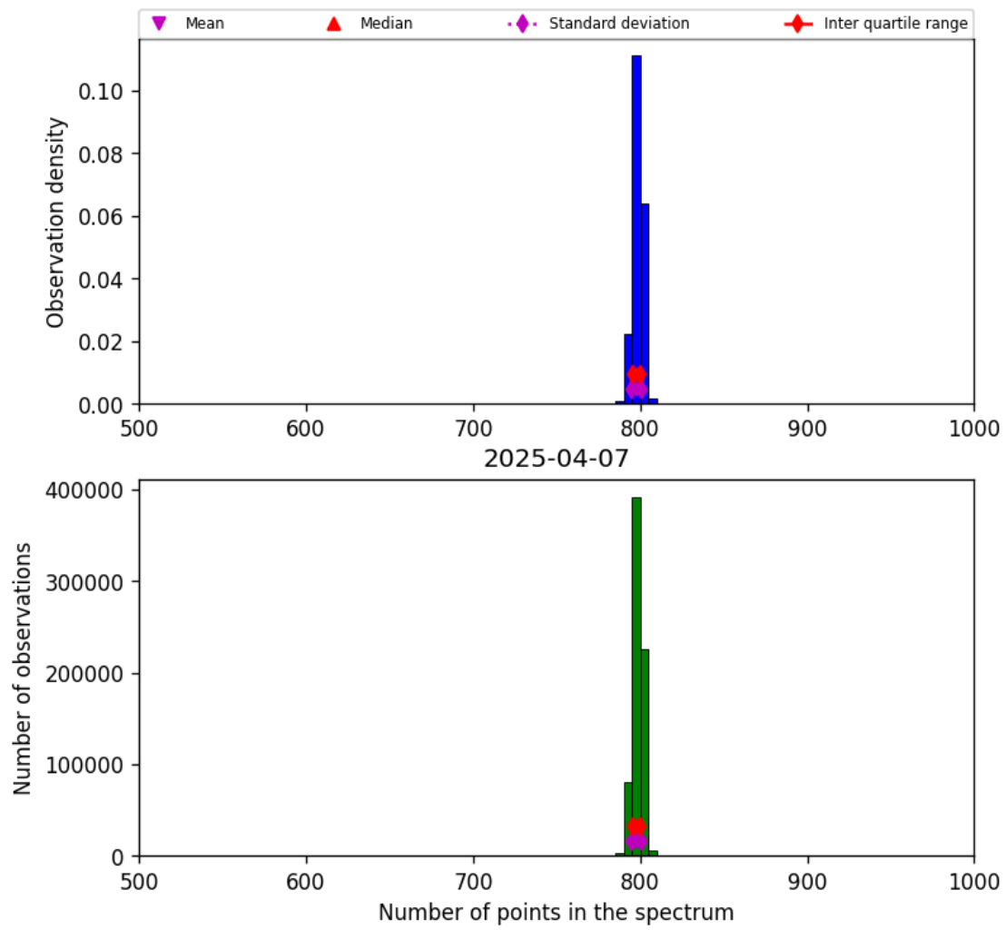
Figure 26: Histogram of “Number of points in the spectrum” for 2025-04-06 to 2025-04-08
