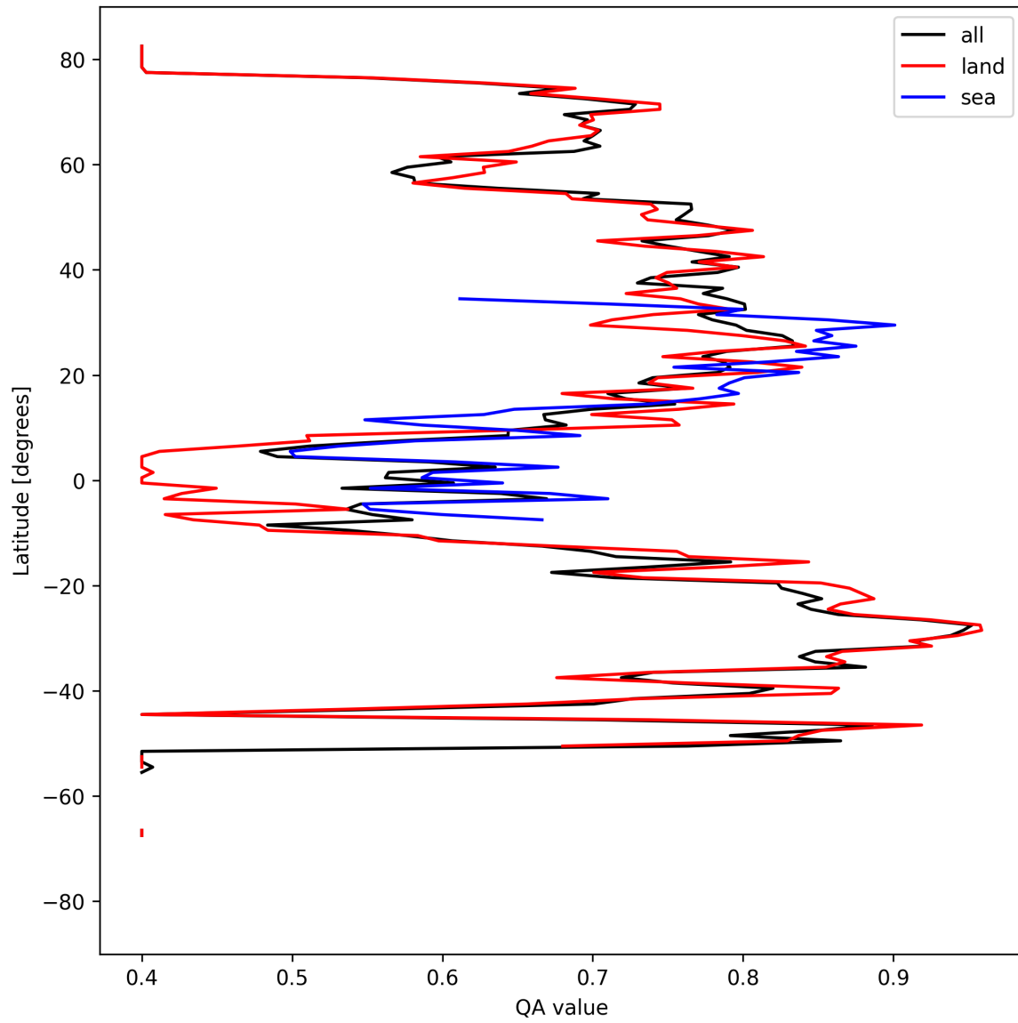
Figure 11: Zonal average of “QA value” for 2025-04-06 to 2025-04-08.
