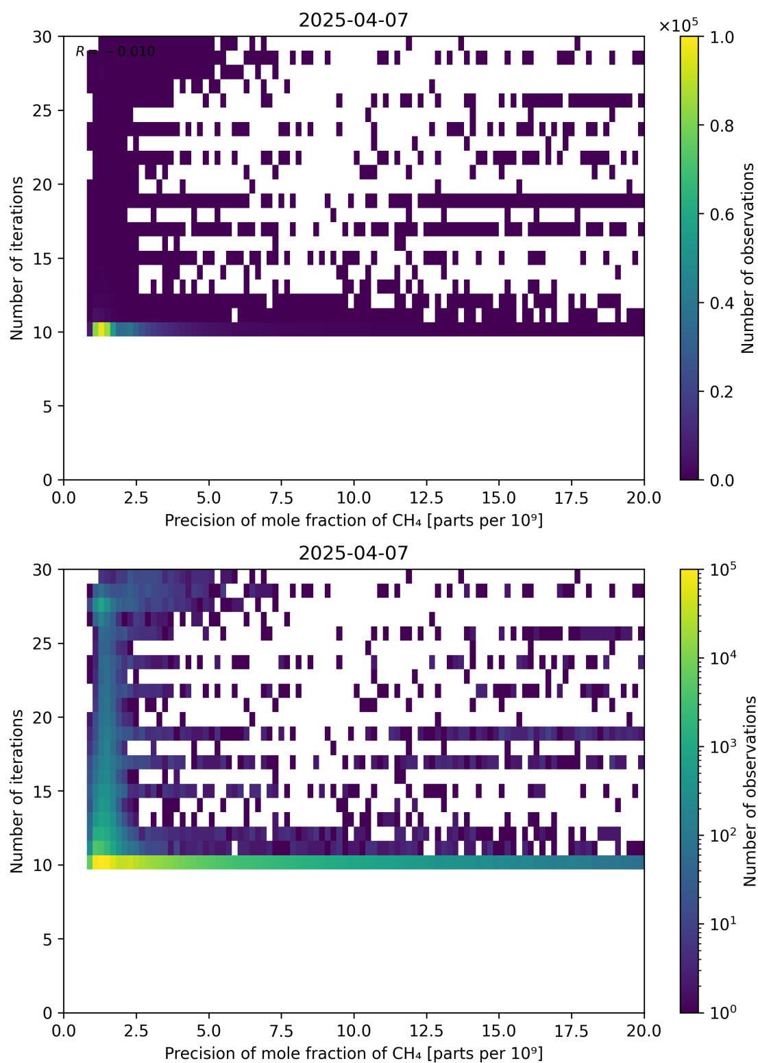
Figure 83: Scatter density plot of “Precision of mole fraction of CH 4 ” against “Number of iterations” for 2025-04-06 to 2025-04-08.
