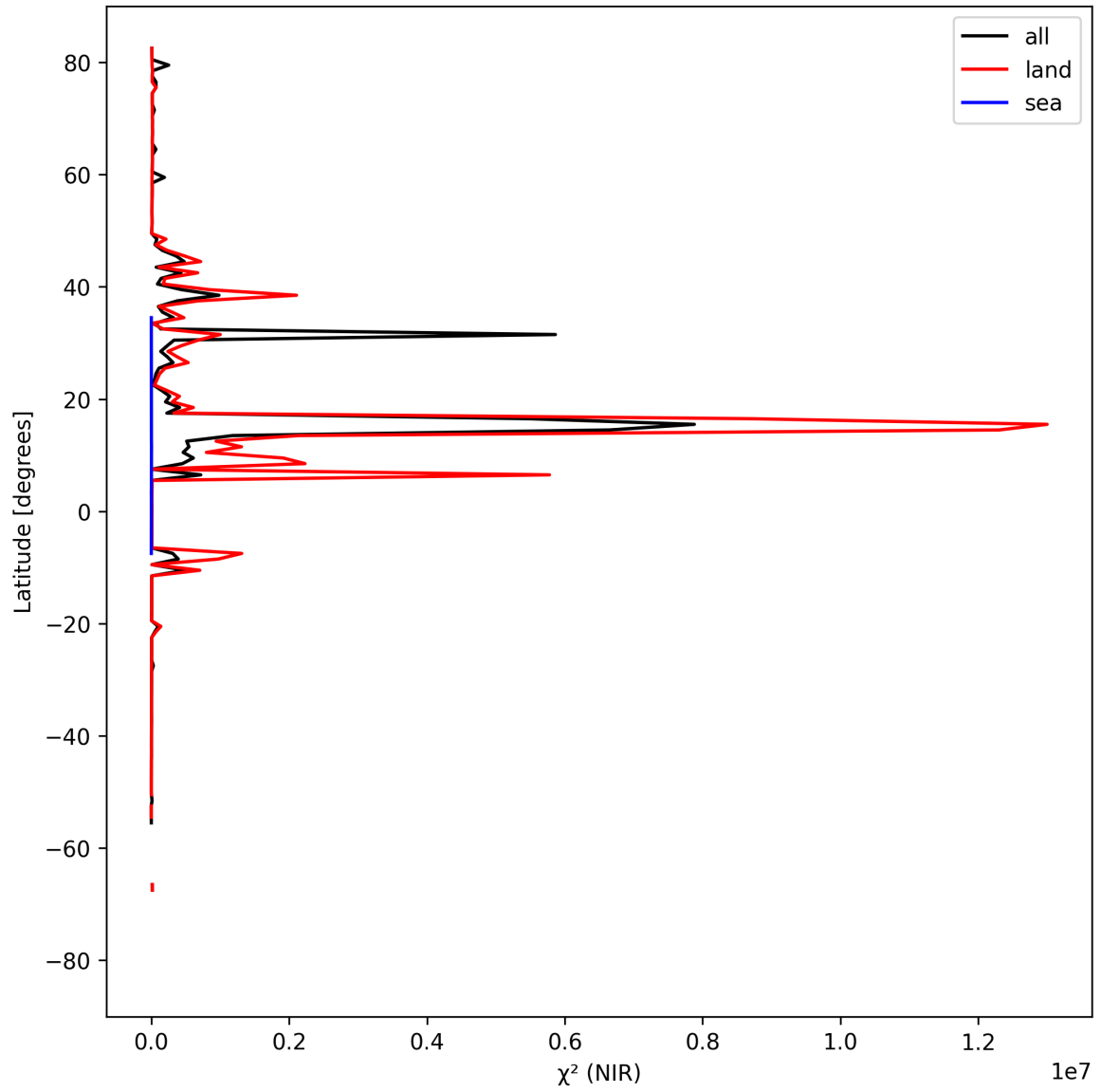
Figure 18: Zonal average of “ \chi^2 (NIR)” for 2025-04-06 to 2025-04-08.
