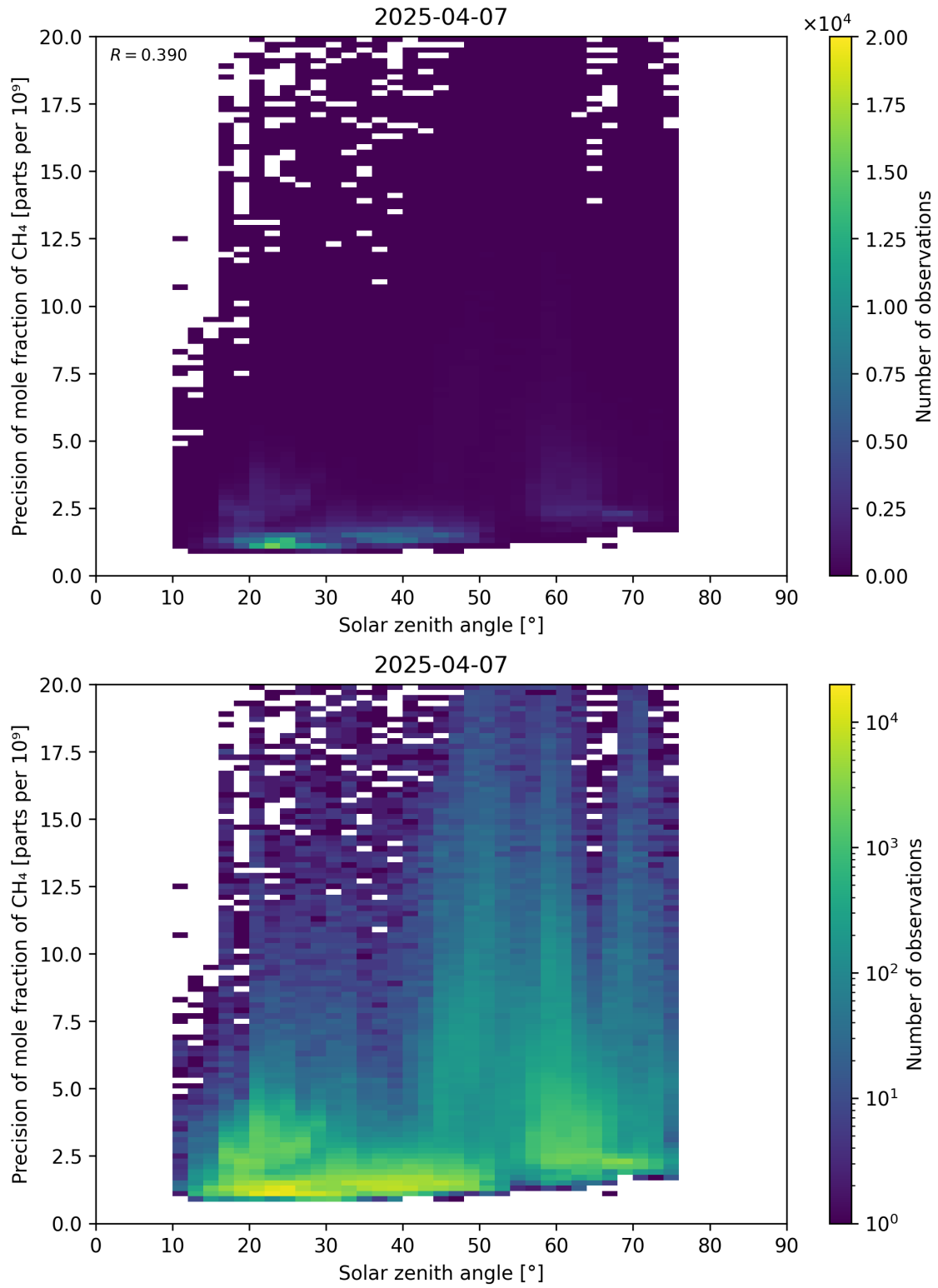
Figure 101: Scatter density plot of “Solar zenith angle” against “Precision of mole fraction of \text{CH}_4 ” for 2025-04-06 to 2025-04-08.
