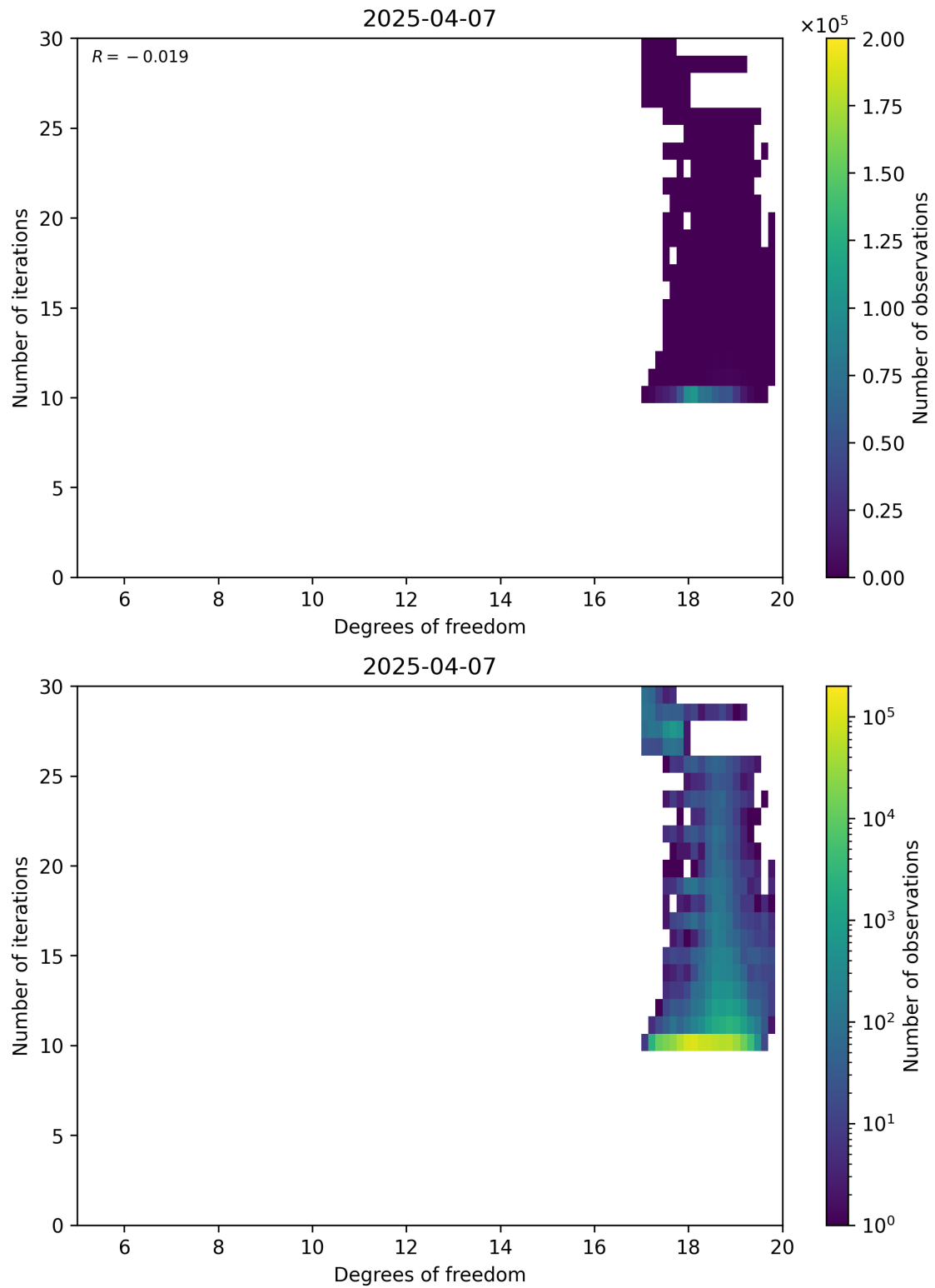
Figure 52: Scatter density plot of “Degrees of freedom” against “Number of iterations” for 2025-04-06 to 2025-04-08.
