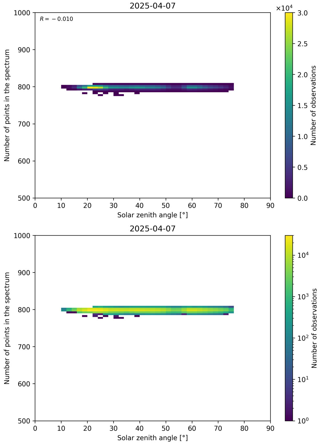
Figure 103: Scatter density plot of “Solar zenith angle” against “Number of points in the spectrum” for 2025-04-06 to 2025-04-08.
