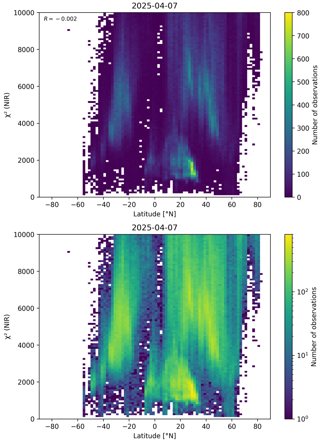
Figure 53: Scatter density plot of “Latitude” against “ \chi^2 (NIR)” for 2025-04-06 to 2025-04-08.
