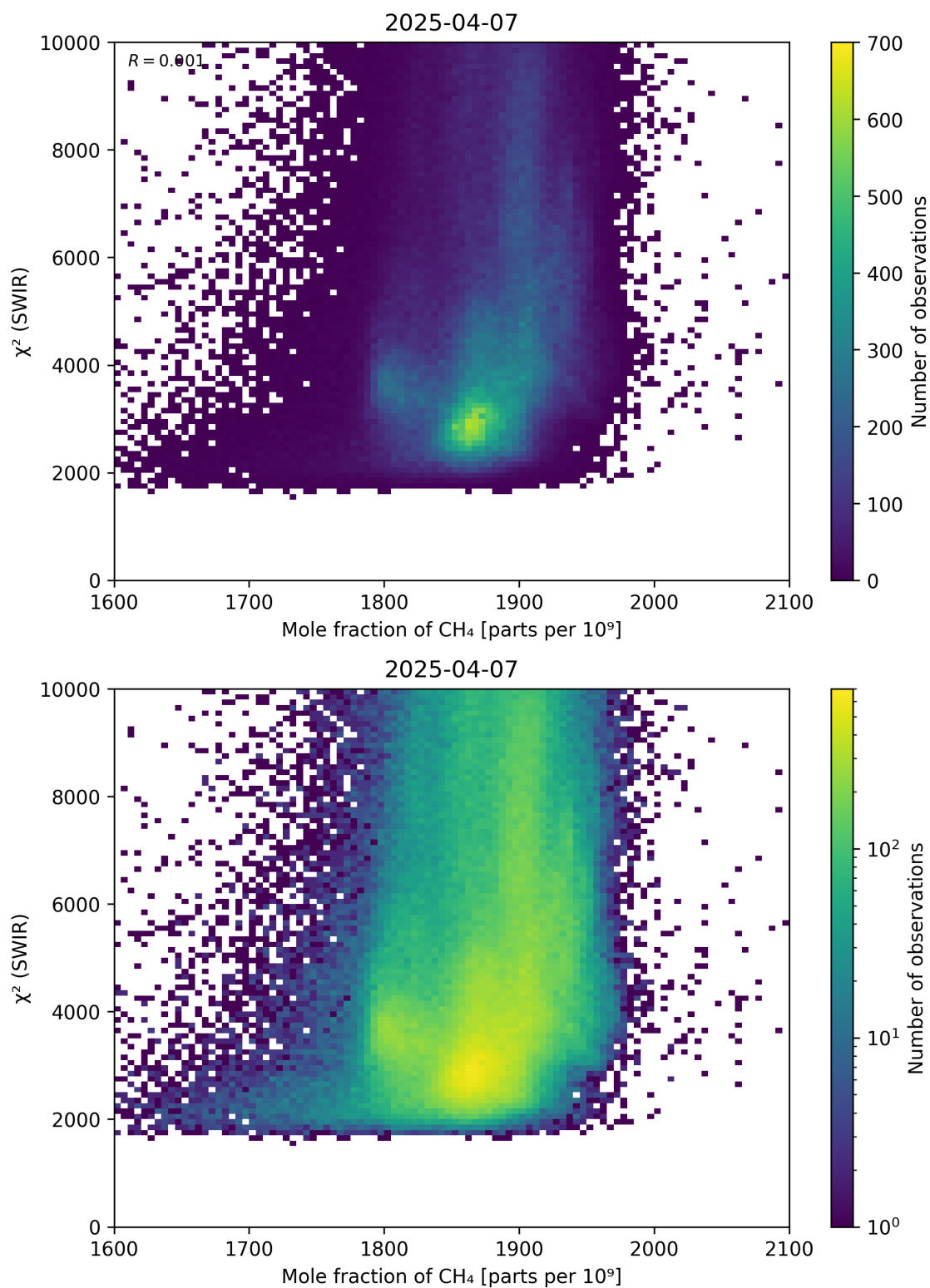
Figure 71: Scatter density plot of “Mole fraction of \text{CH}_4 ” against “ \chi^2 (SWIR)” for 2025-04-06 to 2025-04-08.
