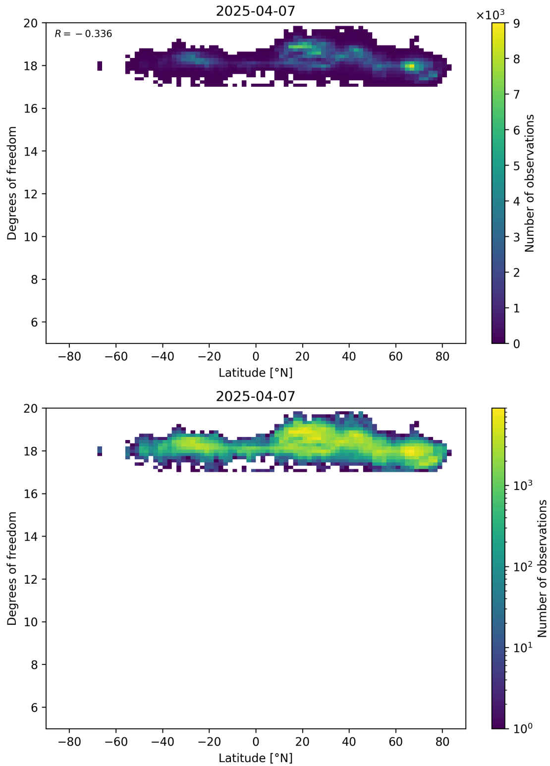
Figure 55: Scatter density plot of “Latitude” against “Degrees of freedom” for 2025-04-06 to 2025-04-08.
