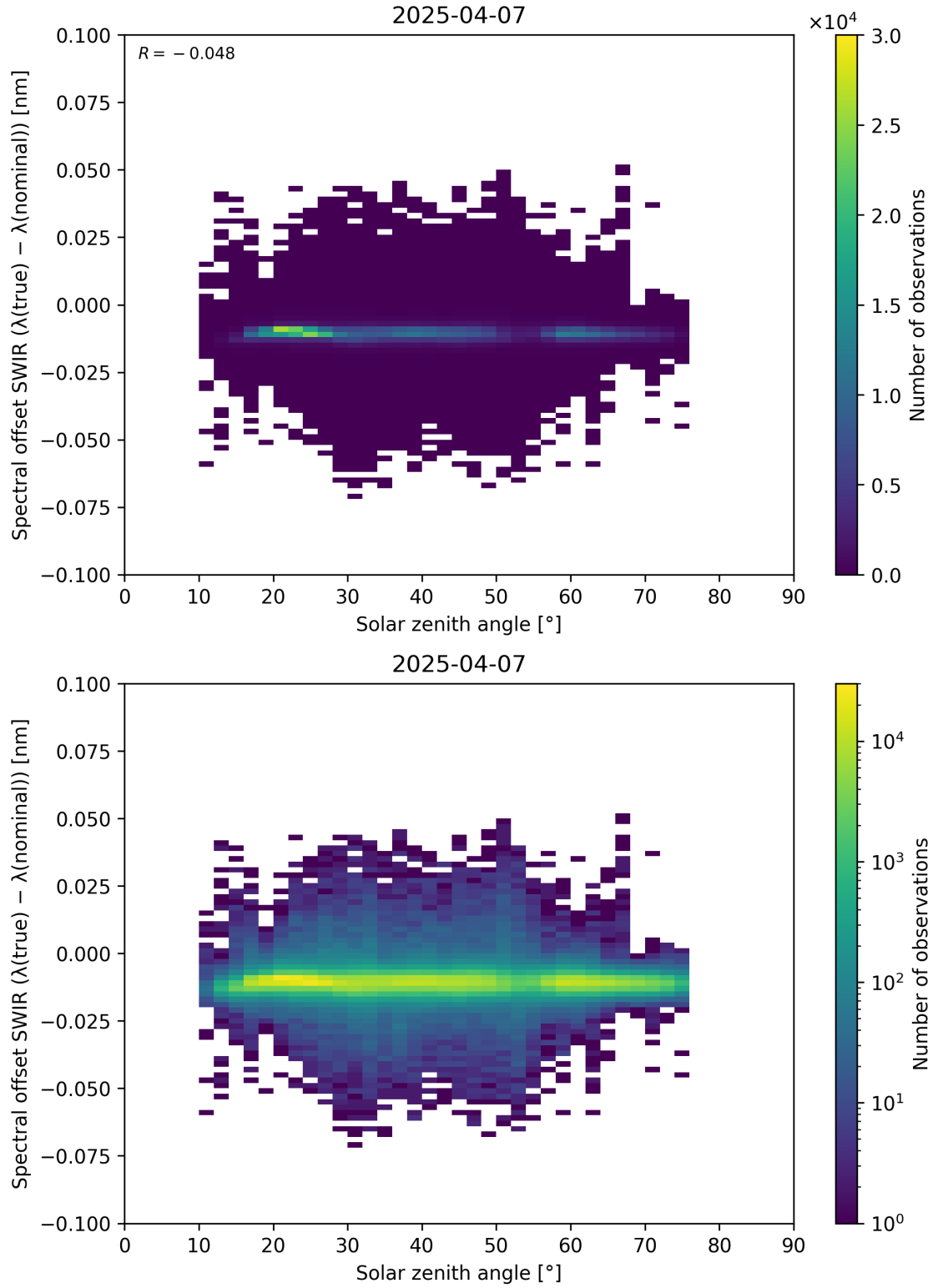
Figure 104: Scatter density plot of “Solar zenith angle” against “Spectral offset SWIR ( \lambda_{\text{true}} - \lambda_{\text{nominal}} )” for 2025-04-06 to 2025-04-08.
