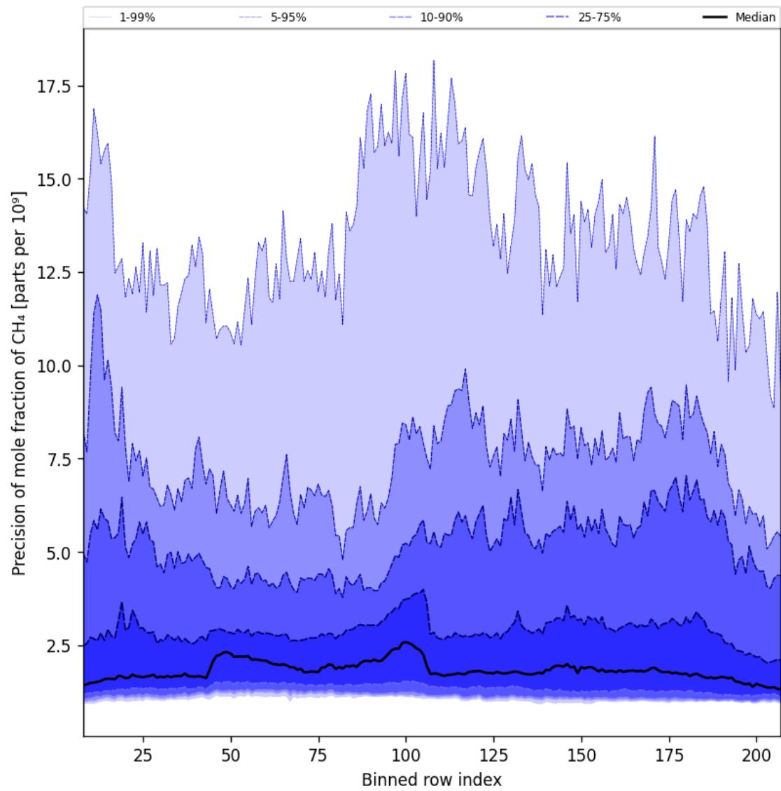
Figure 35: Along track statistics of “Precision of mole fraction of CH 4 ” for 2025-04-06 to 2025-04-08
