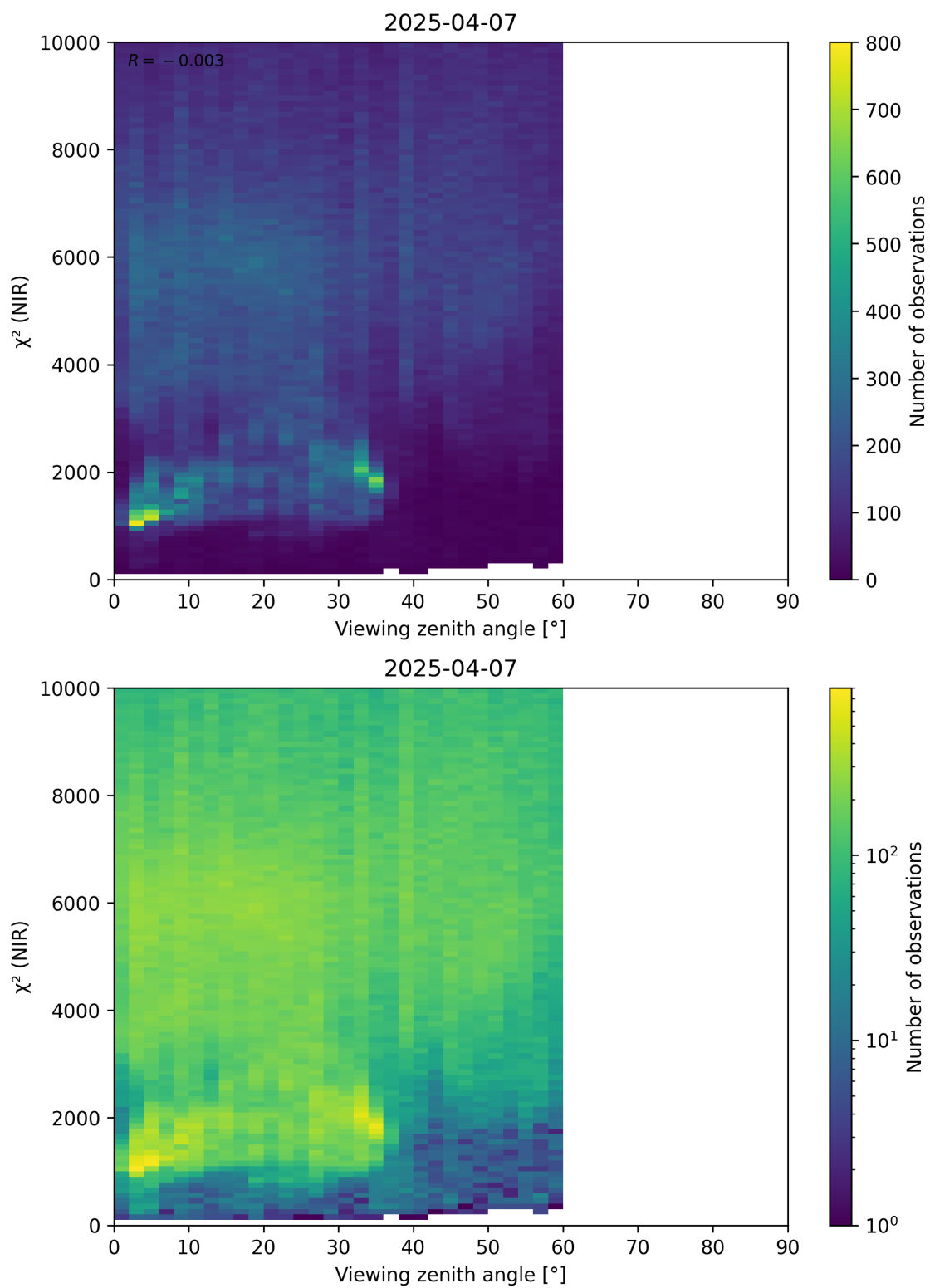
Figure 105: Scatter density plot of “Viewing zenith angle” against “ \chi^2 (NIR)” for 2025-04-06 to 2025-04-08.
