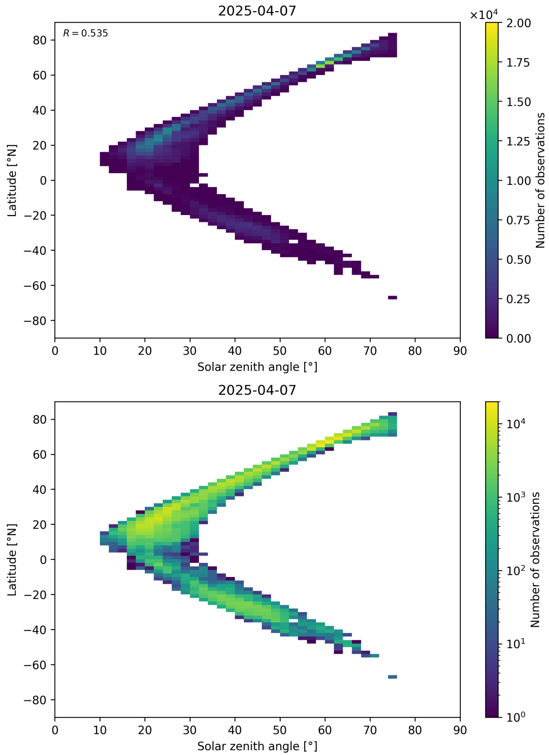
Figure 98: Scatter density plot of “Solar zenith angle” against “Latitude” for 2025-04-06 to 2025-04-08.
