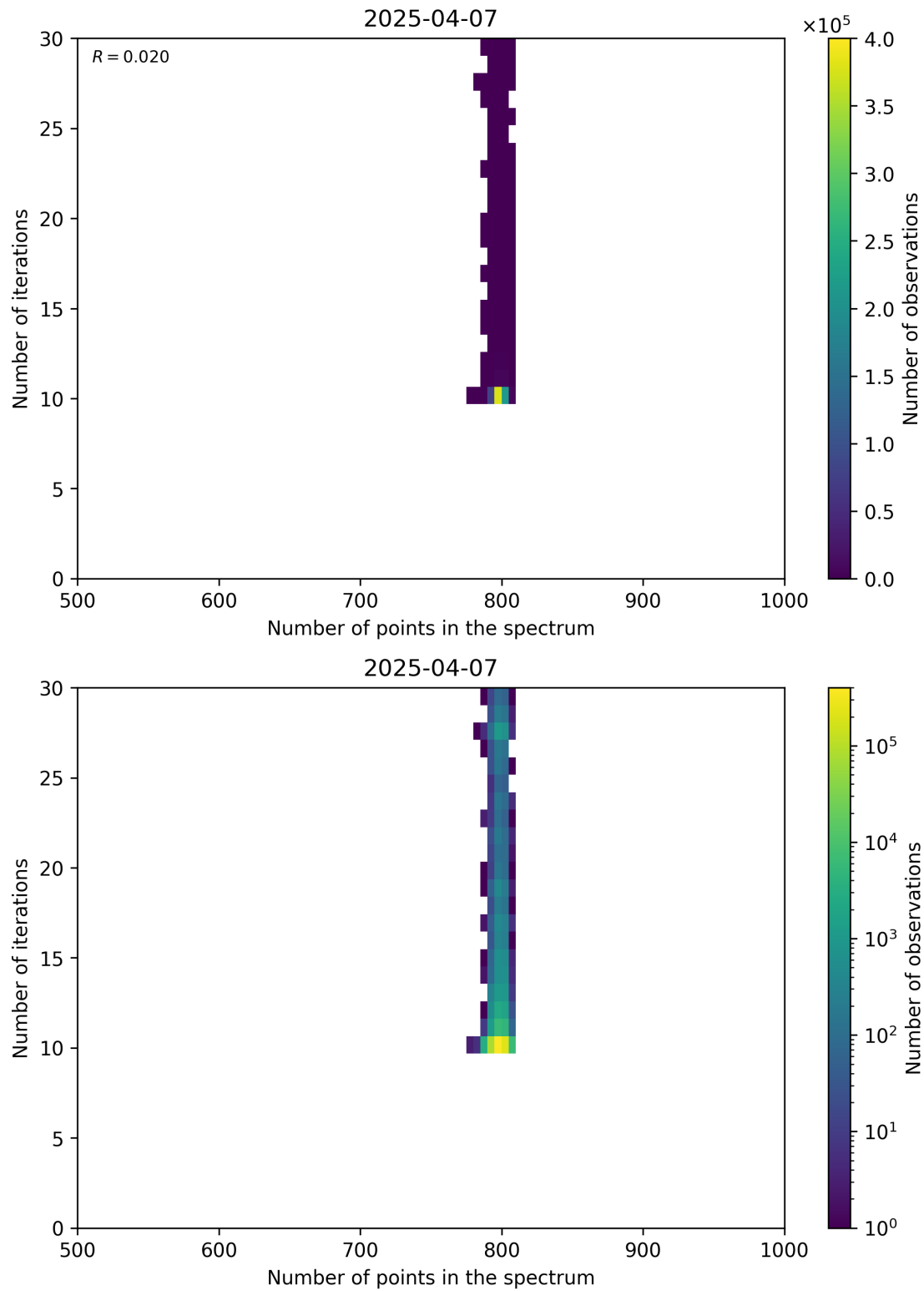
Figure 92: Scatter density plot of “Number of points in the spectrum” against “Number of iterations” for 2025-04-06 to 2025-04-08.
