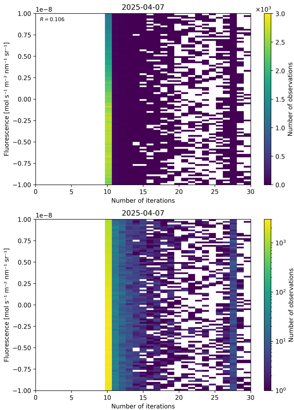
Figure 87: Scatter density plot of “Number of iterations” against “Fluorescence” for 2025-04-06 to 2025-04-08.
