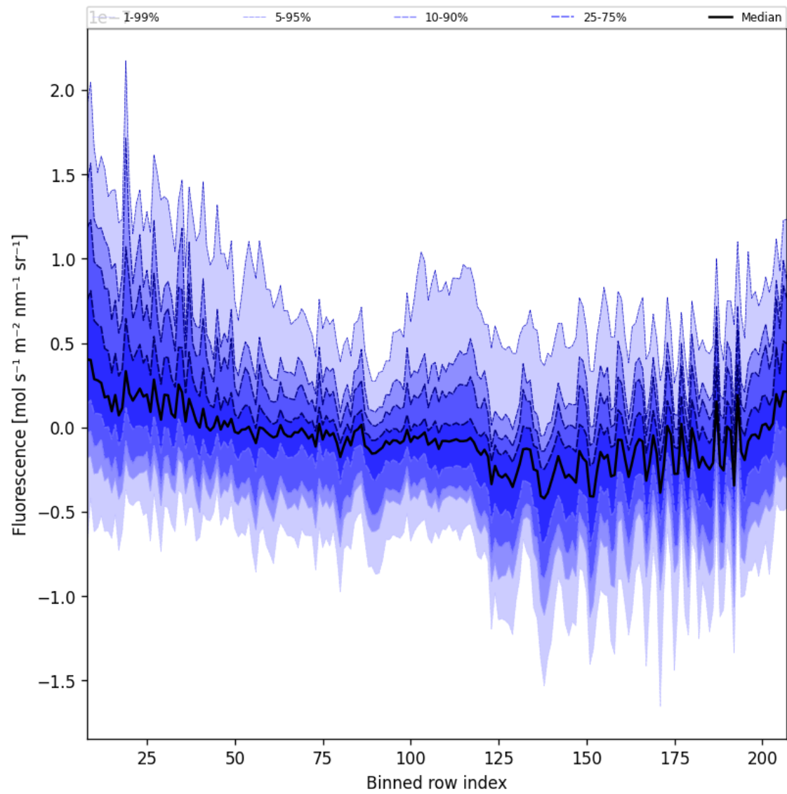
Figure 43: Along track statistics of “Fluorescence” for 2025-04-06 to 2025-04-08
