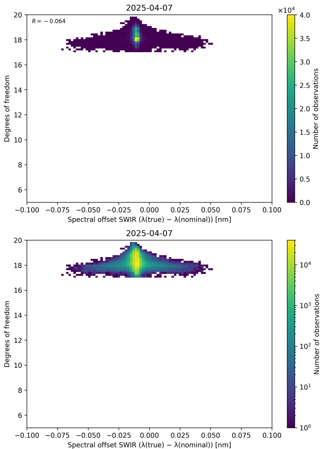
Figure 119: Scatter density plot of “Spectral offset SWIR ( \lambda_{\text{true}} - \lambda_{\text{nominal}} )” against “Degrees of freedom” for 2025-04-06 to 2025-04-08.
