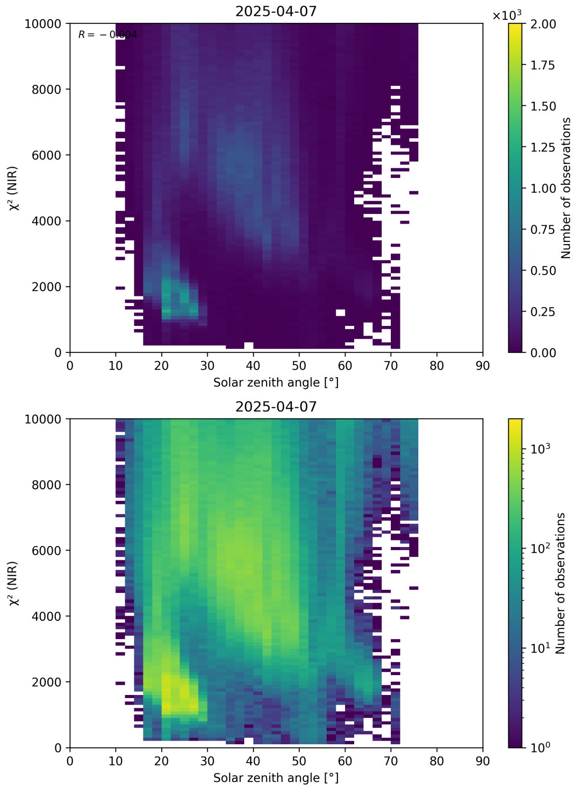
Figure 94: Scatter density plot of “Solar zenith angle” against “ \chi^2 (NIR)” for 2025-04-06 to 2025-04-08.
