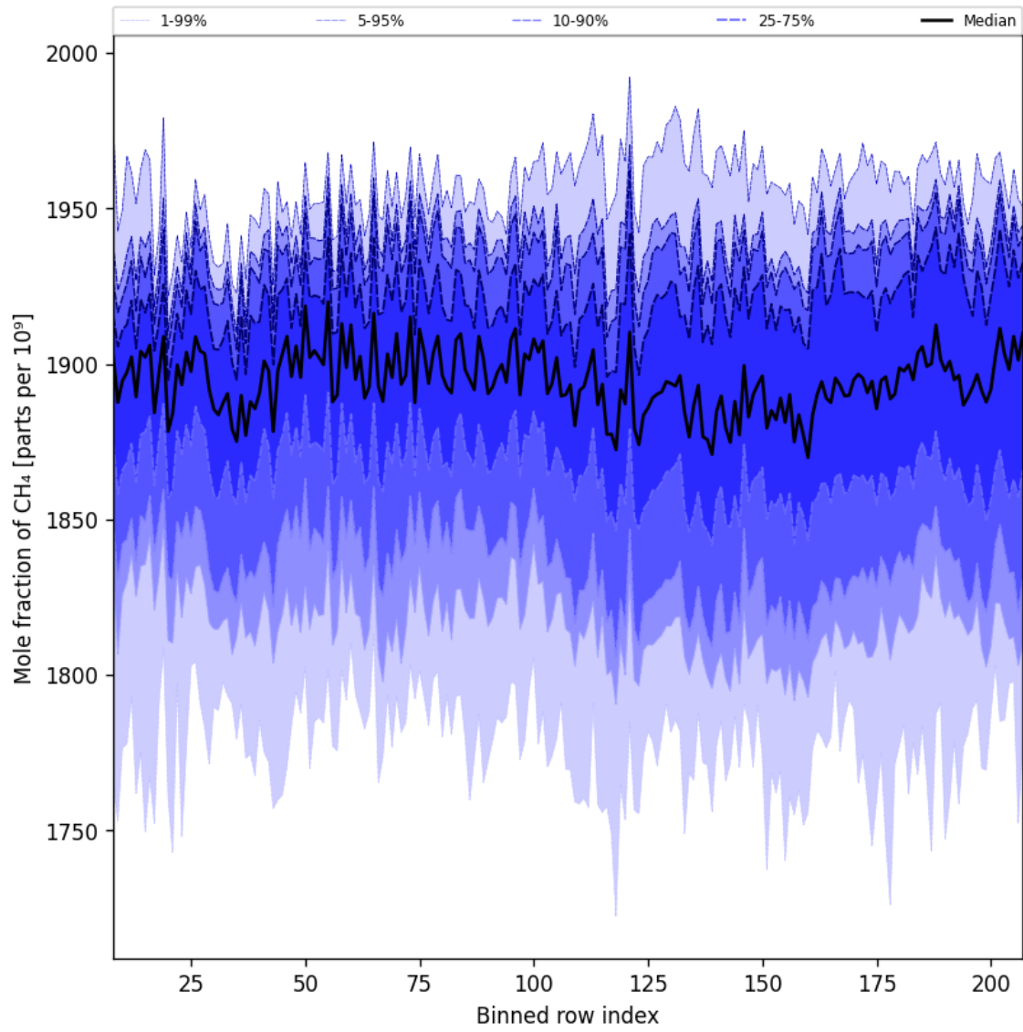
Figure 34: Along track statistics of “Mole fraction of CH 4 ” for 2025-04-06 to 2025-04-08
