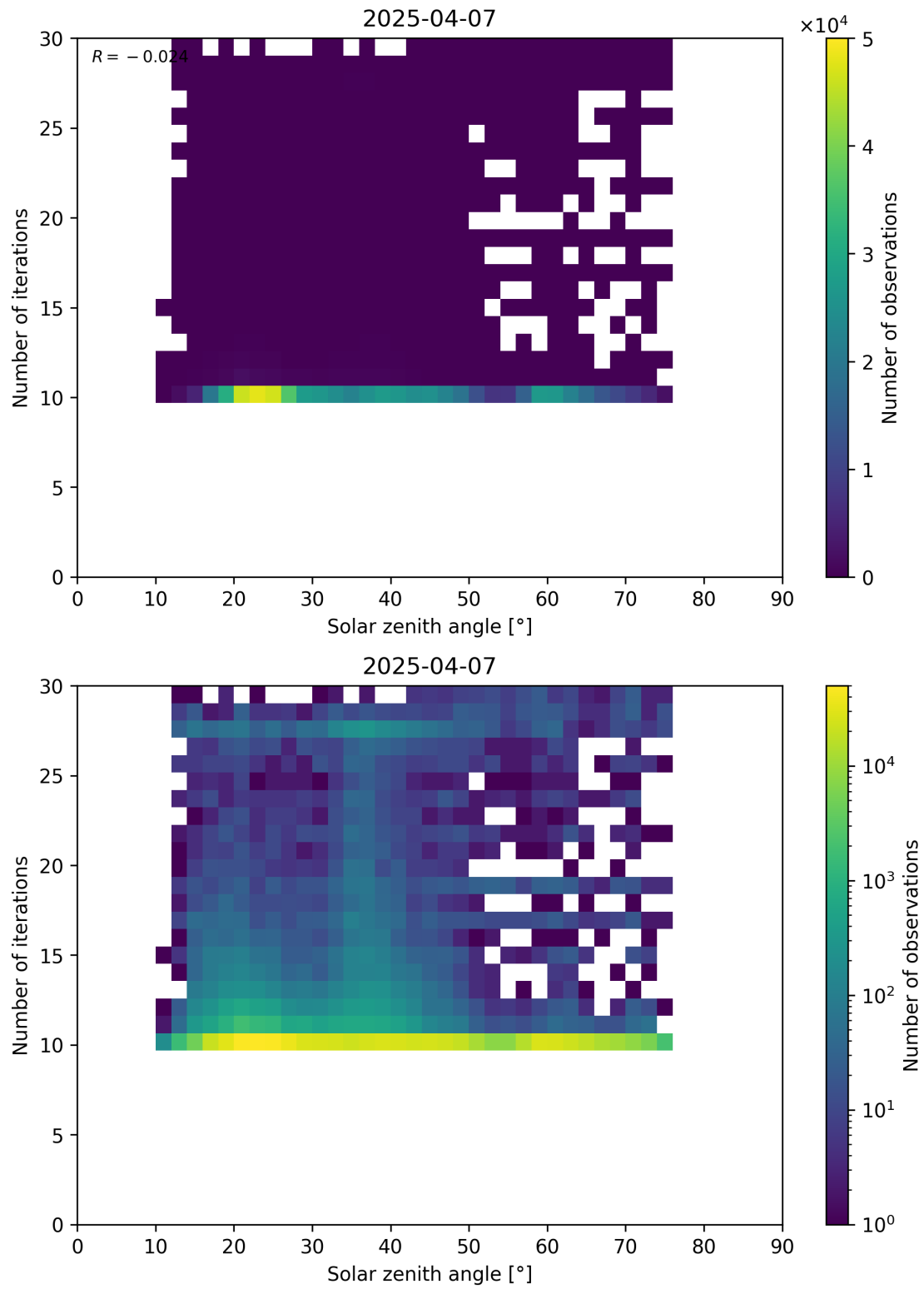
Figure 102: Scatter density plot of “Solar zenith angle” against “Number of iterations” for 2025-04-06 to 2025-04-08.
