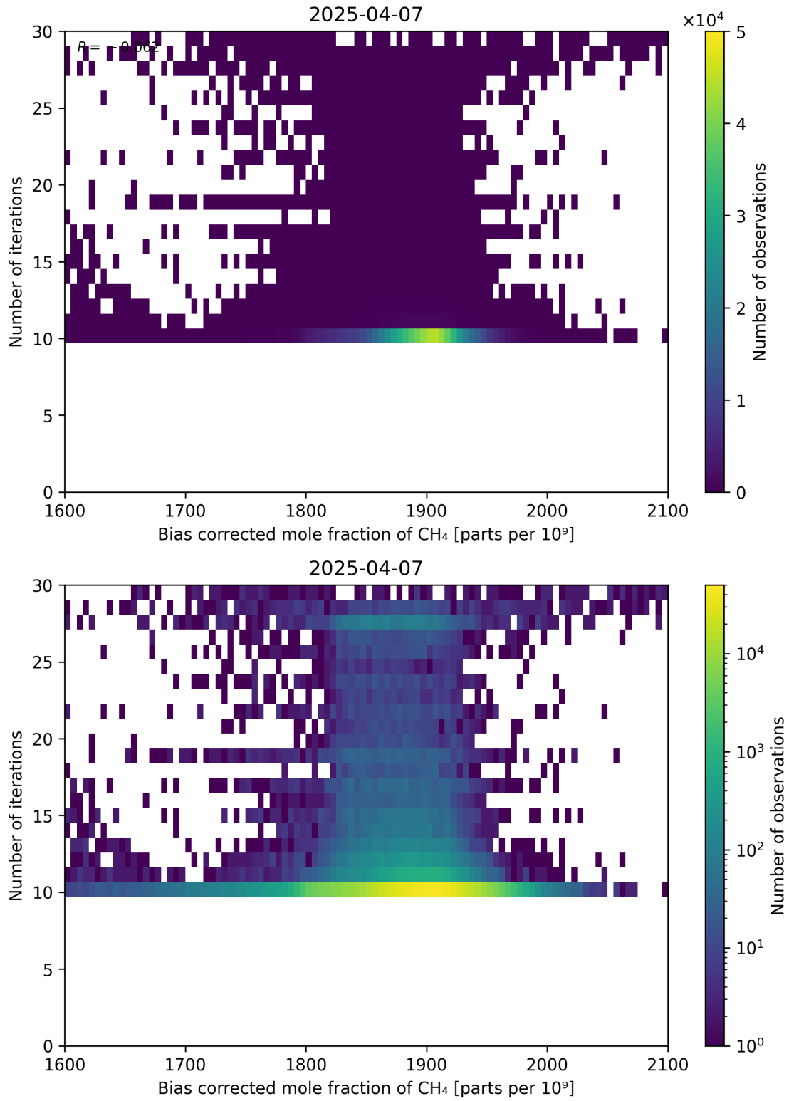
Figure 67: Scatter density plot of “Bias corrected mole fraction of CH 4 ” against “Number of iterations” for 2025-04-06 to 2025-04-08.
