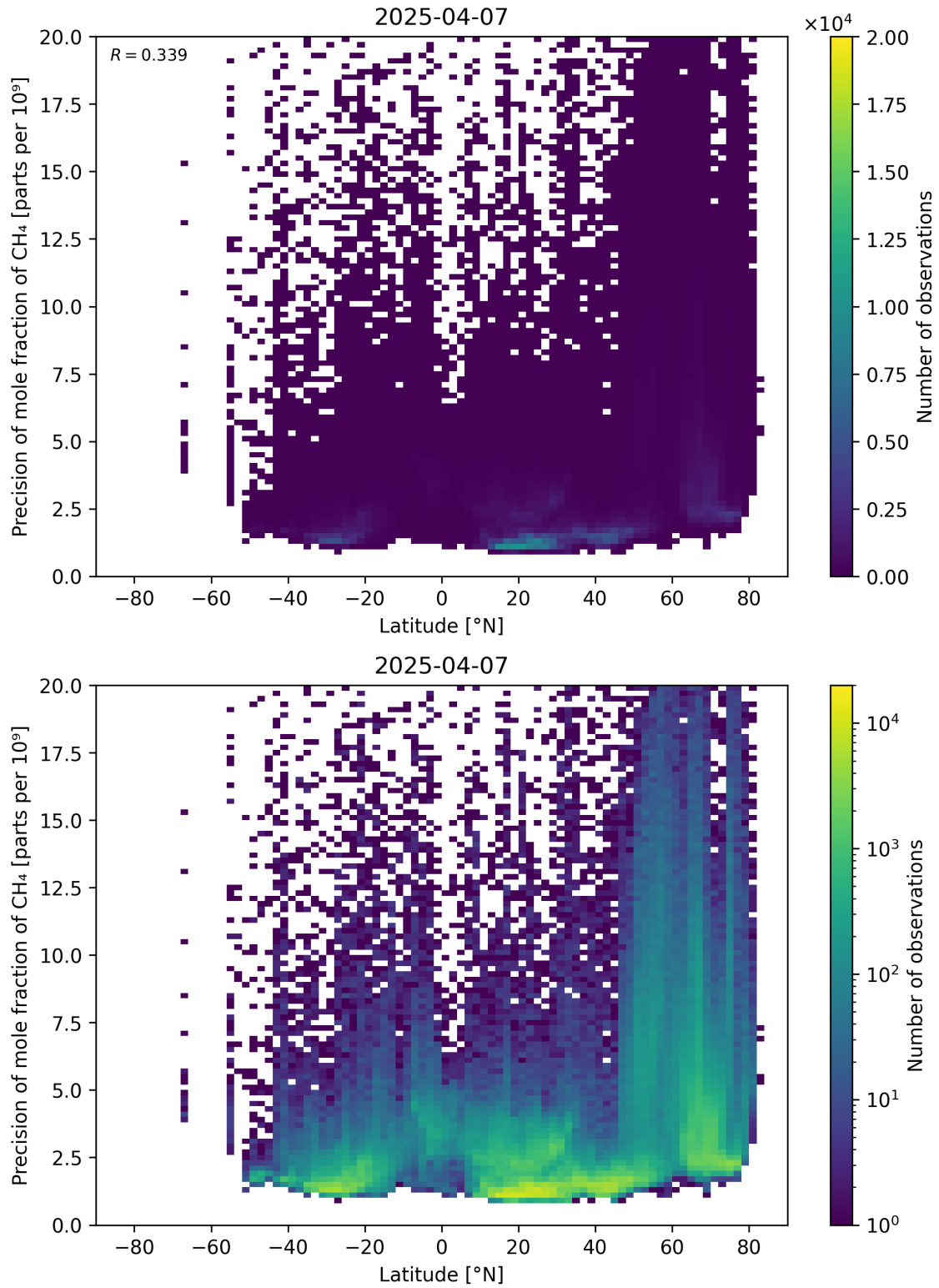
Figure 59: Scatter density plot of “Latitude” against “Precision of mole fraction of \text{CH}_4 ” for 2025-04-06 to 2025-04-08.
