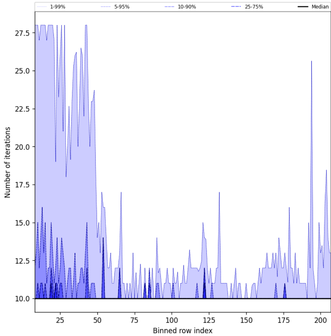
Figure 42: Along track statistics of “Number of iterations” for 2025-04-06 to 2025-04-08
