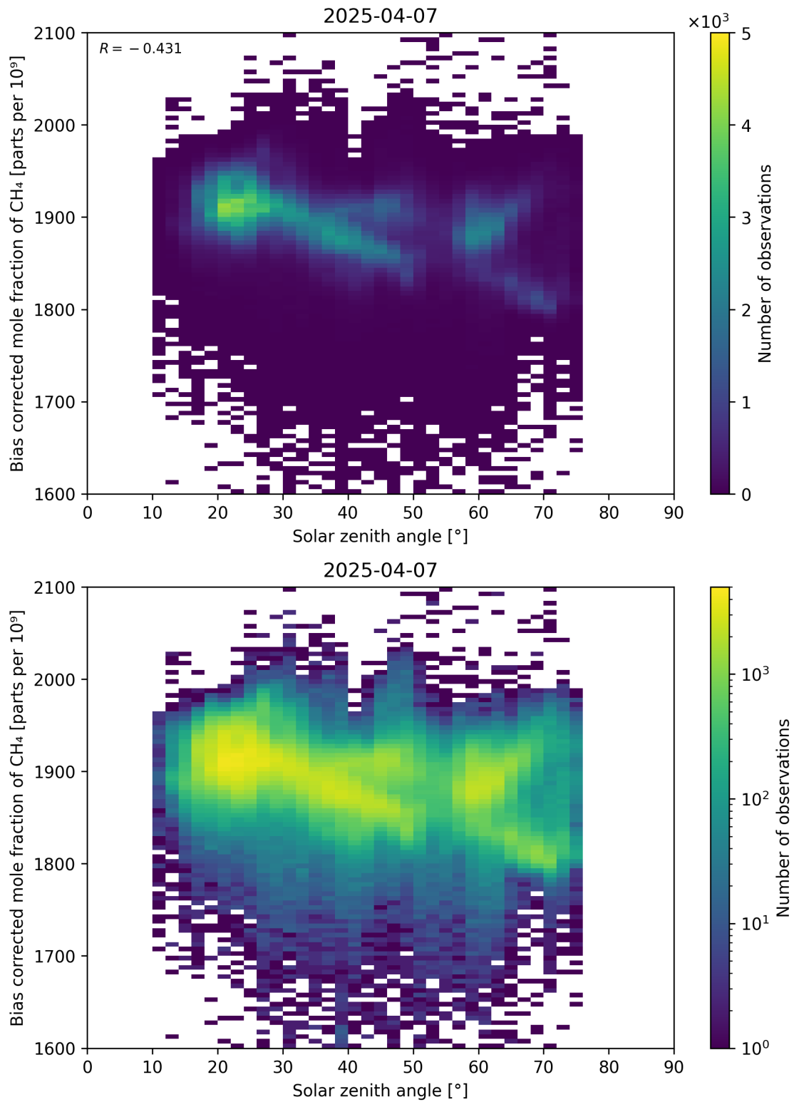
Figure 100: Scatter density plot of “Solar zenith angle” against “Bias corrected mole fraction of \text{CH}_4 ” for 2025-04-06 to 2025-04-08.
