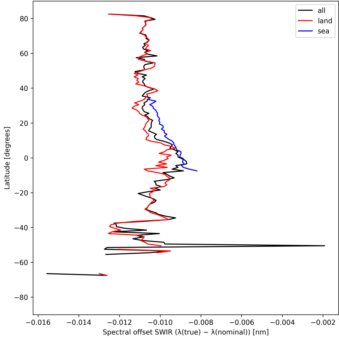
Figure 16: Zonal average of “Spectral offset SWIR ( \lambda_{\text{true}} - \lambda_{\text{nominal}} )” for 2025-04-06 to 2025-04-08.
