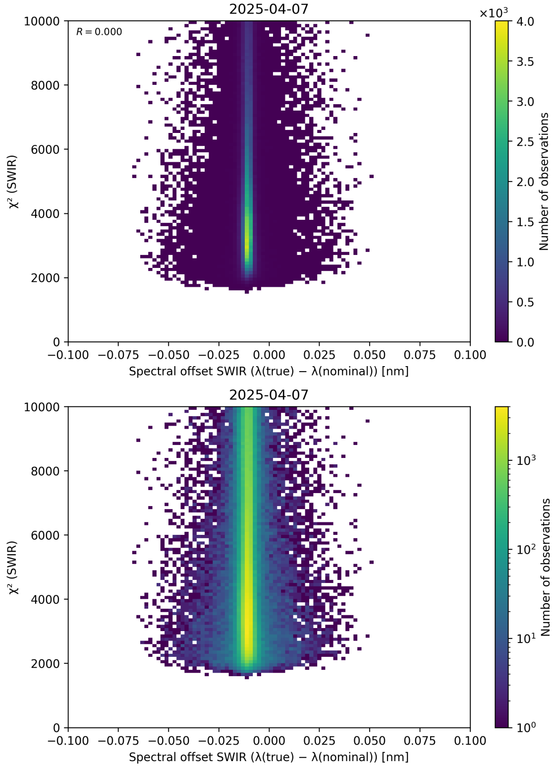
Figure 118: Scatter density plot of “Spectral offset SWIR ( \lambda_{\text{true}} - \lambda_{\text{nominal}} )” against “ \chi^2 (SWIR)” for 2025-04-06 to 2025-04-08.
