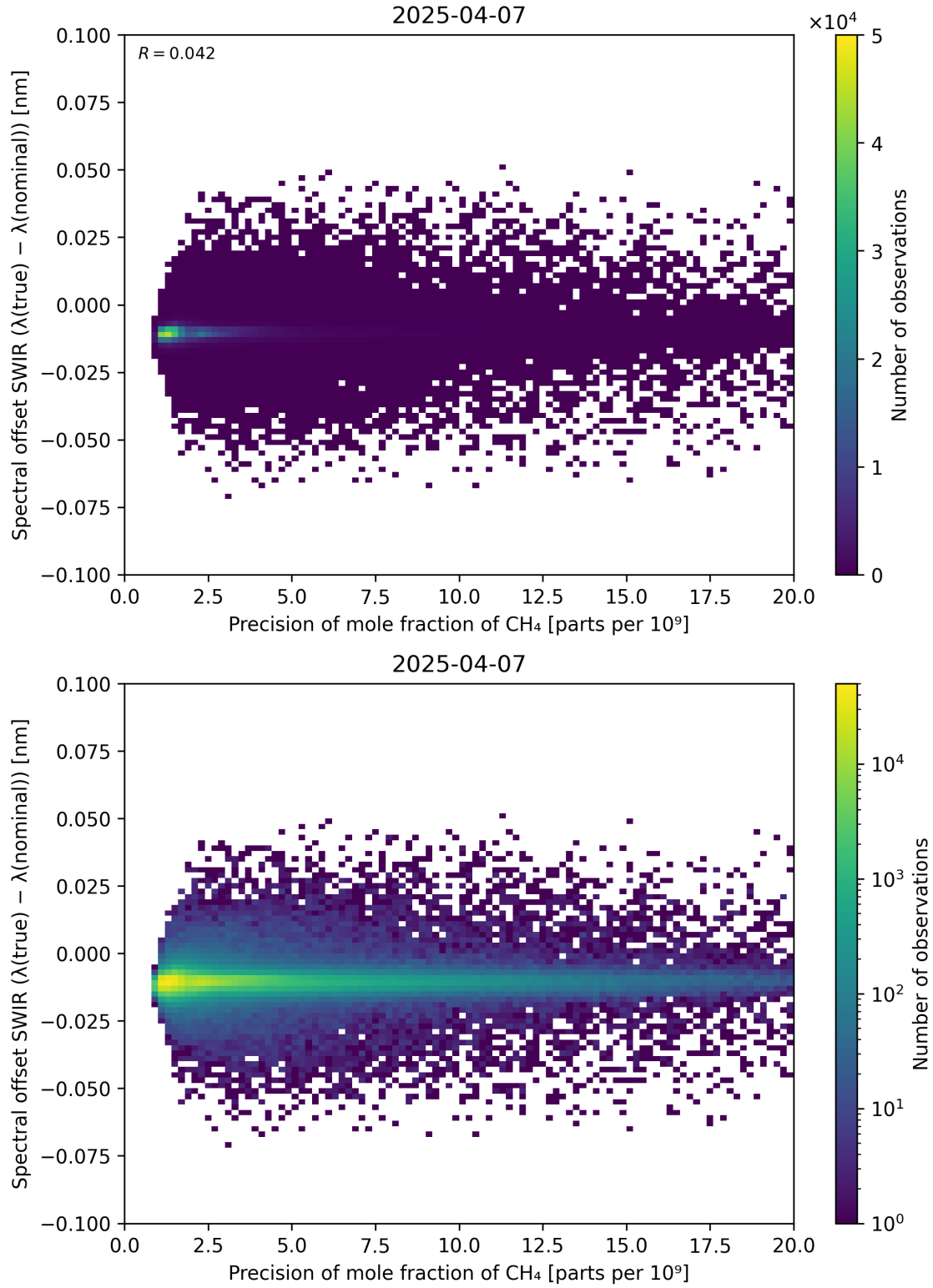
Figure 85: Scatter density plot of “Precision of mole fraction of CH 4 ” against “Spectral offset SWIR ( \lambda_{\text{true}} - \lambda_{\text{nominal}} )” for 2025-04-06 to 2025-04-08.
