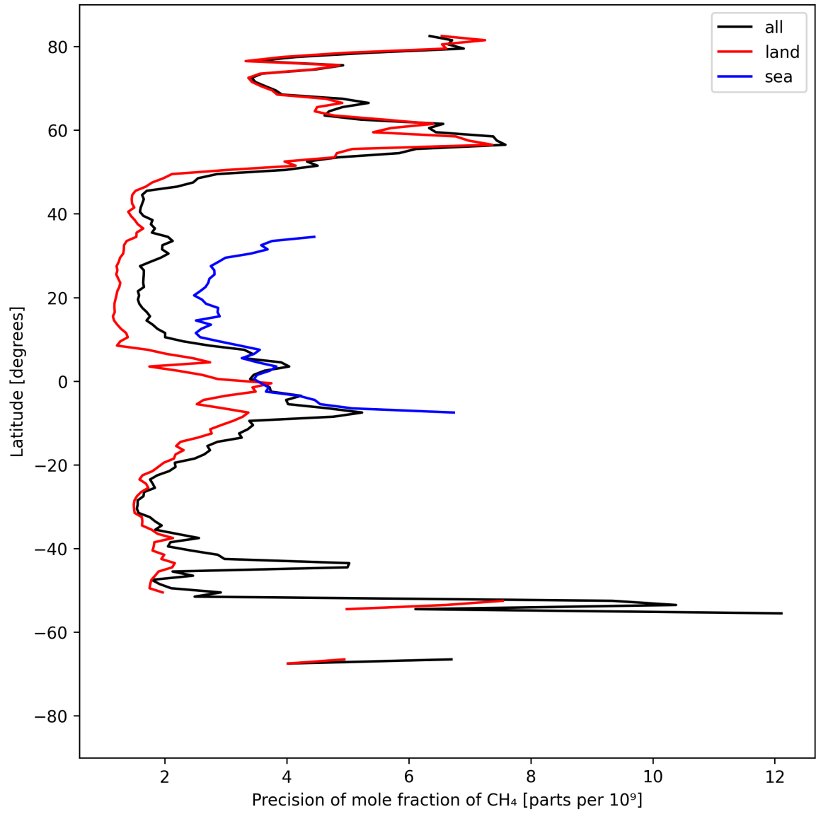
Figure 13: Zonal average of “Precision of mole fraction of CH 4 ” for 2025-04-06 to 2025-04-08.
