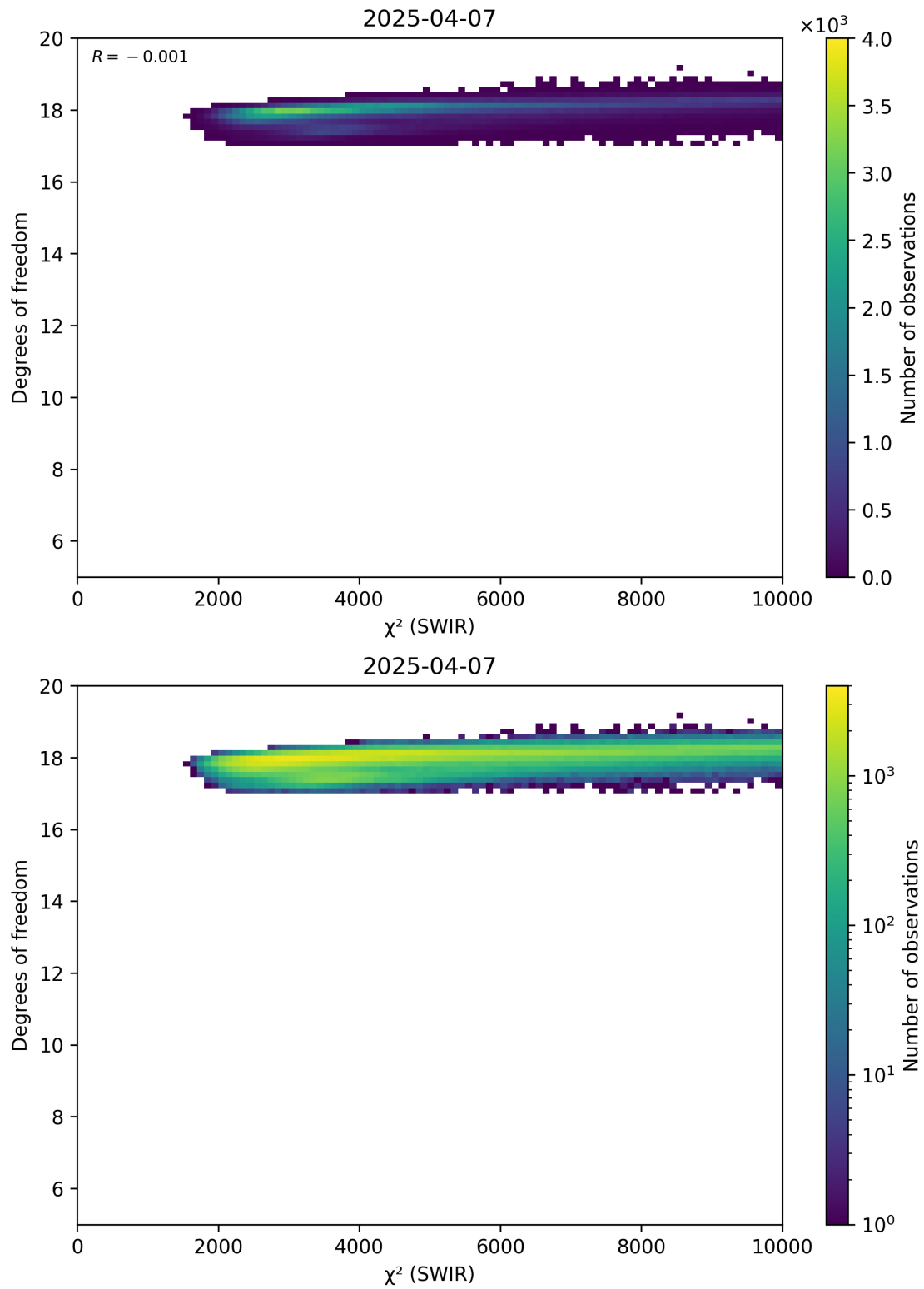
Figure 48: Scatter density plot of “ \chi^2 (SWIR)” against “Degrees of freedom” for 2025-04-06 to 2025-04-08.
