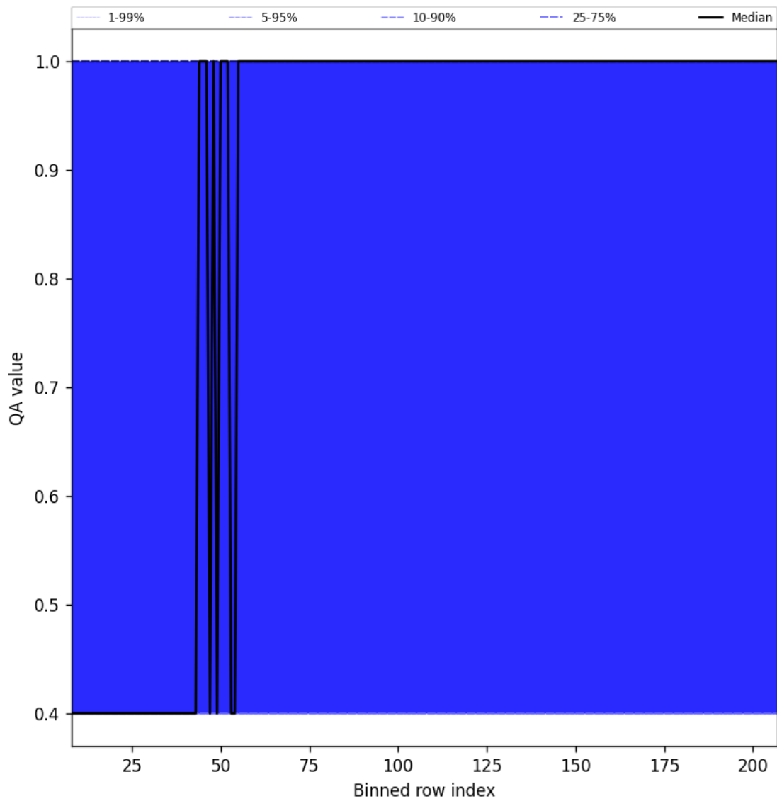
Figure 33: Along track statistics of “QA value” for 2025-04-06 to 2025-04-08
