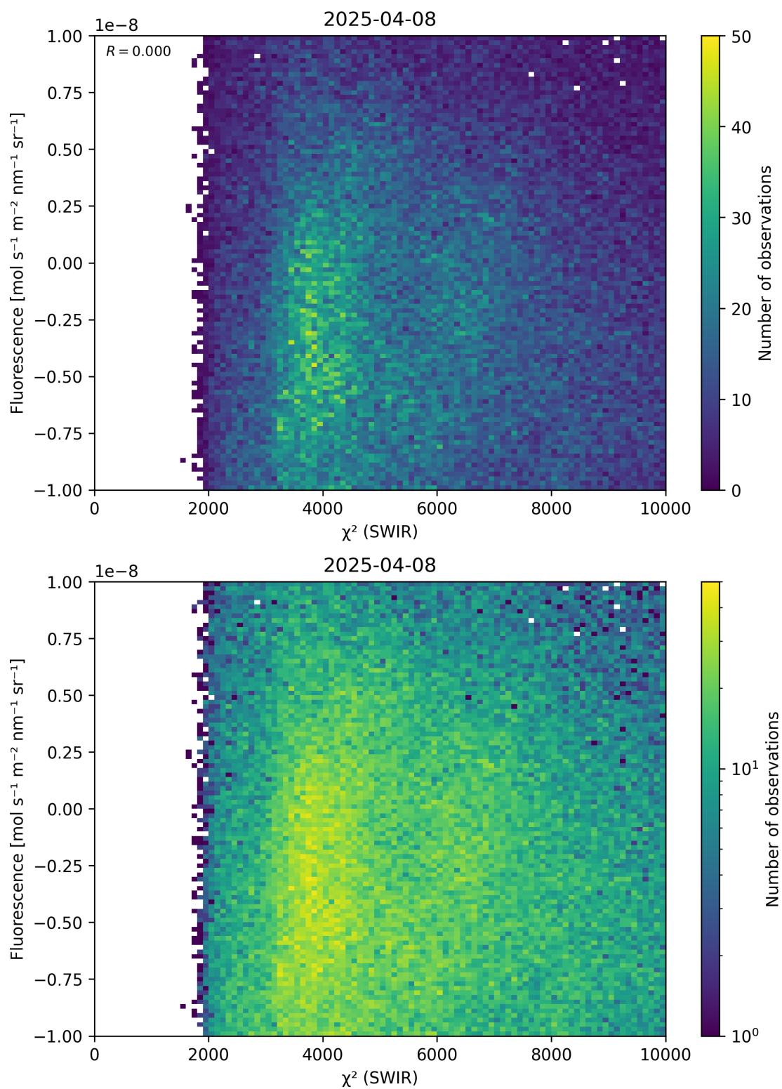
Figure 49: Scatter density plot of “ \chi^2 (SWIR)” against “Fluorescence” for 2025-04-08 to 2025-04-09.
