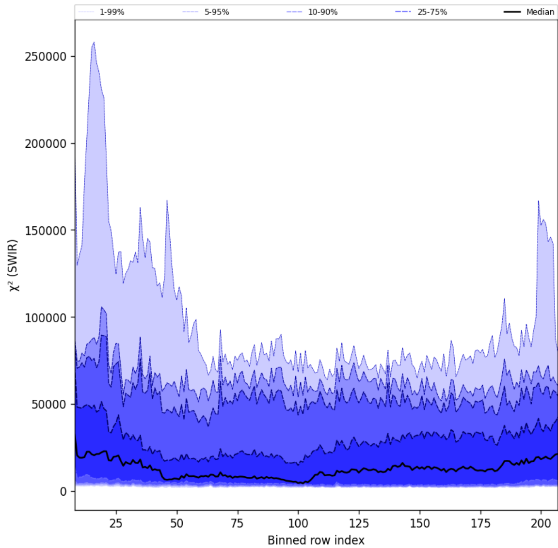
Figure 39: Along track statistics of “ \chi^2 (SWIR)” for 2025-04-08 to 2025-04-09
