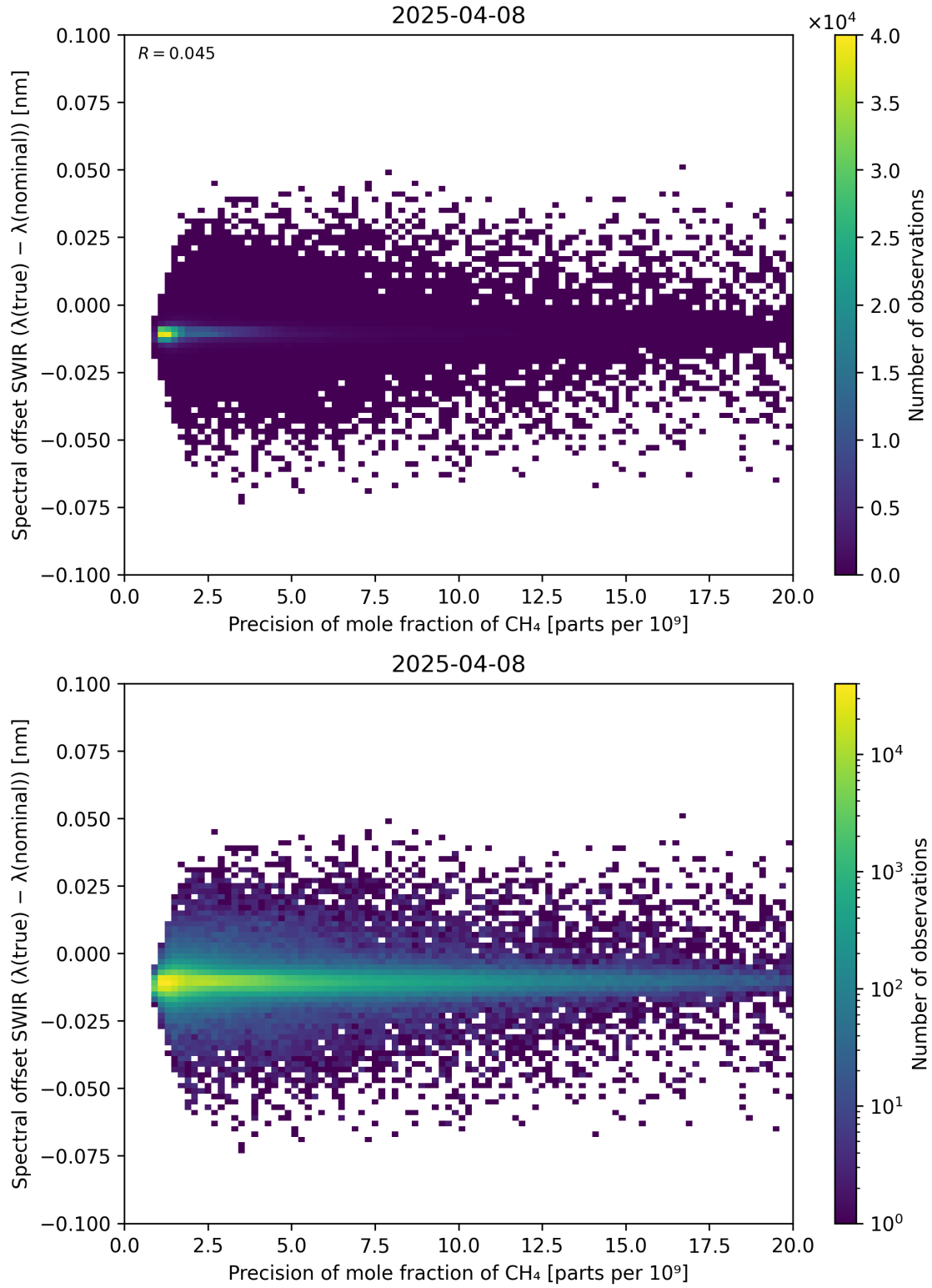
Figure 85: Scatter density plot of “Precision of mole fraction of CH 4 ” against “Spectral offset SWIR ( \lambda_{\text{true}} - \lambda_{\text{nominal}} )” for 2025-04-08 to 2025-04-09.
