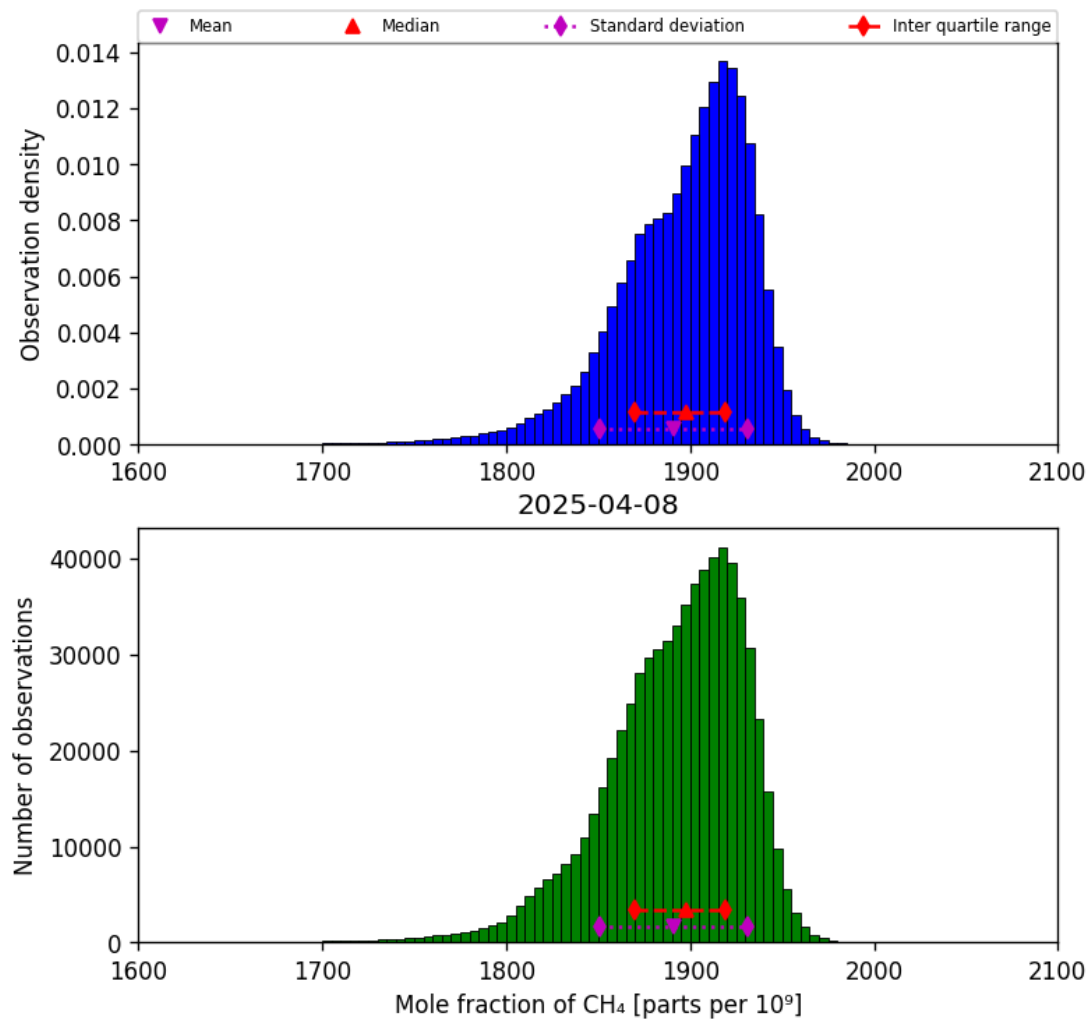
Figure 23: Histogram of “Mole fraction of CH 4 ” for 2025-04-08 to 2025-04-09
