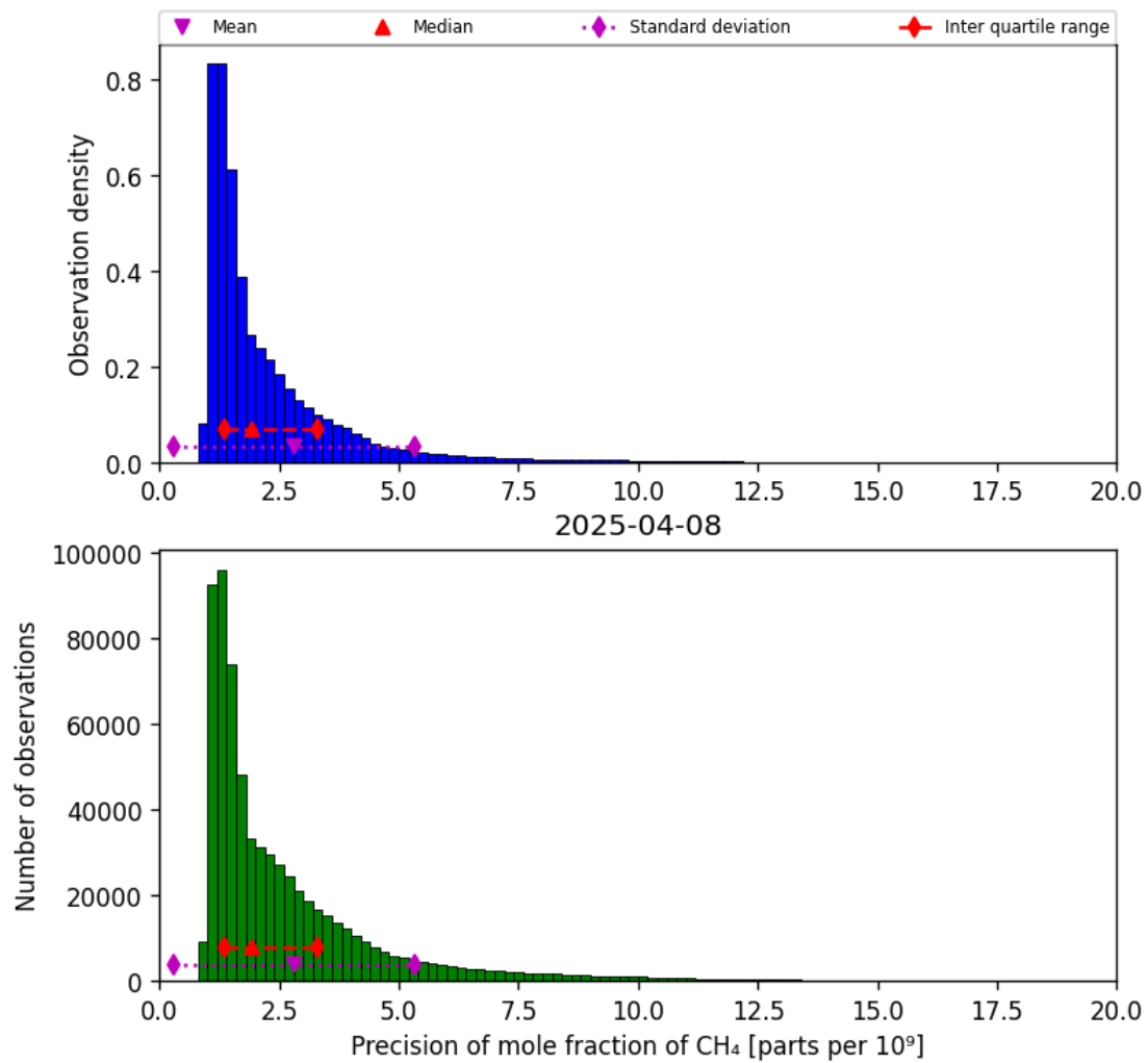
Figure 24: Histogram of “Precision of mole fraction of CH 4 ” for 2025-04-08 to 2025-04-09
