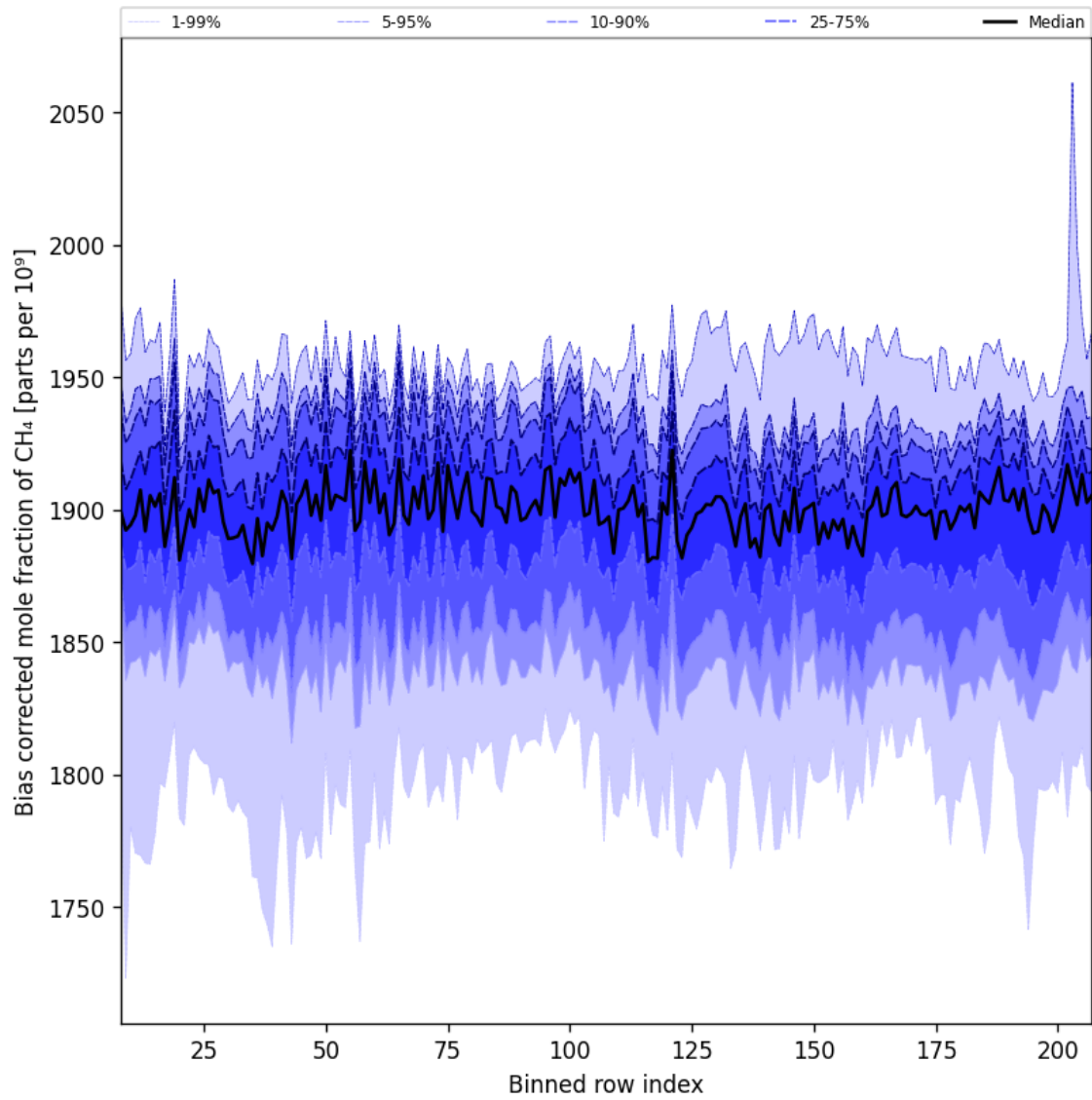
Figure 36: Along track statistics of “Bias corrected mole fraction of CH 4 ” for 2025-04-08 to 2025-04-09
