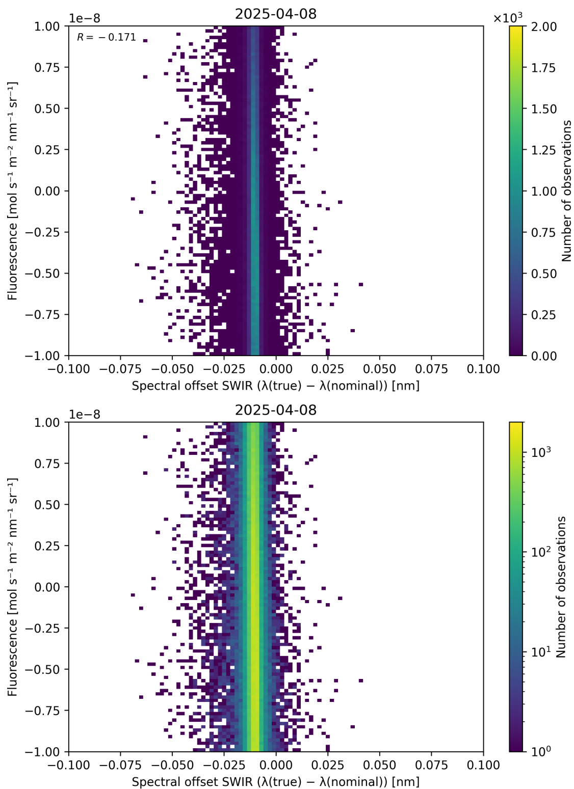
Figure 120: Scatter density plot of “Spectral offset SWIR ( \lambda_{\text{true}} - \lambda_{\text{nominal}} )” against “Fluorescence” for 2025-04-08 to 2025-04-09.
