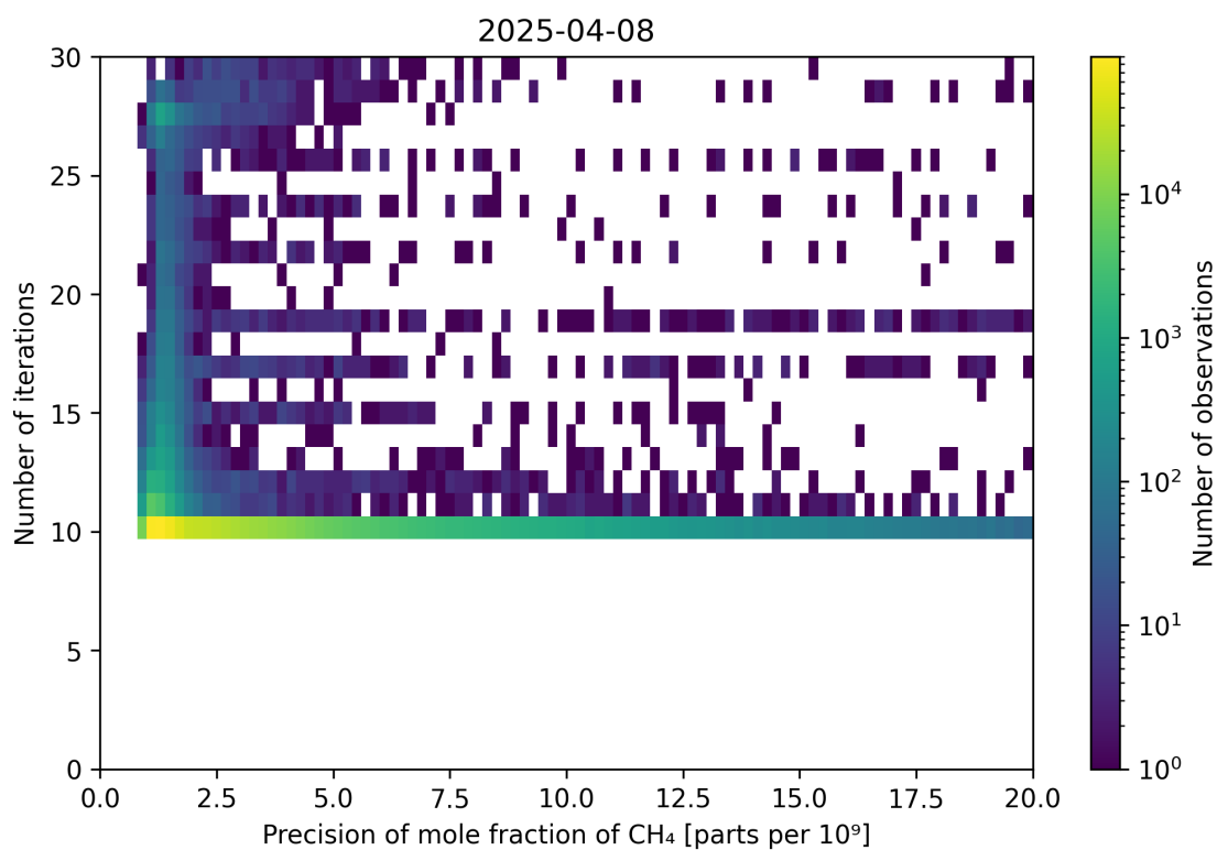
Figure 83: Scatter density plot of “Precision of mole fraction of CH 4 ” against “Number of iterations” for 2025-04-08 to 2025-04-09.
