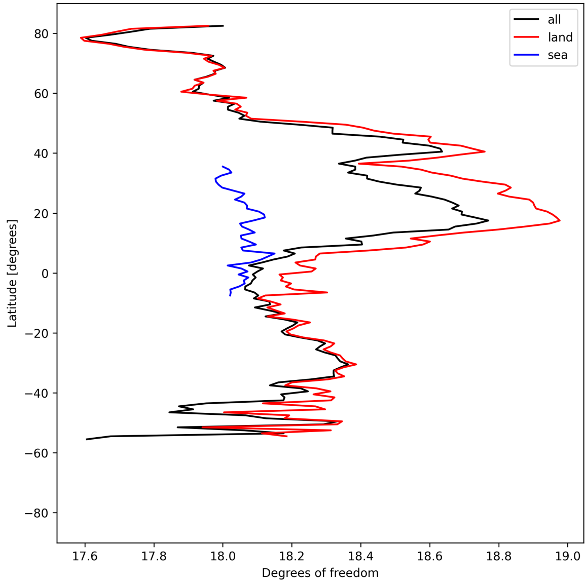
Figure 19: Zonal average of “Degrees of freedom” for 2025-04-08 to 2025-04-09.
