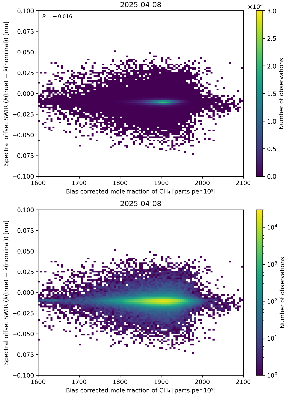
Figure 69: Scatter density plot of “Bias corrected mole fraction of \text{CH}_4 ” against “Spectral offset SWIR ( \lambda_{\text{true}} - \lambda_{\text{nominal}} )” for 2025-04-08 to 2025-04-09.
