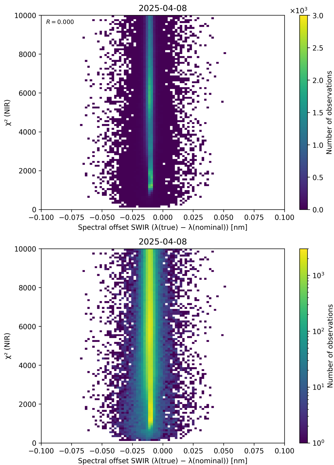
Figure 117: Scatter density plot of “Spectral offset SWIR ( \lambda_{\text{true}} - \lambda_{\text{nominal}} )” against “ \chi^2 (NIR)” for 2025-04-08 to 2025-04-09.
