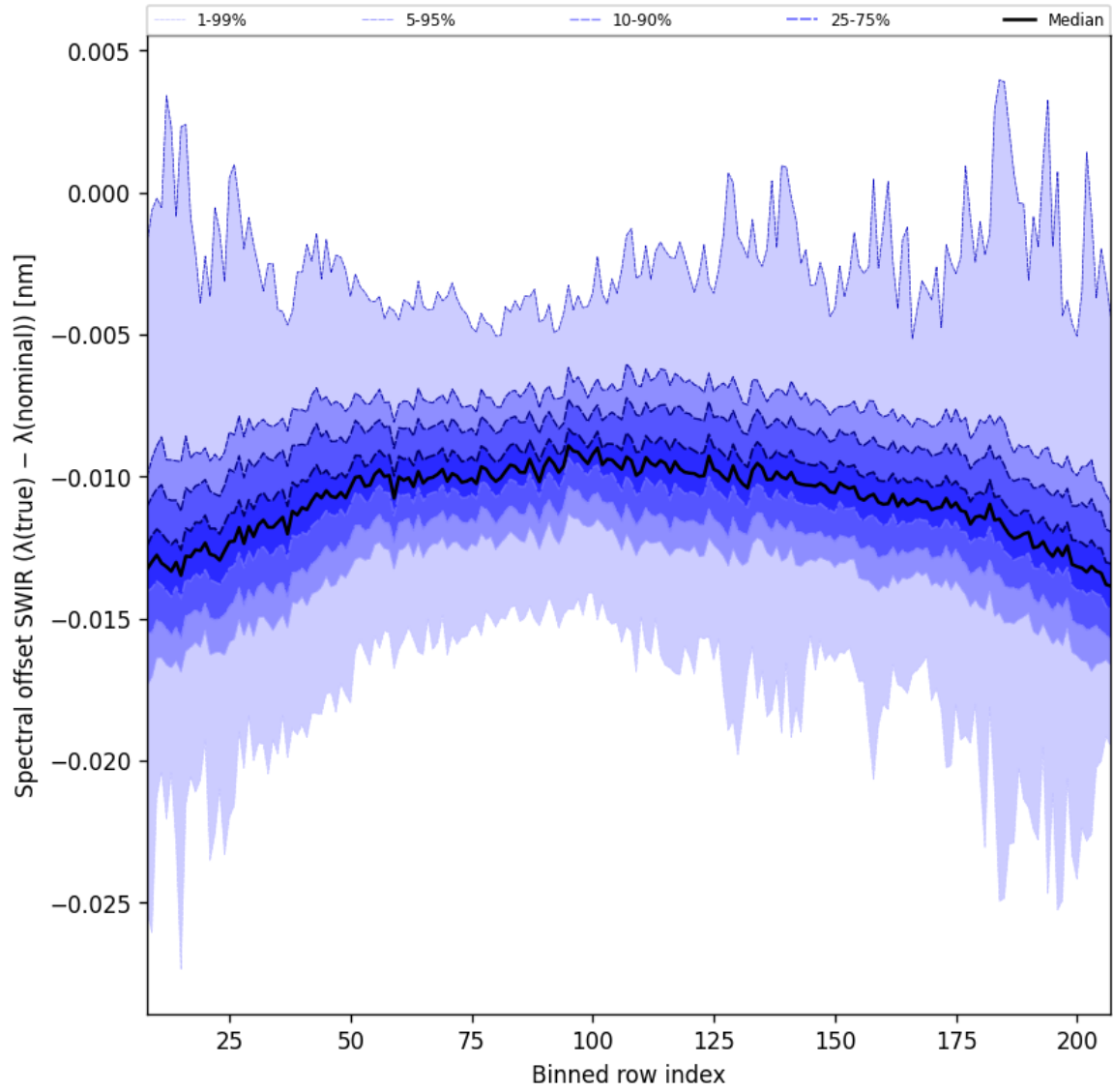
Figure 38: Along track statistics of “Spectral offset SWIR ( \lambda_{\text{true}} - \lambda_{\text{nominal}} )” for 2025-04-08 to 2025-04-09
