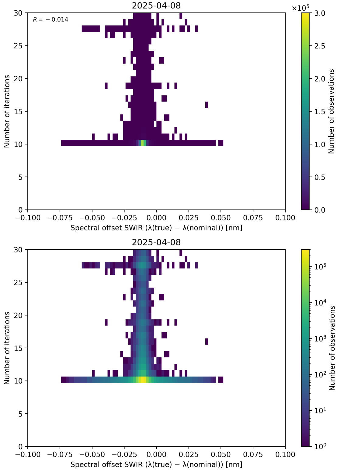
Figure 121: Scatter density plot of “Spectral offset SWIR ( \lambda_{\text{true}} - \lambda_{\text{nominal}} )” against “Number of iterations” for 2025-04-08 to 2025-04-09.
