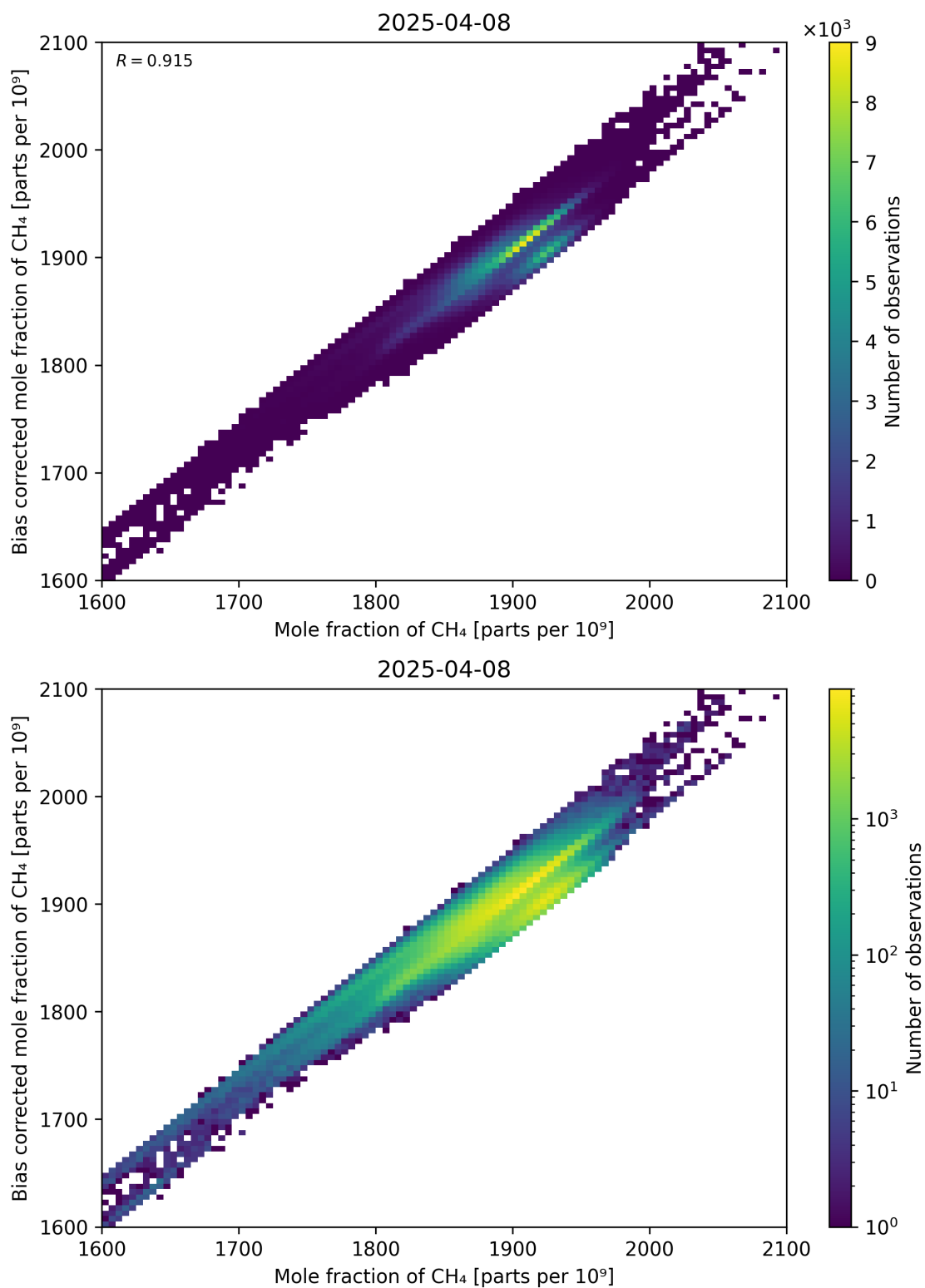
Figure 74: Scatter density plot of “Mole fraction of CH 4 ” against “Bias corrected mole fraction of CH 4 ” for 2025-04-08 to 2025-04-09.
