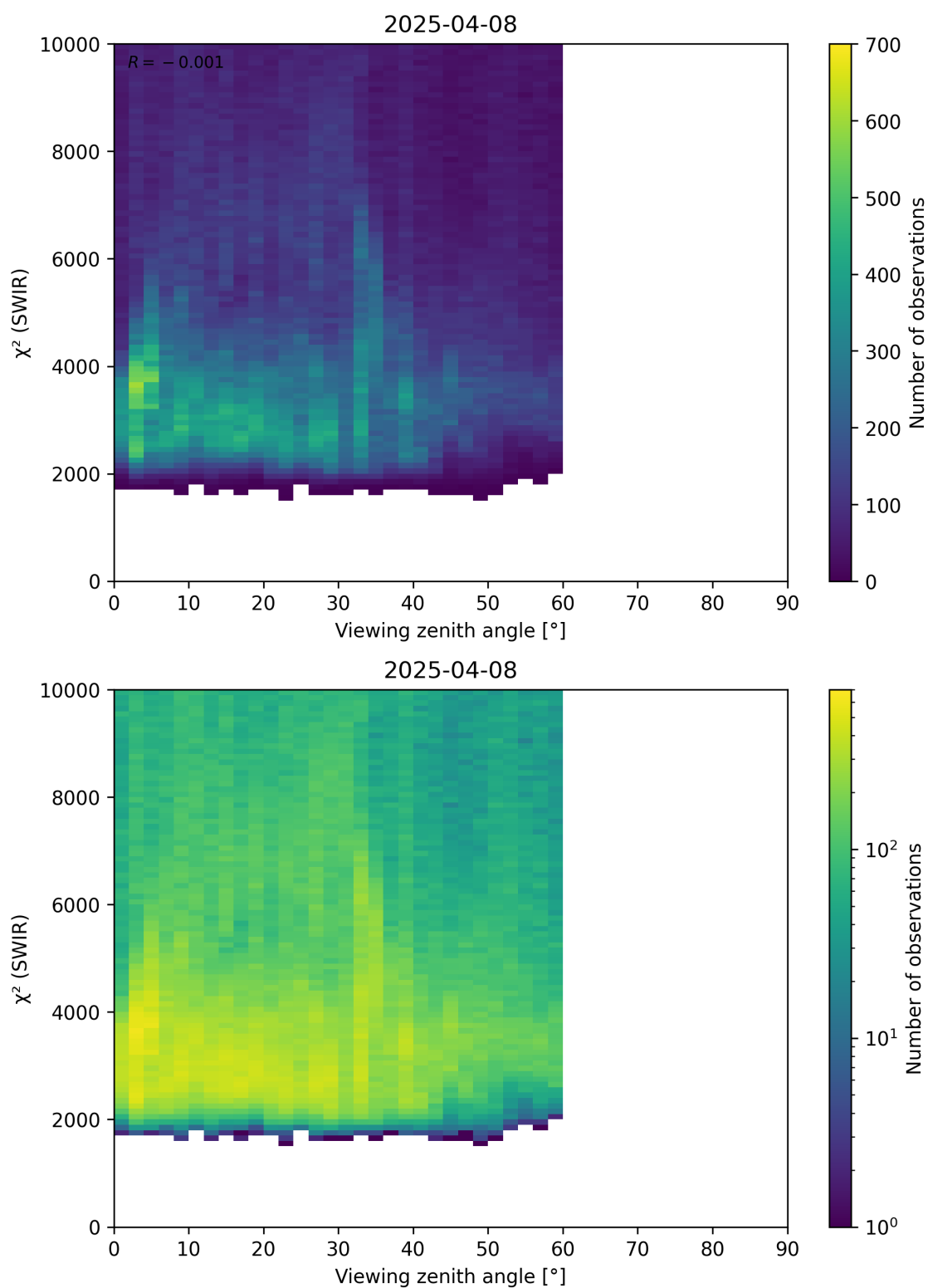
Figure 106: Scatter density plot of “Viewing zenith angle” against “ \chi^2 (SWIR)” for 2025-04-08 to 2025-04-09.
