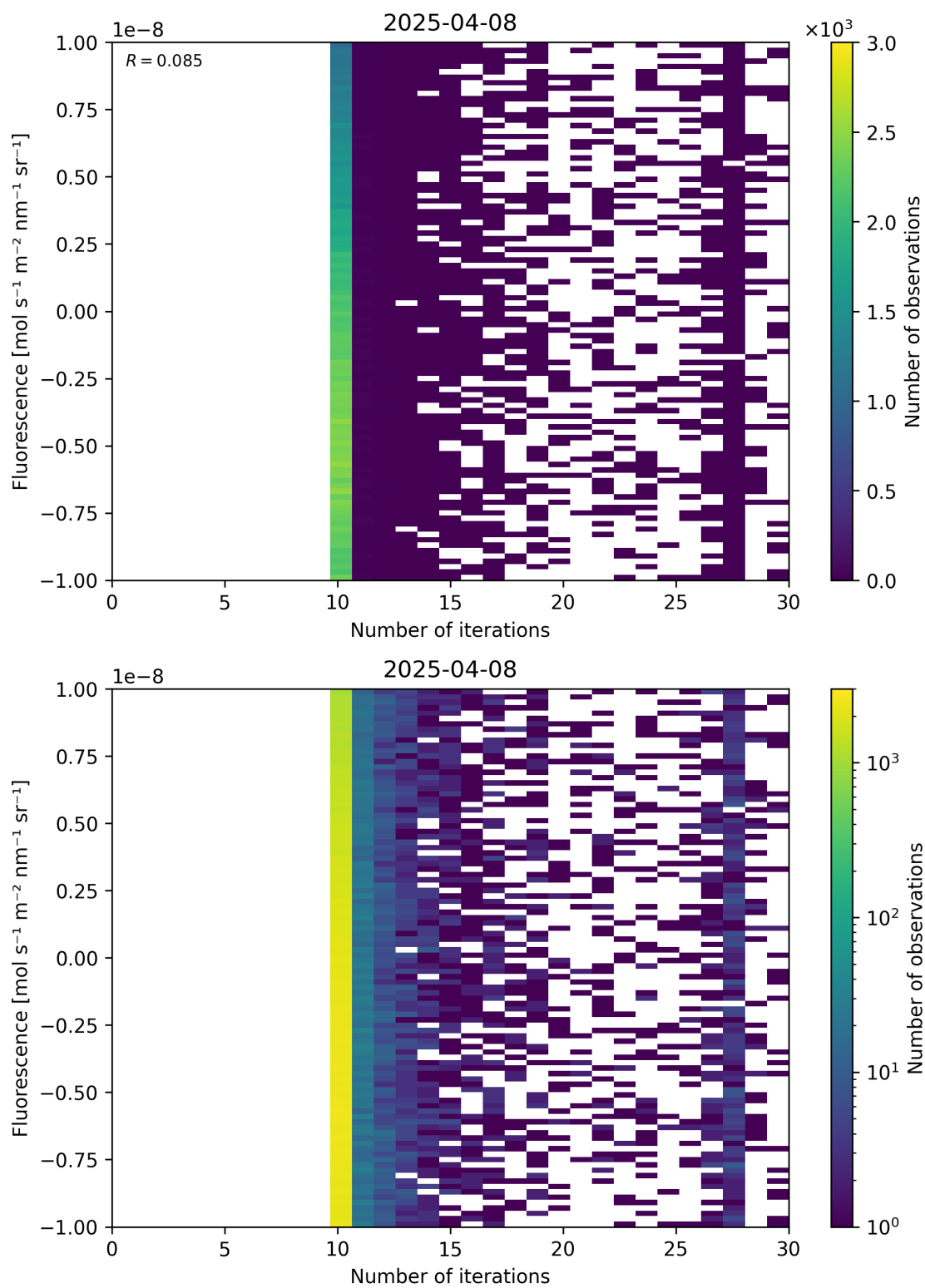
Figure 87: Scatter density plot of “Number of iterations” against “Fluorescence” for 2025-04-08 to 2025-04-09.
