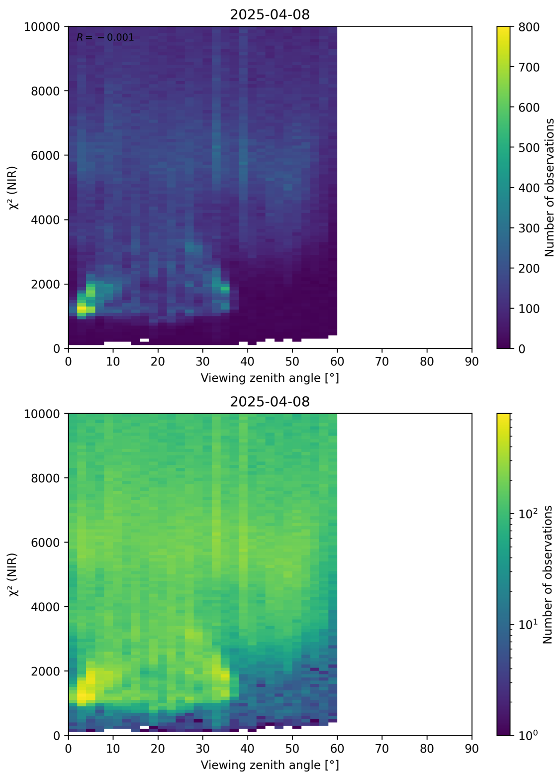
Figure 105: Scatter density plot of “Viewing zenith angle” against “ \chi^2 (NIR)” for 2025-04-08 to 2025-04-09.
