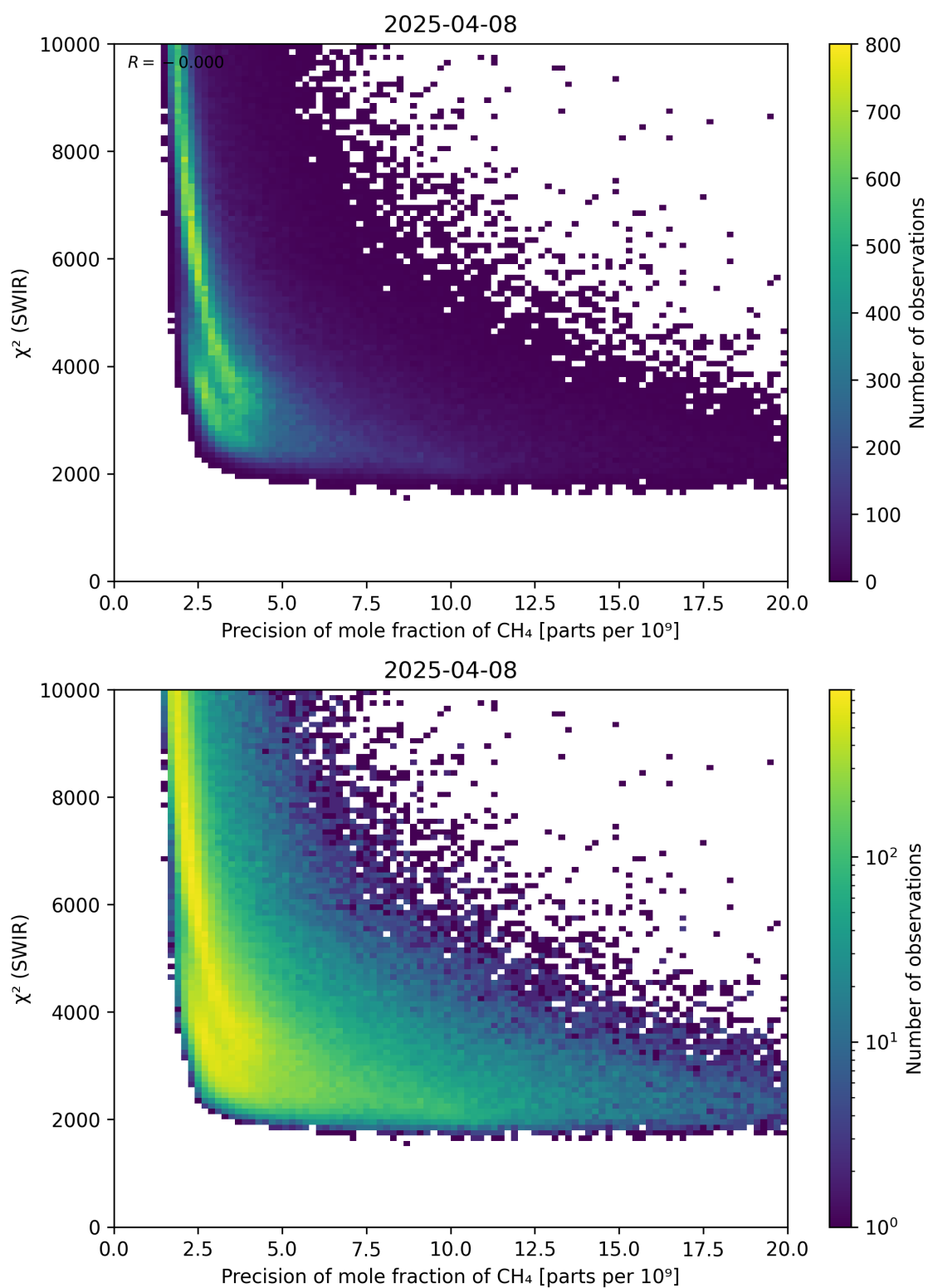
Figure 79: Scatter density plot of “Precision of mole fraction of \text{CH}_4 ” against “ \chi^2 (SWIR)” for 2025-04-08 to 2025-04-09.
