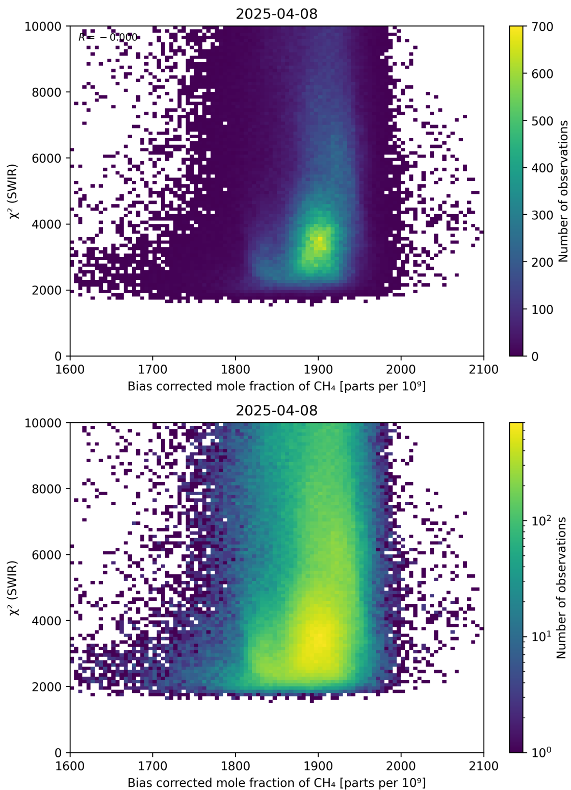
Figure 64: Scatter density plot of “Bias corrected mole fraction of \text{CH}_4 ” against “ \chi^2 (SWIR)” for 2025-04-08 to 2025-04-09.
