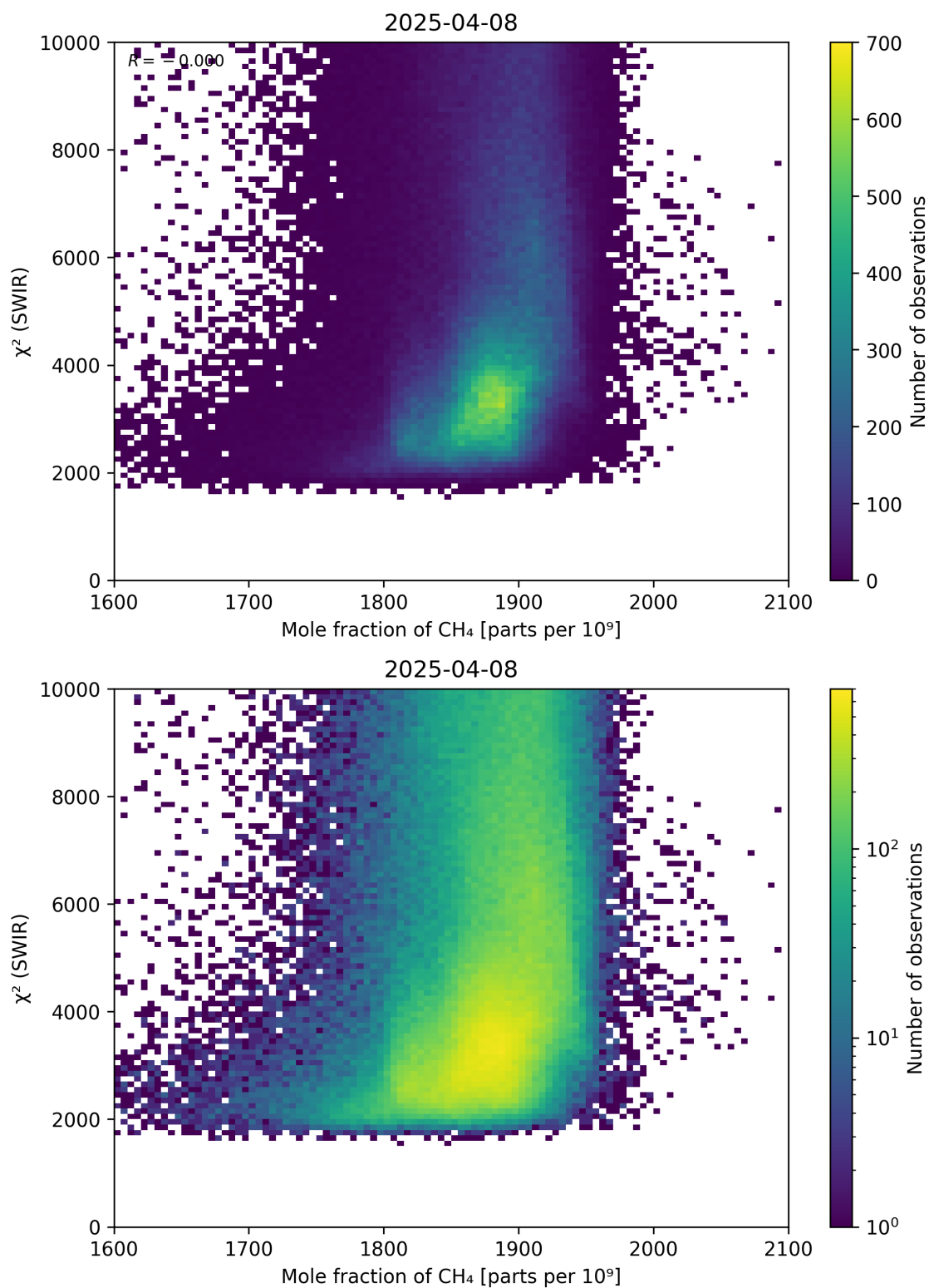
Figure 71: Scatter density plot of “Mole fraction of \text{CH}_4 ” against “ \chi^2 (SWIR)” for 2025-04-08 to 2025-04-09.
