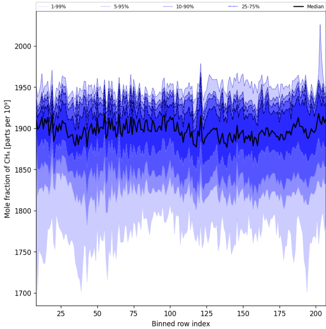
Figure 34: Along track statistics of “Mole fraction of CH 4 ” for 2025-04-08 to 2025-04-09
