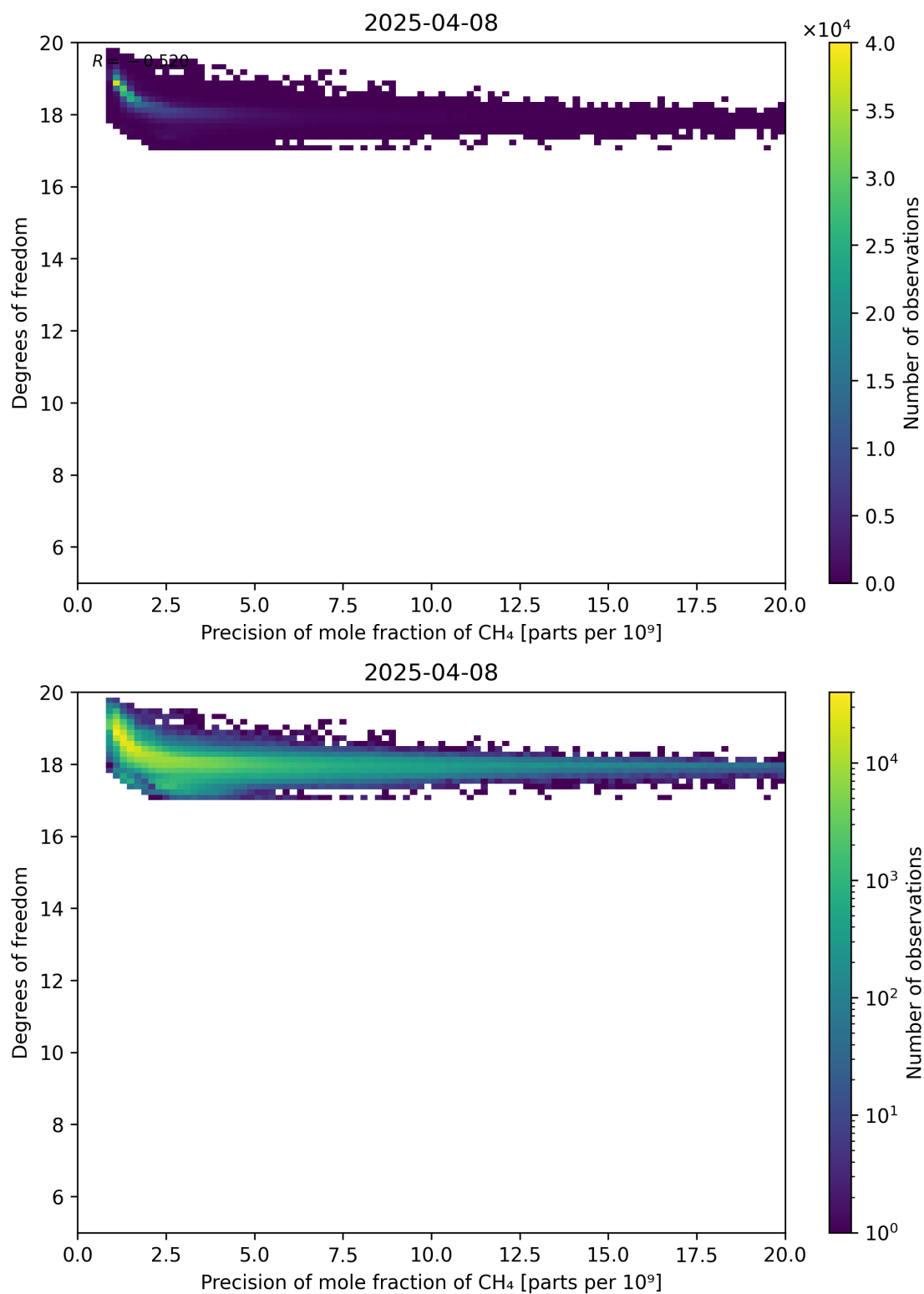
Figure 80: Scatter density plot of “Precision of mole fraction of CH 4 ” against “Degrees of freedom” for 2025-04-08 to 2025-04-09.
