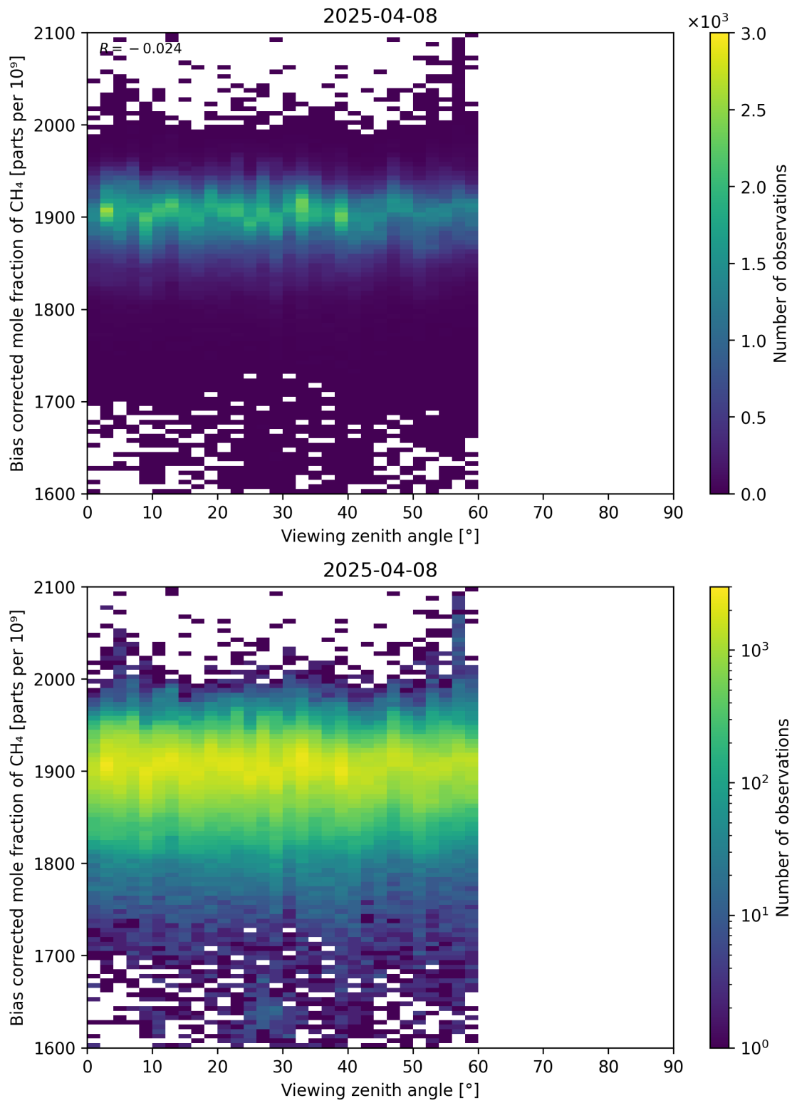
Figure 111: Scatter density plot of “Viewing zenith angle” against “Bias corrected mole fraction of CH 4 ” for 2025-04-08 to 2025-04-09.
