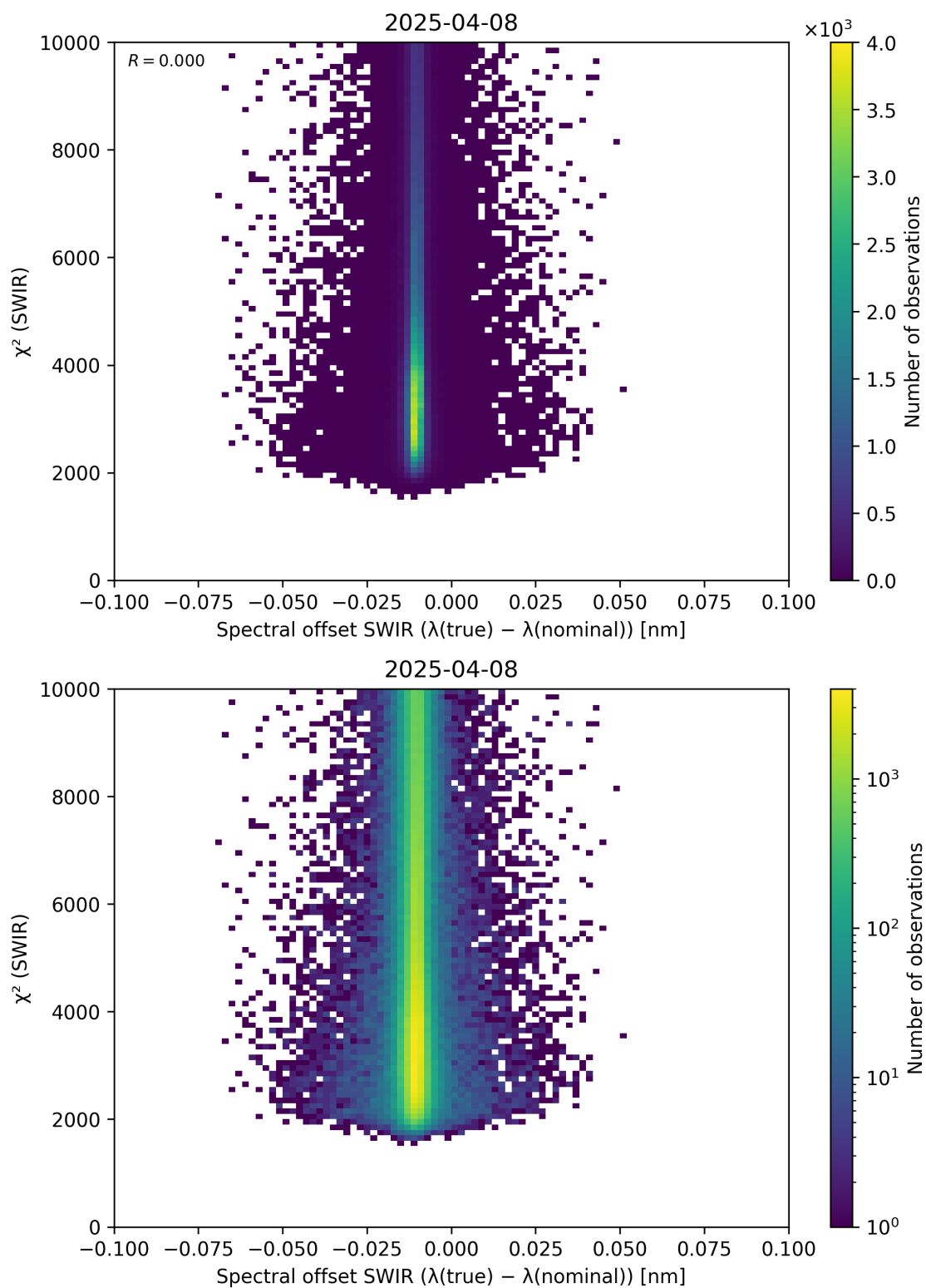
Figure 118: Scatter density plot of “Spectral offset SWIR ( \lambda_{\text{true}} - \lambda_{\text{nominal}} )” against “ \chi^2 (SWIR)” for 2025-04-08 to 2025-04-09.
