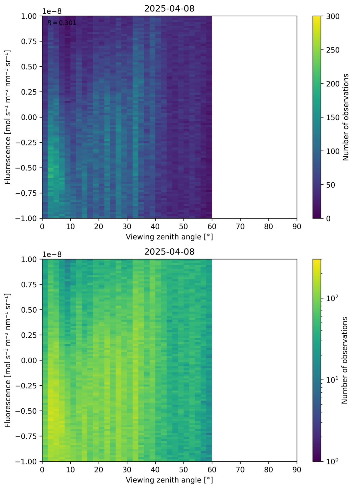
Figure 108: Scatter density plot of “Viewing zenith angle” against “Fluorescence” for 2025-04-08 to 2025-04-09.
