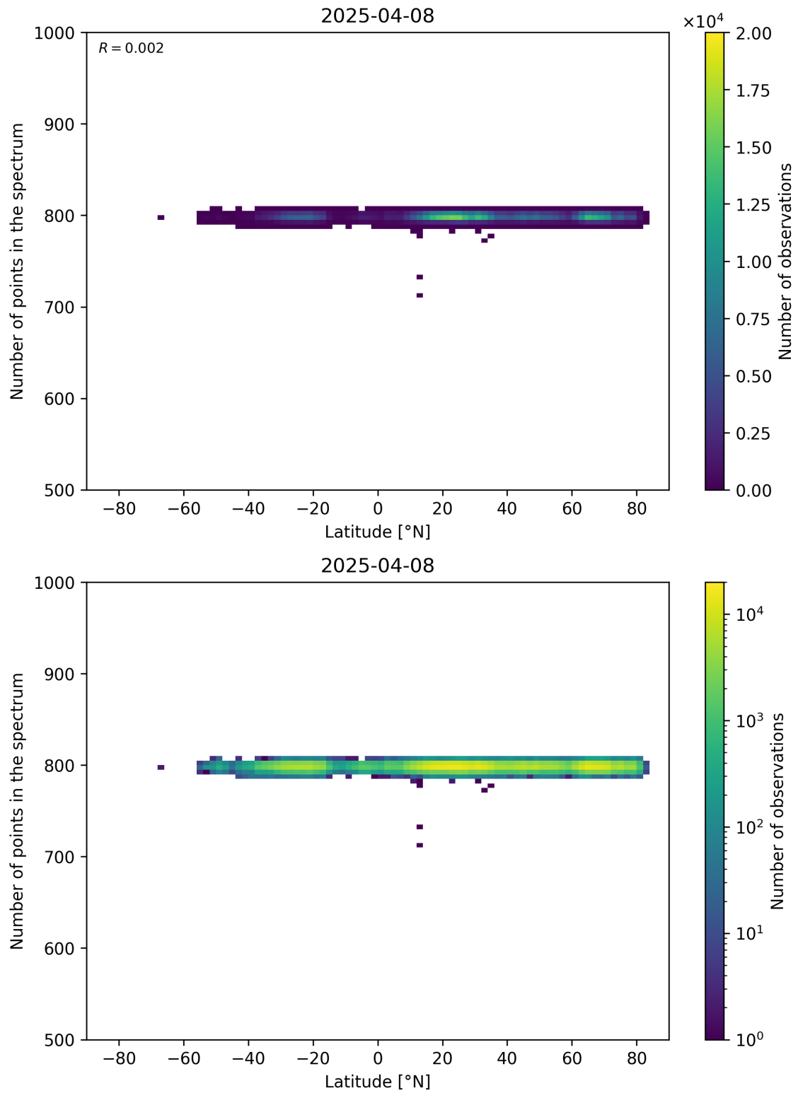
Figure 61: Scatter density plot of “Latitude” against “Number of points in the spectrum” for 2025-04-08 to 2025-04-09.
