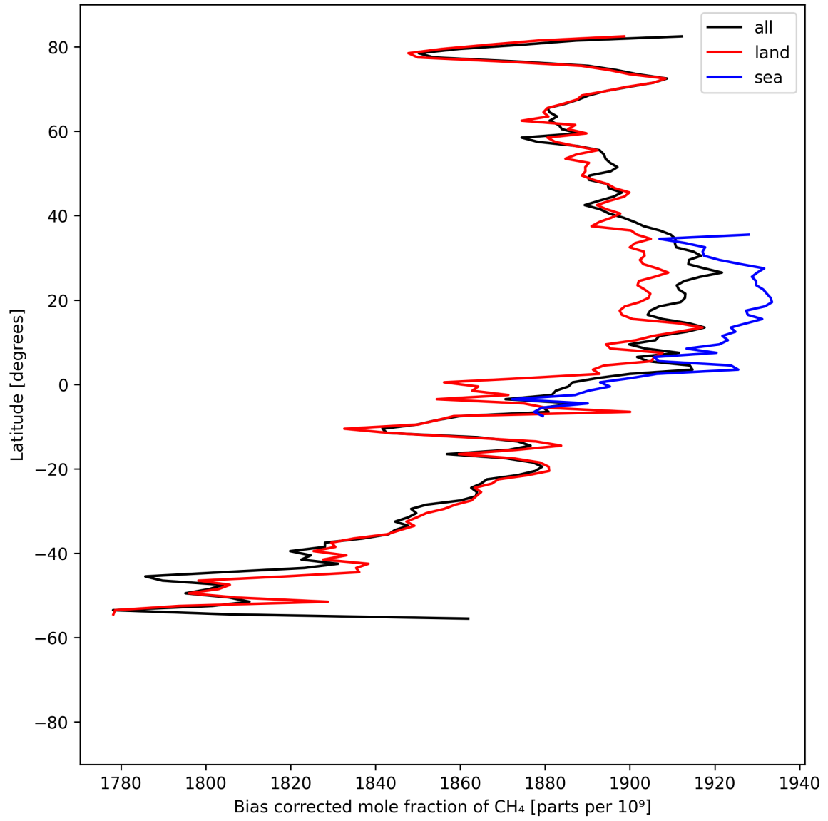
Figure 14: Zonal average of “Bias corrected mole fraction of CH 4 ” for 2025-04-08 to 2025-04-09.
