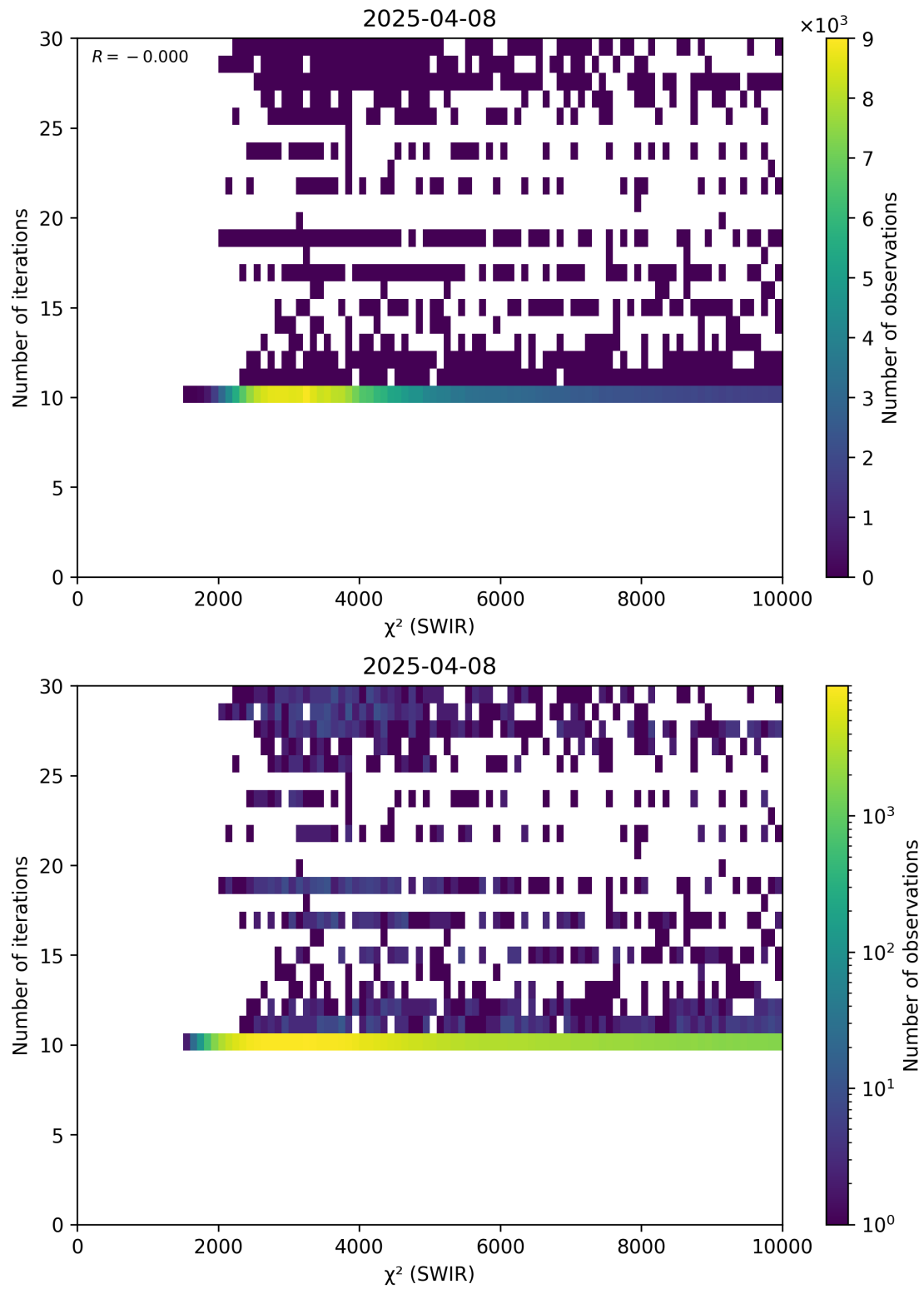
Figure 50: Scatter density plot of “ \chi^2 (SWIR)” against “Number of iterations” for 2025-04-08 to 2025-04-09.
