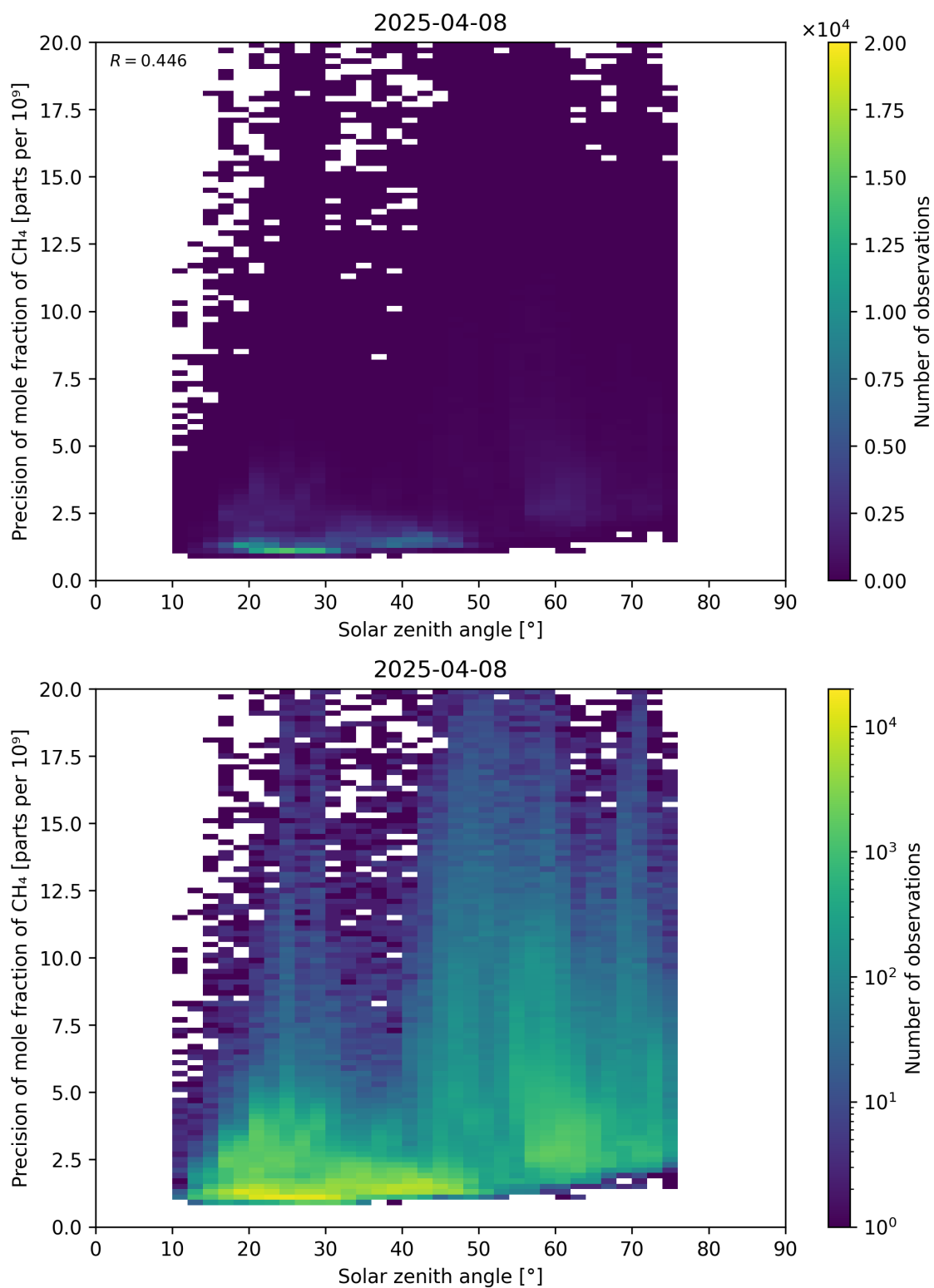
Figure 101: Scatter density plot of “Solar zenith angle” against “Precision of mole fraction of CH 4 ” for 2025-04-08 to 2025-04-09.
