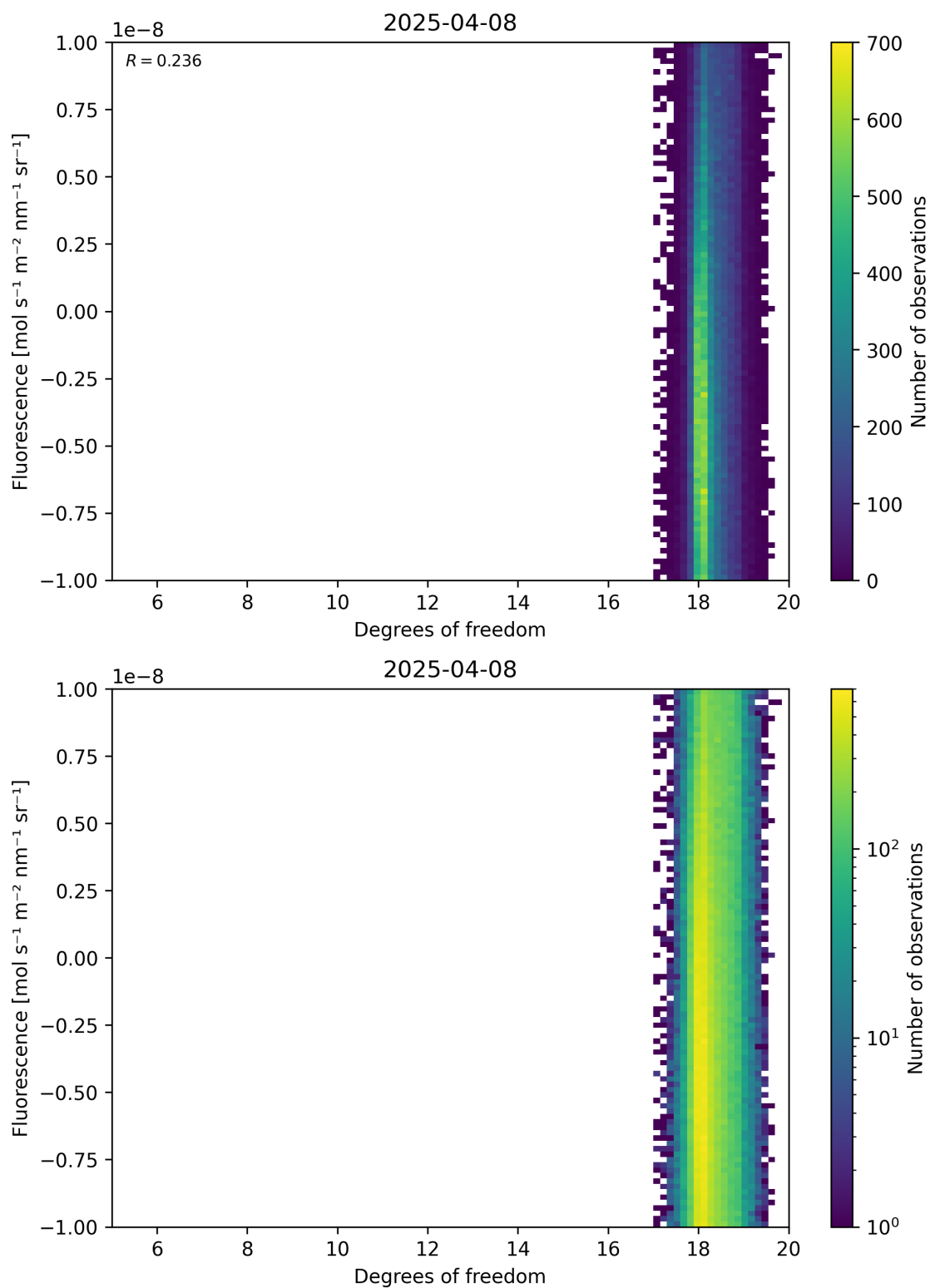
Figure 51: Scatter density plot of “Degrees of freedom” against “Fluorescence” for 2025-04-08 to 2025-04-09.
