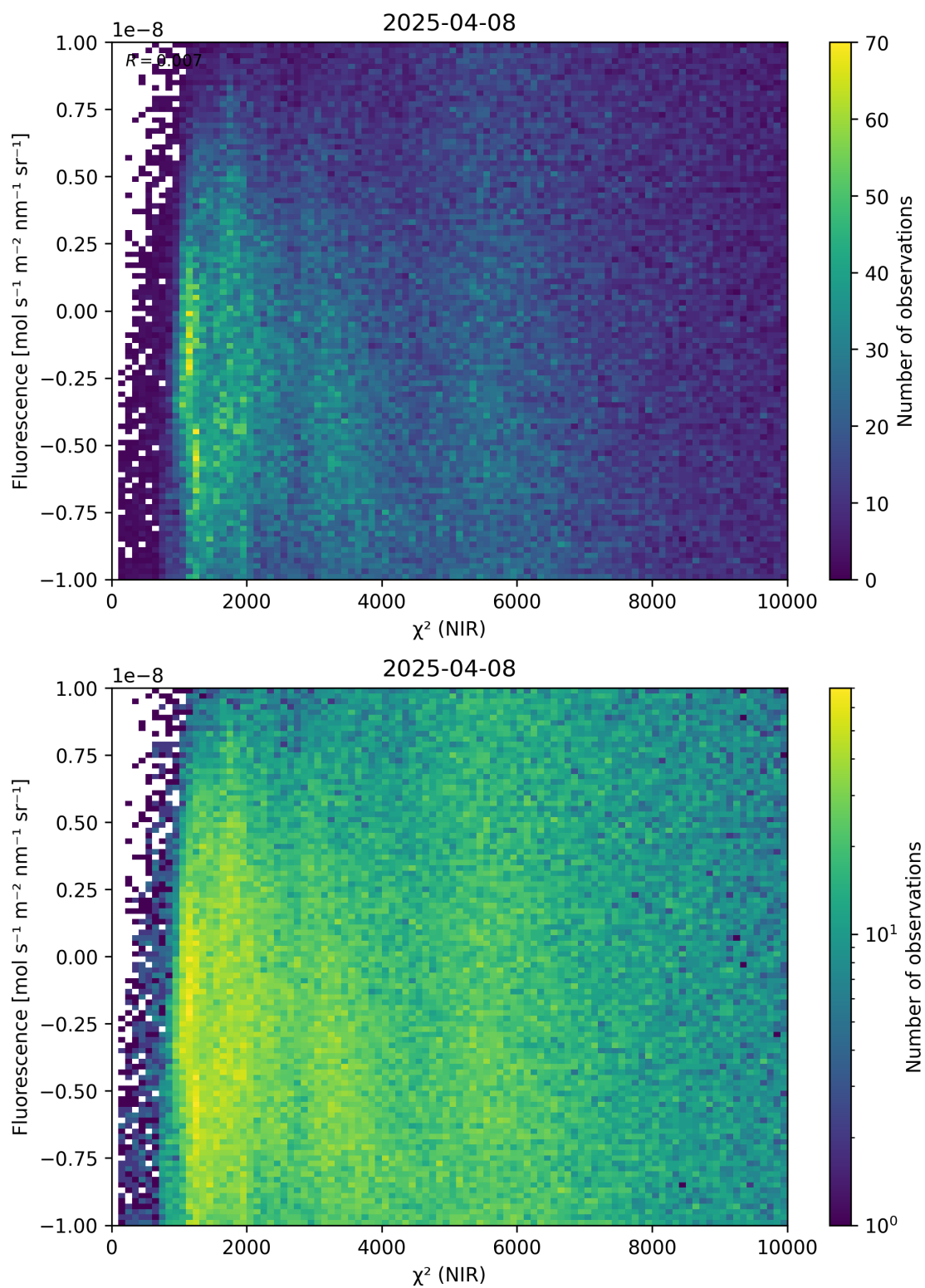
Figure 45: Scatter density plot of “ \chi^2 (NIR)” against “Fluorescence” for 2025-04-08 to 2025-04-09.
