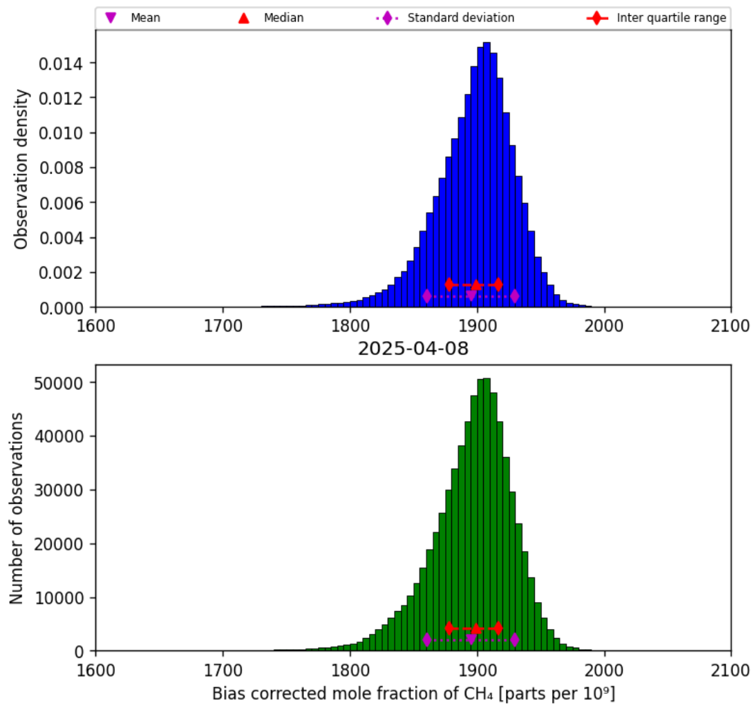
Figure 25: Histogram of “Bias corrected mole fraction of CH 4 ” for 2025-04-08 to 2025-04-09
