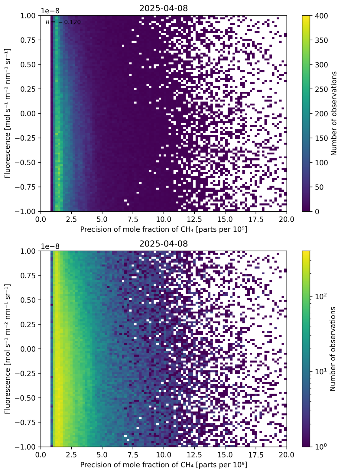
Figure 81: Scatter density plot of “Precision of mole fraction of CH 4 ” against “Fluorescence” for 2025-04-08 to 2025-04-09.
