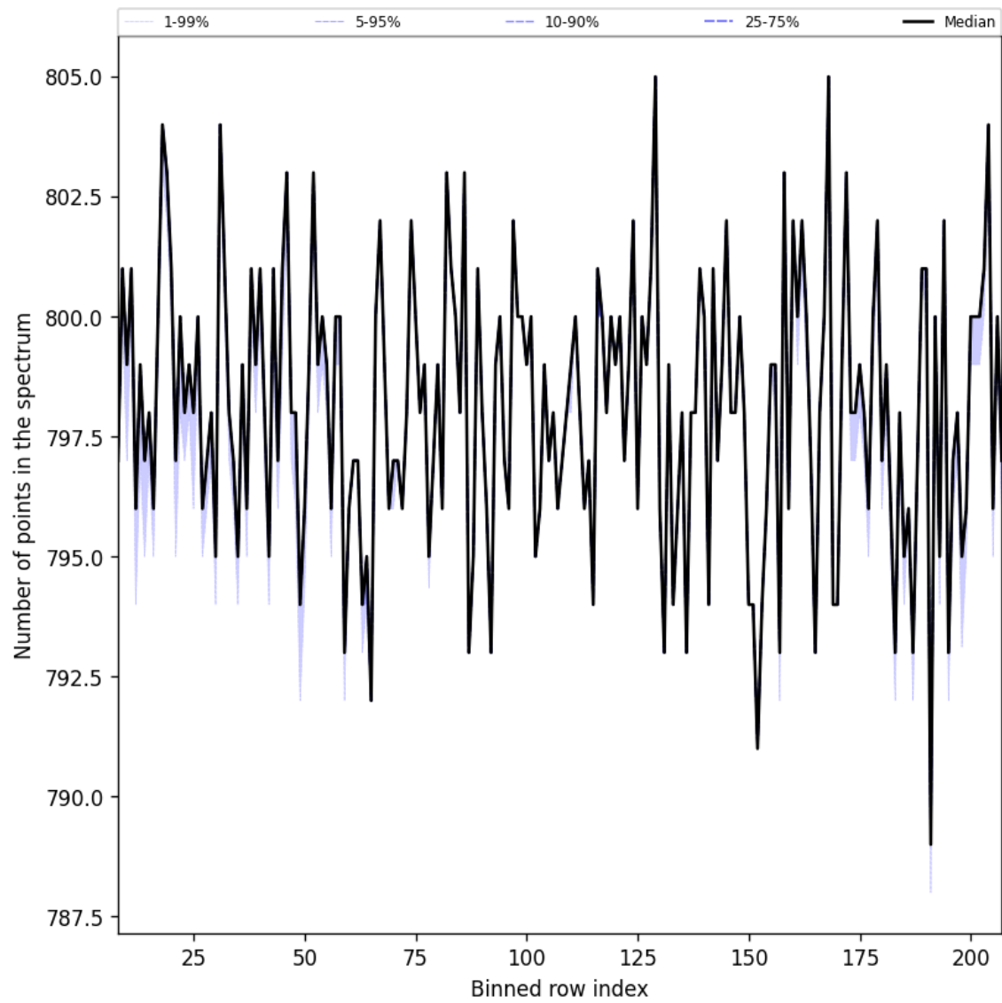
Figure 37: Along track statistics of “Number of points in the spectrum” for 2025-04-08 to 2025-04-09
