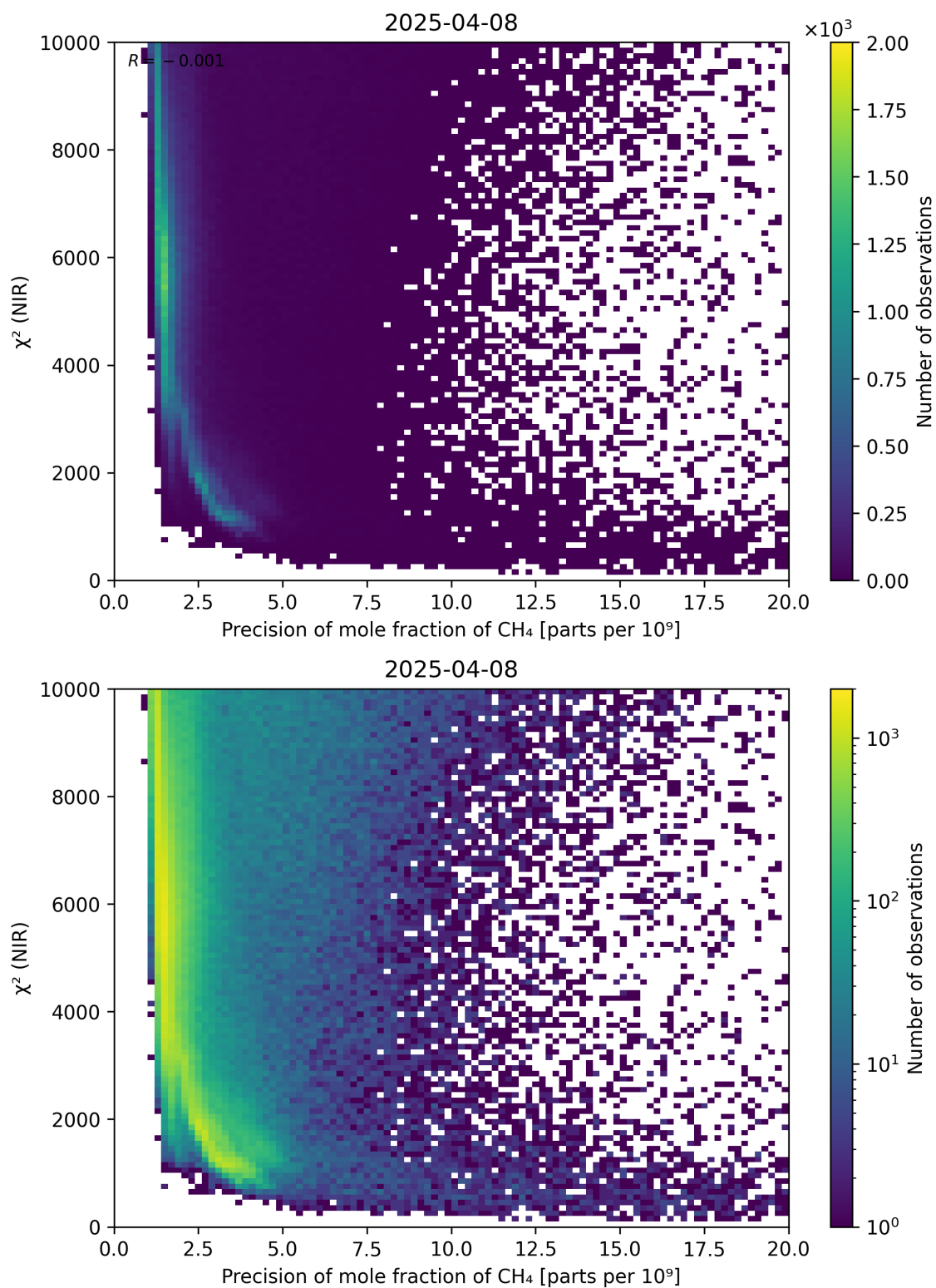
Figure 78: Scatter density plot of “Precision of mole fraction of \text{CH}_4 ” against “ \chi^2 (NIR)” for 2025-04-08 to 2025-04-09.
