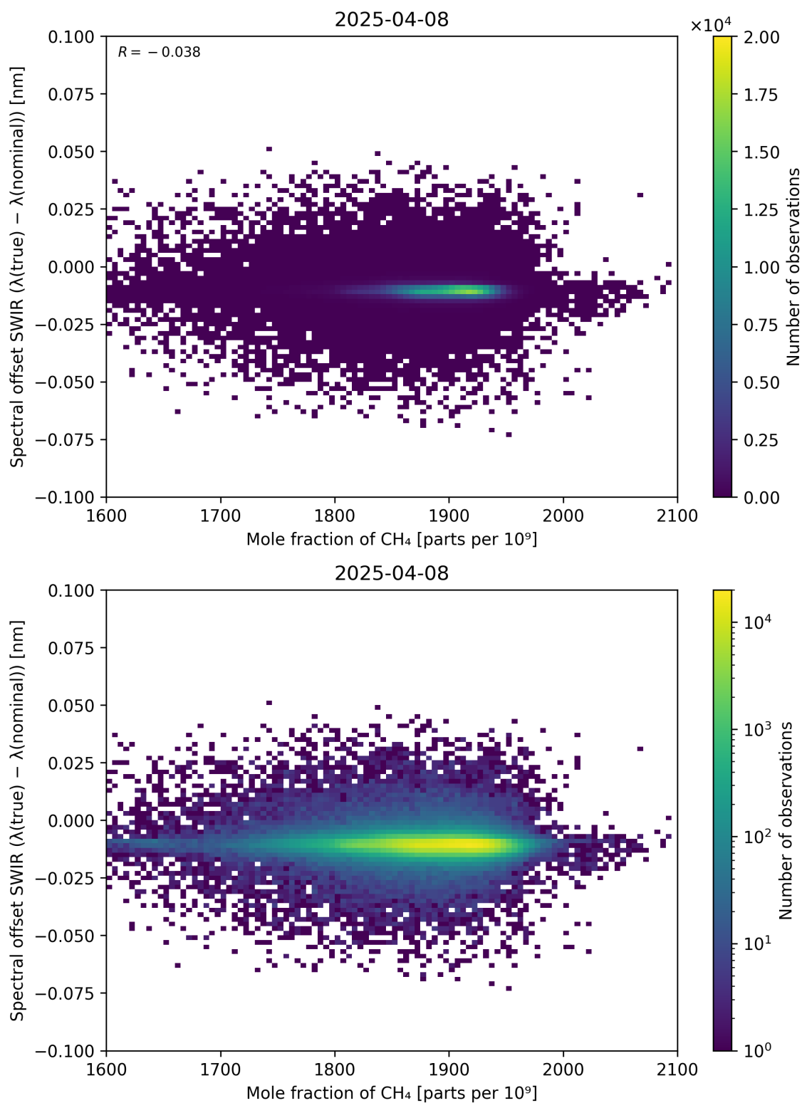
Figure 86: Scatter density plot of “Mole fraction of CH 4 ” against “Spectral offset SWIR ( \lambda_{\text{true}} - \lambda_{\text{nominal}} )” for 2025-04-08 to 2025-04-09.
