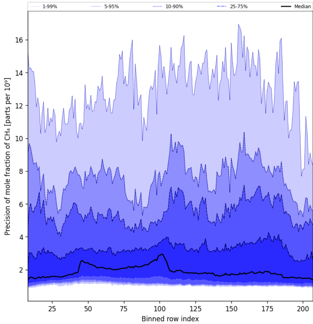
Figure 35: Along track statistics of “Precision of mole fraction of CH 4 ” for 2025-04-08 to 2025-04-09
