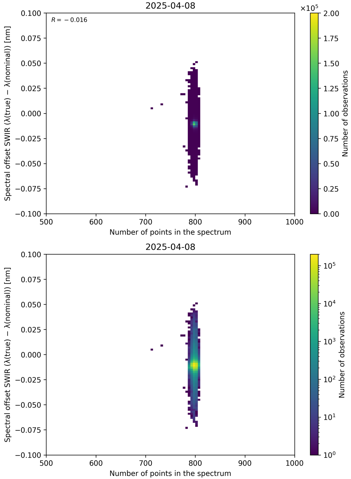
Figure 93: Scatter density plot of “Number of points in the spectrum” against “Spectral offset SWIR ( \lambda_{\text{true}} - \lambda_{\text{nominal}} )” for 2025-04-08 to 2025-04-09.
