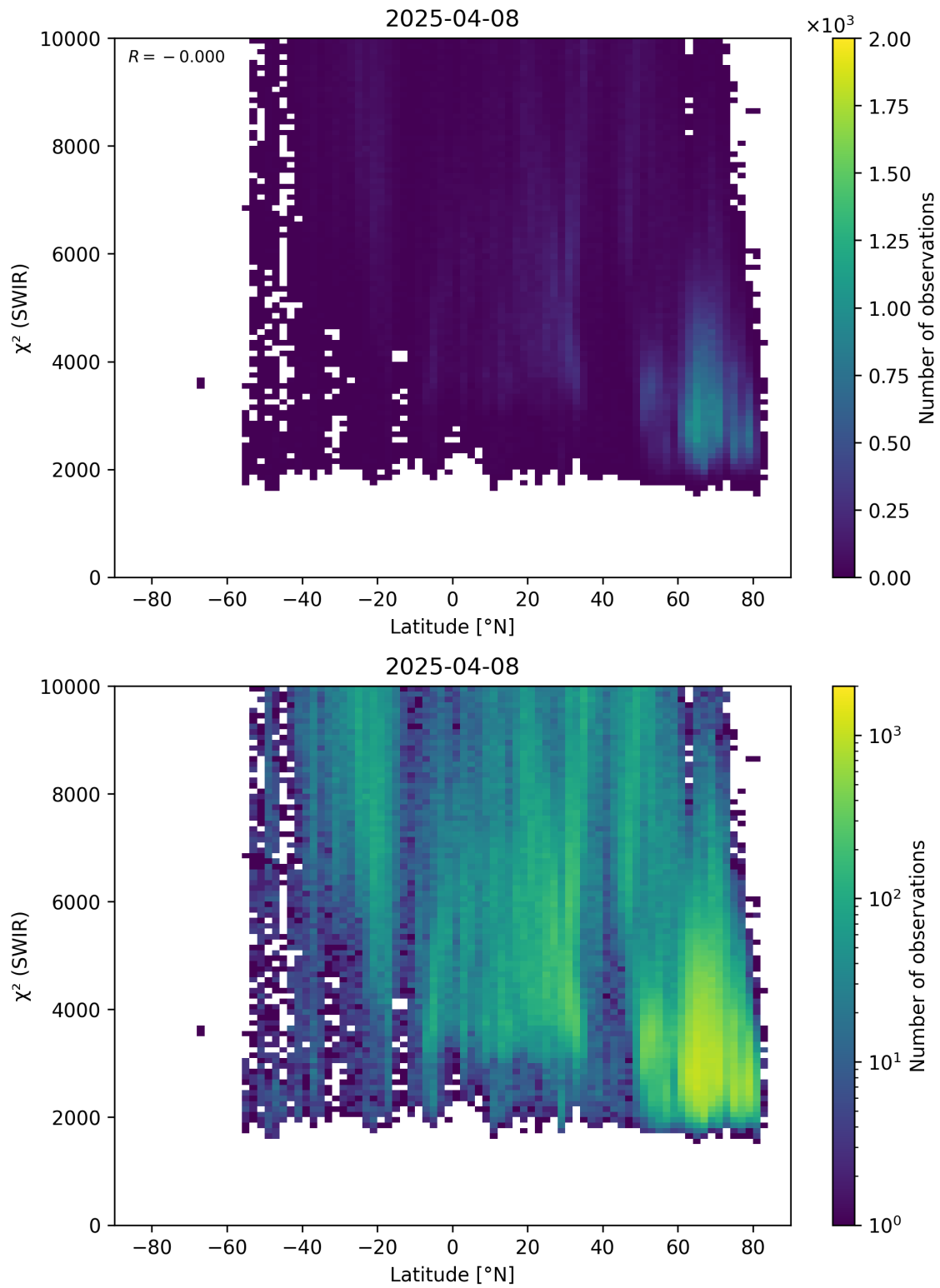
Figure 54: Scatter density plot of “Latitude” against “ \chi^2 (SWIR)” for 2025-04-08 to 2025-04-09.
