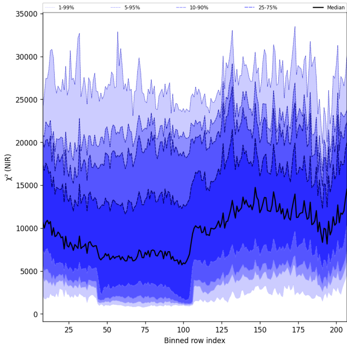
Figure 40: Along track statistics of “ \chi^2 (NIR)” for 2025-04-08 to 2025-04-09
