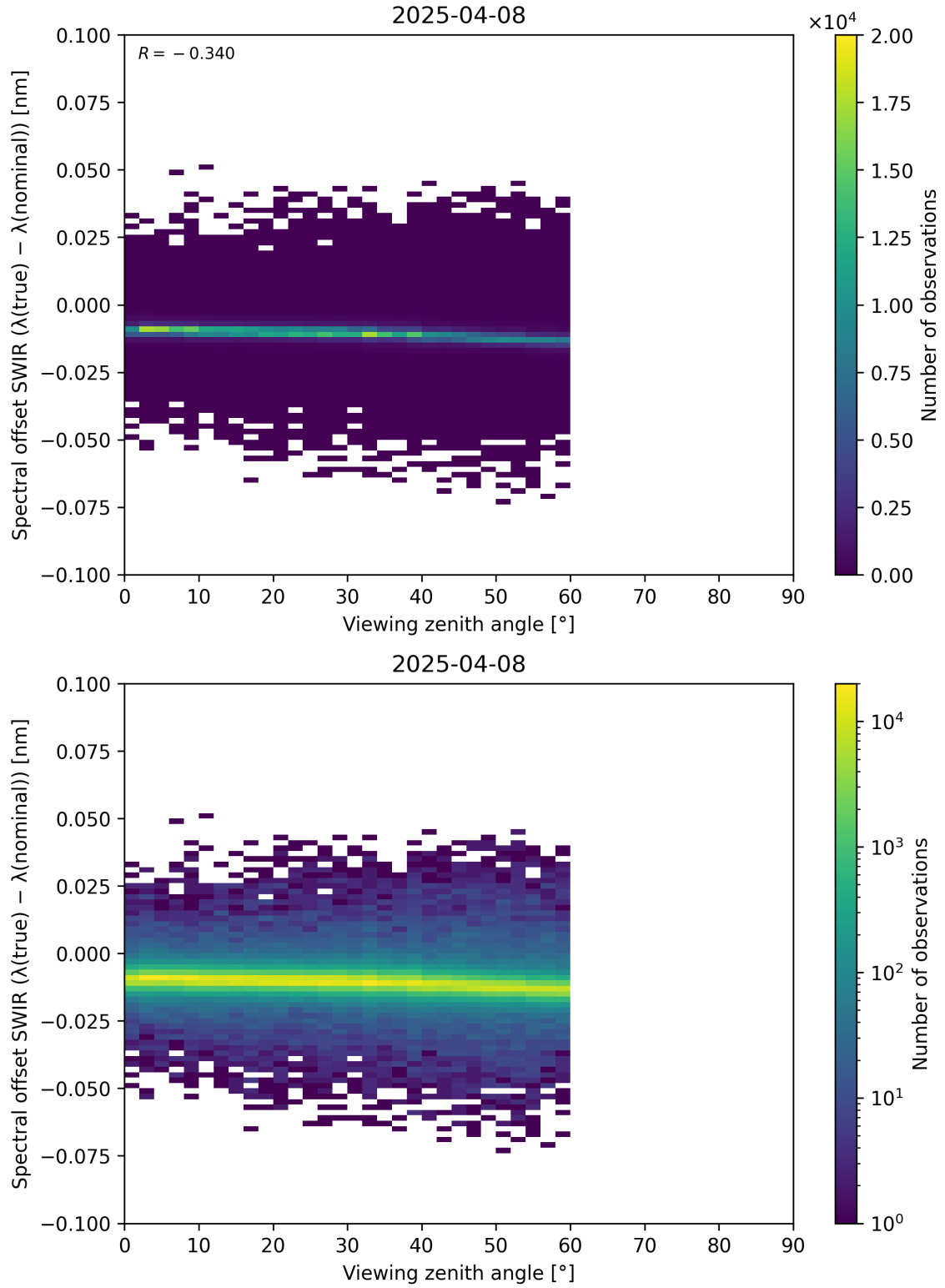
Figure 116: Scatter density plot of “Viewing zenith angle” against “Spectral offset SWIR ( \lambda_{\text{true}} - \lambda_{\text{nominal}} )” for 2025-04-08 to 2025-04-09.
