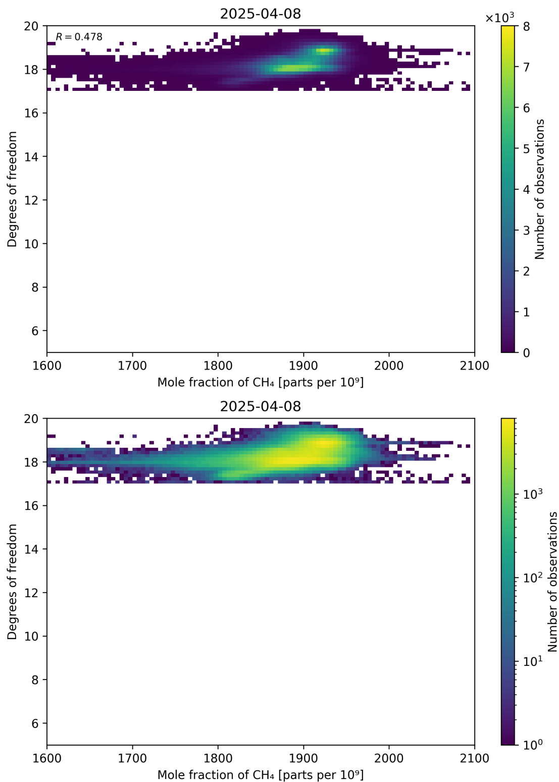
Figure 72: Scatter density plot of “Mole fraction of CH 4 ” against “Degrees of freedom” for 2025-04-08 to 2025-04-09.
