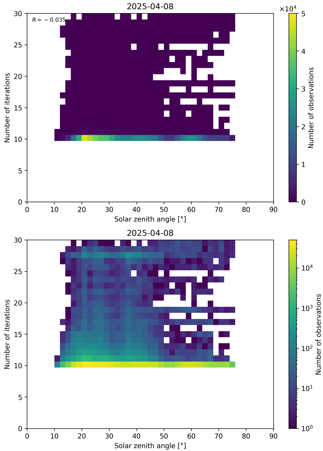
Figure 102: Scatter density plot of “Solar zenith angle” against “Number of iterations” for 2025-04-08 to 2025-04-09.
