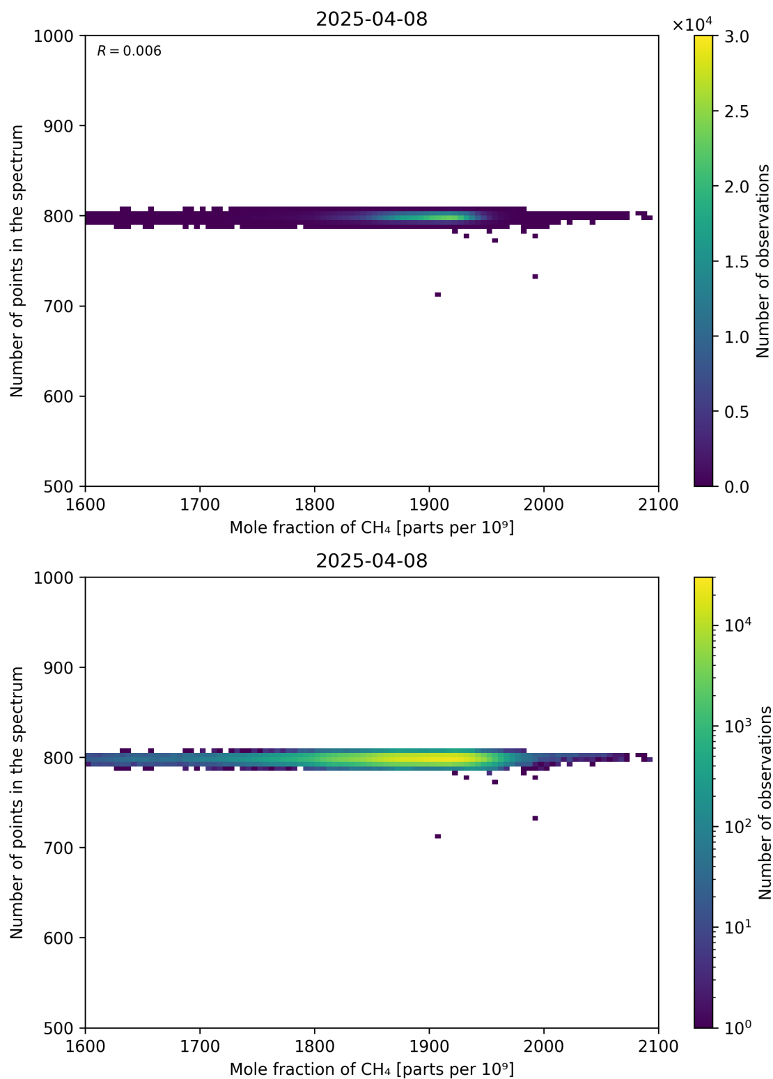
Figure 77: Scatter density plot of “Mole fraction of CH 4 ” against “Number of points in the spectrum” for 2025-04-08 to 2025-04-09.
