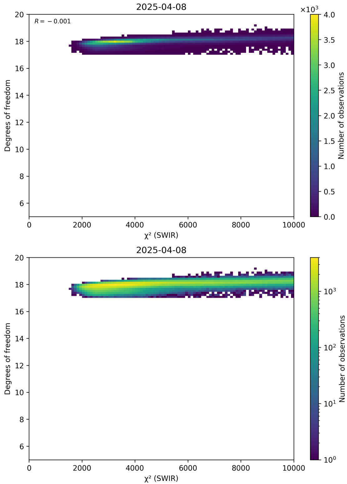
Figure 48: Scatter density plot of “ \chi^2 (SWIR)” against “Degrees of freedom” for 2025-04-08 to 2025-04-09.
