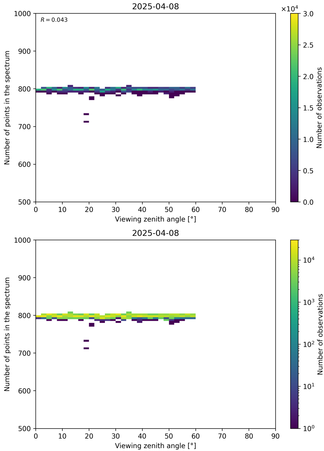
Figure 114: Scatter density plot of “Viewing zenith angle” against “Number of points in the spectrum” for 2025-04-08 to 2025-04-09.
