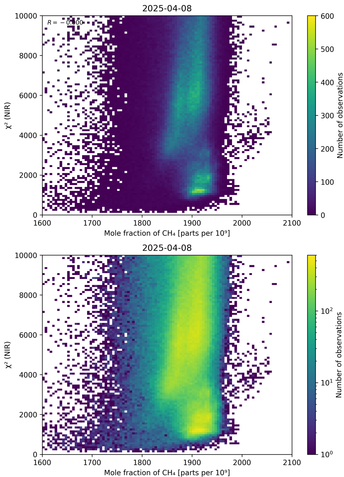
Figure 70: Scatter density plot of “Mole fraction of CH 4 ” against “ \chi^2 (NIR)” for 2025-04-08 to 2025-04-09.
