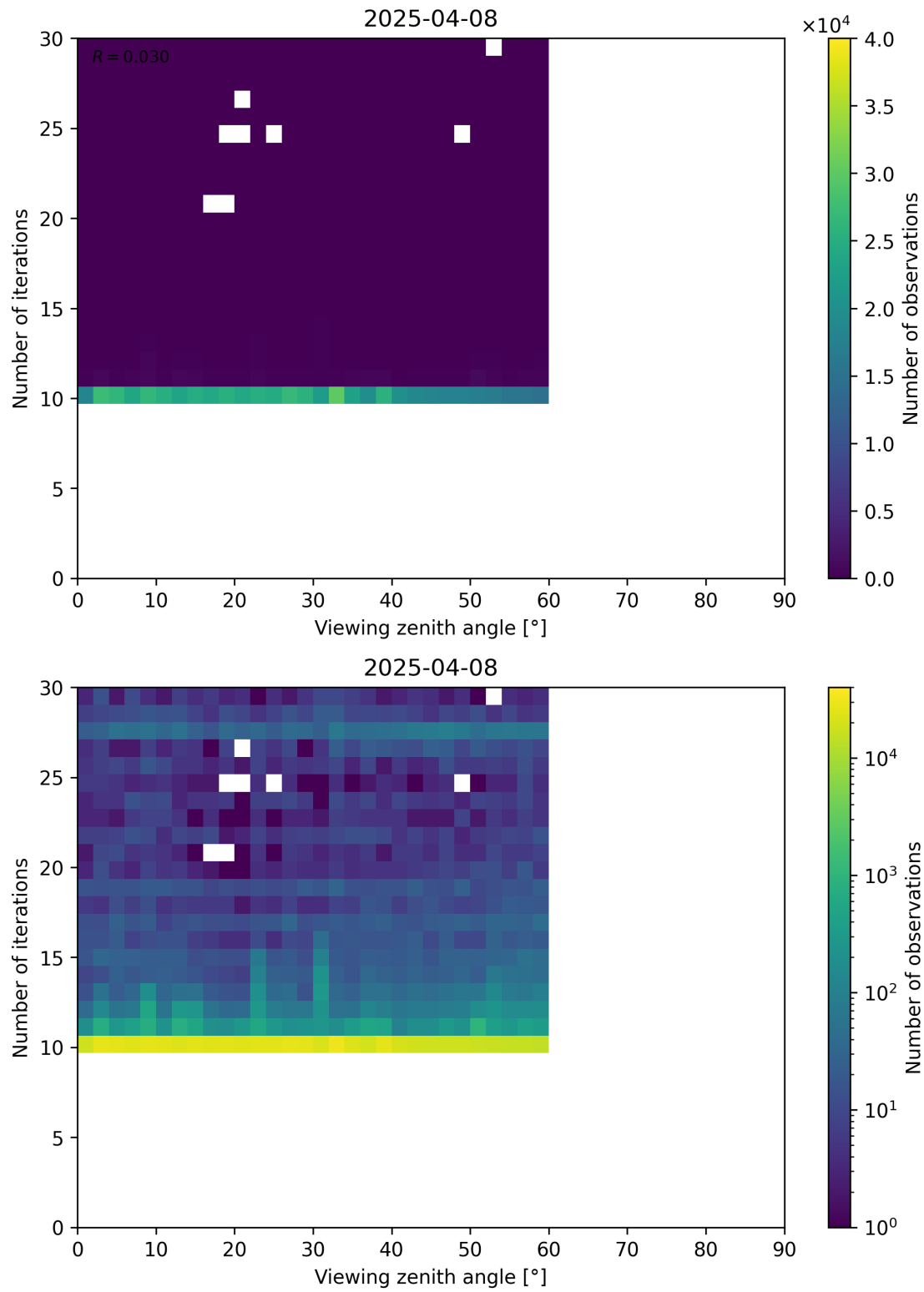
Figure 113: Scatter density plot of “Viewing zenith angle” against “Number of iterations” for 2025-04-08 to 2025-04-09.
