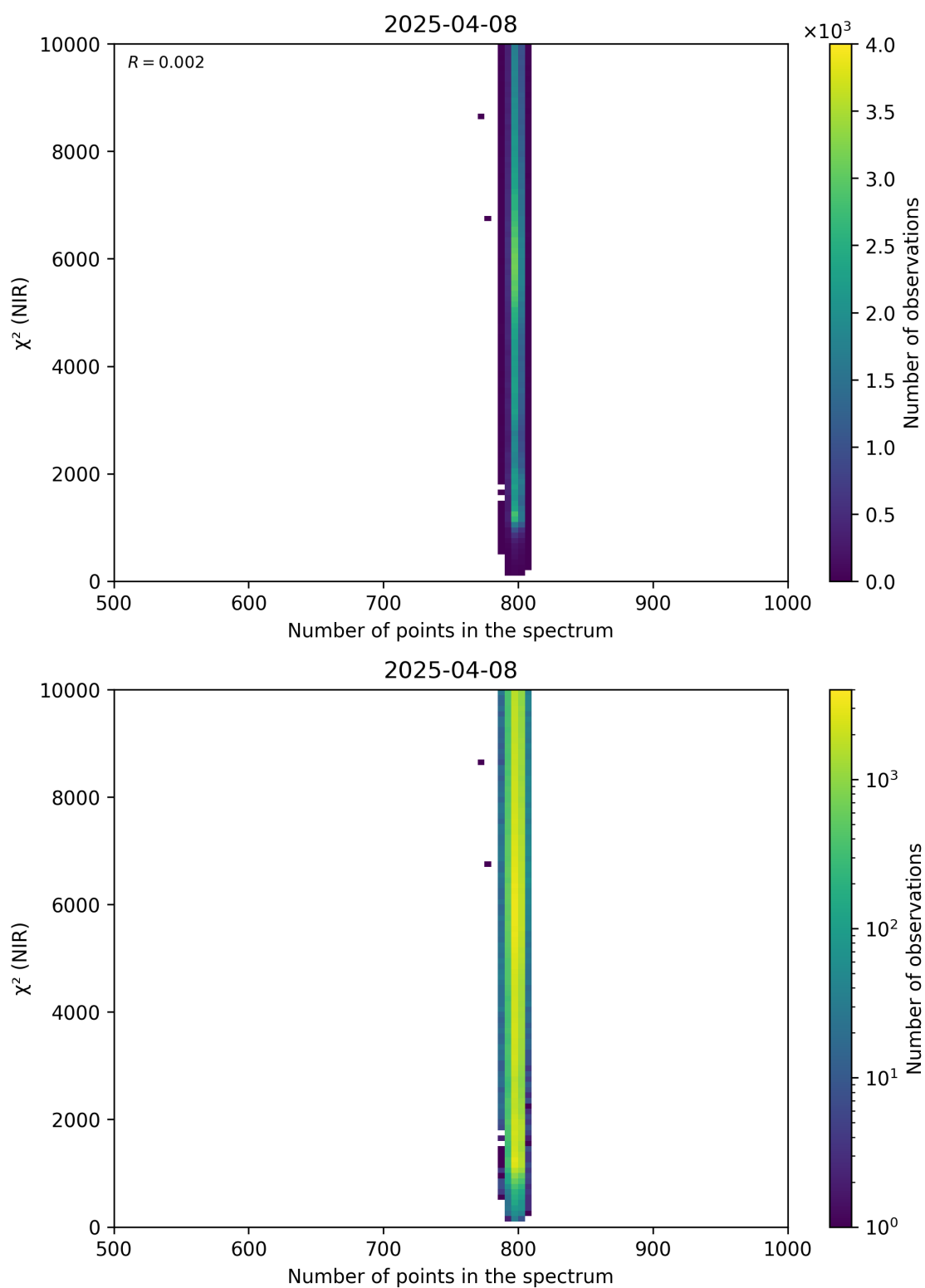
Figure 88: Scatter density plot of “Number of points in the spectrum” against “ \chi^2 (NIR)” for 2025-04-08 to 2025-04-09.
