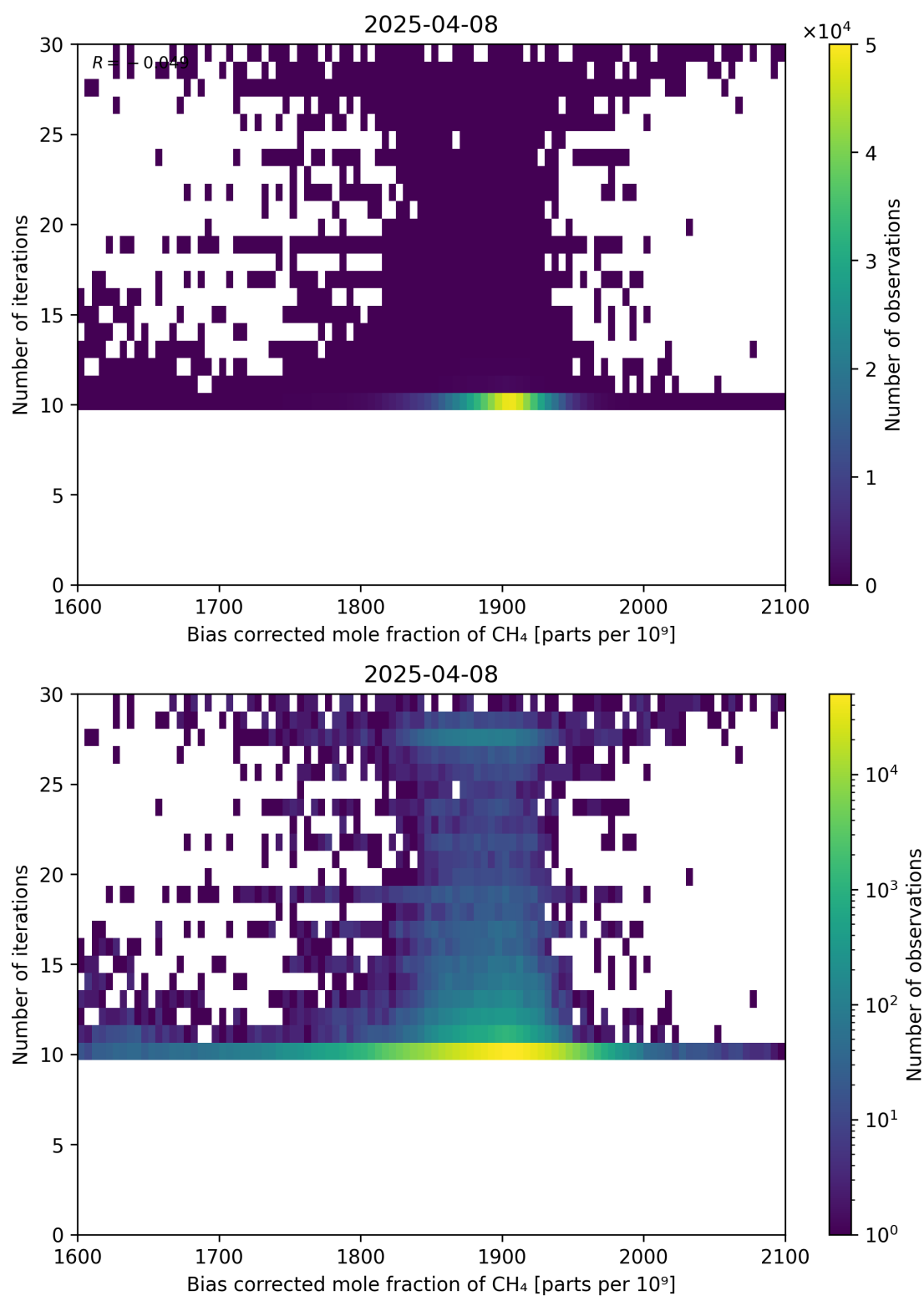
Figure 67: Scatter density plot of “Bias corrected mole fraction of \text{CH}_4 ” against “Number of iterations” for 2025-04-08 to 2025-04-09.
