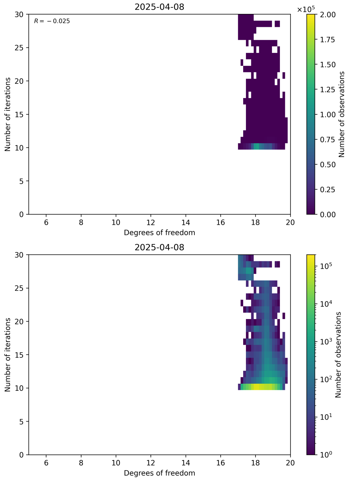
Figure 52: Scatter density plot of “Degrees of freedom” against “Number of iterations” for 2025-04-08 to 2025-04-09.
