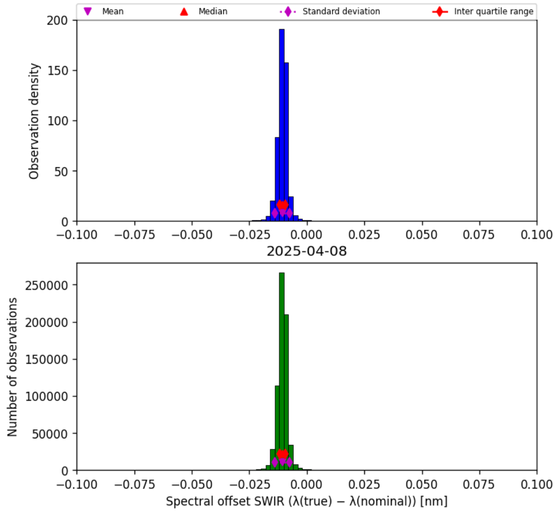
Figure 27: Histogram of “Spectral offset SWIR ( \lambda_{\text{true}} - \lambda_{\text{nominal}} )” for 2025-04-08 to 2025-04-09
