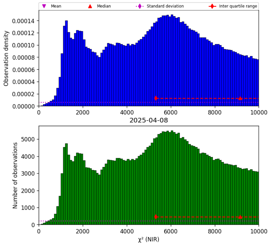
Figure 29: Histogram of “ \chi^2 (NIR)” for 2025-04-08 to 2025-04-09
