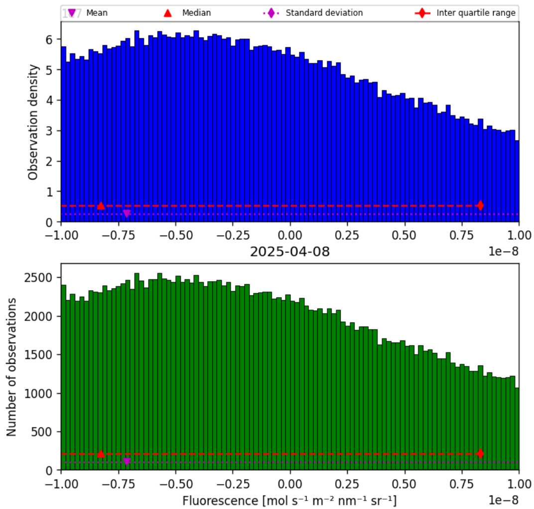
Figure 32: Histogram of “Fluorescence” for 2025-04-08 to 2025-04-09
