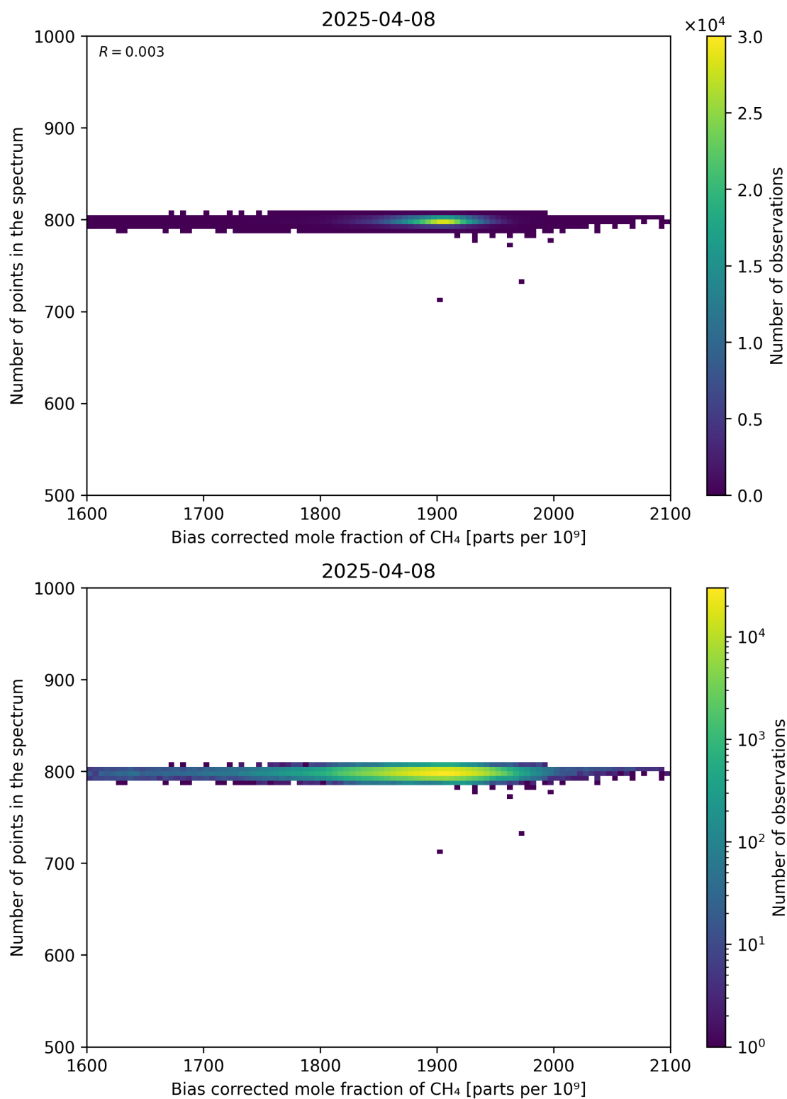
Figure 68: Scatter density plot of “Bias corrected mole fraction of CH 4 ” against “Number of points in the spectrum” for 2025-04-08 to 2025-04-09.
