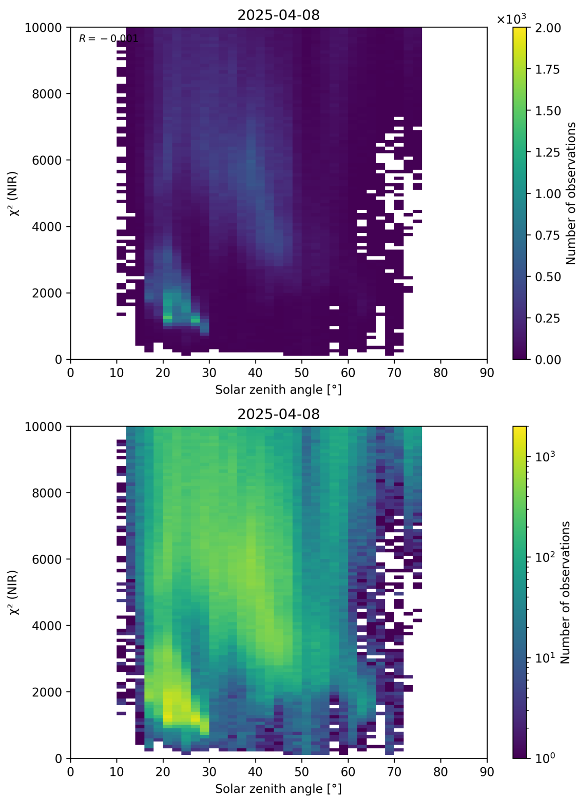
Figure 94: Scatter density plot of “Solar zenith angle” against “ \chi^2 (NIR)” for 2025-04-08 to 2025-04-09.
