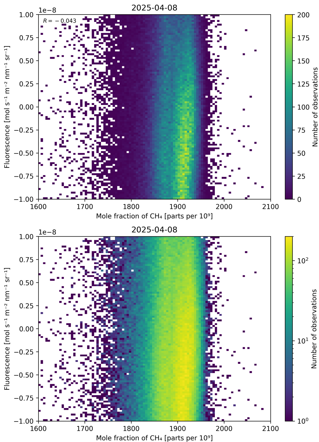
Figure 73: Scatter density plot of “Mole fraction of \text{CH}_4 ” against “Fluorescence” for 2025-04-08 to 2025-04-09.
