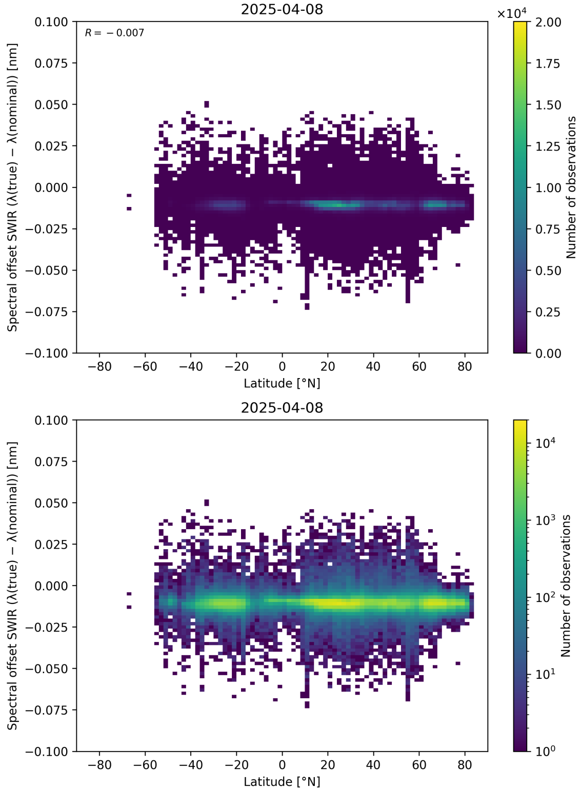
Figure 62: Scatter density plot of “Latitude” against “Spectral offset SWIR ( \lambda_{\text{true}} - \lambda_{\text{nominal}} )” for 2025-04-08 to 2025-04-09.
