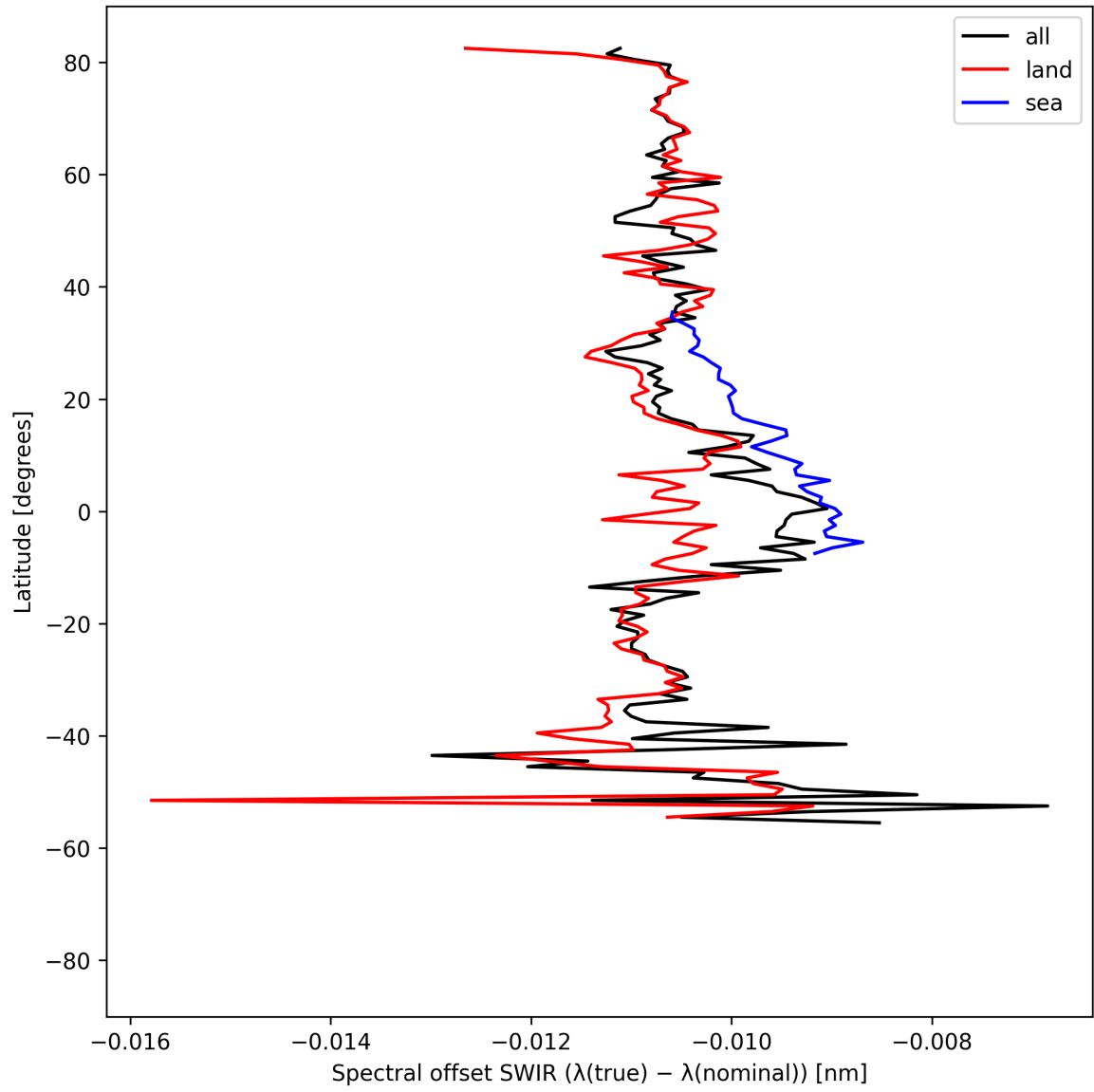
Figure 16: Zonal average of “Spectral offset SWIR ( \lambda_{\text{true}} - \lambda_{\text{nominal}} )” for 2025-04-08 to 2025-04-09.
