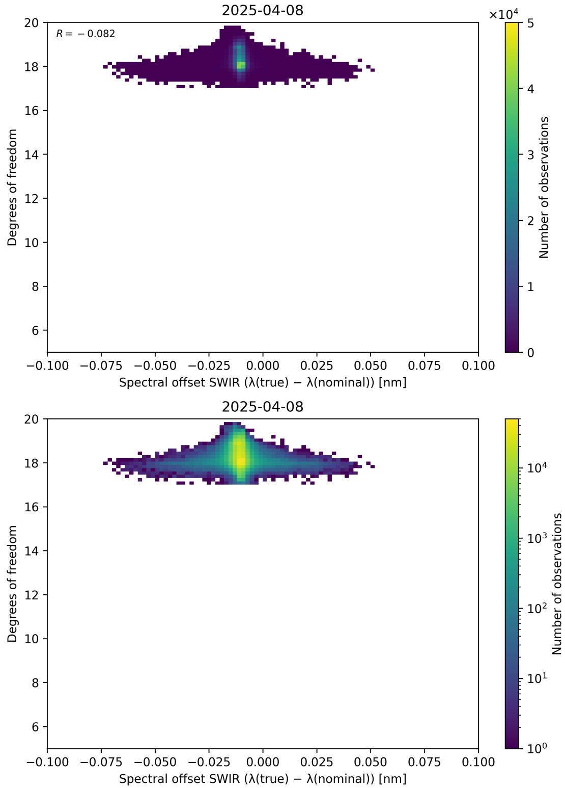
Figure 119: Scatter density plot of “Spectral offset SWIR ( \lambda_{\text{true}} - \lambda_{\text{nominal}} )” against “Degrees of freedom” for 2025-04-08 to 2025-04-09.
