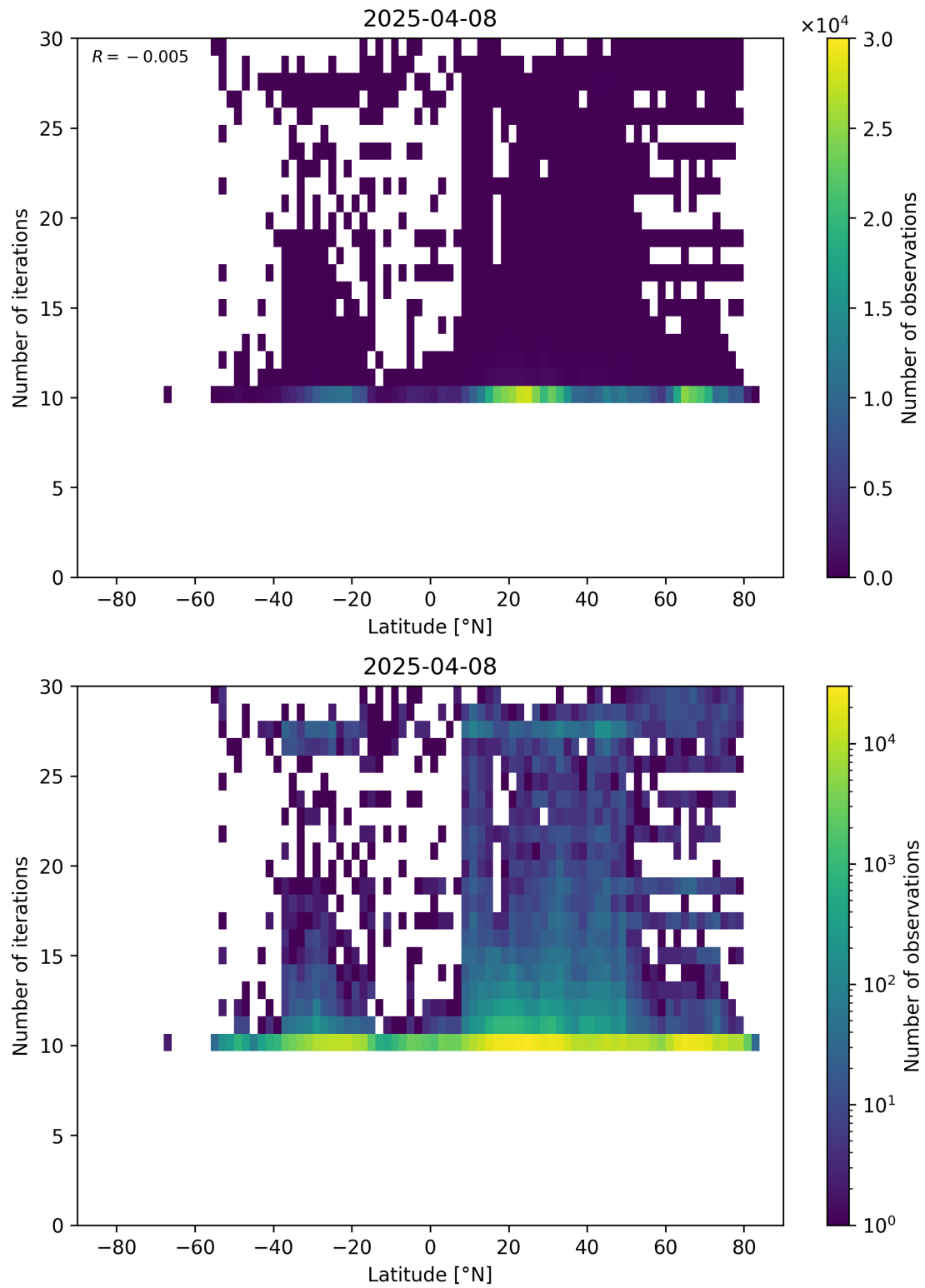
Figure 60: Scatter density plot of “Latitude” against “Number of iterations” for 2025-04-08 to 2025-04-09.
