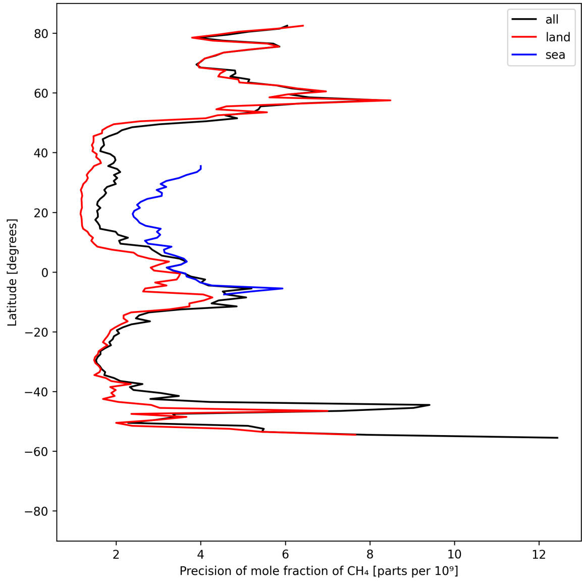
Figure 13: Zonal average of “Precision of mole fraction of CH 4 ” for 2025-04-08 to 2025-04-09.
