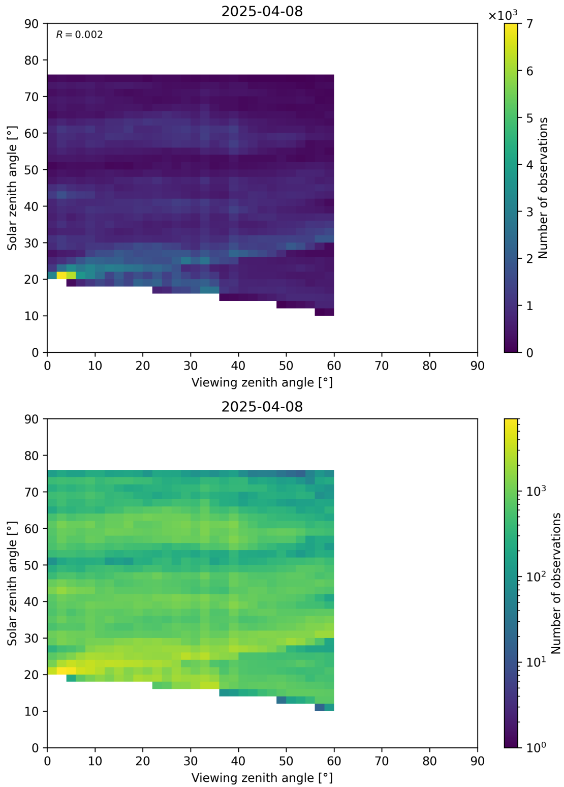
Figure 115: Scatter density plot of “Viewing zenith angle” against “Solar zenith angle” for 2025-04-08 to 2025-04-09.
