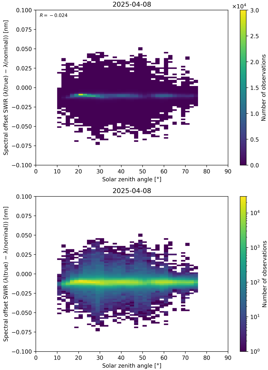
Figure 104: Scatter density plot of “Solar zenith angle” against “Spectral offset SWIR ( \lambda_{\text{true}} - \lambda_{\text{nominal}} )” for 2025-04-08 to 2025-04-09.
