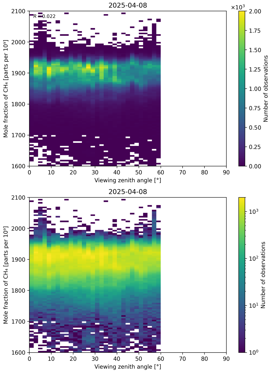
Figure 110: Scatter density plot of “Viewing zenith angle” against “Mole fraction of CH 4 ” for 2025-04-08 to 2025-04-09.
