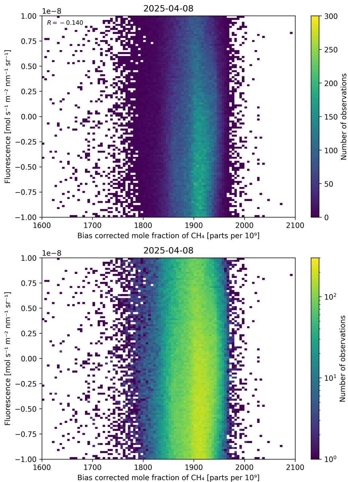
Figure 66: Scatter density plot of “Bias corrected mole fraction of \text{CH}_4 ” against “Fluorescence” for 2025-04-08 to 2025-04-09.
