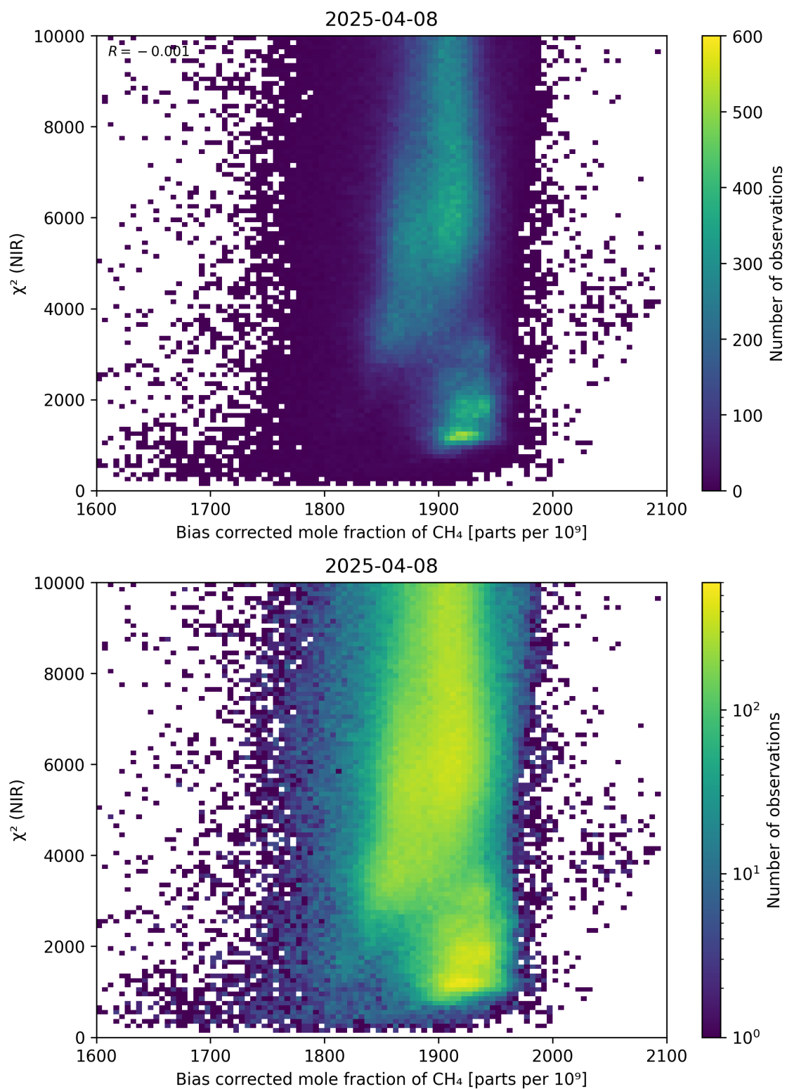
Figure 63: Scatter density plot of “Bias corrected mole fraction of CH 4 ” against “ \chi^2 (NIR)” for 2025-04-08 to 2025-04-09.
