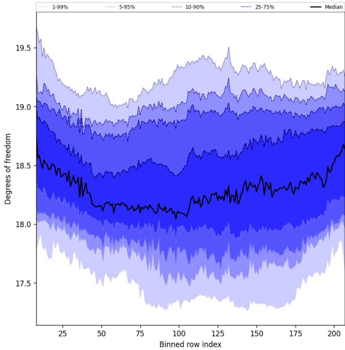
Figure 41: Along track statistics of “Degrees of freedom” for 2025-04-08 to 2025-04-09
