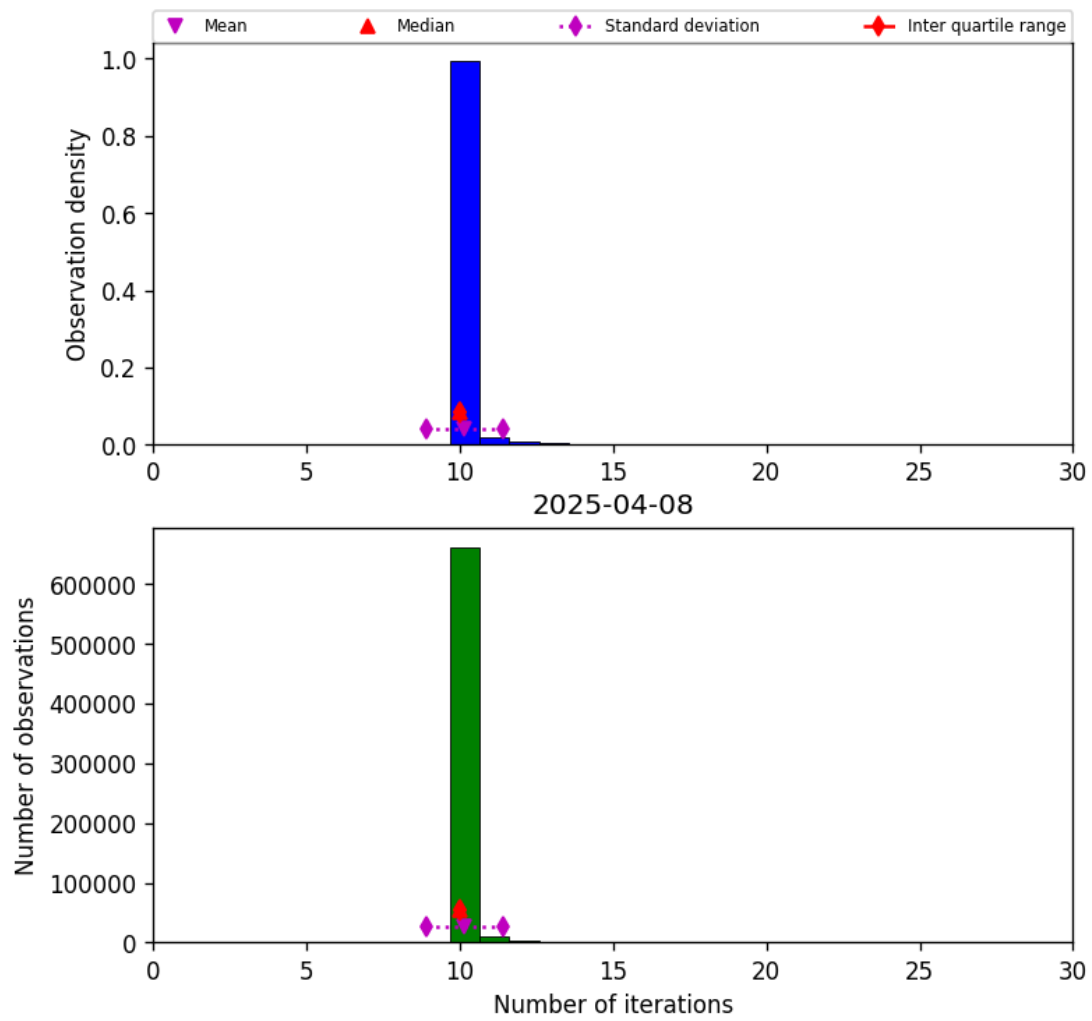
Figure 31: Histogram of “Number of iterations” for 2025-04-08 to 2025-04-09
