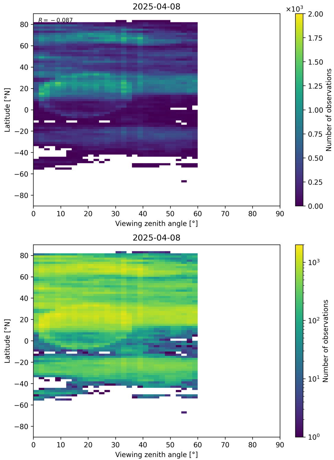
Figure 109: Scatter density plot of “Viewing zenith angle” against “Latitude” for 2025-04-08 to 2025-04-09.
