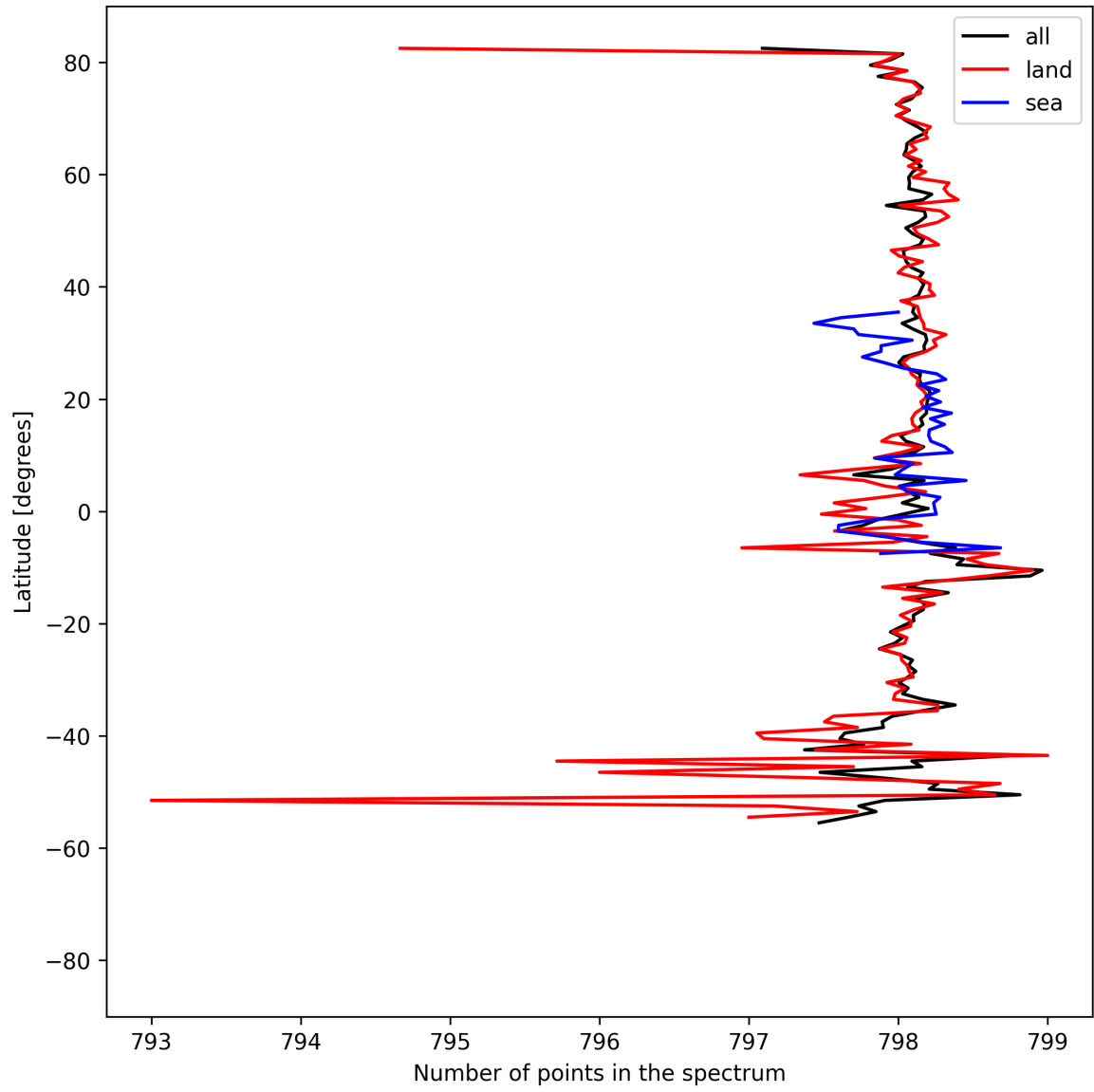
Figure 15: Zonal average of “Number of points in the spectrum” for 2025-04-08 to 2025-04-09.
