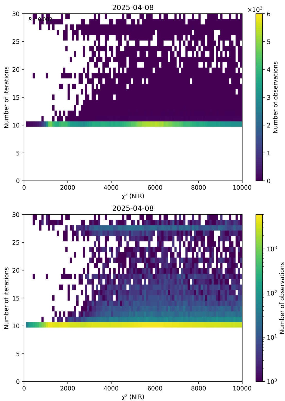
Figure 46: Scatter density plot of “ \chi^2 (NIR)” against “Number of iterations” for 2025-04-08 to 2025-04-09.
