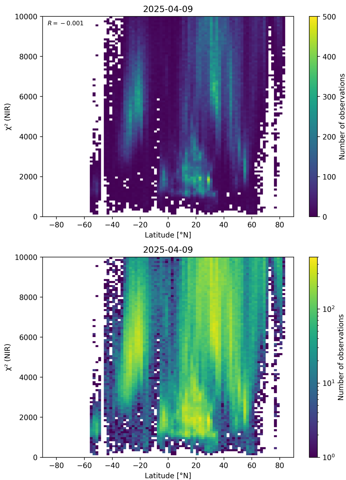
Figure 53: Scatter density plot of “Latitude” against “ \chi^2 (NIR)” for 2025-04-08 to 2025-04-10.
