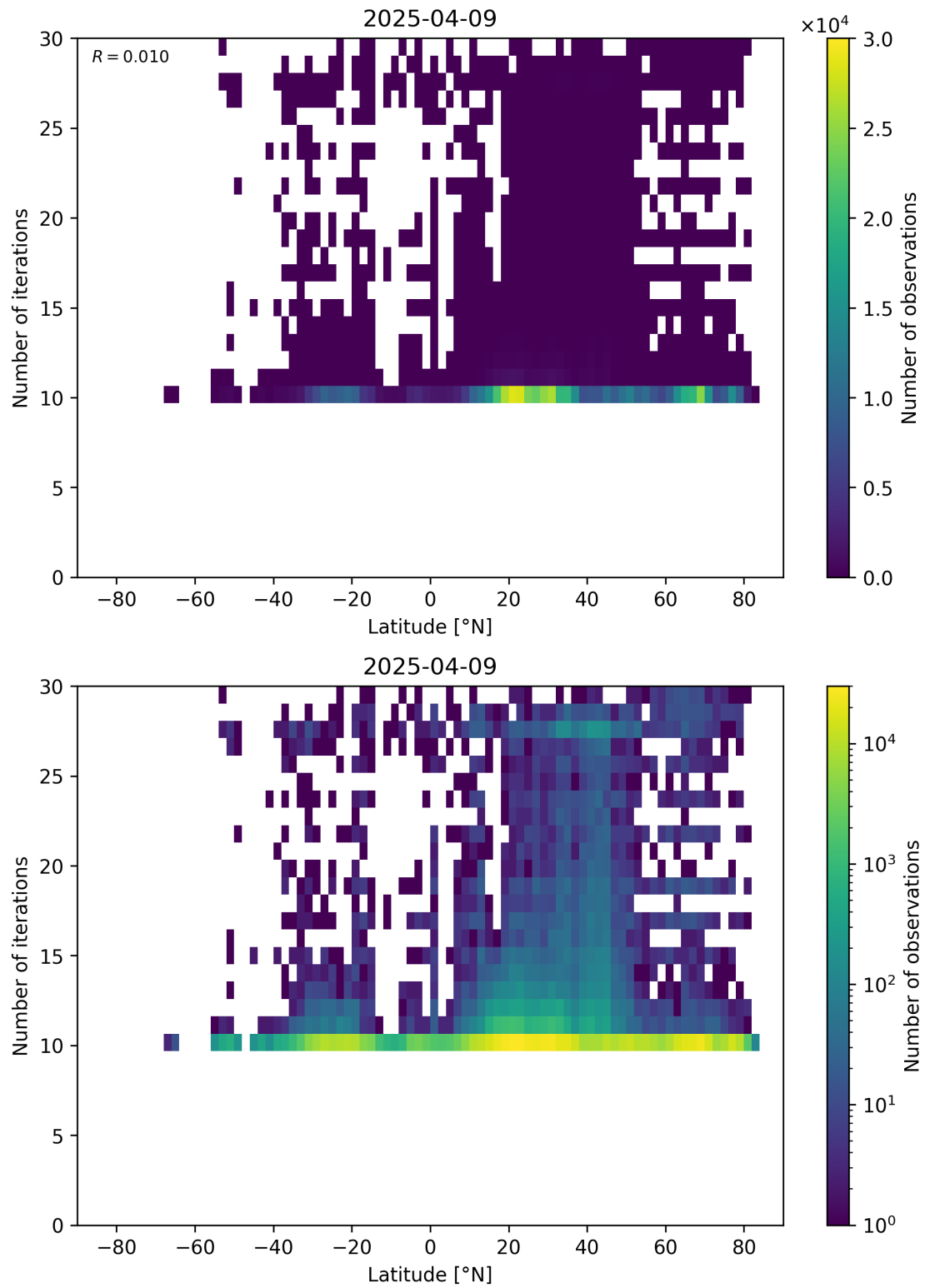
Figure 60: Scatter density plot of “Latitude” against “Number of iterations” for 2025-04-08 to 2025-04-10.
