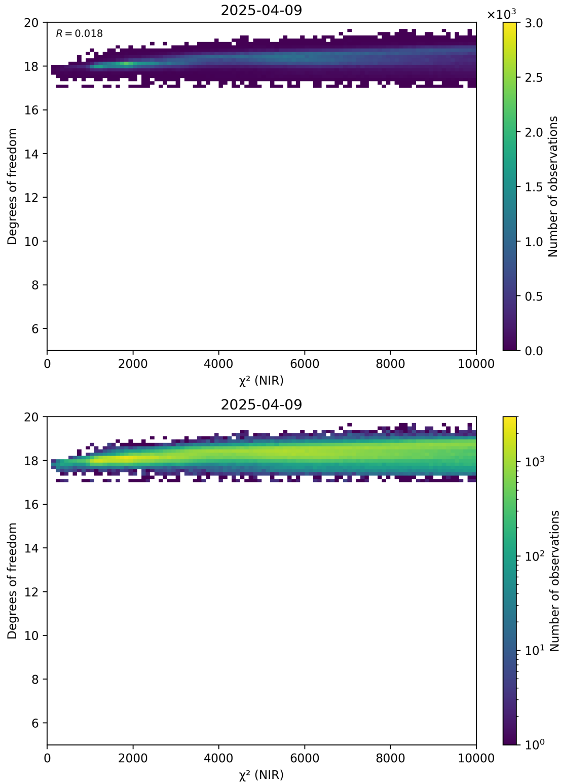
Figure 44: Scatter density plot of “ \chi^2 (NIR)” against “Degrees of freedom” for 2025-04-08 to 2025-04-10.
