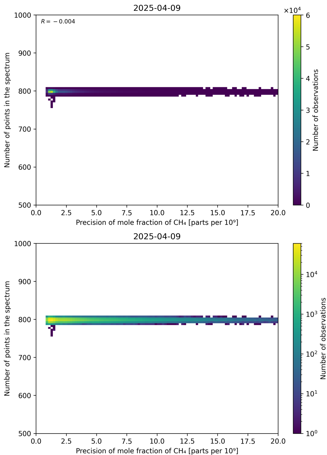
Figure 84: Scatter density plot of “Precision of mole fraction of CH 4 ” against “Number of points in the spectrum” for 2025-04-08 to 2025-04-10.
