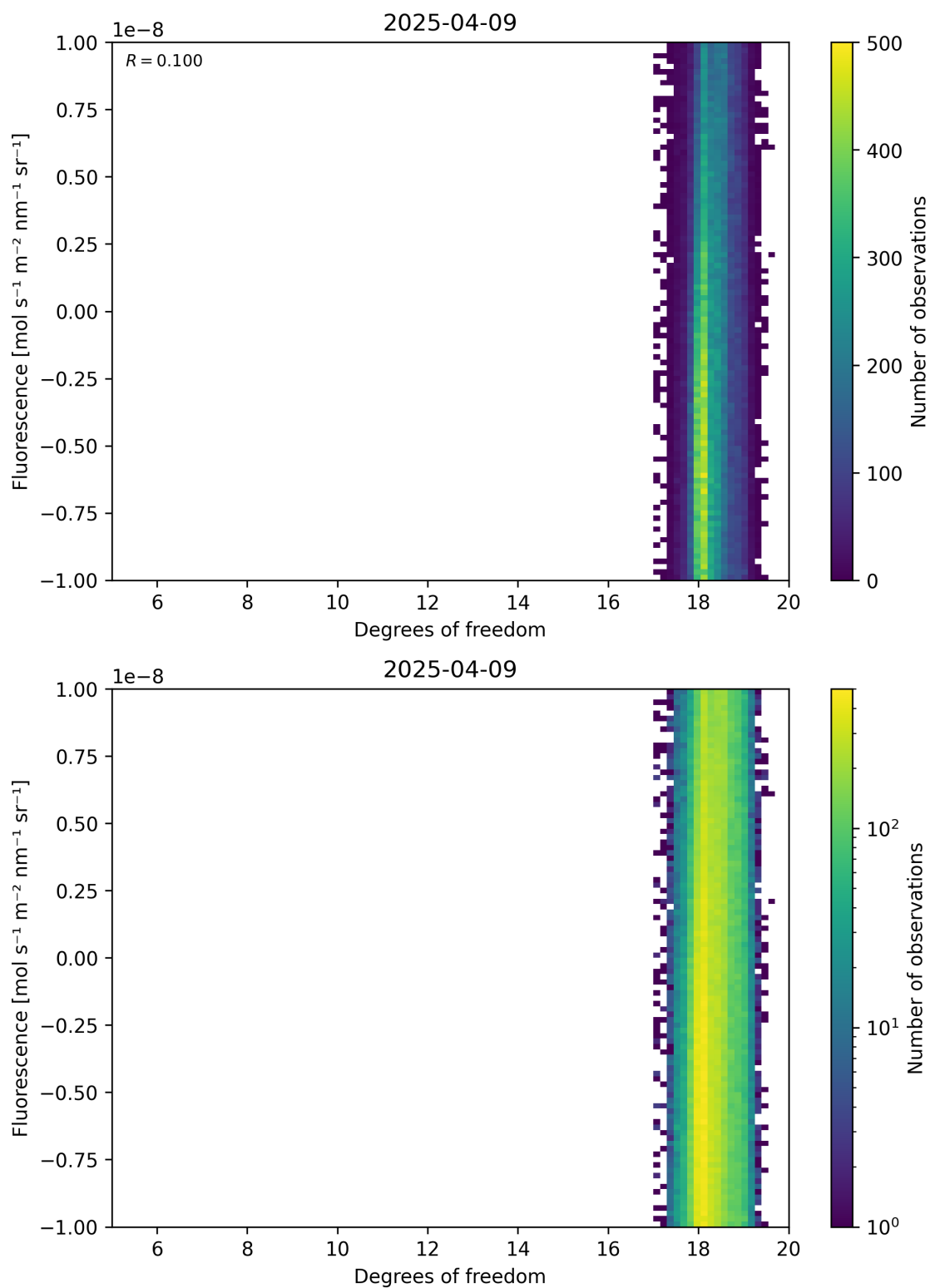
Figure 51: Scatter density plot of “Degrees of freedom” against “Fluorescence” for 2025-04-08 to 2025-04-10.
