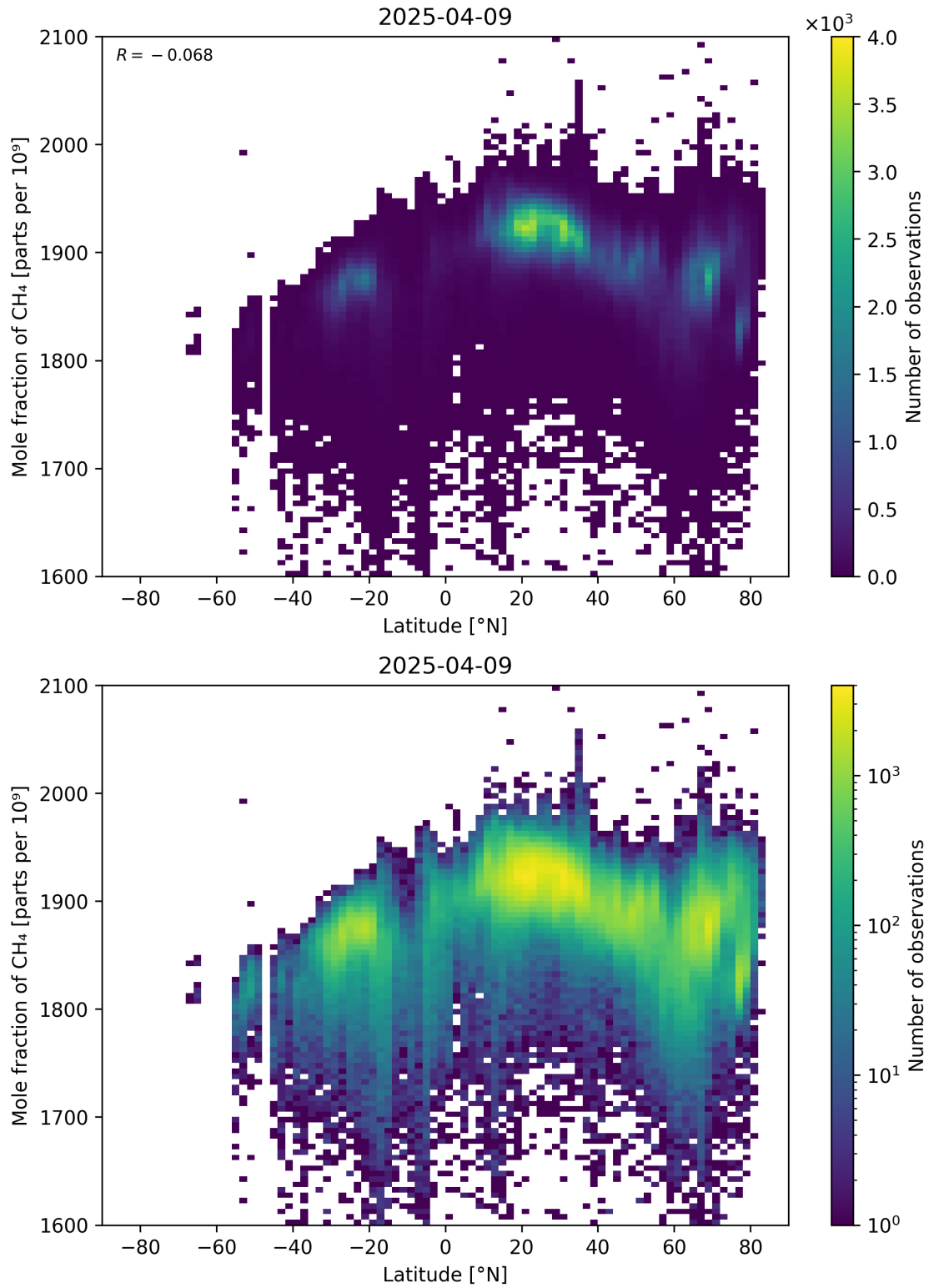
Figure 57: Scatter density plot of “Latitude” against “Mole fraction of CH 4 ” for 2025-04-08 to 2025-04-10.
