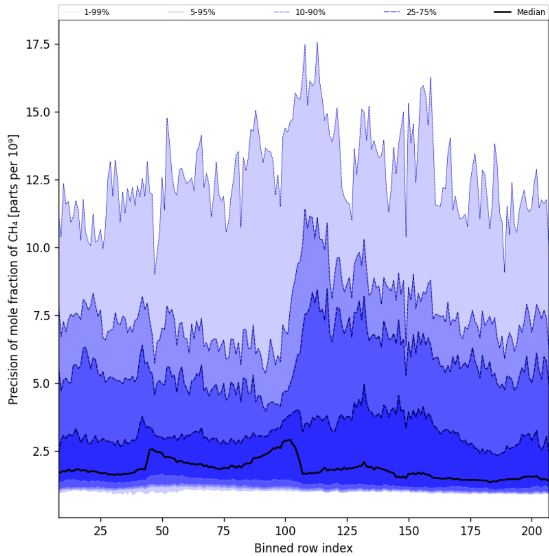
Figure 35: Along track statistics of “Precision of mole fraction of CH 4 ” for 2025-04-08 to 2025-04-10
