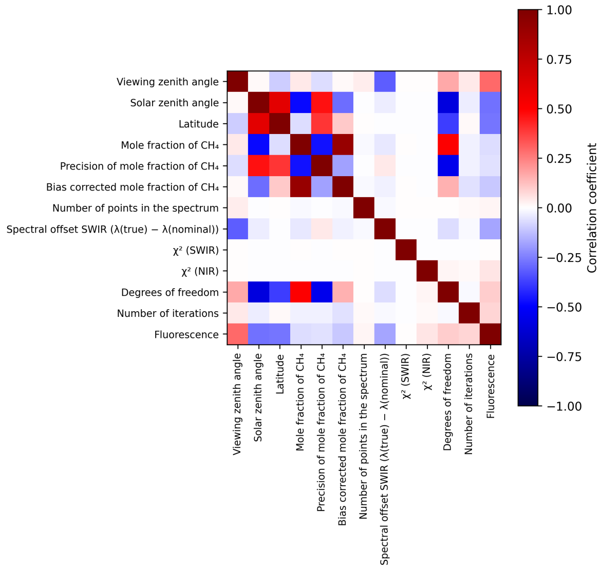
Figure 2: Map of correlation matrix for 2025-04-08 to 2025-04-10.
