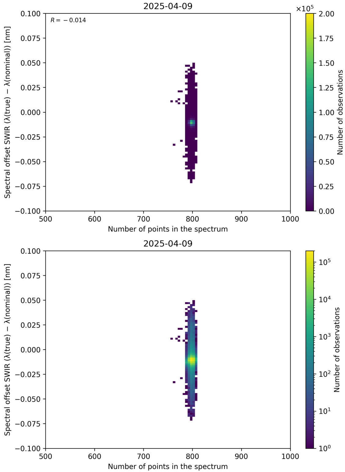
Figure 93: Scatter density plot of “Number of points in the spectrum” against “Spectral offset SWIR ( \lambda_{\text{true}} - \lambda_{\text{nominal}} )” for 2025-04-08 to 2025-04-10.
