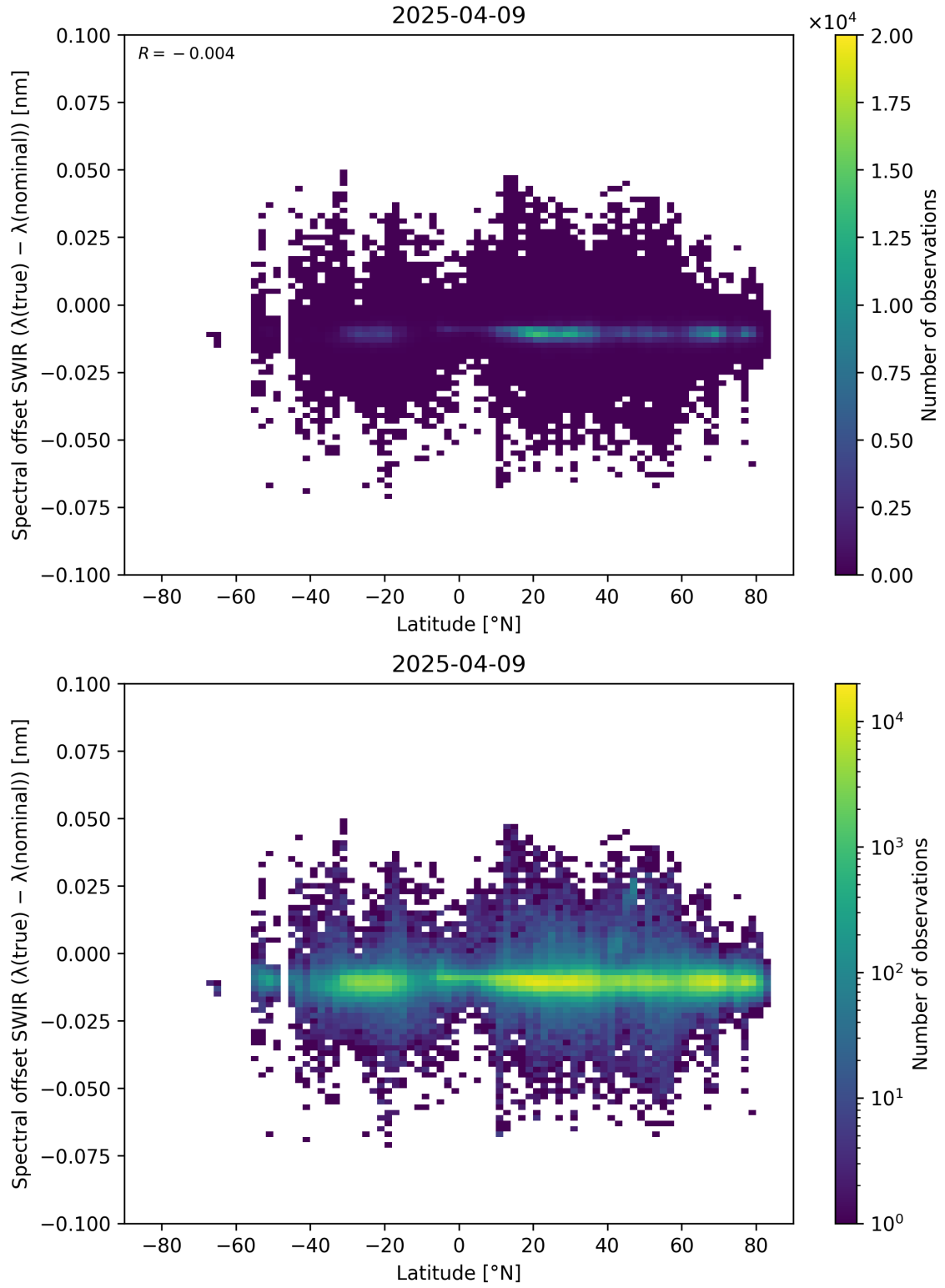
Figure 62: Scatter density plot of “Latitude” against “Spectral offset SWIR ( \lambda_{\text{true}} - \lambda_{\text{nominal}} )” for 2025-04-08 to 2025-04-10.
