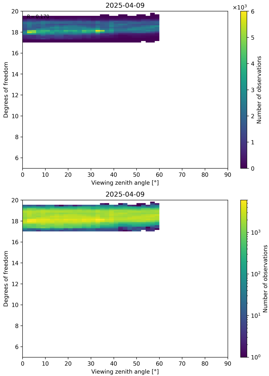
Figure 107: Scatter density plot of “Viewing zenith angle” against “Degrees of freedom” for 2025-04-08 to 2025-04-10.
