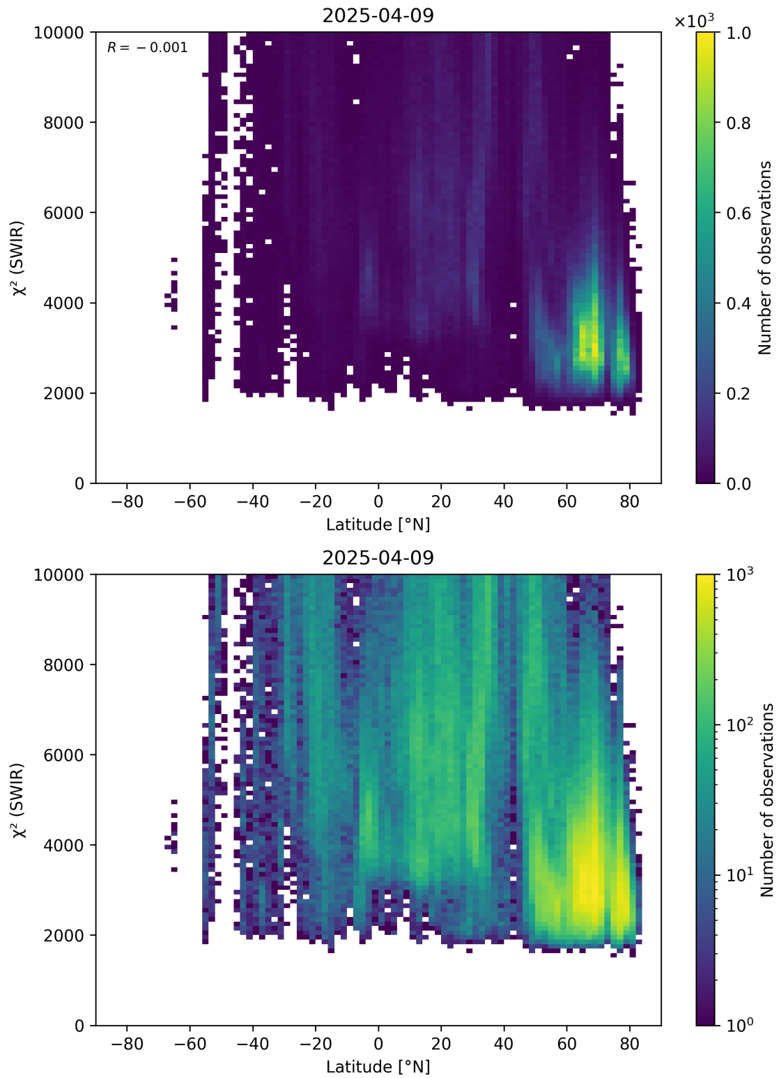
Figure 54: Scatter density plot of “Latitude” against “ \chi^2 (SWIR)” for 2025-04-08 to 2025-04-10.
