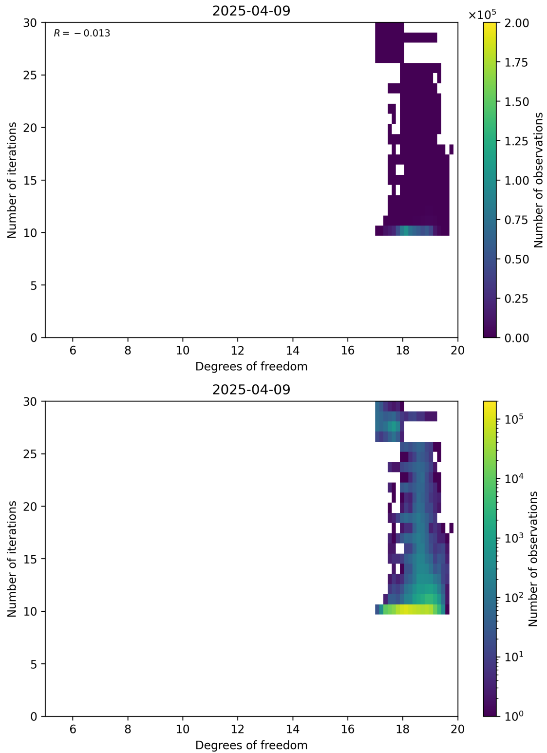
Figure 52: Scatter density plot of “Degrees of freedom” against “Number of iterations” for 2025-04-08 to 2025-04-10.
