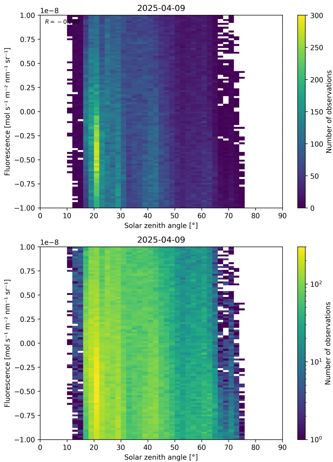
Figure 97: Scatter density plot of “Solar zenith angle” against “Fluorescence” for 2025-04-08 to 2025-04-10.
