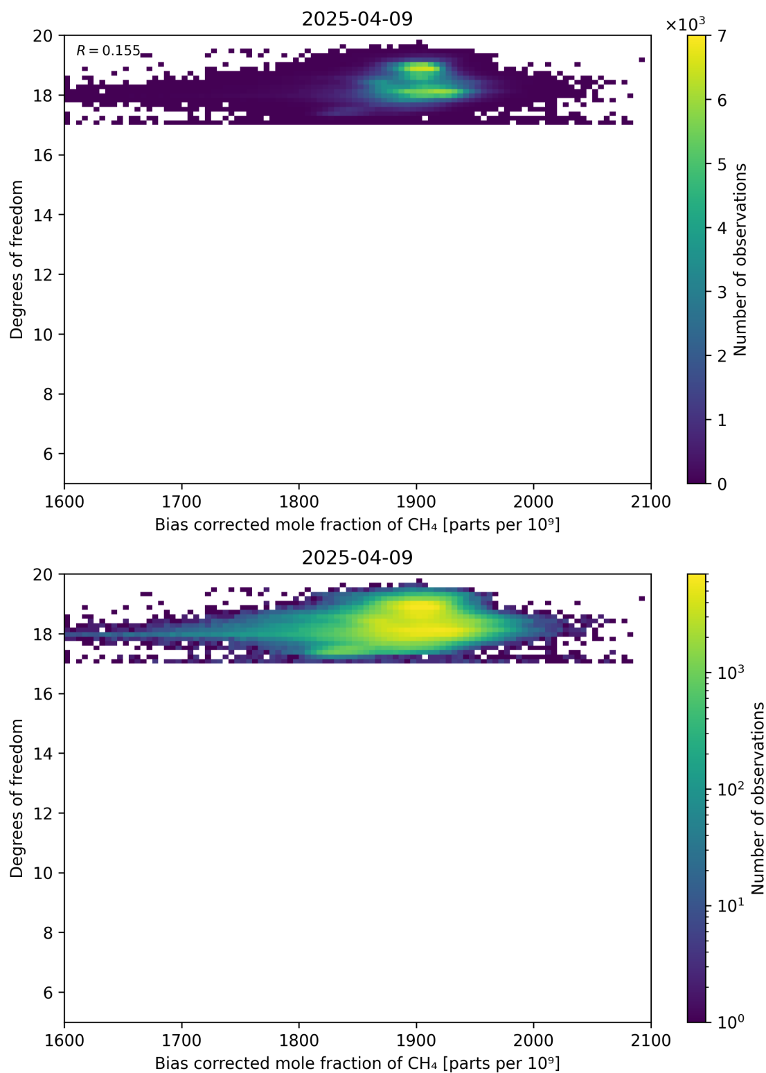
Figure 65: Scatter density plot of “Bias corrected mole fraction of CH 4 ” against “Degrees of freedom” for 2025-04-08 to 2025-04-10.
