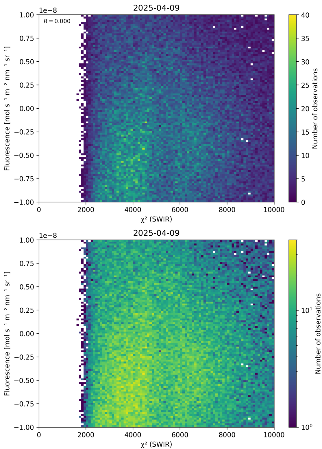
Figure 49: Scatter density plot of “ \chi^2 (SWIR)” against “Fluorescence” for 2025-04-08 to 2025-04-10.
