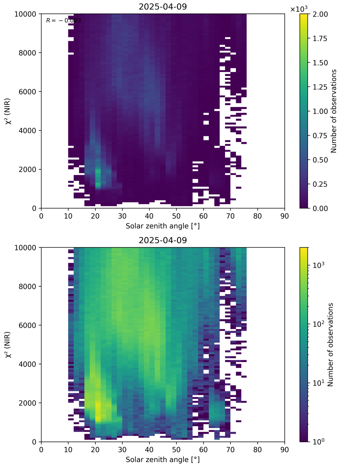
Figure 94: Scatter density plot of “Solar zenith angle” against “ \chi^2 (NIR)” for 2025-04-08 to 2025-04-10.
