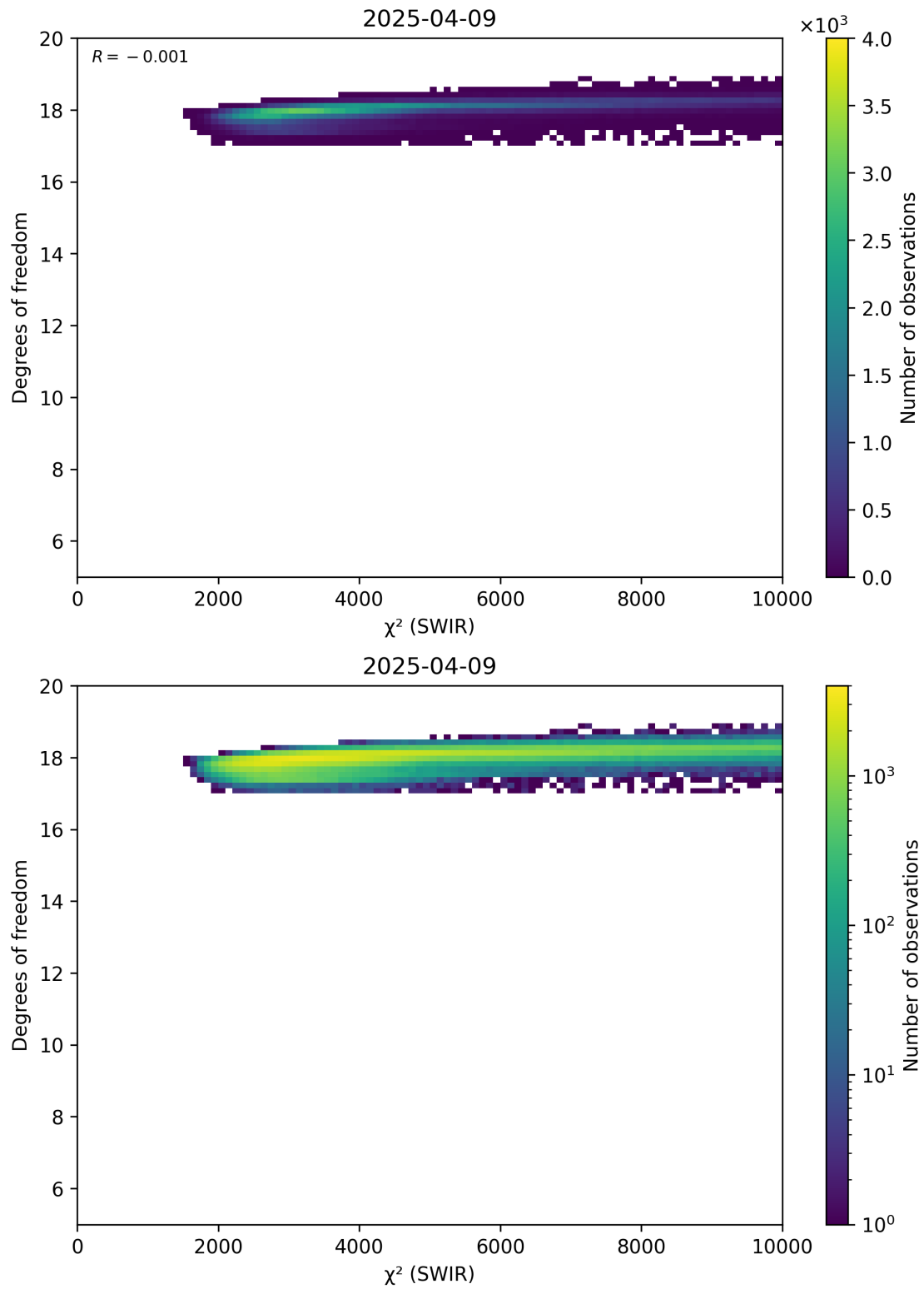
Figure 48: Scatter density plot of “ \chi^2 (SWIR)” against “Degrees of freedom” for 2025-04-08 to 2025-04-10.
