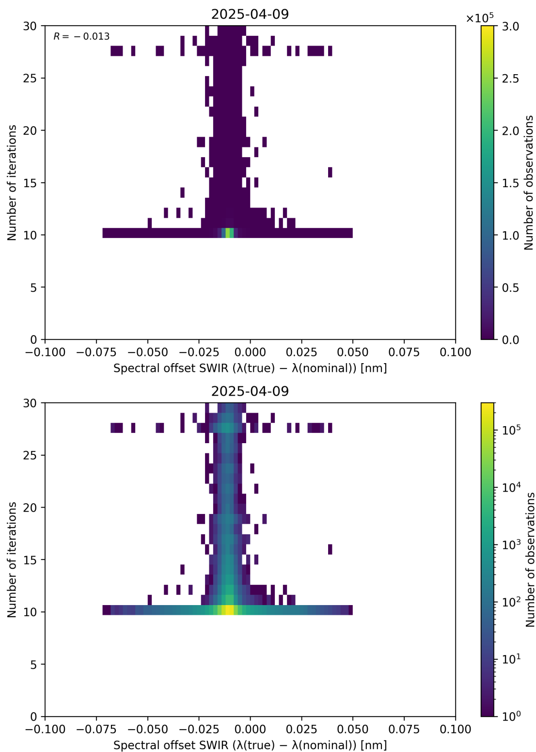
Figure 121: Scatter density plot of “Spectral offset SWIR ( \lambda_{\text{true}} - \lambda_{\text{nominal}} )” against “Number of iterations” for 2025-04-08 to 2025-04-10.
