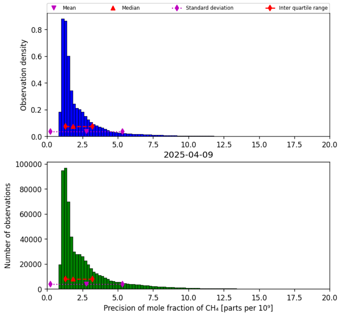
Figure 24: Histogram of “Precision of mole fraction of CH 4 ” for 2025-04-08 to 2025-04-10
