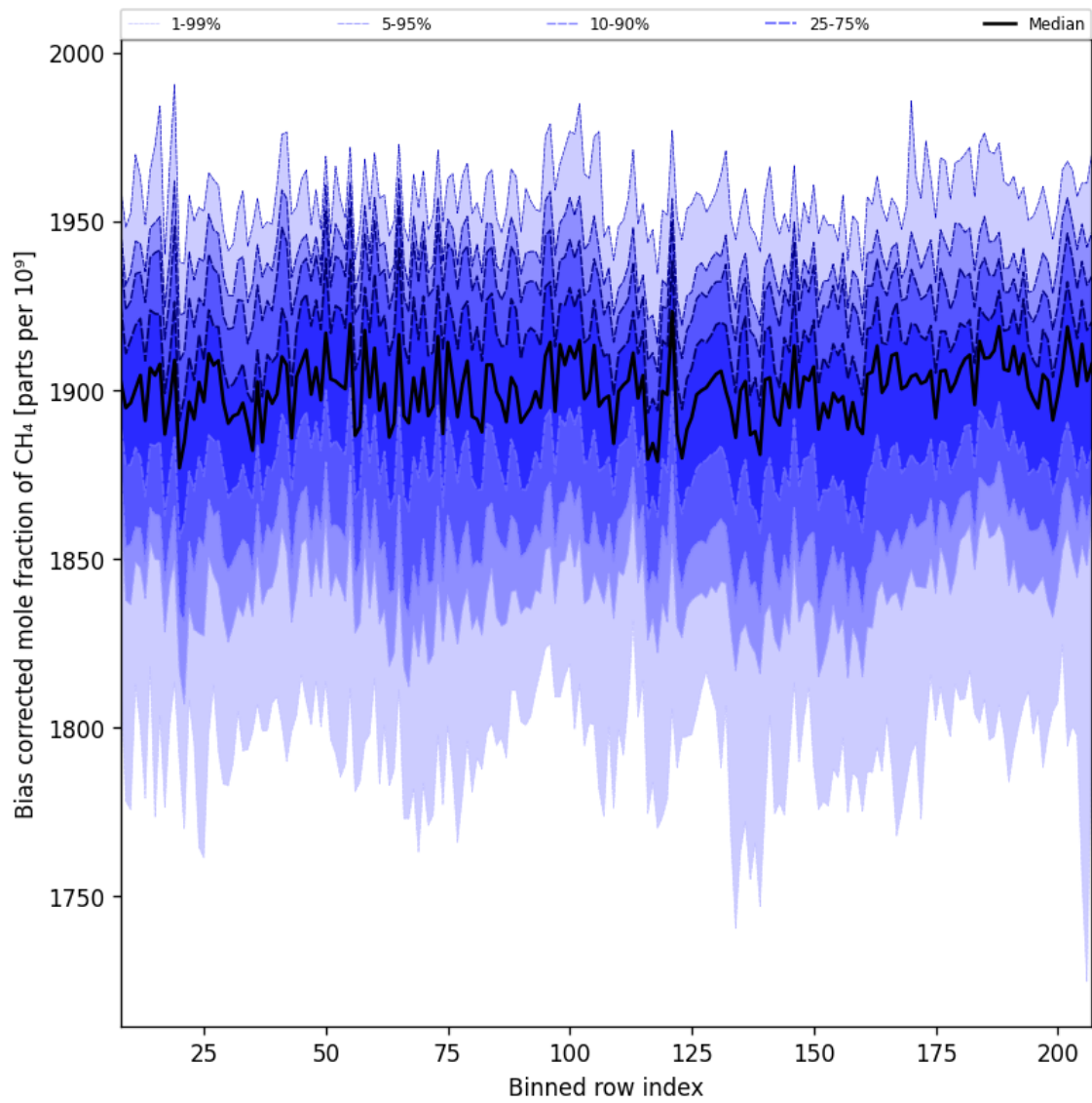
Figure 36: Along track statistics of “Bias corrected mole fraction of CH 4 ” for 2025-04-08 to 2025-04-10
