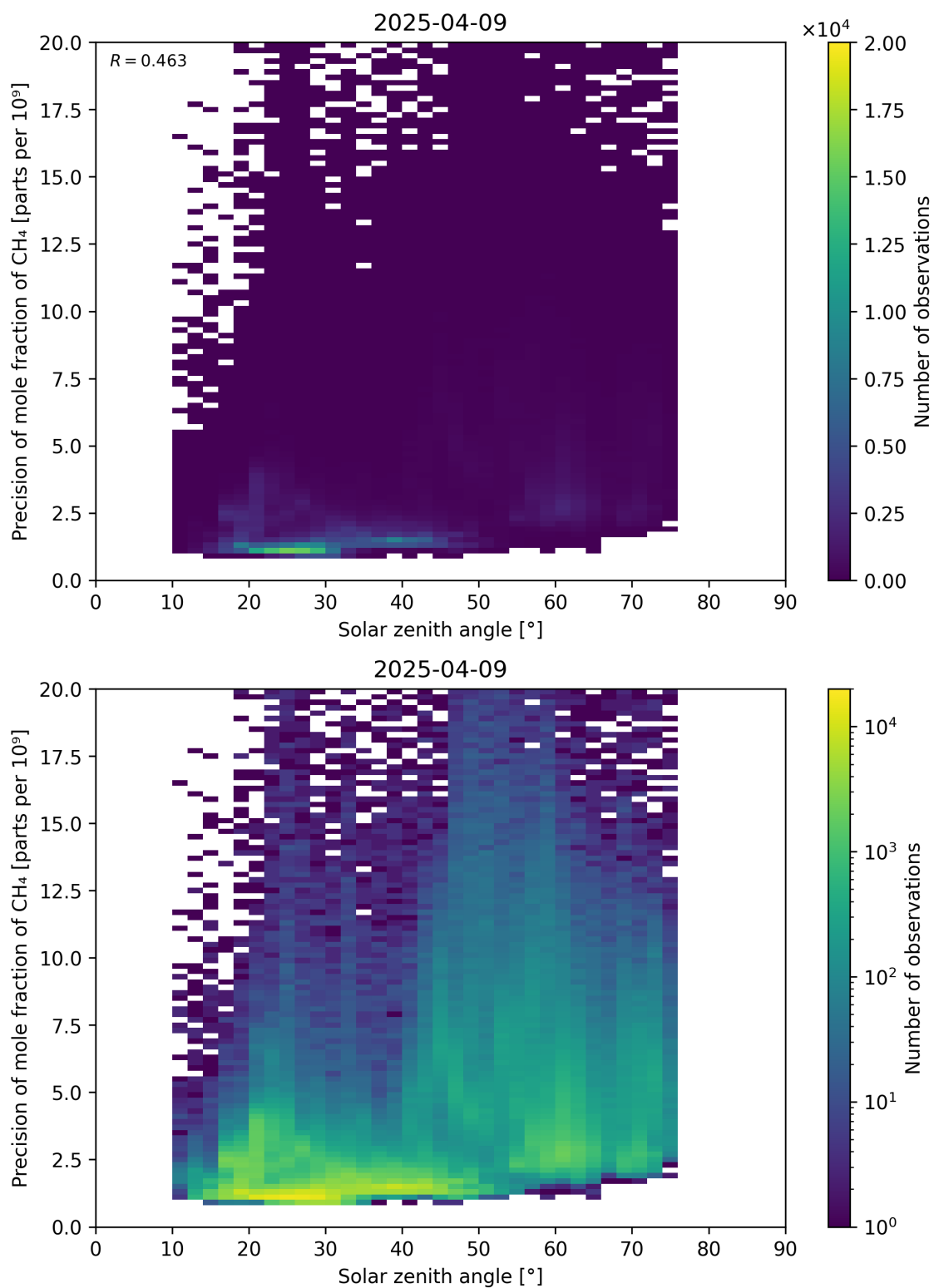
Figure 101: Scatter density plot of “Solar zenith angle” against “Precision of mole fraction of CH 4 ” for 2025-04-08 to 2025-04-10.
