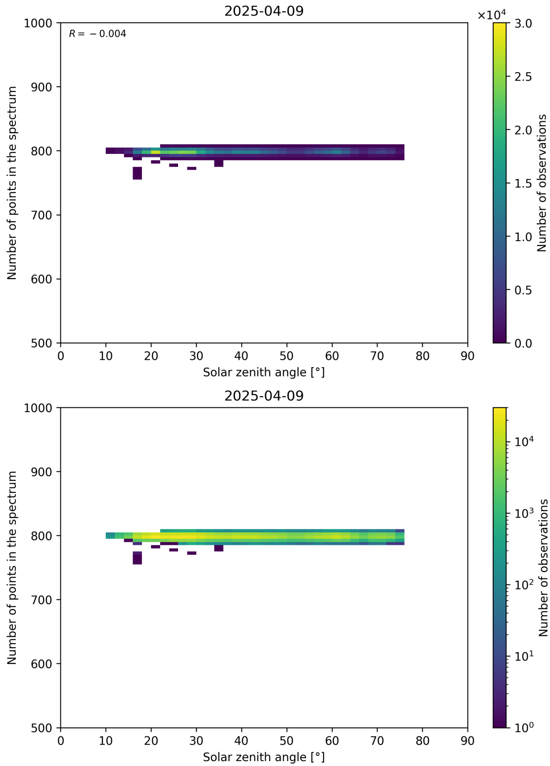
Figure 103: Scatter density plot of “Solar zenith angle” against “Number of points in the spectrum” for 2025-04-08 to 2025-04-10.
