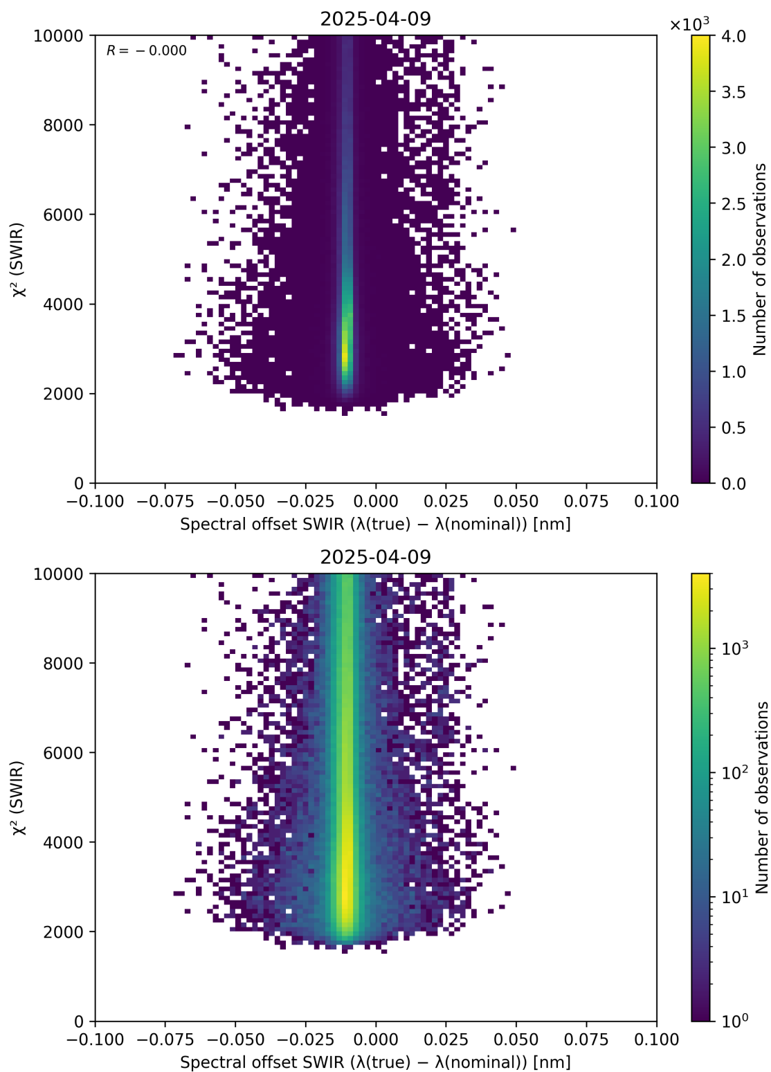
Figure 118: Scatter density plot of “Spectral offset SWIR ( \lambda_{\text{true}} - \lambda_{\text{nominal}} )” against “ \chi^2 (SWIR)” for 2025-04-08 to 2025-04-10.
