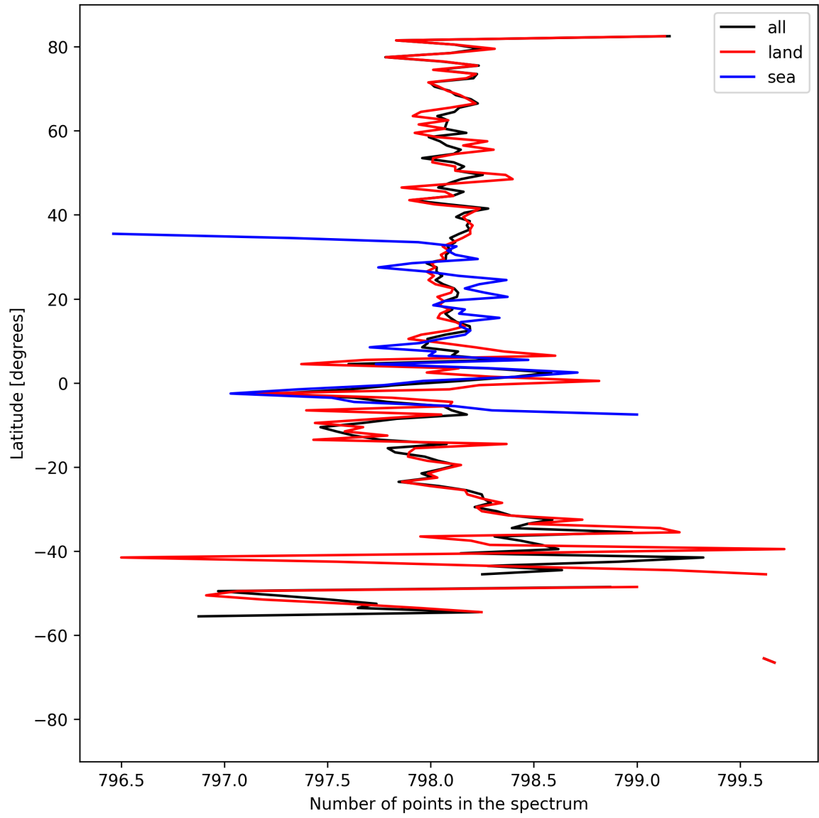
Figure 15: Zonal average of “Number of points in the spectrum” for 2025-04-08 to 2025-04-10.
