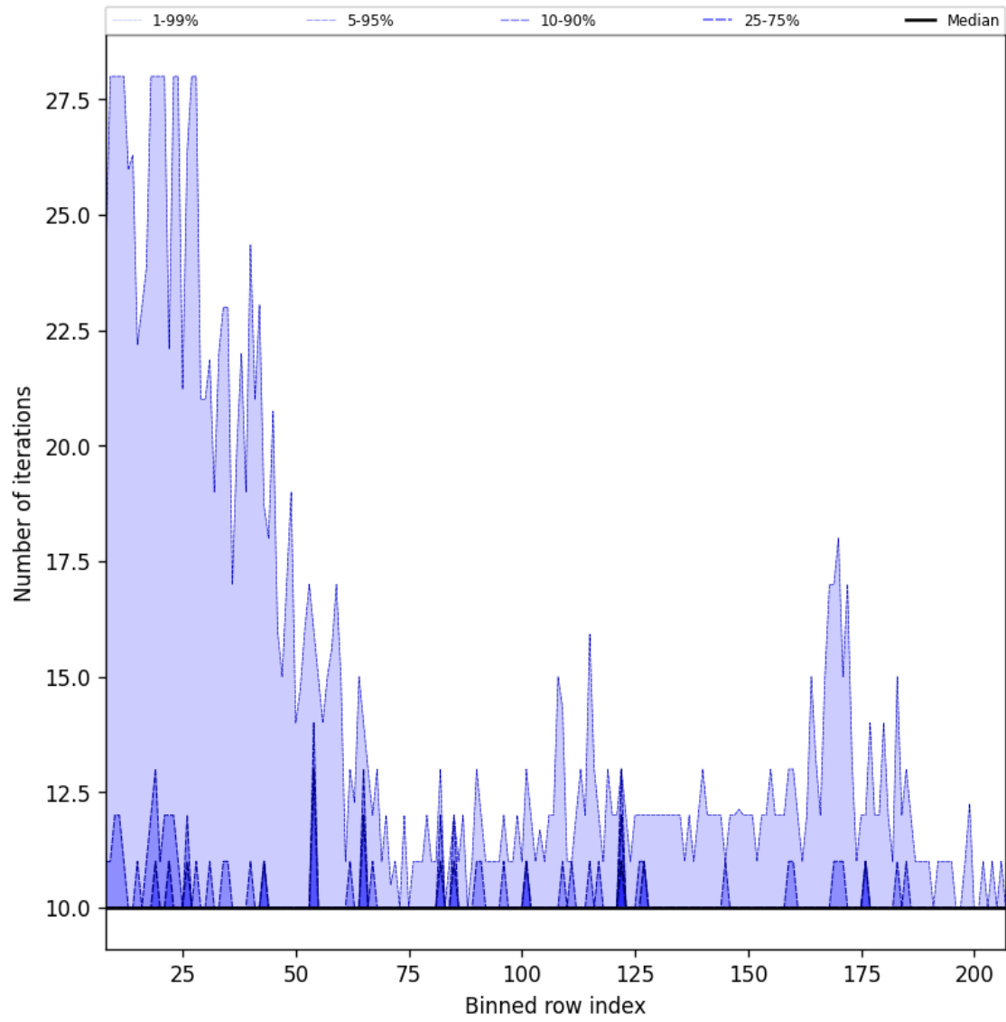
Figure 42: Along track statistics of “Number of iterations” for 2025-04-08 to 2025-04-10
