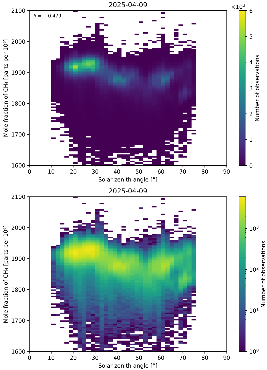
Figure 99: Scatter density plot of “Solar zenith angle” against “Mole fraction of CH 4 ” for 2025-04-08 to 2025-04-10.
