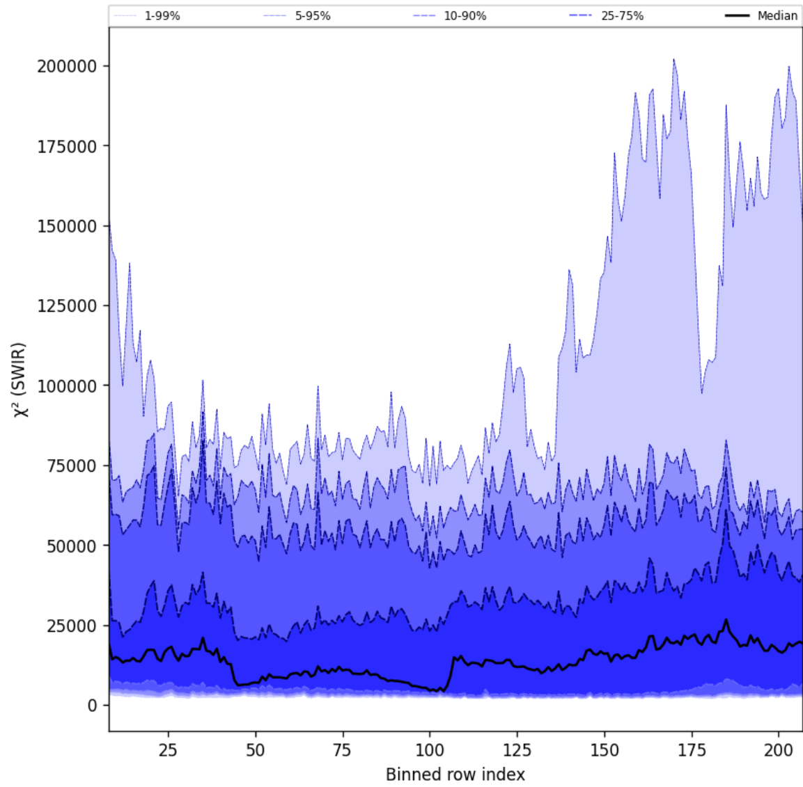
Figure 39: Along track statistics of “ \chi^2 (SWIR)” for 2025-04-08 to 2025-04-10
