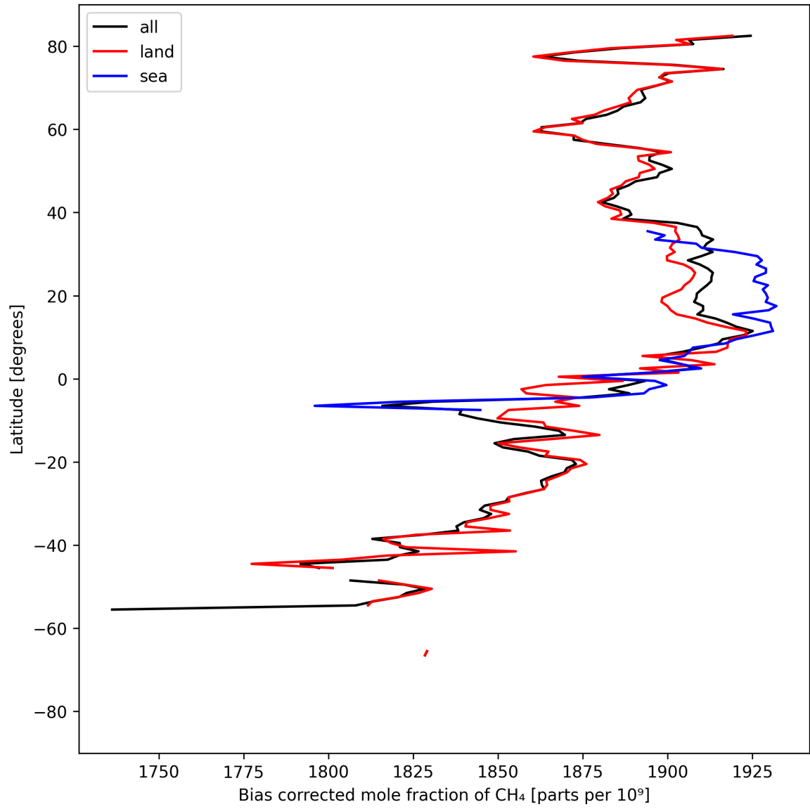
Figure 14: Zonal average of “Bias corrected mole fraction of CH 4 ” for 2025-04-08 to 2025-04-10.
