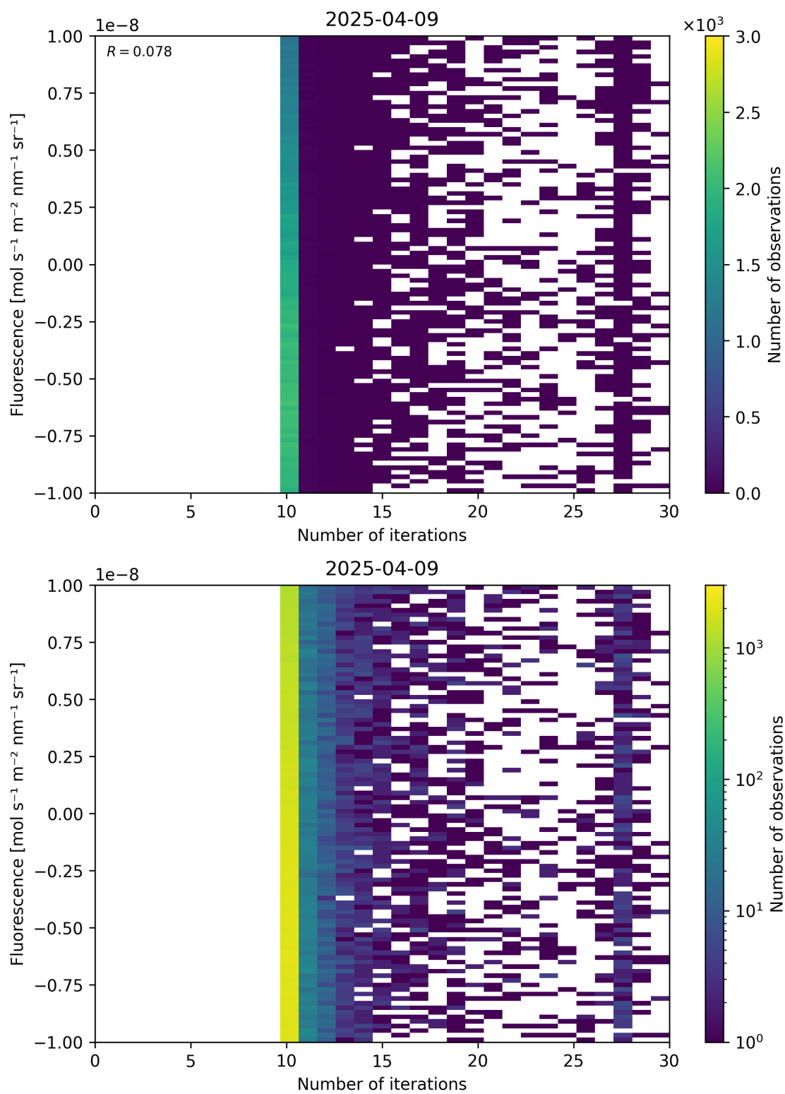
Figure 87: Scatter density plot of “Number of iterations” against “Fluorescence” for 2025-04-08 to 2025-04-10.
