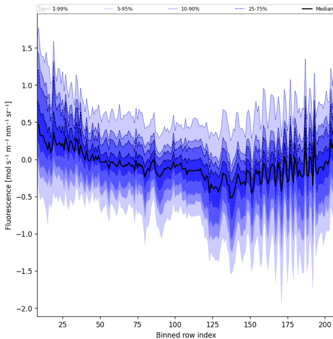
Figure 43: Along track statistics of “Fluorescence” for 2025-04-08 to 2025-04-10
