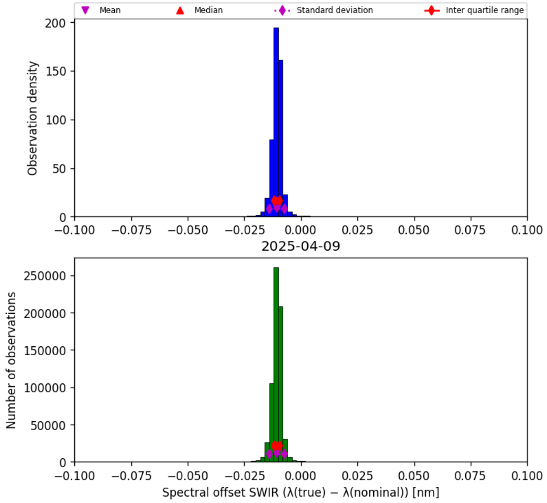
Figure 27: Histogram of “Spectral offset SWIR ( \lambda_{\text{true}} - \lambda_{\text{nominal}} )” for 2025-04-08 to 2025-04-10
