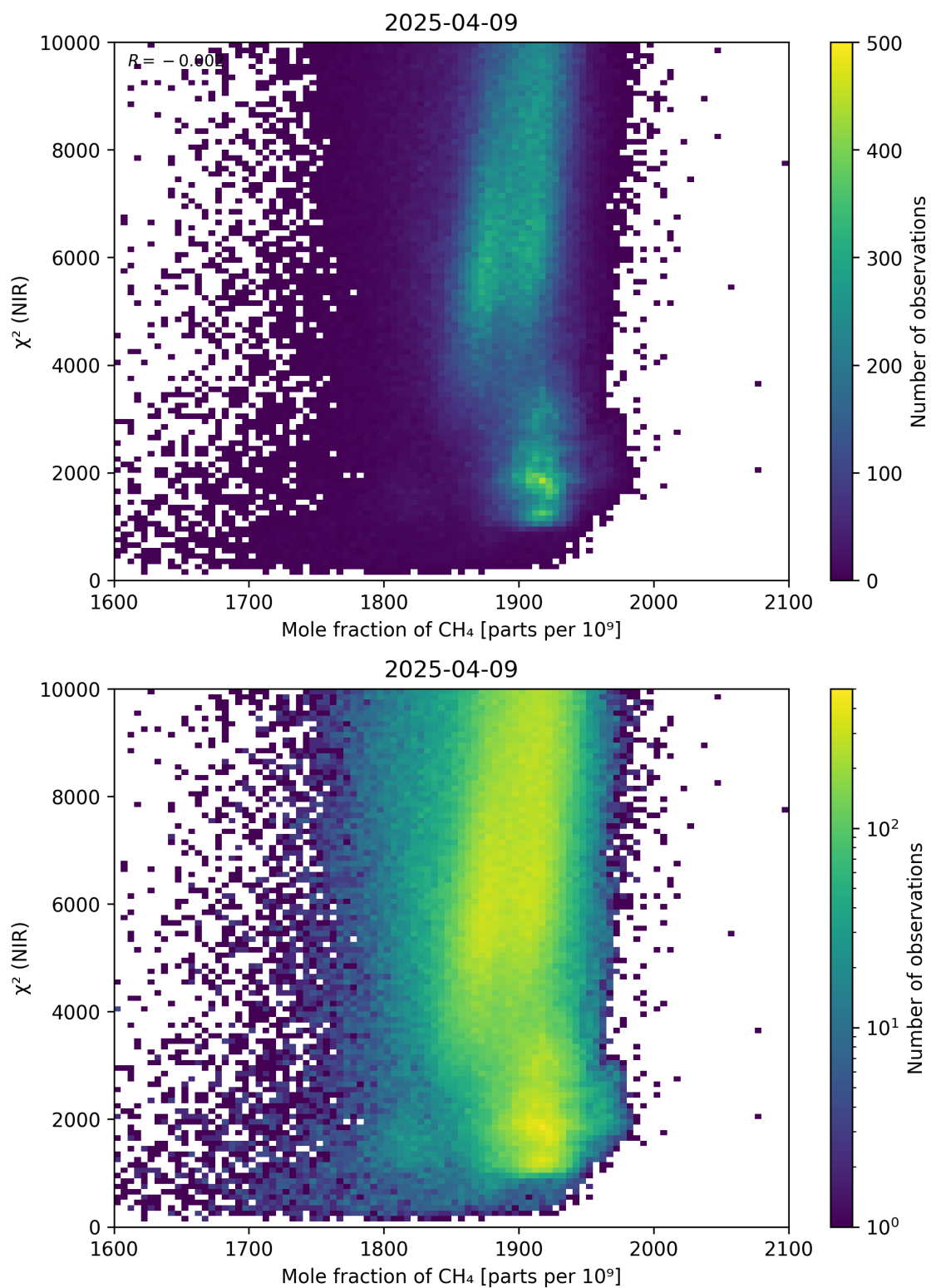
Figure 70: Scatter density plot of “Mole fraction of CH 4 ” against “ \chi^2 (NIR)” for 2025-04-08 to 2025-04-10.
