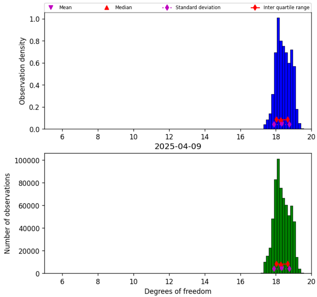
Figure 30: Histogram of “Degrees of freedom” for 2025-04-08 to 2025-04-10
