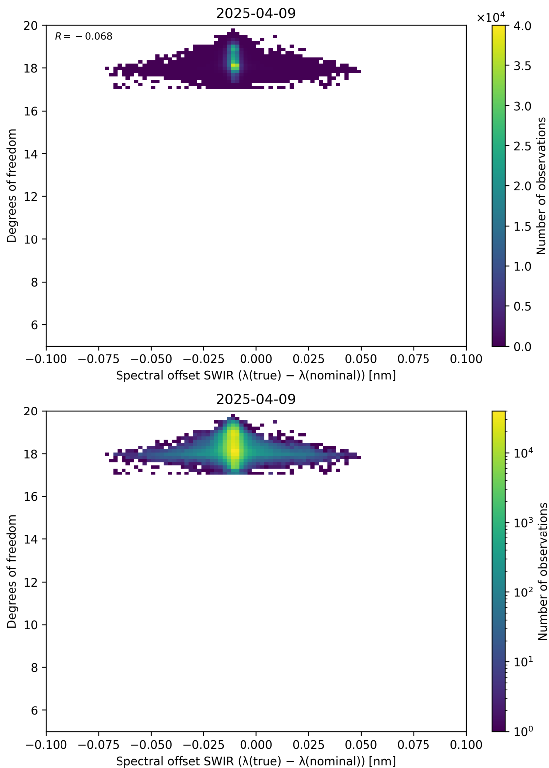
Figure 119: Scatter density plot of “Spectral offset SWIR ( \lambda_{\text{true}} - \lambda_{\text{nominal}} )” against “Degrees of freedom” for 2025-04-08 to 2025-04-10.
