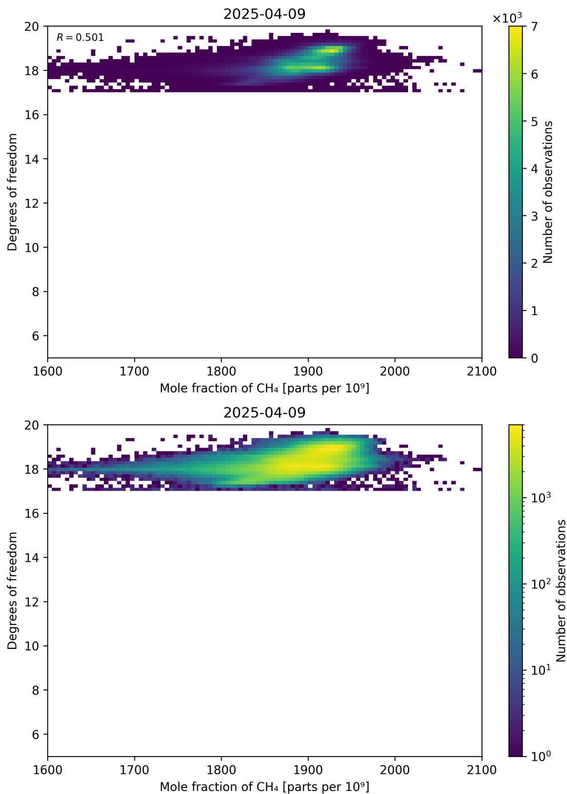
Figure 72: Scatter density plot of “Mole fraction of CH 4 ” against “Degrees of freedom” for 2025-04-08 to 2025-04-10.
