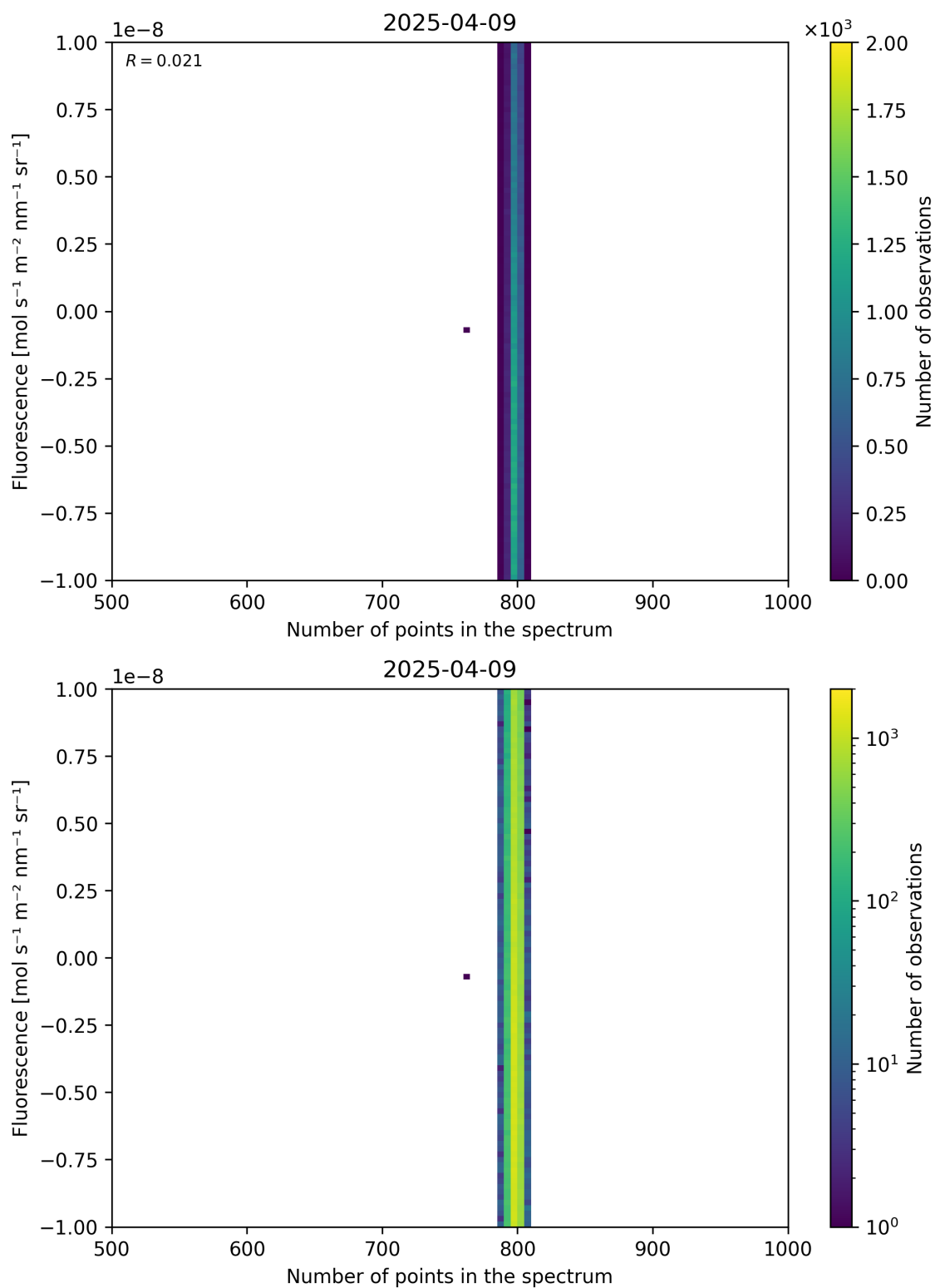
Figure 91: Scatter density plot of “Number of points in the spectrum” against “Fluorescence” for 2025-04-08 to 2025-04-10.
