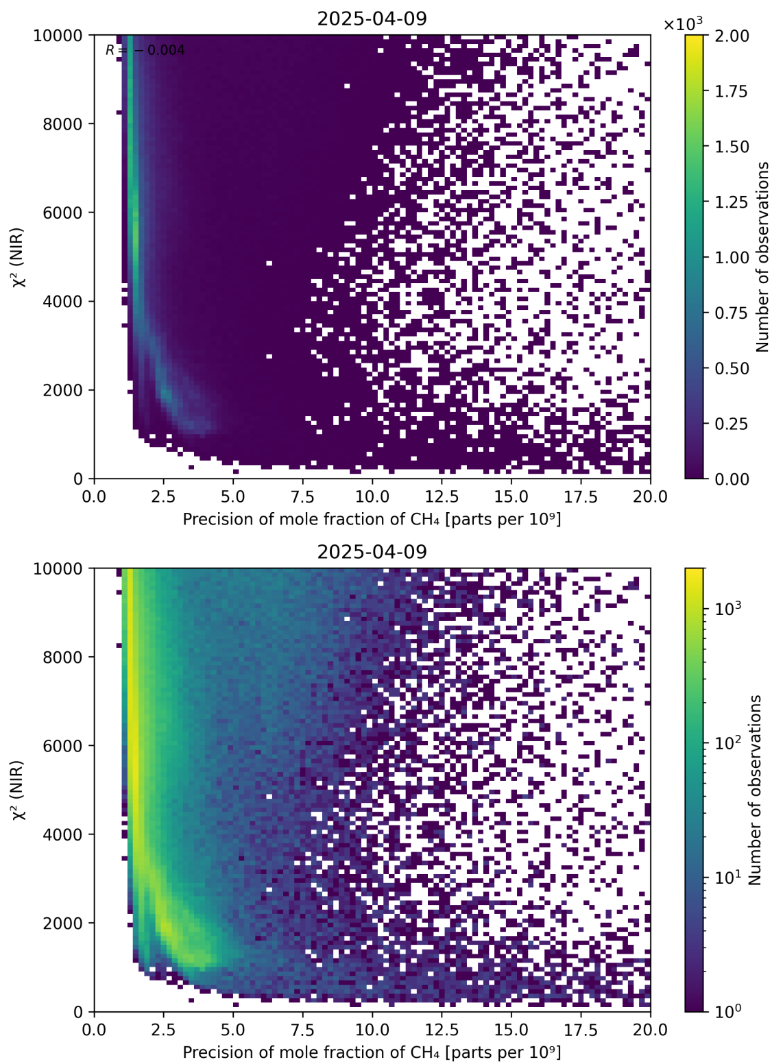
Figure 78: Scatter density plot of “Precision of mole fraction of CH 4 ” against “ \chi^2 (NIR)” for 2025-04-08 to 2025-04-10.
