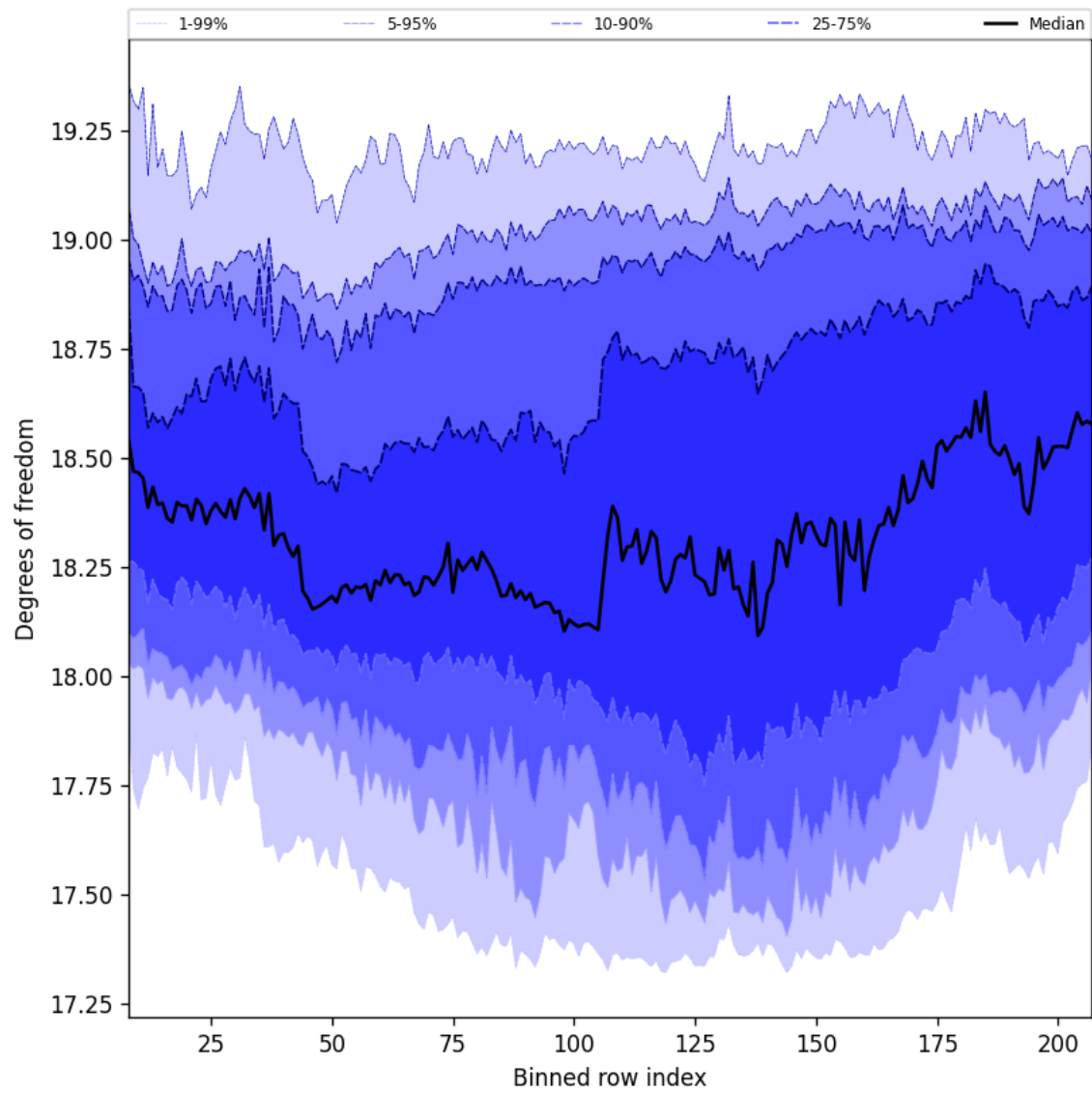
Figure 41: Along track statistics of “Degrees of freedom” for 2025-04-08 to 2025-04-10
