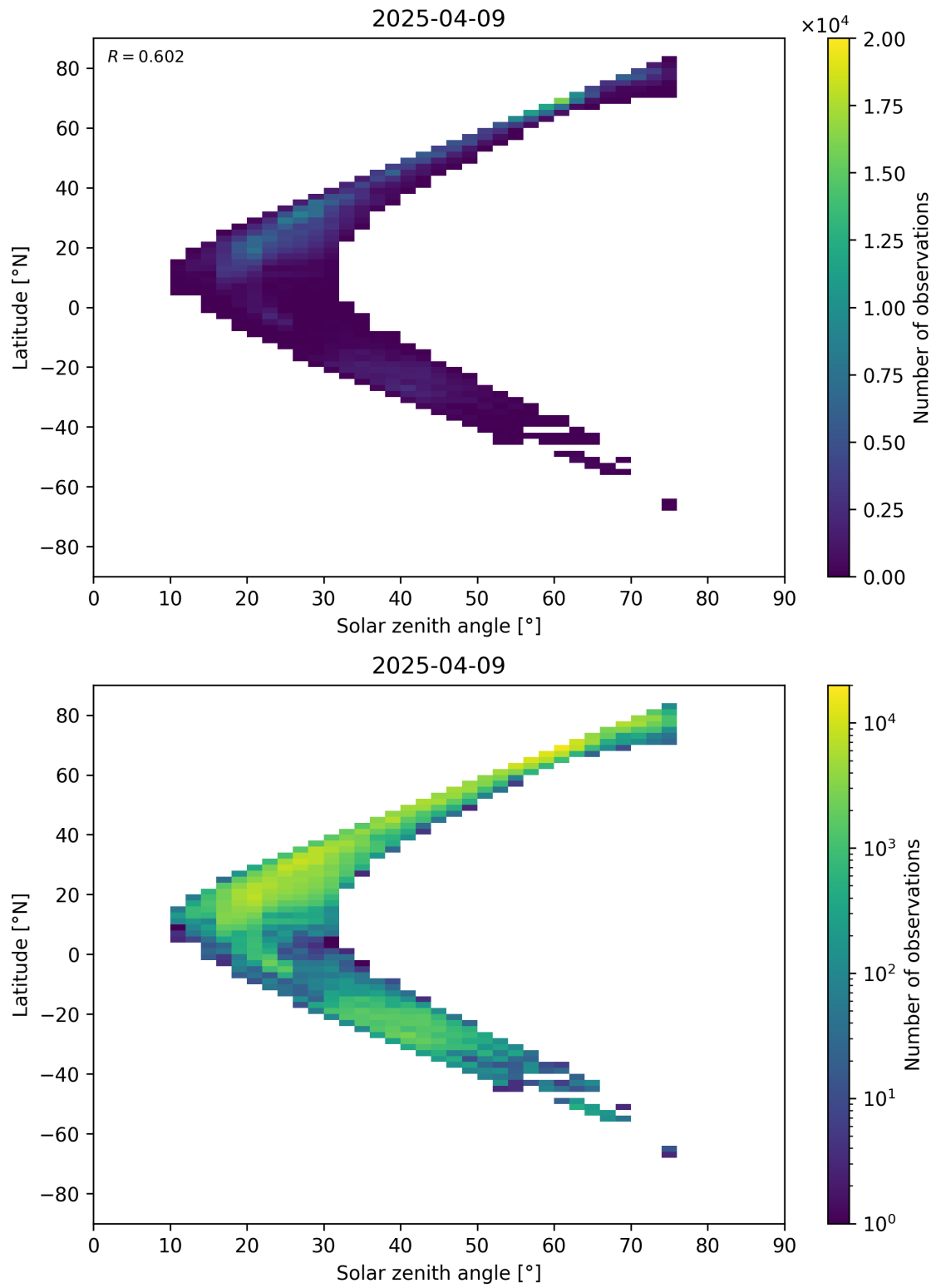
Figure 98: Scatter density plot of “Solar zenith angle” against “Latitude” for 2025-04-08 to 2025-04-10.
