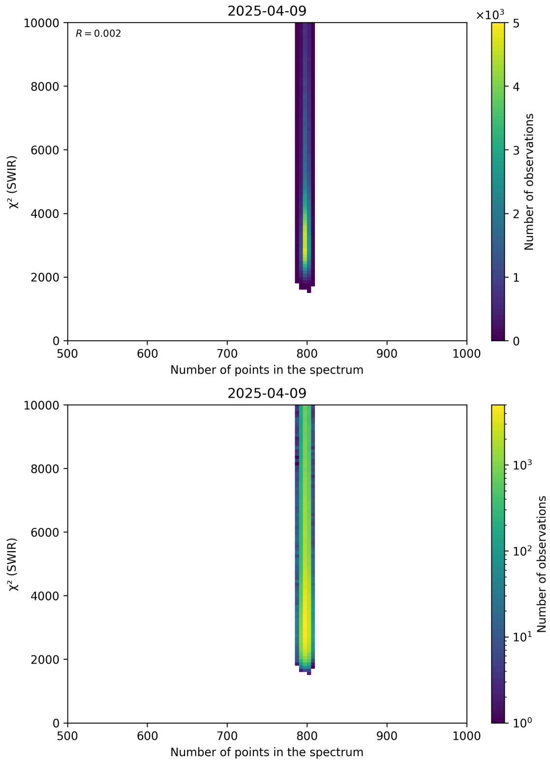
Figure 89: Scatter density plot of “Number of points in the spectrum” against “ \chi^2 (SWIR)” for 2025-04-08 to 2025-04-10.
