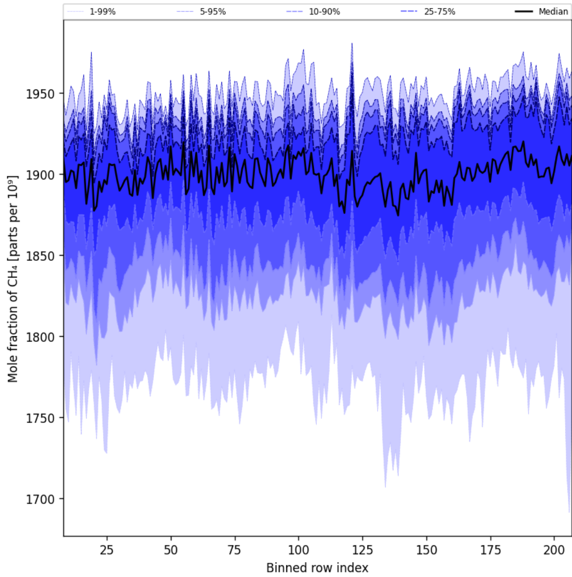
Figure 34: Along track statistics of “Mole fraction of CH 4 ” for 2025-04-08 to 2025-04-10
