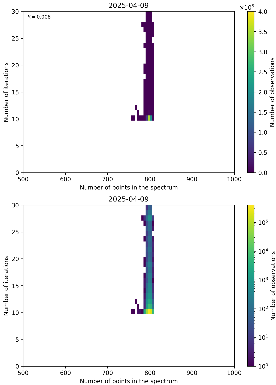
Figure 92: Scatter density plot of “Number of points in the spectrum” against “Number of iterations” for 2025-04-08 to 2025-04-10.
