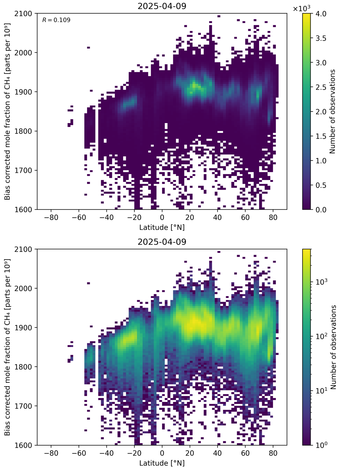
Figure 58: Scatter density plot of “Latitude” against “Bias corrected mole fraction of \text{CH}_4 ” for 2025-04-08 to 2025-04-10.
