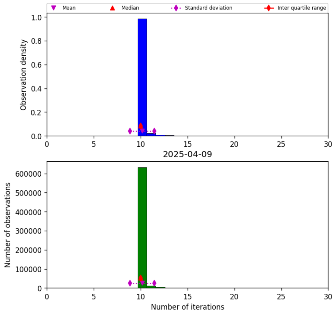
Figure 31: Histogram of “Number of iterations” for 2025-04-08 to 2025-04-10
