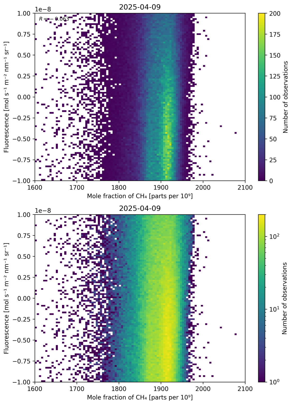
Figure 73: Scatter density plot of “Mole fraction of \text{CH}_4 ” against “Fluorescence” for 2025-04-08 to 2025-04-10.
