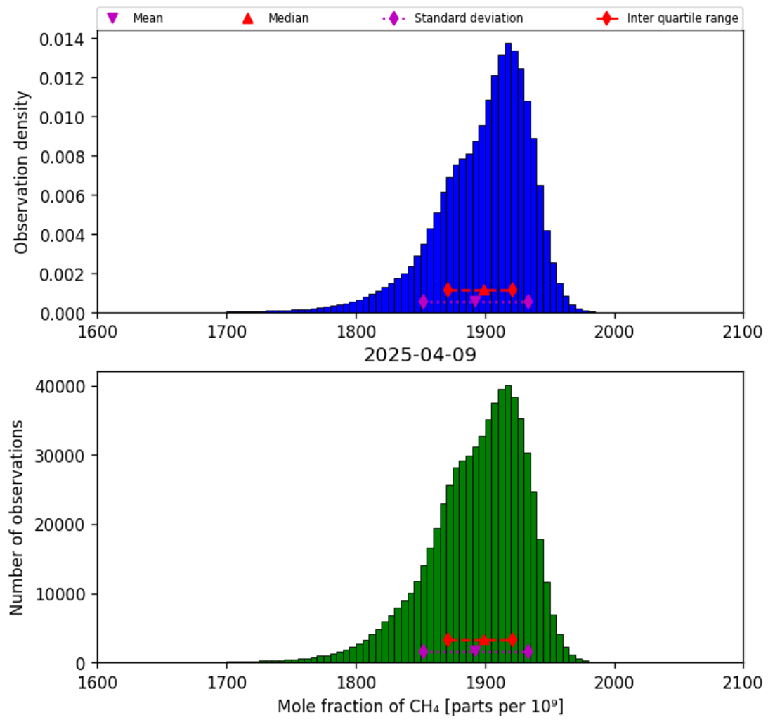
Figure 23: Histogram of “Mole fraction of CH 4 ” for 2025-04-08 to 2025-04-10
