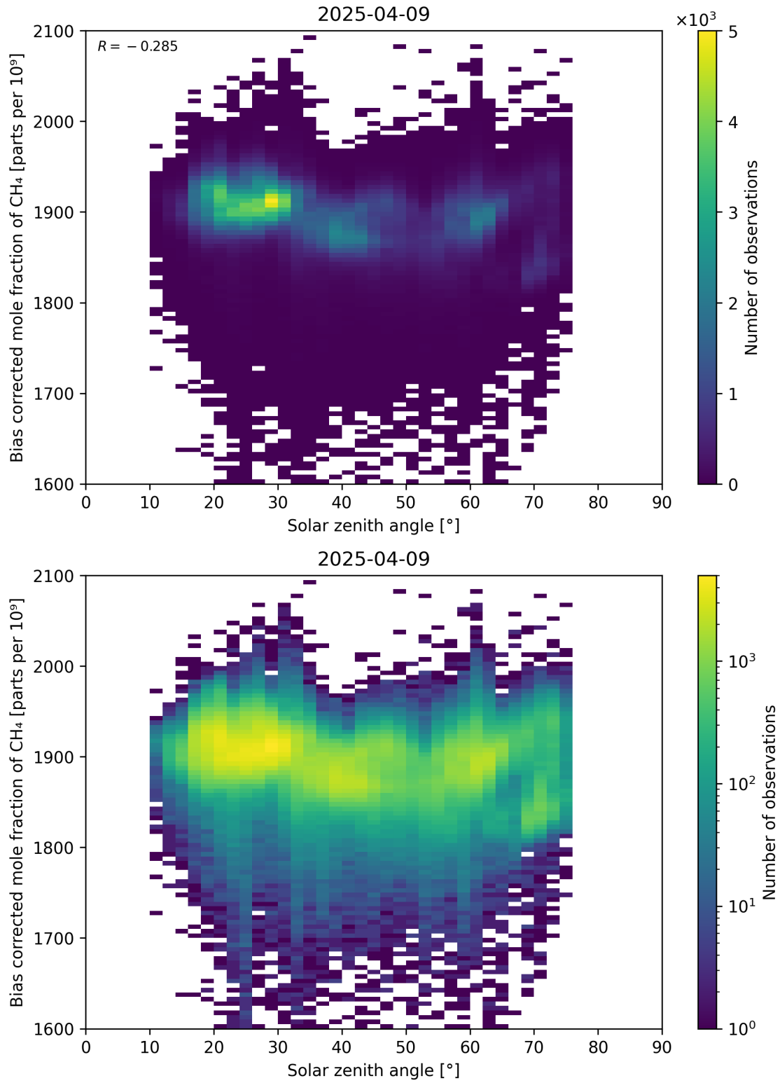
Figure 100: Scatter density plot of “Solar zenith angle” against “Bias corrected mole fraction of CH 4 ” for 2025-04-08 to 2025-04-10.
