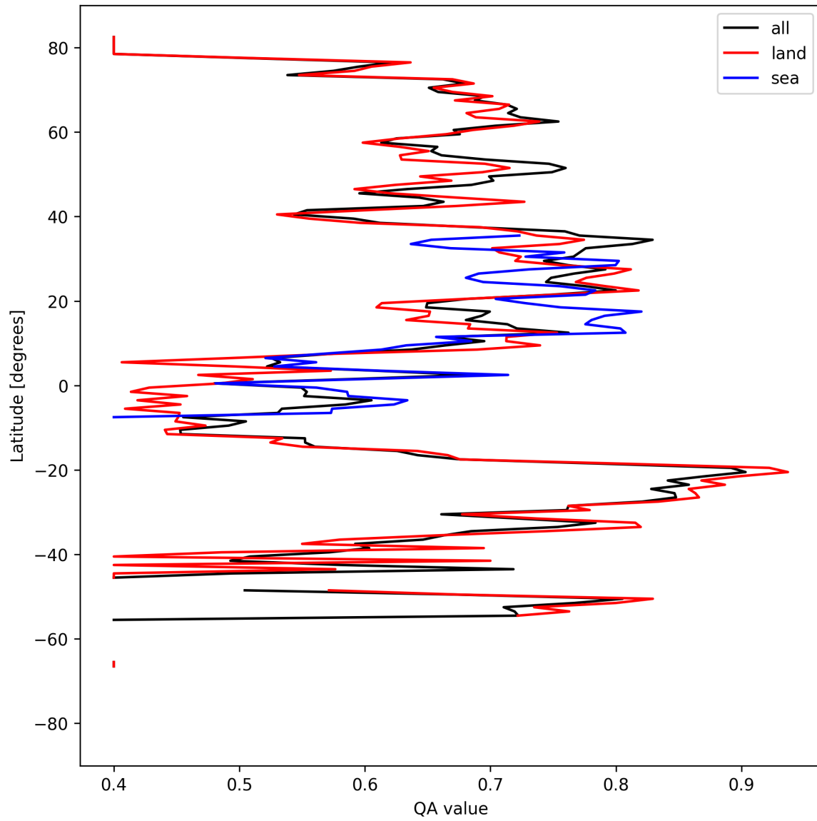
Figure 11: Zonal average of “QA value” for 2025-04-08 to 2025-04-10.
