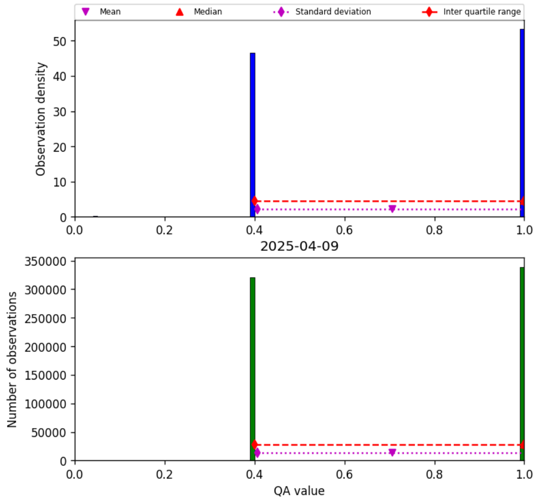
Figure 22: Histogram of “QA value” for 2025-04-08 to 2025-04-10
