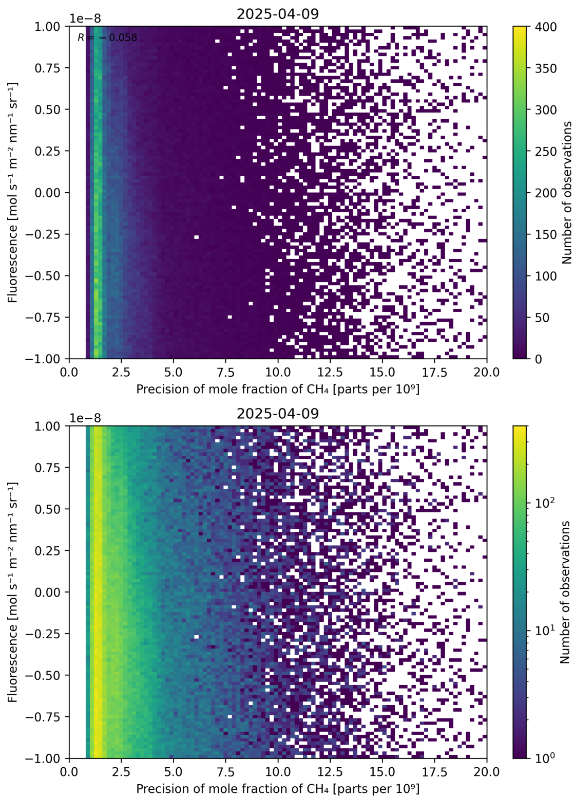
Figure 81: Scatter density plot of “Precision of mole fraction of \text{CH}_4 ” against “Fluorescence” for 2025-04-08 to 2025-04-10.
