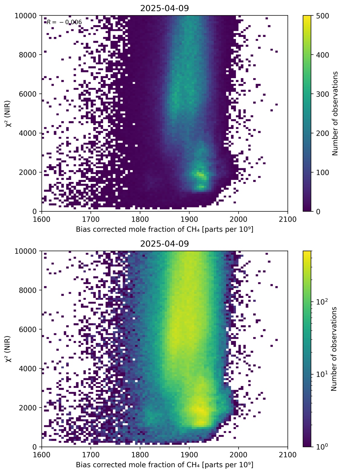
Figure 63: Scatter density plot of “Bias corrected mole fraction of CH 4 ” against “ \chi^2 (NIR)” for 2025-04-08 to 2025-04-10.
