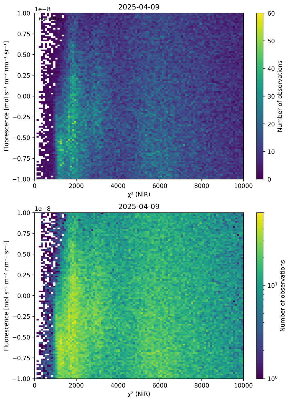
Figure 45: Scatter density plot of “ \chi^2 (NIR)” against “Fluorescence” for 2025-04-08 to 2025-04-10.
