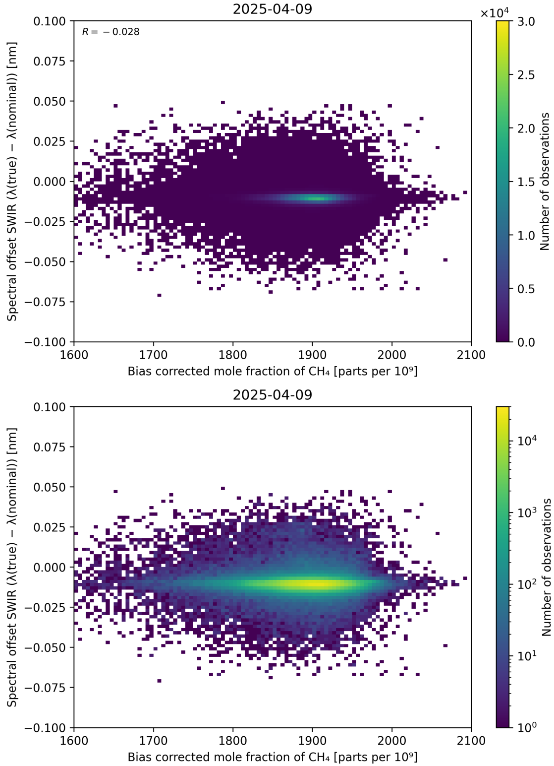
Figure 69: Scatter density plot of “Bias corrected mole fraction of \text{CH}_4 ” against “Spectral offset SWIR ( \lambda_{\text{true}} - \lambda_{\text{nominal}} )” for 2025-04-08 to 2025-04-10.
