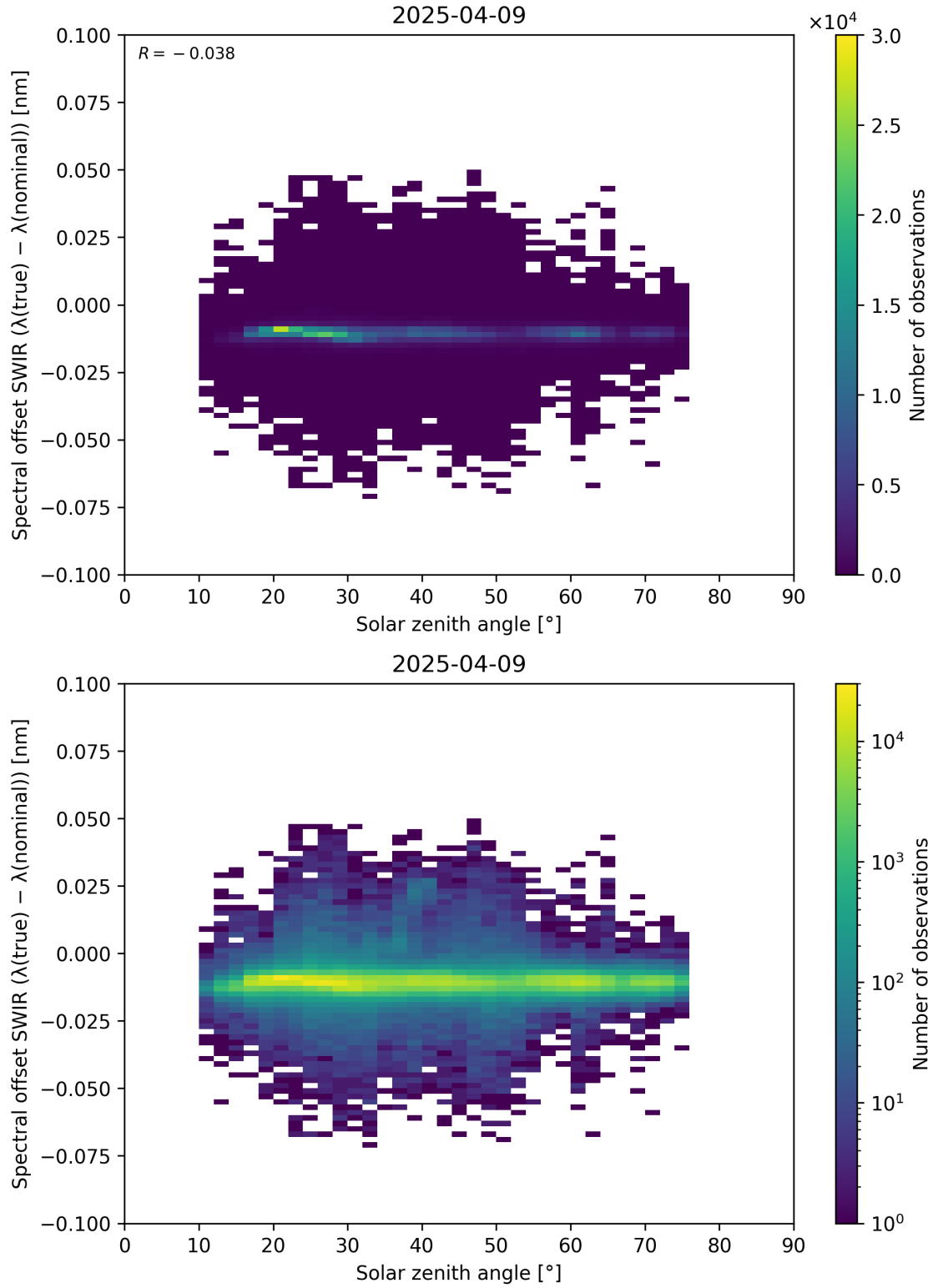
Figure 104: Scatter density plot of “Solar zenith angle” against “Spectral offset SWIR ( \lambda_{\text{true}} - \lambda_{\text{nominal}} )” for 2025-04-08 to 2025-04-10.
