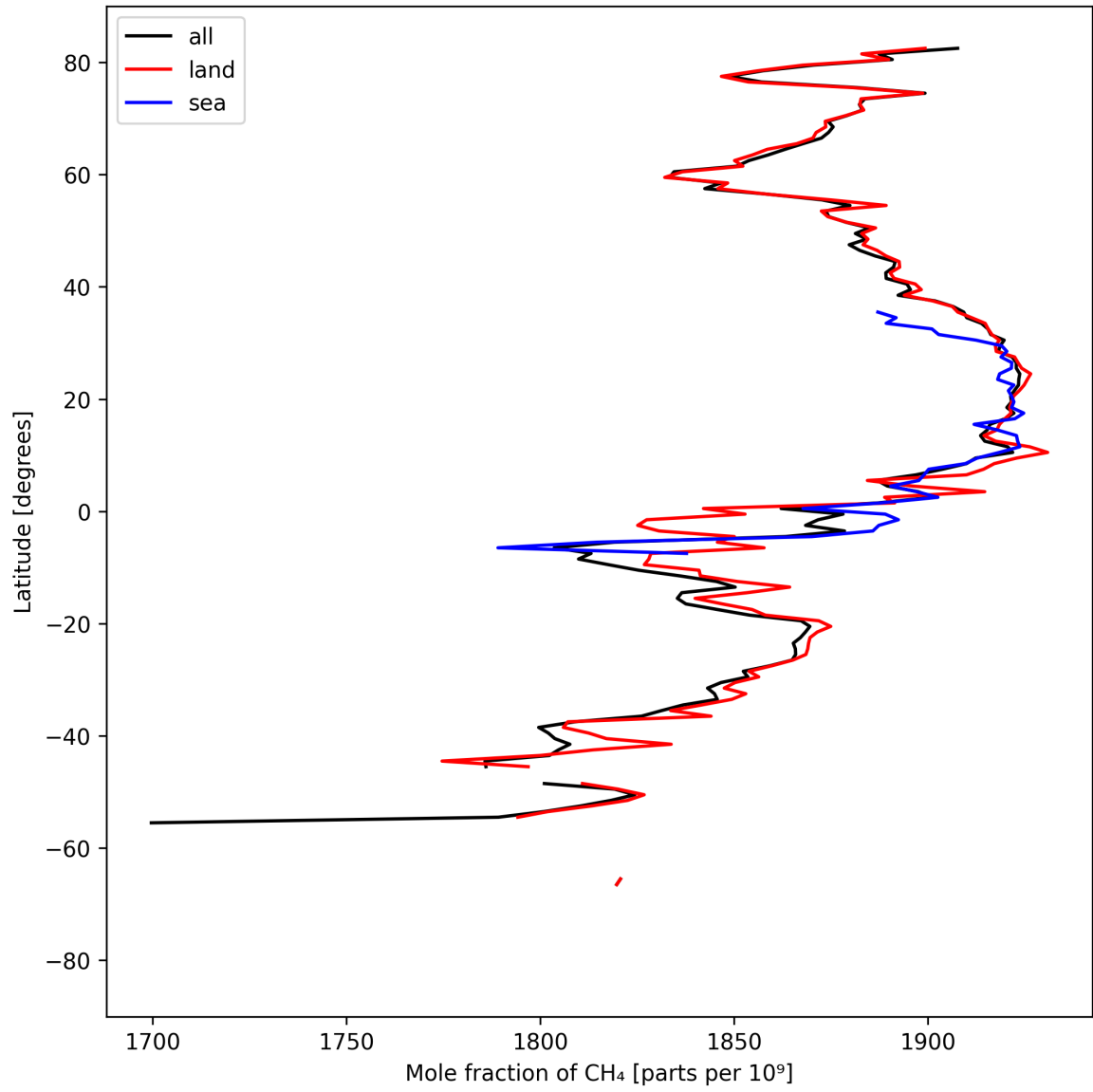
Figure 12: Zonal average of “Mole fraction of \text{CH}_4 ” for 2025-04-08 to 2025-04-10.
