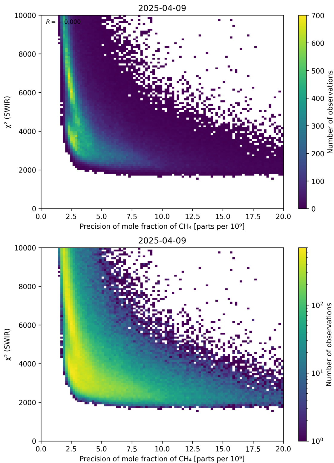
Figure 79: Scatter density plot of “Precision of mole fraction of \text{CH}_4 ” against “ \chi^2 (SWIR)” for 2025-04-08 to 2025-04-10.
