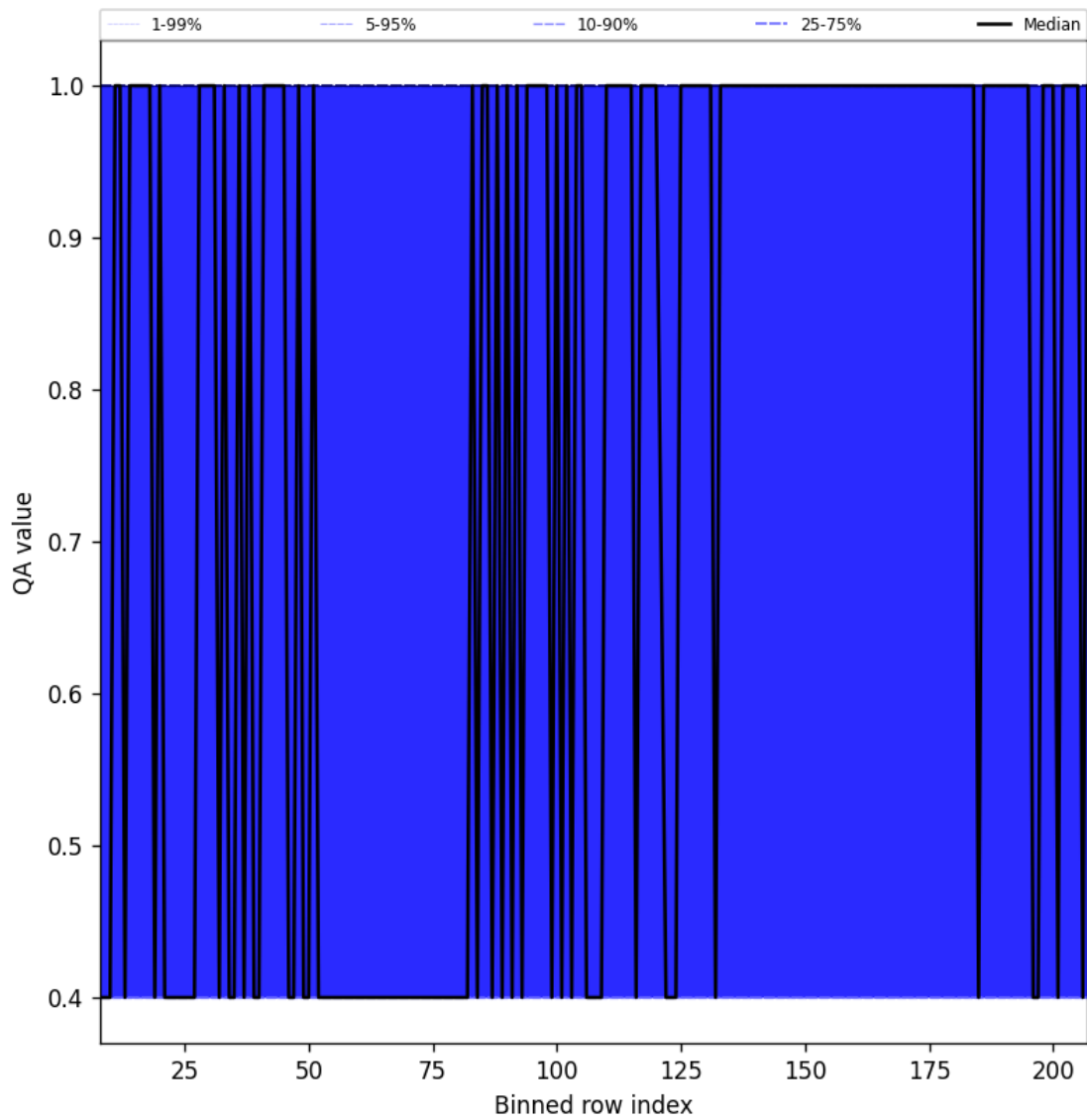
Figure 33: Along track statistics of “QA value” for 2025-04-08 to 2025-04-10
