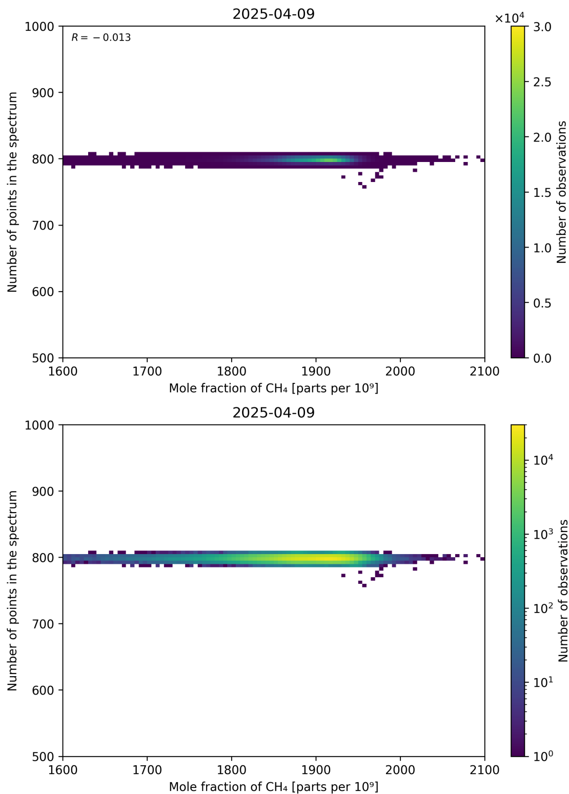
Figure 77: Scatter density plot of “Mole fraction of CH 4 ” against “Number of points in the spectrum” for 2025-04-08 to 2025-04-10.
