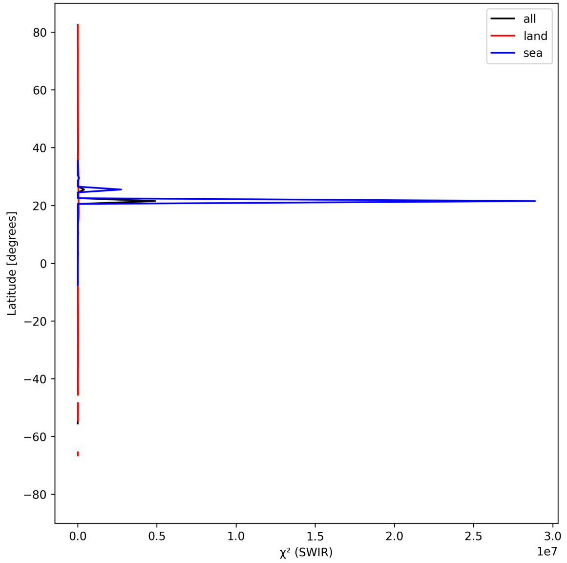
Figure 17: Zonal average of “ \chi^2 (SWIR)” for 2025-04-08 to 2025-04-10.
