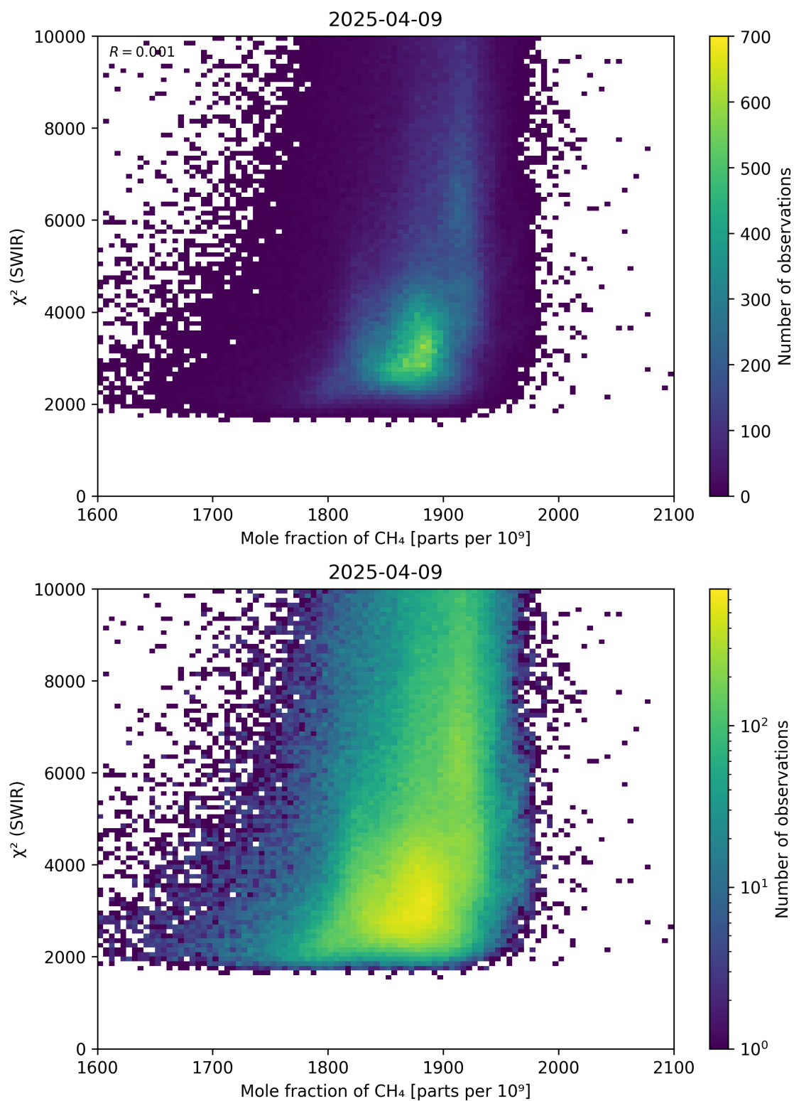
Figure 71: Scatter density plot of “Mole fraction of CH 4 ” against “ \chi^2 (SWIR)” for 2025-04-08 to 2025-04-10.
