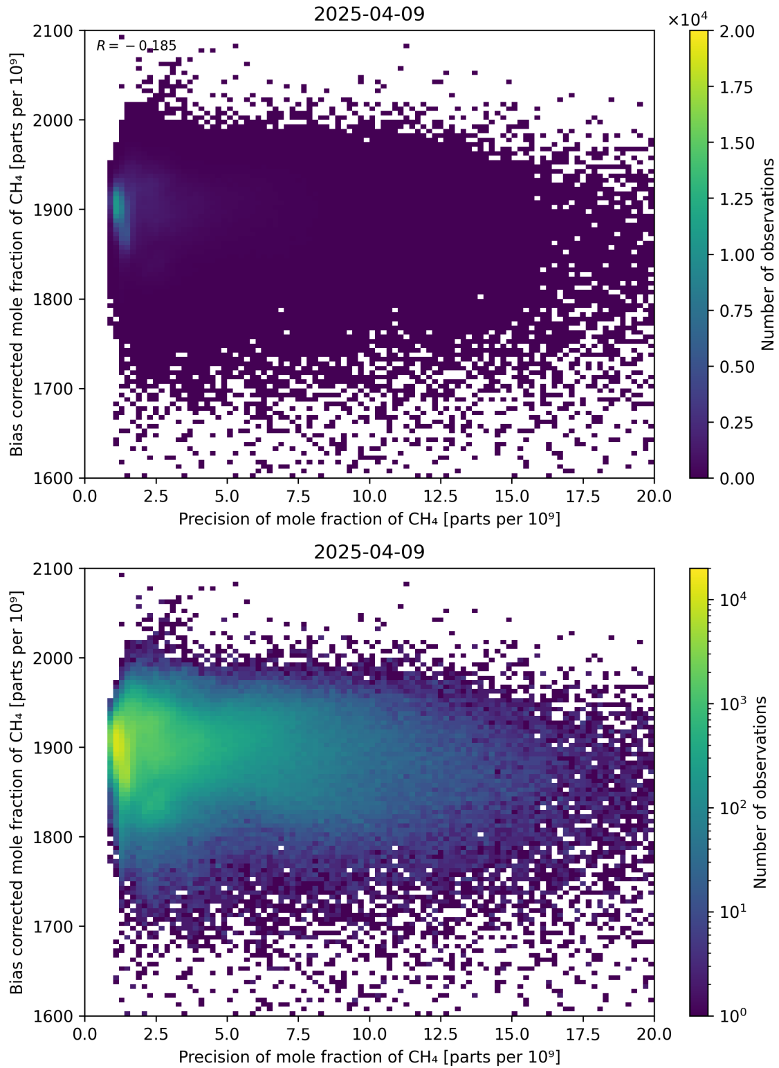
Figure 82: Scatter density plot of “Precision of mole fraction of CH 4 ” against “Bias corrected mole fraction of CH 4 ” for 2025-04-08 to 2025-04-10.
