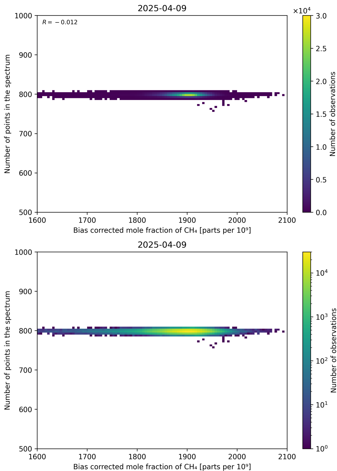
Figure 68: Scatter density plot of “Bias corrected mole fraction of CH 4 ” against “Number of points in the spectrum” for 2025-04-08 to 2025-04-10.
