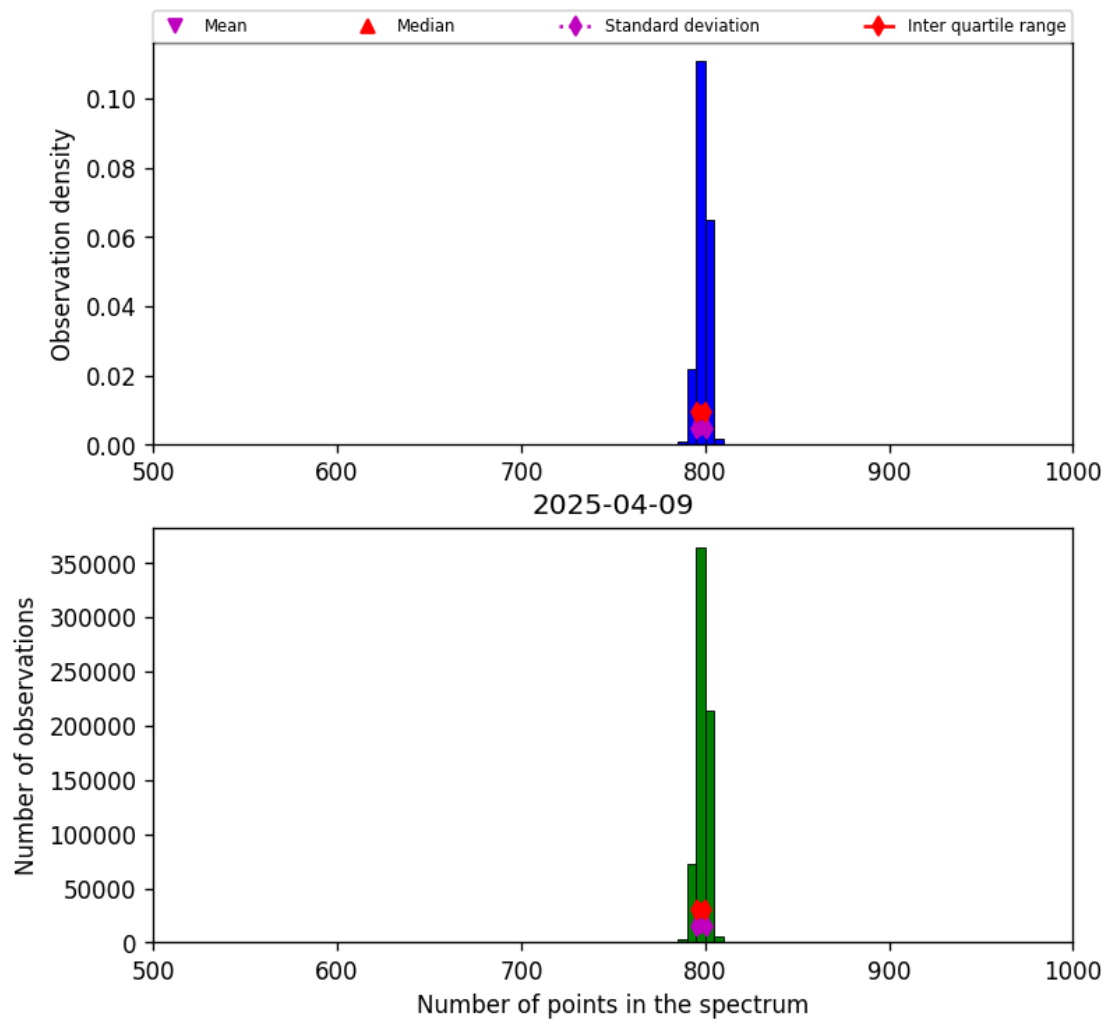
Figure 26: Histogram of “Number of points in the spectrum” for 2025-04-08 to 2025-04-10
