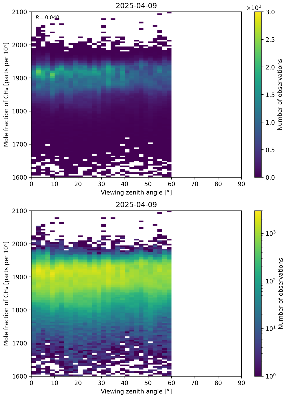
Figure 110: Scatter density plot of “Viewing zenith angle” against “Mole fraction of CH 4 ” for 2025-04-08 to 2025-04-10.
