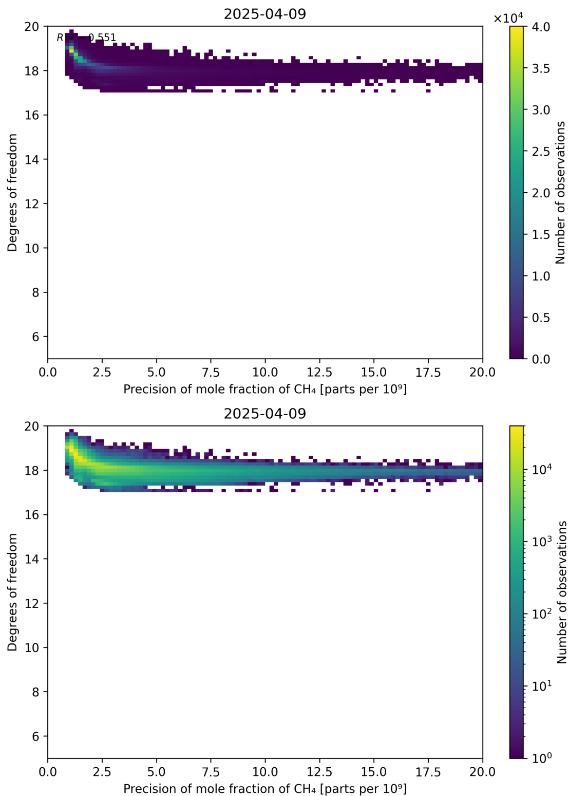
Figure 80: Scatter density plot of “Precision of mole fraction of CH 4 ” against “Degrees of freedom” for 2025-04-08 to 2025-04-10.
