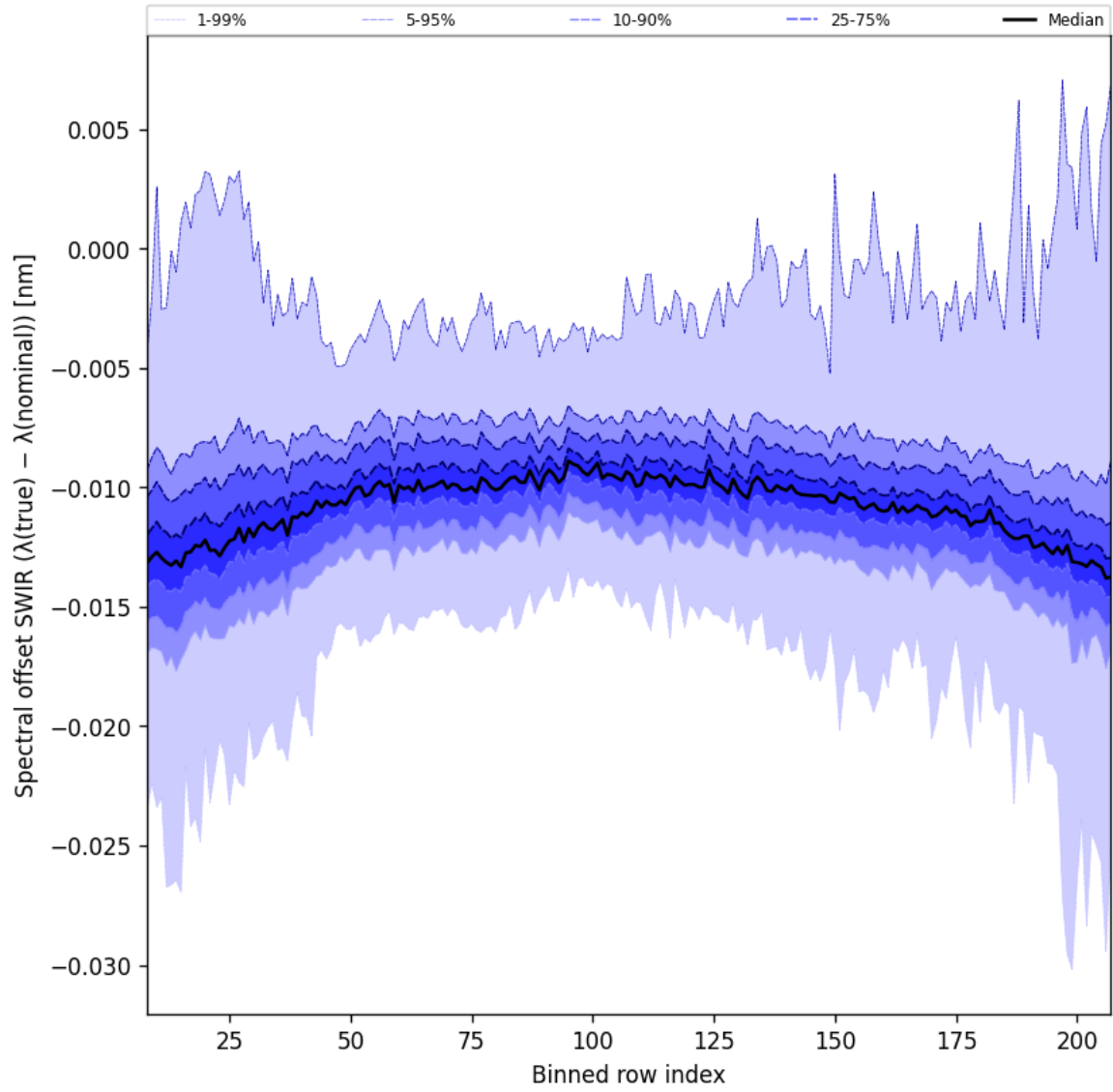
Figure 38: Along track statistics of “Spectral offset SWIR ( \lambda_{\text{true}} - \lambda_{\text{nominal}} )” for 2025-04-08 to 2025-04-10
