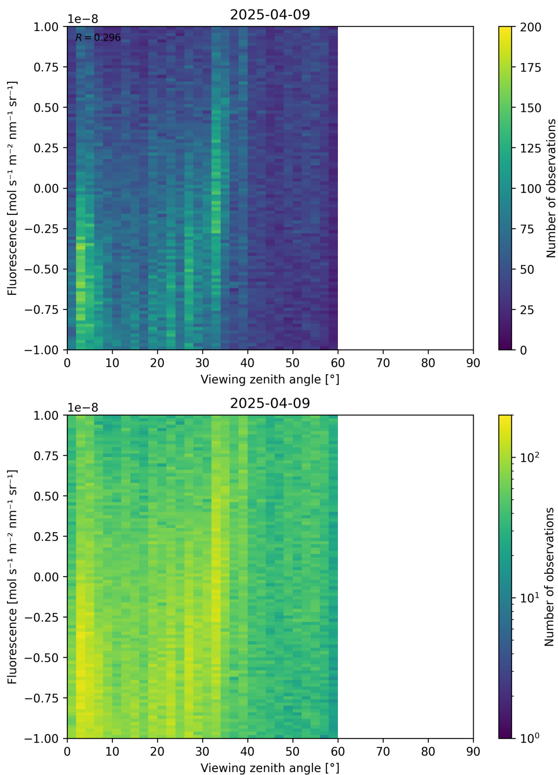
Figure 108: Scatter density plot of “Viewing zenith angle” against “Fluorescence” for 2025-04-08 to 2025-04-10.
