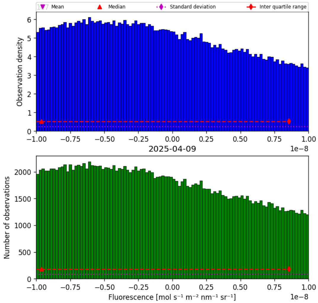
Figure 32: Histogram of “Fluorescence” for 2025-04-08 to 2025-04-10
