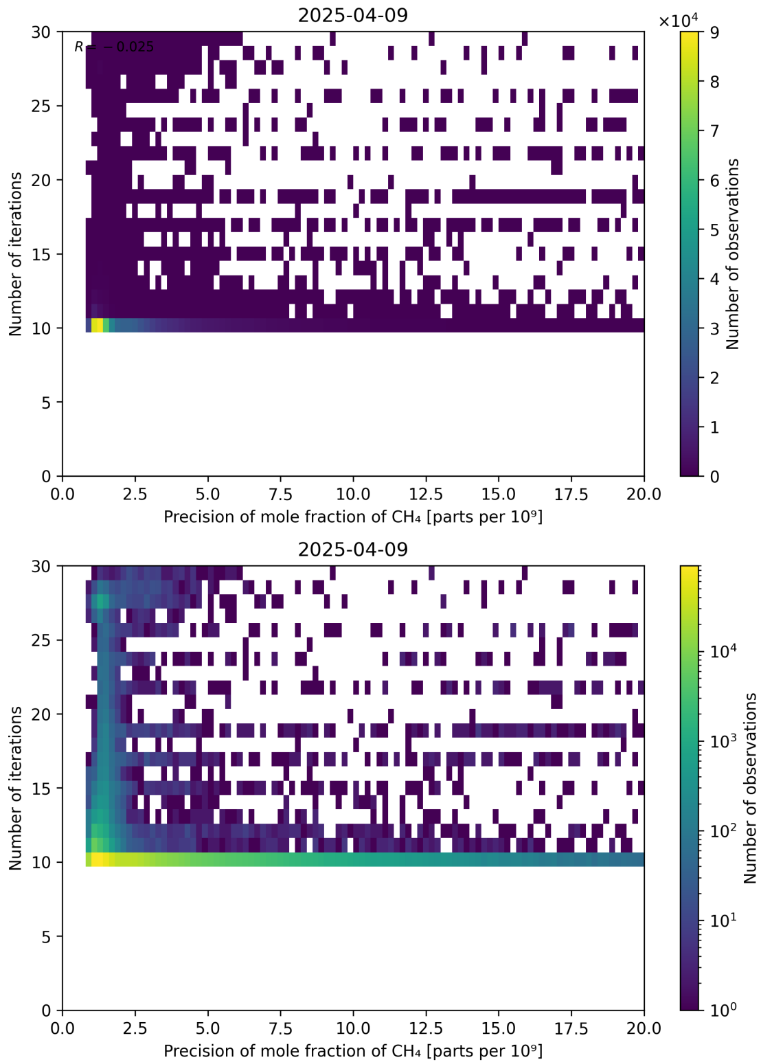
Figure 83: Scatter density plot of “Precision of mole fraction of CH 4 ” against “Number of iterations” for 2025-04-08 to 2025-04-10.
