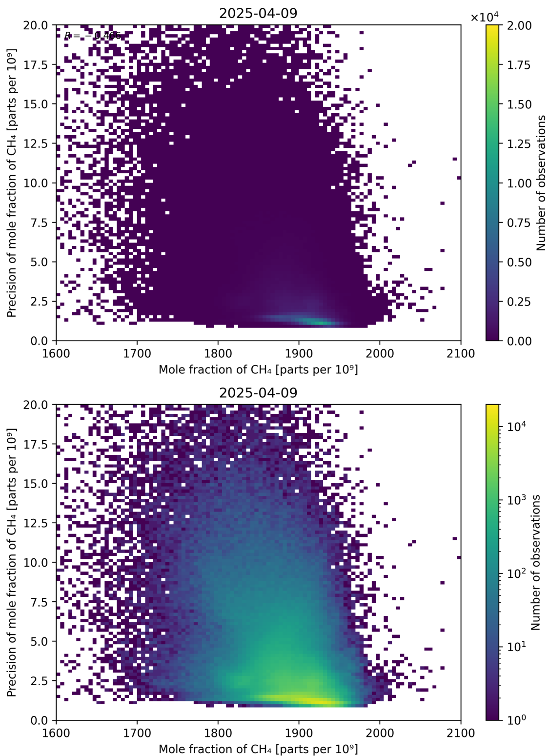
Figure 75: Scatter density plot of “Mole fraction of CH 4 ” against “Precision of mole fraction of CH 4 ” for 2025-04-08 to 2025-04-10.
