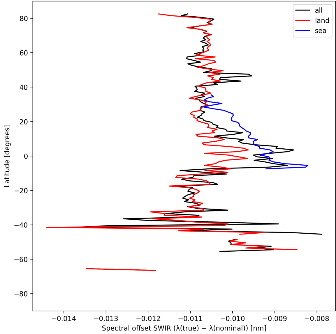
Figure 16: Zonal average of “Spectral offset SWIR ( \lambda_{\text{true}} - \lambda_{\text{nominal}} )” for 2025-04-08 to 2025-04-10.
