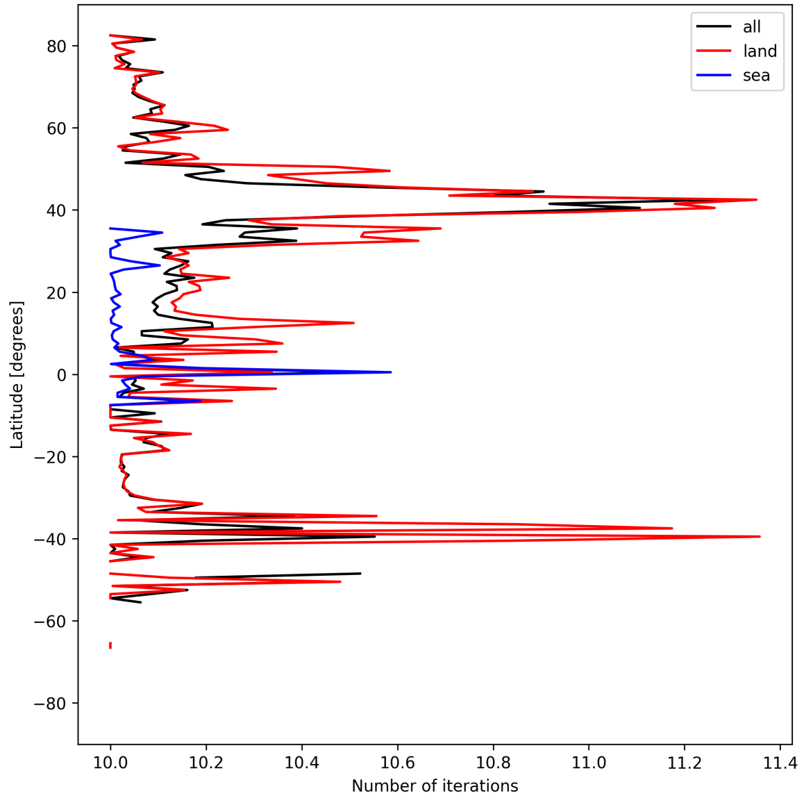
Figure 20: Zonal average of “Number of iterations” for 2025-04-08 to 2025-04-10.
