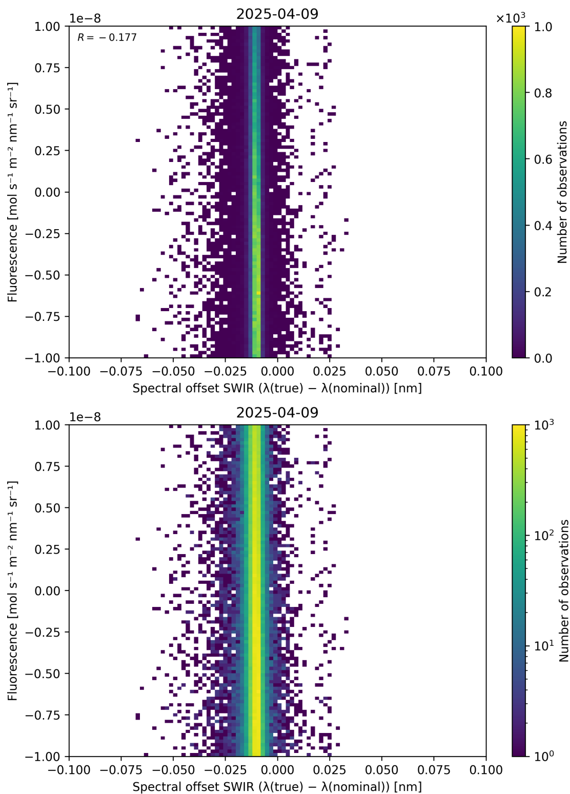
Figure 120: Scatter density plot of “Spectral offset SWIR ( \lambda_{\text{true}} - \lambda_{\text{nominal}} )” against “Fluorescence” for 2025-04-08 to 2025-04-10.
