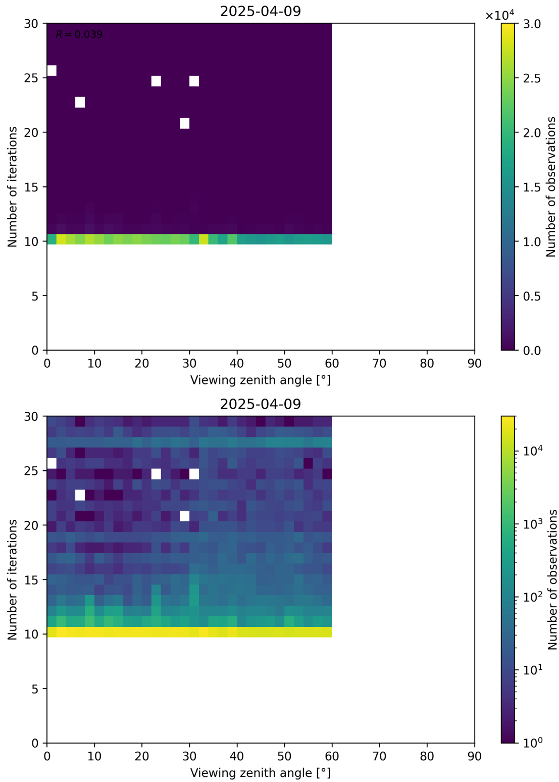
Figure 113: Scatter density plot of “Viewing zenith angle” against “Number of iterations” for 2025-04-08 to 2025-04-10.
