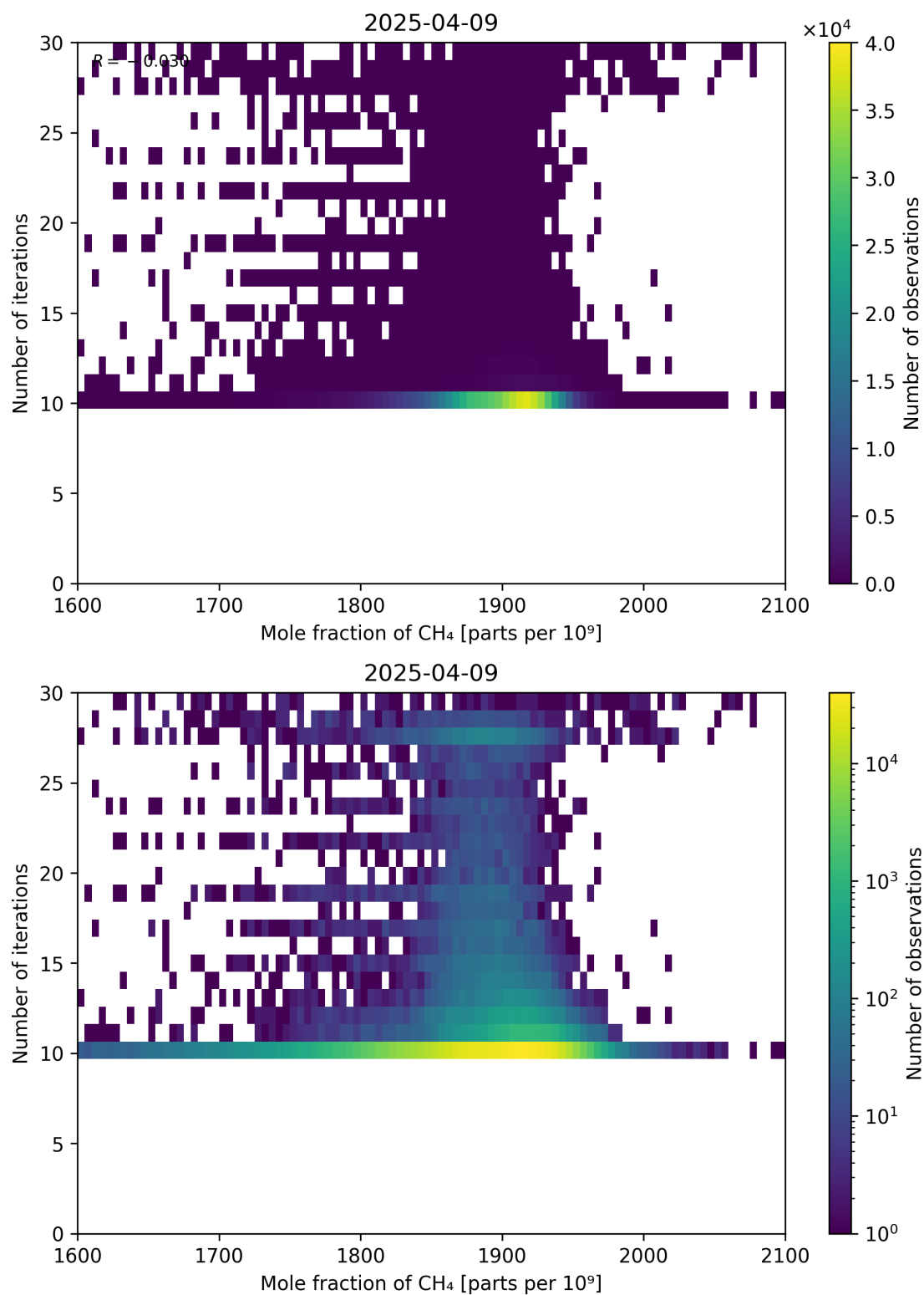
Figure 76: Scatter density plot of “Mole fraction of CH 4 ” against “Number of iterations” for 2025-04-08 to 2025-04-10.
