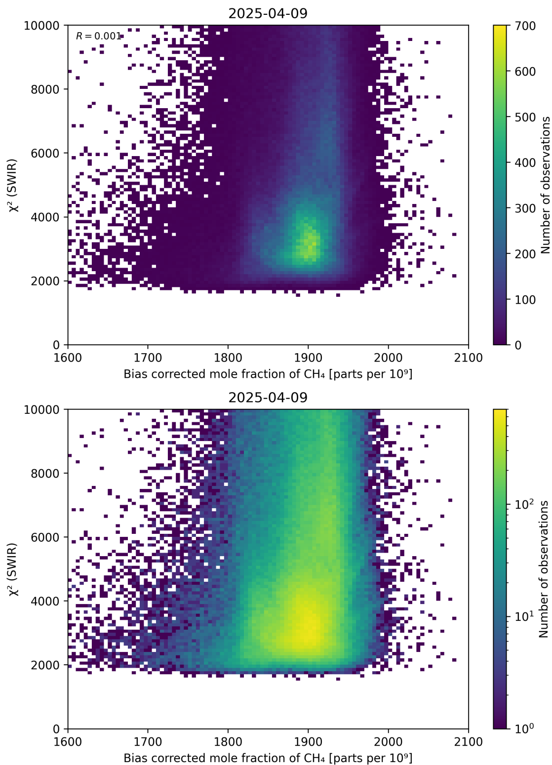
Figure 64: Scatter density plot of “Bias corrected mole fraction of \text{CH}_4 ” against “ \chi^2 (SWIR)” for 2025-04-08 to 2025-04-10.
