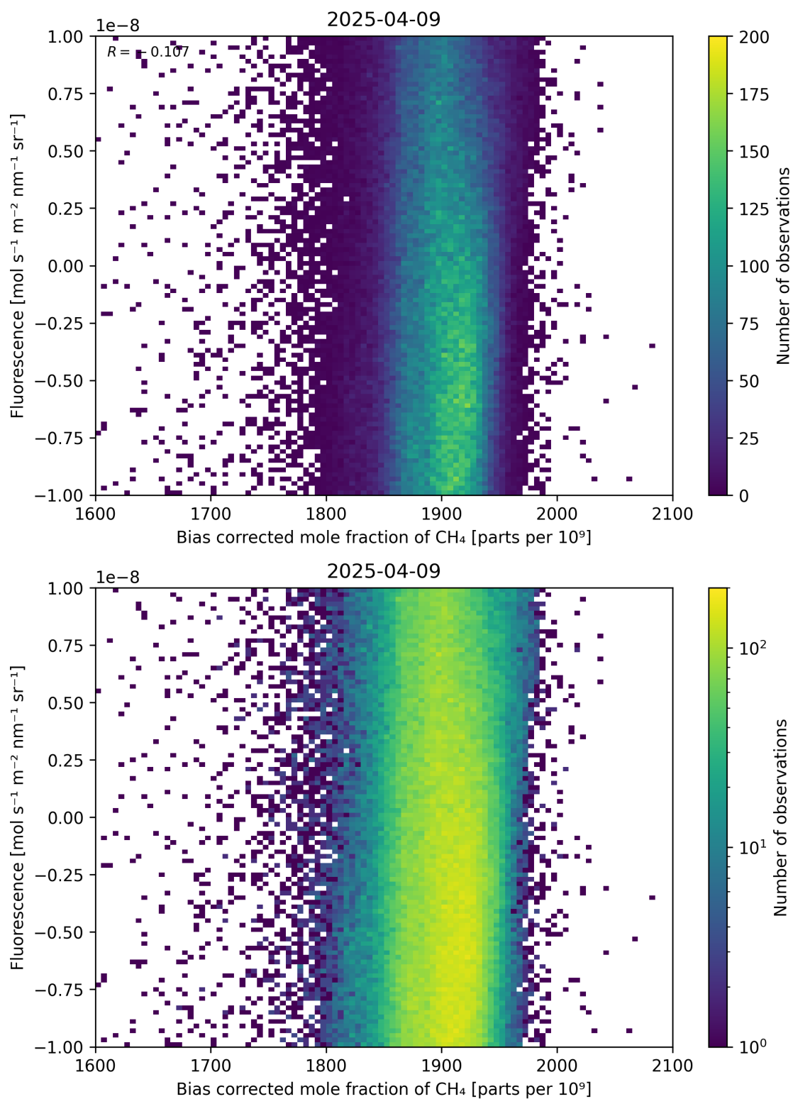
Figure 66: Scatter density plot of “Bias corrected mole fraction of \text{CH}_4 ” against “Fluorescence” for 2025-04-08 to 2025-04-10.
