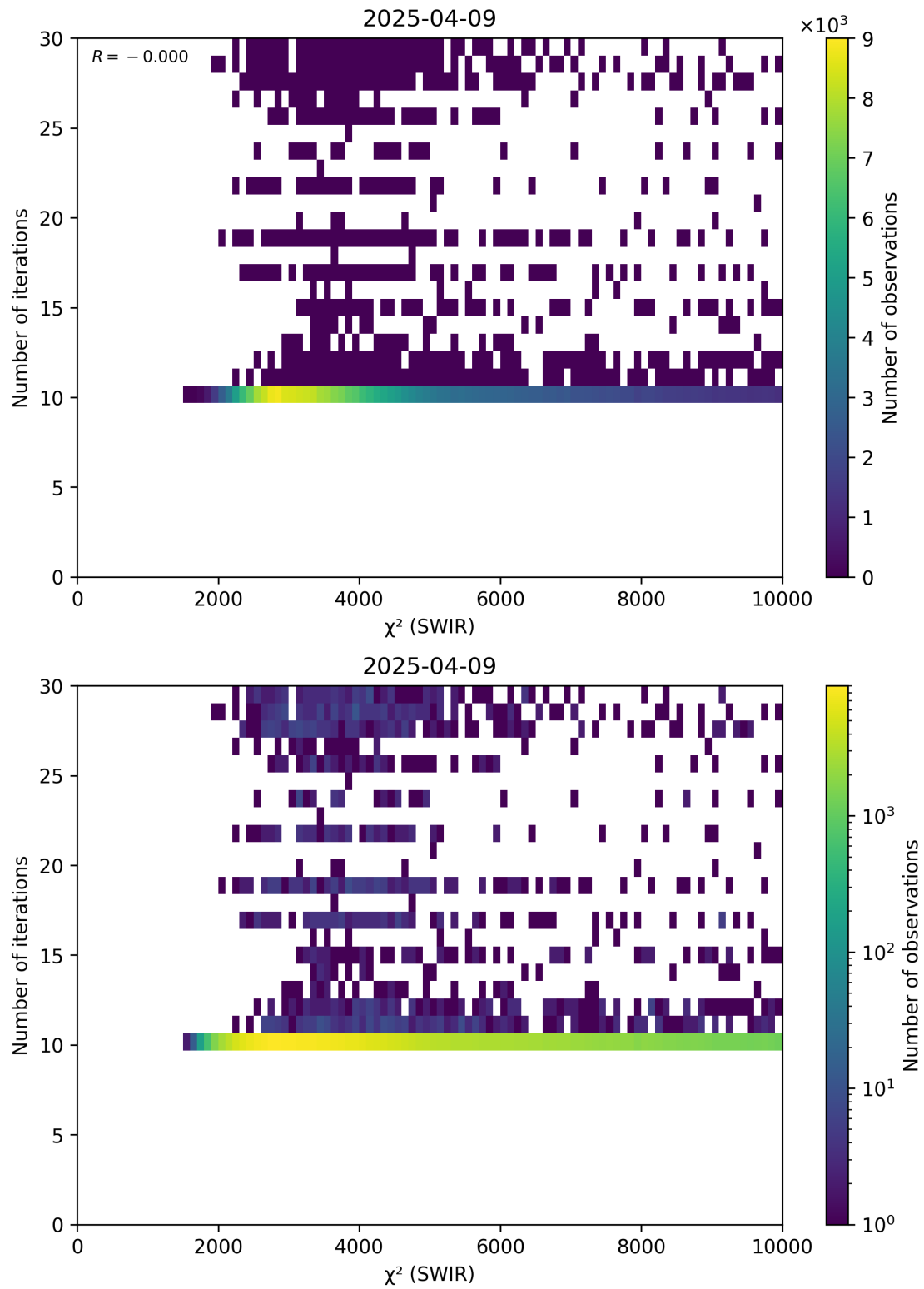
Figure 50: Scatter density plot of “ \chi^2 (SWIR)” against “Number of iterations” for 2025-04-08 to 2025-04-10.
