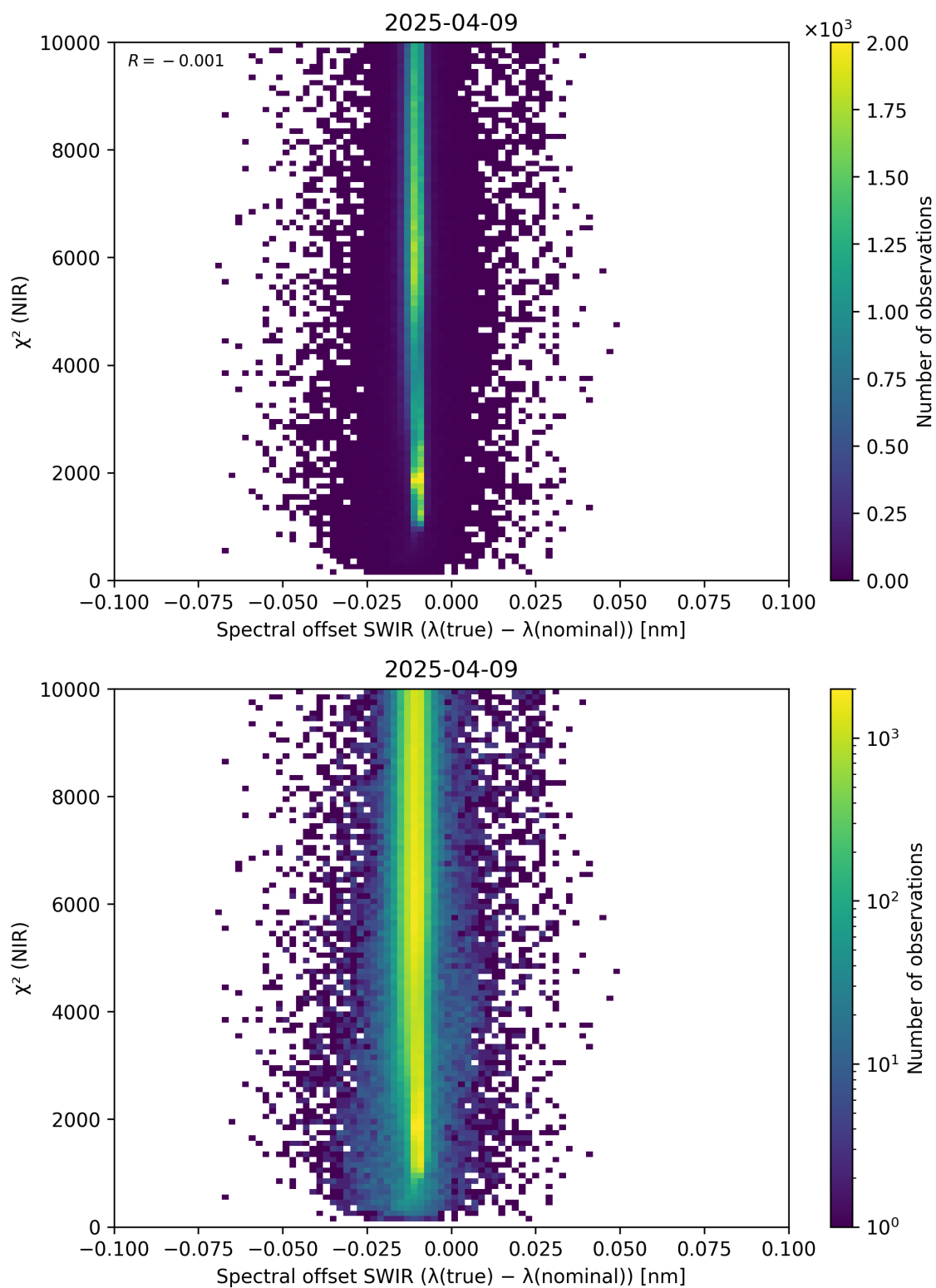
Figure 117: Scatter density plot of “Spectral offset SWIR ( \lambda_{\text{true}} - \lambda_{\text{nominal}} )” against “ \chi^2 (NIR)” for 2025-04-08 to 2025-04-10.
