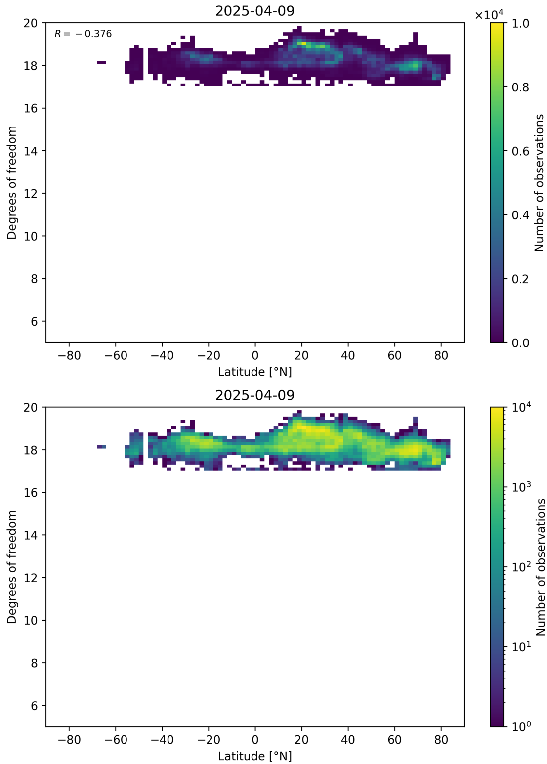
Figure 55: Scatter density plot of “Latitude” against “Degrees of freedom” for 2025-04-08 to 2025-04-10.
