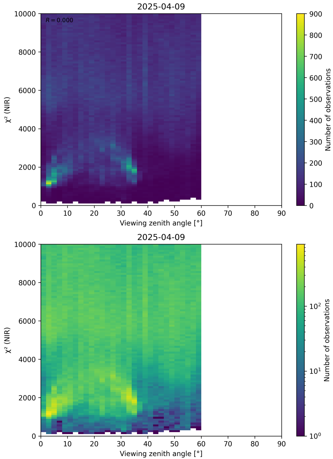
Figure 105: Scatter density plot of “Viewing zenith angle” against “ \chi^2 (NIR)” for 2025-04-08 to 2025-04-10.
