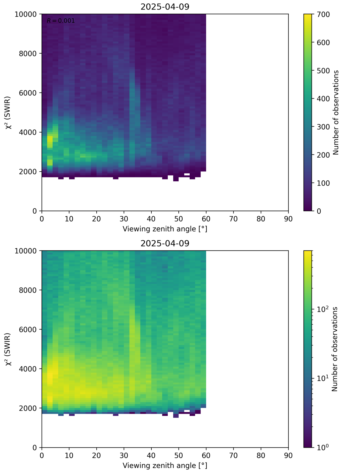
Figure 106: Scatter density plot of “Viewing zenith angle” against “ \chi^2 (SWIR)” for 2025-04-08 to 2025-04-10.
