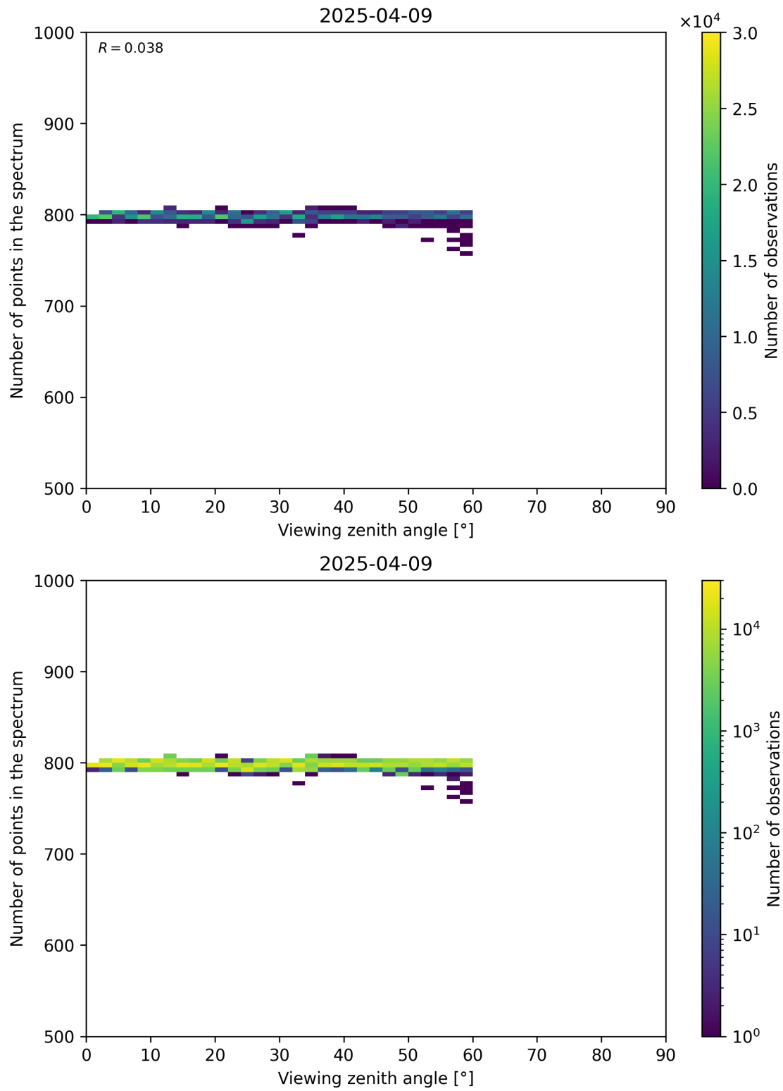
Figure 114: Scatter density plot of “Viewing zenith angle” against “Number of points in the spectrum” for 2025-04-08 to 2025-04-10.
