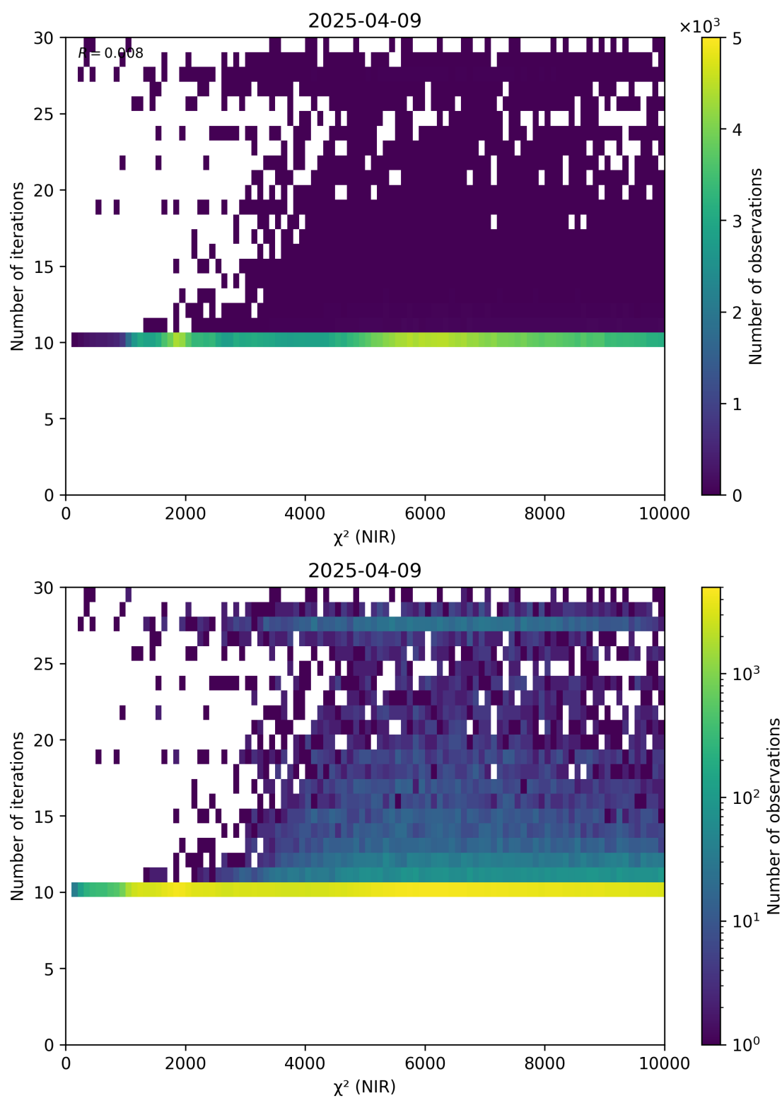
Figure 46: Scatter density plot of “ \chi^2 (NIR)” against “Number of iterations” for 2025-04-08 to 2025-04-10.
