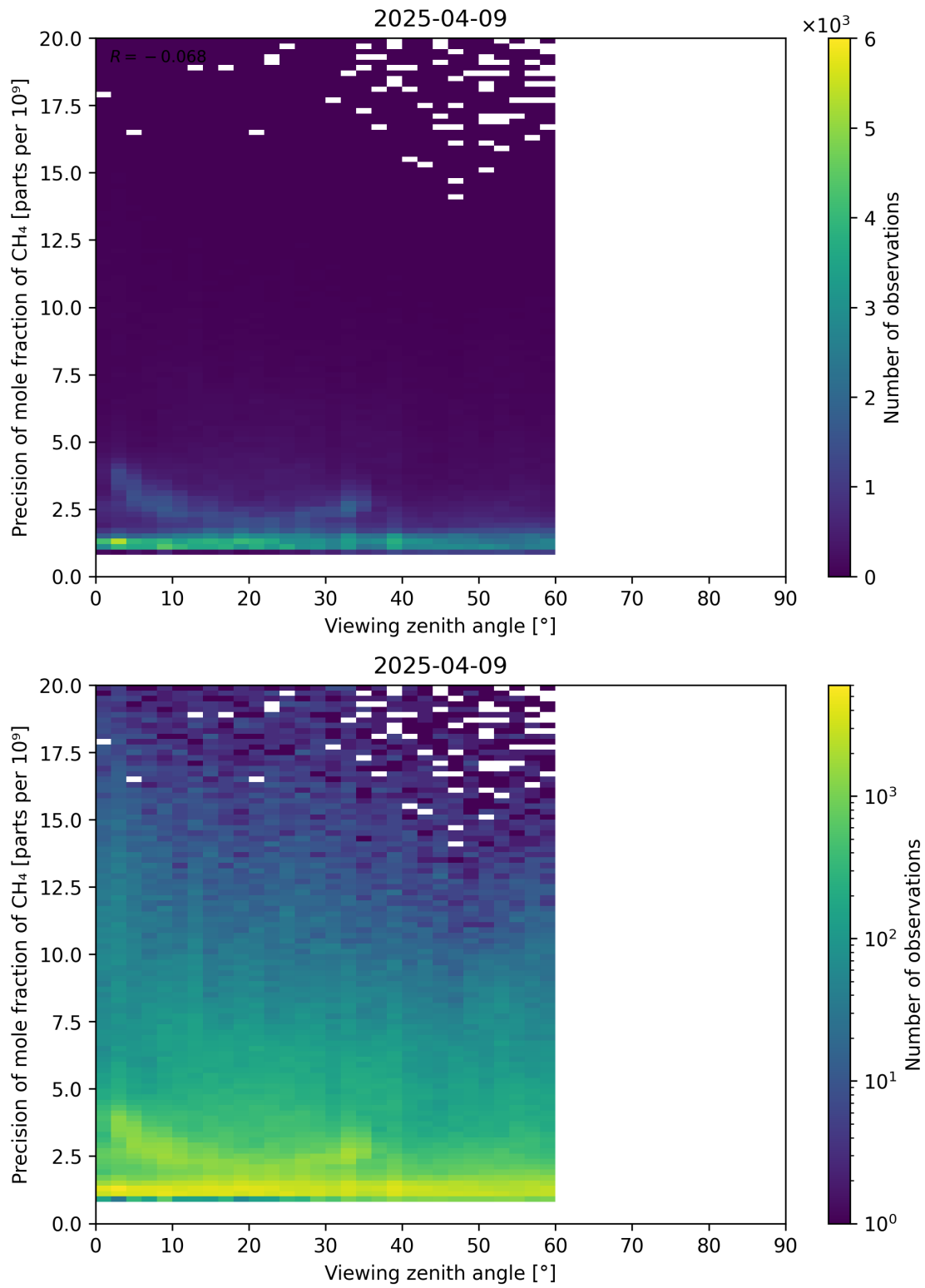
Figure 112: Scatter density plot of “Viewing zenith angle” against “Precision of mole fraction of CH 4 ” for 2025-04-08 to 2025-04-10.
