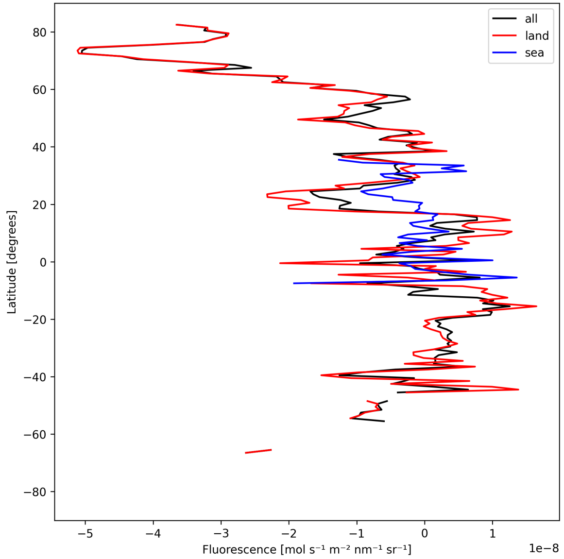
Figure 21: Zonal average of “Fluorescence” for 2025-04-08 to 2025-04-10.
