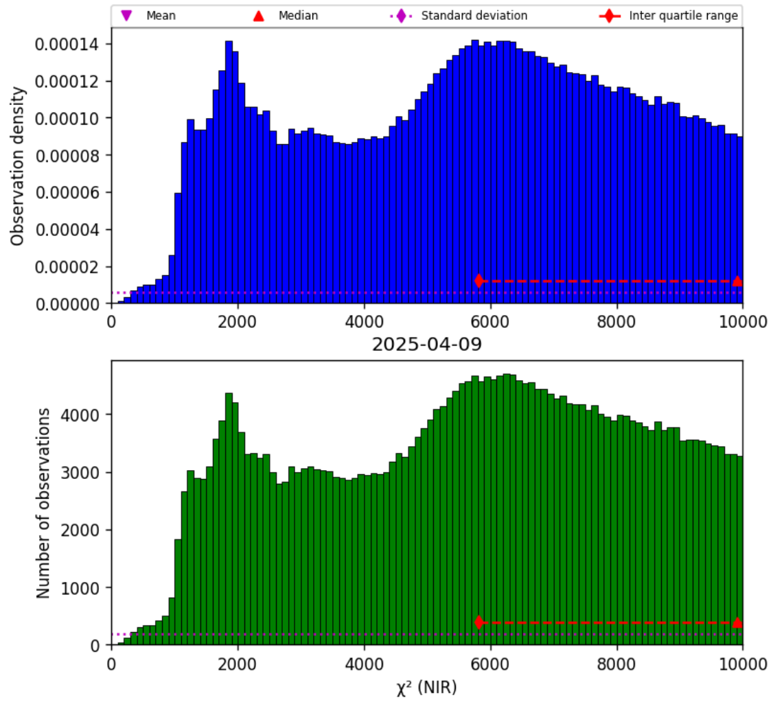
Figure 29: Histogram of " \chi^2 (NIR)" for 2025-04-08 to 2025-04-10
