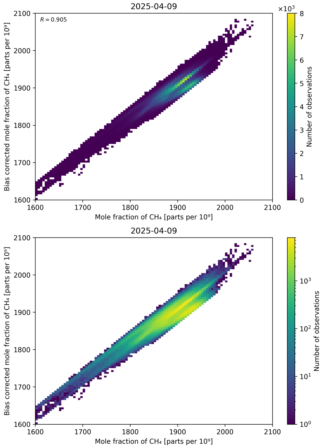
Figure 74: Scatter density plot of “Mole fraction of CH 4 ” against “Bias corrected mole fraction of CH 4 ” for 2025-04-08 to 2025-04-10.
