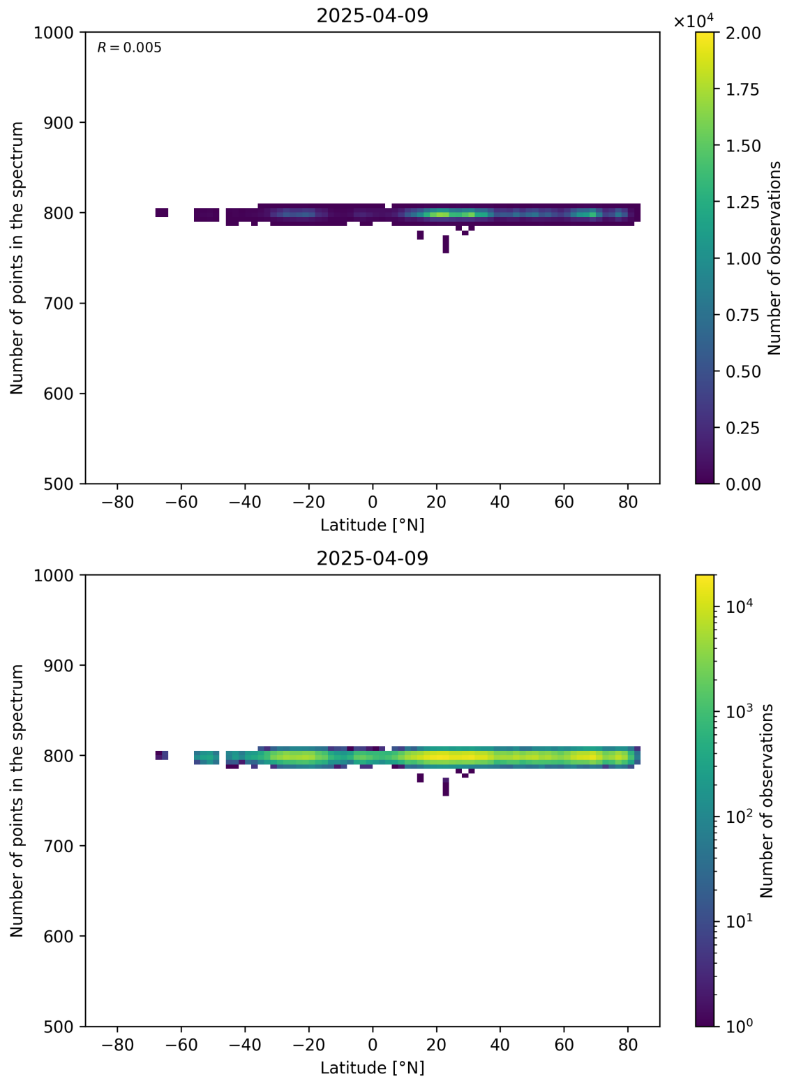
Figure 61: Scatter density plot of “Latitude” against “Number of points in the spectrum” for 2025-04-08 to 2025-04-10.
