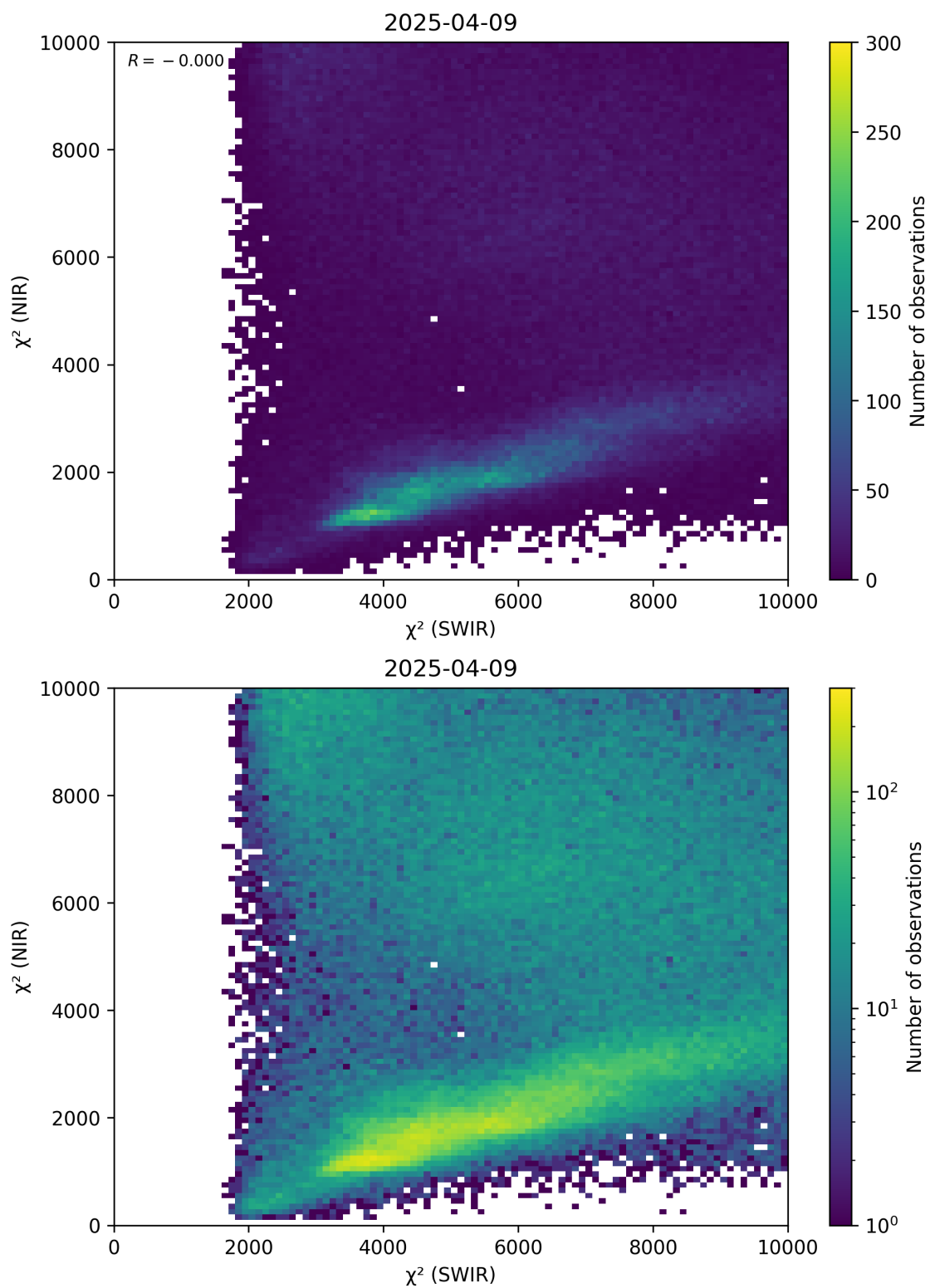
Figure 47: Scatter density plot of “ \chi^2 (SWIR)” against “ \chi^2 (NIR)” for 2025-04-08 to 2025-04-10.
