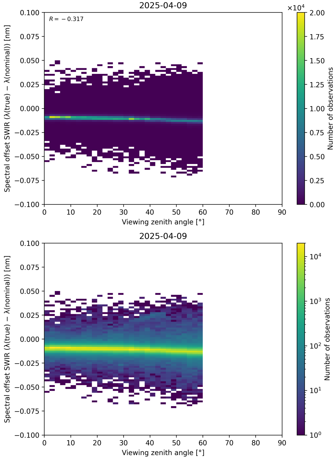
Figure 116: Scatter density plot of “Viewing zenith angle” against “Spectral offset SWIR ( \lambda_{\text{true}} - \lambda_{\text{nominal}} )” for 2025-04-08 to 2025-04-10.
