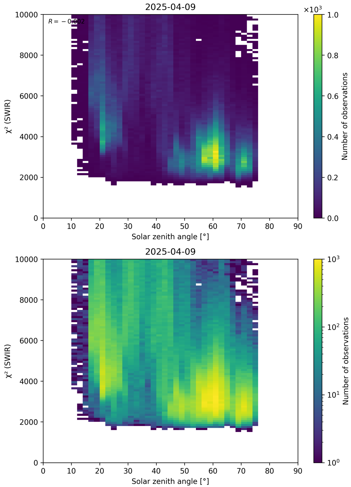
Figure 95: Scatter density plot of “Solar zenith angle” against “ \chi^2 (SWIR)” for 2025-04-08 to 2025-04-10.
