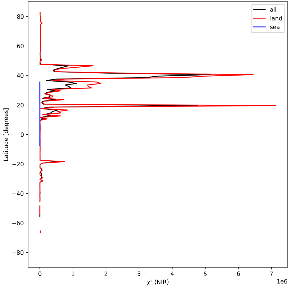
Figure 18: Zonal average of “ \chi^2 (NIR)” for 2025-04-08 to 2025-04-10.
