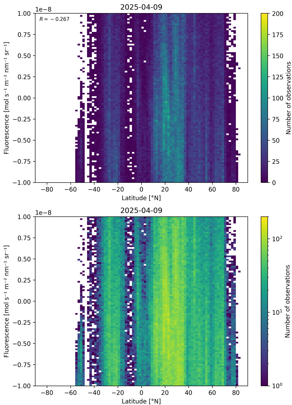
Figure 56: Scatter density plot of “Latitude” against “Fluorescence” for 2025-04-08 to 2025-04-10.
