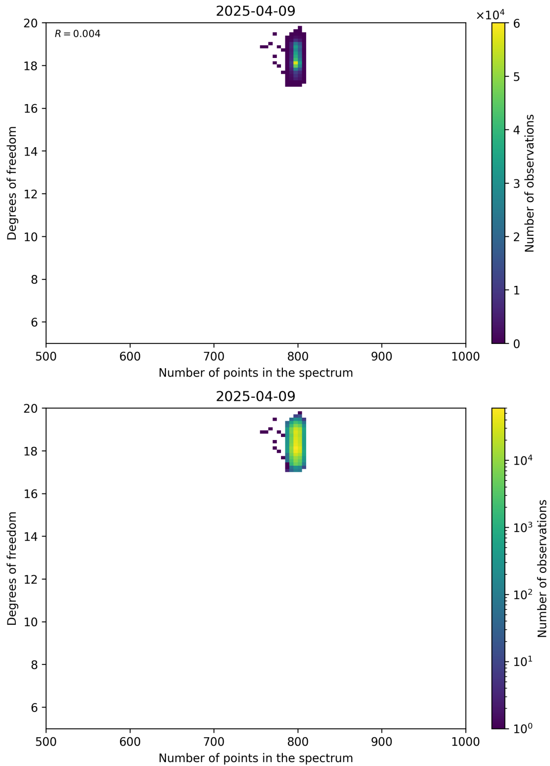
Figure 90: Scatter density plot of “Number of points in the spectrum” against “Degrees of freedom” for 2025-04-08 to 2025-04-10.
