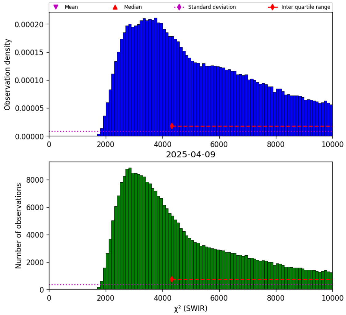
Figure 28: Histogram of “ \chi^2 (SWIR)” for 2025-04-08 to 2025-04-10
