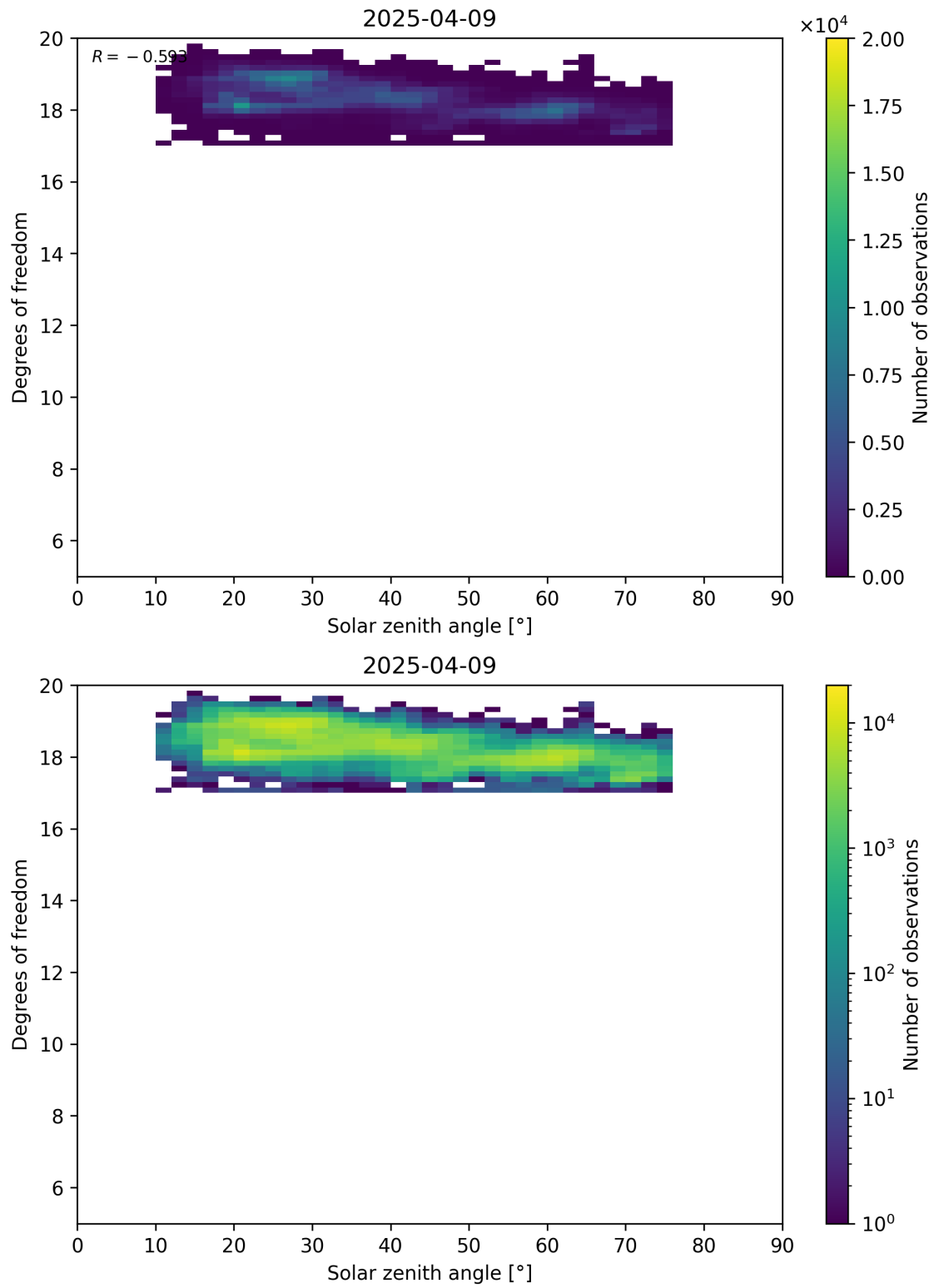
Figure 96: Scatter density plot of “Solar zenith angle” against “Degrees of freedom” for 2025-04-08 to 2025-04-10.
