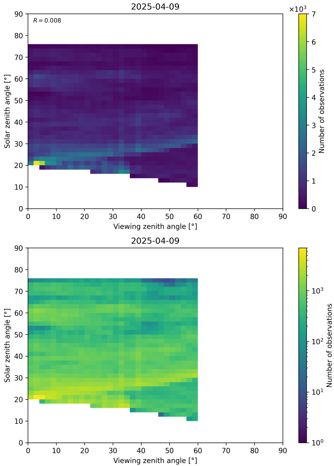
Figure 115: Scatter density plot of “Viewing zenith angle” against “Solar zenith angle” for 2025-04-08 to 2025-04-10.
