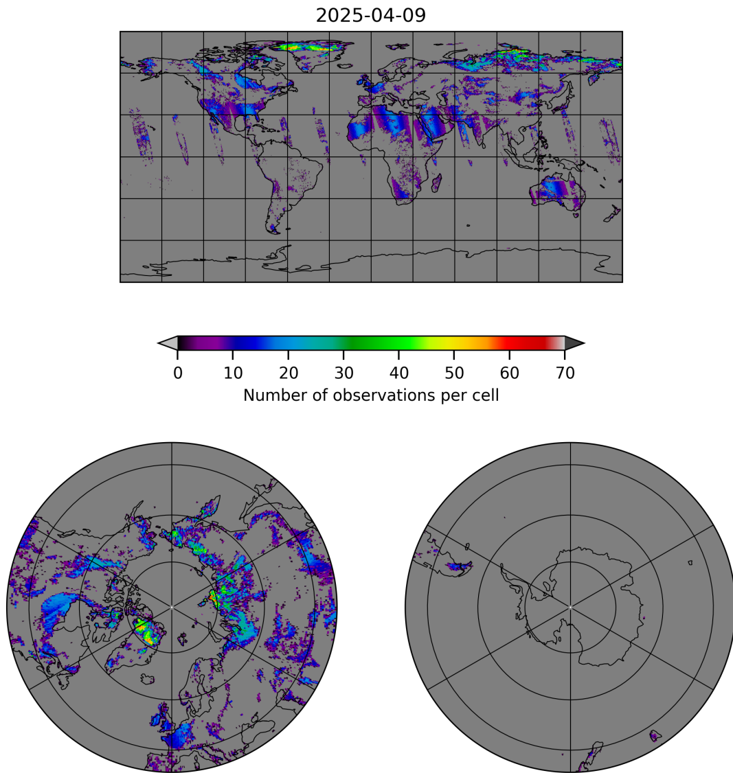
Figure 10: Map of the number of observations for 2025-04-08 to 2025-04-10
