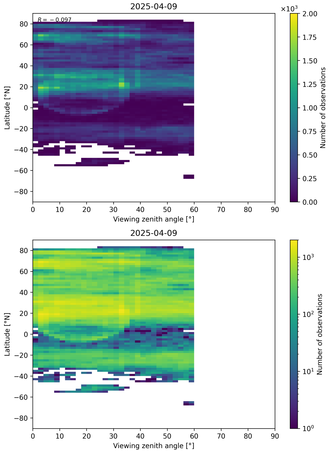
Figure 109: Scatter density plot of “Viewing zenith angle” against “Latitude” for 2025-04-08 to 2025-04-10.
