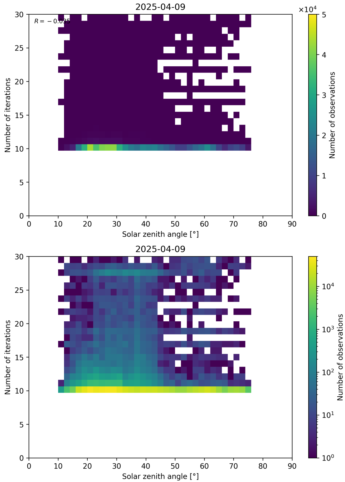
Figure 102: Scatter density plot of “Solar zenith angle” against “Number of iterations” for 2025-04-08 to 2025-04-10.
