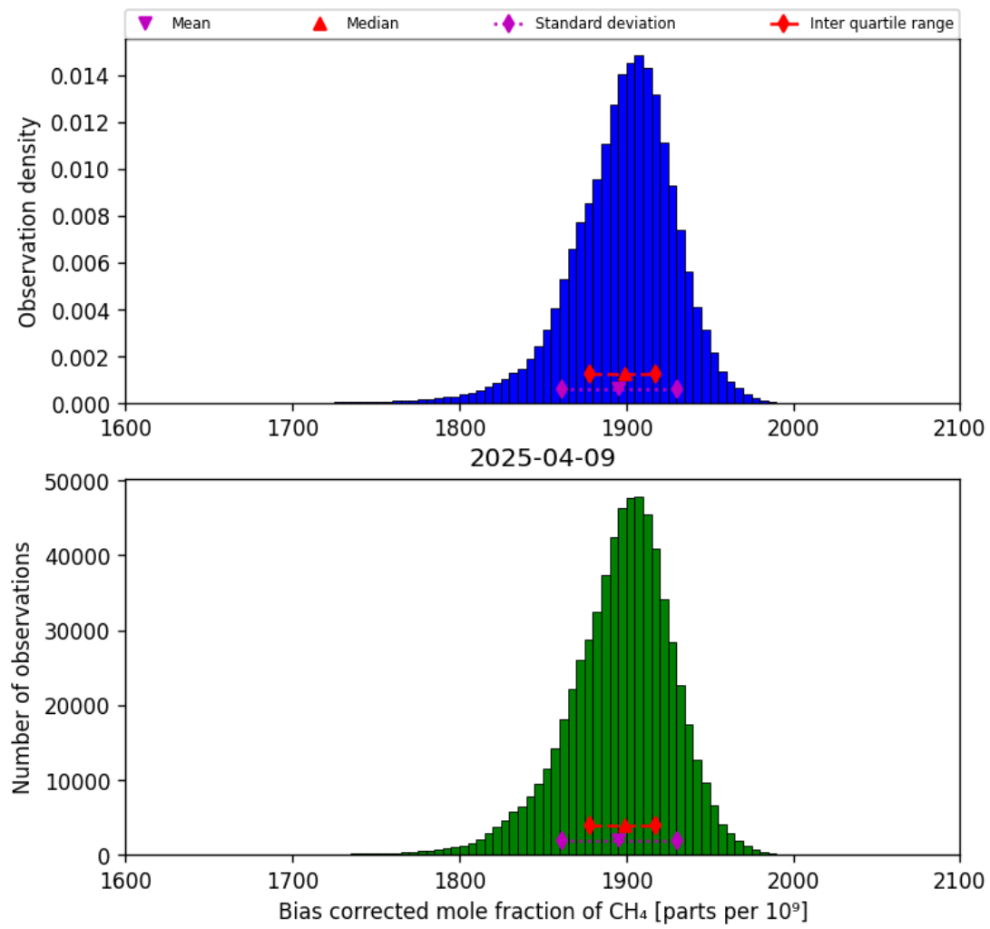
Figure 25: Histogram of “Bias corrected mole fraction of CH 4 ” for 2025-04-08 to 2025-04-10
