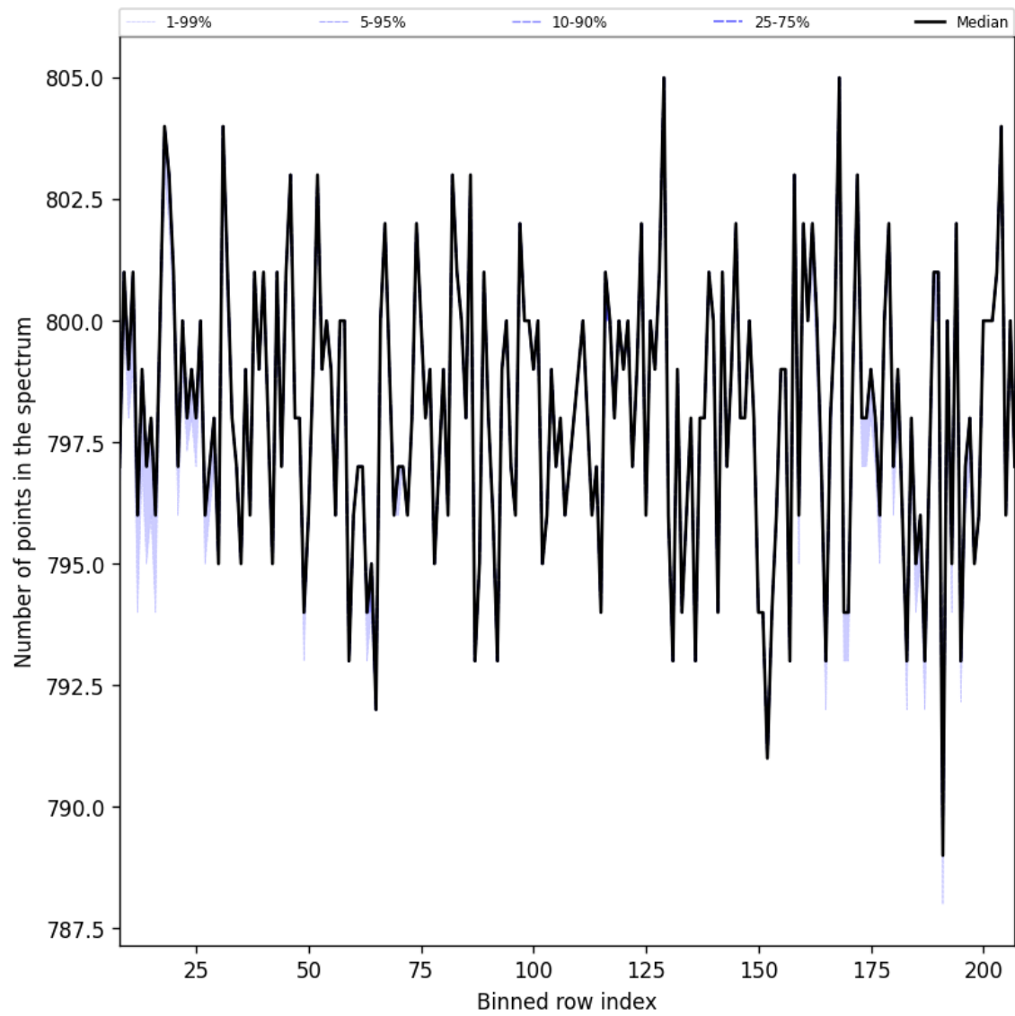
Figure 37: Along track statistics of “Number of points in the spectrum” for 2025-04-08 to 2025-04-10
