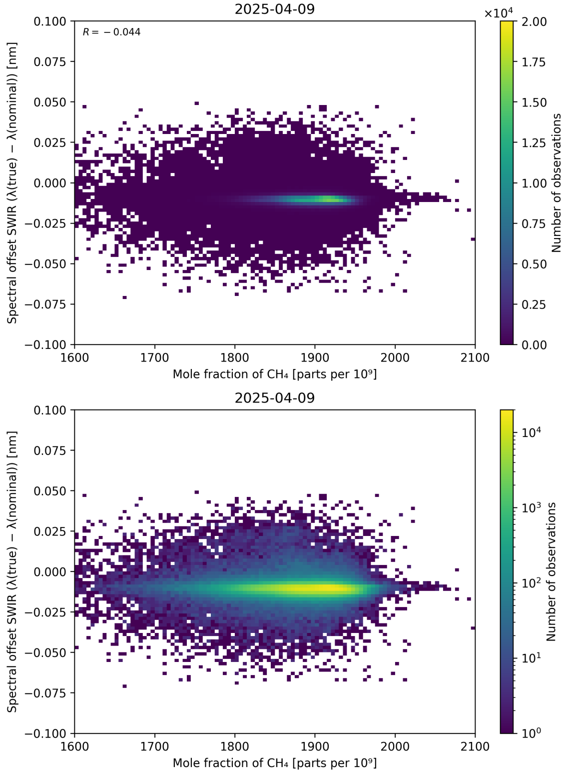
Figure 86: Scatter density plot of “Mole fraction of CH 4 ” against “Spectral offset SWIR ( \lambda_{\text{true}} - \lambda_{\text{nominal}} )” for 2025-04-08 to 2025-04-10.
