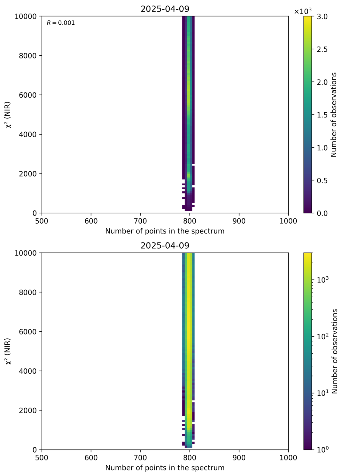
Figure 88: Scatter density plot of “Number of points in the spectrum” against “ \chi^2 (NIR)” for 2025-04-08 to 2025-04-10.
