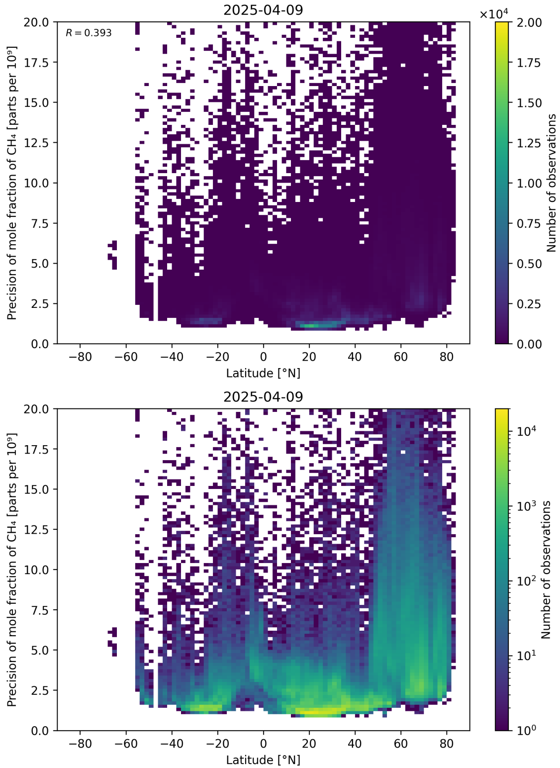
Figure 59: Scatter density plot of “Latitude” against “Precision of mole fraction of \text{CH}_4 ” for 2025-04-08 to 2025-04-10.
