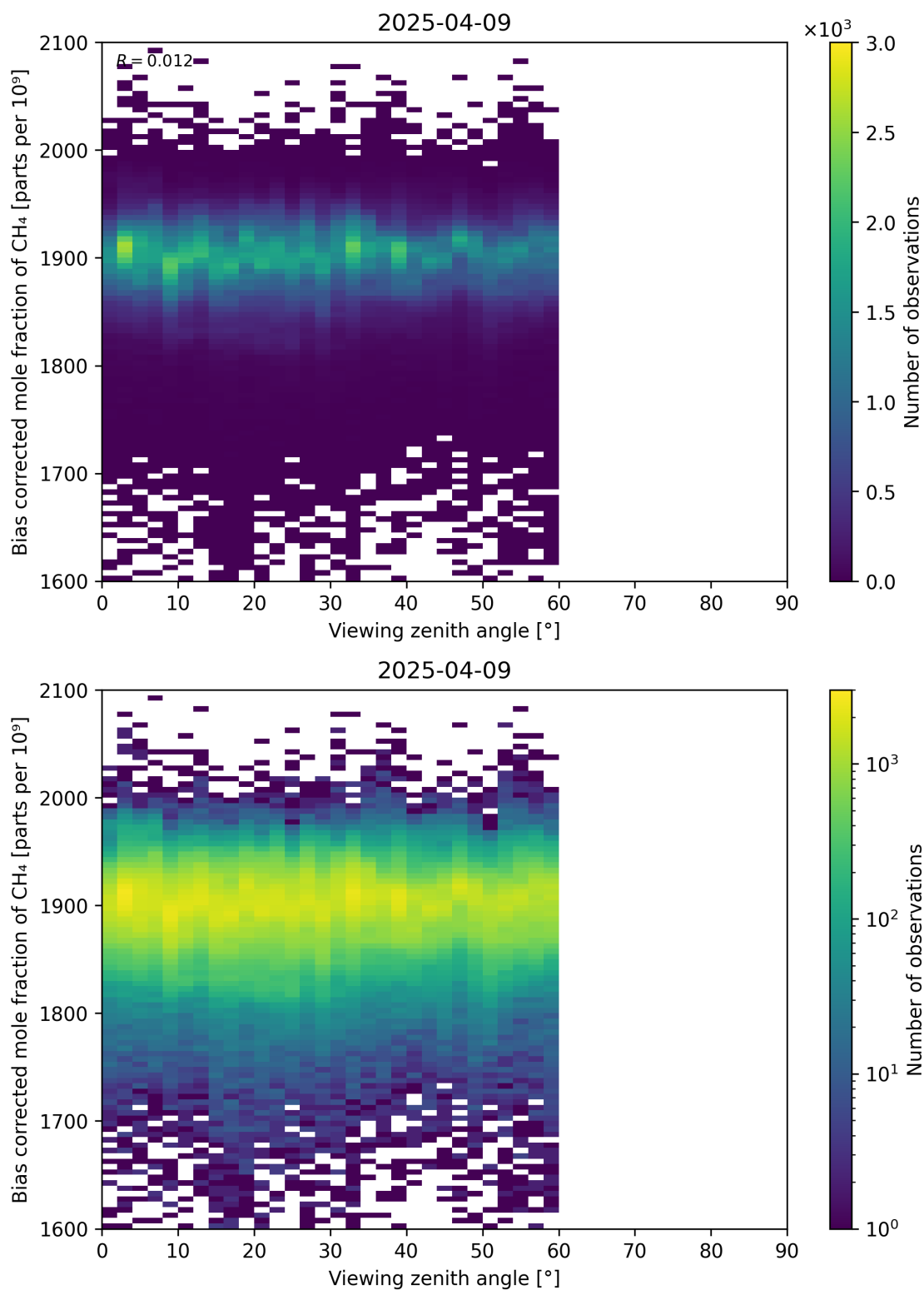
Figure 111: Scatter density plot of “Viewing zenith angle” against “Bias corrected mole fraction of CH 4 ” for 2025-04-08 to 2025-04-10.
