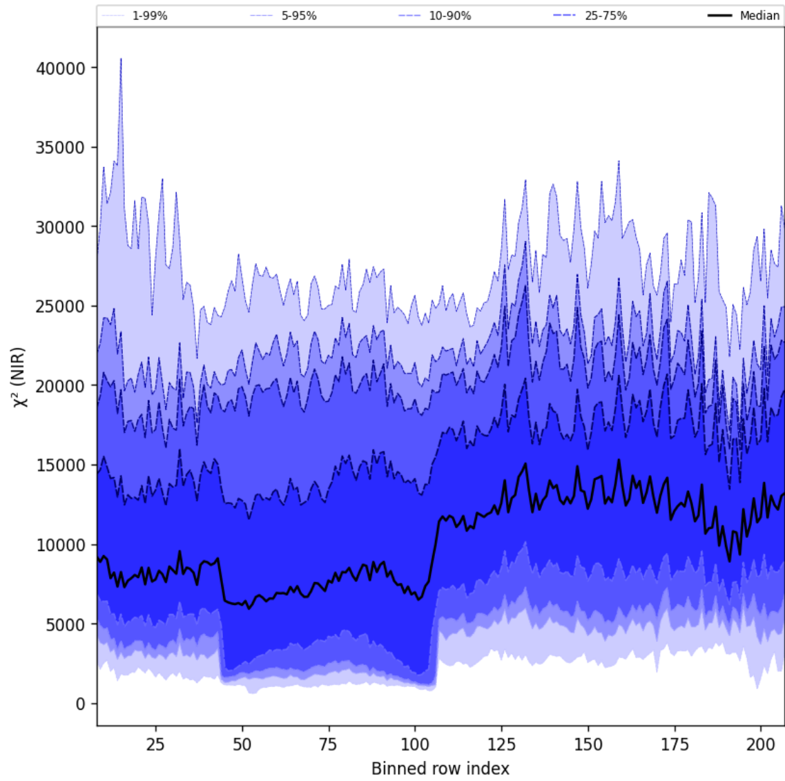
Figure 40: Along track statistics of “ \chi^2 (NIR)” for 2025-04-08 to 2025-04-10
