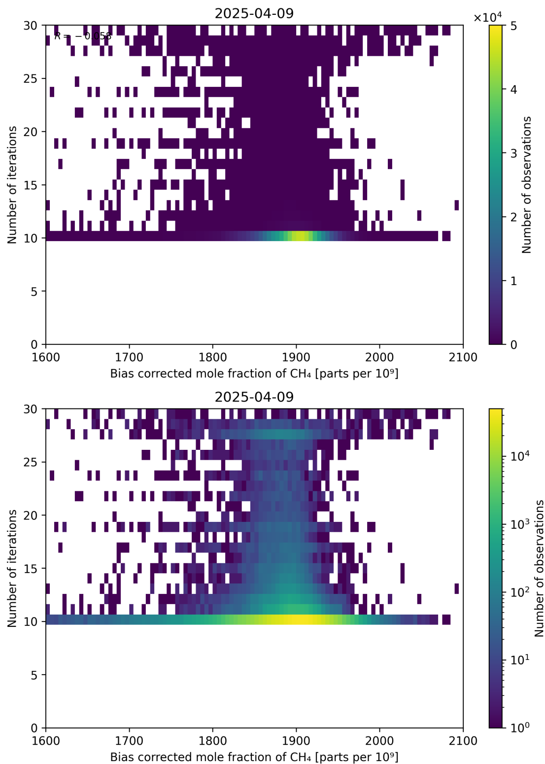
Figure 67: Scatter density plot of “Bias corrected mole fraction of CH 4 ” against “Number of iterations” for 2025-04-08 to 2025-04-10.
