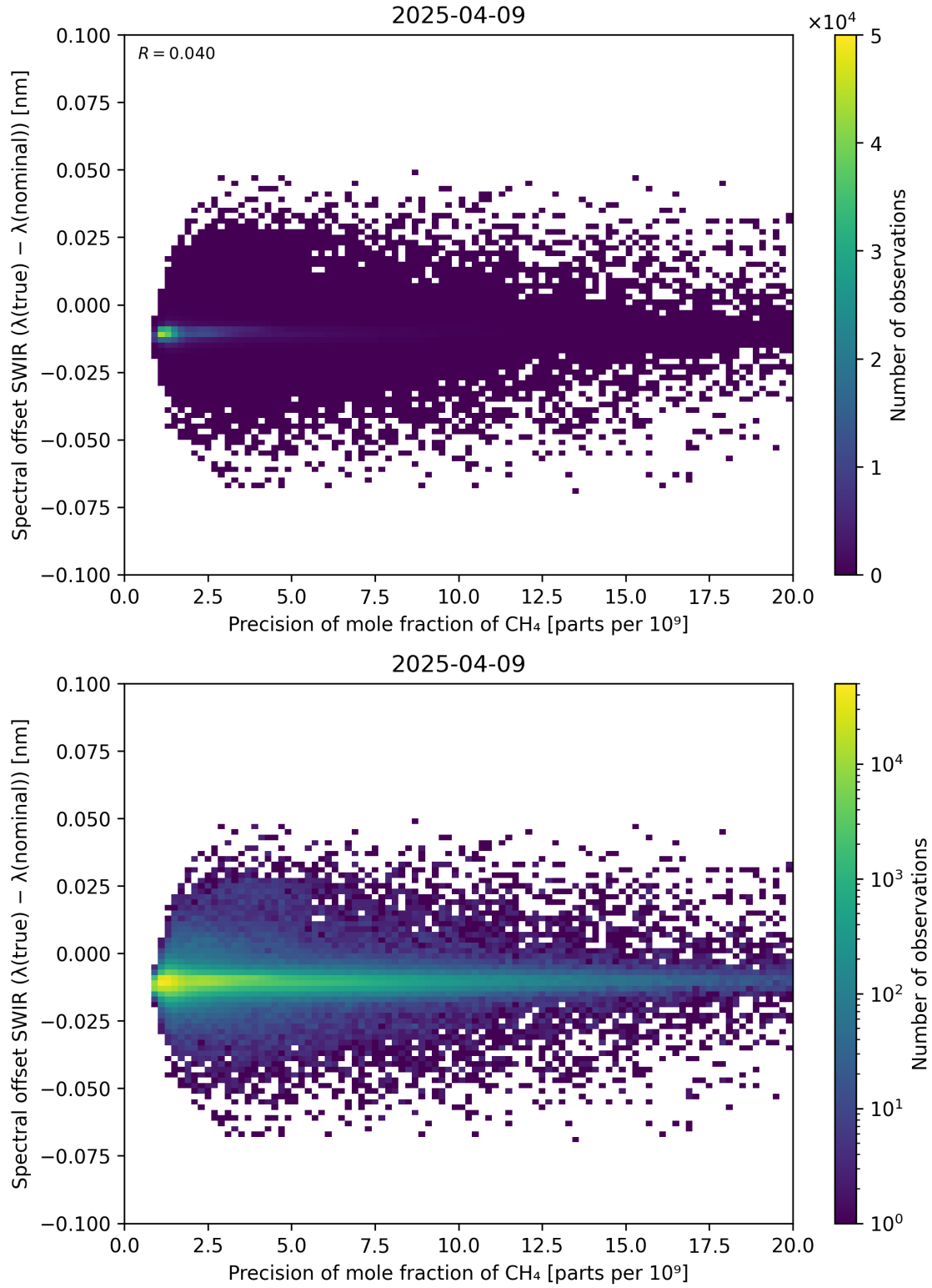
Figure 85: Scatter density plot of “Precision of mole fraction of CH 4 ” against “Spectral offset SWIR ( \lambda_{\text{true}} - \lambda_{\text{nominal}} )” for 2025-04-08 to 2025-04-10.
