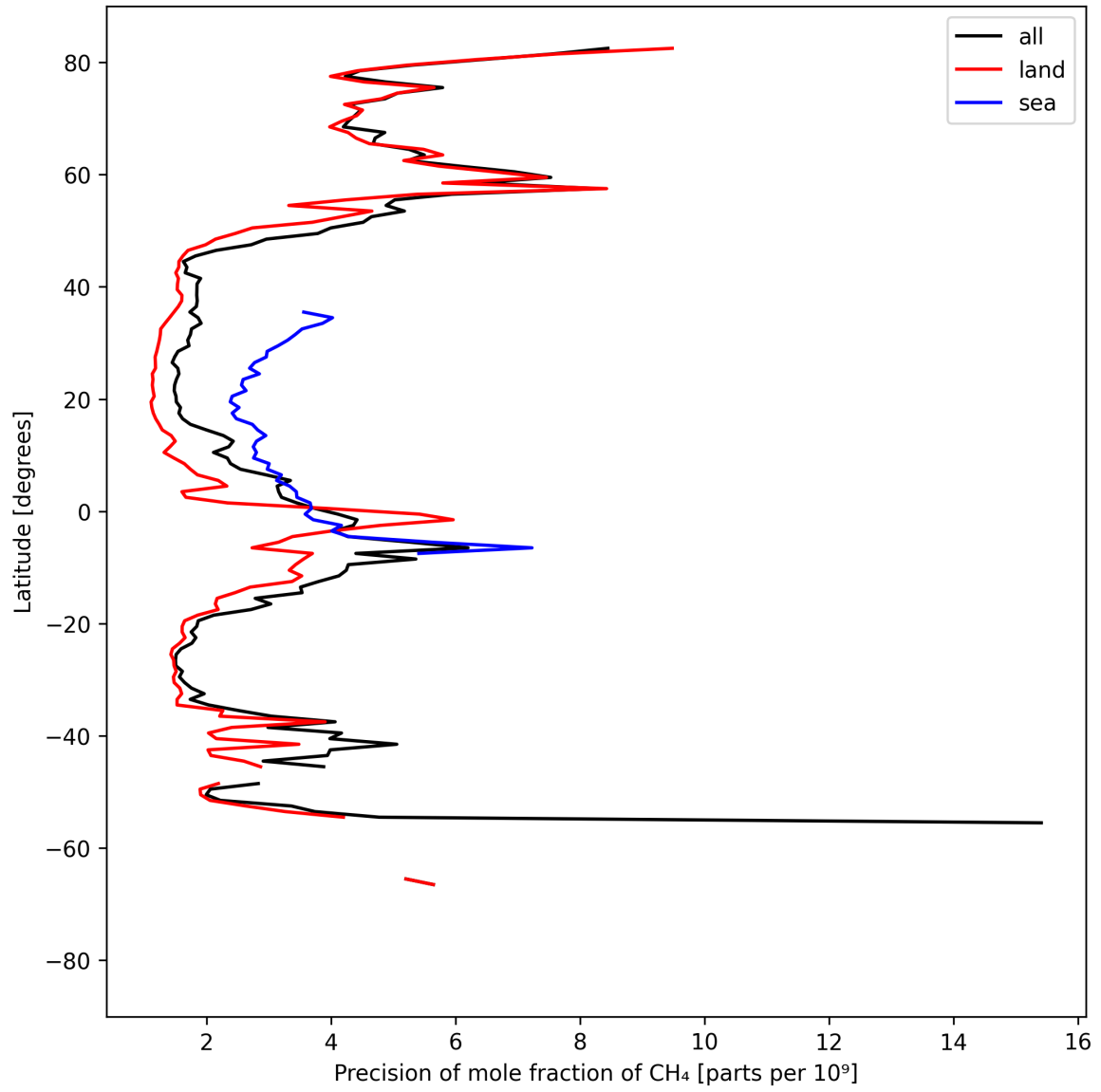
Figure 13: Zonal average of “Precision of mole fraction of CH 4 ” for 2025-04-08 to 2025-04-10.
