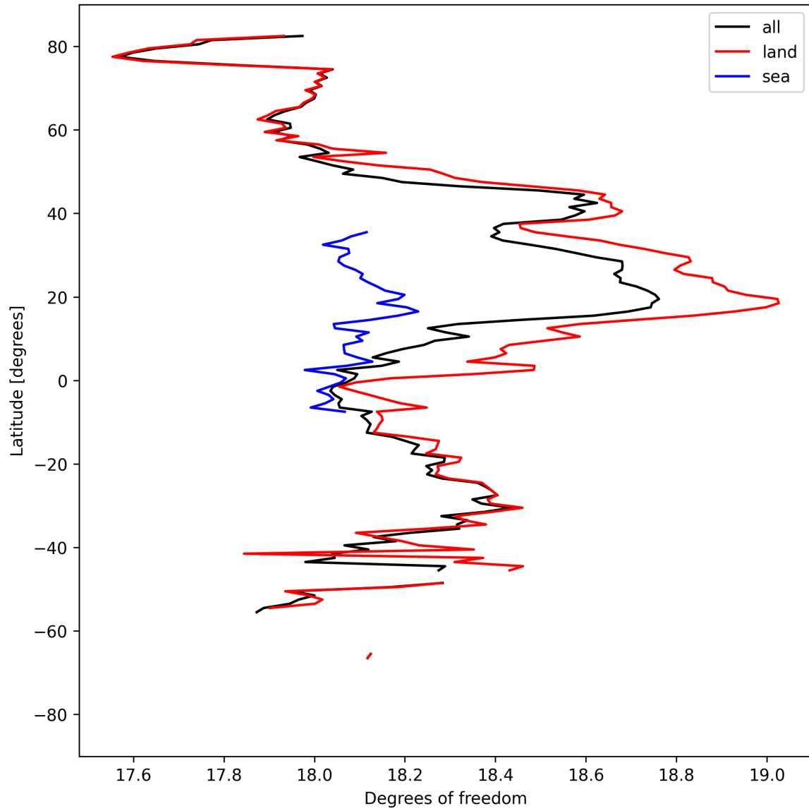
Figure 19: Zonal average of “Degrees of freedom” for 2025-04-08 to 2025-04-10.
