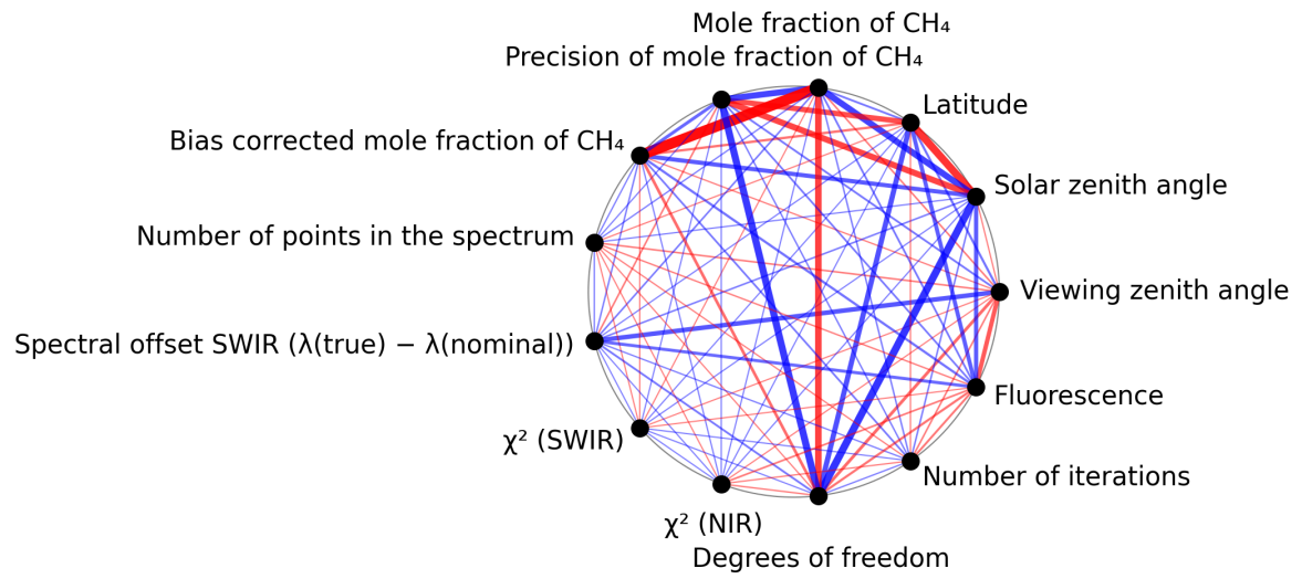
Figure 1: Map of correlation graph for 2025-04-08 to 2025-04-10.
