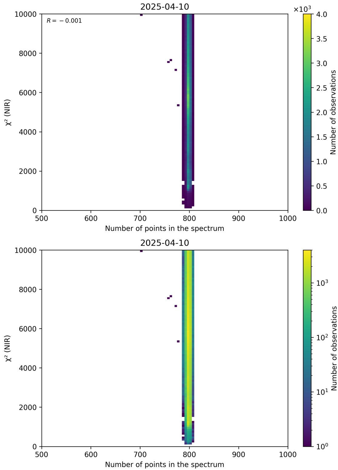
Figure 88: Scatter density plot of “Number of points in the spectrum” against “ \chi^2 (NIR)” for 2025-04-09 to 2025-04-11.
