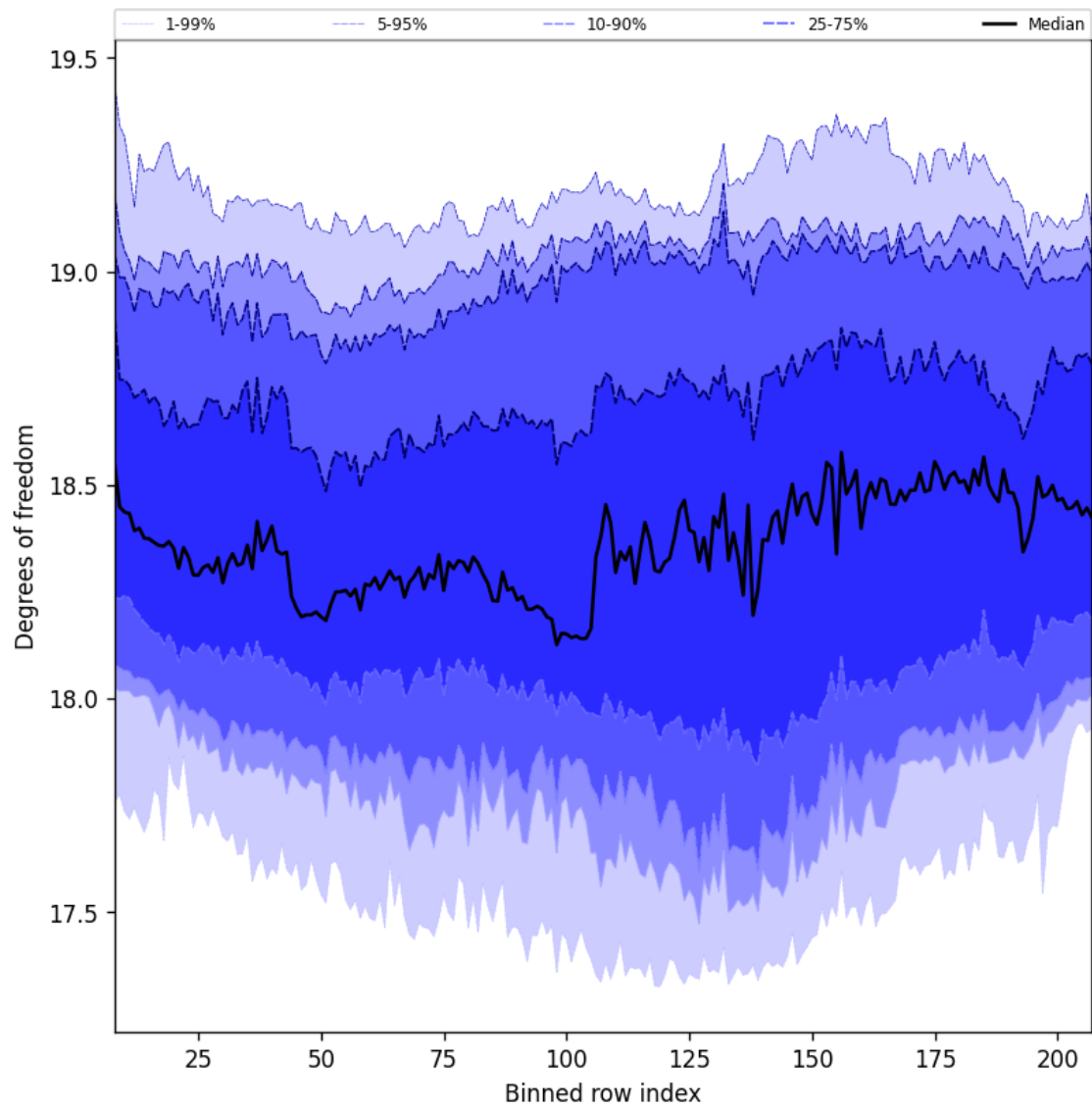
Figure 41: Along track statistics of “Degrees of freedom” for 2025-04-09 to 2025-04-11
