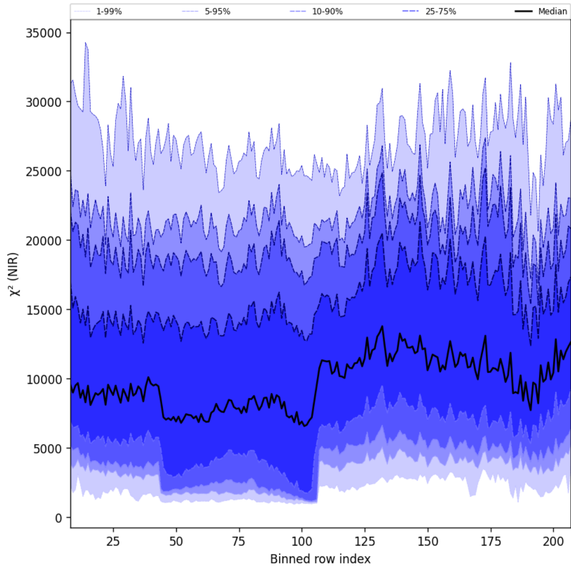
Figure 40: Along track statistics of “ \chi^2 (NIR)” for 2025-04-09 to 2025-04-11
