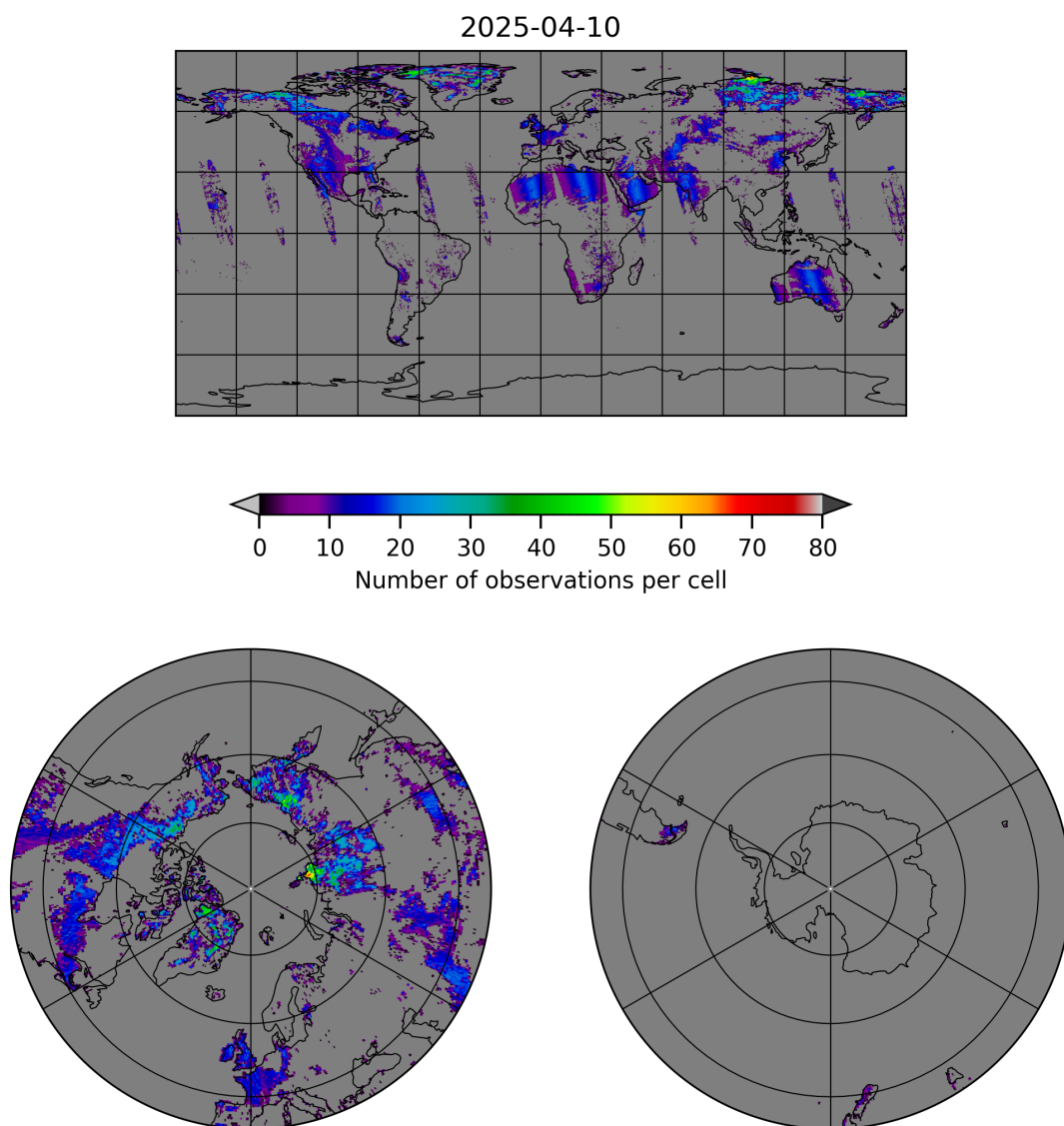
Figure 10: Map of the number of observations for 2025-04-09 to 2025-04-11
