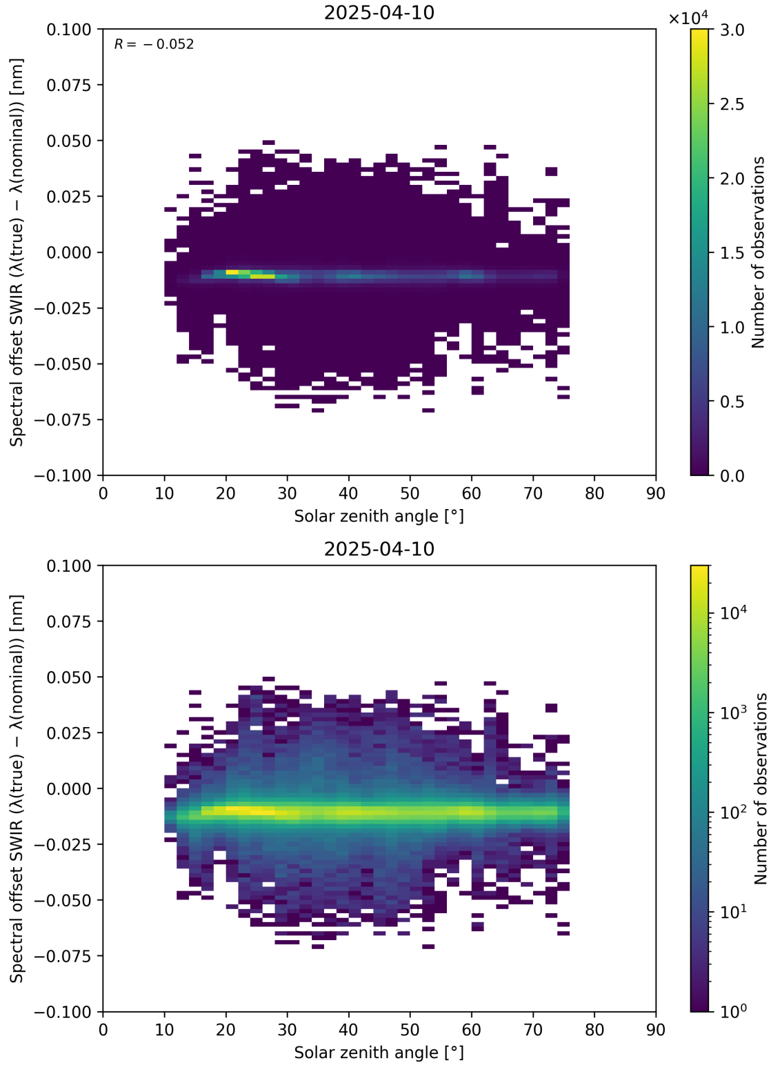
Figure 104: Scatter density plot of “Solar zenith angle” against “Spectral offset SWIR ( \lambda_{\text{true}} - \lambda_{\text{nominal}} )” for 2025-04-09 to 2025-04-11.
