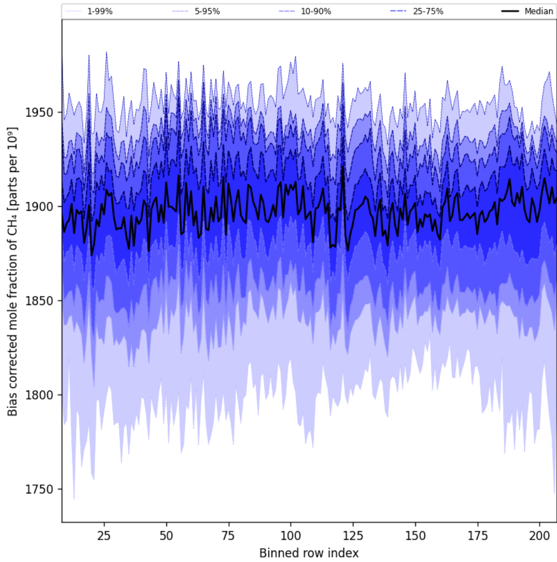
Figure 36: Along track statistics of “Bias corrected mole fraction of CH 4 ” for 2025-04-09 to 2025-04-11
