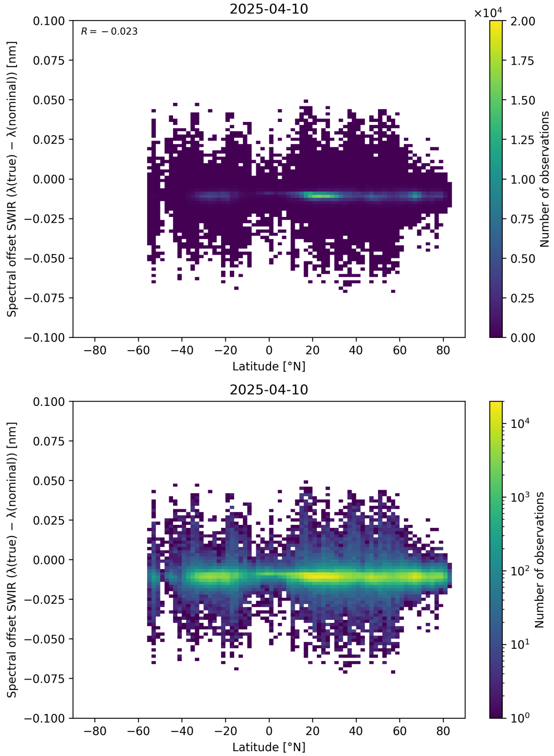
Figure 62: Scatter density plot of “Latitude” against “Spectral offset SWIR ( \lambda_{\text{true}} - \lambda_{\text{nominal}} )” for 2025-04-09 to 2025-04-11.
