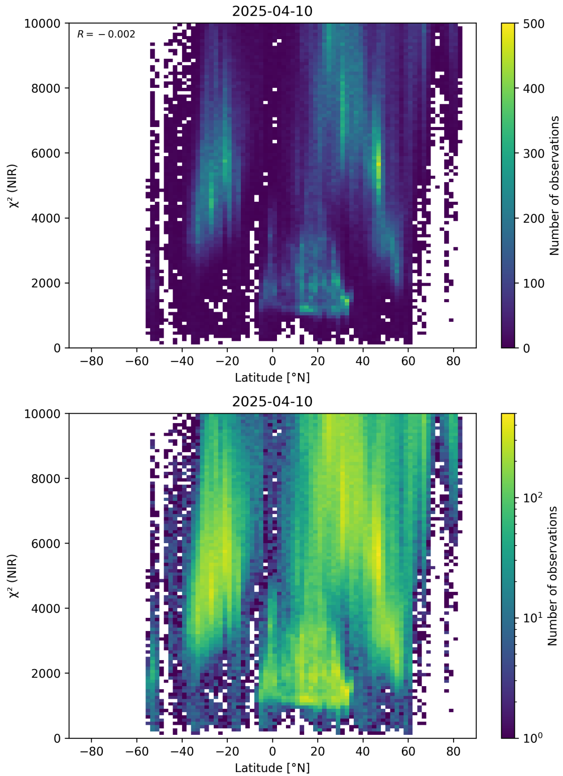
Figure 53: Scatter density plot of “Latitude” against “ \chi^2 (NIR)” for 2025-04-09 to 2025-04-11.
