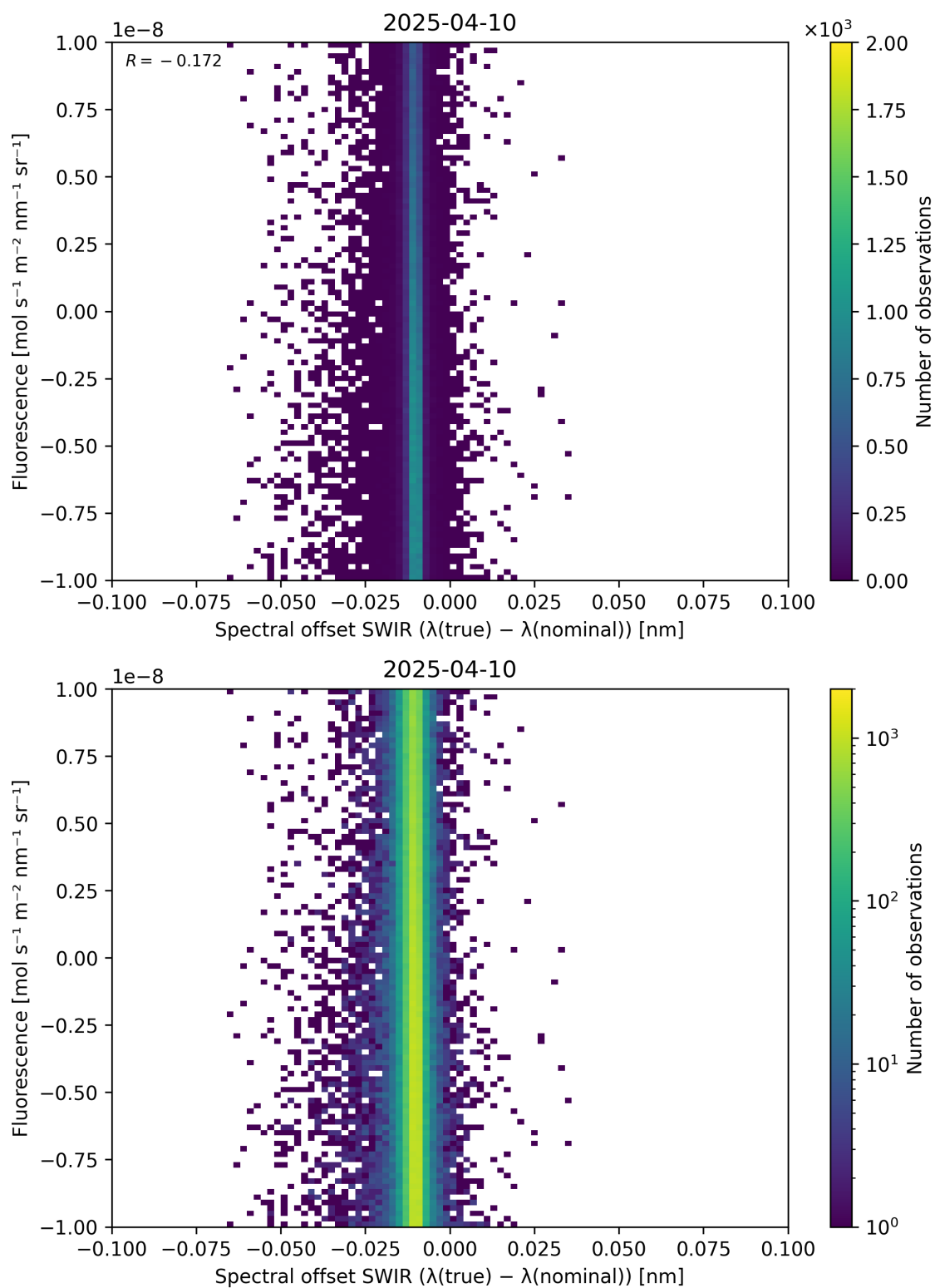
Figure 120: Scatter density plot of “Spectral offset SWIR ( \lambda_{\text{true}} - \lambda_{\text{nominal}} )” against “Fluorescence” for 2025-04-09 to 2025-04-11.
