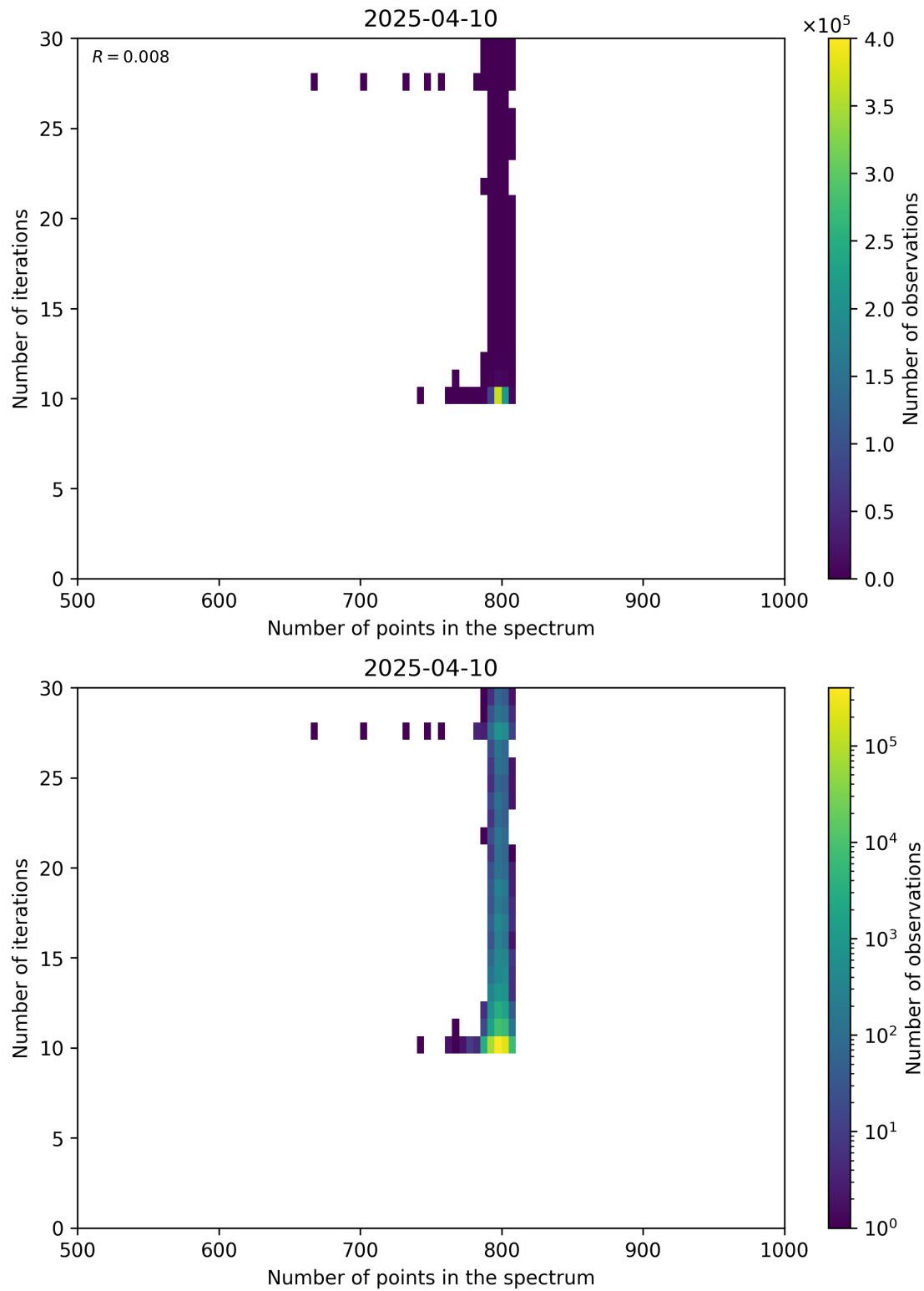
Figure 92: Scatter density plot of “Number of points in the spectrum” against “Number of iterations” for 2025-04-09 to 2025-04-11.
