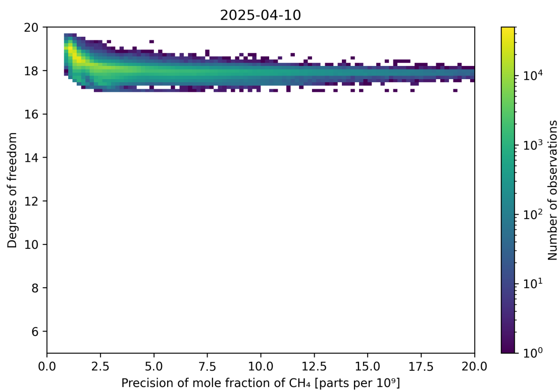
Figure 80: Scatter density plot of “Precision of mole fraction of CH 4 ” against “Degrees of freedom” for 2025-04-09 to 2025-04-11.
