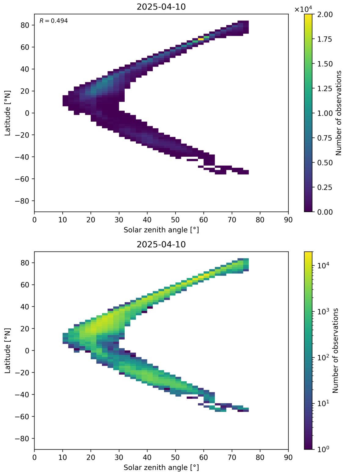
Figure 98: Scatter density plot of “Solar zenith angle” against “Latitude” for 2025-04-09 to 2025-04-11.
