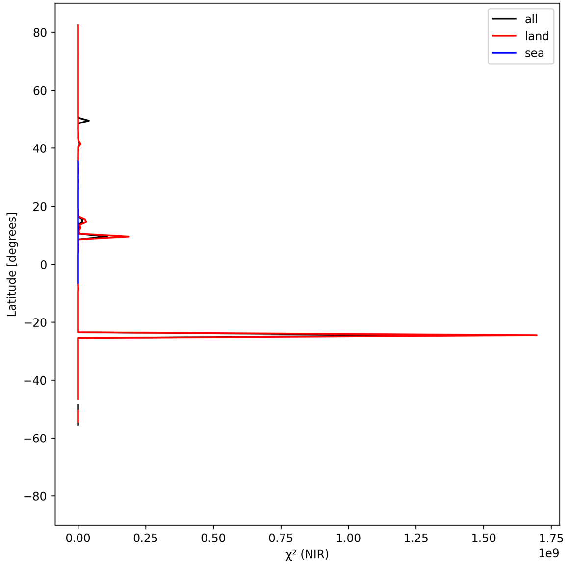
Figure 18: Zonal average of “ \chi^2 (NIR)” for 2025-04-09 to 2025-04-11.
