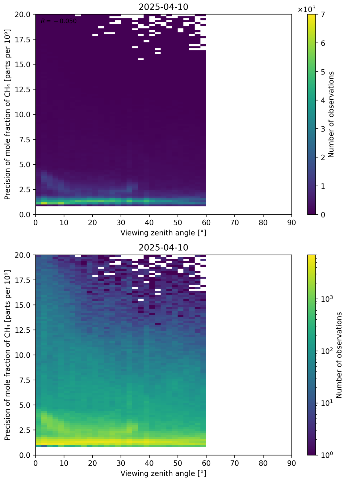
Figure 112: Scatter density plot of “Viewing zenith angle” against “Precision of mole fraction of CH 4 ” for 2025-04-09 to 2025-04-11.
