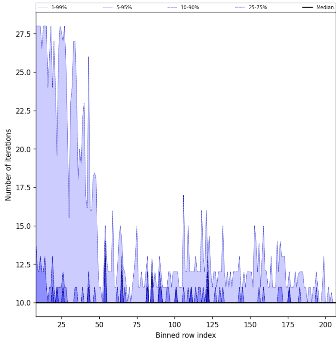
Figure 42: Along track statistics of “Number of iterations” for 2025-04-09 to 2025-04-11
