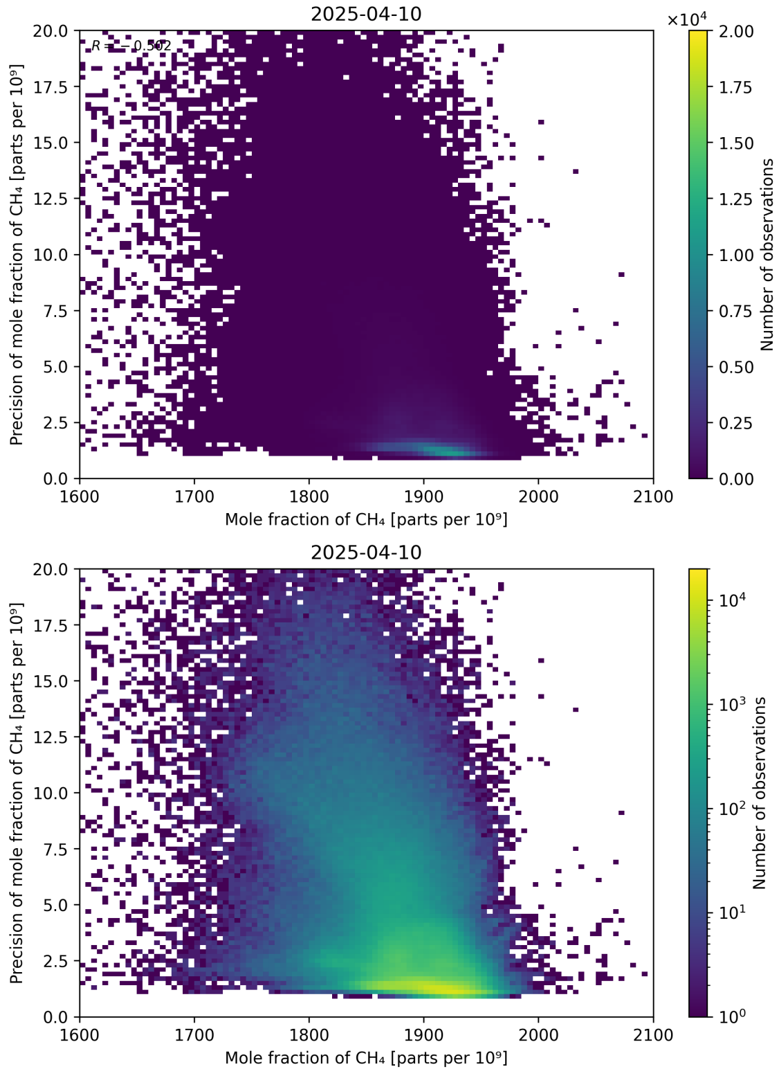
Figure 75: Scatter density plot of “Mole fraction of CH 4 ” against “Precision of mole fraction of CH 4 ” for 2025-04-09 to 2025-04-11.
