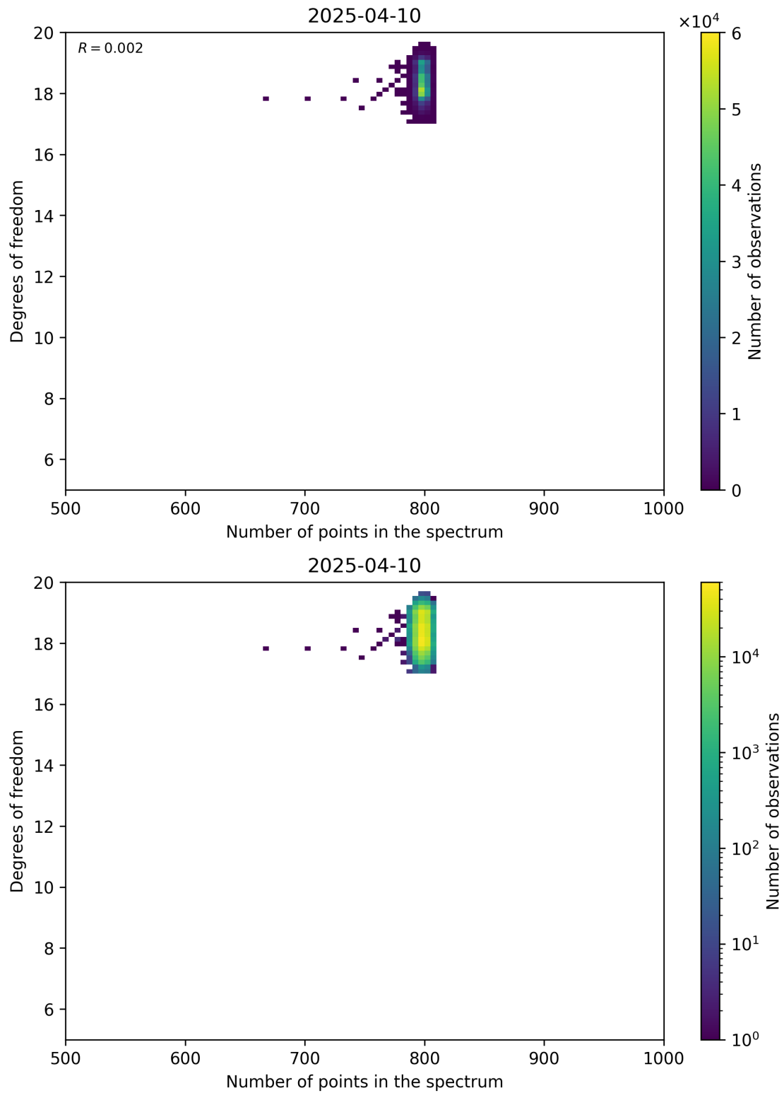
Figure 90: Scatter density plot of “Number of points in the spectrum” against “Degrees of freedom” for 2025-04-09 to 2025-04-11.
