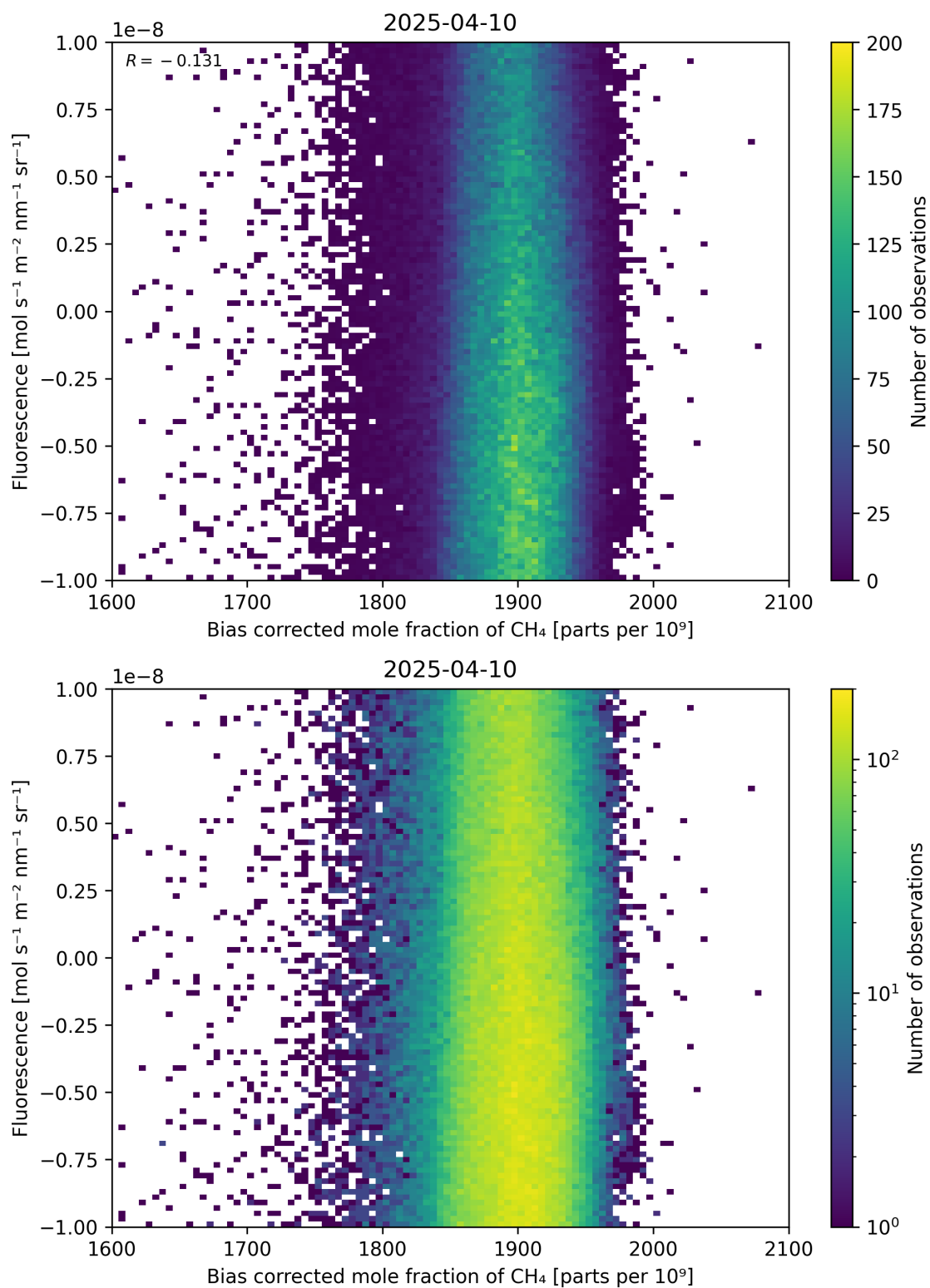
Figure 66: Scatter density plot of “Bias corrected mole fraction of \text{CH}_4 ” against “Fluorescence” for 2025-04-09 to 2025-04-11.
