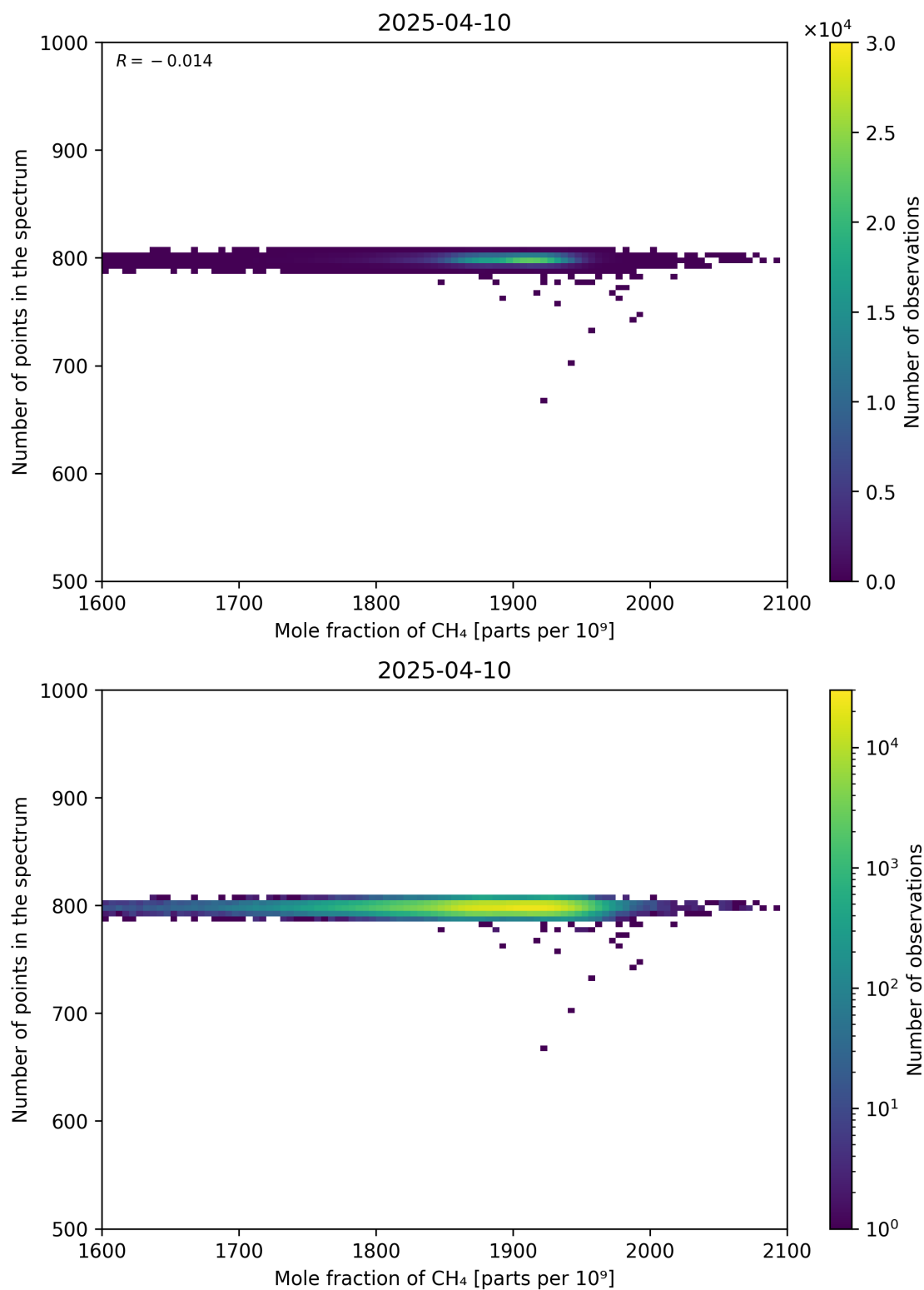
Figure 77: Scatter density plot of “Mole fraction of CH 4 ” against “Number of points in the spectrum” for 2025-04-09 to 2025-04-11.
