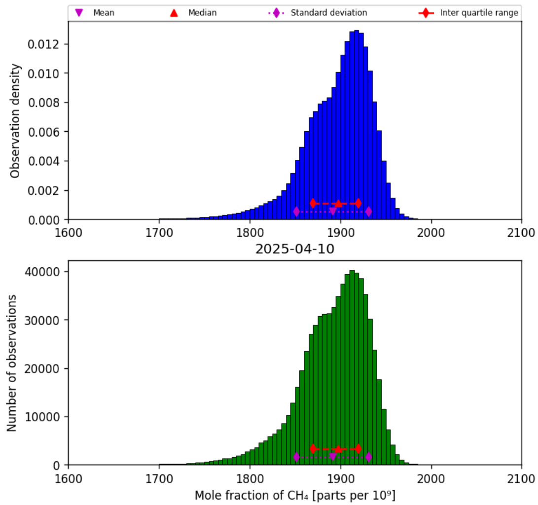
Figure 23: Histogram of “Mole fraction of CH 4 ” for 2025-04-09 to 2025-04-11
