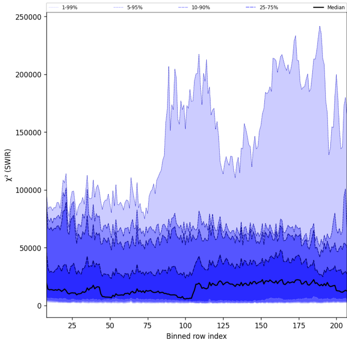
Figure 39: Along track statistics of " \chi^2 (SWIR)" for 2025-04-09 to 2025-04-11
