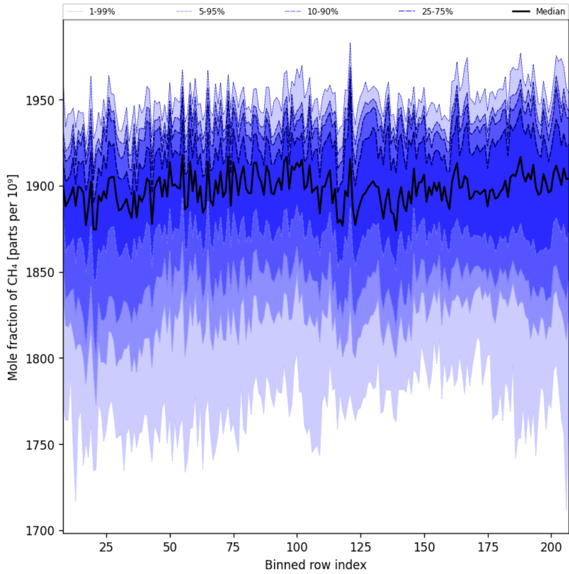
Figure 34: Along track statistics of “Mole fraction of CH 4 ” for 2025-04-09 to 2025-04-11
