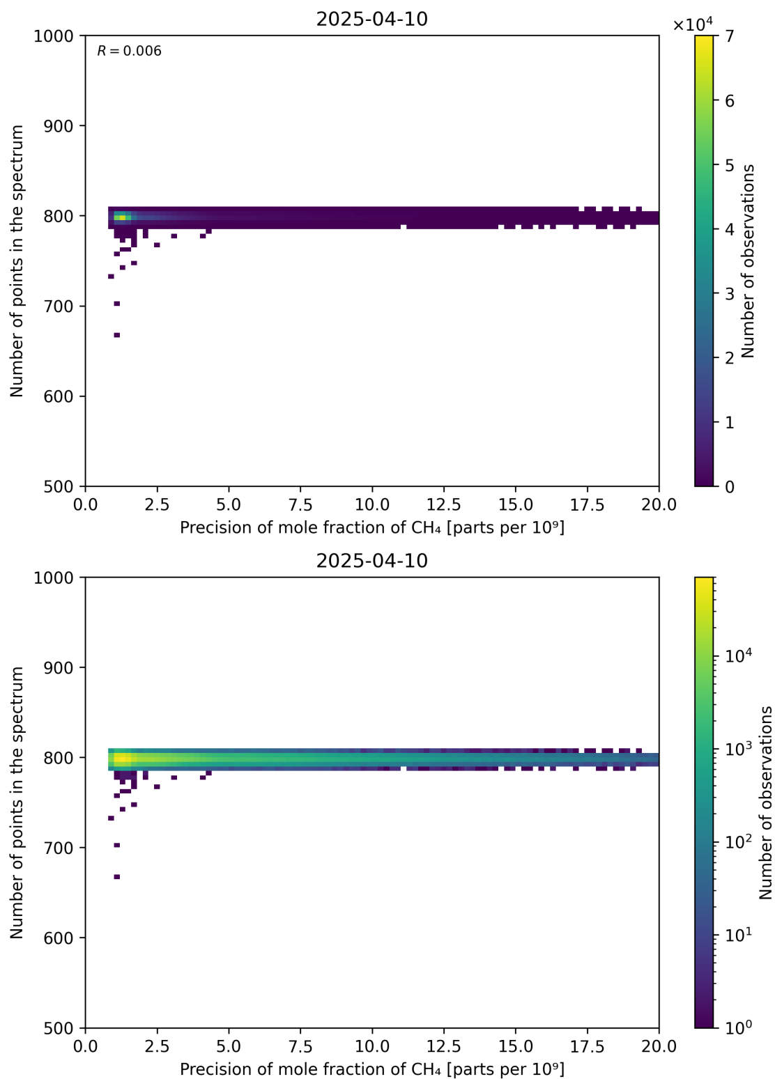
Figure 84: Scatter density plot of “Precision of mole fraction of CH 4 ” against “Number of points in the spectrum” for 2025-04-09 to 2025-04-11.
