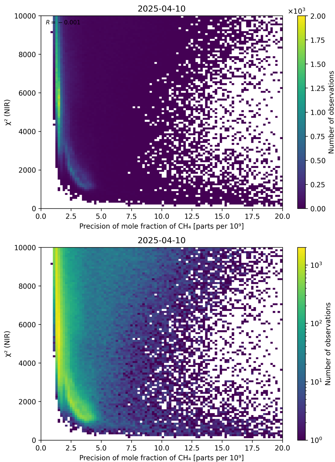
Figure 78: Scatter density plot of “Precision of mole fraction of CH 4 ” against “ \chi^2 (NIR)” for 2025-04-09 to 2025-04-11.
