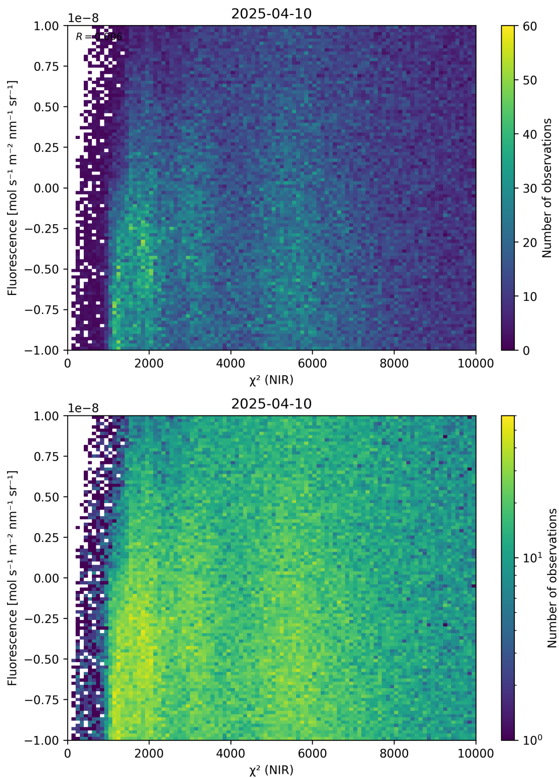
Figure 45: Scatter density plot of “ \chi^2 (NIR)” against “Fluorescence” for 2025-04-09 to 2025-04-11.
