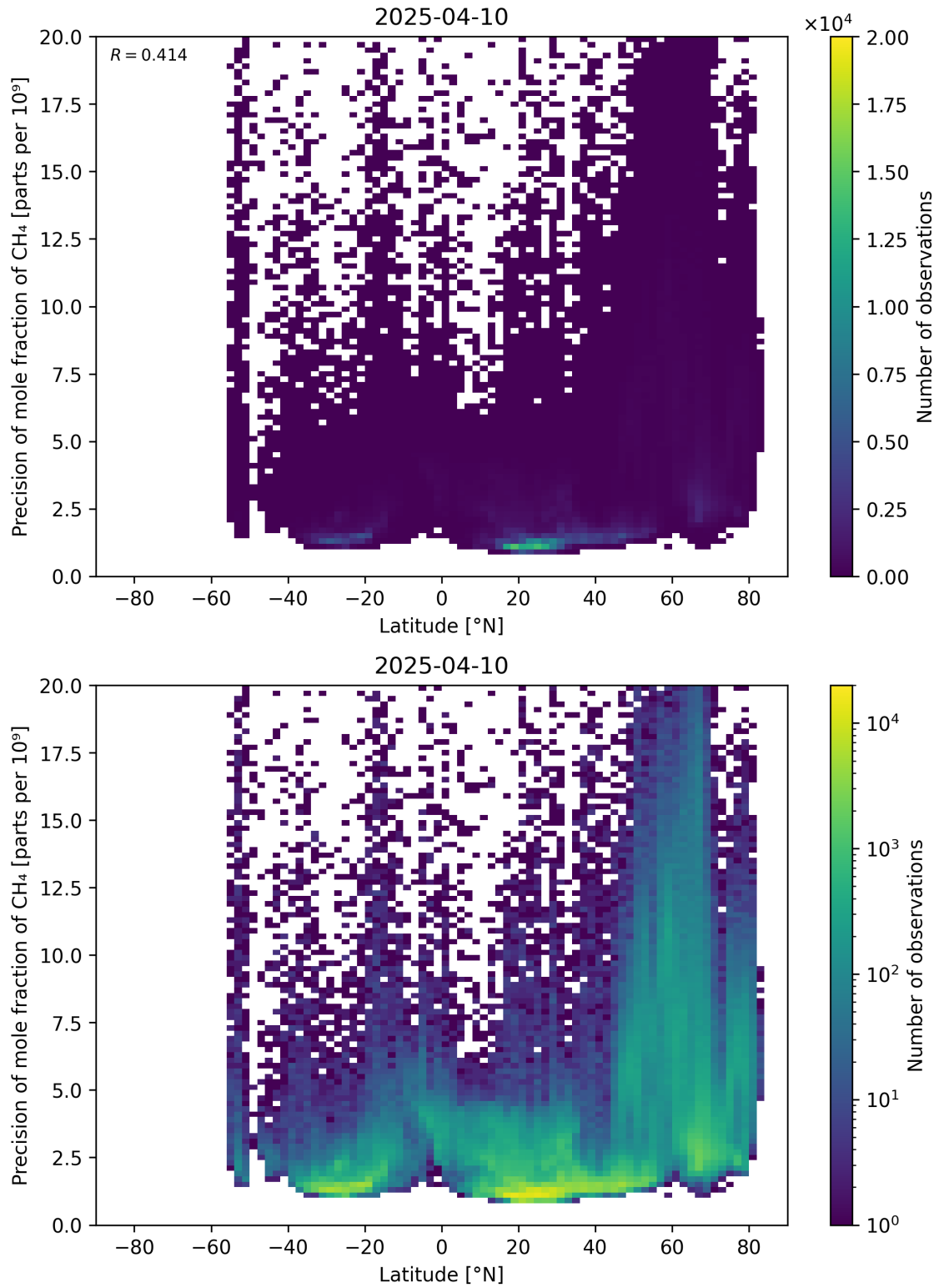
Figure 59: Scatter density plot of “Latitude” against “Precision of mole fraction of \text{CH}_4 ” for 2025-04-09 to 2025-04-11.
