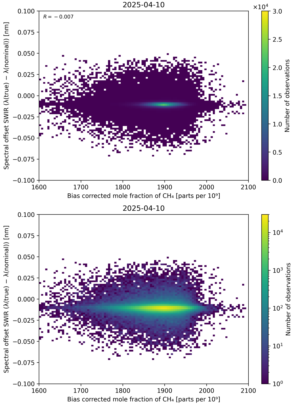
Figure 69: Scatter density plot of “Bias corrected mole fraction of \text{CH}_4 ” against “Spectral offset SWIR ( \lambda_{\text{true}} - \lambda_{\text{nominal}} )” for 2025-04-09 to 2025-04-11.
