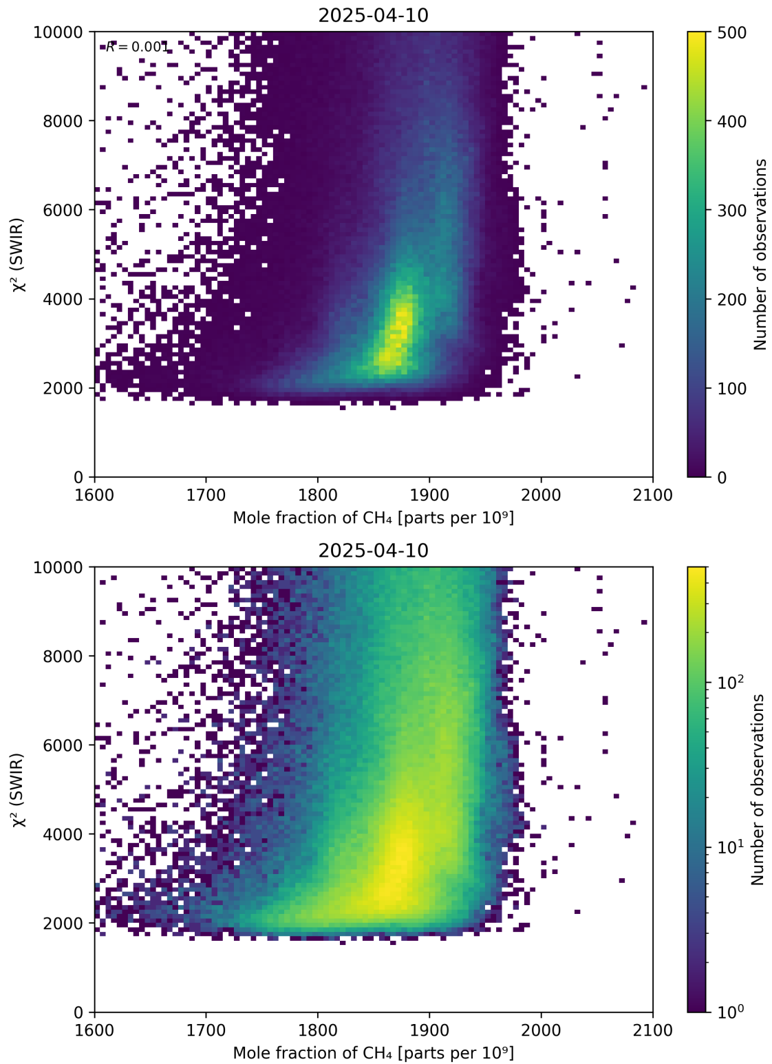
Figure 71: Scatter density plot of “Mole fraction of \text{CH}_4 ” against “ \chi^2 (SWIR)” for 2025-04-09 to 2025-04-11.
