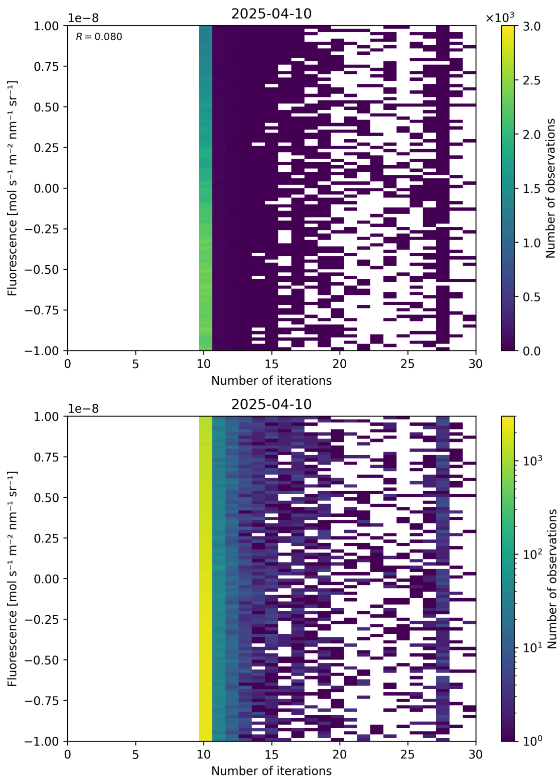
Figure 87: Scatter density plot of “Number of iterations” against “Fluorescence” for 2025-04-09 to 2025-04-11.
