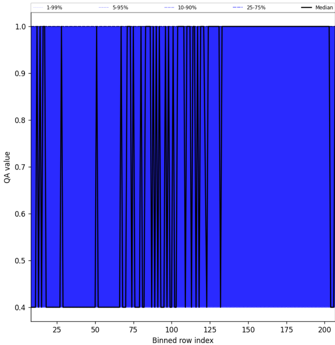
Figure 33: Along track statistics of “QA value” for 2025-04-09 to 2025-04-11
