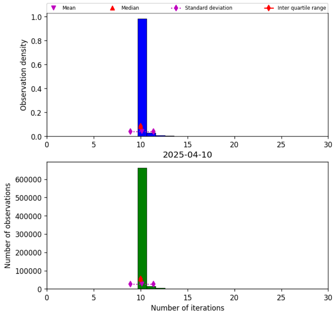
Figure 31: Histogram of “Number of iterations” for 2025-04-09 to 2025-04-11
