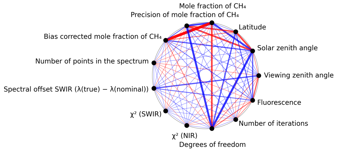
Figure 1: Map of correlation graph for 2025-04-09 to 2025-04-11.
