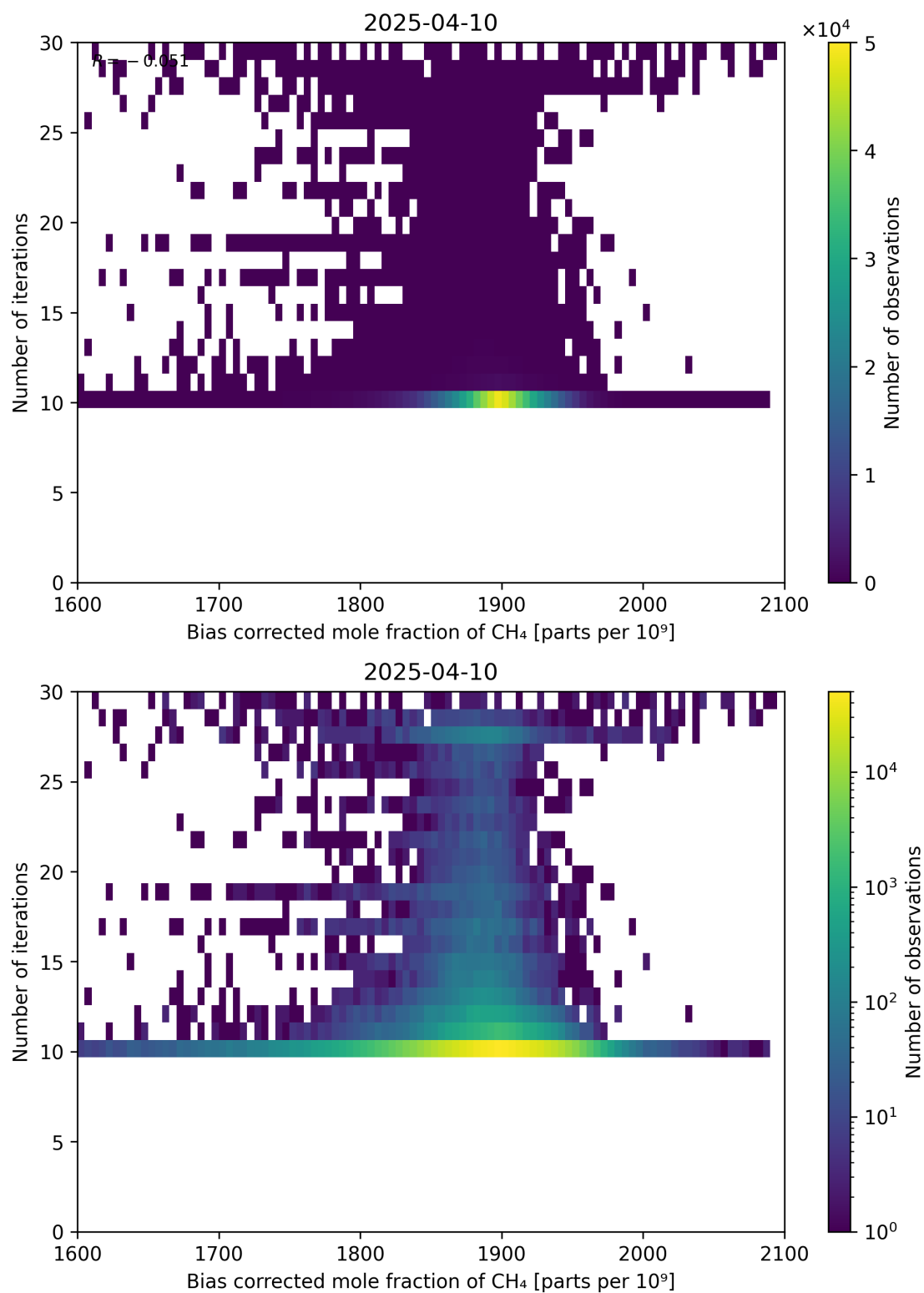
Figure 67: Scatter density plot of “Bias corrected mole fraction of CH 4 ” against “Number of iterations” for 2025-04-09 to 2025-04-11.
