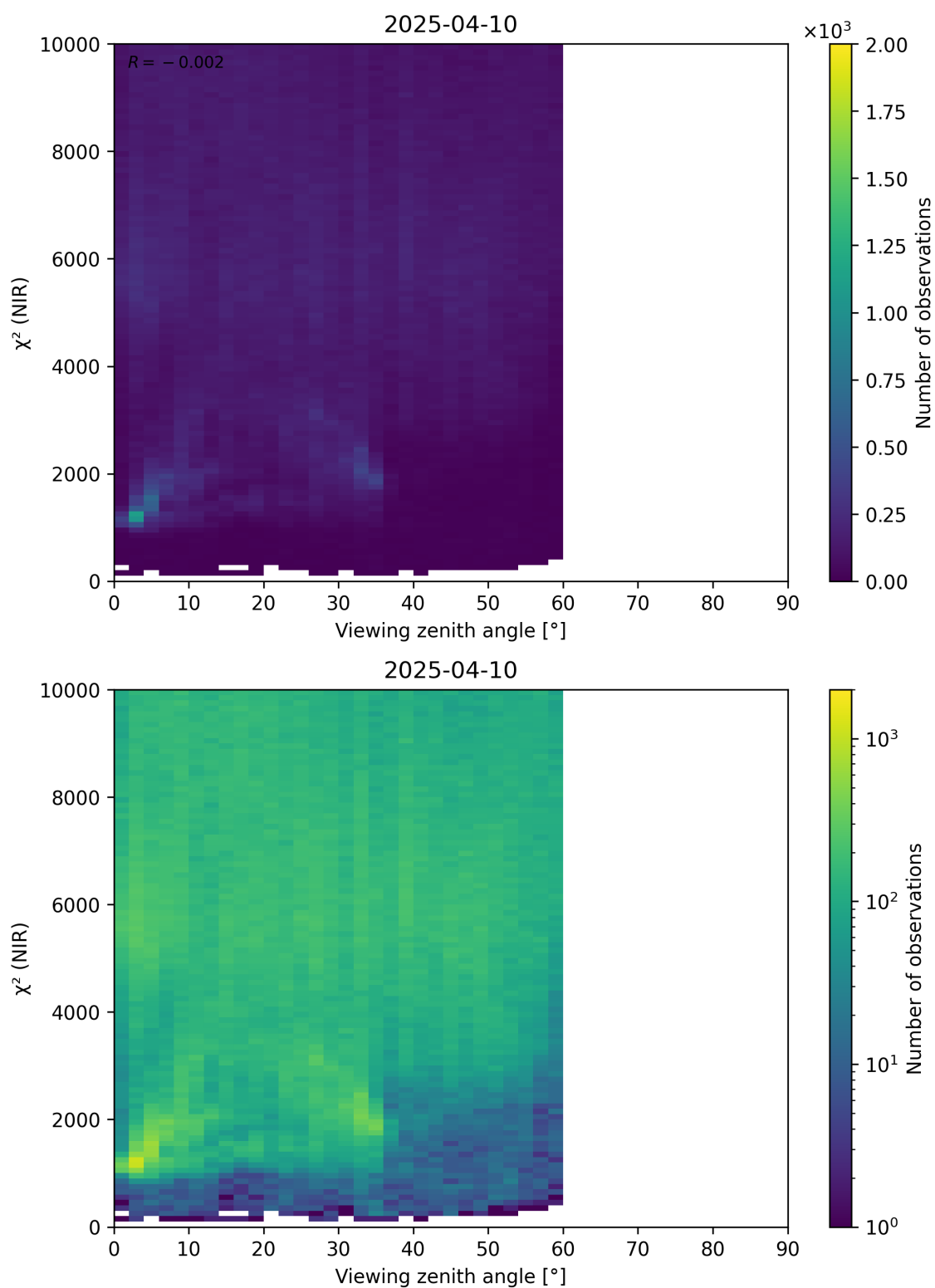
Figure 105: Scatter density plot of “Viewing zenith angle” against “ \chi^2 (NIR)” for 2025-04-09 to 2025-04-11.
