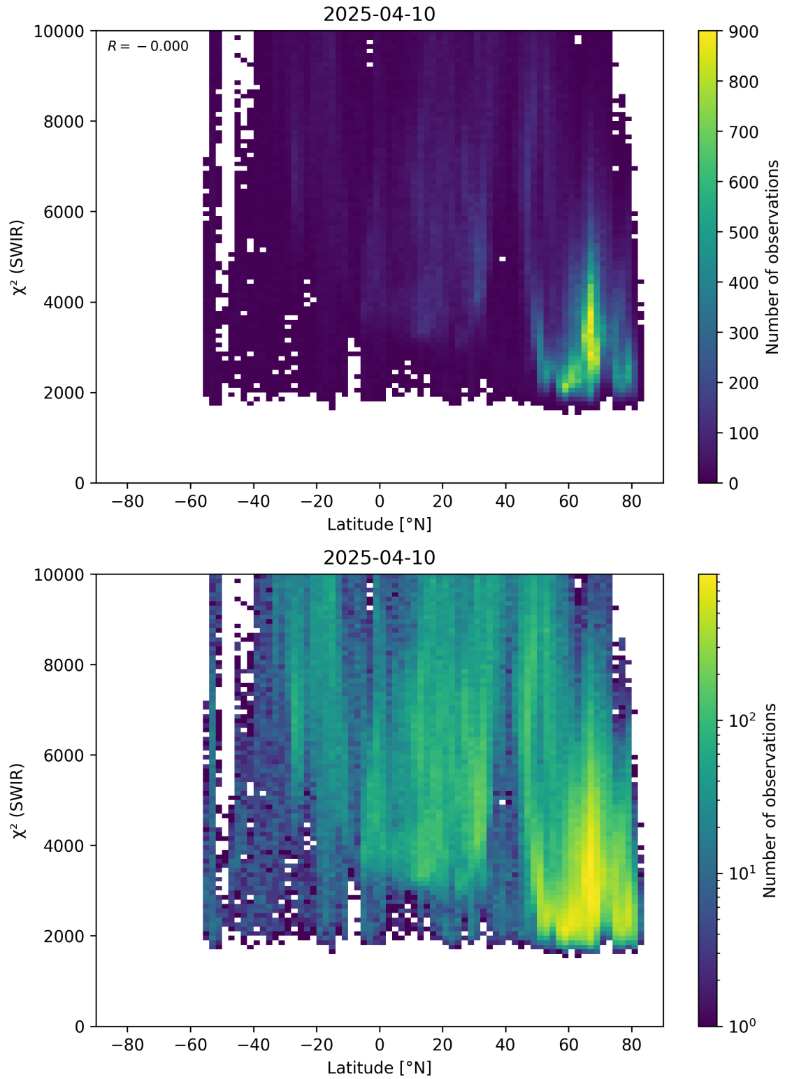
Figure 54: Scatter density plot of “Latitude” against “ \chi^2 (SWIR)” for 2025-04-09 to 2025-04-11.
