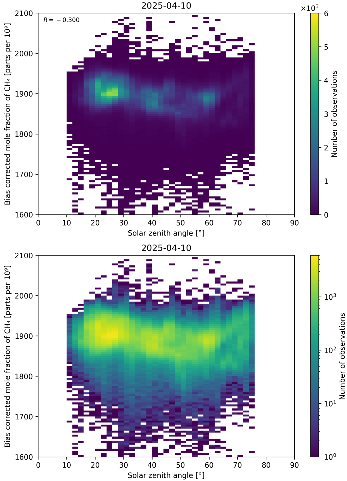
Figure 100: Scatter density plot of “Solar zenith angle” against “Bias corrected mole fraction of CH 4 ” for 2025-04-09 to 2025-04-11.
