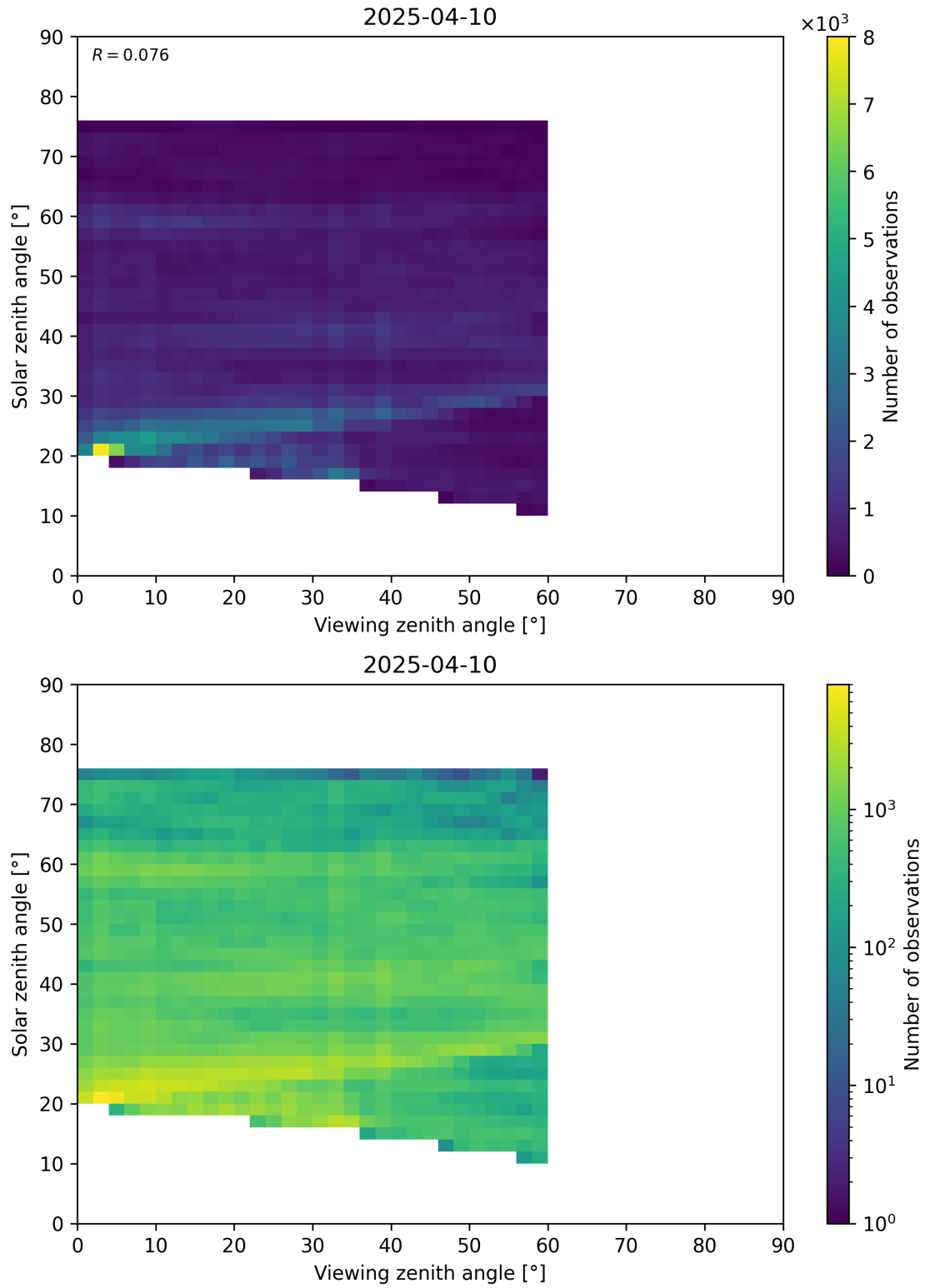
Figure 115: Scatter density plot of “Viewing zenith angle” against “Solar zenith angle” for 2025-04-09 to 2025-04-11.
