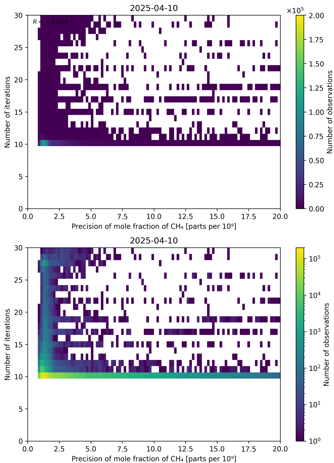
Figure 83: Scatter density plot of “Precision of mole fraction of CH 4 ” against “Number of iterations” for 2025-04-09 to 2025-04-11.
