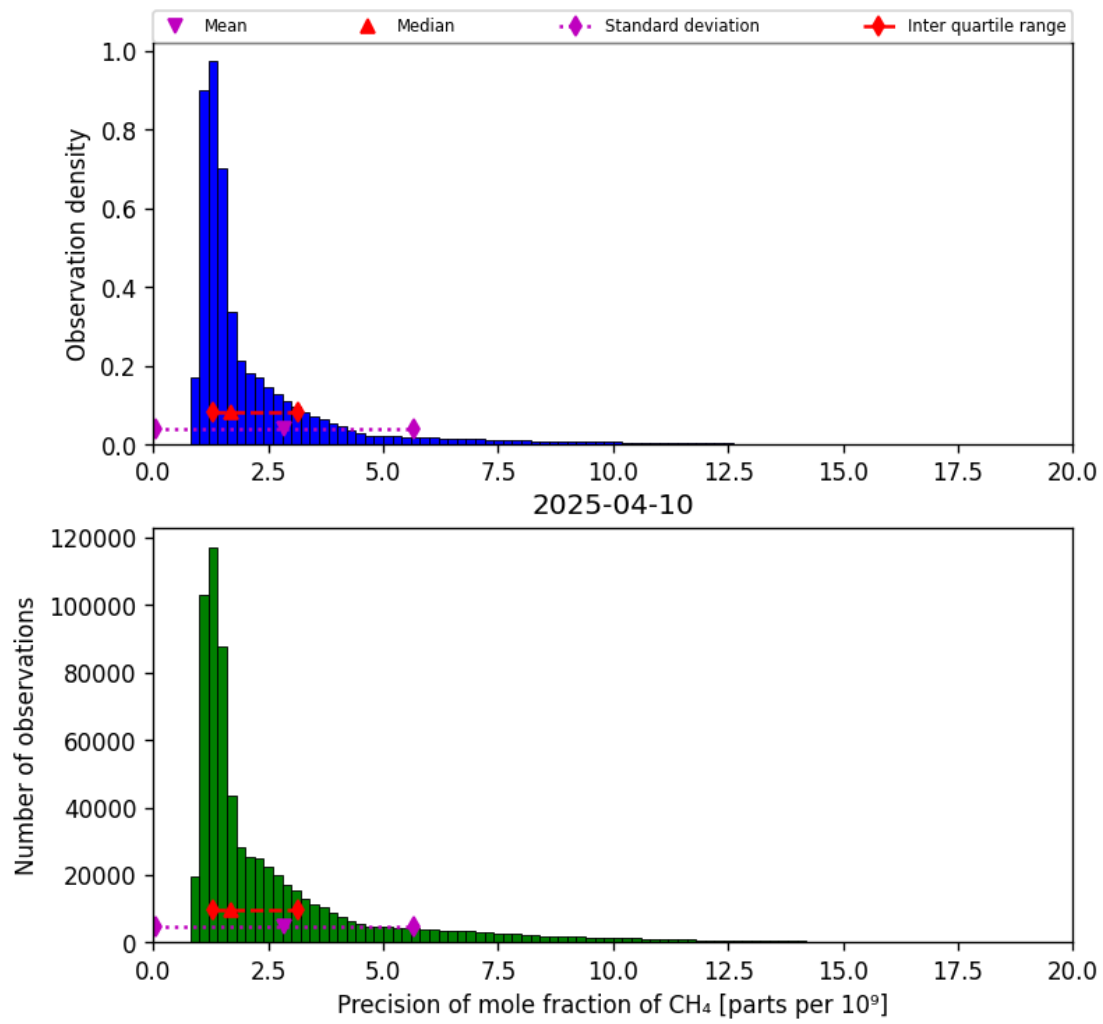
Figure 24: Histogram of “Precision of mole fraction of CH 4 ” for 2025-04-09 to 2025-04-11
