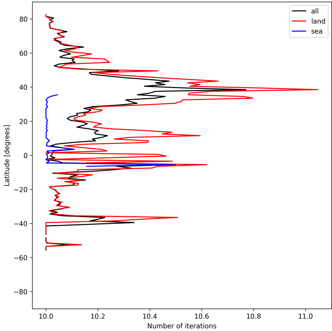
Figure 20: Zonal average of “Number of iterations” for 2025-04-09 to 2025-04-11.
