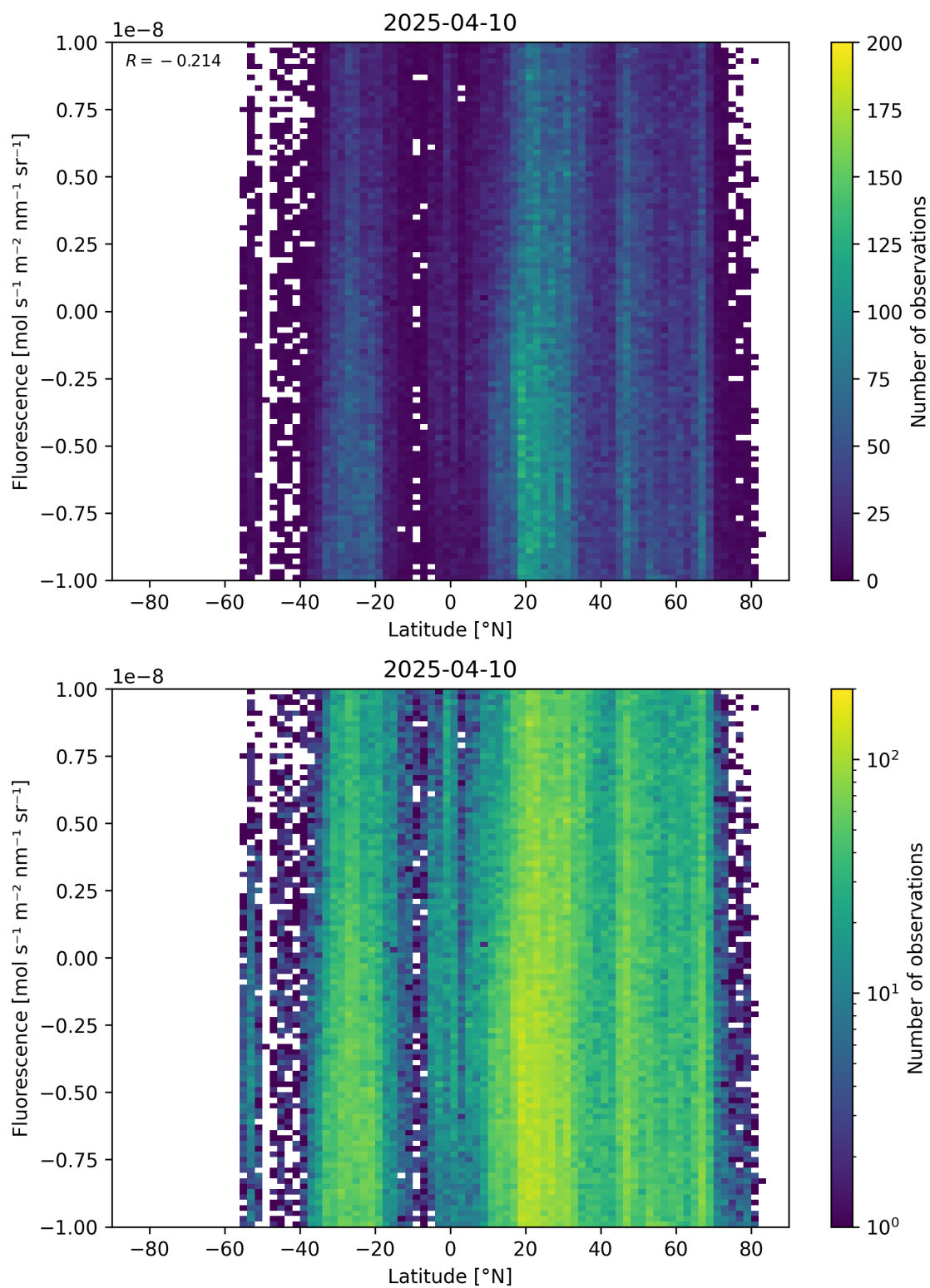
Figure 56: Scatter density plot of “Latitude” against “Fluorescence” for 2025-04-09 to 2025-04-11.
