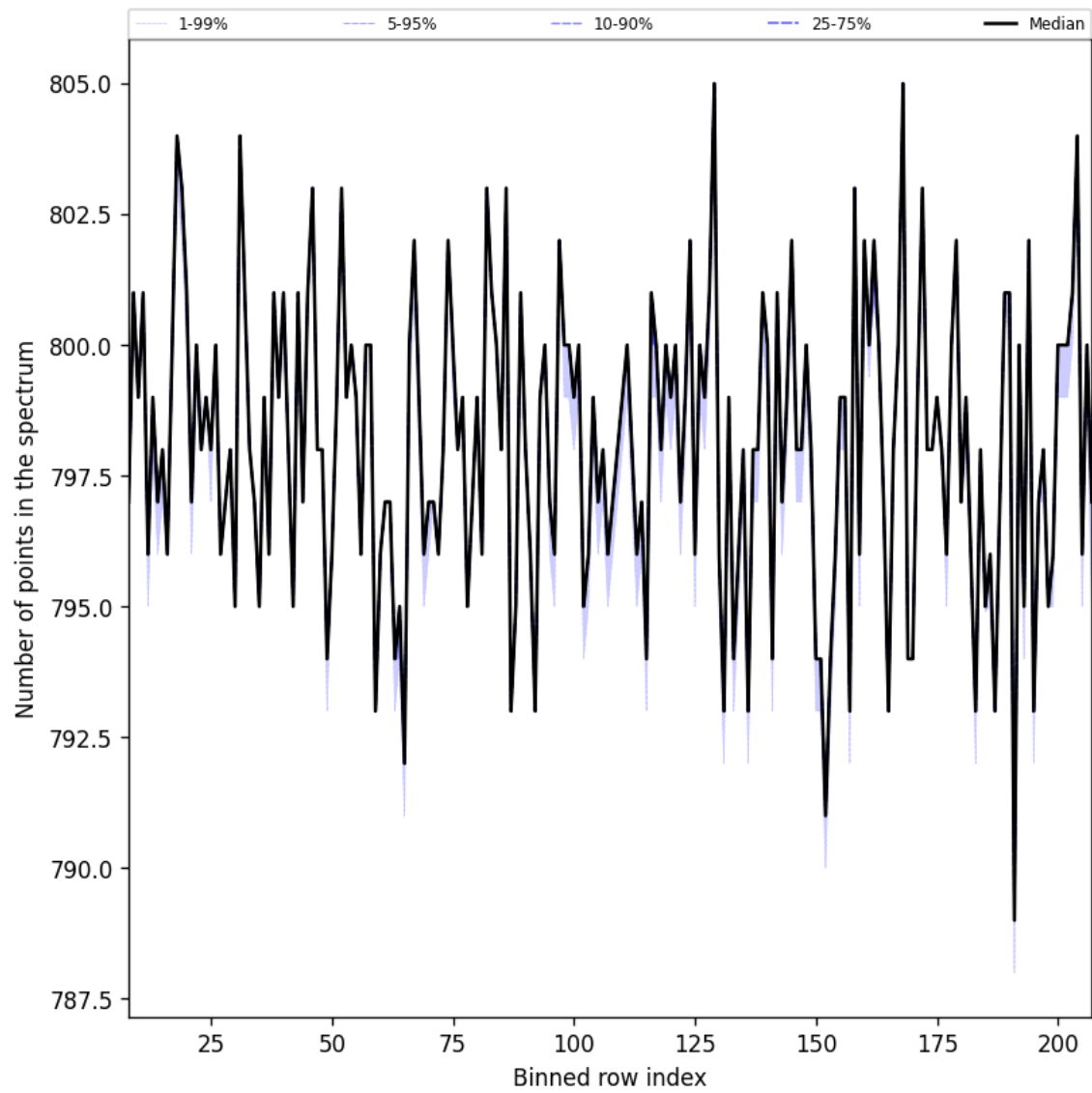
Figure 37: Along track statistics of “Number of points in the spectrum” for 2025-04-09 to 2025-04-11
