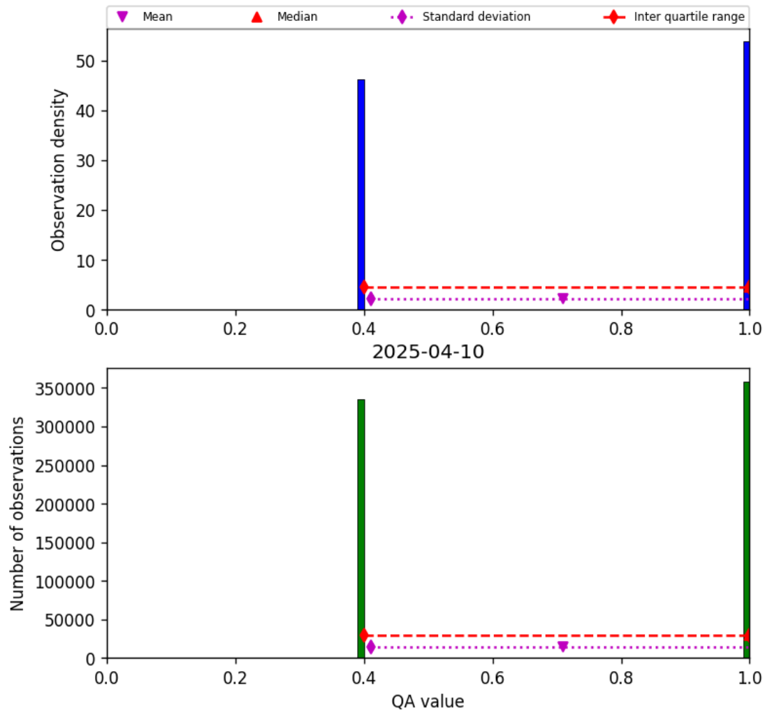
Figure 22: Histogram of “QA value” for 2025-04-09 to 2025-04-11
