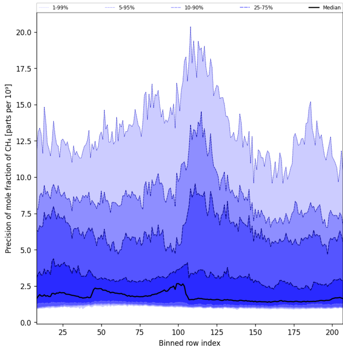
Figure 35: Along track statistics of “Precision of mole fraction of CH 4 ” for 2025-04-09 to 2025-04-11
