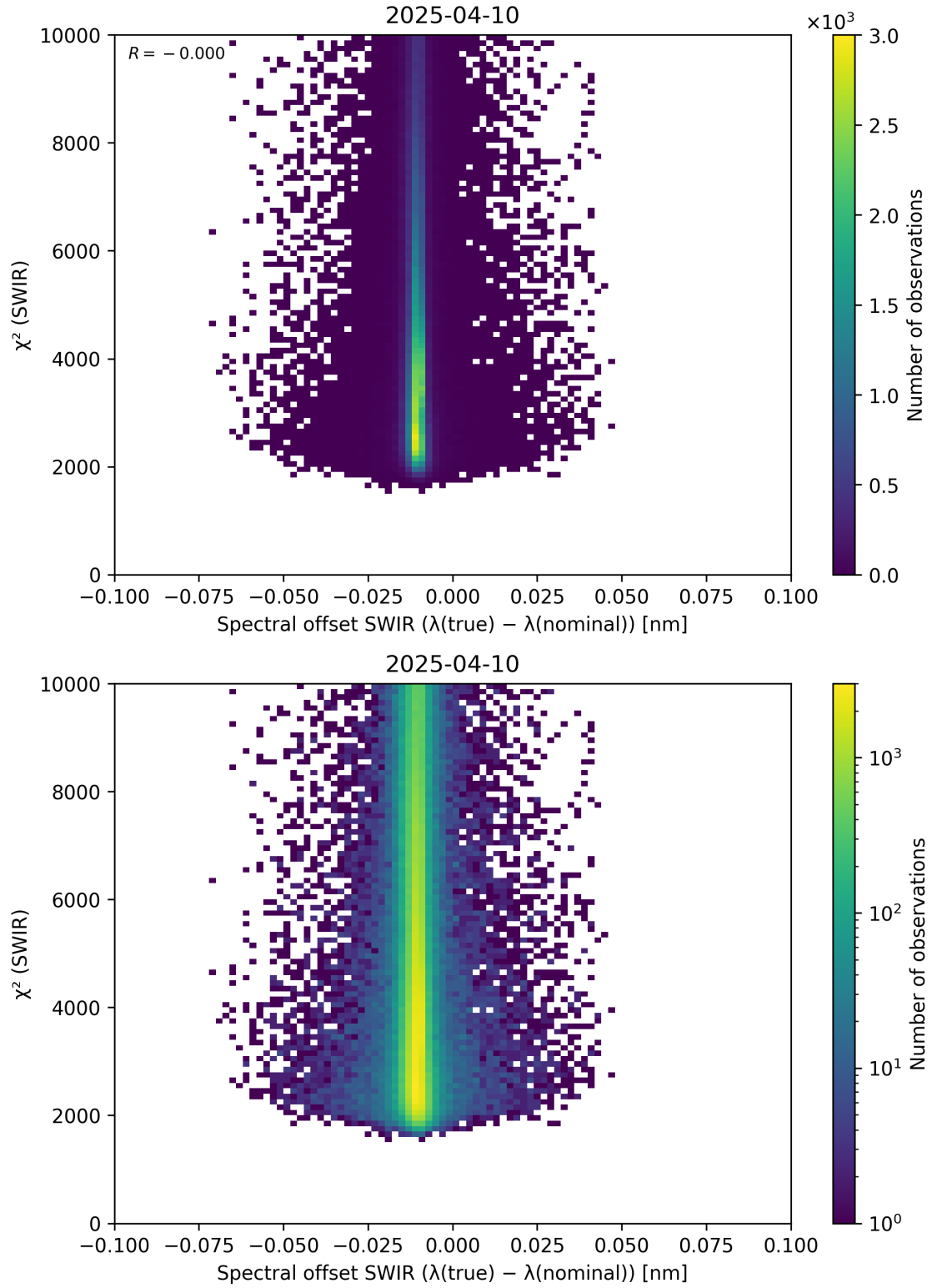
Figure 118: Scatter density plot of “Spectral offset SWIR ( \lambda_{\text{true}} - \lambda_{\text{nominal}} )” against “ \chi^2 (SWIR)” for 2025-04-09 to 2025-04-11.
