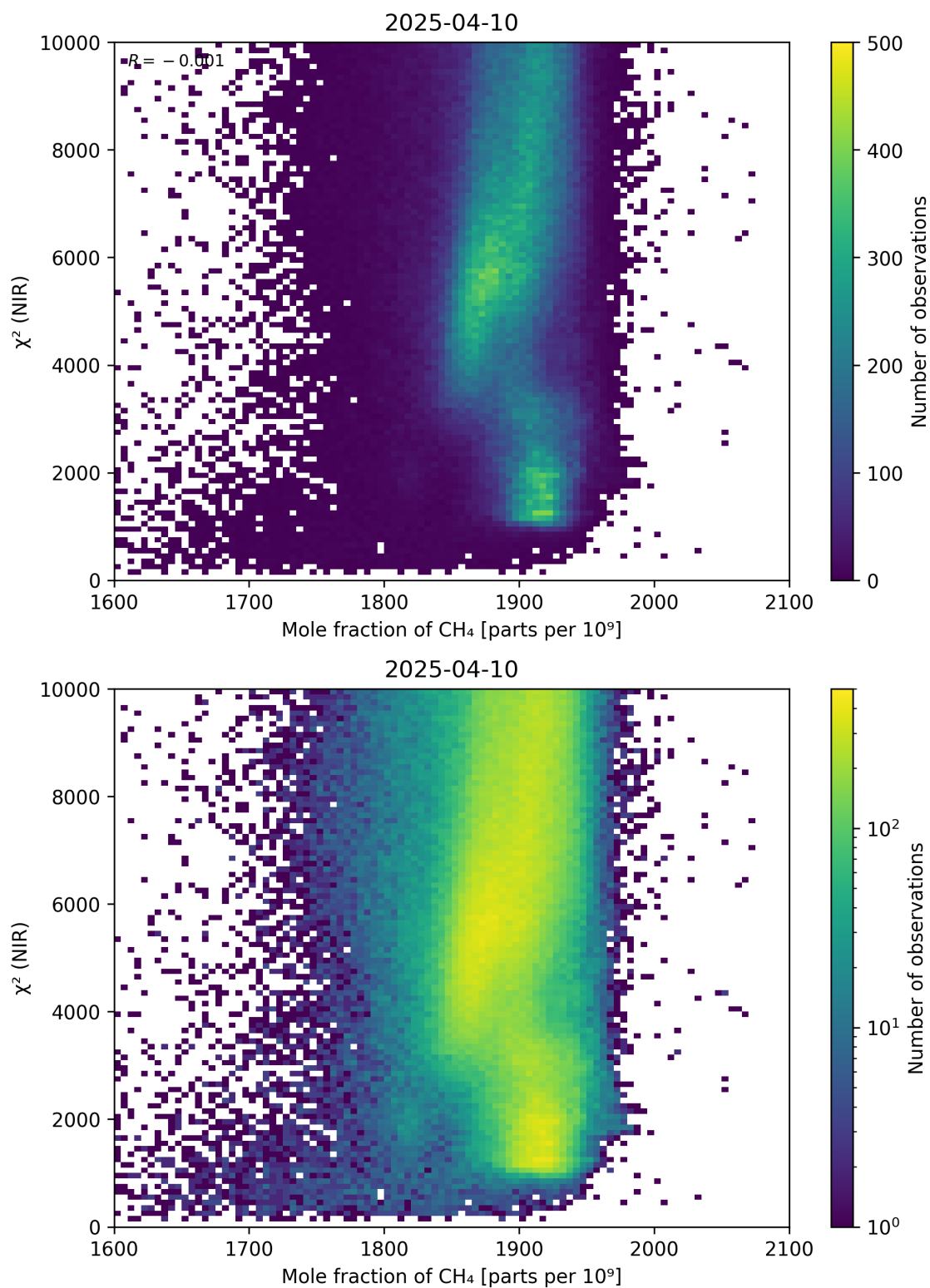
Figure 70: Scatter density plot of “Mole fraction of CH 4 ” against “ \chi^2 (NIR)” for 2025-04-09 to 2025-04-11.
