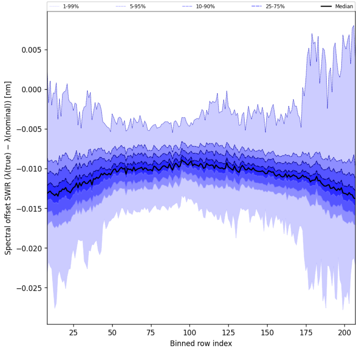
Figure 38: Along track statistics of “Spectral offset SWIR ( \lambda_{\text{true}} - \lambda_{\text{nominal}} )” for 2025-04-09 to 2025-04-11
