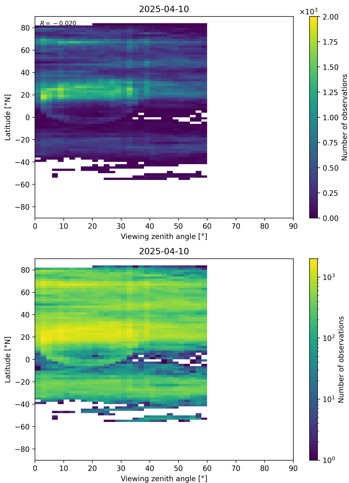
Figure 109: Scatter density plot of “Viewing zenith angle” against “Latitude” for 2025-04-09 to 2025-04-11.
