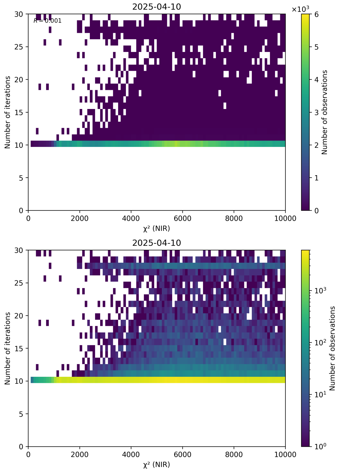
Figure 46: Scatter density plot of “ \chi^2 (NIR)” against “Number of iterations” for 2025-04-09 to 2025-04-11.
