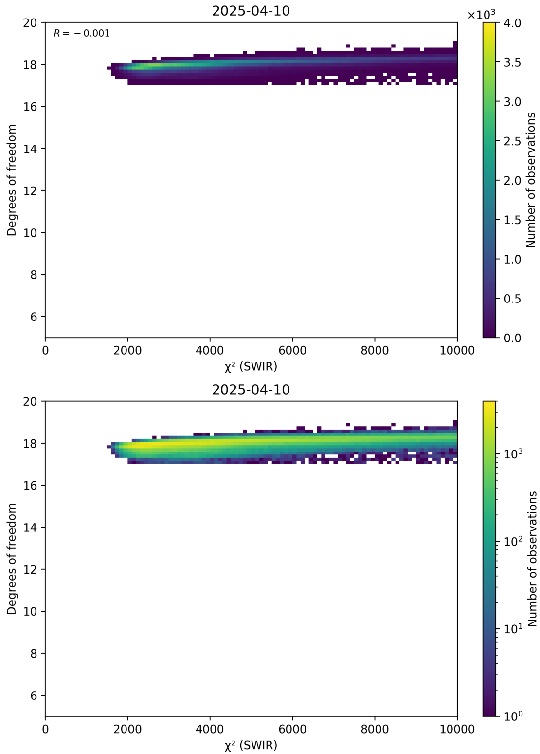
Figure 48: Scatter density plot of “ \chi^2 (SWIR)” against “Degrees of freedom” for 2025-04-09 to 2025-04-11.
