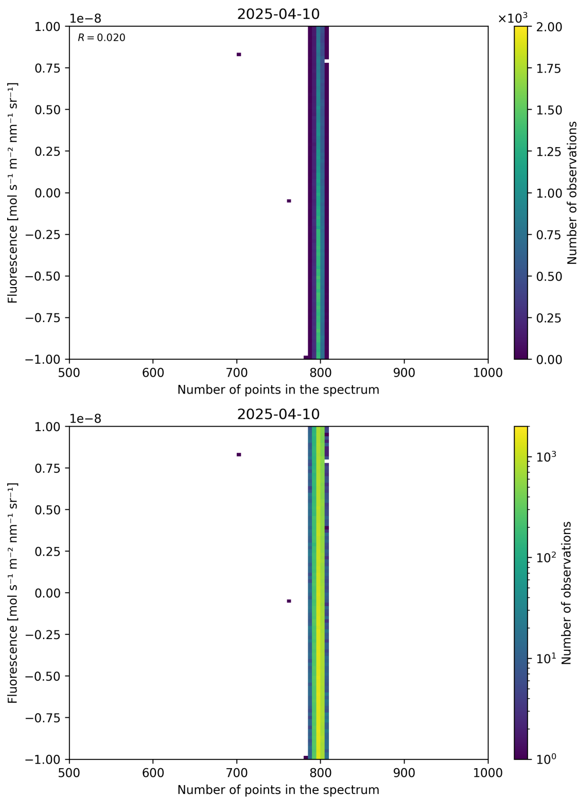
Figure 91: Scatter density plot of “Number of points in the spectrum” against “Fluorescence” for 2025-04-09 to 2025-04-11.
