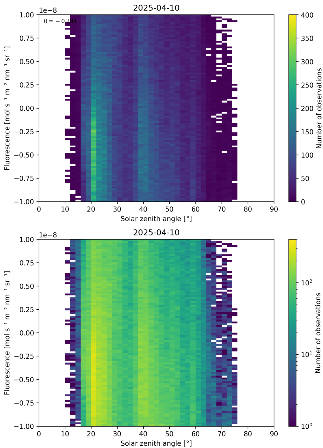
Figure 97: Scatter density plot of “Solar zenith angle” against “Fluorescence” for 2025-04-09 to 2025-04-11.
