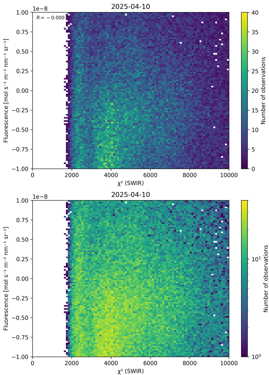
Figure 49: Scatter density plot of “ \chi^2 (SWIR)” against “Fluorescence” for 2025-04-09 to 2025-04-11.
