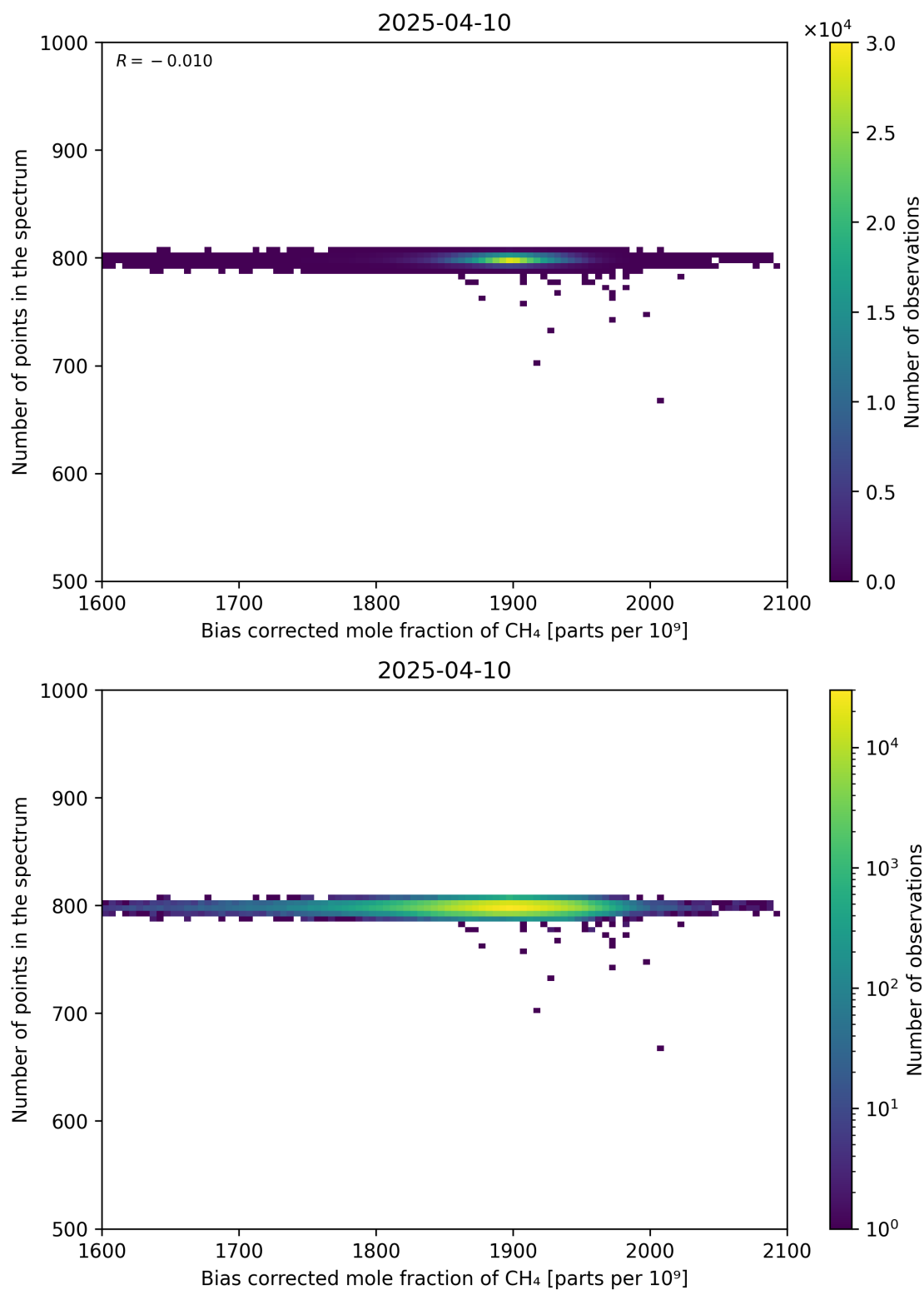
Figure 68: Scatter density plot of “Bias corrected mole fraction of CH 4 ” against “Number of points in the spectrum” for 2025-04-09 to 2025-04-11.
