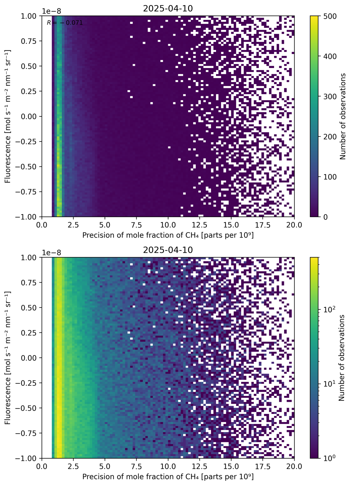
Figure 81: Scatter density plot of “Precision of mole fraction of CH 4 ” against “Fluorescence” for 2025-04-09 to 2025-04-11.
