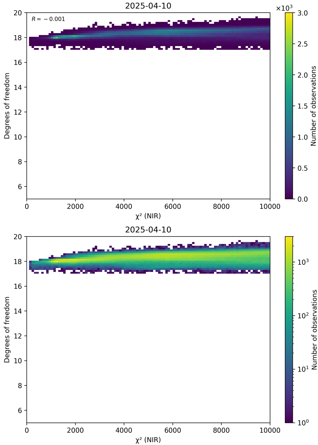
Figure 44: Scatter density plot of “ \chi^2 (NIR)” against “Degrees of freedom” for 2025-04-09 to 2025-04-11.
