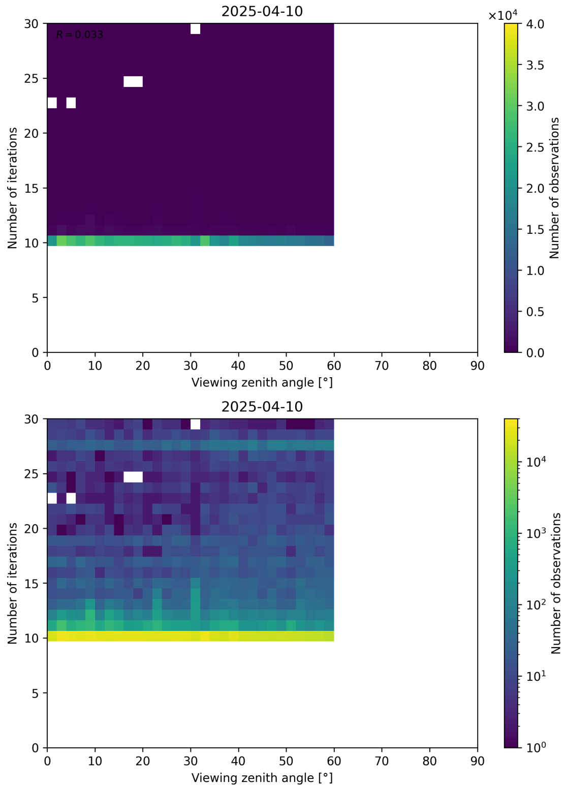
Figure 113: Scatter density plot of “Viewing zenith angle” against “Number of iterations” for 2025-04-09 to 2025-04-11.
