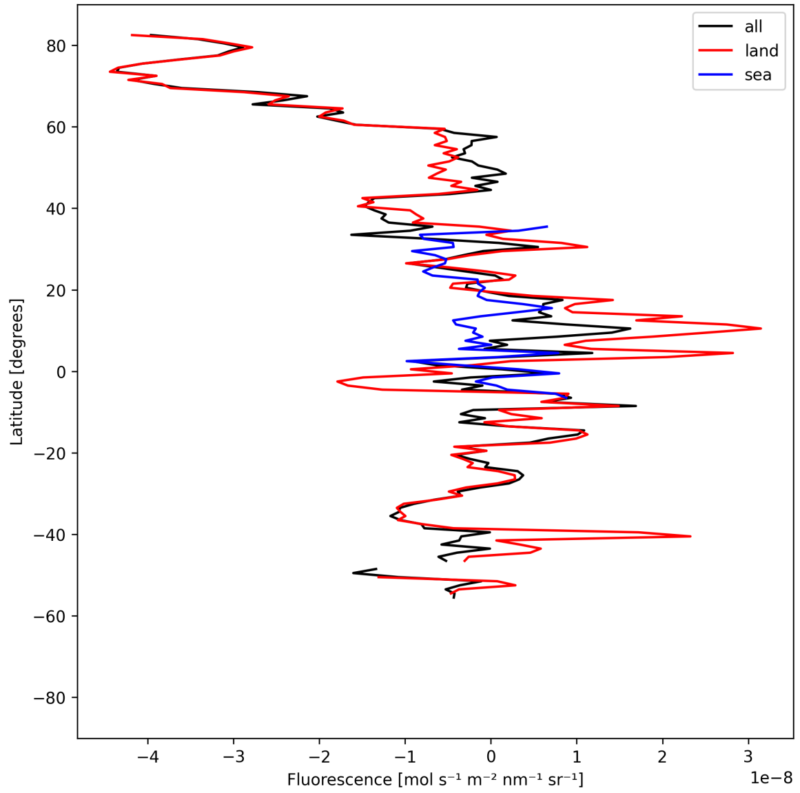
Figure 21: Zonal average of “Fluorescence” for 2025-04-09 to 2025-04-11.
