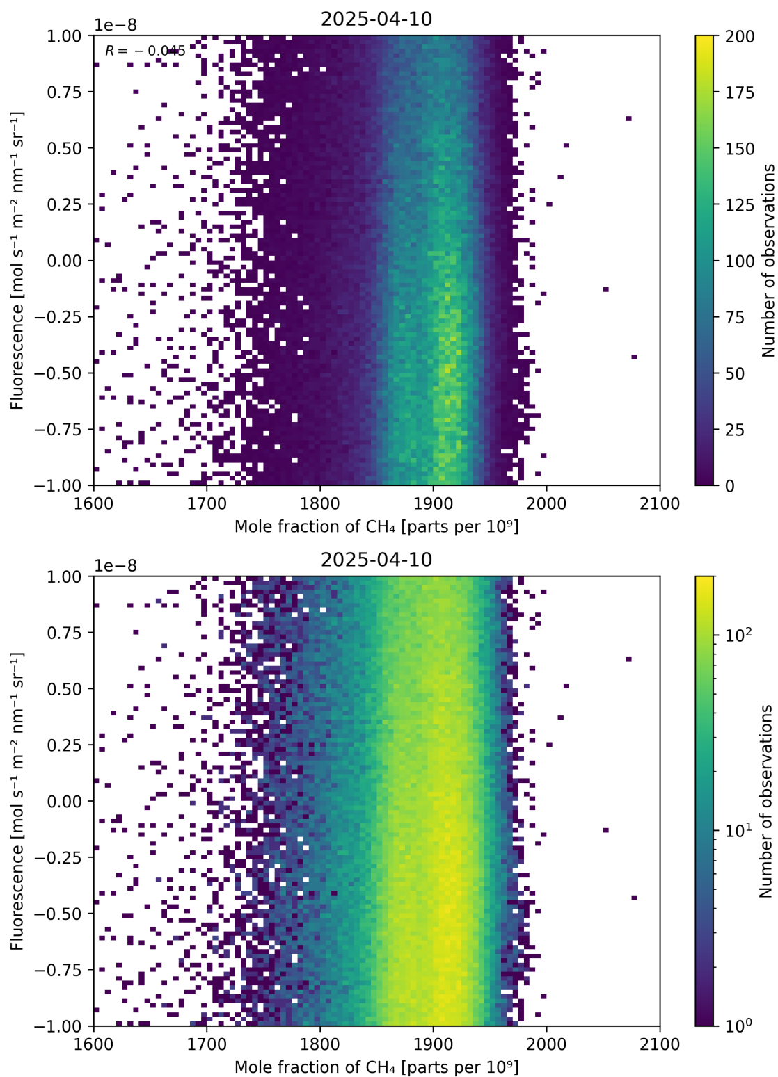
Figure 73: Scatter density plot of “Mole fraction of \text{CH}_4 ” against “Fluorescence” for 2025-04-09 to 2025-04-11.
