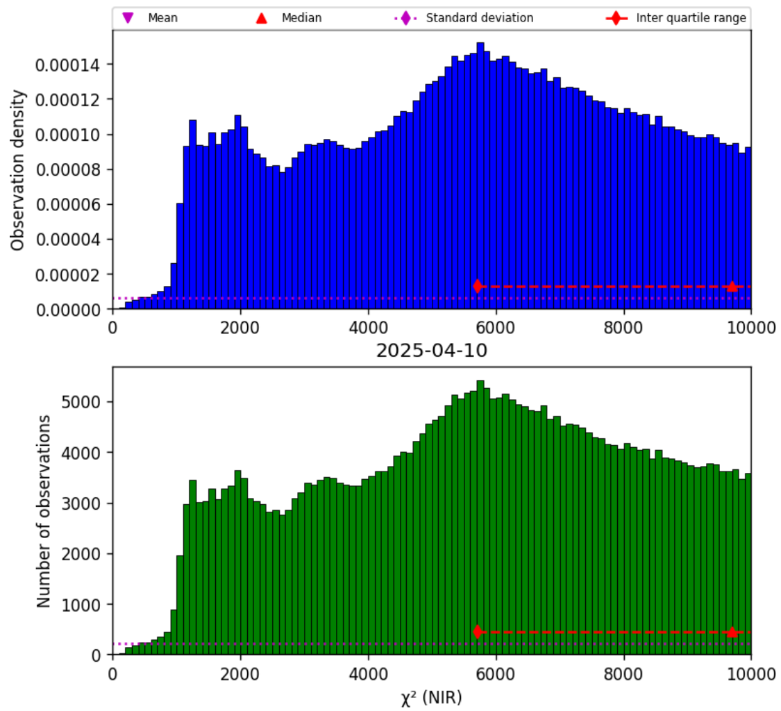
Figure 29: Histogram of “ \chi^2 (NIR)” for 2025-04-09 to 2025-04-11
