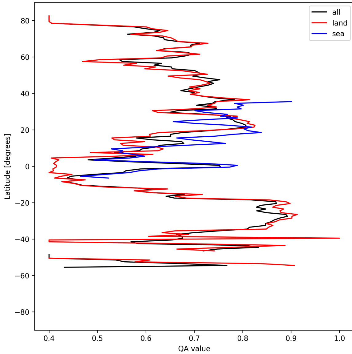
Figure 11: Zonal average of “QA value” for 2025-04-09 to 2025-04-11.
