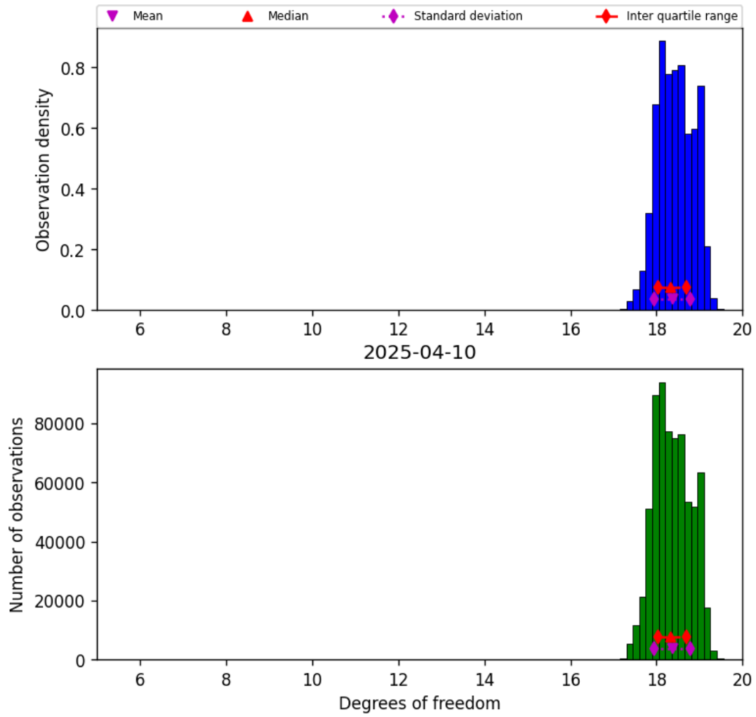
Figure 30: Histogram of “Degrees of freedom” for 2025-04-09 to 2025-04-11
