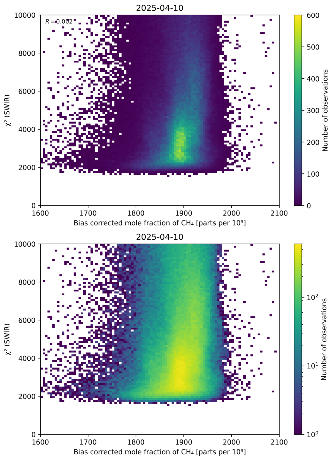
Figure 64: Scatter density plot of “Bias corrected mole fraction of CH 4 ” against “ \chi^2 (SWIR)” for 2025-04-09 to 2025-04-11.
