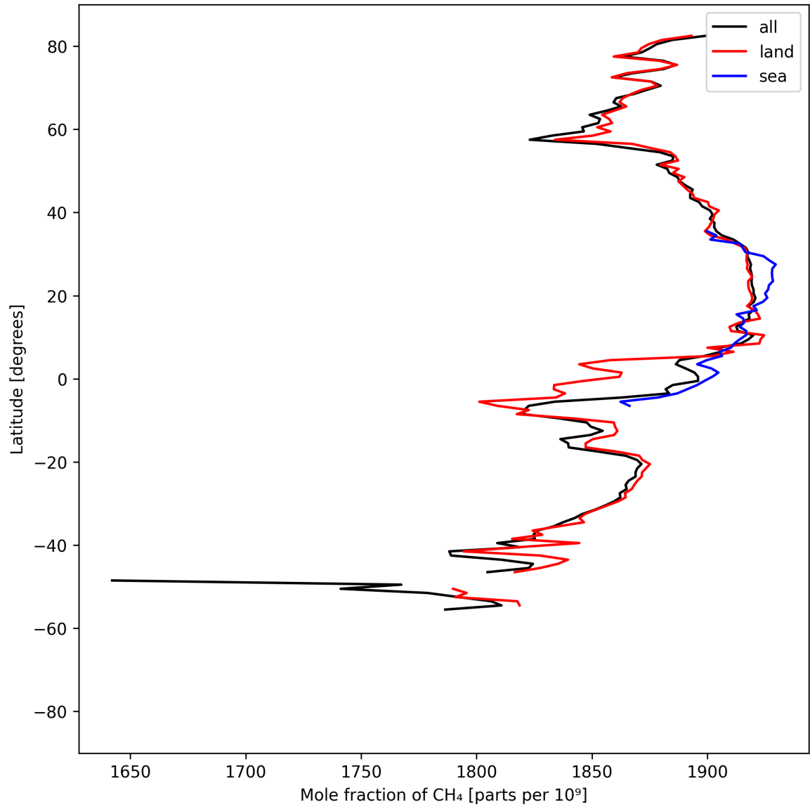
Figure 12: Zonal average of “Mole fraction of \text{CH}_4 ” for 2025-04-09 to 2025-04-11.
