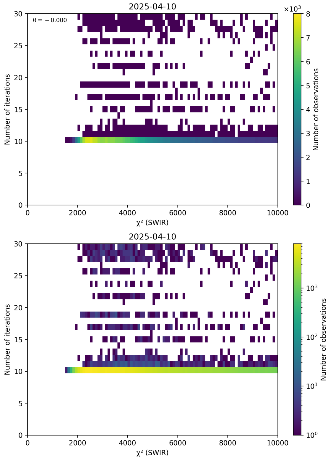
Figure 50: Scatter density plot of “ \chi^2 (SWIR)” against “Number of iterations” for 2025-04-09 to 2025-04-11.
