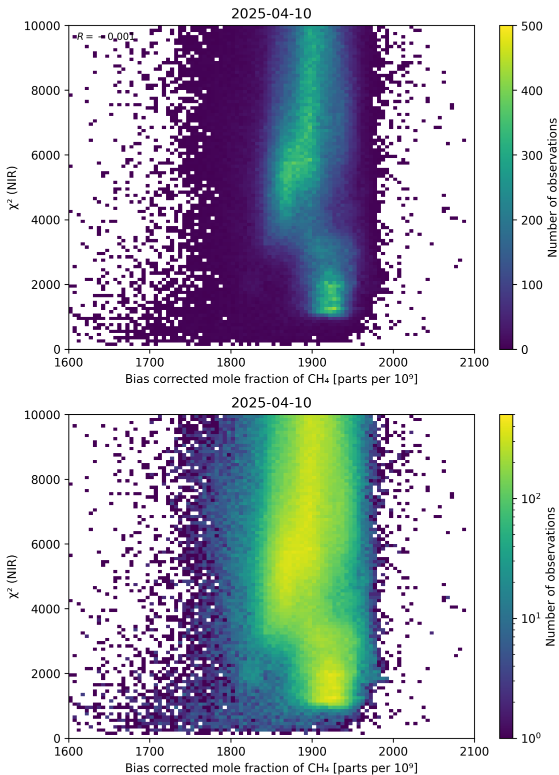
Figure 63: Scatter density plot of “Bias corrected mole fraction of CH 4 ” against “ \chi^2 (NIR)” for 2025-04-09 to 2025-04-11.
