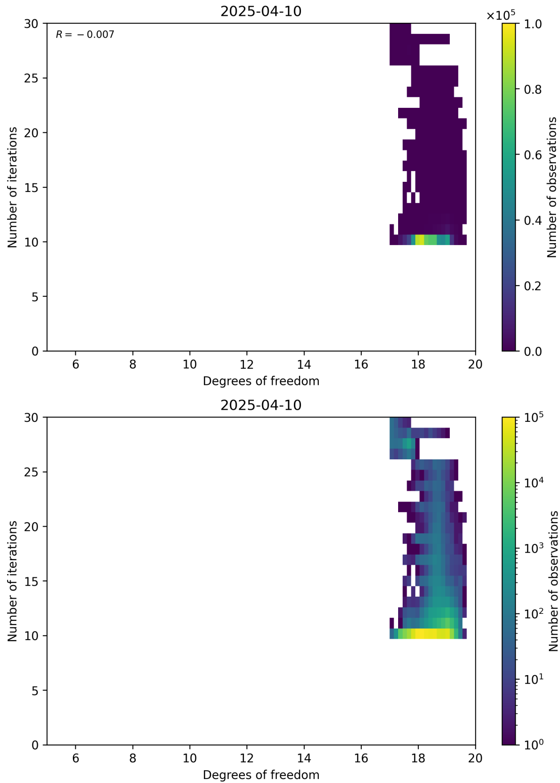
Figure 52: Scatter density plot of “Degrees of freedom” against “Number of iterations” for 2025-04-09 to 2025-04-11.
