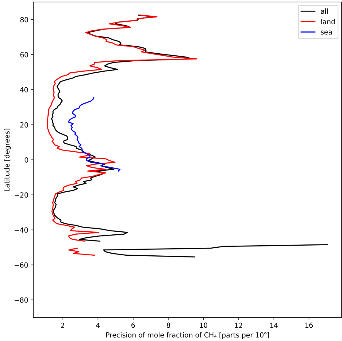
Figure 13: Zonal average of “Precision of mole fraction of CH 4 ” for 2025-04-09 to 2025-04-11.
