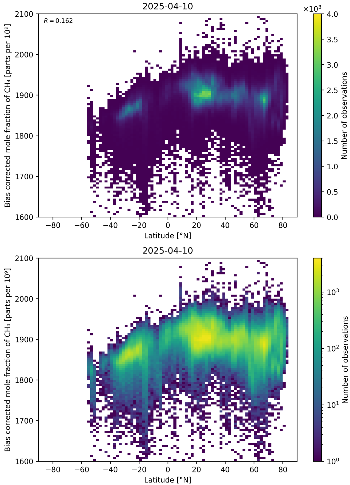
Figure 58: Scatter density plot of “Latitude” against “Bias corrected mole fraction of CH 4 ” for 2025-04-09 to 2025-04-11.
