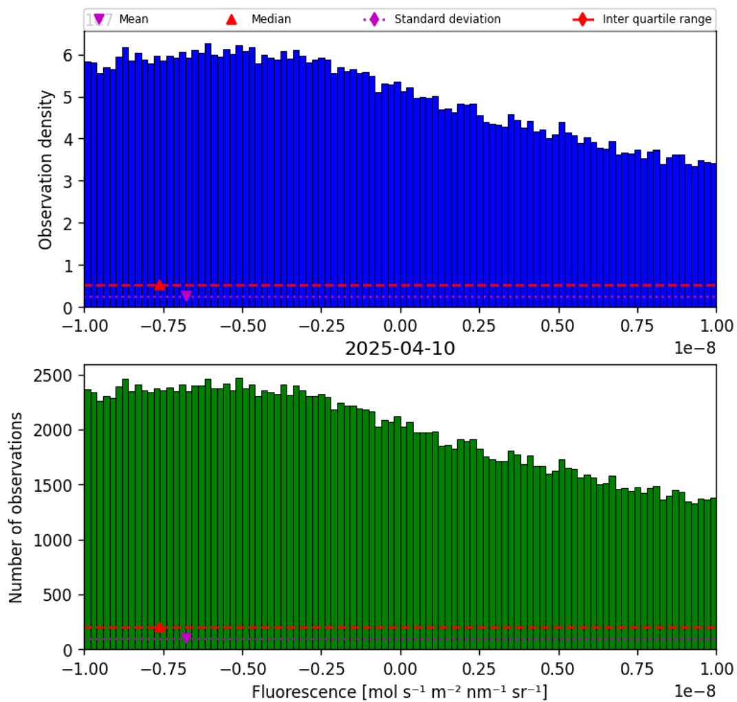
Figure 32: Histogram of “Fluorescence” for 2025-04-09 to 2025-04-11
