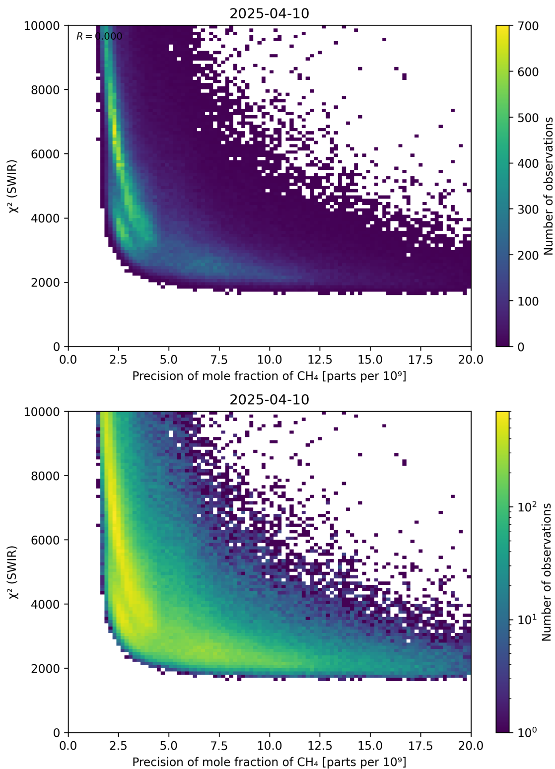
Figure 79: Scatter density plot of “Precision of mole fraction of \text{CH}_4 ” against “ \chi^2 (SWIR)” for 2025-04-09 to 2025-04-11.
