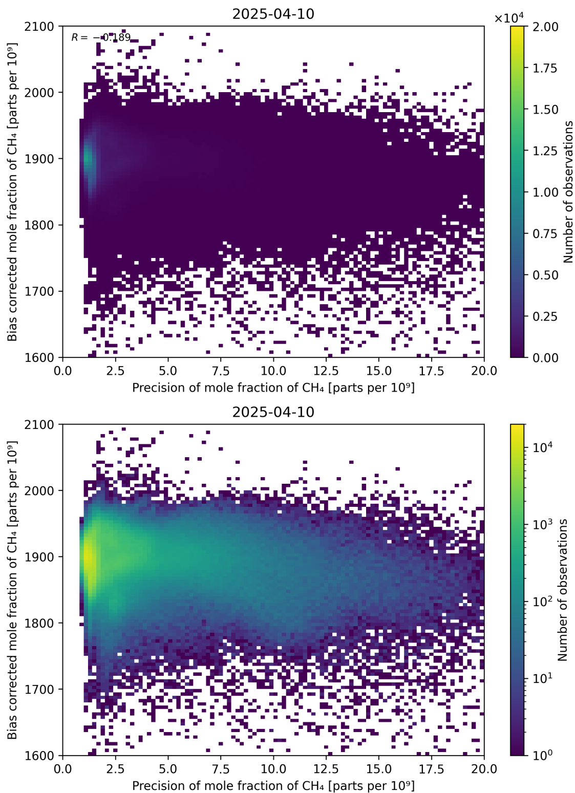
Figure 82: Scatter density plot of “Precision of mole fraction of CH 4 ” against “Bias corrected mole fraction of CH 4 ” for 2025-04-09 to 2025-04-11.
