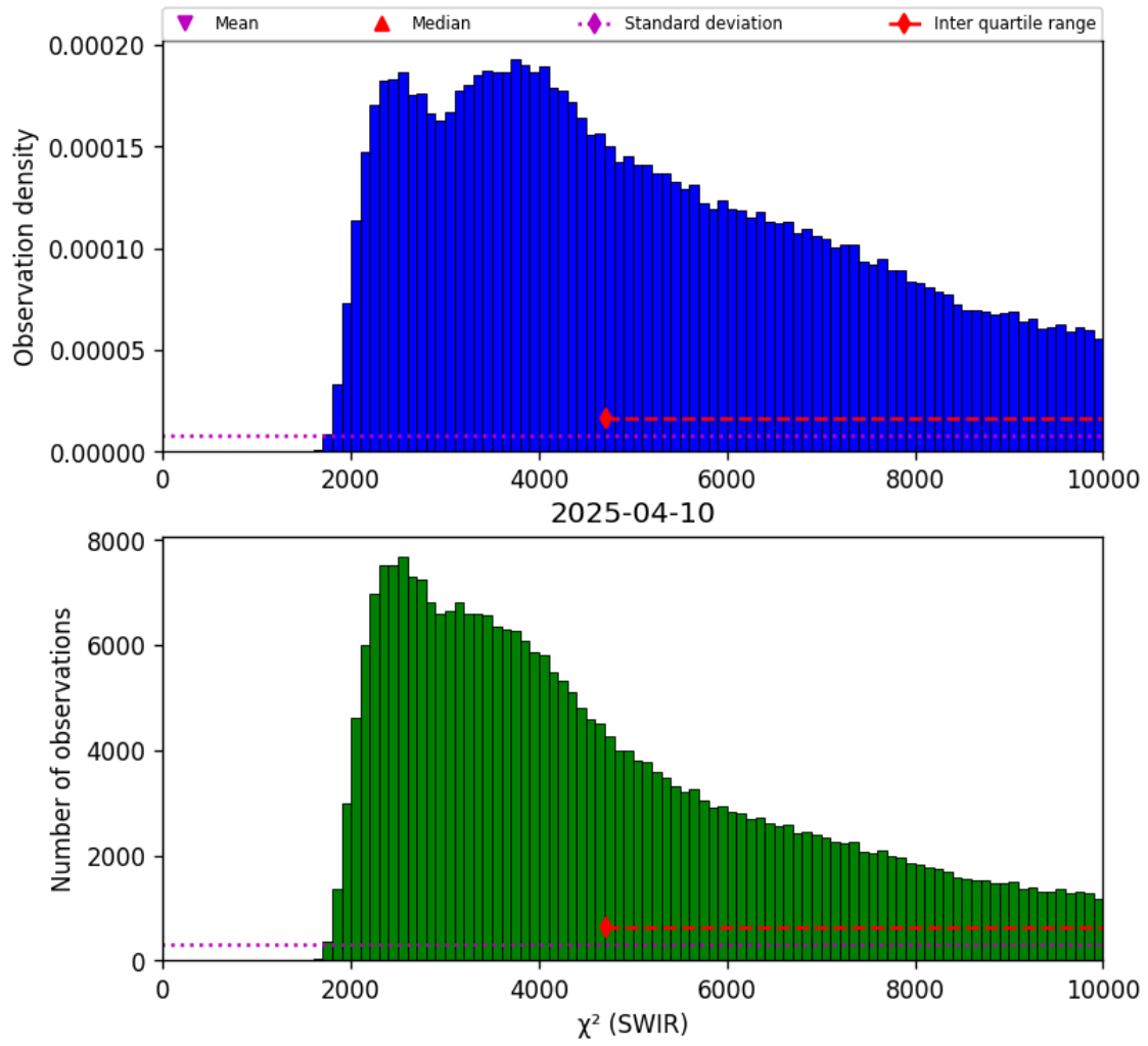
Figure 28: Histogram of “ \chi^2 (SWIR)” for 2025-04-09 to 2025-04-11
