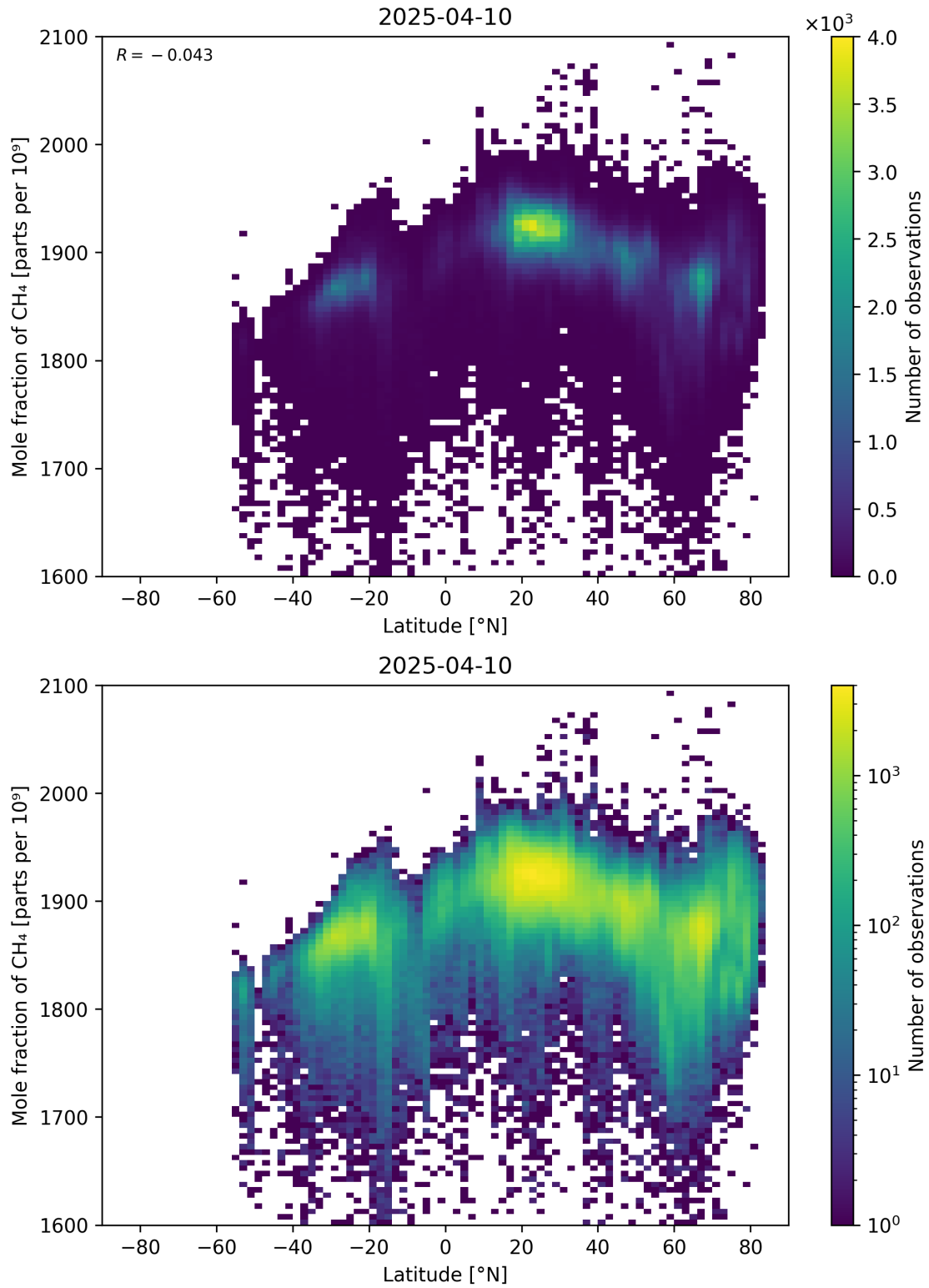
Figure 57: Scatter density plot of “Latitude” against “Mole fraction of CH 4 ” for 2025-04-09 to 2025-04-11.
