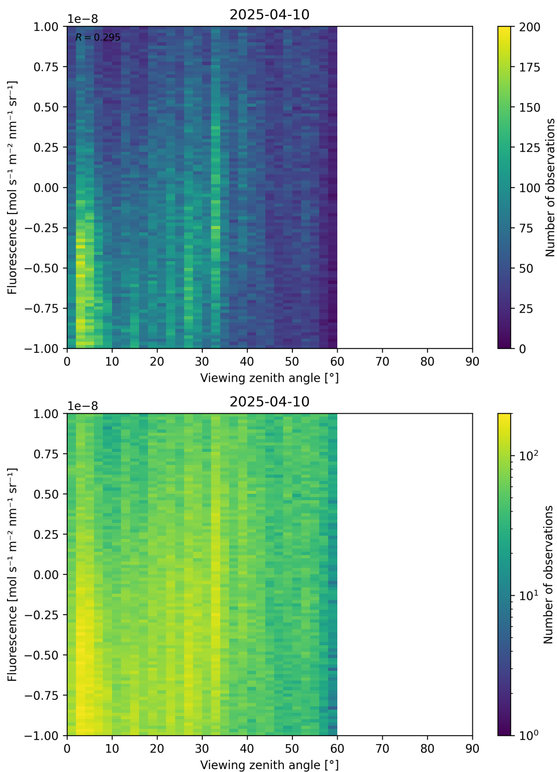
Figure 108: Scatter density plot of “Viewing zenith angle” against “Fluorescence” for 2025-04-09 to 2025-04-11.
