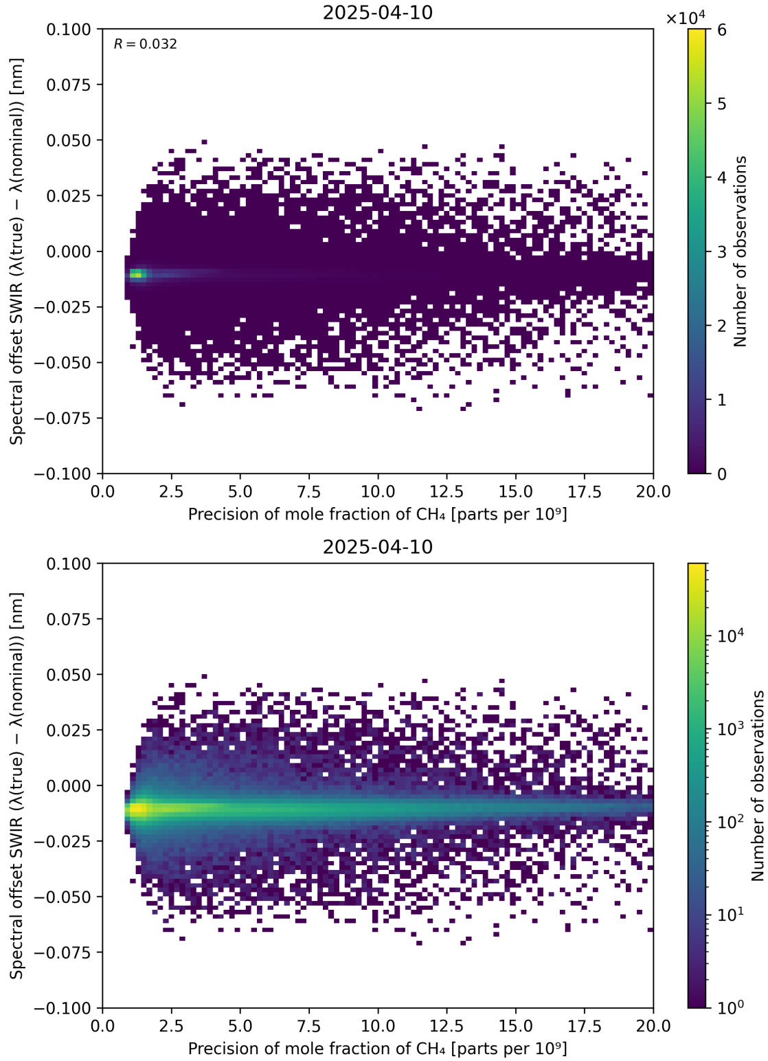
Figure 85: Scatter density plot of “Precision of mole fraction of CH 4 ” against “Spectral offset SWIR ( \lambda_{\text{true}} - \lambda_{\text{nominal}} )” for 2025-04-09 to 2025-04-11.
