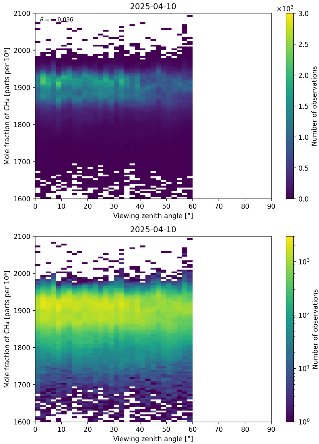
Figure 110: Scatter density plot of “Viewing zenith angle” against “Mole fraction of CH 4 ” for 2025-04-09 to 2025-04-11.
