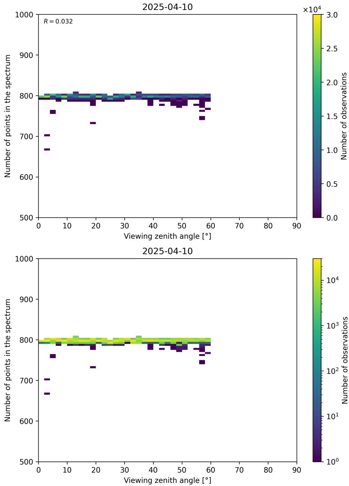
Figure 114: Scatter density plot of “Viewing zenith angle” against “Number of points in the spectrum” for 2025-04-09 to 2025-04-11.
