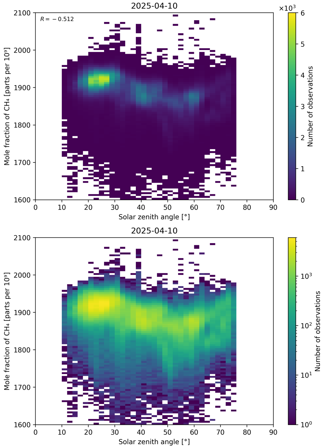
Figure 99: Scatter density plot of “Solar zenith angle” against “Mole fraction of CH 4 ” for 2025-04-09 to 2025-04-11.
