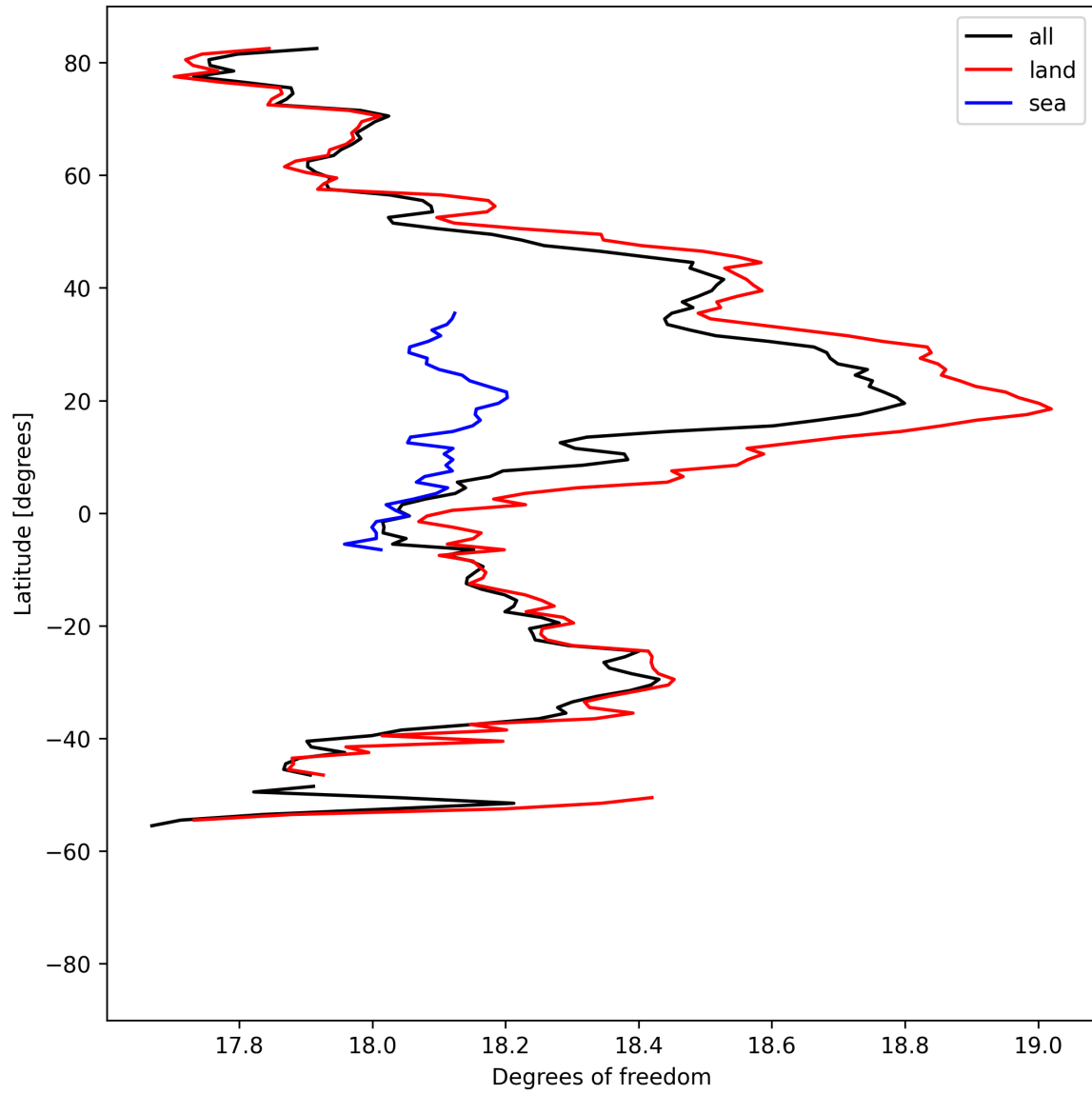
Figure 19: Zonal average of “Degrees of freedom” for 2025-04-09 to 2025-04-11.
