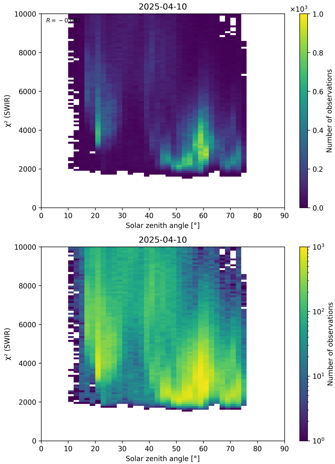
Figure 95: Scatter density plot of “Solar zenith angle” against “ \chi^2 (SWIR)” for 2025-04-09 to 2025-04-11.
