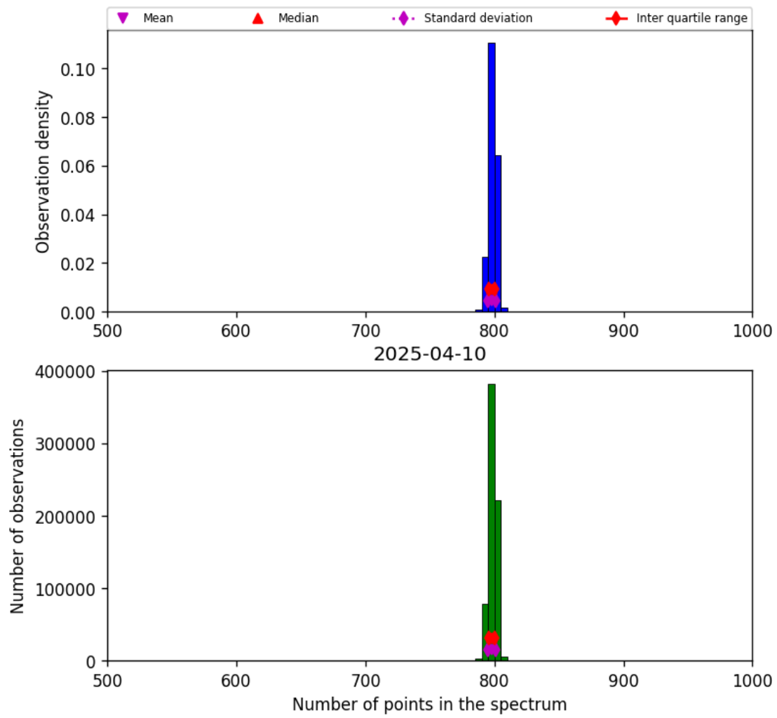
Figure 26: Histogram of “Number of points in the spectrum” for 2025-04-09 to 2025-04-11
