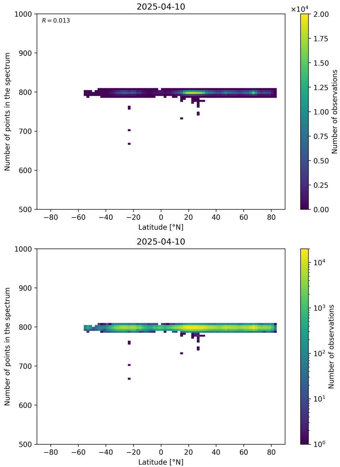
Figure 61: Scatter density plot of “Latitude” against “Number of points in the spectrum” for 2025-04-09 to 2025-04-11.
