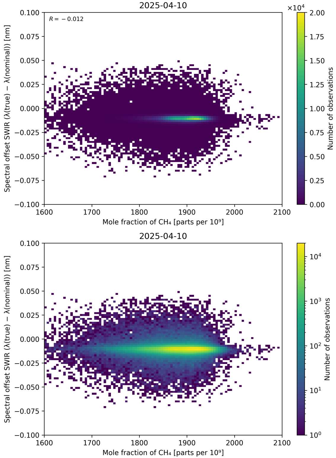
Figure 86: Scatter density plot of “Mole fraction of \text{CH}_4 ” against “Spectral offset SWIR ( \lambda_{\text{true}} - \lambda_{\text{nominal}} )” for 2025-04-09 to 2025-04-11.
