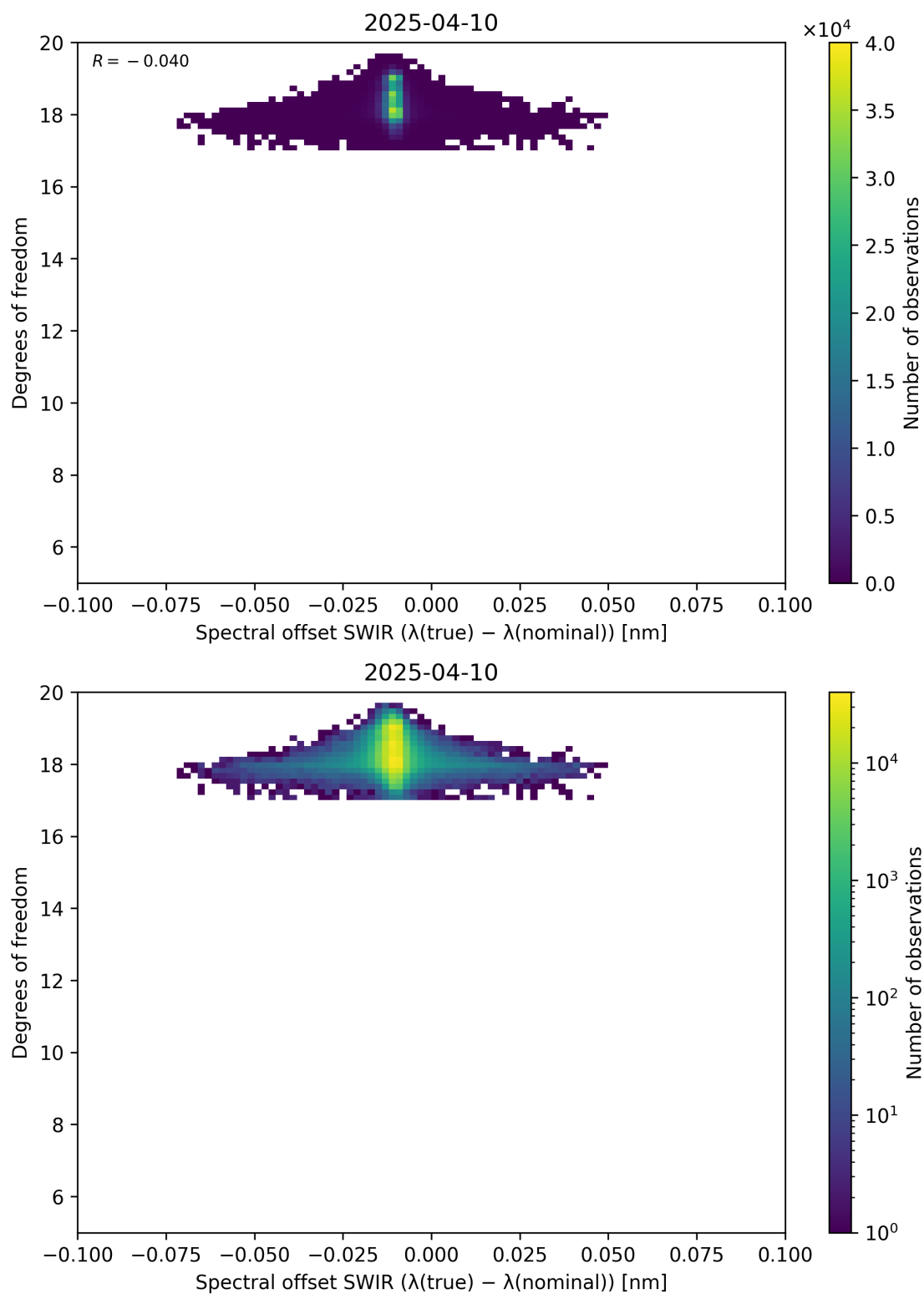
Figure 119: Scatter density plot of “Spectral offset SWIR ( \lambda_{\text{true}} - \lambda_{\text{nominal}} )” against “Degrees of freedom” for 2025-04-09 to 2025-04-11.
