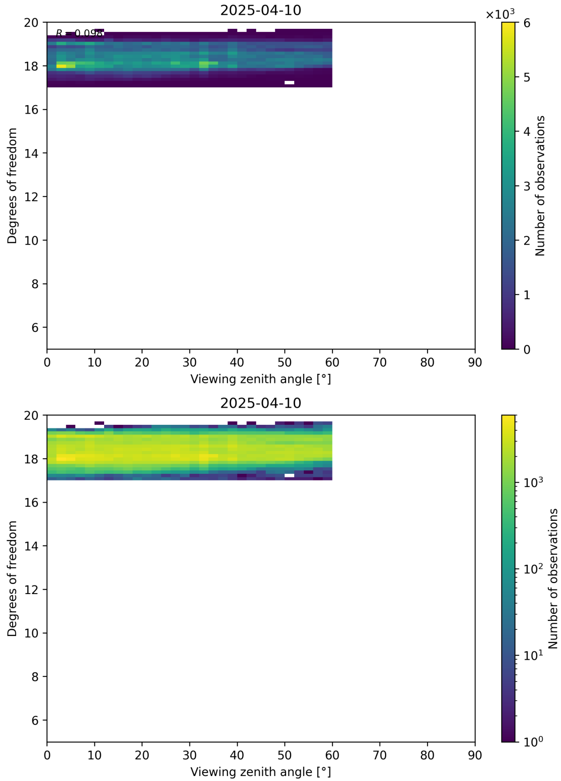
Figure 107: Scatter density plot of “Viewing zenith angle” against “Degrees of freedom” for 2025-04-09 to 2025-04-11.
