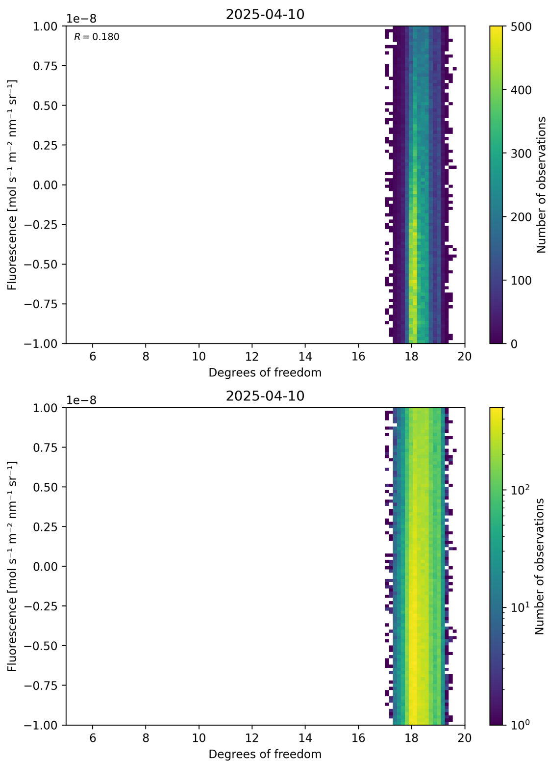
Figure 51: Scatter density plot of “Degrees of freedom” against “Fluorescence” for 2025-04-09 to 2025-04-11.
