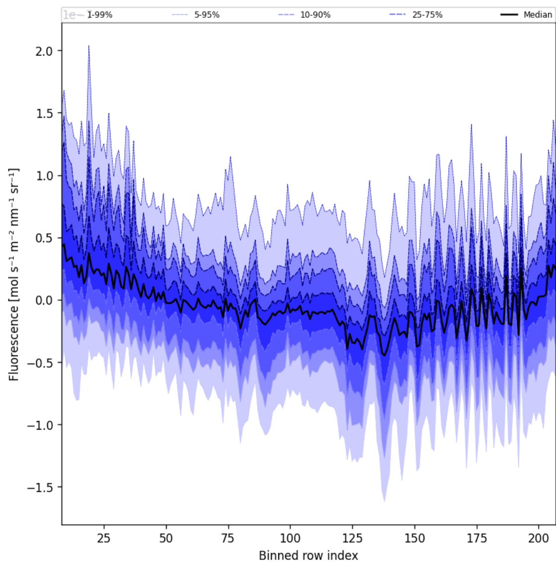
Figure 43: Along track statistics of “Fluorescence” for 2025-04-09 to 2025-04-11
