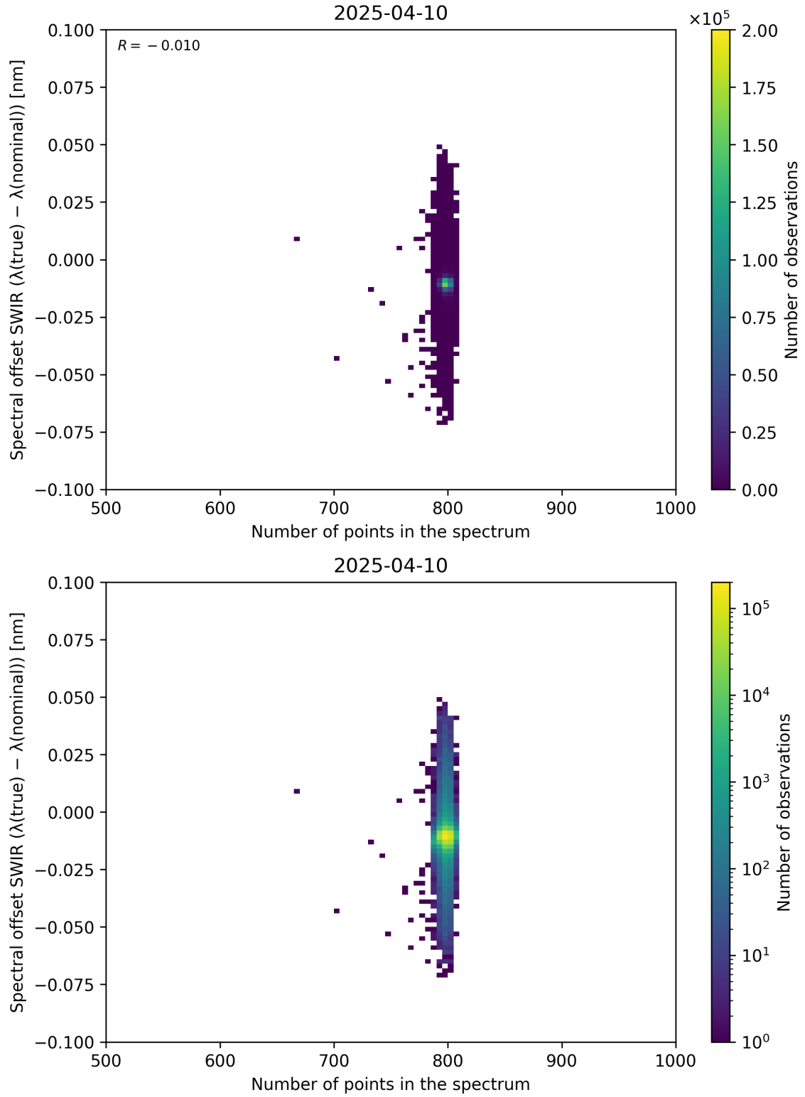
Figure 93: Scatter density plot of “Number of points in the spectrum” against “Spectral offset SWIR ( \lambda_{\text{true}} - \lambda_{\text{nominal}} )” for 2025-04-09 to 2025-04-11.
