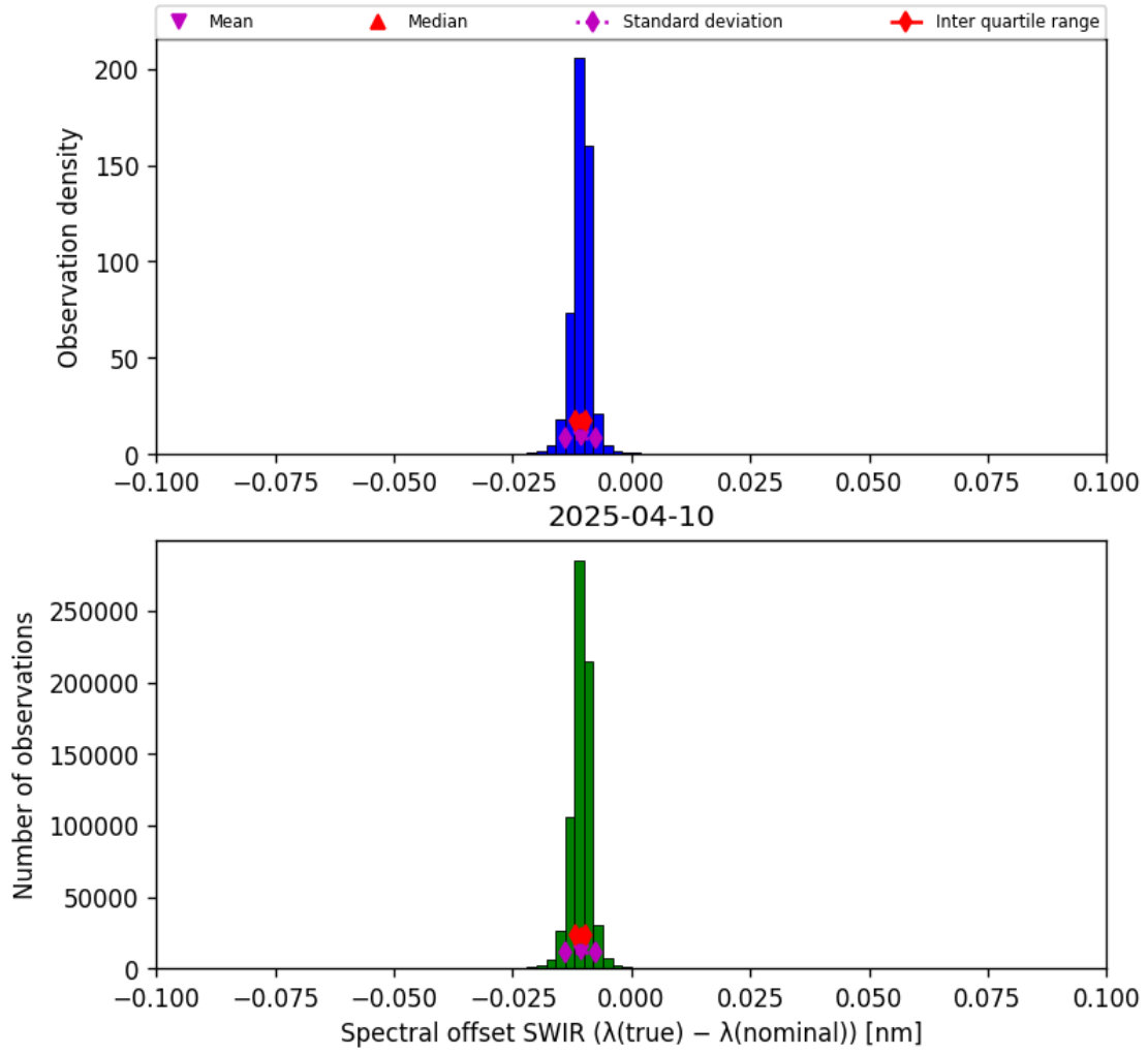
Figure 27: Histogram of “Spectral offset SWIR ( \lambda_{\text{true}} - \lambda_{\text{nominal}} )” for 2025-04-09 to 2025-04-11
