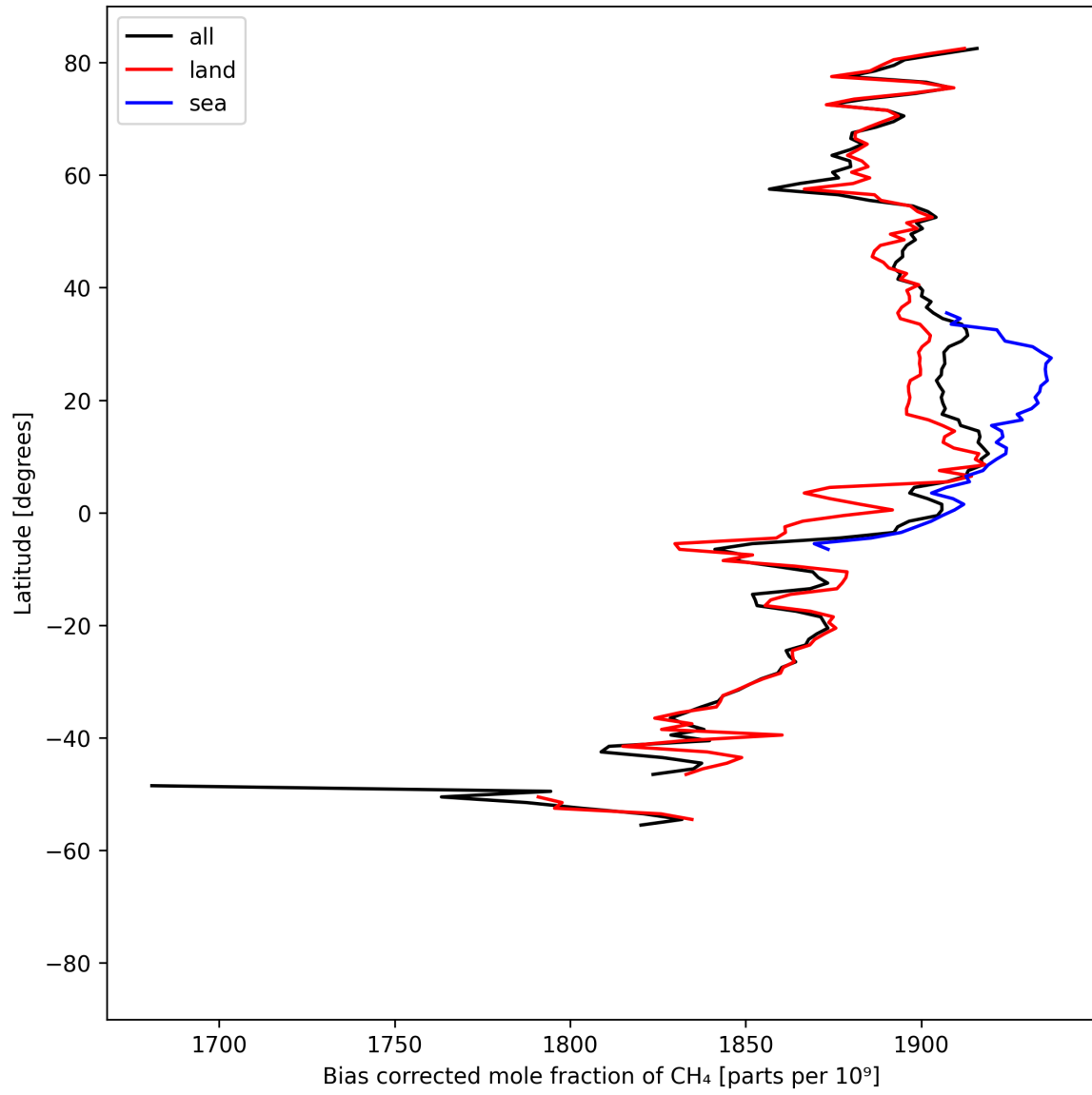
Figure 14: Zonal average of “Bias corrected mole fraction of \text{CH}_4 ” for 2025-04-09 to 2025-04-11.
