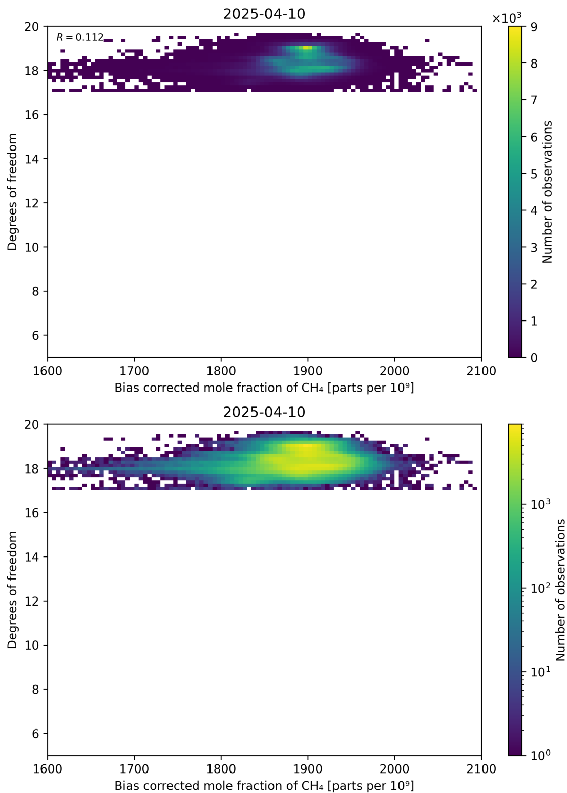
Figure 65: Scatter density plot of “Bias corrected mole fraction of CH 4 ” against “Degrees of freedom” for 2025-04-09 to 2025-04-11.
