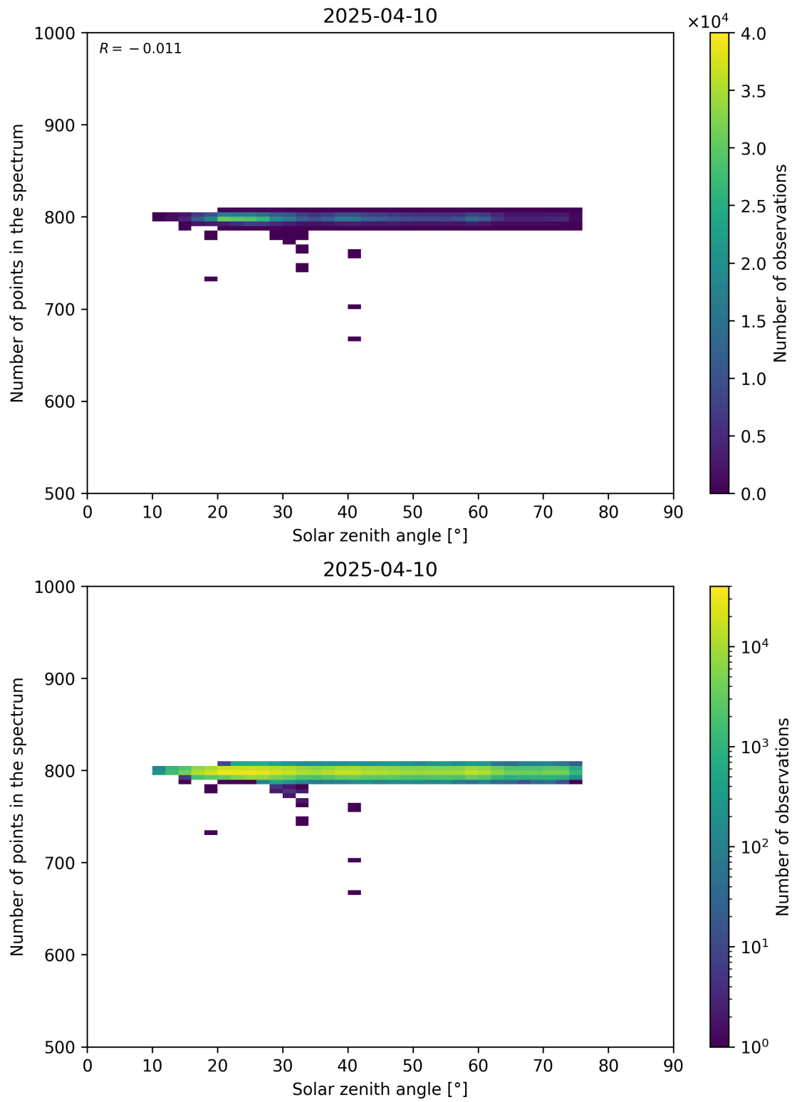
Figure 103: Scatter density plot of “Solar zenith angle” against “Number of points in the spectrum” for 2025-04-09 to 2025-04-11.
