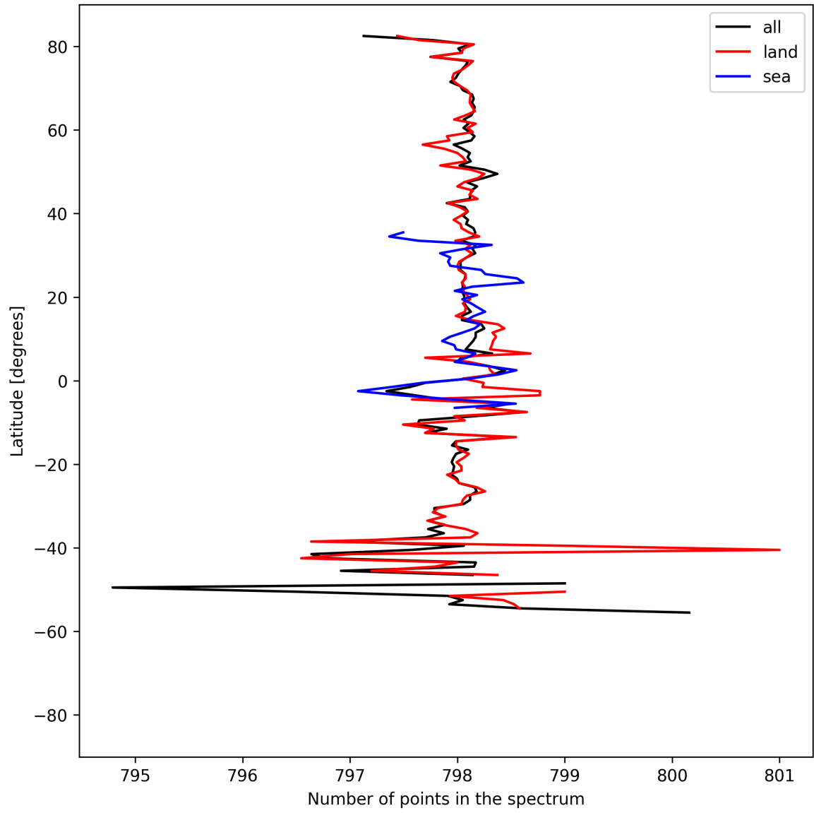
Figure 15: Zonal average of “Number of points in the spectrum” for 2025-04-09 to 2025-04-11.
