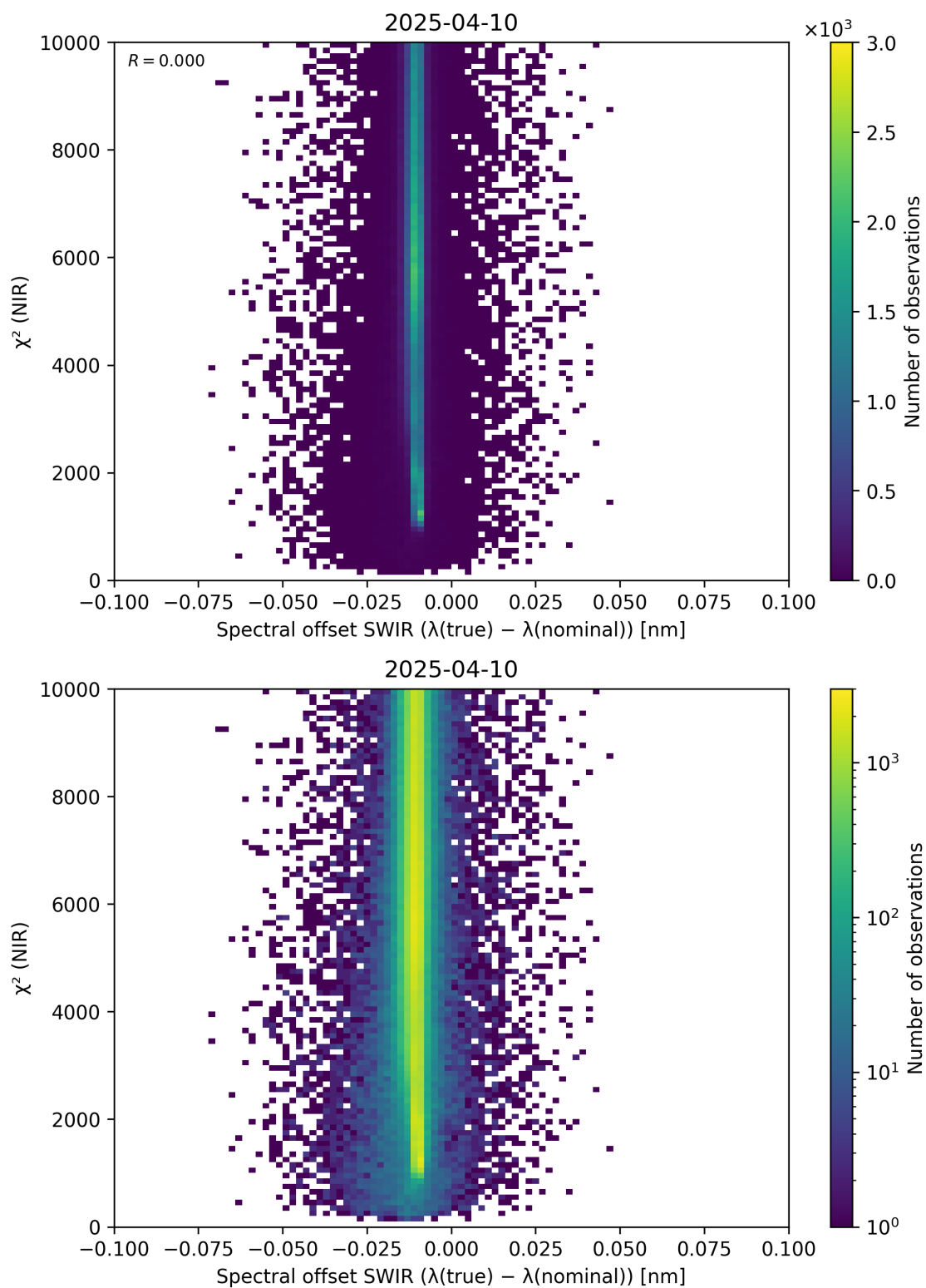
Figure 117: Scatter density plot of “Spectral offset SWIR ( \lambda_{\text{true}} - \lambda_{\text{nominal}} )” against “ \chi^2 (NIR)” for 2025-04-09 to 2025-04-11.
