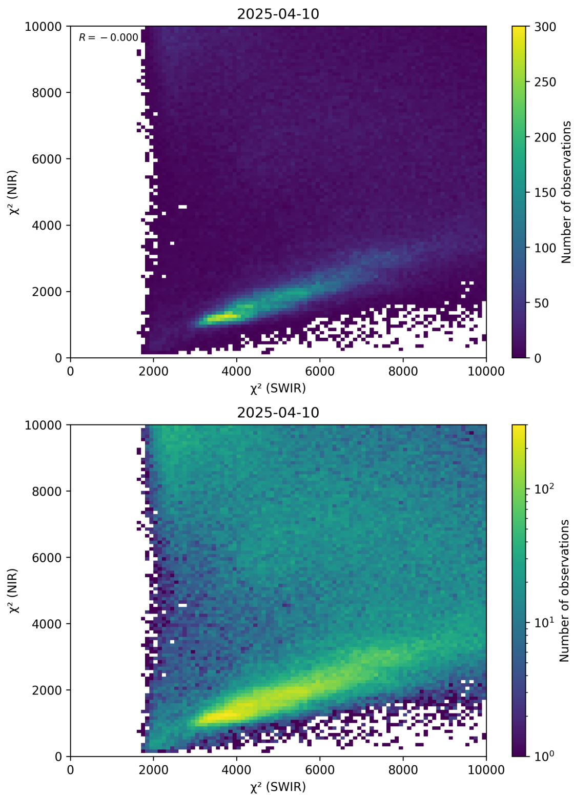
Figure 47: Scatter density plot of “ \chi^2 (SWIR)” against “ \chi^2 (NIR)” for 2025-04-09 to 2025-04-11.
