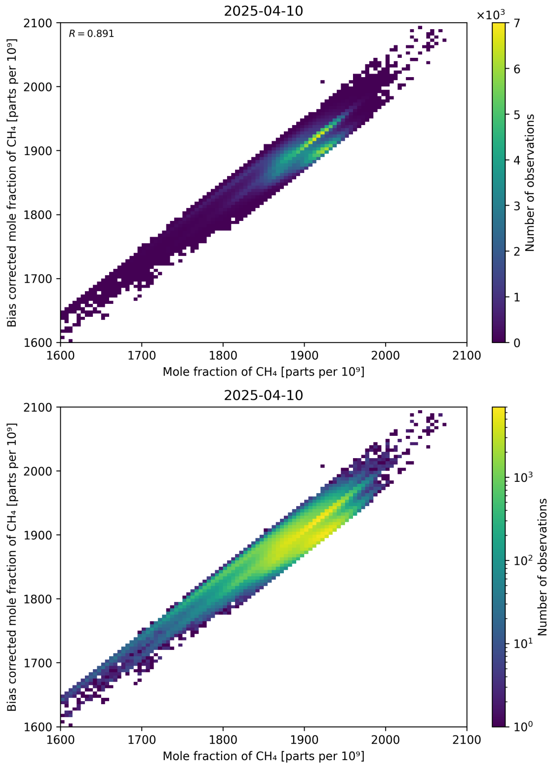
Figure 74: Scatter density plot of “Mole fraction of CH 4 ” against “Bias corrected mole fraction of CH 4 ” for 2025-04-09 to 2025-04-11.
