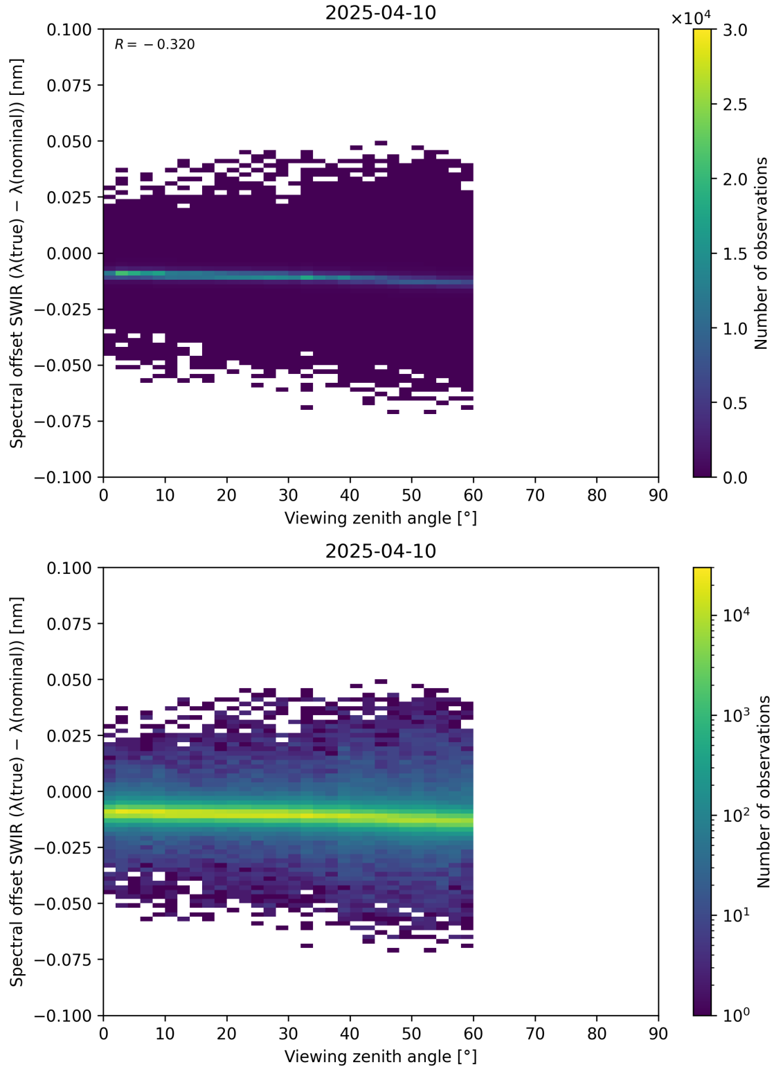
Figure 116: Scatter density plot of “Viewing zenith angle” against “Spectral offset SWIR ( \lambda_{\text{true}} - \lambda_{\text{nominal}} )” for 2025-04-09 to 2025-04-11.
