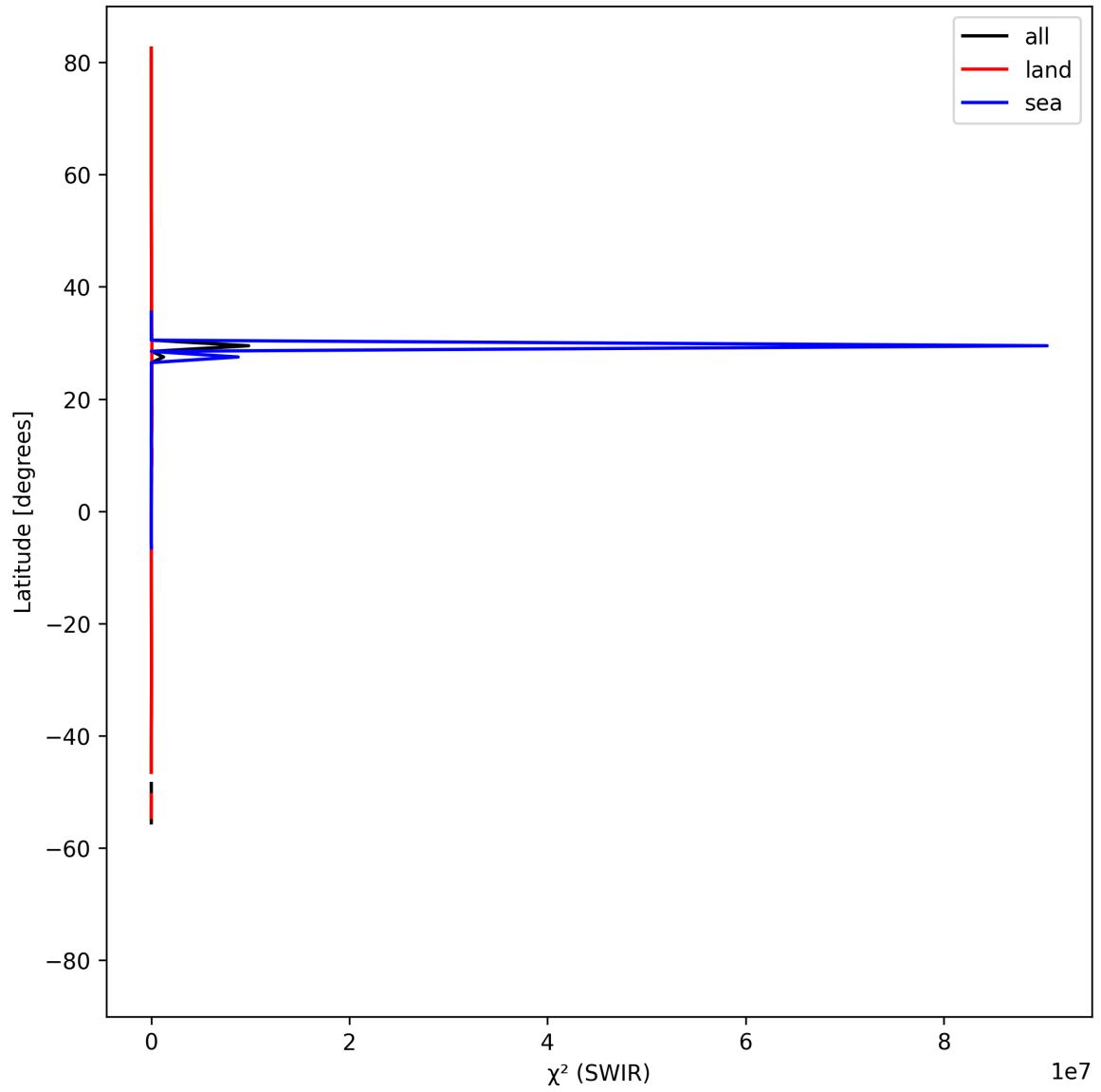
Figure 17: Zonal average of “ \chi^2 (SWIR)” for 2025-04-09 to 2025-04-11.
