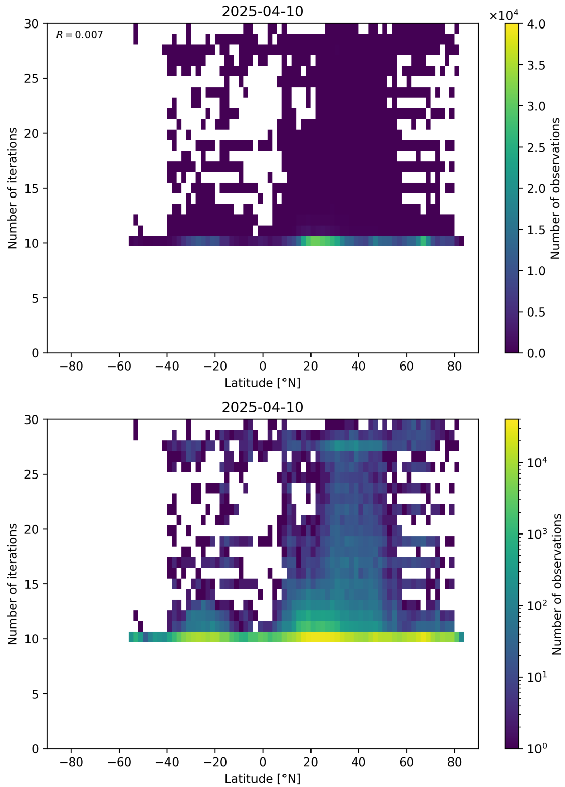
Figure 60: Scatter density plot of “Latitude” against “Number of iterations” for 2025-04-09 to 2025-04-11.
