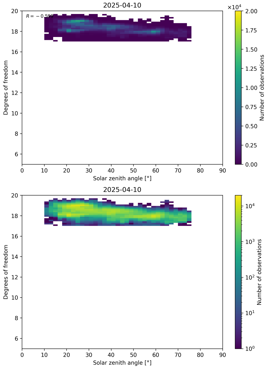
Figure 96: Scatter density plot of “Solar zenith angle” against “Degrees of freedom” for 2025-04-09 to 2025-04-11.
