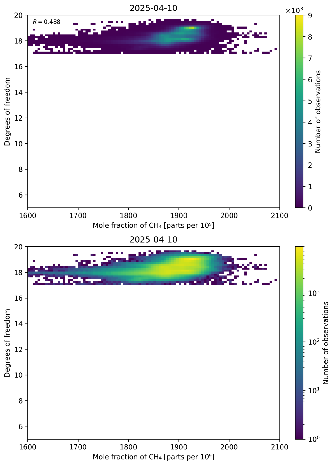
Figure 72: Scatter density plot of “Mole fraction of CH 4 ” against “Degrees of freedom” for 2025-04-09 to 2025-04-11.
