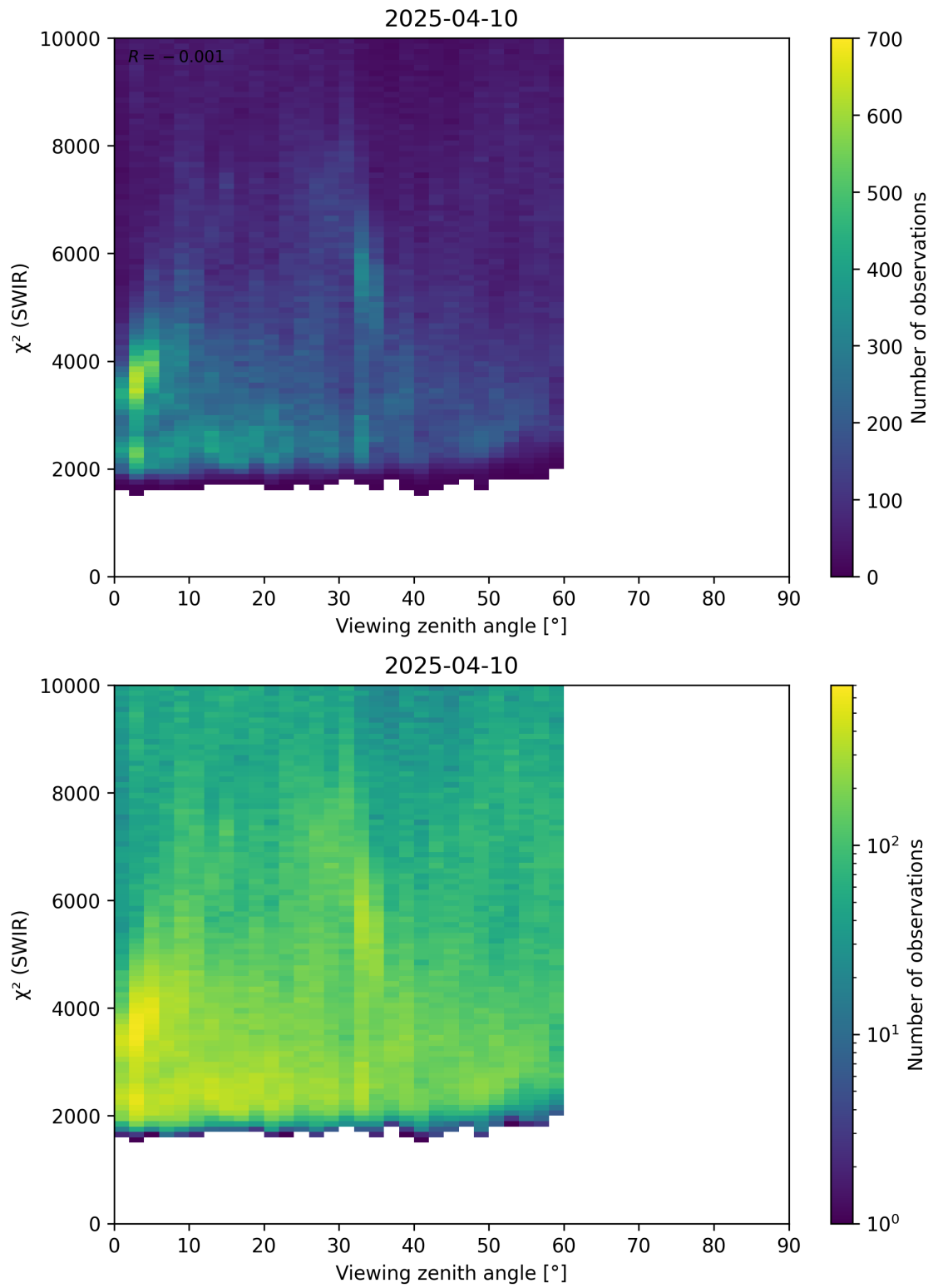
Figure 106: Scatter density plot of “Viewing zenith angle” against “ \chi^2 (SWIR)” for 2025-04-09 to 2025-04-11.
