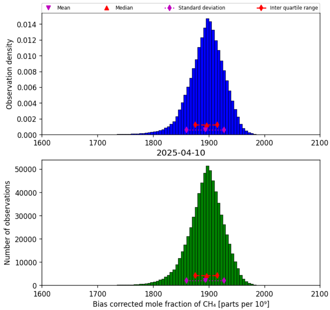
Figure 25: Histogram of “Bias corrected mole fraction of CH 4 ” for 2025-04-09 to 2025-04-11
