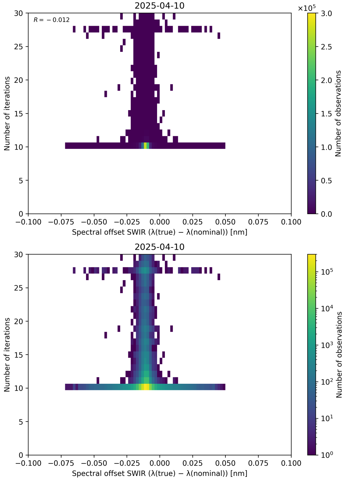
Figure 121: Scatter density plot of “Spectral offset SWIR ( \lambda_{\text{true}} - \lambda_{\text{nominal}} )” against “Number of iterations” for 2025-04-09 to 2025-04-11.
