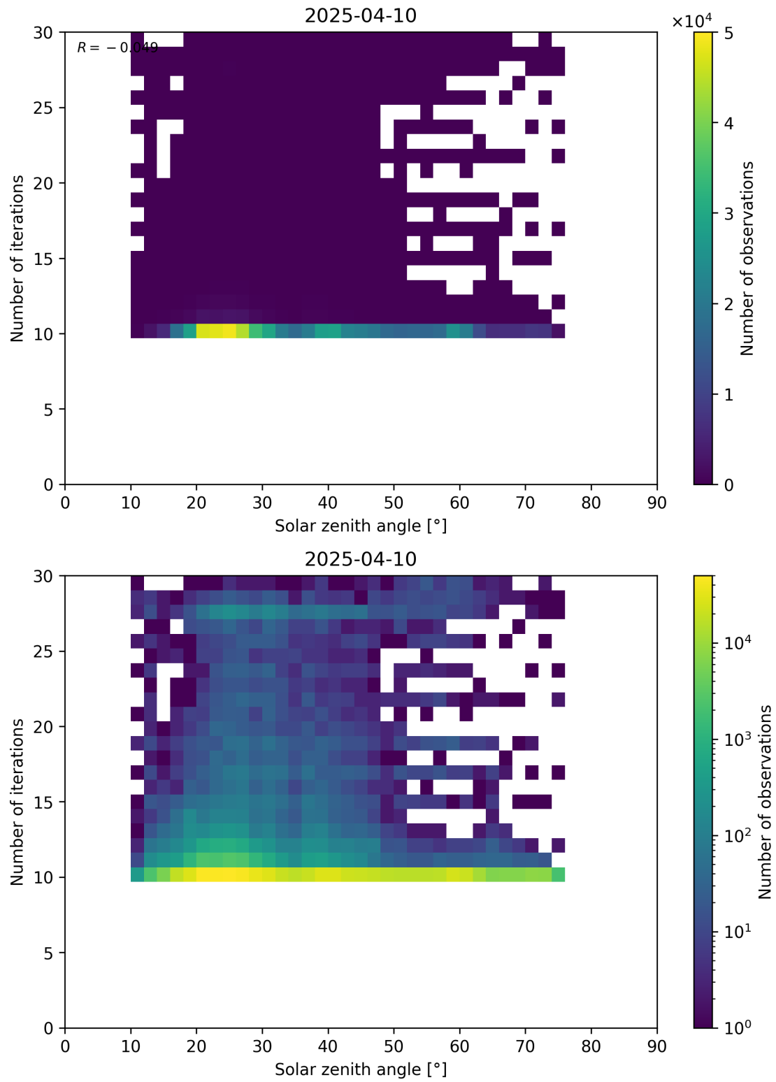
Figure 102: Scatter density plot of “Solar zenith angle” against “Number of iterations” for 2025-04-09 to 2025-04-11.
