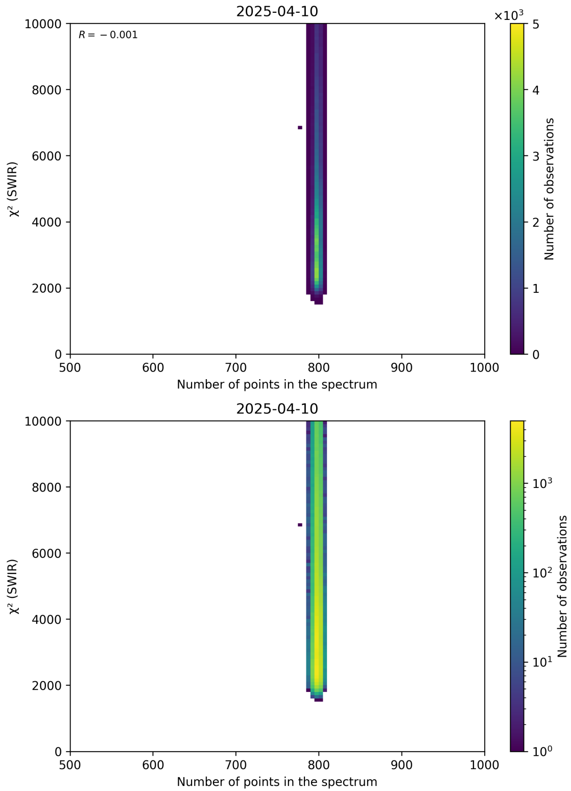
Figure 89: Scatter density plot of “Number of points in the spectrum” against “ \chi^2 (SWIR)” for 2025-04-09 to 2025-04-11.
