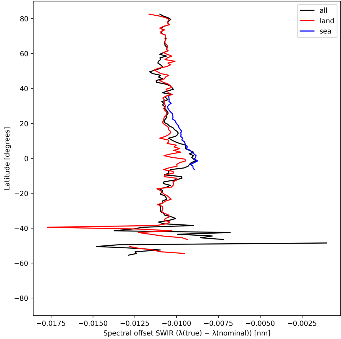
Figure 16: Zonal average of “Spectral offset SWIR ( \lambda_{\text{true}} - \lambda_{\text{nominal}} )” for 2025-04-09 to 2025-04-11.
