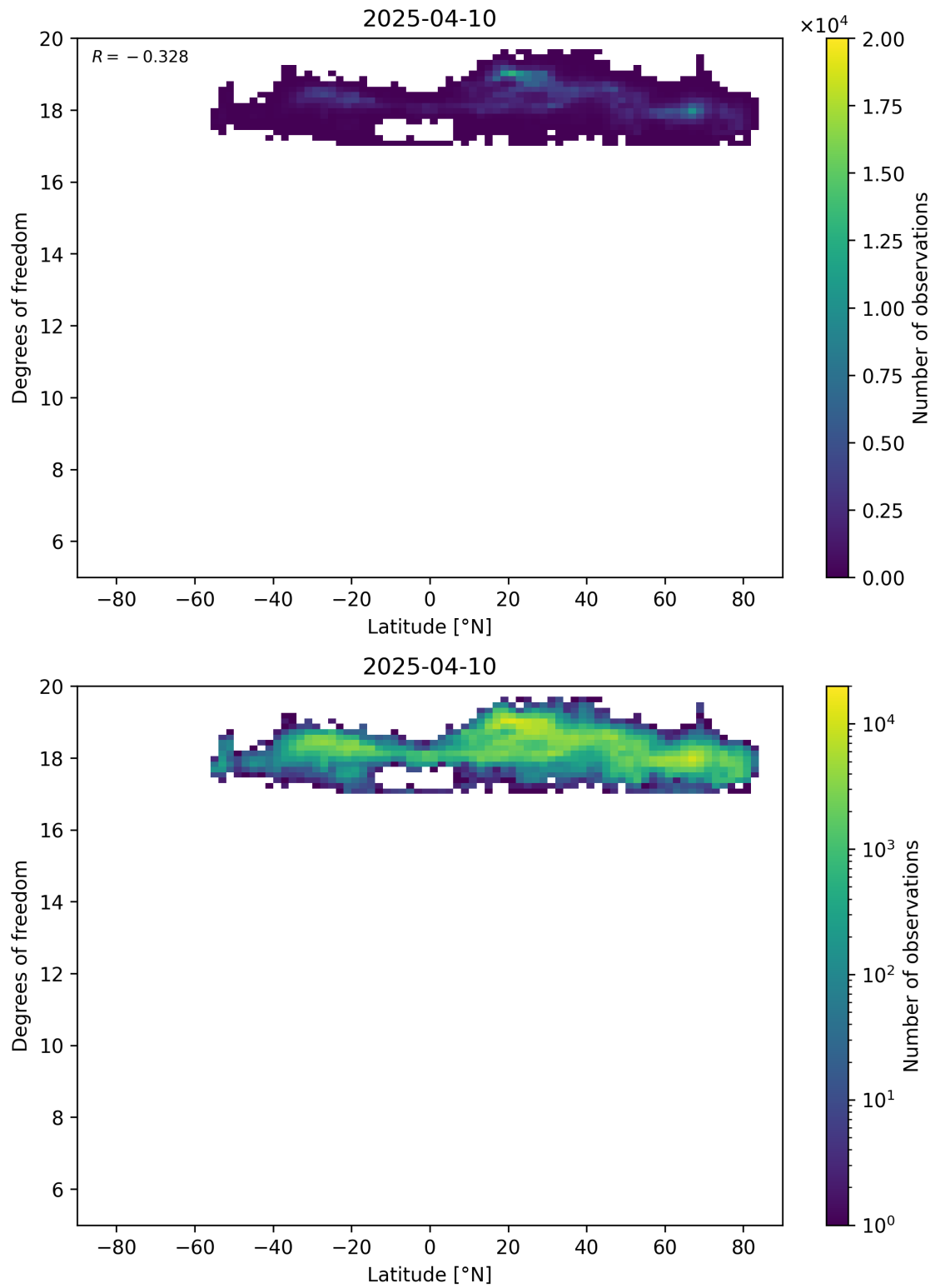
Figure 55: Scatter density plot of “Latitude” against “Degrees of freedom” for 2025-04-09 to 2025-04-11.
