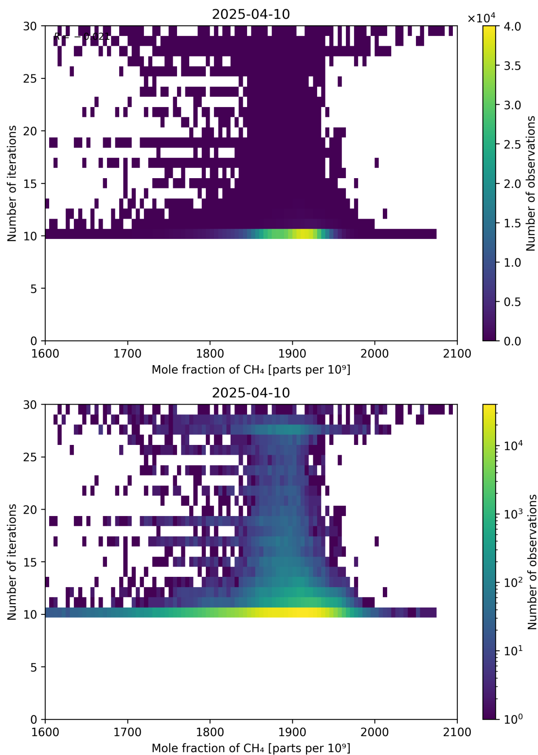
Figure 76: Scatter density plot of “Mole fraction of CH 4 ” against “Number of iterations” for 2025-04-09 to 2025-04-11.
