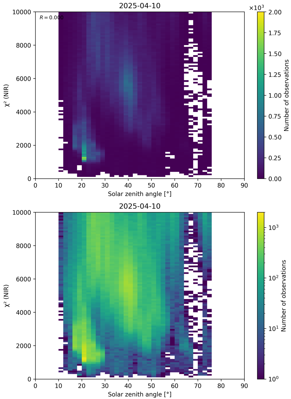
Figure 94: Scatter density plot of “Solar zenith angle” against “ \chi^2 (NIR)” for 2025-04-09 to 2025-04-11.
