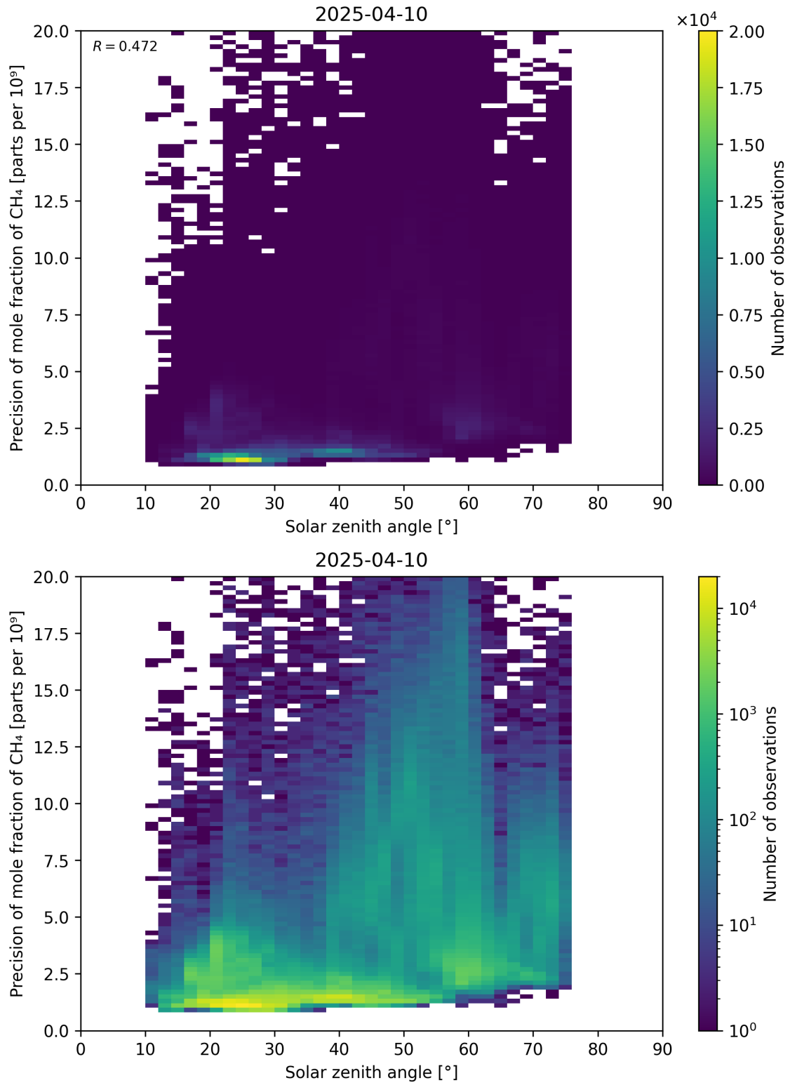
Figure 101: Scatter density plot of “Solar zenith angle” against “Precision of mole fraction of CH 4 ” for 2025-04-09 to 2025-04-11.
