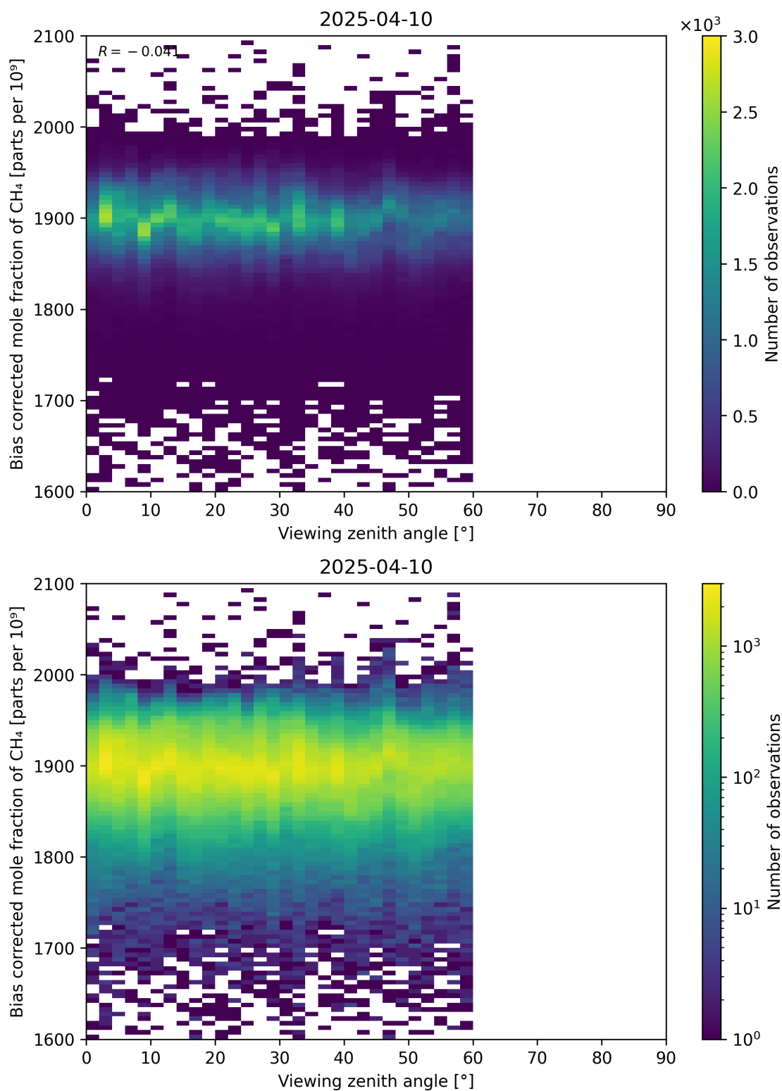
Figure 111: Scatter density plot of “Viewing zenith angle” against “Bias corrected mole fraction of CH 4 ” for 2025-04-09 to 2025-04-11.
