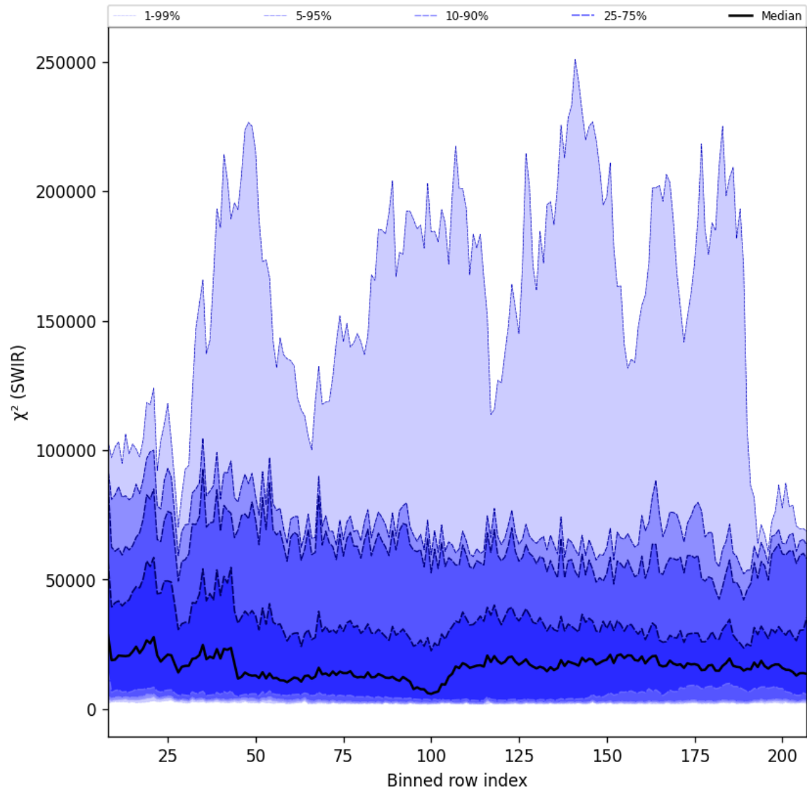
Figure 39: Along track statistics of “ \chi^2 (SWIR)” for 2025-04-10 to 2025-04-12
