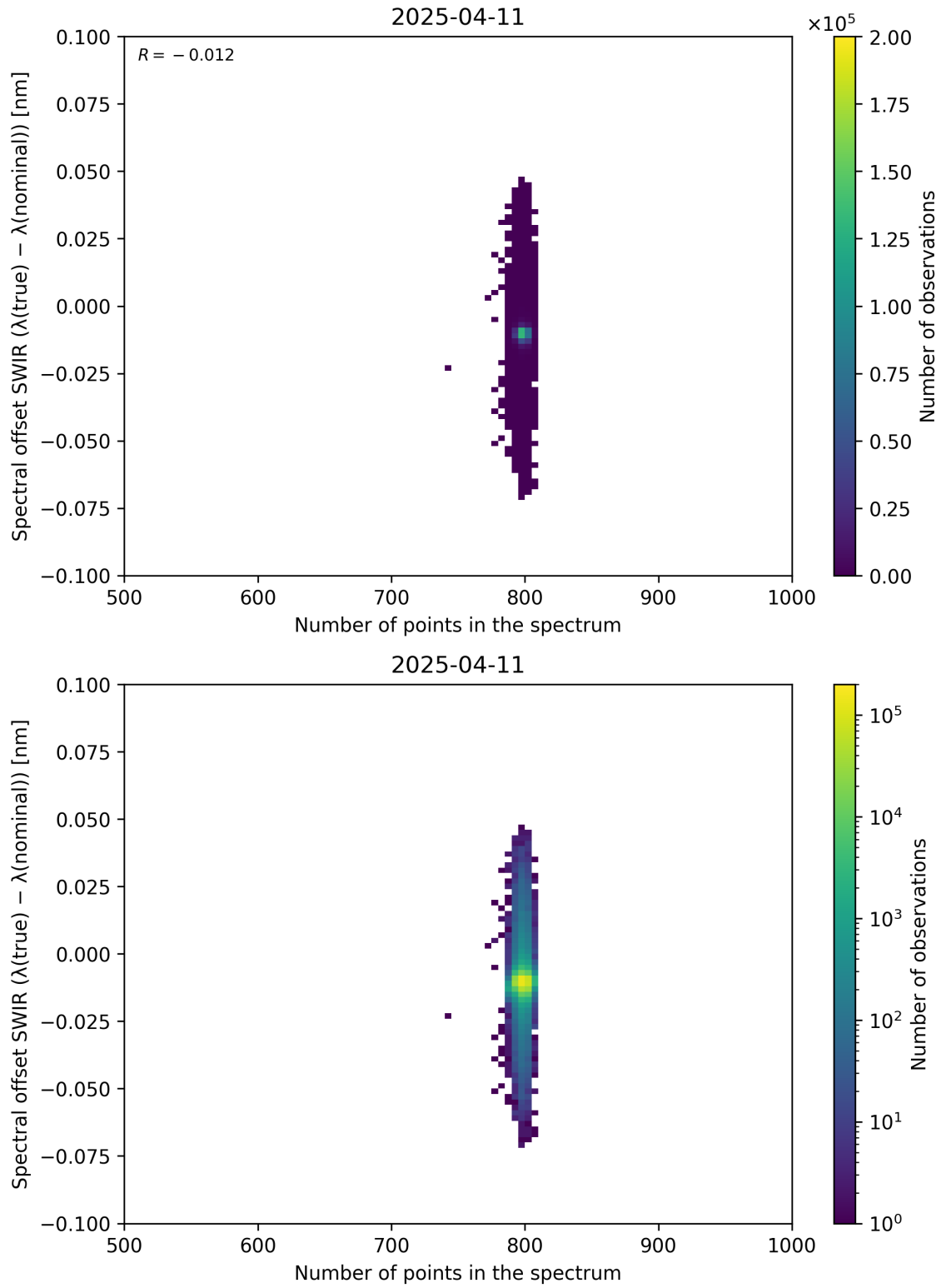
Figure 93: Scatter density plot of “Number of points in the spectrum” against “Spectral offset SWIR ( \lambda_{\text{true}} - \lambda_{\text{nominal}} )” for 2025-04-10 to 2025-04-12.
