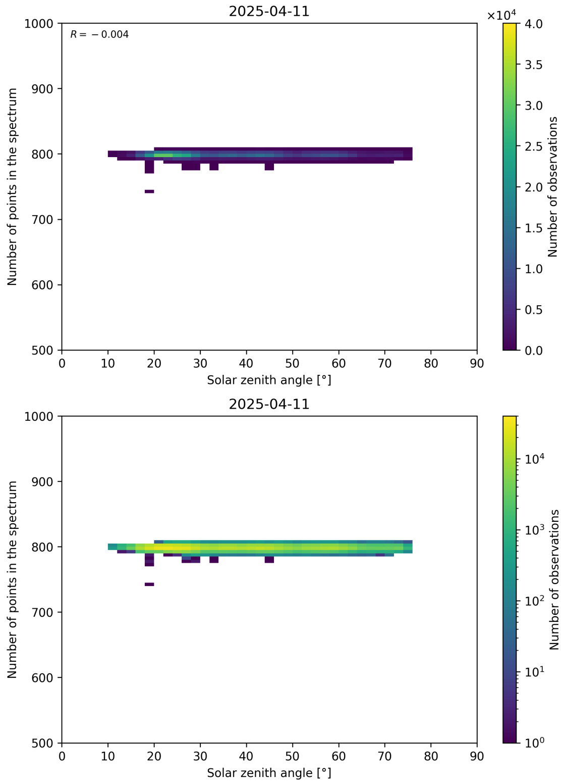
Figure 103: Scatter density plot of “Solar zenith angle” against “Number of points in the spectrum” for 2025-04-10 to 2025-04-12.
