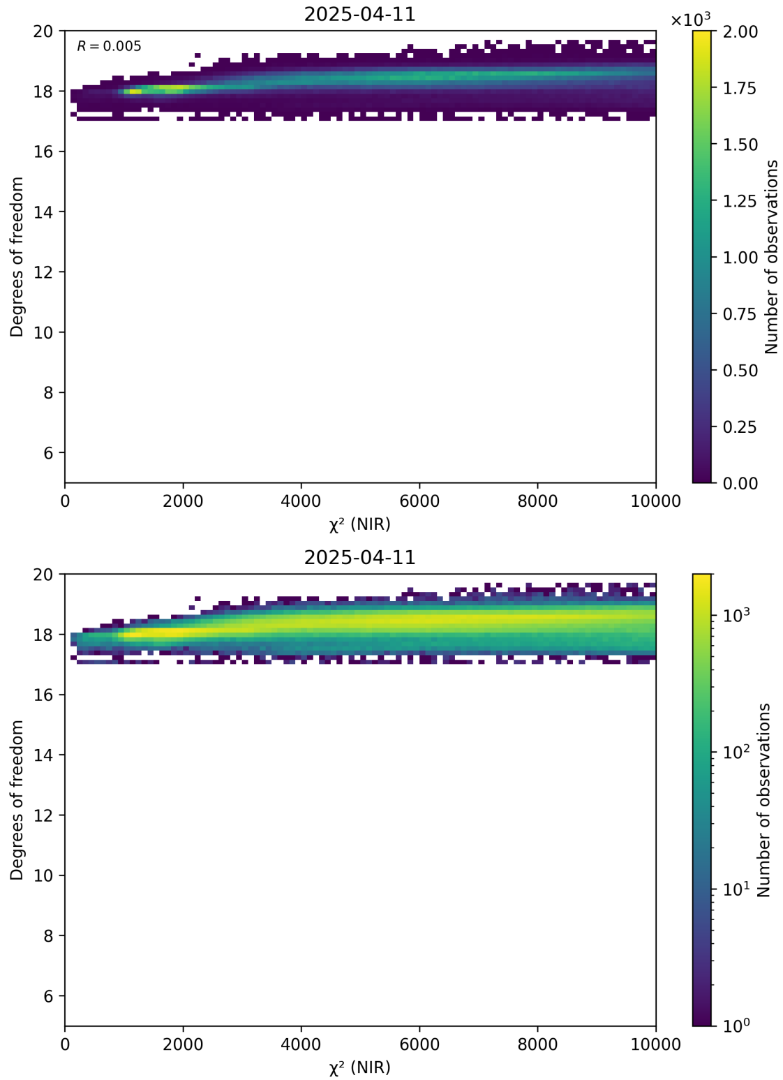
Figure 44: Scatter density plot of “ \chi^2 (NIR)” against “Degrees of freedom” for 2025-04-10 to 2025-04-12.
