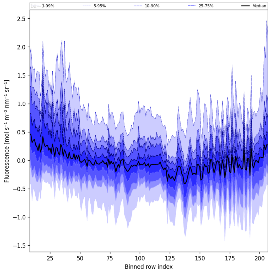
Figure 43: Along track statistics of “Fluorescence” for 2025-04-10 to 2025-04-12
