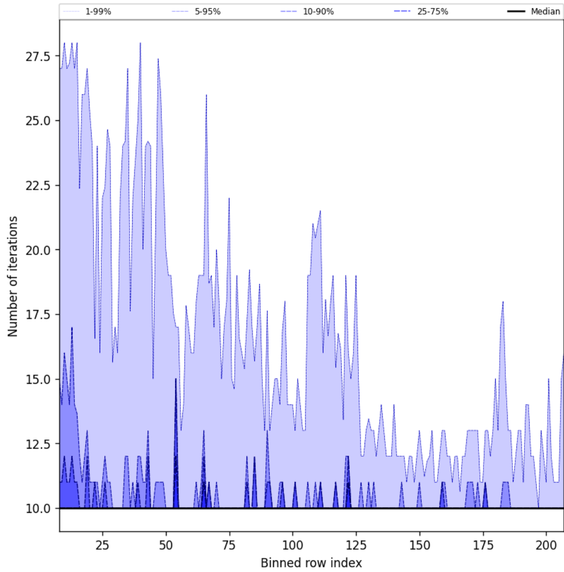
Figure 42: Along track statistics of “Number of iterations” for 2025-04-10 to 2025-04-12
