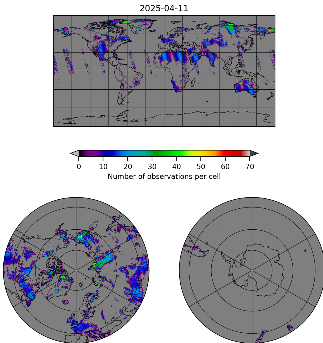
Figure 10: Map of the number of observations for 2025-04-10 to 2025-04-12
