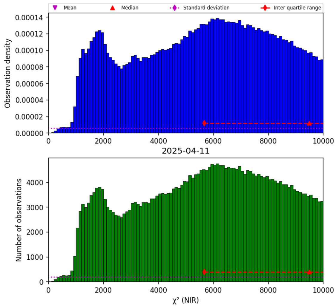
Figure 29: Histogram of “ \chi^2 (NIR)” for 2025-04-10 to 2025-04-12
