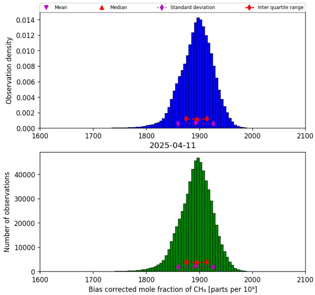
Figure 25: Histogram of “Bias corrected mole fraction of CH 4 ” for 2025-04-10 to 2025-04-12
