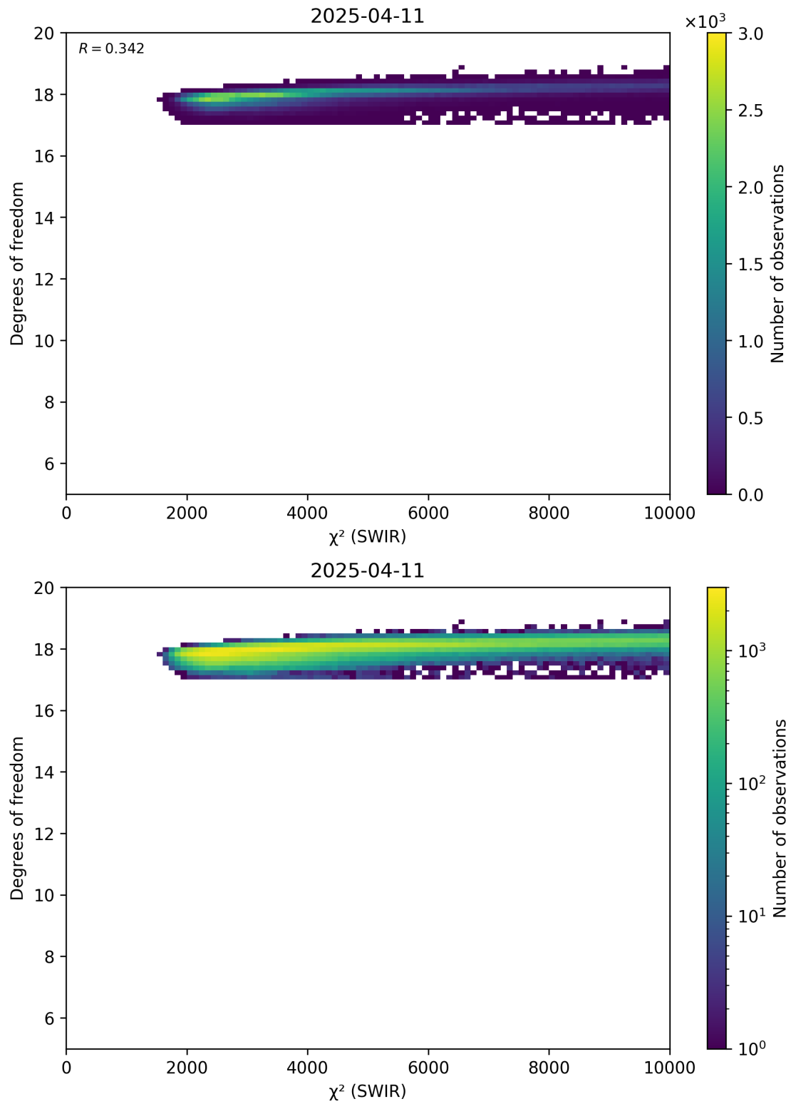
Figure 48: Scatter density plot of " \chi^2 (SWIR)" against "Degrees of freedom" for 2025-04-10 to 2025-04-12.
