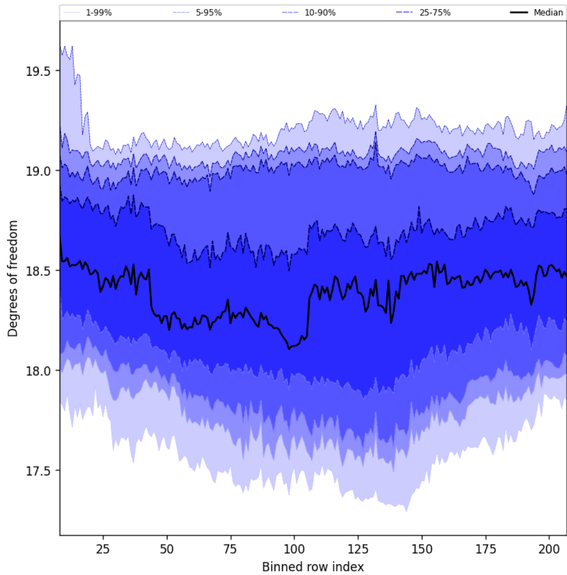
Figure 41: Along track statistics of “Degrees of freedom” for 2025-04-10 to 2025-04-12
