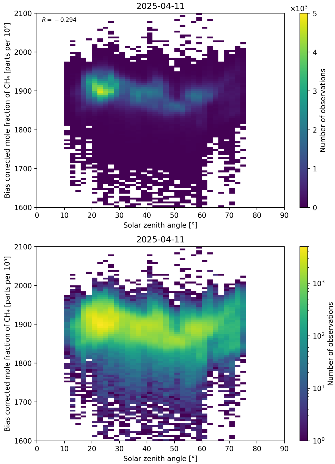
Figure 100: Scatter density plot of “Solar zenith angle” against “Bias corrected mole fraction of CH 4 ” for 2025-04-10 to 2025-04-12.
