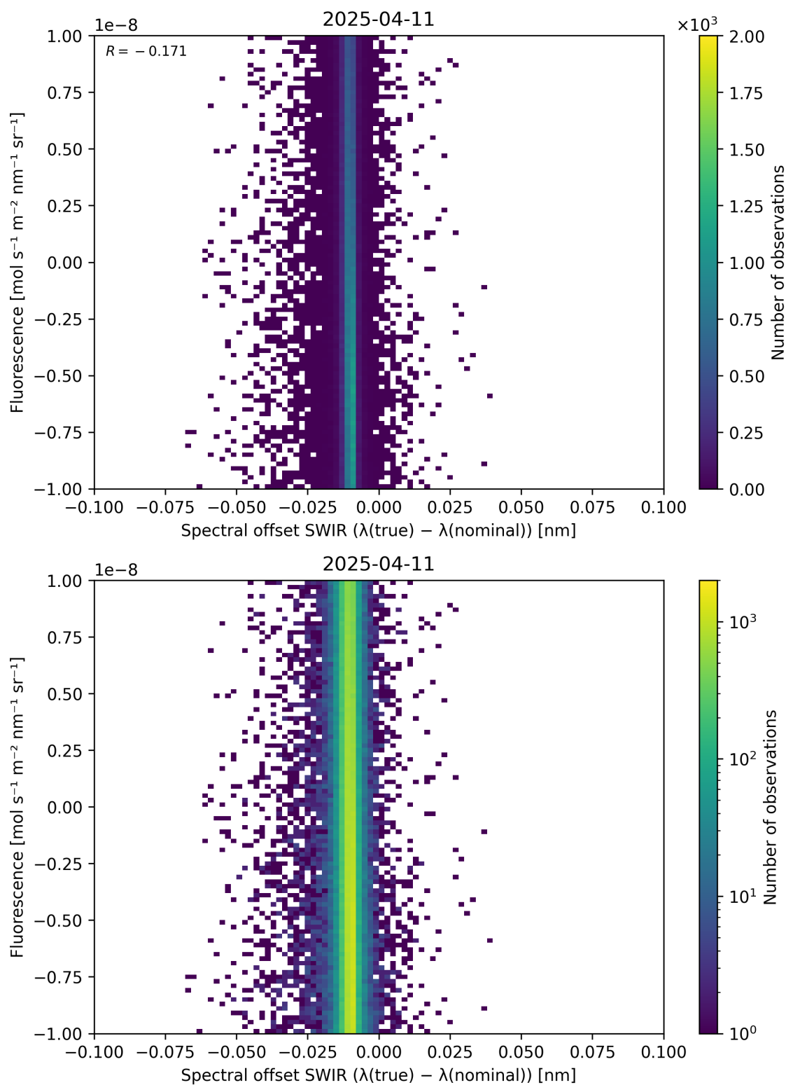
Figure 120: Scatter density plot of “Spectral offset SWIR ( \lambda_{\text{true}} - \lambda_{\text{nominal}} )” against “Fluorescence” for 2025-04-10 to 2025-04-12.
