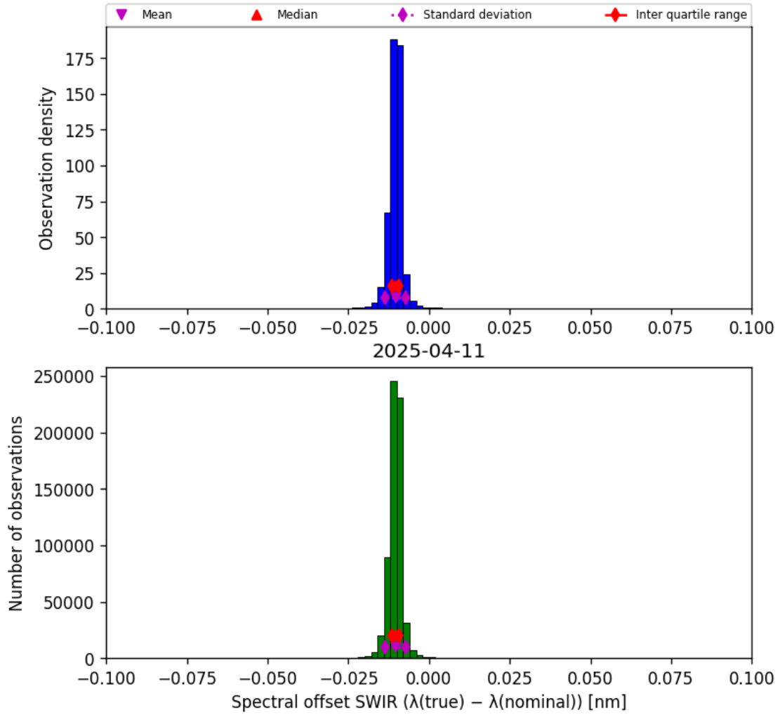
Figure 27: Histogram of “Spectral offset SWIR ( \lambda_{\text{true}} - \lambda_{\text{nominal}} )” for 2025-04-10 to 2025-04-12
