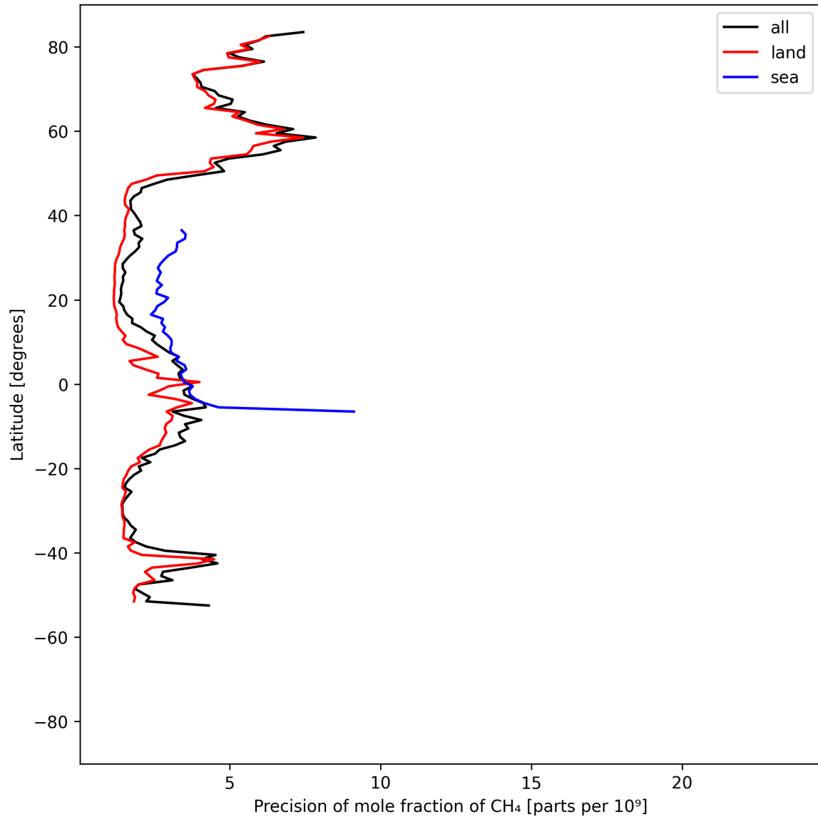
Figure 13: Zonal average of “Precision of mole fraction of CH 4 ” for 2025-04-10 to 2025-04-12.
