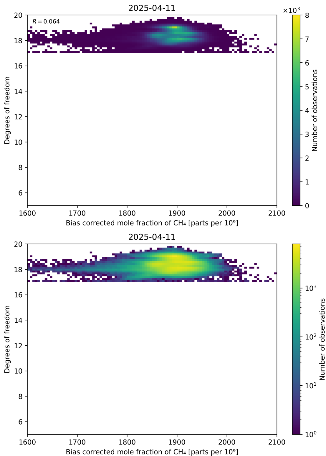
Figure 65: Scatter density plot of “Bias corrected mole fraction of CH 4 ” against “Degrees of freedom” for 2025-04-10 to 2025-04-12.
