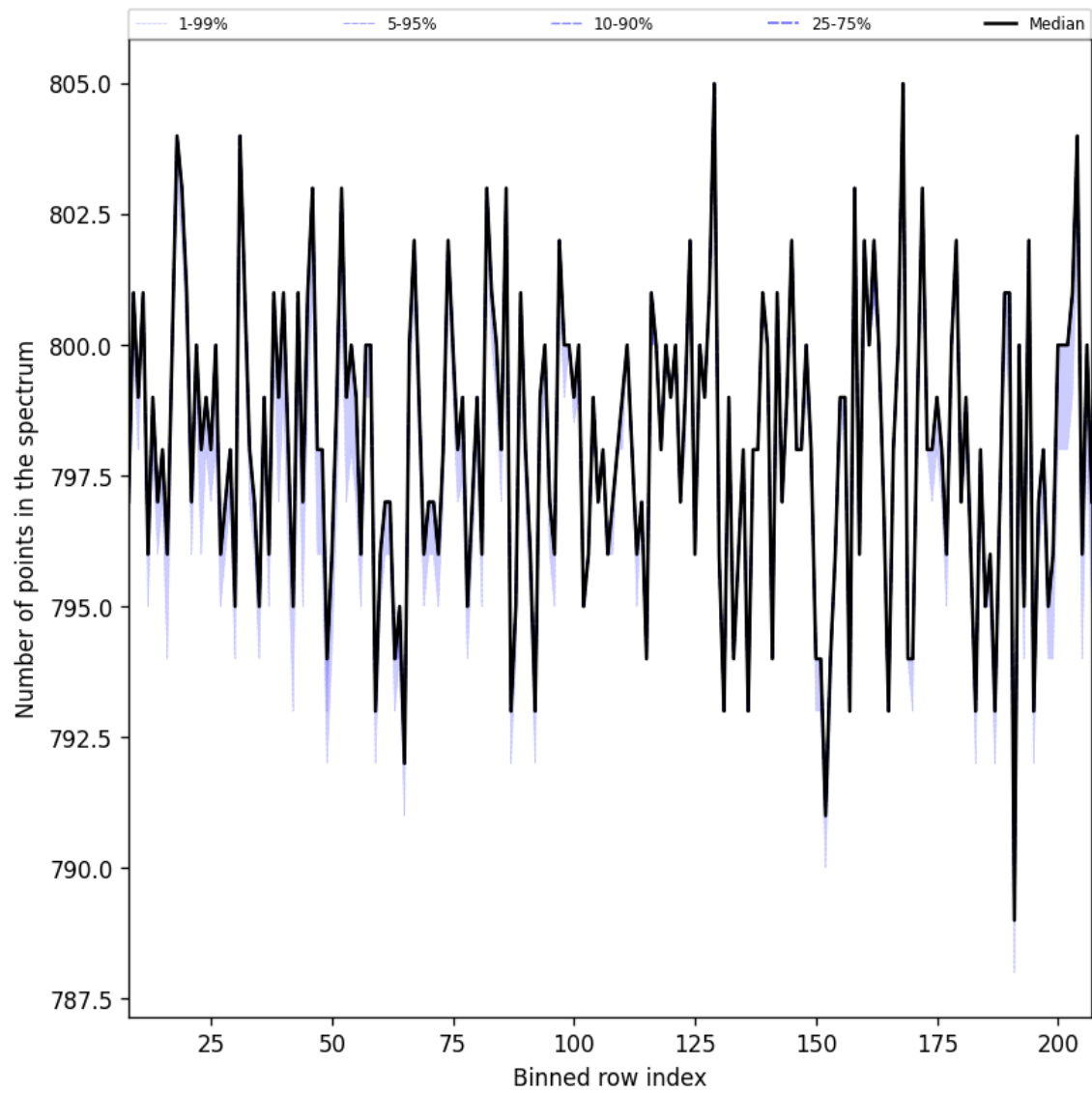
Figure 37: Along track statistics of “Number of points in the spectrum” for 2025-04-10 to 2025-04-12
