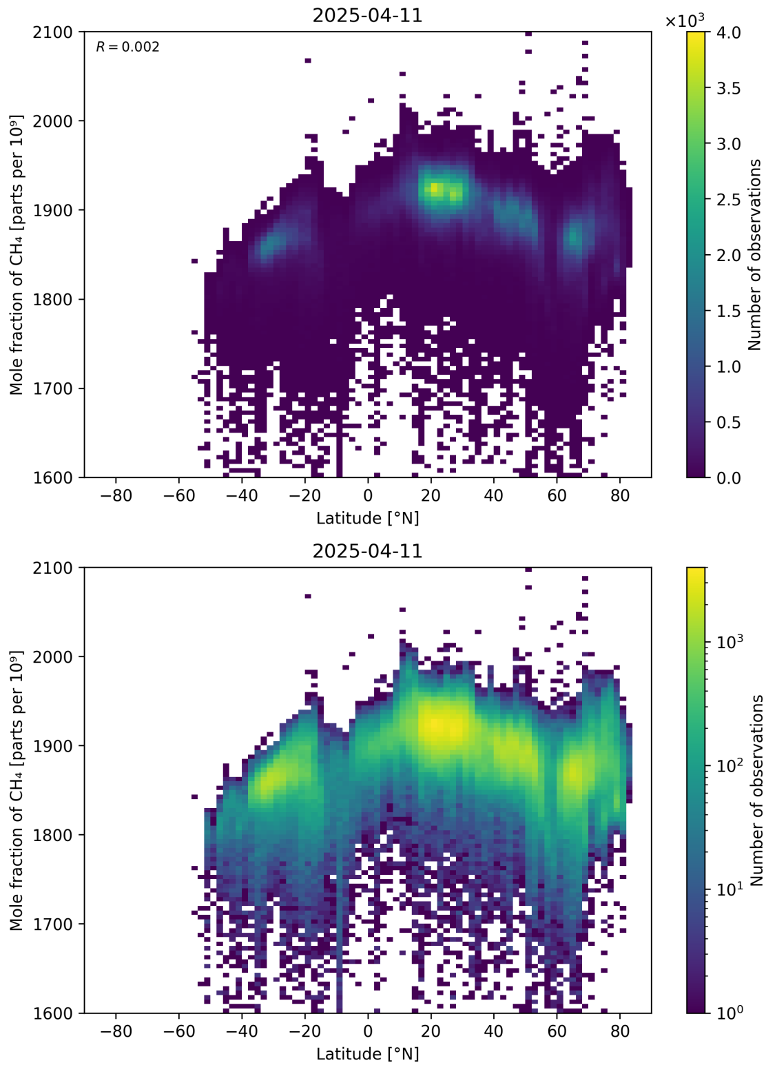
Figure 57: Scatter density plot of “Latitude” against “Mole fraction of \text{CH}_4 ” for 2025-04-10 to 2025-04-12.
