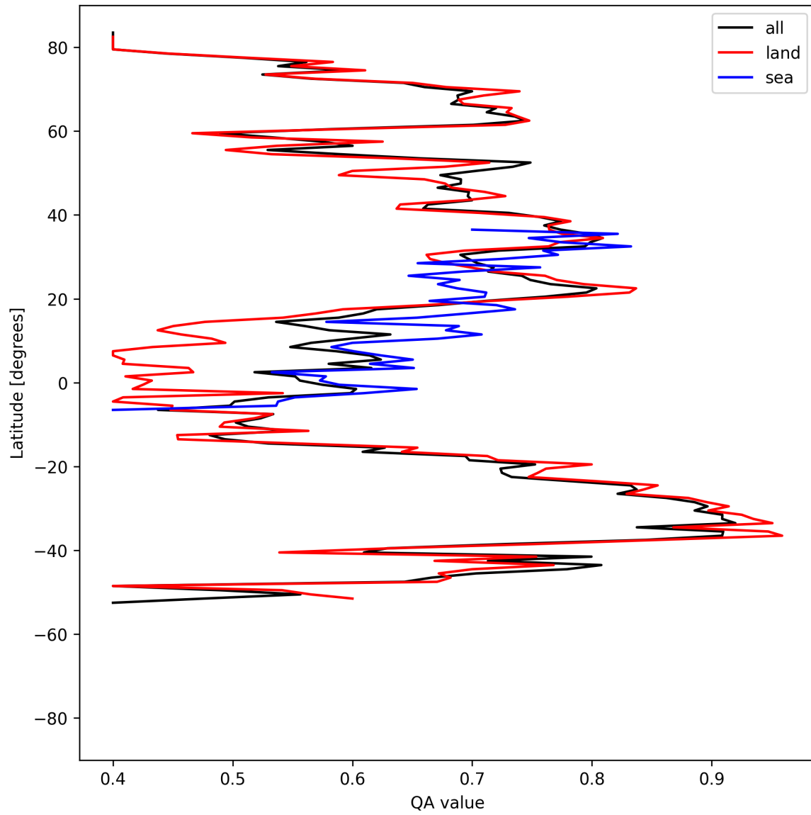
Figure 11: Zonal average of “QA value” for 2025-04-10 to 2025-04-12.
