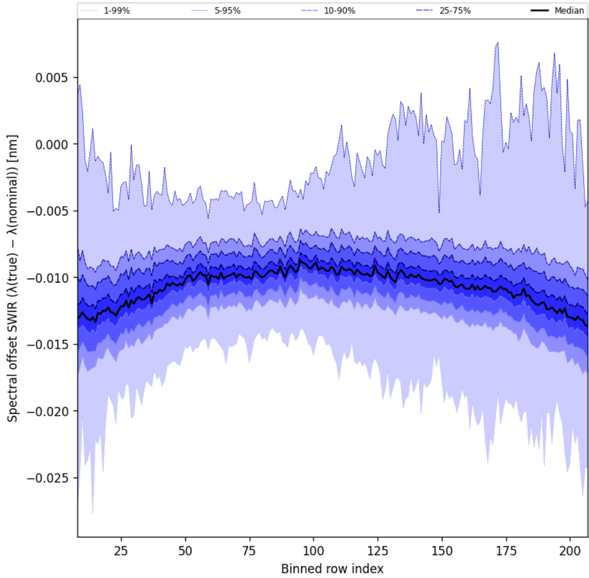
Figure 38: Along track statistics of “Spectral offset SWIR ( \lambda_{\text{true}} - \lambda_{\text{nominal}} )” for 2025-04-10 to 2025-04-12
