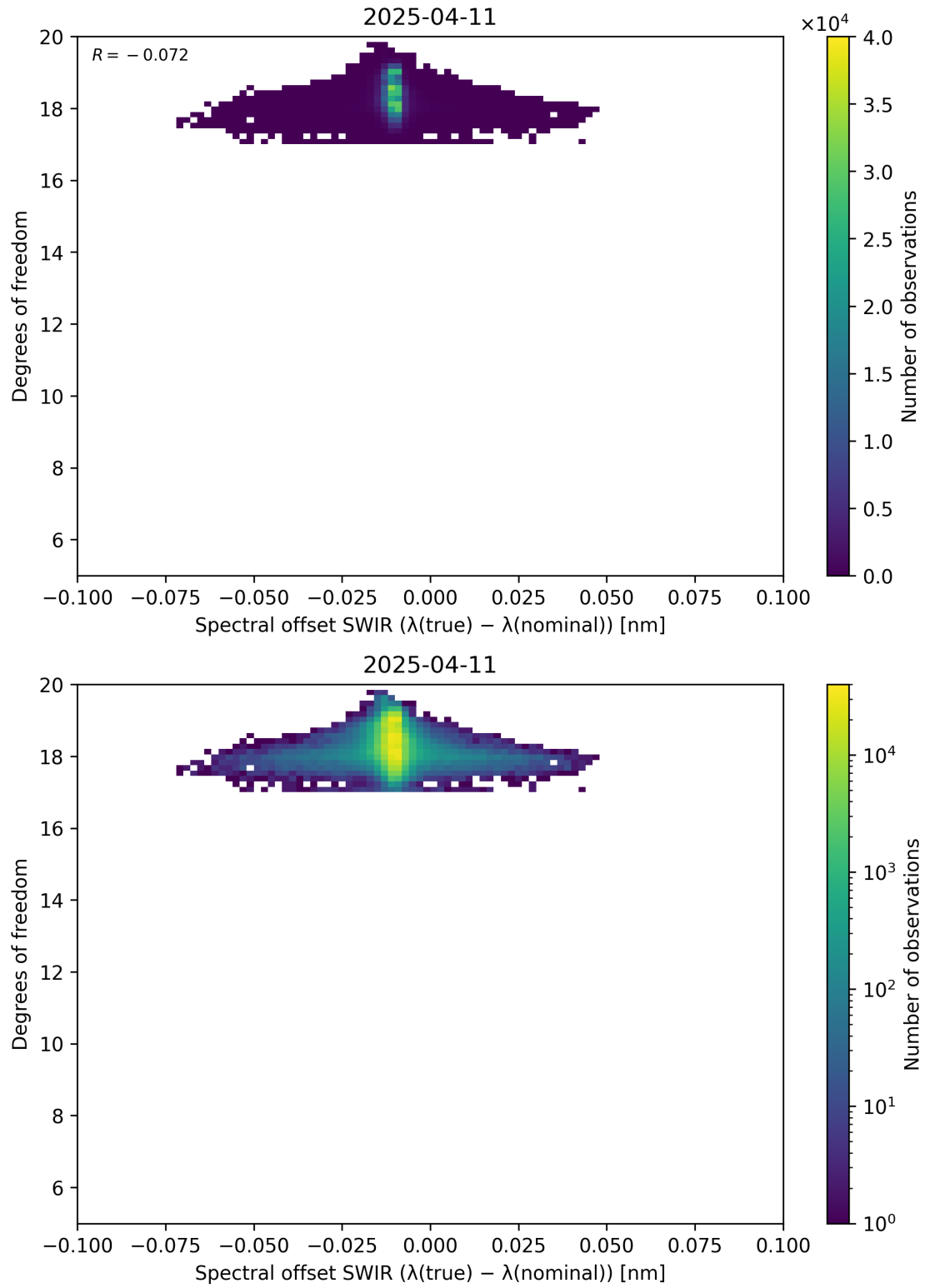
Figure 119: Scatter density plot of “Spectral offset SWIR ( \lambda_{\text{true}} - \lambda_{\text{nominal}} )” against “Degrees of freedom” for 2025-04-10 to 2025-04-12.
