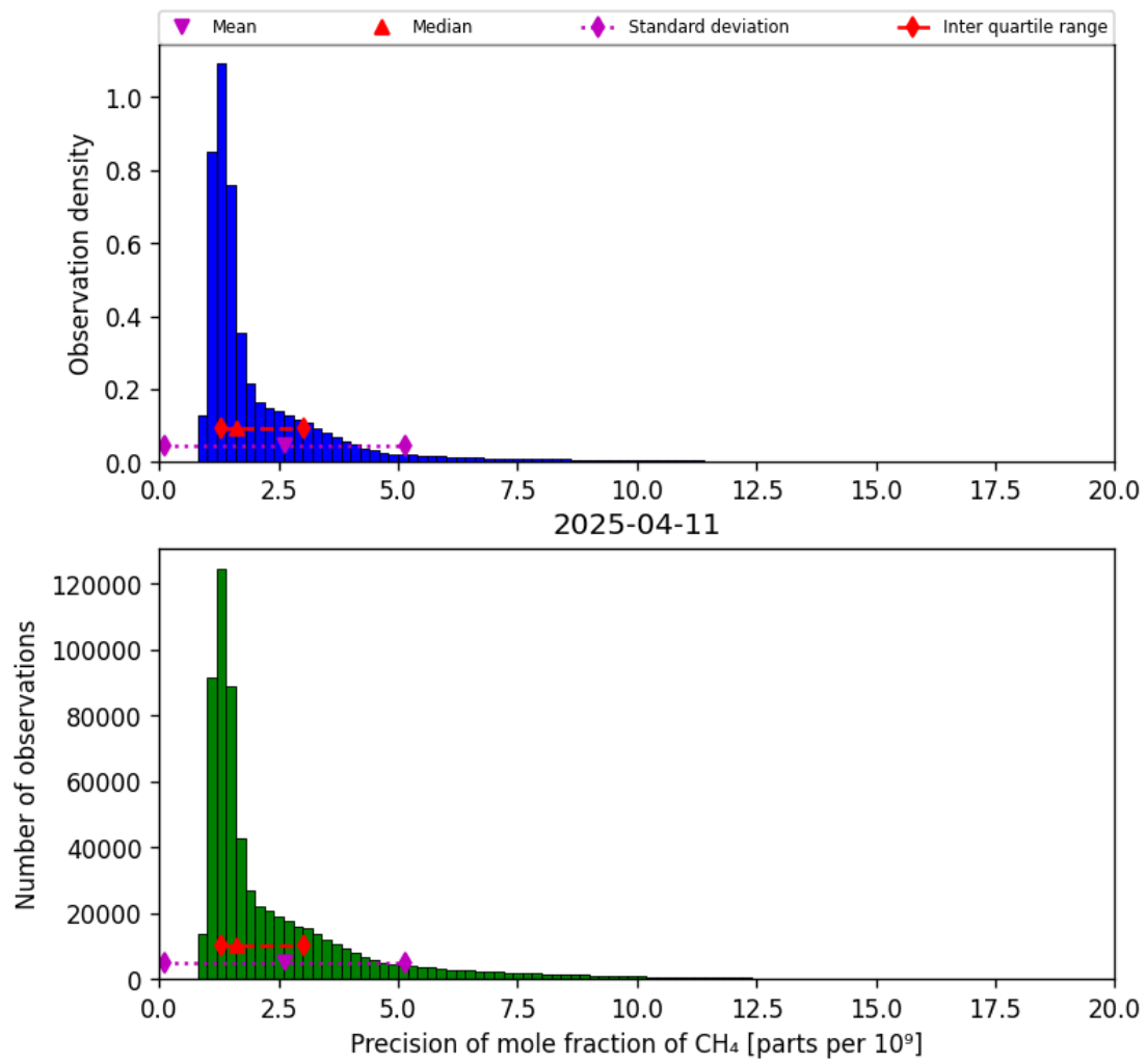
Figure 24: Histogram of “Precision of mole fraction of CH 4 ” for 2025-04-10 to 2025-04-12
