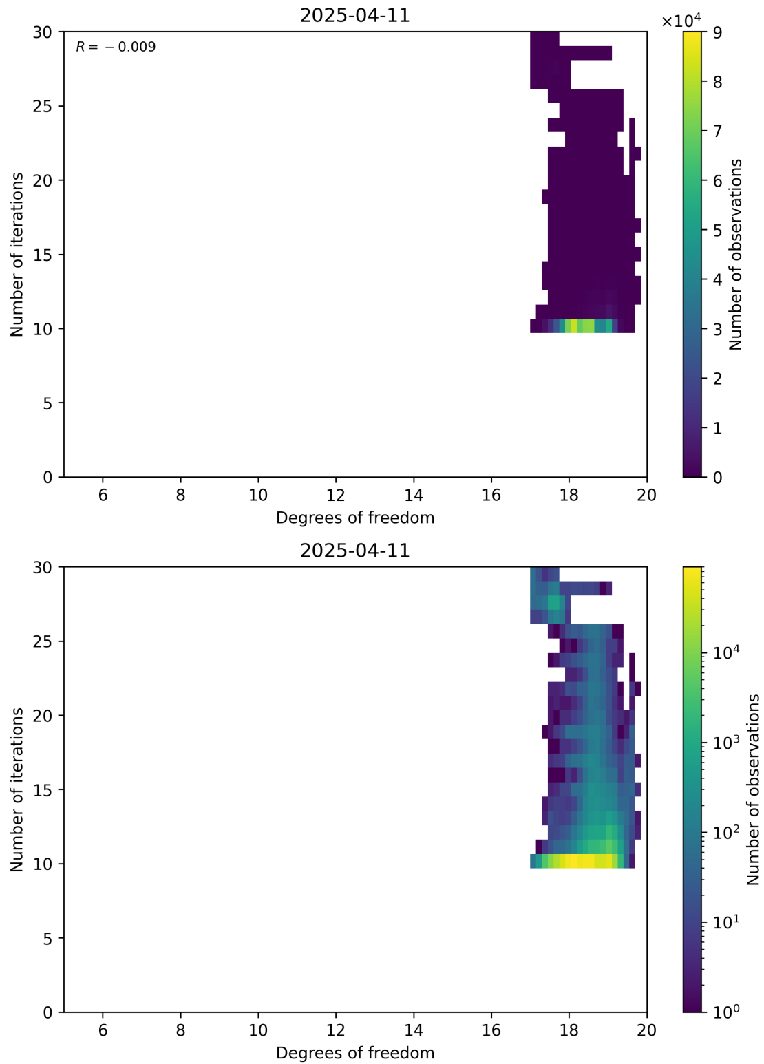
Figure 52: Scatter density plot of “Degrees of freedom” against “Number of iterations” for 2025-04-10 to 2025-04-12.
