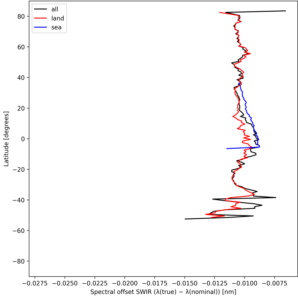
Figure 16: Zonal average of “Spectral offset SWIR ( \lambda_{\text{true}} - \lambda_{\text{nominal}} )” for 2025-04-10 to 2025-04-12.
