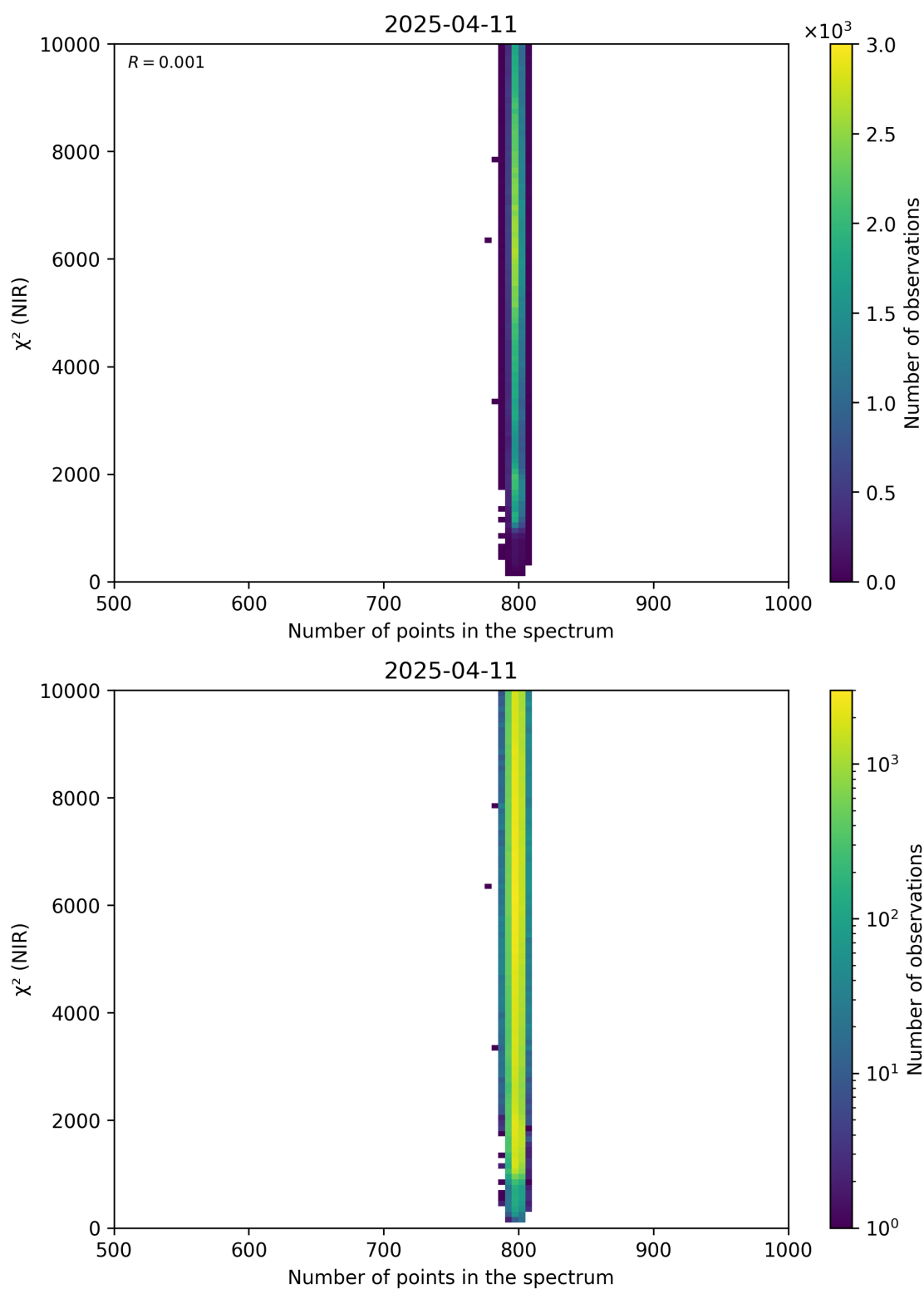
Figure 88: Scatter density plot of “Number of points in the spectrum” against “ \chi^2 (NIR)” for 2025-04-10 to 2025-04-12.
