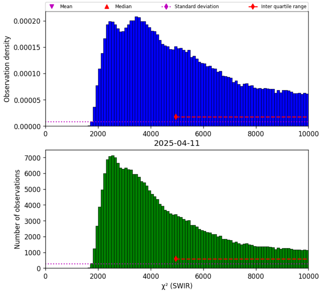
Figure 28: Histogram of “ \chi^2 (SWIR)” for 2025-04-10 to 2025-04-12
