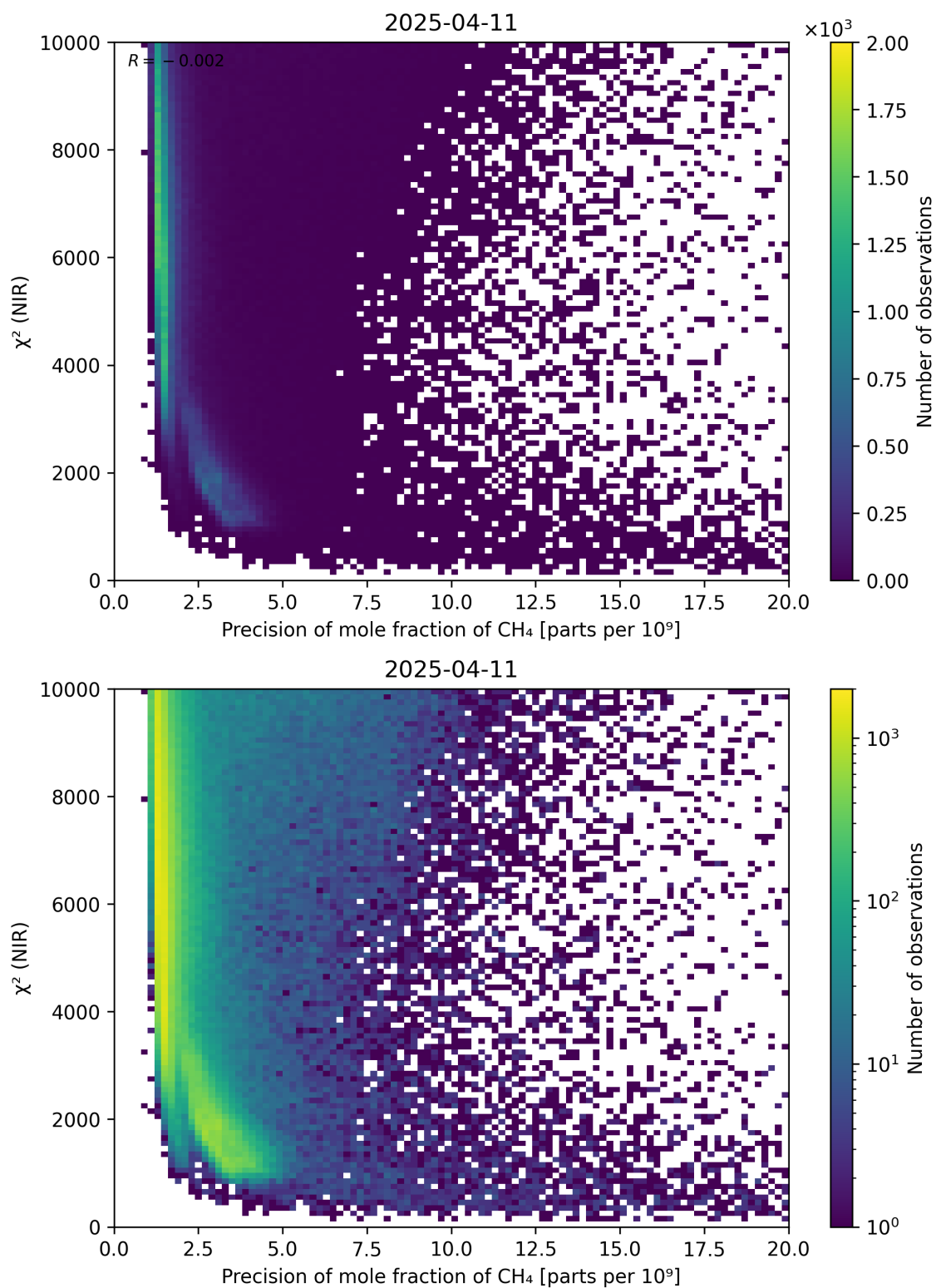
Figure 78: Scatter density plot of “Precision of mole fraction of CH 4 ” against “ \chi^2 (NIR)” for 2025-04-10 to 2025-04-12.
