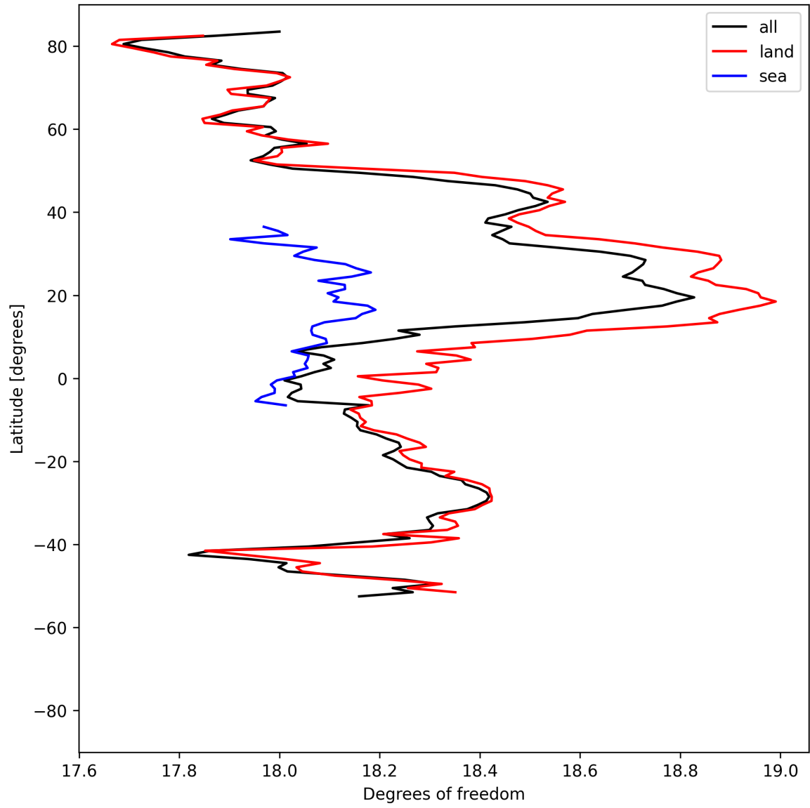
Figure 19: Zonal average of “Degrees of freedom” for 2025-04-10 to 2025-04-12.
