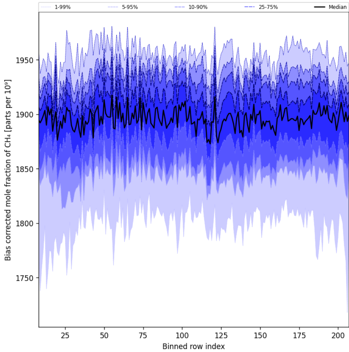
Figure 36: Along track statistics of “Bias corrected mole fraction of CH 4 ” for 2025-04-10 to 2025-04-12
