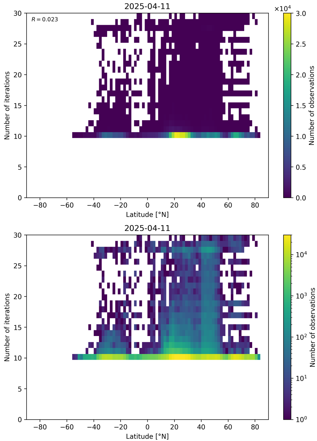
Figure 60: Scatter density plot of “Latitude” against “Number of iterations” for 2025-04-10 to 2025-04-12.
