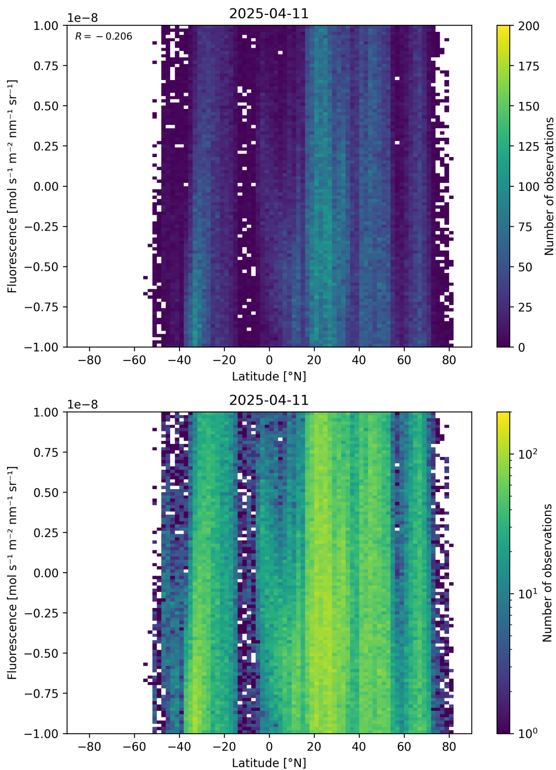
Figure 56: Scatter density plot of “Latitude” against “Fluorescence” for 2025-04-10 to 2025-04-12.
