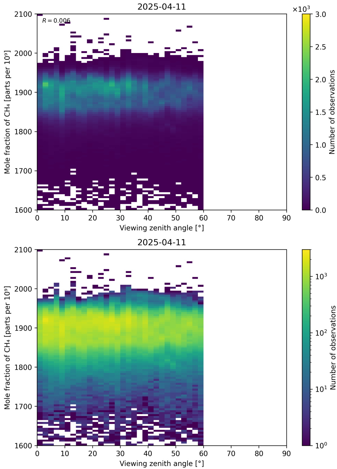
Figure 110: Scatter density plot of “Viewing zenith angle” against “Mole fraction of CH 4 ” for 2025-04-10 to 2025-04-12.
