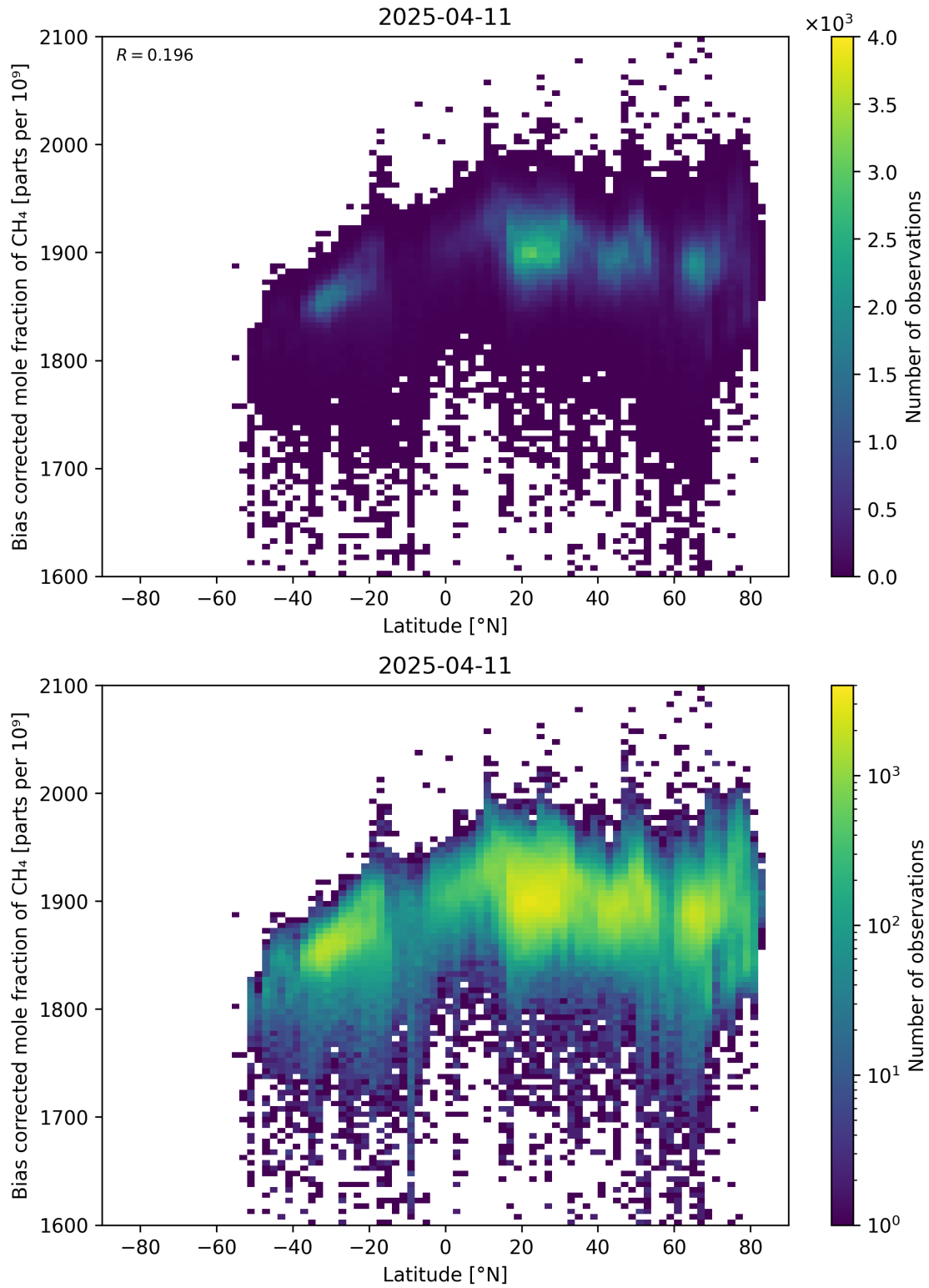
Figure 58: Scatter density plot of “Latitude” against “Bias corrected mole fraction of \text{CH}_4 ” for 2025-04-10 to 2025-04-12.
