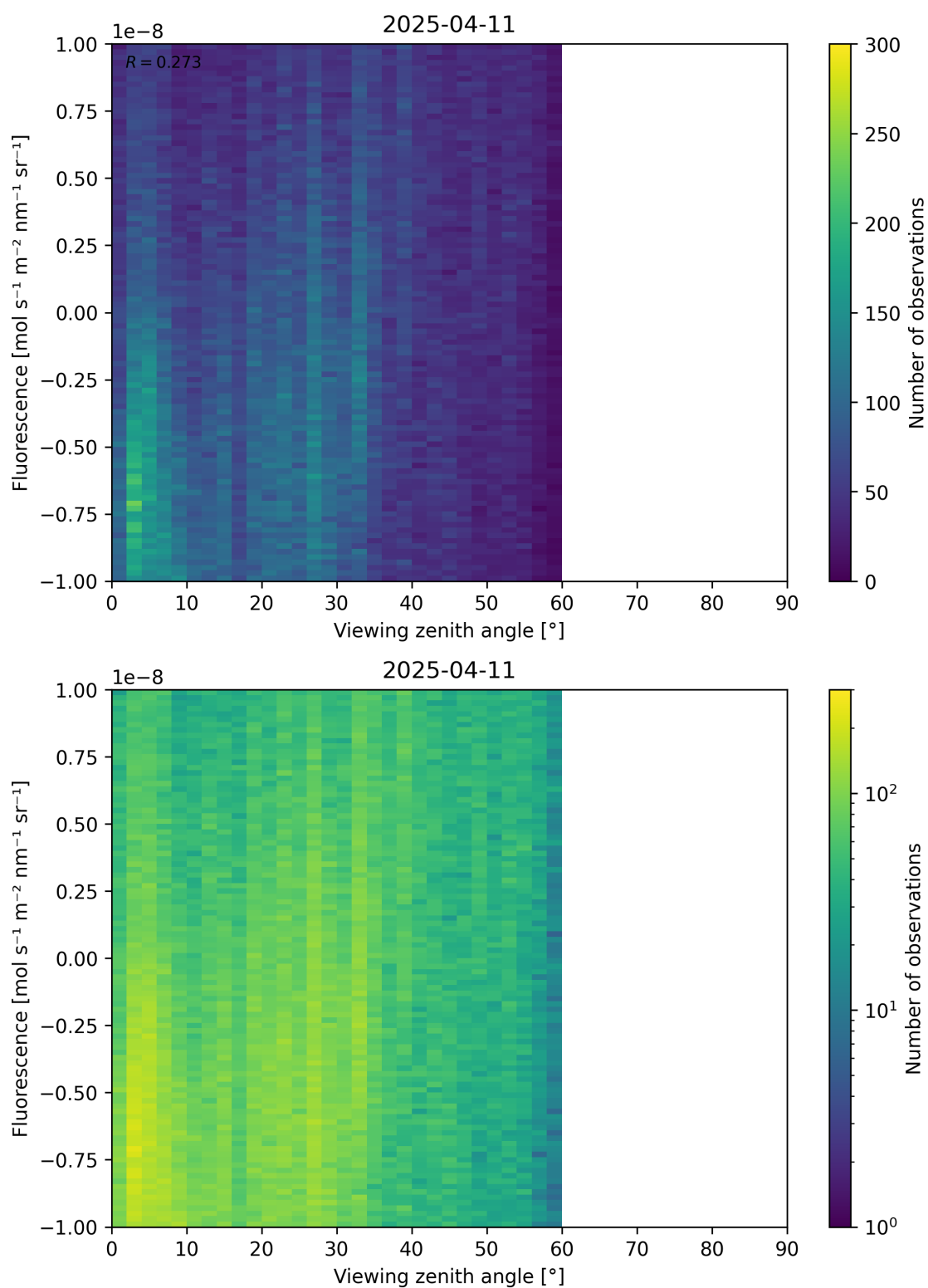
Figure 108: Scatter density plot of “Viewing zenith angle” against “Fluorescence” for 2025-04-10 to 2025-04-12.
