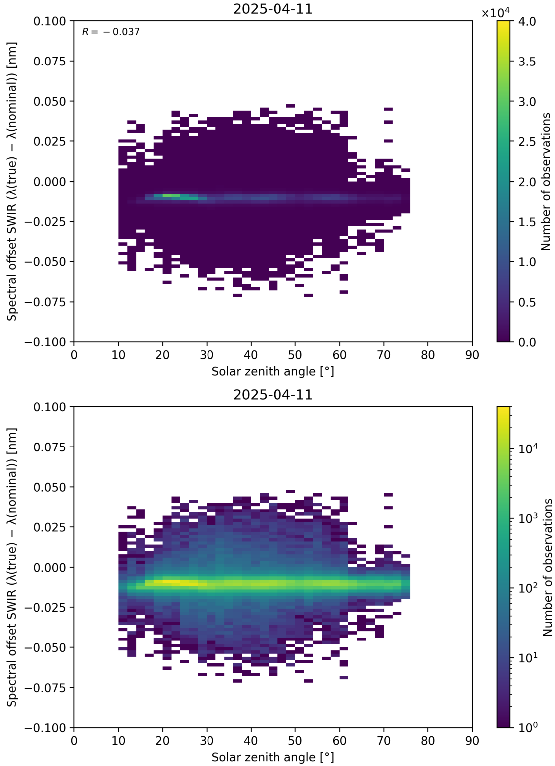
Figure 104: Scatter density plot of “Solar zenith angle” against “Spectral offset SWIR ( \lambda_{\text{true}} - \lambda_{\text{nominal}} )” for 2025-04-10 to 2025-04-12.
