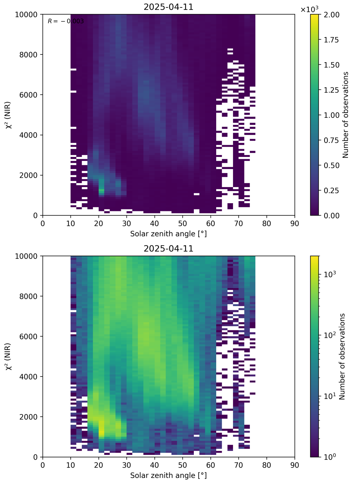
Figure 94: Scatter density plot of “Solar zenith angle” against “ \chi^2 (NIR)” for 2025-04-10 to 2025-04-12.
