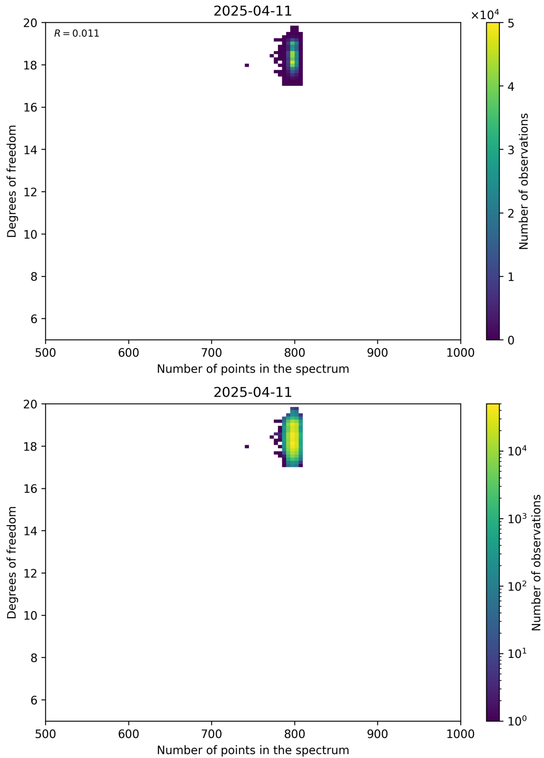
Figure 90: Scatter density plot of “Number of points in the spectrum” against “Degrees of freedom” for 2025-04-10 to 2025-04-12.
