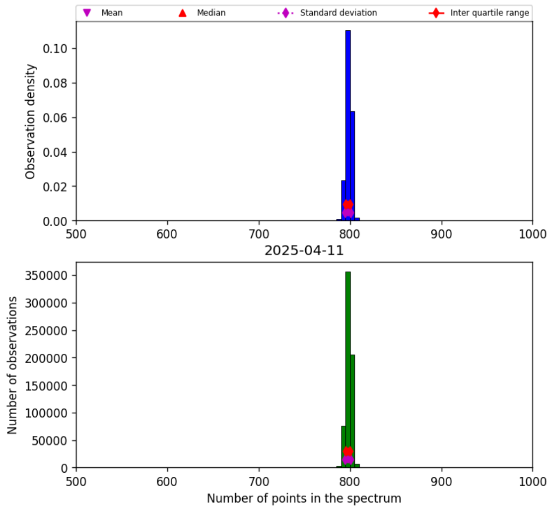
Figure 26: Histogram of “Number of points in the spectrum” for 2025-04-10 to 2025-04-12
