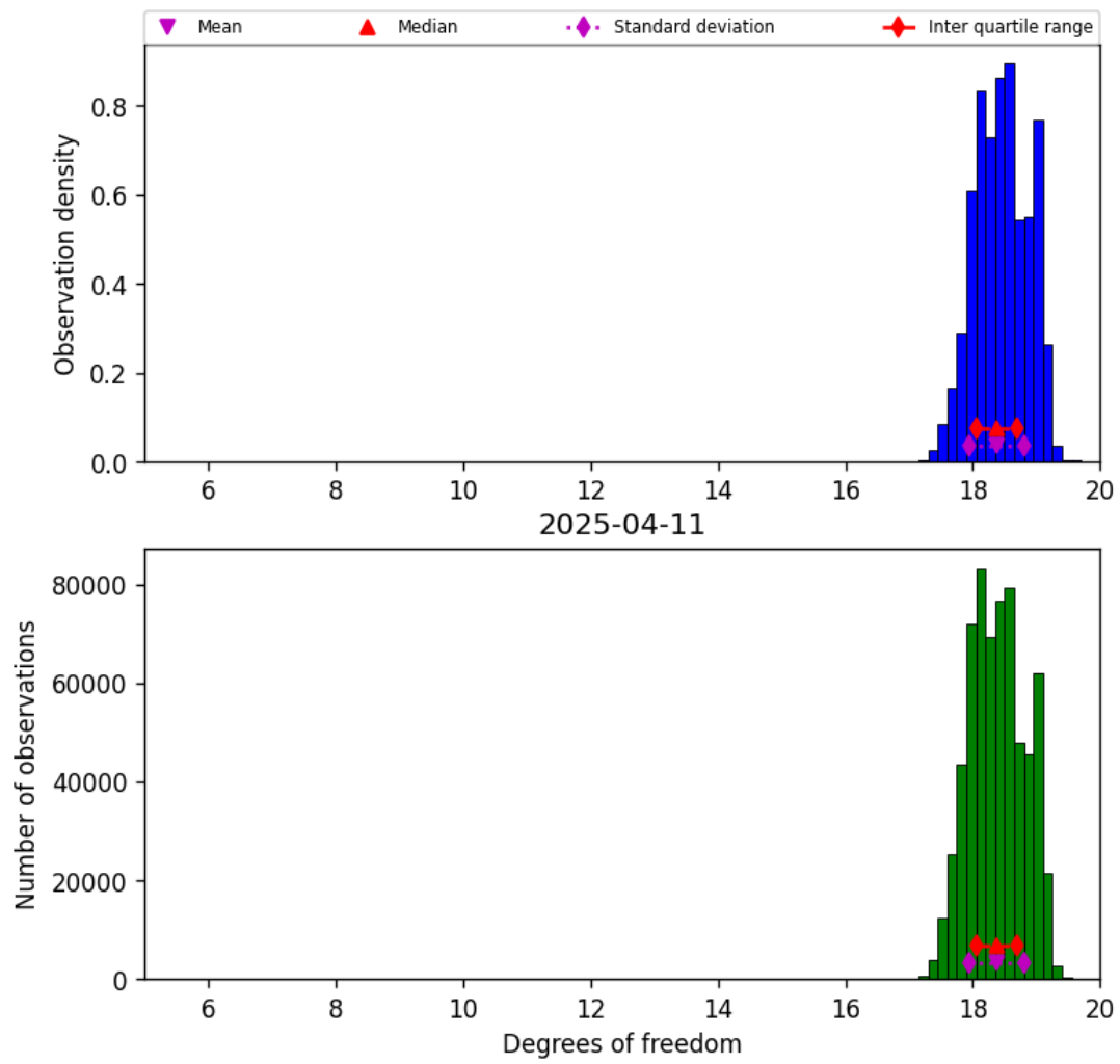
Figure 30: Histogram of “Degrees of freedom” for 2025-04-10 to 2025-04-12
