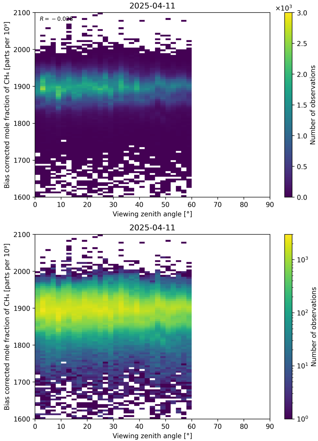
Figure 111: Scatter density plot of “Viewing zenith angle” against “Bias corrected mole fraction of CH 4 ” for 2025-04-10 to 2025-04-12.
