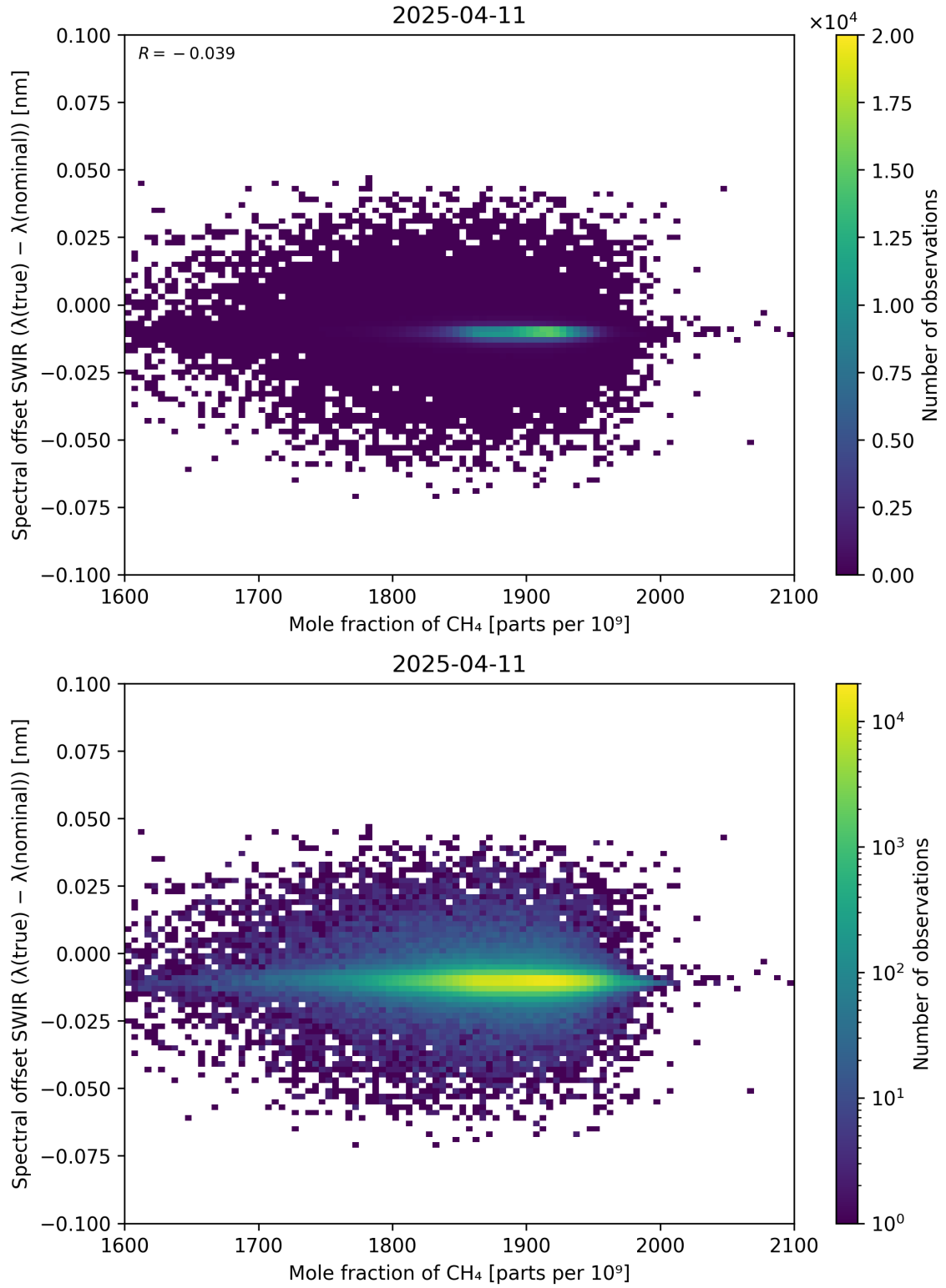
Figure 86: Scatter density plot of “Mole fraction of CH 4 ” against “Spectral offset SWIR ( \lambda_{\text{true}} - \lambda_{\text{nominal}} )” for 2025-04-10 to 2025-04-12.
