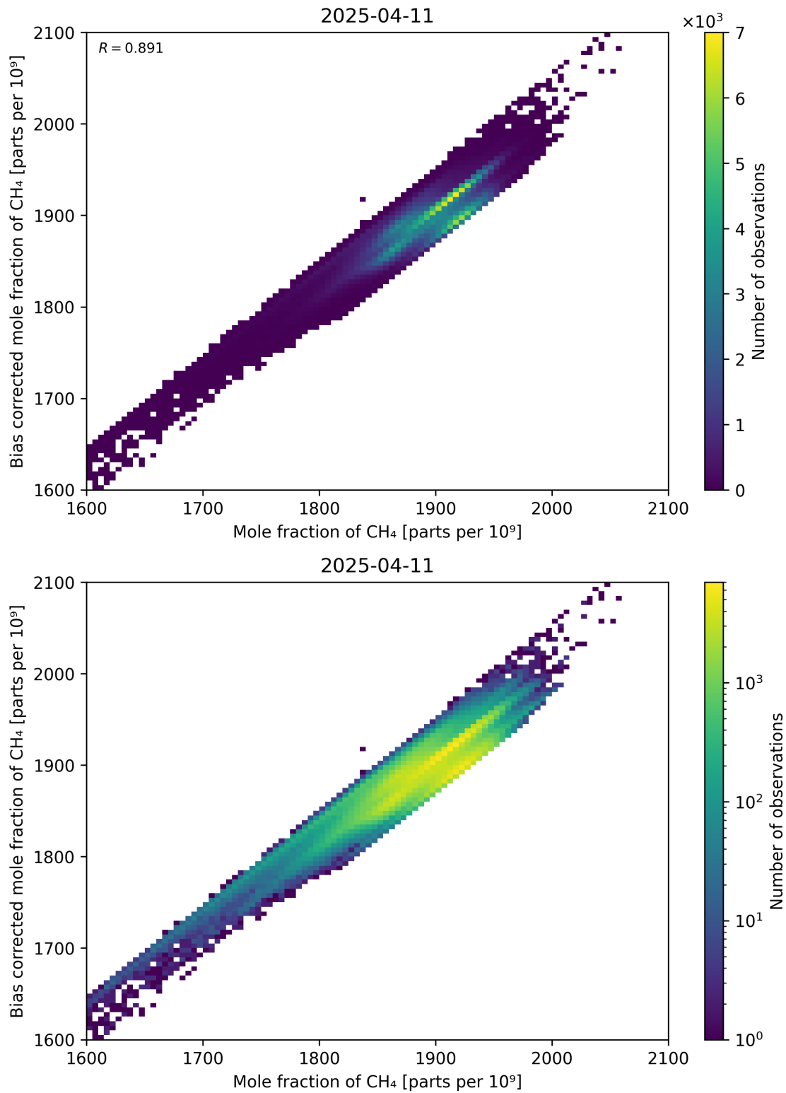
Figure 74: Scatter density plot of “Mole fraction of CH 4 ” against “Bias corrected mole fraction of CH 4 ” for 2025-04-10 to 2025-04-12.
