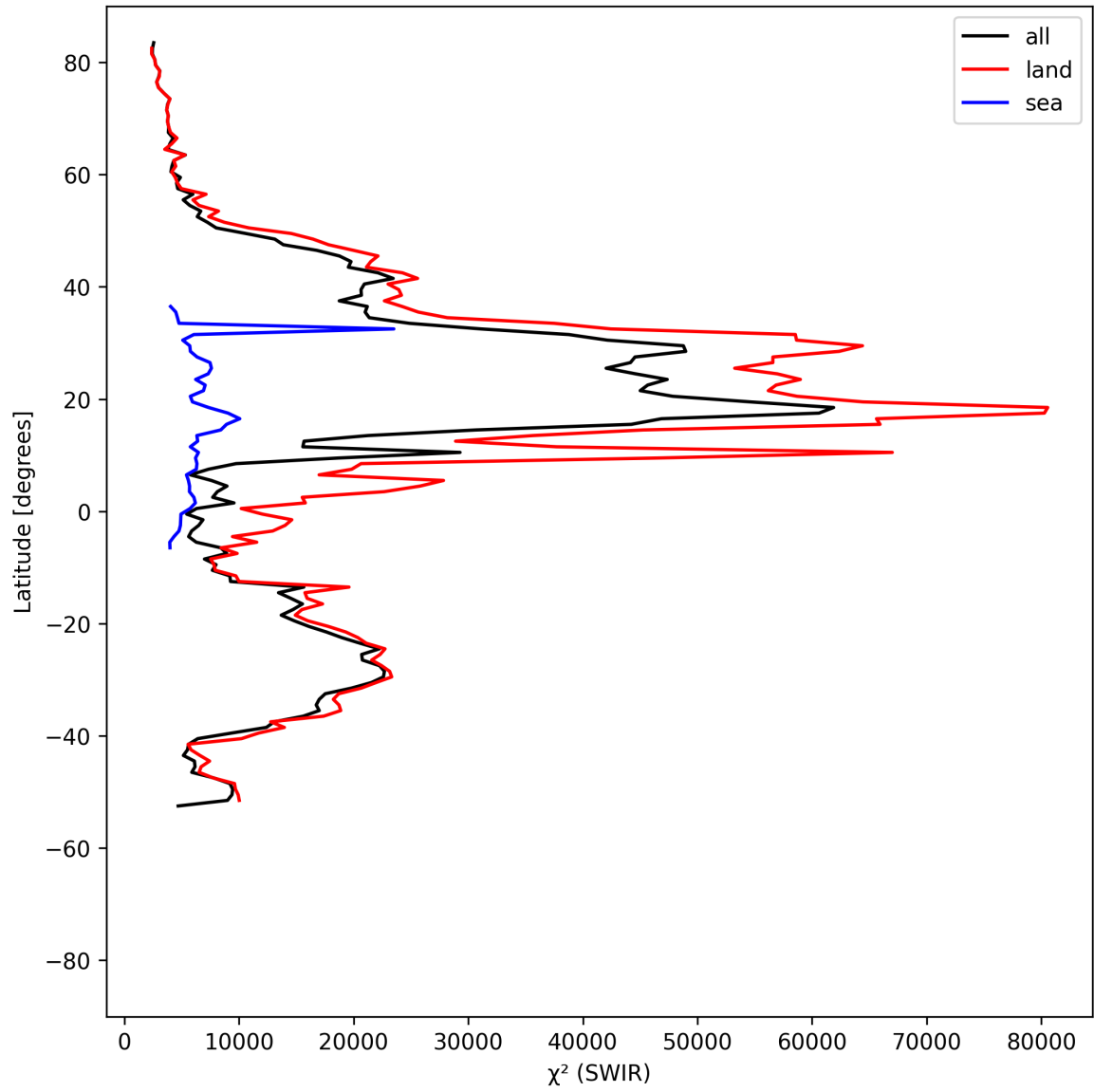
Figure 17: Zonal average of “ \chi^2 (SWIR)” for 2025-04-10 to 2025-04-12.
