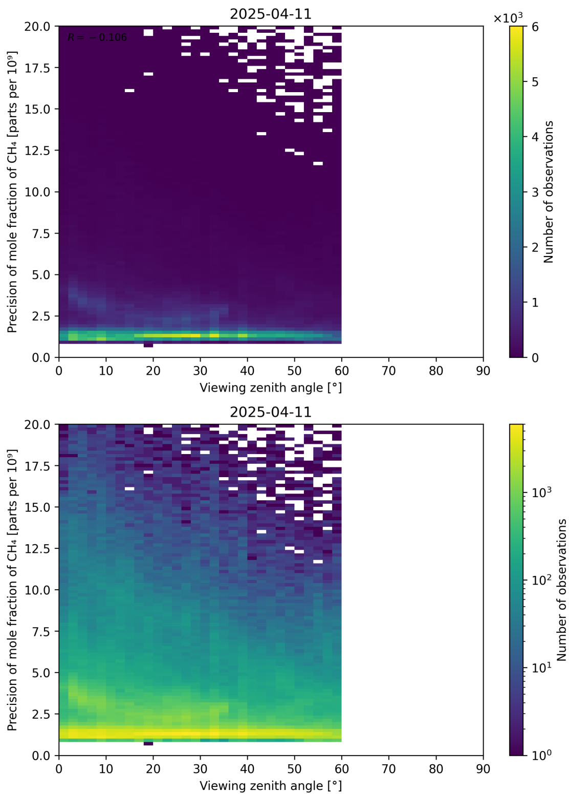
Figure 112: Scatter density plot of “Viewing zenith angle” against “Precision of mole fraction of \text{CH}_4 ” for 2025-04-10 to 2025-04-12.
