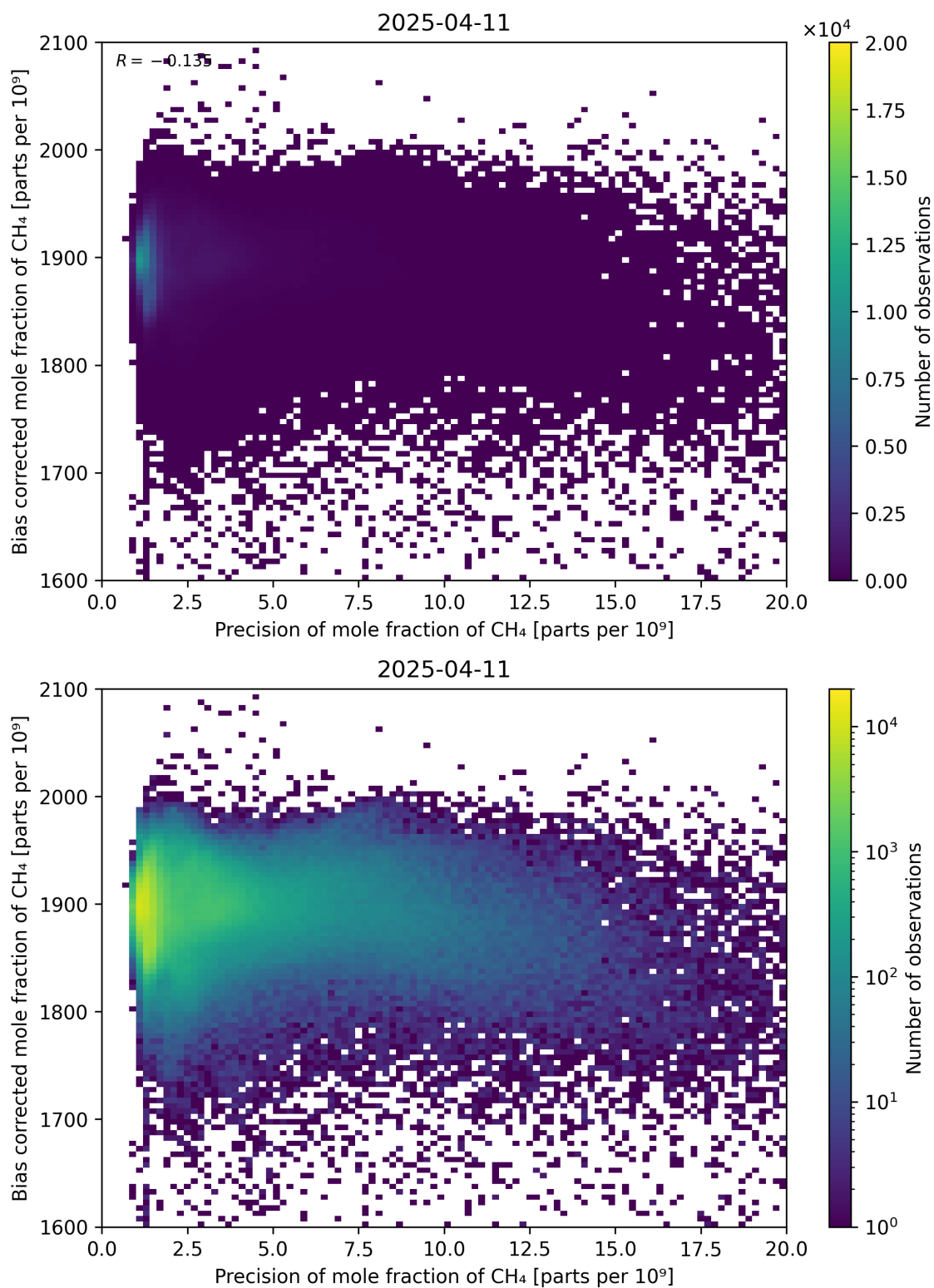
Figure 82: Scatter density plot of “Precision of mole fraction of CH 4 ” against “Bias corrected mole fraction of CH 4 ” for 2025-04-10 to 2025-04-12.
