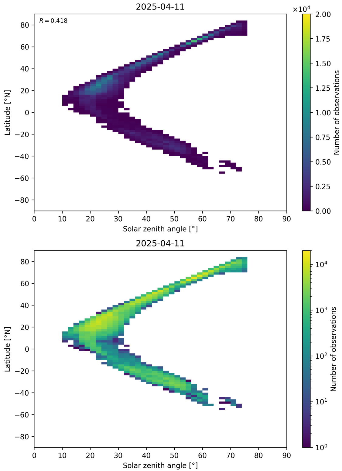
Figure 98: Scatter density plot of “Solar zenith angle” against “Latitude” for 2025-04-10 to 2025-04-12.
