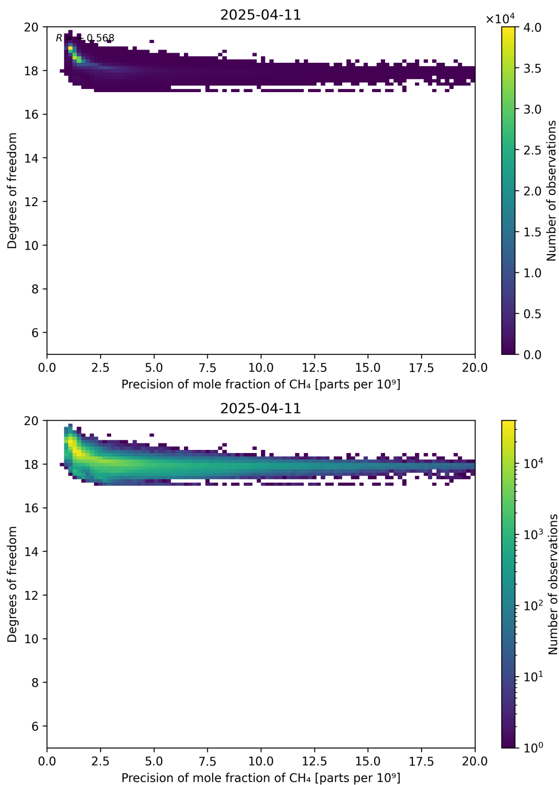
Figure 80: Scatter density plot of “Precision of mole fraction of CH 4 ” against “Degrees of freedom” for 2025-04-10 to 2025-04-12.
