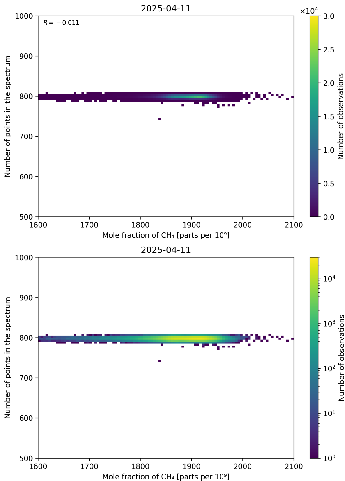
Figure 77: Scatter density plot of “Mole fraction of CH 4 ” against “Number of points in the spectrum” for 2025-04-10 to 2025-04-12.
