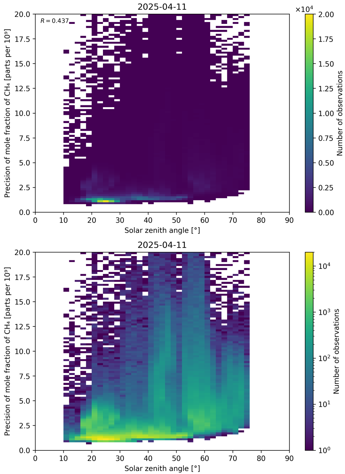
Figure 101: Scatter density plot of “Solar zenith angle” against “Precision of mole fraction of \text{CH}_4 ” for 2025-04-10 to 2025-04-12.
