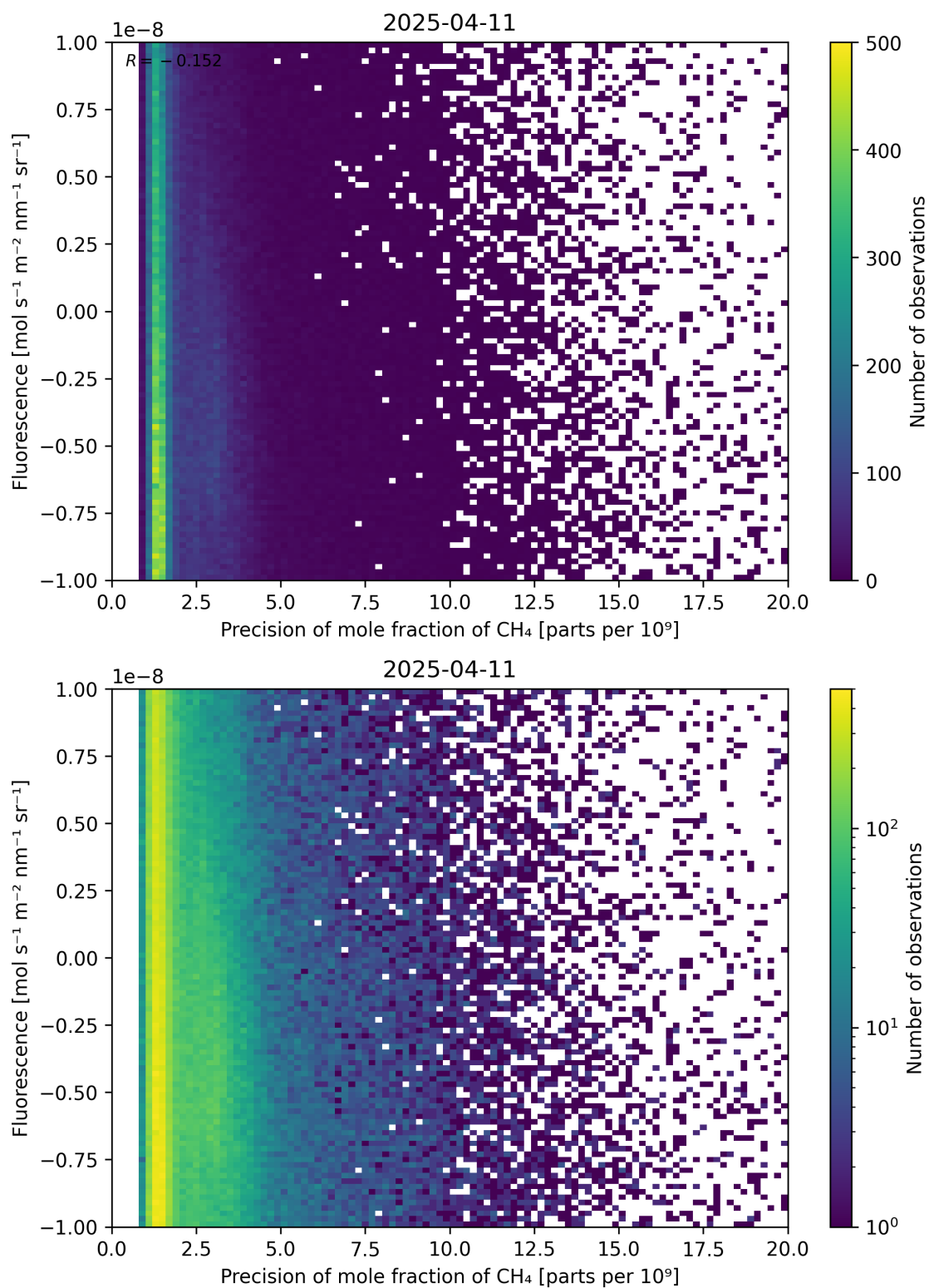
Figure 81: Scatter density plot of “Precision of mole fraction of CH 4 ” against “Fluorescence” for 2025-04-10 to 2025-04-12.
