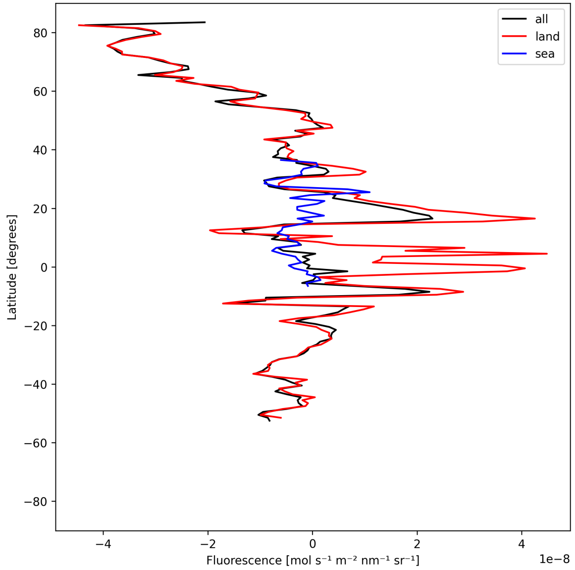
Figure 21: Zonal average of “Fluorescence” for 2025-04-10 to 2025-04-12.
