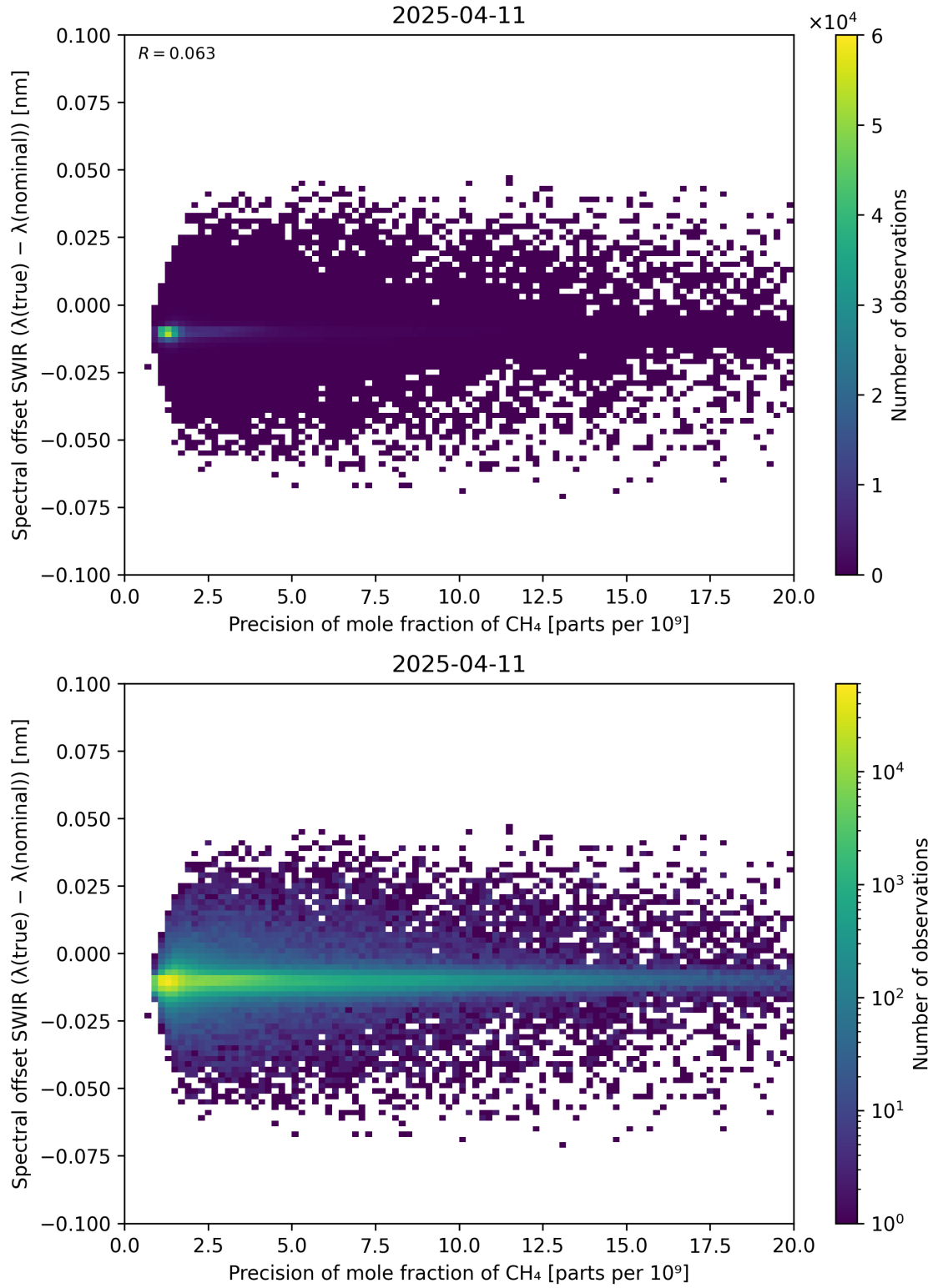
Figure 85: Scatter density plot of “Precision of mole fraction of CH 4 ” against “Spectral offset SWIR ( \lambda_{\text{true}} - \lambda_{\text{nominal}} )” for 2025-04-10 to 2025-04-12.
