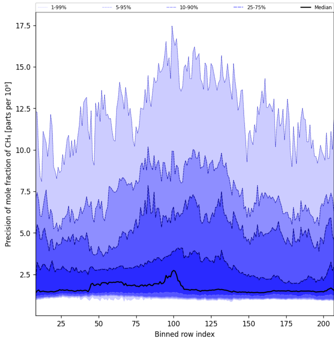
Figure 35: Along track statistics of “Precision of mole fraction of CH 4 ” for 2025-04-10 to 2025-04-12
