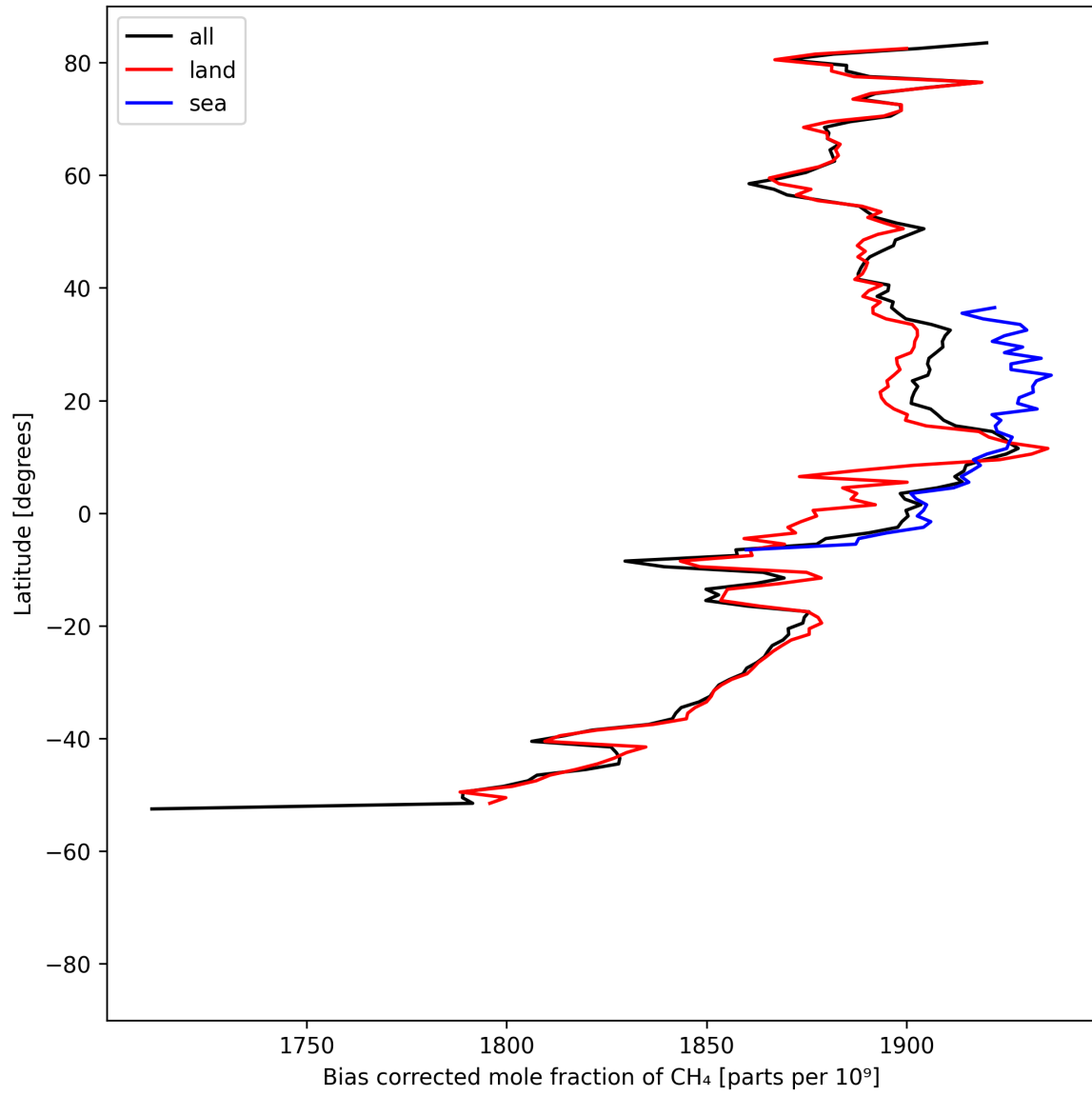
Figure 14: Zonal average of “Bias corrected mole fraction of \text{CH}_4 ” for 2025-04-10 to 2025-04-12.
