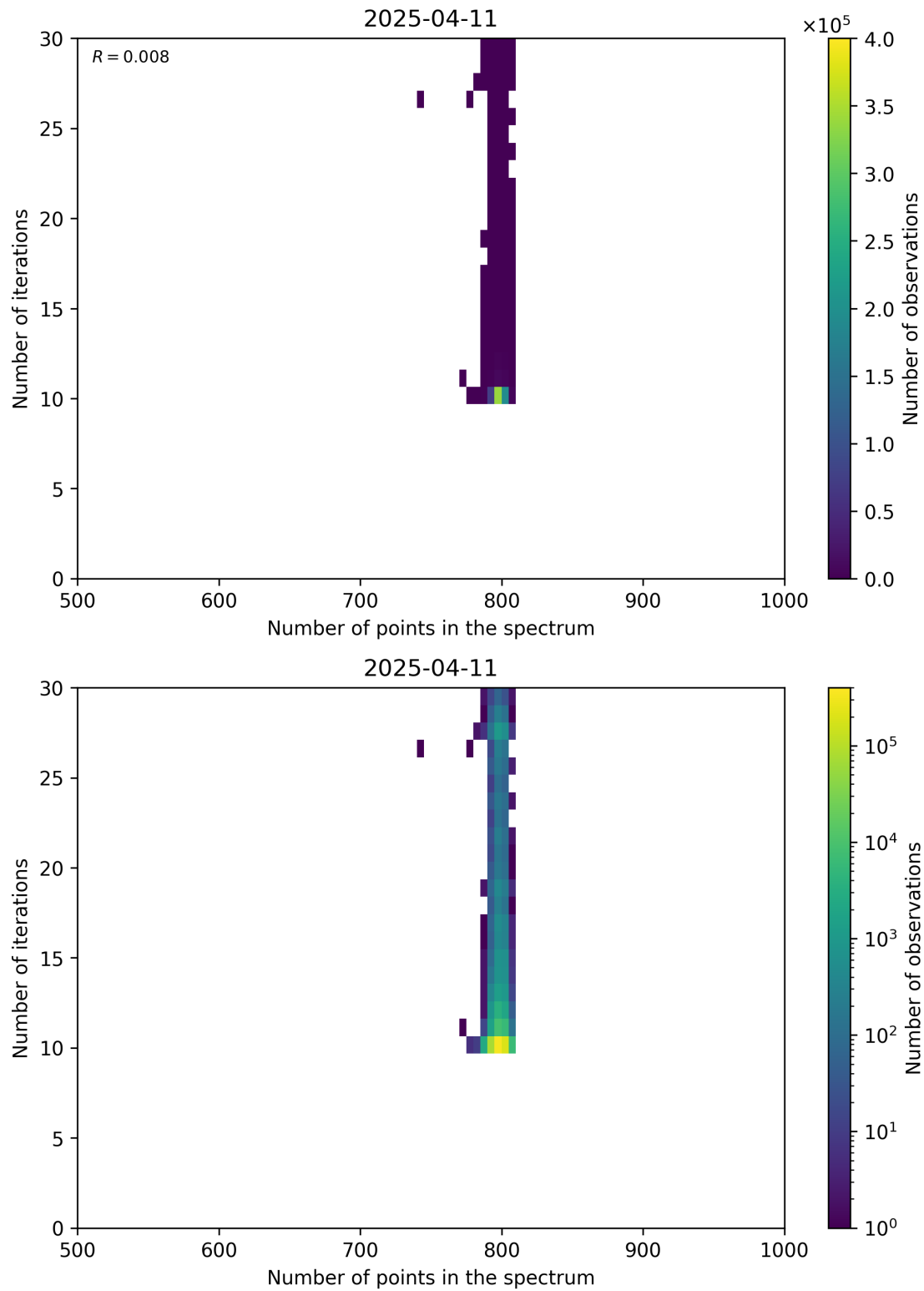
Figure 92: Scatter density plot of “Number of points in the spectrum” against “Number of iterations” for 2025-04-10 to 2025-04-12.
