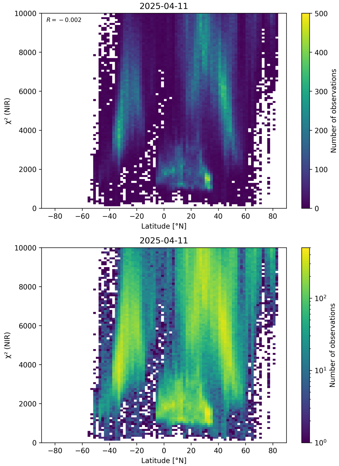
Figure 53: Scatter density plot of “Latitude” against “ \chi^2 (NIR)” for 2025-04-10 to 2025-04-12.
