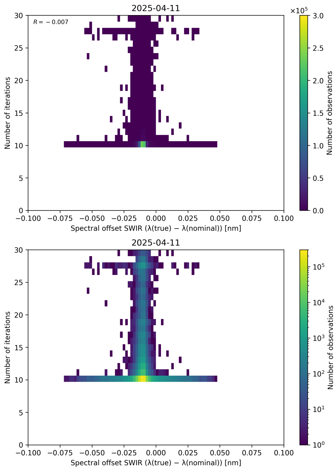
Figure 121: Scatter density plot of “Spectral offset SWIR ( \lambda_{\text{true}} - \lambda_{\text{nominal}} )” against “Number of iterations” for 2025-04-10 to 2025-04-12.
