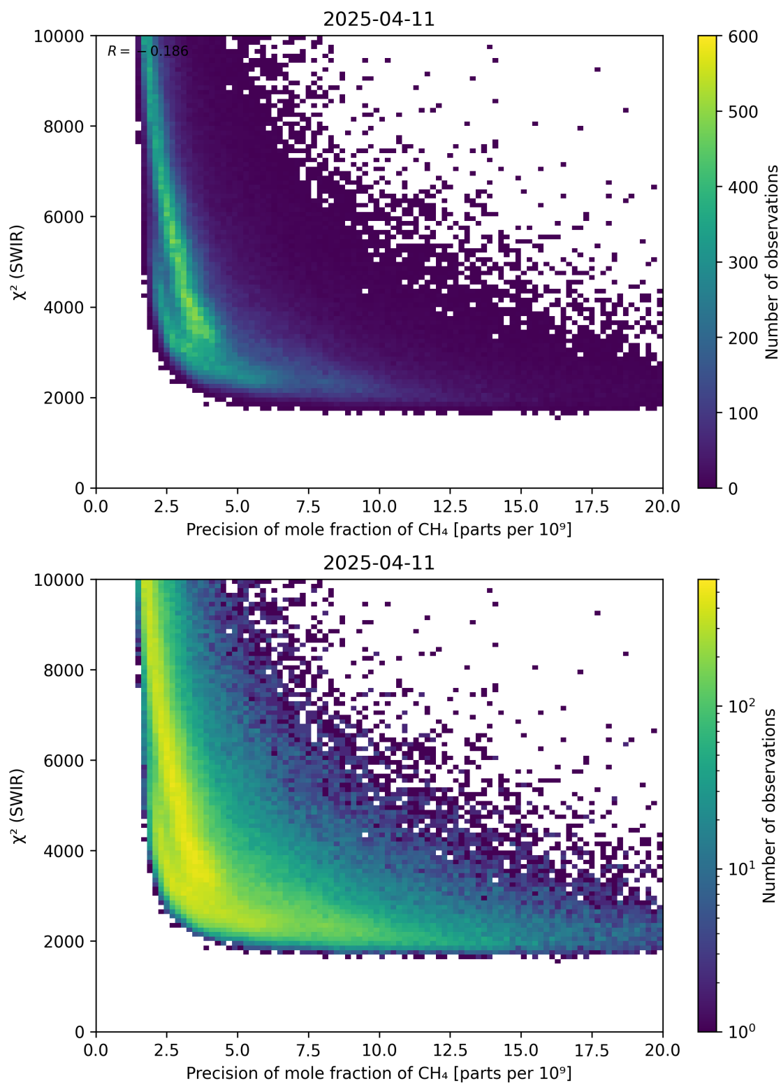
Figure 79: Scatter density plot of “Precision of mole fraction of \text{CH}_4 ” against “ \chi^2 (SWIR)” for 2025-04-10 to 2025-04-12.
