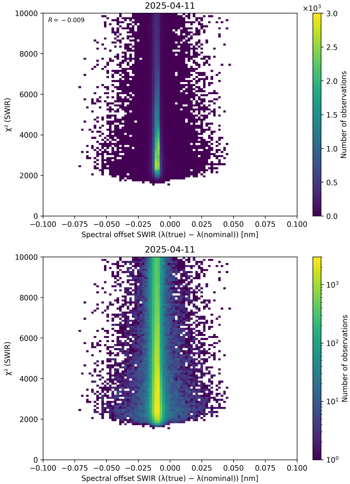
Figure 118: Scatter density plot of “Spectral offset SWIR ( \lambda_{\text{true}} - \lambda_{\text{nominal}} )” against “ \chi^2 (SWIR)” for 2025-04-10 to 2025-04-12.
