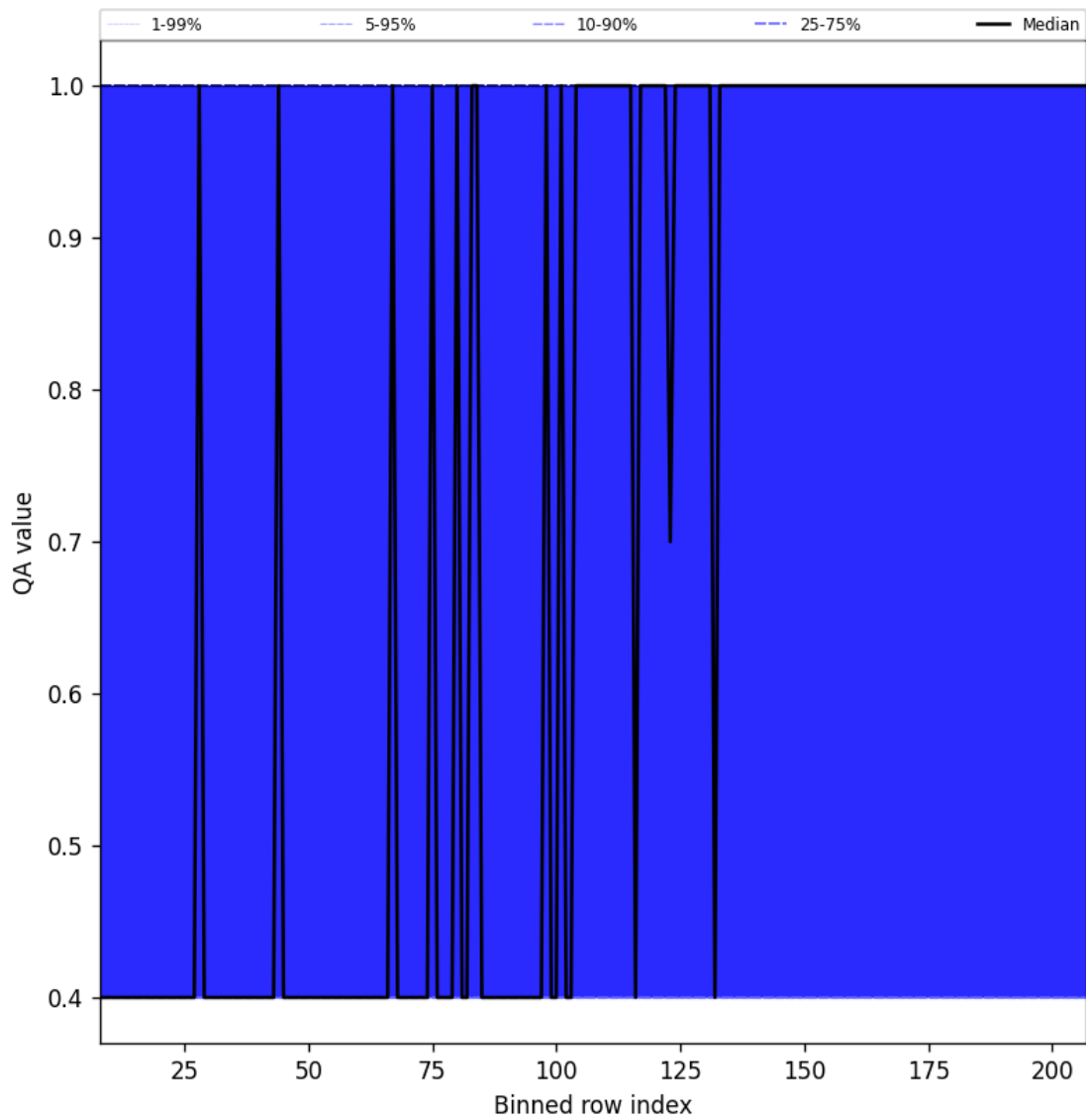
Figure 33: Along track statistics of “QA value” for 2025-04-10 to 2025-04-12
