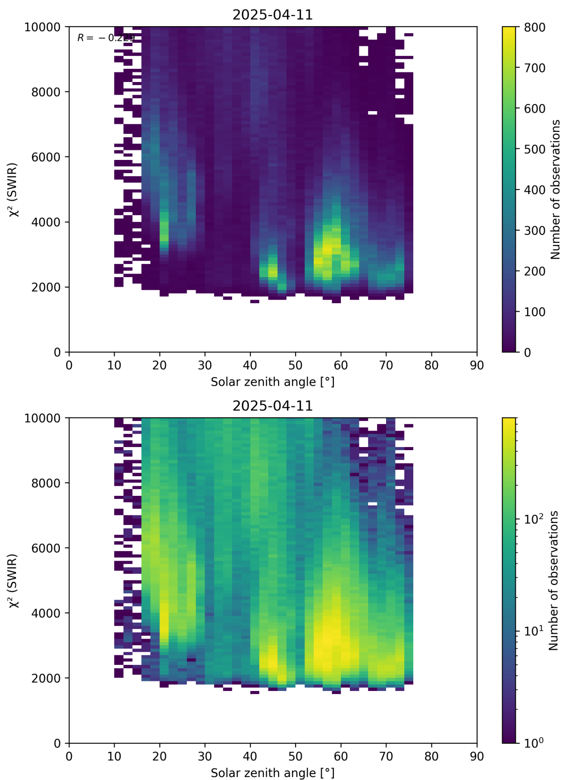
Figure 95: Scatter density plot of “Solar zenith angle” against “ \chi^2 (SWIR)” for 2025-04-10 to 2025-04-12.
