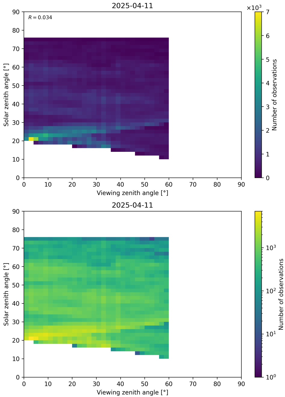
Figure 115: Scatter density plot of “Viewing zenith angle” against “Solar zenith angle” for 2025-04-10 to 2025-04-12.
