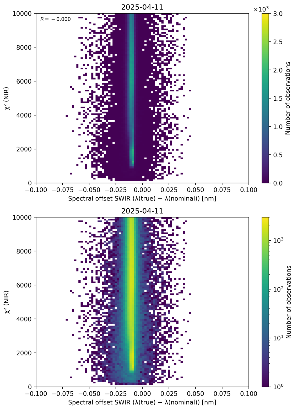
Figure 117: Scatter density plot of “Spectral offset SWIR ( \lambda_{\text{true}} - \lambda_{\text{nominal}} )” against “ \chi^2 (NIR)” for 2025-04-10 to 2025-04-12.
