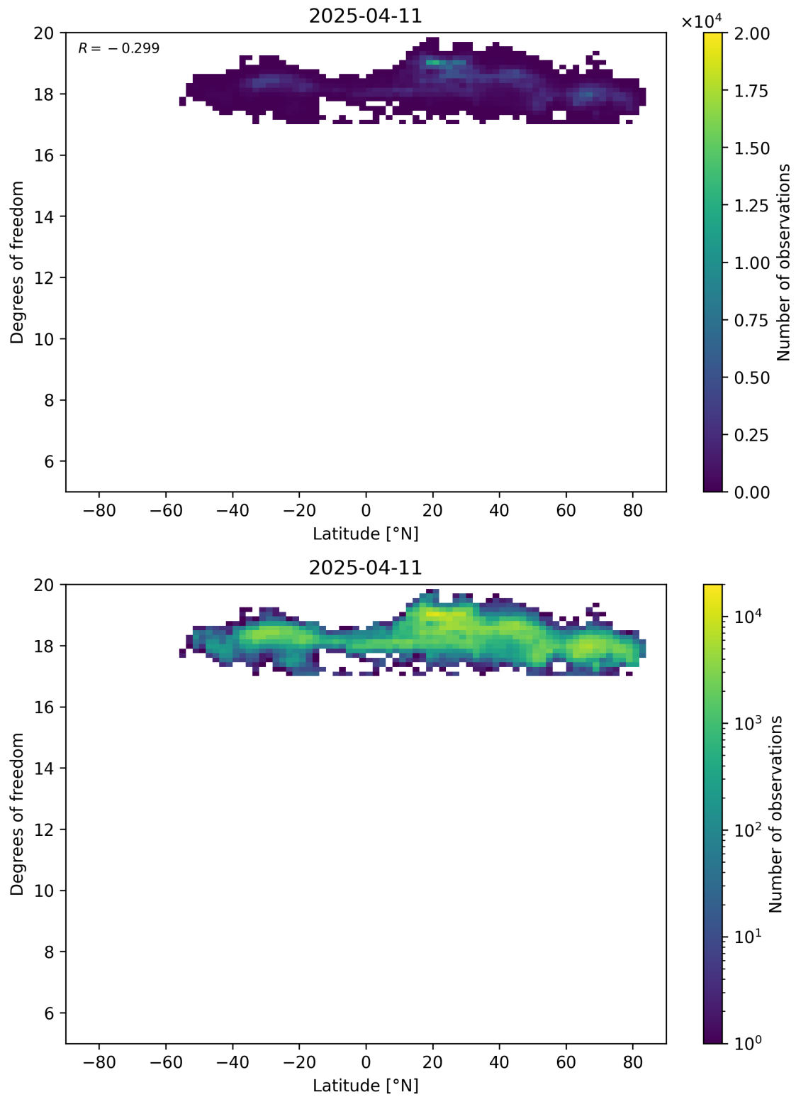
Figure 55: Scatter density plot of “Latitude” against “Degrees of freedom” for 2025-04-10 to 2025-04-12.
