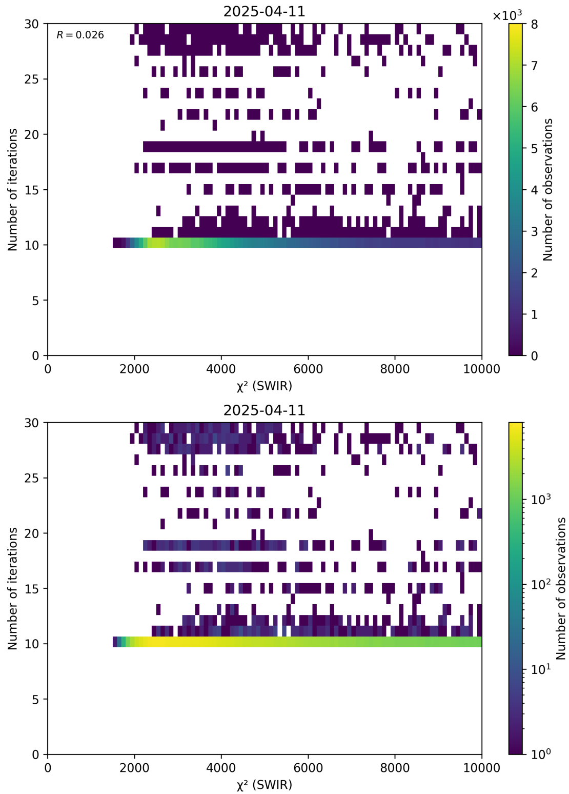
Figure 50: Scatter density plot of “ \chi^2 (SWIR)” against “Number of iterations” for 2025-04-10 to 2025-04-12.
