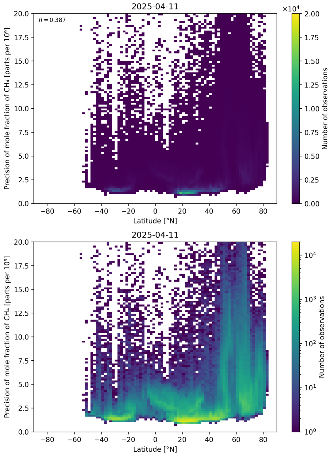
Figure 59: Scatter density plot of “Latitude” against “Precision of mole fraction of \text{CH}_4 ” for 2025-04-10 to 2025-04-12.
