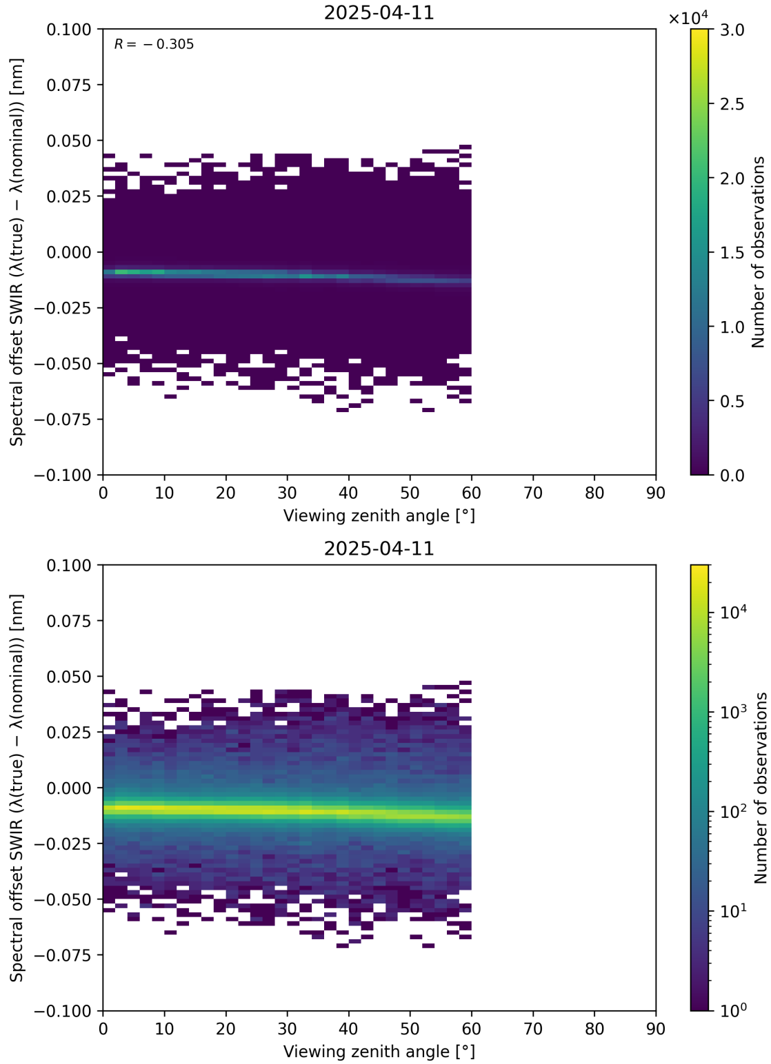
Figure 116: Scatter density plot of “Viewing zenith angle” against “Spectral offset SWIR ( \lambda_{\text{true}} - \lambda_{\text{nominal}} )” for 2025-04-10 to 2025-04-12.
