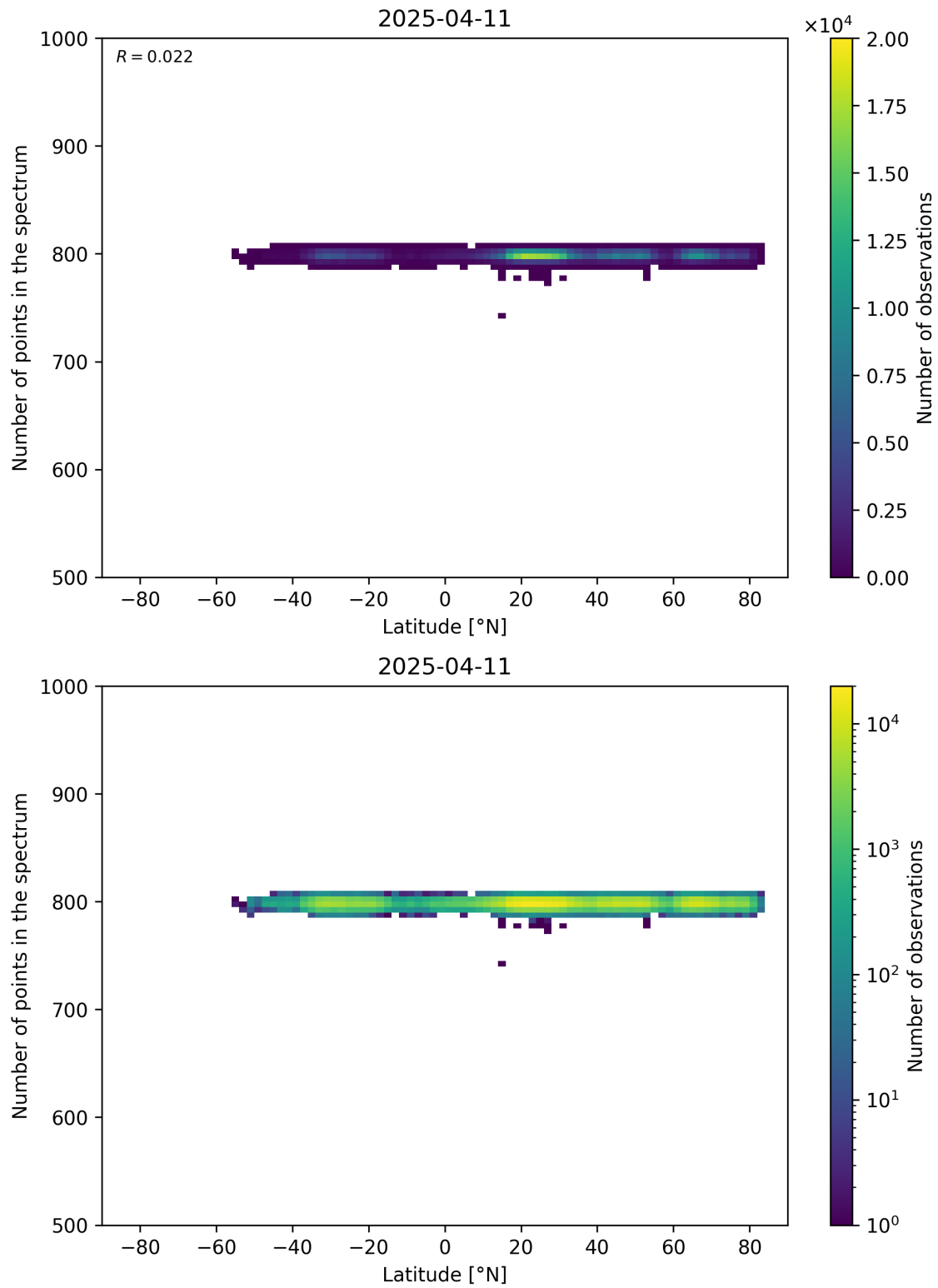
Figure 61: Scatter density plot of “Latitude” against “Number of points in the spectrum” for 2025-04-10 to 2025-04-12.
