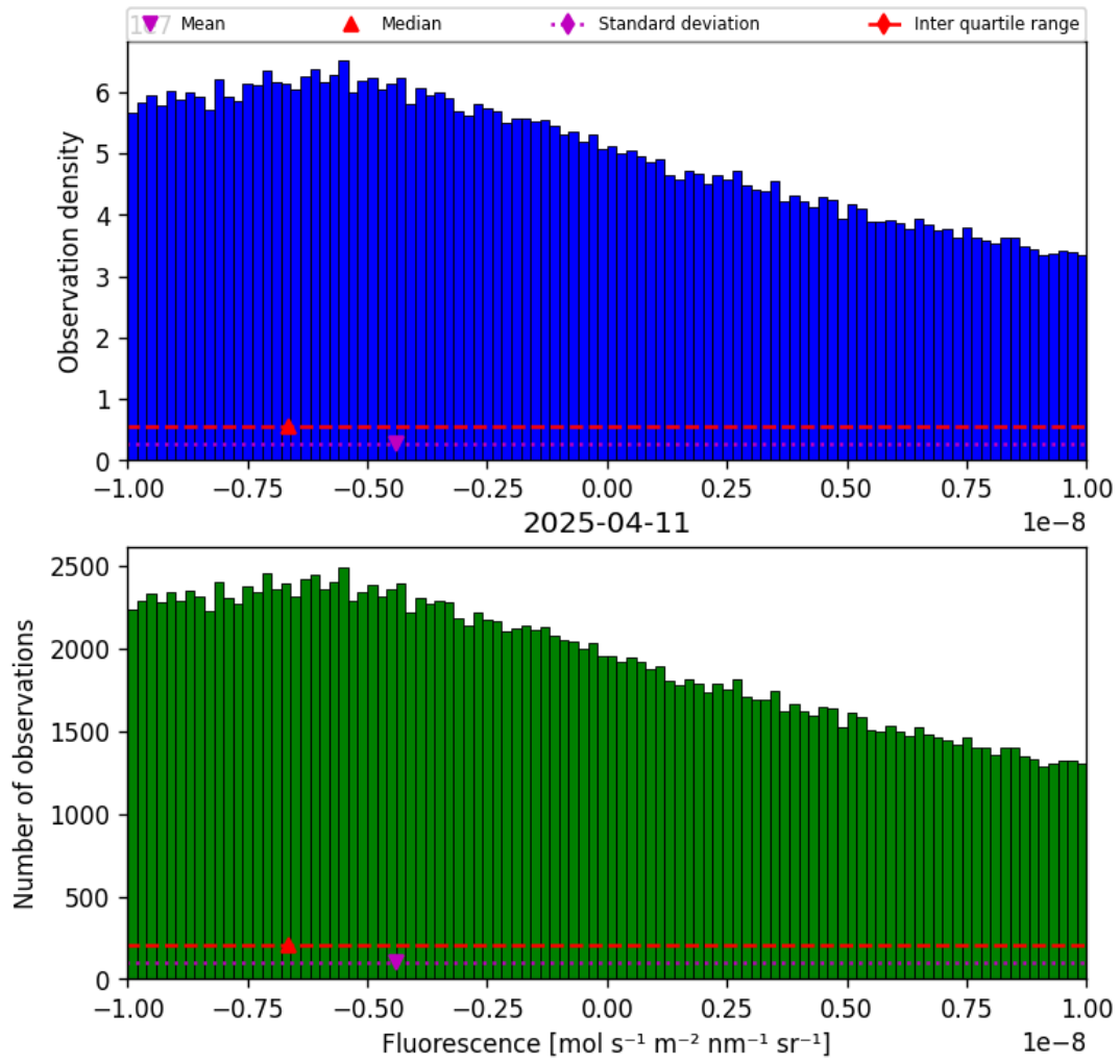
Figure 32: Histogram of “Fluorescence” for 2025-04-10 to 2025-04-12
