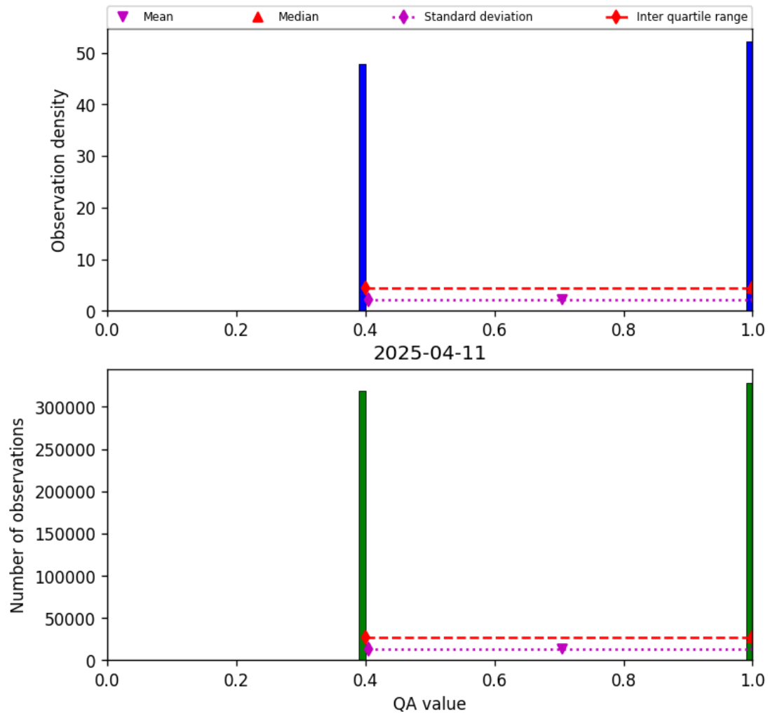
Figure 22: Histogram of “QA value” for 2025-04-10 to 2025-04-12
