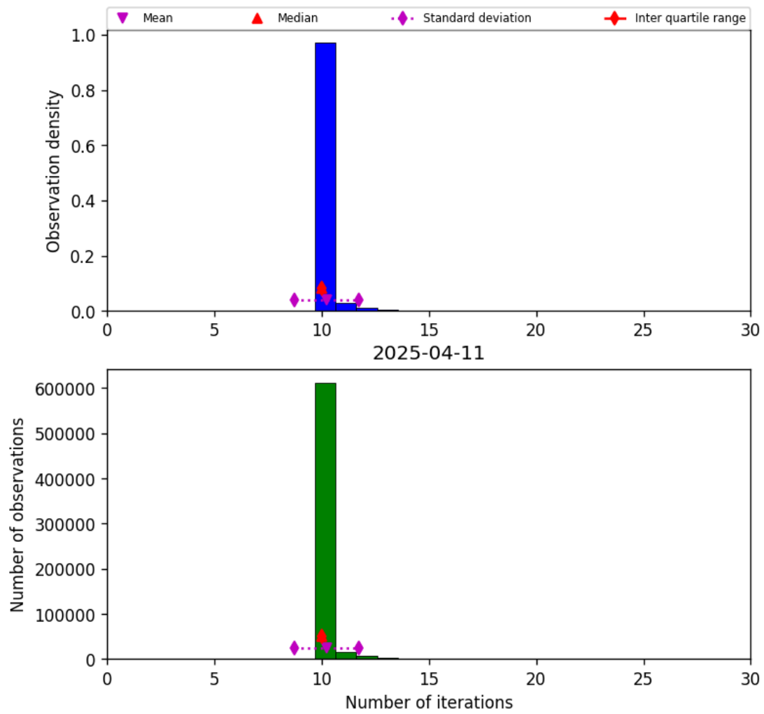
Figure 31: Histogram of “Number of iterations” for 2025-04-10 to 2025-04-12
