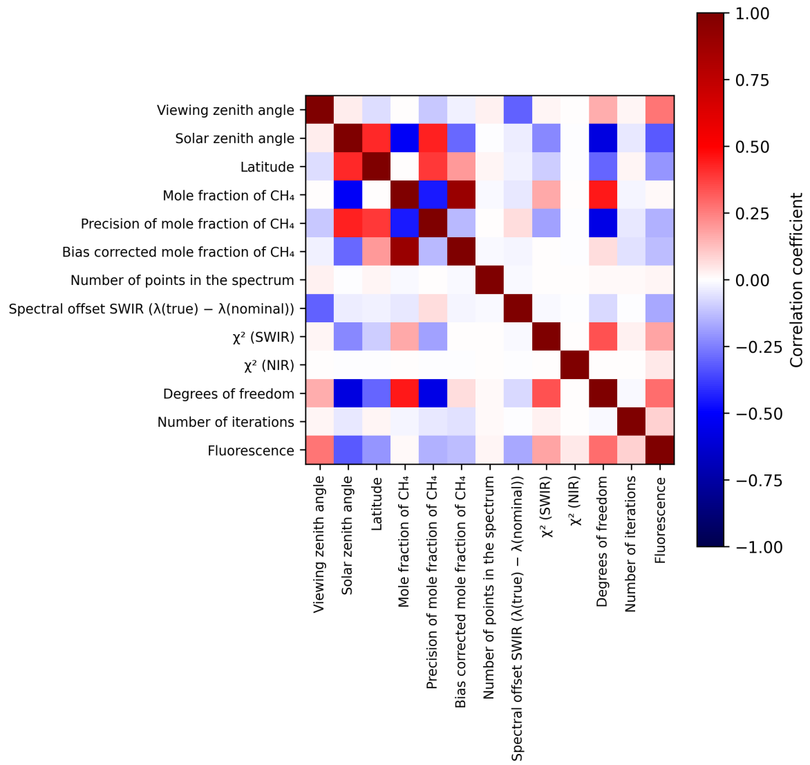
Figure 2: Map of correlation matrix for 2025-04-10 to 2025-04-12.
