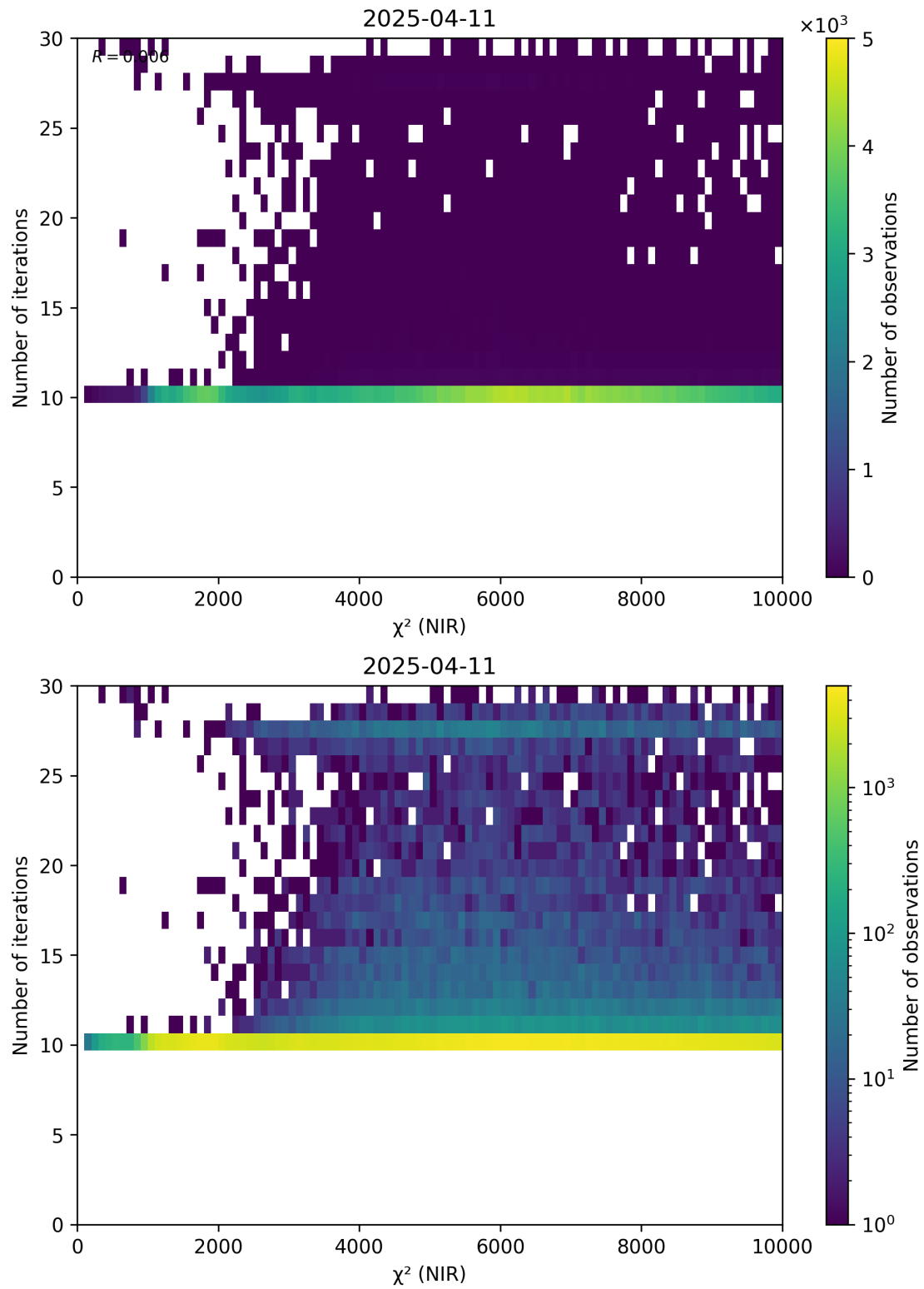
Figure 46: Scatter density plot of “ \chi^2 (NIR)” against “Number of iterations” for 2025-04-10 to 2025-04-12.
