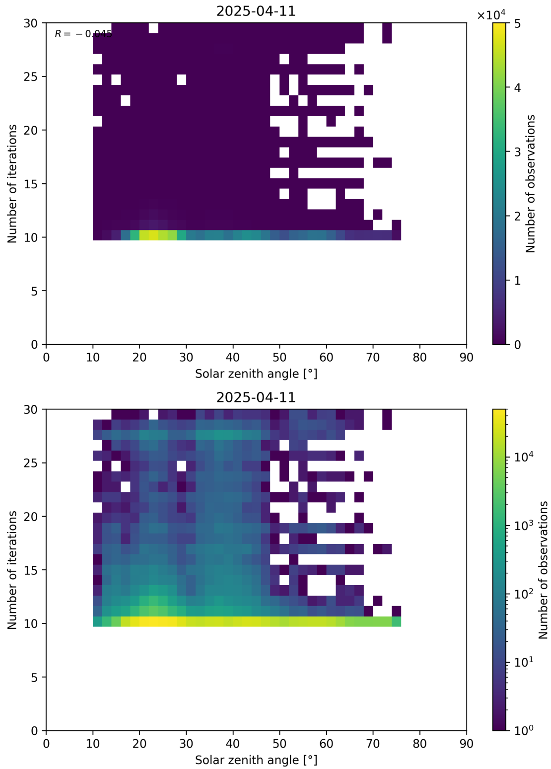
Figure 102: Scatter density plot of “Solar zenith angle” against “Number of iterations” for 2025-04-10 to 2025-04-12.
