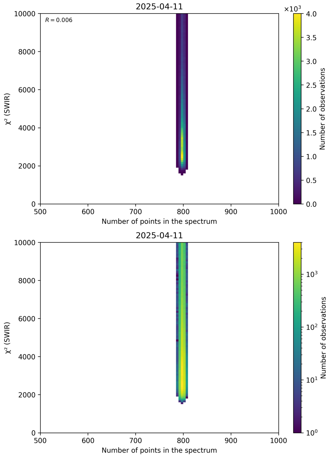
Figure 89: Scatter density plot of “Number of points in the spectrum” against “ \chi^2 (SWIR)” for 2025-04-10 to 2025-04-12.
