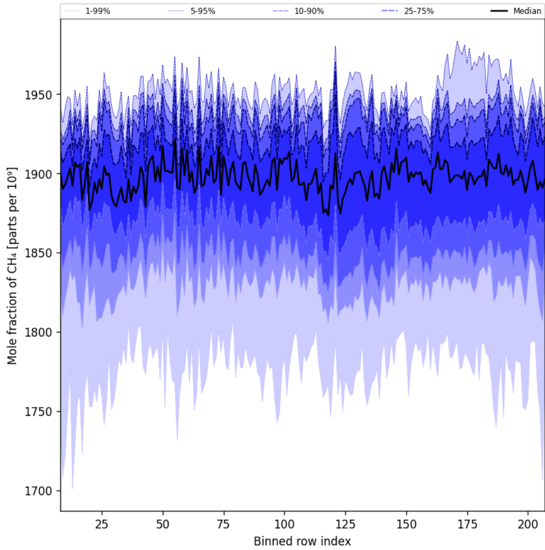
Figure 34: Along track statistics of “Mole fraction of CH 4 ” for 2025-04-10 to 2025-04-12
