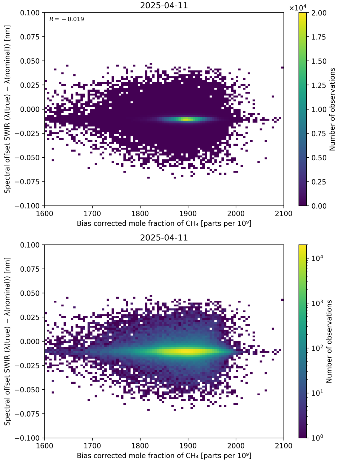
Figure 69: Scatter density plot of “Bias corrected mole fraction of \text{CH}_4 ” against “Spectral offset SWIR ( \lambda_{\text{true}} - \lambda_{\text{nominal}} )” for 2025-04-10 to 2025-04-12.
