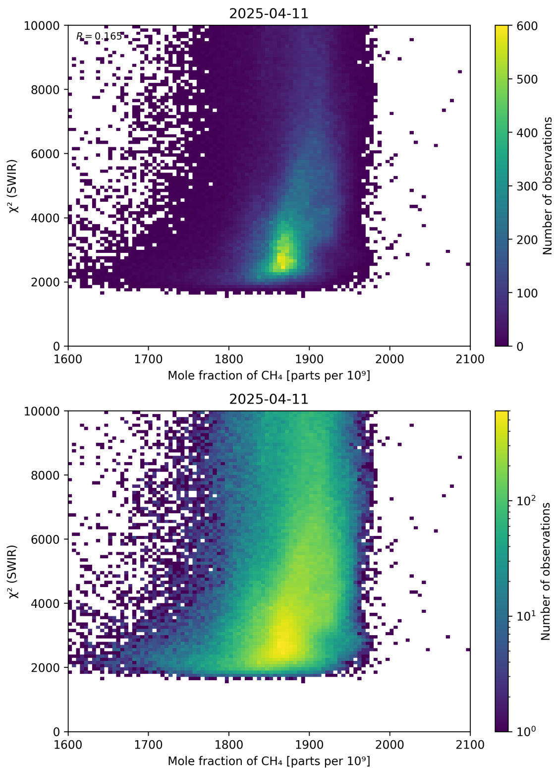
Figure 71: Scatter density plot of “Mole fraction of CH 4 ” against “ \chi^2 (SWIR)” for 2025-04-10 to 2025-04-12.
