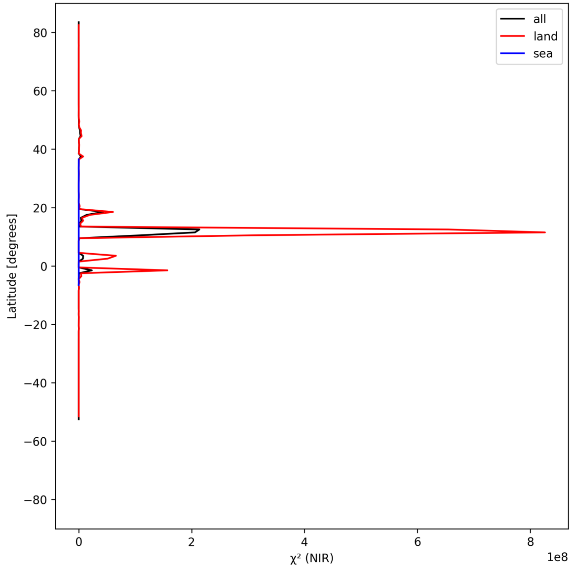
Figure 18: Zonal average of “ \chi^2 (NIR)” for 2025-04-10 to 2025-04-12.
