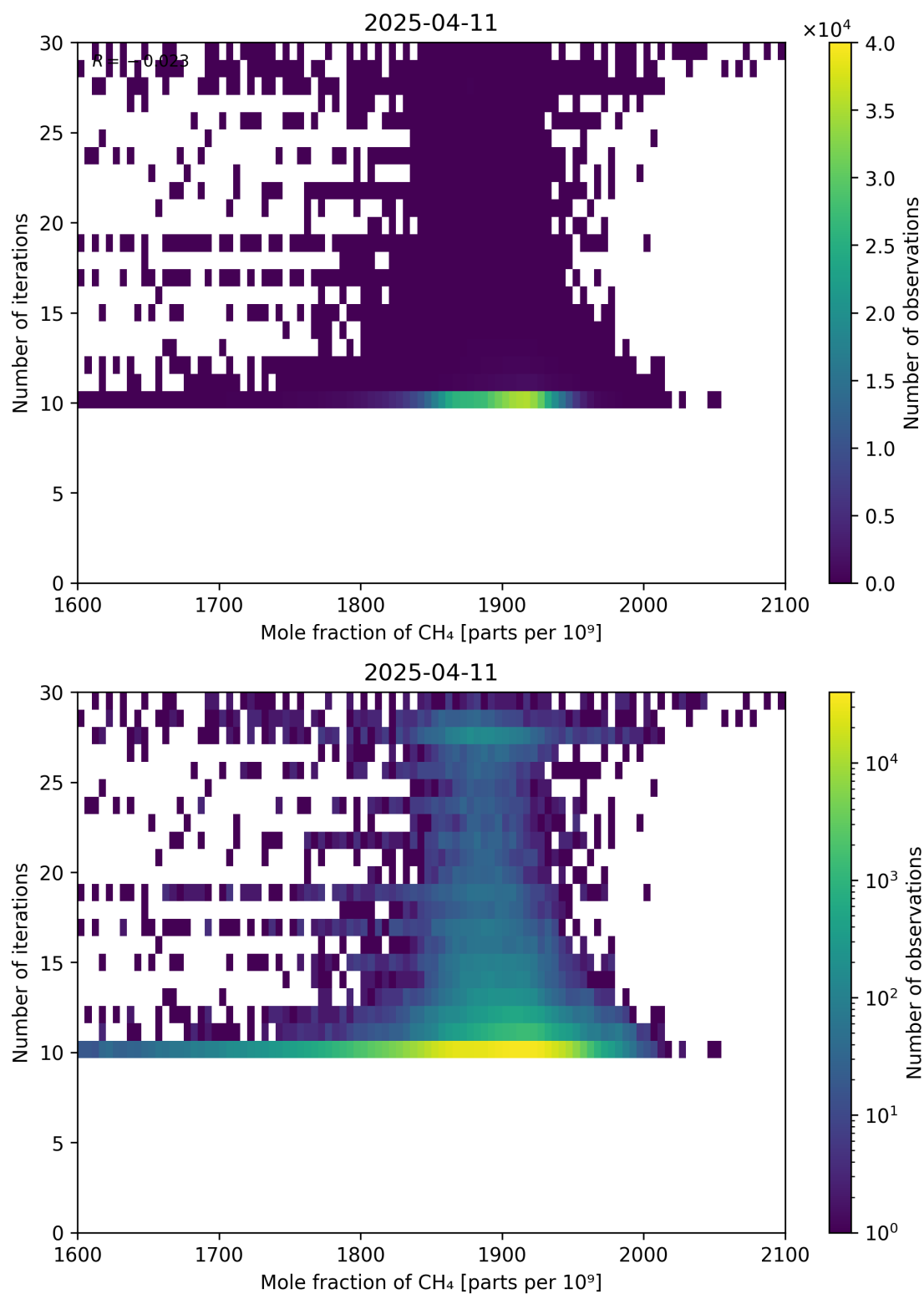
Figure 76: Scatter density plot of “Mole fraction of CH 4 ” against “Number of iterations” for 2025-04-10 to 2025-04-12.
