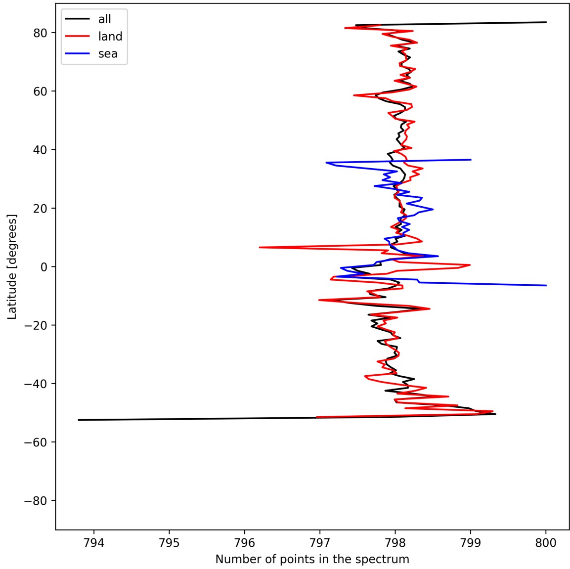
Figure 15: Zonal average of “Number of points in the spectrum” for 2025-04-10 to 2025-04-12.
