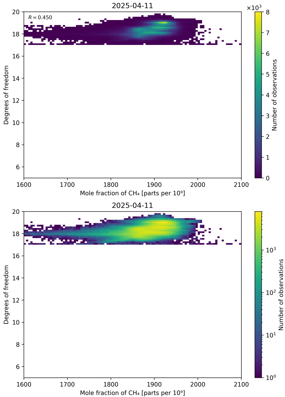
Figure 72: Scatter density plot of “Mole fraction of CH 4 ” against “Degrees of freedom” for 2025-04-10 to 2025-04-12.
