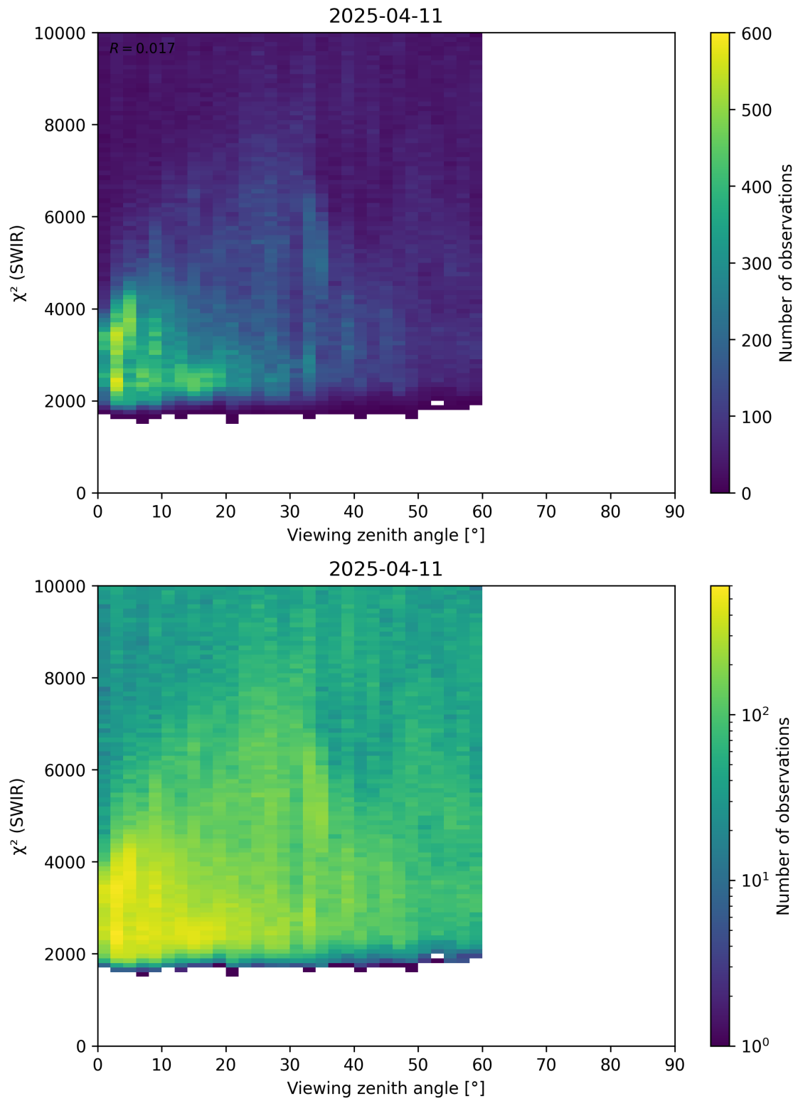
Figure 106: Scatter density plot of “Viewing zenith angle” against “ \chi^2 (SWIR)” for 2025-04-10 to 2025-04-12.
