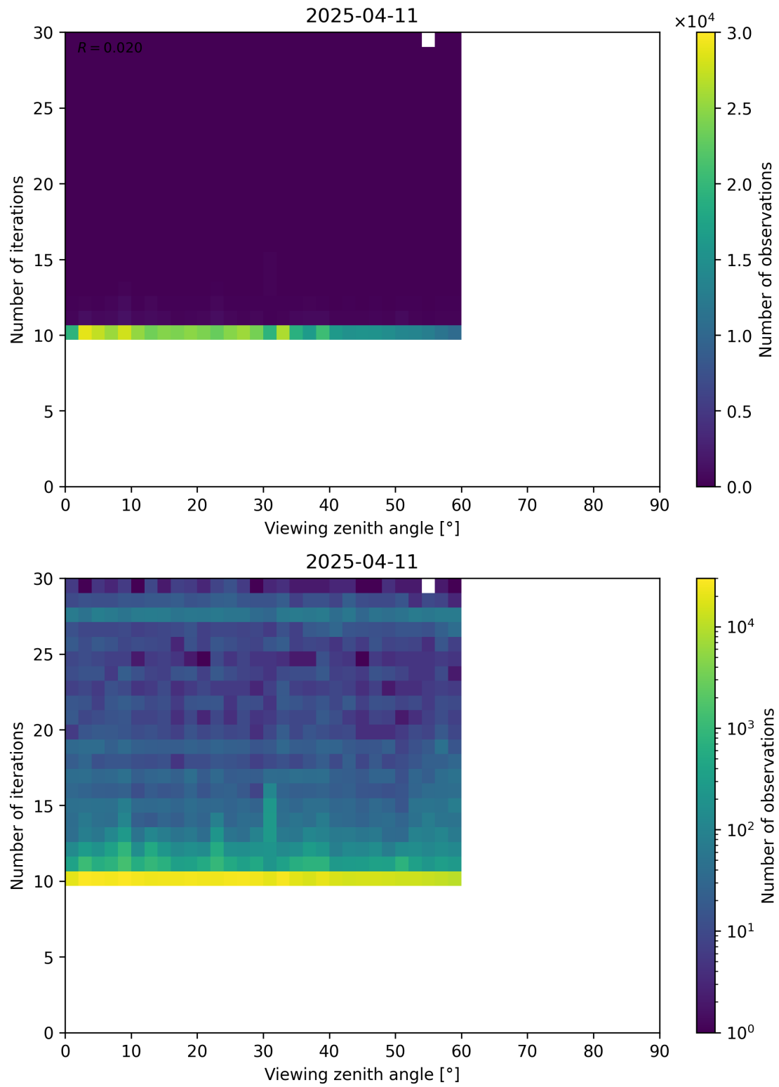
Figure 113: Scatter density plot of “Viewing zenith angle” against “Number of iterations” for 2025-04-10 to 2025-04-12.
