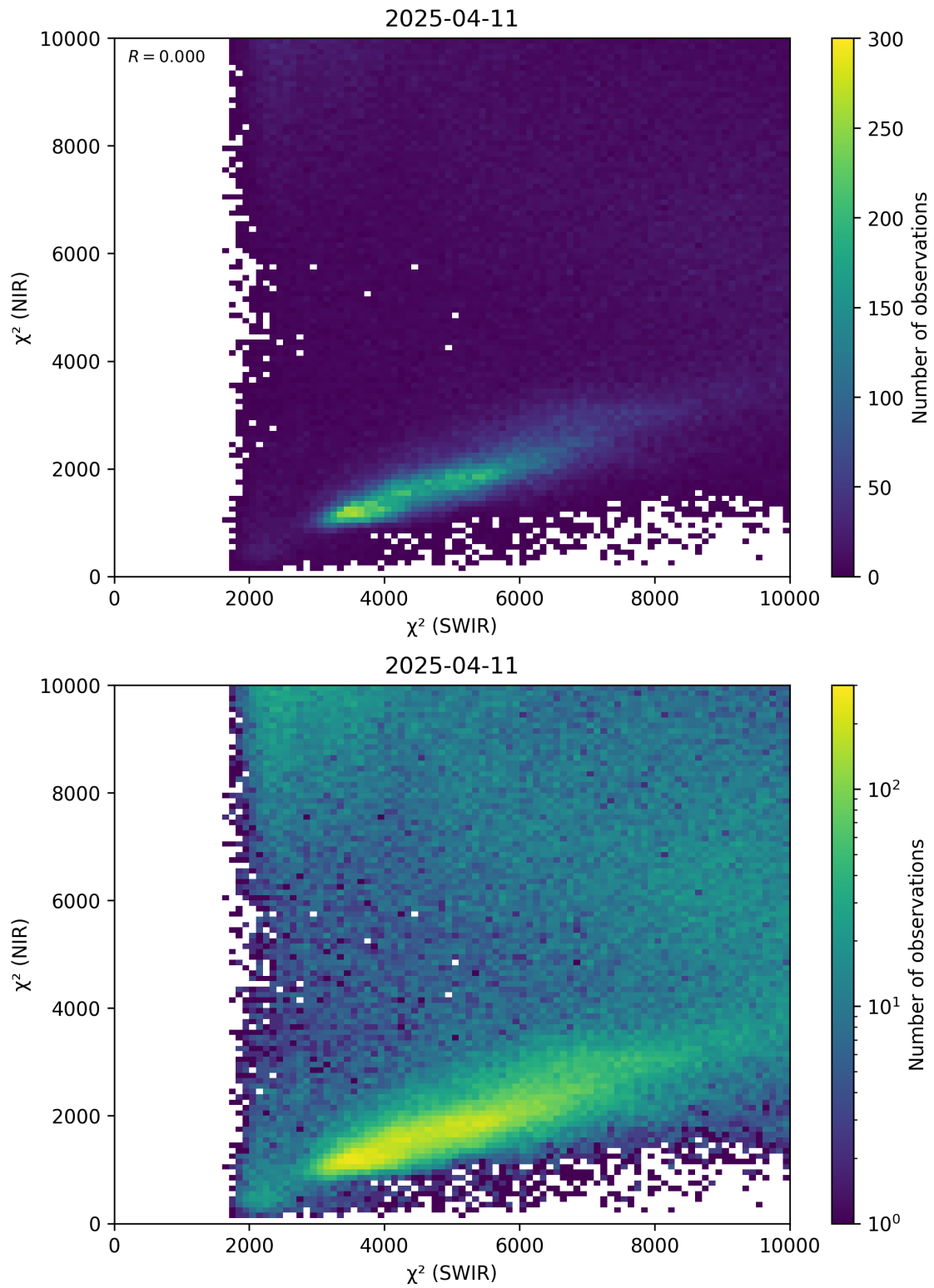
Figure 47: Scatter density plot of “ \chi^2 (SWIR)” against “ \chi^2 (NIR)” for 2025-04-10 to 2025-04-12.
