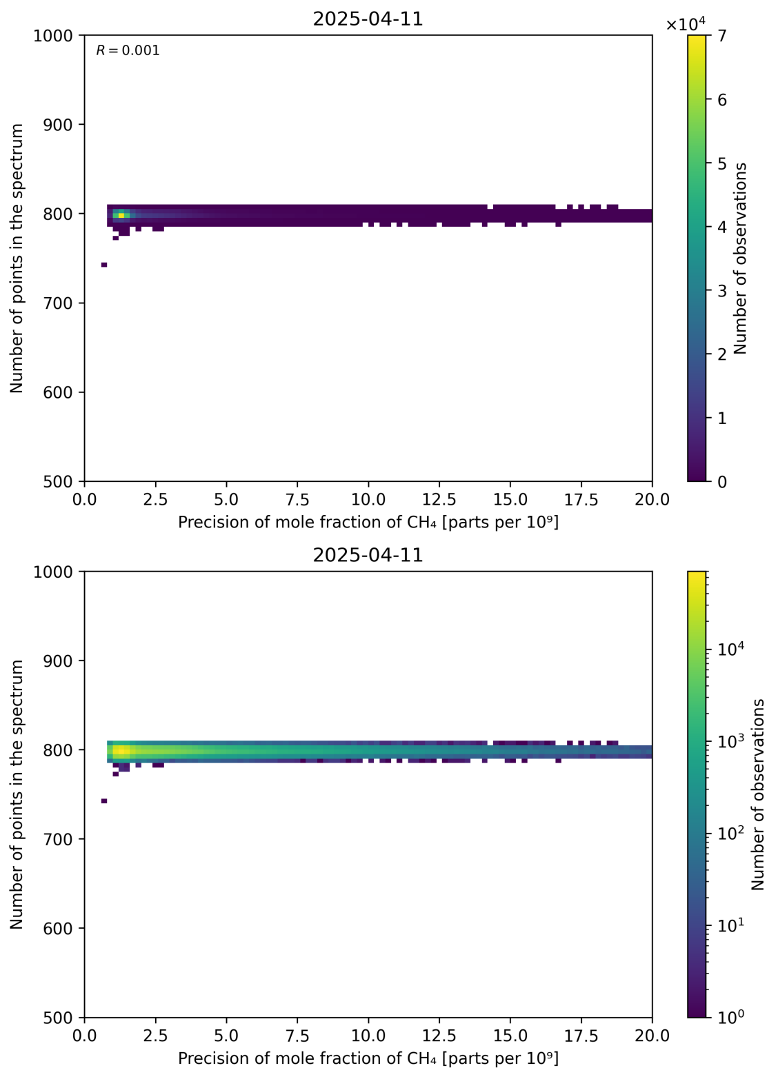
Figure 84: Scatter density plot of “Precision of mole fraction of CH 4 ” against “Number of points in the spectrum” for 2025-04-10 to 2025-04-12.
