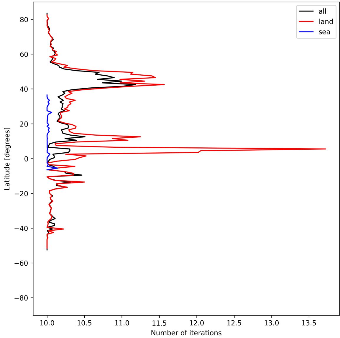
Figure 20: Zonal average of “Number of iterations” for 2025-04-10 to 2025-04-12.
