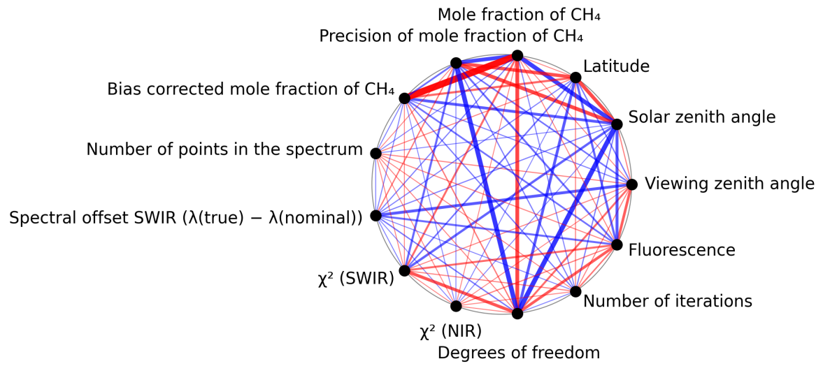
Figure 1: Map of correlation graph for 2025-04-10 to 2025-04-12.
