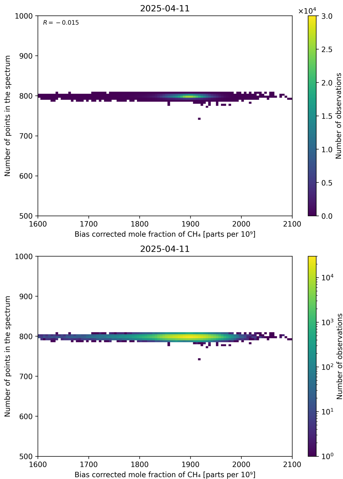
Figure 68: Scatter density plot of “Bias corrected mole fraction of CH 4 ” against “Number of points in the spectrum” for 2025-04-10 to 2025-04-12.
