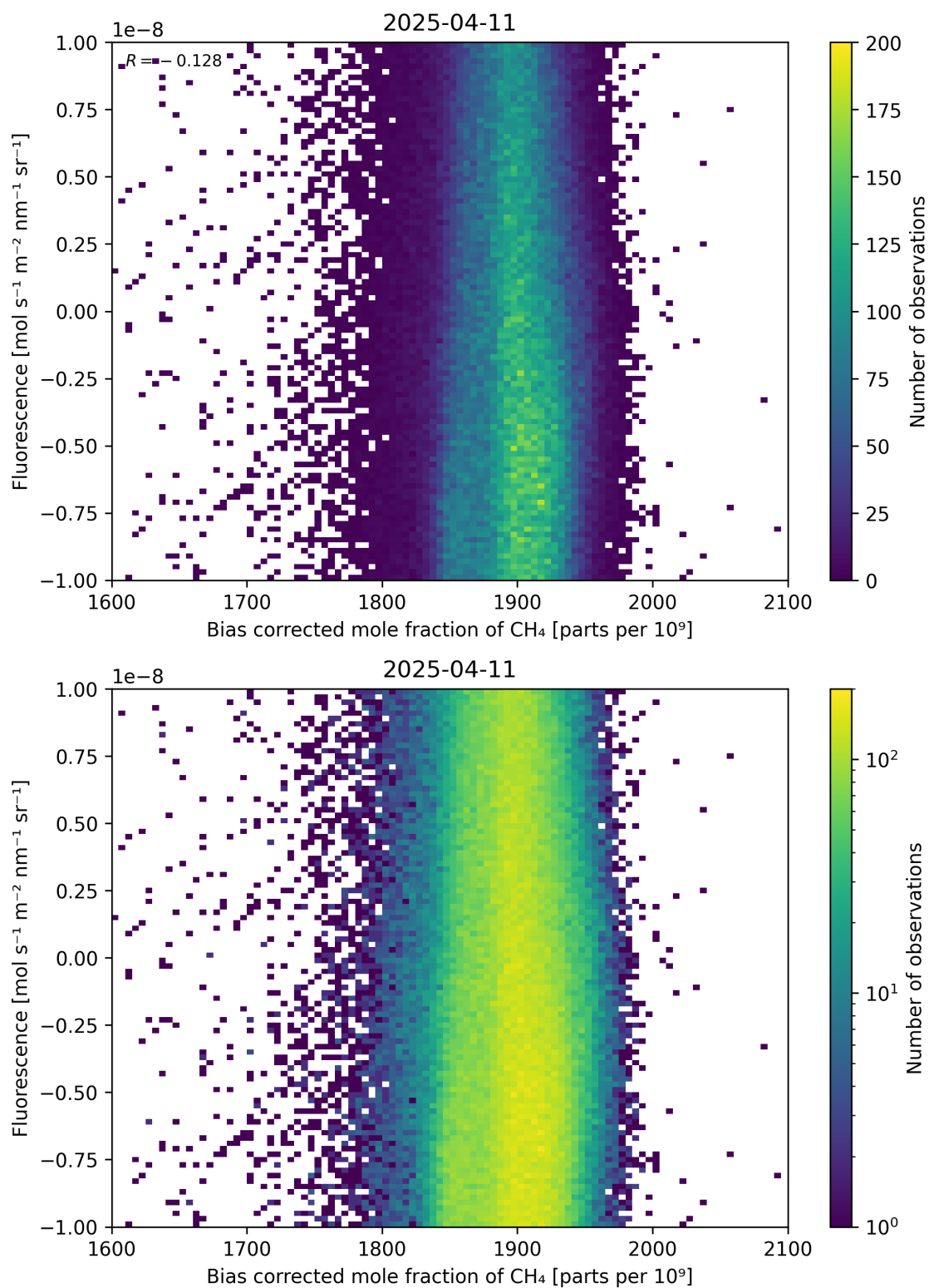
Figure 66: Scatter density plot of “Bias corrected mole fraction of \text{CH}_4 ” against “Fluorescence” for 2025-04-10 to 2025-04-12.
