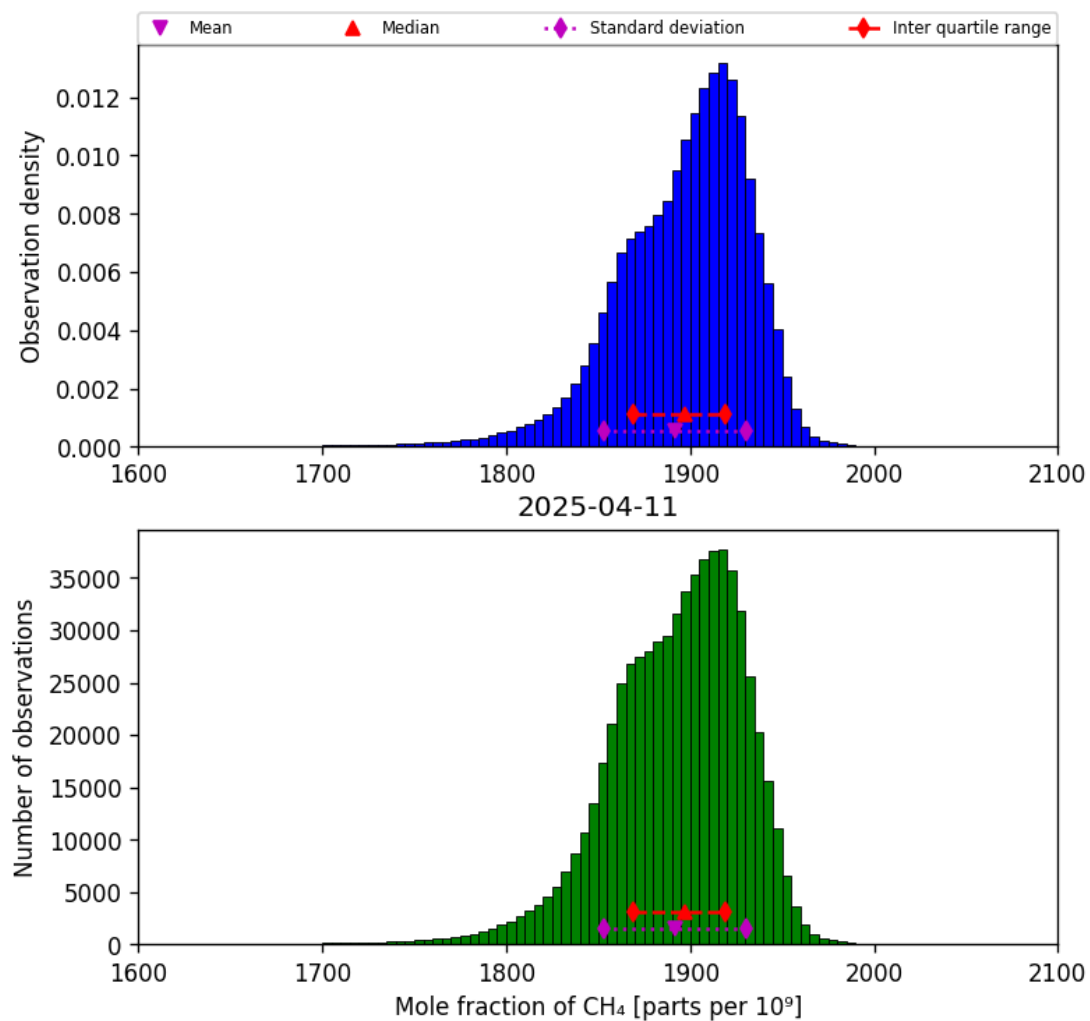
Figure 23: Histogram of “Mole fraction of CH 4 ” for 2025-04-10 to 2025-04-12
