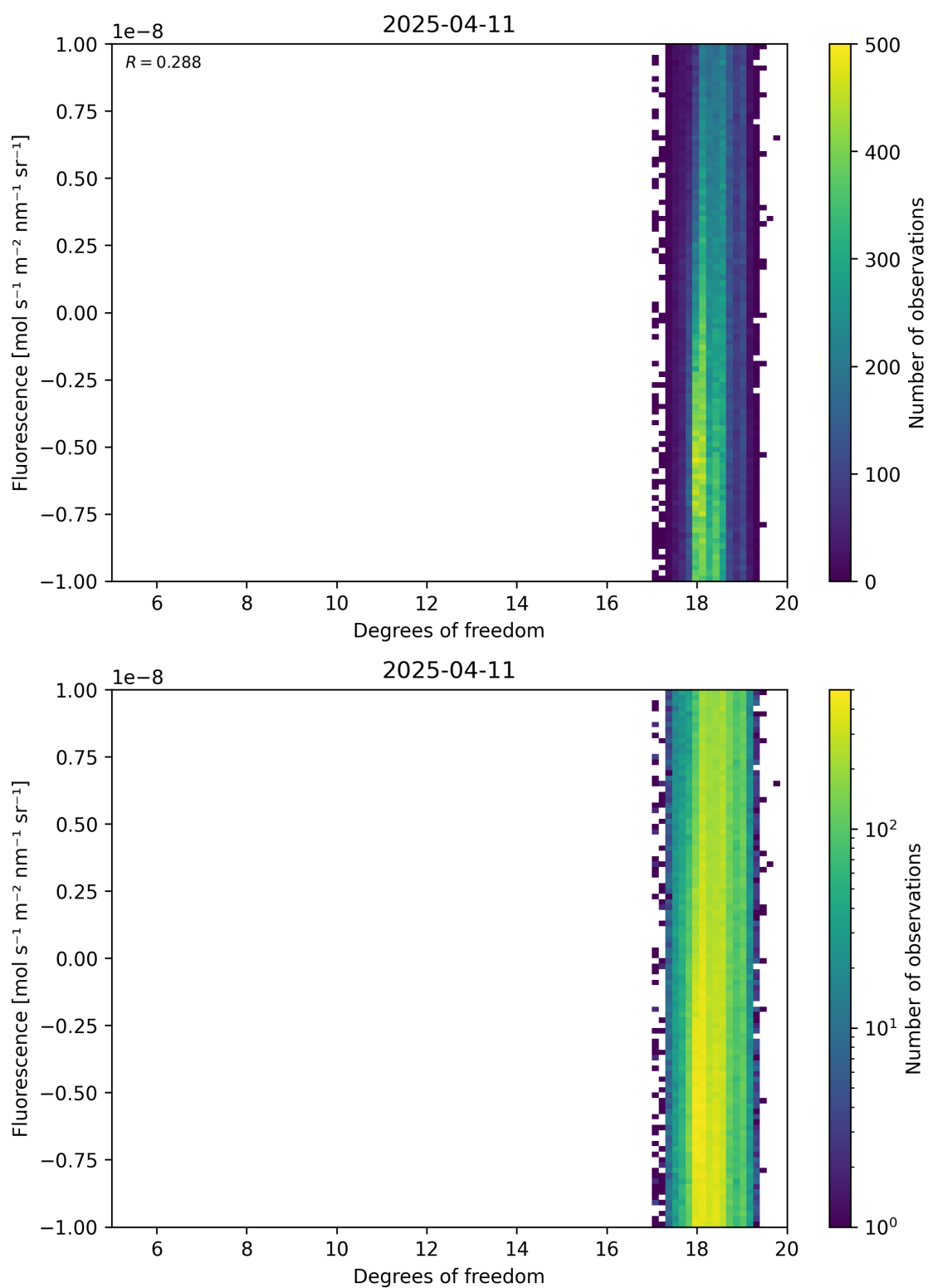
Figure 51: Scatter density plot of “Degrees of freedom” against “Fluorescence” for 2025-04-10 to 2025-04-12.
