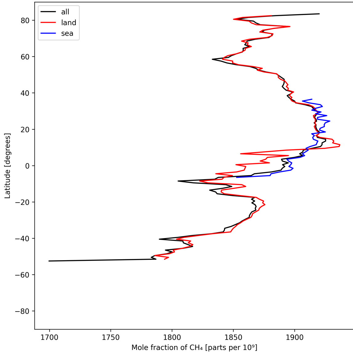
Figure 12: Zonal average of “Mole fraction of \text{CH}_4 ” for 2025-04-10 to 2025-04-12.
