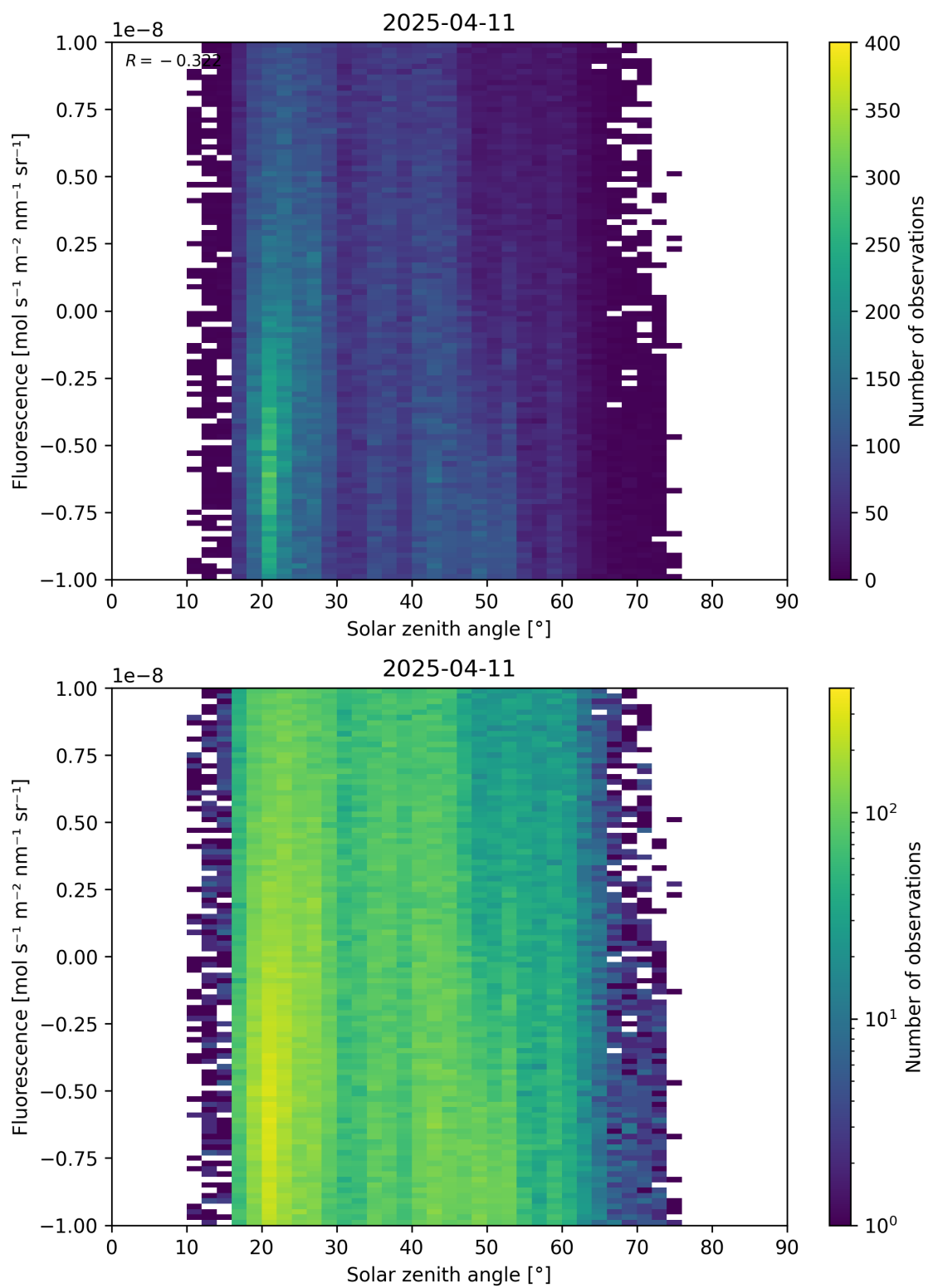
Figure 97: Scatter density plot of “Solar zenith angle” against “Fluorescence” for 2025-04-10 to 2025-04-12.
