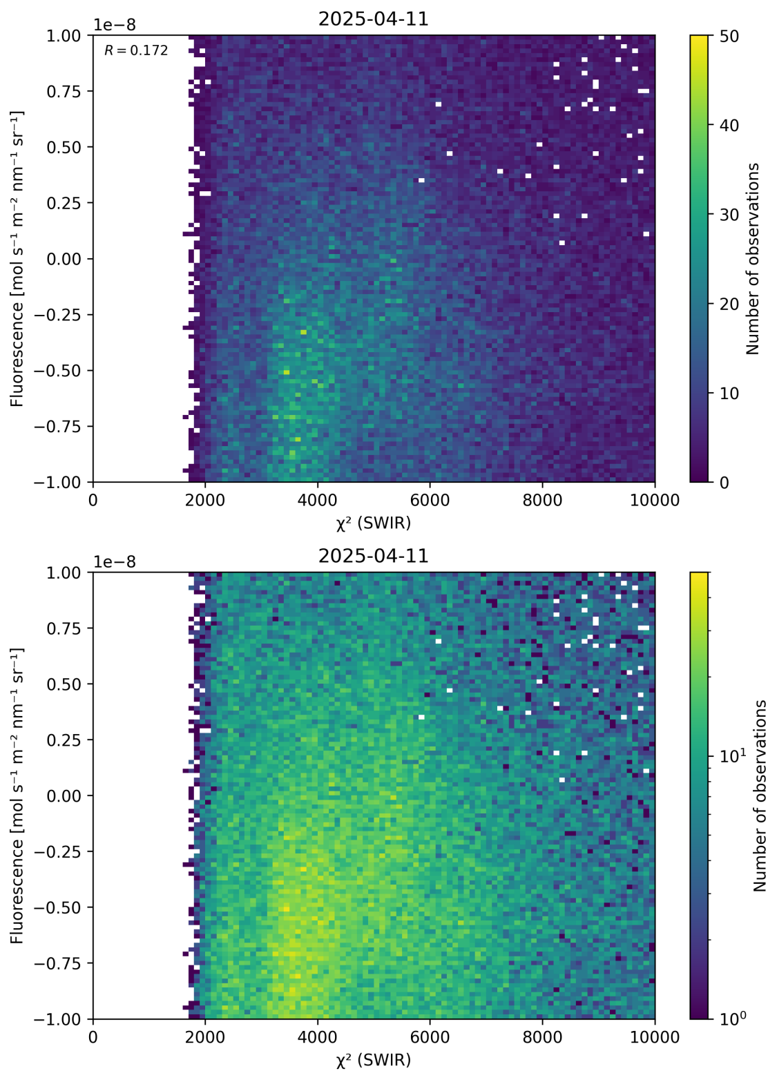
Figure 49: Scatter density plot of “ \chi^2 (SWIR)” against “Fluorescence” for 2025-04-10 to 2025-04-12.
