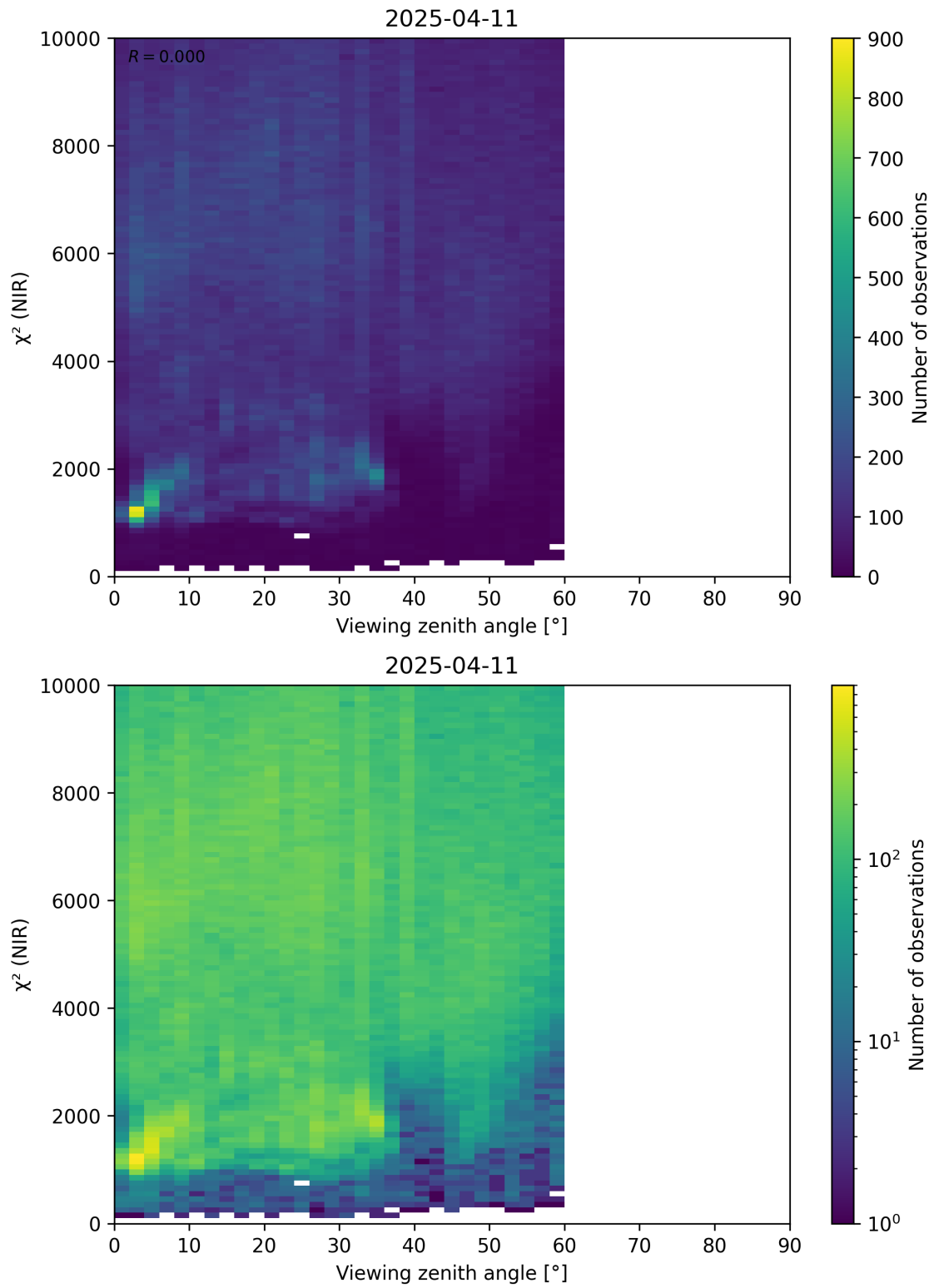
Figure 105: Scatter density plot of “Viewing zenith angle” against “ \chi^2 (NIR)” for 2025-04-10 to 2025-04-12.
