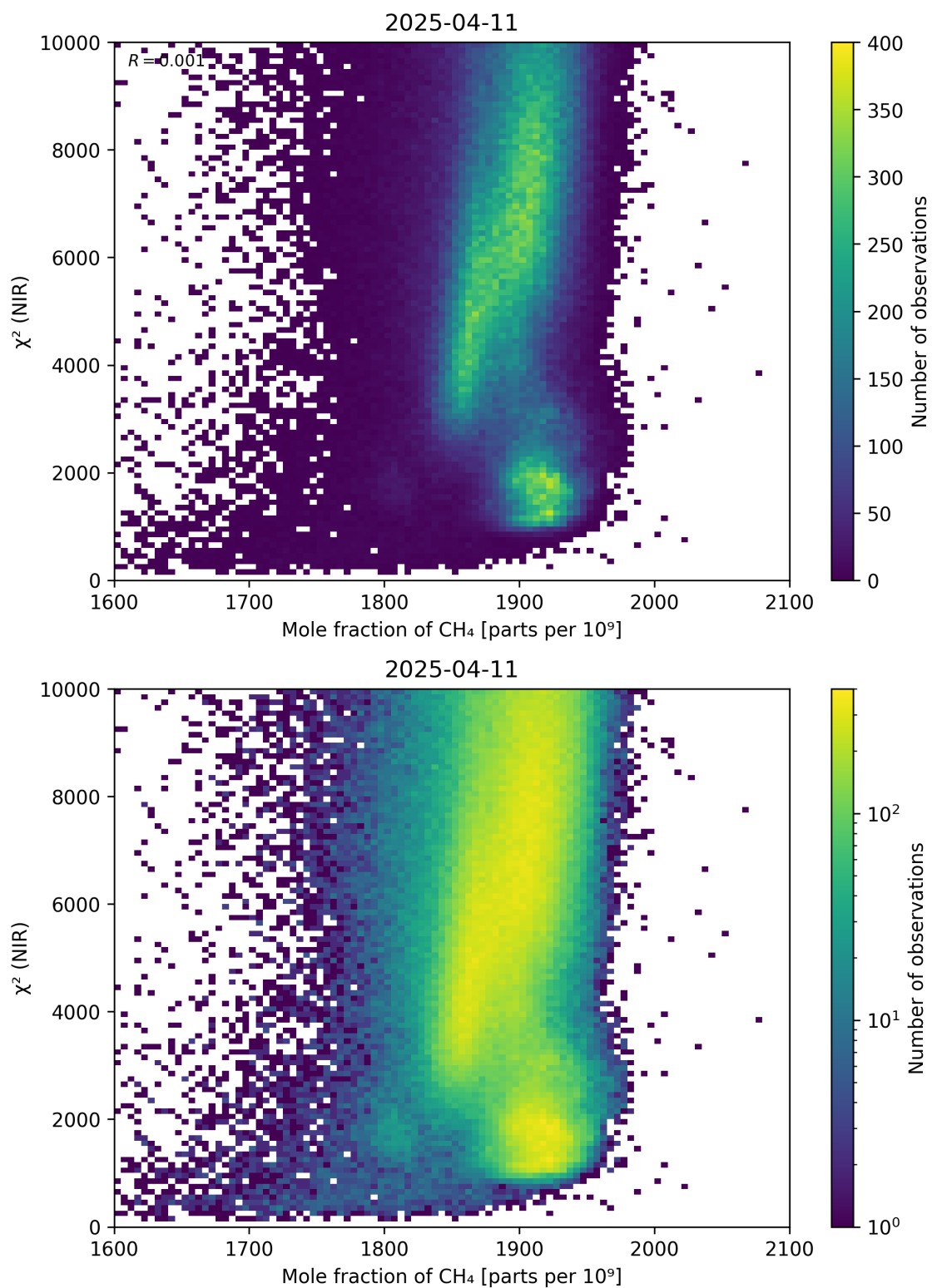
Figure 70: Scatter density plot of “Mole fraction of \text{CH}_4 ” against “ \chi^2 (NIR)” for 2025-04-10 to 2025-04-12.
