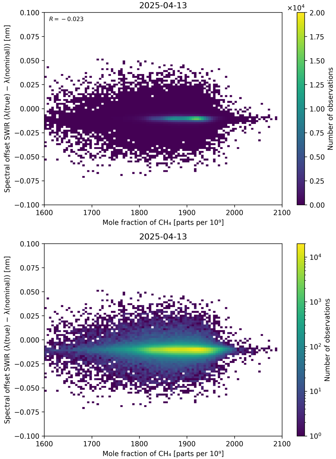
Figure 86: Scatter density plot of “Mole fraction of \text{CH}_4 ” against “Spectral offset SWIR ( \lambda_{\text{true}} - \lambda_{\text{nominal}} )” for 2025-04-13 to 2025-04-14.
