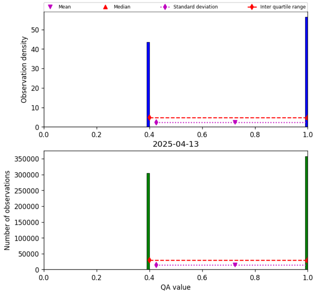
Figure 22: Histogram of “QA value” for 2025-04-13 to 2025-04-14
