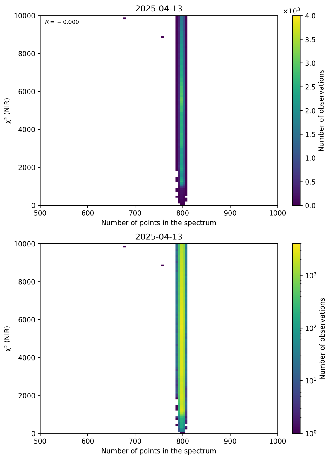
Figure 88: Scatter density plot of “Number of points in the spectrum” against “ \chi^2 (NIR)” for 2025-04-13 to 2025-04-14.
