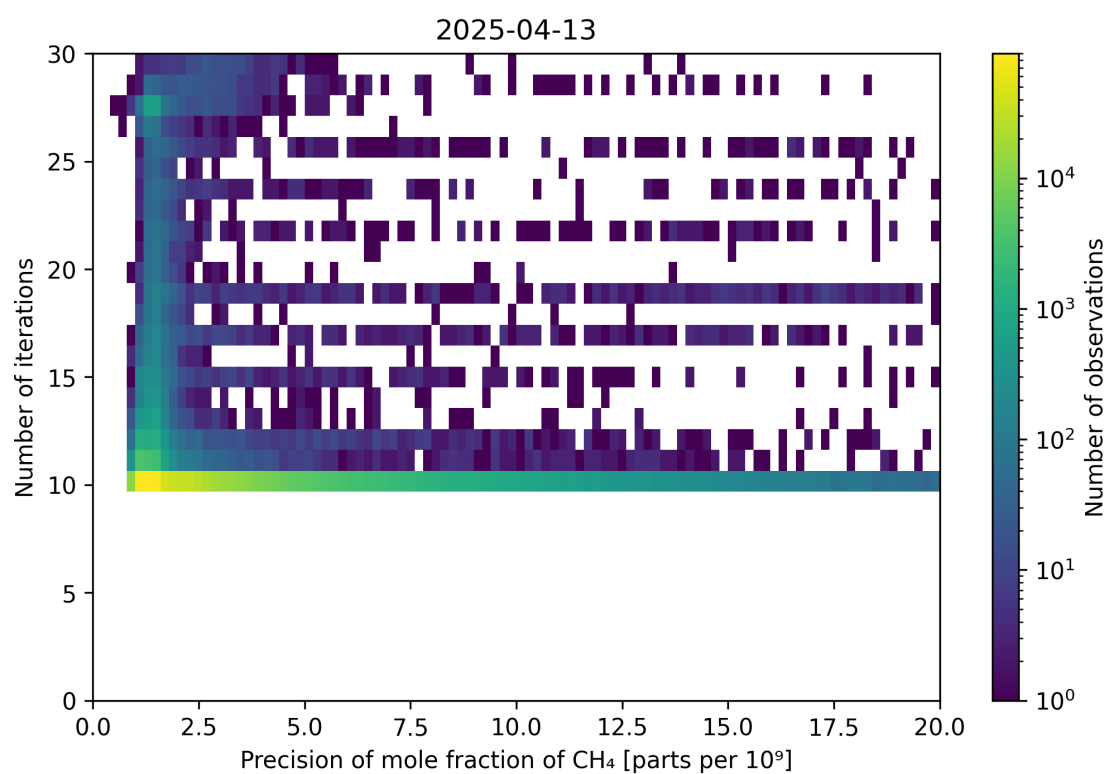
Figure 83: Scatter density plot of “Precision of mole fraction of CH 4 ” against “Number of iterations” for 2025-04-13 to 2025-04-14.
