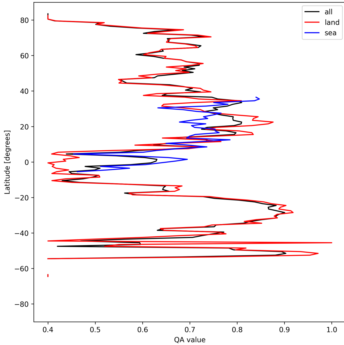
Figure 11: Zonal average of “QA value” for 2025-04-13 to 2025-04-14.
