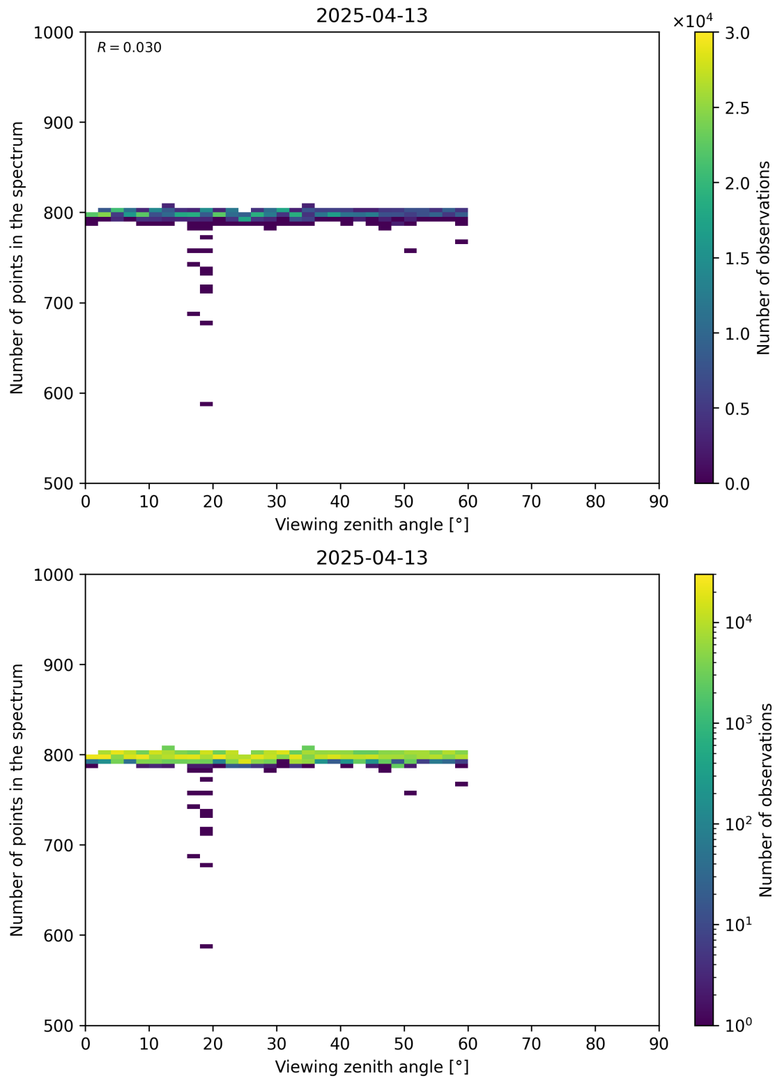
Figure 114: Scatter density plot of “Viewing zenith angle” against “Number of points in the spectrum” for 2025-04-13 to 2025-04-14.
