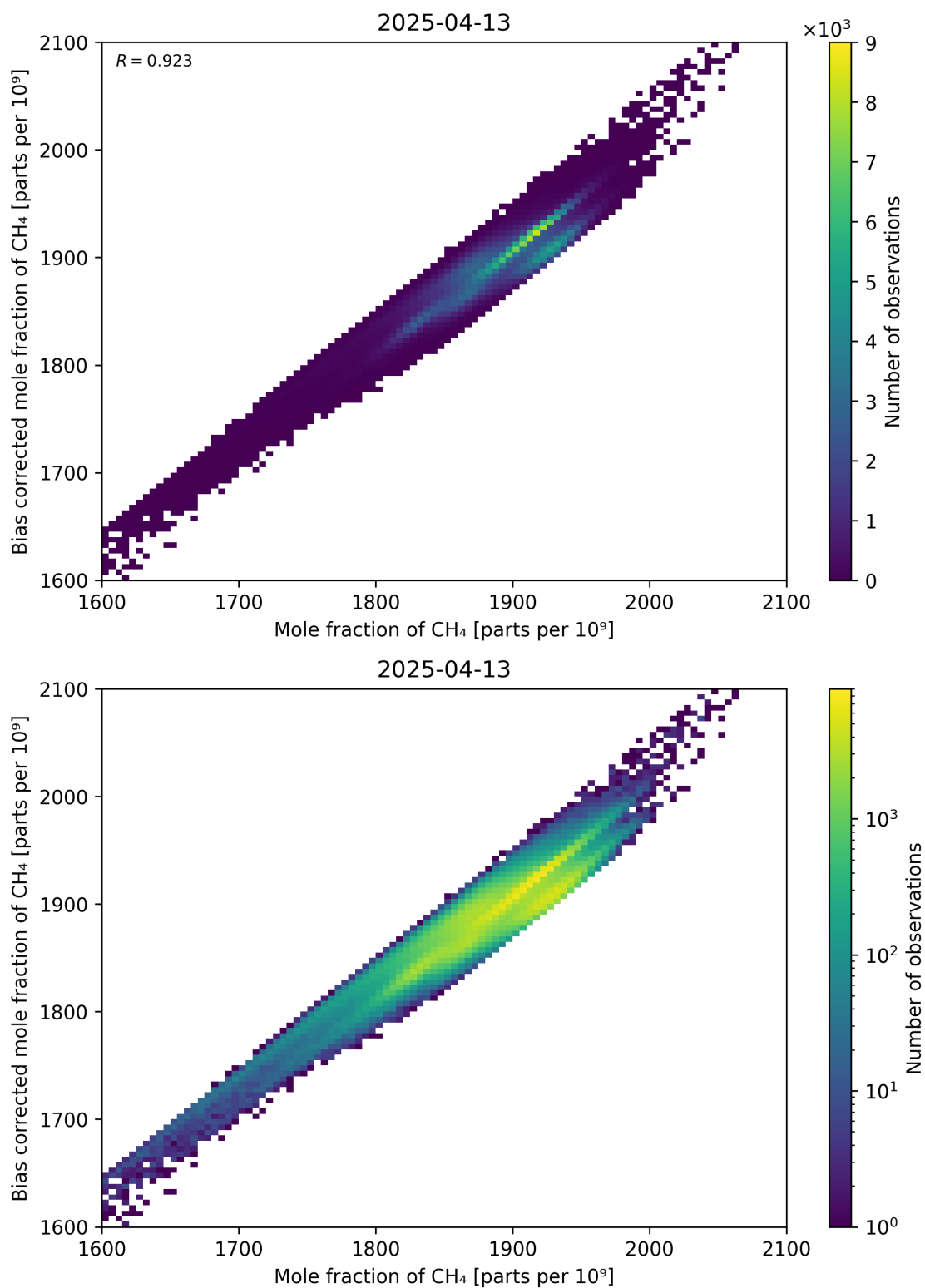
Figure 74: Scatter density plot of “Mole fraction of CH 4 ” against “Bias corrected mole fraction of CH 4 ” for 2025-04-13 to 2025-04-14.
