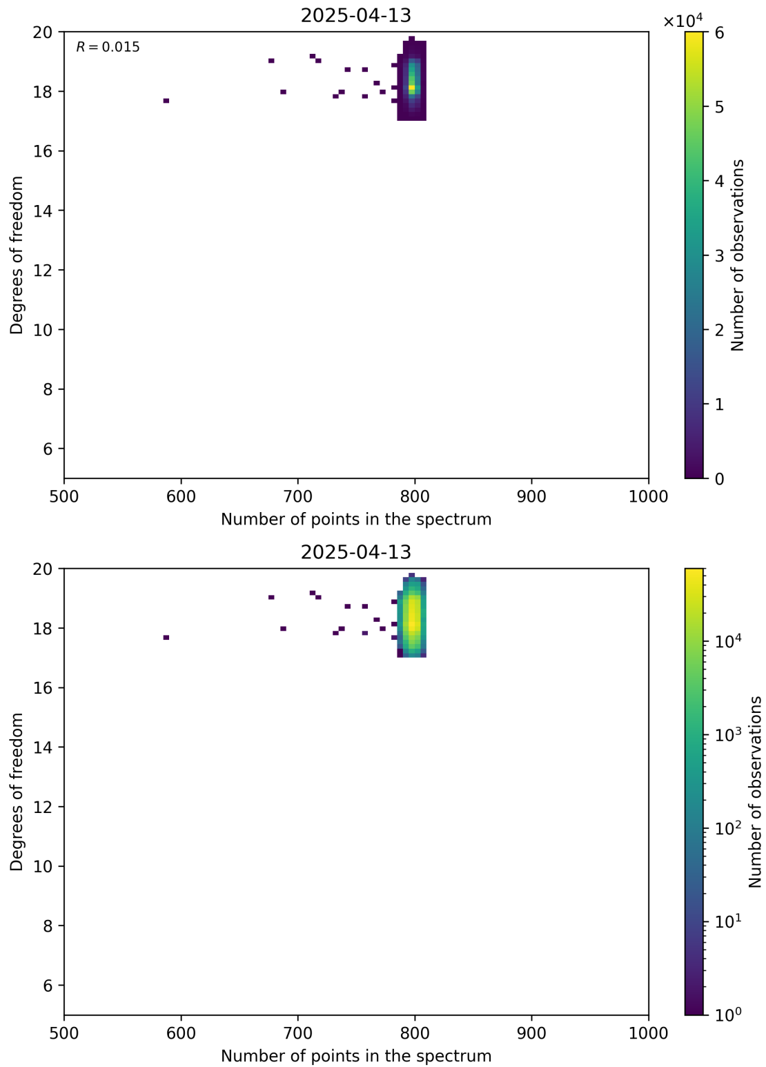
Figure 90: Scatter density plot of “Number of points in the spectrum” against “Degrees of freedom” for 2025-04-13 to 2025-04-14.
