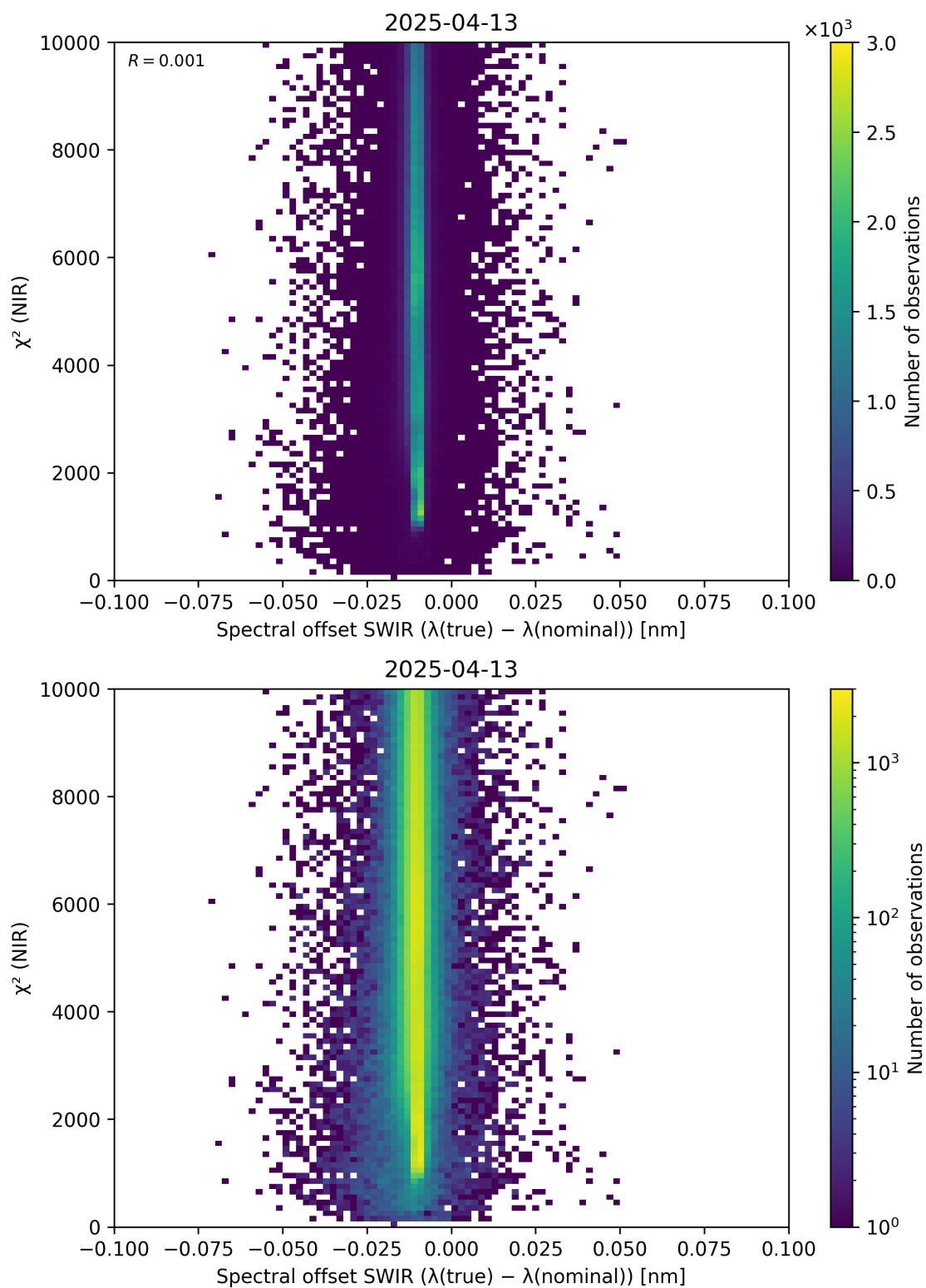
Figure 117: Scatter density plot of “Spectral offset SWIR ( \lambda_{\text{true}} - \lambda_{\text{nominal}} )” against “ \chi^2 (NIR)” for 2025-04-13 to 2025-04-14.
