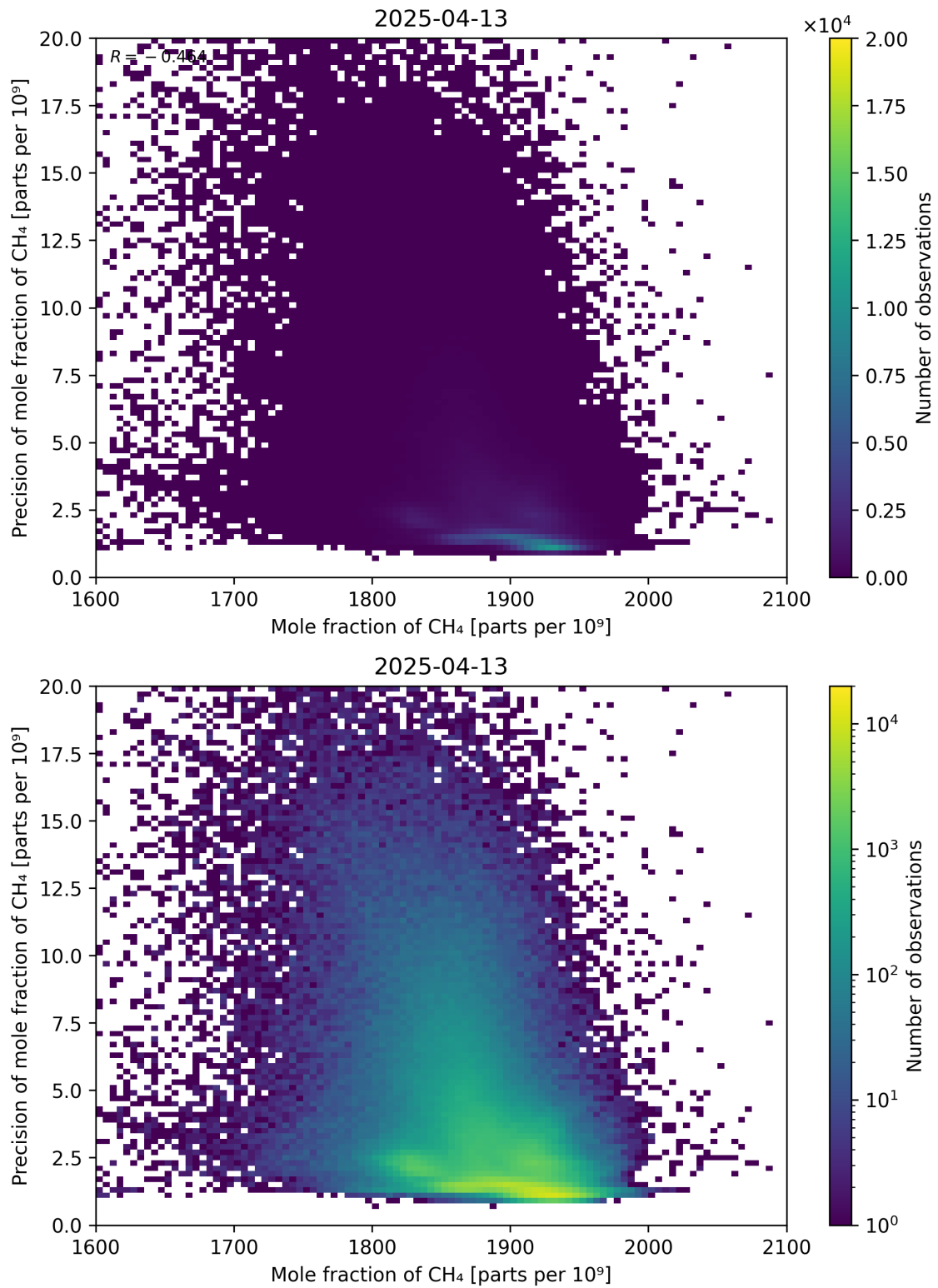
Figure 75: Scatter density plot of “Mole fraction of CH 4 ” against “Precision of mole fraction of CH 4 ” for 2025-04-13 to 2025-04-14.
