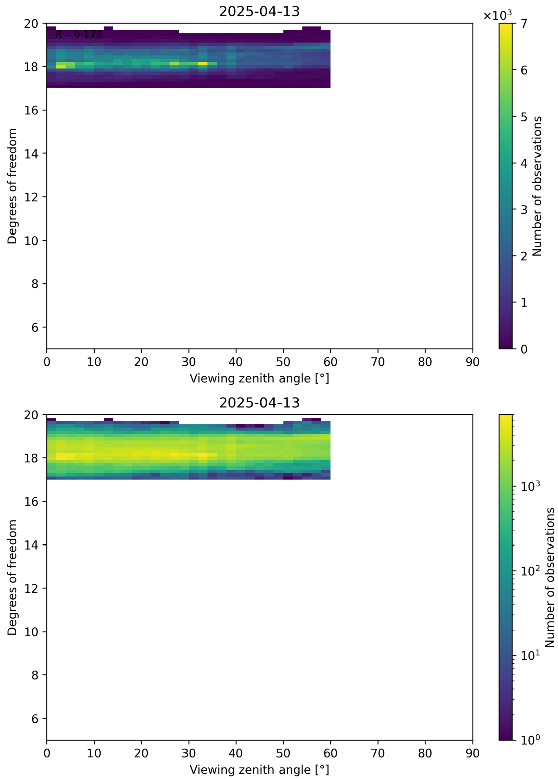
Figure 107: Scatter density plot of “Viewing zenith angle” against “Degrees of freedom” for 2025-04-13 to 2025-04-14.
