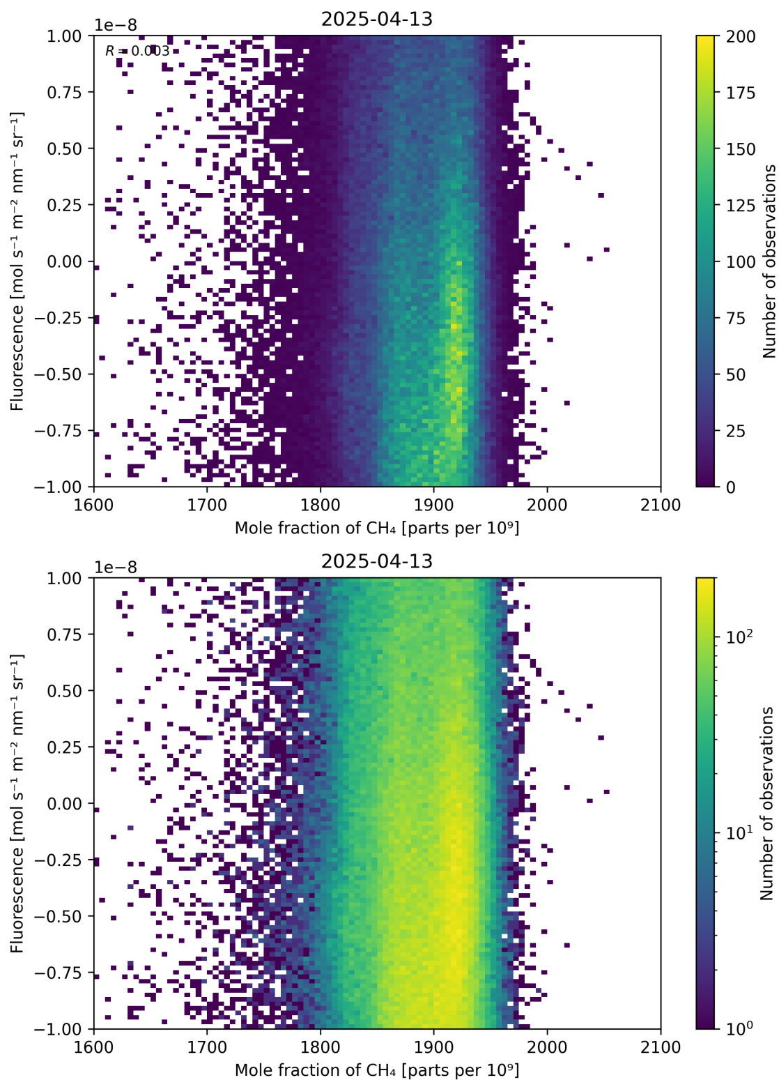
Figure 73: Scatter density plot of “Mole fraction of \text{CH}_4 ” against “Fluorescence” for 2025-04-13 to 2025-04-14.
