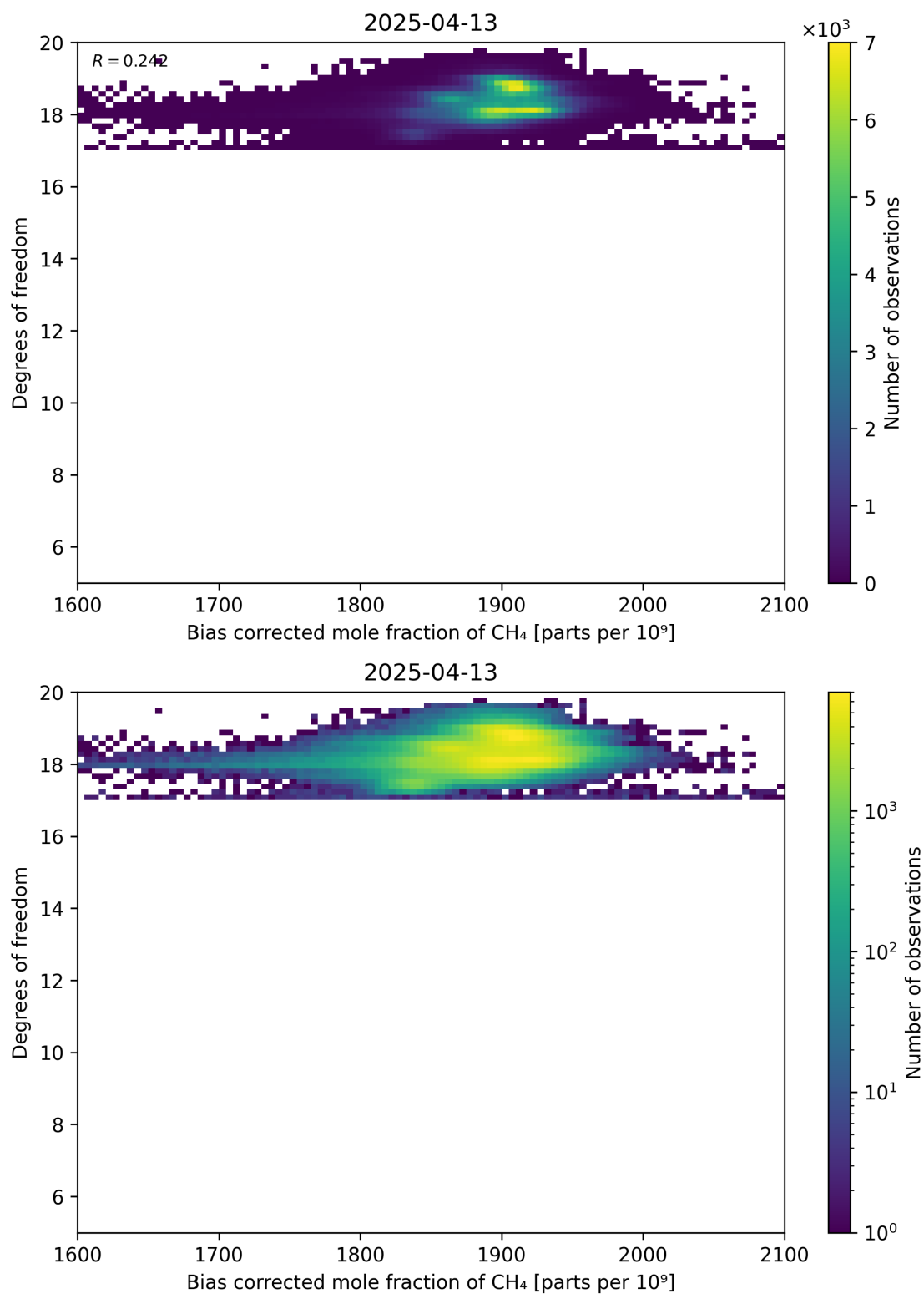
Figure 65: Scatter density plot of “Bias corrected mole fraction of CH 4 ” against “Degrees of freedom” for 2025-04-13 to 2025-04-14.
