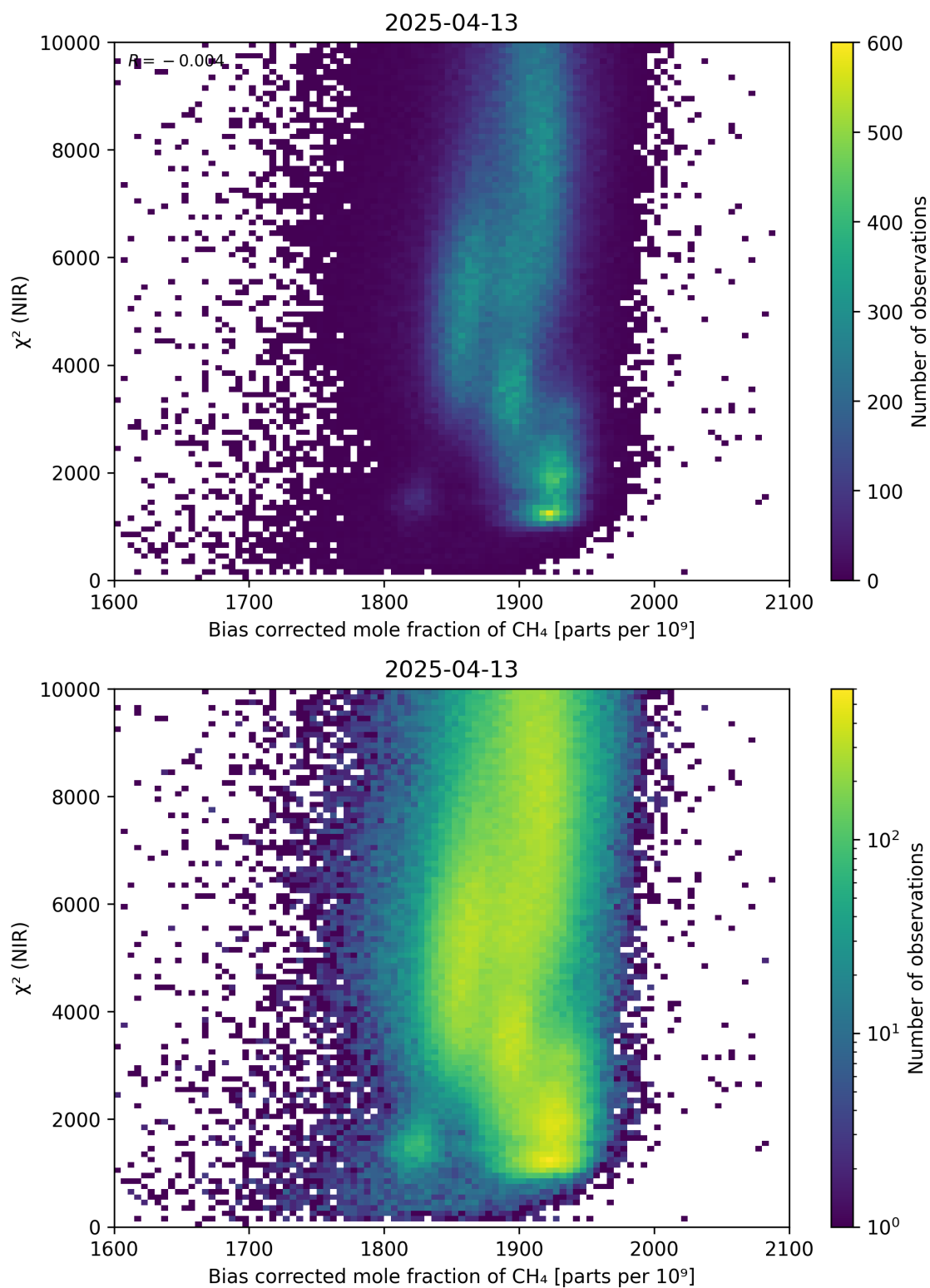
Figure 63: Scatter density plot of “Bias corrected mole fraction of CH 4 ” against “ \chi^2 (NIR)” for 2025-04-13 to 2025-04-14.
