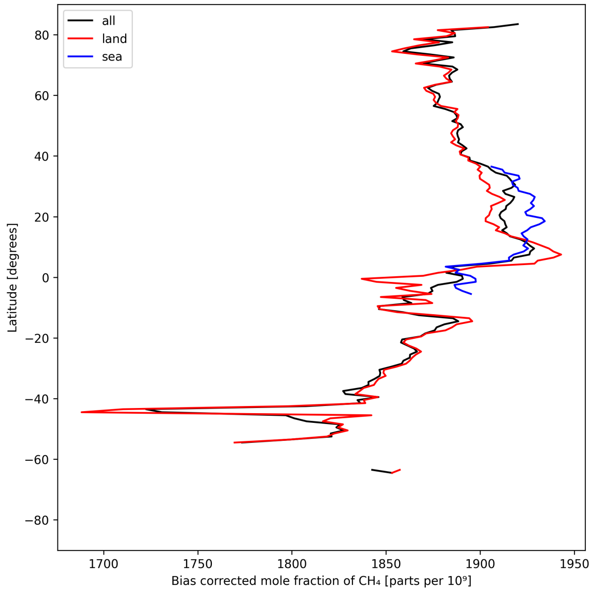
Figure 14: Zonal average of “Bias corrected mole fraction of CH 4 ” for 2025-04-13 to 2025-04-14.
