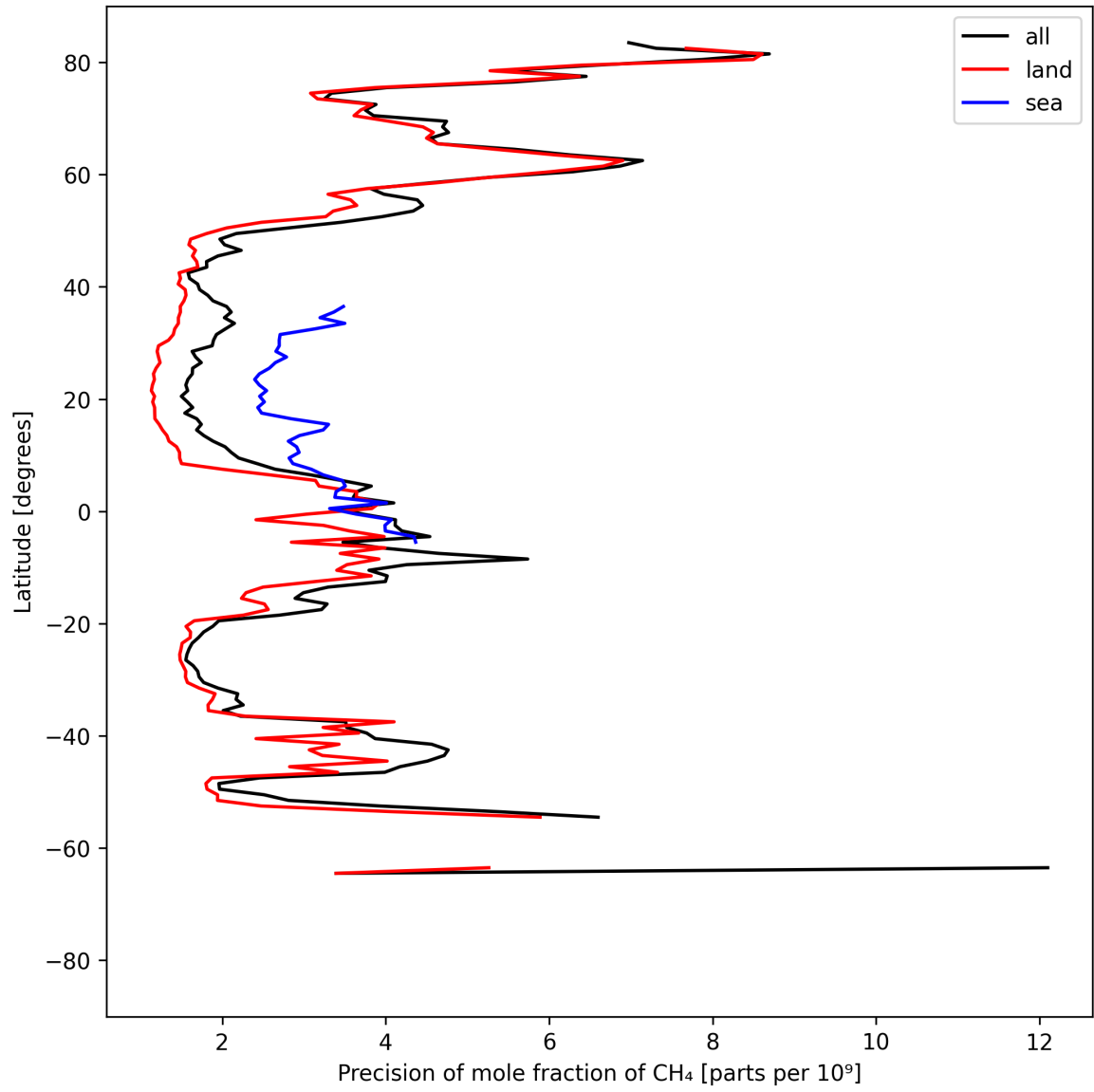
Figure 13: Zonal average of “Precision of mole fraction of CH 4 ” for 2025-04-13 to 2025-04-14.
