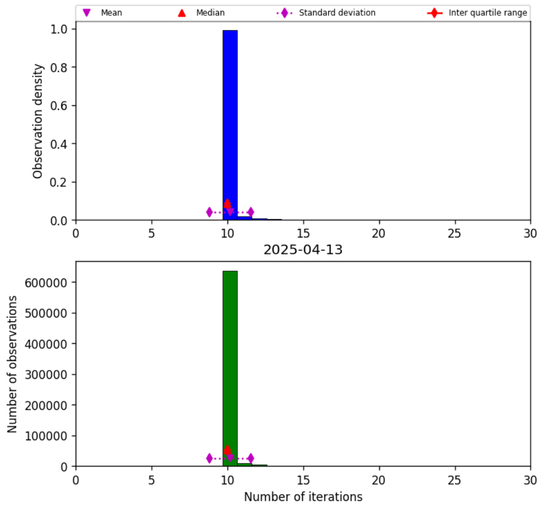
Figure 31: Histogram of “Number of iterations” for 2025-04-13 to 2025-04-14
