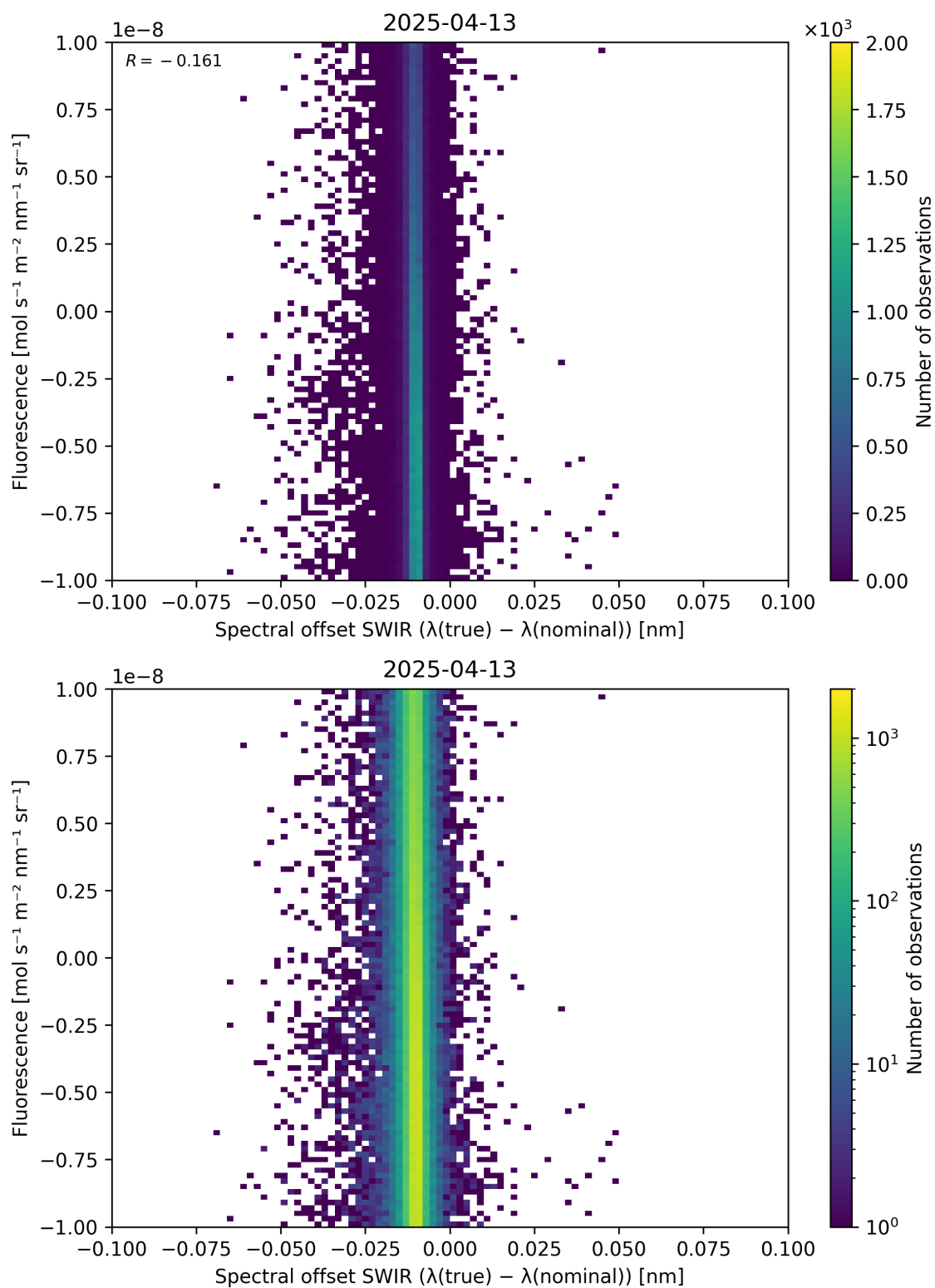
Figure 120: Scatter density plot of “Spectral offset SWIR ( \lambda_{\text{true}} - \lambda_{\text{nominal}} )” against “Fluorescence” for 2025-04-13 to 2025-04-14.
