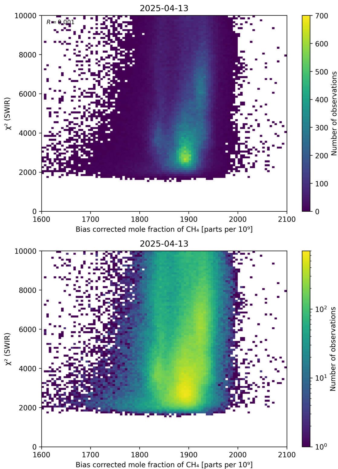
Figure 64: Scatter density plot of “Bias corrected mole fraction of \text{CH}_4 ” against “ \chi^2 (SWIR)” for 2025-04-13 to 2025-04-14.
