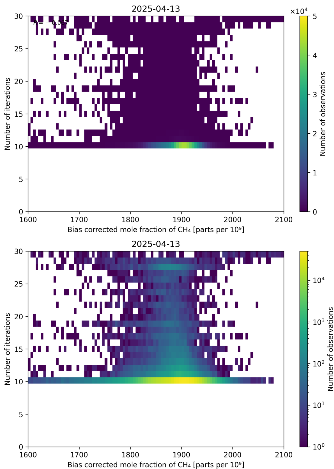
Figure 67: Scatter density plot of “Bias corrected mole fraction of CH 4 ” against “Number of iterations” for 2025-04-13 to 2025-04-14.
