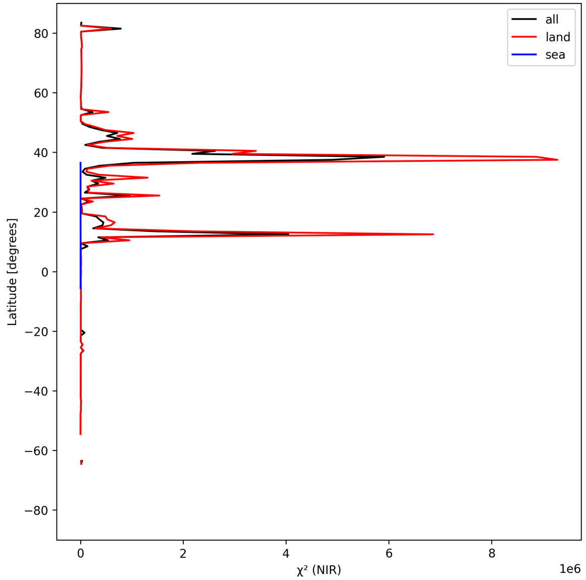
Figure 18: Zonal average of “ \chi^2 (NIR)” for 2025-04-13 to 2025-04-14.
