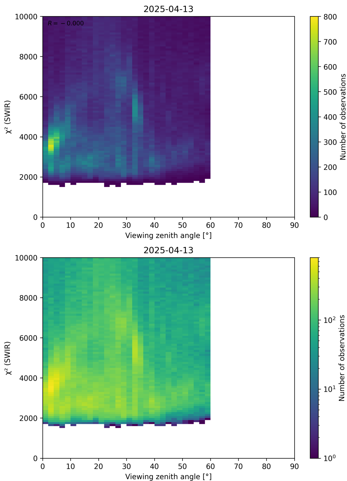
Figure 106: Scatter density plot of “Viewing zenith angle” against “ \chi^2 (SWIR)” for 2025-04-13 to 2025-04-14.
