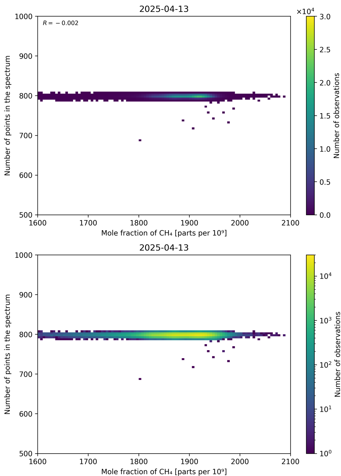
Figure 77: Scatter density plot of “Mole fraction of CH 4 ” against “Number of points in the spectrum” for 2025-04-13 to 2025-04-14.
