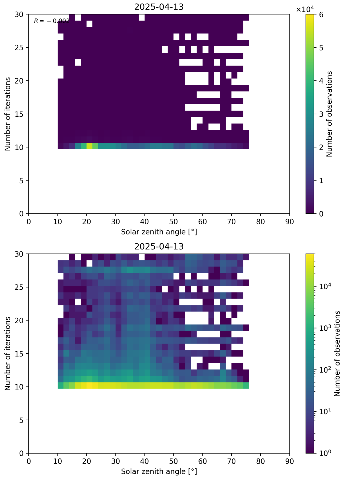
Figure 102: Scatter density plot of “Solar zenith angle” against “Number of iterations” for 2025-04-13 to 2025-04-14.
