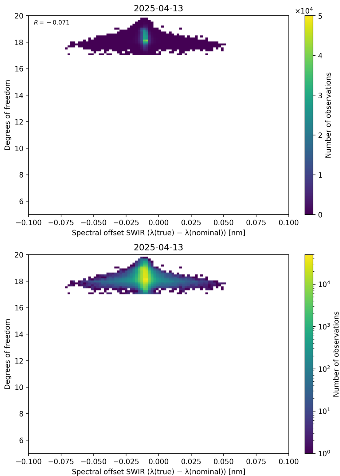
Figure 119: Scatter density plot of “Spectral offset SWIR ( \lambda_{\text{true}} - \lambda_{\text{nominal}} )” against “Degrees of freedom” for 2025-04-13 to 2025-04-14.
