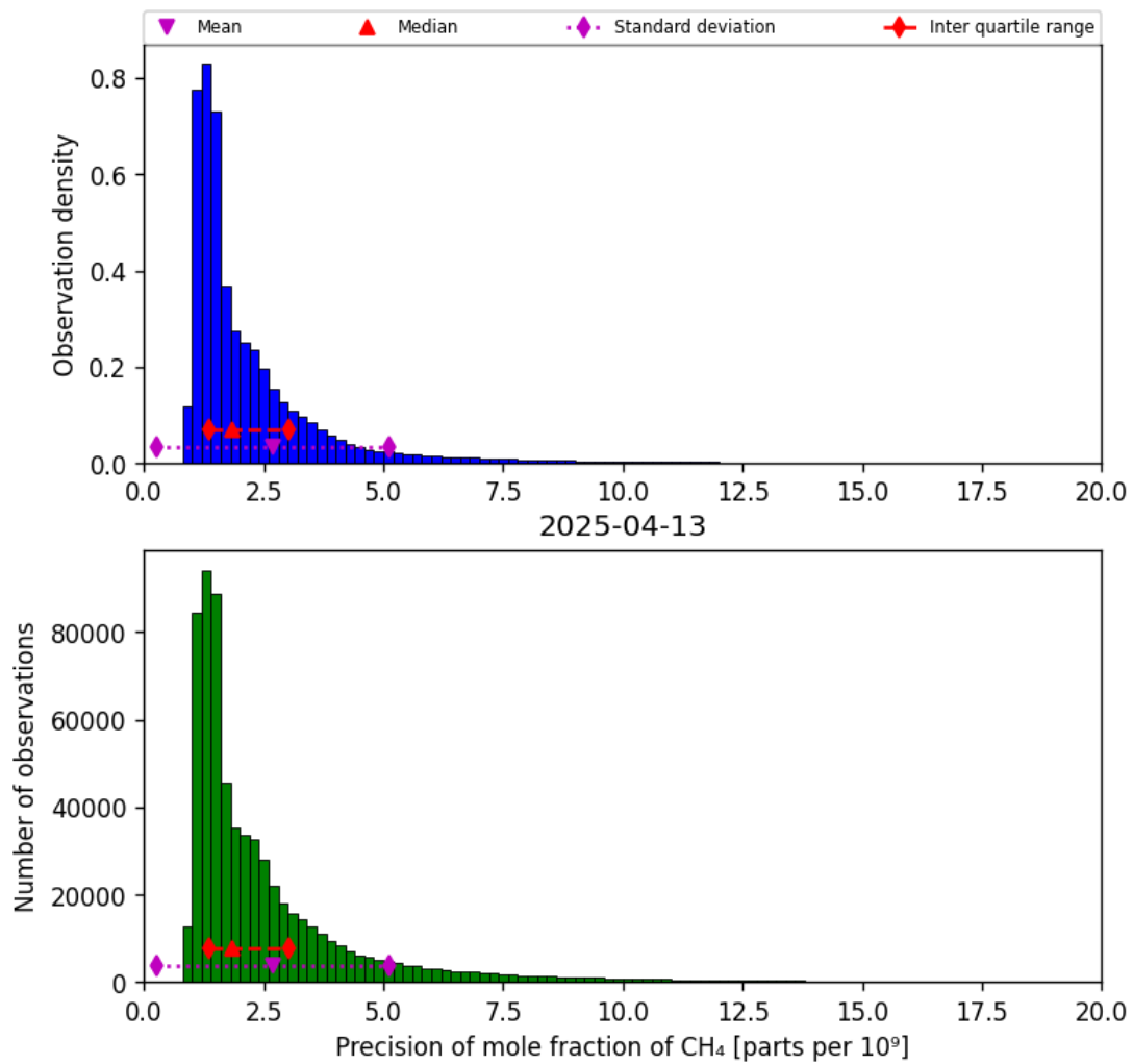
Figure 24: Histogram of “Precision of mole fraction of CH 4 ” for 2025-04-13 to 2025-04-14
