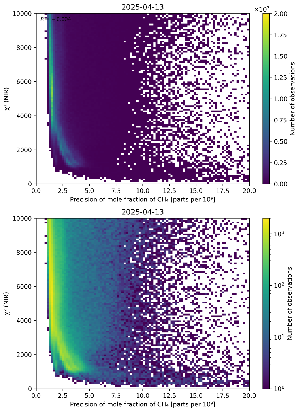
Figure 78: Scatter density plot of “Precision of mole fraction of \text{CH}_4 ” against “ \chi^2 (NIR)” for 2025-04-13 to 2025-04-14.
