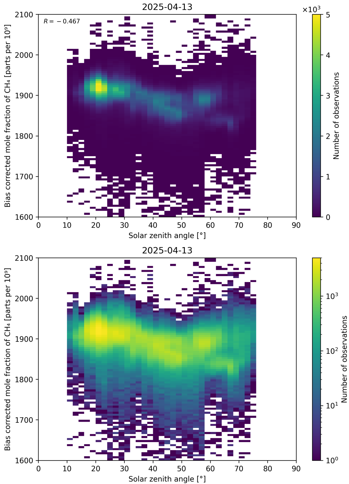
Figure 100: Scatter density plot of “Solar zenith angle” against “Bias corrected mole fraction of \text{CH}_4 ” for 2025-04-13 to 2025-04-14.
