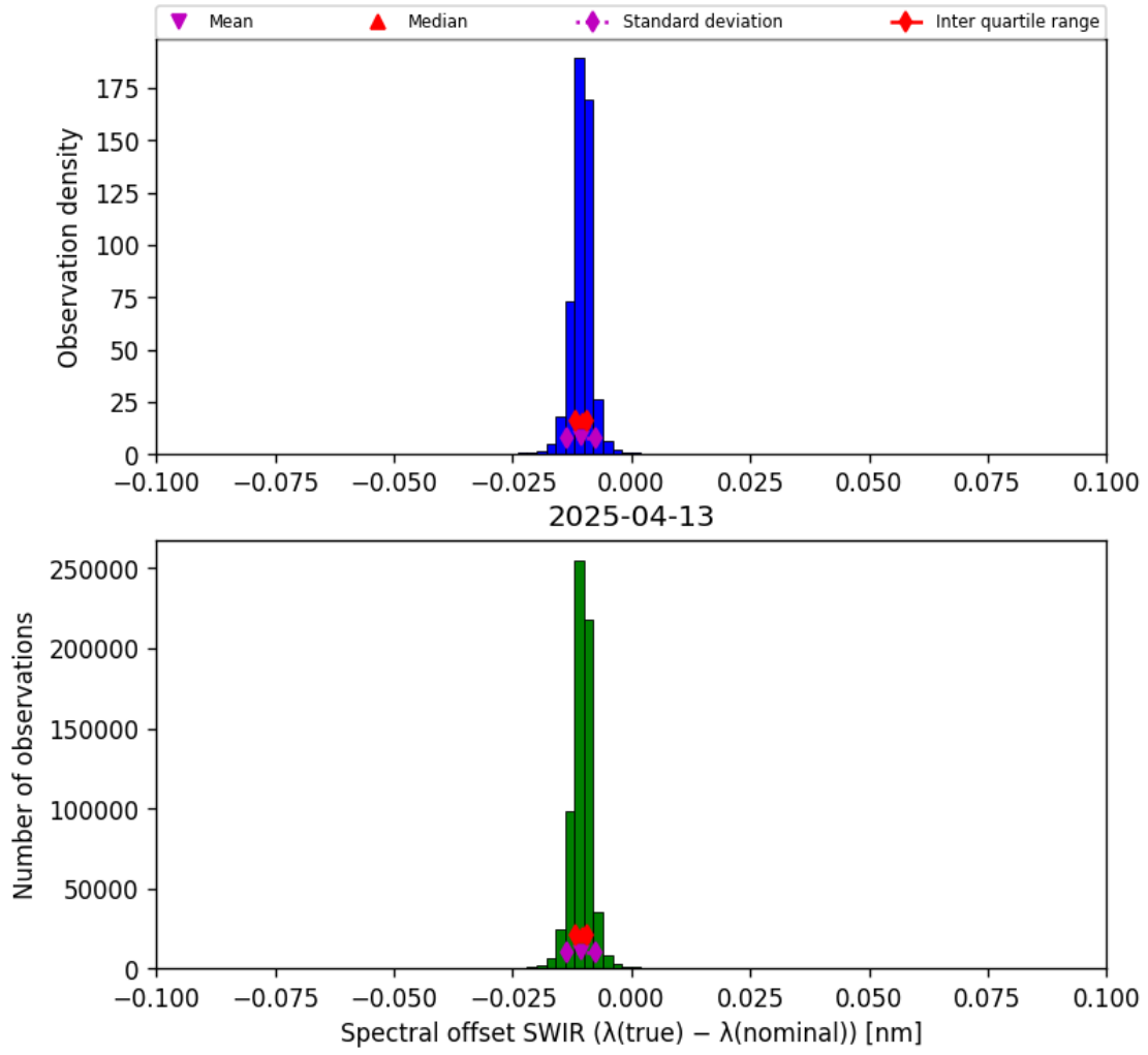
Figure 27: Histogram of “Spectral offset SWIR ( \lambda_{\text{true}} - \lambda_{\text{nominal}} )” for 2025-04-13 to 2025-04-14
