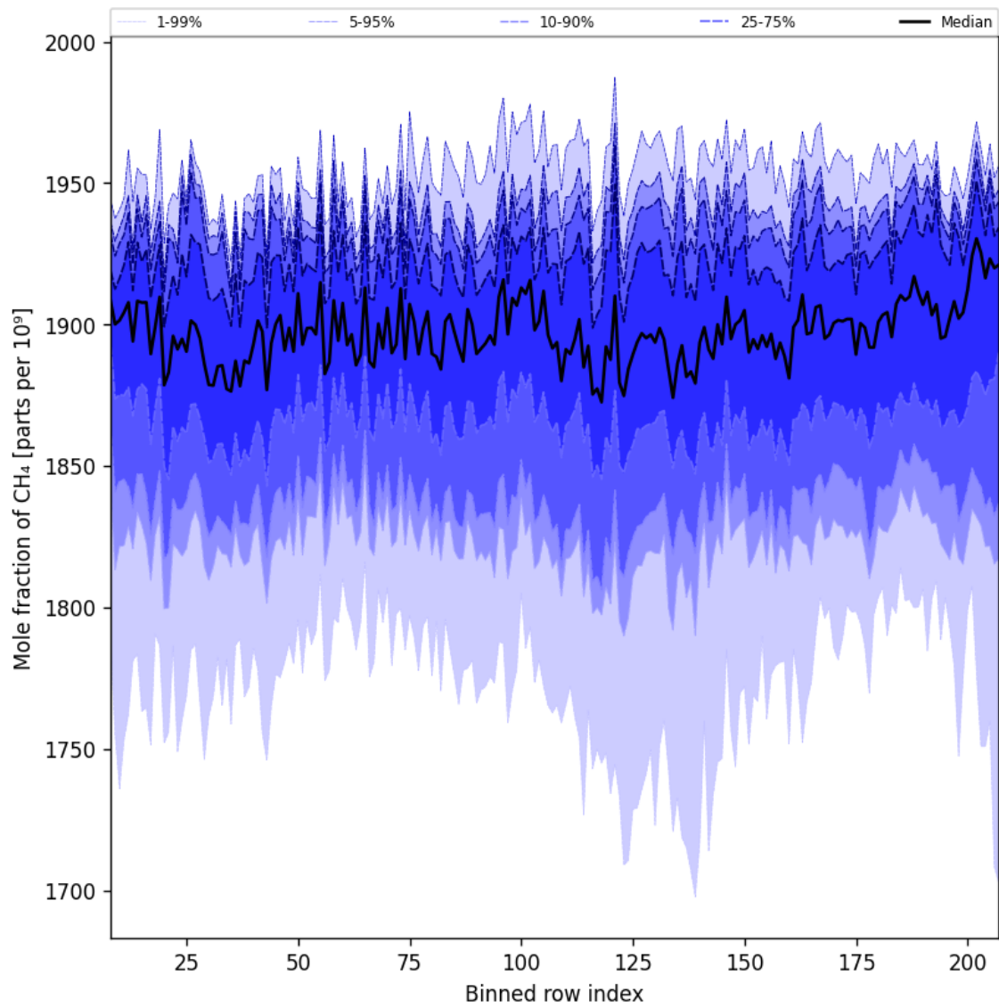
Figure 34: Along track statistics of “Mole fraction of CH 4 ” for 2025-04-13 to 2025-04-14
