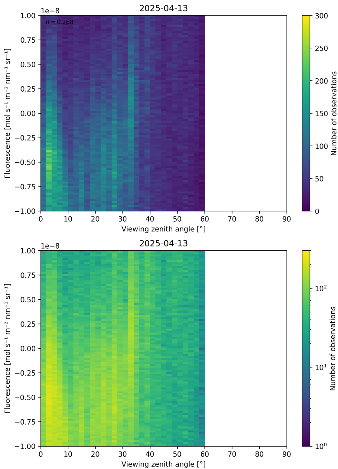
Figure 108: Scatter density plot of “Viewing zenith angle” against “Fluorescence” for 2025-04-13 to 2025-04-14.
