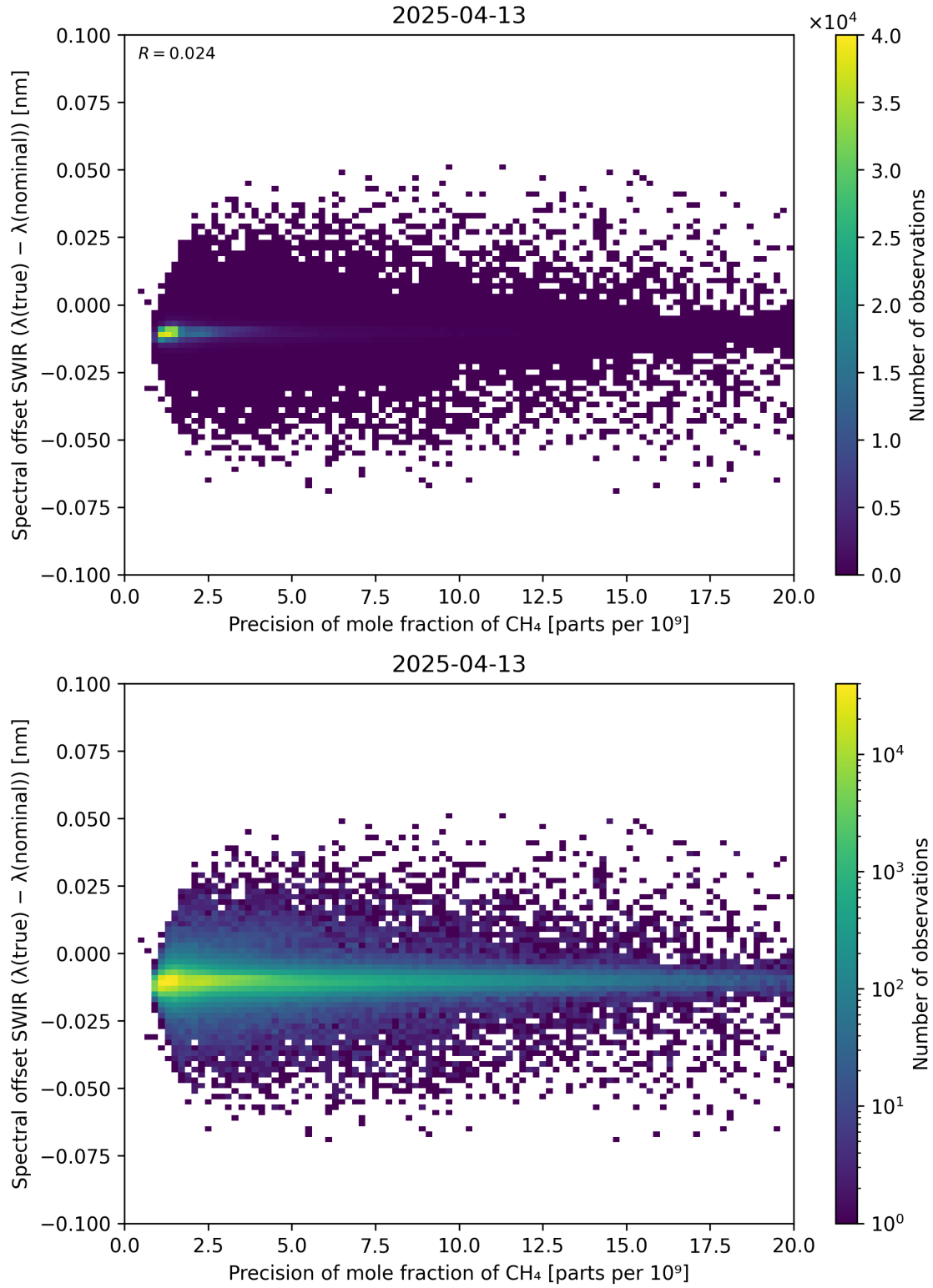
Figure 85: Scatter density plot of “Precision of mole fraction of CH 4 ” against “Spectral offset SWIR ( \lambda_{\text{true}} - \lambda_{\text{nominal}} )” for 2025-04-13 to 2025-04-14.
