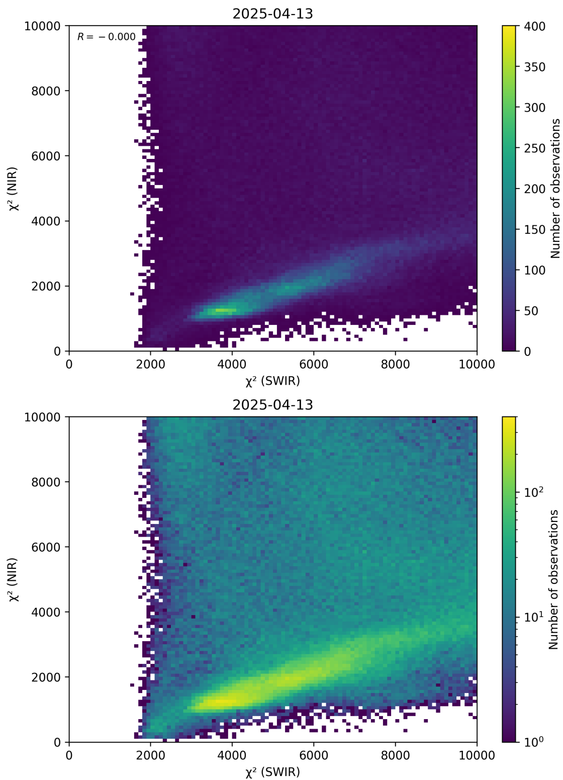
Figure 47: Scatter density plot of “ \chi^2 (SWIR)” against “ \chi^2 (NIR)” for 2025-04-13 to 2025-04-14.
