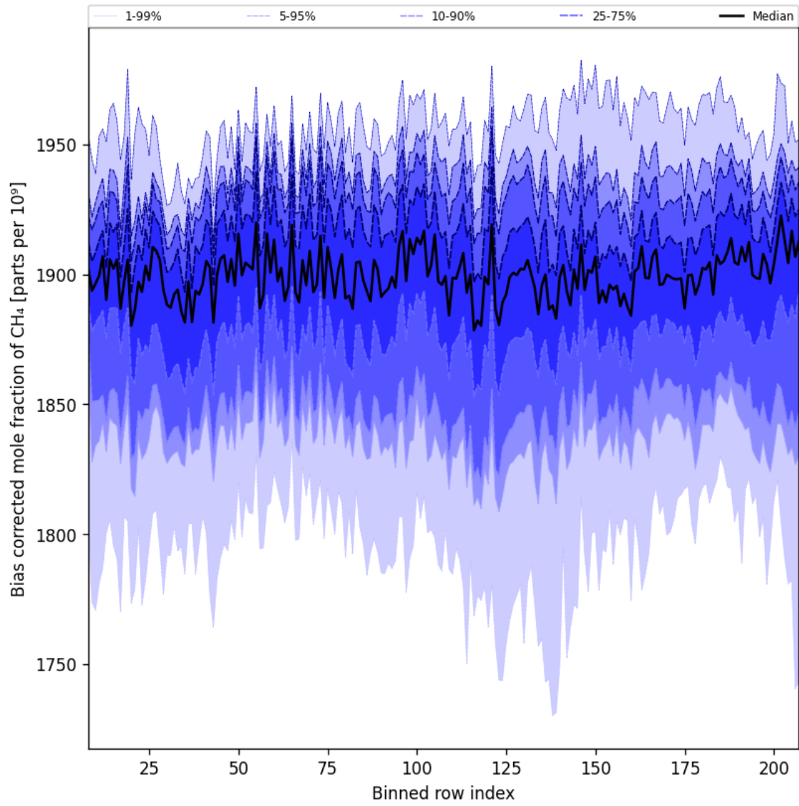
Figure 36: Along track statistics of “Bias corrected mole fraction of CH 4 ” for 2025-04-13 to 2025-04-14
