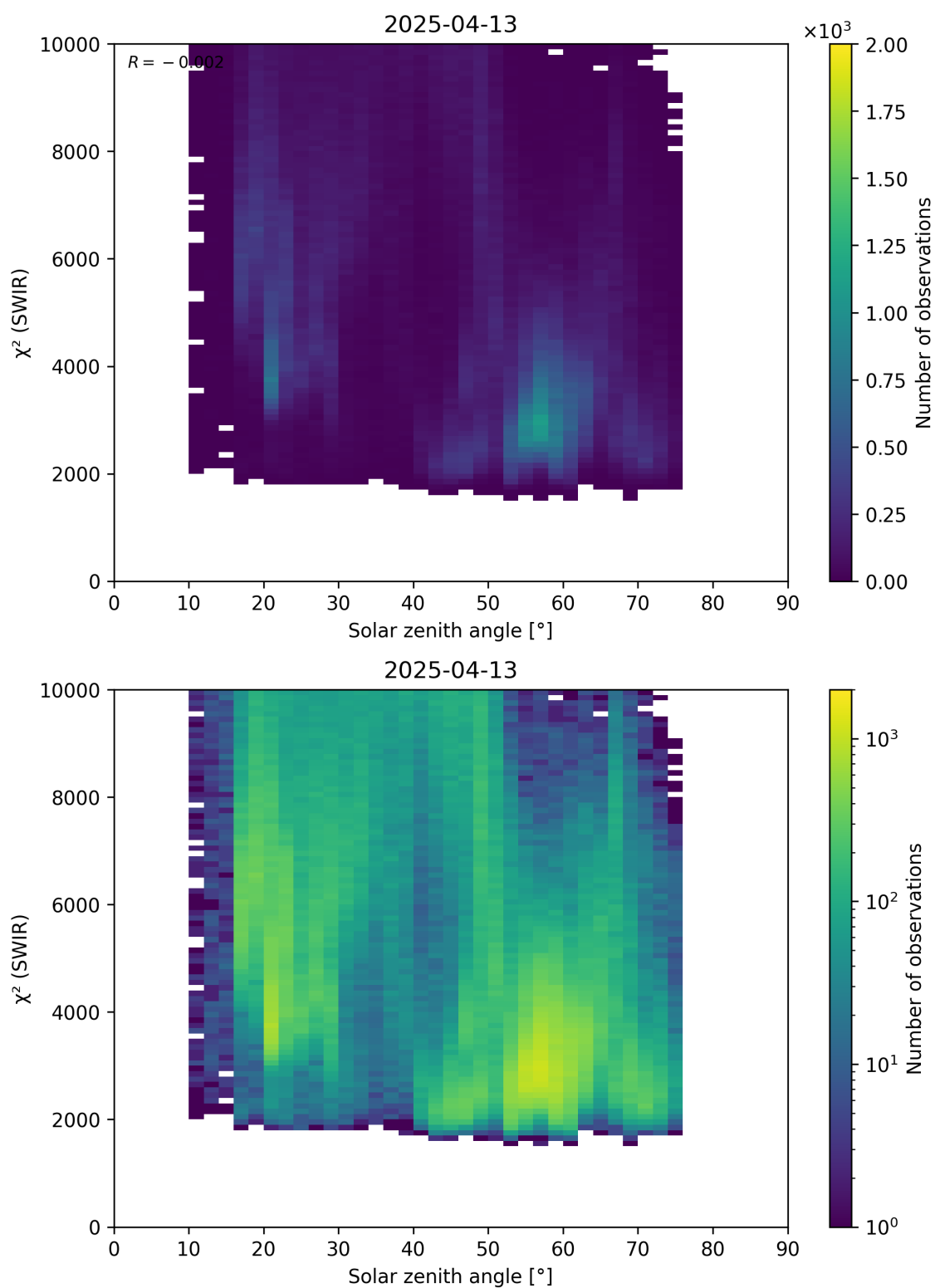
Figure 95: Scatter density plot of “Solar zenith angle” against “ \chi^2 (SWIR)” for 2025-04-13 to 2025-04-14.
