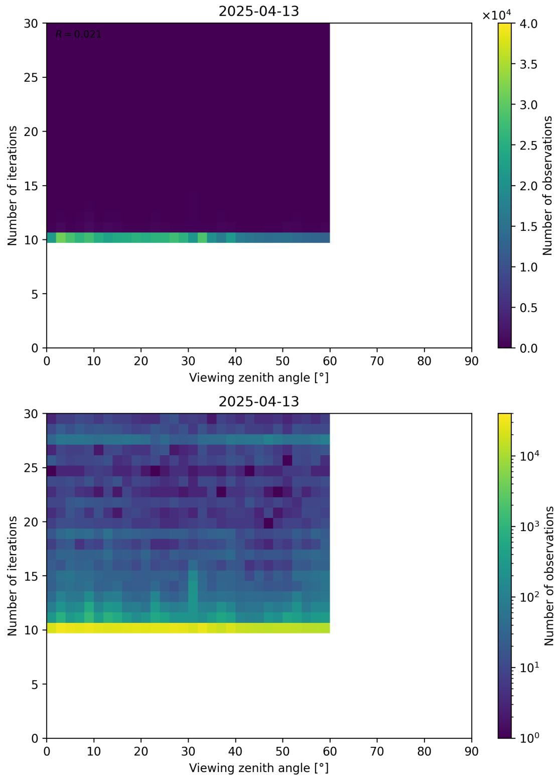
Figure 113: Scatter density plot of “Viewing zenith angle” against “Number of iterations” for 2025-04-13 to 2025-04-14.
