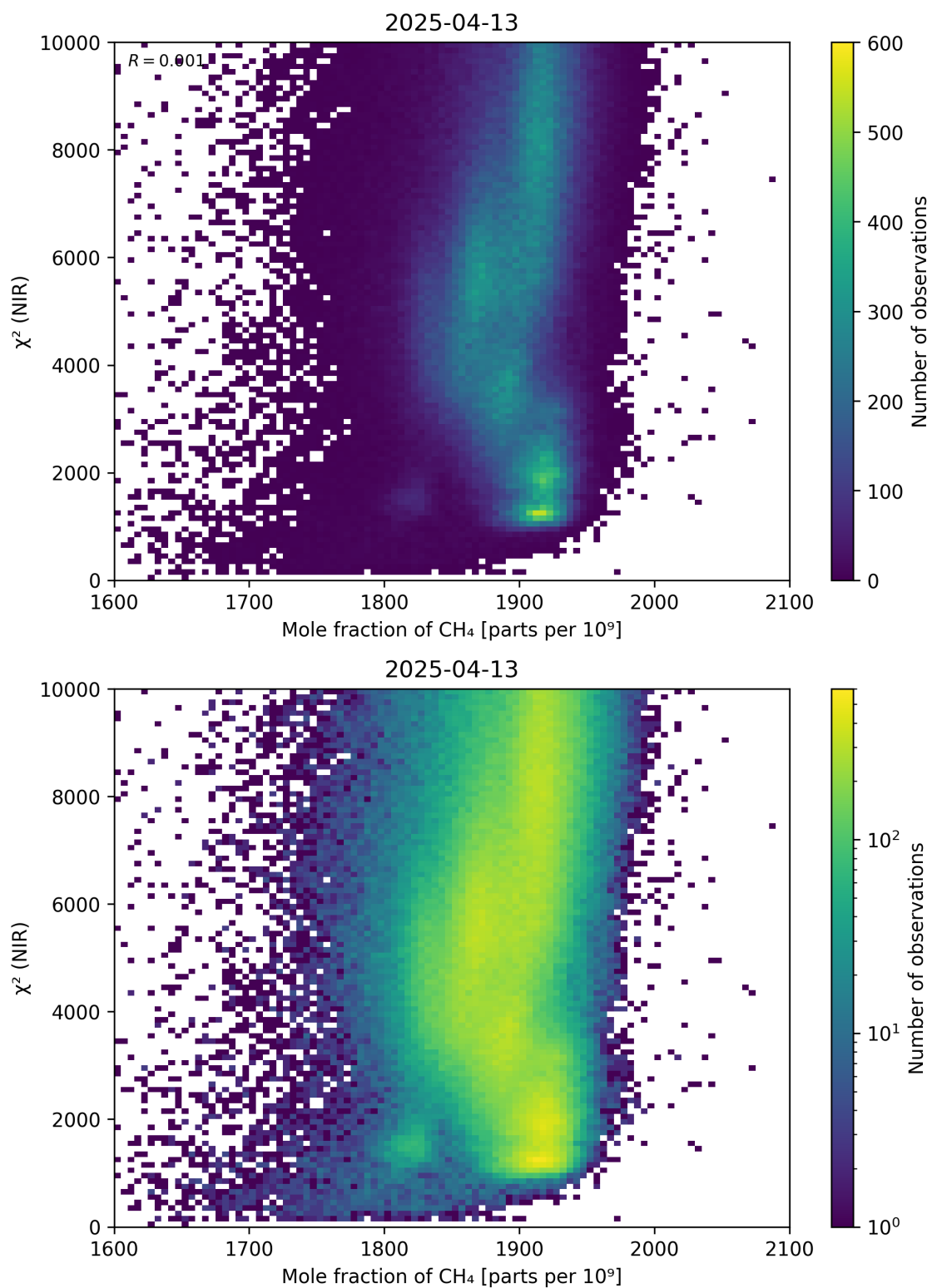
Figure 70: Scatter density plot of “Mole fraction of CH 4 ” against “ \chi^2 (NIR)” for 2025-04-13 to 2025-04-14.
