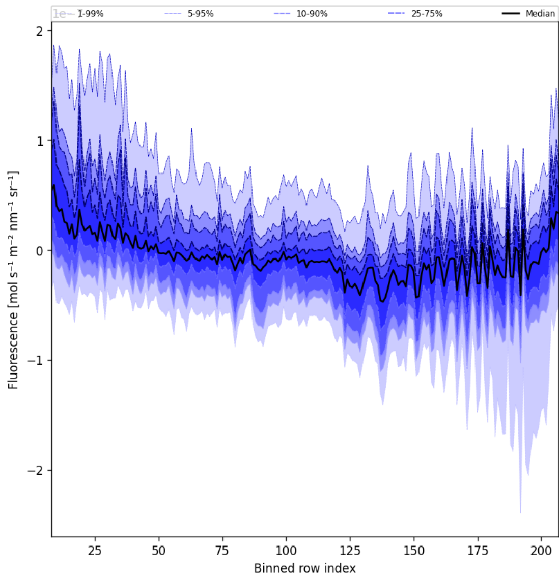
Figure 43: Along track statistics of “Fluorescence” for 2025-04-13 to 2025-04-14
