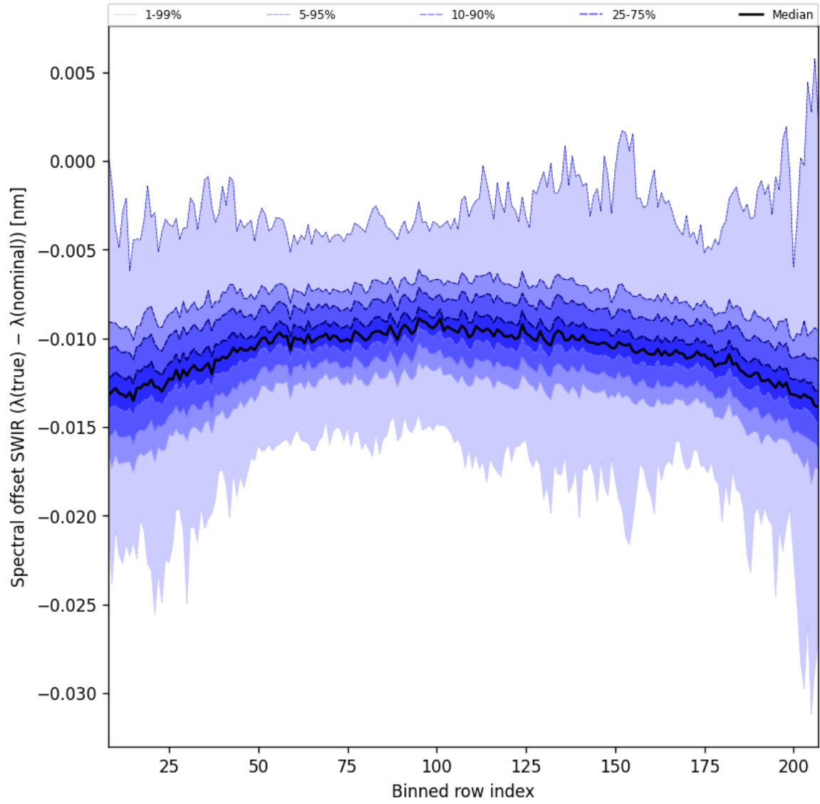
Figure 38: Along track statistics of “Spectral offset SWIR ( \lambda_{\text{true}} - \lambda_{\text{nominal}} )” for 2025-04-13 to 2025-04-14
