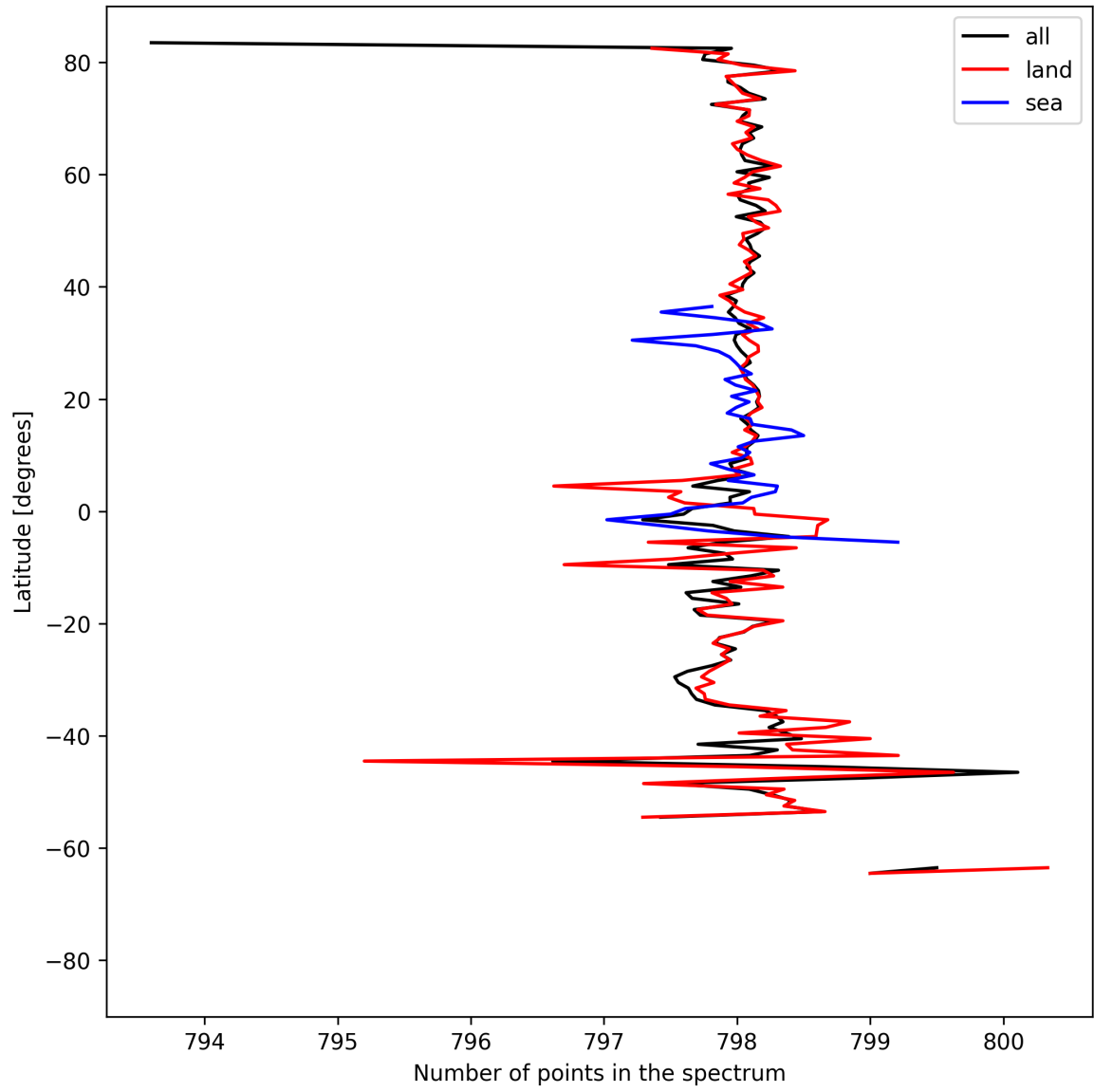
Figure 15: Zonal average of “Number of points in the spectrum” for 2025-04-13 to 2025-04-14.
