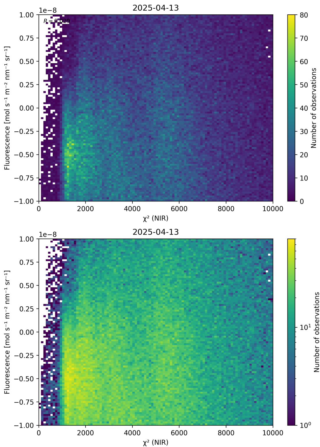
Figure 45: Scatter density plot of “ \chi^2 (NIR)” against “Fluorescence” for 2025-04-13 to 2025-04-14.
