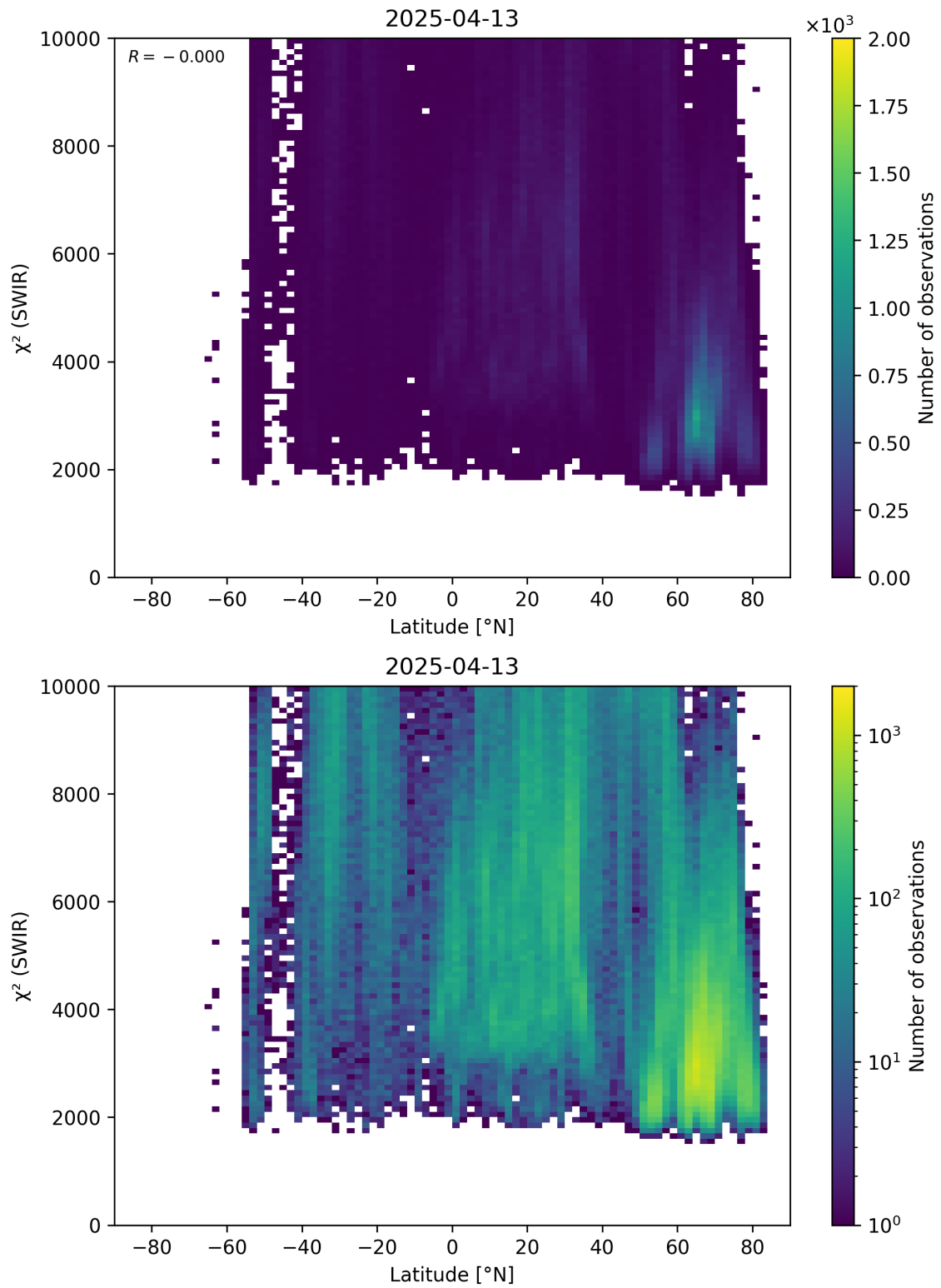
Figure 54: Scatter density plot of “Latitude” against “ \chi^2 (SWIR)” for 2025-04-13 to 2025-04-14.
