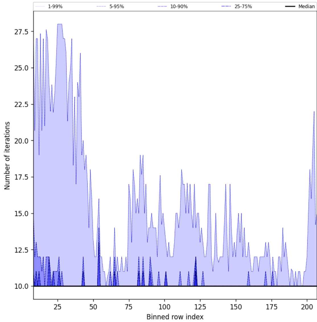
Figure 42: Along track statistics of “Number of iterations” for 2025-04-13 to 2025-04-14
