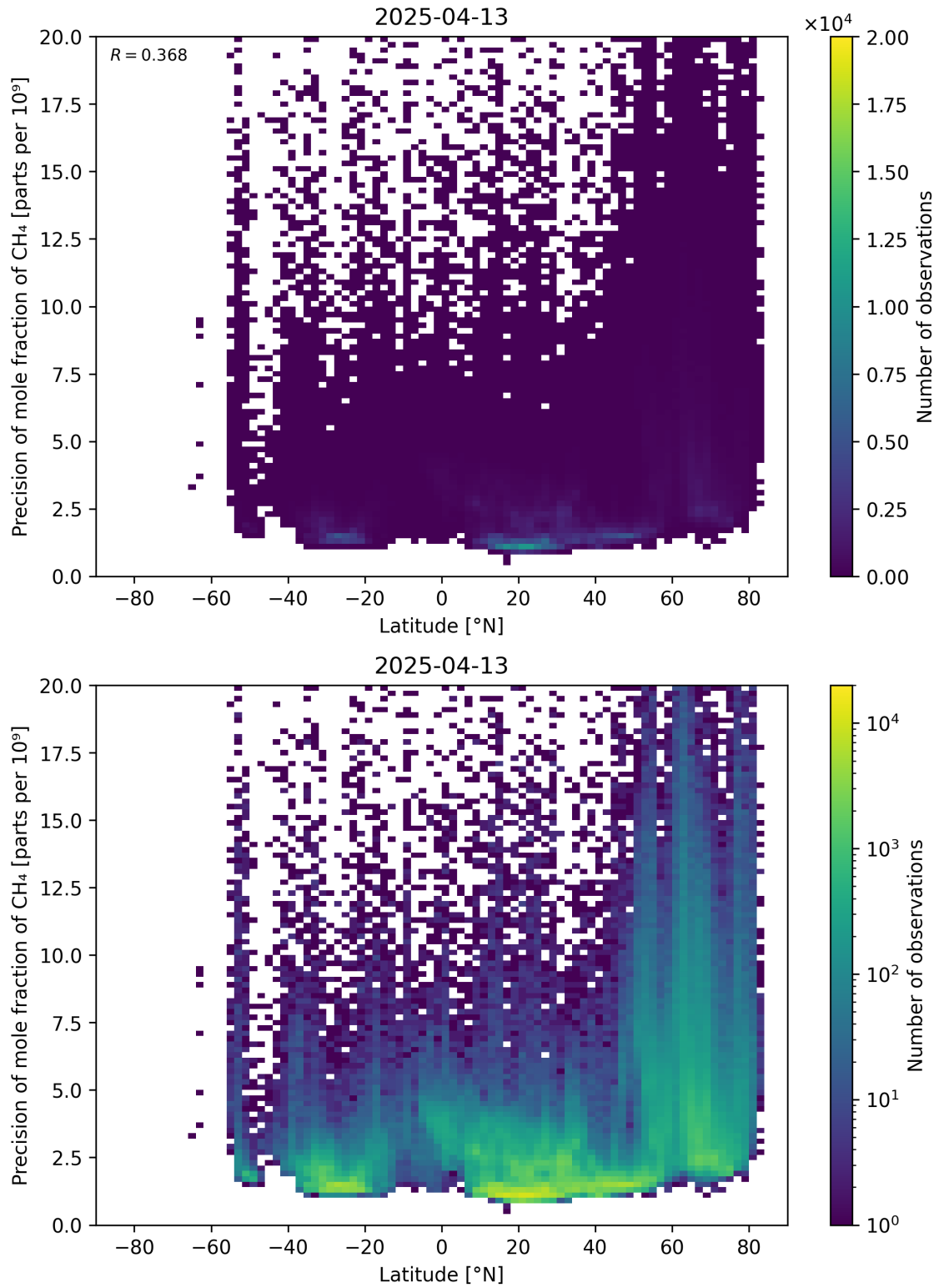
Figure 59: Scatter density plot of “Latitude” against “Precision of mole fraction of \text{CH}_4 ” for 2025-04-13 to 2025-04-14.
