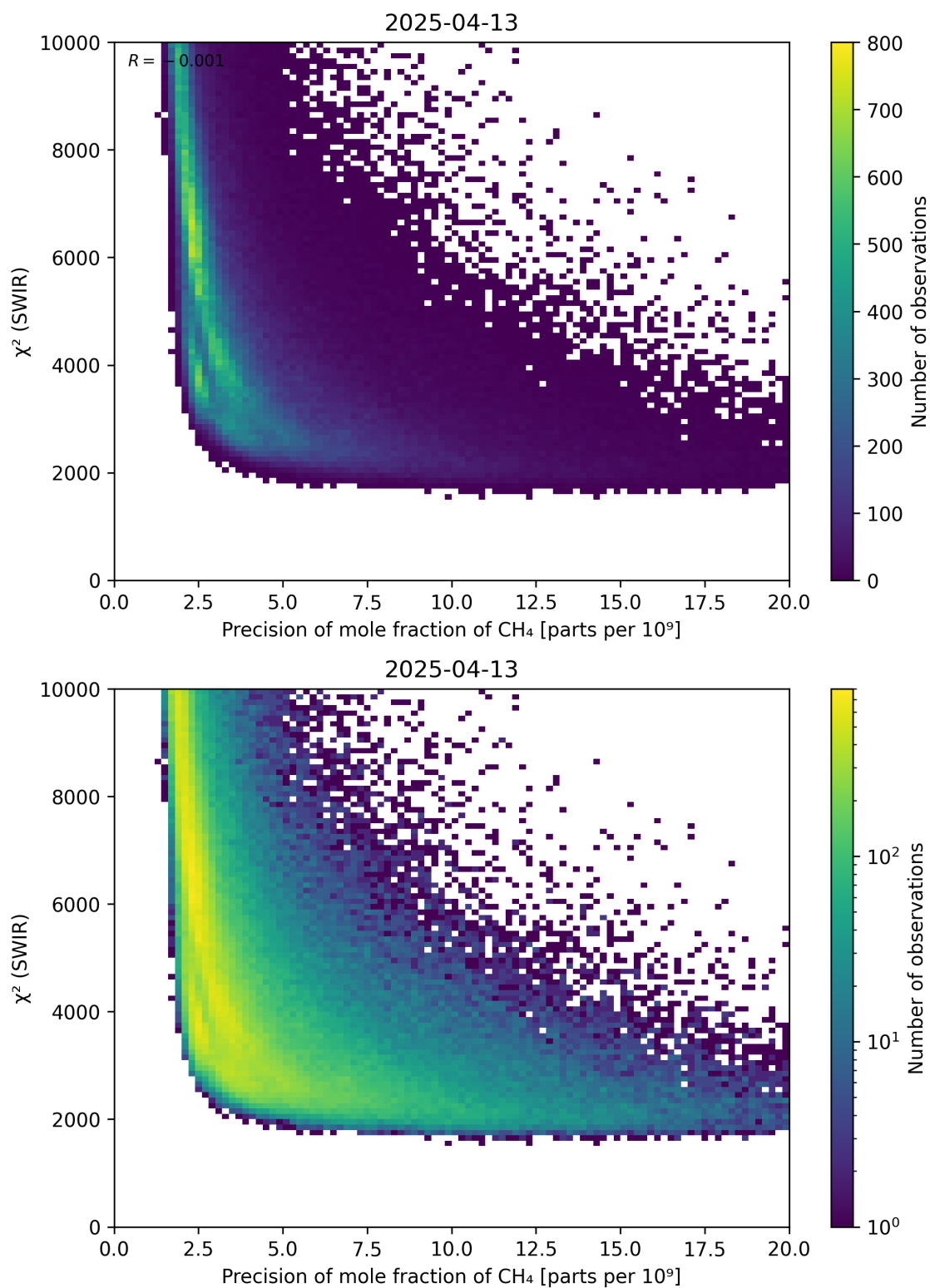
Figure 79: Scatter density plot of “Precision of mole fraction of \text{CH}_4 ” against “ \chi^2 (SWIR)” for 2025-04-13 to 2025-04-14.
