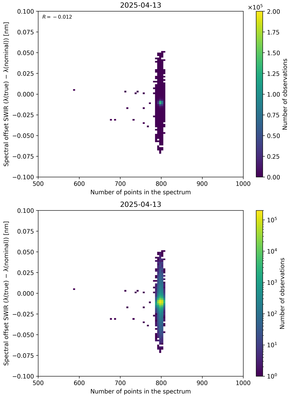
Figure 93: Scatter density plot of “Number of points in the spectrum” against “Spectral offset SWIR ( \lambda_{\text{true}} - \lambda_{\text{nominal}} )” for 2025-04-13 to 2025-04-14.
