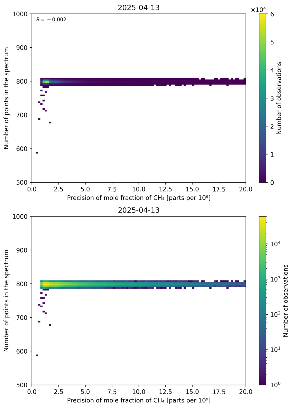
Figure 84: Scatter density plot of “Precision of mole fraction of CH 4 ” against “Number of points in the spectrum” for 2025-04-13 to 2025-04-14.
