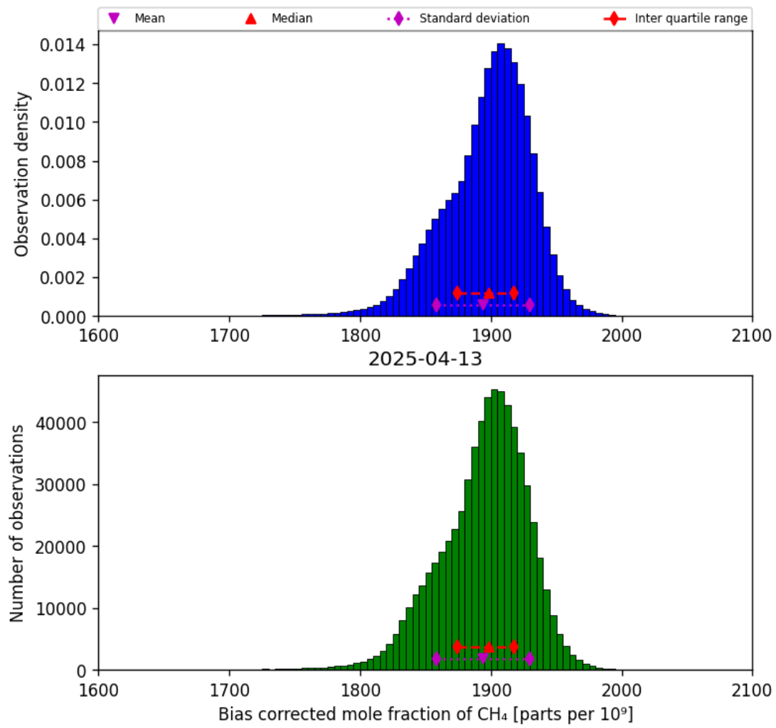
Figure 25: Histogram of “Bias corrected mole fraction of CH 4 ” for 2025-04-13 to 2025-04-14
