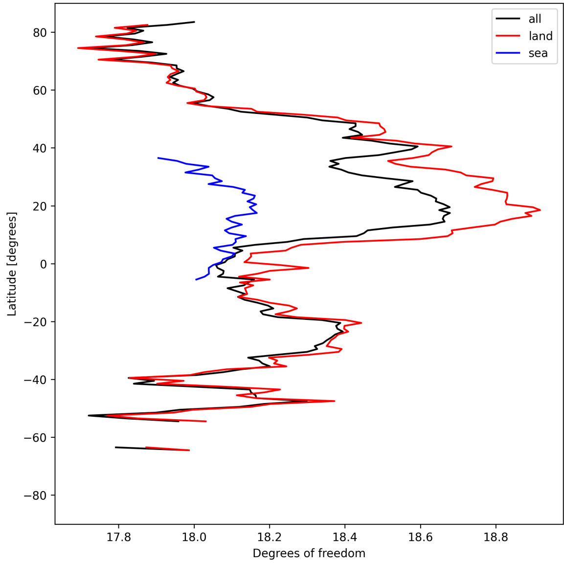
Figure 19: Zonal average of “Degrees of freedom” for 2025-04-13 to 2025-04-14.
