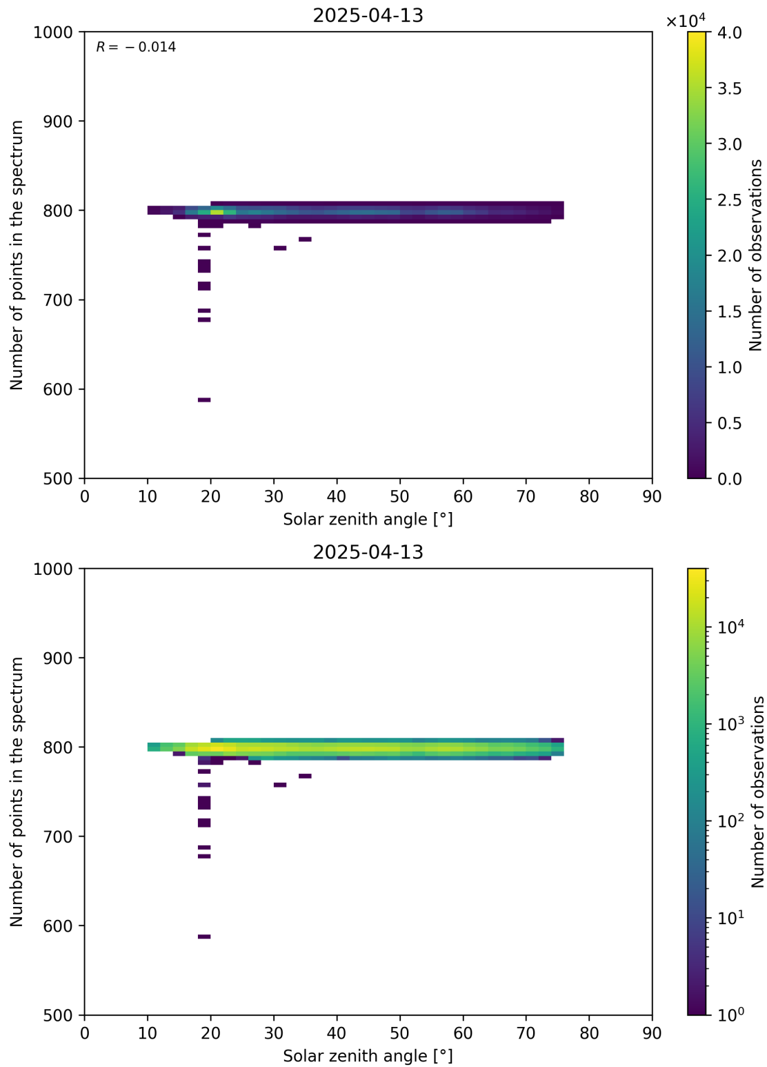
Figure 103: Scatter density plot of “Solar zenith angle” against “Number of points in the spectrum” for 2025-04-13 to 2025-04-14.
