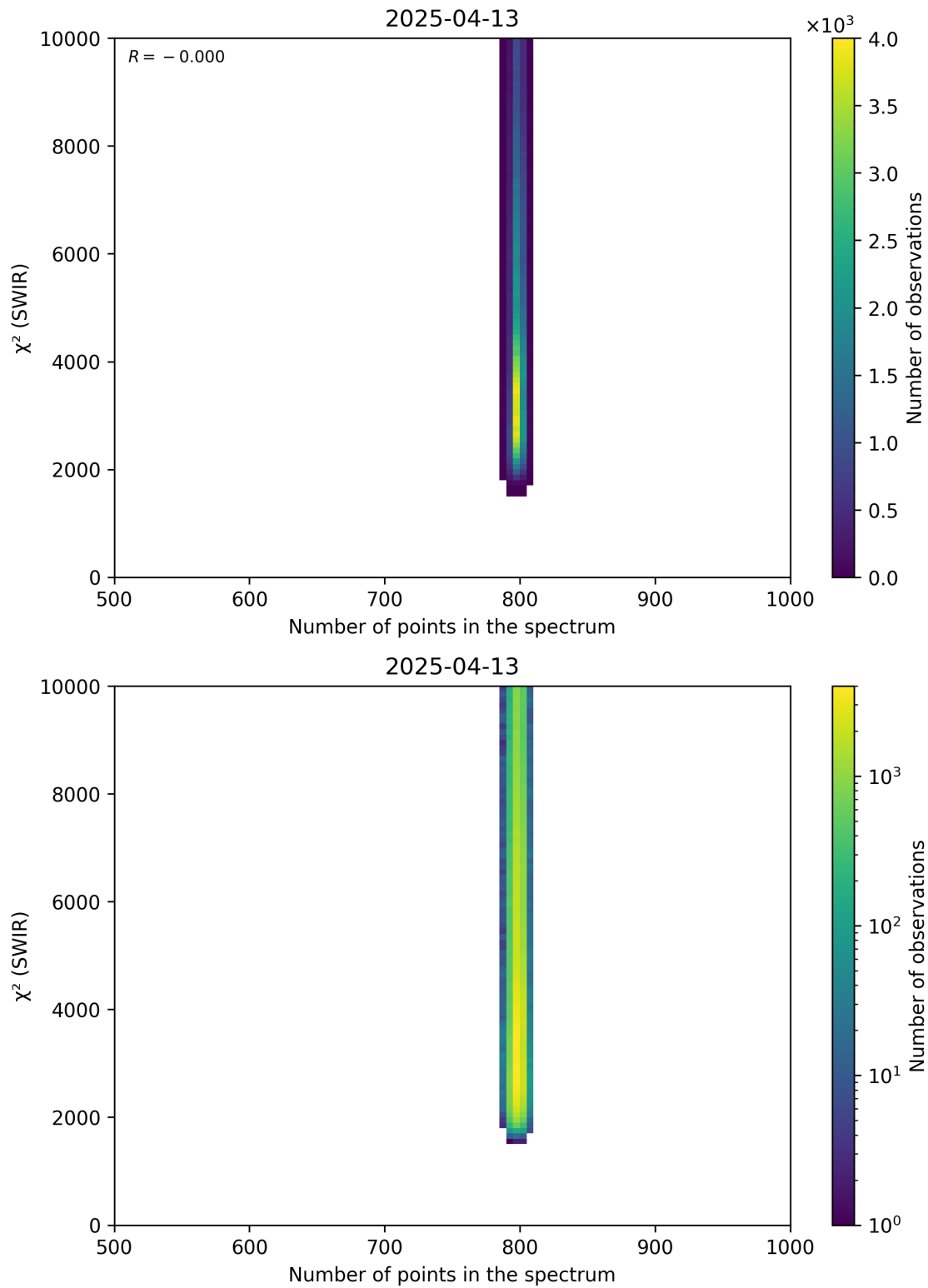
Figure 89: Scatter density plot of “Number of points in the spectrum” against “ \chi^2 (SWIR)” for 2025-04-13 to 2025-04-14.
