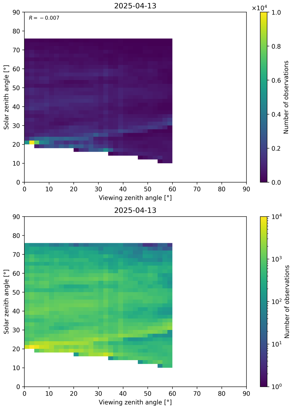
Figure 115: Scatter density plot of “Viewing zenith angle” against “Solar zenith angle” for 2025-04-13 to 2025-04-14.
