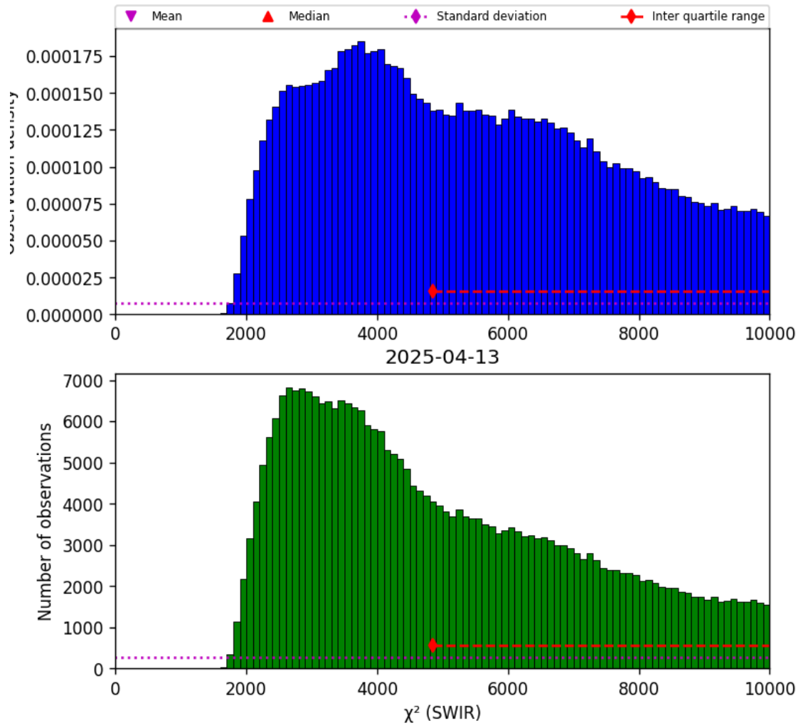
Figure 28: Histogram of “ \chi^2 (SWIR)” for 2025-04-13 to 2025-04-14
