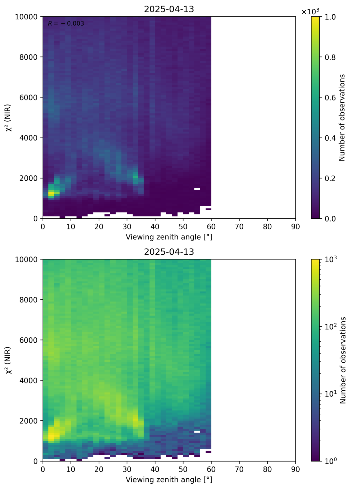
Figure 105: Scatter density plot of “Viewing zenith angle” against “ \chi^2 (NIR)” for 2025-04-13 to 2025-04-14.
