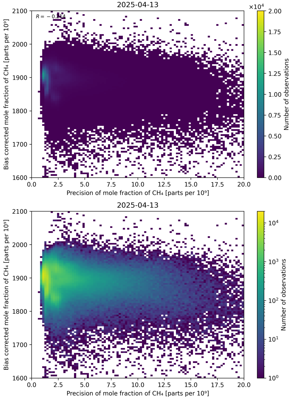
Figure 82: Scatter density plot of “Precision of mole fraction of CH 4 ” against “Bias corrected mole fraction of CH 4 ” for 2025-04-13 to 2025-04-14.
