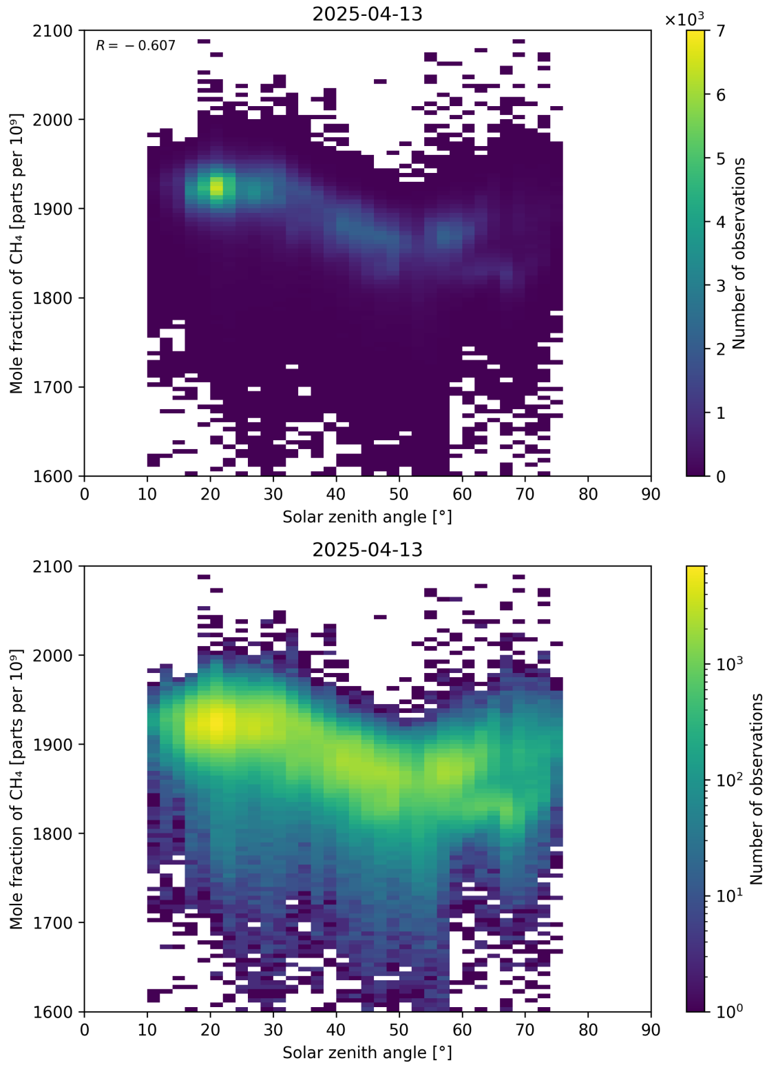
Figure 99: Scatter density plot of “Solar zenith angle” against “Mole fraction of CH 4 ” for 2025-04-13 to 2025-04-14.
