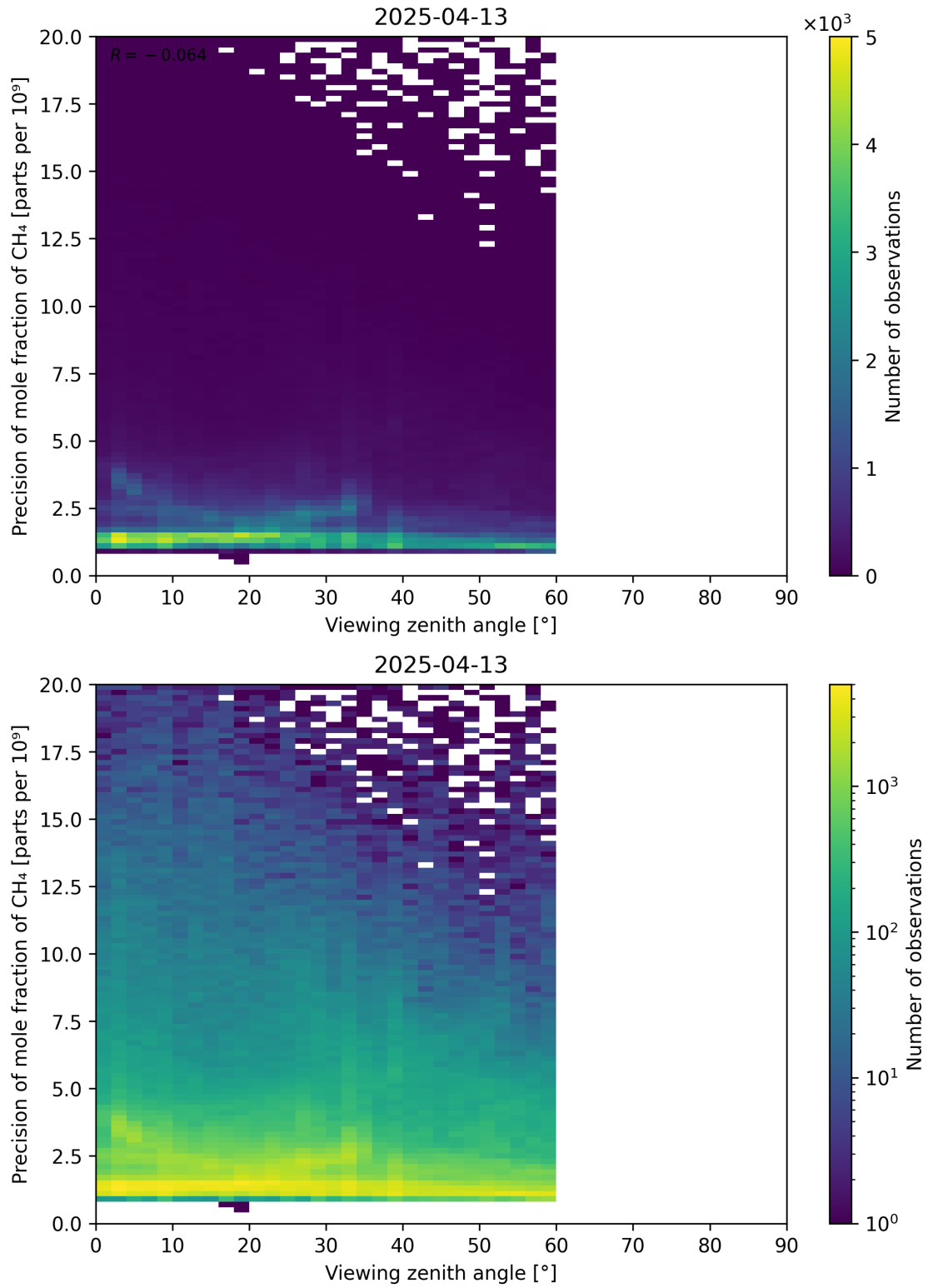
Figure 112: Scatter density plot of “Viewing zenith angle” against “Precision of mole fraction of CH 4 ” for 2025-04-13 to 2025-04-14.
