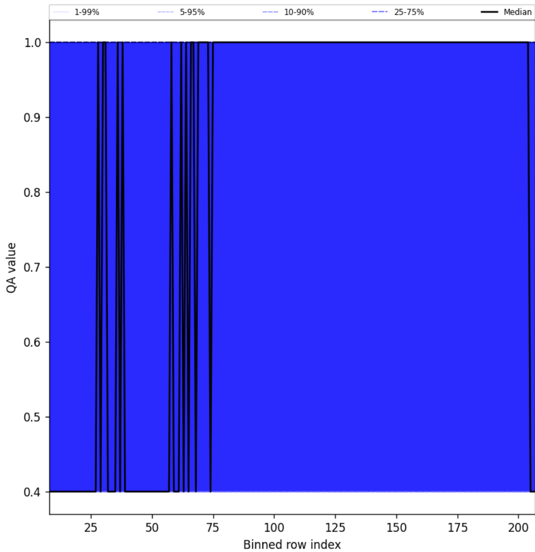
Figure 33: Along track statistics of “QA value” for 2025-04-13 to 2025-04-14
