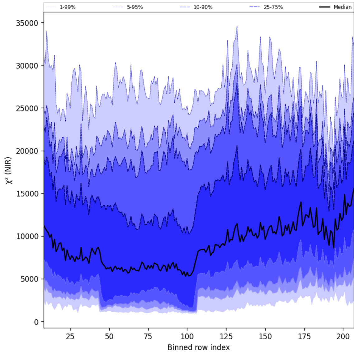
Figure 40: Along track statistics of “ \chi^2 (NIR)” for 2025-04-13 to 2025-04-14
