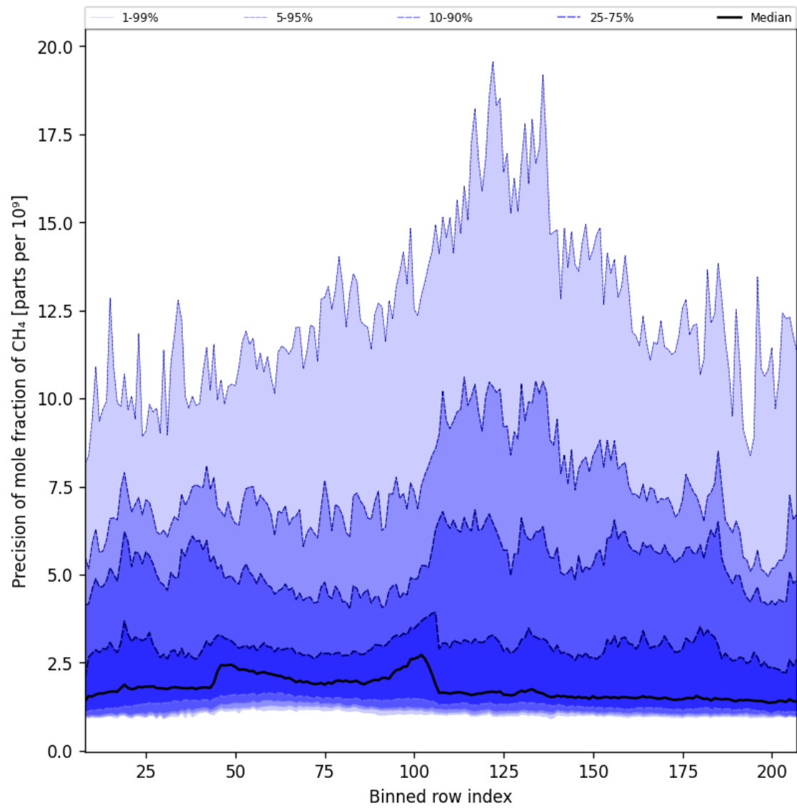
Figure 35: Along track statistics of “Precision of mole fraction of CH 4 ” for 2025-04-13 to 2025-04-14
