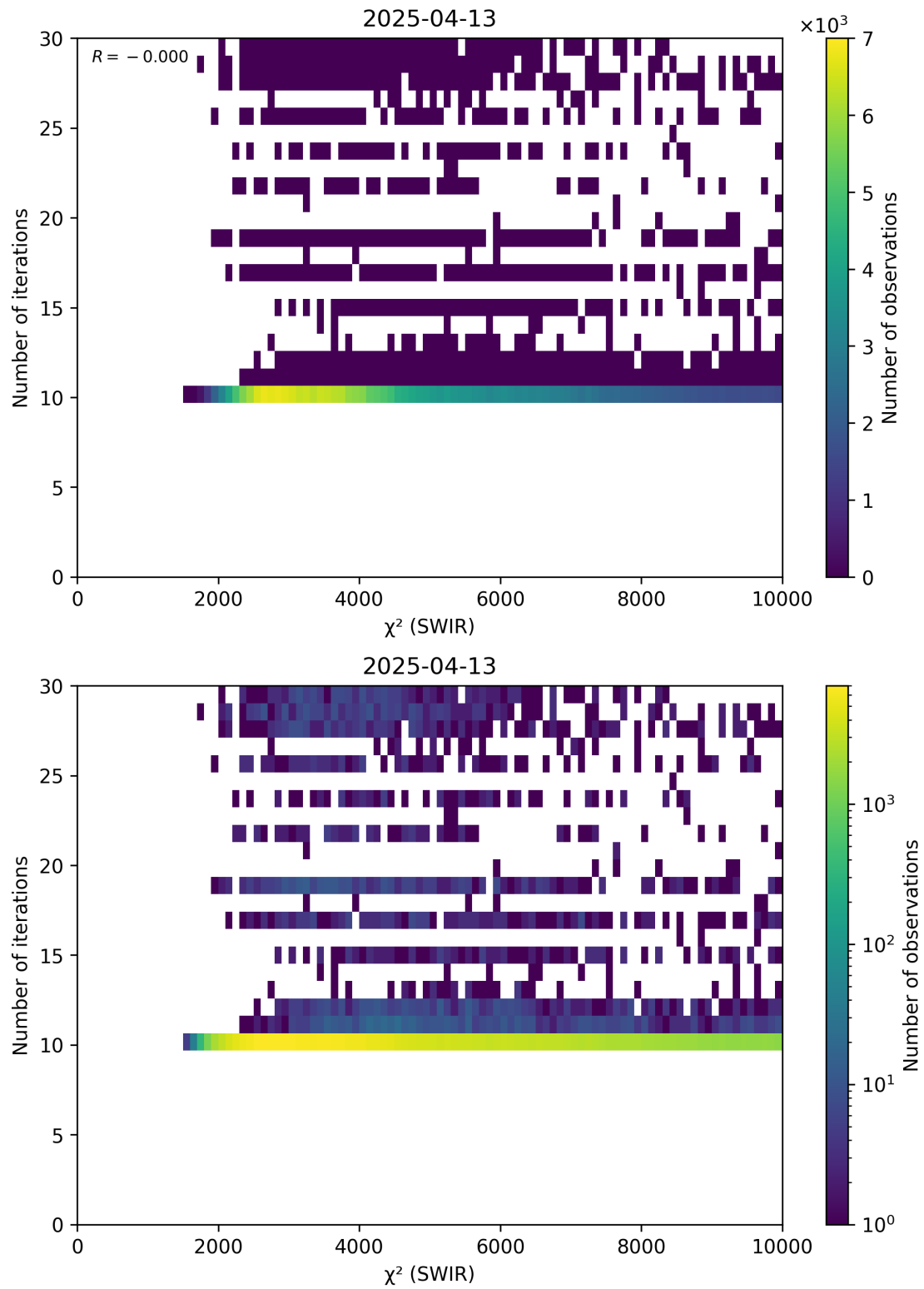
Figure 50: Scatter density plot of “ \chi^2 (SWIR)” against “Number of iterations” for 2025-04-13 to 2025-04-14.
