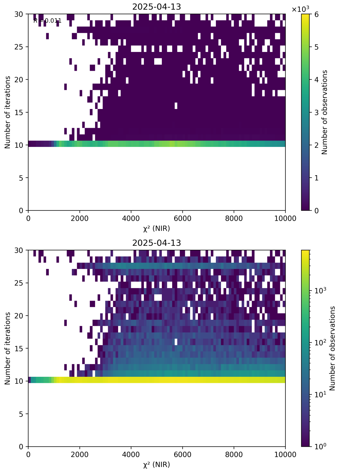
Figure 46: Scatter density plot of “ \chi^2 (NIR)” against “Number of iterations” for 2025-04-13 to 2025-04-14.
