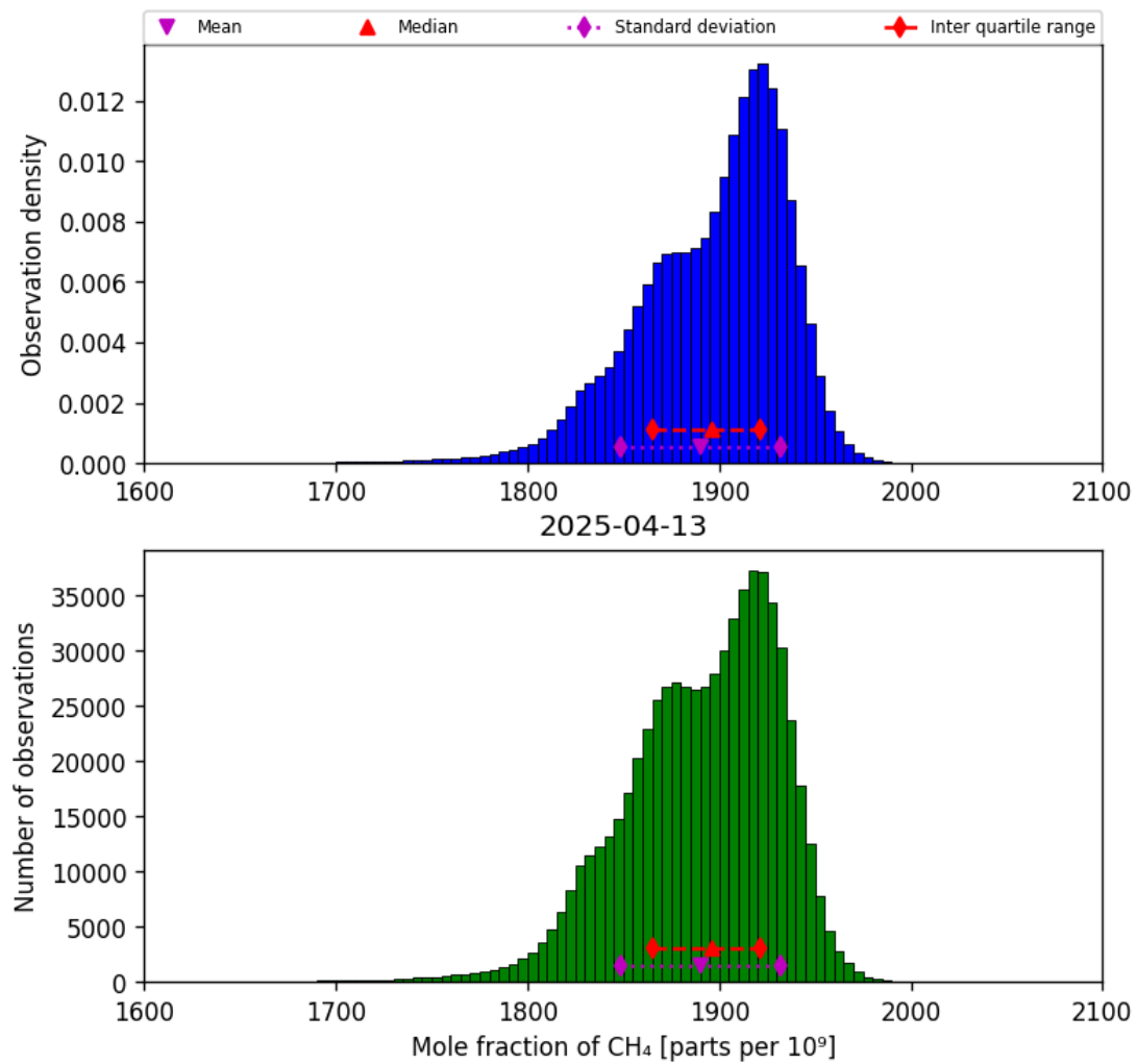
Figure 23: Histogram of “Mole fraction of CH 4 ” for 2025-04-13 to 2025-04-14
