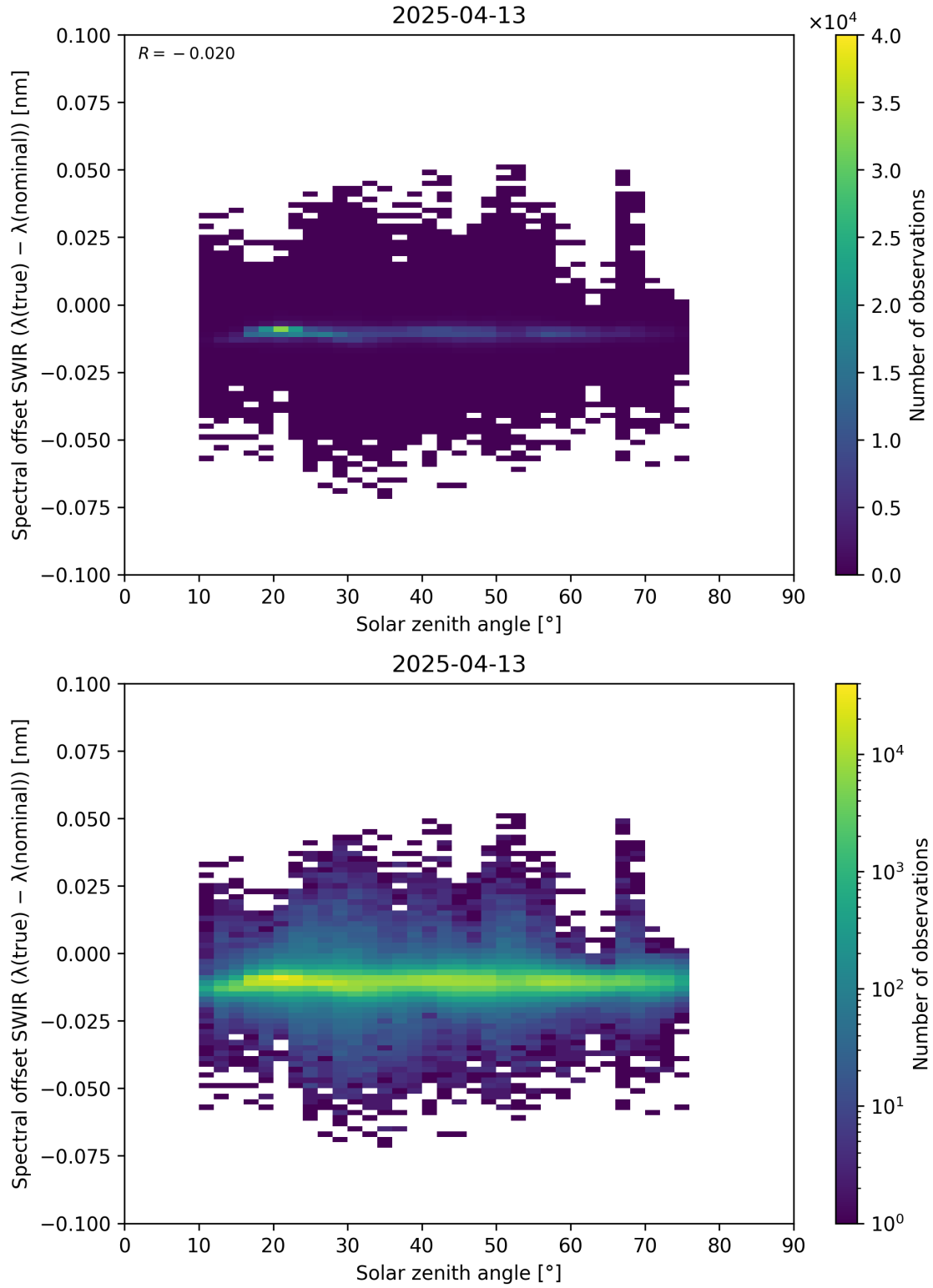
Figure 104: Scatter density plot of “Solar zenith angle” against “Spectral offset SWIR ( \lambda_{\text{true}} - \lambda_{\text{nominal}} )” for 2025-04-13 to 2025-04-14.
