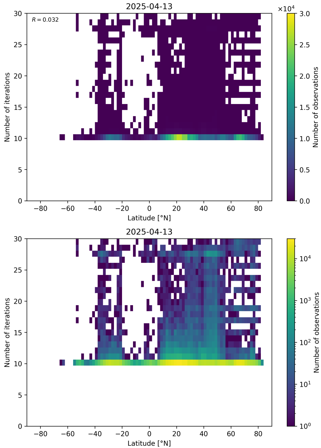
Figure 60: Scatter density plot of “Latitude” against “Number of iterations” for 2025-04-13 to 2025-04-14.
