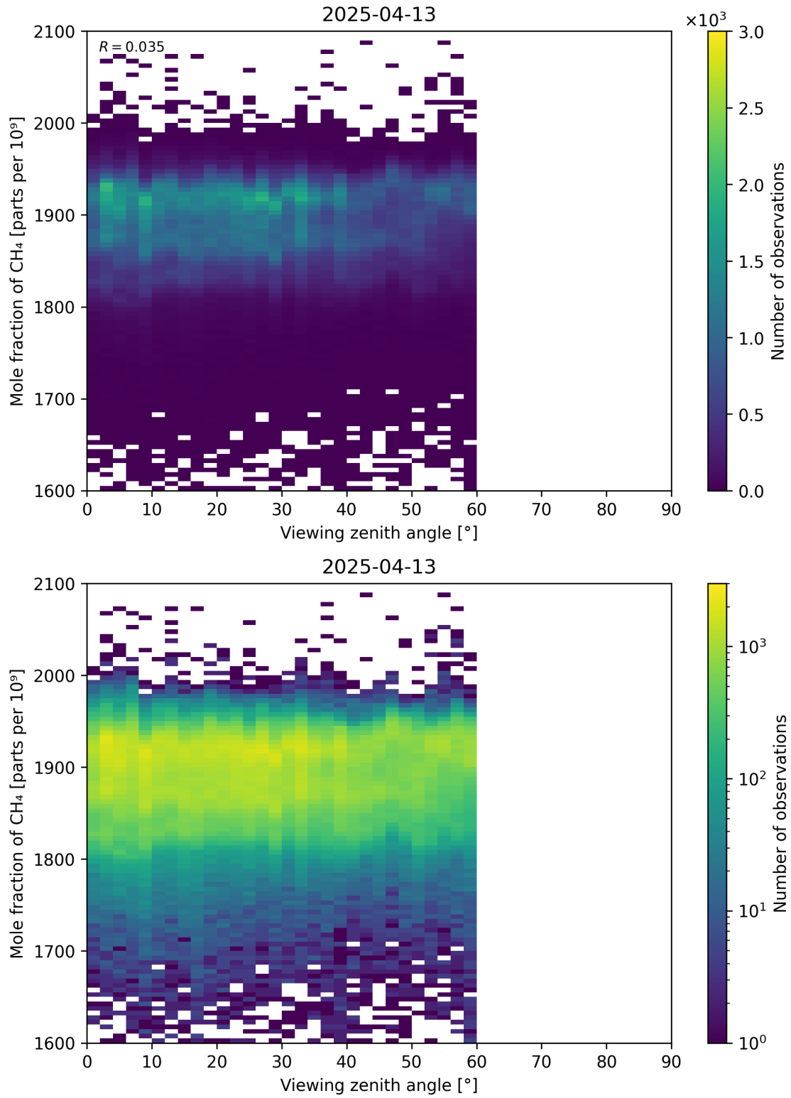
Figure 110: Scatter density plot of “Viewing zenith angle” against “Mole fraction of CH 4 ” for 2025-04-13 to 2025-04-14.
