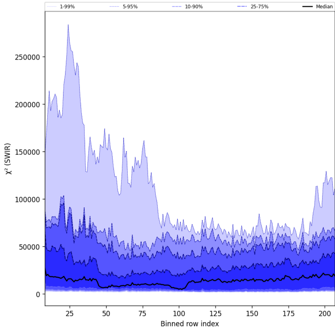
Figure 39: Along track statistics of “ \chi^2 (SWIR)” for 2025-04-13 to 2025-04-14
