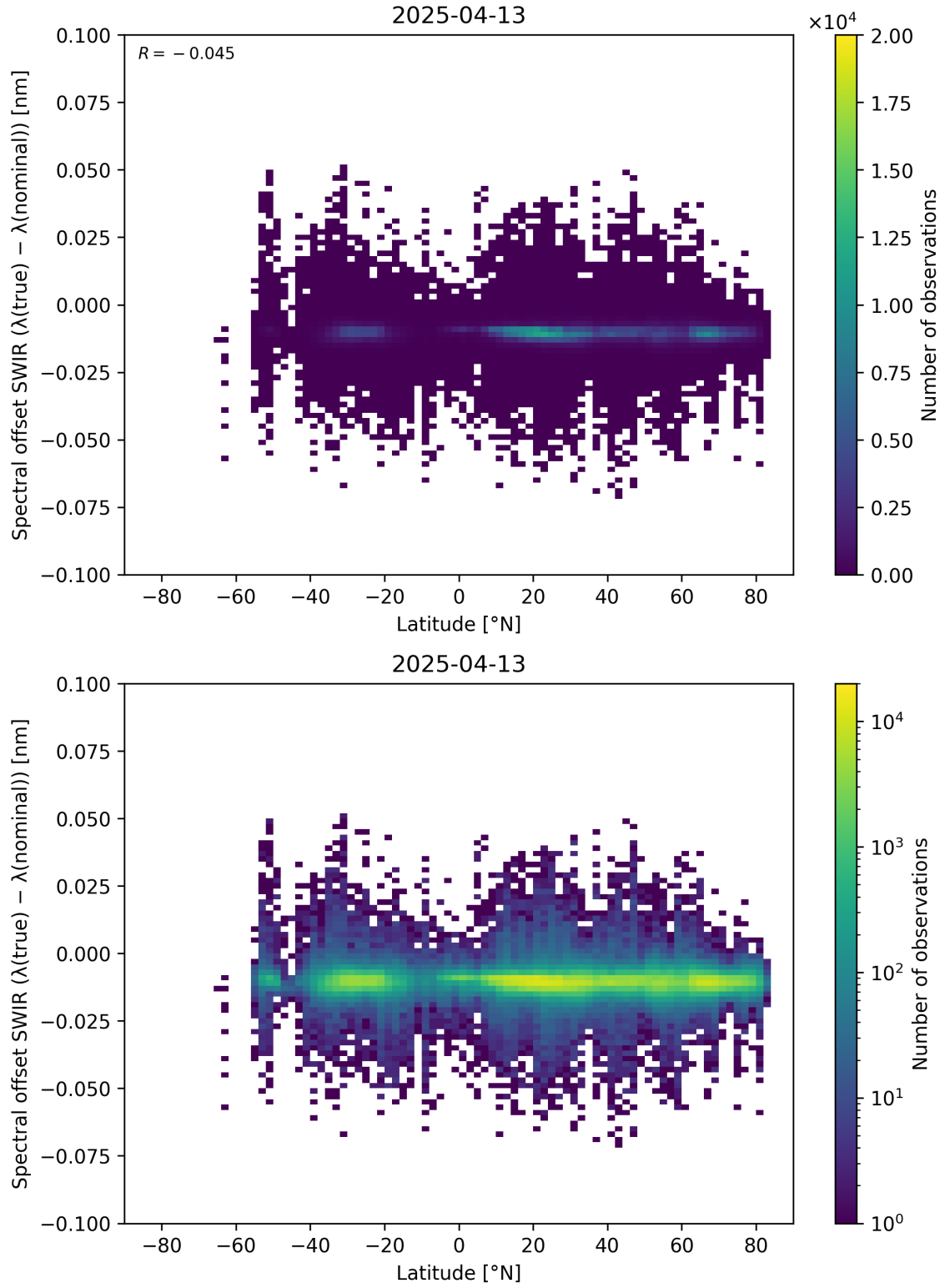
Figure 62: Scatter density plot of “Latitude” against “Spectral offset SWIR ( \lambda_{\text{true}} - \lambda_{\text{nominal}} )” for 2025-04-13 to 2025-04-14.
