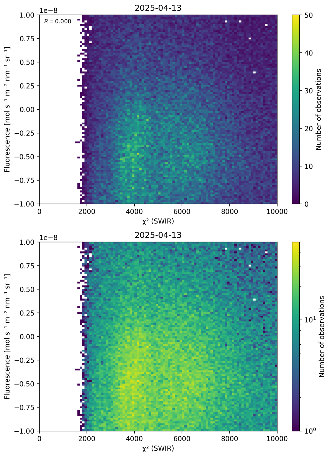
Figure 49: Scatter density plot of “ \chi^2 (SWIR)” against “Fluorescence” for 2025-04-13 to 2025-04-14.
