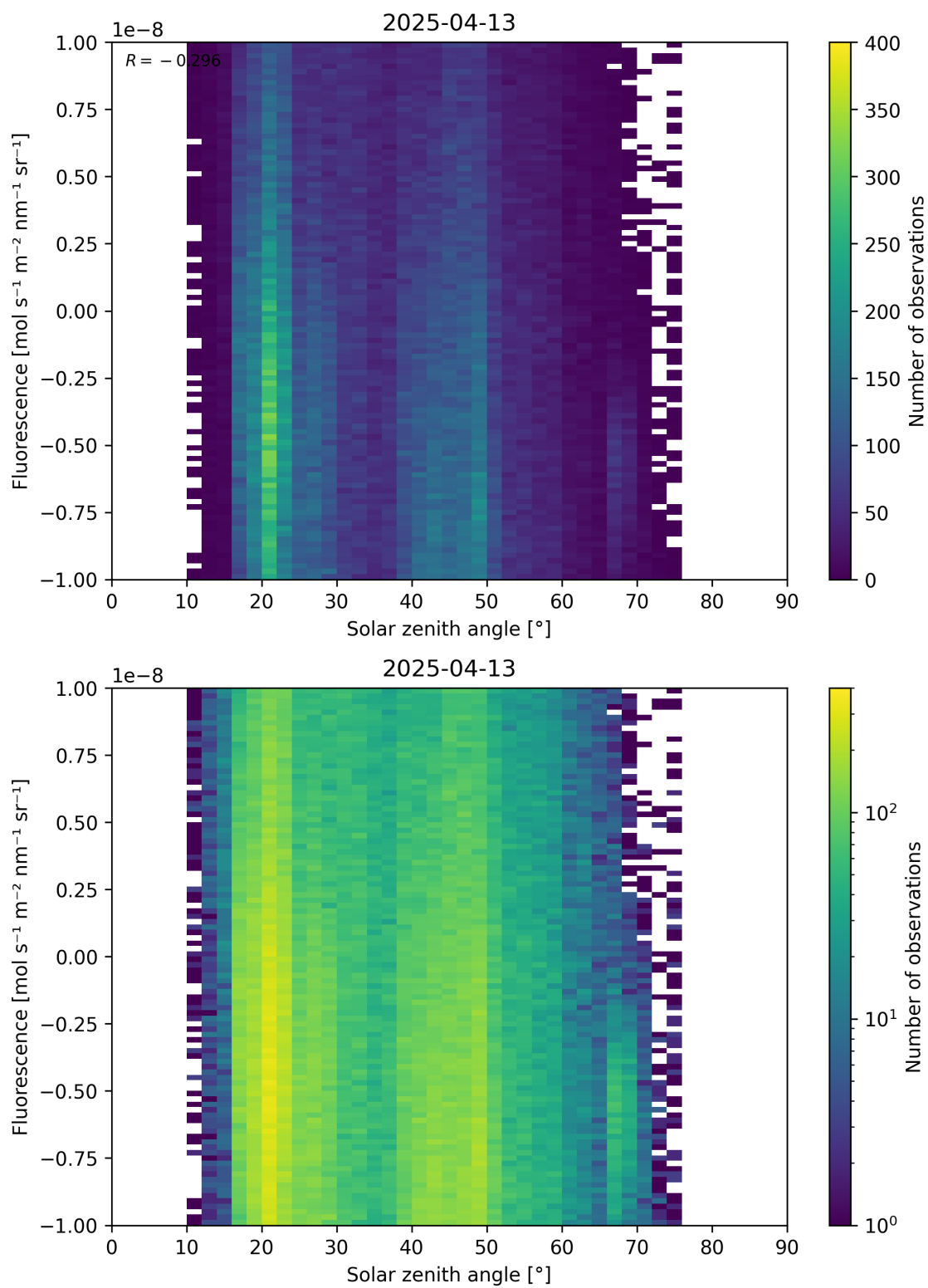
Figure 97: Scatter density plot of “Solar zenith angle” against “Fluorescence” for 2025-04-13 to 2025-04-14.
