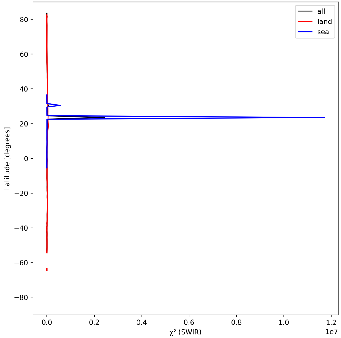
Figure 17: Zonal average of “ \chi^2 (SWIR)” for 2025-04-13 to 2025-04-14.
