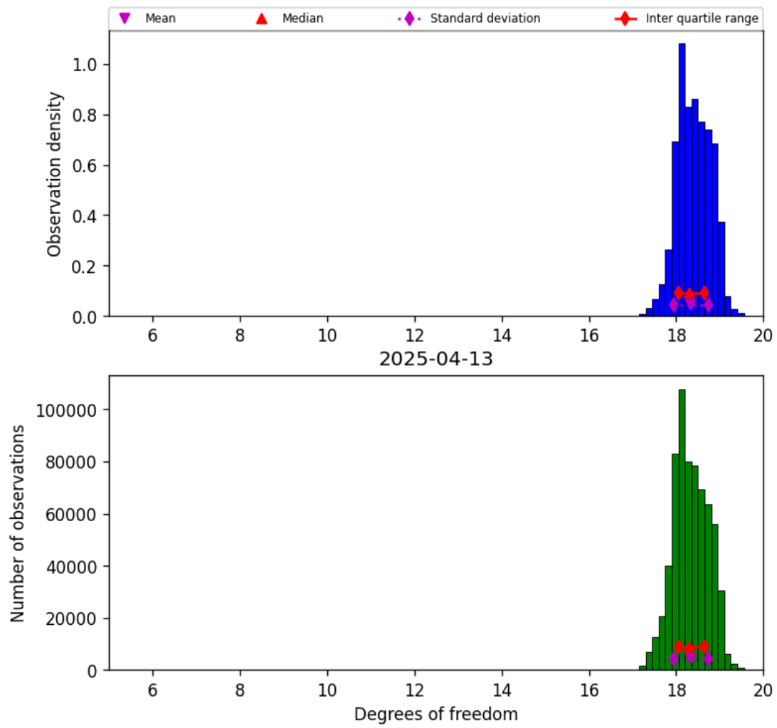
Figure 30: Histogram of “Degrees of freedom” for 2025-04-13 to 2025-04-14
