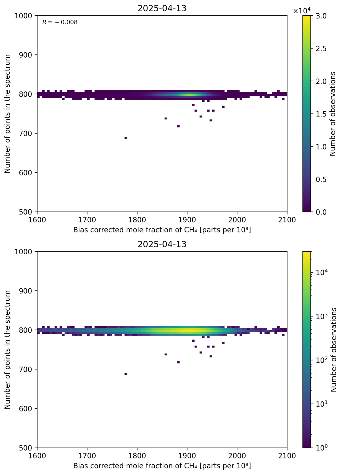
Figure 68: Scatter density plot of “Bias corrected mole fraction of CH 4 ” against “Number of points in the spectrum” for 2025-04-13 to 2025-04-14.
