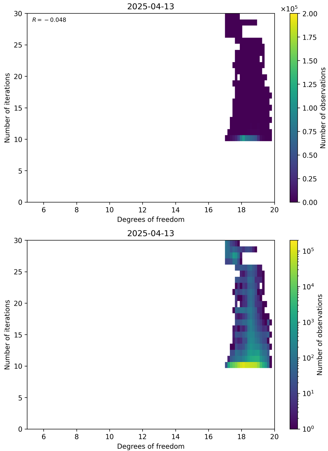
Figure 52: Scatter density plot of “Degrees of freedom” against “Number of iterations” for 2025-04-13 to 2025-04-14.
