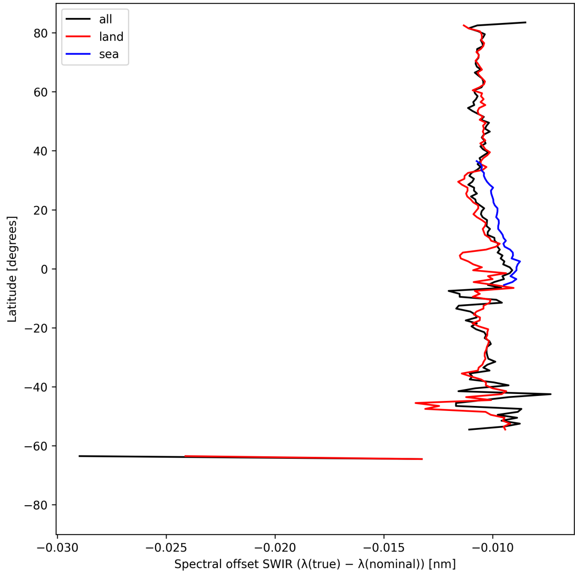
Figure 16: Zonal average of “Spectral offset SWIR ( \lambda_{\text{true}} - \lambda_{\text{nominal}} )” for 2025-04-13 to 2025-04-14.
