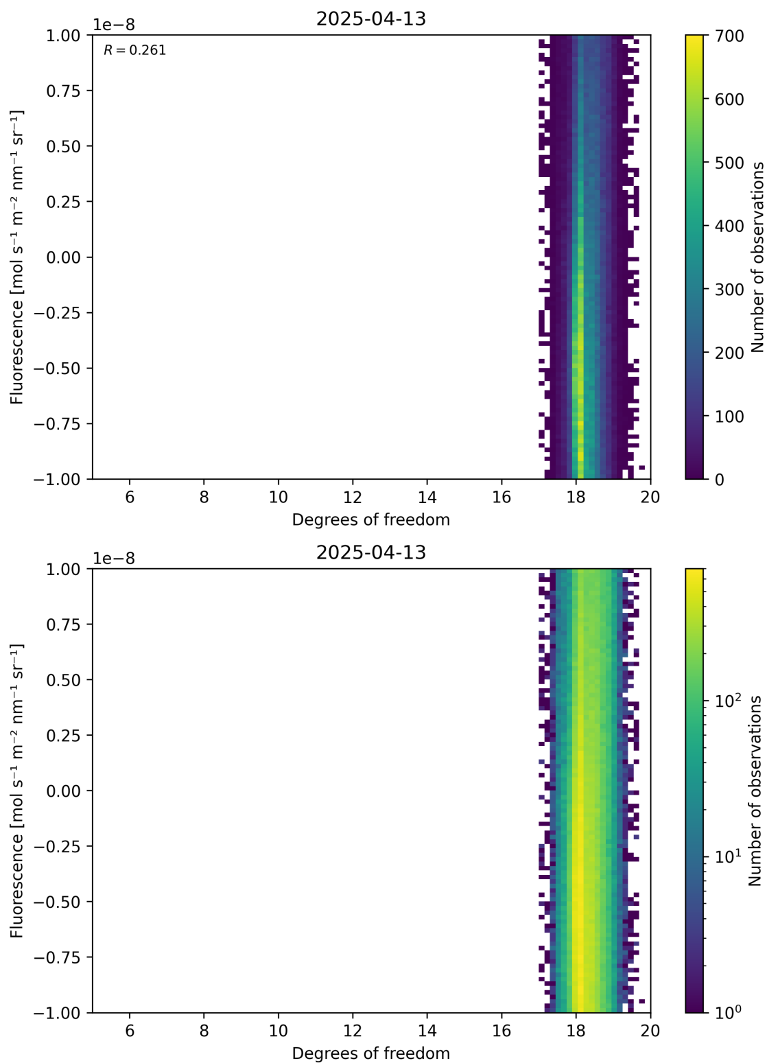
Figure 51: Scatter density plot of “Degrees of freedom” against “Fluorescence” for 2025-04-13 to 2025-04-14.
