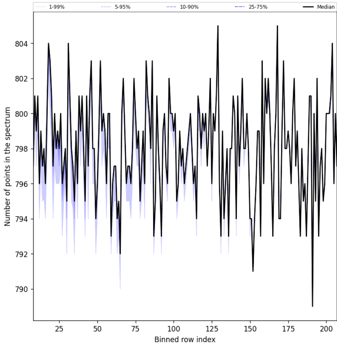
Figure 37: Along track statistics of “Number of points in the spectrum” for 2025-04-13 to 2025-04-14
