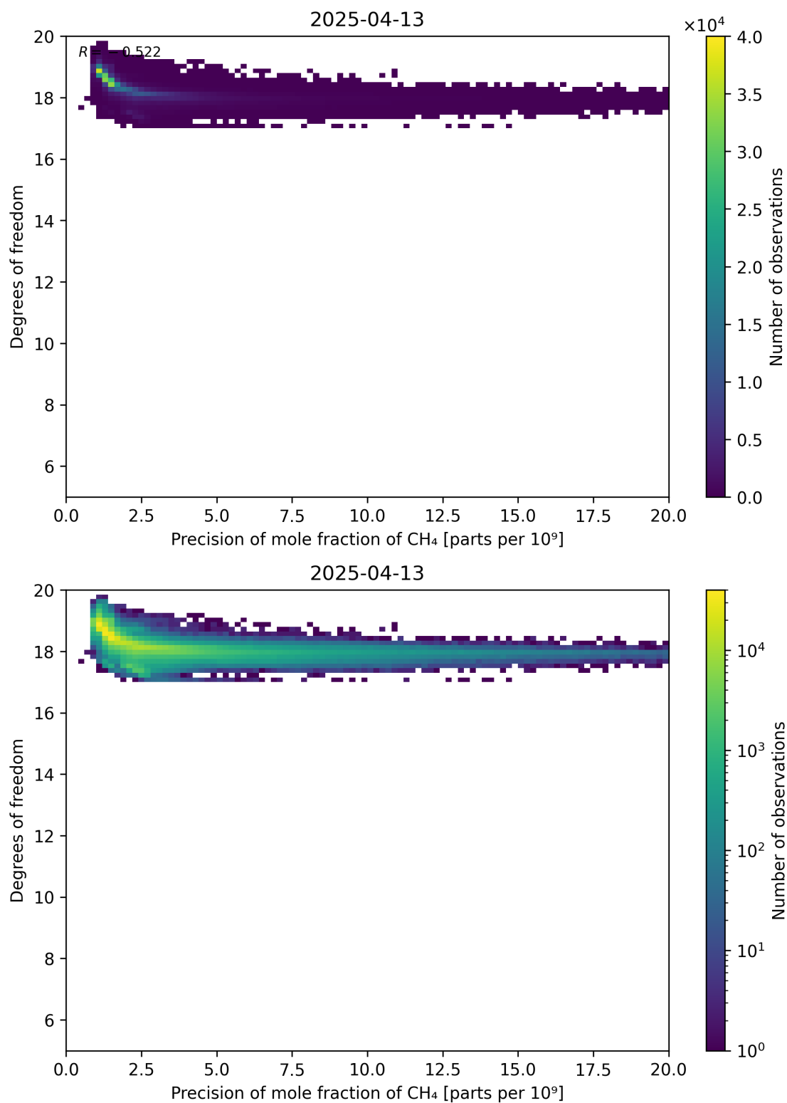
Figure 80: Scatter density plot of “Precision of mole fraction of CH 4 ” against “Degrees of freedom” for 2025-04-13 to 2025-04-14.
