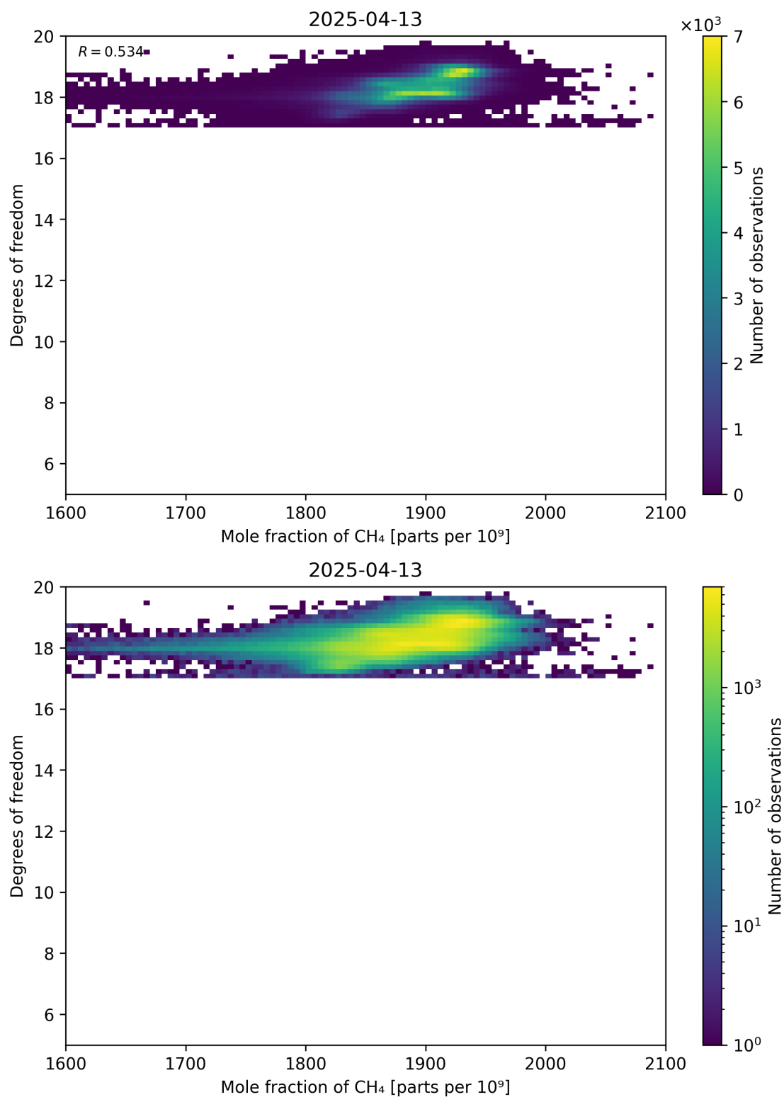
Figure 72: Scatter density plot of “Mole fraction of CH 4 ” against “Degrees of freedom” for 2025-04-13 to 2025-04-14.
