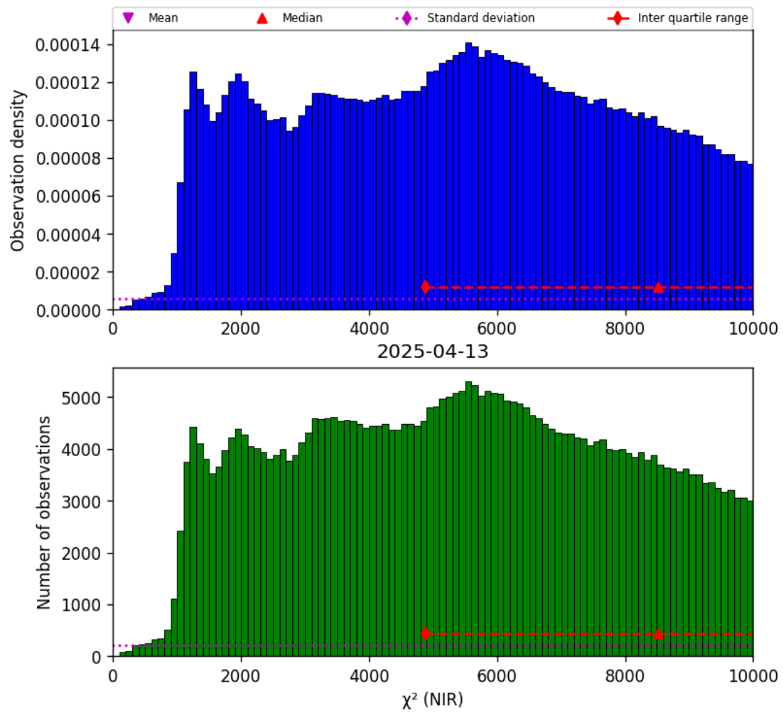
Figure 29: Histogram of " \chi^2 (NIR)" for 2025-04-13 to 2025-04-14
