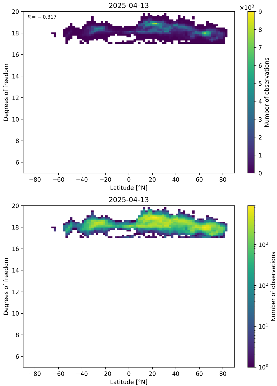
Figure 55: Scatter density plot of “Latitude” against “Degrees of freedom” for 2025-04-13 to 2025-04-14.
