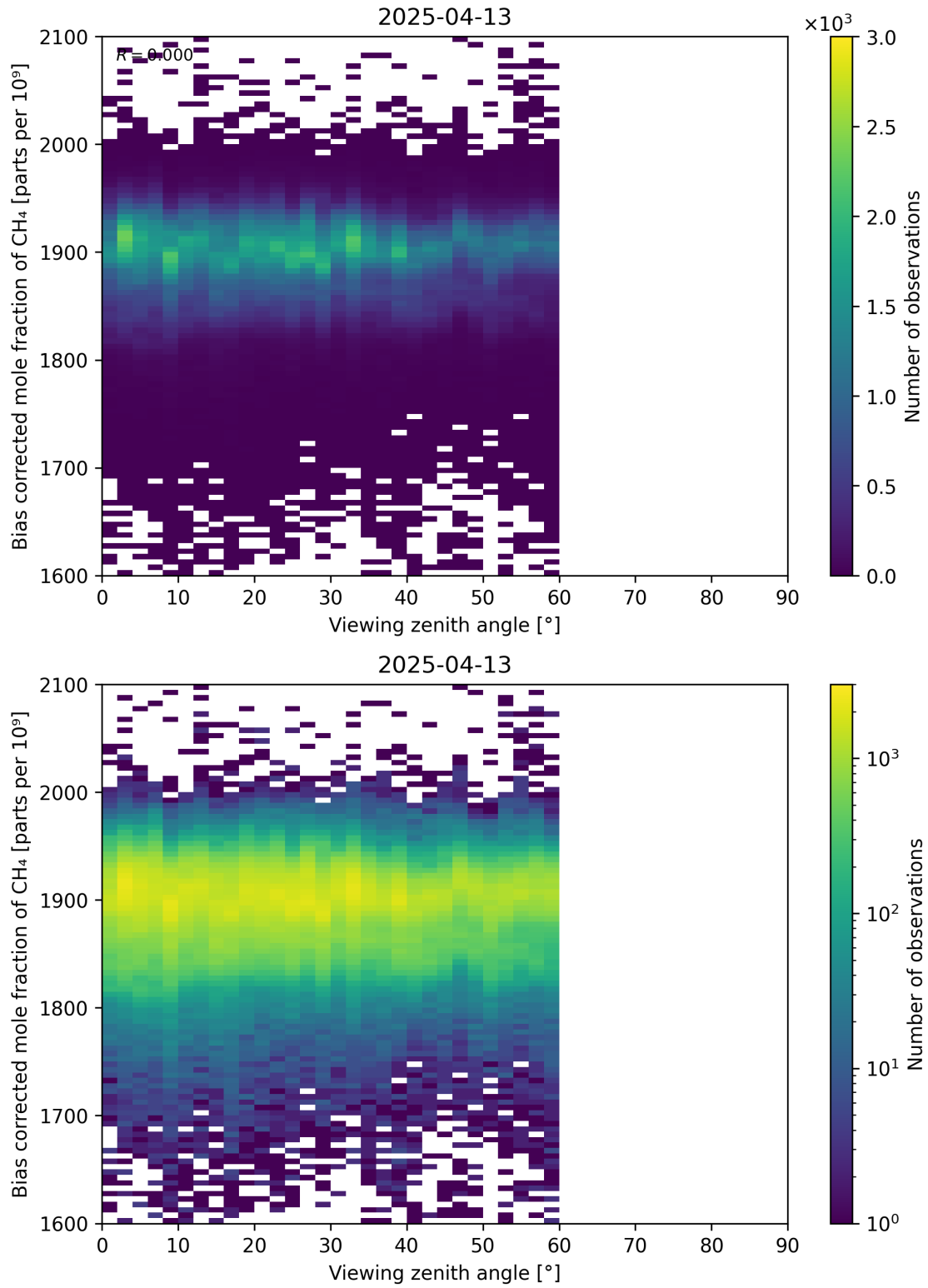
Figure 111: Scatter density plot of “Viewing zenith angle” against “Bias corrected mole fraction of CH 4 ” for 2025-04-13 to 2025-04-14.
