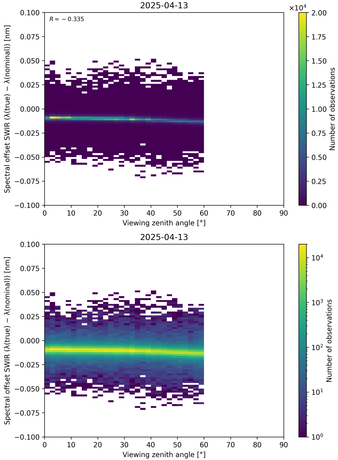
Figure 116: Scatter density plot of “Viewing zenith angle” against “Spectral offset SWIR ( \lambda_{\text{true}} - \lambda_{\text{nominal}} )” for 2025-04-13 to 2025-04-14.
