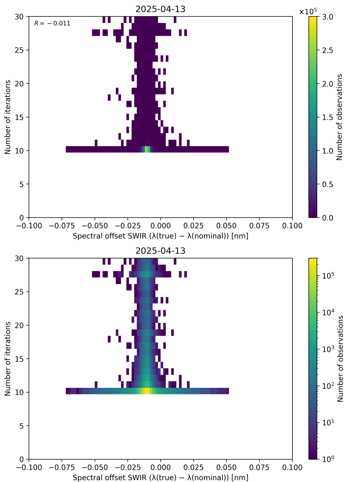
Figure 121: Scatter density plot of “Spectral offset SWIR ( \lambda_{\text{true}} - \lambda_{\text{nominal}} )” against “Number of iterations” for 2025-04-13 to 2025-04-14.
