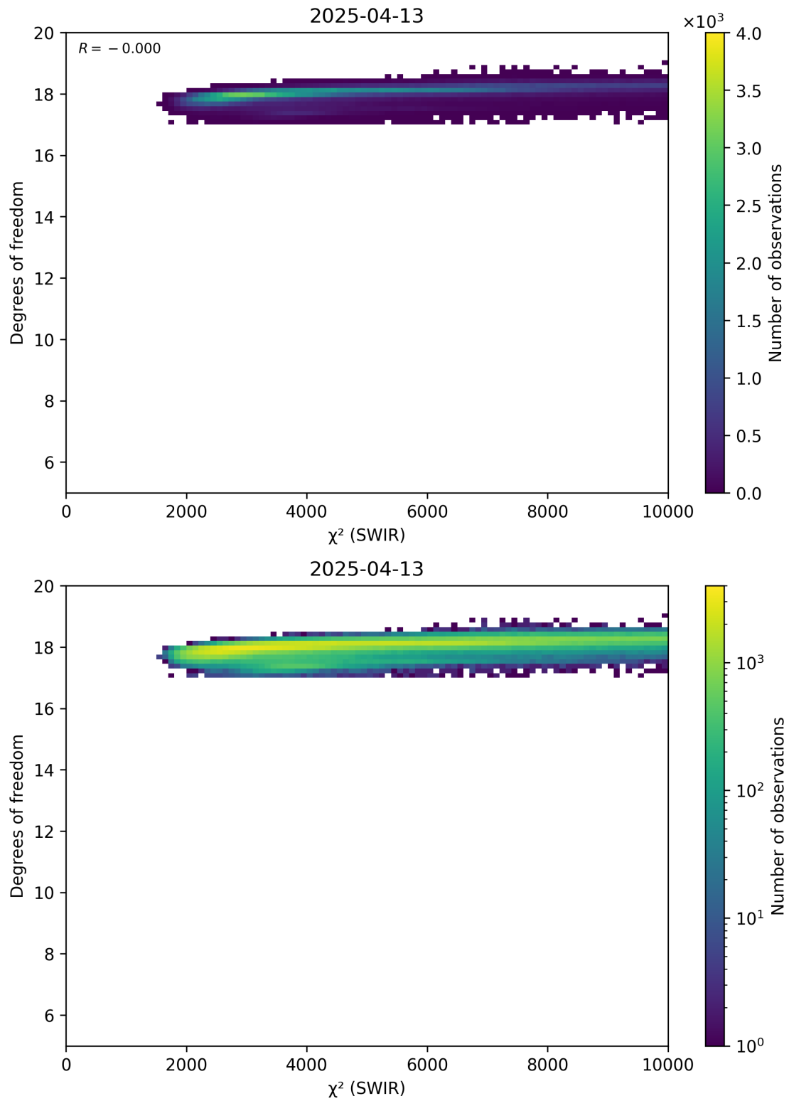
Figure 48: Scatter density plot of “ \chi^2 (SWIR)” against “Degrees of freedom” for 2025-04-13 to 2025-04-14.
