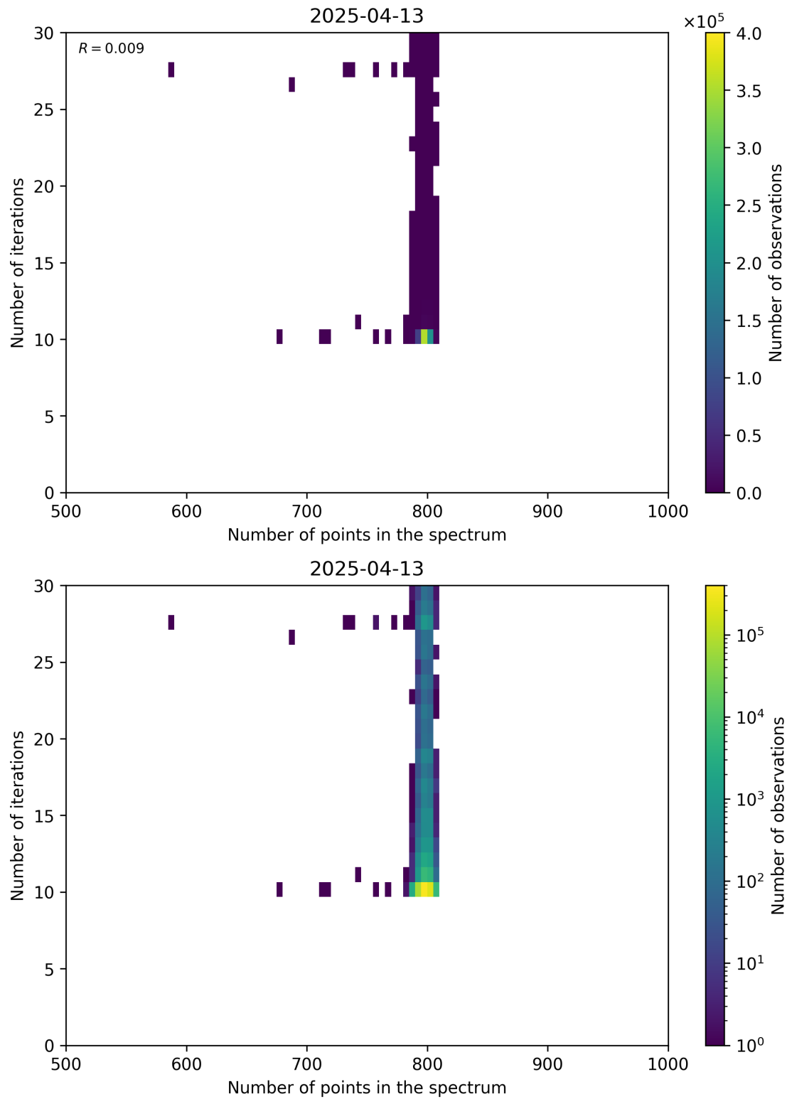
Figure 92: Scatter density plot of “Number of points in the spectrum” against “Number of iterations” for 2025-04-13 to 2025-04-14.
