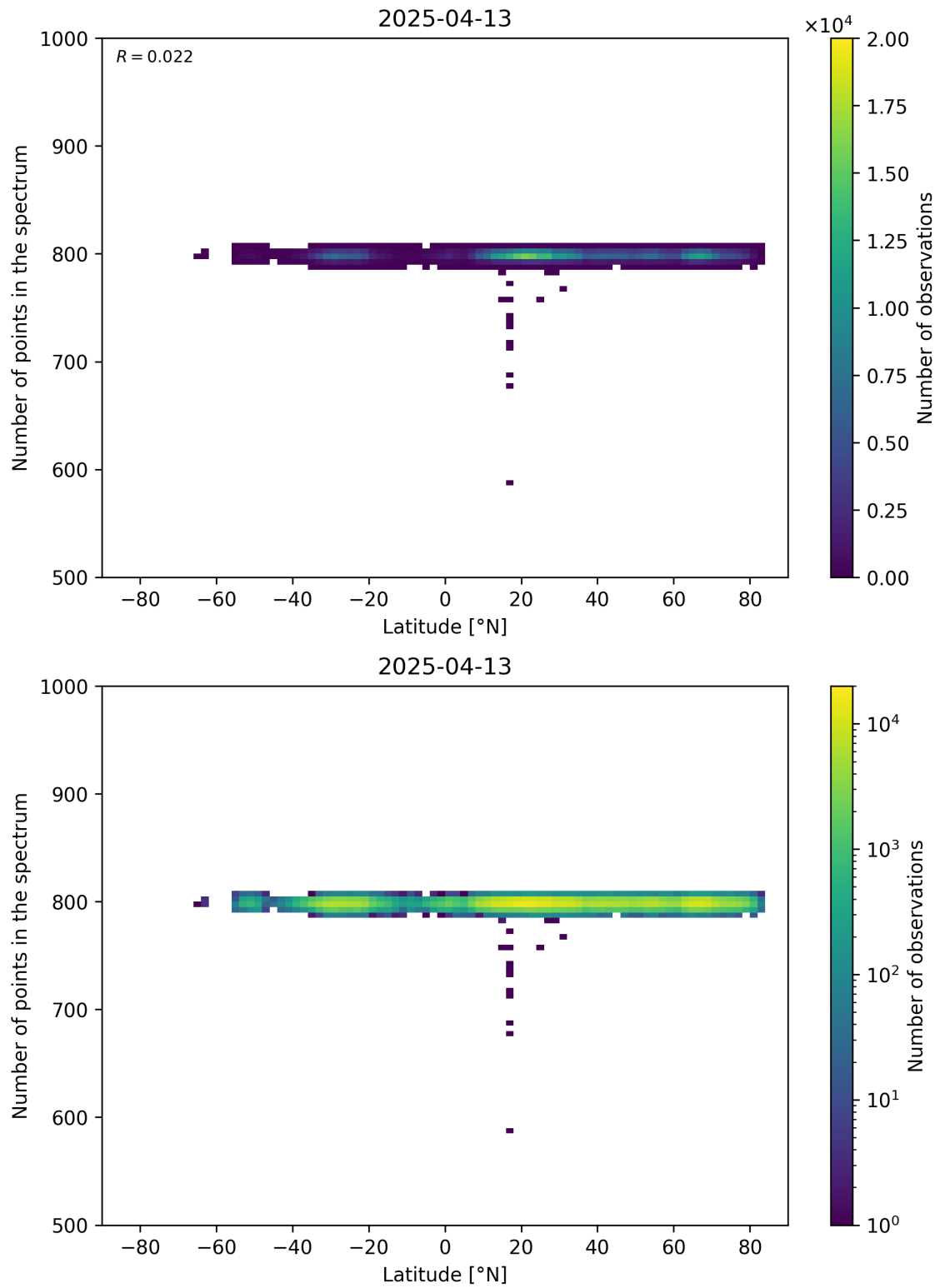
Figure 61: Scatter density plot of “Latitude” against “Number of points in the spectrum” for 2025-04-13 to 2025-04-14.
