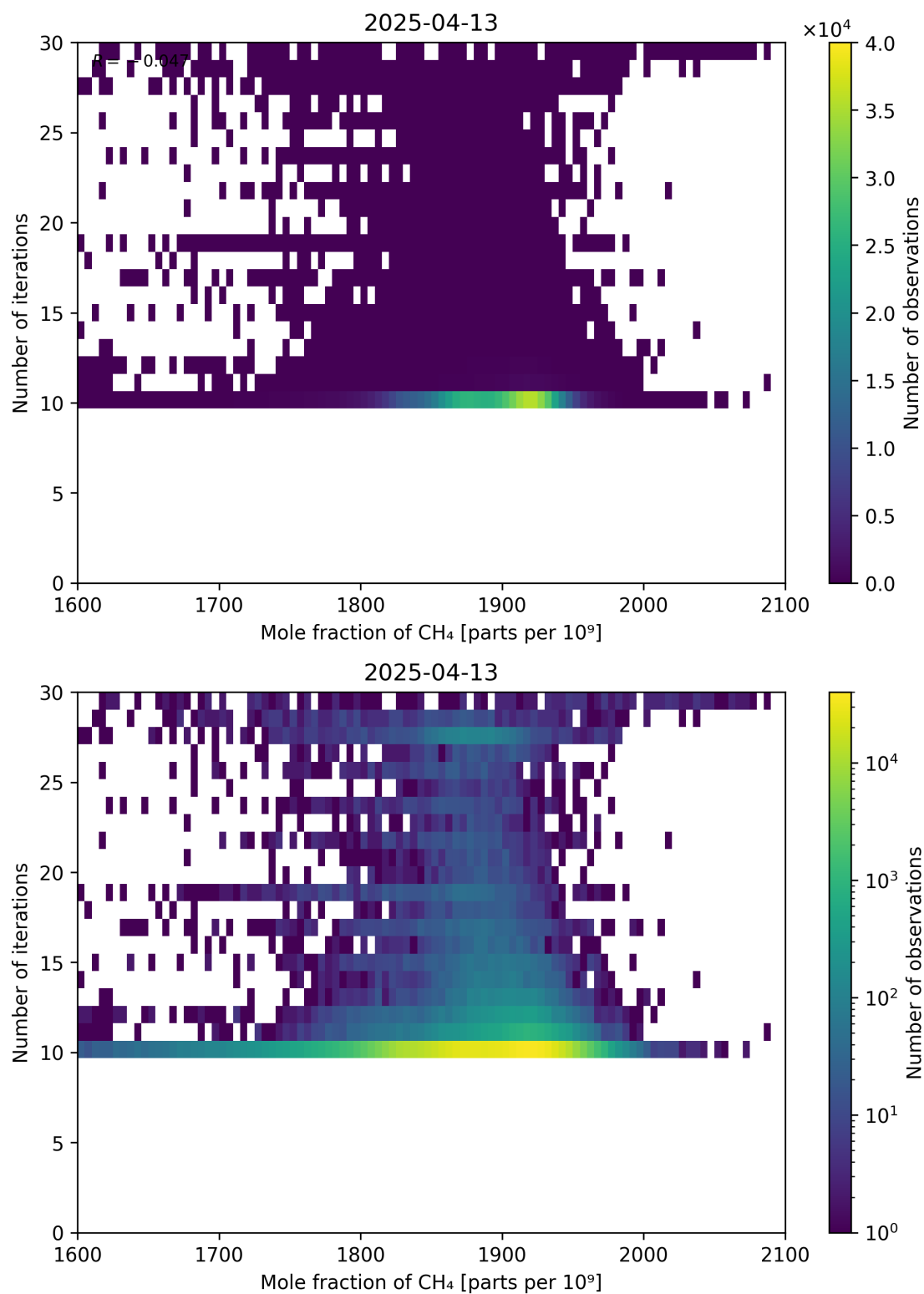
Figure 76: Scatter density plot of “Mole fraction of CH 4 ” against “Number of iterations” for 2025-04-13 to 2025-04-14.
