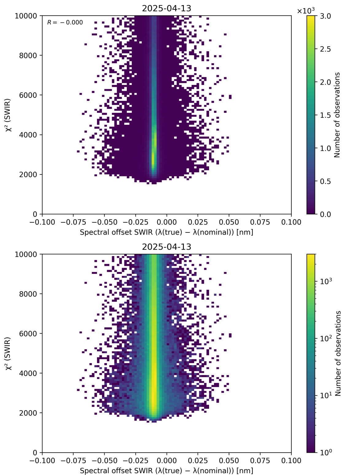
Figure 118: Scatter density plot of “Spectral offset SWIR ( \lambda_{\text{true}} - \lambda_{\text{nominal}} )” against “ \chi^2 (SWIR)” for 2025-04-13 to 2025-04-14.
