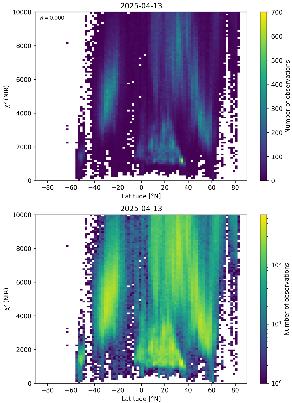
Figure 53: Scatter density plot of “Latitude” against “ \chi^2 (NIR)” for 2025-04-13 to 2025-04-14.
