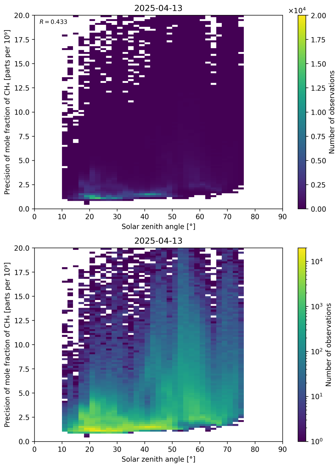
Figure 101: Scatter density plot of “Solar zenith angle” against “Precision of mole fraction of CH 4 ” for 2025-04-13 to 2025-04-14.
