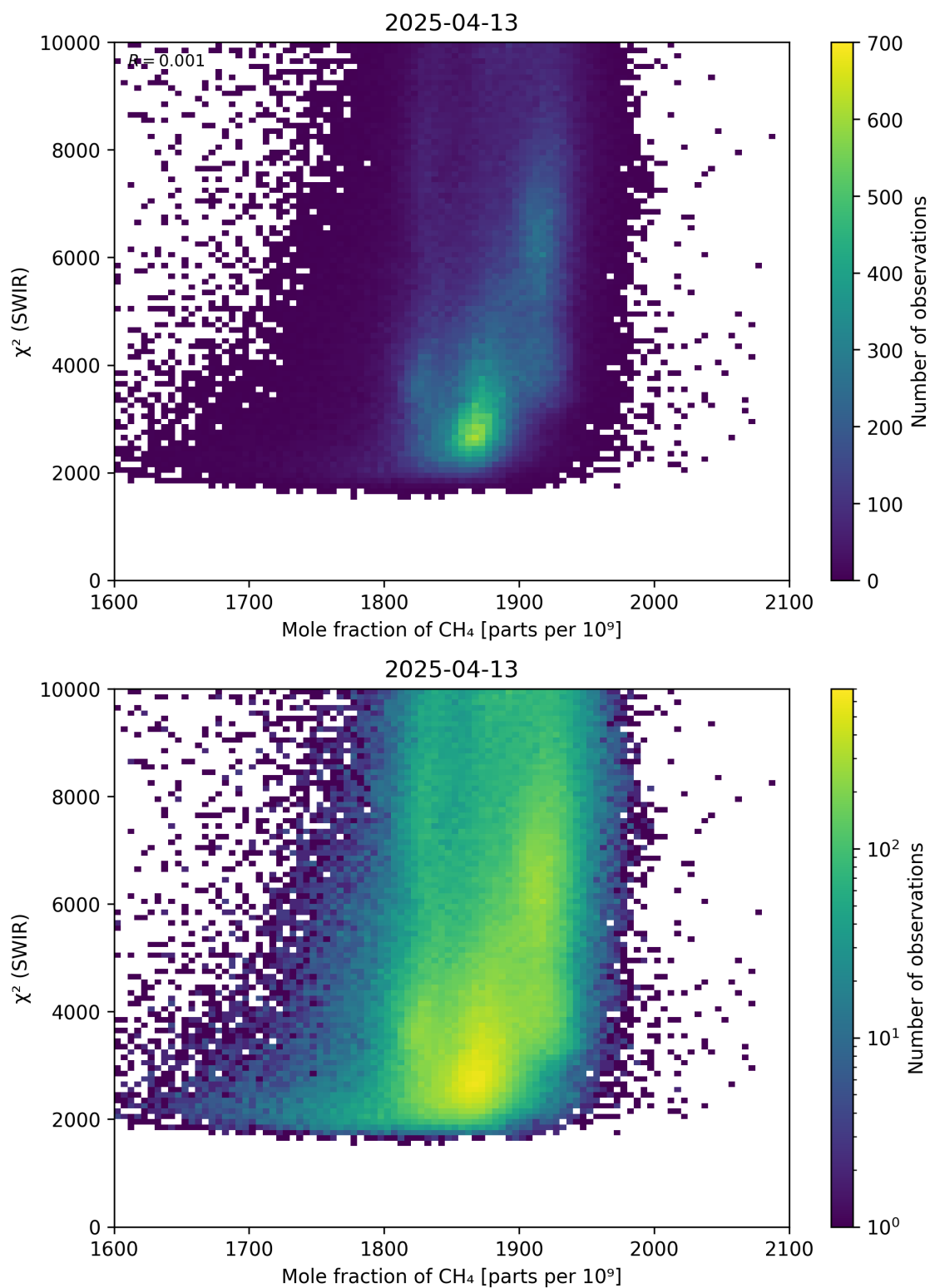
Figure 71: Scatter density plot of “Mole fraction of CH 4 ” against “ \chi^2 (SWIR)” for 2025-04-13 to 2025-04-14.
