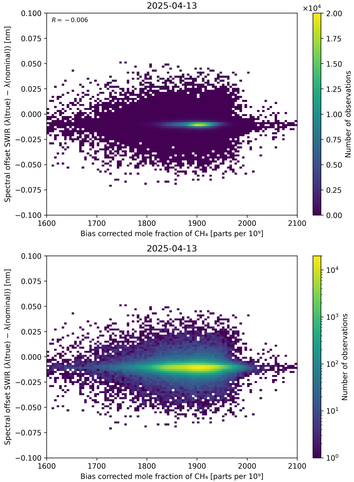
Figure 69: Scatter density plot of “Bias corrected mole fraction of \text{CH}_4 ” against “Spectral offset SWIR ( \lambda_{\text{true}} - \lambda_{\text{nominal}} )” for 2025-04-13 to 2025-04-14.
