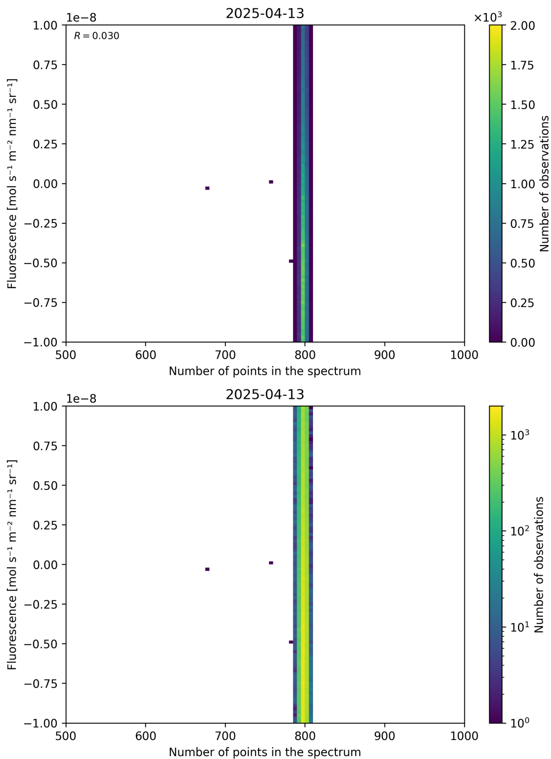
Figure 91: Scatter density plot of “Number of points in the spectrum” against “Fluorescence” for 2025-04-13 to 2025-04-14.
