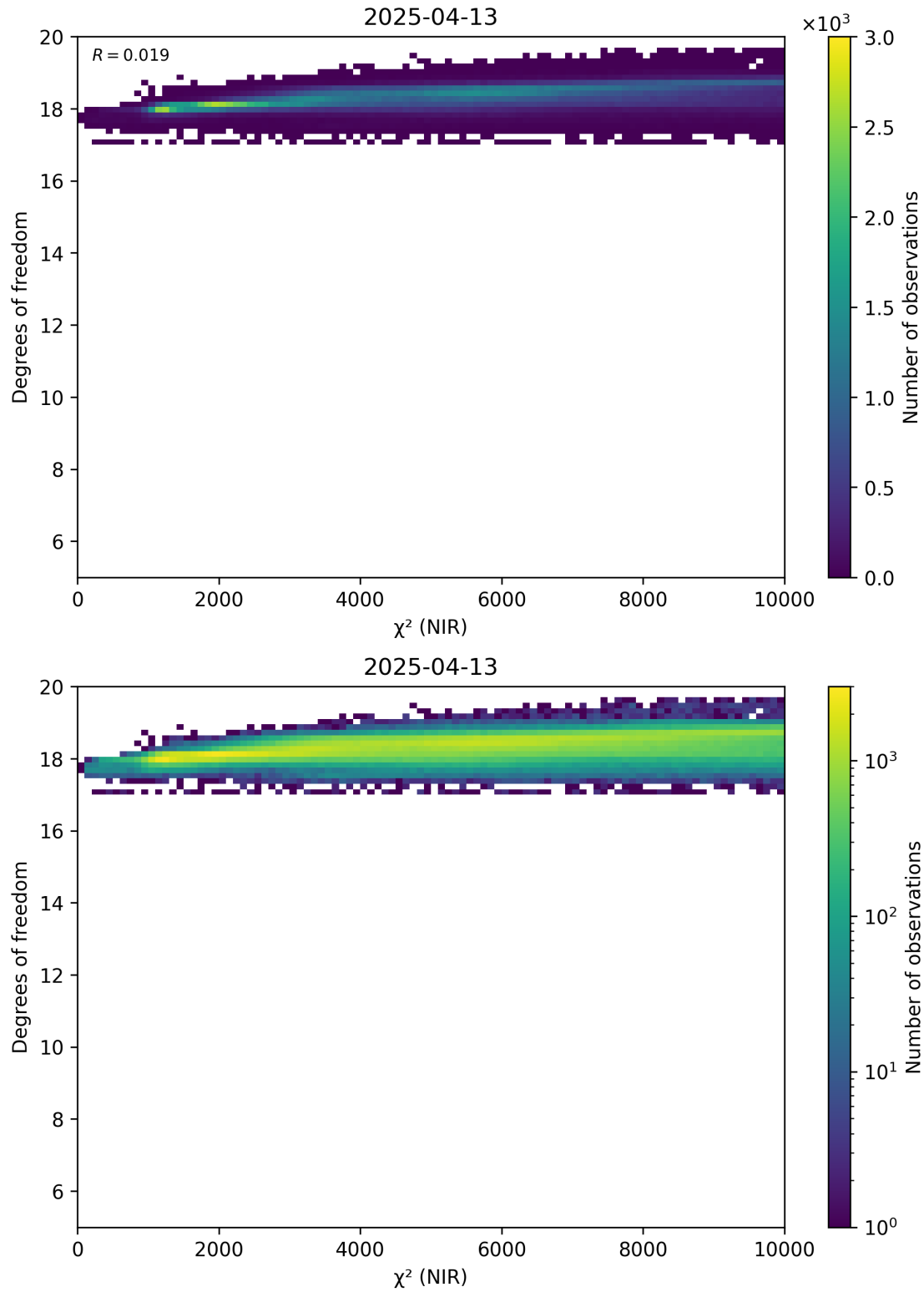
Figure 44: Scatter density plot of “ \chi^2 (NIR)” against “Degrees of freedom” for 2025-04-13 to 2025-04-14.
