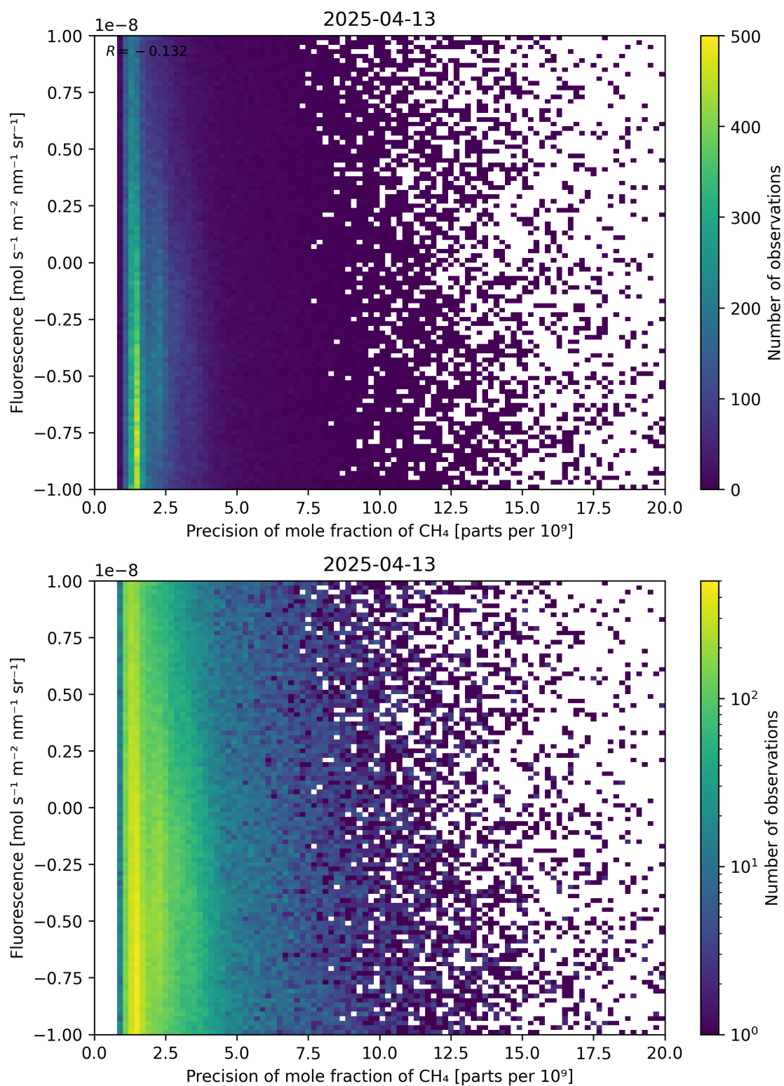
Figure 81: Scatter density plot of “Precision of mole fraction of CH 4 ” against “Fluorescence” for 2025-04-13 to 2025-04-14.
