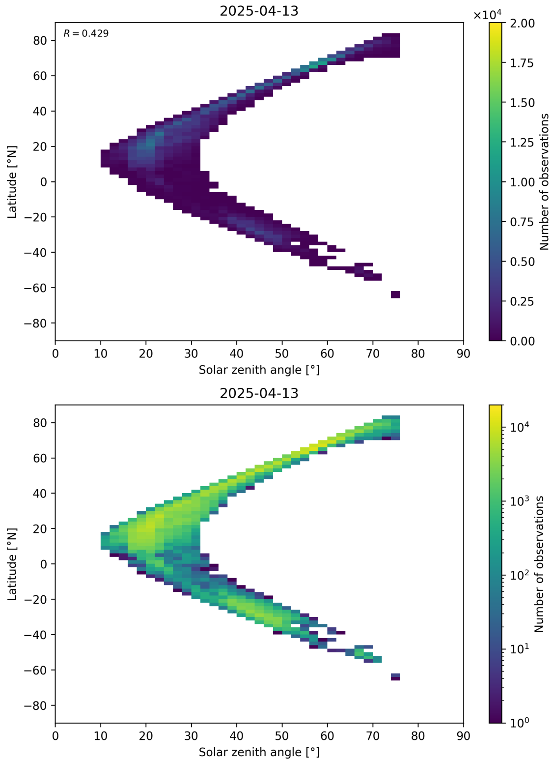
Figure 98: Scatter density plot of “Solar zenith angle” against “Latitude” for 2025-04-13 to 2025-04-14.
