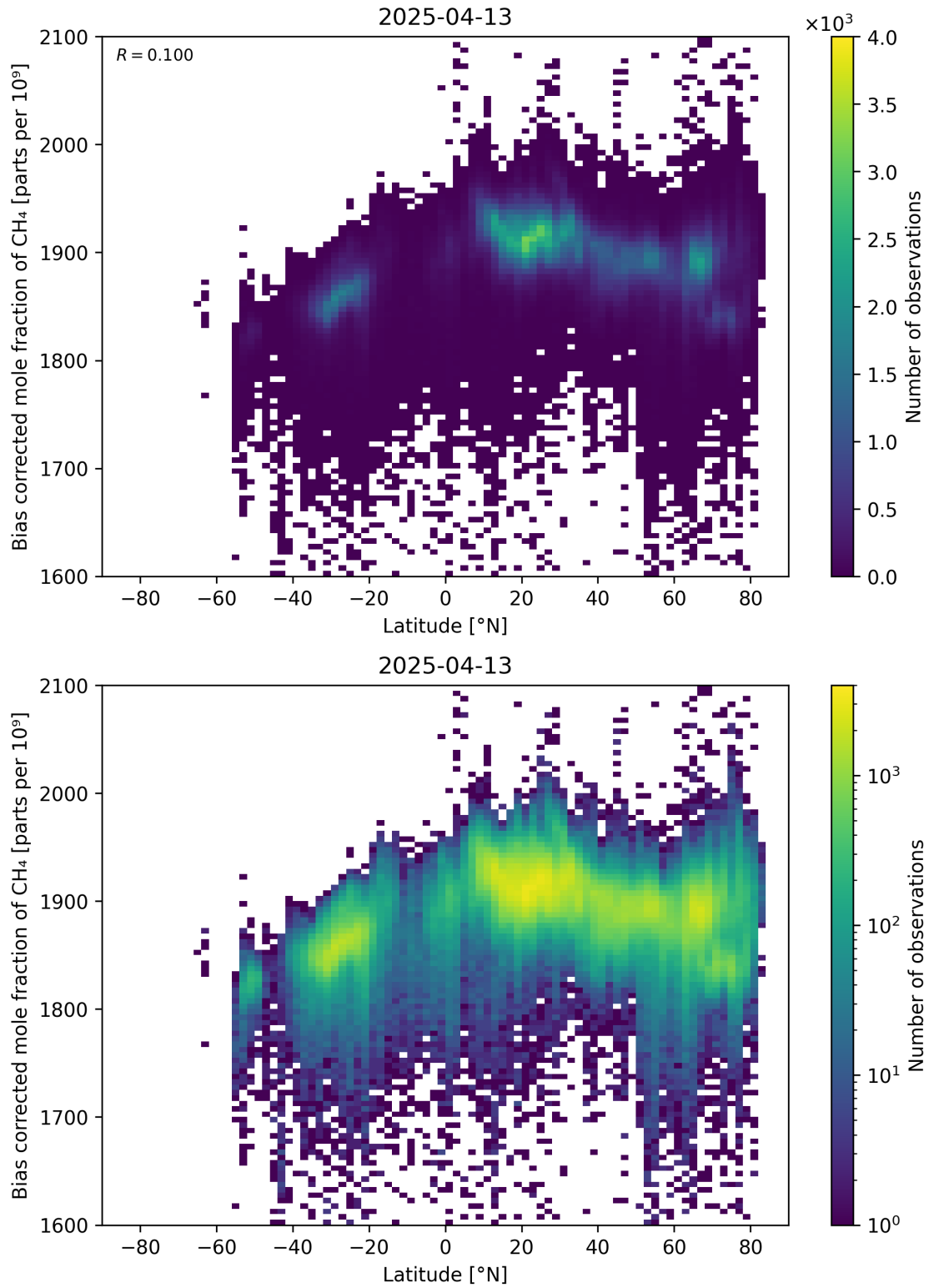
Figure 58: Scatter density plot of “Latitude” against “Bias corrected mole fraction of CH 4 ” for 2025-04-13 to 2025-04-14.
