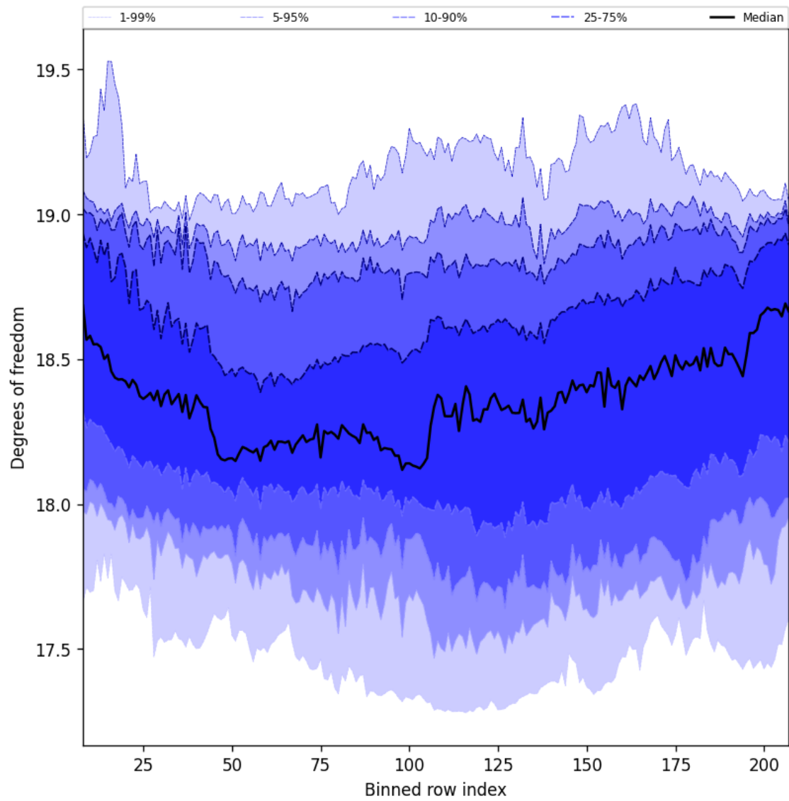
Figure 41: Along track statistics of “Degrees of freedom” for 2025-04-13 to 2025-04-14
