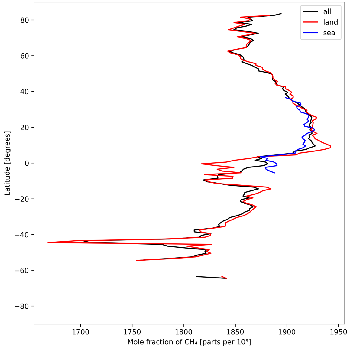
Figure 12: Zonal average of “Mole fraction of \text{CH}_4 ” for 2025-04-13 to 2025-04-14.
