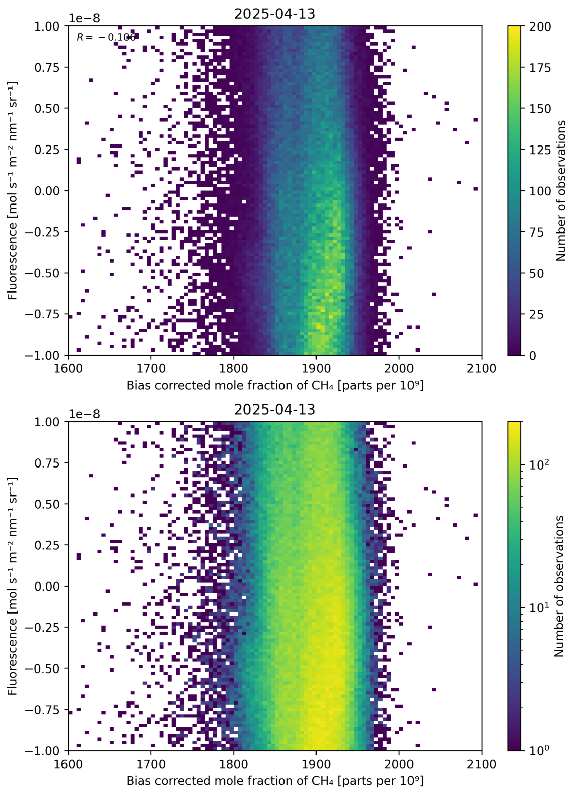
Figure 66: Scatter density plot of “Bias corrected mole fraction of \text{CH}_4 ” against “Fluorescence” for 2025-04-13 to 2025-04-14.
