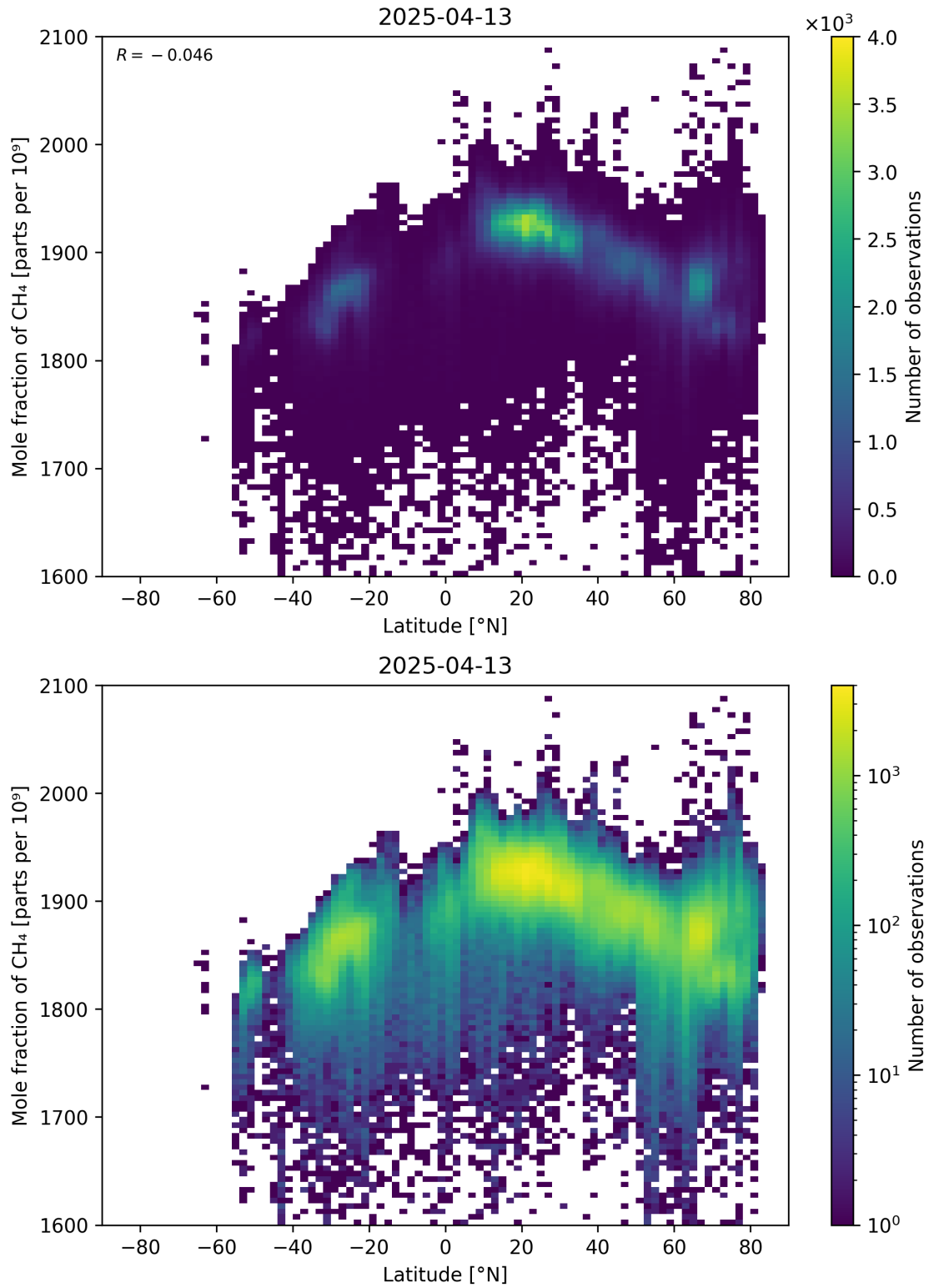
Figure 57: Scatter density plot of “Latitude” against “Mole fraction of CH 4 ” for 2025-04-13 to 2025-04-14.
