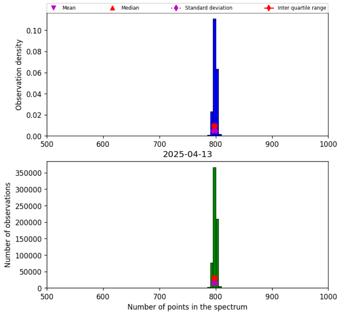
Figure 26: Histogram of “Number of points in the spectrum” for 2025-04-13 to 2025-04-14
