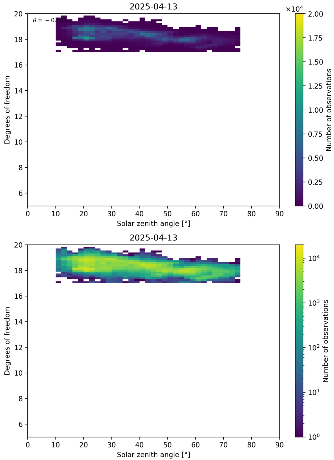
Figure 96: Scatter density plot of “Solar zenith angle” against “Degrees of freedom” for 2025-04-13 to 2025-04-14.
