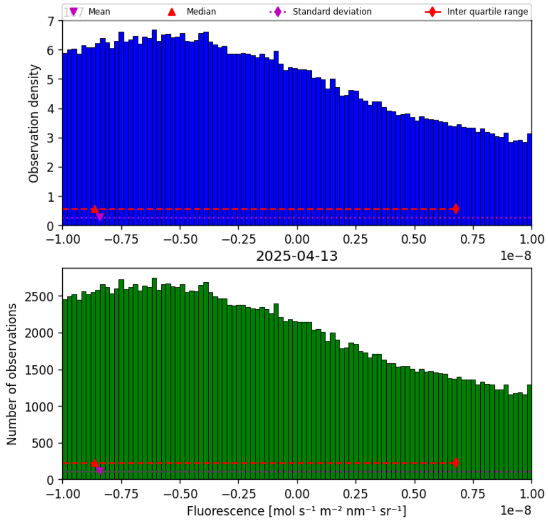
Figure 32: Histogram of “Fluorescence” for 2025-04-13 to 2025-04-14
