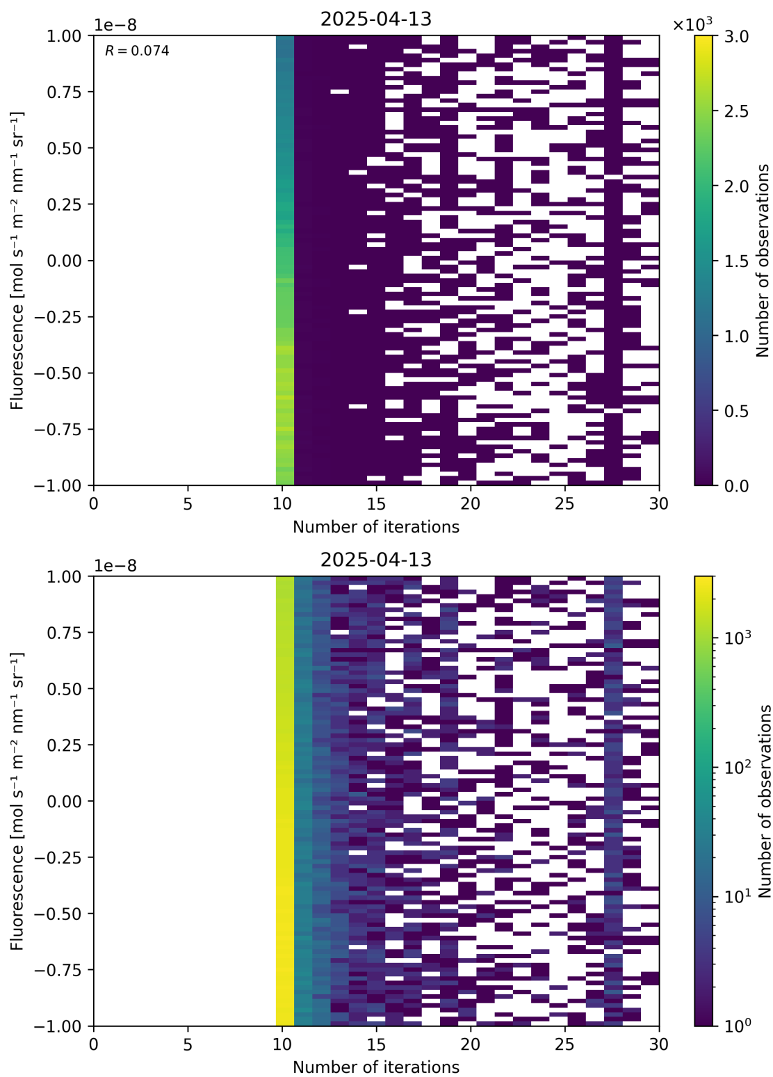
Figure 87: Scatter density plot of “Number of iterations” against “Fluorescence” for 2025-04-13 to 2025-04-14.
