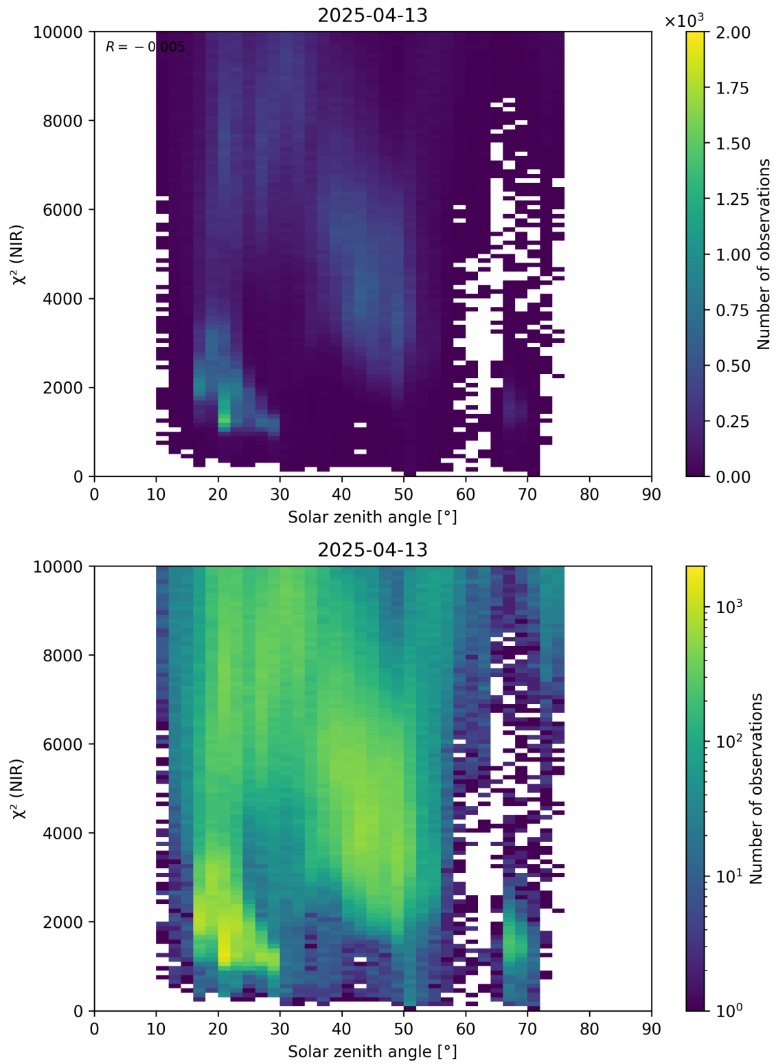
Figure 94: Scatter density plot of “Solar zenith angle” against “ \chi^2 (NIR)” for 2025-04-13 to 2025-04-14.
