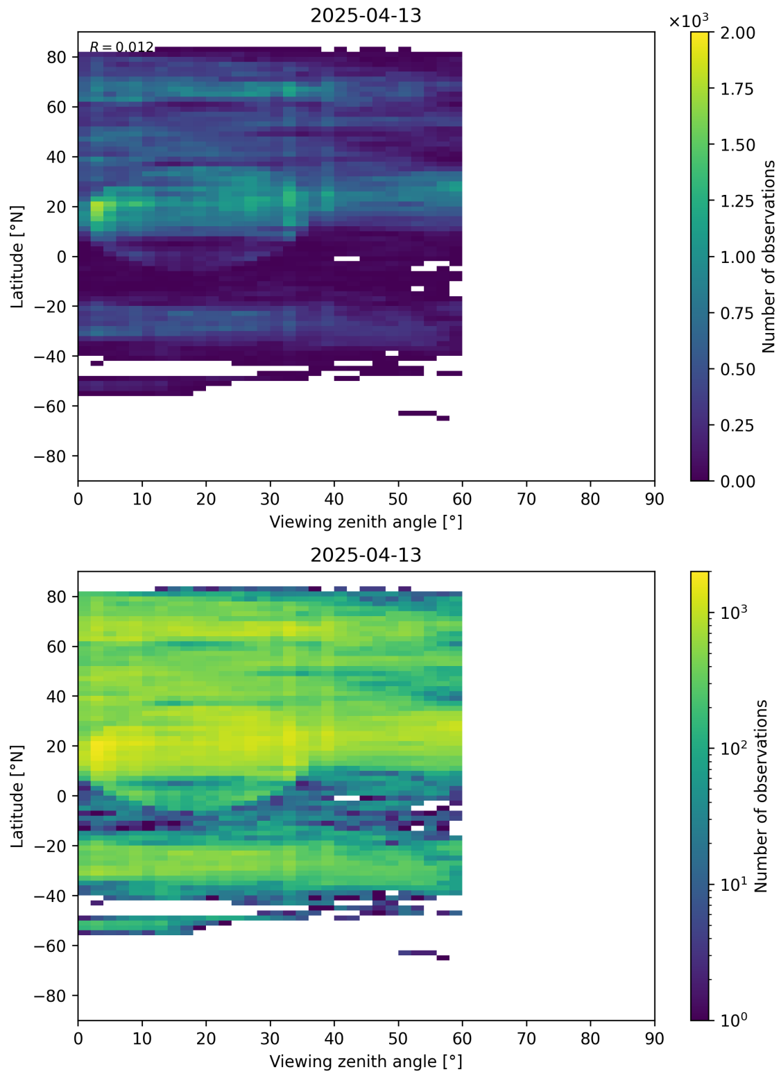
Figure 109: Scatter density plot of “Viewing zenith angle” against “Latitude” for 2025-04-13 to 2025-04-14.
