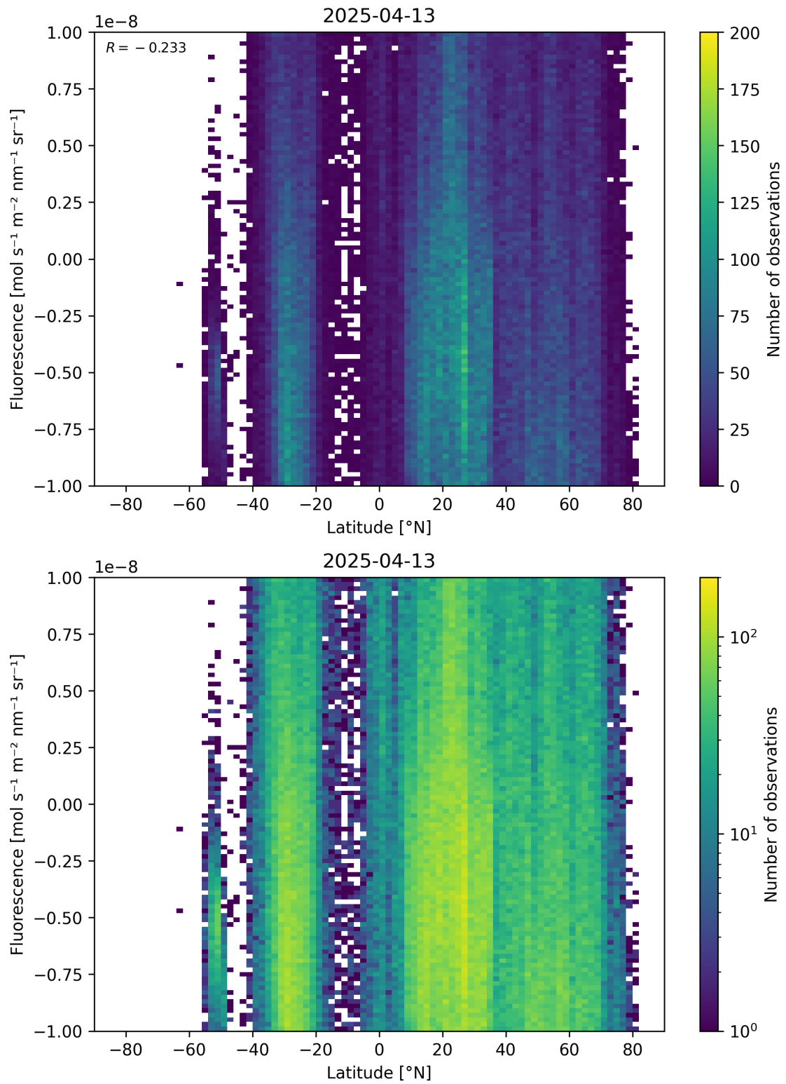
Figure 56: Scatter density plot of “Latitude” against “Fluorescence” for 2025-04-13 to 2025-04-14.
