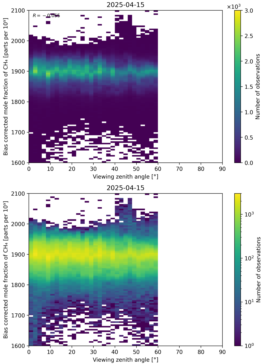
Figure 111: Scatter density plot of “Viewing zenith angle” against “Bias corrected mole fraction of CH 4 ” for 2025-04-14 to 2025-04-16.
