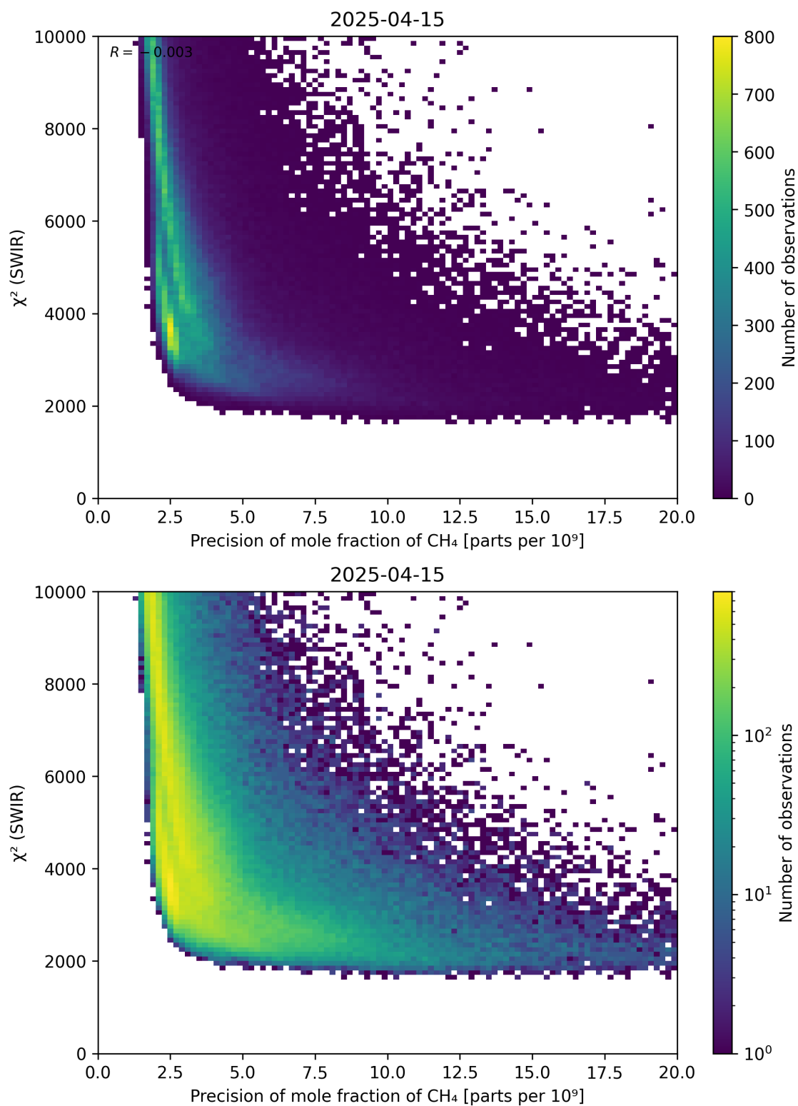
Figure 79: Scatter density plot of “Precision of mole fraction of \text{CH}_4 ” against “ \chi^2 (SWIR)” for 2025-04-14 to 2025-04-16.
