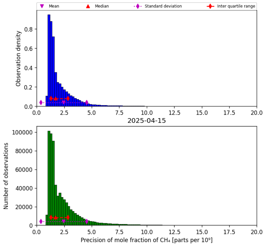
Figure 24: Histogram of “Precision of mole fraction of CH 4 ” for 2025-04-14 to 2025-04-16
