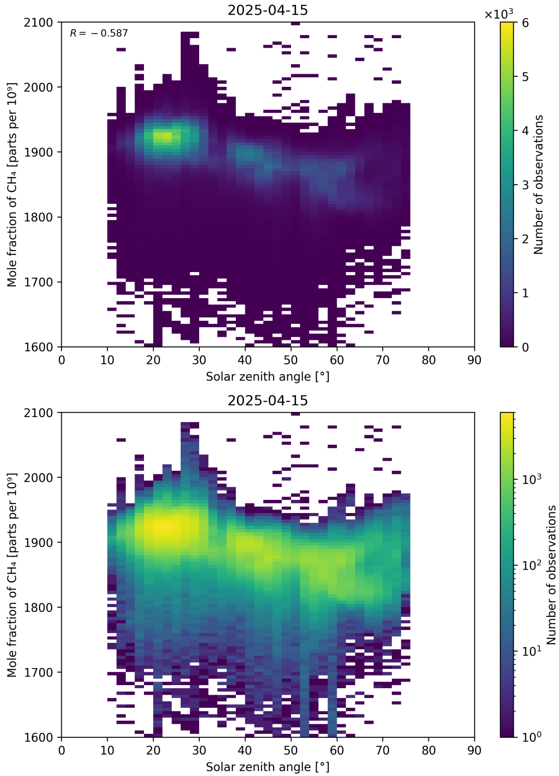
Figure 99: Scatter density plot of “Solar zenith angle” against “Mole fraction of CH 4 ” for 2025-04-14 to 2025-04-16.
