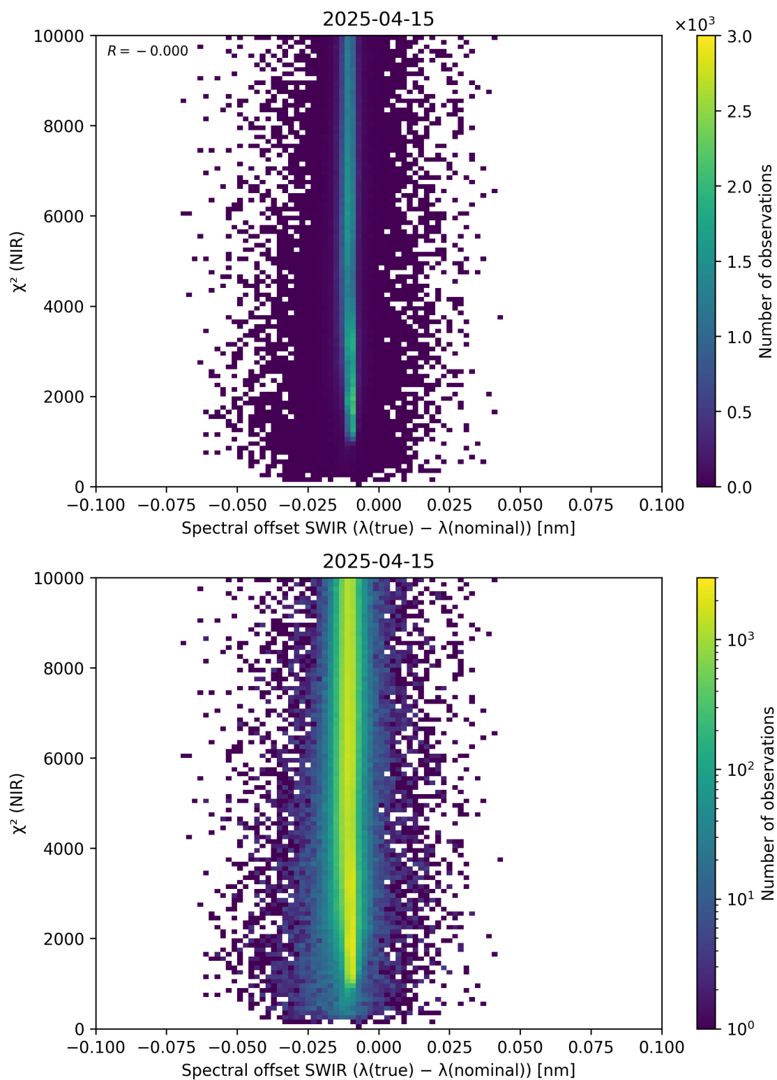
Figure 117: Scatter density plot of “Spectral offset SWIR ( \lambda_{\text{true}} - \lambda_{\text{nominal}} )” against “ \chi^2 (NIR)” for 2025-04-14 to 2025-04-16.
