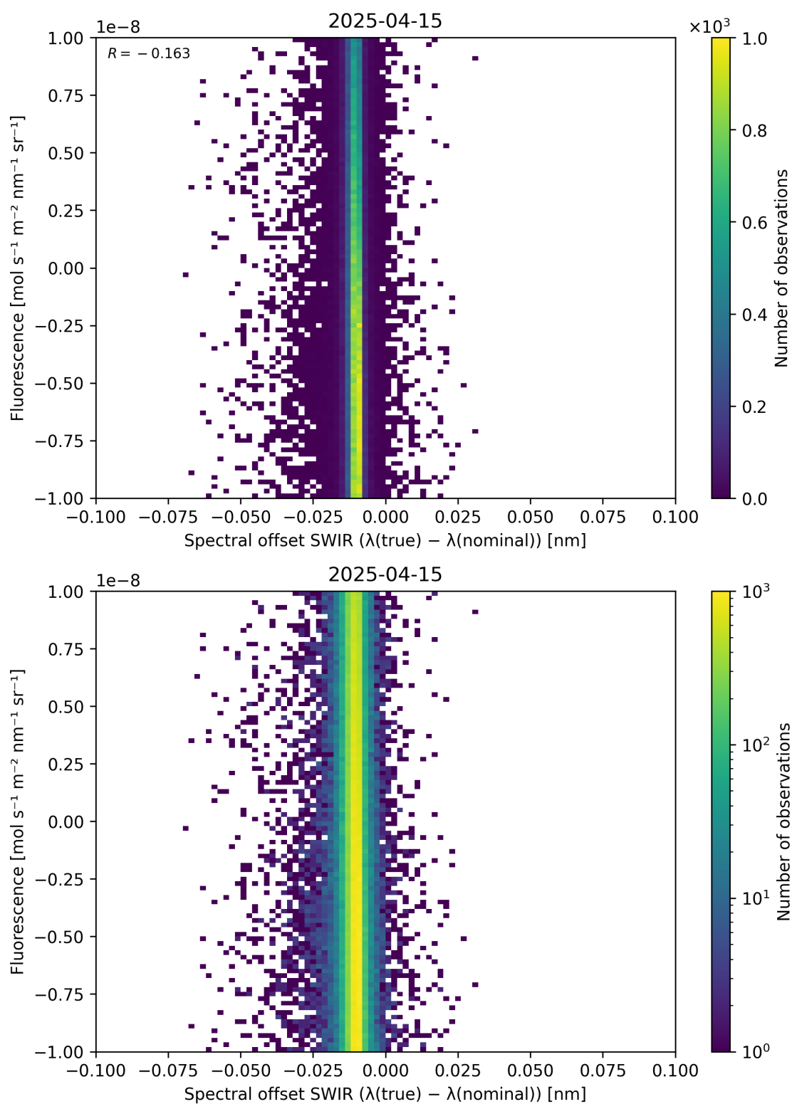
Figure 120: Scatter density plot of “Spectral offset SWIR ( \lambda_{\text{true}} - \lambda_{\text{nominal}} )” against “Fluorescence” for 2025-04-14 to 2025-04-16.
