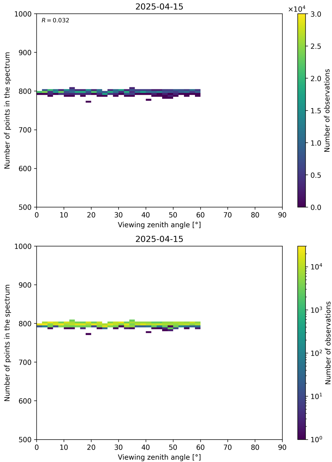
Figure 114: Scatter density plot of “Viewing zenith angle” against “Number of points in the spectrum” for 2025-04-14 to 2025-04-16.
