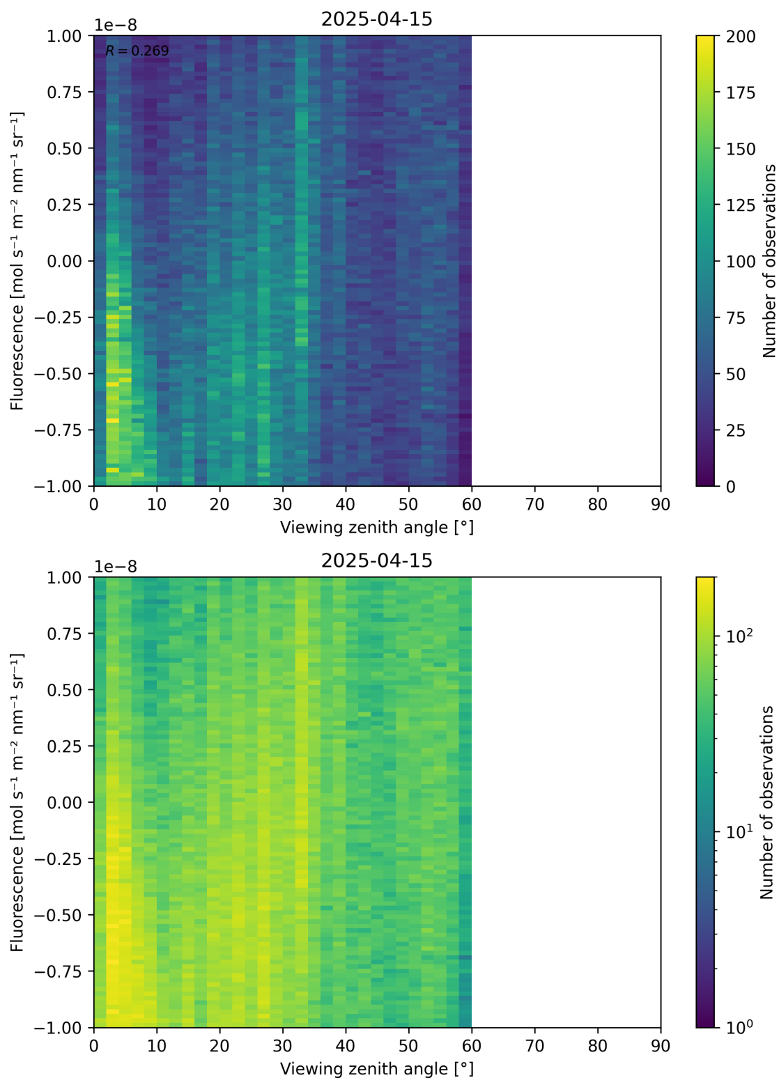
Figure 108: Scatter density plot of “Viewing zenith angle” against “Fluorescence” for 2025-04-14 to 2025-04-16.
