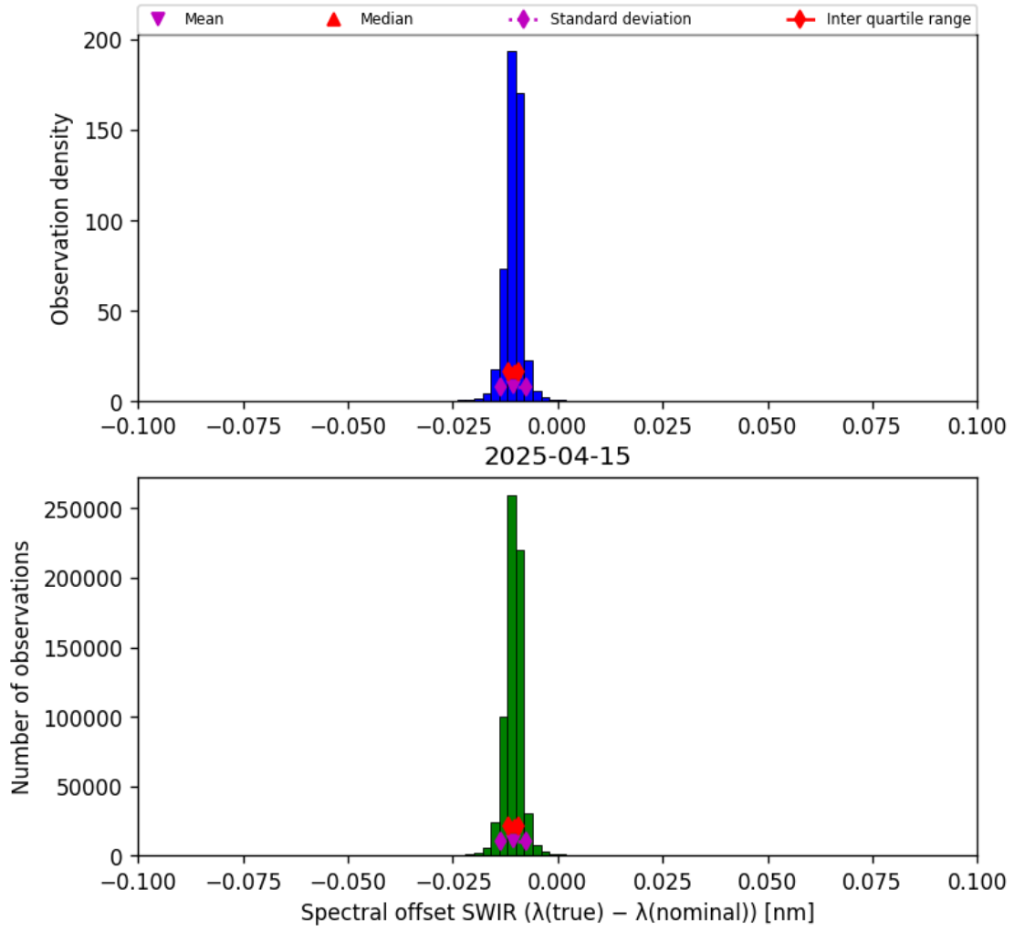
Figure 27: Histogram of “Spectral offset SWIR ( \lambda_{\text{true}} - \lambda_{\text{nominal}} )” for 2025-04-14 to 2025-04-16
