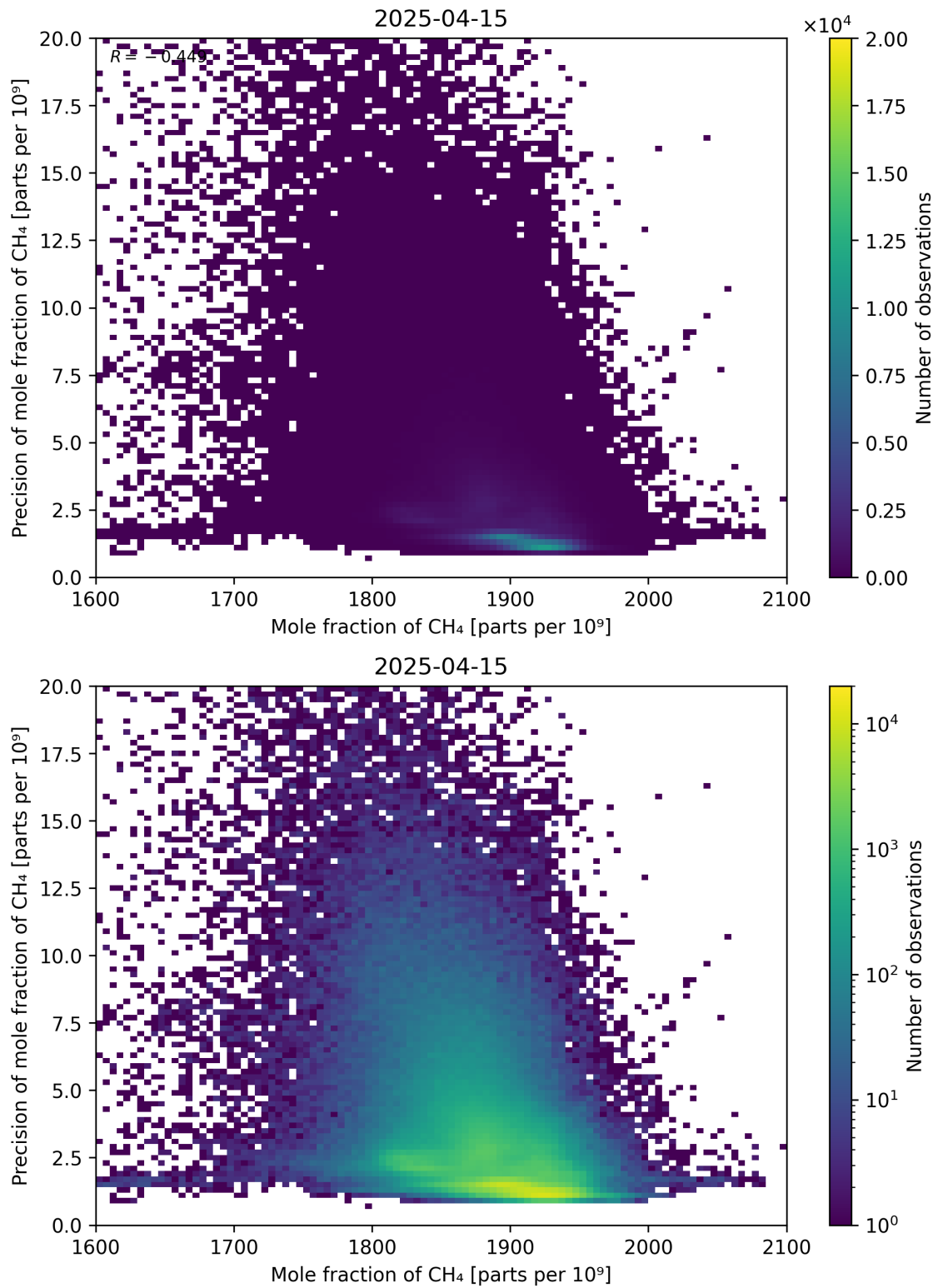
Figure 75: Scatter density plot of “Mole fraction of CH 4 ” against “Precision of mole fraction of CH 4 ” for 2025-04-14 to 2025-04-16.
