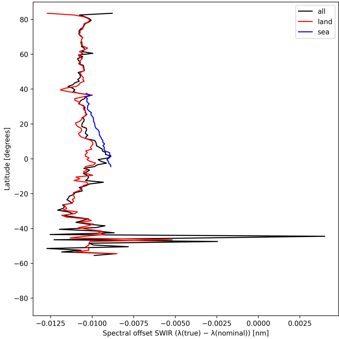
Figure 16: Zonal average of “Spectral offset SWIR ( \lambda_{\text{true}} - \lambda_{\text{nominal}} )” for 2025-04-14 to 2025-04-16.
