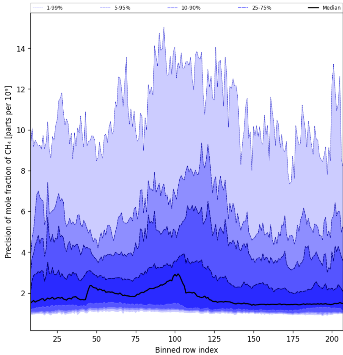
Figure 35: Along track statistics of “Precision of mole fraction of CH 4 ” for 2025-04-14 to 2025-04-16
