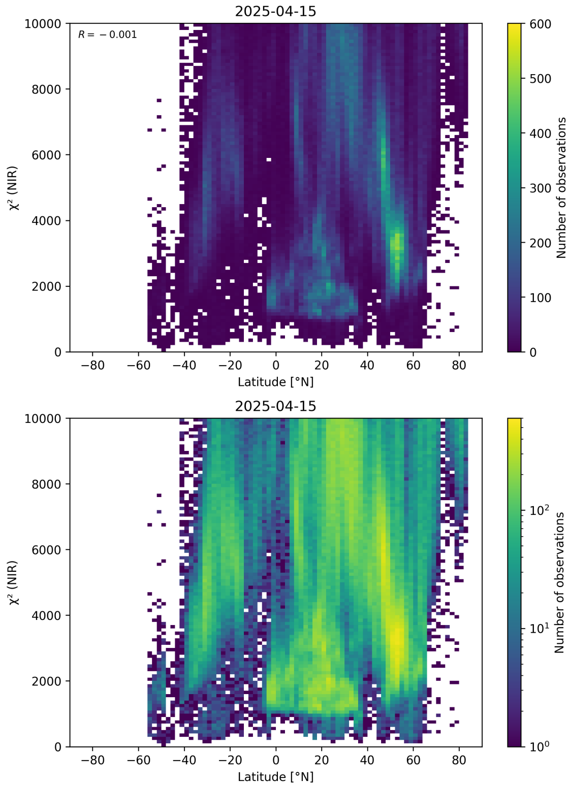
Figure 53: Scatter density plot of “Latitude” against “ \chi^2 (NIR)” for 2025-04-14 to 2025-04-16.
