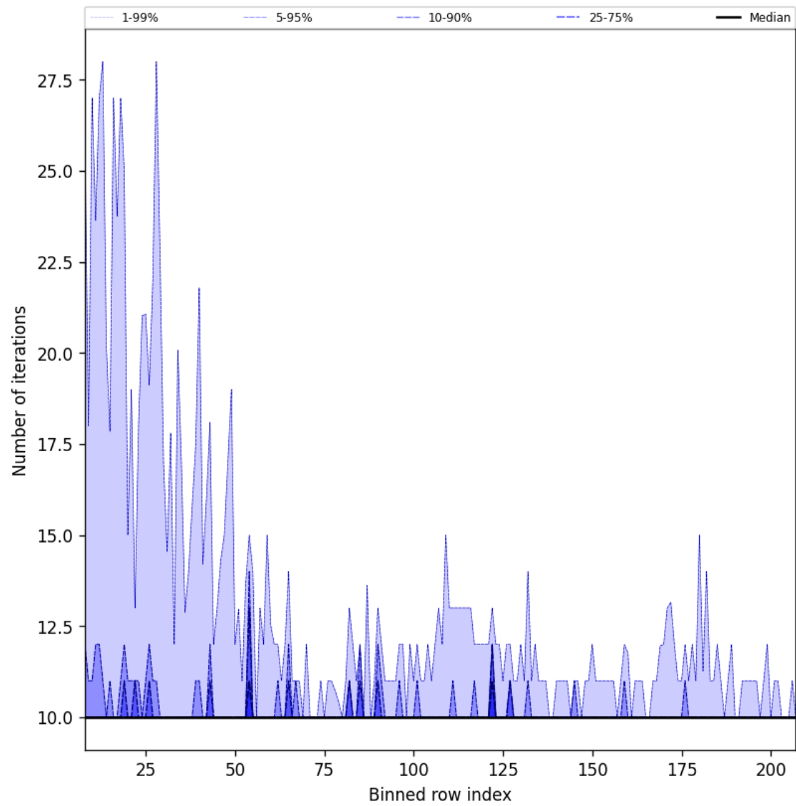
Figure 42: Along track statistics of “Number of iterations” for 2025-04-14 to 2025-04-16
