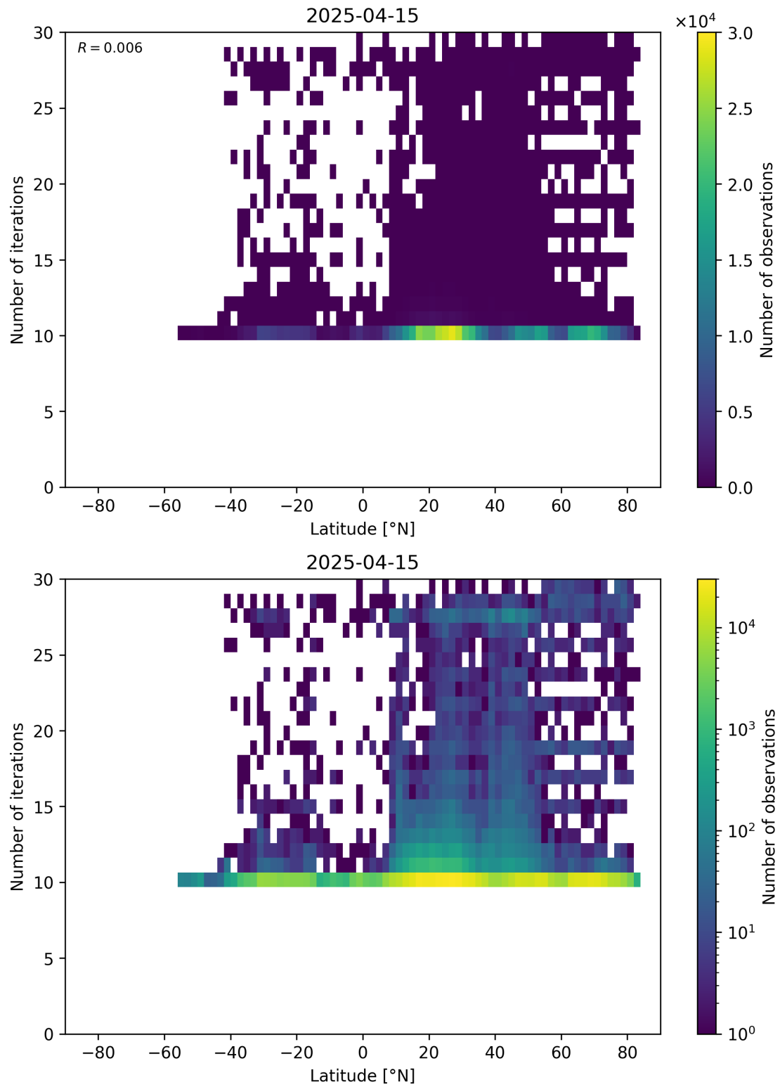
Figure 60: Scatter density plot of “Latitude” against “Number of iterations” for 2025-04-14 to 2025-04-16.
