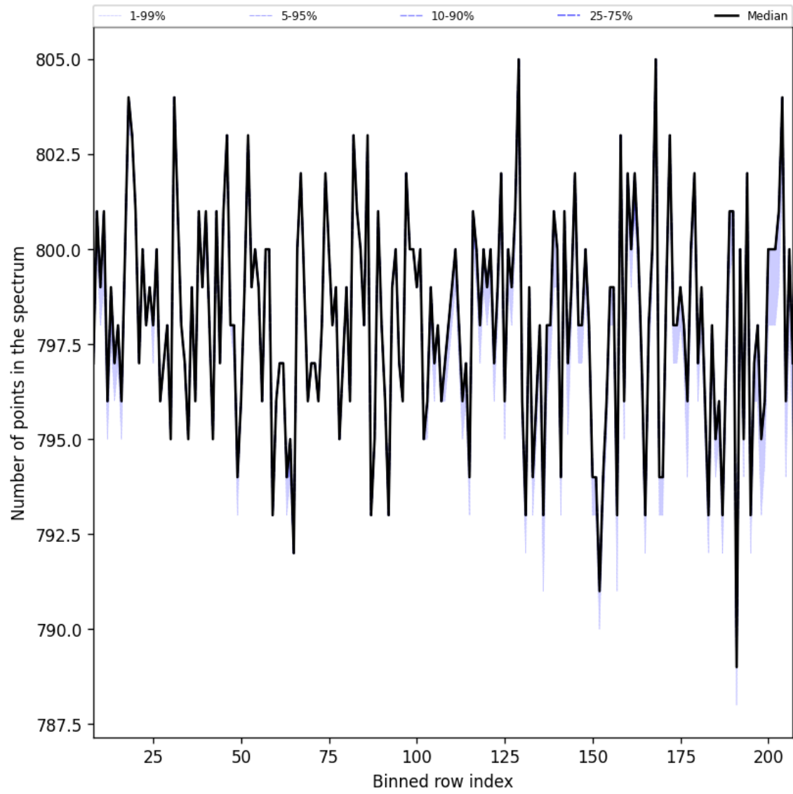
Figure 37: Along track statistics of “Number of points in the spectrum” for 2025-04-14 to 2025-04-16
