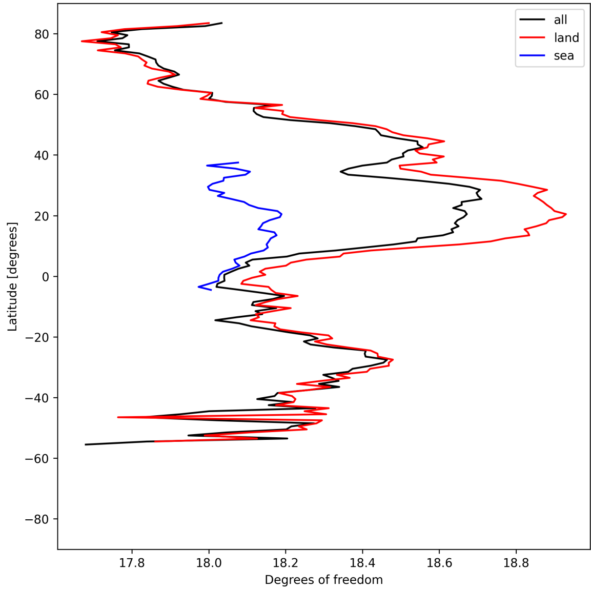
Figure 19: Zonal average of “Degrees of freedom” for 2025-04-14 to 2025-04-16.
