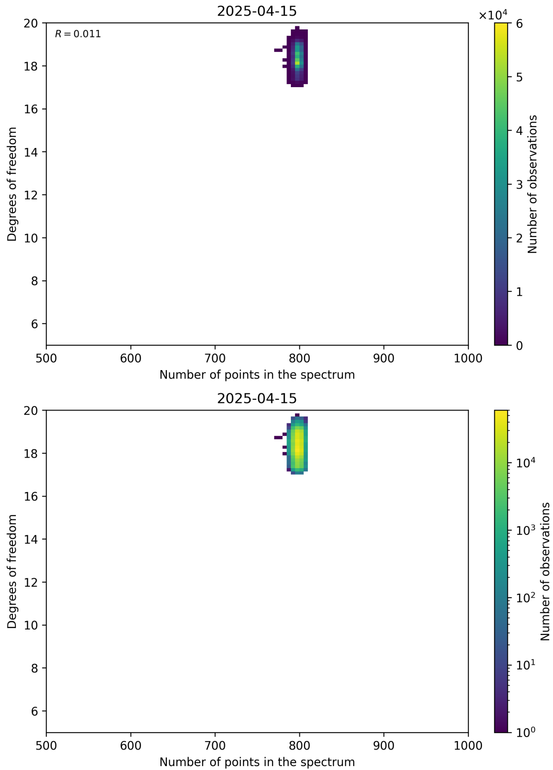
Figure 90: Scatter density plot of “Number of points in the spectrum” against “Degrees of freedom” for 2025-04-14 to 2025-04-16.
