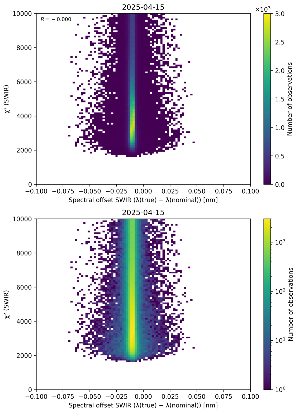
Figure 118: Scatter density plot of “Spectral offset SWIR ( \lambda_{\text{true}} - \lambda_{\text{nominal}} )” against “ \chi^2 (SWIR)” for 2025-04-14 to 2025-04-16.
