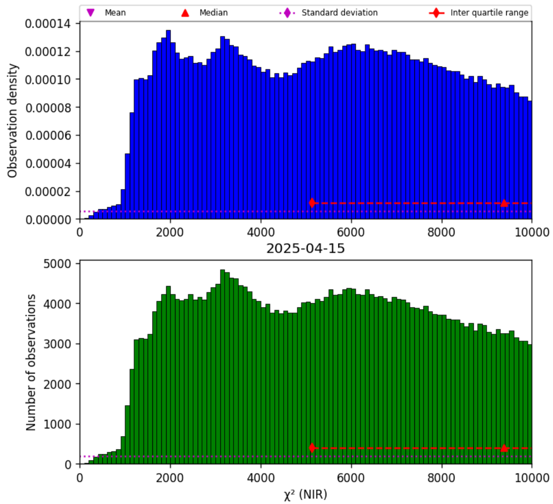
Figure 29: Histogram of “ \chi^2 (NIR)” for 2025-04-14 to 2025-04-16
