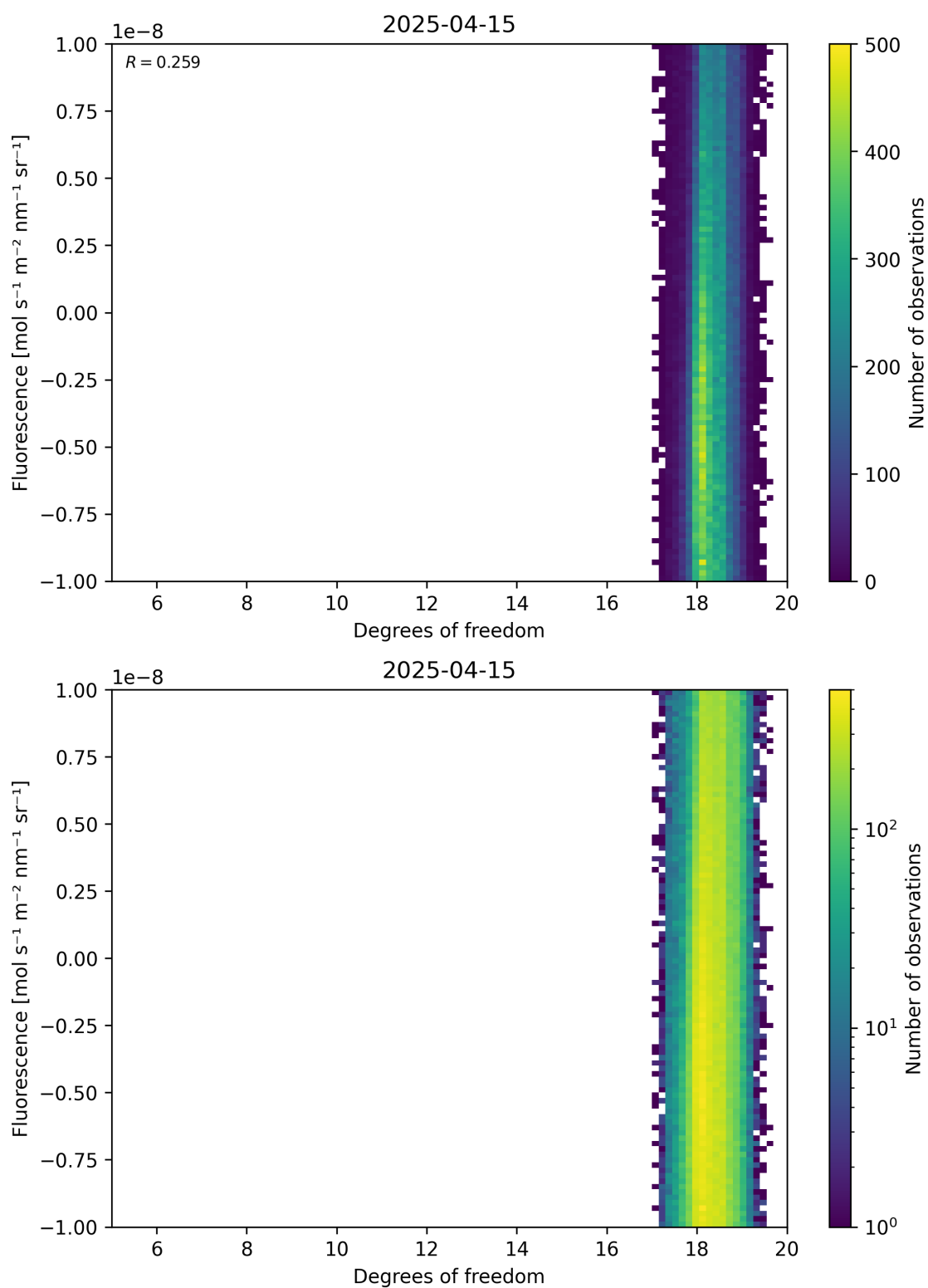
Figure 51: Scatter density plot of “Degrees of freedom” against “Fluorescence” for 2025-04-14 to 2025-04-16.
