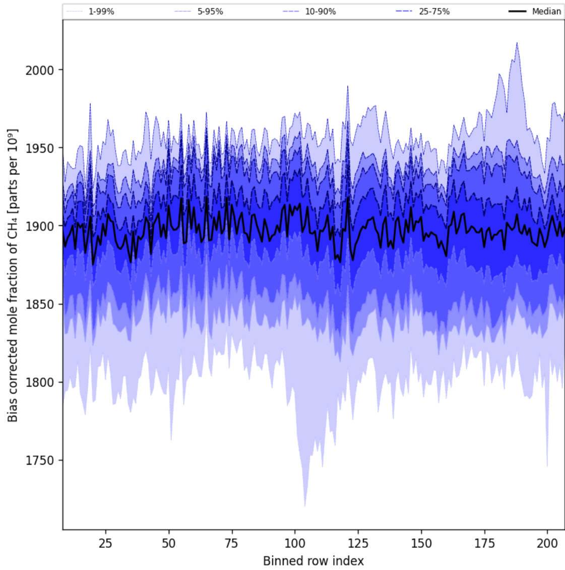
Figure 36: Along track statistics of “Bias corrected mole fraction of CH 4 ” for 2025-04-14 to 2025-04-16
