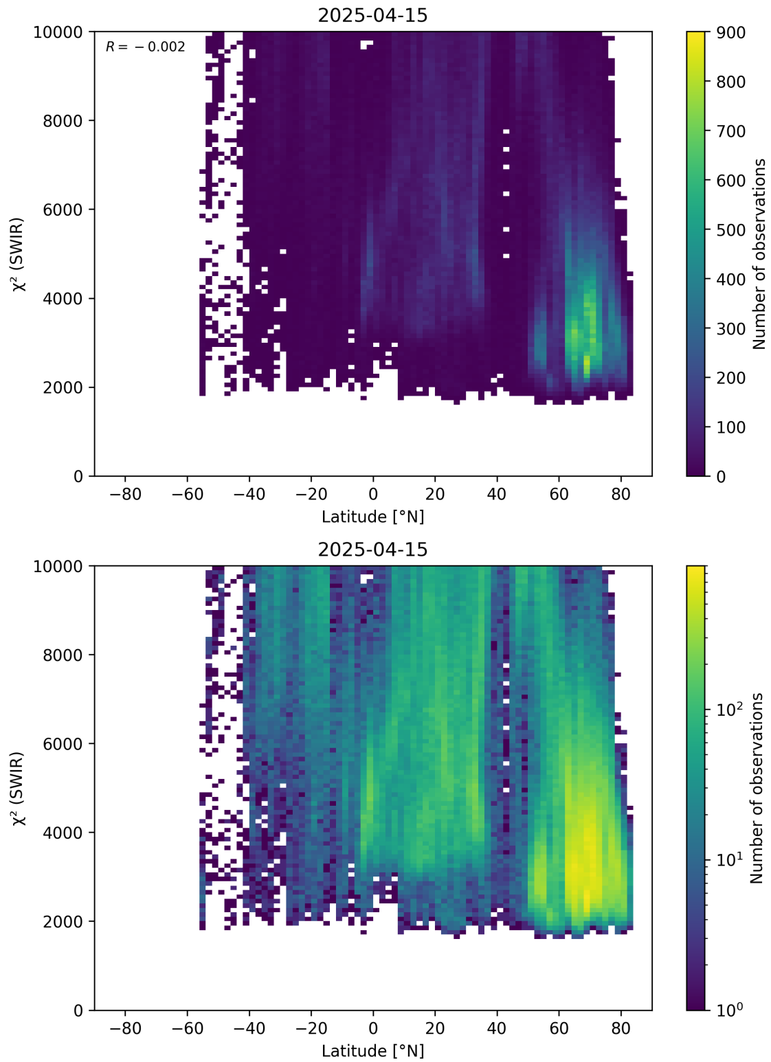
Figure 54: Scatter density plot of “Latitude” against “ \chi^2 (SWIR)” for 2025-04-14 to 2025-04-16.
