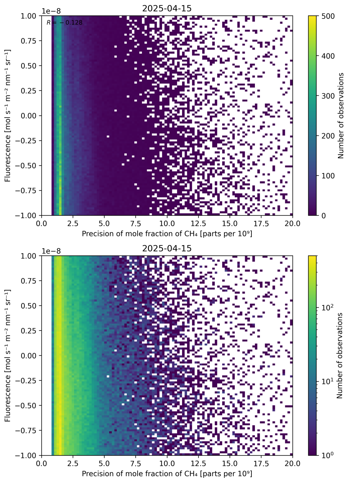
Figure 81: Scatter density plot of “Precision of mole fraction of CH 4 ” against “Fluorescence” for 2025-04-14 to 2025-04-16.
