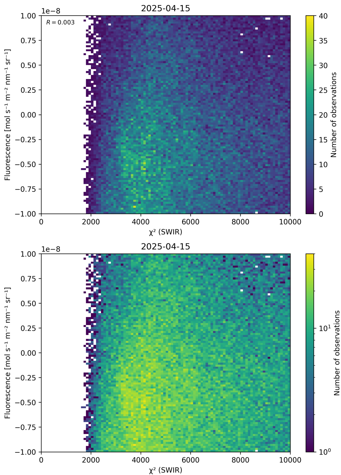
Figure 49: Scatter density plot of “ \chi^2 (SWIR)” against “Fluorescence” for 2025-04-14 to 2025-04-16.
