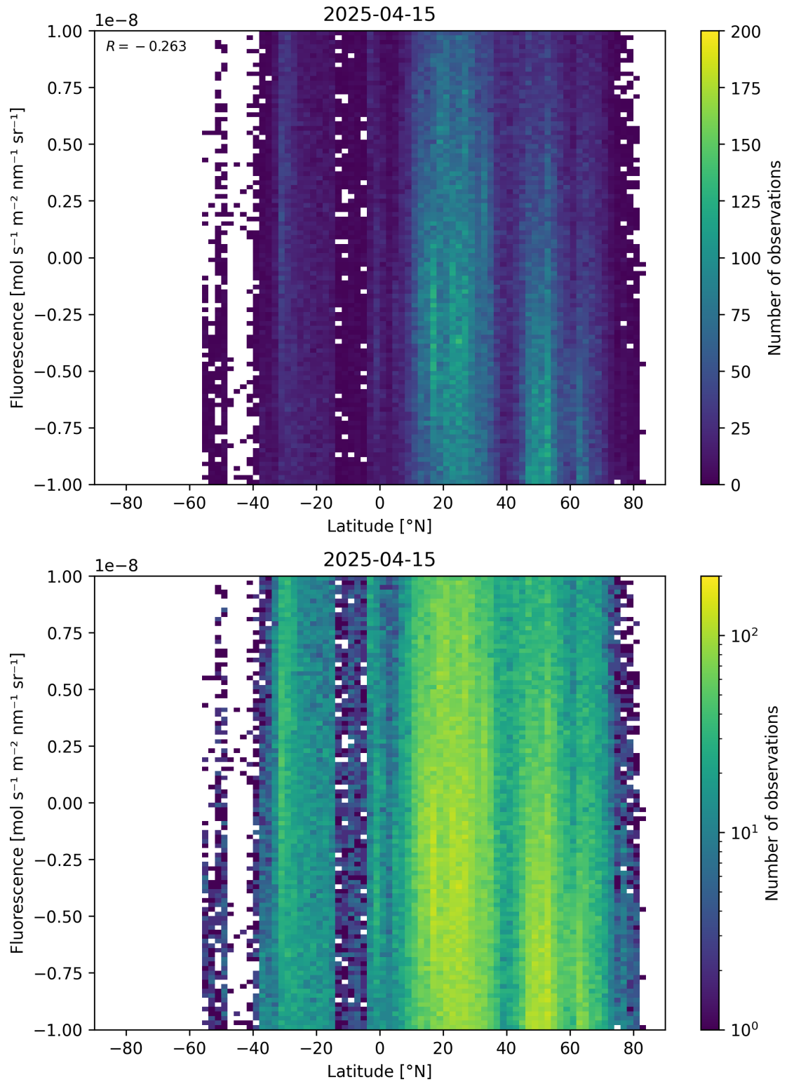
Figure 56: Scatter density plot of “Latitude” against “Fluorescence” for 2025-04-14 to 2025-04-16.
