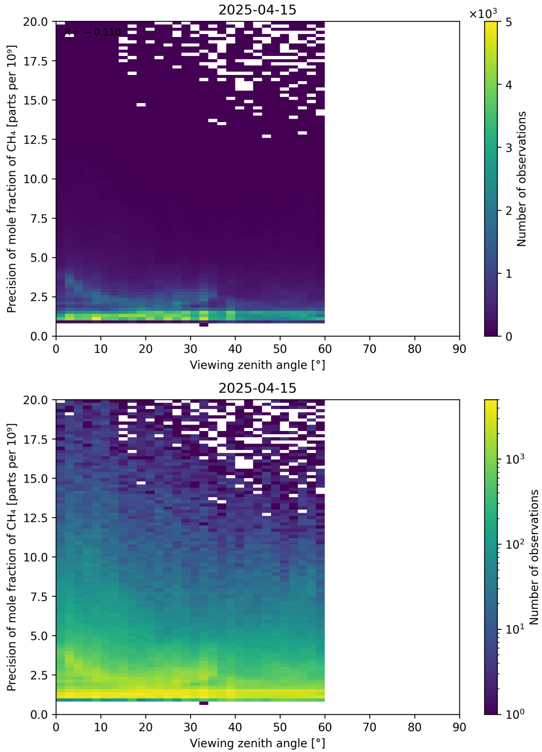
Figure 112: Scatter density plot of “Viewing zenith angle” against “Precision of mole fraction of CH 4 ” for 2025-04-14 to 2025-04-16.
