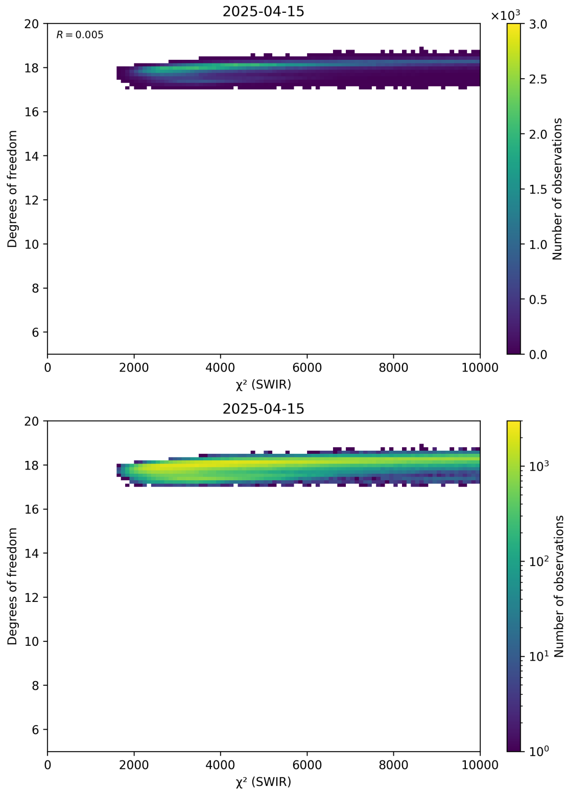
Figure 48: Scatter density plot of “ \chi^2 (SWIR)” against “Degrees of freedom” for 2025-04-14 to 2025-04-16.
