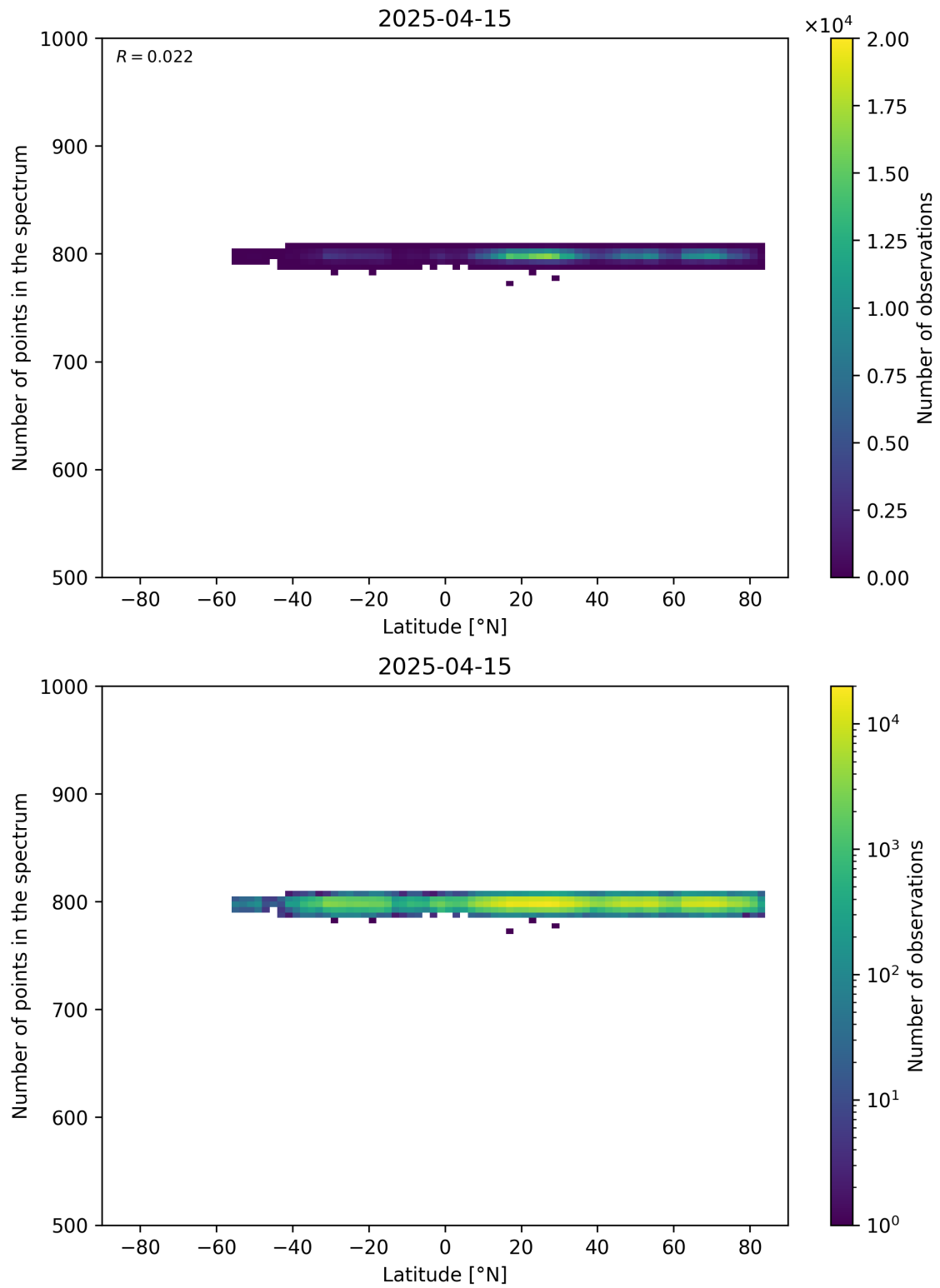
Figure 61: Scatter density plot of “Latitude” against “Number of points in the spectrum” for 2025-04-14 to 2025-04-16.
