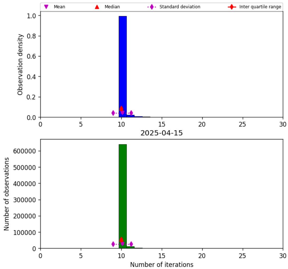
Figure 31: Histogram of “Number of iterations” for 2025-04-14 to 2025-04-16
