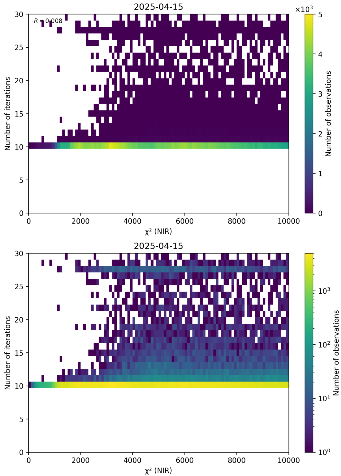
Figure 46: Scatter density plot of “ \chi^2 (NIR)” against “Number of iterations” for 2025-04-14 to 2025-04-16.
