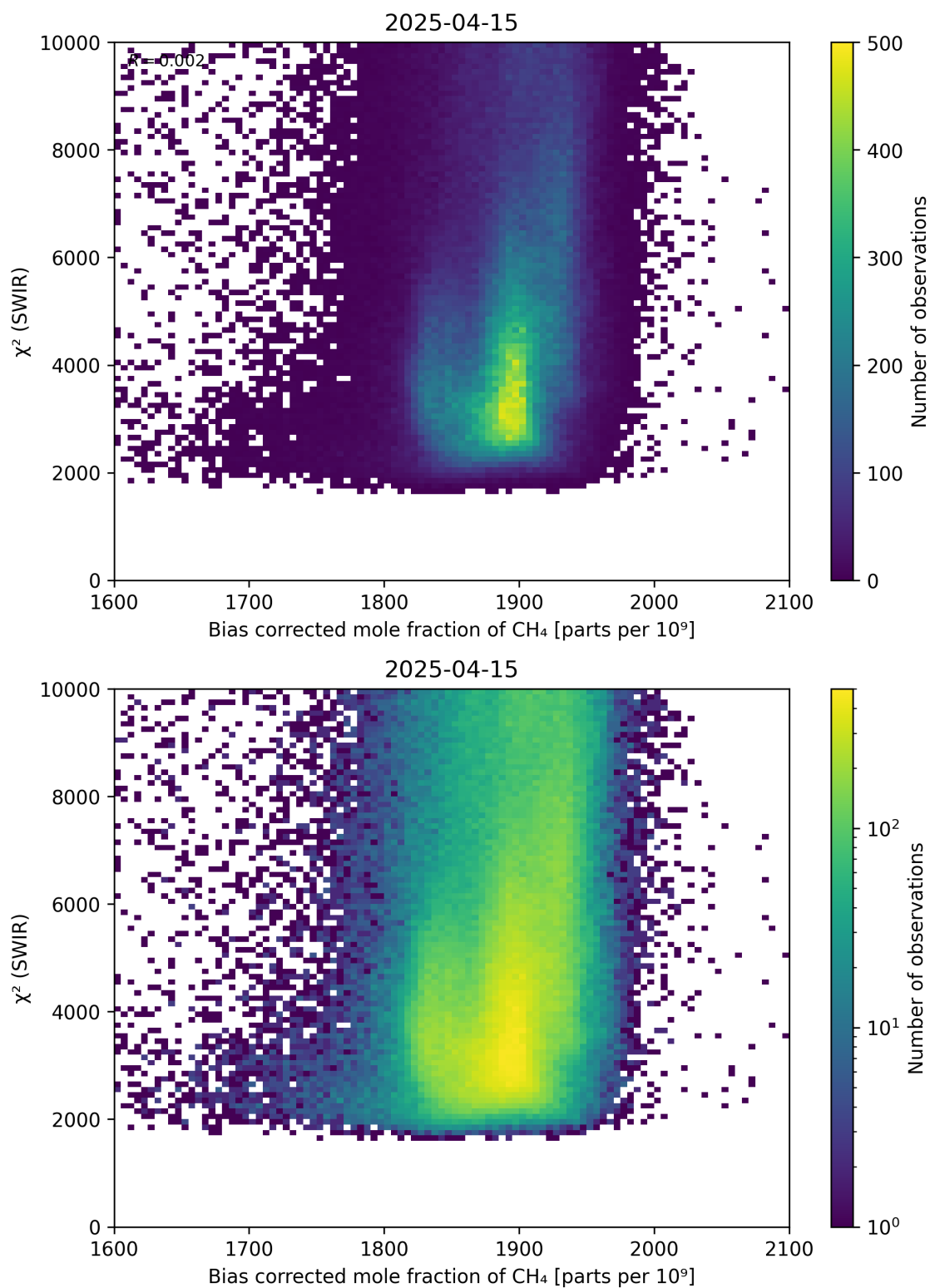
Figure 64: Scatter density plot of “Bias corrected mole fraction of CH 4 ” against “ \chi^2 (SWIR)” for 2025-04-14 to 2025-04-16.
