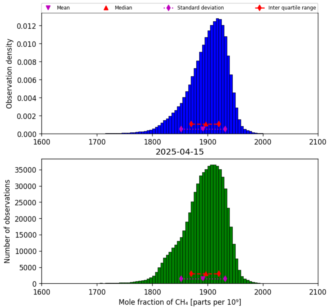
Figure 23: Histogram of “Mole fraction of CH 4 ” for 2025-04-14 to 2025-04-16
