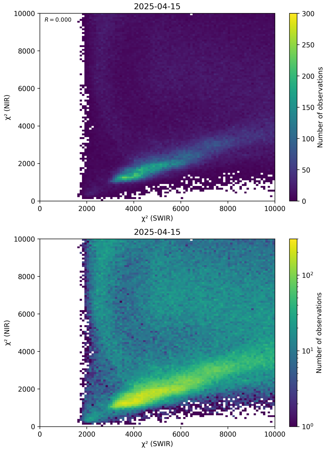
Figure 47: Scatter density plot of “ \chi^2 (SWIR)” against “ \chi^2 (NIR)” for 2025-04-14 to 2025-04-16.
