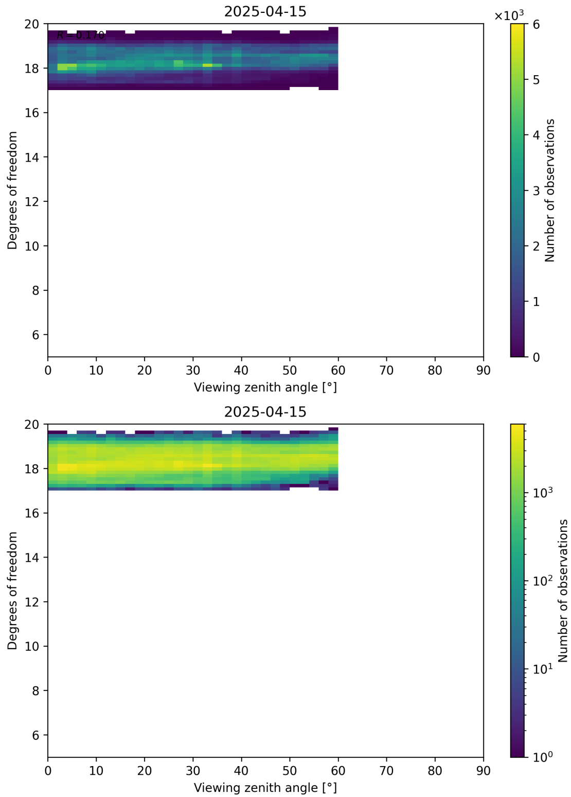
Figure 107: Scatter density plot of “Viewing zenith angle” against “Degrees of freedom” for 2025-04-14 to 2025-04-16.
