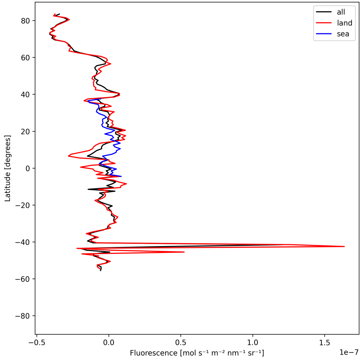
Figure 21: Zonal average of “Fluorescence” for 2025-04-14 to 2025-04-16.
