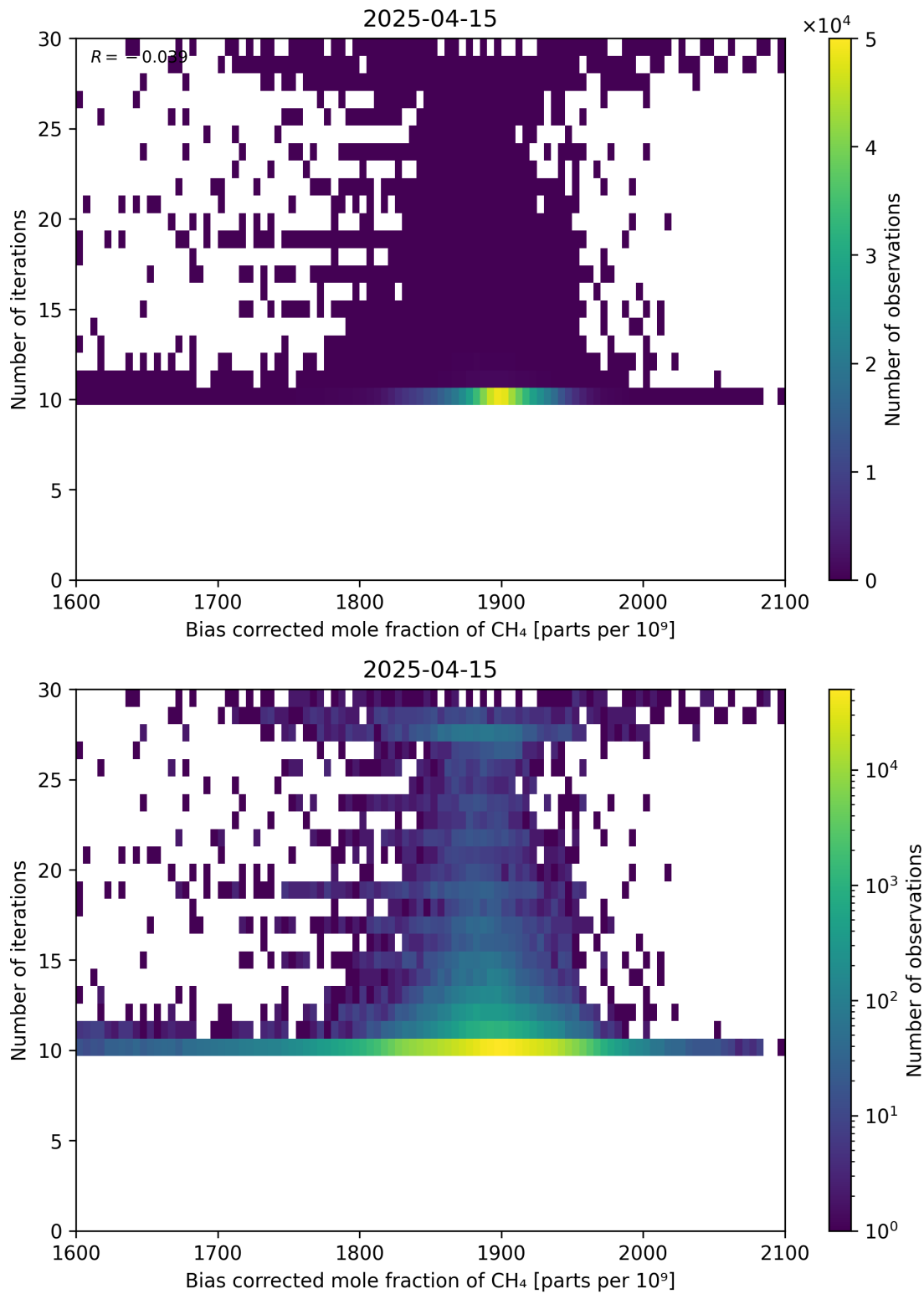
Figure 67: Scatter density plot of “Bias corrected mole fraction of \text{CH}_4 ” against “Number of iterations” for 2025-04-14 to 2025-04-16.
