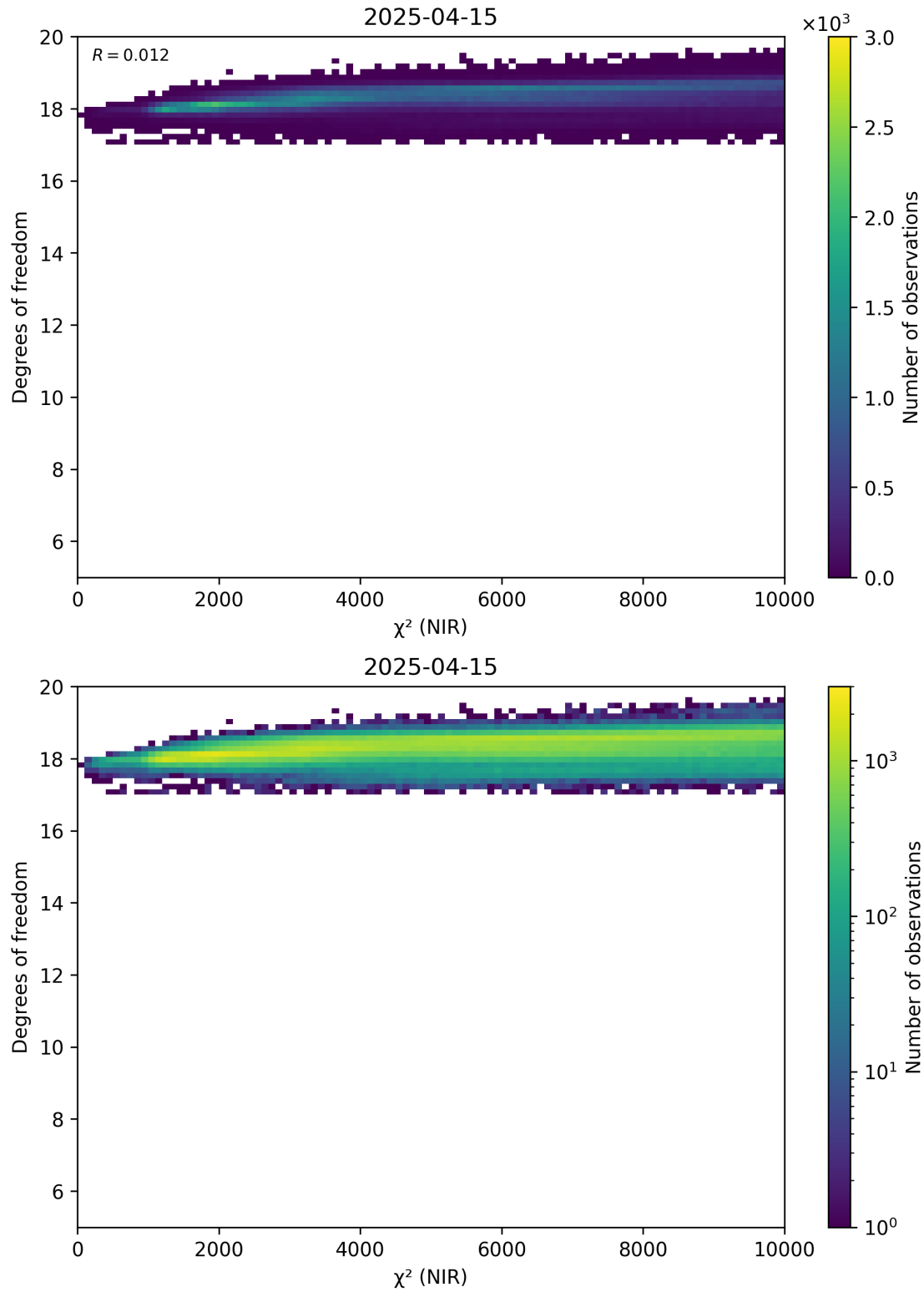
Figure 44: Scatter density plot of “ \chi^2 (NIR)” against “Degrees of freedom” for 2025-04-14 to 2025-04-16.
