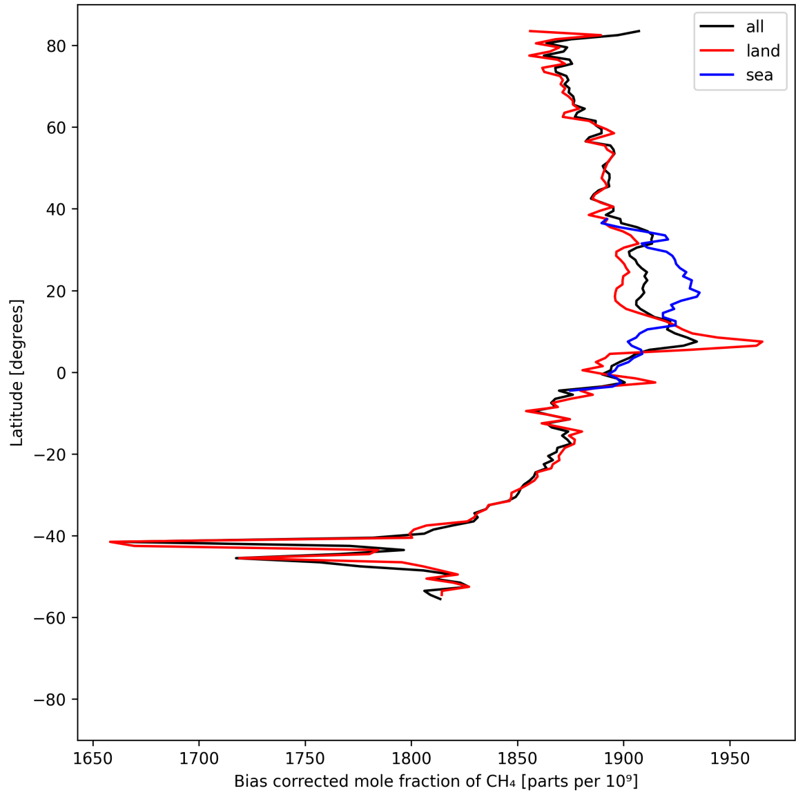
Figure 14: Zonal average of “Bias corrected mole fraction of \text{CH}_4 ” for 2025-04-14 to 2025-04-16.
