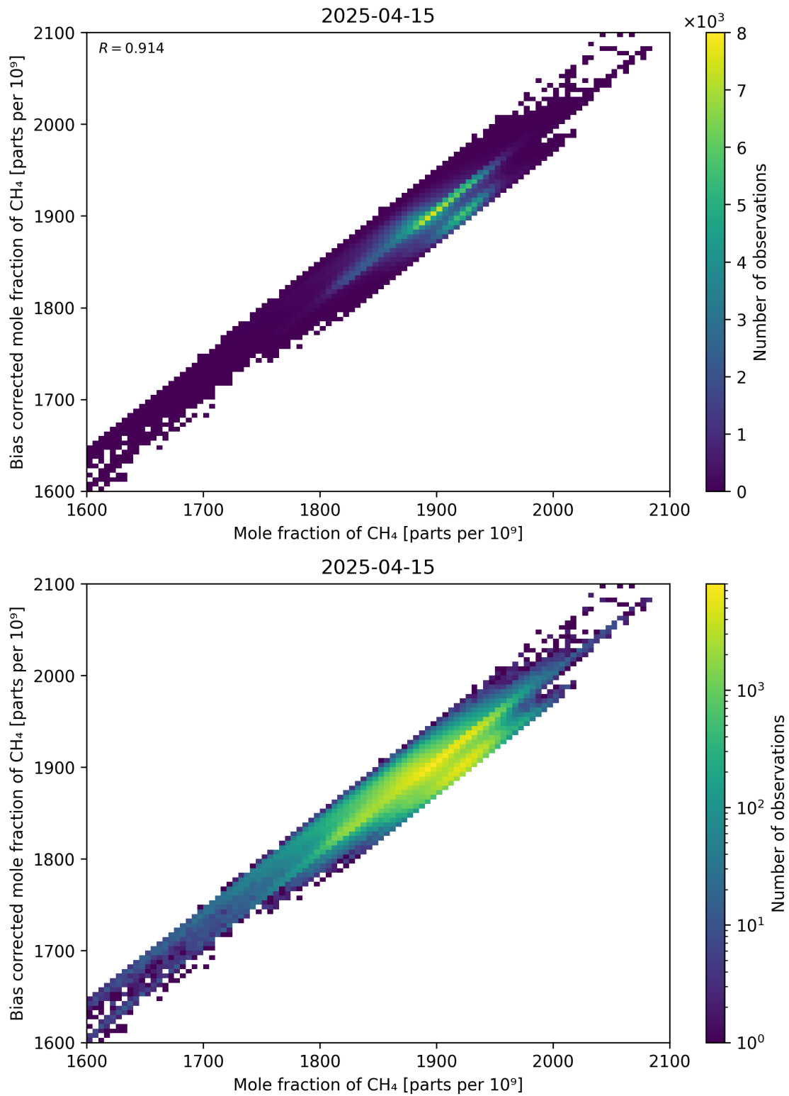
Figure 74: Scatter density plot of “Mole fraction of CH 4 ” against “Bias corrected mole fraction of CH 4 ” for 2025-04-14 to 2025-04-16.
