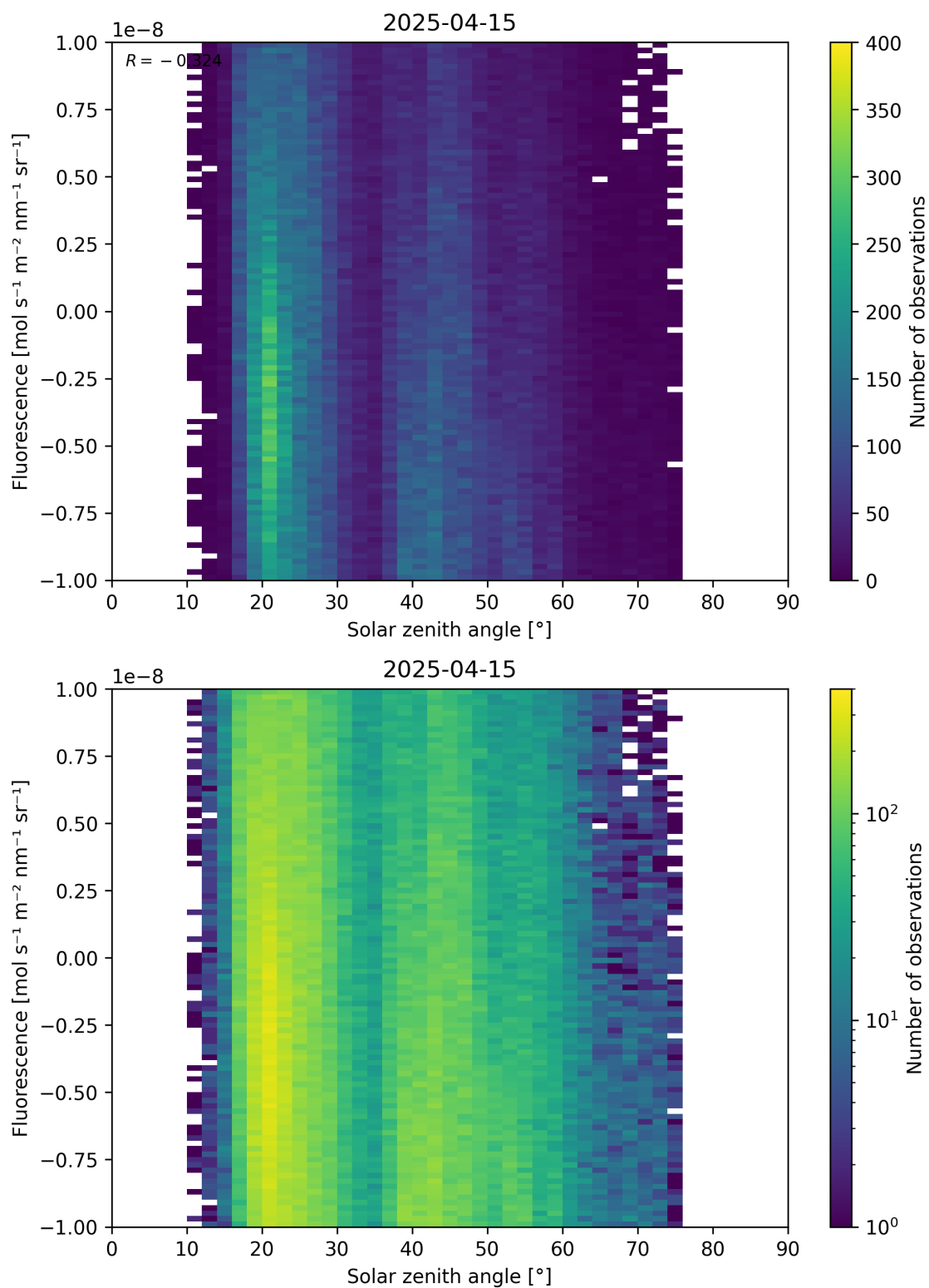
Figure 97: Scatter density plot of “Solar zenith angle” against “Fluorescence” for 2025-04-14 to 2025-04-16.
