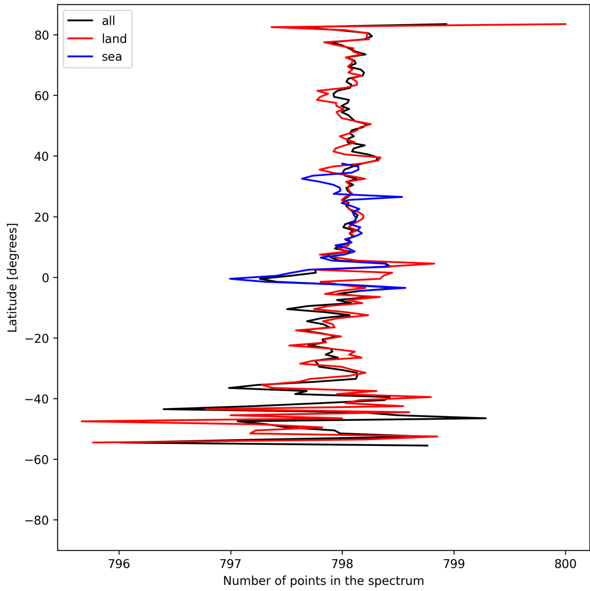
Figure 15: Zonal average of “Number of points in the spectrum” for 2025-04-14 to 2025-04-16.
