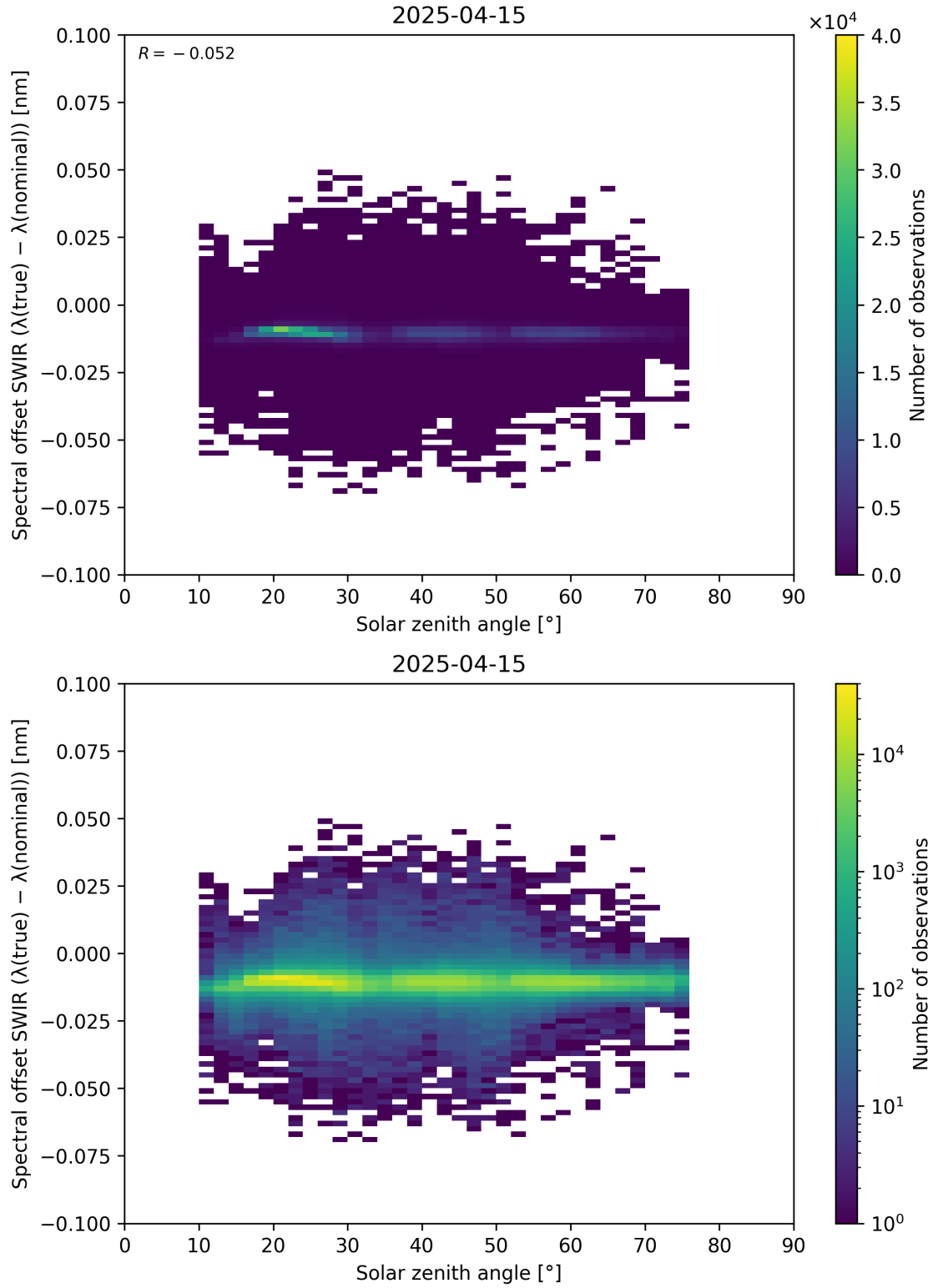
Figure 104: Scatter density plot of “Solar zenith angle” against “Spectral offset SWIR ( \lambda_{\text{true}} - \lambda_{\text{nominal}} )” for 2025-04-14 to 2025-04-16.
