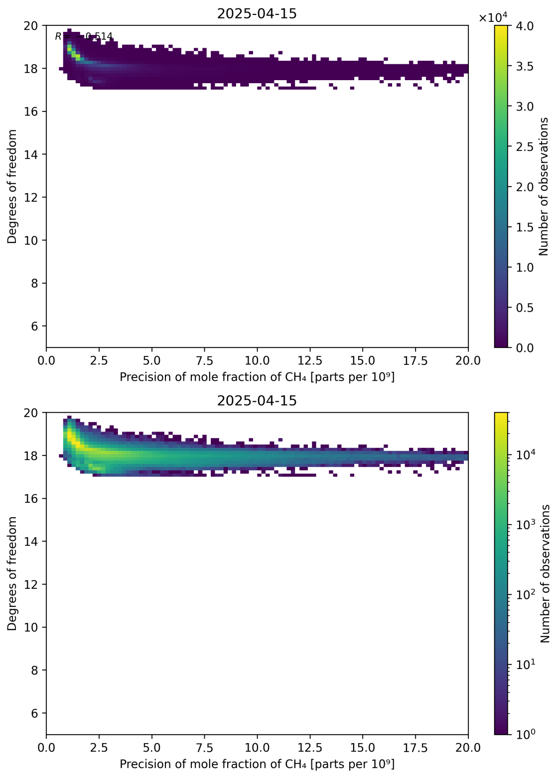
Figure 80: Scatter density plot of “Precision of mole fraction of CH 4 ” against “Degrees of freedom” for 2025-04-14 to 2025-04-16.
