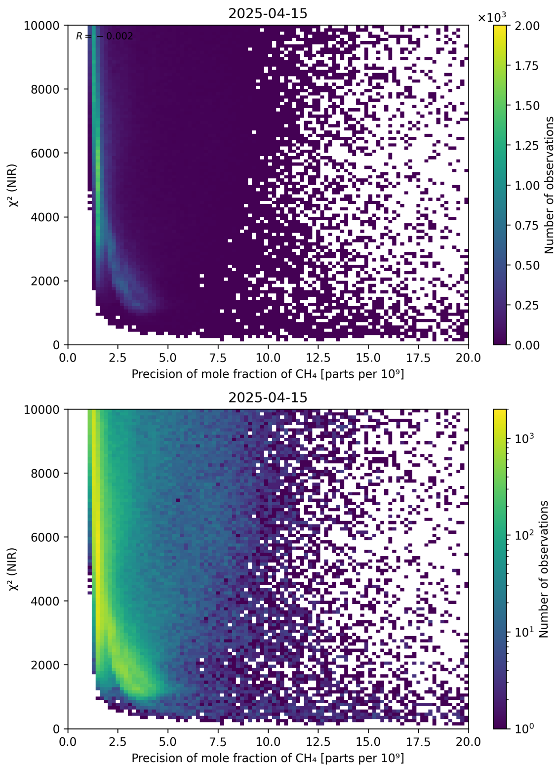
Figure 78: Scatter density plot of “Precision of mole fraction of CH 4 ” against “ \chi^2 (NIR)” for 2025-04-14 to 2025-04-16.
