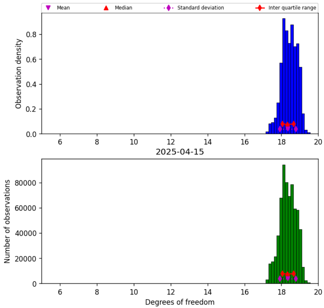
Figure 30: Histogram of “Degrees of freedom” for 2025-04-14 to 2025-04-16
