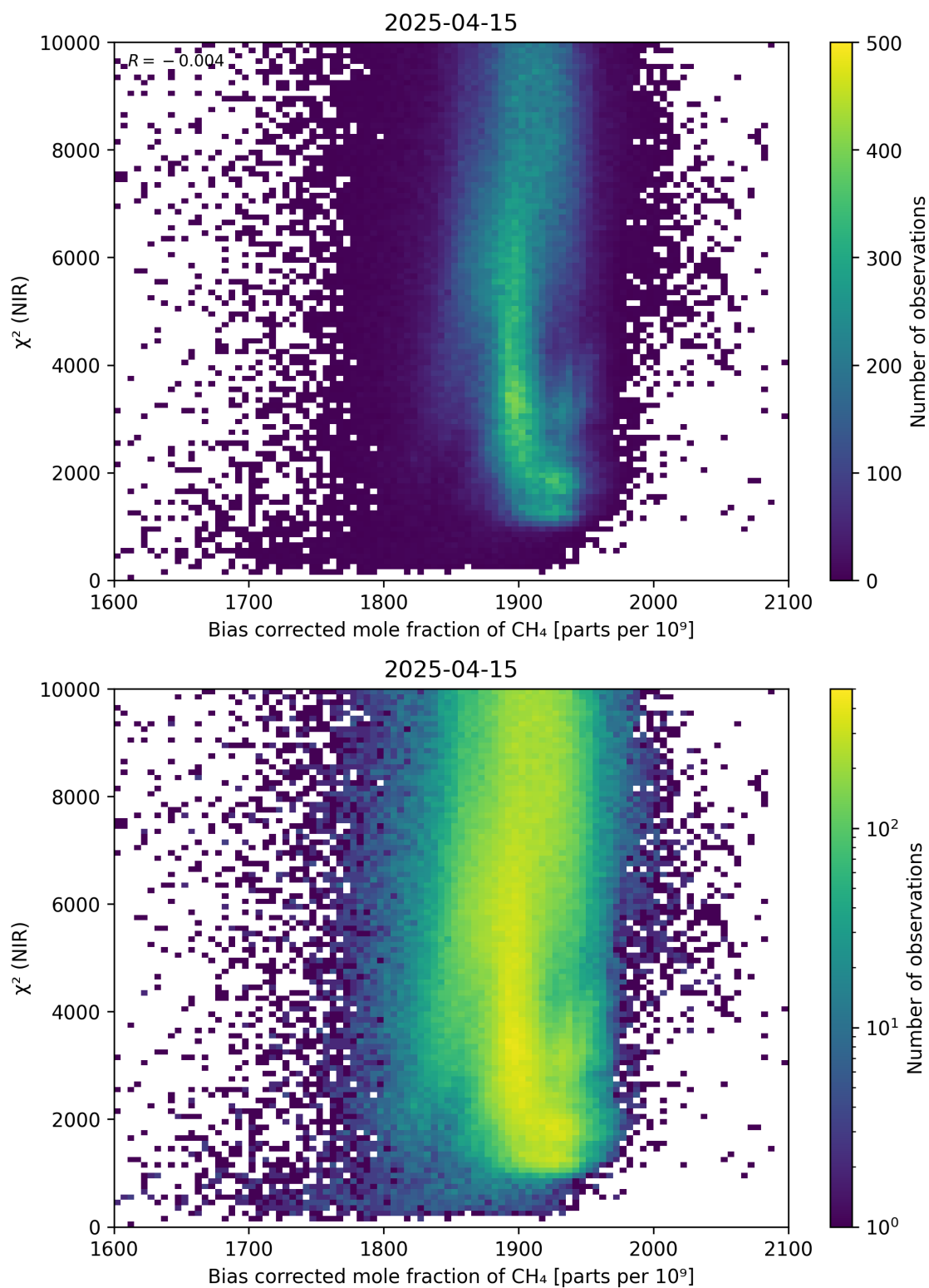
Figure 63: Scatter density plot of “Bias corrected mole fraction of \text{CH}_4 ” against “ \chi^2 (NIR)” for 2025-04-14 to 2025-04-16.
