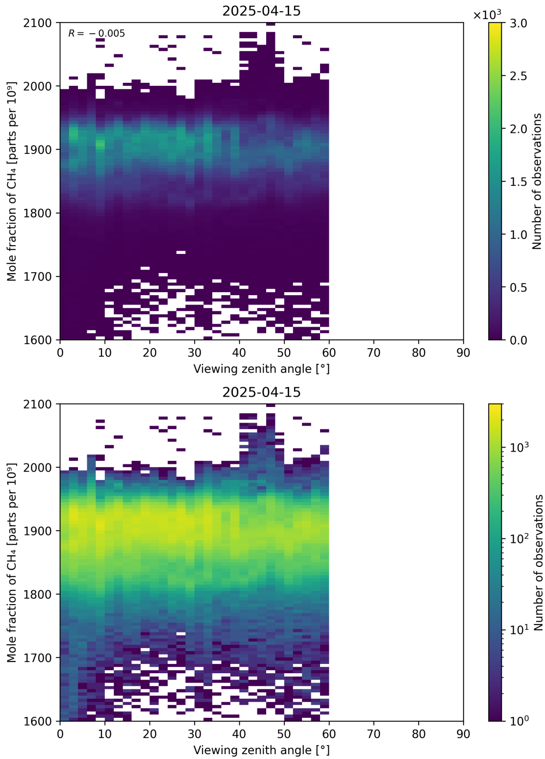
Figure 110: Scatter density plot of “Viewing zenith angle” against “Mole fraction of CH 4 ” for 2025-04-14 to 2025-04-16.
