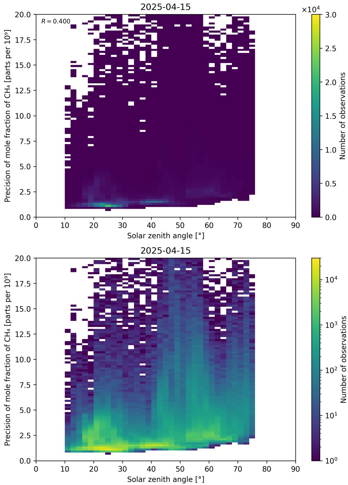
Figure 101: Scatter density plot of “Solar zenith angle” against “Precision of mole fraction of \text{CH}_4 ” for 2025-04-14 to 2025-04-16.
