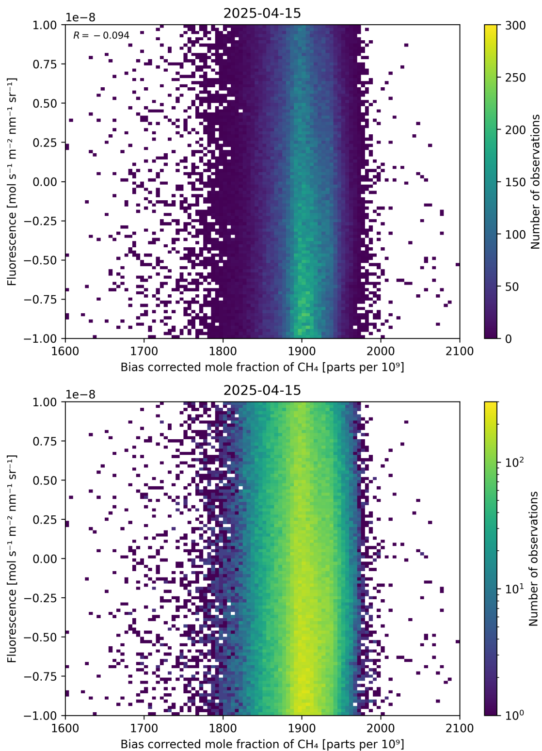
Figure 66: Scatter density plot of “Bias corrected mole fraction of \text{CH}_4 ” against “Fluorescence” for 2025-04-14 to 2025-04-16.
