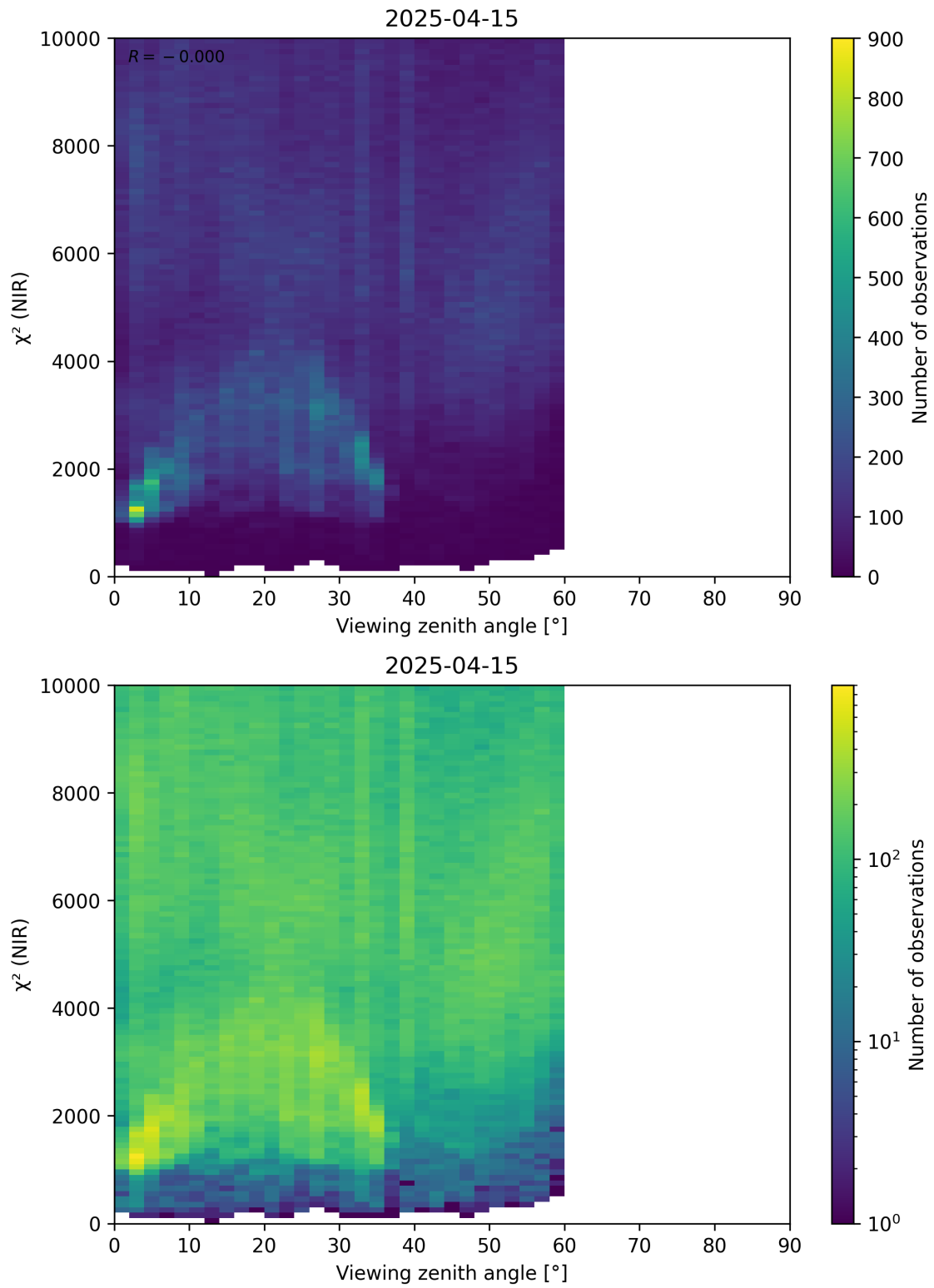
Figure 105: Scatter density plot of “Viewing zenith angle” against “ \chi^2 (NIR)” for 2025-04-14 to 2025-04-16.
