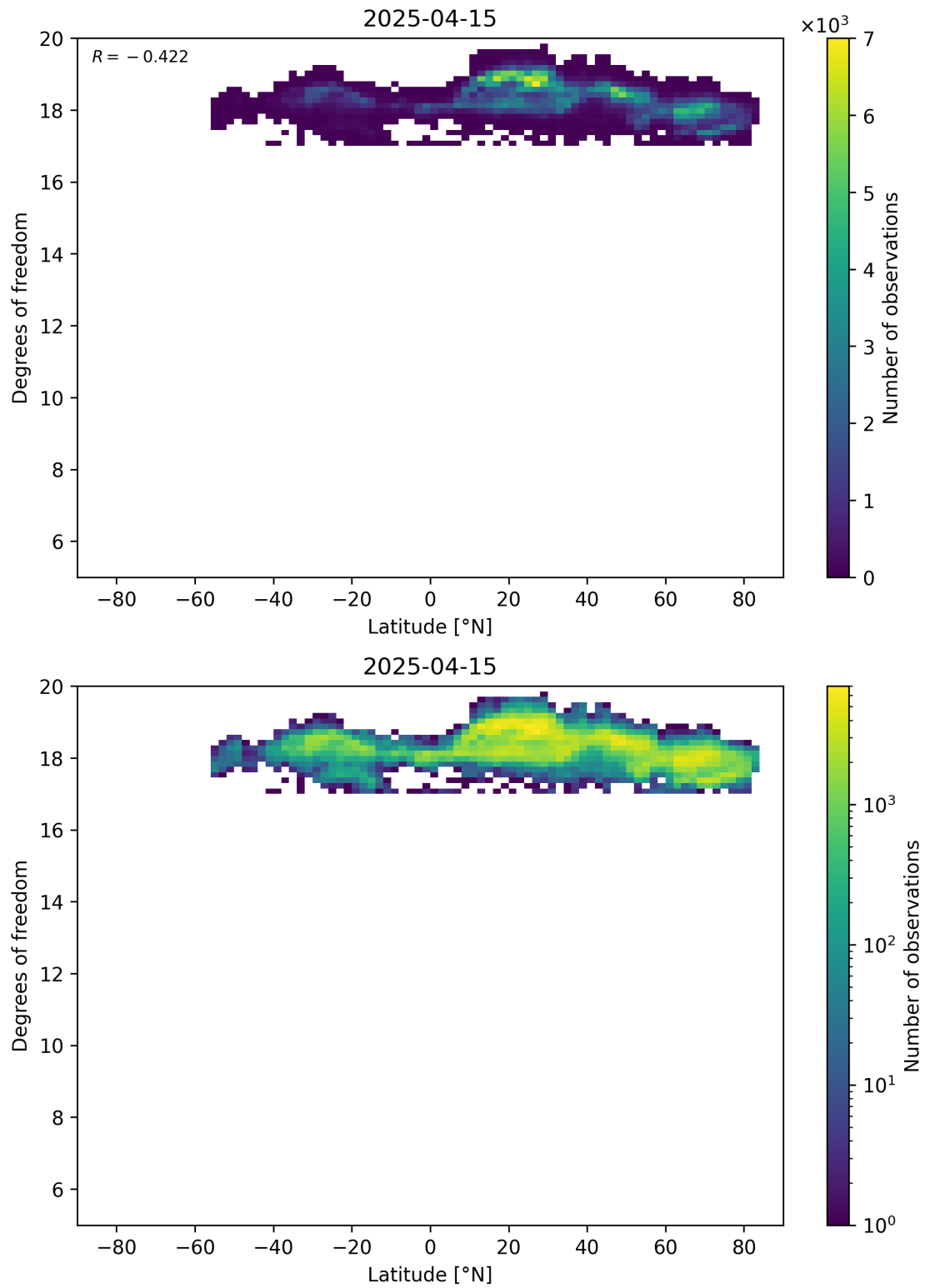
Figure 55: Scatter density plot of “Latitude” against “Degrees of freedom” for 2025-04-14 to 2025-04-16.
