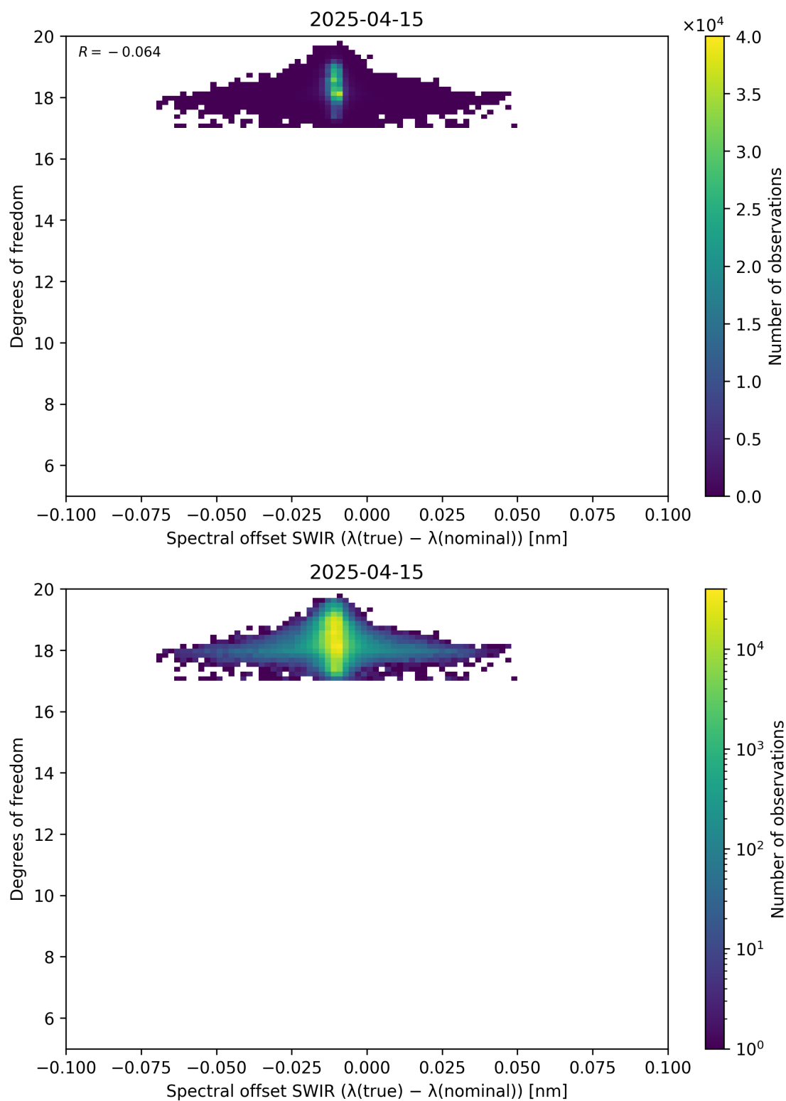
Figure 119: Scatter density plot of “Spectral offset SWIR ( \lambda_{\text{true}} - \lambda_{\text{nominal}} )” against “Degrees of freedom” for 2025-04-14 to 2025-04-16.
