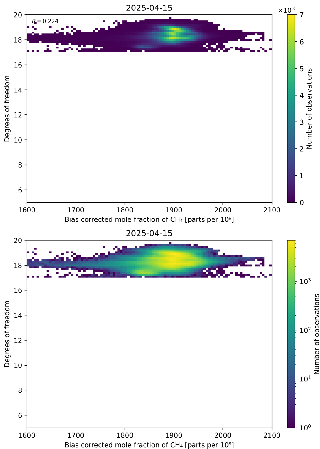
Figure 65: Scatter density plot of “Bias corrected mole fraction of CH 4 ” against “Degrees of freedom” for 2025-04-14 to 2025-04-16.
