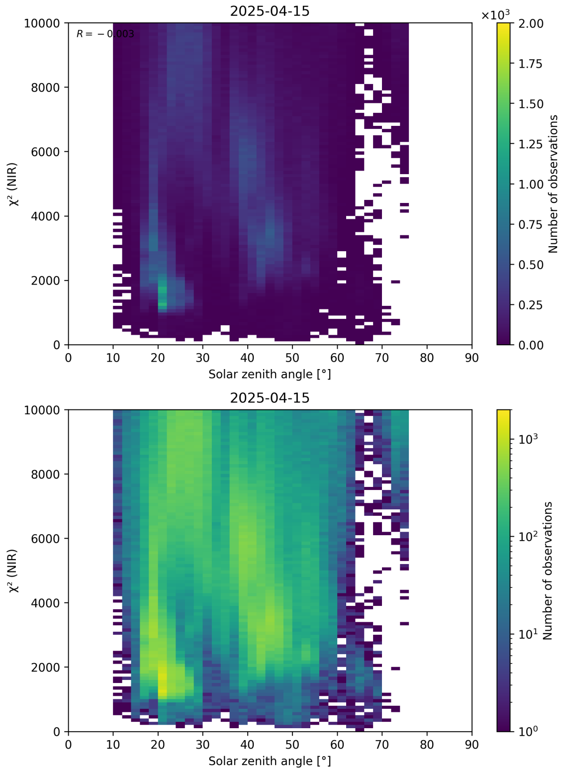
Figure 94: Scatter density plot of “Solar zenith angle” against “ \chi^2 (NIR)” for 2025-04-14 to 2025-04-16.
