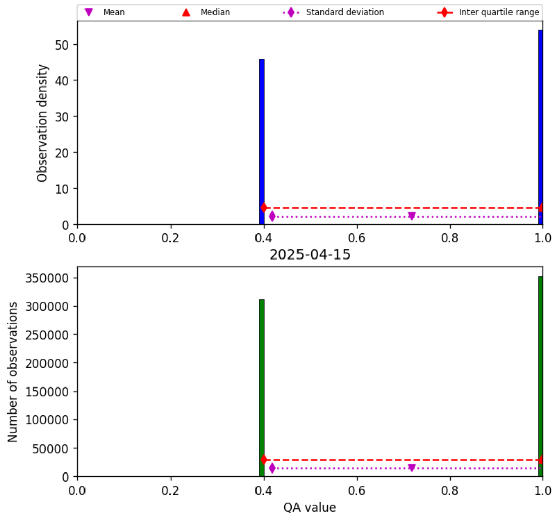
Figure 22: Histogram of “QA value” for 2025-04-14 to 2025-04-16
