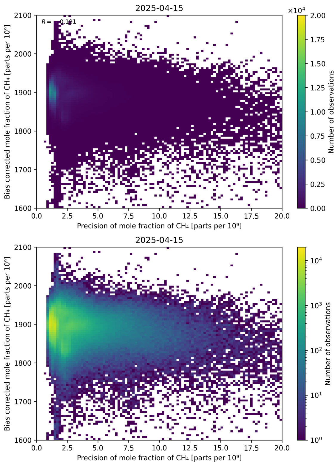
Figure 82: Scatter density plot of “Precision of mole fraction of \text{CH}_4 ” against “Bias corrected mole fraction of \text{CH}_4 ” for 2025-04-14 to 2025-04-16.
