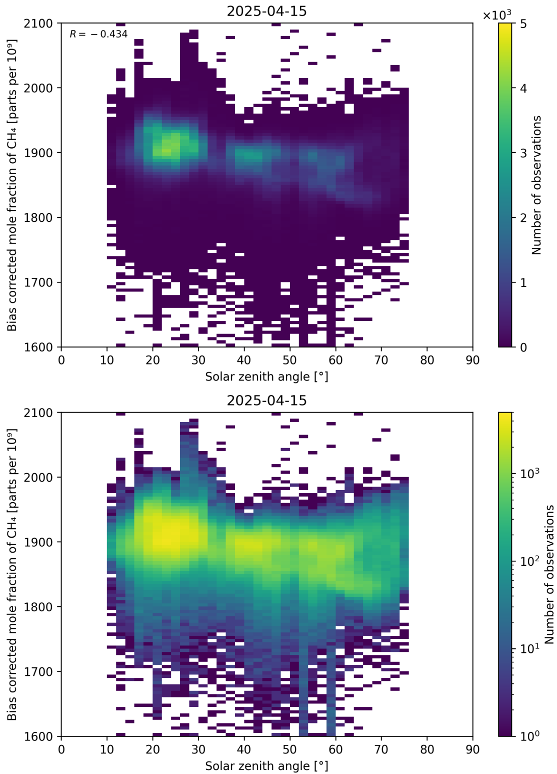
Figure 100: Scatter density plot of “Solar zenith angle” against “Bias corrected mole fraction of \text{CH}_4 ” for 2025-04-14 to 2025-04-16.
