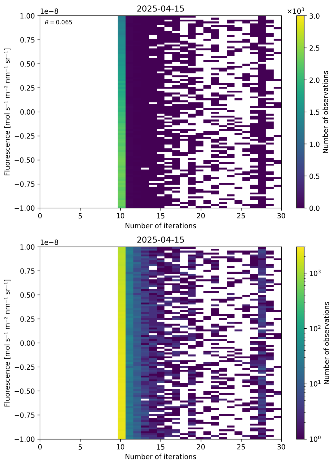
Figure 87: Scatter density plot of “Number of iterations” against “Fluorescence” for 2025-04-14 to 2025-04-16.
