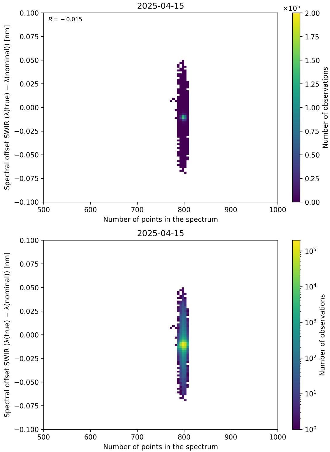
Figure 93: Scatter density plot of “Number of points in the spectrum” against “Spectral offset SWIR ( \lambda_{\text{true}} - \lambda_{\text{nominal}} )” for 2025-04-14 to 2025-04-16.
