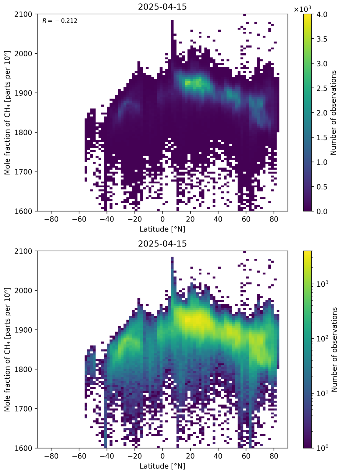
Figure 57: Scatter density plot of “Latitude” against “Mole fraction of \text{CH}_4 ” for 2025-04-14 to 2025-04-16.
