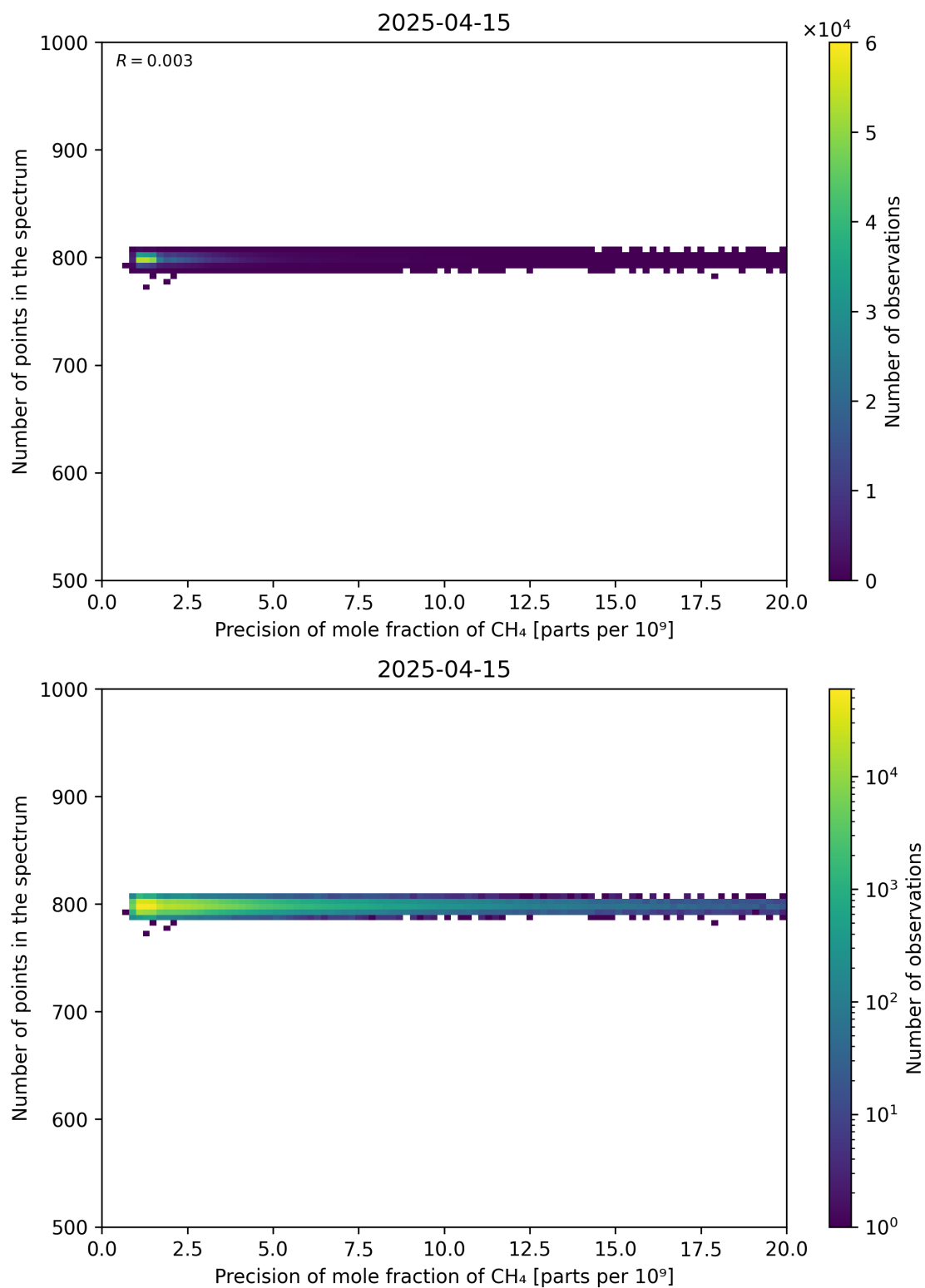
Figure 84: Scatter density plot of “Precision of mole fraction of CH 4 ” against “Number of points in the spectrum” for 2025-04-14 to 2025-04-16.
