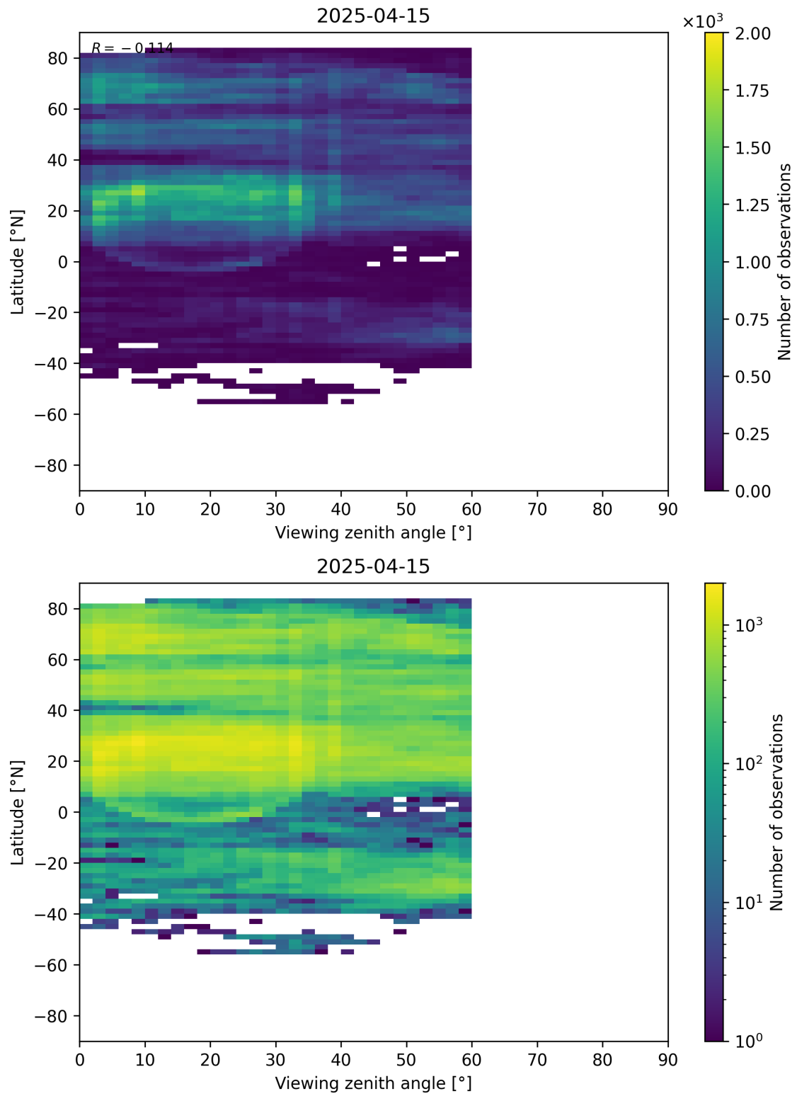
Figure 109: Scatter density plot of “Viewing zenith angle” against “Latitude” for 2025-04-14 to 2025-04-16.
