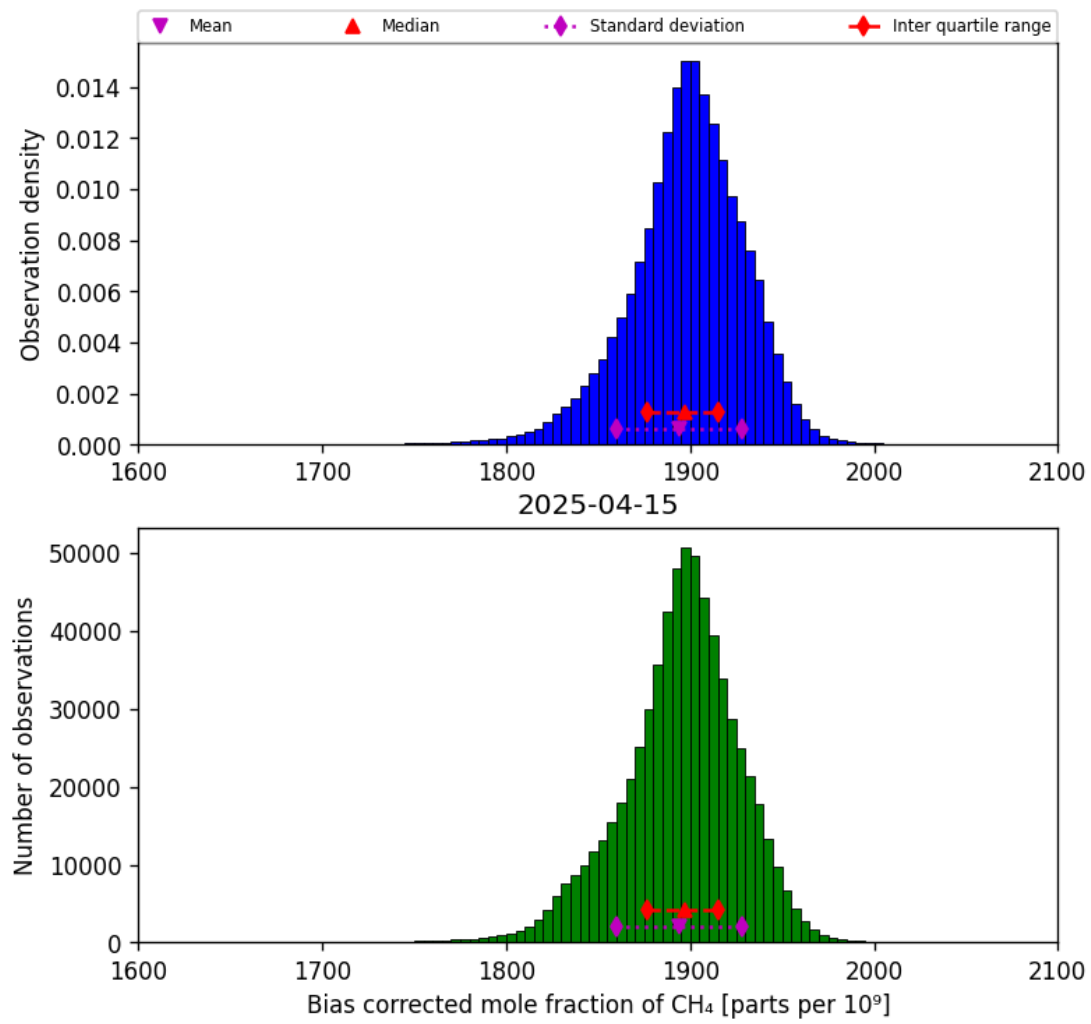
Figure 25: Histogram of “Bias corrected mole fraction of CH 4 ” for 2025-04-14 to 2025-04-16
