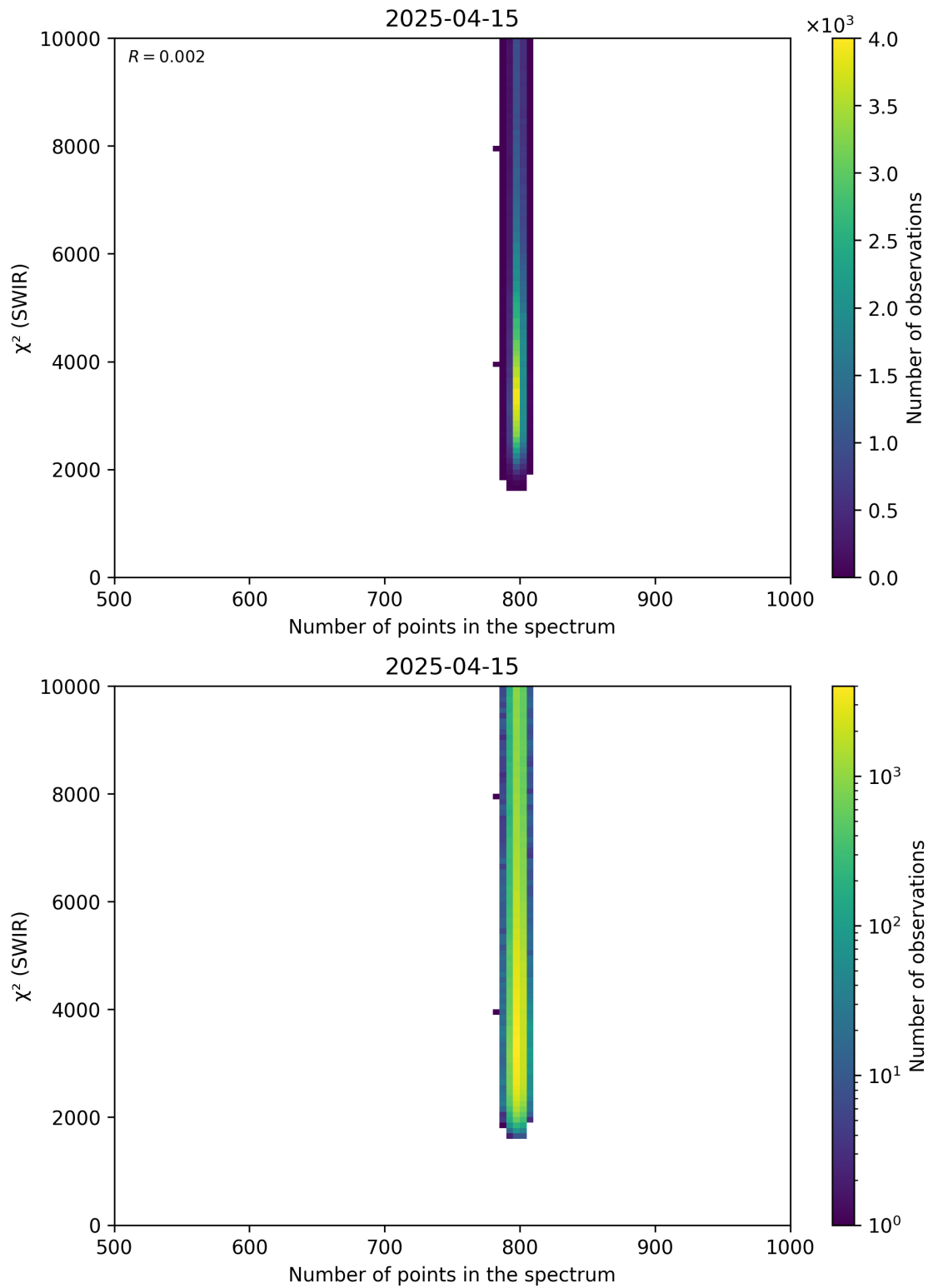
Figure 89: Scatter density plot of “Number of points in the spectrum” against “ \chi^2 (SWIR)” for 2025-04-14 to 2025-04-16.
