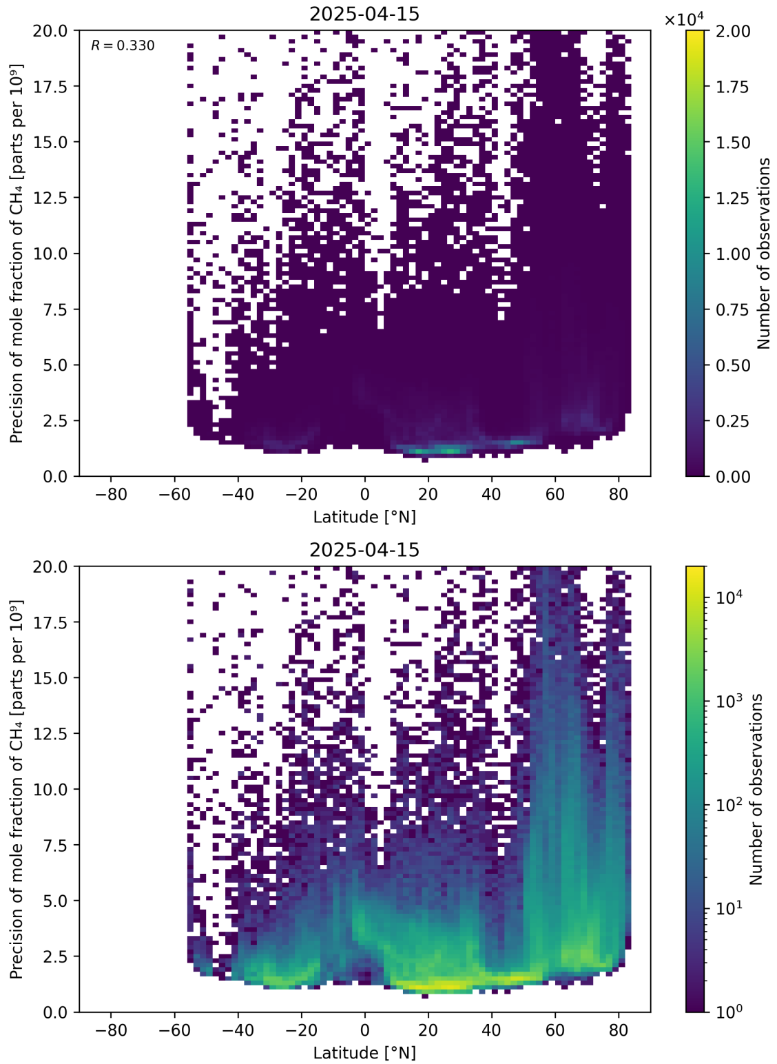
Figure 59: Scatter density plot of “Latitude” against “Precision of mole fraction of \text{CH}_4 ” for 2025-04-14 to 2025-04-16.
