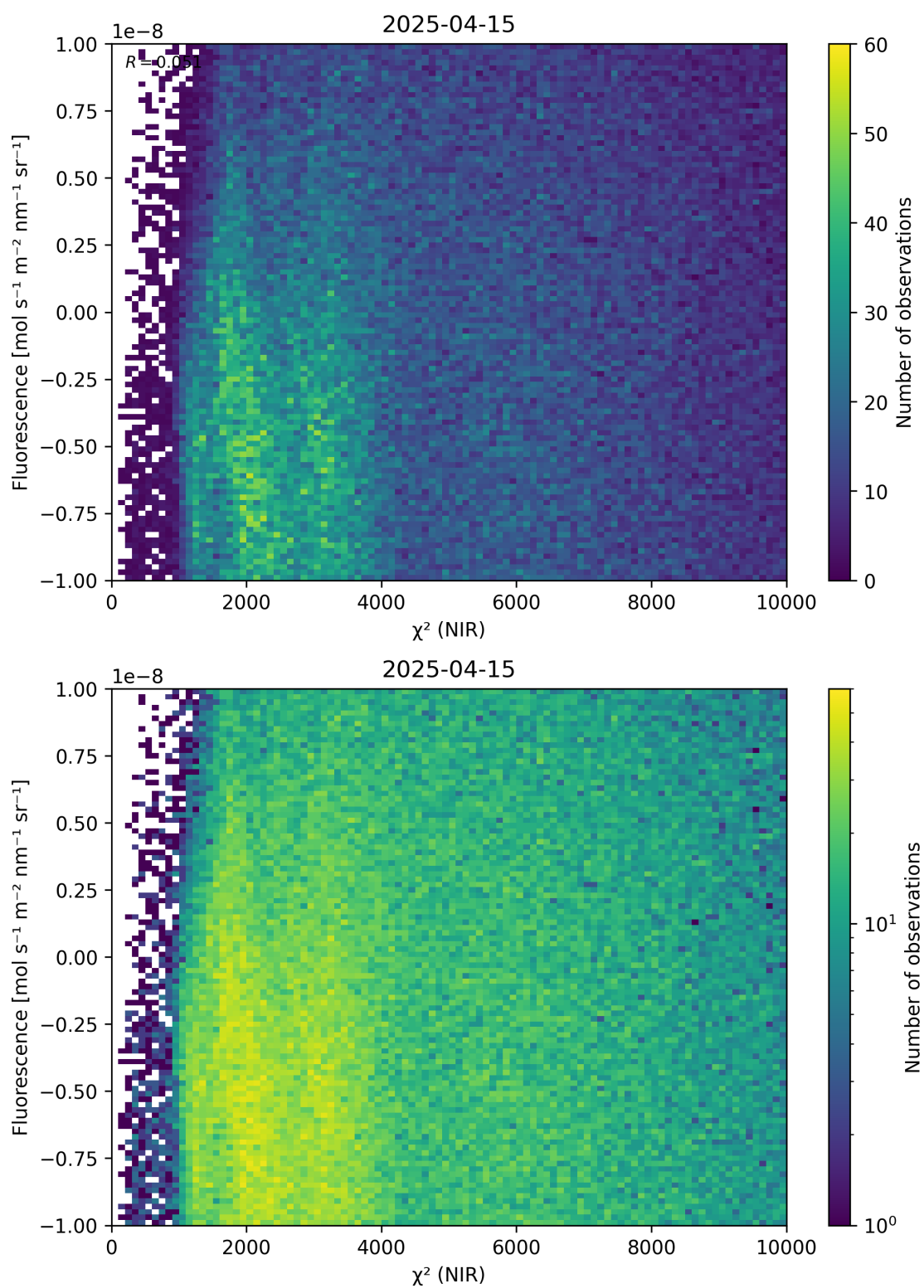
Figure 45: Scatter density plot of “ \chi^2 (NIR)” against “Fluorescence” for 2025-04-14 to 2025-04-16.
