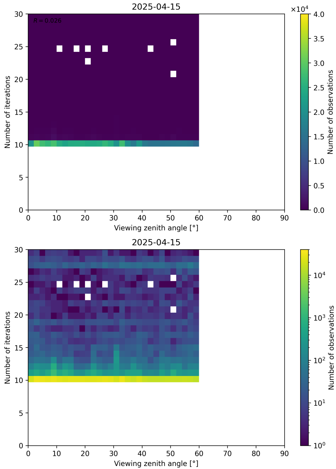
Figure 113: Scatter density plot of “Viewing zenith angle” against “Number of iterations” for 2025-04-14 to 2025-04-16.
