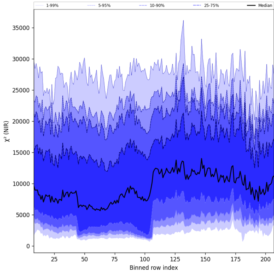
Figure 40: Along track statistics of " \chi^2 (NIR)" for 2025-04-14 to 2025-04-16
