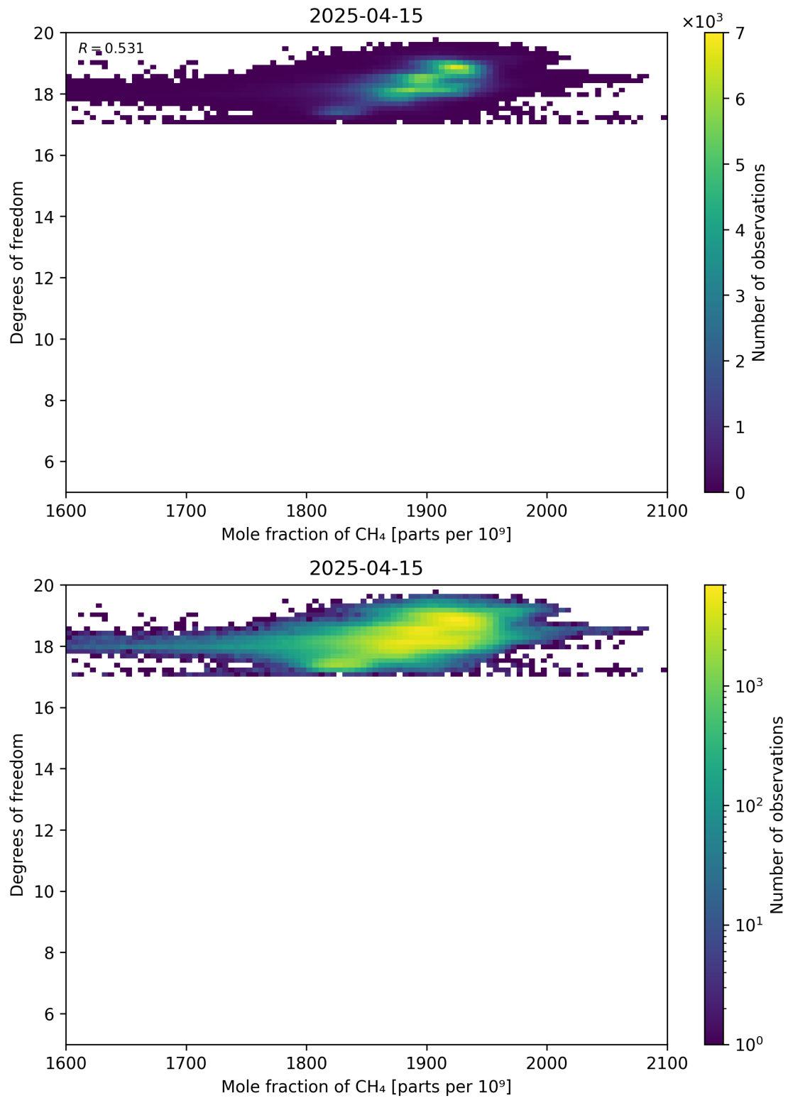
Figure 72: Scatter density plot of “Mole fraction of CH 4 ” against “Degrees of freedom” for 2025-04-14 to 2025-04-16.
