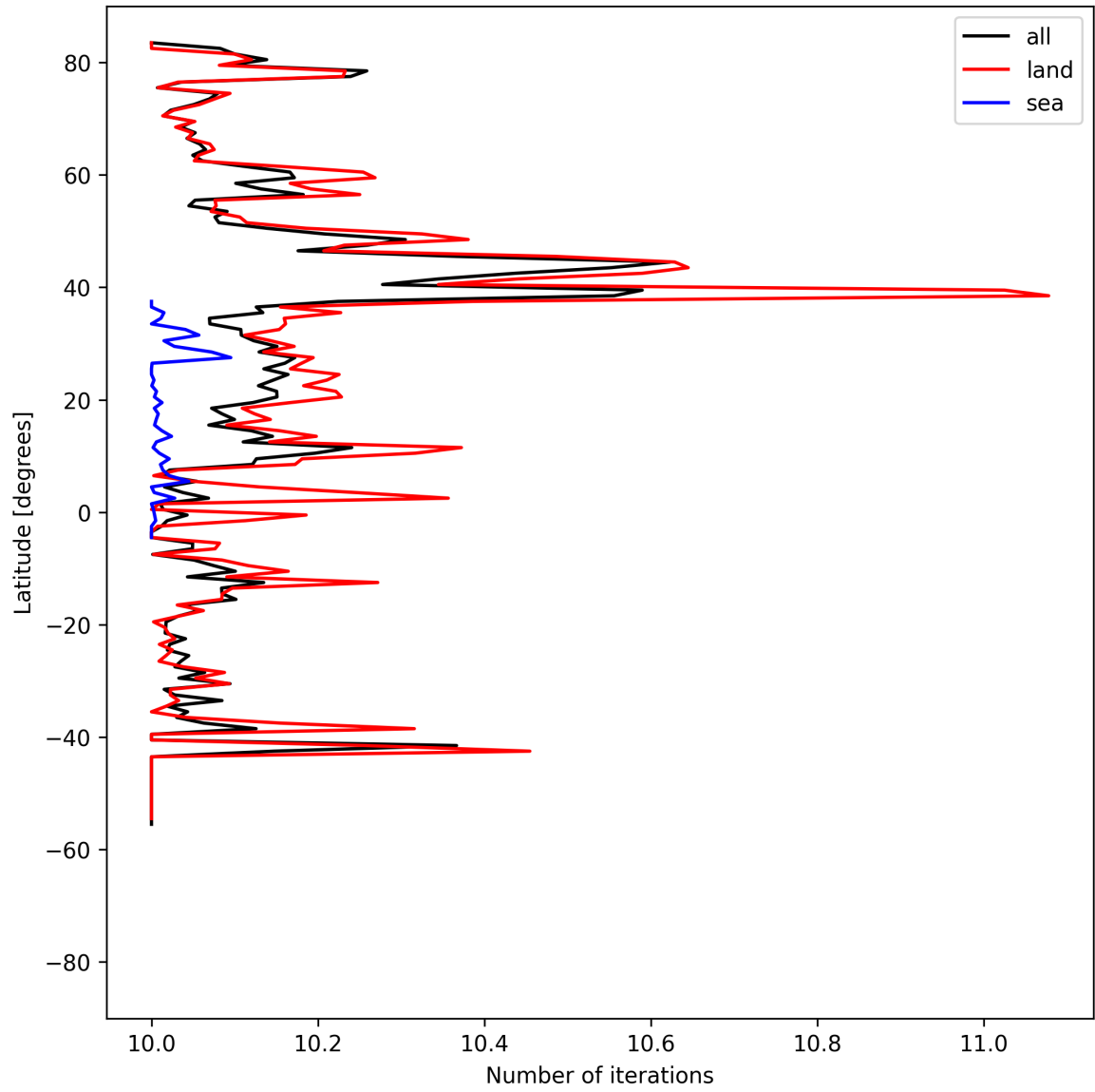
Figure 20: Zonal average of “Number of iterations” for 2025-04-14 to 2025-04-16.
