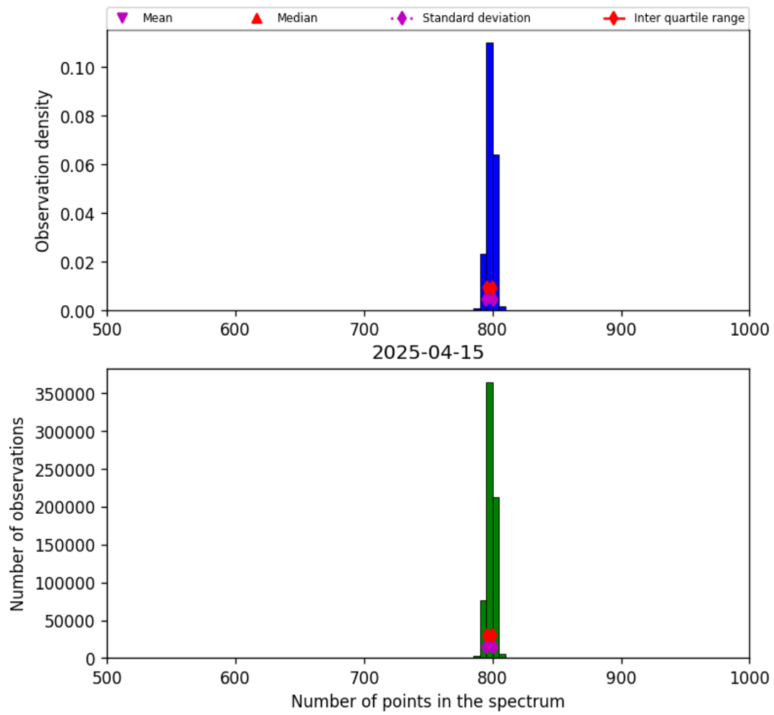
Figure 26: Histogram of “Number of points in the spectrum” for 2025-04-14 to 2025-04-16
