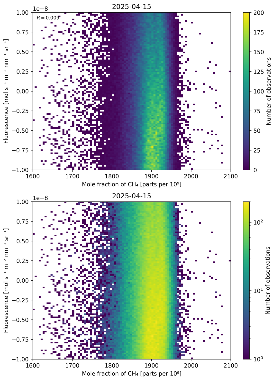
Figure 73: Scatter density plot of “Mole fraction of \text{CH}_4 ” against “Fluorescence” for 2025-04-14 to 2025-04-16.
