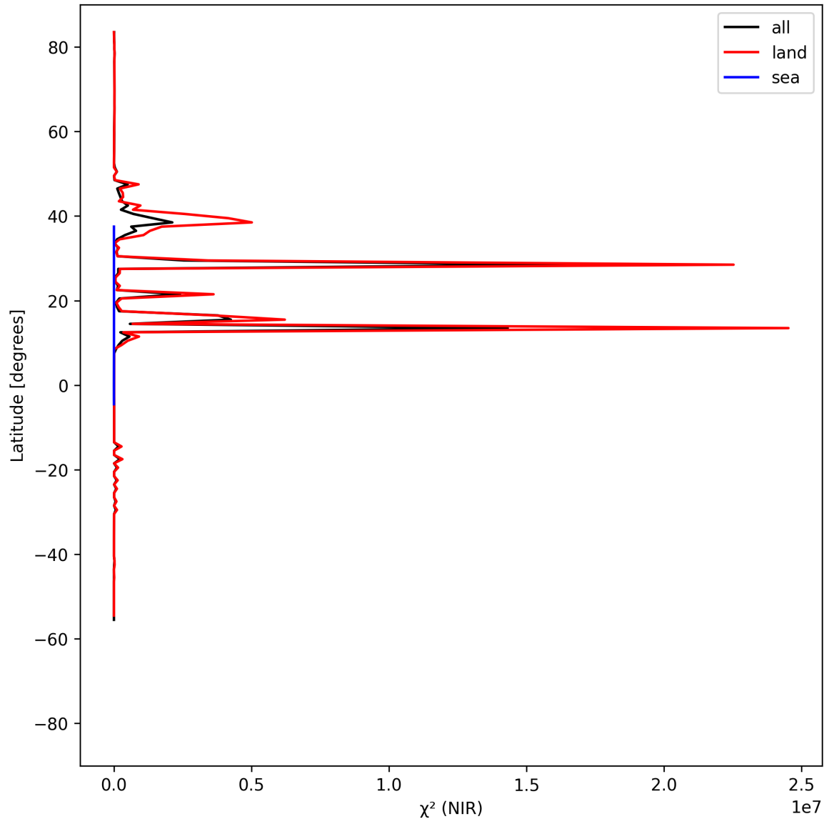
Figure 18: Zonal average of “ \chi^2 (NIR)” for 2025-04-14 to 2025-04-16.
