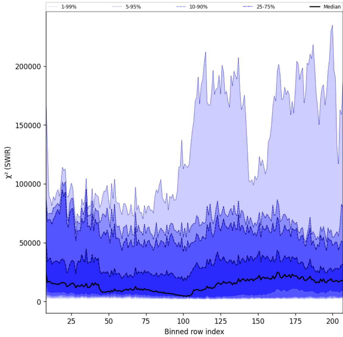
Figure 39: Along track statistics of “ \chi^2 (SWIR)” for 2025-04-14 to 2025-04-16
