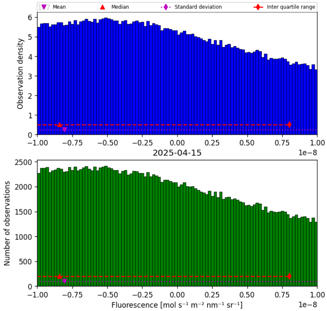
Figure 32: Histogram of “Fluorescence” for 2025-04-14 to 2025-04-16
