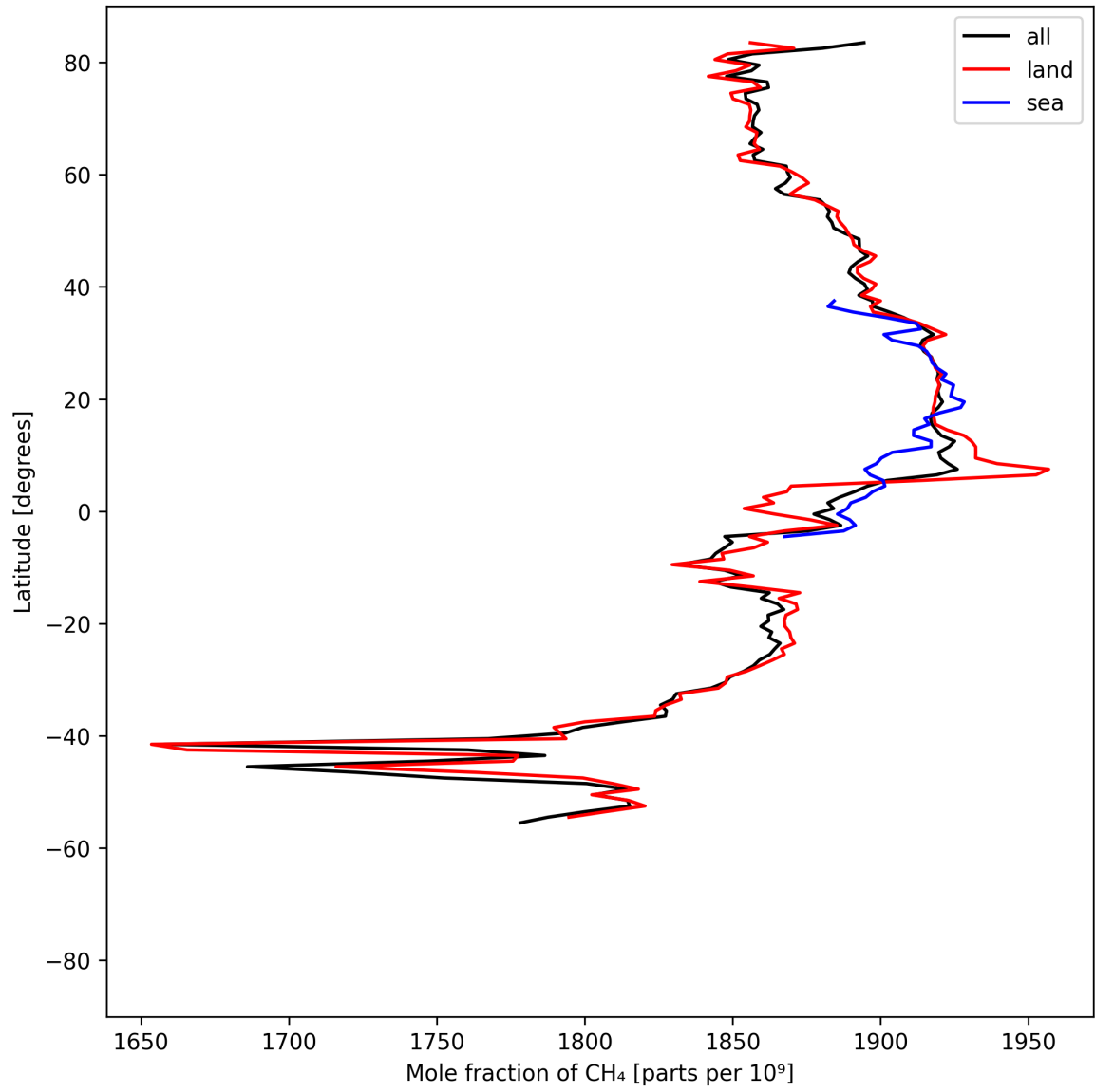
Figure 12: Zonal average of “Mole fraction of \text{CH}_4 ” for 2025-04-14 to 2025-04-16.
