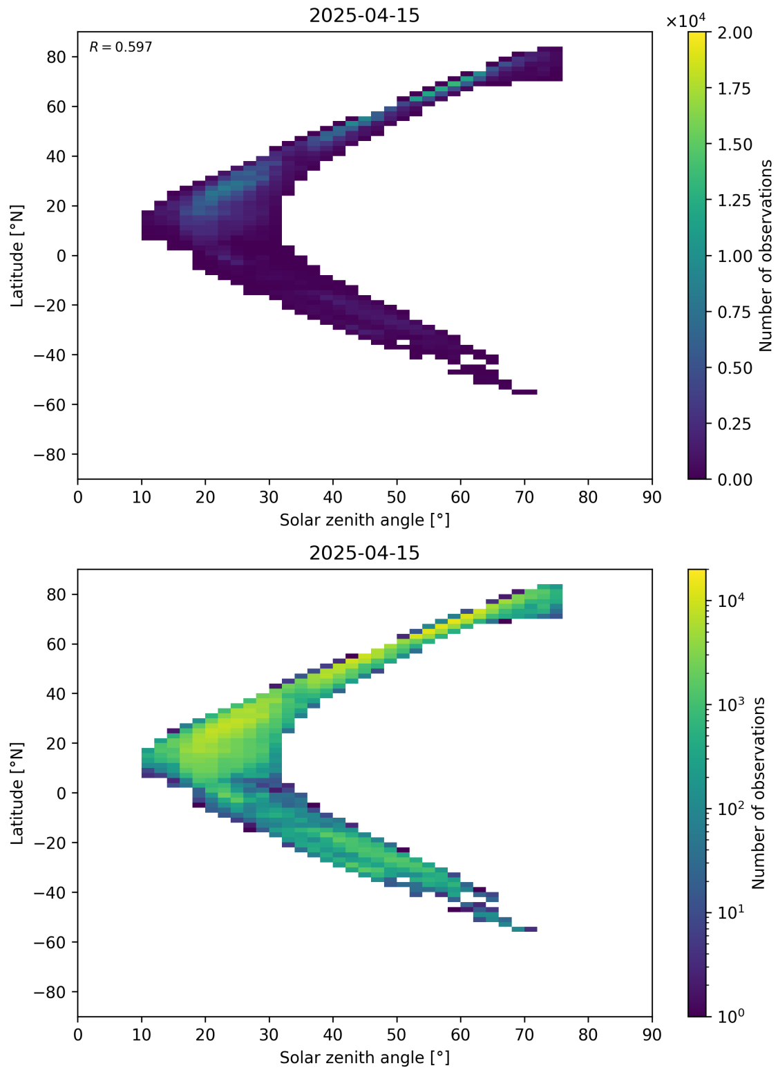
Figure 98: Scatter density plot of “Solar zenith angle” against “Latitude” for 2025-04-14 to 2025-04-16.
