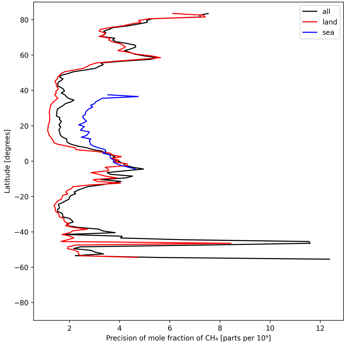
Figure 13: Zonal average of “Precision of mole fraction of CH 4 ” for 2025-04-14 to 2025-04-16.
