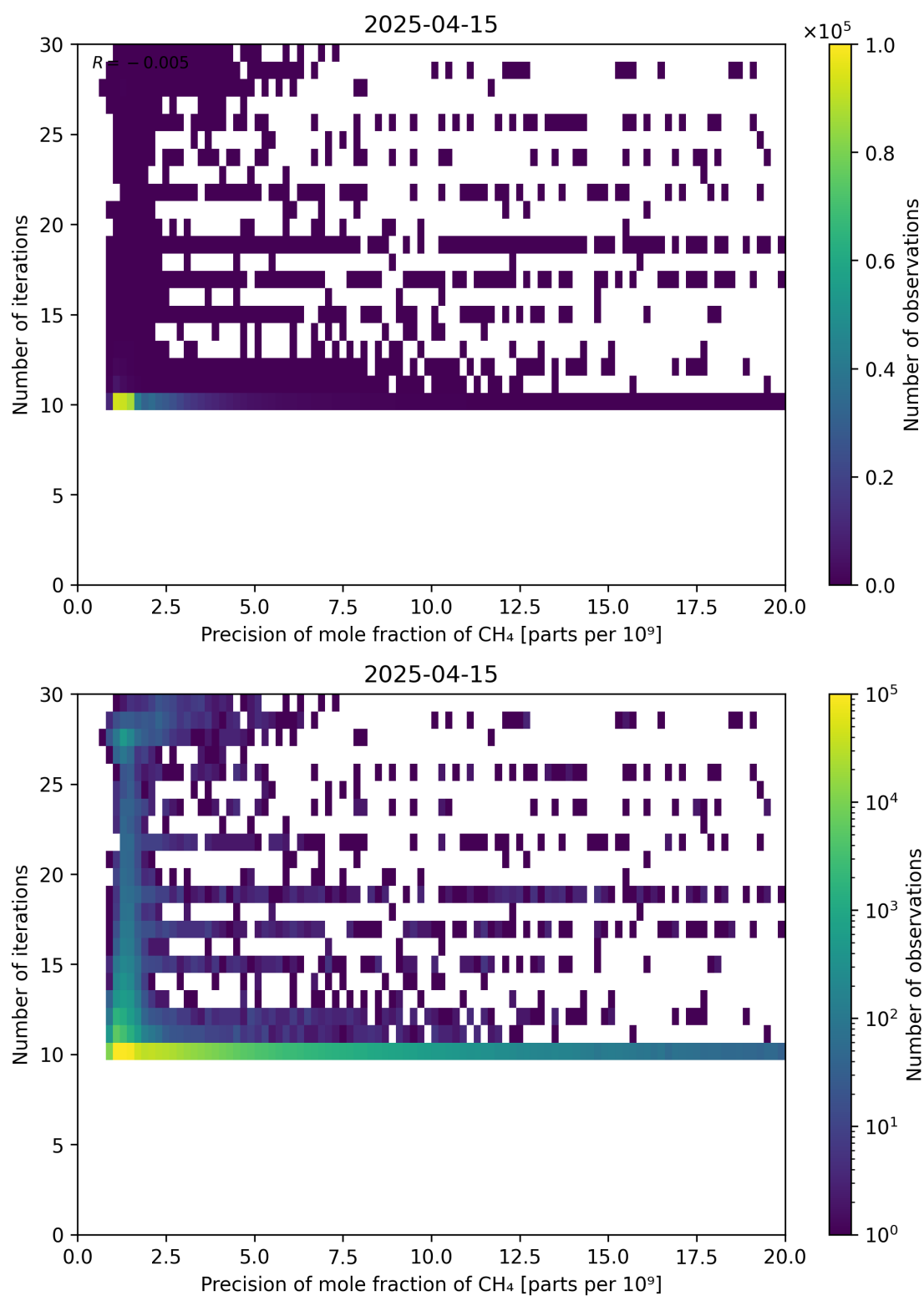
Figure 83: Scatter density plot of “Precision of mole fraction of CH 4 ” against “Number of iterations” for 2025-04-14 to 2025-04-16.
