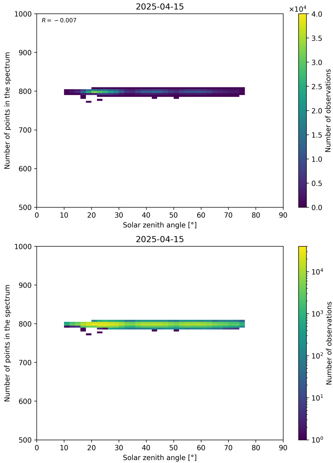
Figure 103: Scatter density plot of “Solar zenith angle” against “Number of points in the spectrum” for 2025-04-14 to 2025-04-16.
