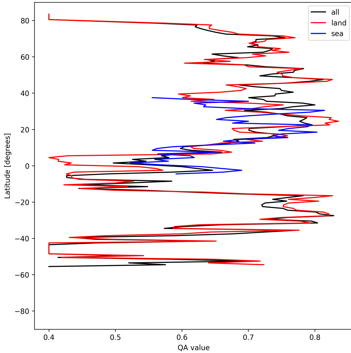
Figure 11: Zonal average of “QA value” for 2025-04-14 to 2025-04-16.
