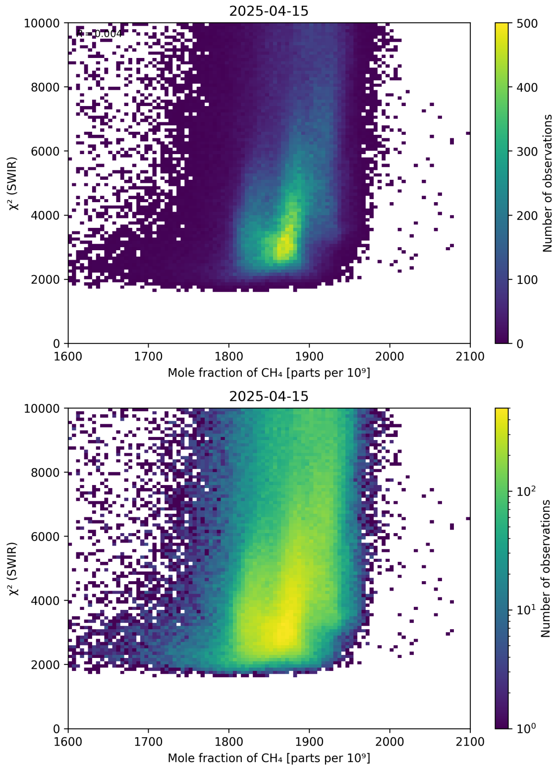
Figure 71: Scatter density plot of “Mole fraction of CH 4 ” against “ \chi^2 (SWIR)” for 2025-04-14 to 2025-04-16.
