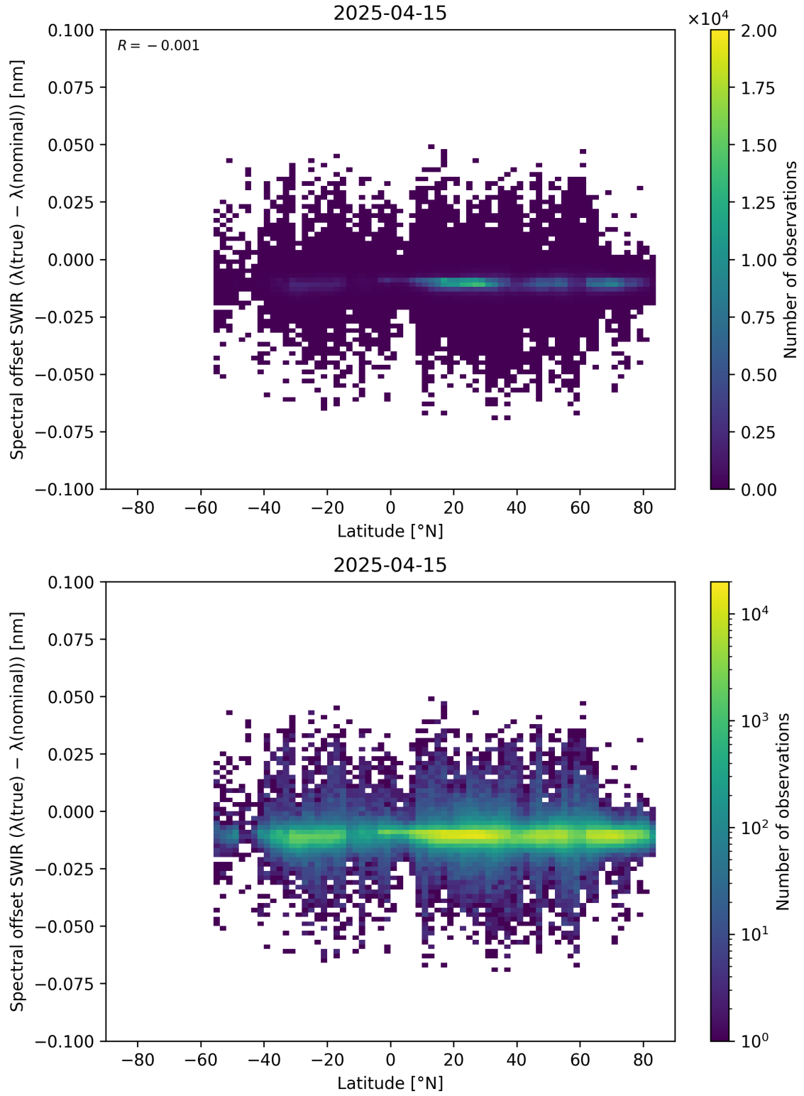
Figure 62: Scatter density plot of “Latitude” against “Spectral offset SWIR ( \lambda_{\text{true}} - \lambda_{\text{nominal}} )” for 2025-04-14 to 2025-04-16.
