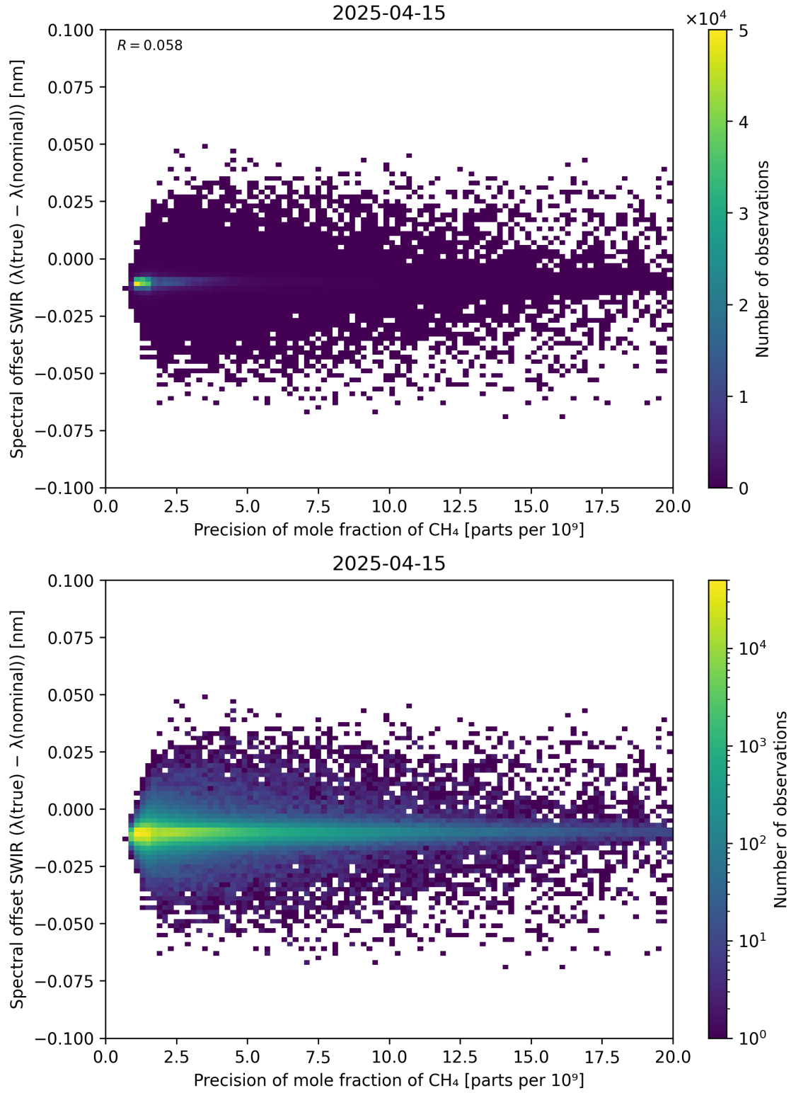
Figure 85: Scatter density plot of “Precision of mole fraction of \text{CH}_4 ” against “Spectral offset SWIR ( \lambda_{\text{true}} - \lambda_{\text{nominal}} )” for 2025-04-14 to 2025-04-16.
