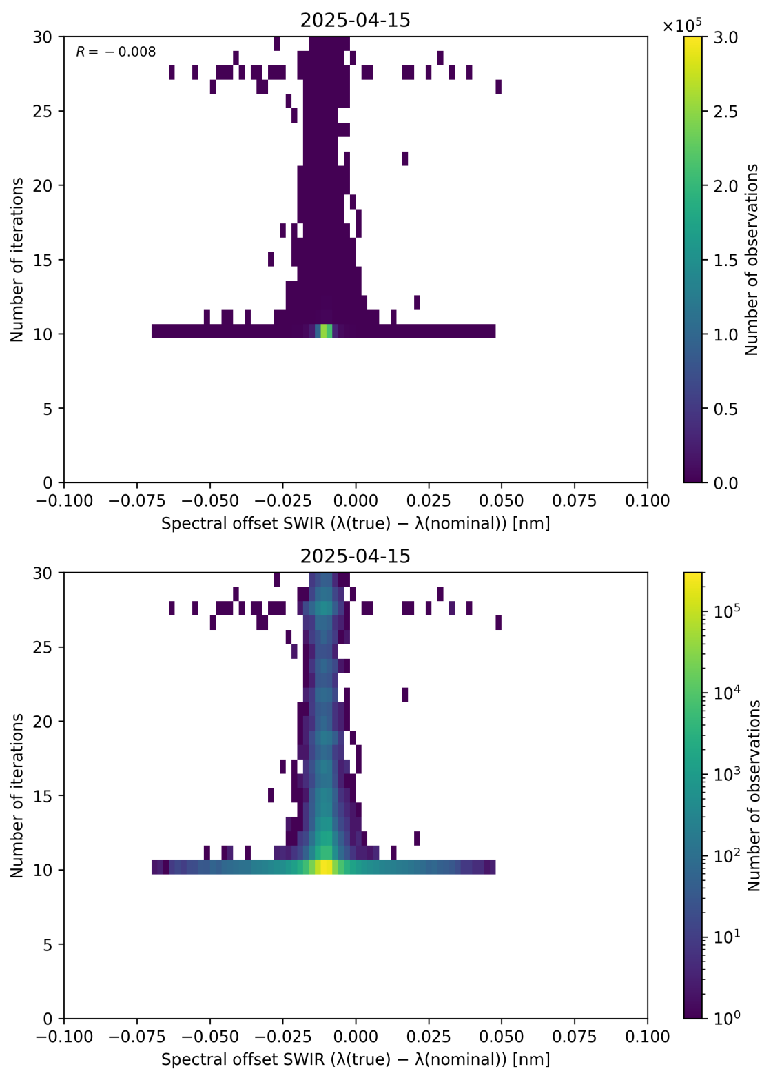
Figure 121: Scatter density plot of “Spectral offset SWIR ( \lambda_{\text{true}} - \lambda_{\text{nominal}} )” against “Number of iterations” for 2025-04-14 to 2025-04-16.
