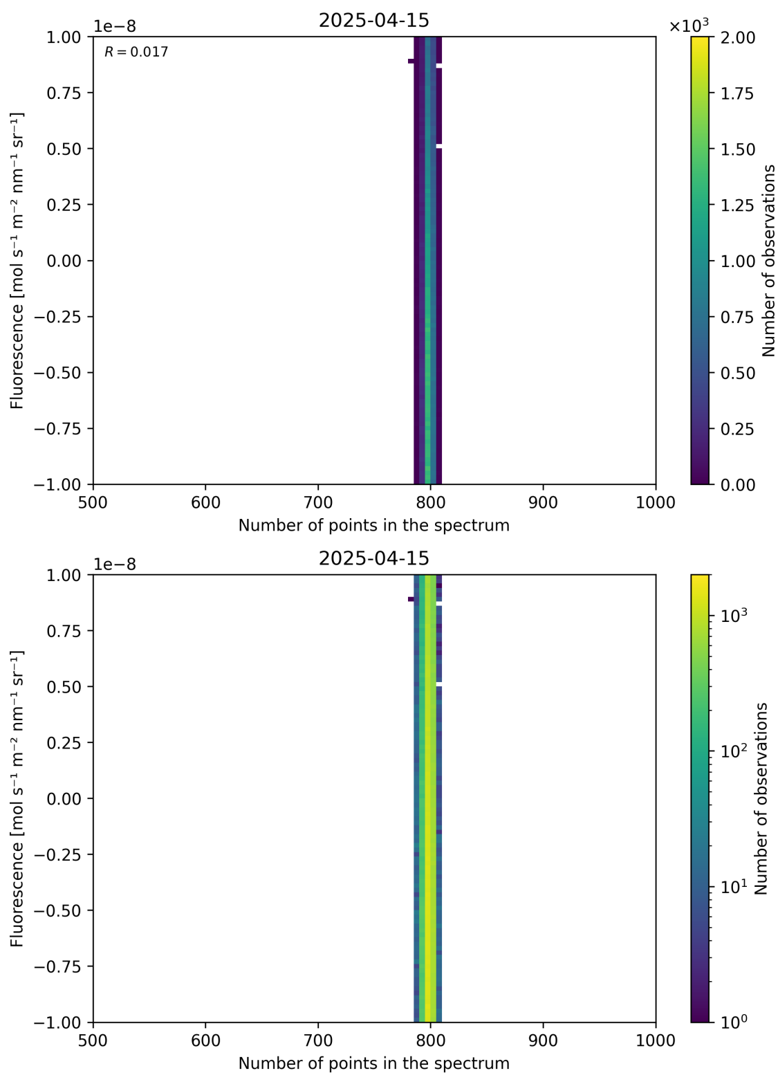
Figure 91: Scatter density plot of “Number of points in the spectrum” against “Fluorescence” for 2025-04-14 to 2025-04-16.
