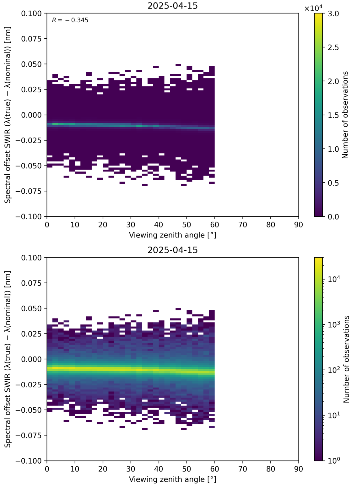
Figure 116: Scatter density plot of “Viewing zenith angle” against “Spectral offset SWIR ( \lambda_{\text{true}} - \lambda_{\text{nominal}} )” for 2025-04-14 to 2025-04-16.
