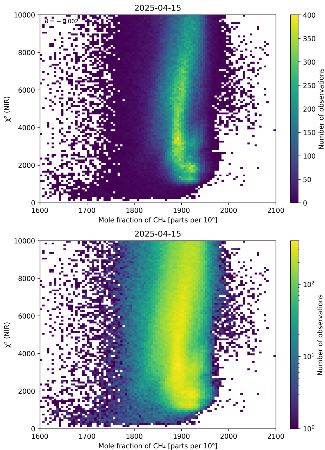
Figure 70: Scatter density plot of “Mole fraction of \text{CH}_4 ” against “ \chi^2 (NIR)” for 2025-04-14 to 2025-04-16.
