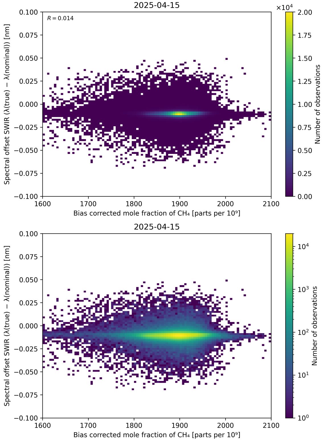
Figure 69: Scatter density plot of “Bias corrected mole fraction of \text{CH}_4 ” against “Spectral offset SWIR ( \lambda_{\text{true}} - \lambda_{\text{nominal}} )” for 2025-04-14 to 2025-04-16.
