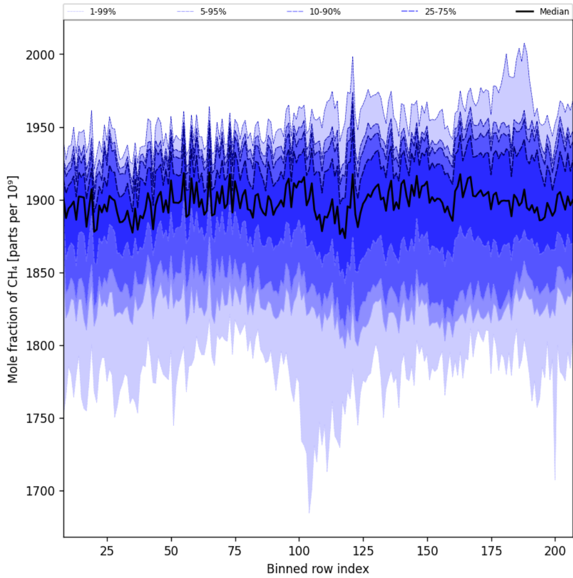
Figure 34: Along track statistics of “Mole fraction of CH 4 ” for 2025-04-14 to 2025-04-16
