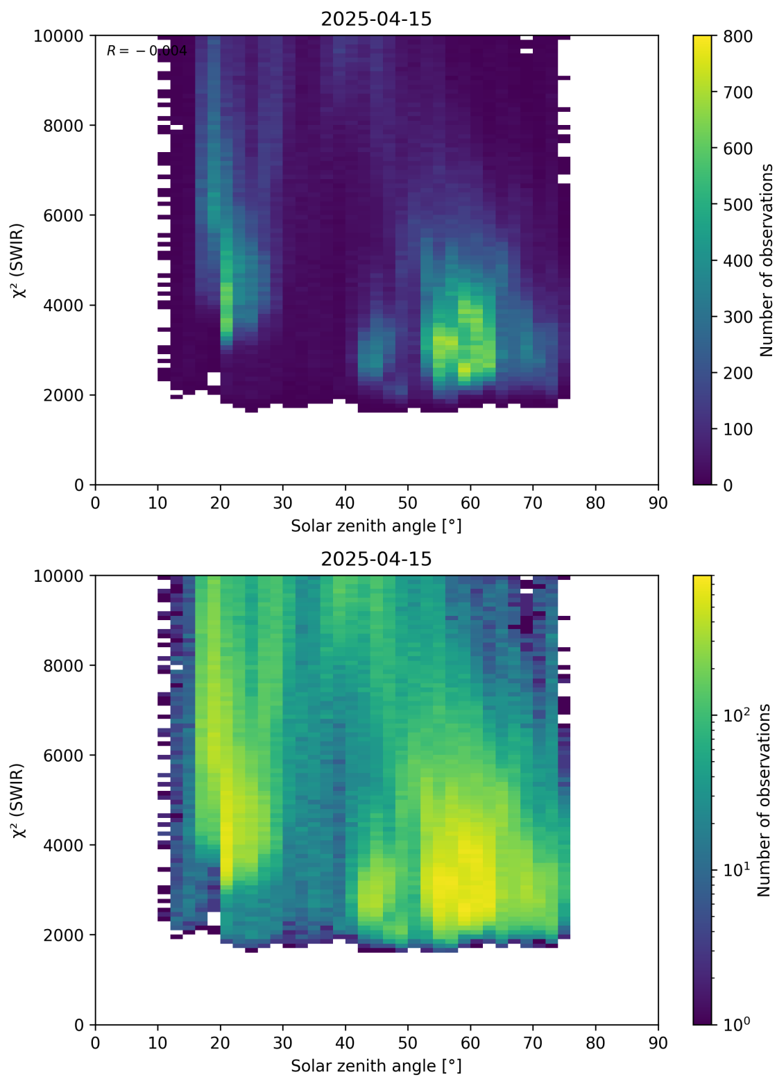
Figure 95: Scatter density plot of “Solar zenith angle” against “ \chi^2 (SWIR)” for 2025-04-14 to 2025-04-16.
