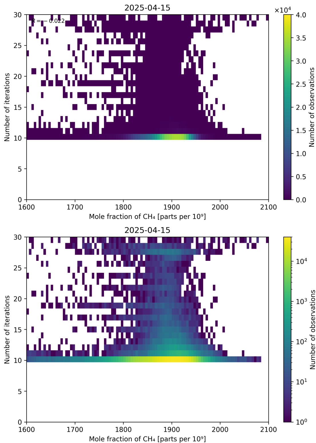
Figure 76: Scatter density plot of “Mole fraction of CH 4 ” against “Number of iterations” for 2025-04-14 to 2025-04-16.
