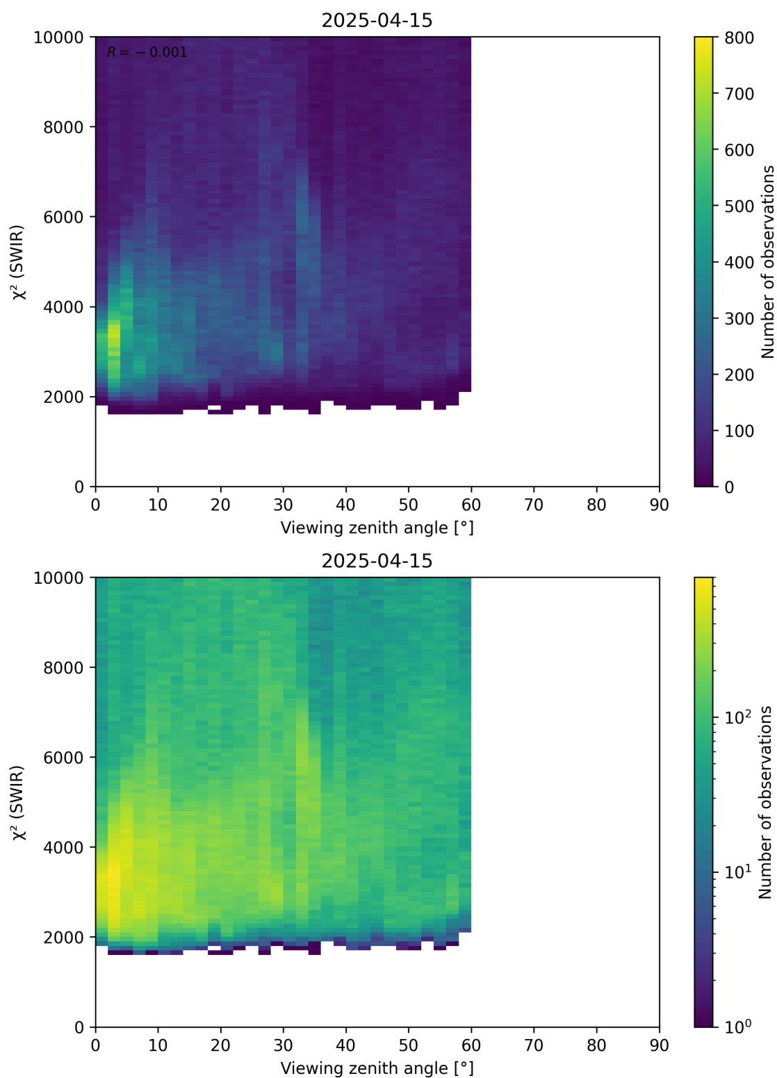
Figure 106: Scatter density plot of “Viewing zenith angle” against “ \chi^2 (SWIR)” for 2025-04-14 to 2025-04-16.
