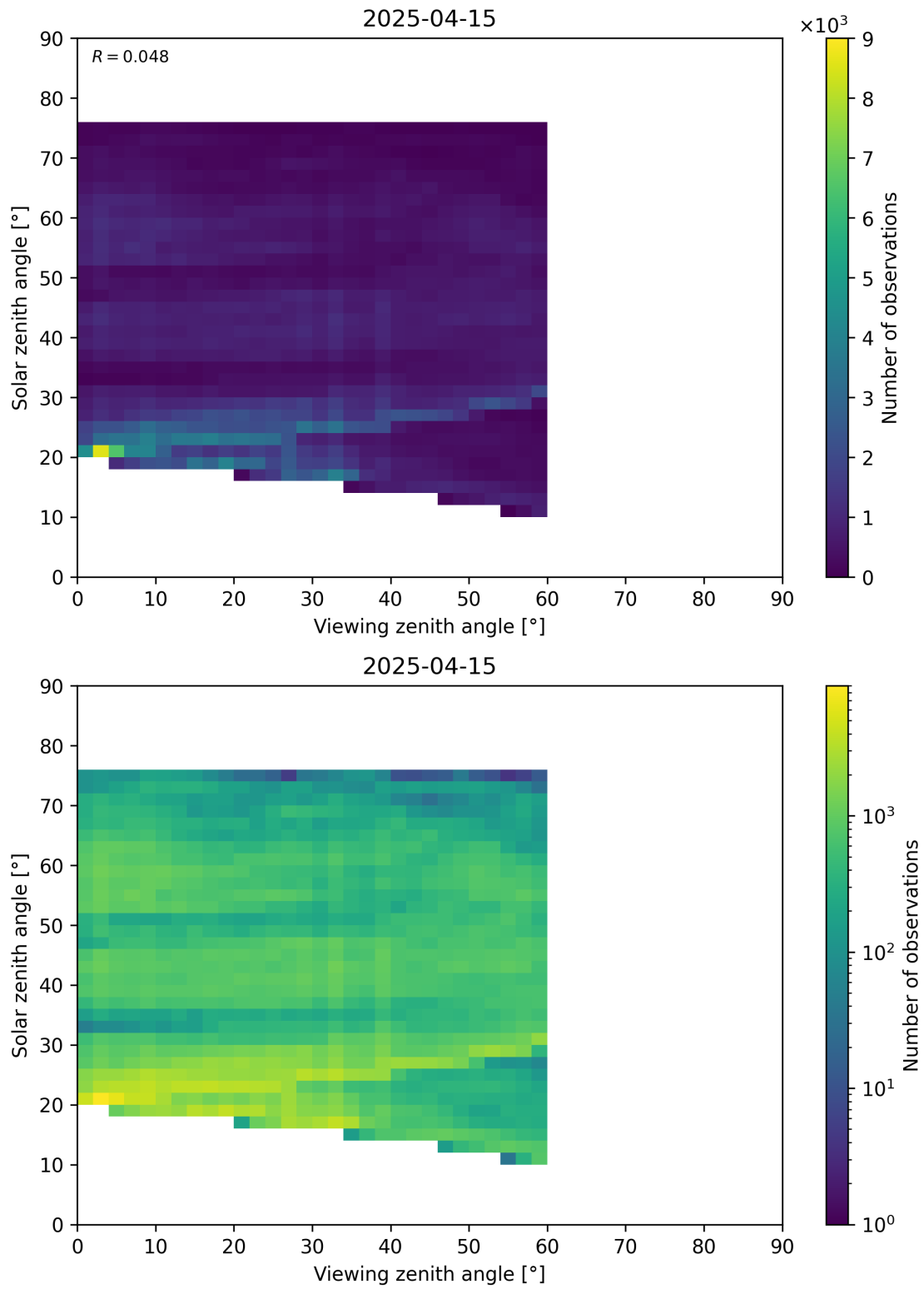
Figure 115: Scatter density plot of “Viewing zenith angle” against “Solar zenith angle” for 2025-04-14 to 2025-04-16.
