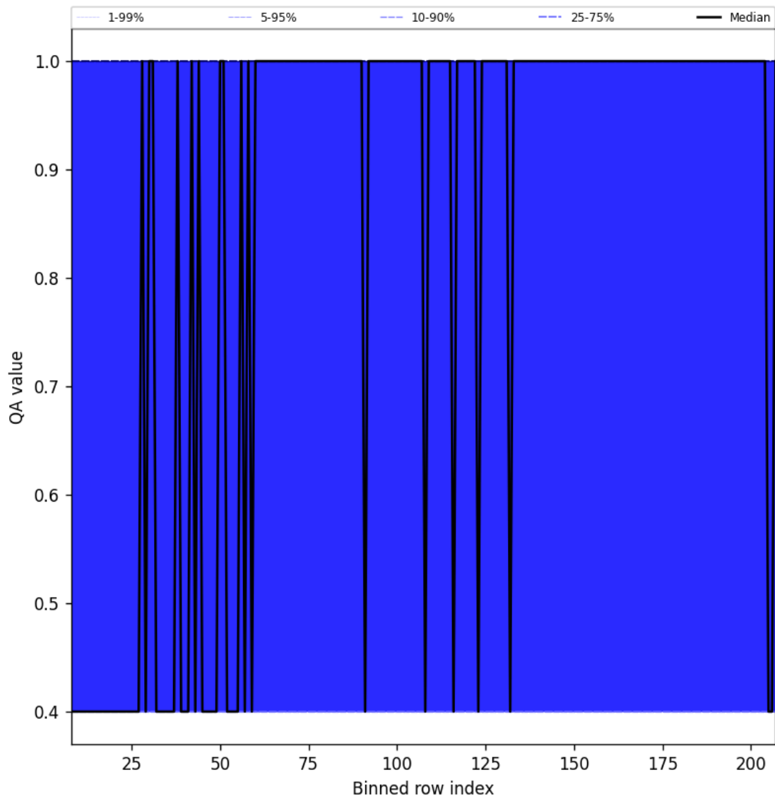
Figure 33: Along track statistics of “QA value” for 2025-04-14 to 2025-04-16
