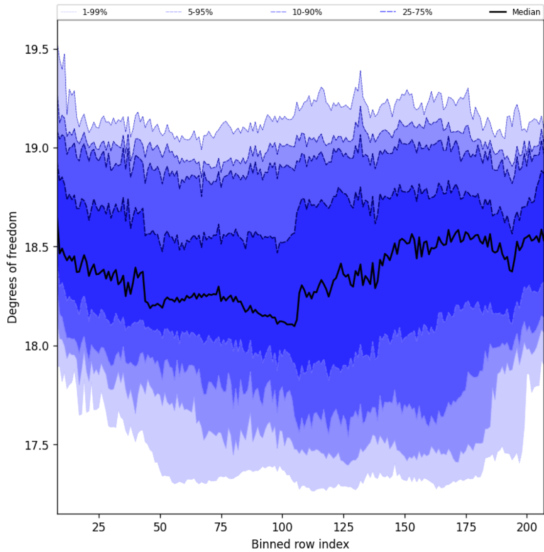
Figure 41: Along track statistics of “Degrees of freedom” for 2025-04-14 to 2025-04-16
