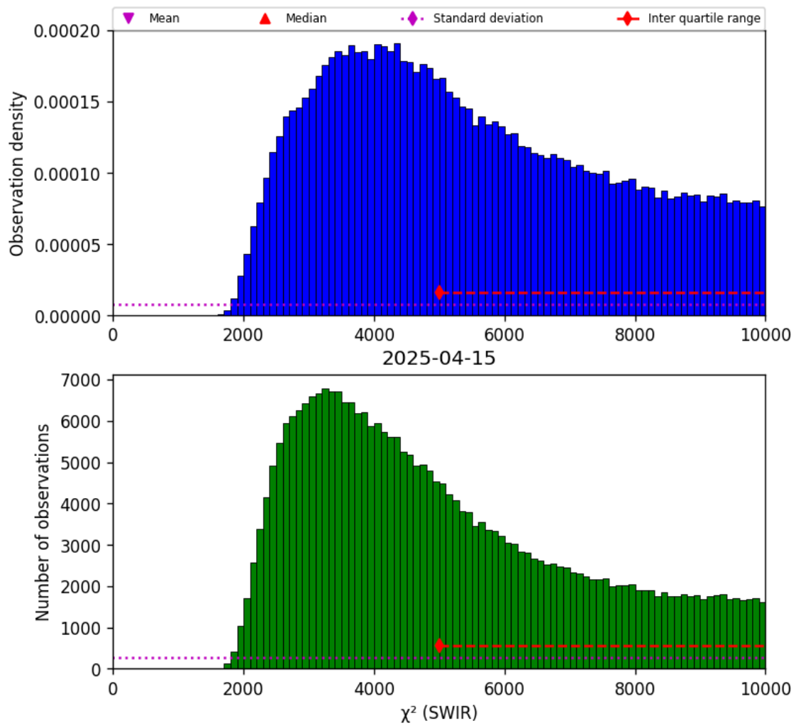
Figure 28: Histogram of “ \chi^2 (SWIR)” for 2025-04-14 to 2025-04-16
