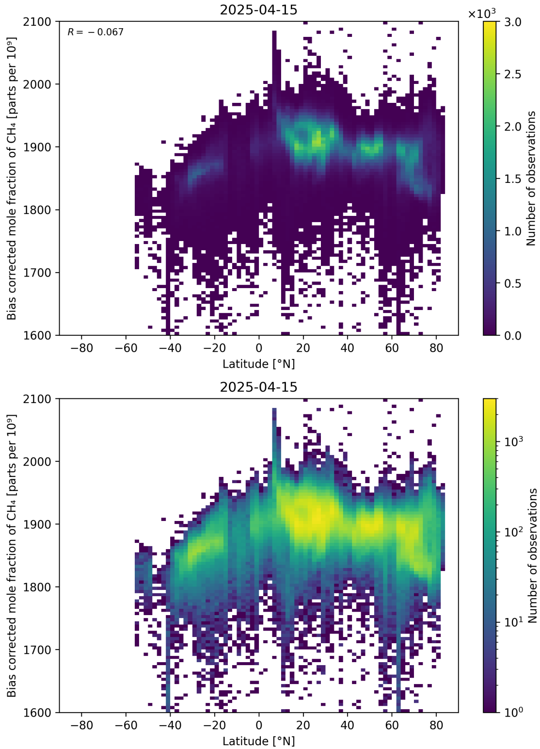
Figure 58: Scatter density plot of “Latitude” against “Bias corrected mole fraction of CH 4 ” for 2025-04-14 to 2025-04-16.
