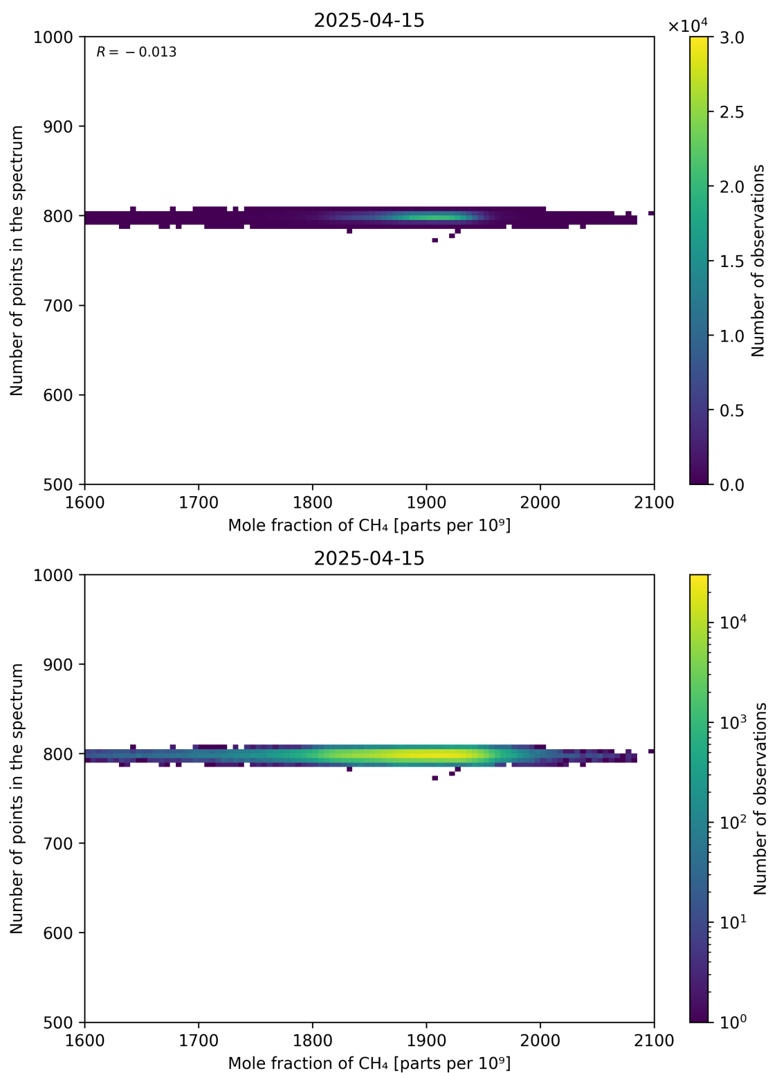
Figure 77: Scatter density plot of “Mole fraction of CH 4 ” against “Number of points in the spectrum” for 2025-04-14 to 2025-04-16.
