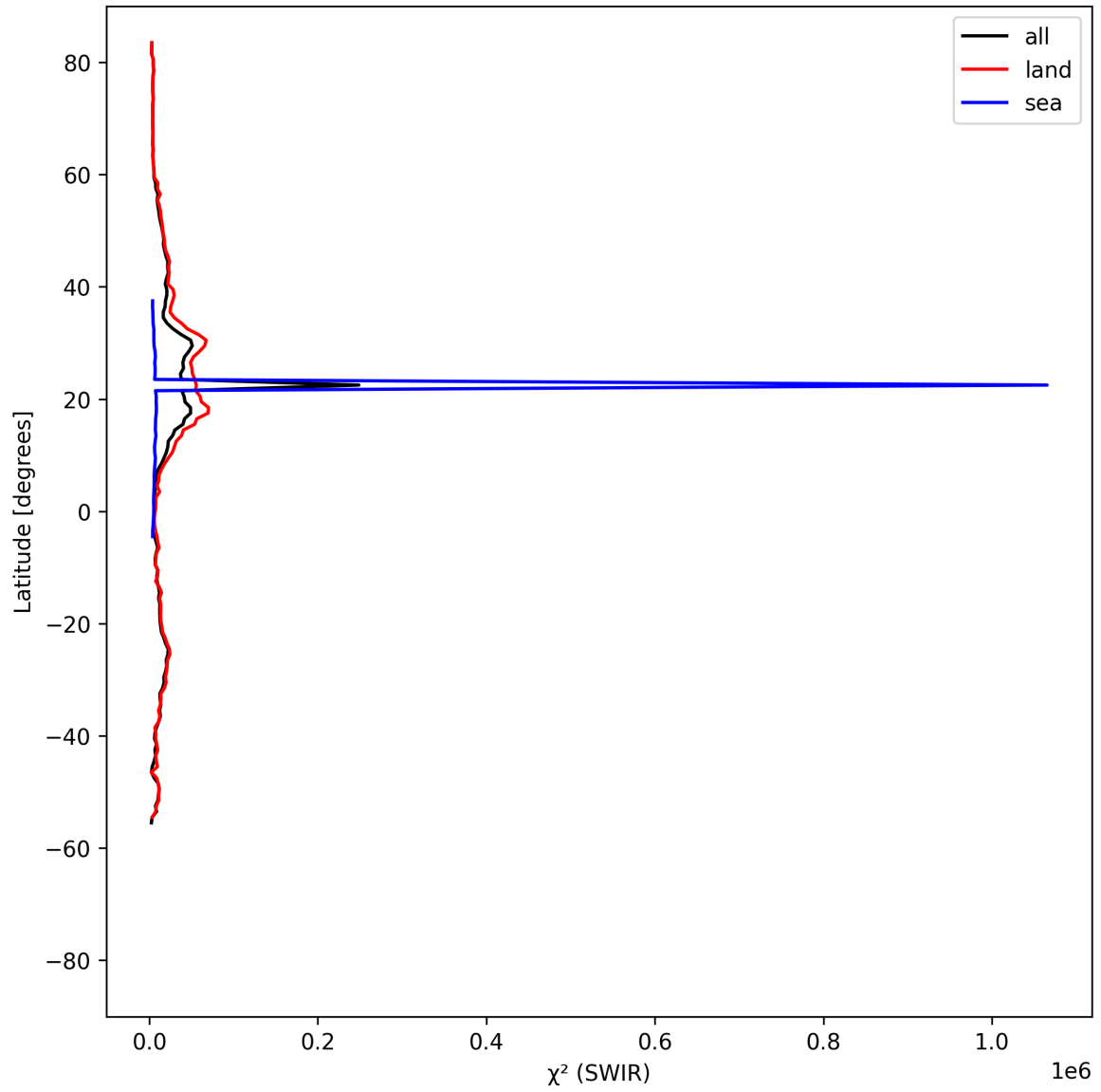
Figure 17: Zonal average of “ \chi^2 (SWIR)” for 2025-04-14 to 2025-04-16.
