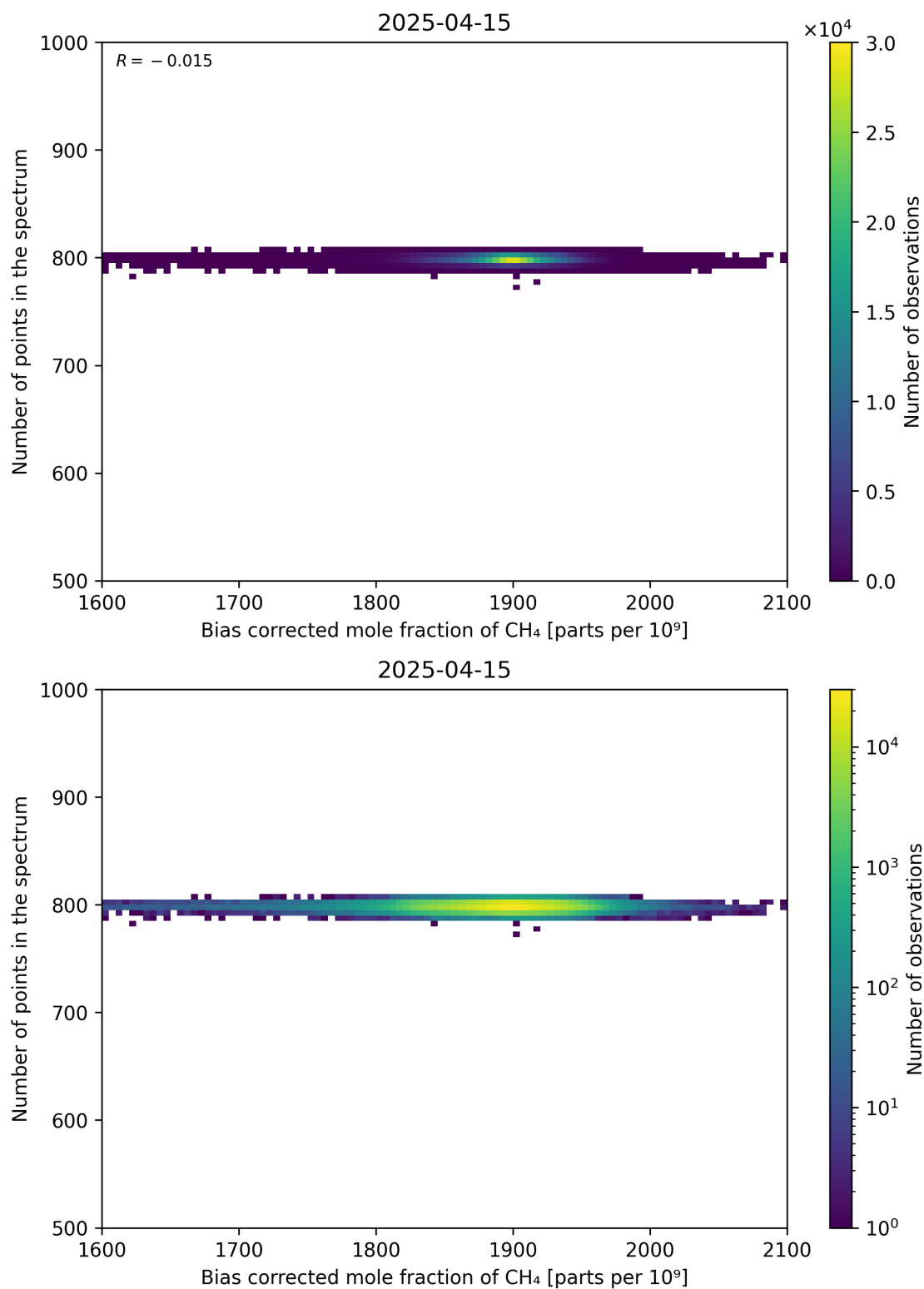
Figure 68: Scatter density plot of “Bias corrected mole fraction of CH 4 ” against “Number of points in the spectrum” for 2025-04-14 to 2025-04-16.
