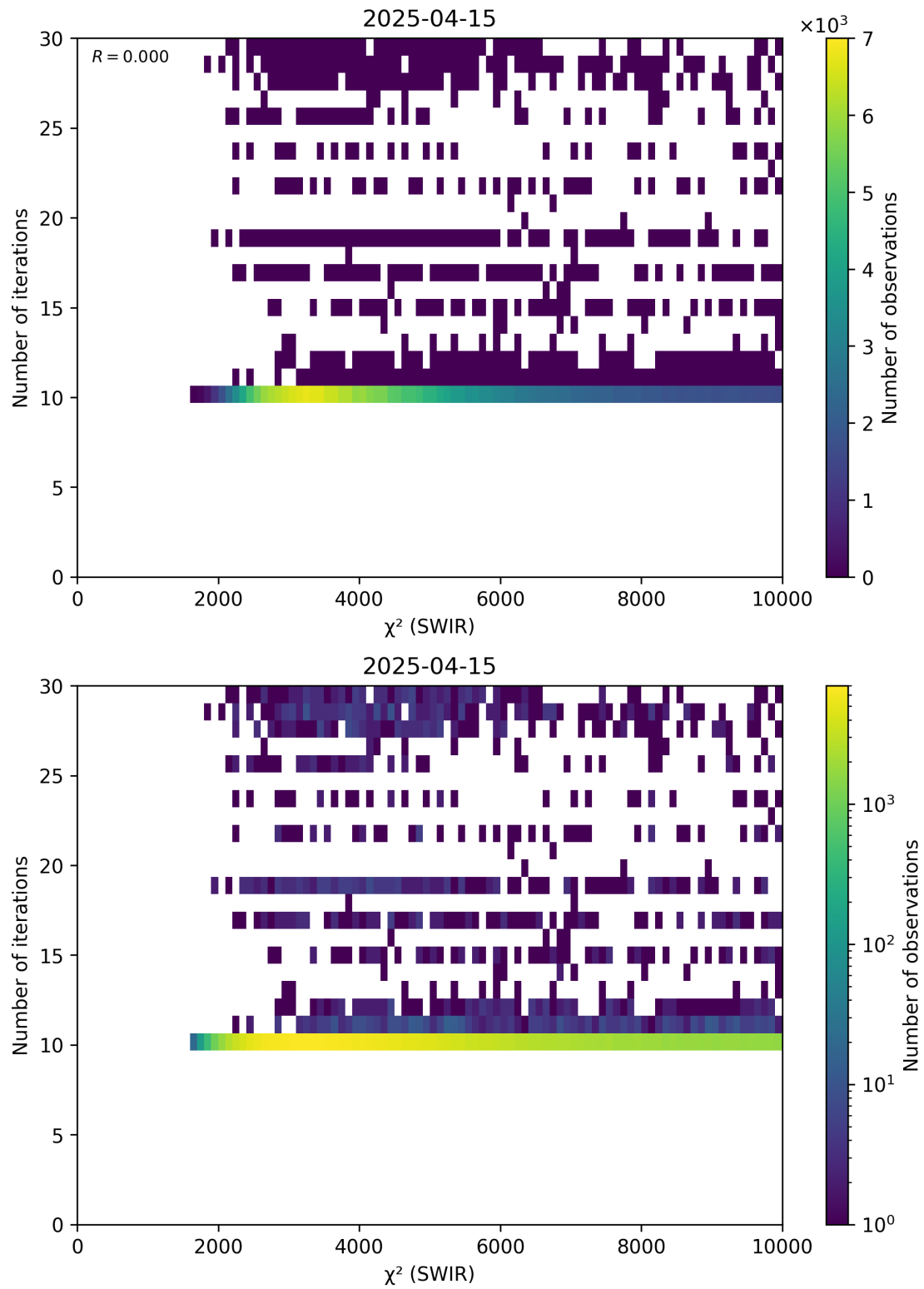
Figure 50: Scatter density plot of “ \chi^2 (SWIR)” against “Number of iterations” for 2025-04-14 to 2025-04-16.
