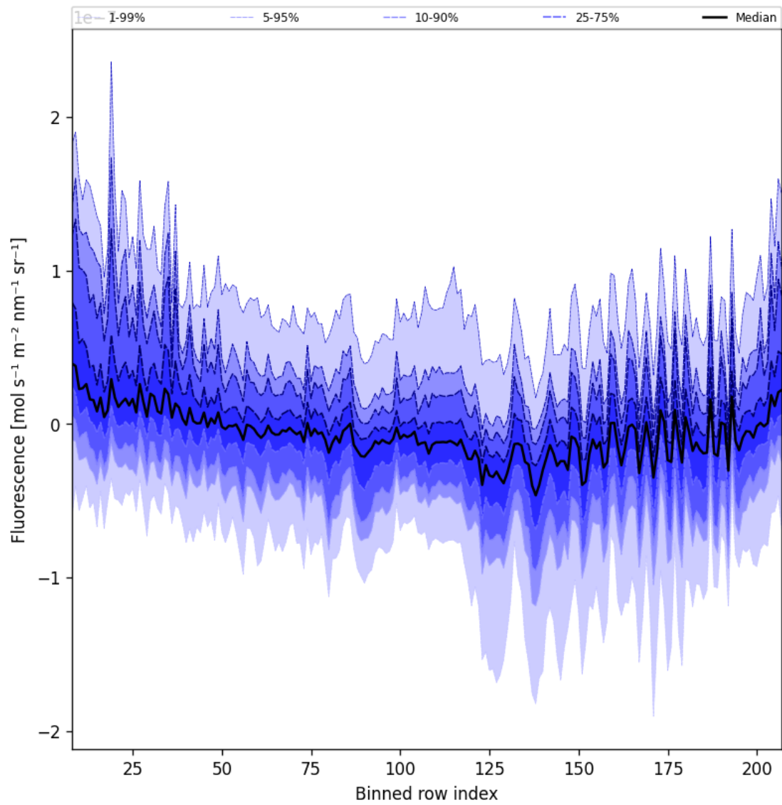
Figure 43: Along track statistics of "Fluorescence" for 2025-04-14 to 2025-04-16
