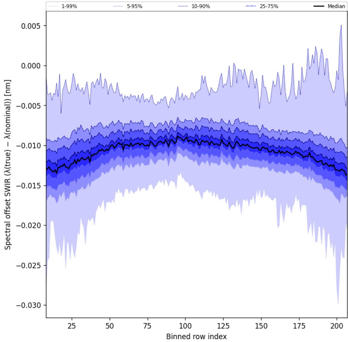
Figure 38: Along track statistics of “Spectral offset SWIR ( \lambda_{\text{true}} - \lambda_{\text{nominal}} )” for 2025-04-14 to 2025-04-16
