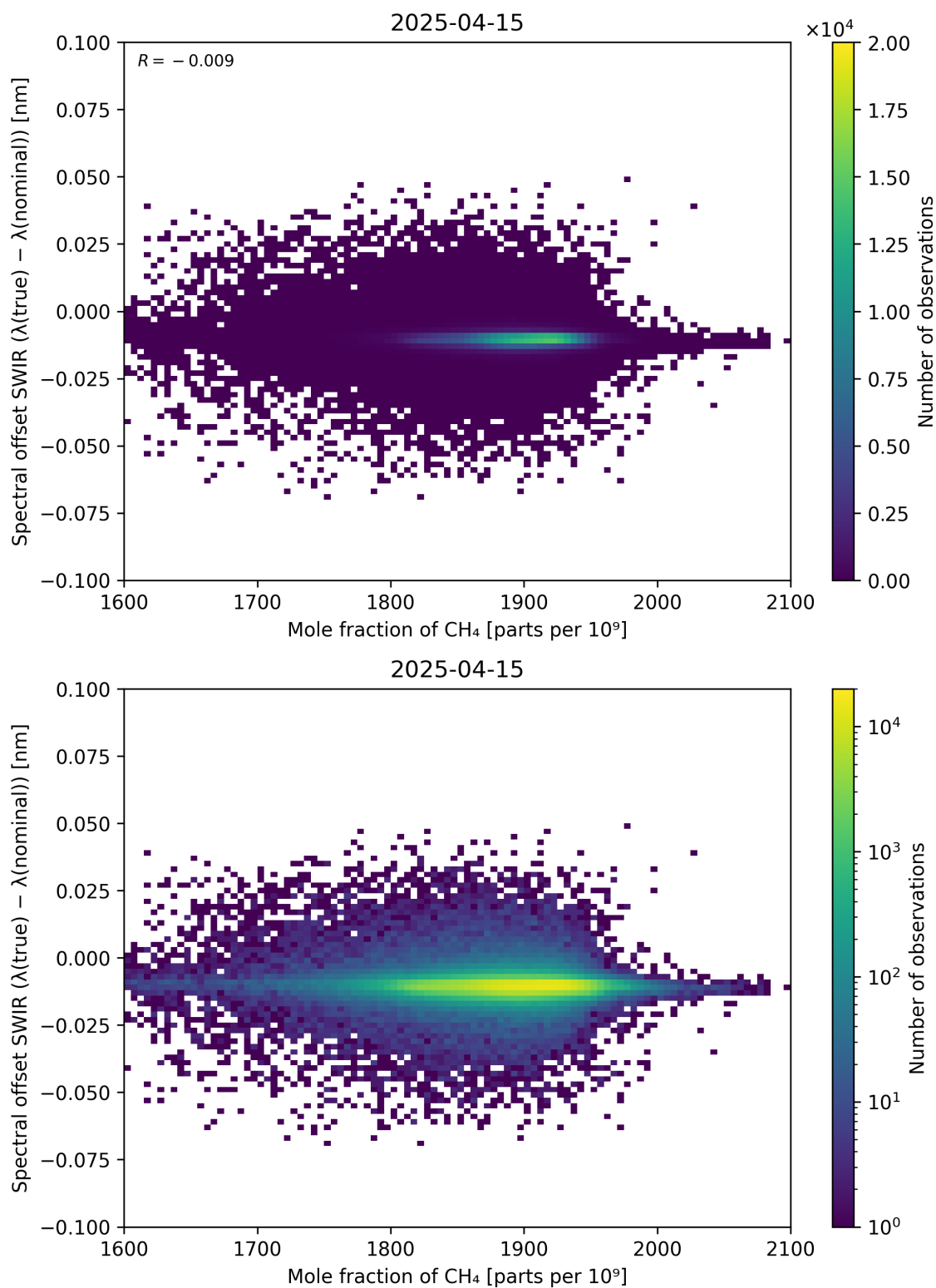
Figure 86: Scatter density plot of “Mole fraction of CH 4 ” against “Spectral offset SWIR ( \lambda_{\text{true}} - \lambda_{\text{nominal}} )” for 2025-04-14 to 2025-04-16.
