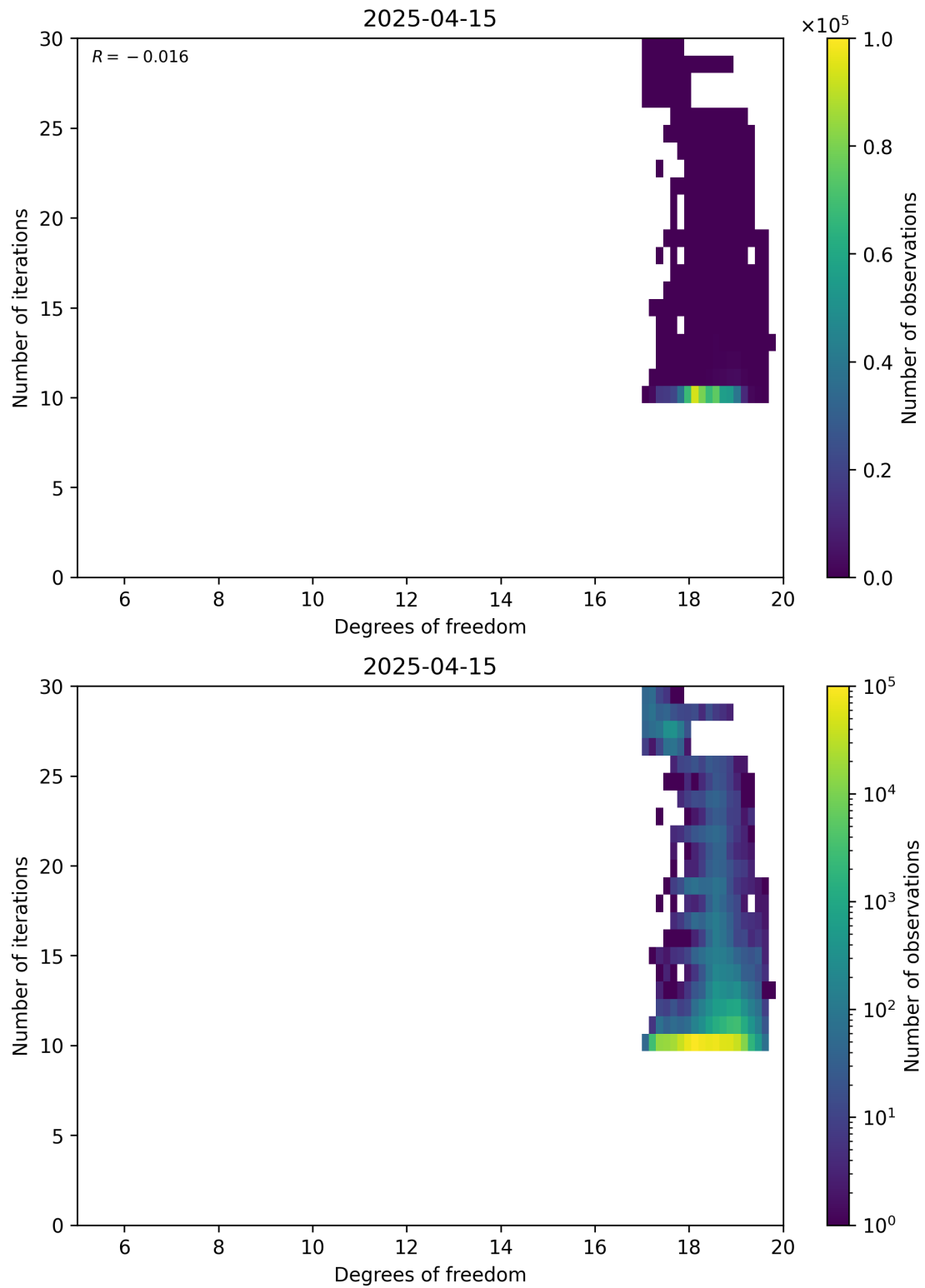
Figure 52: Scatter density plot of “Degrees of freedom” against “Number of iterations” for 2025-04-14 to 2025-04-16.
