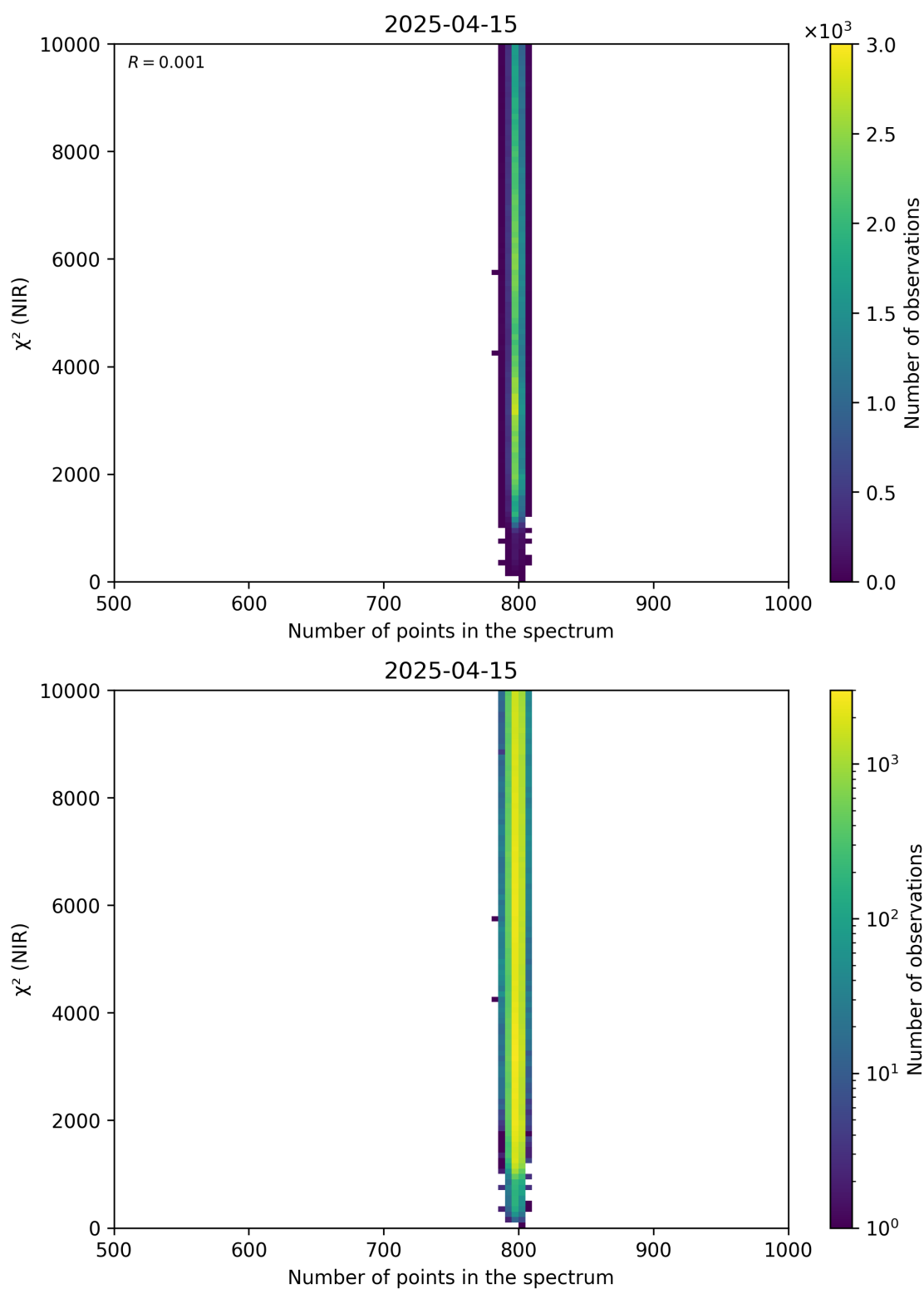
Figure 88: Scatter density plot of “Number of points in the spectrum” against “ \chi^2 (NIR)” for 2025-04-14 to 2025-04-16.
