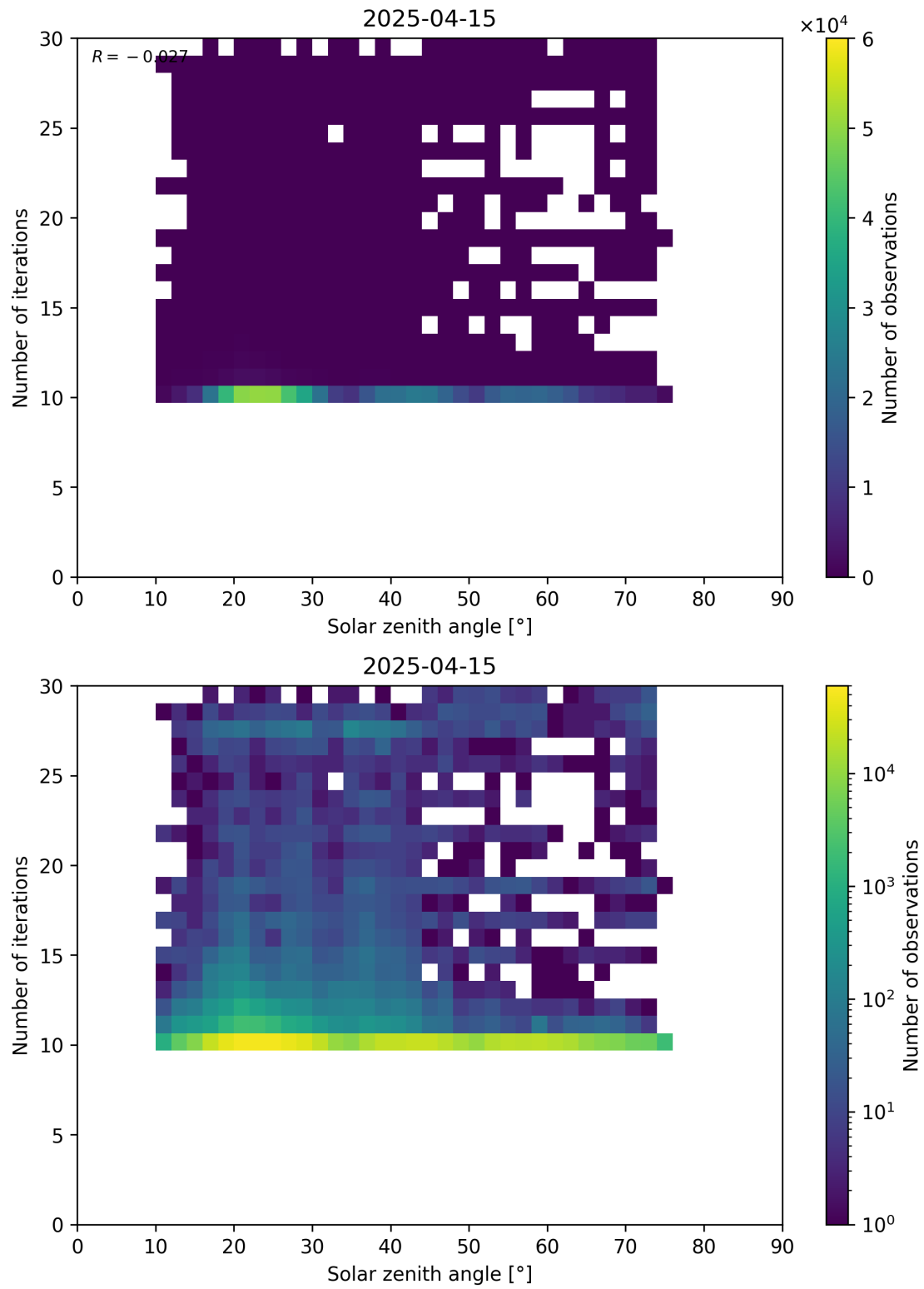
Figure 102: Scatter density plot of “Solar zenith angle” against “Number of iterations” for 2025-04-14 to 2025-04-16.
