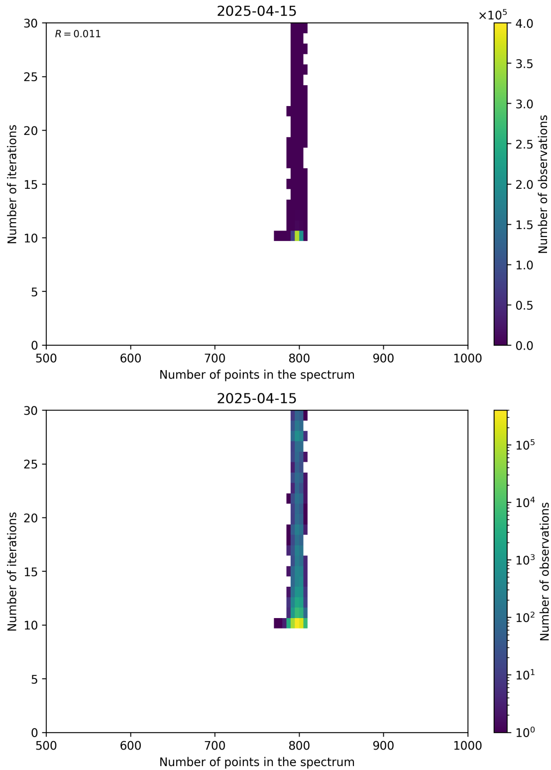
Figure 92: Scatter density plot of “Number of points in the spectrum” against “Number of iterations” for 2025-04-14 to 2025-04-16.
