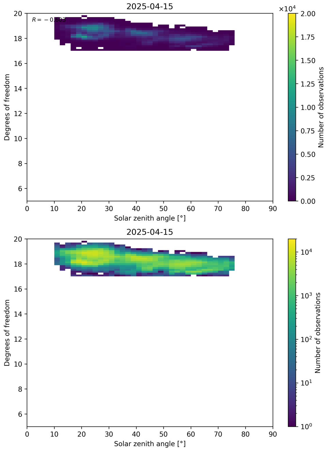
Figure 96: Scatter density plot of “Solar zenith angle” against “Degrees of freedom” for 2025-04-14 to 2025-04-16.
