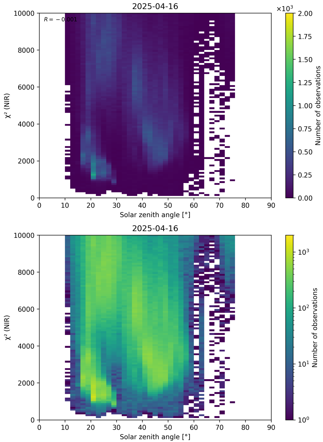
Figure 94: Scatter density plot of “Solar zenith angle” against “ \chi^2 (NIR)” for 2025-04-15 to 2025-04-17.
