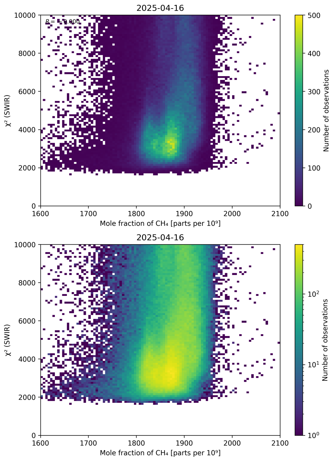
Figure 71: Scatter density plot of “Mole fraction of CH 4 ” against “ \chi^2 (SWIR)” for 2025-04-15 to 2025-04-17.
