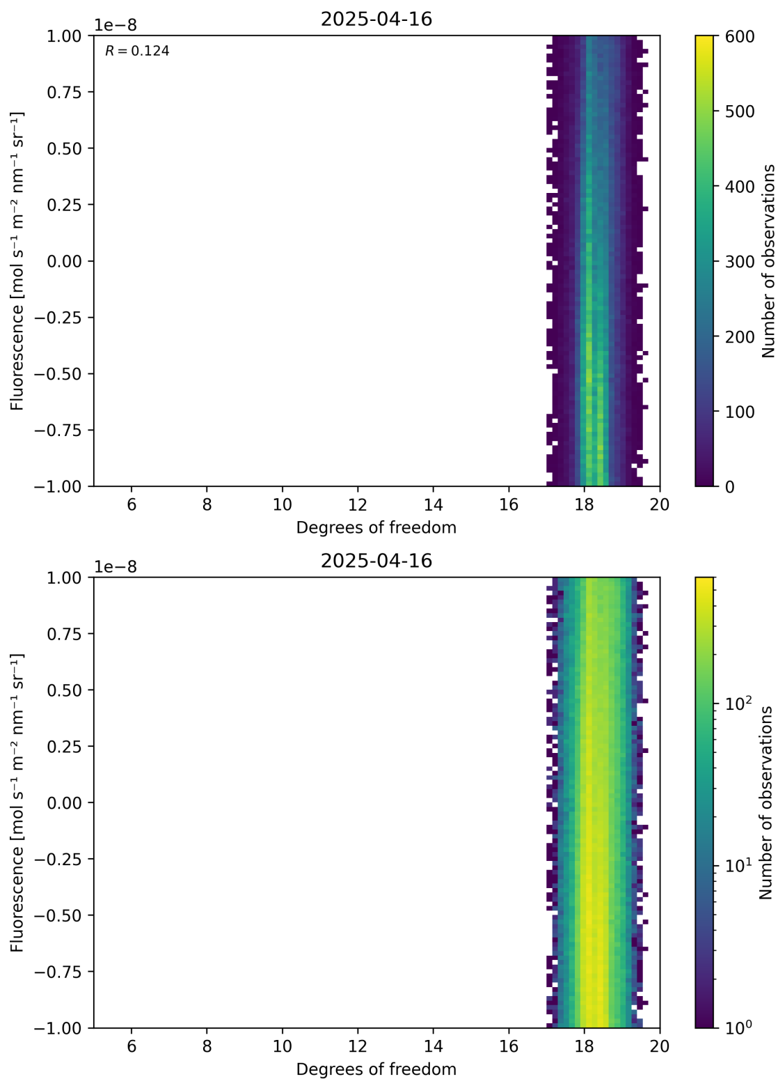
Figure 51: Scatter density plot of “Degrees of freedom” against “Fluorescence” for 2025-04-15 to 2025-04-17.
