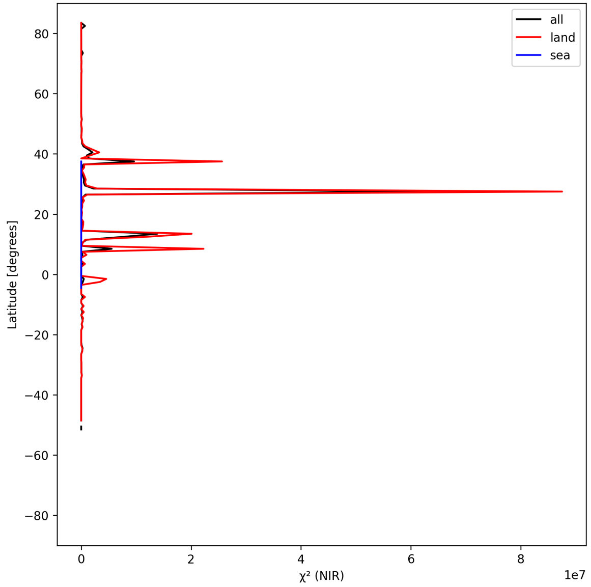
Figure 18: Zonal average of “ \chi^2 (NIR)” for 2025-04-15 to 2025-04-17.
