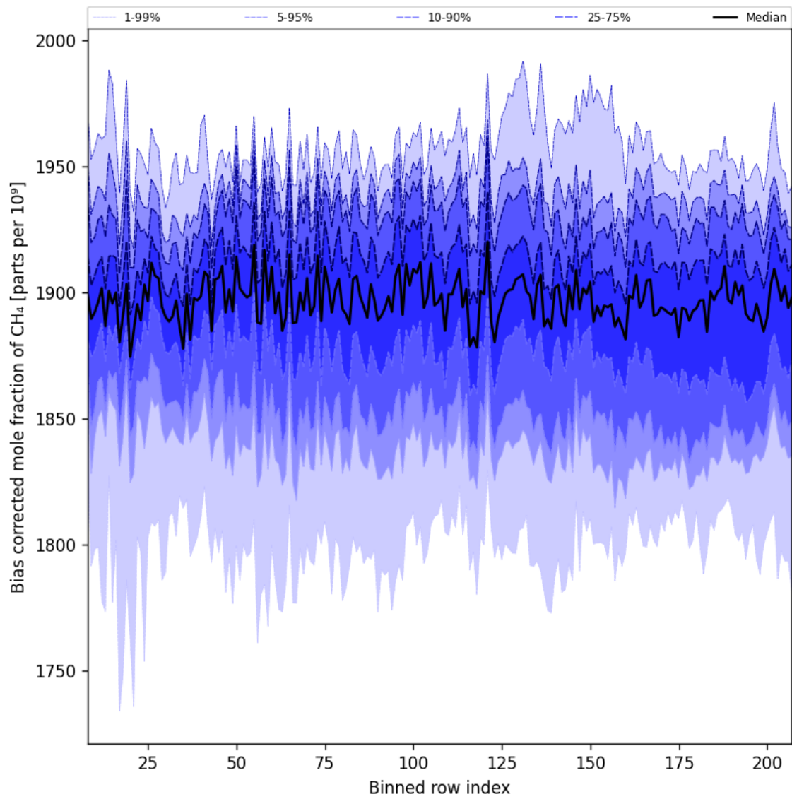
Figure 36: Along track statistics of “Bias corrected mole fraction of CH 4 ” for 2025-04-15 to 2025-04-17
