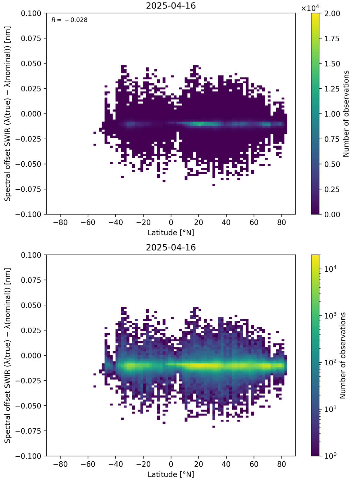
Figure 62: Scatter density plot of “Latitude” against “Spectral offset SWIR ( \lambda_{\text{true}} - \lambda_{\text{nominal}} )” for 2025-04-15 to 2025-04-17.
