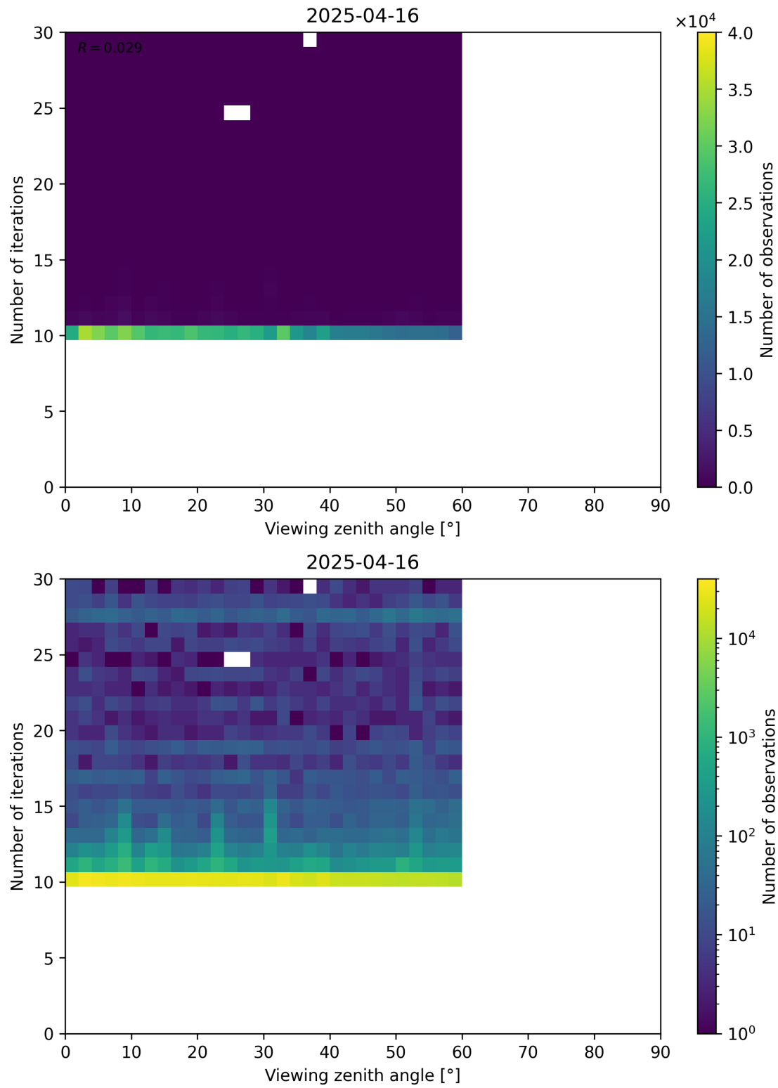
Figure 113: Scatter density plot of “Viewing zenith angle” against “Number of iterations” for 2025-04-15 to 2025-04-17.
