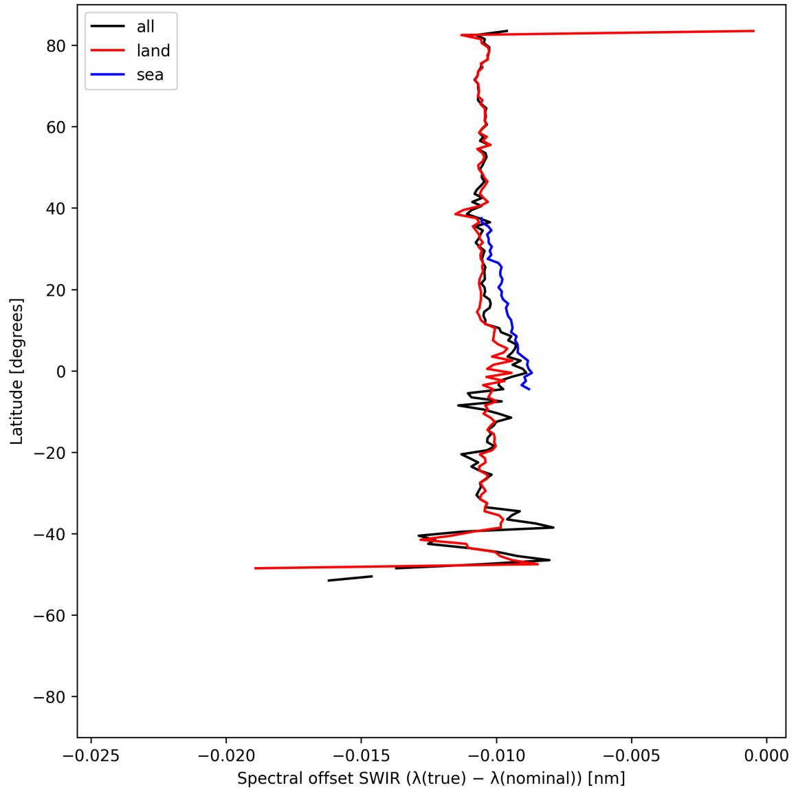
Figure 16: Zonal average of “Spectral offset SWIR ( \lambda_{\text{true}} - \lambda_{\text{nominal}} )” for 2025-04-15 to 2025-04-17.
