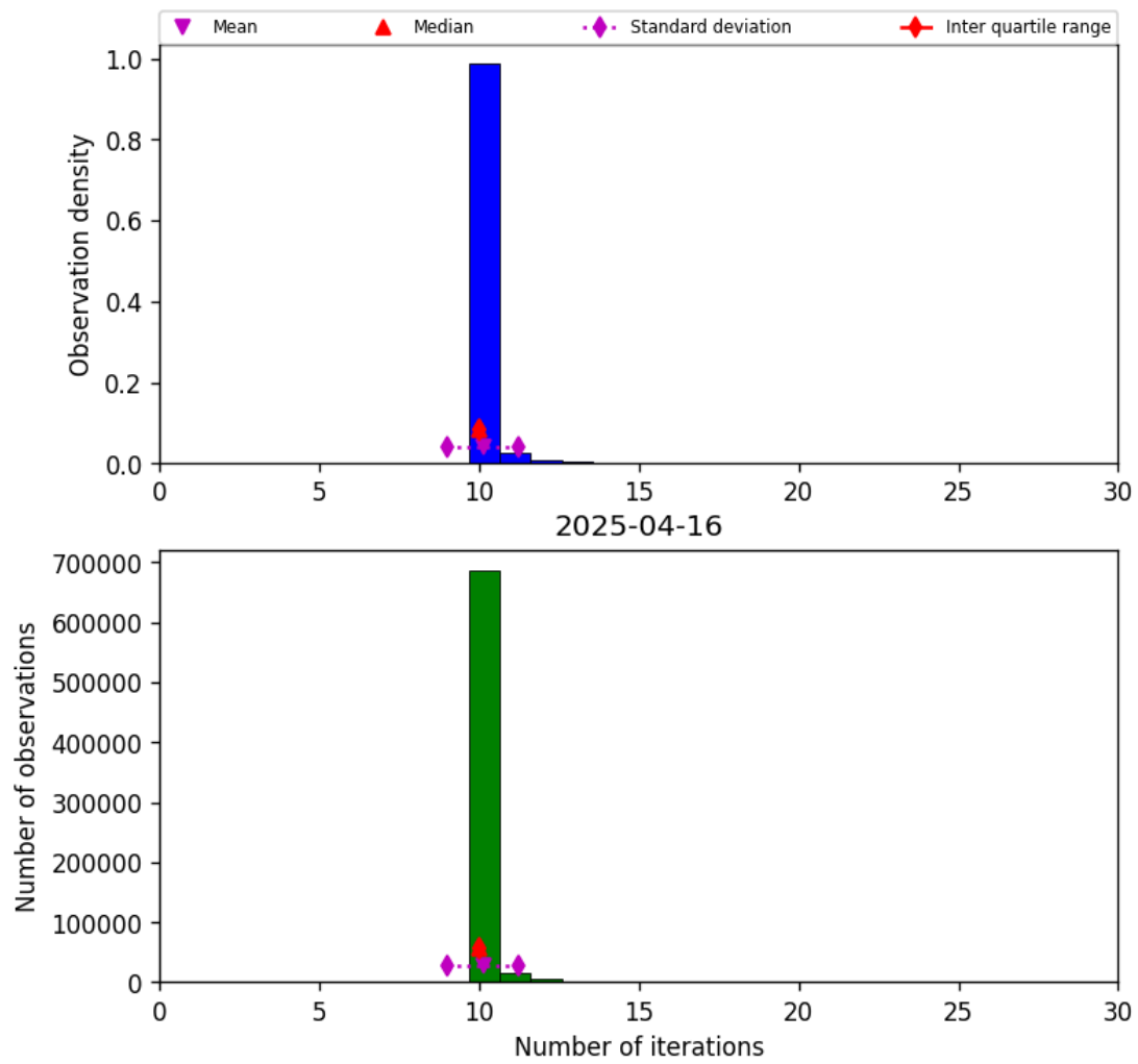
Figure 31: Histogram of “Number of iterations” for 2025-04-15 to 2025-04-17
