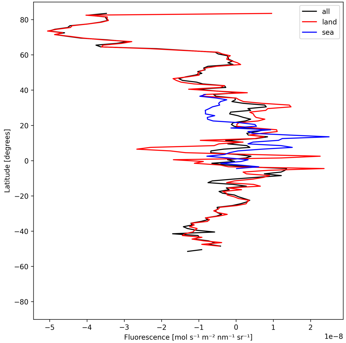
Figure 21: Zonal average of “Fluorescence” for 2025-04-15 to 2025-04-17.
