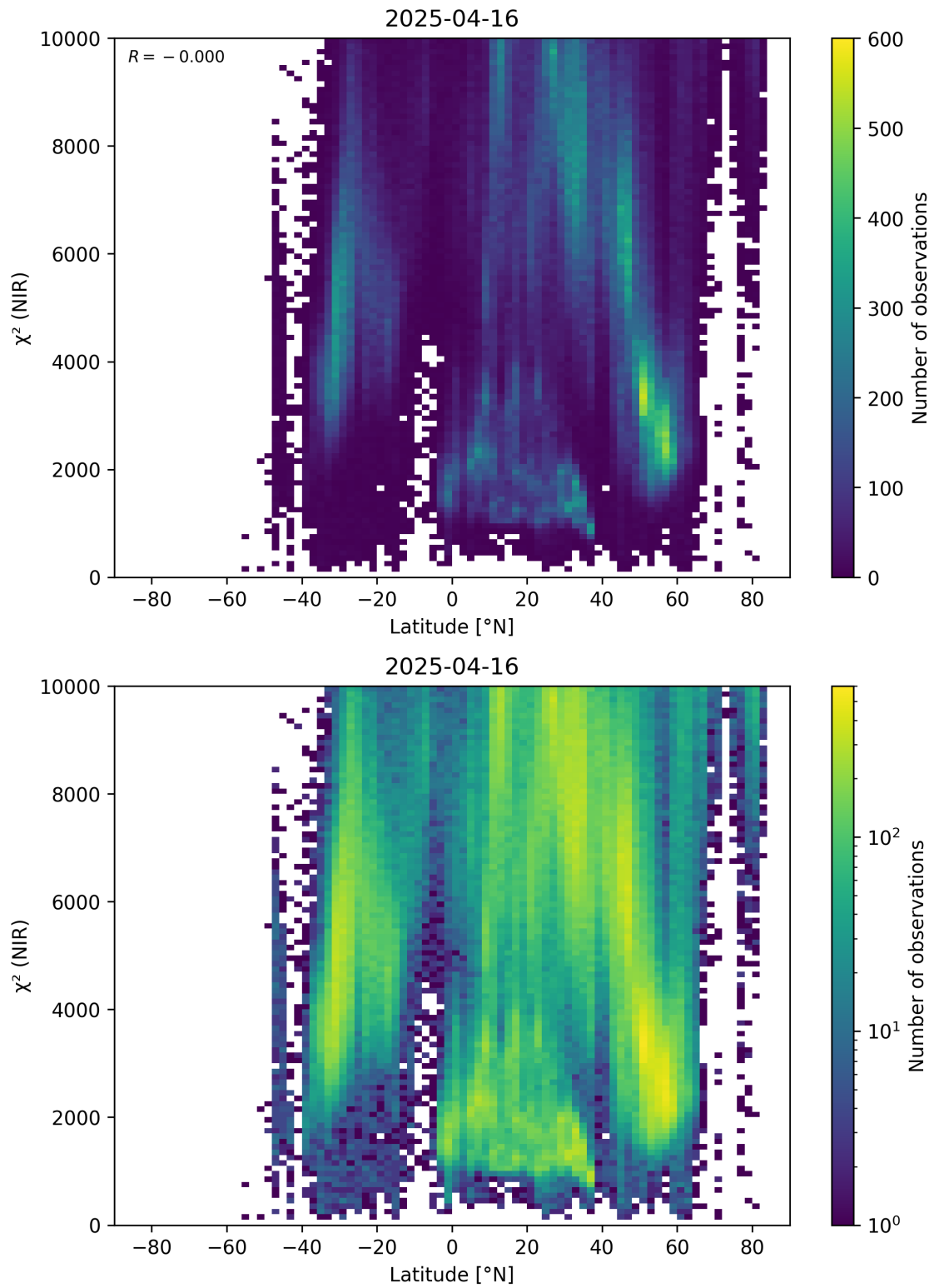
Figure 53: Scatter density plot of “Latitude” against “ \chi^2 (NIR)” for 2025-04-15 to 2025-04-17.
