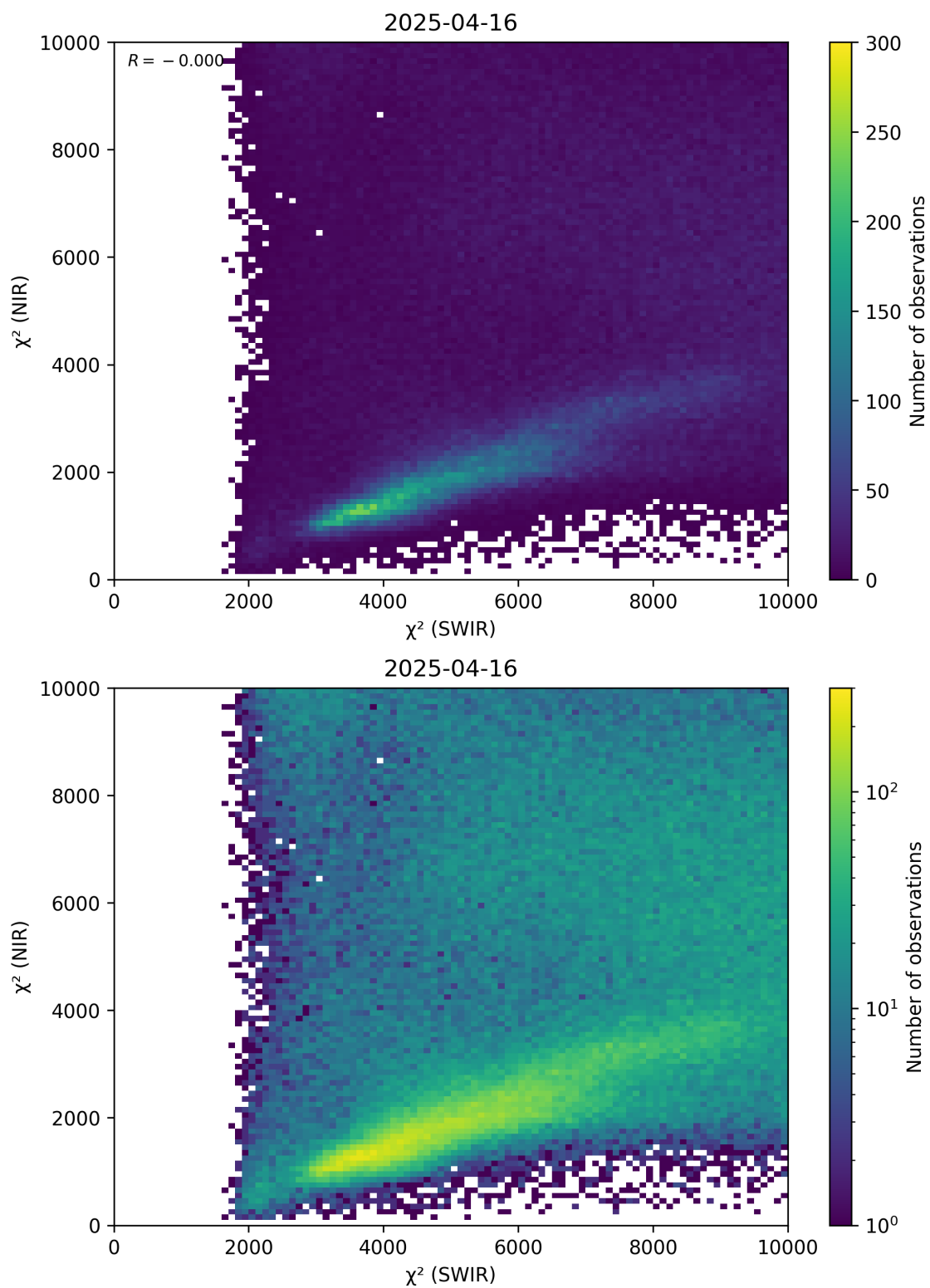
Figure 47: Scatter density plot of “ \chi^2 (SWIR)” against “ \chi^2 (NIR)” for 2025-04-15 to 2025-04-17.
