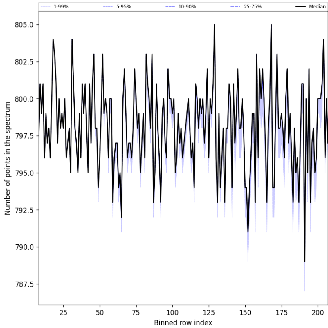
Figure 37: Along track statistics of “Number of points in the spectrum” for 2025-04-15 to 2025-04-17
