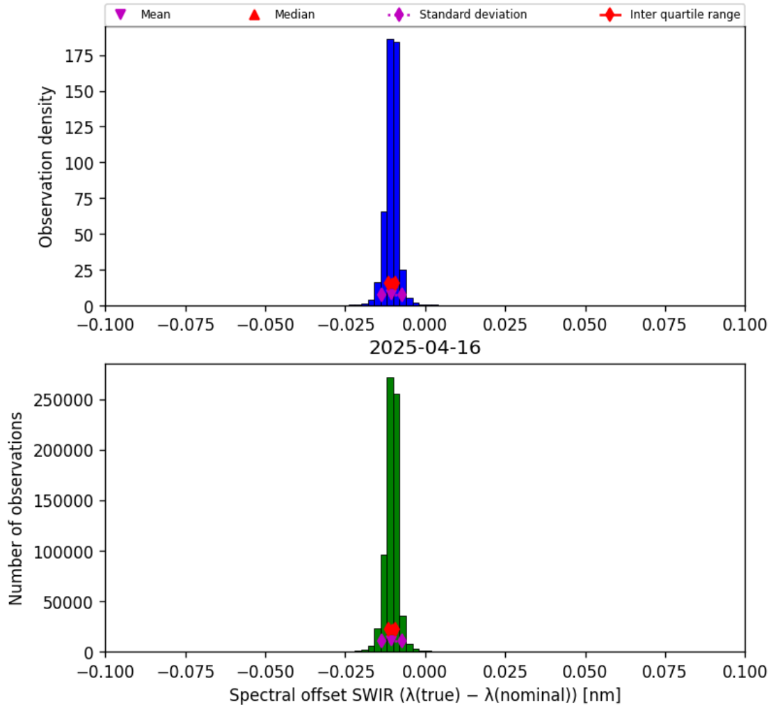
Figure 27: Histogram of “Spectral offset SWIR ( \lambda_{\text{true}} - \lambda_{\text{nominal}} )” for 2025-04-15 to 2025-04-17
