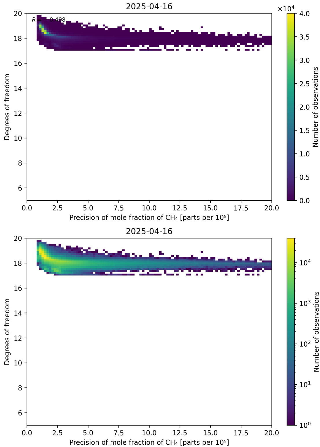
Figure 80: Scatter density plot of “Precision of mole fraction of CH 4 ” against “Degrees of freedom” for 2025-04-15 to 2025-04-17.
