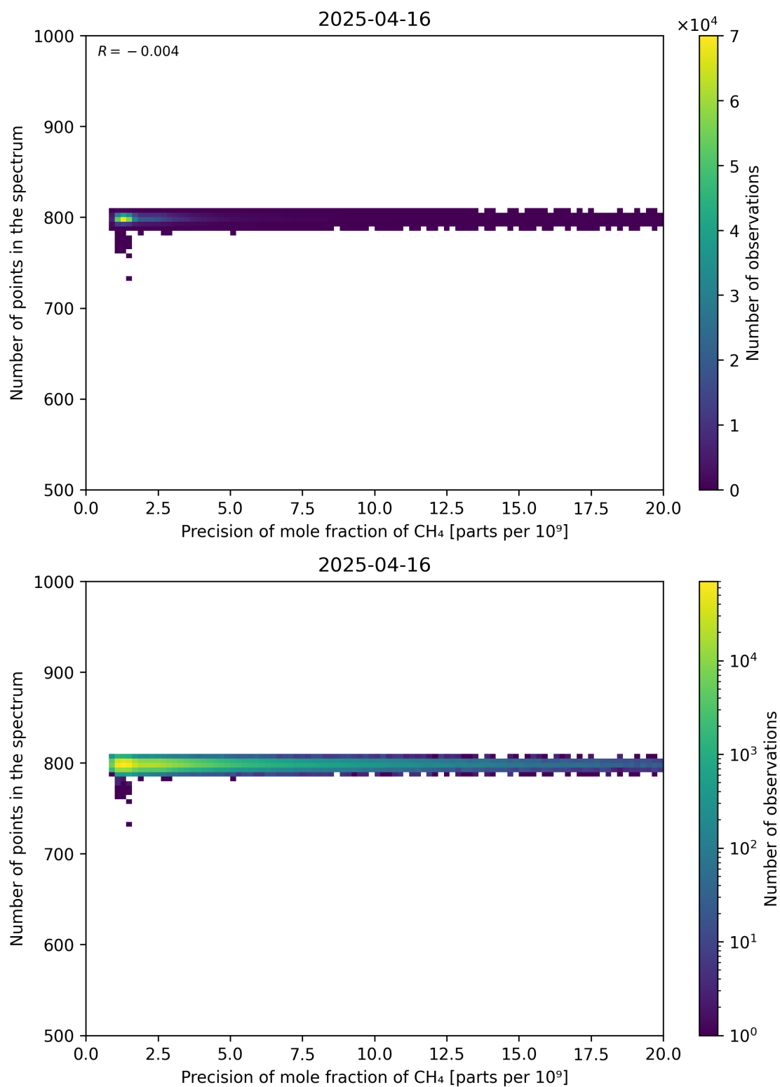
Figure 84: Scatter density plot of “Precision of mole fraction of CH 4 ” against “Number of points in the spectrum” for 2025-04-15 to 2025-04-17.
