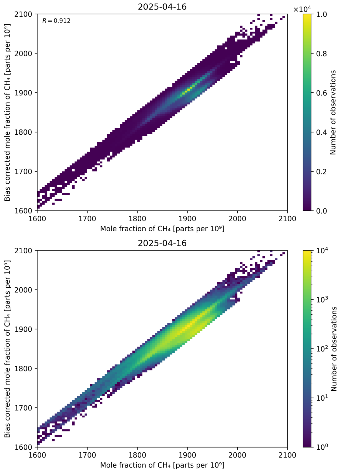
Figure 74: Scatter density plot of “Mole fraction of CH 4 ” against “Bias corrected mole fraction of CH 4 ” for 2025-04-15 to 2025-04-17.
