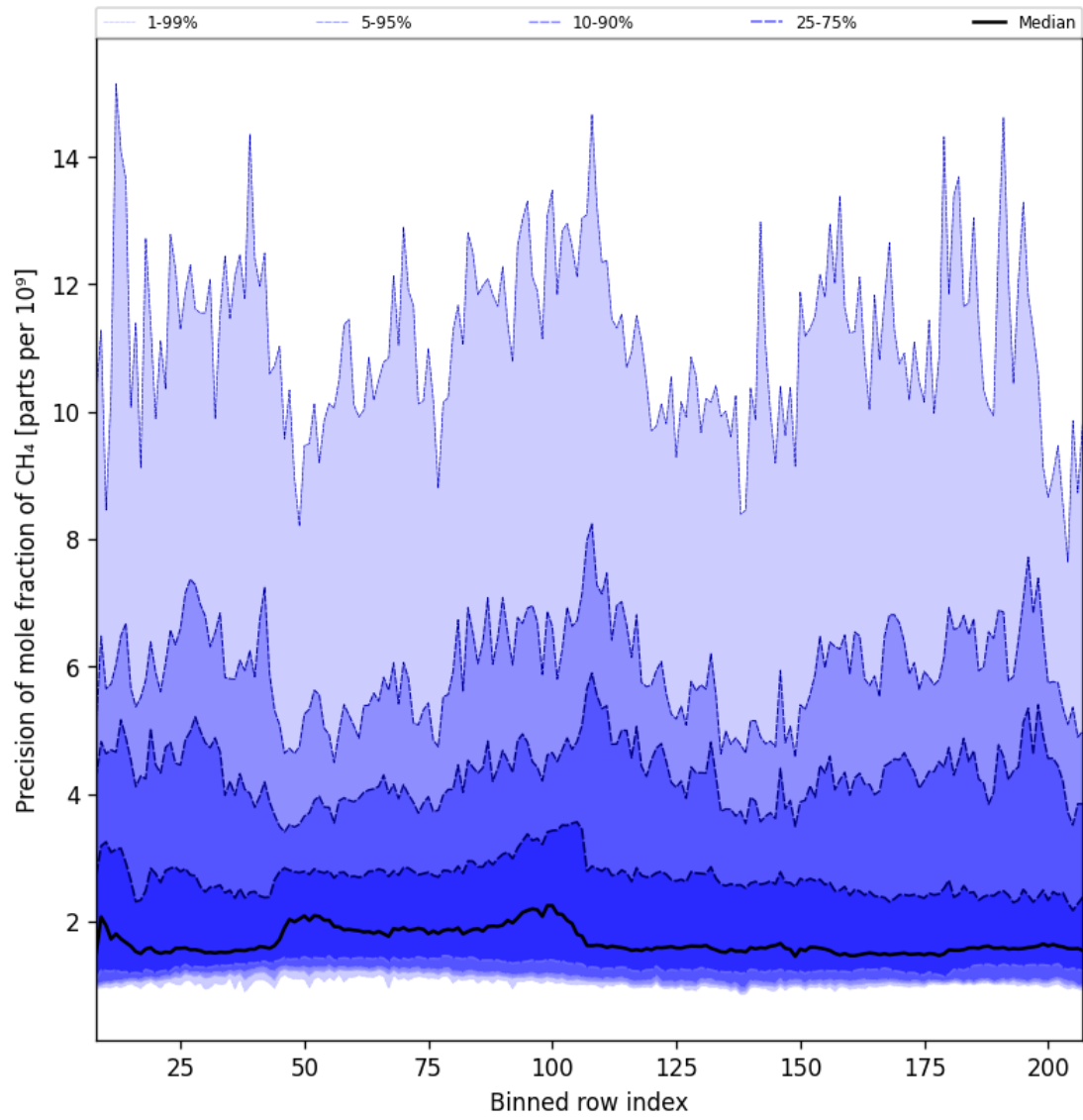
Figure 35: Along track statistics of “Precision of mole fraction of CH 4 ” for 2025-04-15 to 2025-04-17
