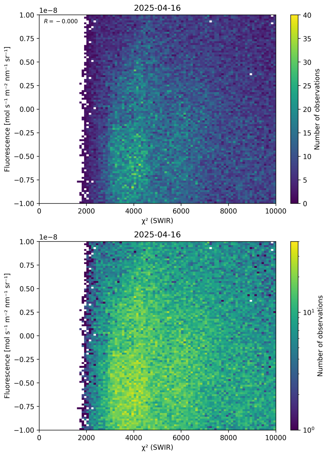
Figure 49: Scatter density plot of “ \chi^2 (SWIR)” against “Fluorescence” for 2025-04-15 to 2025-04-17.
