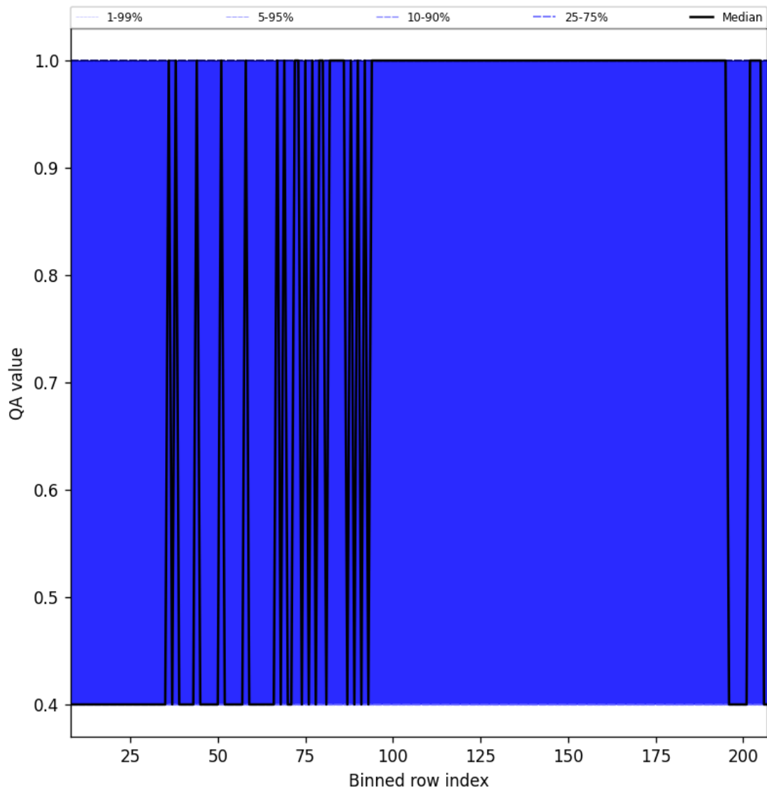
Figure 33: Along track statistics of “QA value” for 2025-04-15 to 2025-04-17
