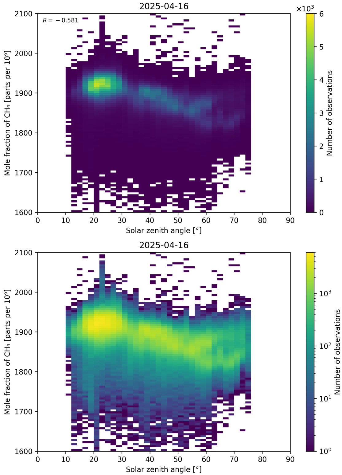
Figure 99: Scatter density plot of “Solar zenith angle” against “Mole fraction of CH 4 ” for 2025-04-15 to 2025-04-17.
