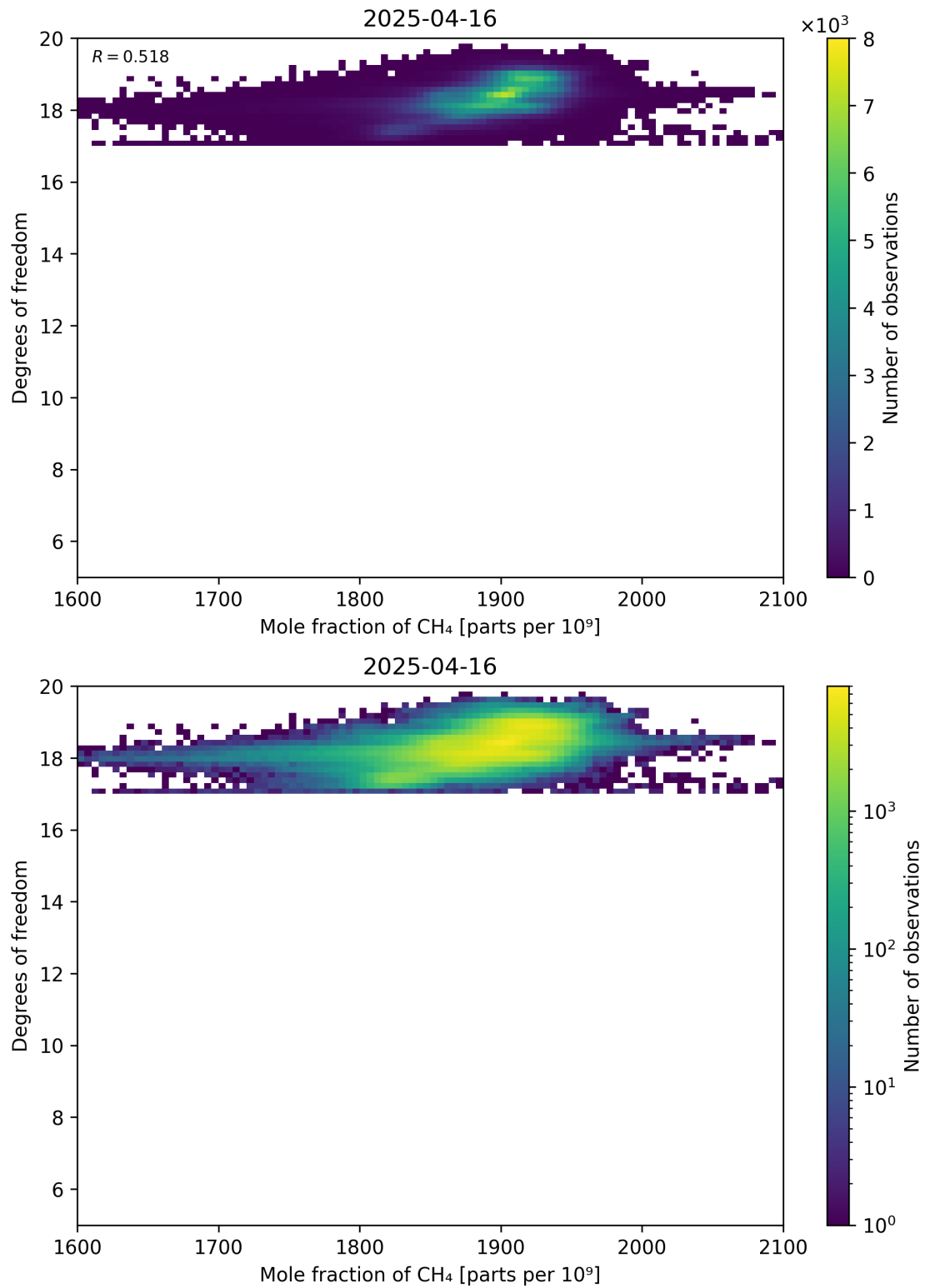
Figure 72: Scatter density plot of “Mole fraction of CH 4 ” against “Degrees of freedom” for 2025-04-15 to 2025-04-17.
