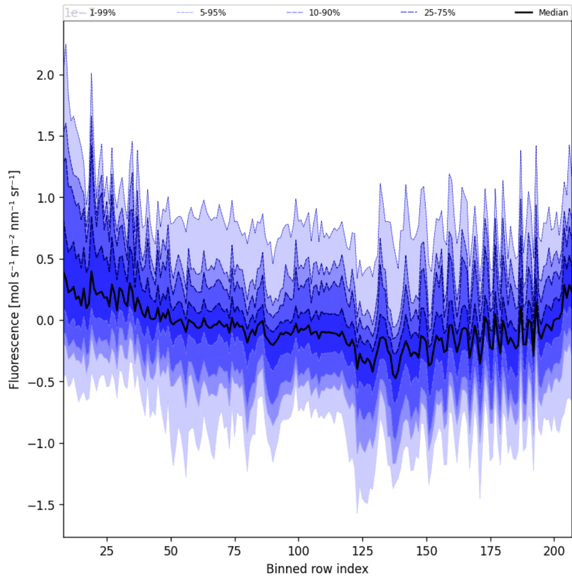
Figure 43: Along track statistics of “Fluorescence” for 2025-04-15 to 2025-04-17
