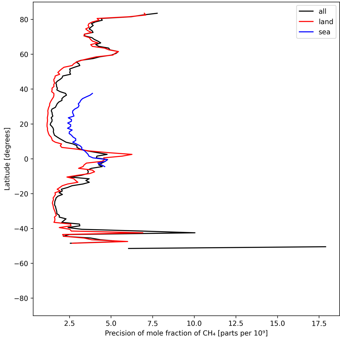
Figure 13: Zonal average of “Precision of mole fraction of CH 4 ” for 2025-04-15 to 2025-04-17.
