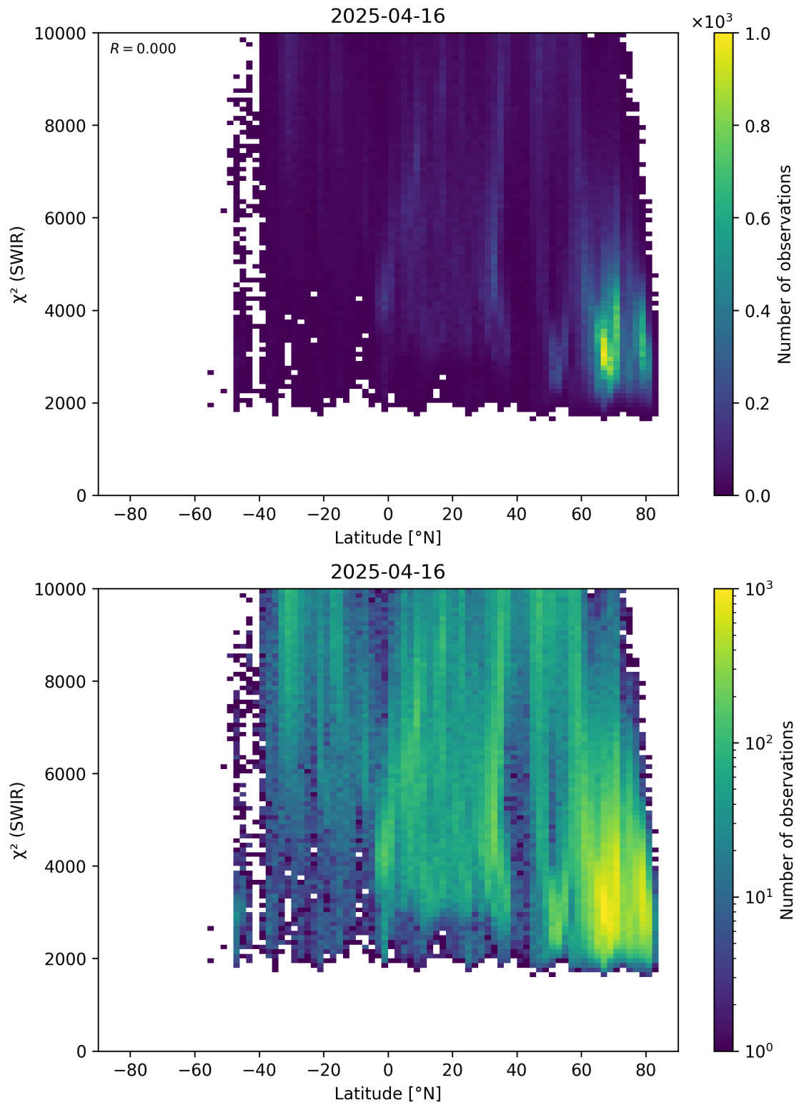
Figure 54: Scatter density plot of “Latitude” against “ \chi^2 (SWIR)” for 2025-04-15 to 2025-04-17.
