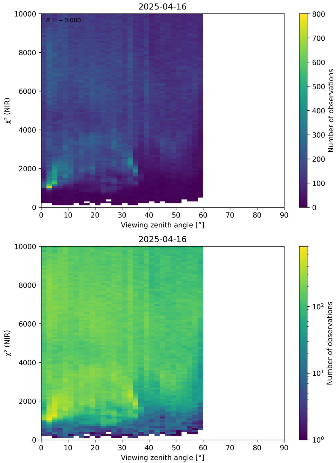
Figure 105: Scatter density plot of “Viewing zenith angle” against “ \chi^2 (NIR)” for 2025-04-15 to 2025-04-17.
