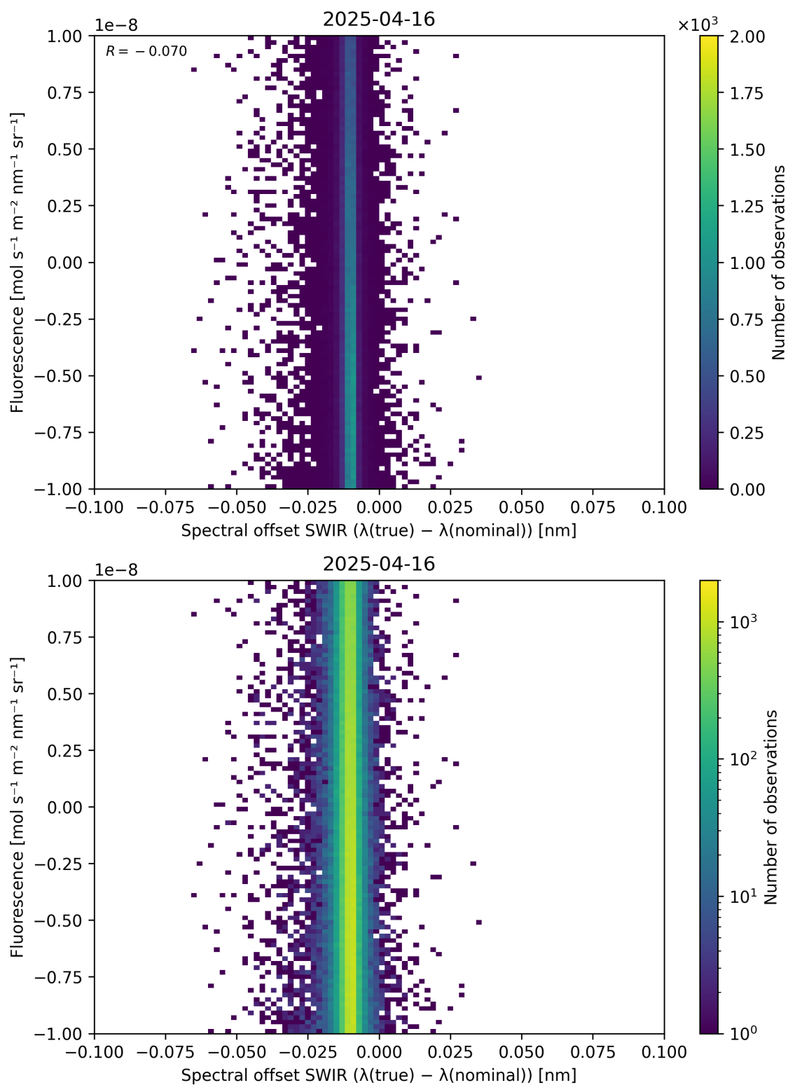
Figure 120: Scatter density plot of “Spectral offset SWIR ( \lambda_{\text{true}} - \lambda_{\text{nominal}} )” against “Fluorescence” for 2025-04-15 to 2025-04-17.
