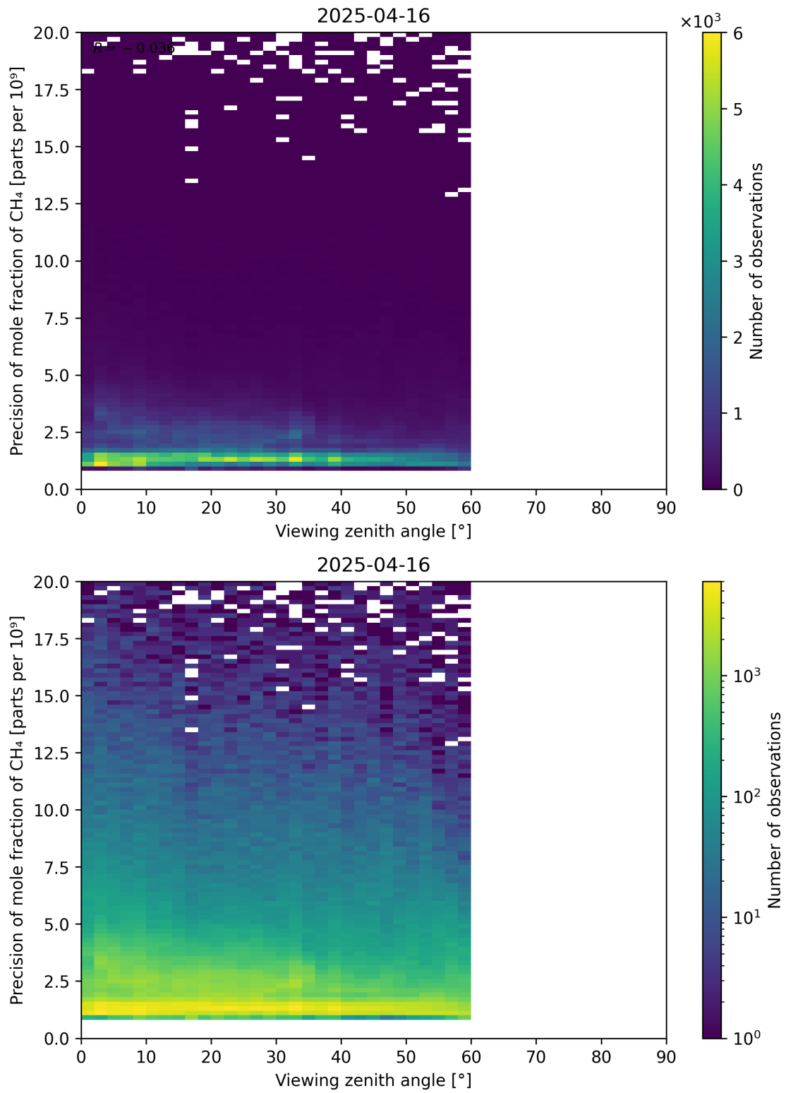
Figure 112: Scatter density plot of “Viewing zenith angle” against “Precision of mole fraction of CH 4 ” for 2025-04-15 to 2025-04-17.
