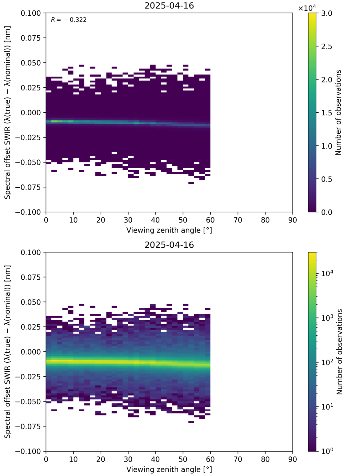
Figure 116: Scatter density plot of “Viewing zenith angle” against “Spectral offset SWIR ( \lambda_{\text{true}} - \lambda_{\text{nominal}} )” for 2025-04-15 to 2025-04-17.
