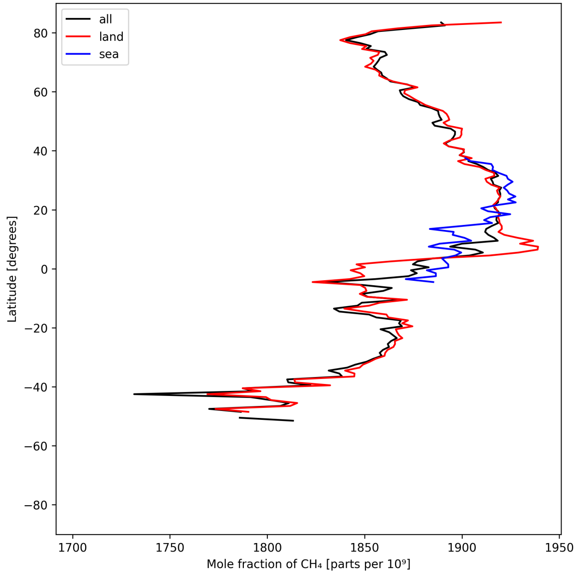
Figure 12: Zonal average of “Mole fraction of \text{CH}_4 ” for 2025-04-15 to 2025-04-17.
