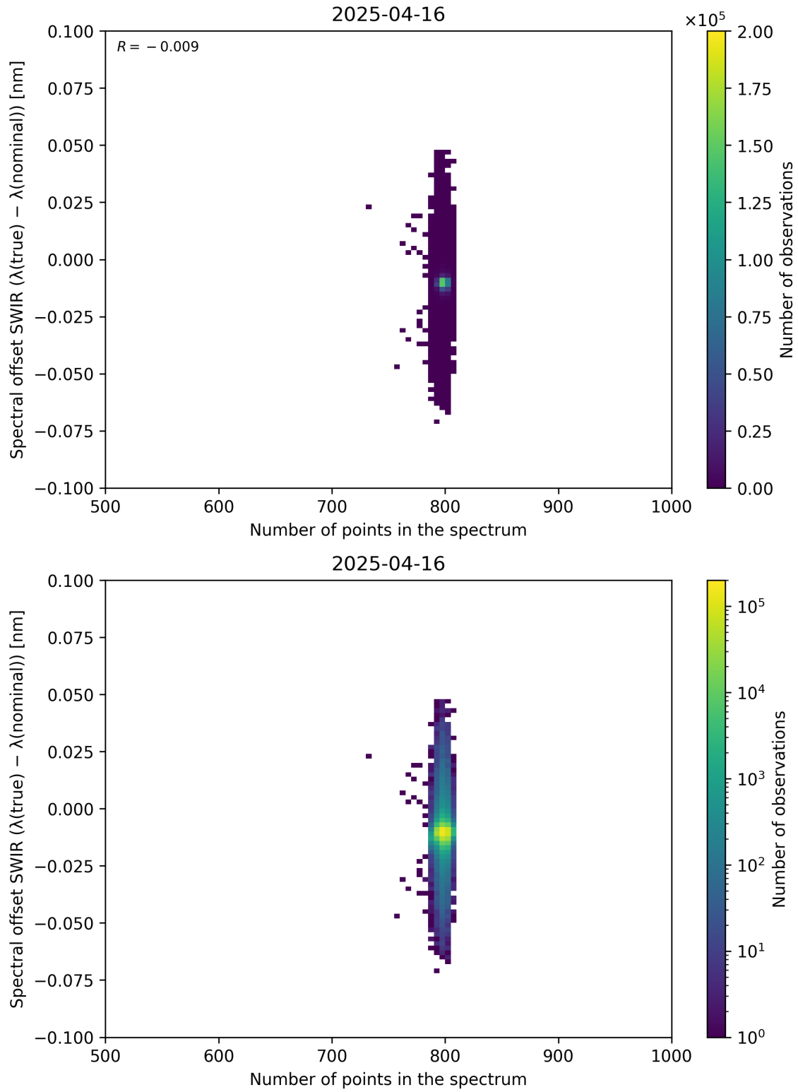
Figure 93: Scatter density plot of “Number of points in the spectrum” against “Spectral offset SWIR ( \lambda_{\text{true}} - \lambda_{\text{nominal}} )” for 2025-04-15 to 2025-04-17.
