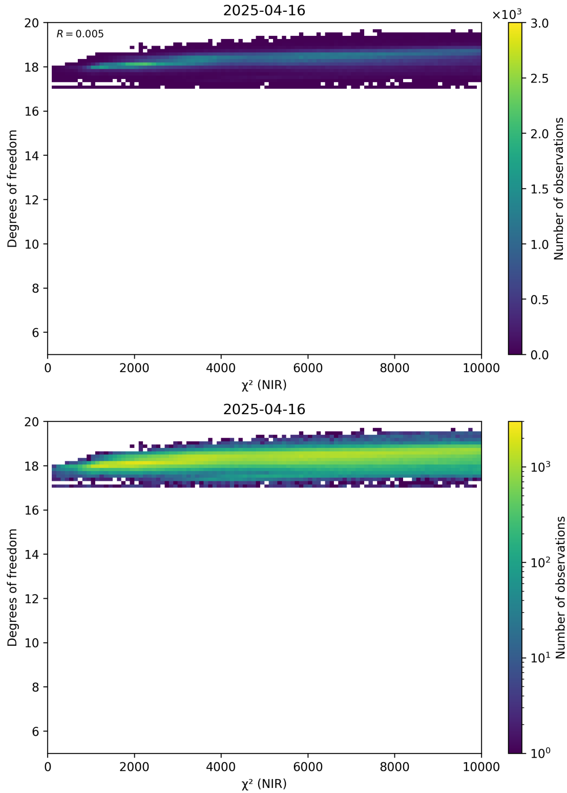
Figure 44: Scatter density plot of “ \chi^2 (NIR)” against “Degrees of freedom” for 2025-04-15 to 2025-04-17.
