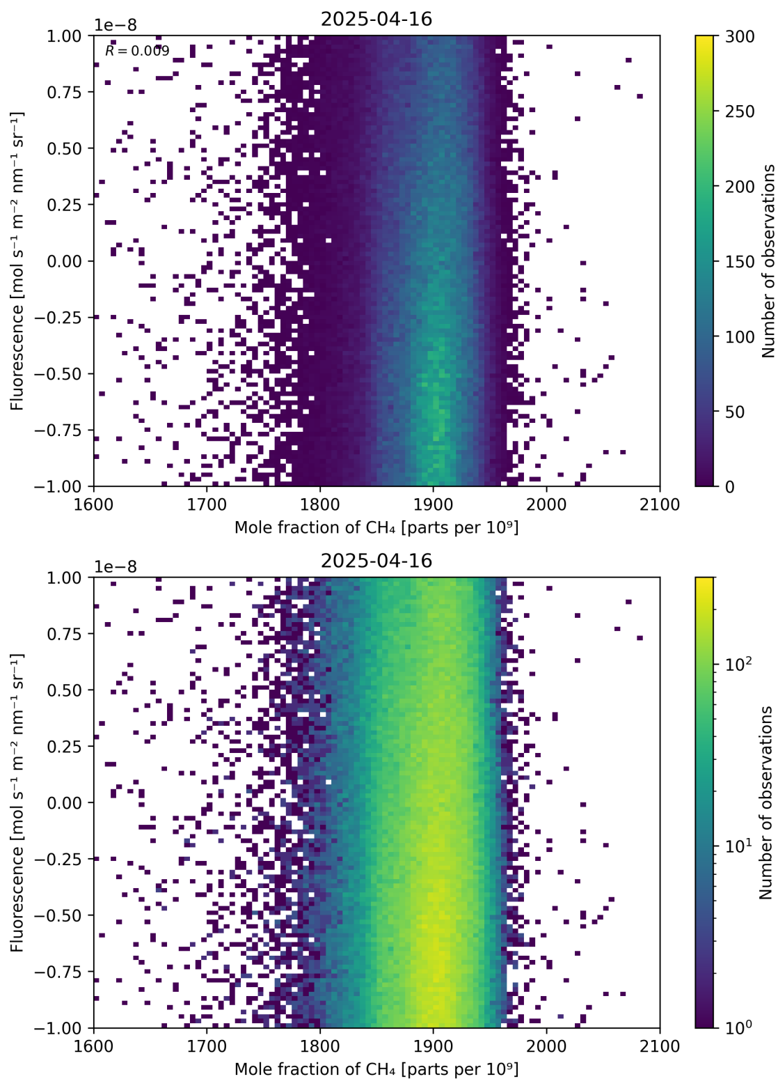
Figure 73: Scatter density plot of “Mole fraction of \text{CH}_4 ” against “Fluorescence” for 2025-04-15 to 2025-04-17.
