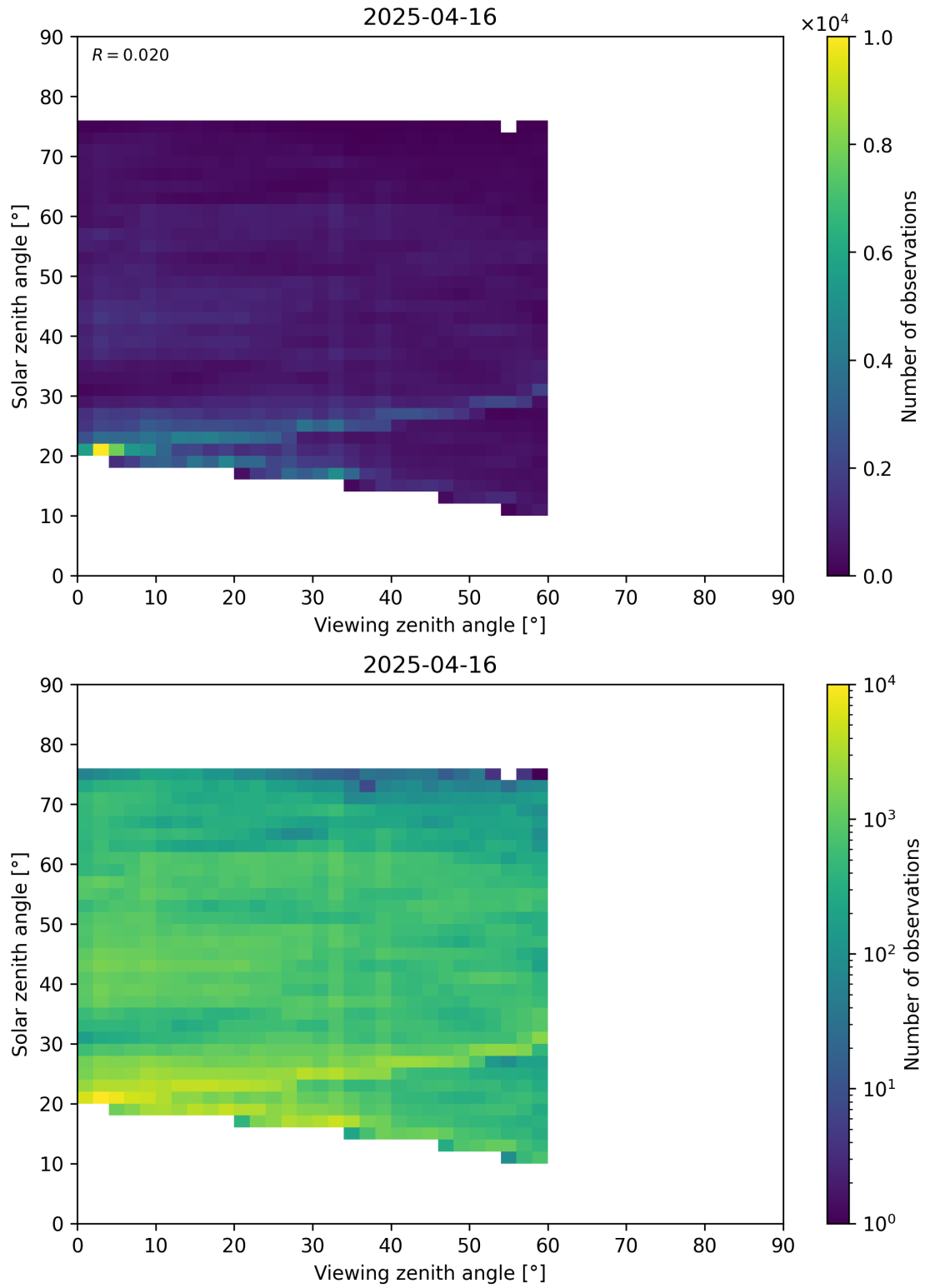
Figure 115: Scatter density plot of “Viewing zenith angle” against “Solar zenith angle” for 2025-04-15 to 2025-04-17.
