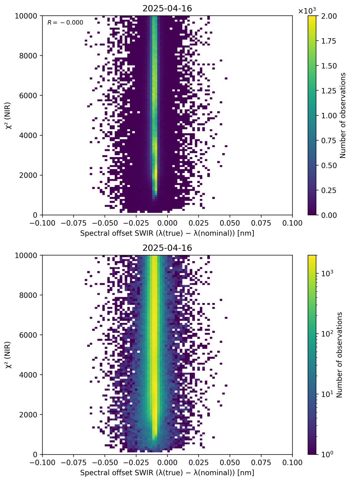
Figure 117: Scatter density plot of “Spectral offset SWIR ( \lambda_{\text{true}} - \lambda_{\text{nominal}} )” against “ \chi^2 (NIR)” for 2025-04-15 to 2025-04-17.
