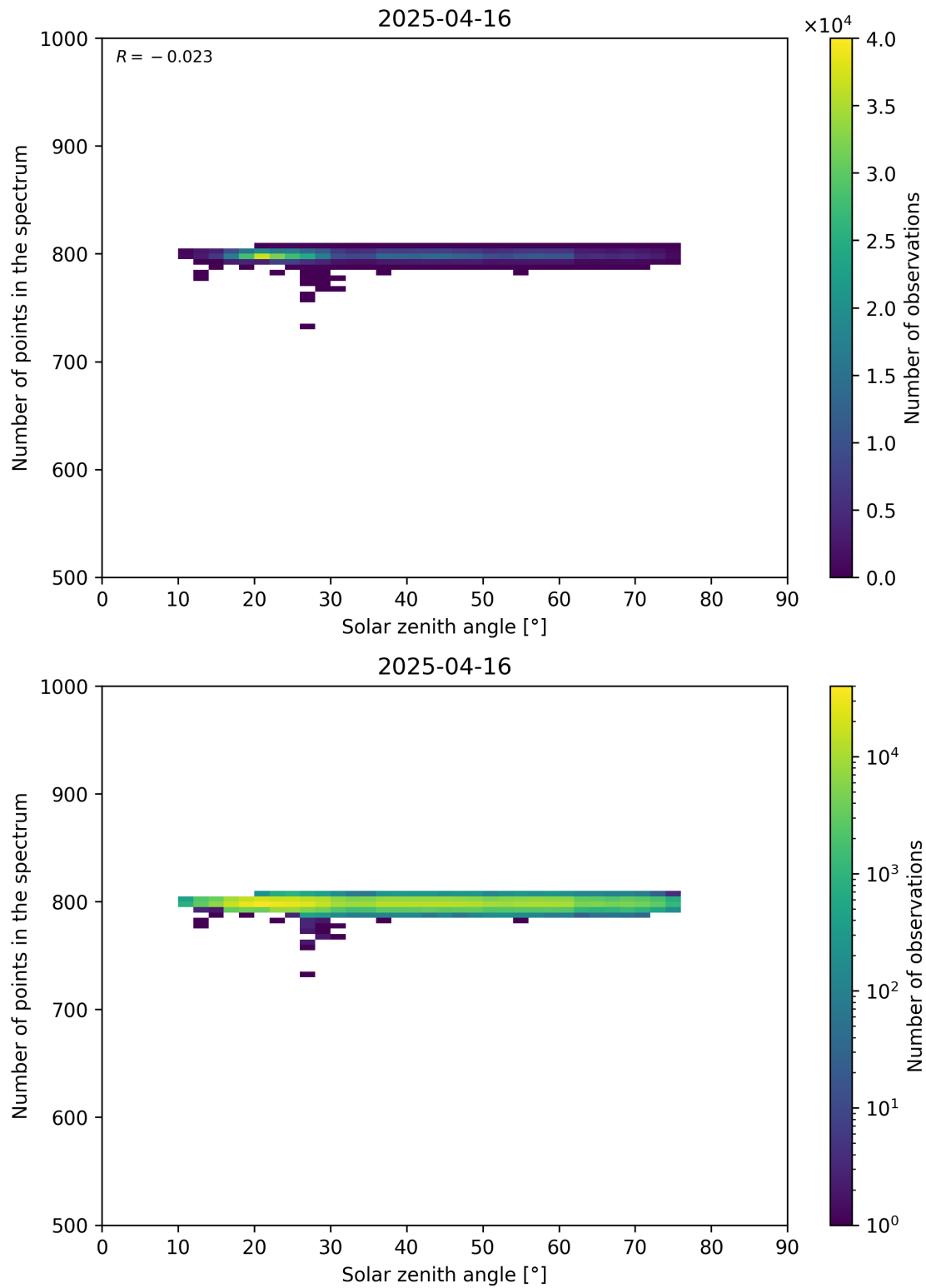
Figure 103: Scatter density plot of “Solar zenith angle” against “Number of points in the spectrum” for 2025-04-15 to 2025-04-17.
