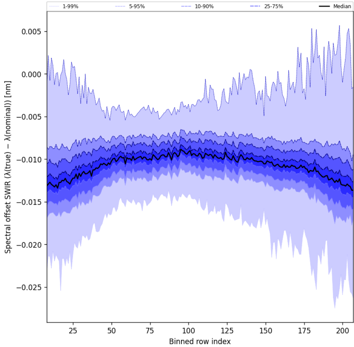
Figure 38: Along track statistics of “Spectral offset SWIR ( \lambda_{\text{true}} - \lambda_{\text{nominal}} )” for 2025-04-15 to 2025-04-17
