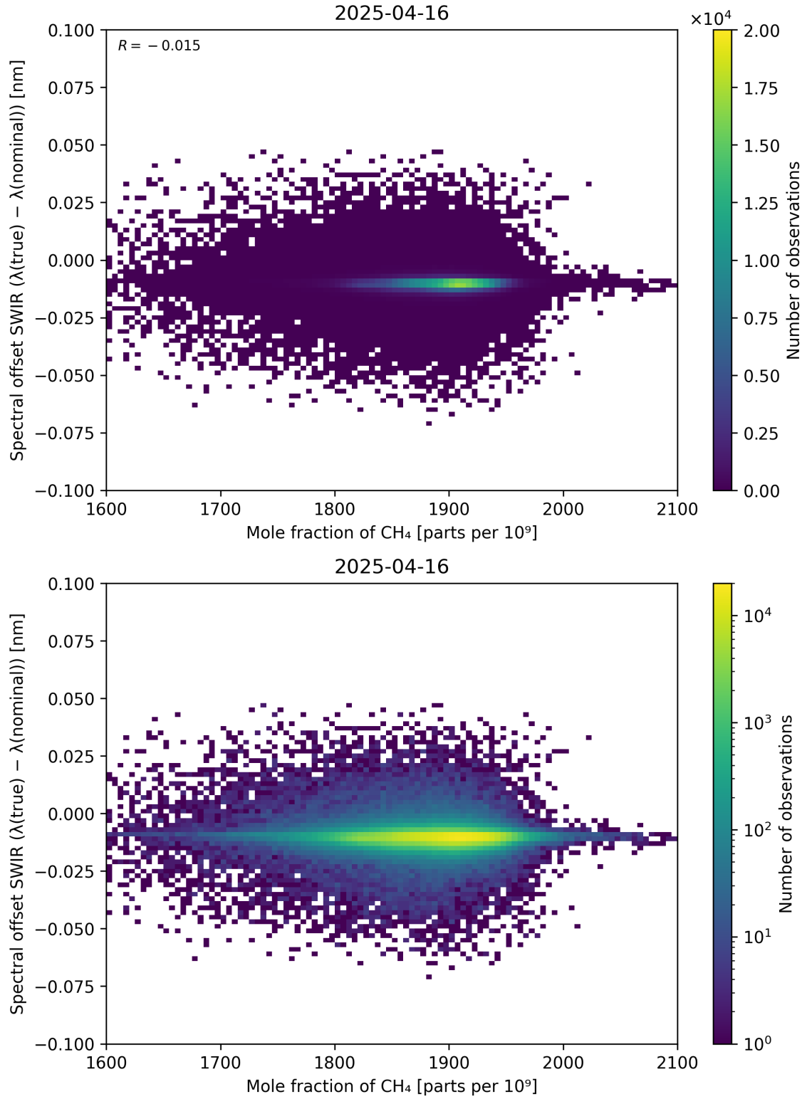
Figure 86: Scatter density plot of “Mole fraction of CH 4 ” against “Spectral offset SWIR ( \lambda_{\text{true}} - \lambda_{\text{nominal}} )” for 2025-04-15 to 2025-04-17.
