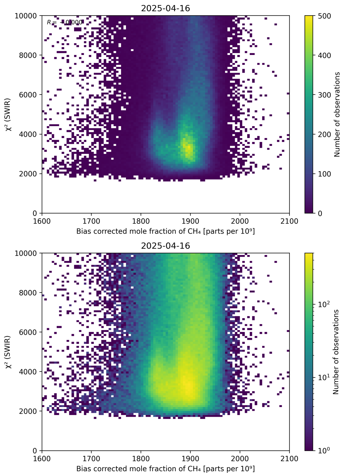
Figure 64: Scatter density plot of “Bias corrected mole fraction of \text{CH}_4 ” against “ \chi^2 (SWIR)” for 2025-04-15 to 2025-04-17.
