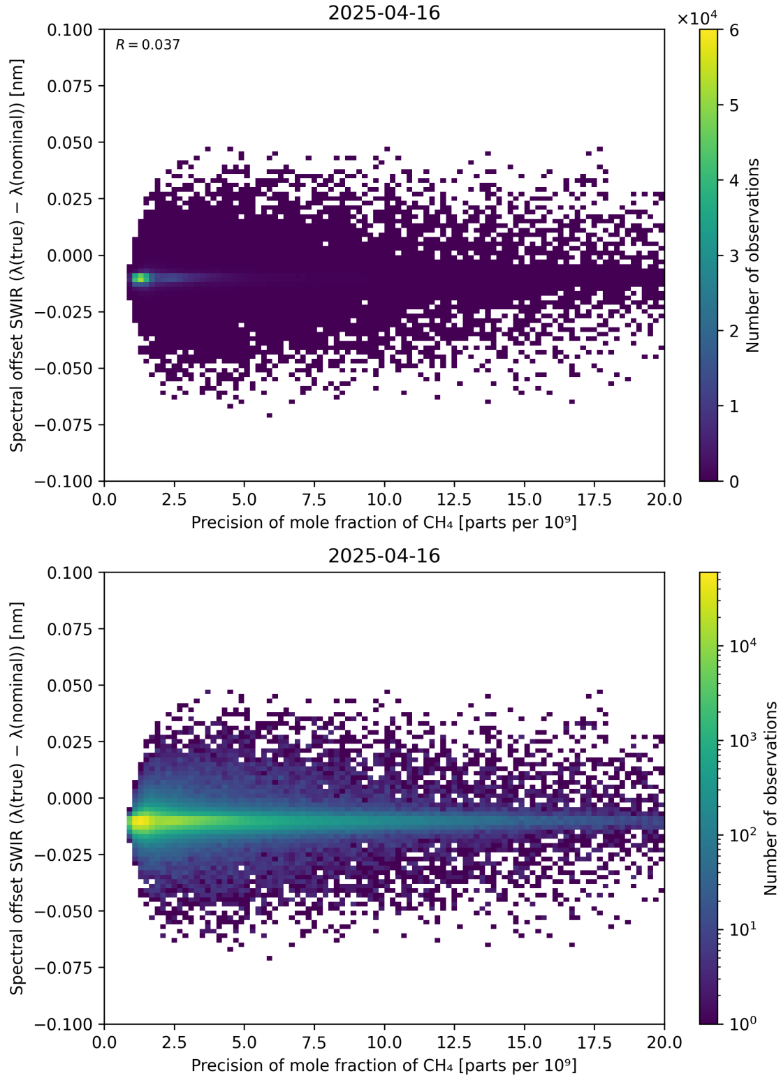
Figure 85: Scatter density plot of “Precision of mole fraction of CH 4 ” against “Spectral offset SWIR ( \lambda_{\text{true}} - \lambda_{\text{nominal}} )” for 2025-04-15 to 2025-04-17.
