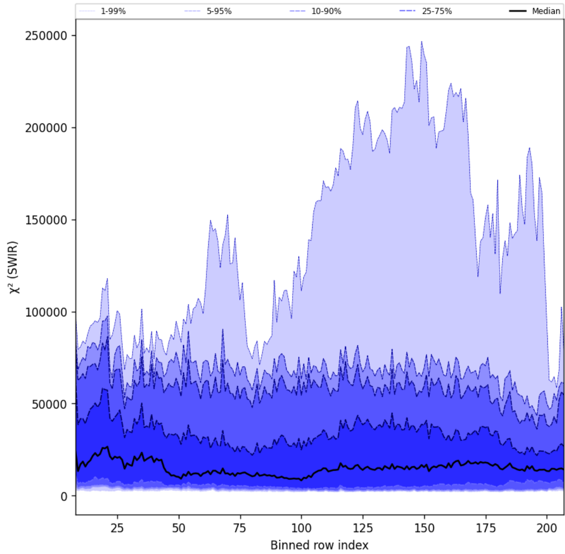
Figure 39: Along track statistics of “ \chi^2 (SWIR)” for 2025-04-15 to 2025-04-17
