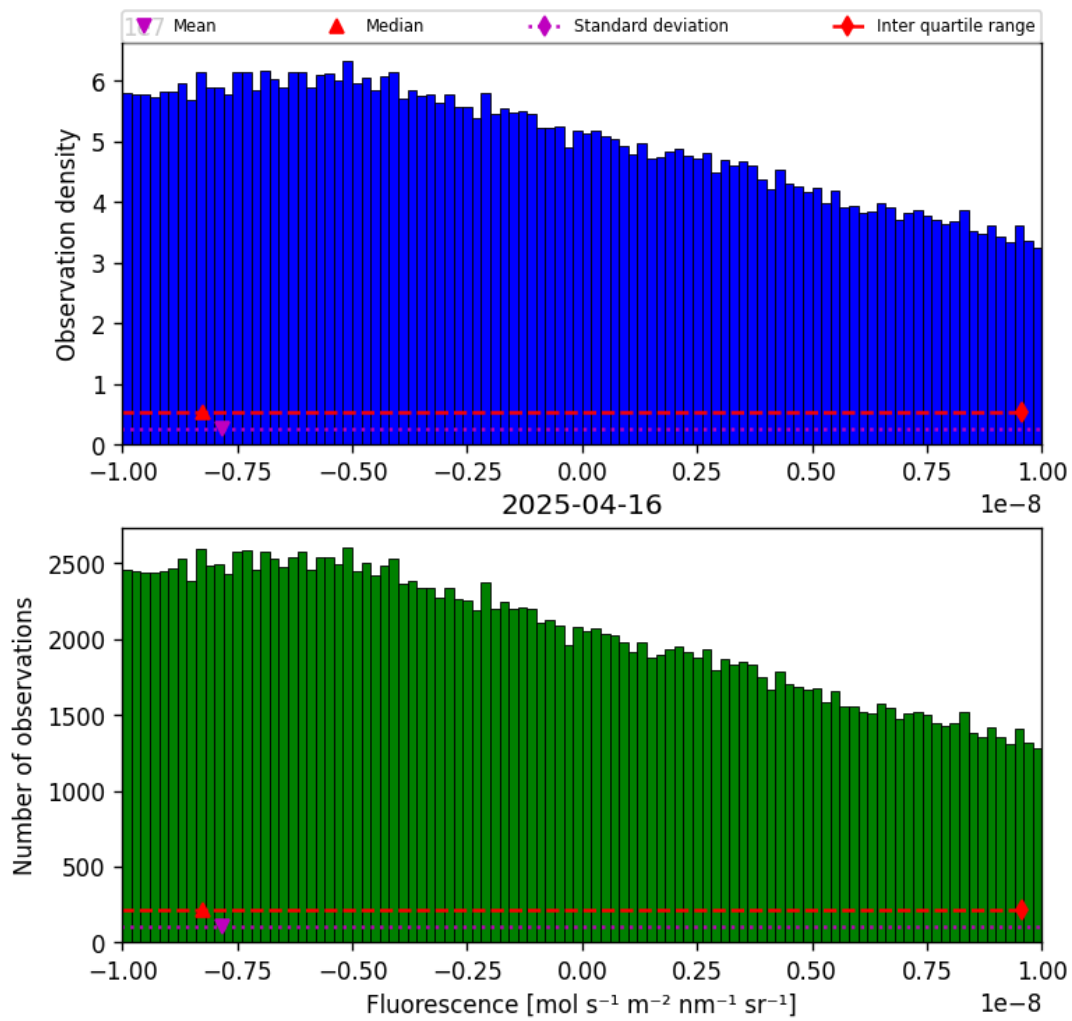
Figure 32: Histogram of “Fluorescence” for 2025-04-15 to 2025-04-17
