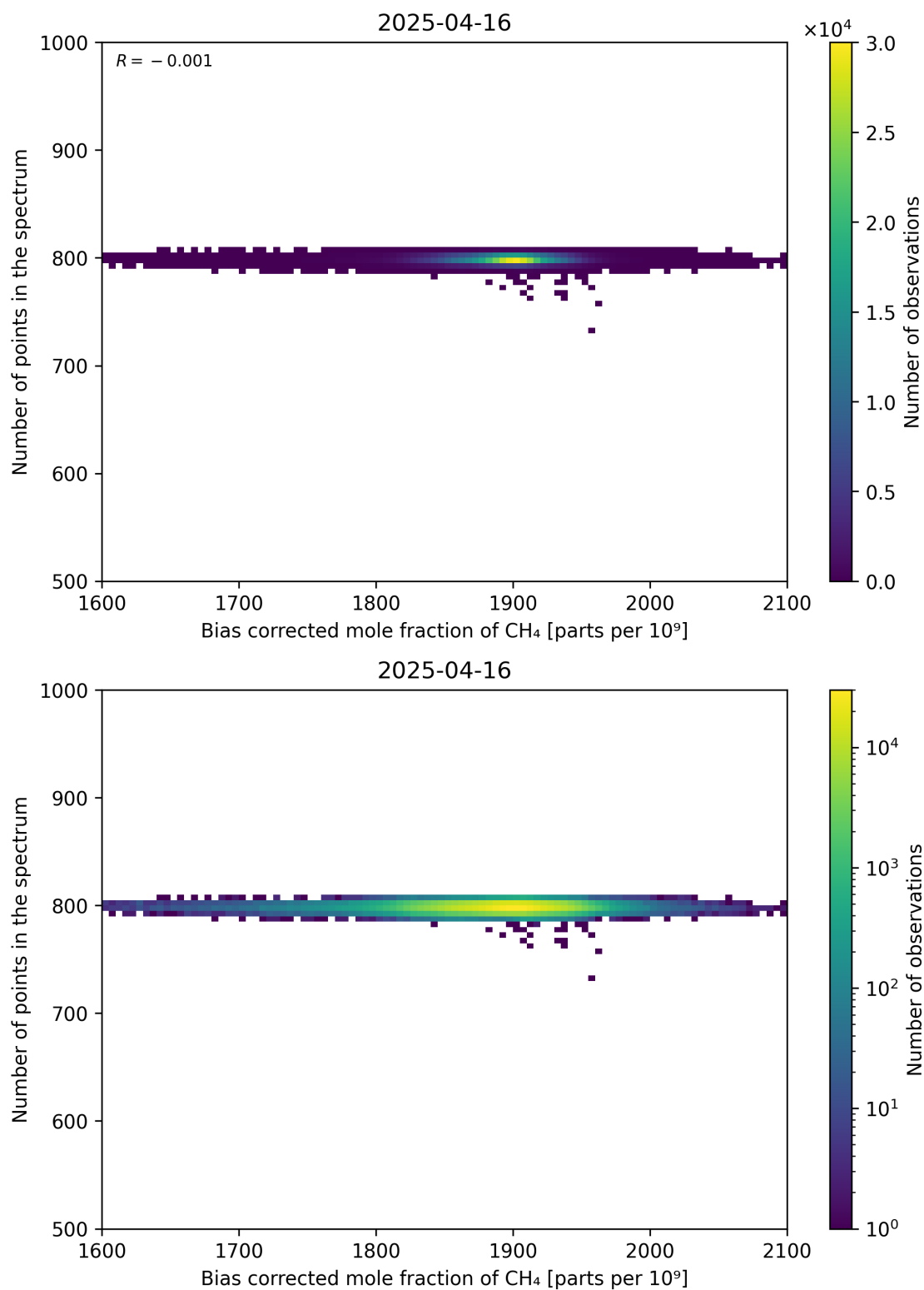
Figure 68: Scatter density plot of “Bias corrected mole fraction of CH 4 ” against “Number of points in the spectrum” for 2025-04-15 to 2025-04-17.
