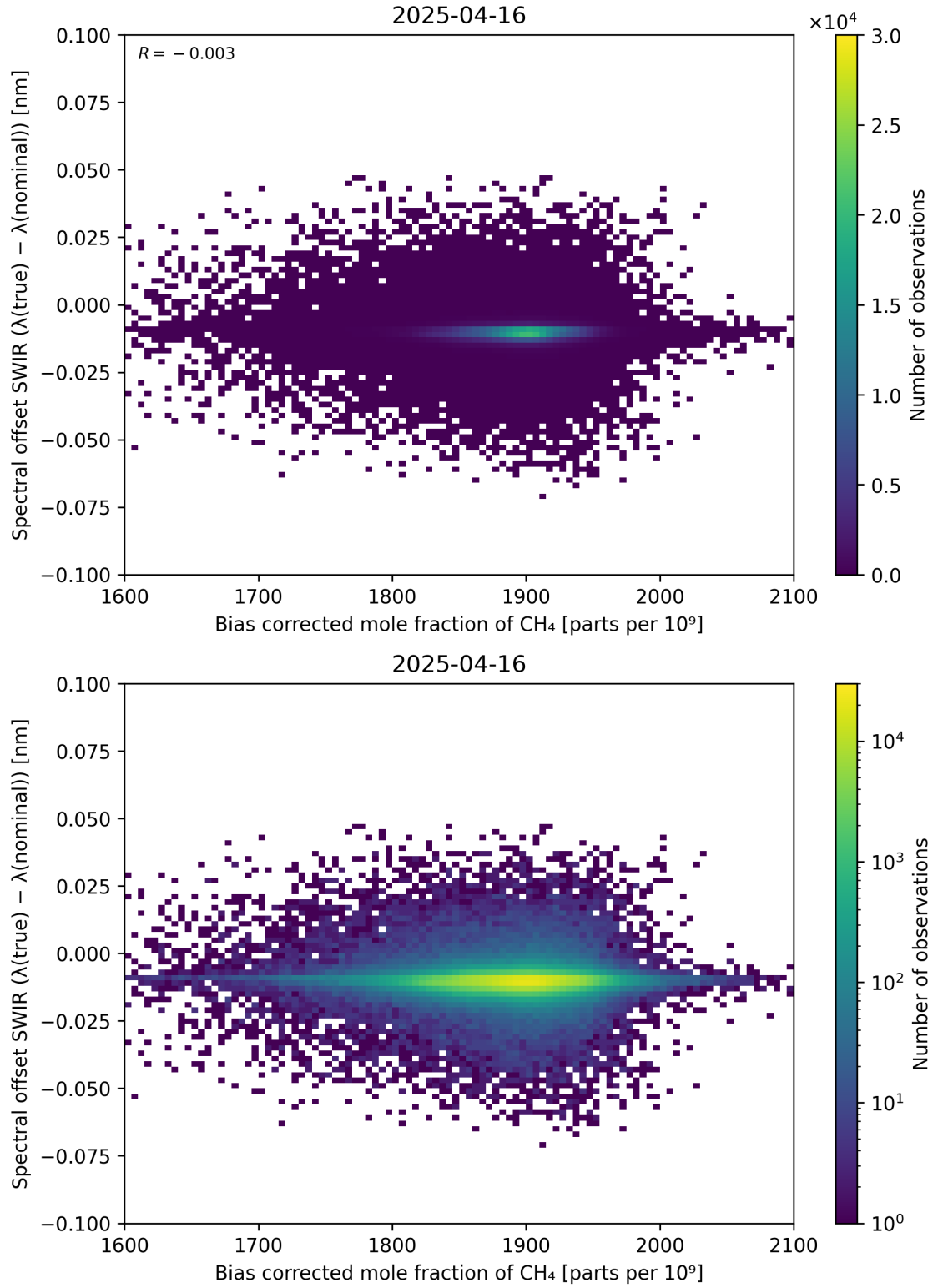
Figure 69: Scatter density plot of “Bias corrected mole fraction of CH 4 ” against “Spectral offset SWIR ( \lambda_{\text{true}} - \lambda_{\text{nominal}} )” for 2025-04-15 to 2025-04-17.
