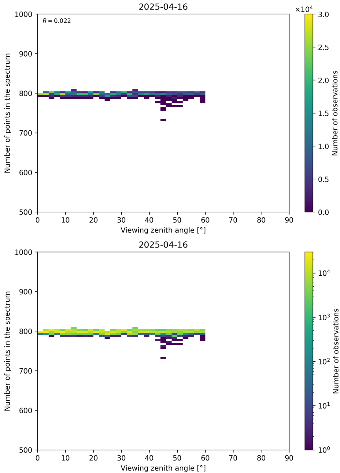
Figure 114: Scatter density plot of “Viewing zenith angle” against “Number of points in the spectrum” for 2025-04-15 to 2025-04-17.
