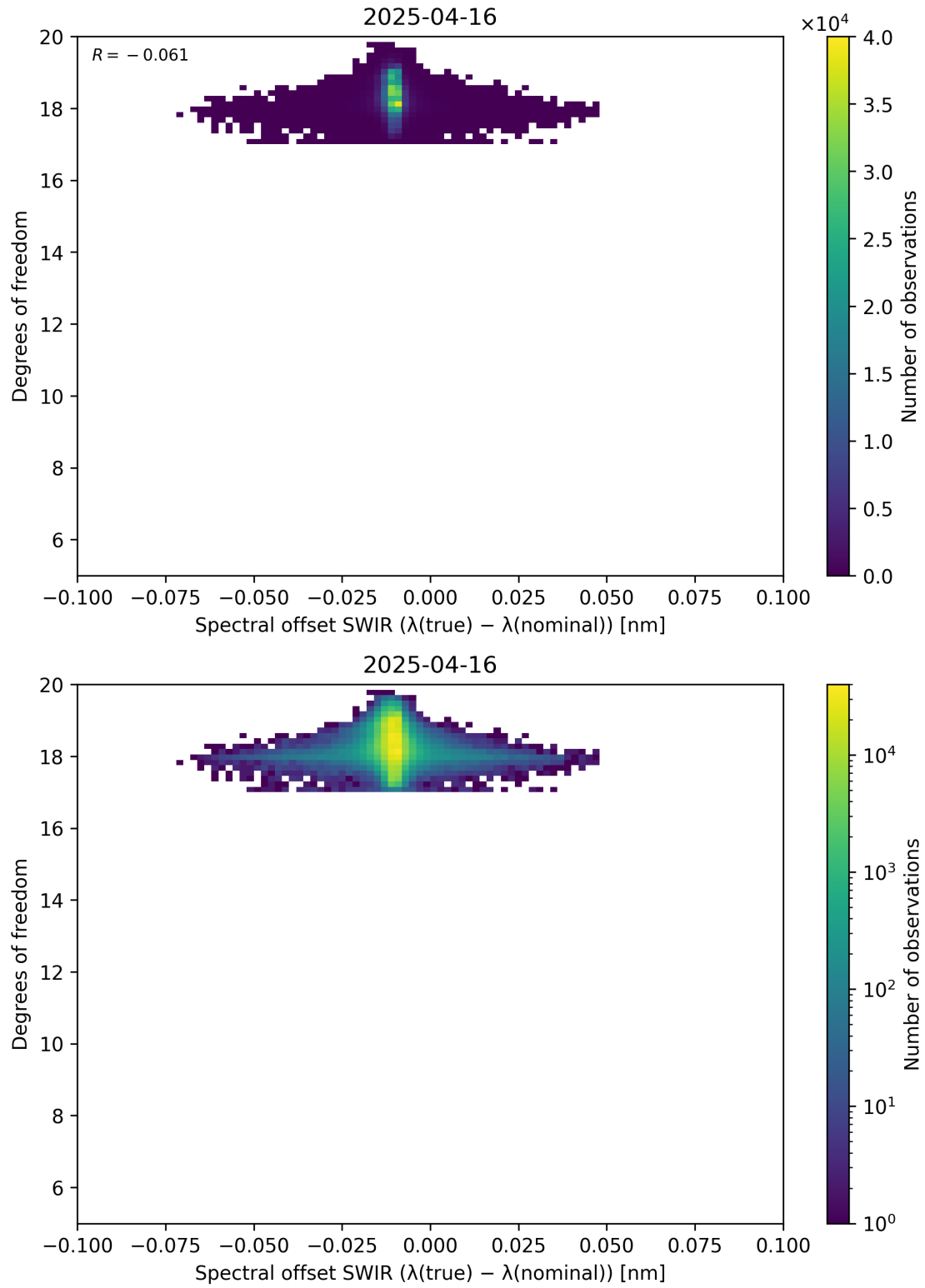
Figure 119: Scatter density plot of “Spectral offset SWIR ( \lambda_{\text{true}} - \lambda_{\text{nominal}} )” against “Degrees of freedom” for 2025-04-15 to 2025-04-17.
