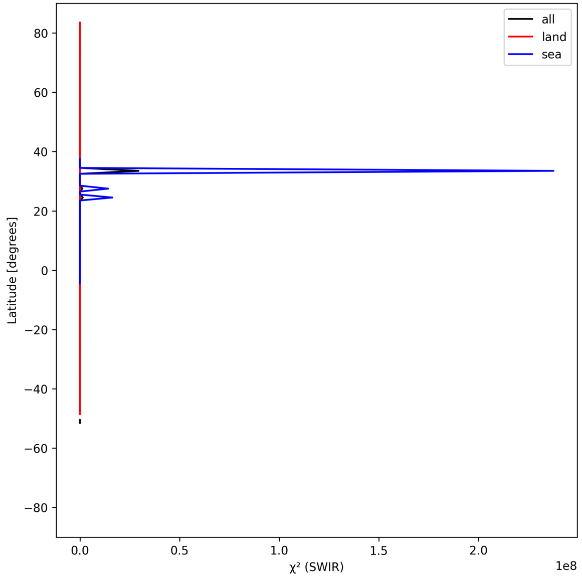
Figure 17: Zonal average of “ \chi^2 (SWIR)” for 2025-04-15 to 2025-04-17.
