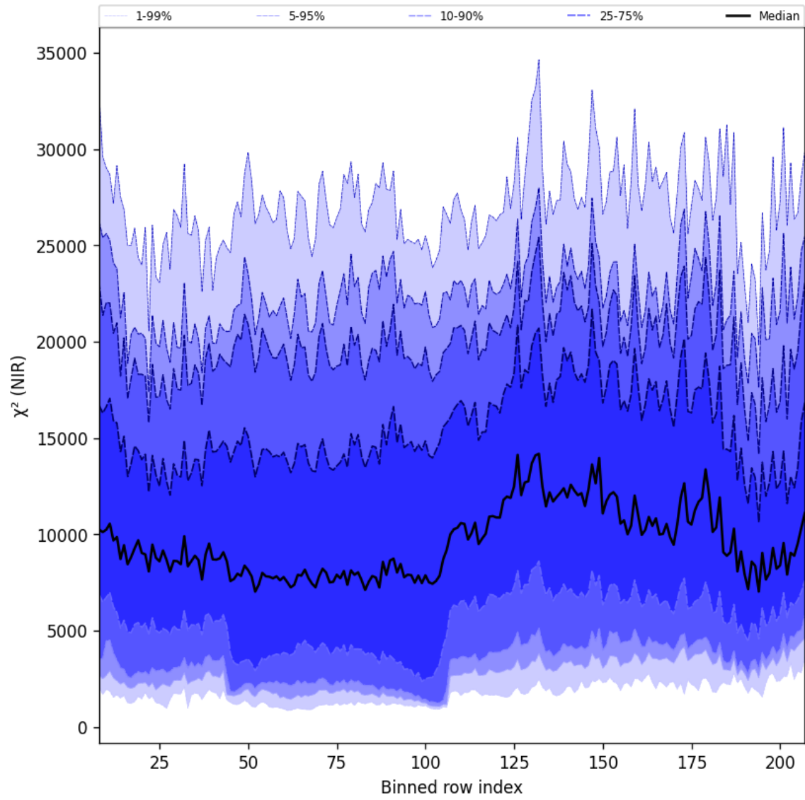
Figure 40: Along track statistics of “ \chi^2 (NIR)” for 2025-04-15 to 2025-04-17
