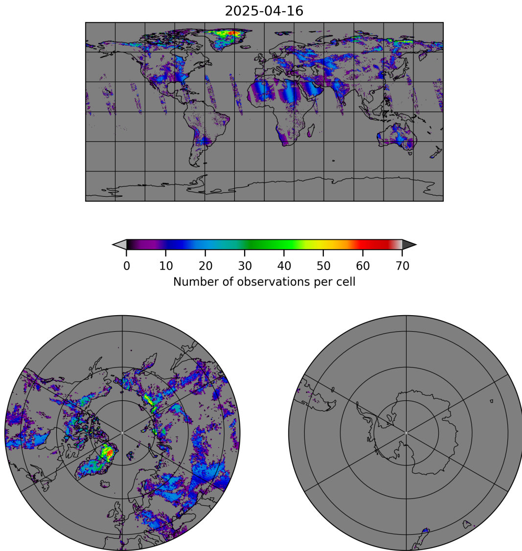
Figure 10: Map of the number of observations for 2025-04-15 to 2025-04-17
