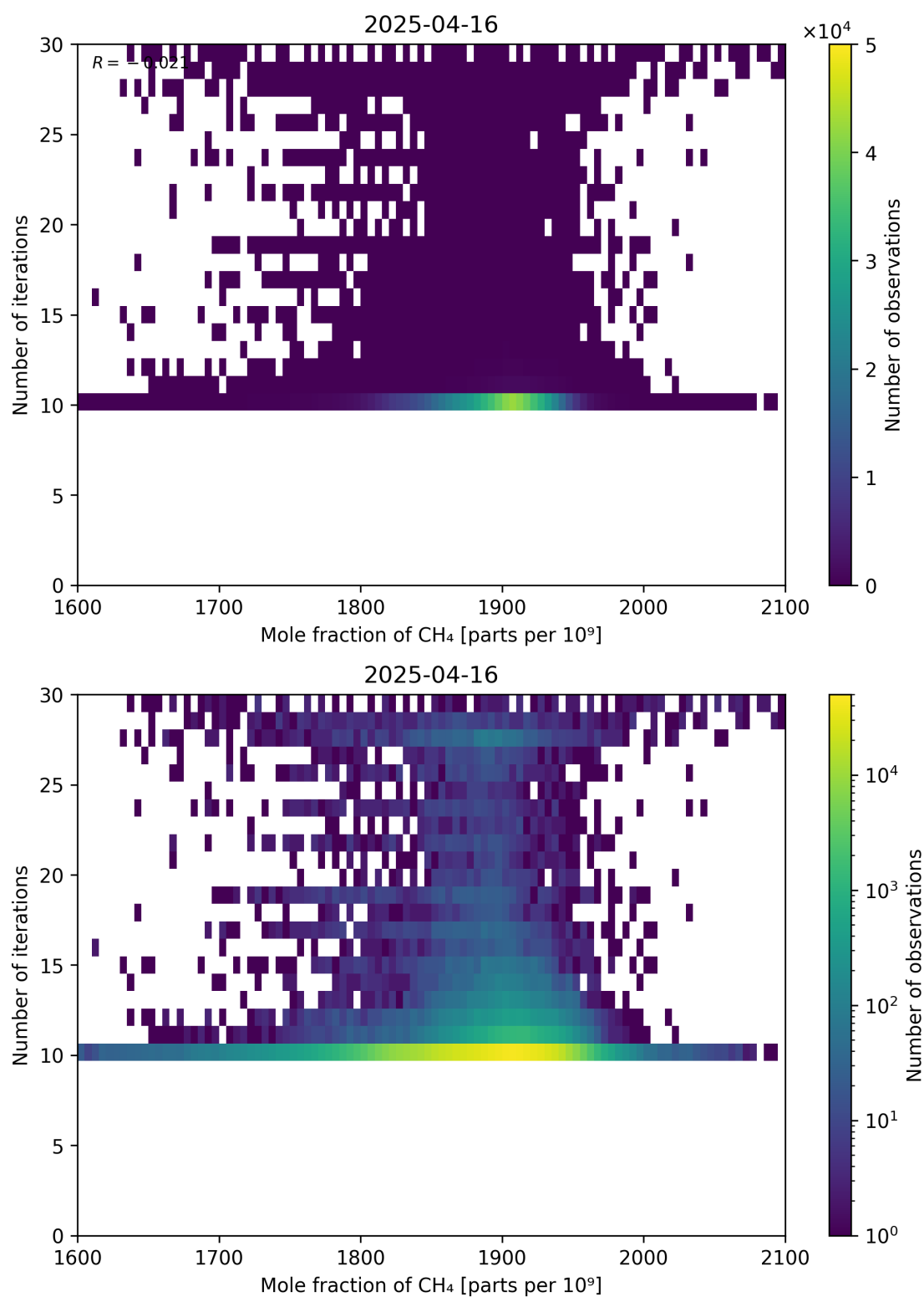
Figure 76: Scatter density plot of “Mole fraction of CH 4 ” against “Number of iterations” for 2025-04-15 to 2025-04-17.
