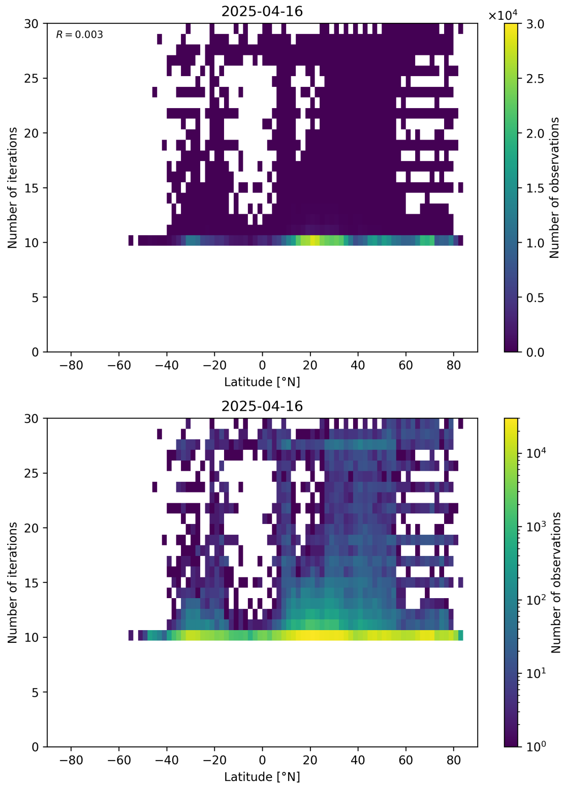
Figure 60: Scatter density plot of “Latitude” against “Number of iterations” for 2025-04-15 to 2025-04-17.
