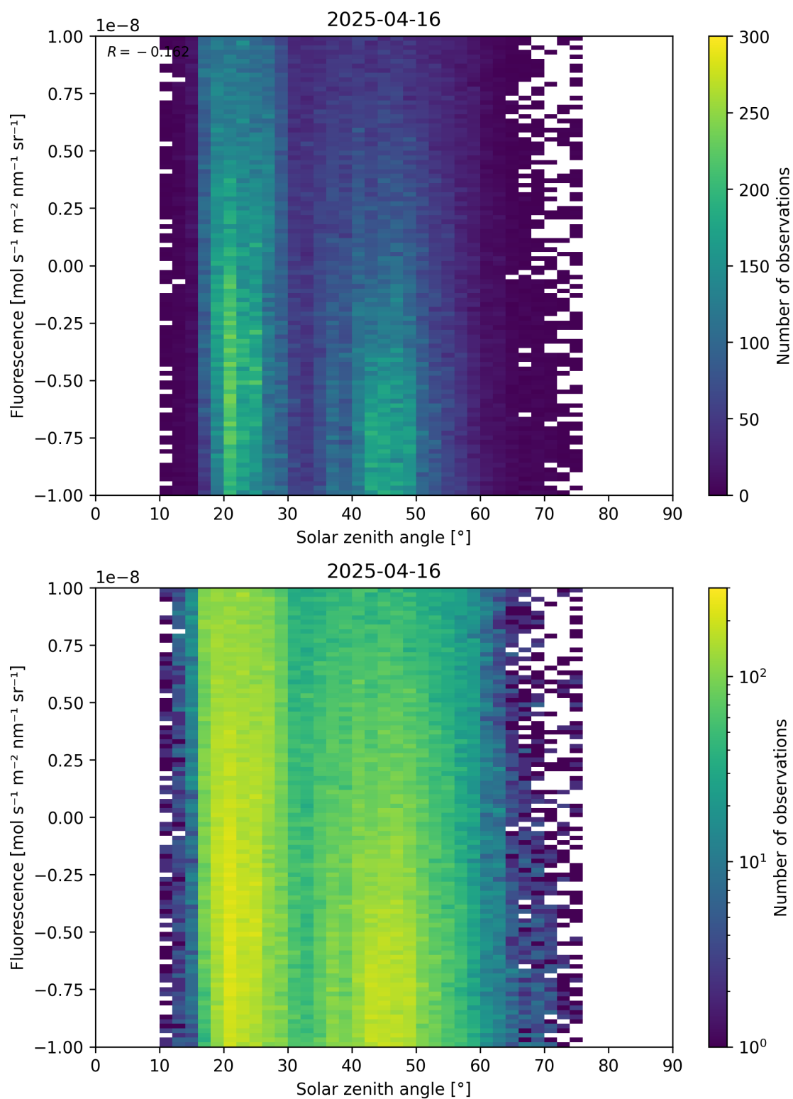
Figure 97: Scatter density plot of “Solar zenith angle” against “Fluorescence” for 2025-04-15 to 2025-04-17.
