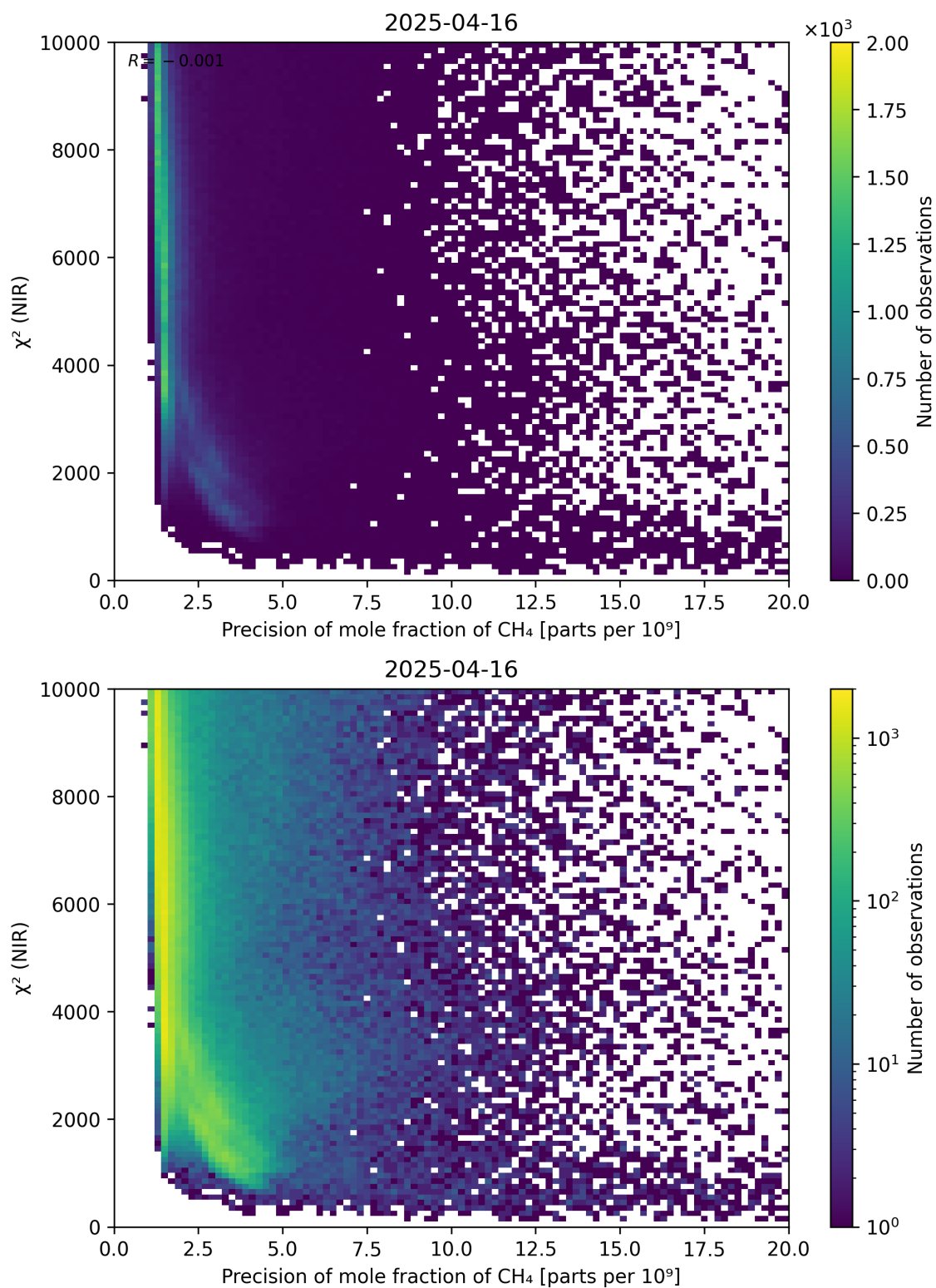
Figure 78: Scatter density plot of “Precision of mole fraction of \text{CH}_4 ” against “ \chi^2 (NIR)” for 2025-04-15 to 2025-04-17.
