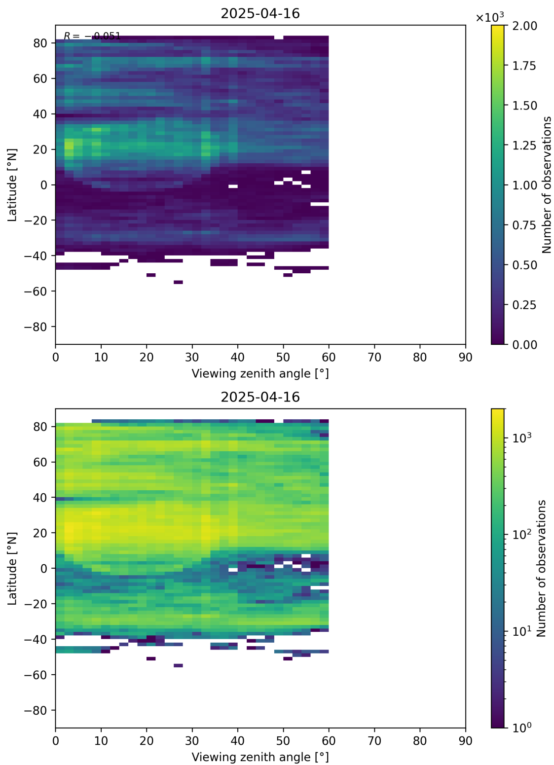
Figure 109: Scatter density plot of “Viewing zenith angle” against “Latitude” for 2025-04-15 to 2025-04-17.
