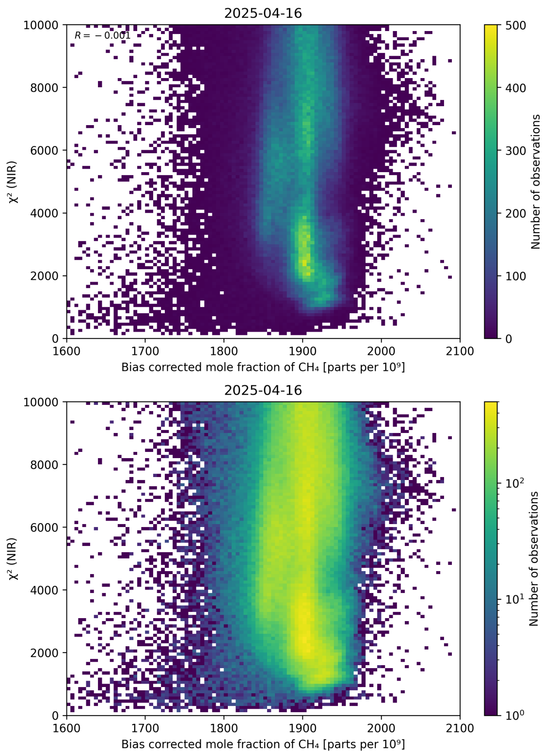
Figure 63: Scatter density plot of “Bias corrected mole fraction of CH 4 ” against “ \chi^2 (NIR)” for 2025-04-15 to 2025-04-17.
