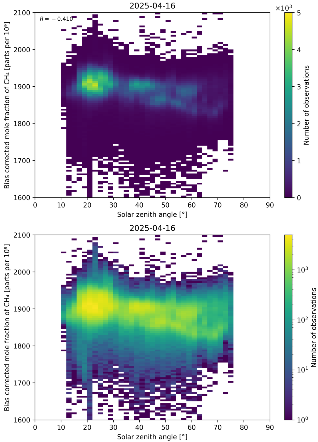
Figure 100: Scatter density plot of “Solar zenith angle” against “Bias corrected mole fraction of \text{CH}_4 ” for 2025-04-15 to 2025-04-17.
