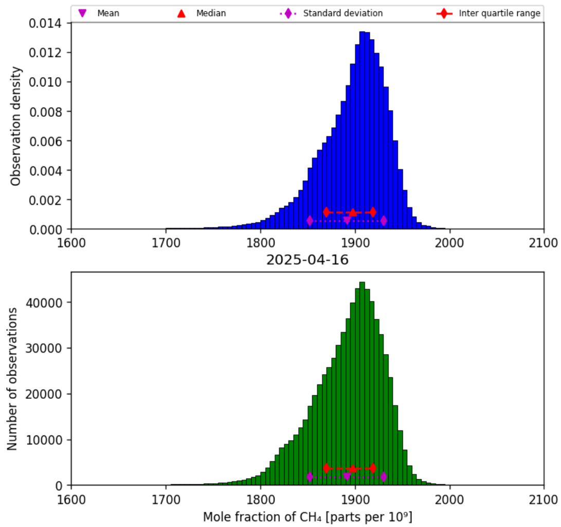
Figure 23: Histogram of “Mole fraction of CH 4 ” for 2025-04-15 to 2025-04-17
