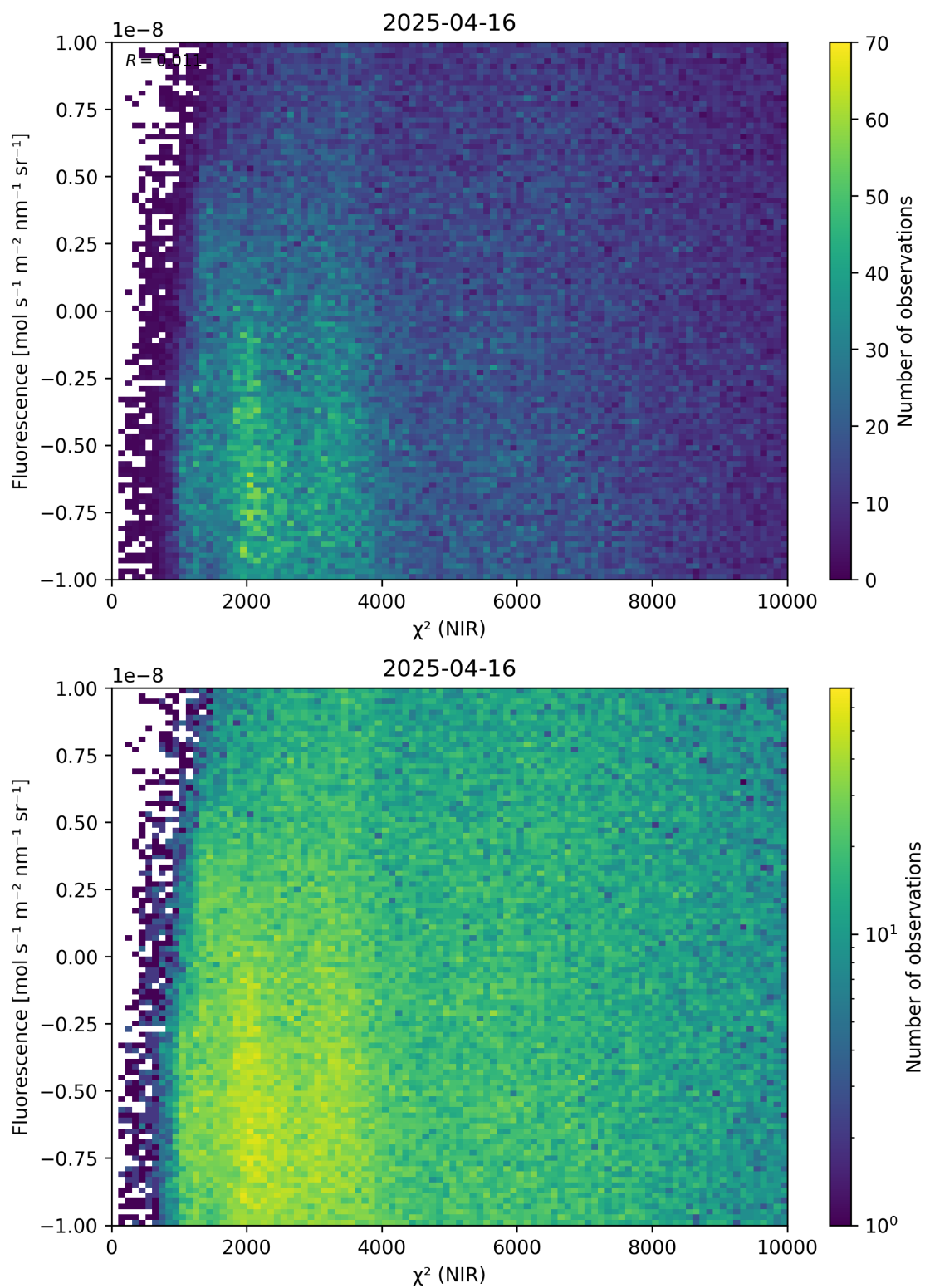
Figure 45: Scatter density plot of “ \chi^2 (NIR)” against “Fluorescence” for 2025-04-15 to 2025-04-17.
