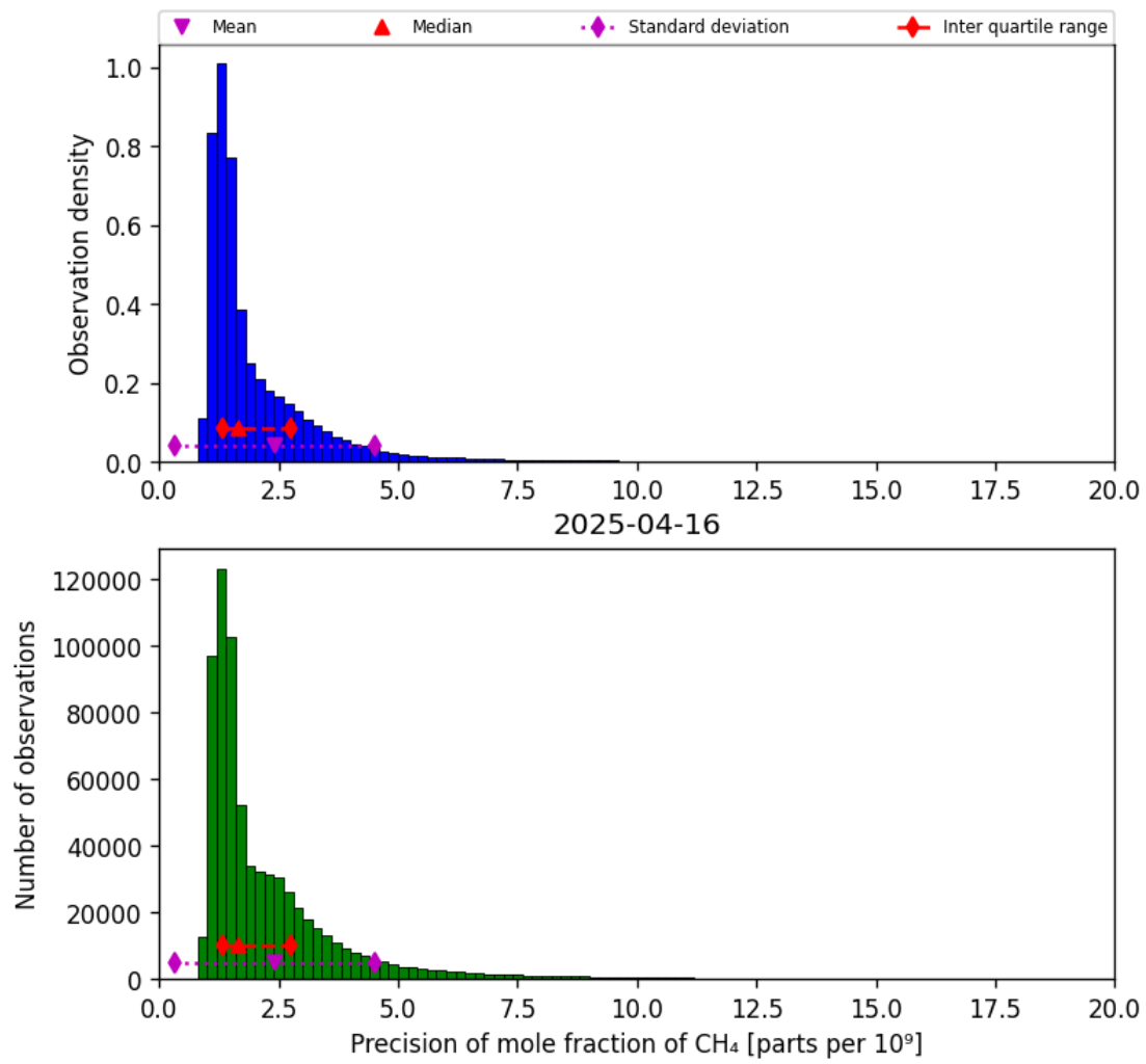
Figure 24: Histogram of “Precision of mole fraction of CH 4 ” for 2025-04-15 to 2025-04-17
