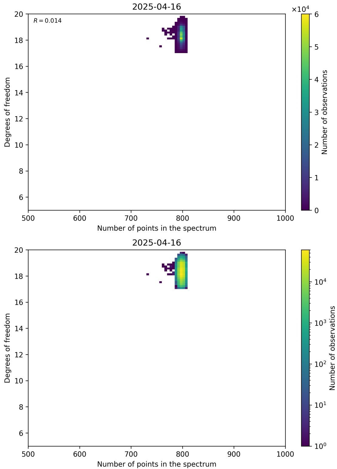
Figure 90: Scatter density plot of “Number of points in the spectrum” against “Degrees of freedom” for 2025-04-15 to 2025-04-17.
