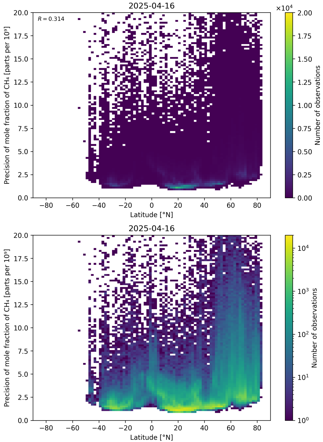
Figure 59: Scatter density plot of “Latitude” against “Precision of mole fraction of \text{CH}_4 ” for 2025-04-15 to 2025-04-17.
