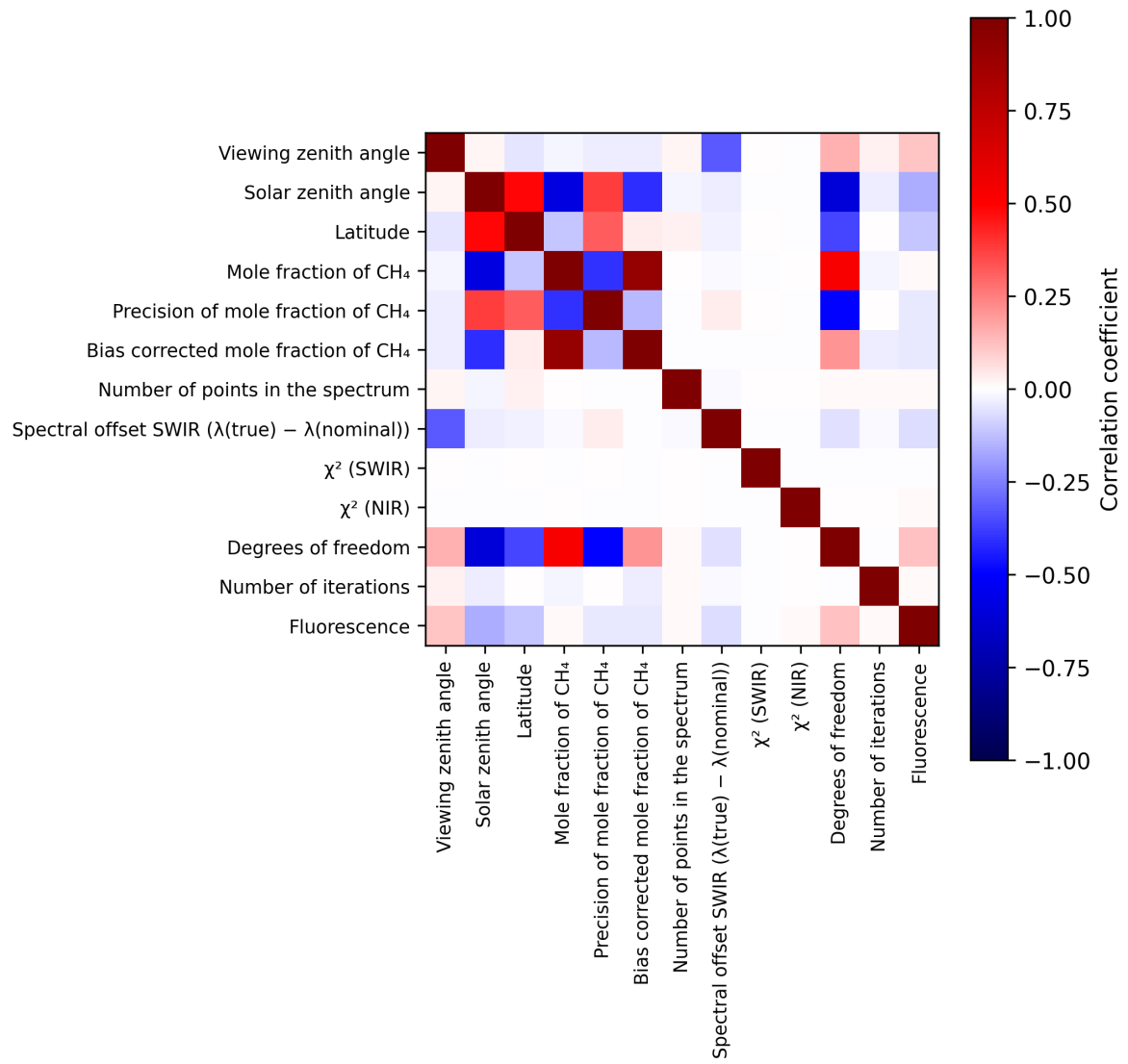
Figure 2: Map of correlation matrix for 2025-04-15 to 2025-04-17.
