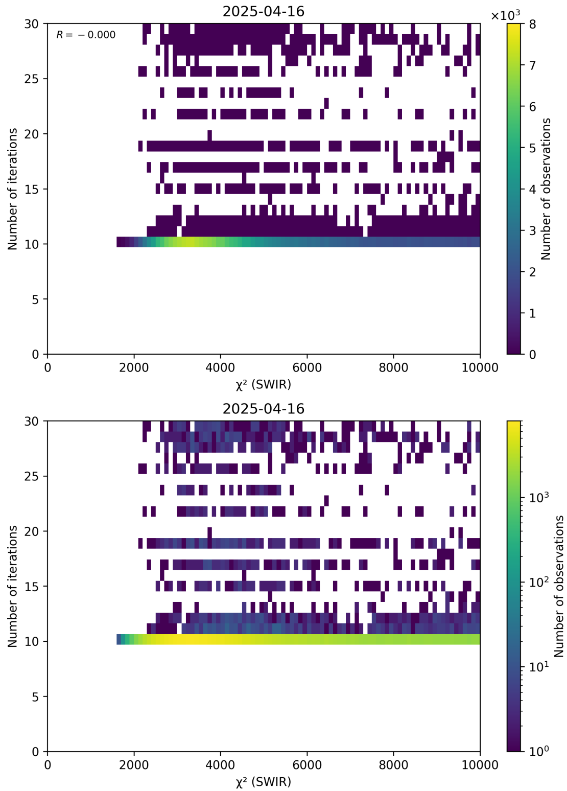
Figure 50: Scatter density plot of “ \chi^2 (SWIR)” against “Number of iterations” for 2025-04-15 to 2025-04-17.
