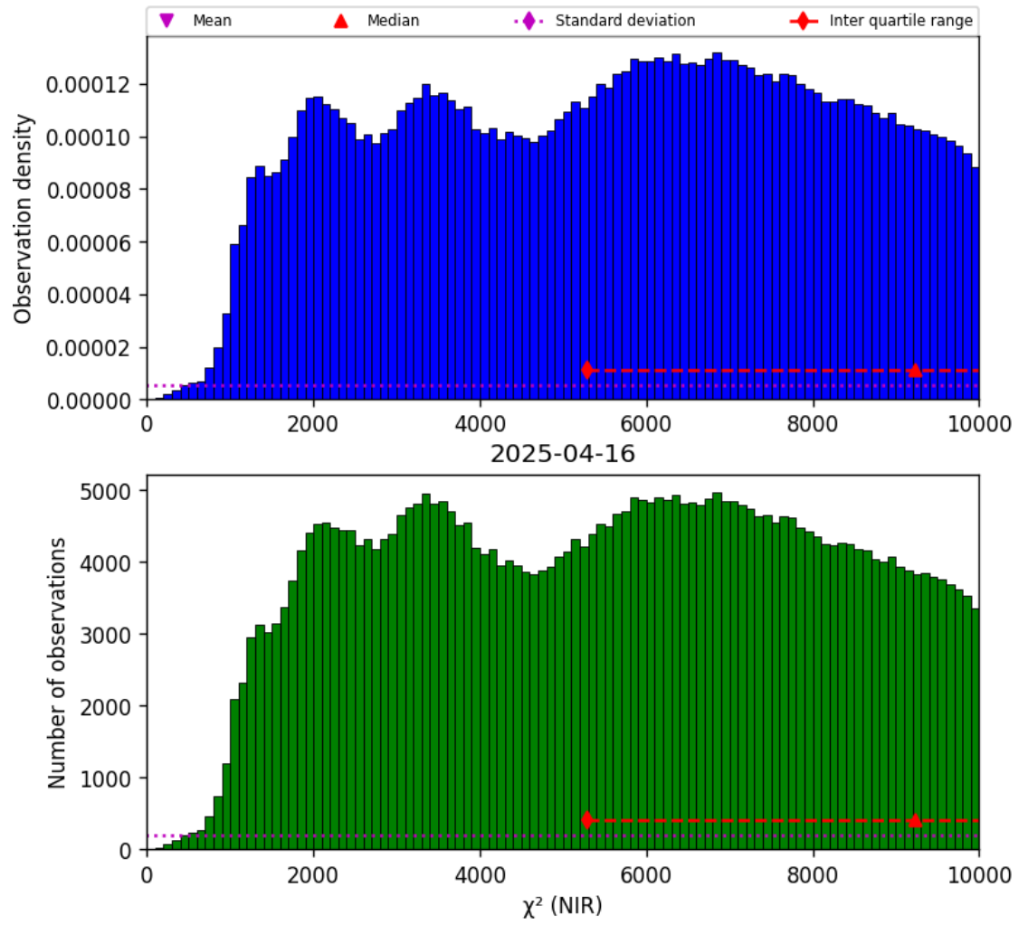
Figure 29: Histogram of “ \chi^2 (NIR)” for 2025-04-15 to 2025-04-17
