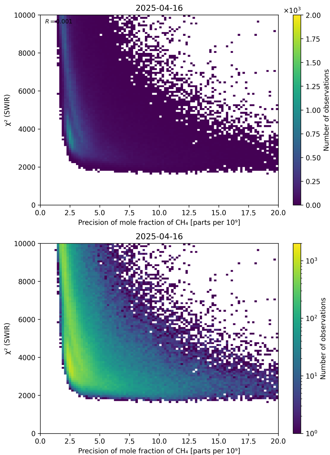
Figure 79: Scatter density plot of “Precision of mole fraction of CH 4 ” against “ \chi^2 (SWIR)” for 2025-04-15 to 2025-04-17.
