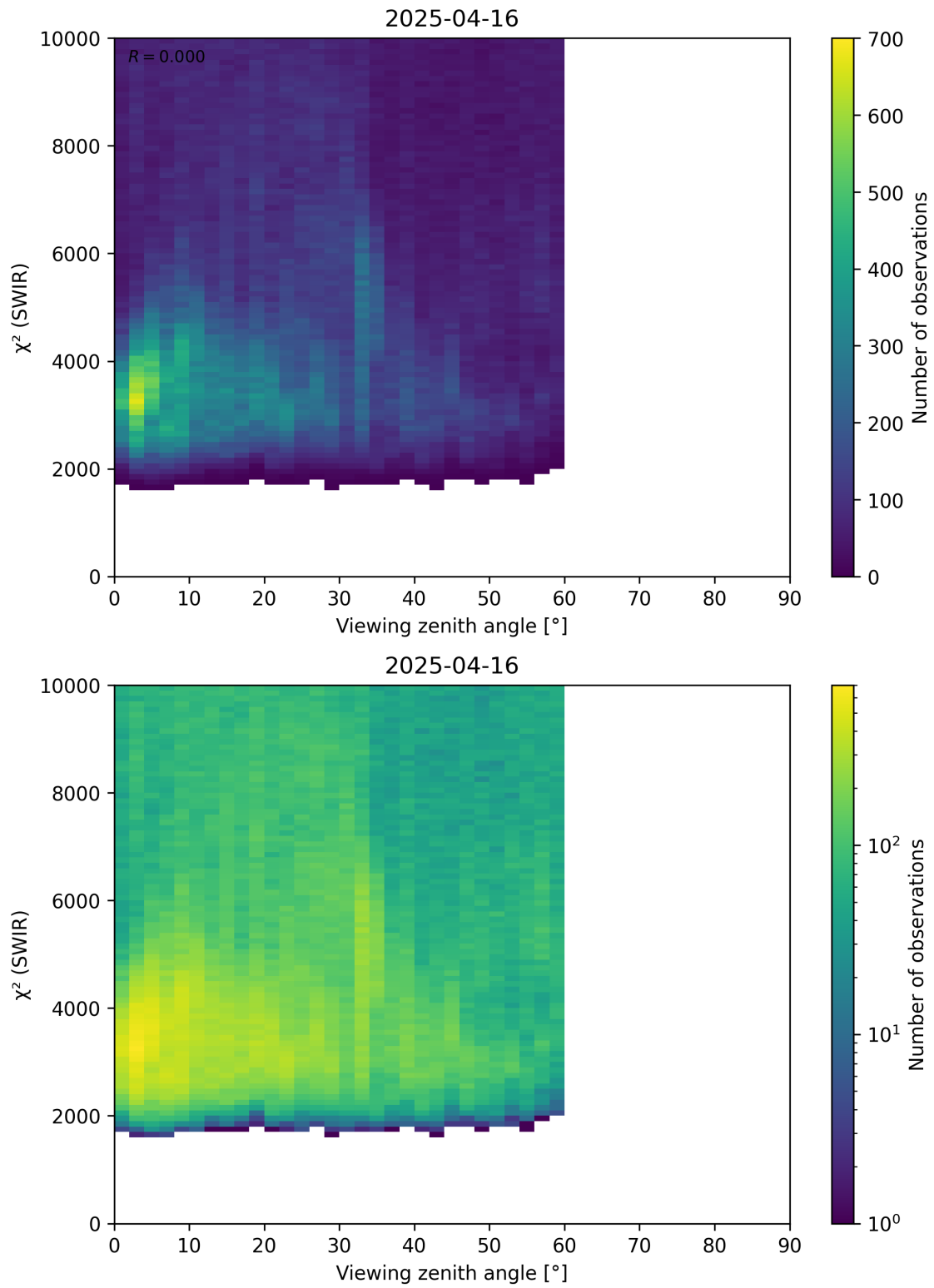
Figure 106: Scatter density plot of “Viewing zenith angle” against “ \chi^2 (SWIR)” for 2025-04-15 to 2025-04-17.
