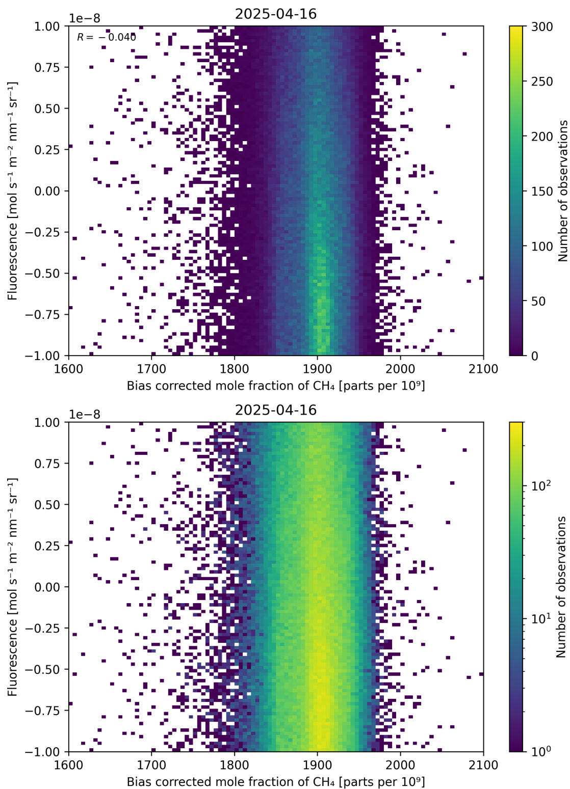
Figure 66: Scatter density plot of “Bias corrected mole fraction of CH 4 ” against “Fluorescence” for 2025-04-15 to 2025-04-17.
