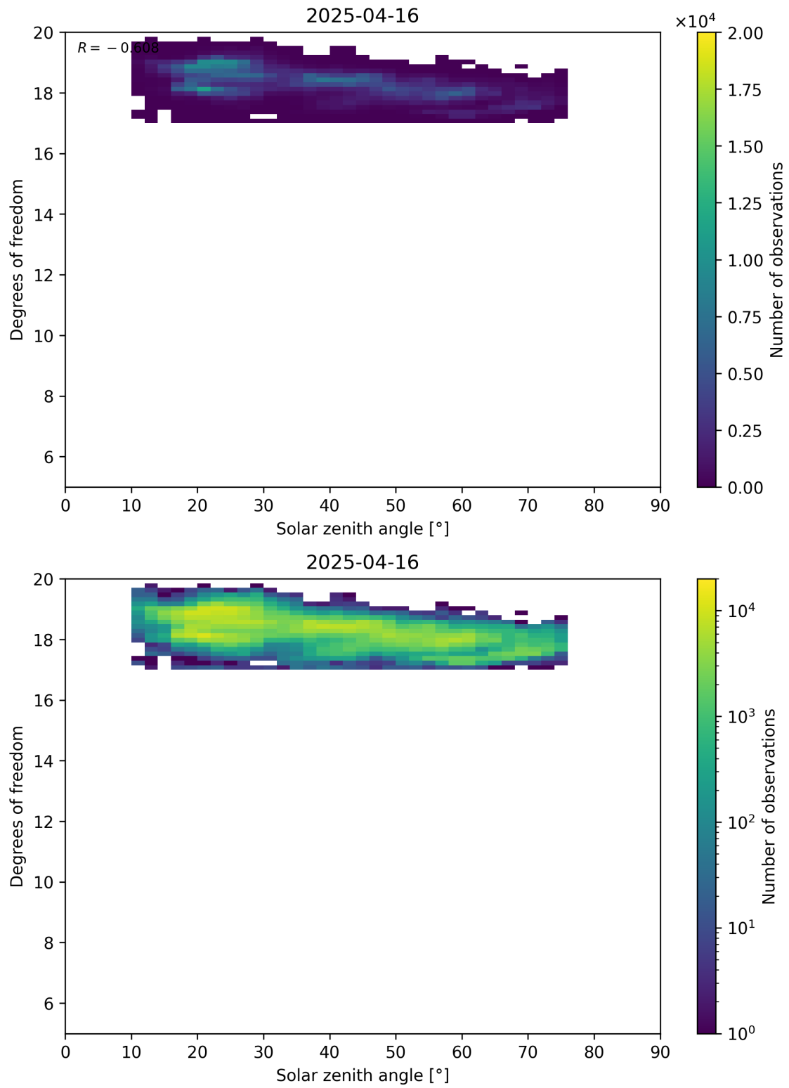
Figure 96: Scatter density plot of “Solar zenith angle” against “Degrees of freedom” for 2025-04-15 to 2025-04-17.
