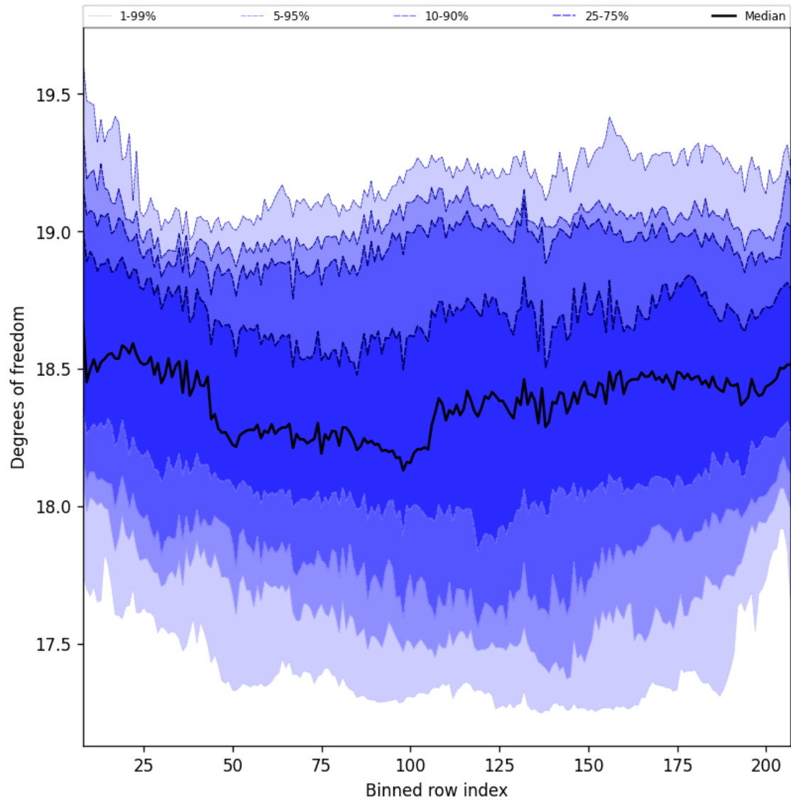
Figure 41: Along track statistics of “Degrees of freedom” for 2025-04-15 to 2025-04-17
