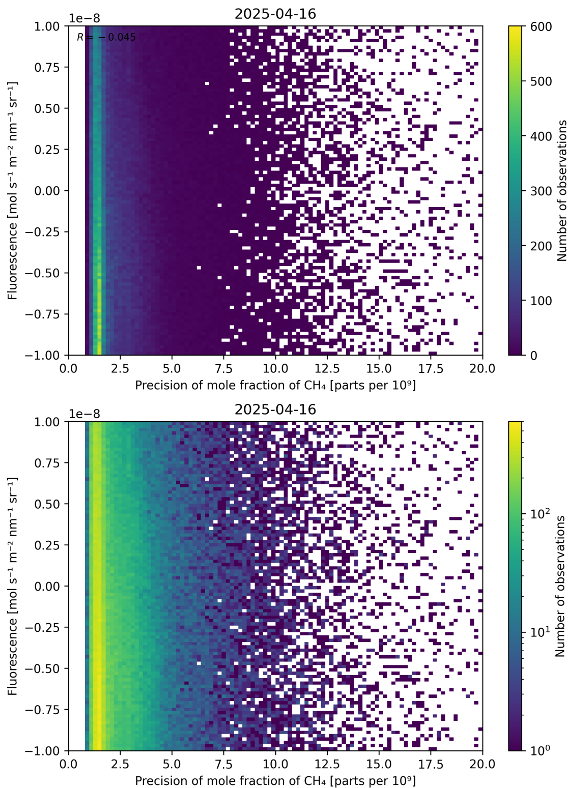
Figure 81: Scatter density plot of “Precision of mole fraction of CH 4 ” against “Fluorescence” for 2025-04-15 to 2025-04-17.
