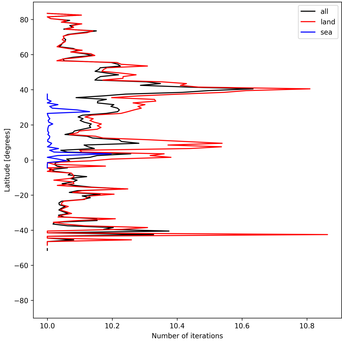
Figure 20: Zonal average of “Number of iterations” for 2025-04-15 to 2025-04-17.
