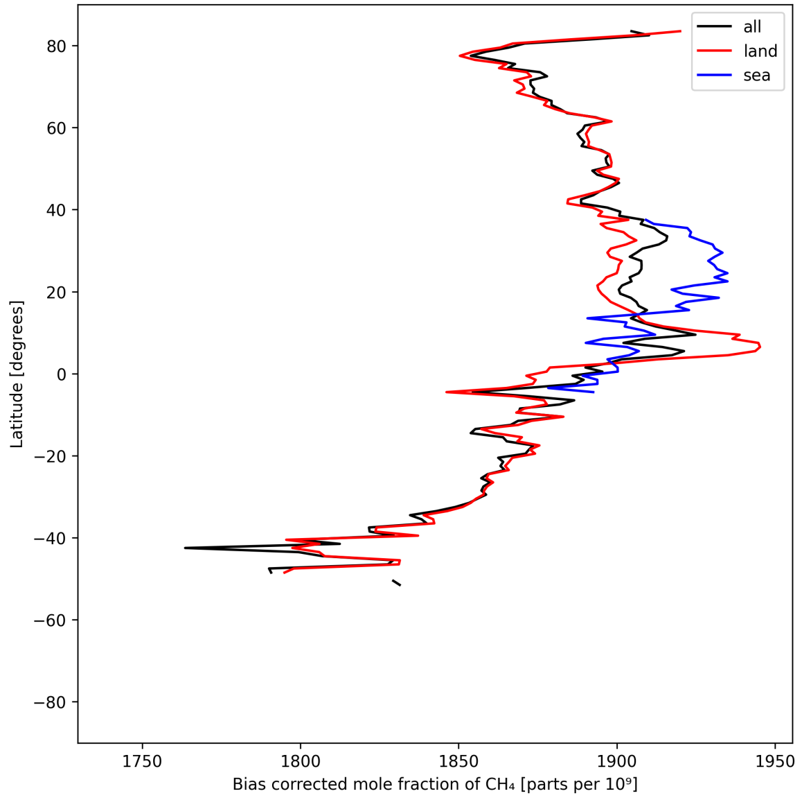
Figure 14: Zonal average of “Bias corrected mole fraction of CH 4 ” for 2025-04-15 to 2025-04-17.
