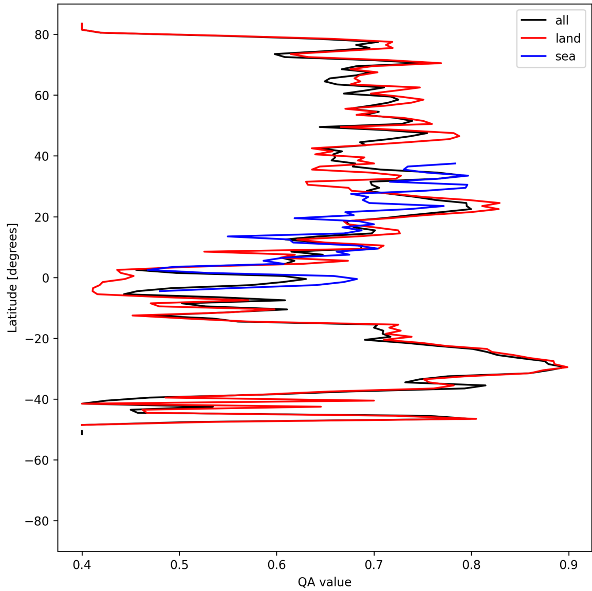
Figure 11: Zonal average of “QA value” for 2025-04-15 to 2025-04-17.
