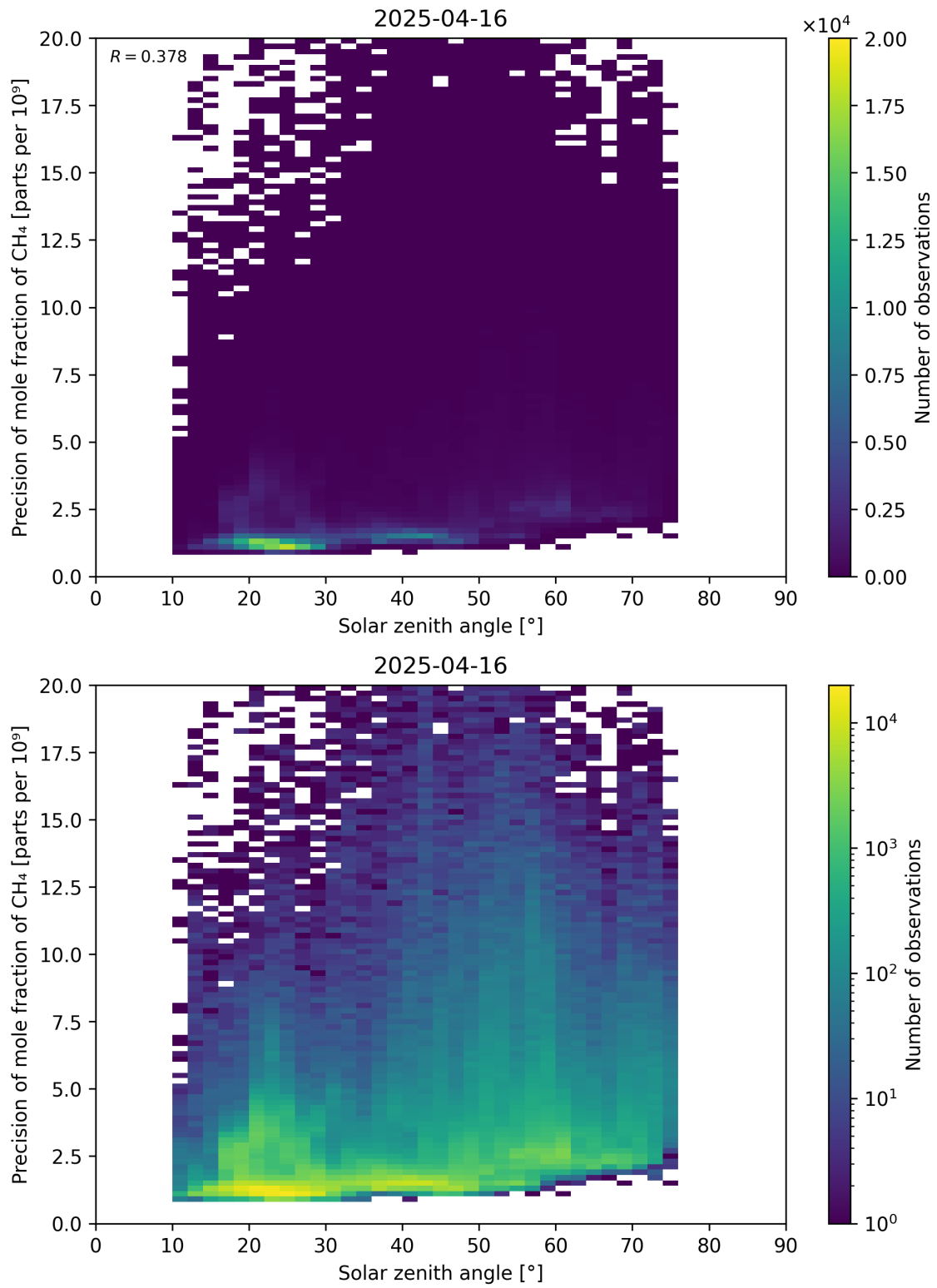
Figure 101: Scatter density plot of “Solar zenith angle” against “Precision of mole fraction of \text{CH}_4 ” for 2025-04-15 to 2025-04-17.
