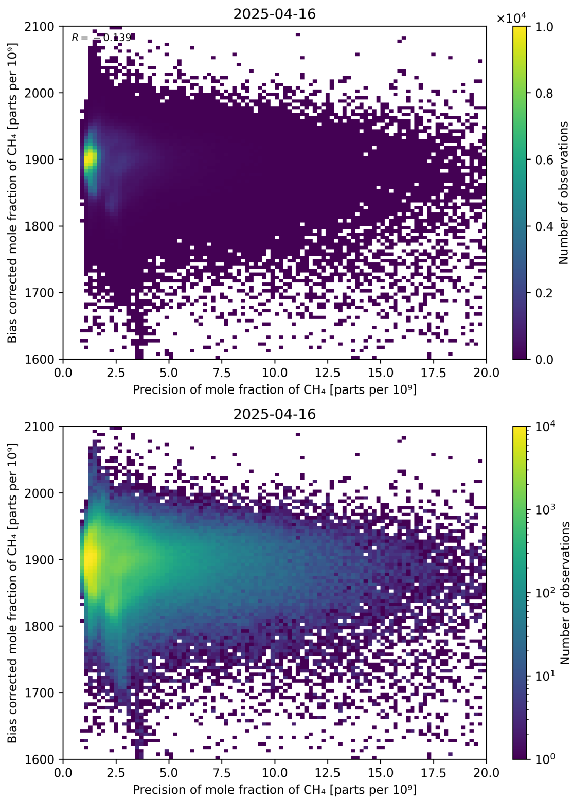
Figure 82: Scatter density plot of “Precision of mole fraction of CH 4 ” against “Bias corrected mole fraction of CH 4 ” for 2025-04-15 to 2025-04-17.
