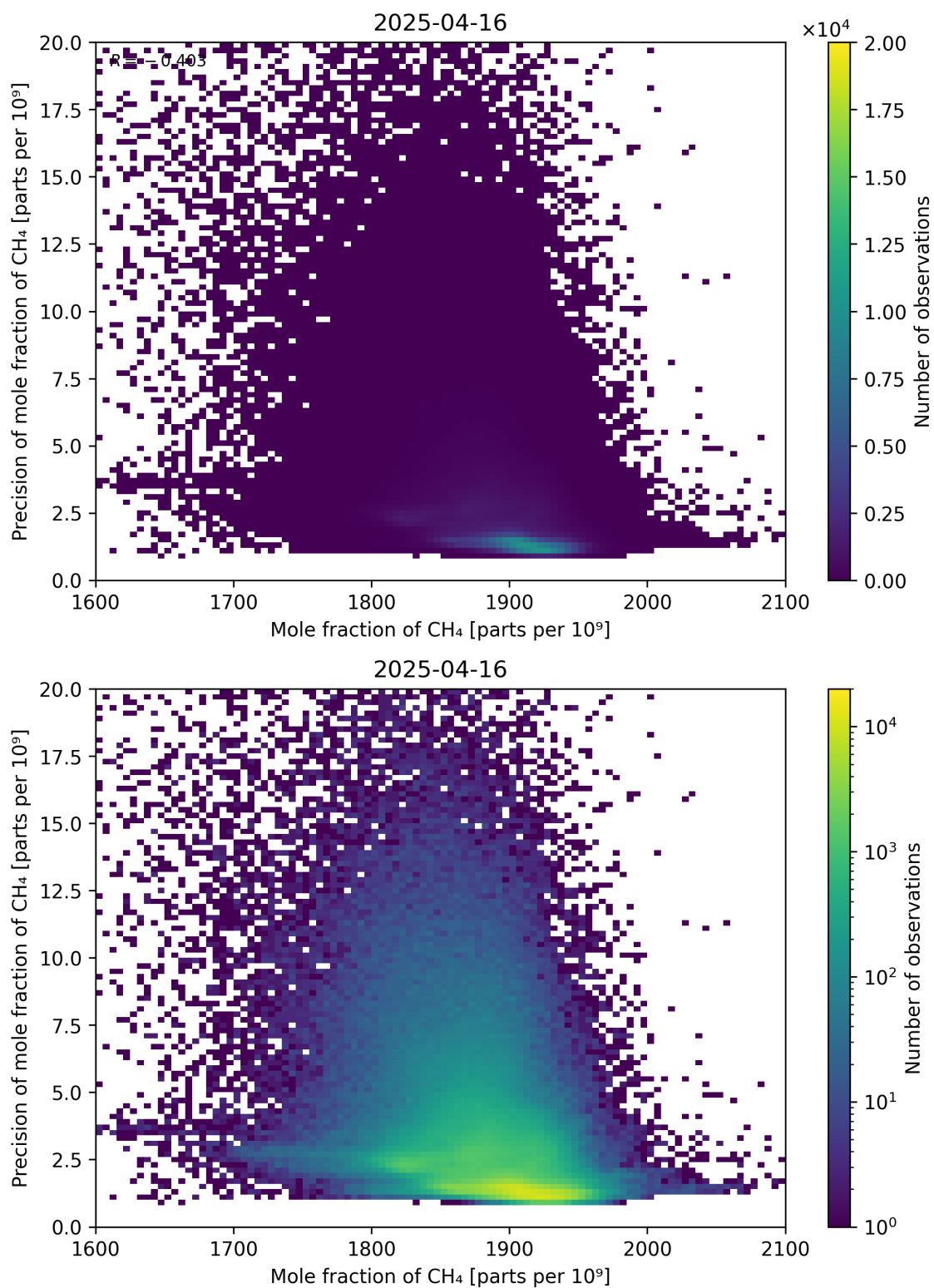
Figure 75: Scatter density plot of “Mole fraction of CH 4 ” against “Precision of mole fraction of CH 4 ” for 2025-04-15 to 2025-04-17.
