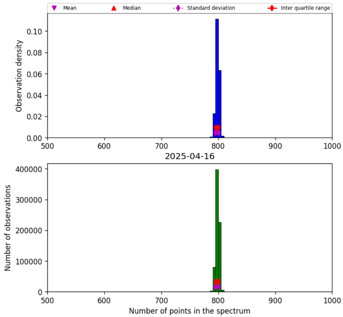
Figure 26: Histogram of “Number of points in the spectrum” for 2025-04-15 to 2025-04-17
