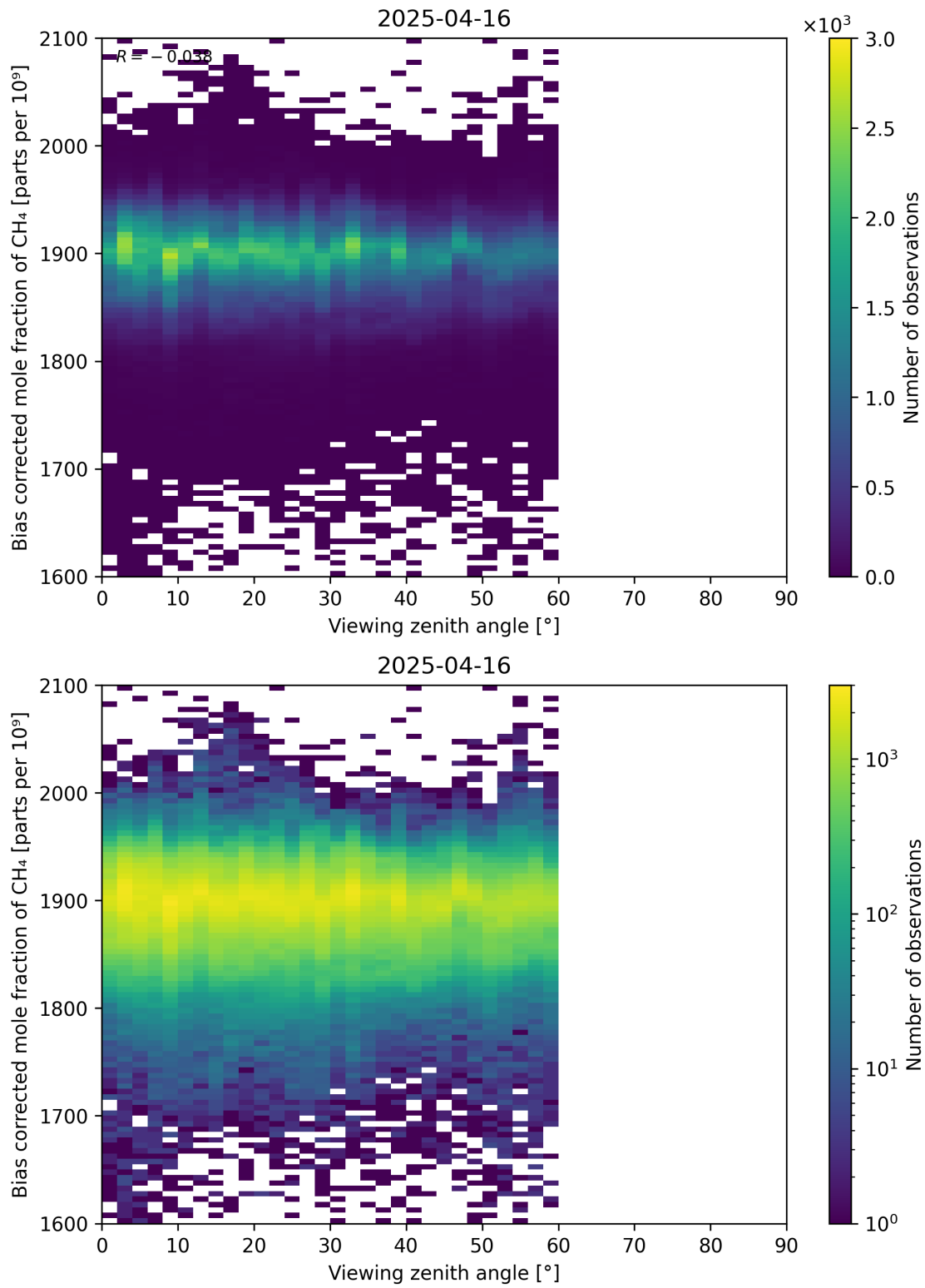
Figure 111: Scatter density plot of “Viewing zenith angle” against “Bias corrected mole fraction of CH 4 ” for 2025-04-15 to 2025-04-17.
