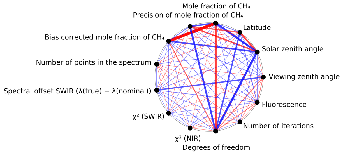
Figure 1: Map of correlation graph for 2025-04-15 to 2025-04-17.
