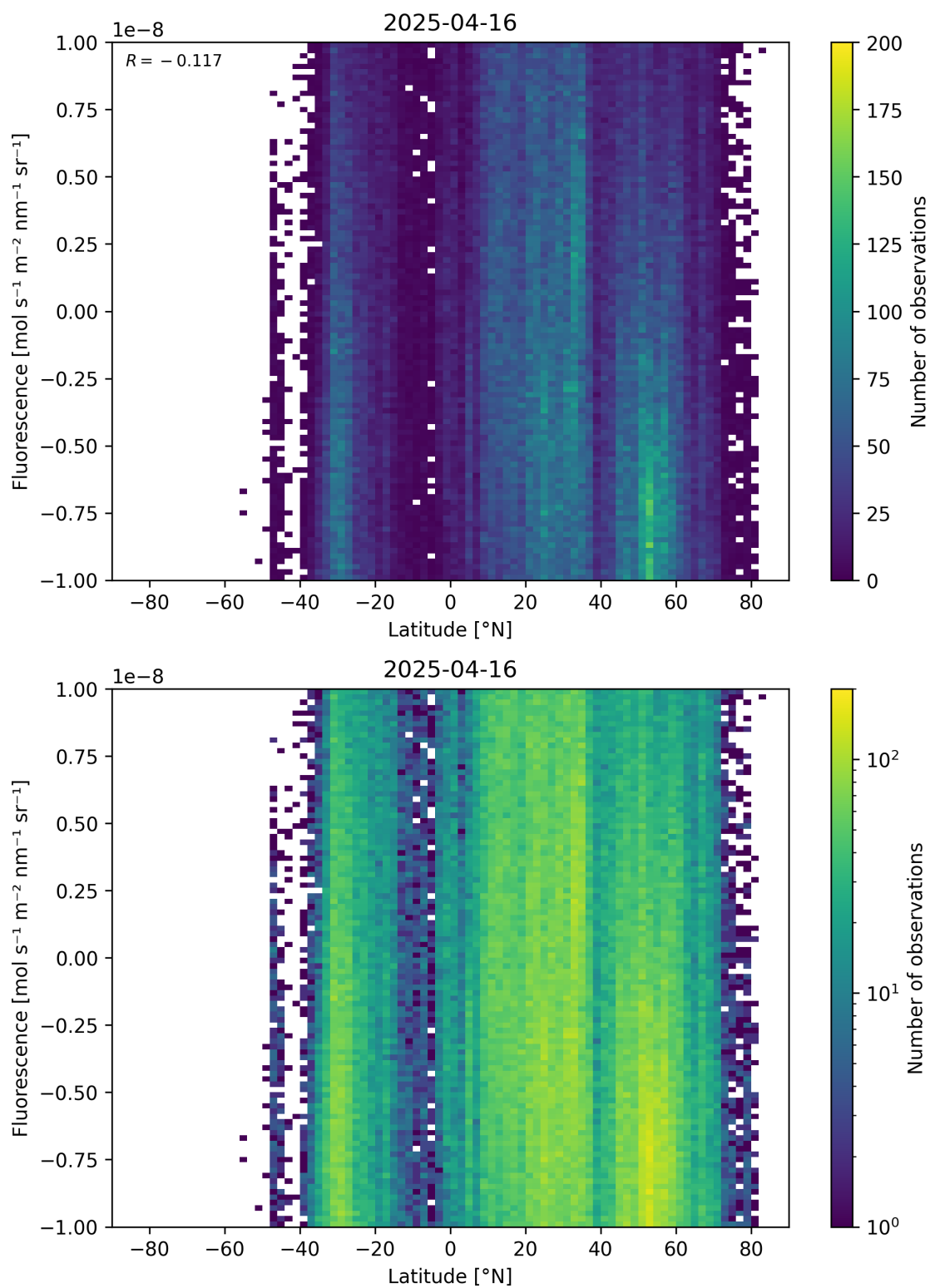
Figure 56: Scatter density plot of “Latitude” against “Fluorescence” for 2025-04-15 to 2025-04-17.
