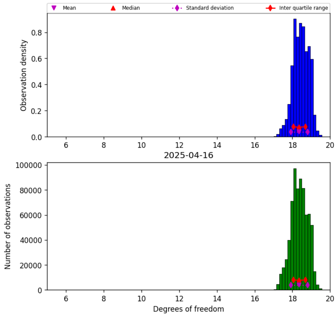
Figure 30: Histogram of “Degrees of freedom” for 2025-04-15 to 2025-04-17
