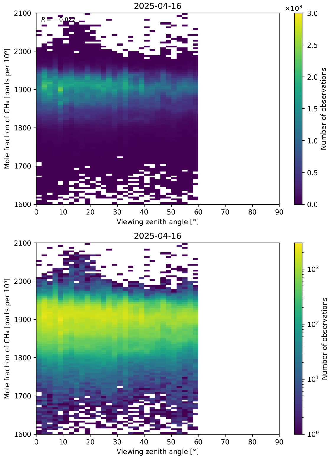
Figure 110: Scatter density plot of “Viewing zenith angle” against “Mole fraction of CH 4 ” for 2025-04-15 to 2025-04-17.
