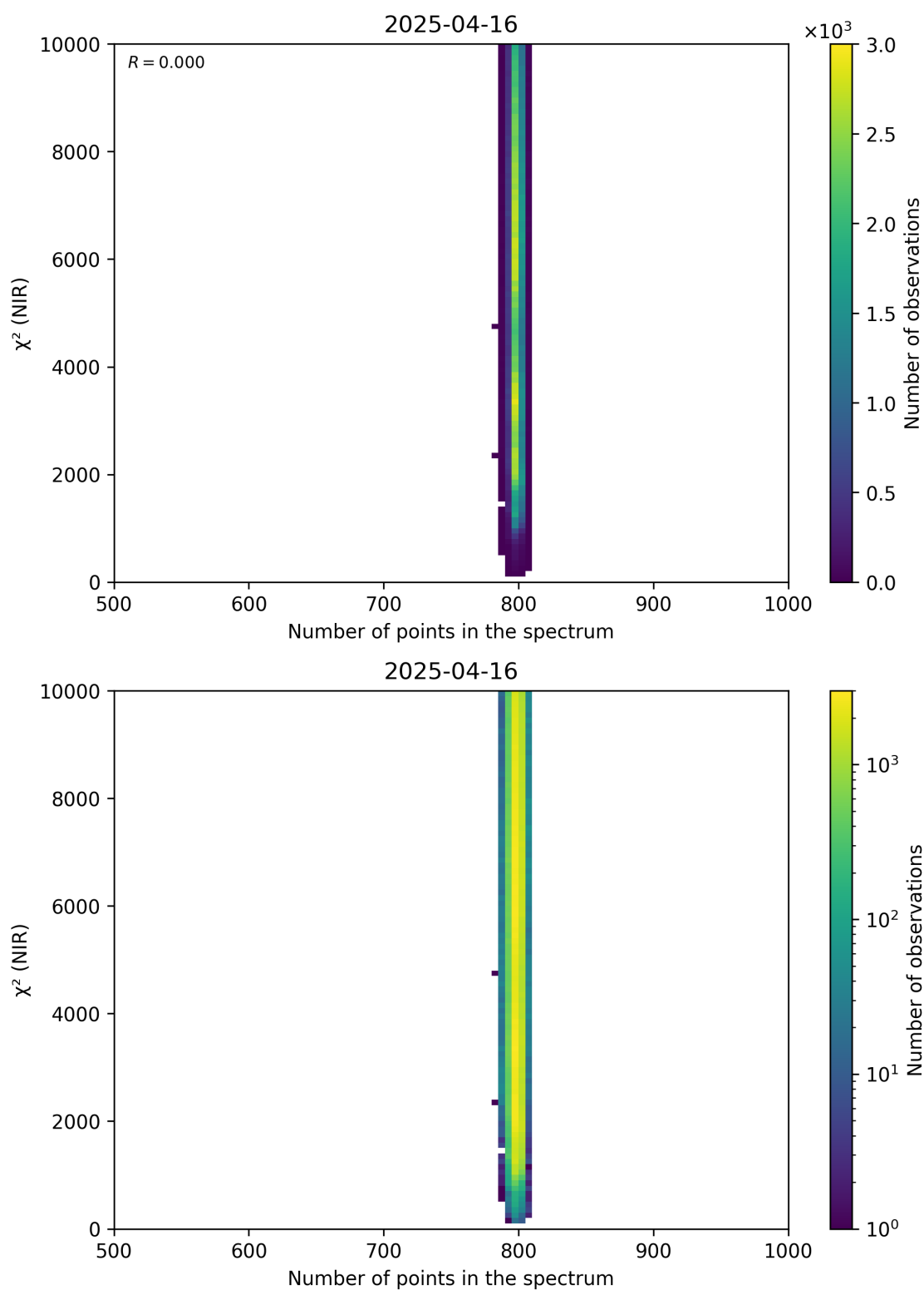
Figure 88: Scatter density plot of “Number of points in the spectrum” against “ \chi^2 (NIR)” for 2025-04-15 to 2025-04-17.
