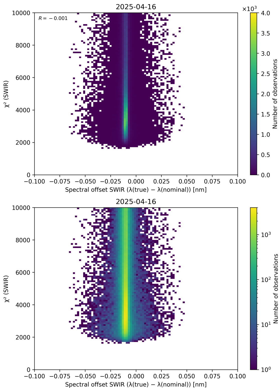
Figure 118: Scatter density plot of “Spectral offset SWIR ( \lambda_{\text{true}} - \lambda_{\text{nominal}} )” against “ \chi^2 (SWIR)” for 2025-04-15 to 2025-04-17.
