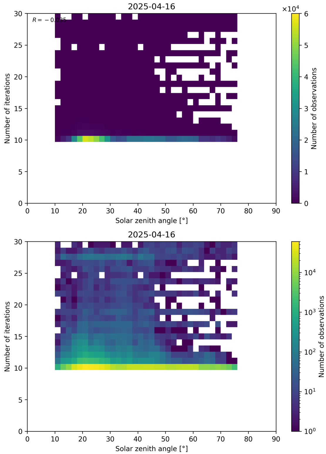
Figure 102: Scatter density plot of “Solar zenith angle” against “Number of iterations” for 2025-04-15 to 2025-04-17.
