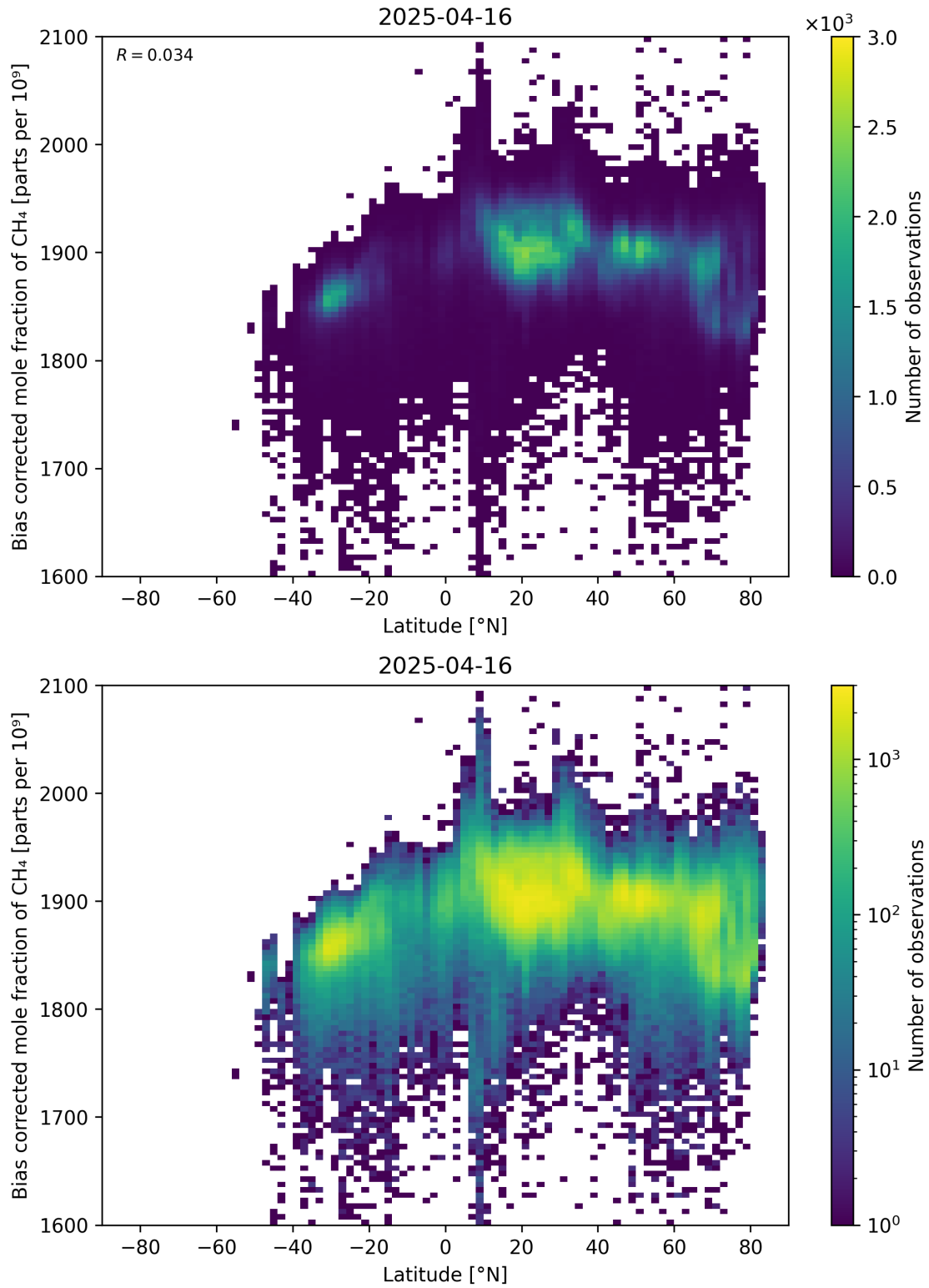
Figure 58: Scatter density plot of “Latitude” against “Bias corrected mole fraction of \text{CH}_4 ” for 2025-04-15 to 2025-04-17.
