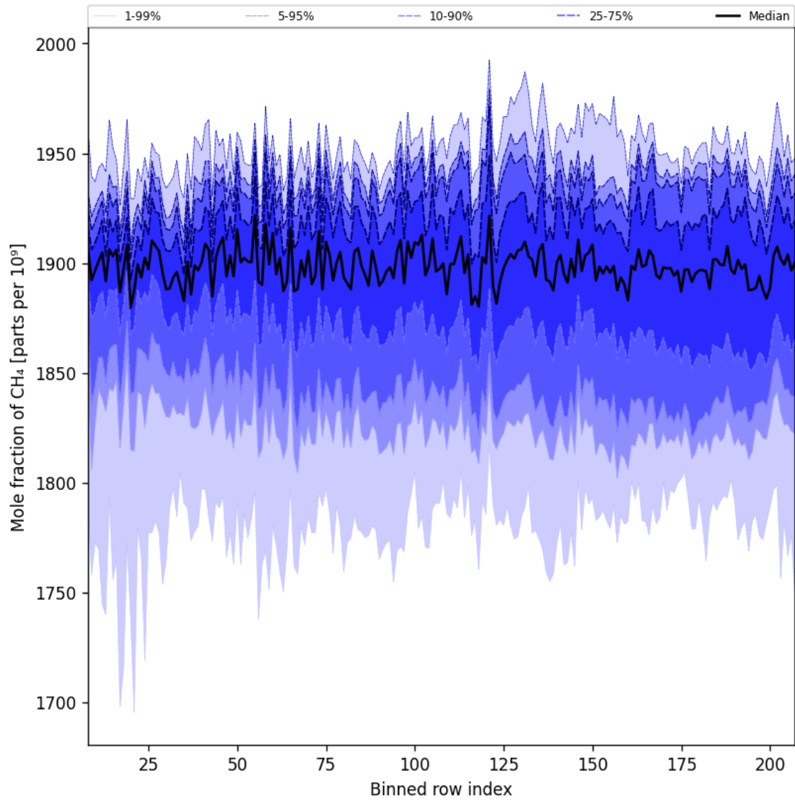
Figure 34: Along track statistics of “Mole fraction of CH 4 ” for 2025-04-15 to 2025-04-17
