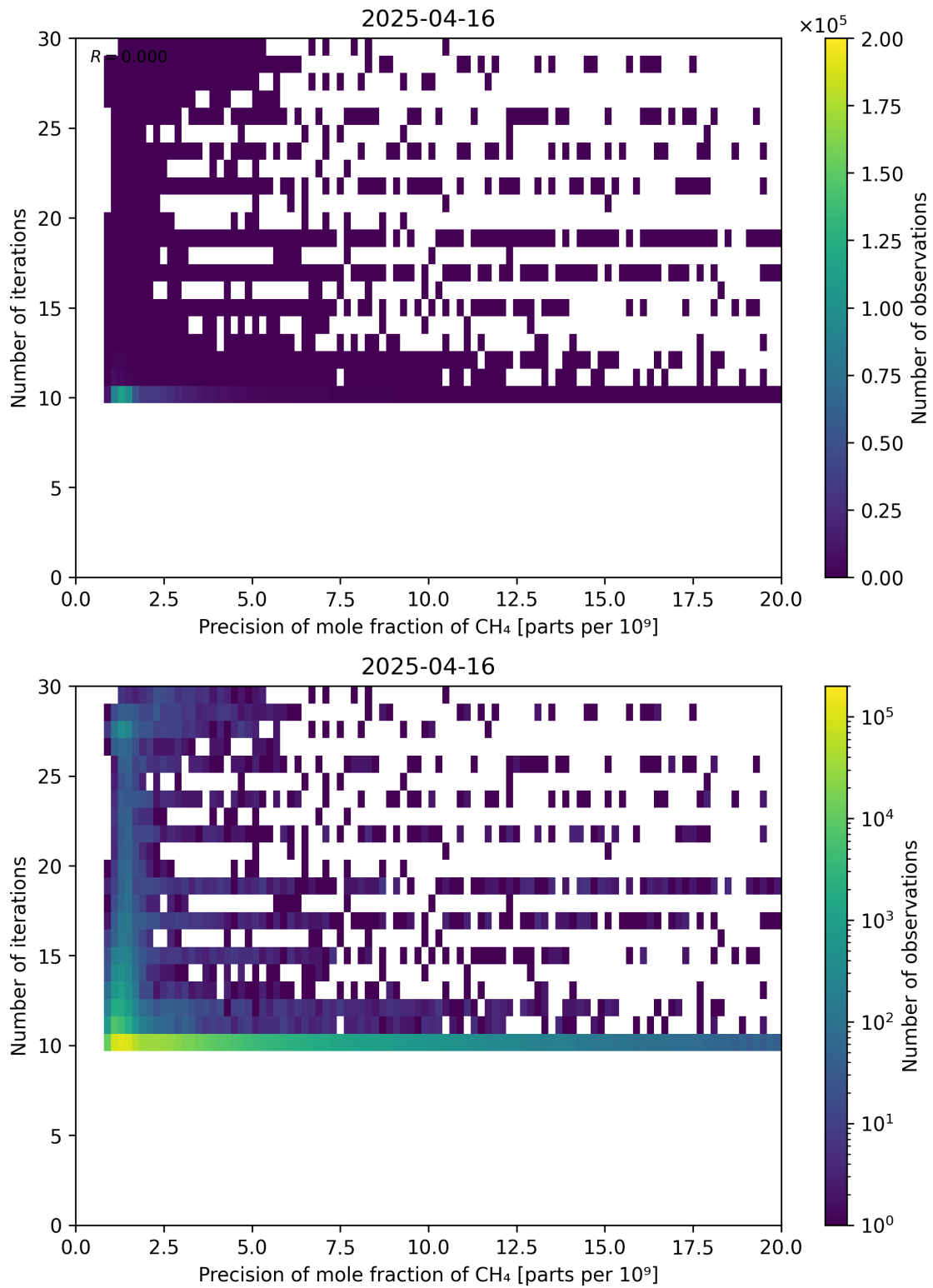
Figure 83: Scatter density plot of “Precision of mole fraction of CH 4 ” against “Number of iterations” for 2025-04-15 to 2025-04-17.
