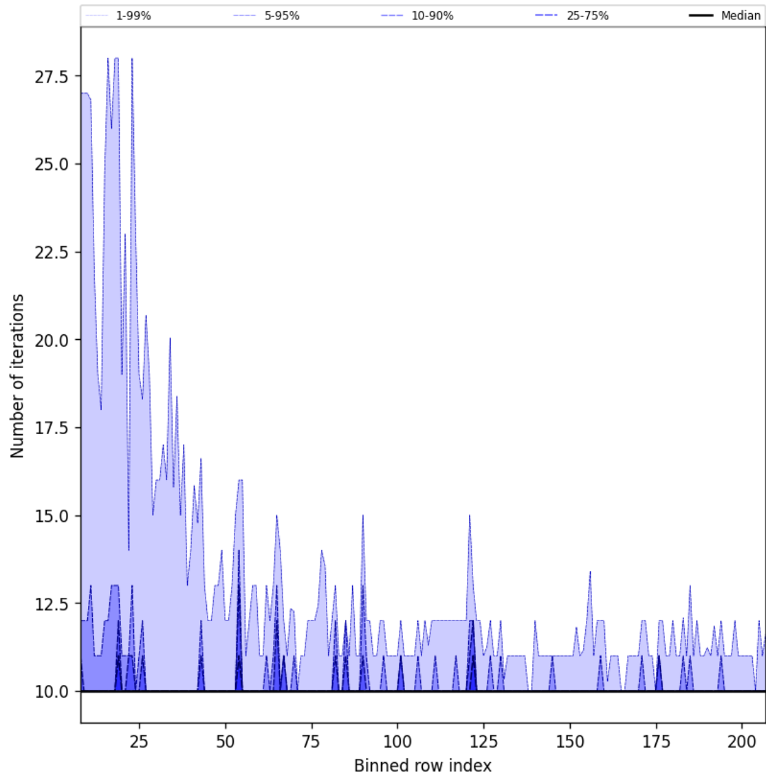
Figure 42: Along track statistics of “Number of iterations” for 2025-04-15 to 2025-04-17
