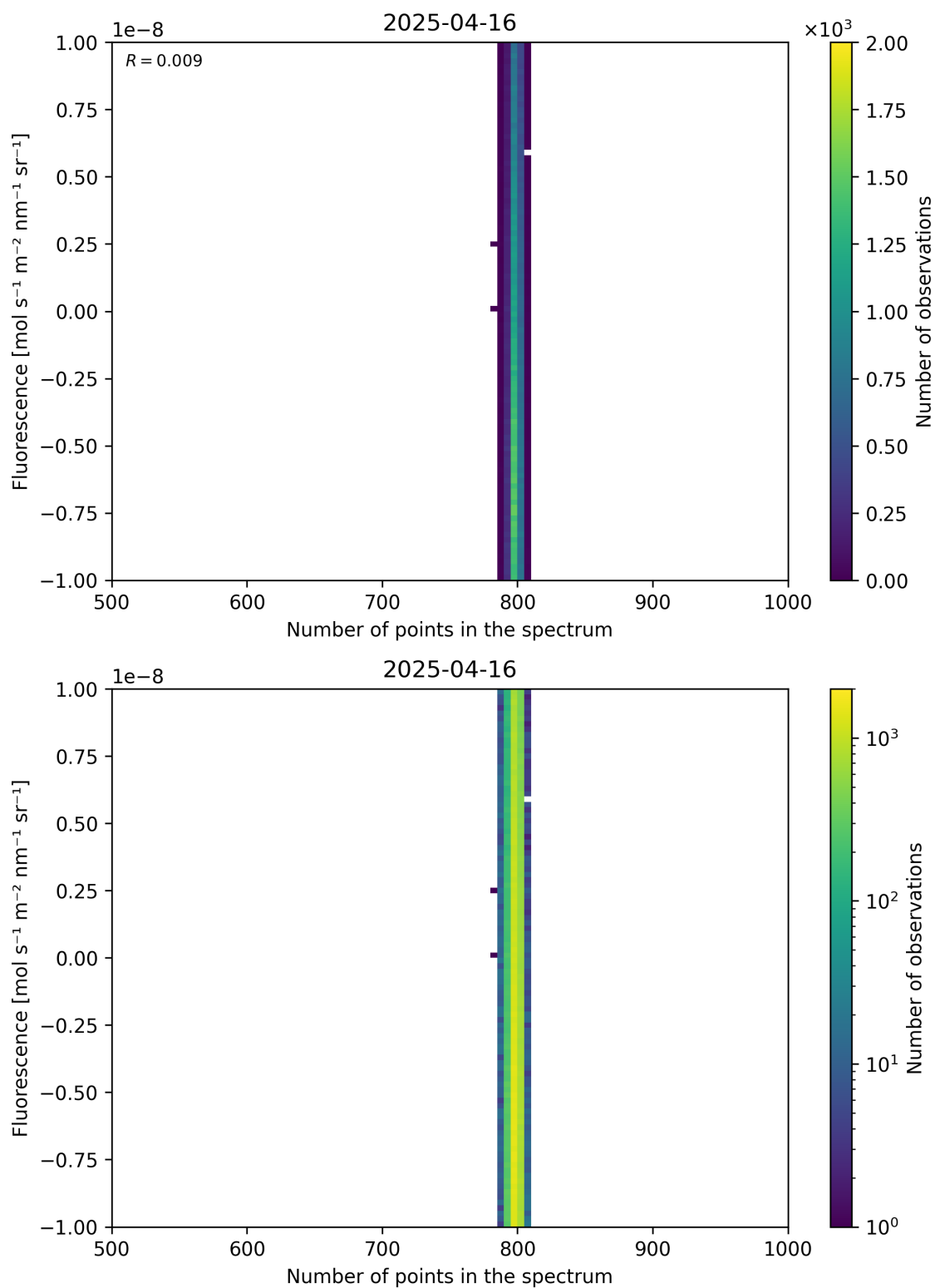
Figure 91: Scatter density plot of “Number of points in the spectrum” against “Fluorescence” for 2025-04-15 to 2025-04-17.
