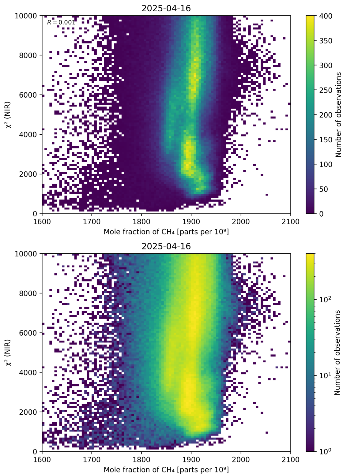
Figure 70: Scatter density plot of “Mole fraction of \text{CH}_4 ” against “ \chi^2 (NIR)” for 2025-04-15 to 2025-04-17.
