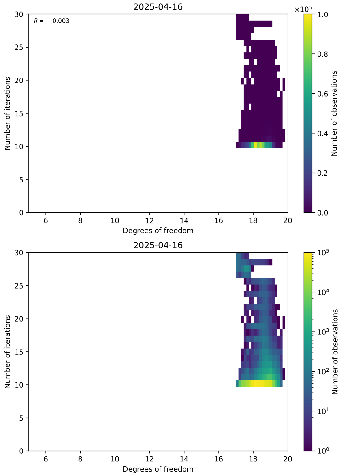
Figure 52: Scatter density plot of “Degrees of freedom” against “Number of iterations” for 2025-04-15 to 2025-04-17.
