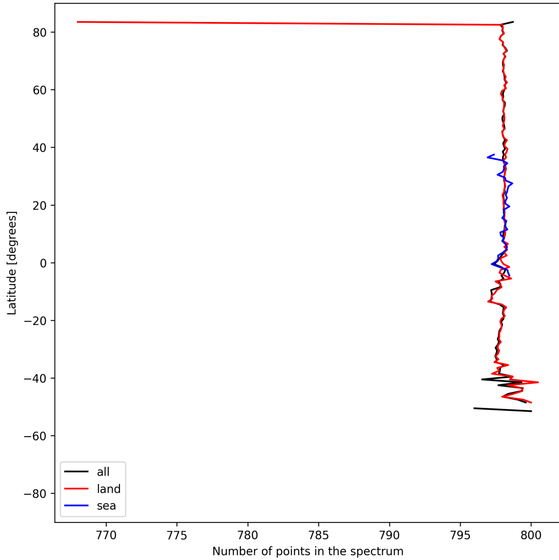
Figure 15: Zonal average of “Number of points in the spectrum” for 2025-04-15 to 2025-04-17.
