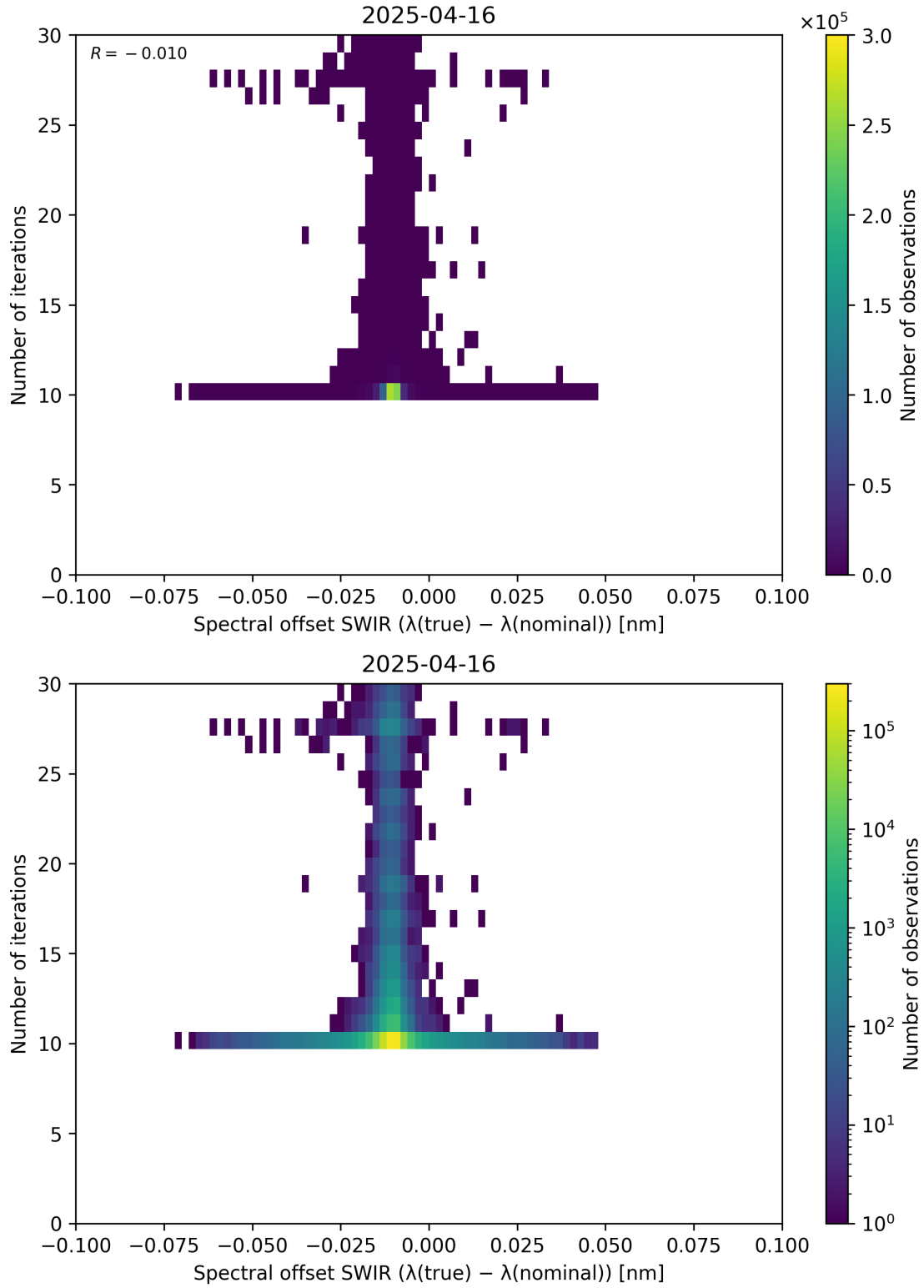
Figure 121: Scatter density plot of “Spectral offset SWIR ( \lambda_{\text{true}} - \lambda_{\text{nominal}} )” against “Number of iterations” for 2025-04-15 to 2025-04-17.
