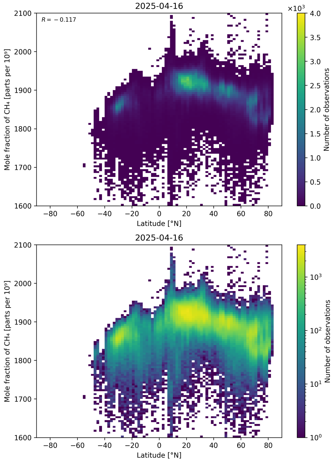
Figure 57: Scatter density plot of “Latitude” against “Mole fraction of CH 4 ” for 2025-04-15 to 2025-04-17.
