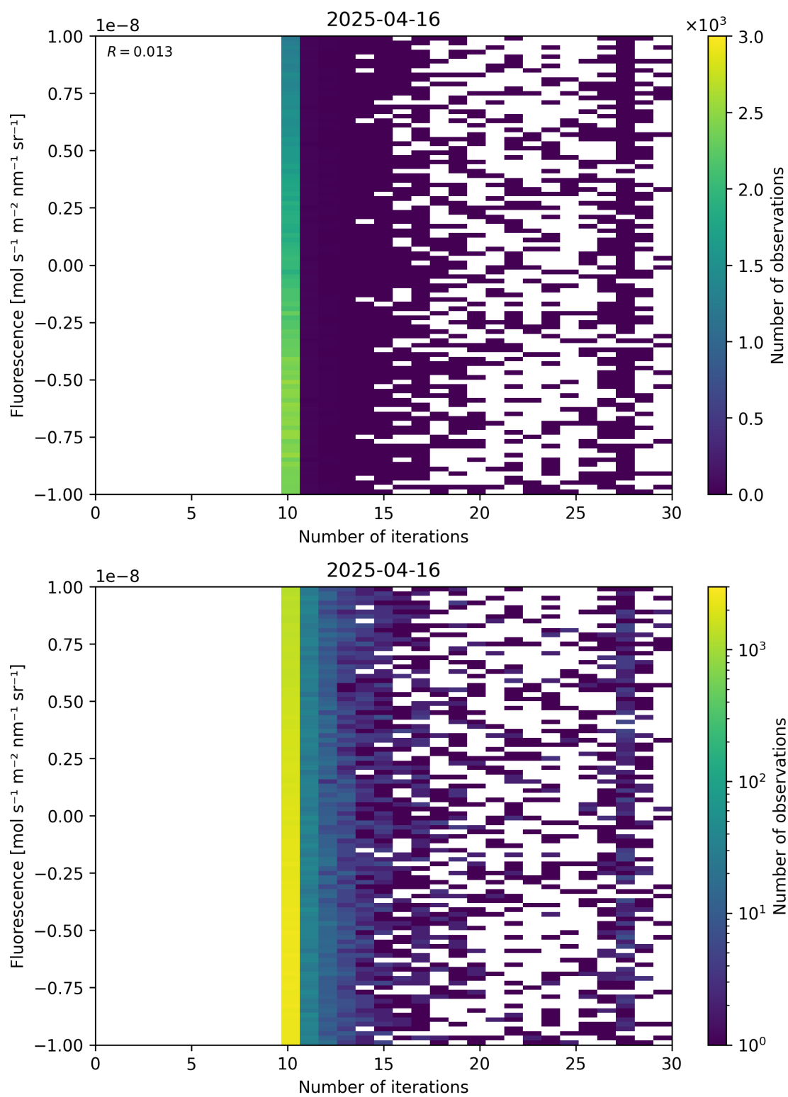
Figure 87: Scatter density plot of “Number of iterations” against “Fluorescence” for 2025-04-15 to 2025-04-17.
