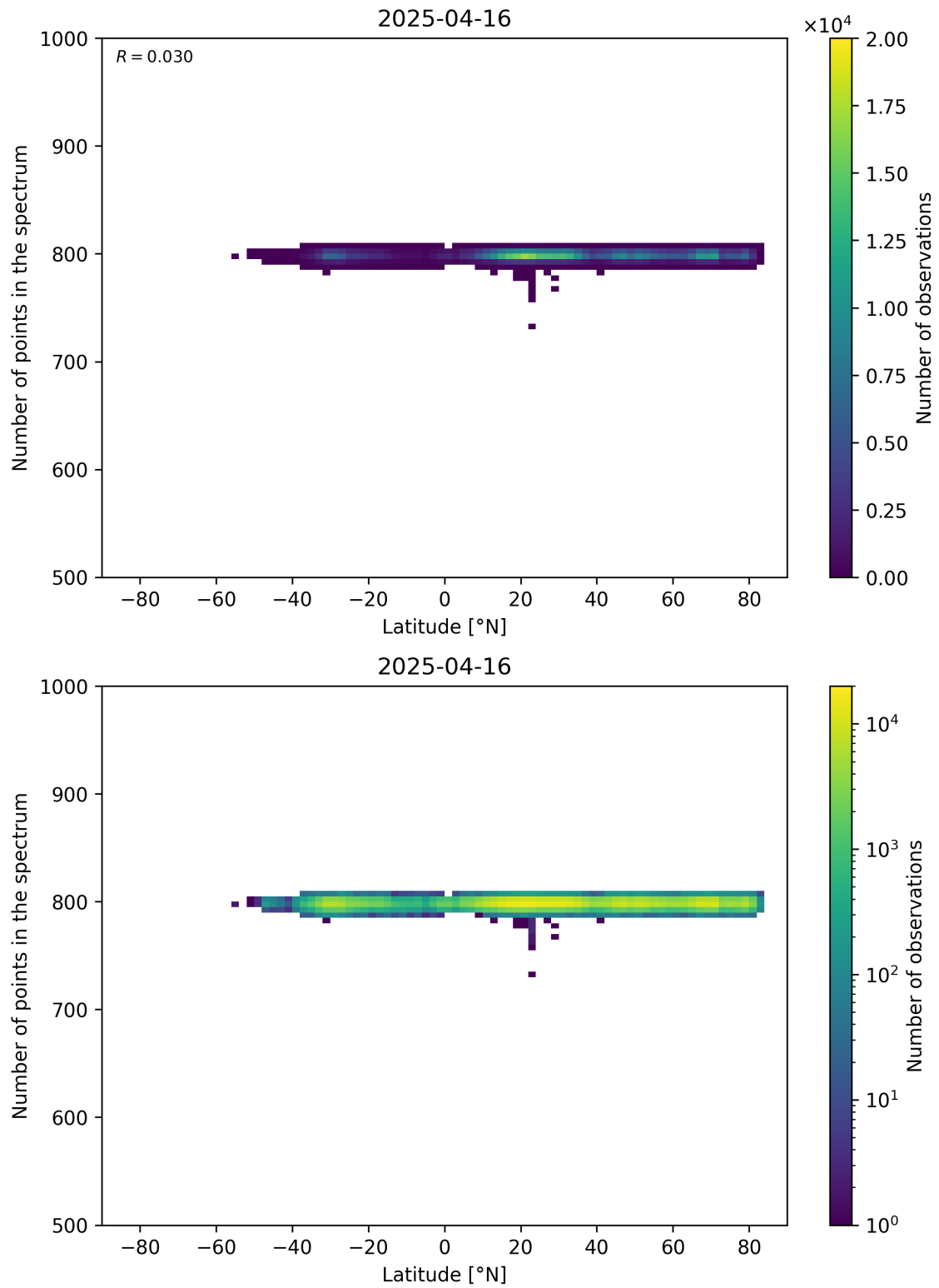
Figure 61: Scatter density plot of “Latitude” against “Number of points in the spectrum” for 2025-04-15 to 2025-04-17.
