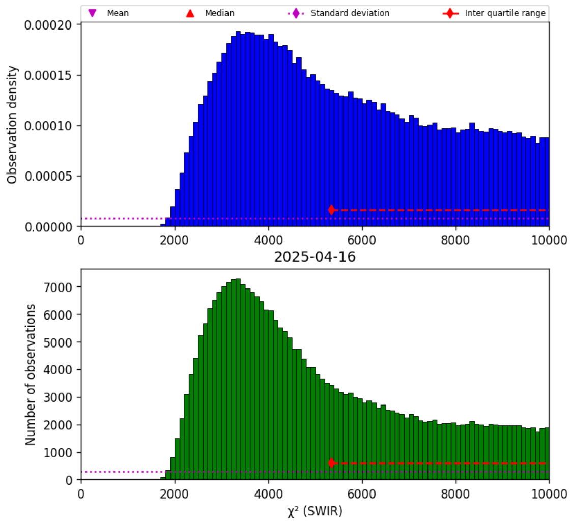
Figure 28: Histogram of “ \chi^2 (SWIR)” for 2025-04-15 to 2025-04-17
