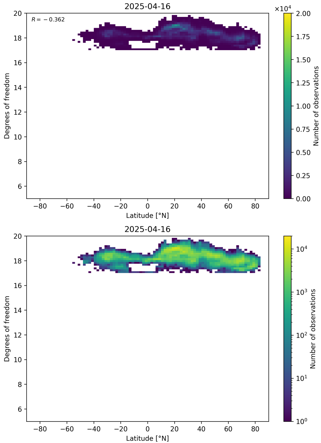
Figure 55: Scatter density plot of “Latitude” against “Degrees of freedom” for 2025-04-15 to 2025-04-17.
