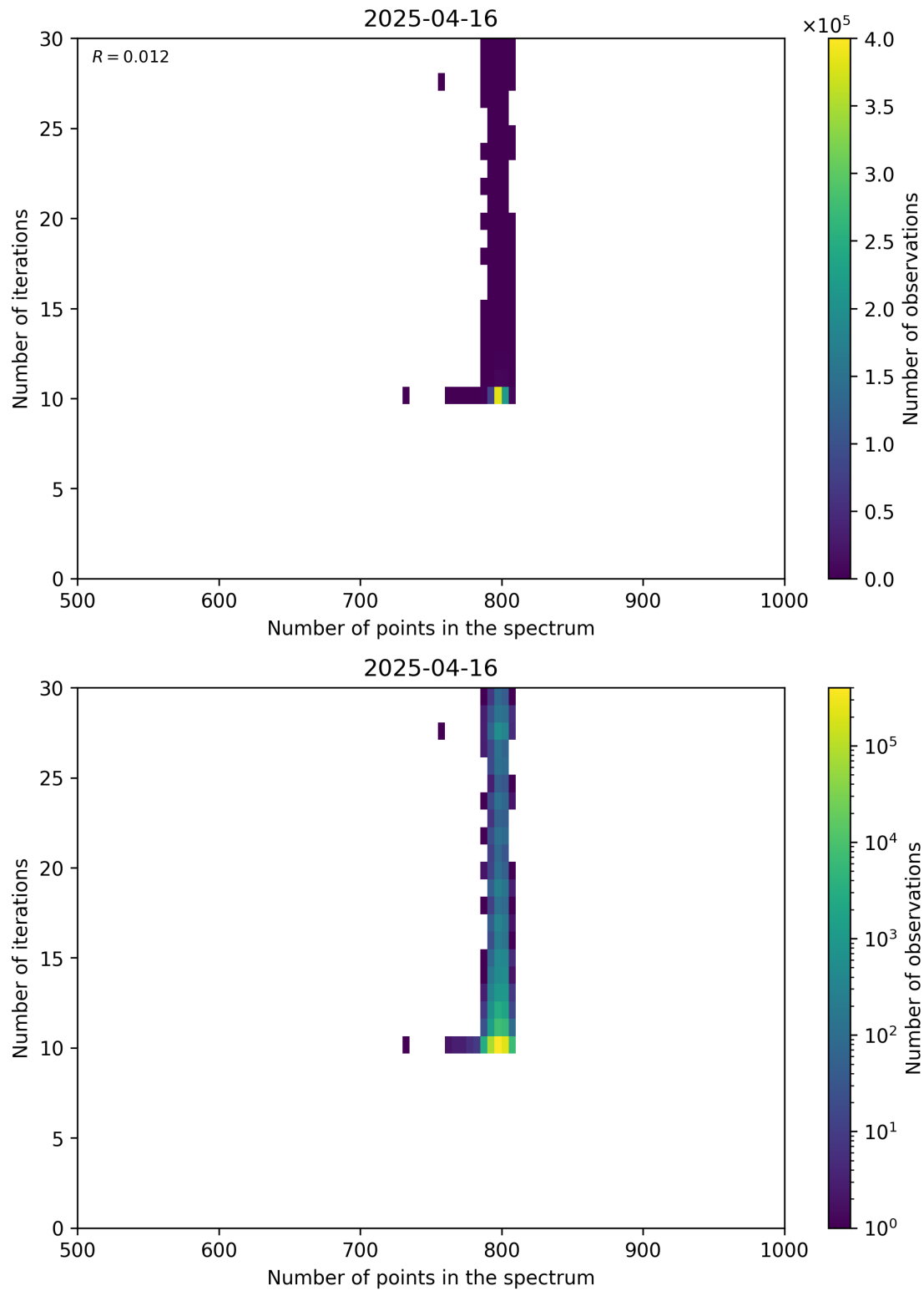
Figure 92: Scatter density plot of “Number of points in the spectrum” against “Number of iterations” for 2025-04-15 to 2025-04-17.
