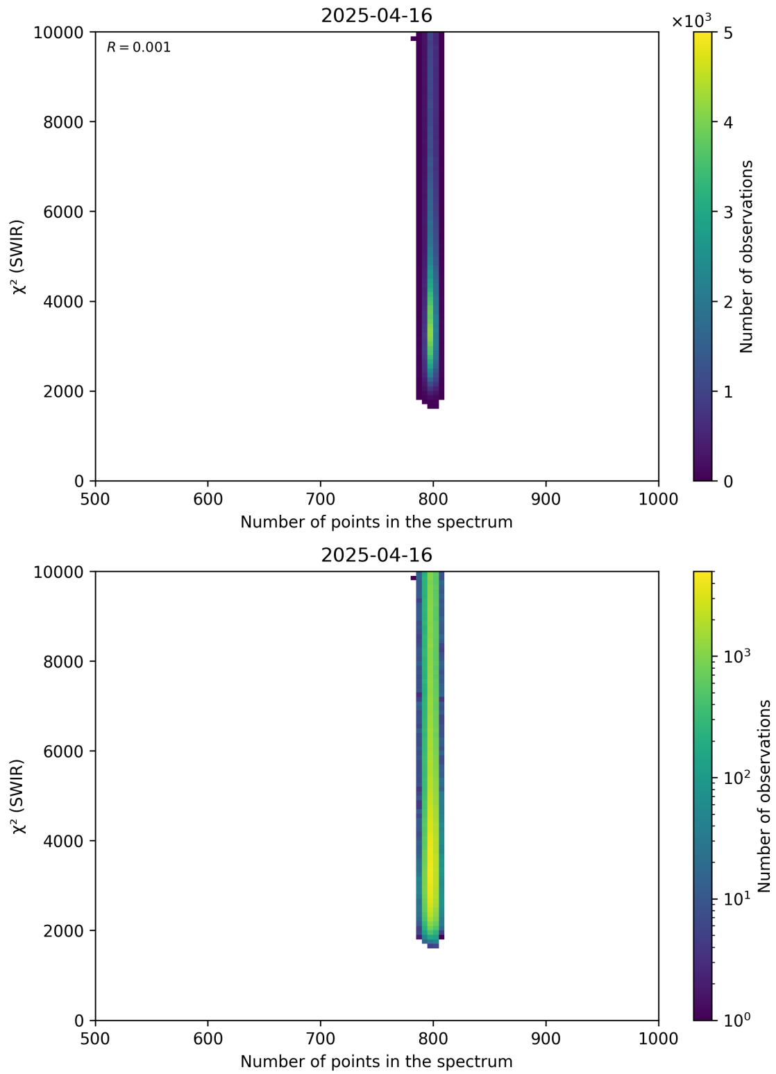
Figure 89: Scatter density plot of “Number of points in the spectrum” against “ \chi^2 (SWIR)” for 2025-04-15 to 2025-04-17.
