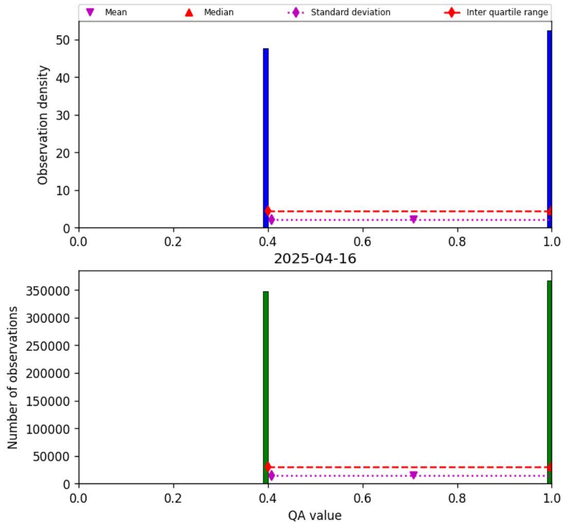
Figure 22: Histogram of “QA value” for 2025-04-15 to 2025-04-17
