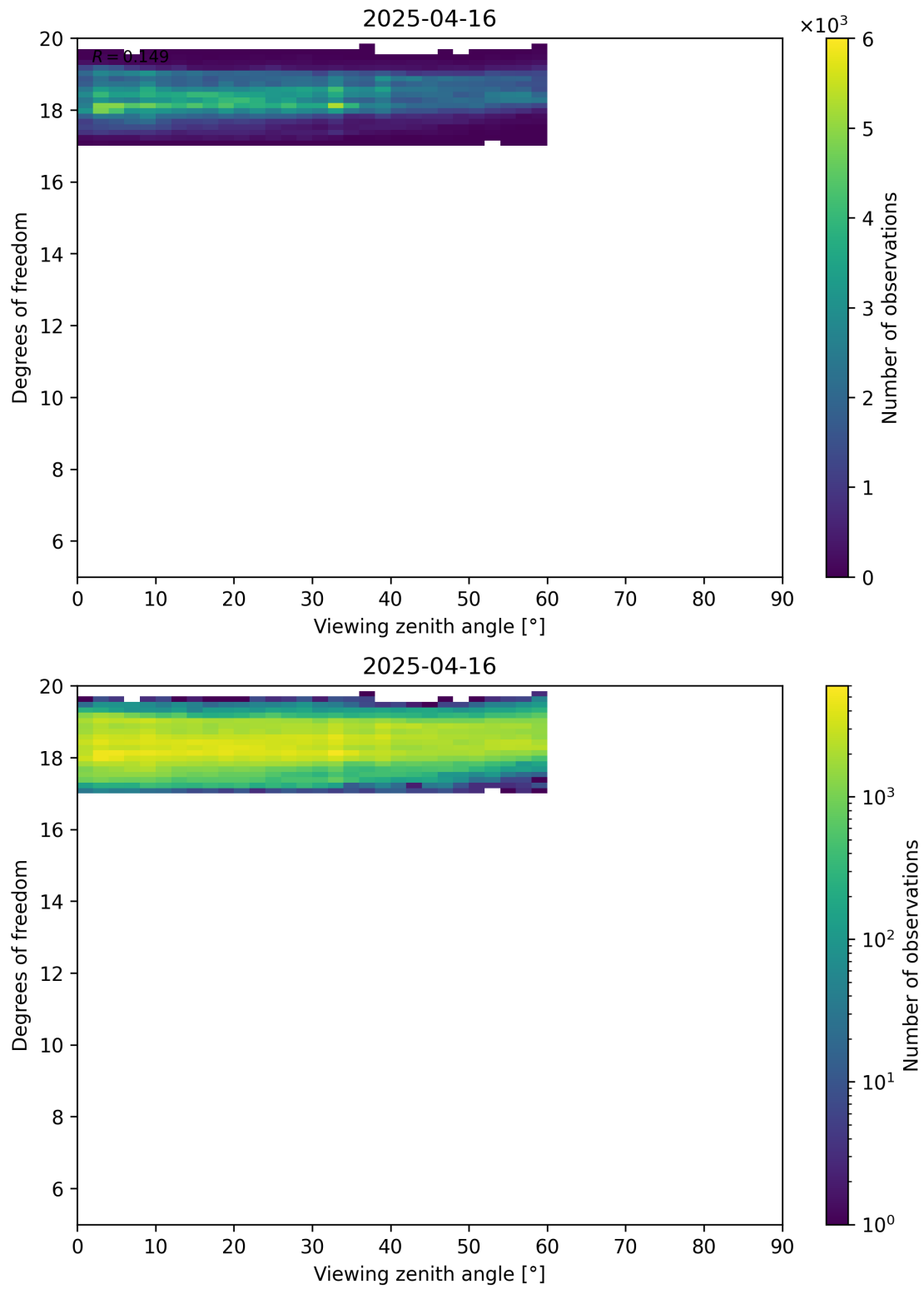
Figure 107: Scatter density plot of “Viewing zenith angle” against “Degrees of freedom” for 2025-04-15 to 2025-04-17.
