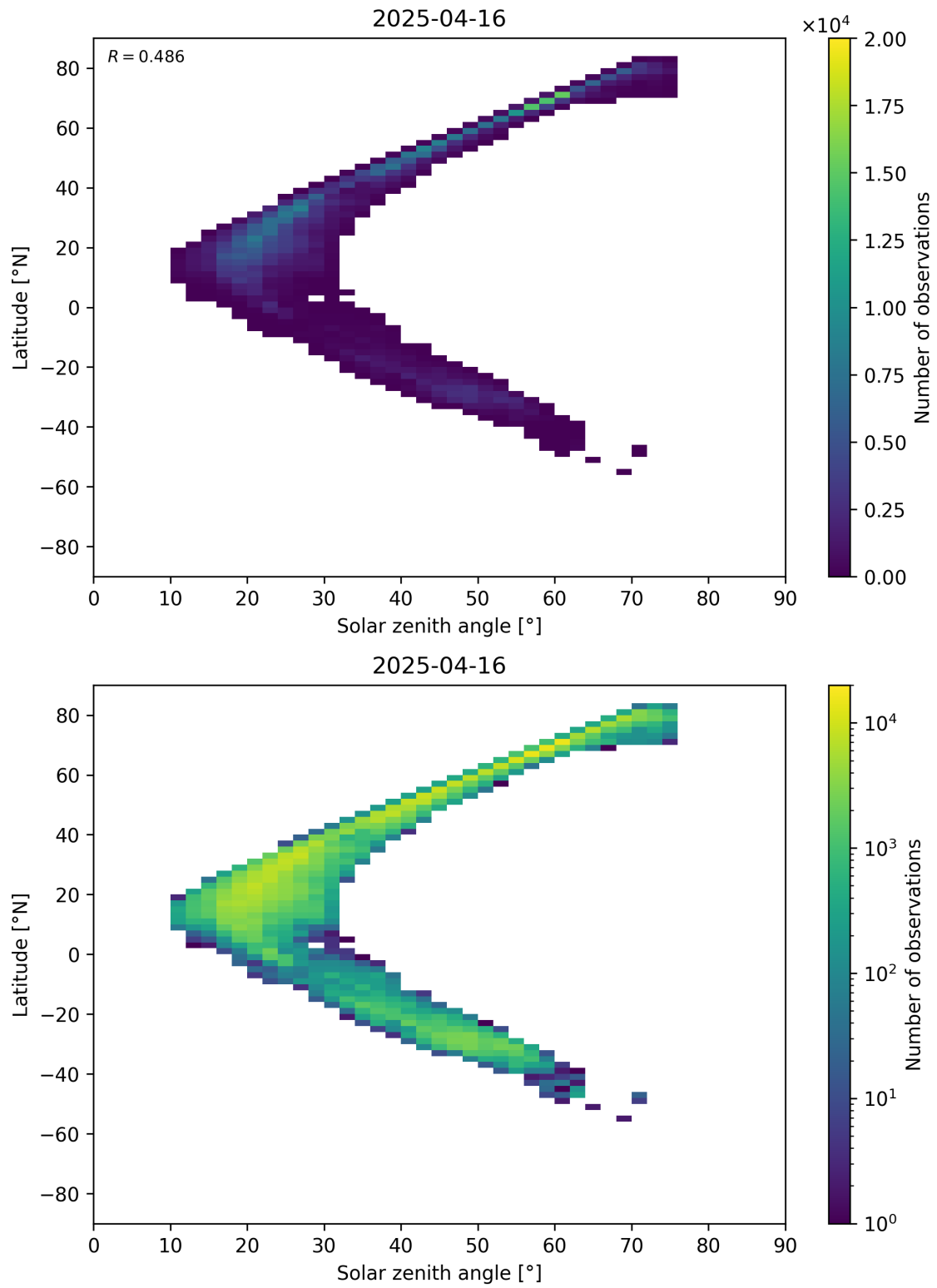
Figure 98: Scatter density plot of “Solar zenith angle” against “Latitude” for 2025-04-15 to 2025-04-17.
