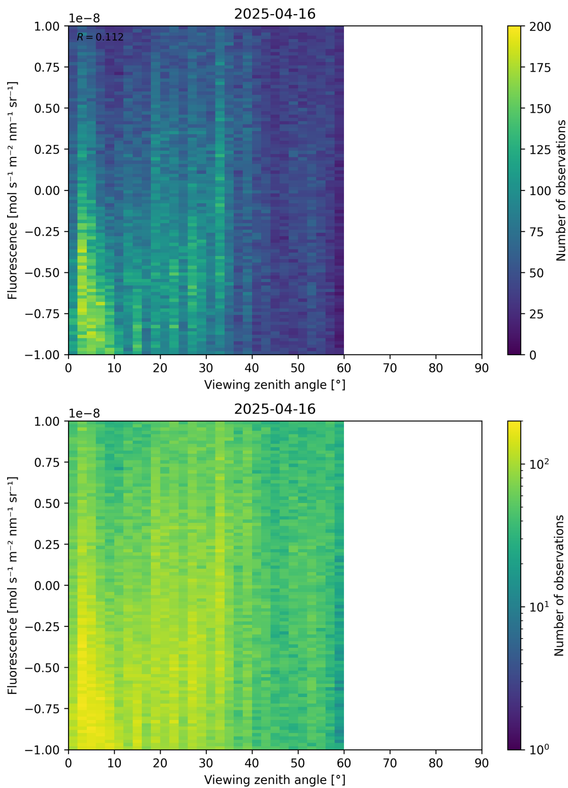
Figure 108: Scatter density plot of “Viewing zenith angle” against “Fluorescence” for 2025-04-15 to 2025-04-17.
