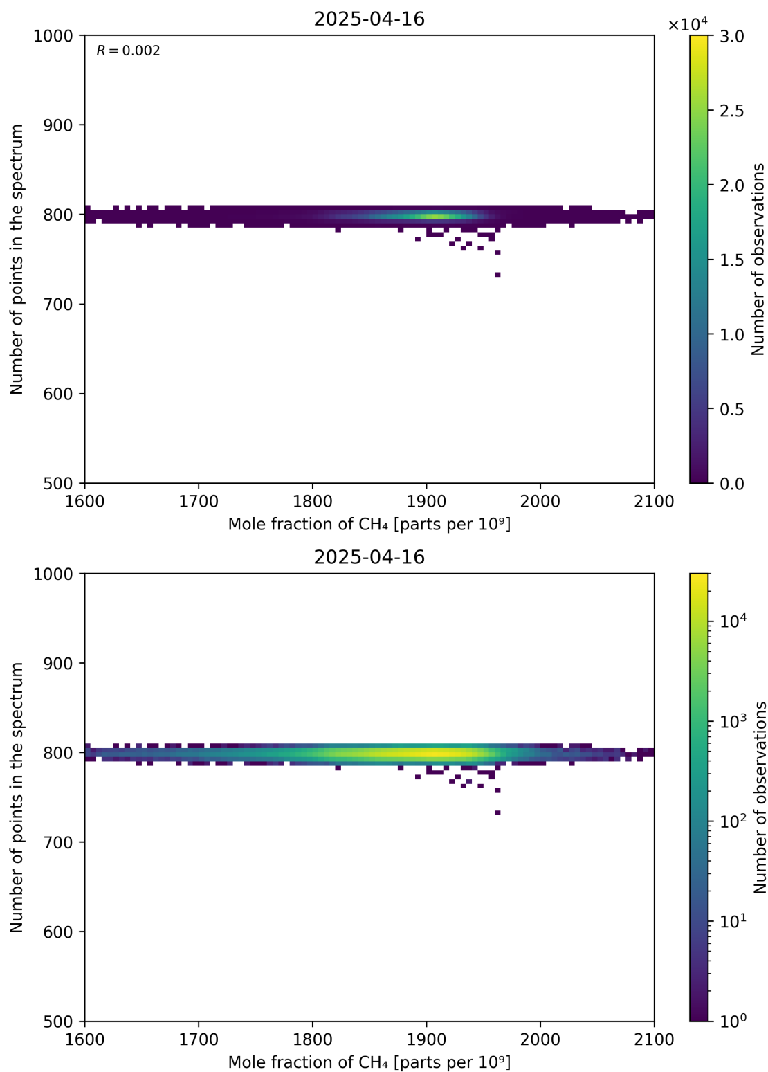
Figure 77: Scatter density plot of “Mole fraction of CH 4 ” against “Number of points in the spectrum” for 2025-04-15 to 2025-04-17.
