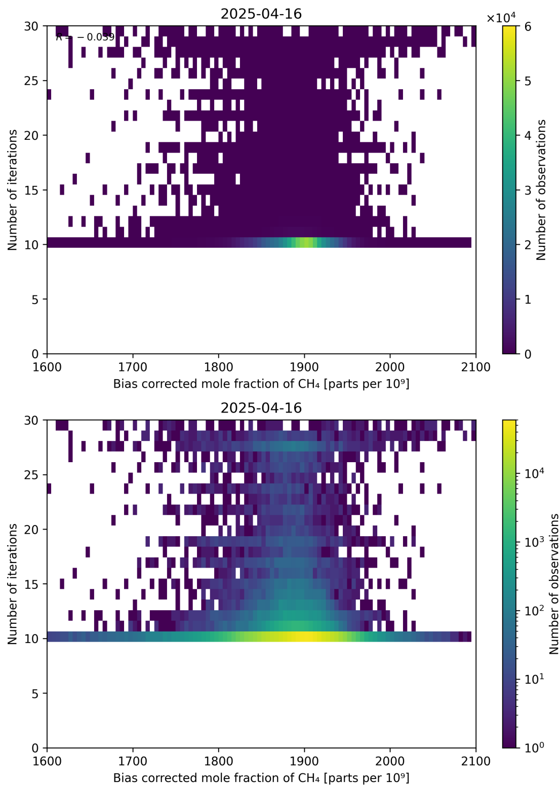
Figure 67: Scatter density plot of “Bias corrected mole fraction of \text{CH}_4 ” against “Number of iterations” for 2025-04-15 to 2025-04-17.
