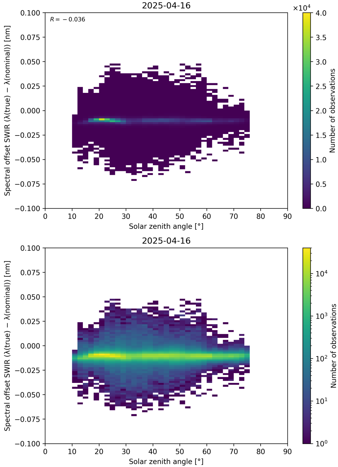
Figure 104: Scatter density plot of “Solar zenith angle” against “Spectral offset SWIR ( \lambda_{\text{true}} - \lambda_{\text{nominal}} )” for 2025-04-15 to 2025-04-17.
