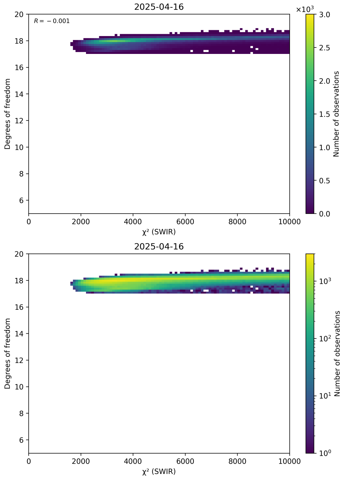
Figure 48: Scatter density plot of “ \chi^2 (SWIR)” against “Degrees of freedom” for 2025-04-15 to 2025-04-17.
