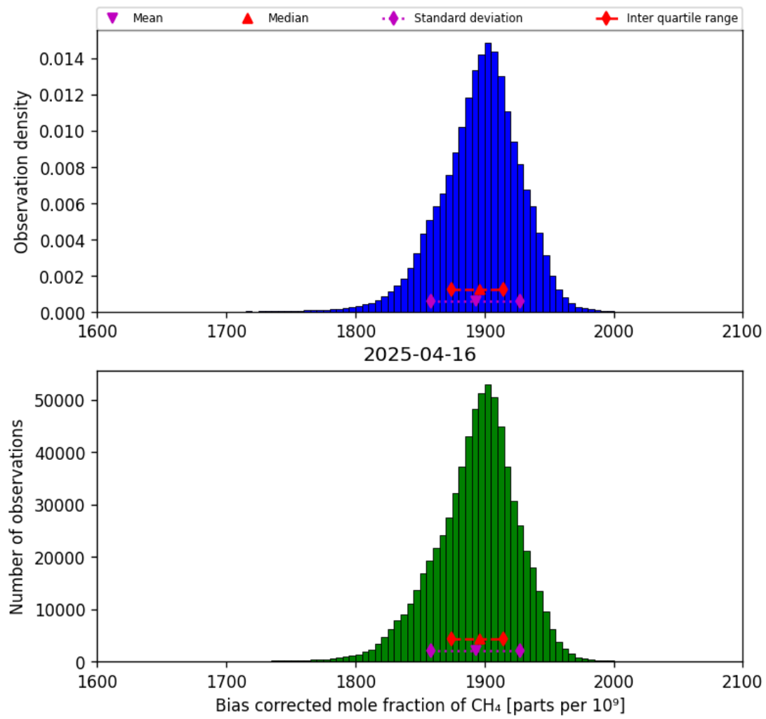
Figure 25: Histogram of “Bias corrected mole fraction of CH 4 ” for 2025-04-15 to 2025-04-17
