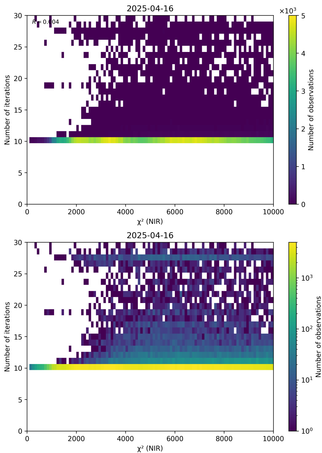
Figure 46: Scatter density plot of “ \chi^2 (NIR)” against “Number of iterations” for 2025-04-15 to 2025-04-17.
