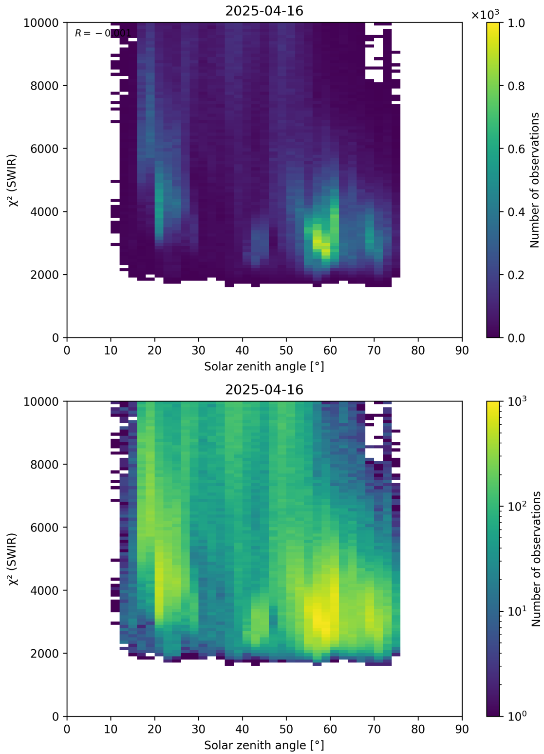
Figure 95: Scatter density plot of “Solar zenith angle” against “ \chi^2 (SWIR)” for 2025-04-15 to 2025-04-17.
