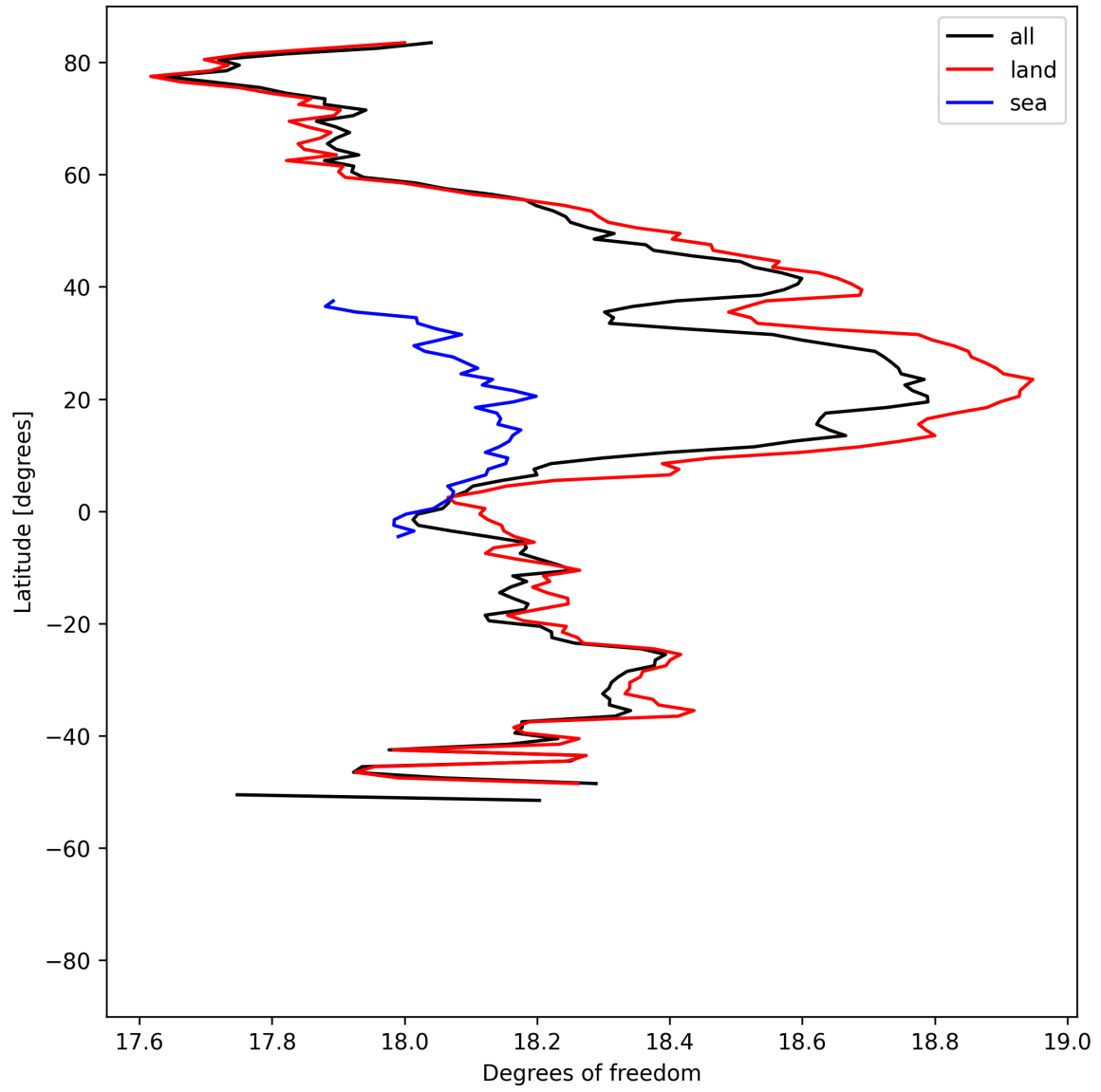
Figure 19: Zonal average of “Degrees of freedom” for 2025-04-15 to 2025-04-17.
