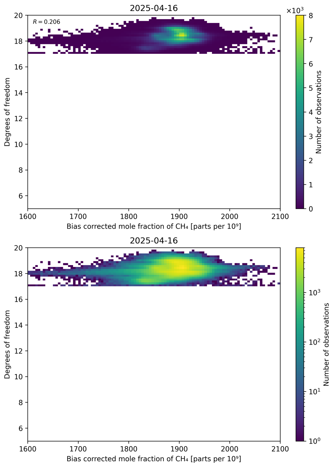
Figure 65: Scatter density plot of “Bias corrected mole fraction of CH 4 ” against “Degrees of freedom” for 2025-04-15 to 2025-04-17.
