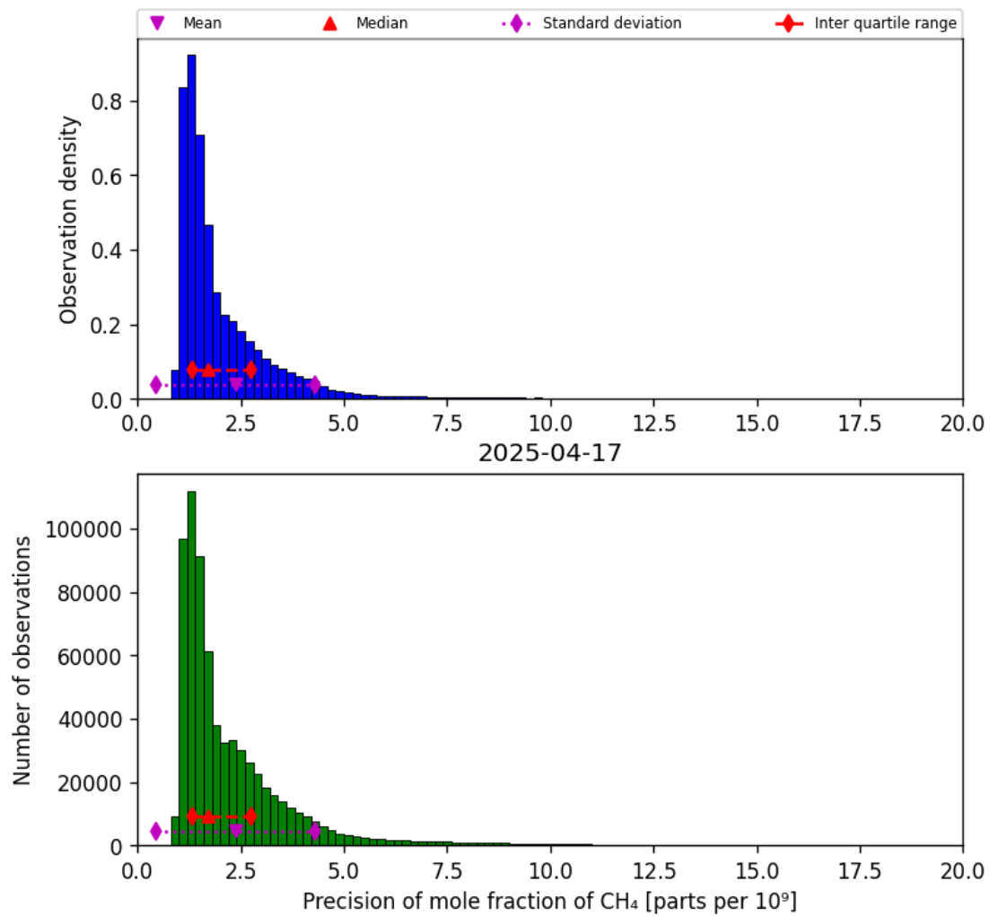
Figure 24: Histogram of “Precision of mole fraction of CH 4 ” for 2025-04-16 to 2025-04-18
