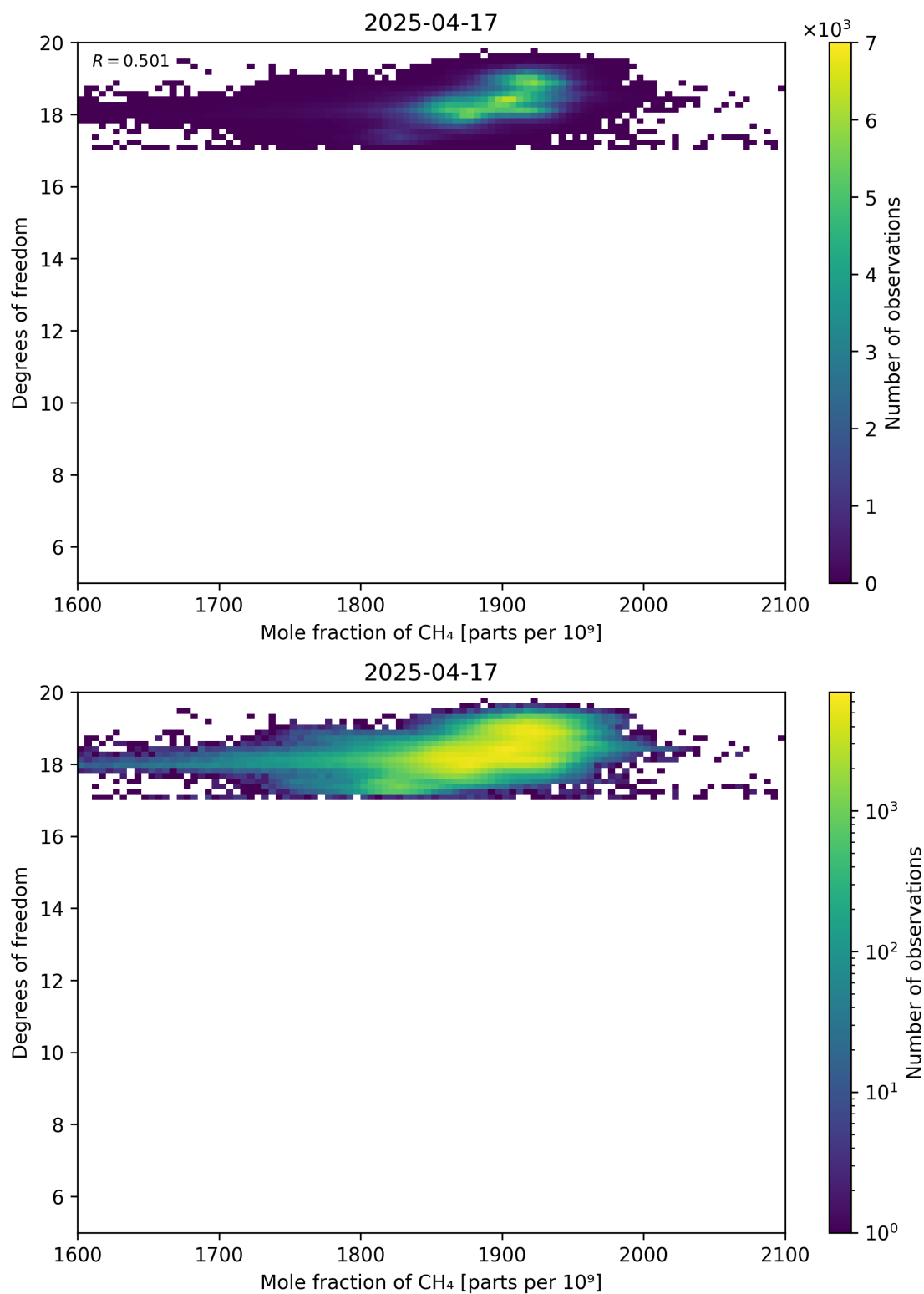
Figure 72: Scatter density plot of “Mole fraction of CH 4 ” against “Degrees of freedom” for 2025-04-16 to 2025-04-18.
