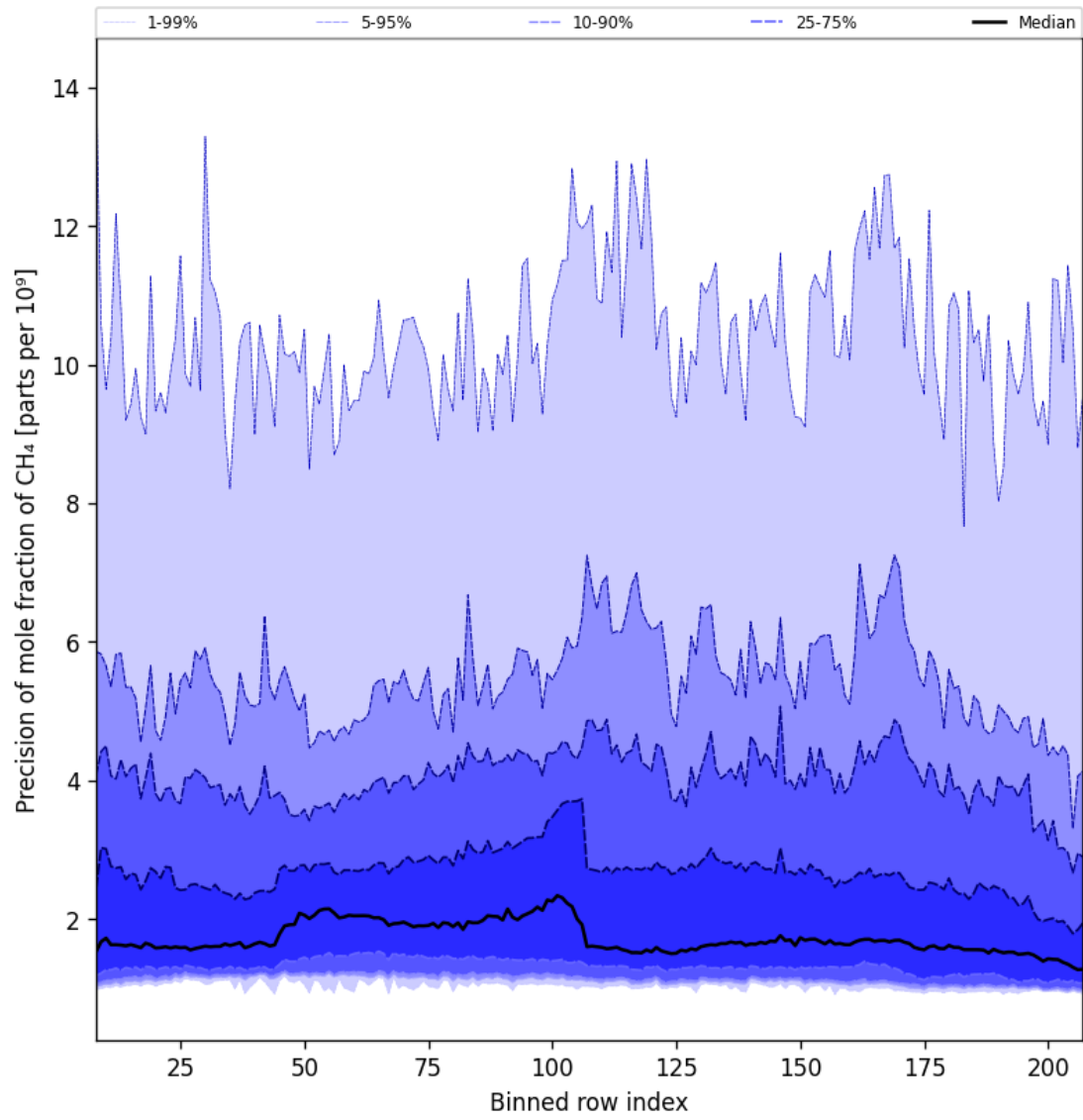
Figure 35: Along track statistics of “Precision of mole fraction of CH 4 ” for 2025-04-16 to 2025-04-18
