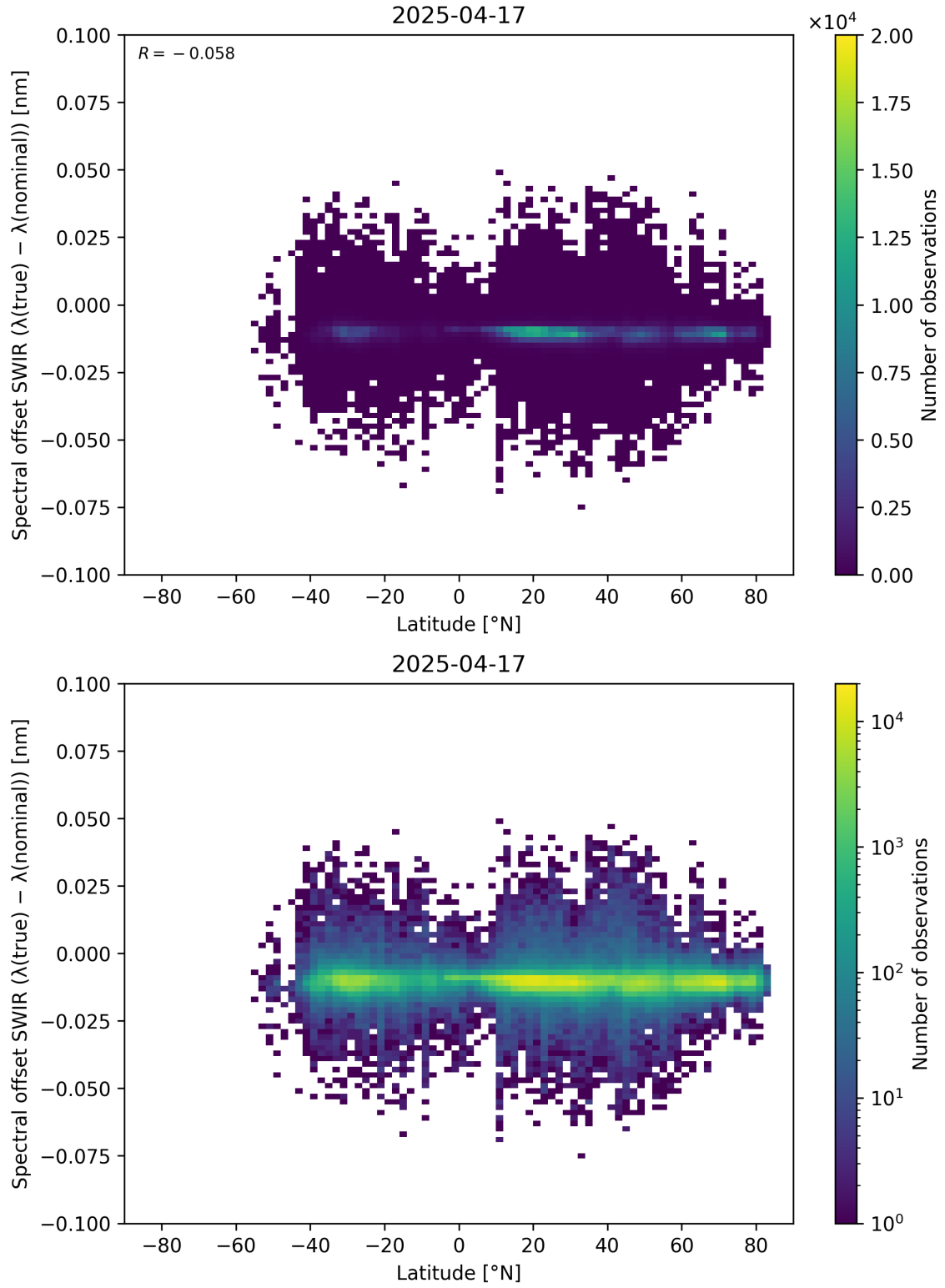
Figure 62: Scatter density plot of “Latitude” against “Spectral offset SWIR ( \lambda_{\text{true}} - \lambda_{\text{nominal}} )” for 2025-04-16 to 2025-04-18.
