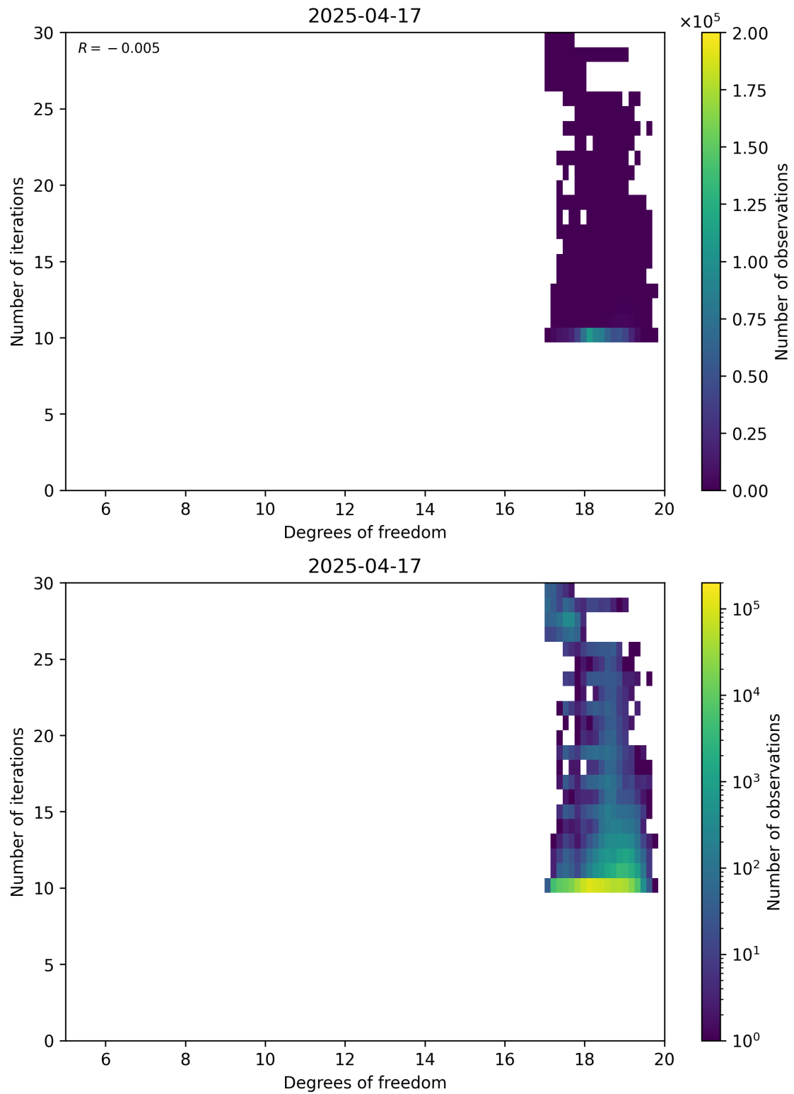
Figure 52: Scatter density plot of “Degrees of freedom” against “Number of iterations” for 2025-04-16 to 2025-04-18.
