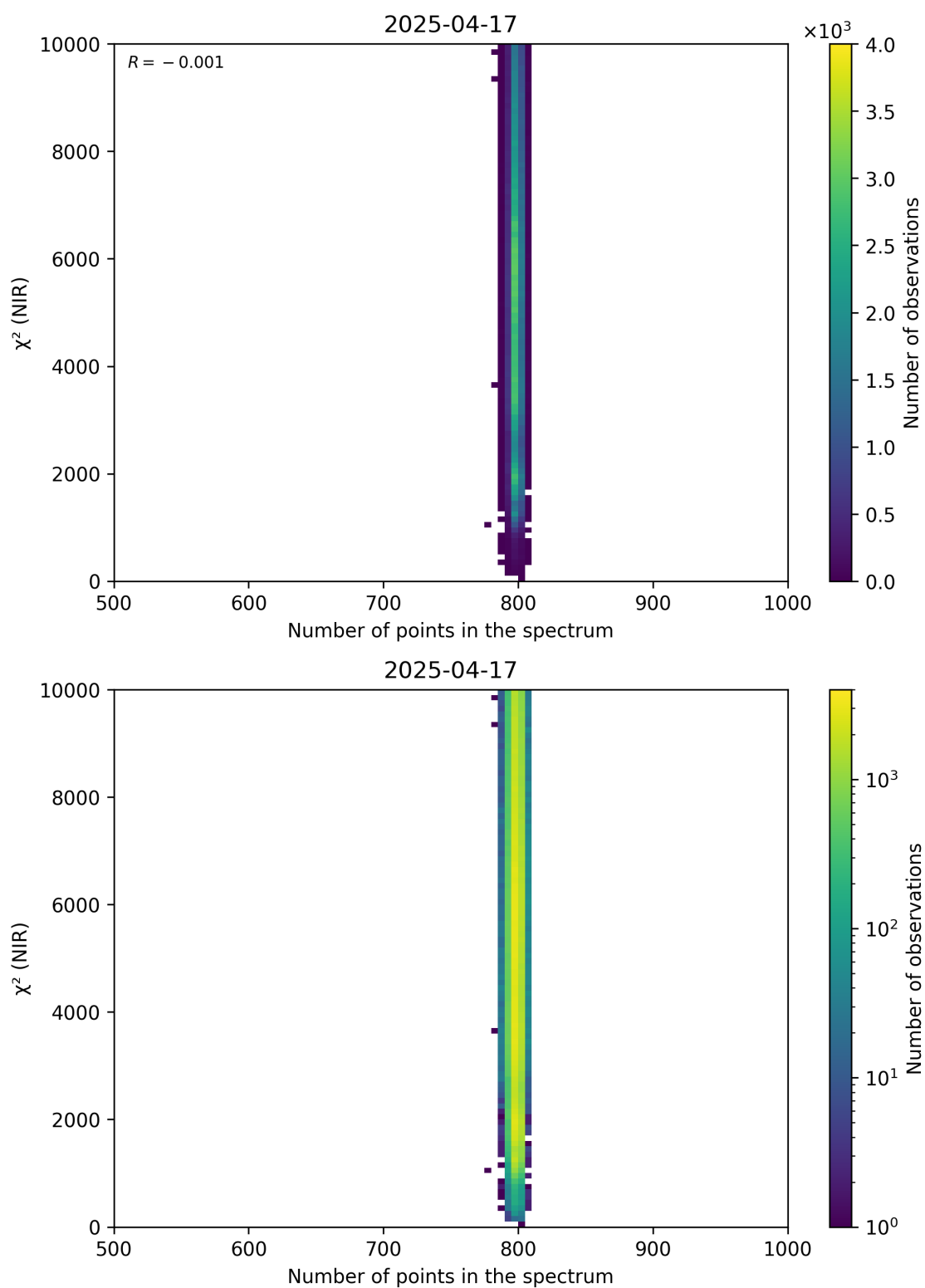
Figure 88: Scatter density plot of “Number of points in the spectrum” against “ \chi^2 (NIR)” for 2025-04-16 to 2025-04-18.
