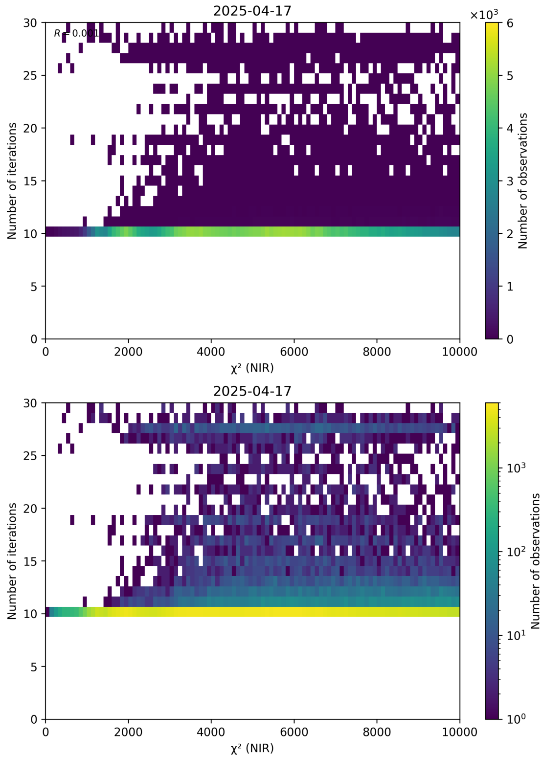
Figure 46: Scatter density plot of “ \chi^2 (NIR)” against “Number of iterations” for 2025-04-16 to 2025-04-18.
