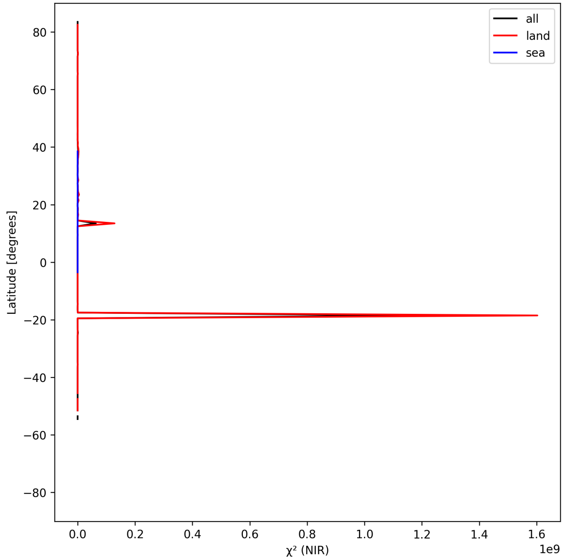
Figure 18: Zonal average of “ \chi^2 (NIR)” for 2025-04-16 to 2025-04-18.
