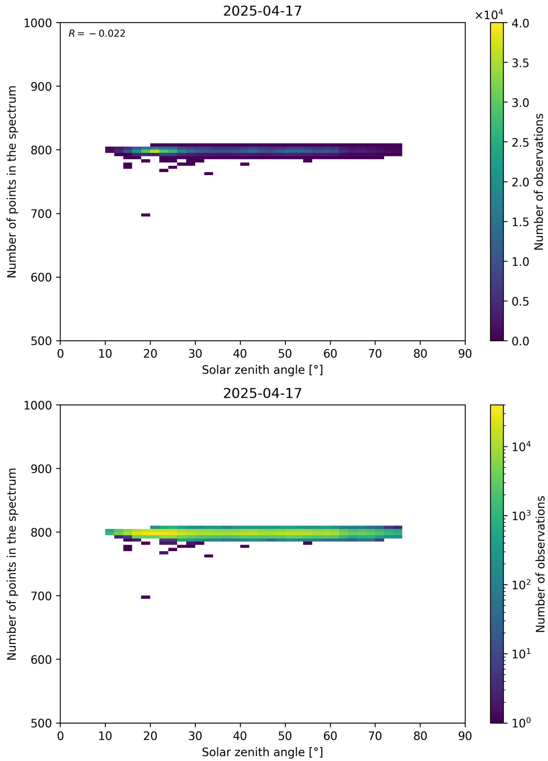
Figure 103: Scatter density plot of “Solar zenith angle” against “Number of points in the spectrum” for 2025-04-16 to 2025-04-18.
