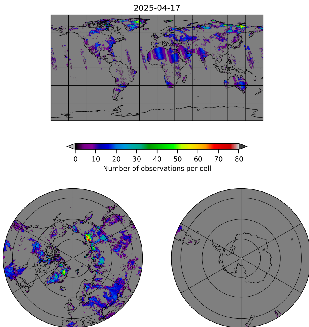
Figure 10: Map of the number of observations for 2025-04-16 to 2025-04-18
