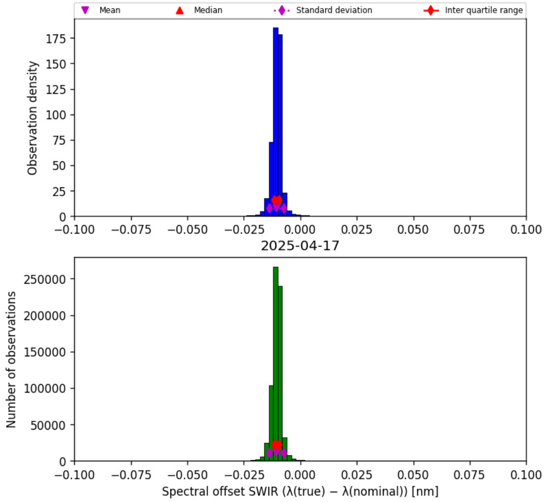
Figure 27: Histogram of “Spectral offset SWIR ( \lambda_{\text{true}} - \lambda_{\text{nominal}} )” for 2025-04-16 to 2025-04-18
