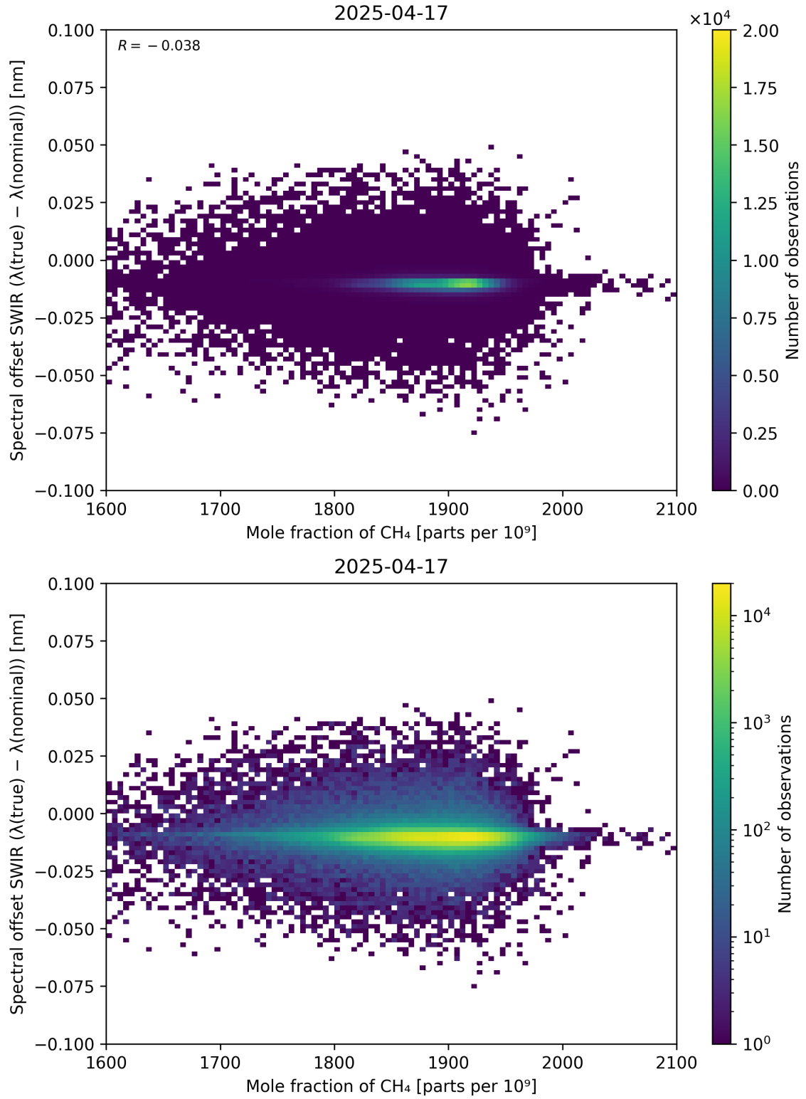
Figure 86: Scatter density plot of “Mole fraction of CH 4 ” against “Spectral offset SWIR ( \lambda_{\text{true}} - \lambda_{\text{nominal}} )” for 2025-04-16 to 2025-04-18.
