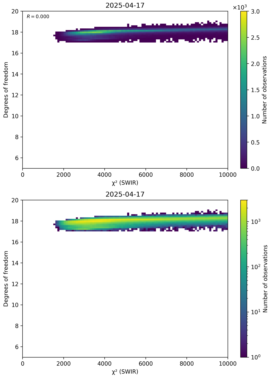
Figure 48: Scatter density plot of “ \chi^2 (SWIR)” against “Degrees of freedom” for 2025-04-16 to 2025-04-18.
