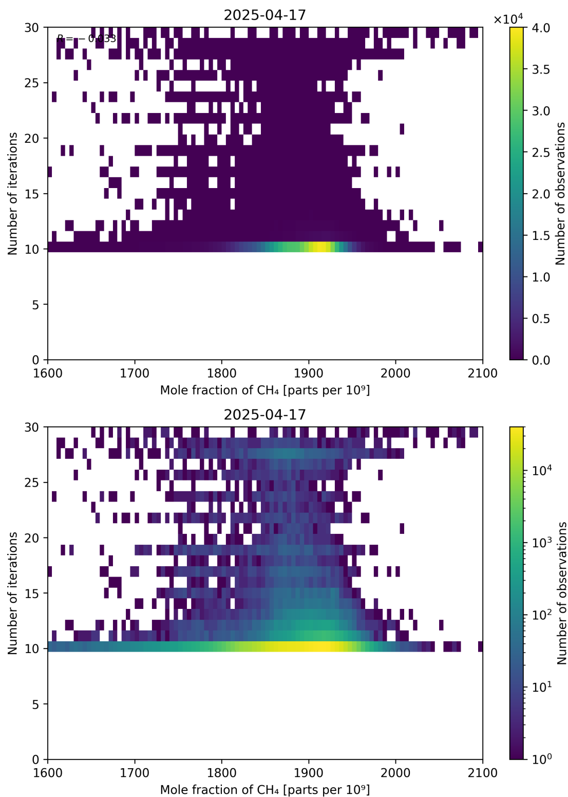
Figure 76: Scatter density plot of “Mole fraction of CH 4 ” against “Number of iterations” for 2025-04-16 to 2025-04-18.
