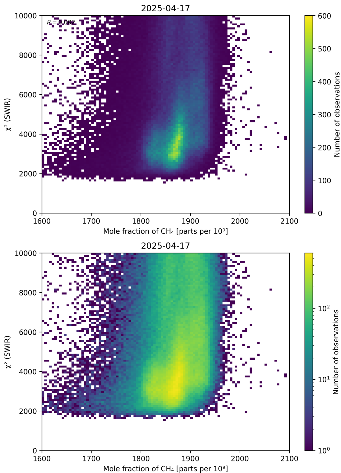
Figure 71: Scatter density plot of “Mole fraction of \text{CH}_4 ” against “ \chi^2 (SWIR)” for 2025-04-16 to 2025-04-18.
