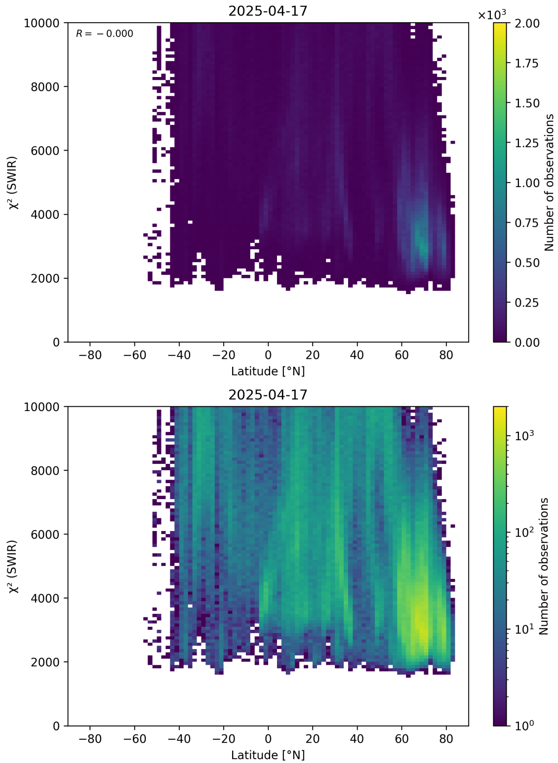
Figure 54: Scatter density plot of “Latitude” against “ \chi^2 (SWIR)” for 2025-04-16 to 2025-04-18.
