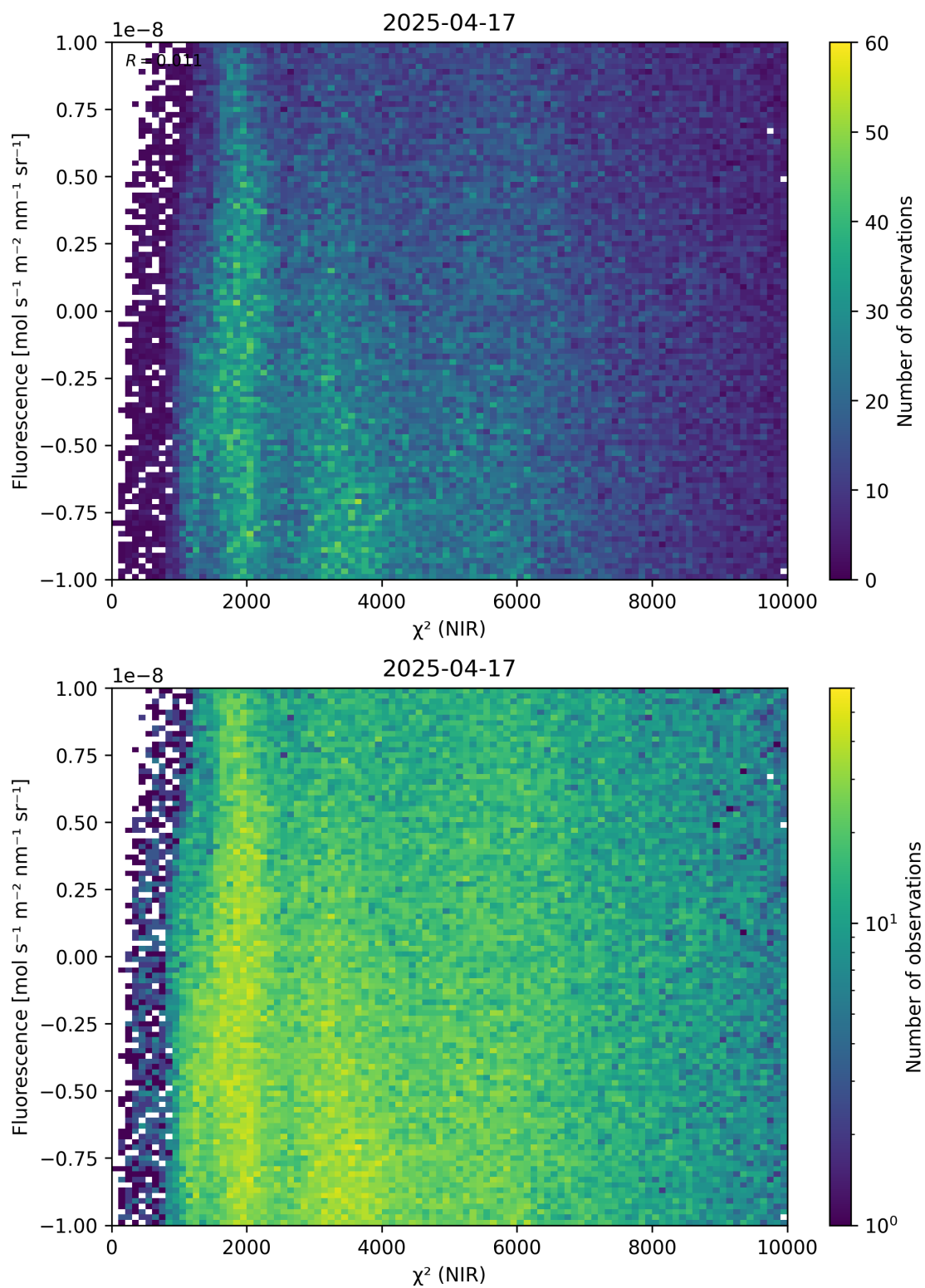
Figure 45: Scatter density plot of “ \chi^2 (NIR)” against “Fluorescence” for 2025-04-16 to 2025-04-18.
