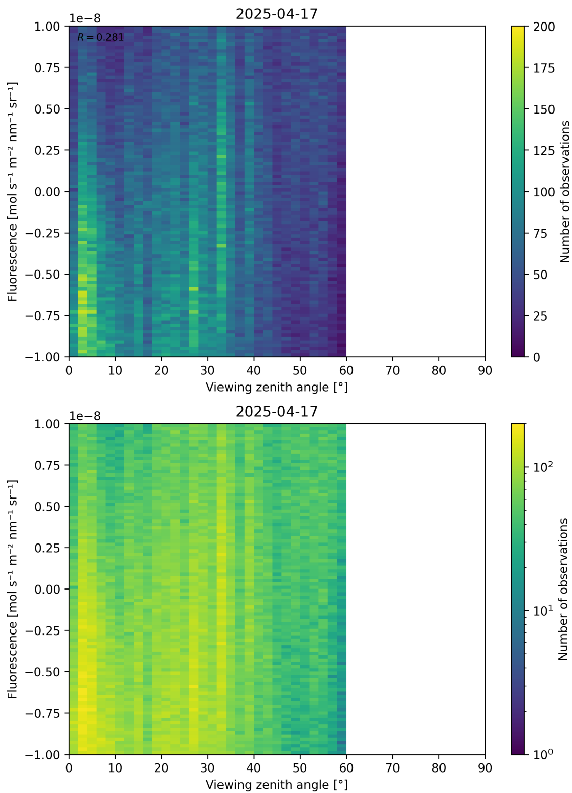
Figure 108: Scatter density plot of “Viewing zenith angle” against “Fluorescence” for 2025-04-16 to 2025-04-18.
