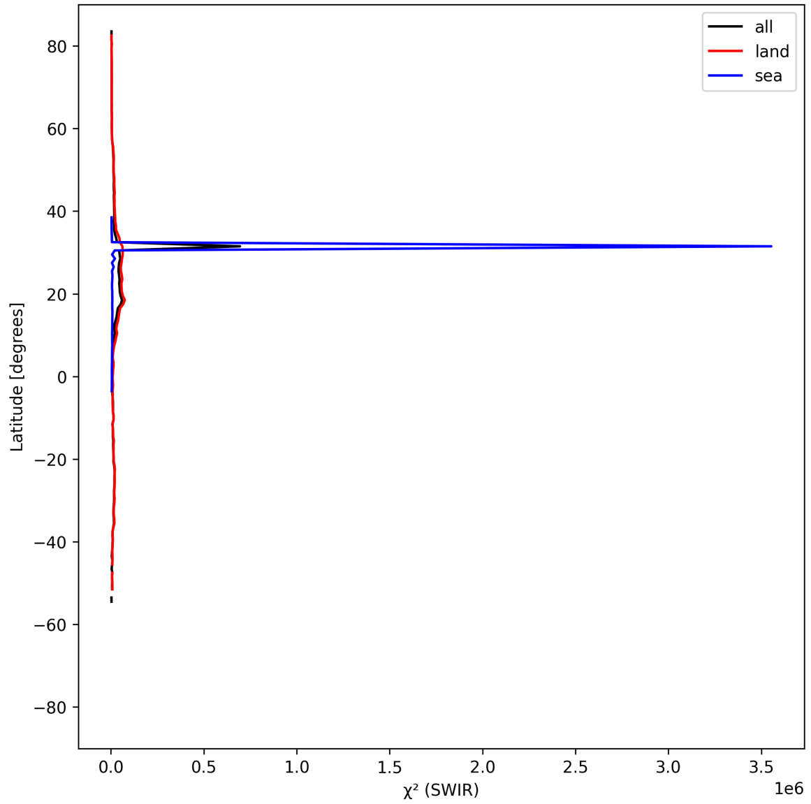
Figure 17: Zonal average of “ \chi^2 (SWIR)” for 2025-04-16 to 2025-04-18.
