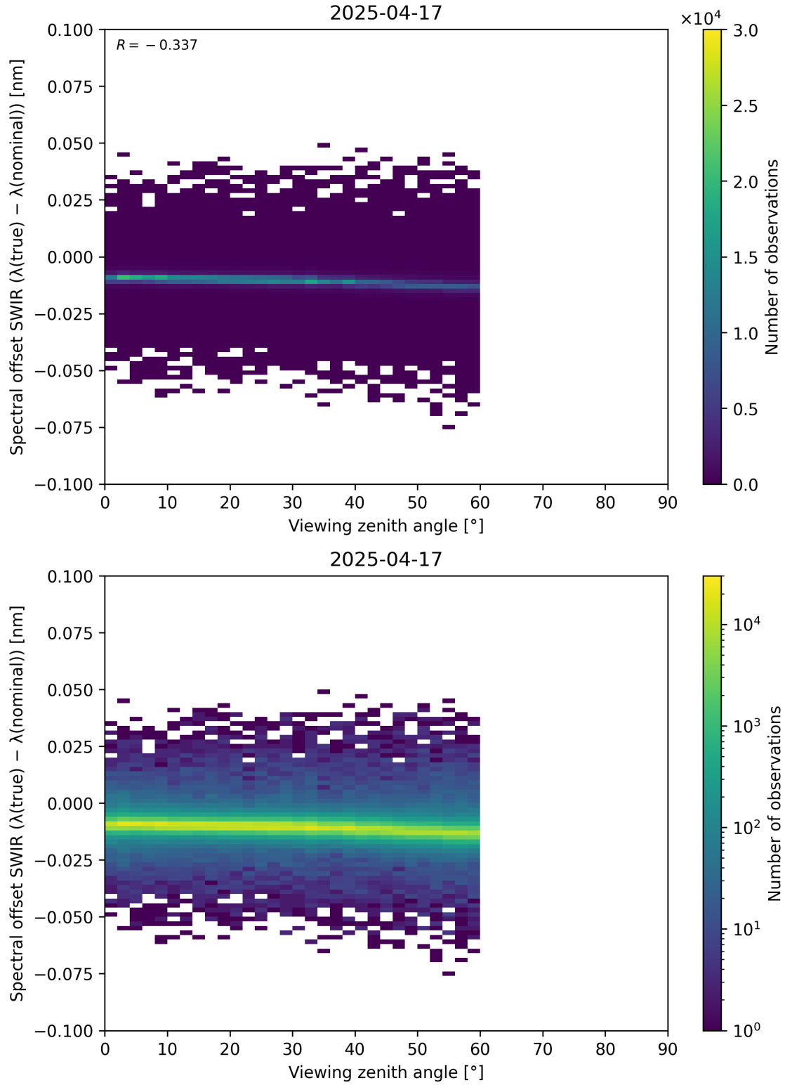
Figure 116: Scatter density plot of “Viewing zenith angle” against “Spectral offset SWIR ( \lambda_{\text{true}} - \lambda_{\text{nominal}} )” for 2025-04-16 to 2025-04-18.
