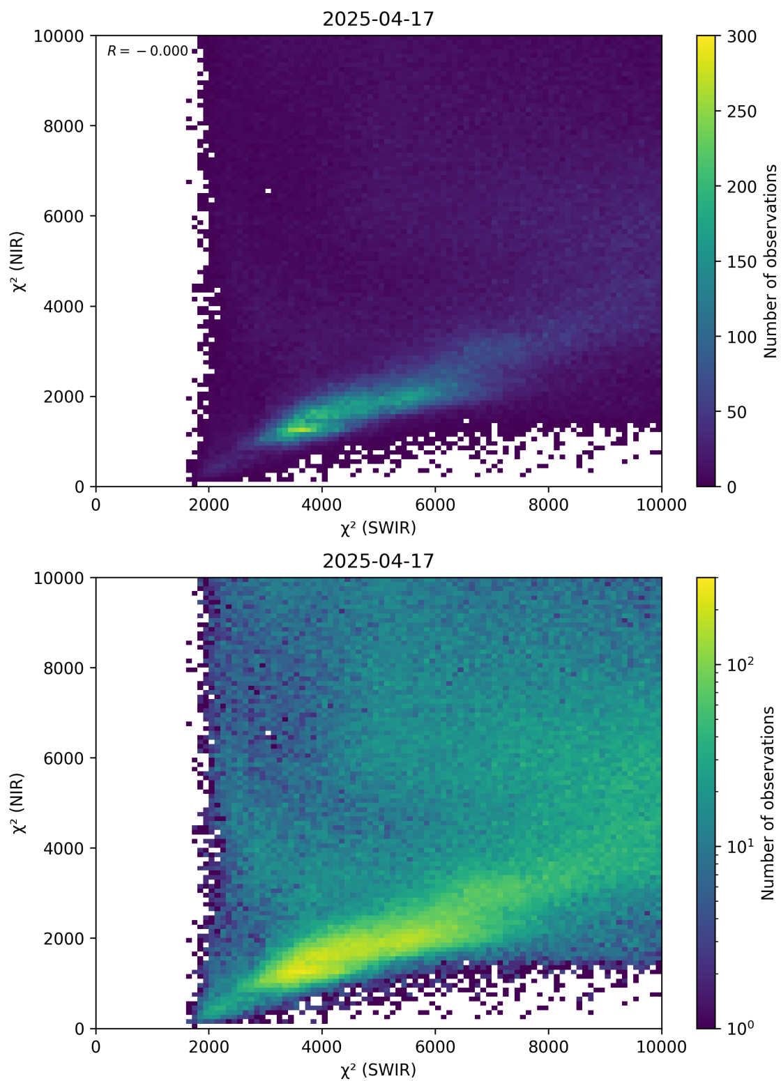
Figure 47: Scatter density plot of “ \chi^2 (SWIR)” against “ \chi^2 (NIR)” for 2025-04-16 to 2025-04-18.
