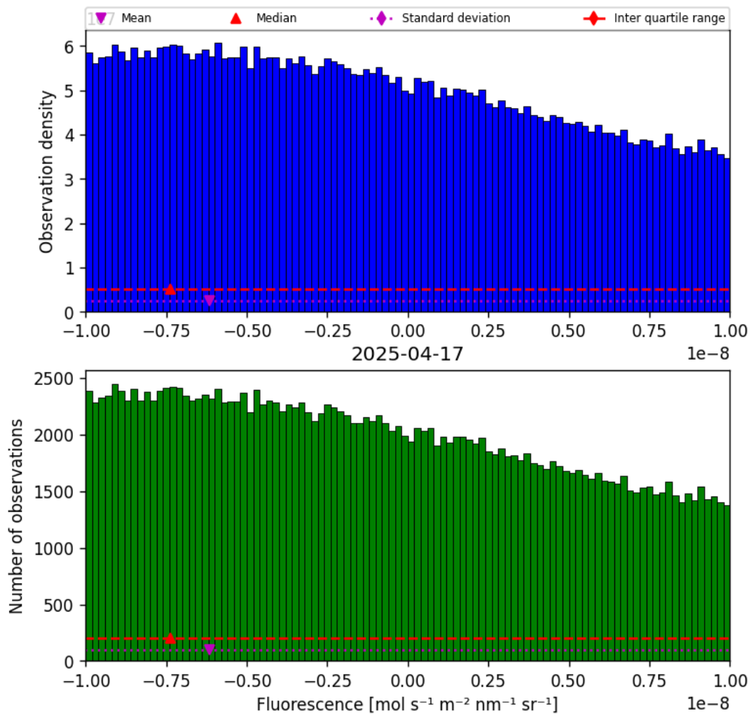
Figure 32: Histogram of “Fluorescence” for 2025-04-16 to 2025-04-18
