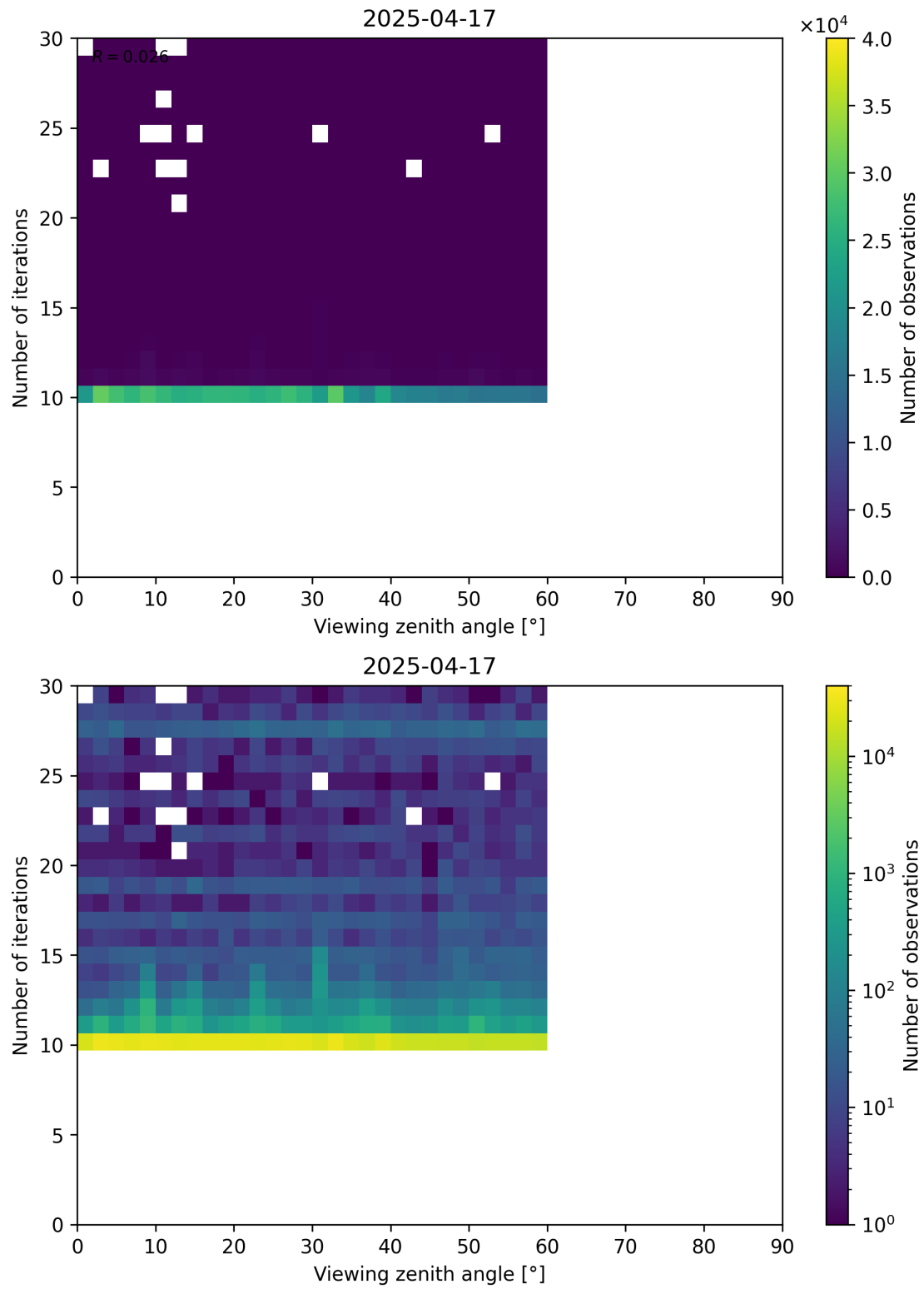
Figure 113: Scatter density plot of “Viewing zenith angle” against “Number of iterations” for 2025-04-16 to 2025-04-18.
