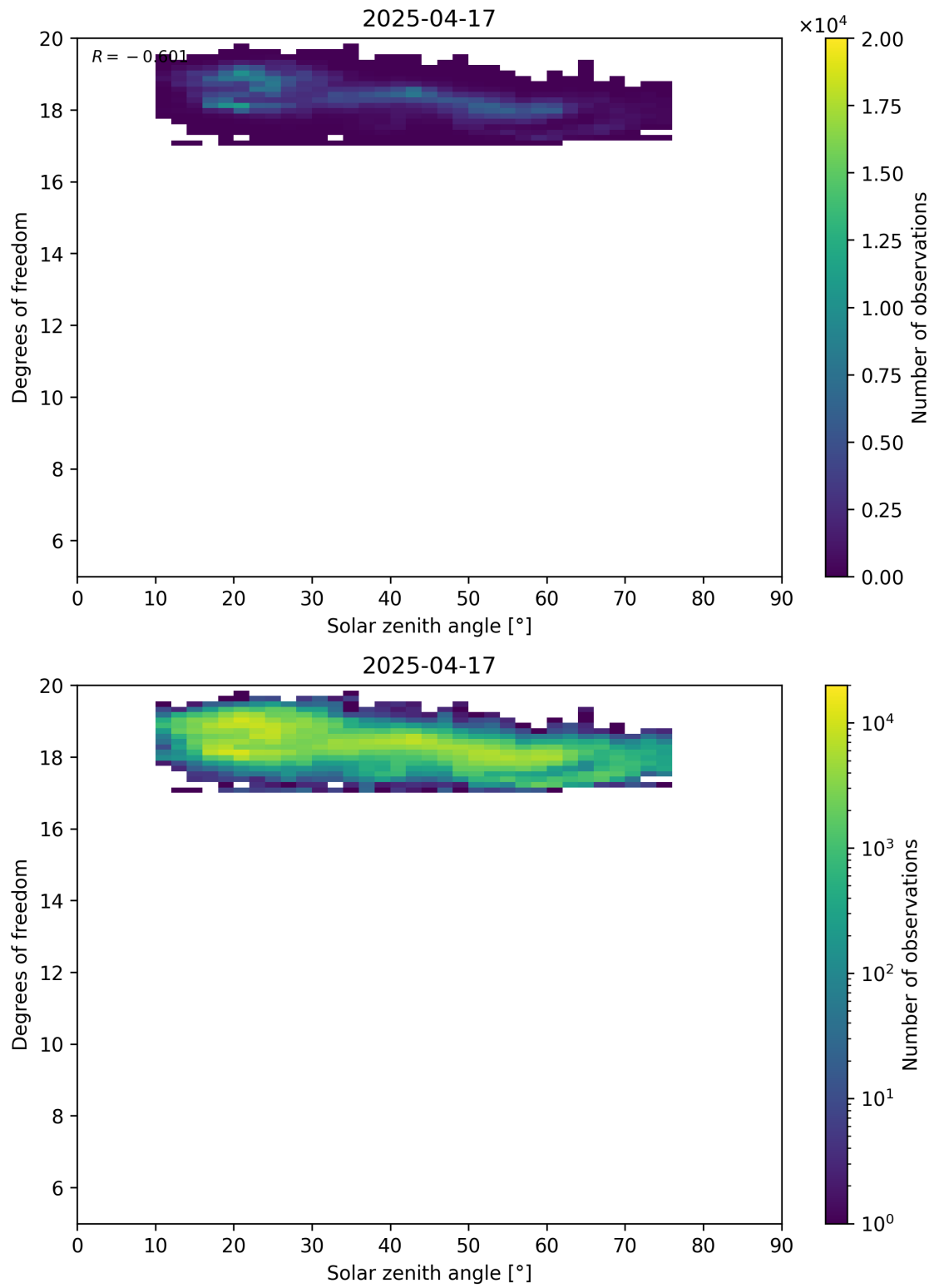
Figure 96: Scatter density plot of “Solar zenith angle” against “Degrees of freedom” for 2025-04-16 to 2025-04-18.
