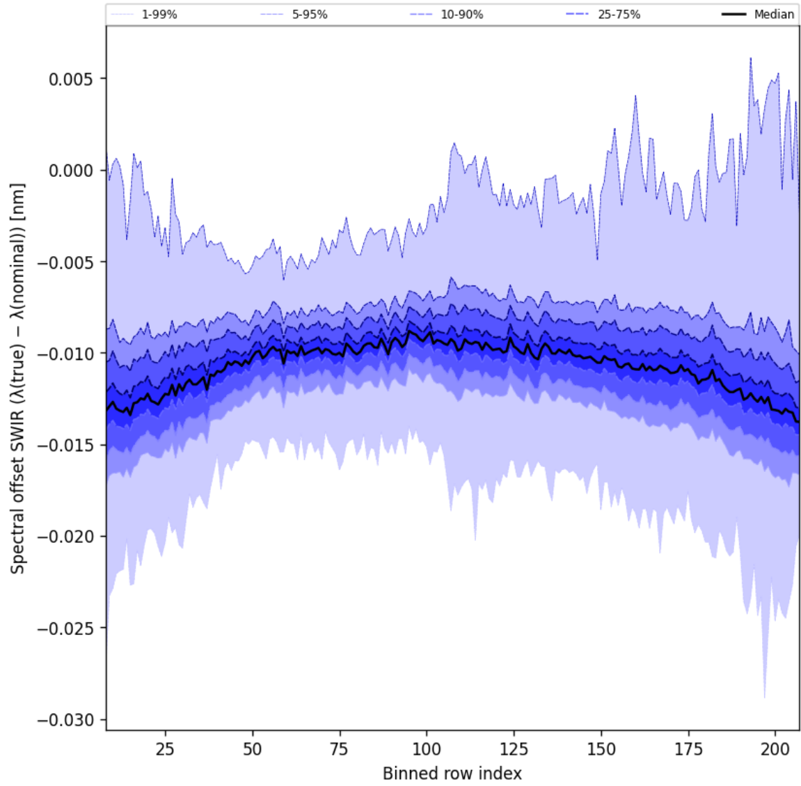
Figure 38: Along track statistics of “Spectral offset SWIR ( \lambda_{\text{true}} - \lambda_{\text{nominal}} )” for 2025-04-16 to 2025-04-18
