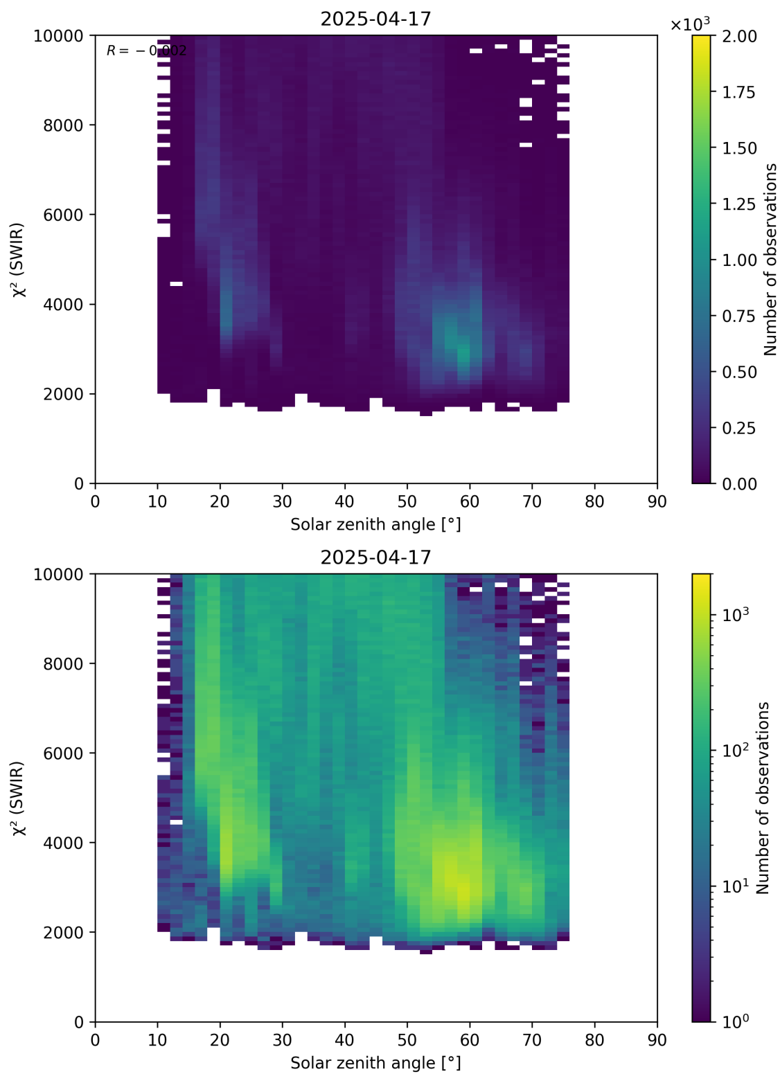
Figure 95: Scatter density plot of “Solar zenith angle” against “ \chi^2 (SWIR)” for 2025-04-16 to 2025-04-18.
