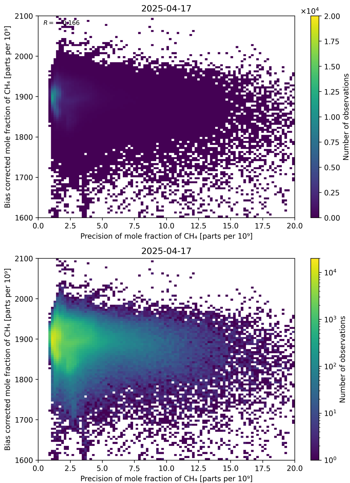
Figure 82: Scatter density plot of “Precision of mole fraction of CH 4 ” against “Bias corrected mole fraction of CH 4 ” for 2025-04-16 to 2025-04-18.
