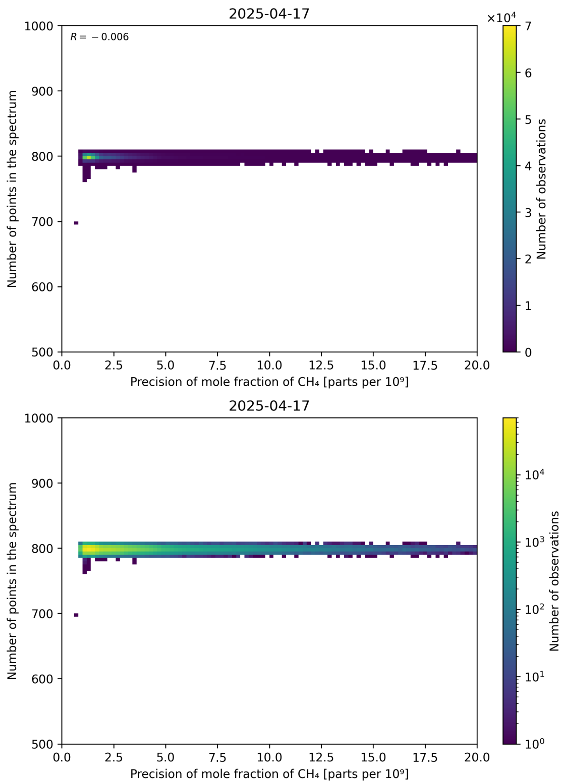
Figure 84: Scatter density plot of “Precision of mole fraction of CH 4 ” against “Number of points in the spectrum” for 2025-04-16 to 2025-04-18.
