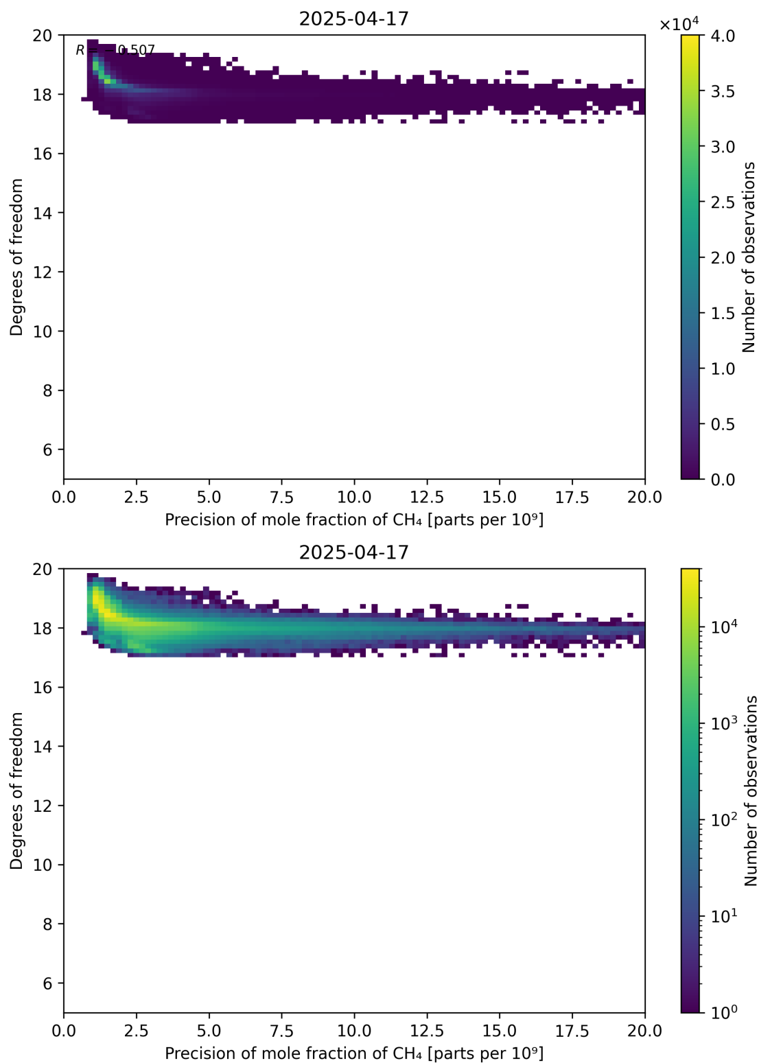
Figure 80: Scatter density plot of “Precision of mole fraction of CH 4 ” against “Degrees of freedom” for 2025-04-16 to 2025-04-18.
