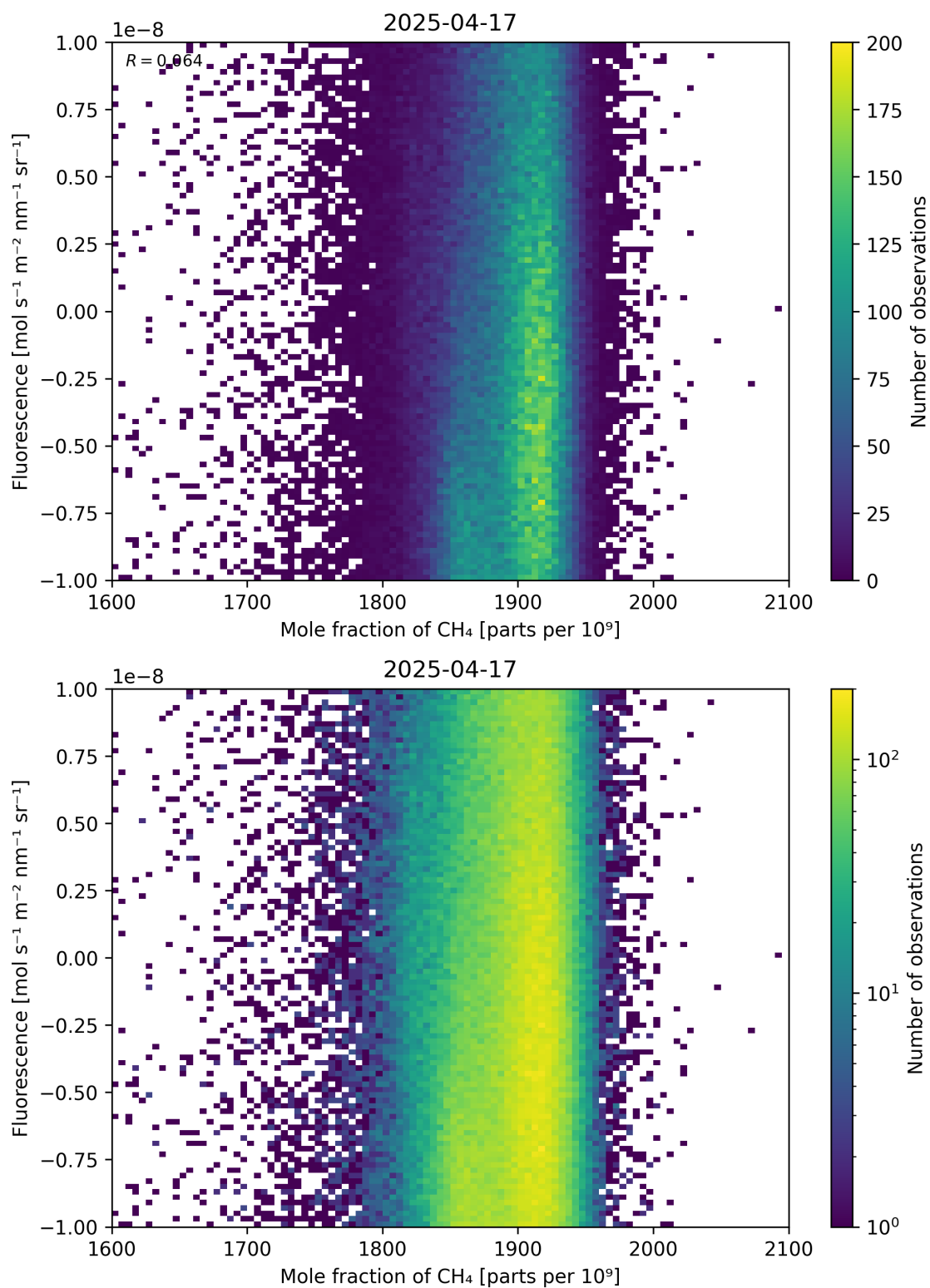
Figure 73: Scatter density plot of “Mole fraction of \text{CH}_4 ” against “Fluorescence” for 2025-04-16 to 2025-04-18.
