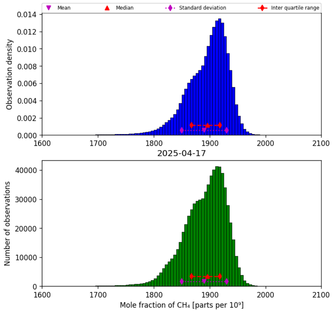
Figure 23: Histogram of “Mole fraction of CH 4 ” for 2025-04-16 to 2025-04-18
