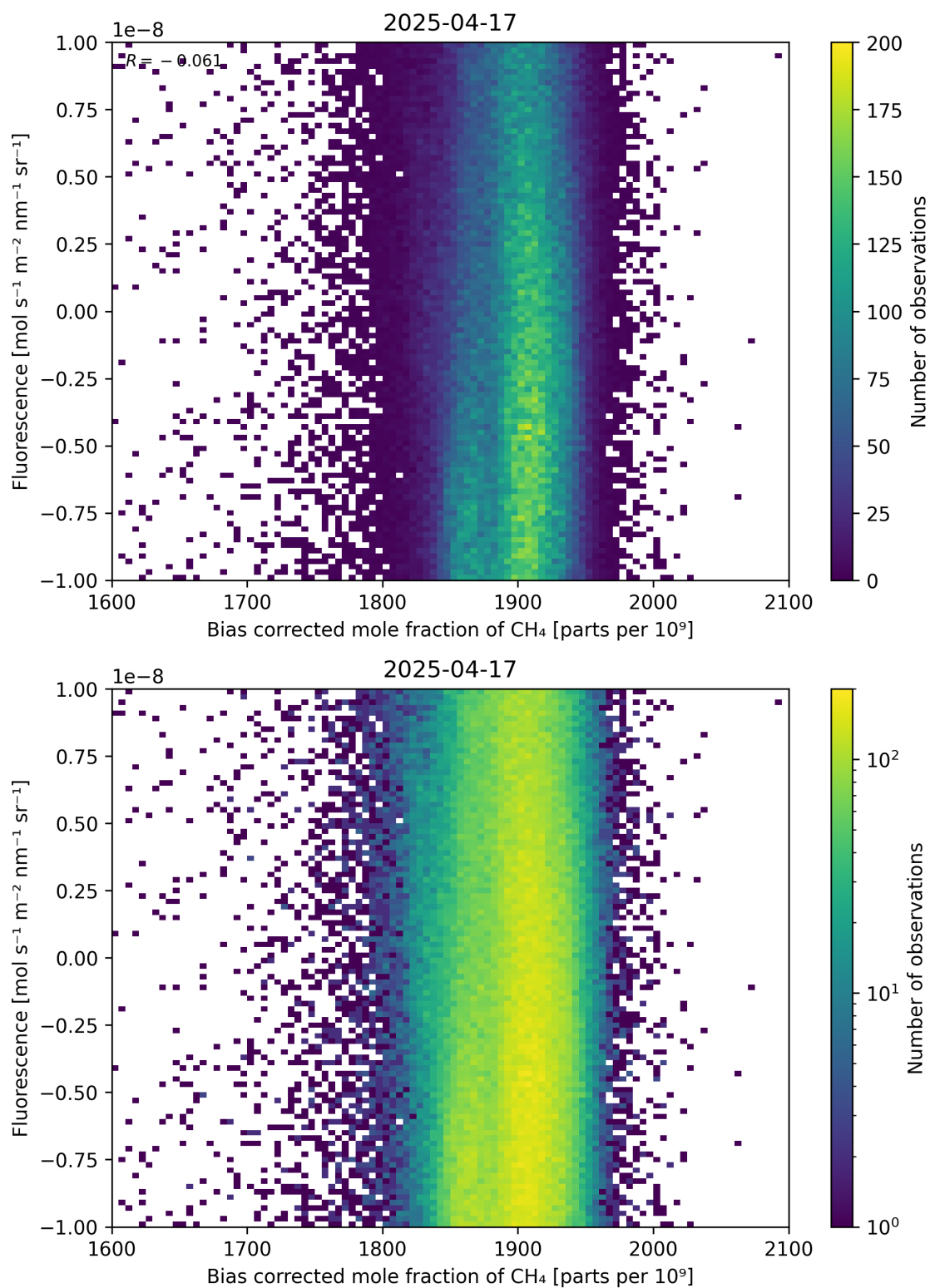
Figure 66: Scatter density plot of “Bias corrected mole fraction of \text{CH}_4 ” against “Fluorescence” for 2025-04-16 to 2025-04-18.
