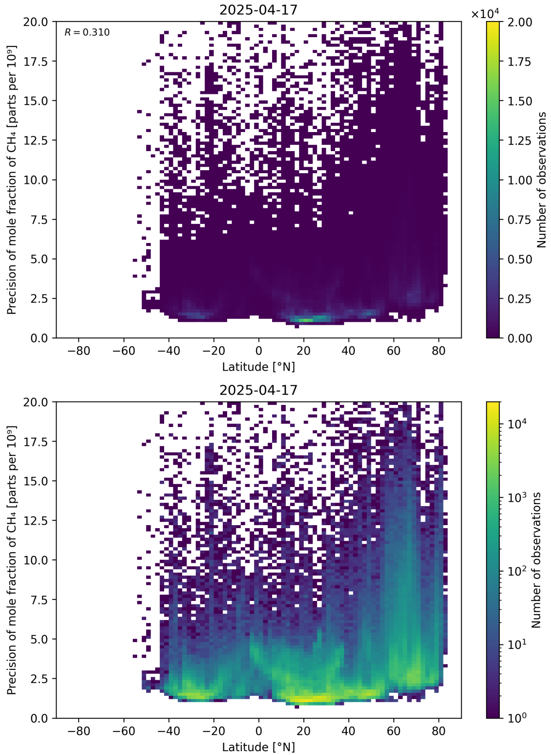
Figure 59: Scatter density plot of “Latitude” against “Precision of mole fraction of \text{CH}_4 ” for 2025-04-16 to 2025-04-18.
