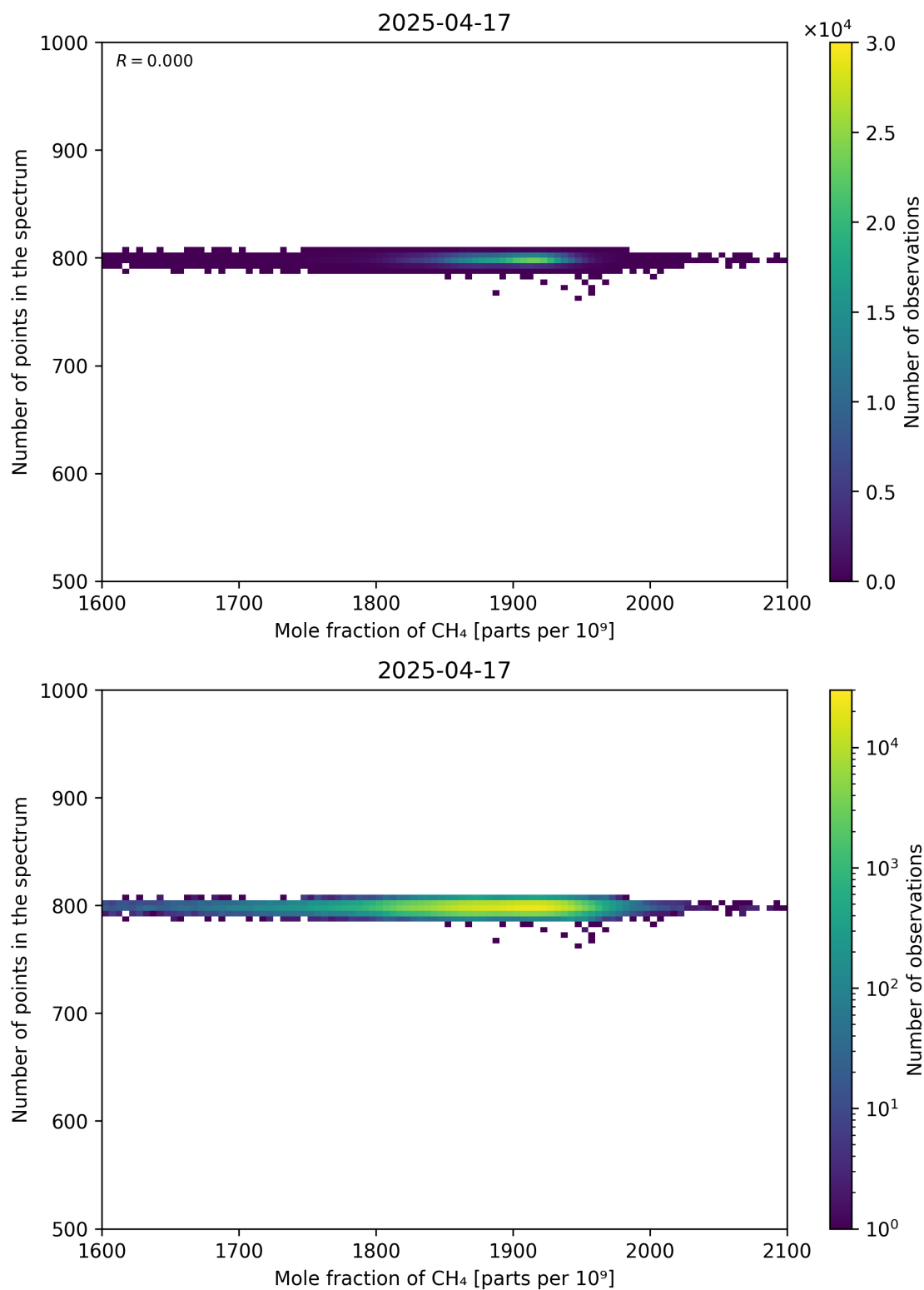
Figure 77: Scatter density plot of “Mole fraction of CH 4 ” against “Number of points in the spectrum” for 2025-04-16 to 2025-04-18.
