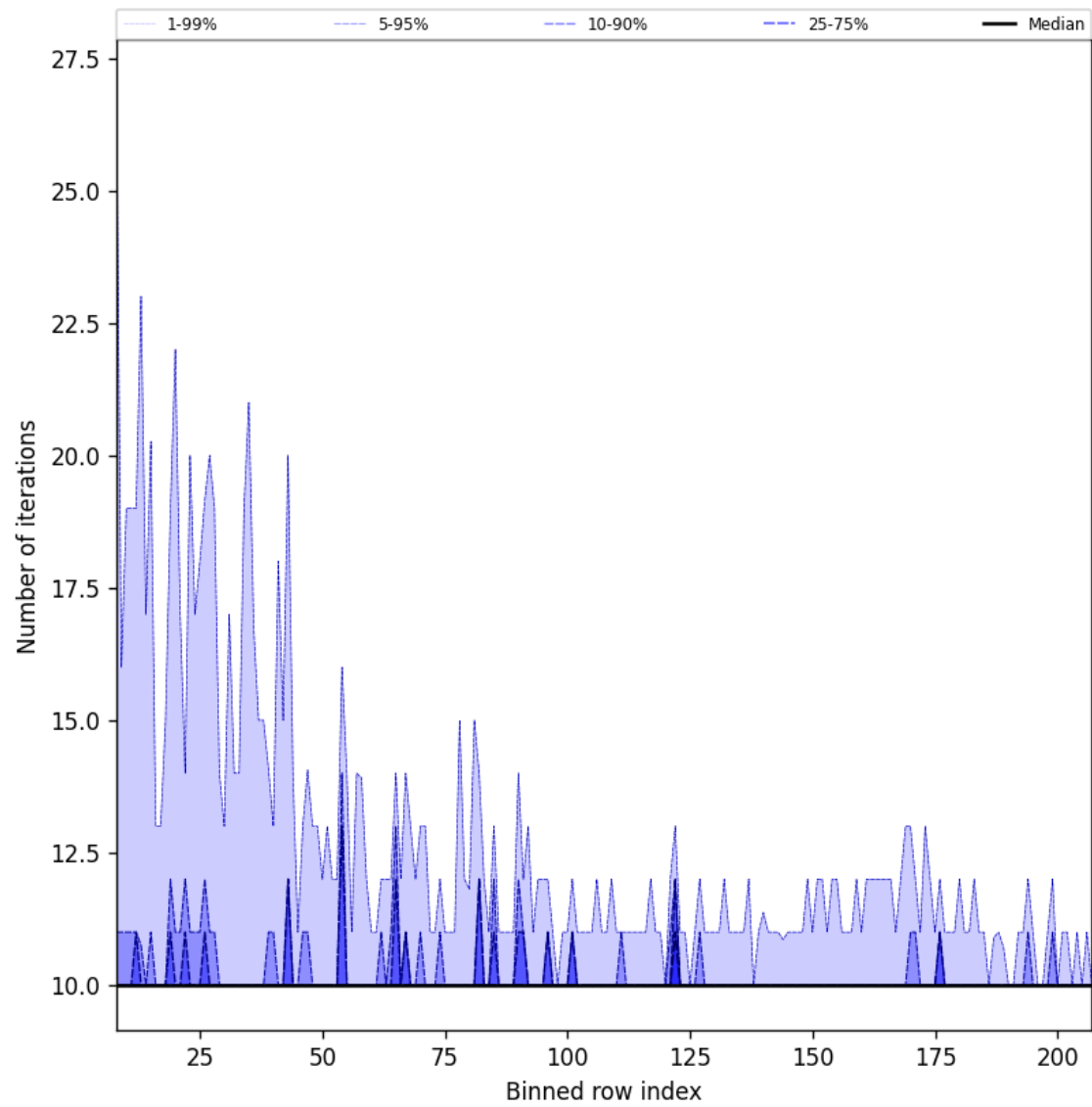
Figure 42: Along track statistics of “Number of iterations” for 2025-04-16 to 2025-04-18
