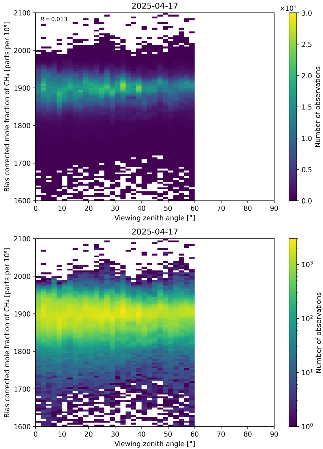
Figure 111: Scatter density plot of “Viewing zenith angle” against “Bias corrected mole fraction of CH 4 ” for 2025-04-16 to 2025-04-18.
