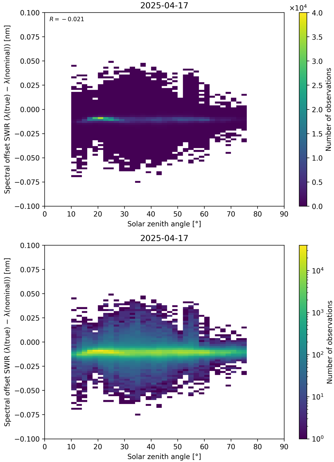
Figure 104: Scatter density plot of “Solar zenith angle” against “Spectral offset SWIR ( \lambda_{\text{true}} - \lambda_{\text{nominal}} )” for 2025-04-16 to 2025-04-18.
