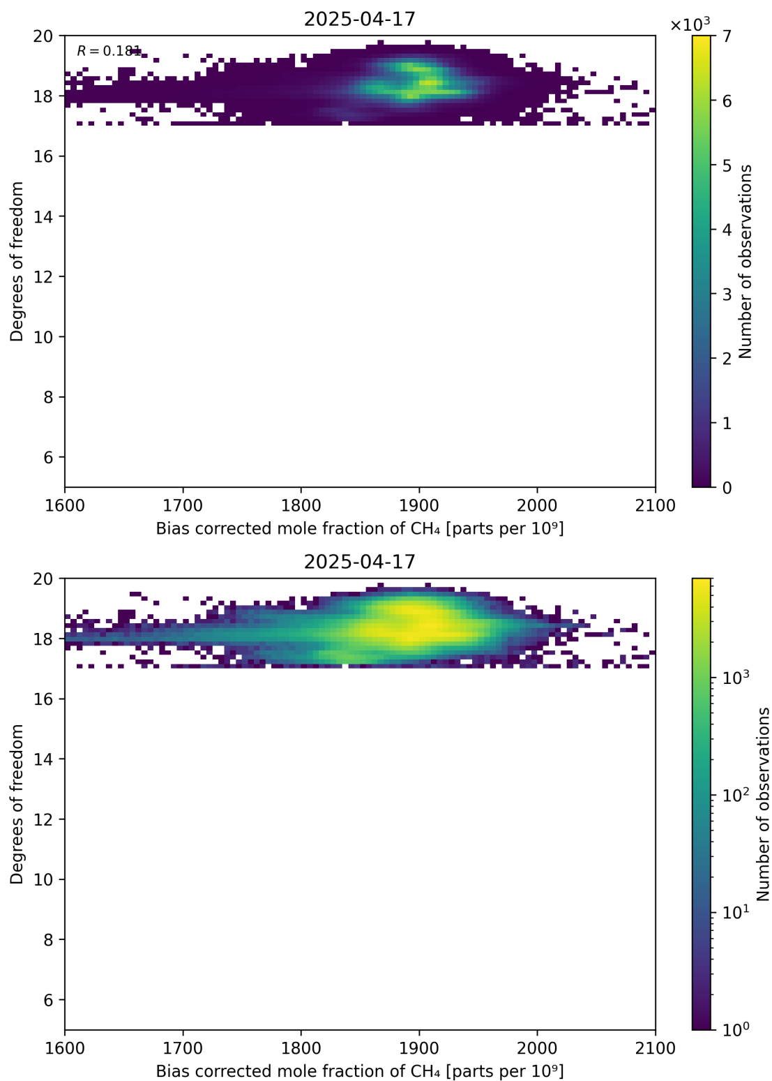
Figure 65: Scatter density plot of “Bias corrected mole fraction of CH 4 ” against “Degrees of freedom” for 2025-04-16 to 2025-04-18.
