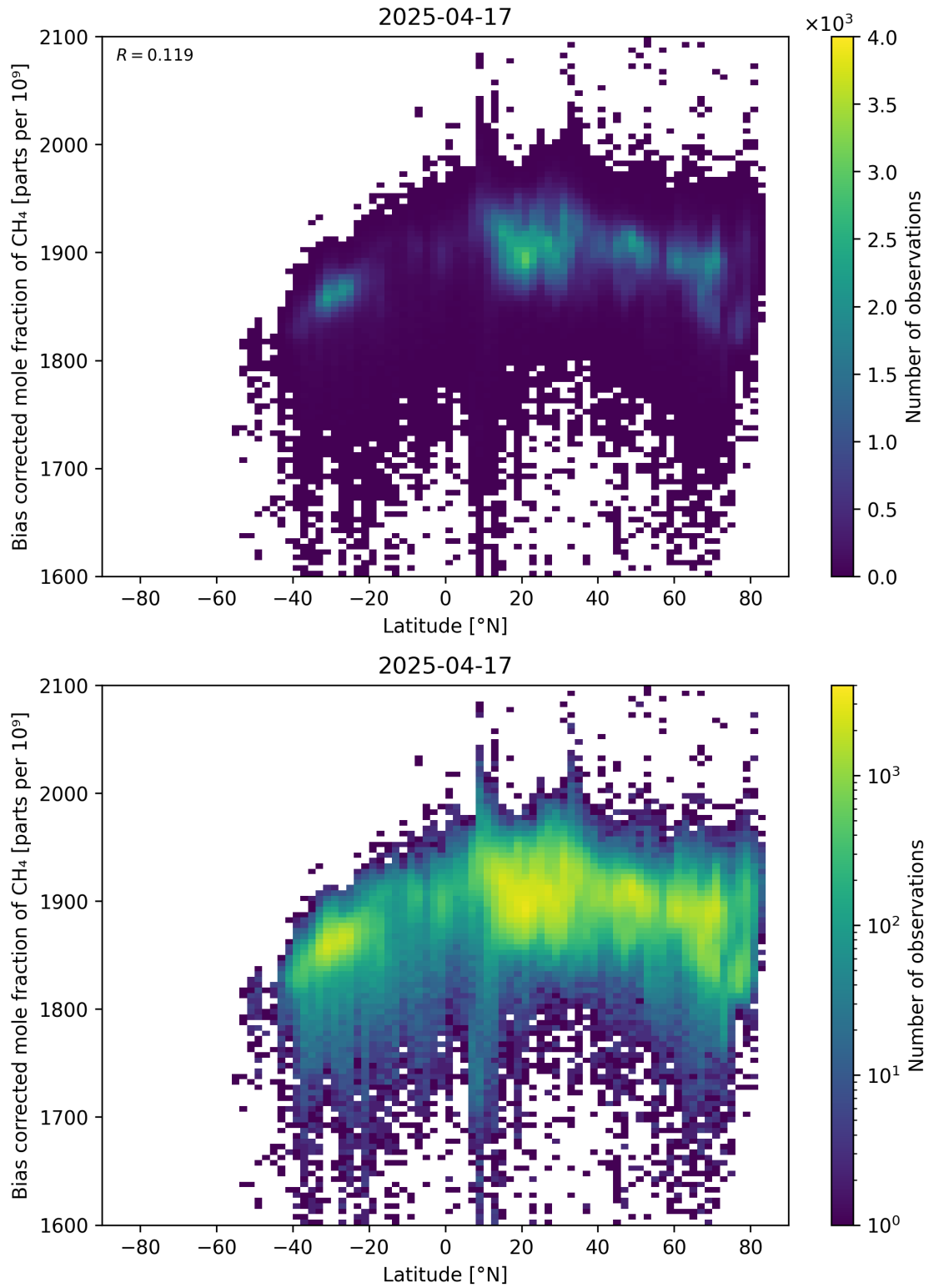
Figure 58: Scatter density plot of “Latitude” against “Bias corrected mole fraction of \text{CH}_4 ” for 2025-04-16 to 2025-04-18.
