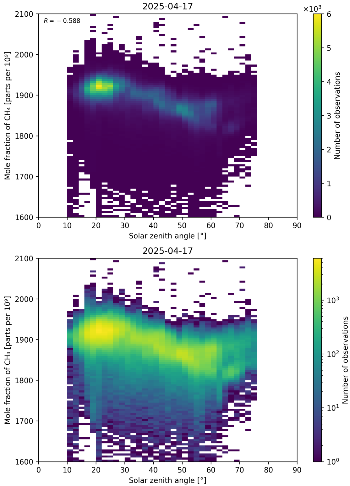
Figure 99: Scatter density plot of “Solar zenith angle” against “Mole fraction of \text{CH}_4 ” for 2025-04-16 to 2025-04-18.
