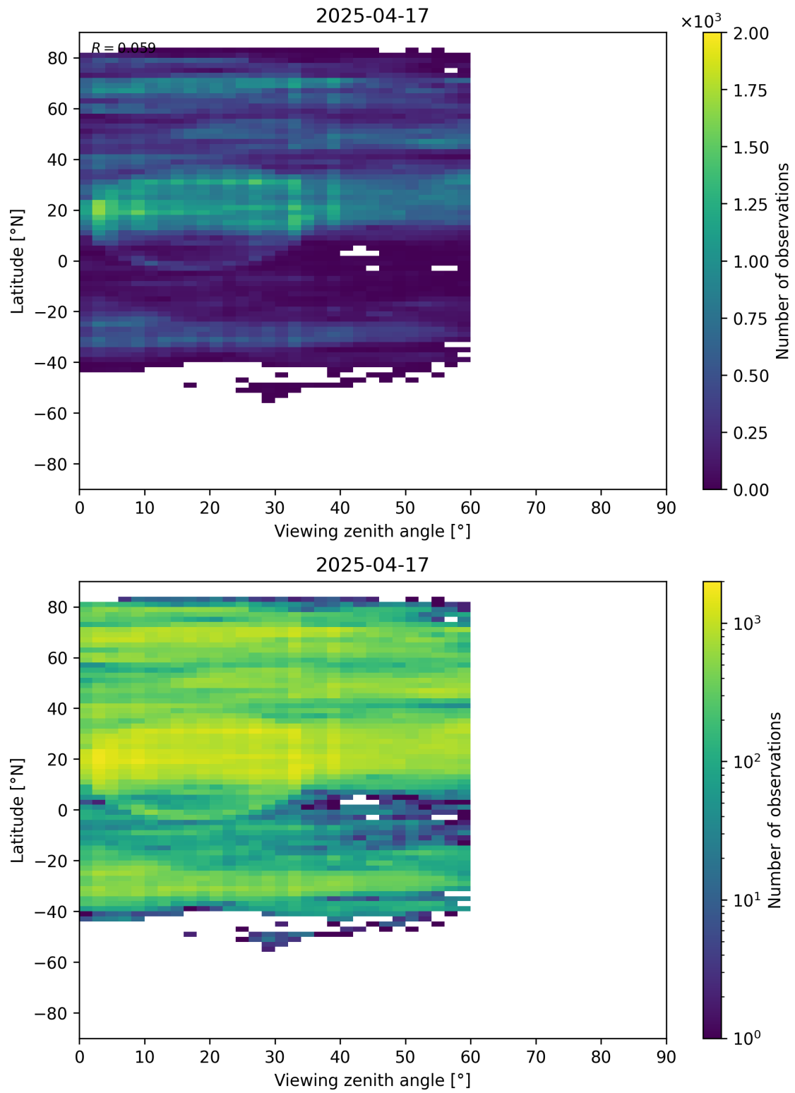
Figure 109: Scatter density plot of “Viewing zenith angle” against “Latitude” for 2025-04-16 to 2025-04-18.
