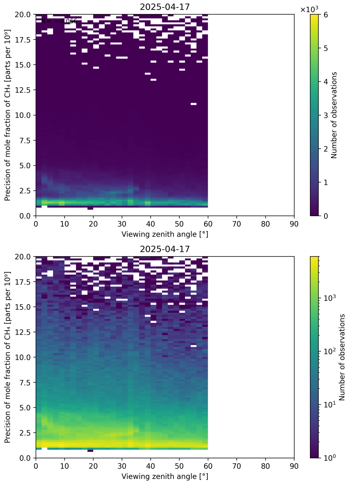
Figure 112: Scatter density plot of “Viewing zenith angle” against “Precision of mole fraction of CH 4 ” for 2025-04-16 to 2025-04-18.
