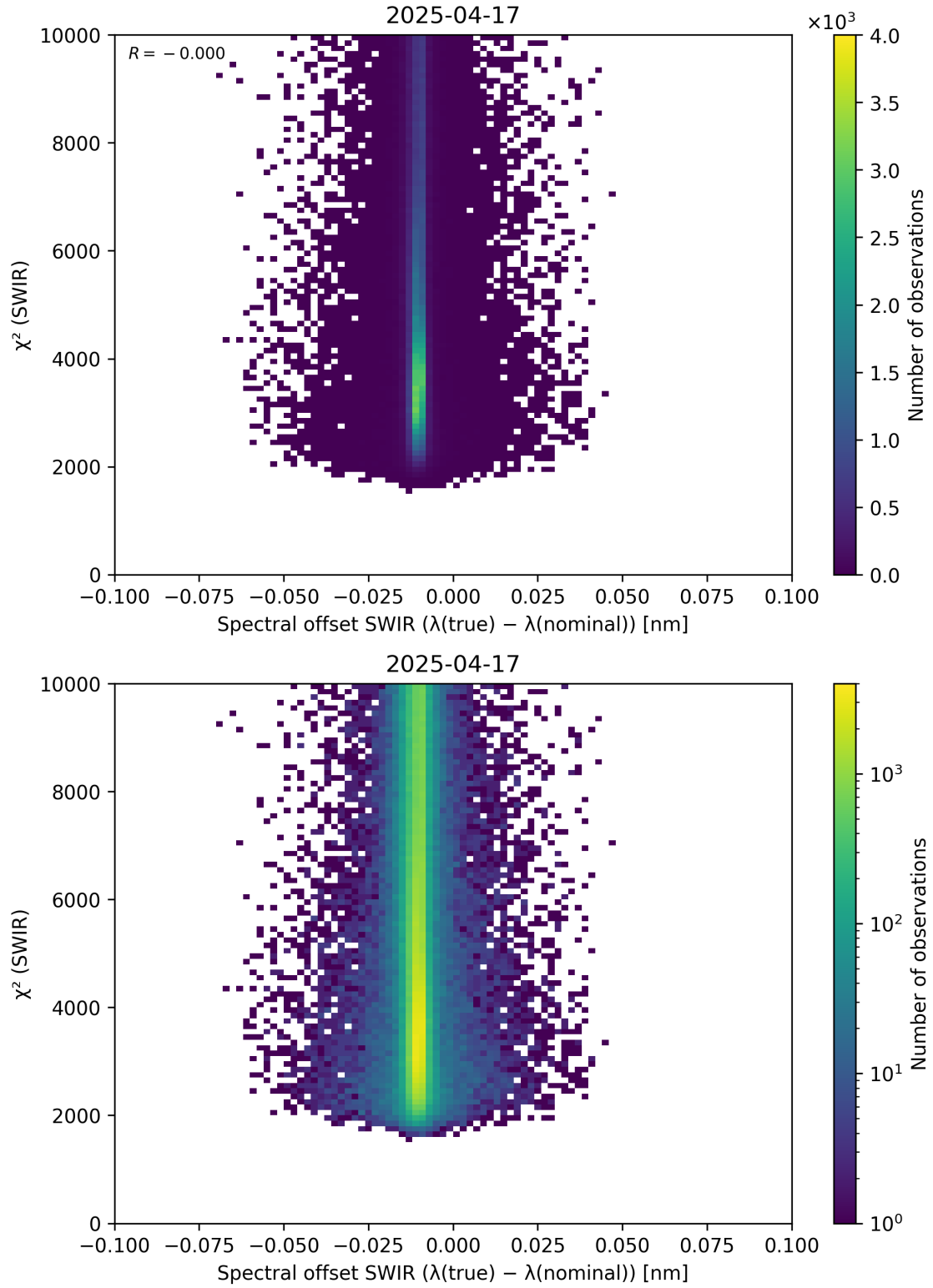
Figure 118: Scatter density plot of “Spectral offset SWIR ( \lambda_{\text{true}} - \lambda_{\text{nominal}} )” against “ \chi^2 (SWIR)” for 2025-04-16 to 2025-04-18.
