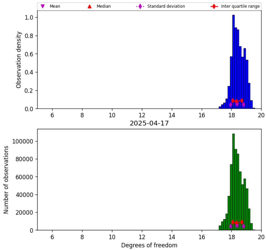
Figure 30: Histogram of “Degrees of freedom” for 2025-04-16 to 2025-04-18
