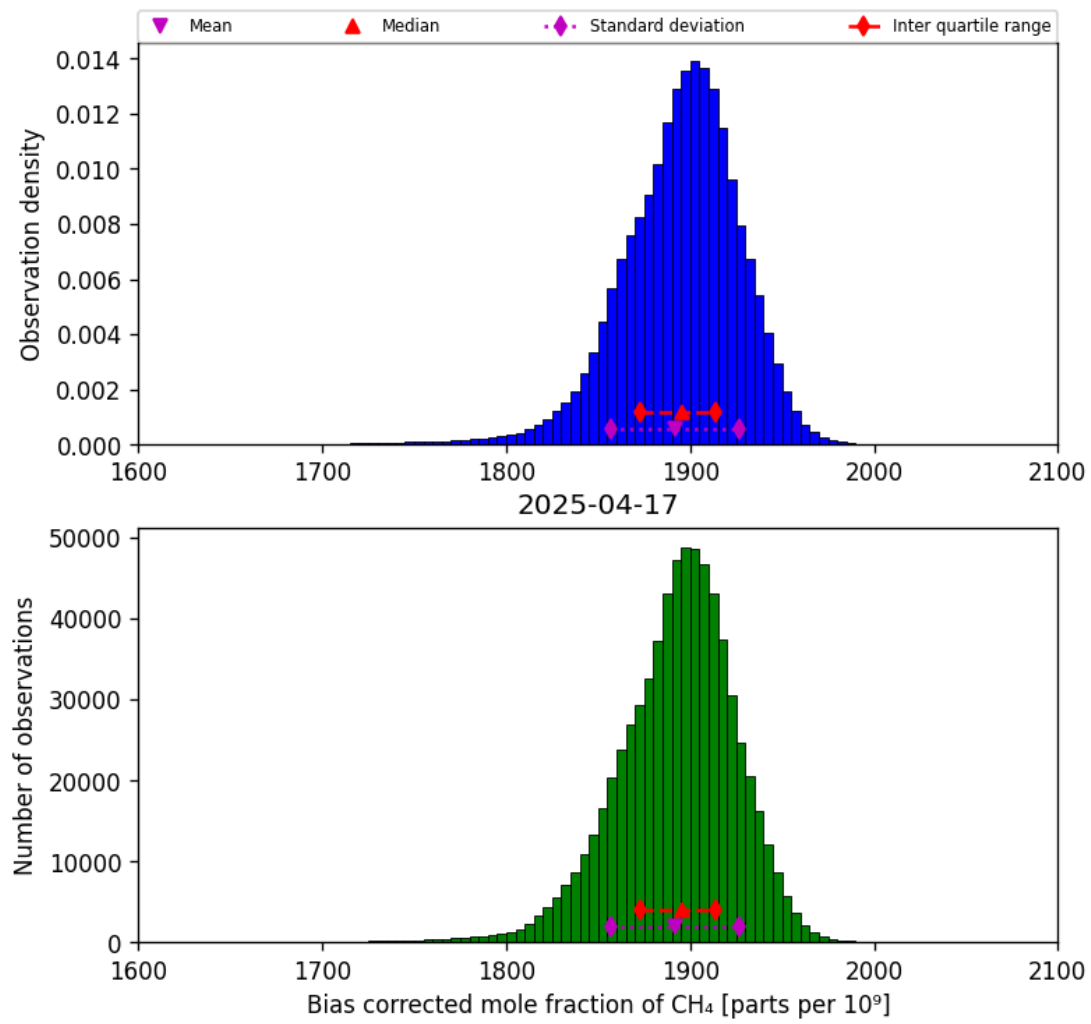
Figure 25: Histogram of “Bias corrected mole fraction of CH 4 ” for 2025-04-16 to 2025-04-18
