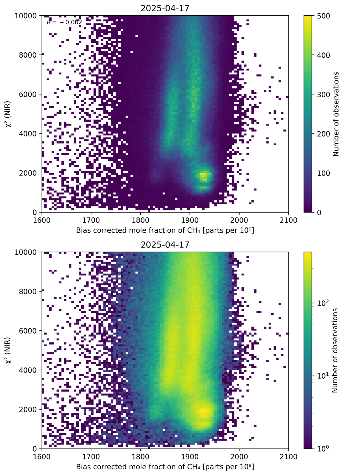
Figure 63: Scatter density plot of “Bias corrected mole fraction of CH 4 ” against “ \chi^2 (NIR)” for 2025-04-16 to 2025-04-18.
