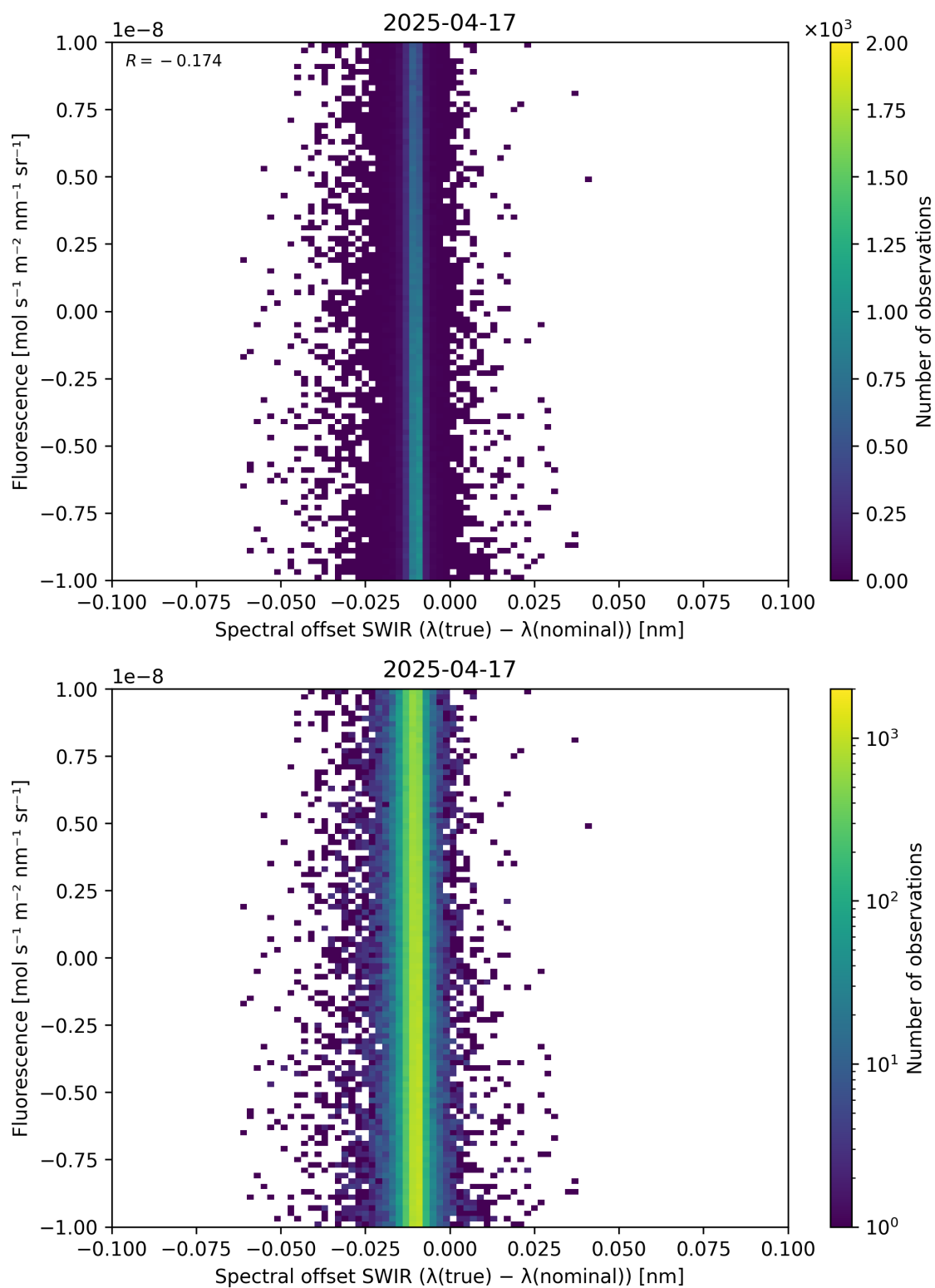
Figure 120: Scatter density plot of “Spectral offset SWIR ( \lambda_{\text{true}} - \lambda_{\text{nominal}} )” against “Fluorescence” for 2025-04-16 to 2025-04-18.
