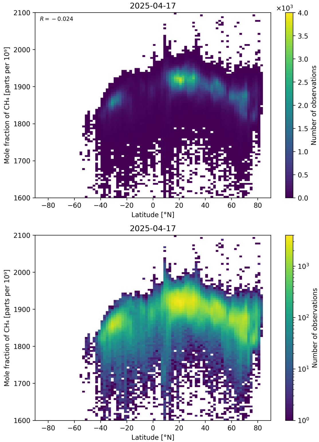
Figure 57: Scatter density plot of “Latitude” against “Mole fraction of CH 4 ” for 2025-04-16 to 2025-04-18.
