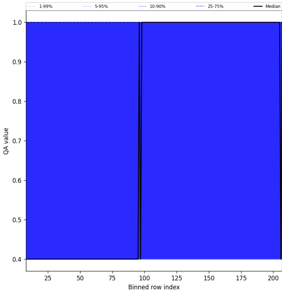
Figure 33: Along track statistics of “QA value” for 2025-04-16 to 2025-04-18
