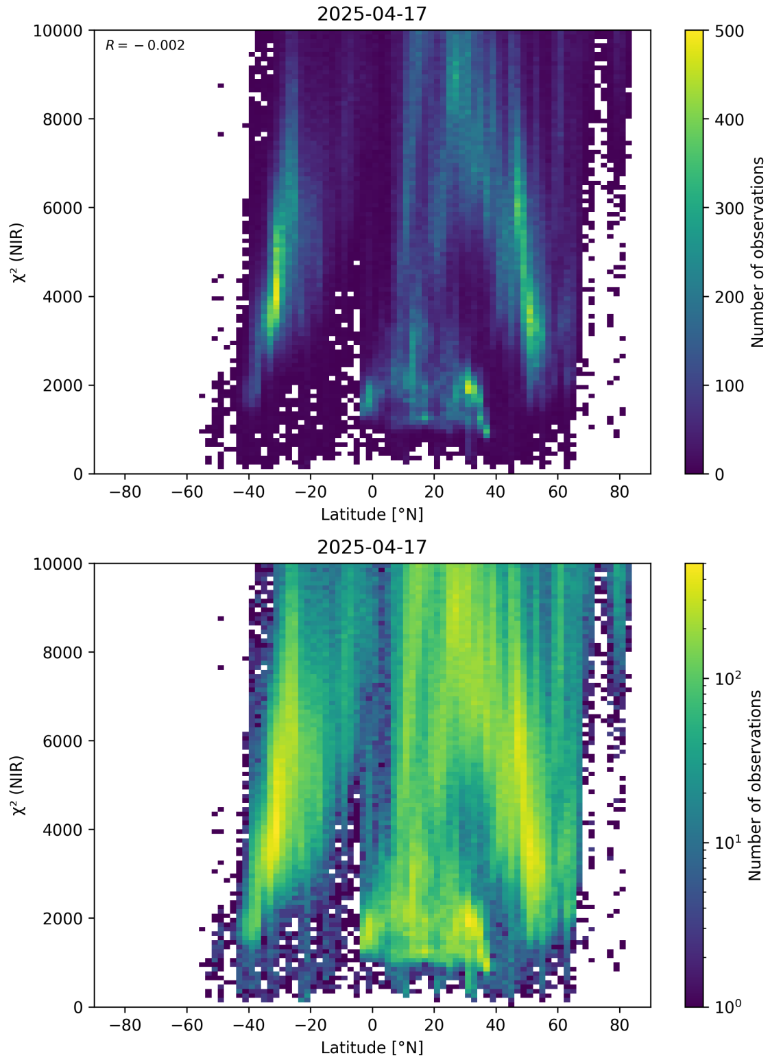
Figure 53: Scatter density plot of “Latitude” against “ \chi^2 (NIR)” for 2025-04-16 to 2025-04-18.
