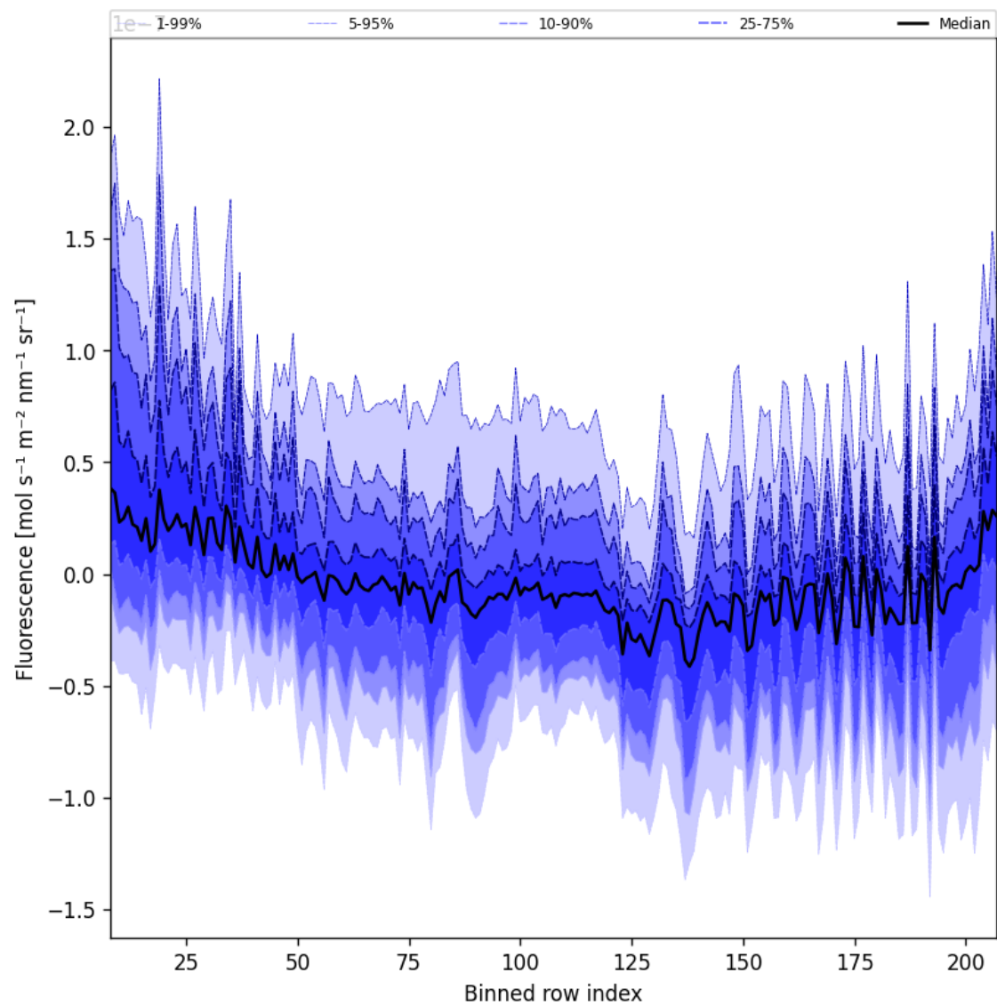
Figure 43: Along track statistics of “Fluorescence” for 2025-04-16 to 2025-04-18
