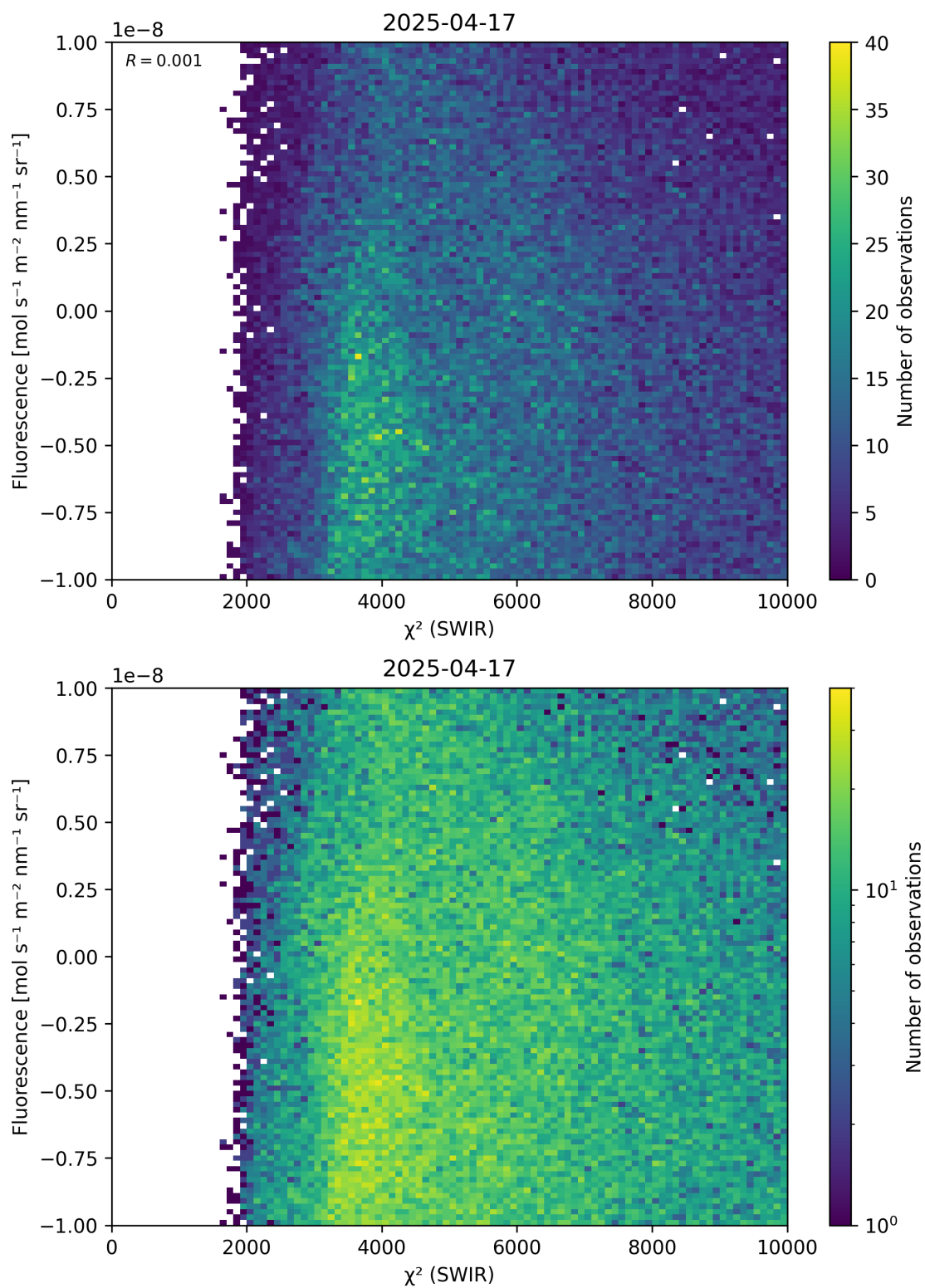
Figure 49: Scatter density plot of “ \chi^2 (SWIR)” against “Fluorescence” for 2025-04-16 to 2025-04-18.
