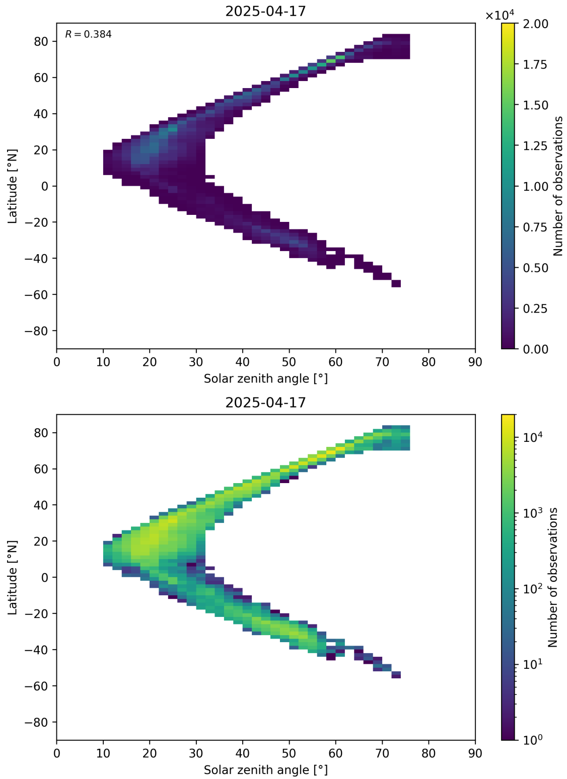
Figure 98: Scatter density plot of “Solar zenith angle” against “Latitude” for 2025-04-16 to 2025-04-18.
