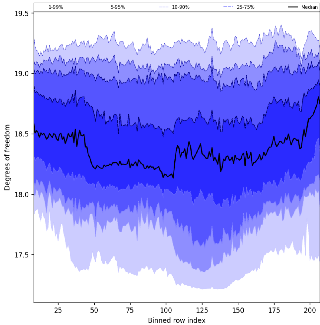
Figure 41: Along track statistics of “Degrees of freedom” for 2025-04-16 to 2025-04-18
