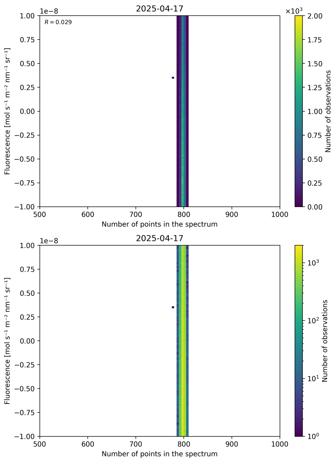
Figure 91: Scatter density plot of “Number of points in the spectrum” against “Fluorescence” for 2025-04-16 to 2025-04-18.
