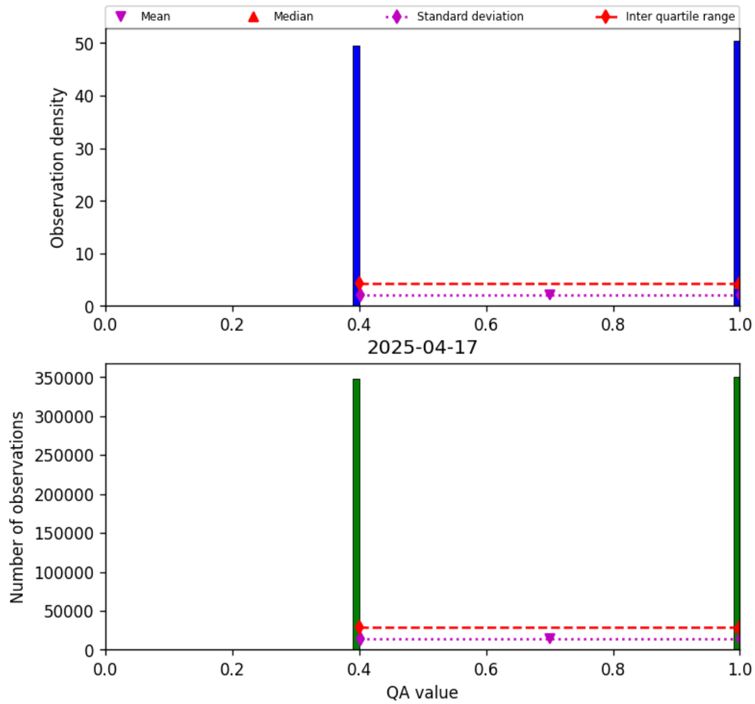
Figure 22: Histogram of “QA value” for 2025-04-16 to 2025-04-18
