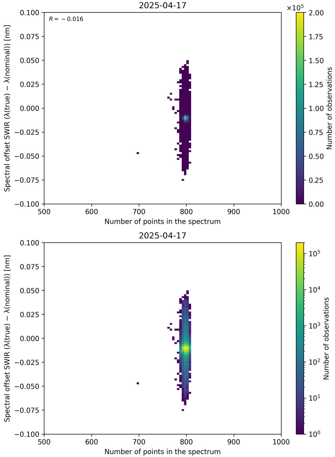
Figure 93: Scatter density plot of “Number of points in the spectrum” against “Spectral offset SWIR ( \lambda_{\text{true}} - \lambda_{\text{nominal}} )” for 2025-04-16 to 2025-04-18.
