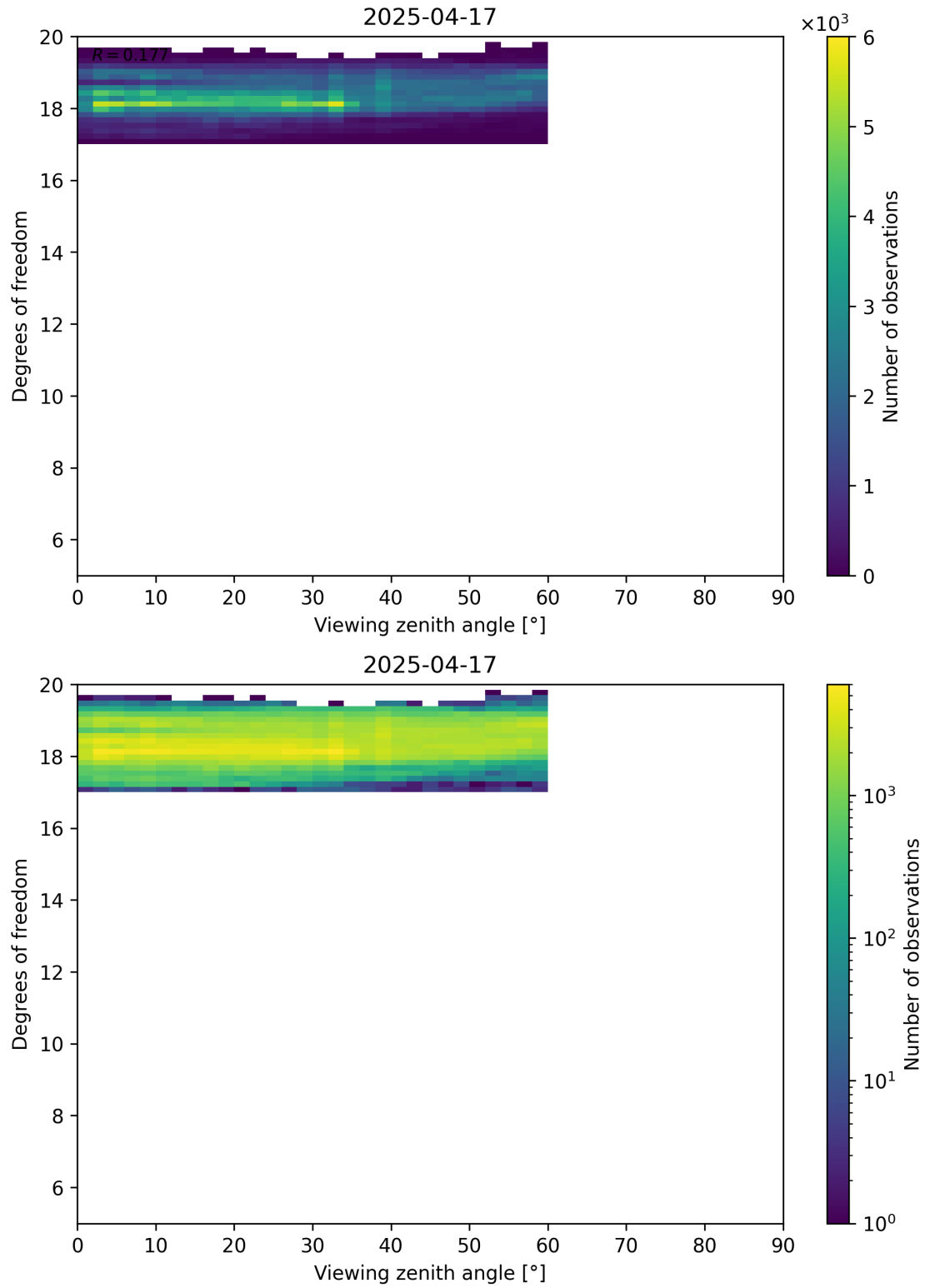
Figure 107: Scatter density plot of “Viewing zenith angle” against “Degrees of freedom” for 2025-04-16 to 2025-04-18.
