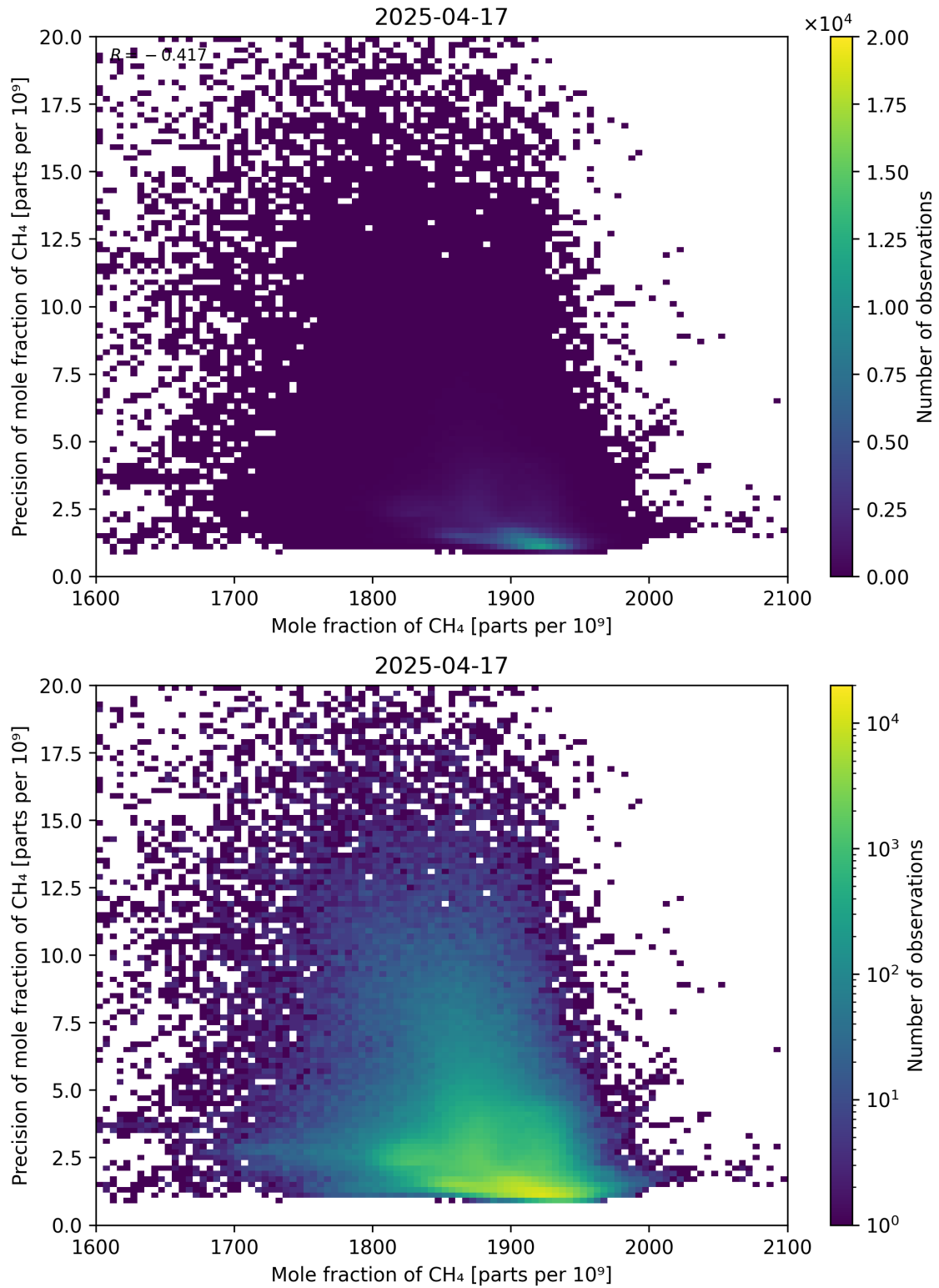
Figure 75: Scatter density plot of “Mole fraction of CH 4 ” against “Precision of mole fraction of CH 4 ” for 2025-04-16 to 2025-04-18.
