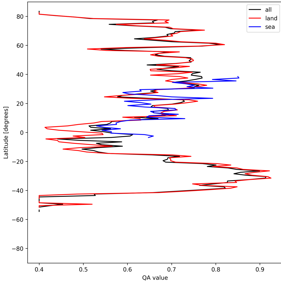
Figure 11: Zonal average of “QA value” for 2025-04-16 to 2025-04-18.
