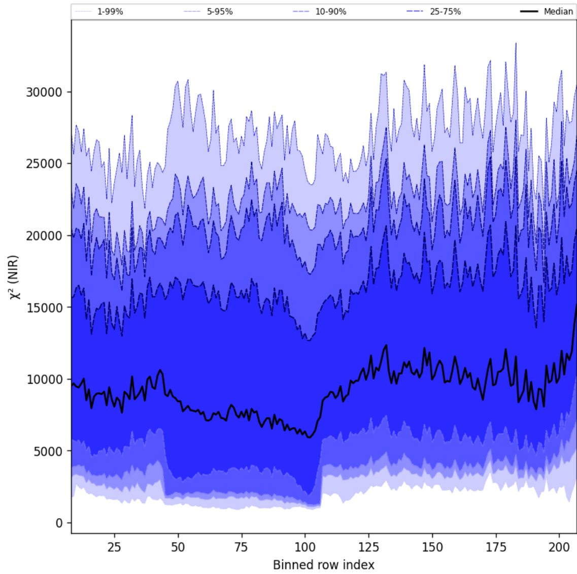
Figure 40: Along track statistics of “ \chi^2 (NIR)” for 2025-04-16 to 2025-04-18
