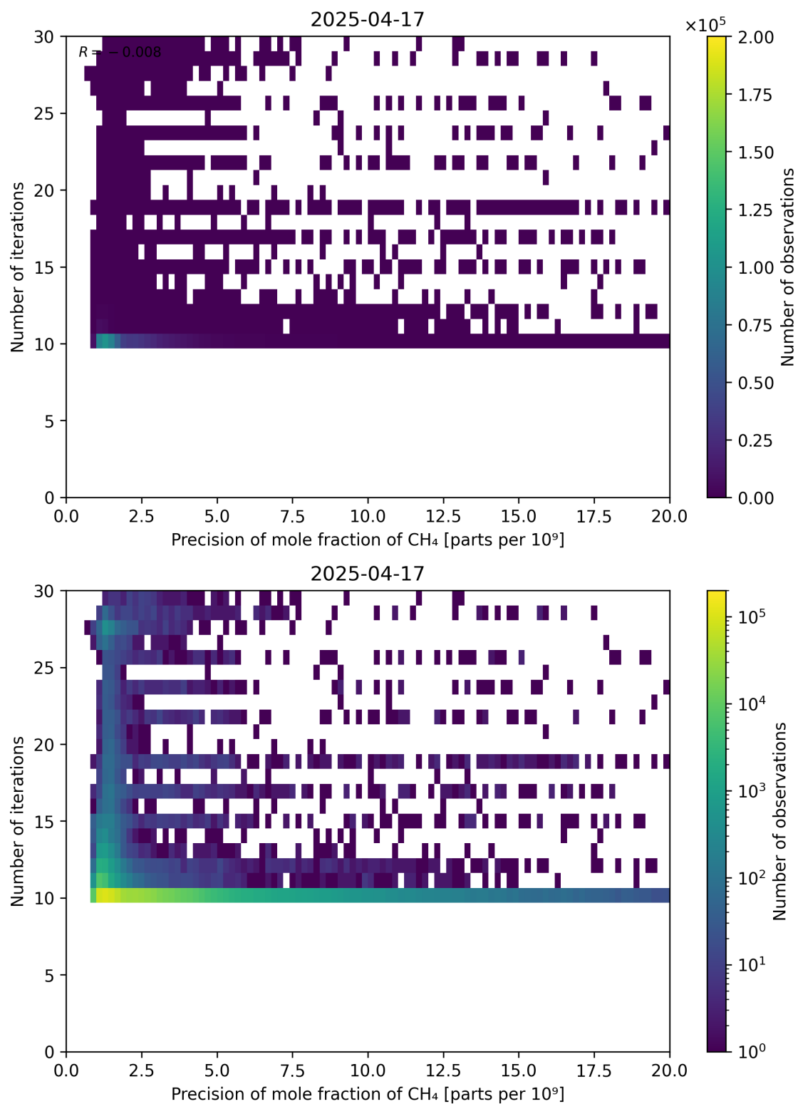
Figure 83: Scatter density plot of “Precision of mole fraction of CH 4 ” against “Number of iterations” for 2025-04-16 to 2025-04-18.
