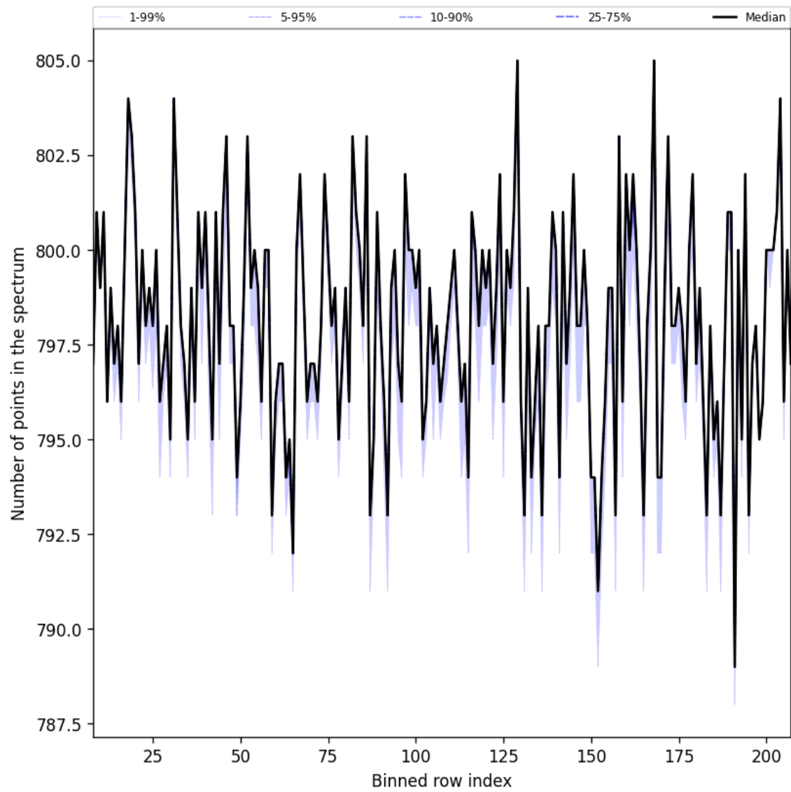
Figure 37: Along track statistics of “Number of points in the spectrum” for 2025-04-16 to 2025-04-18
