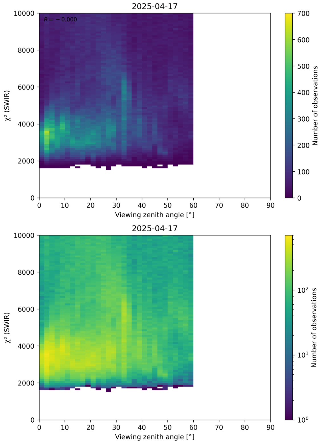
Figure 106: Scatter density plot of “Viewing zenith angle” against “ \chi^2 (SWIR)” for 2025-04-16 to 2025-04-18.
