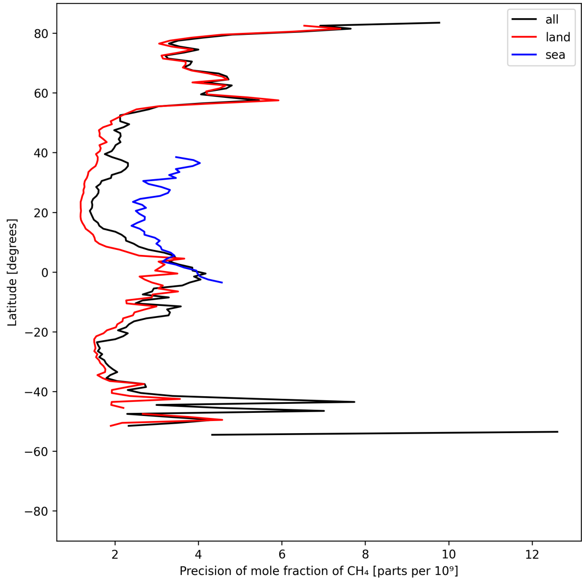
Figure 13: Zonal average of “Precision of mole fraction of CH 4 ” for 2025-04-16 to 2025-04-18.
