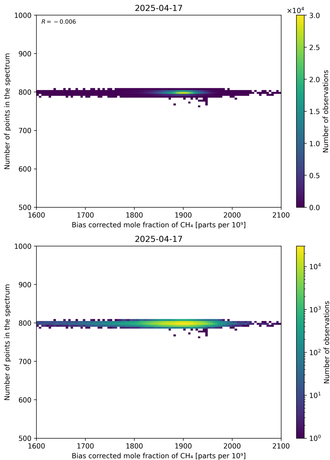
Figure 68: Scatter density plot of “Bias corrected mole fraction of CH 4 ” against “Number of points in the spectrum” for 2025-04-16 to 2025-04-18.
