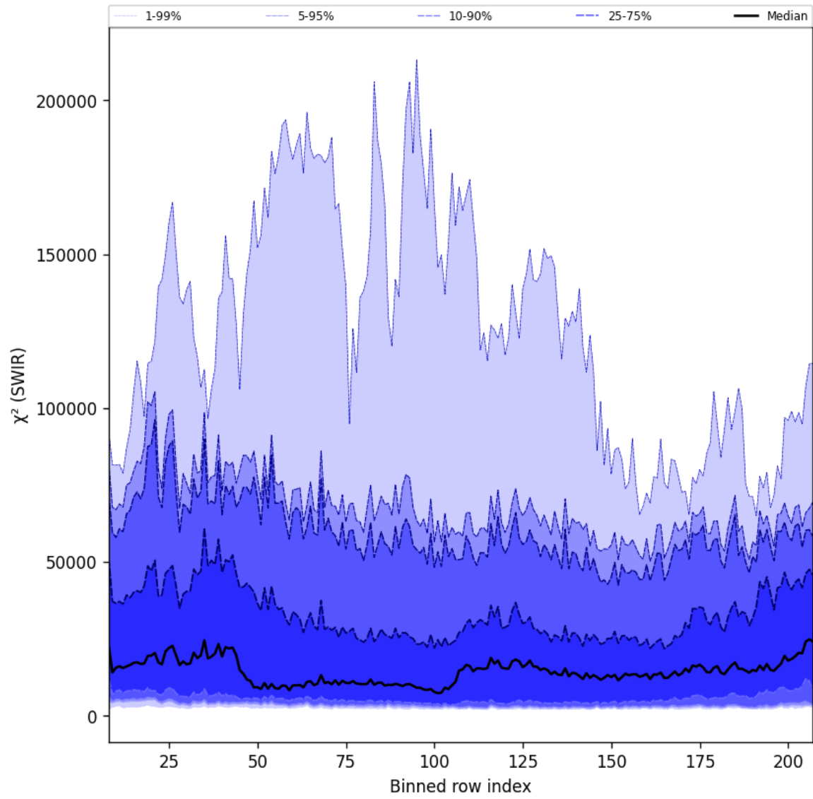
Figure 39: Along track statistics of “ \chi^2 (SWIR)” for 2025-04-16 to 2025-04-18
