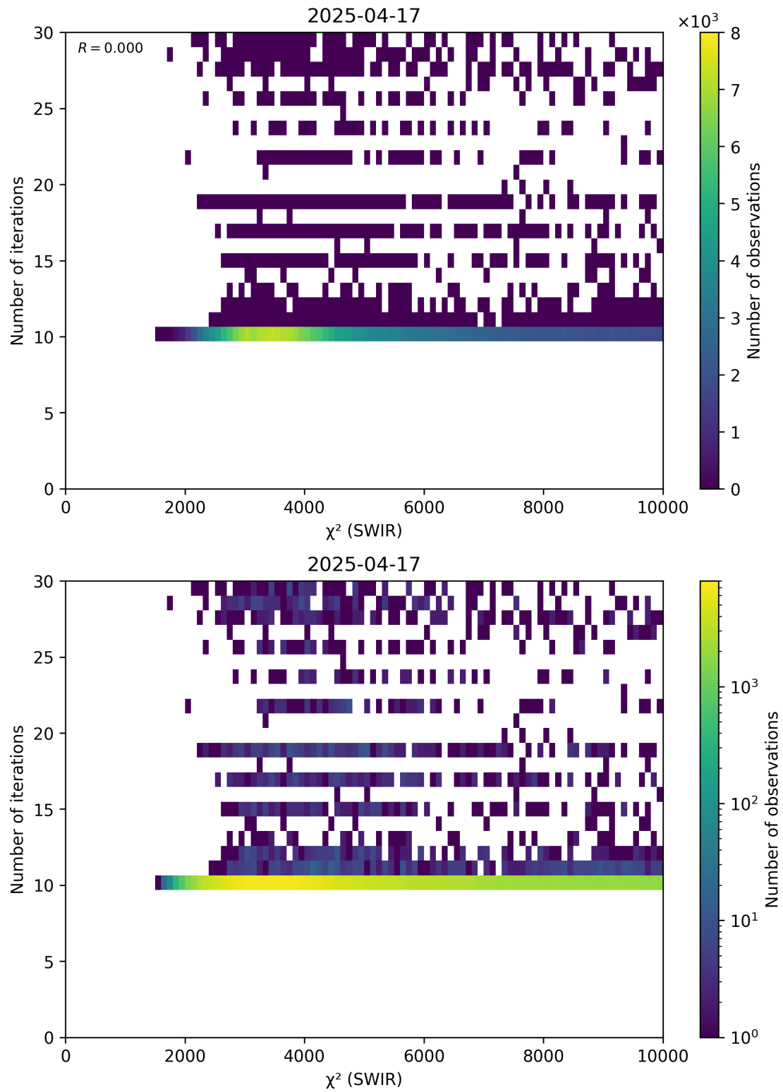
Figure 50: Scatter density plot of “ \chi^2 (SWIR)” against “Number of iterations” for 2025-04-16 to 2025-04-18.
