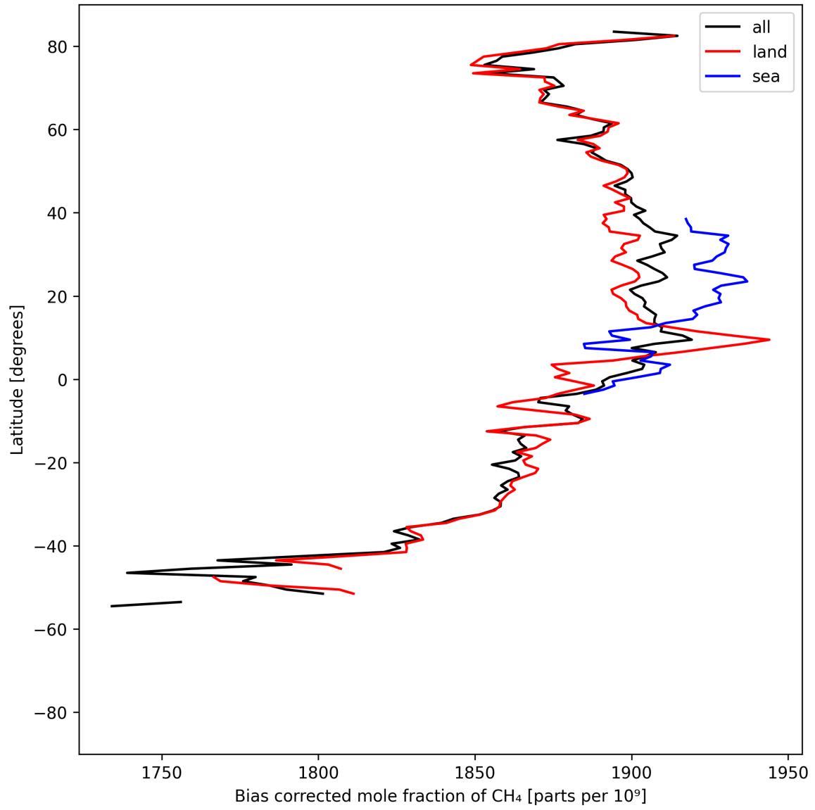
Figure 14: Zonal average of “Bias corrected mole fraction of CH 4 ” for 2025-04-16 to 2025-04-18.
