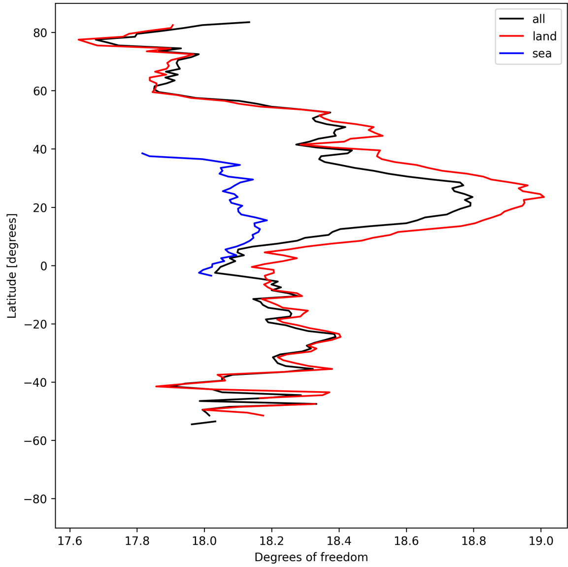
Figure 19: Zonal average of “Degrees of freedom” for 2025-04-16 to 2025-04-18.
