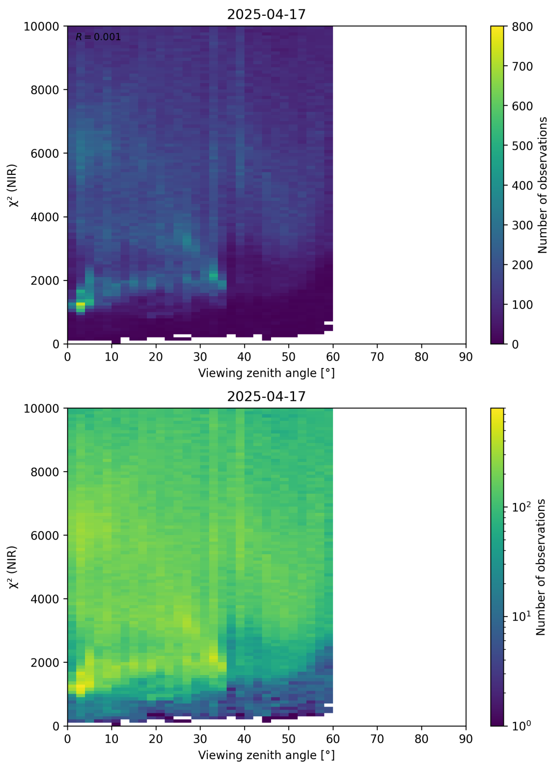
Figure 105: Scatter density plot of “Viewing zenith angle” against “ \chi^2 (NIR)” for 2025-04-16 to 2025-04-18.
