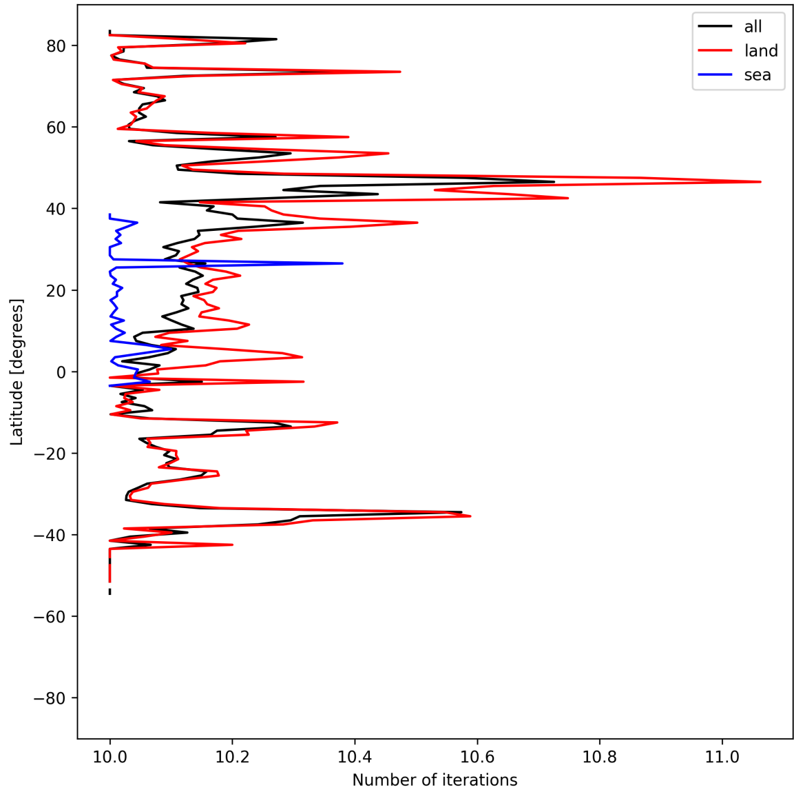
Figure 20: Zonal average of “Number of iterations” for 2025-04-16 to 2025-04-18.
