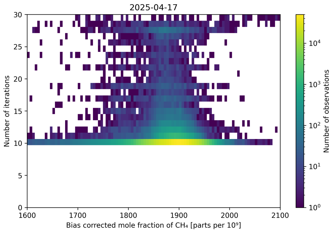
Figure 67: Scatter density plot of “Bias corrected mole fraction of CH 4 ” against “Number of iterations” for 2025-04-16 to 2025-04-18.
