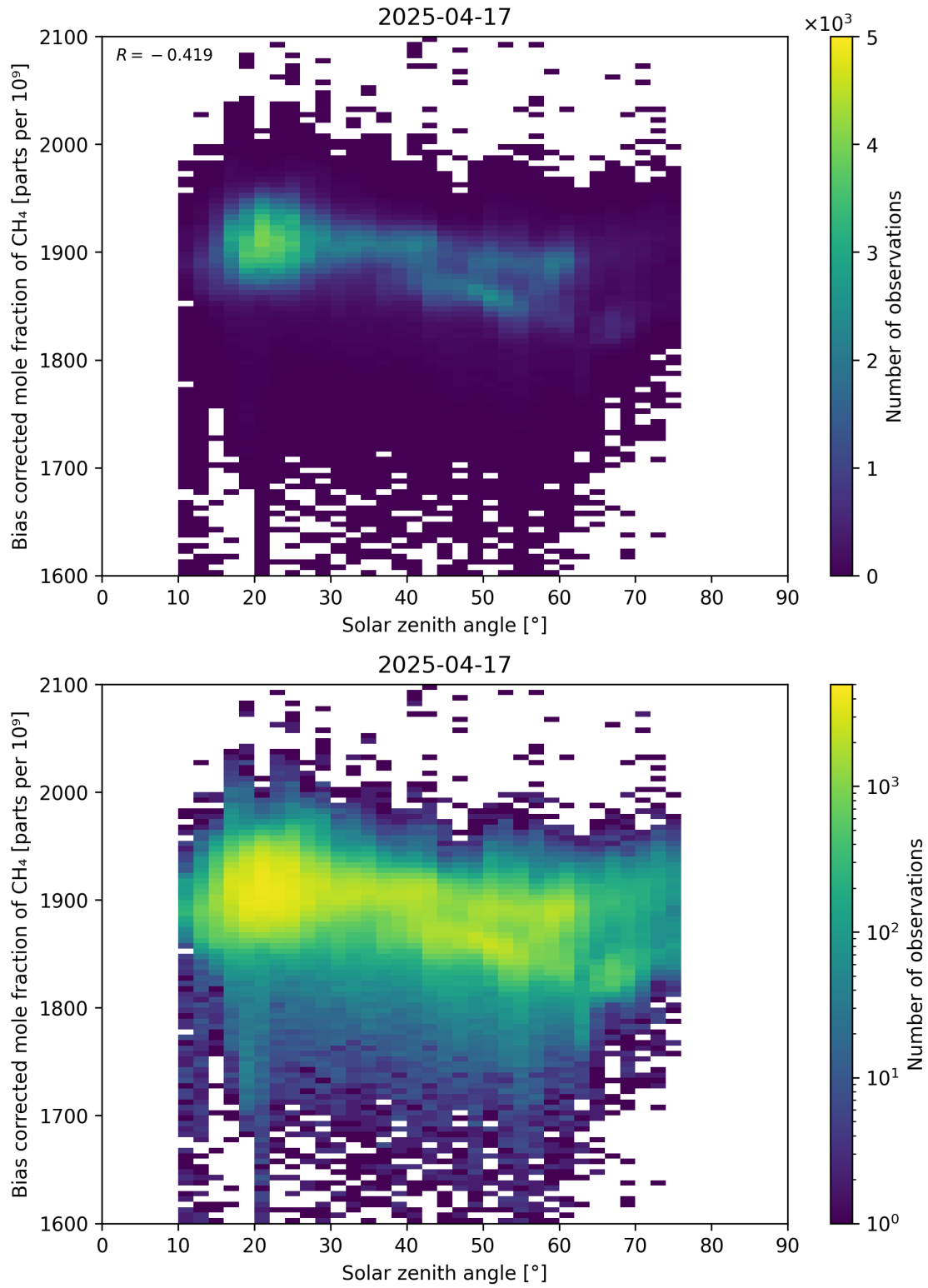
Figure 100: Scatter density plot of “Solar zenith angle” against “Bias corrected mole fraction of \text{CH}_4 ” for 2025-04-16 to 2025-04-18.
