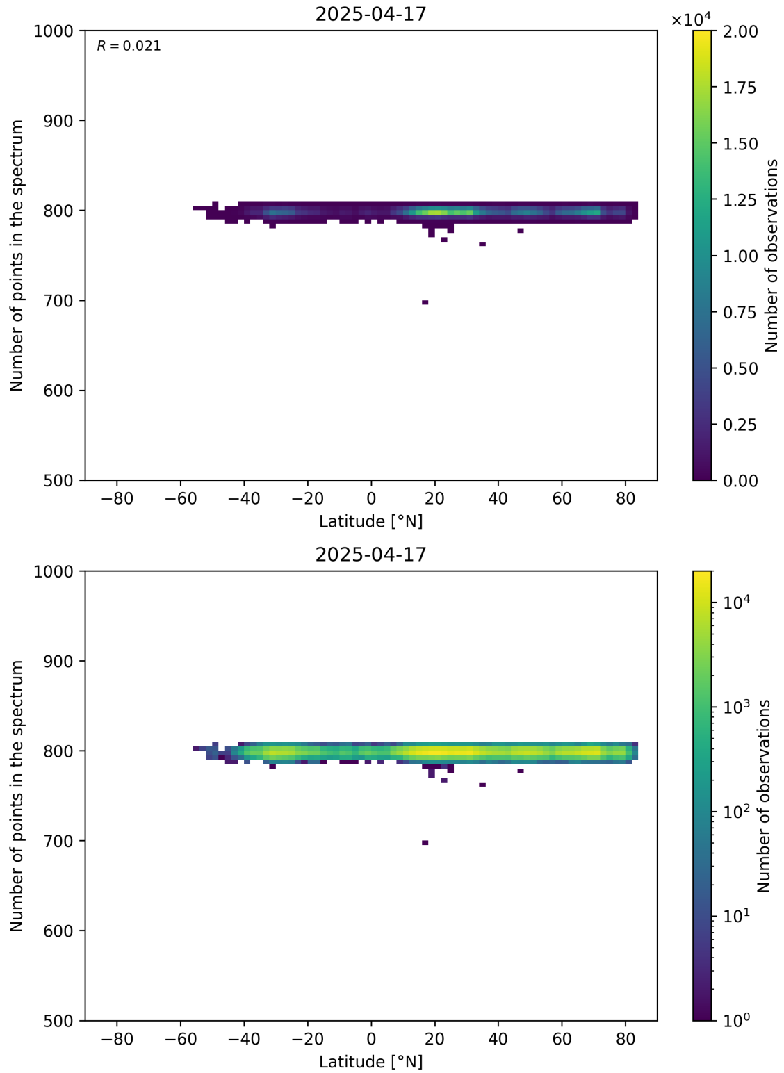
Figure 61: Scatter density plot of “Latitude” against “Number of points in the spectrum” for 2025-04-16 to 2025-04-18.
