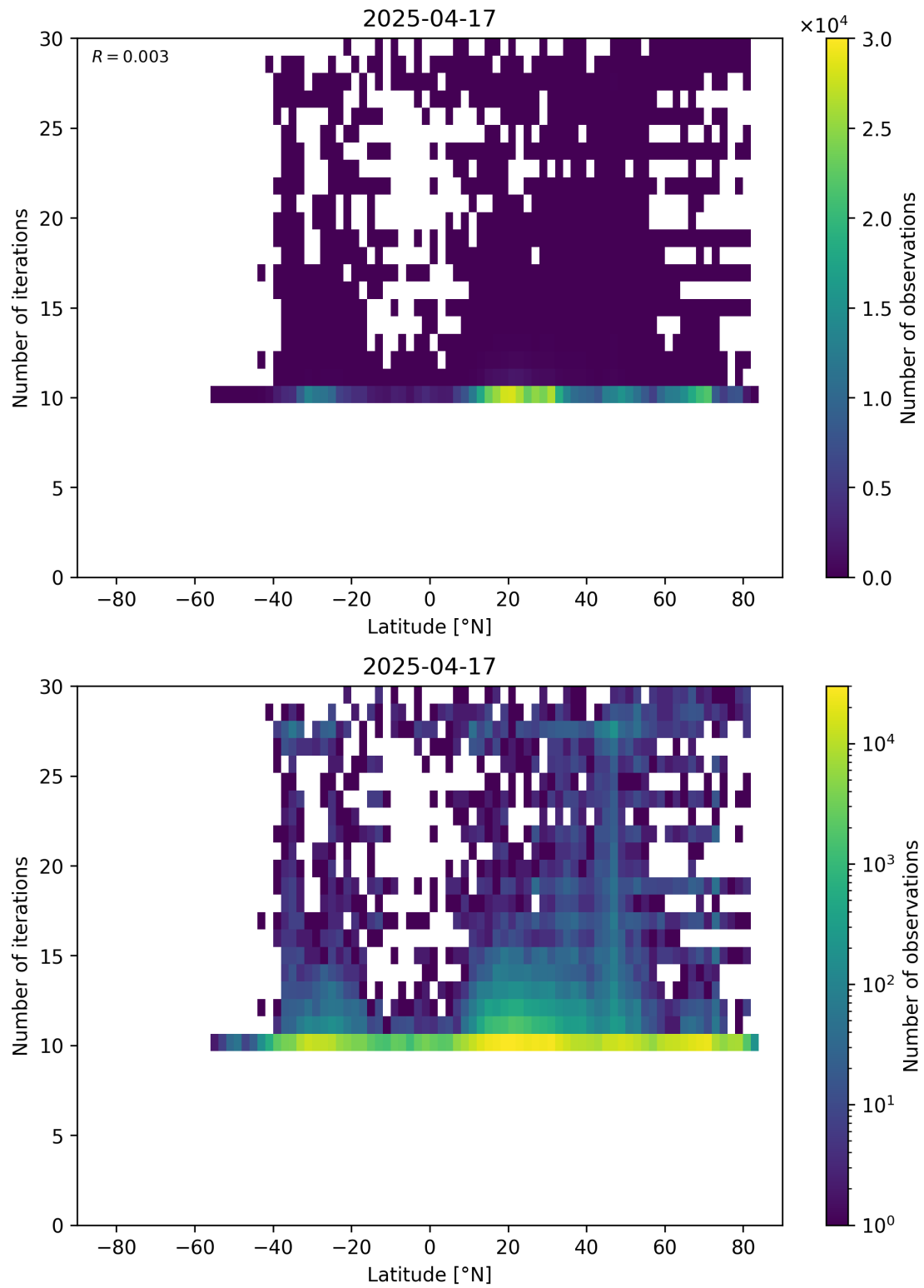
Figure 60: Scatter density plot of “Latitude” against “Number of iterations” for 2025-04-16 to 2025-04-18.
