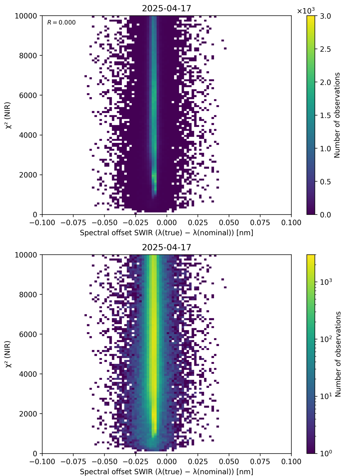
Figure 117: Scatter density plot of “Spectral offset SWIR ( \lambda_{\text{true}} - \lambda_{\text{nominal}} )” against “ \chi^2 (NIR)” for 2025-04-16 to 2025-04-18.
