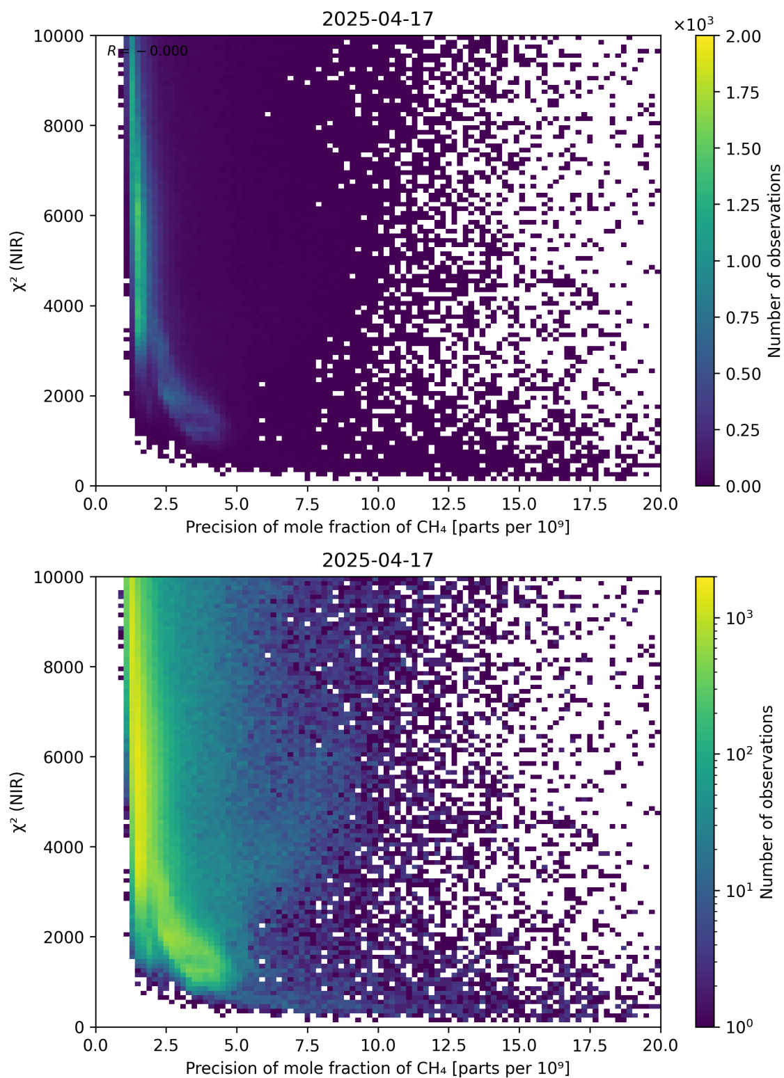
Figure 78: Scatter density plot of “Precision of mole fraction of CH 4 ” against “ \chi^2 (NIR)” for 2025-04-16 to 2025-04-18.
