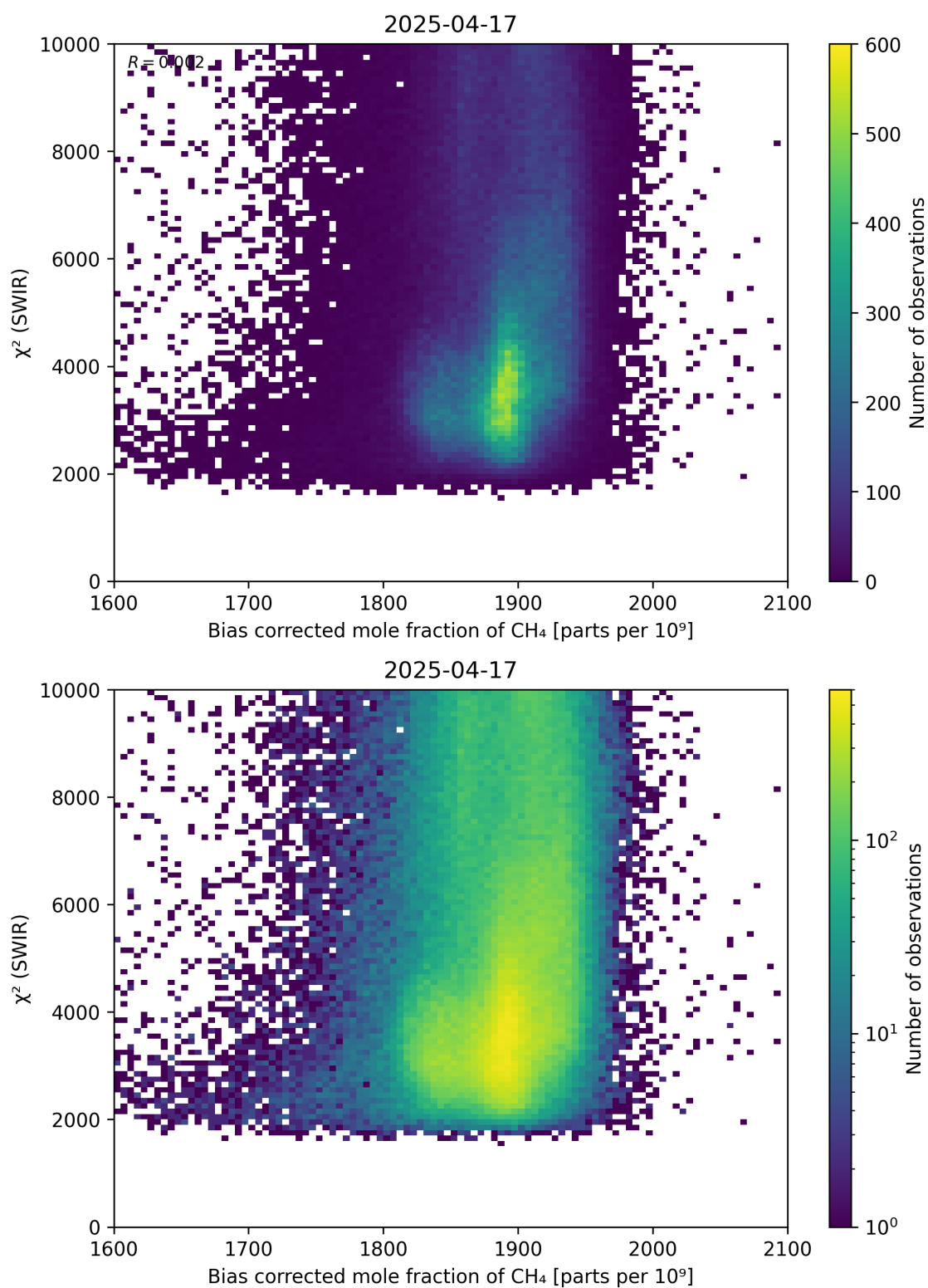
Figure 64: Scatter density plot of “Bias corrected mole fraction of \text{CH}_4 ” against “ \chi^2 (SWIR)” for 2025-04-16 to 2025-04-18.
