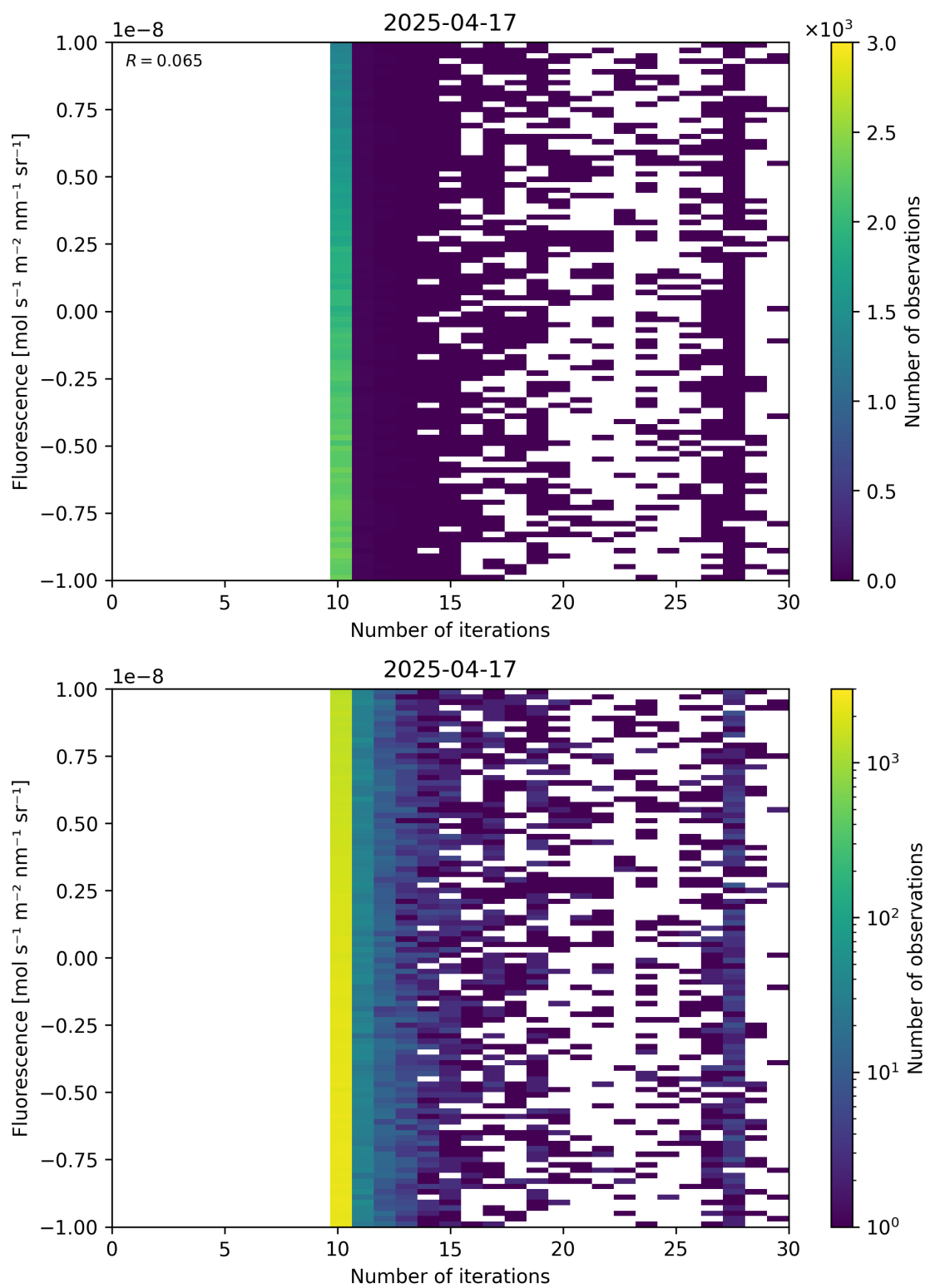
Figure 87: Scatter density plot of “Number of iterations” against “Fluorescence” for 2025-04-16 to 2025-04-18.
