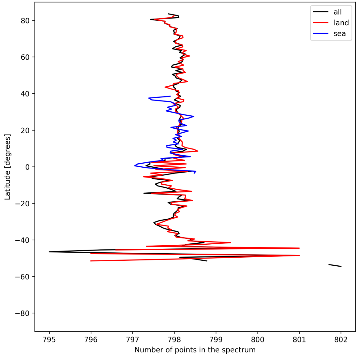
Figure 15: Zonal average of “Number of points in the spectrum” for 2025-04-16 to 2025-04-18.
