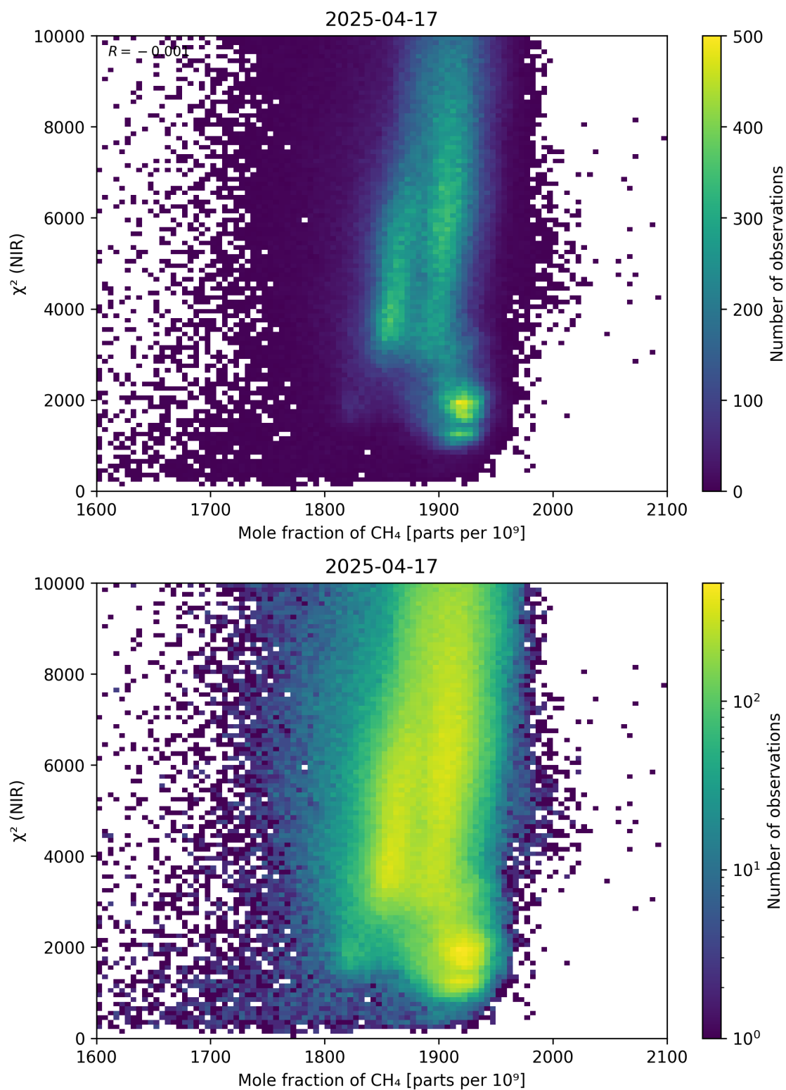
Figure 70: Scatter density plot of “Mole fraction of CH 4 ” against “ \chi^2 (NIR)” for 2025-04-16 to 2025-04-18.
