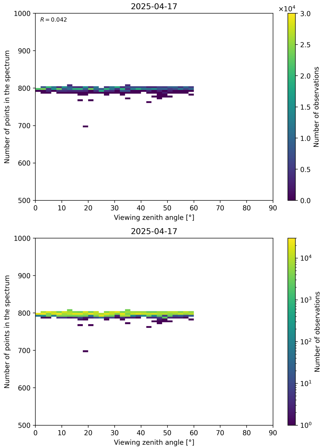
Figure 114: Scatter density plot of “Viewing zenith angle” against “Number of points in the spectrum” for 2025-04-16 to 2025-04-18.
