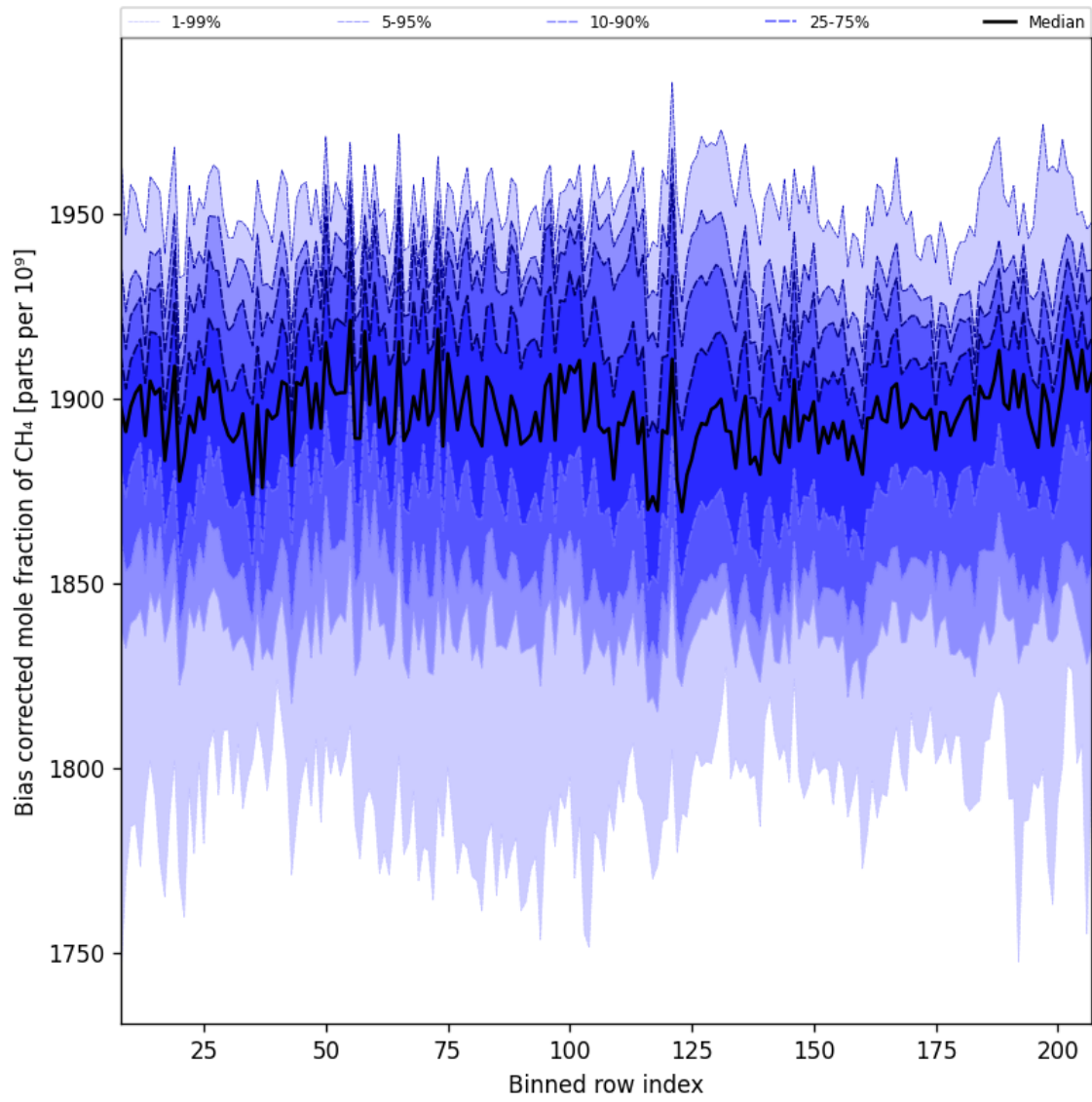
Figure 36: Along track statistics of “Bias corrected mole fraction of CH 4 ” for 2025-04-16 to 2025-04-18
