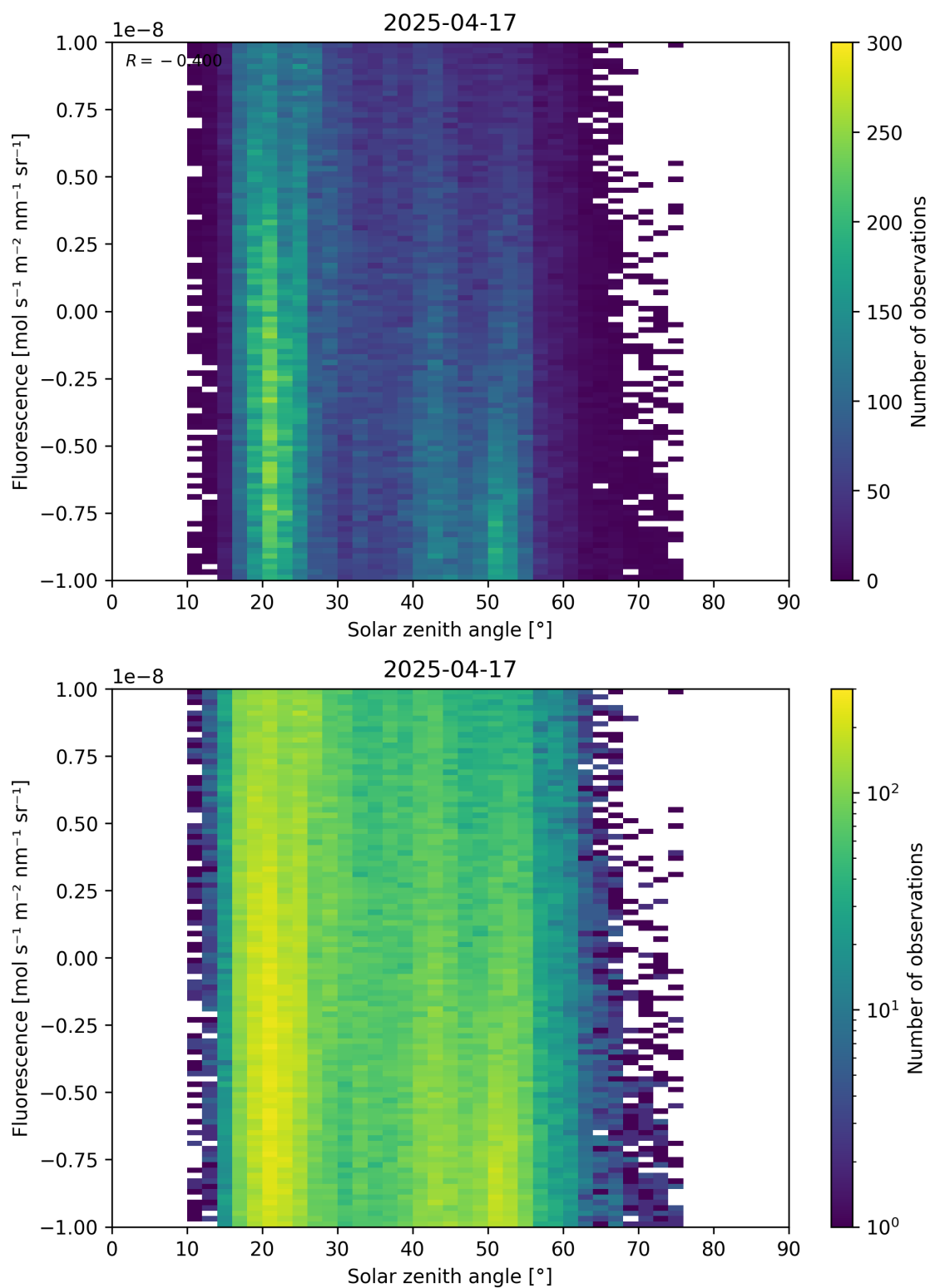
Figure 97: Scatter density plot of “Solar zenith angle” against “Fluorescence” for 2025-04-16 to 2025-04-18.
