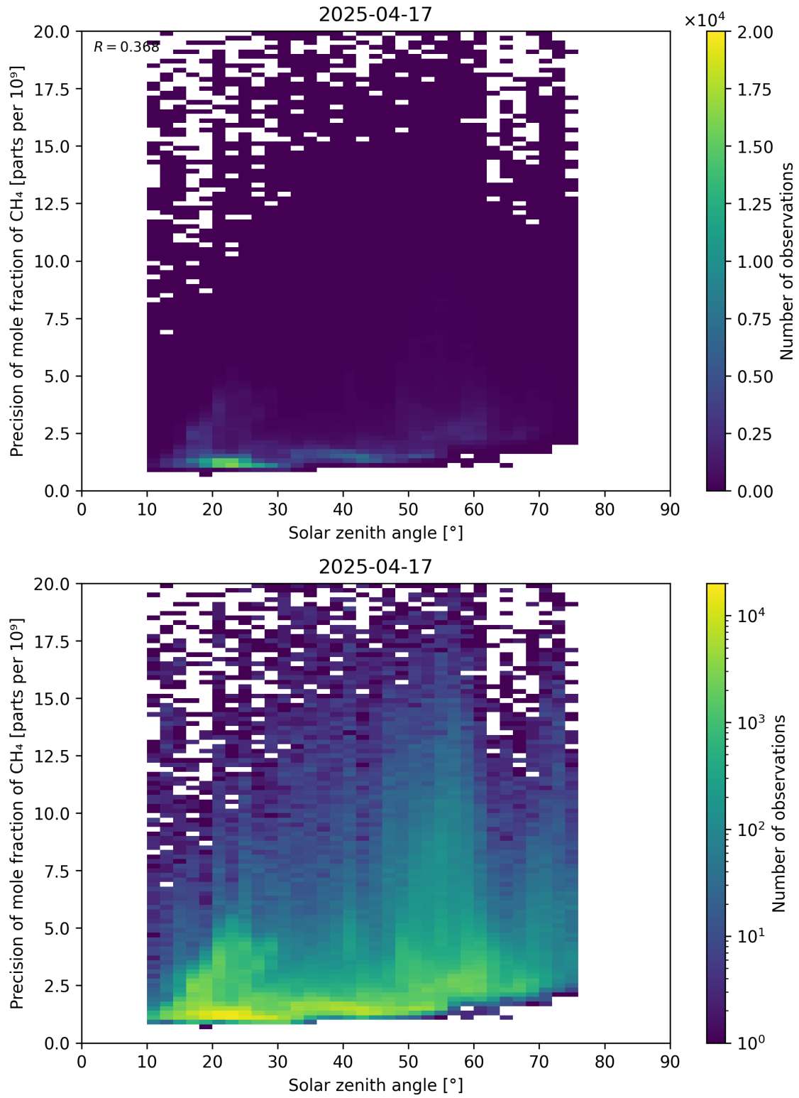
Figure 101: Scatter density plot of “Solar zenith angle” against “Precision of mole fraction of CH 4 ” for 2025-04-16 to 2025-04-18.
