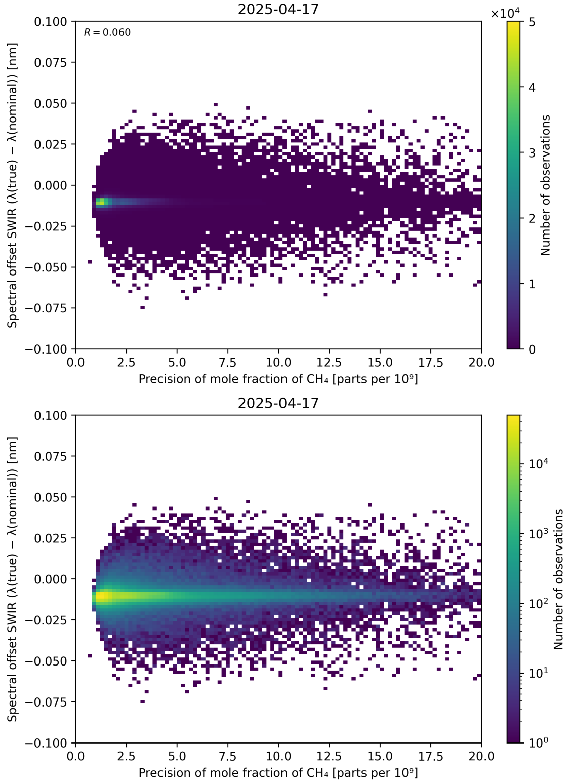
Figure 85: Scatter density plot of “Precision of mole fraction of CH 4 ” against “Spectral offset SWIR ( \lambda_{\text{true}} - \lambda_{\text{nominal}} )” for 2025-04-16 to 2025-04-18.
