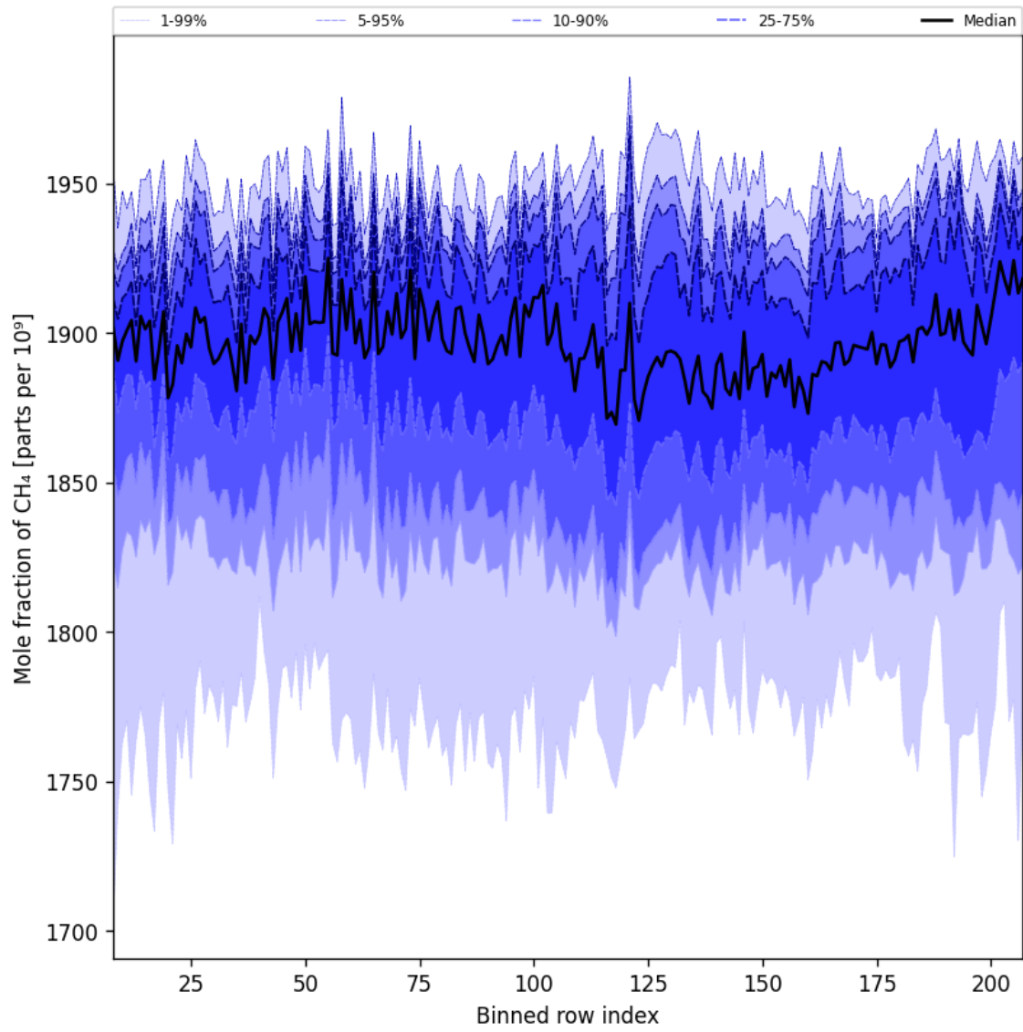
Figure 34: Along track statistics of “Mole fraction of CH 4 ” for 2025-04-16 to 2025-04-18
