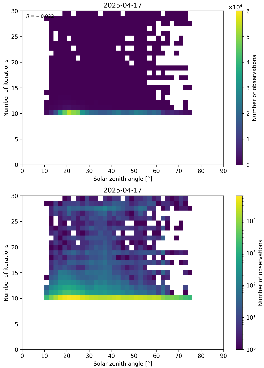
Figure 102: Scatter density plot of “Solar zenith angle” against “Number of iterations” for 2025-04-16 to 2025-04-18.
