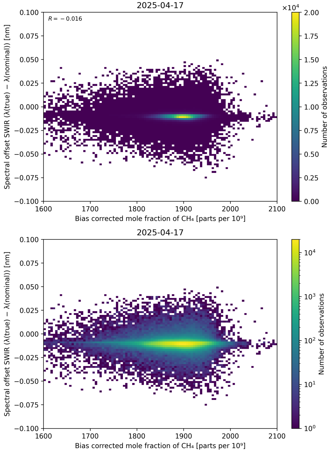
Figure 69: Scatter density plot of “Bias corrected mole fraction of CH 4 ” against “Spectral offset SWIR ( \lambda_{\text{true}} - \lambda_{\text{nominal}} )” for 2025-04-16 to 2025-04-18.
