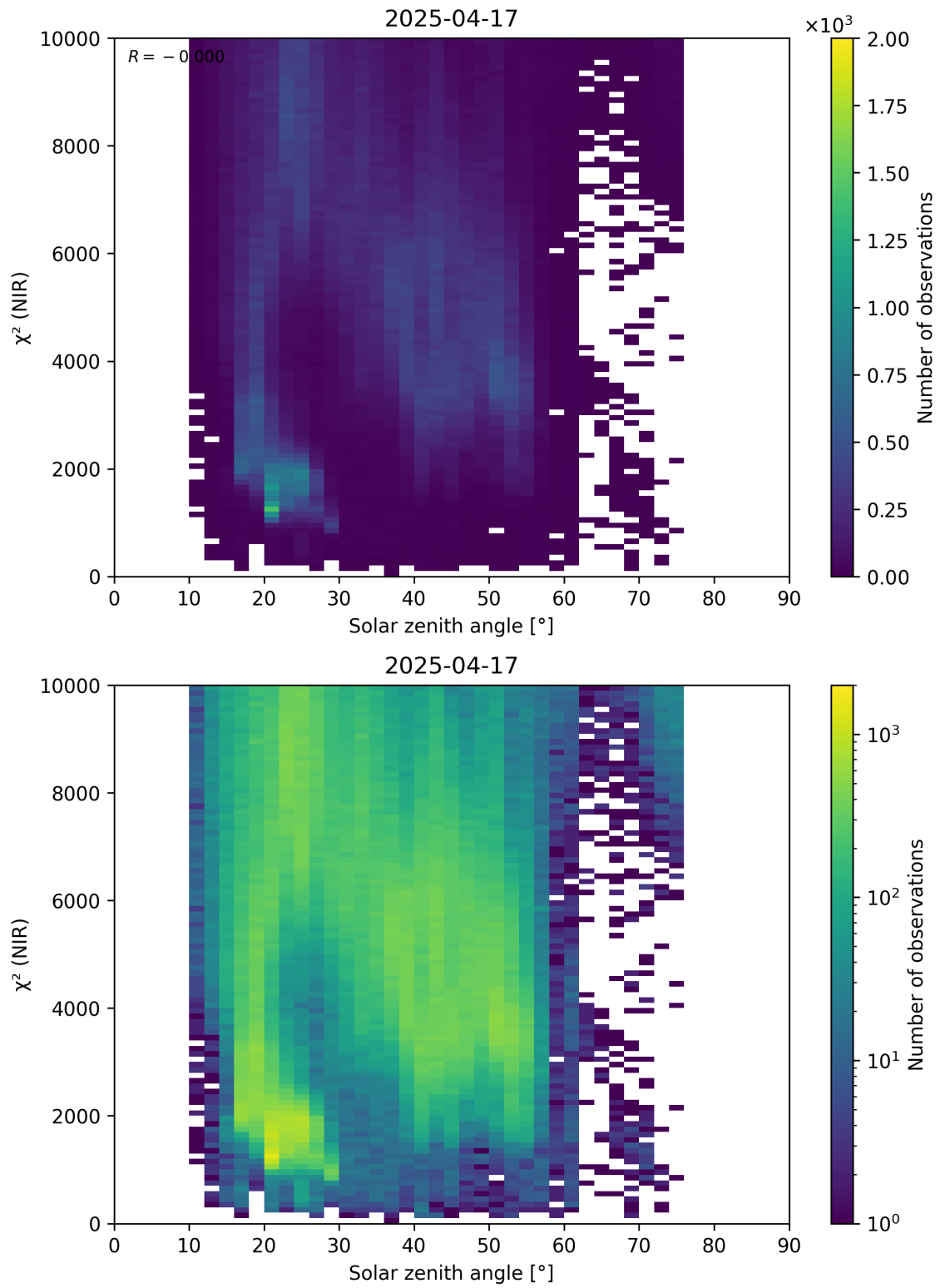
Figure 94: Scatter density plot of “Solar zenith angle” against “ \chi^2 (NIR)” for 2025-04-16 to 2025-04-18.
