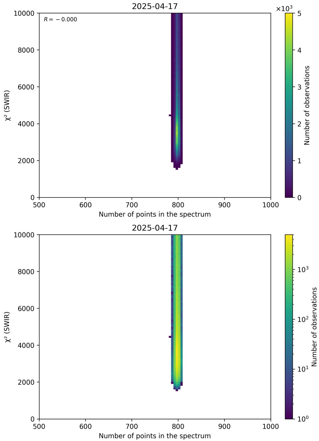
Figure 89: Scatter density plot of “Number of points in the spectrum” against “ \chi^2 (SWIR)” for 2025-04-16 to 2025-04-18.
