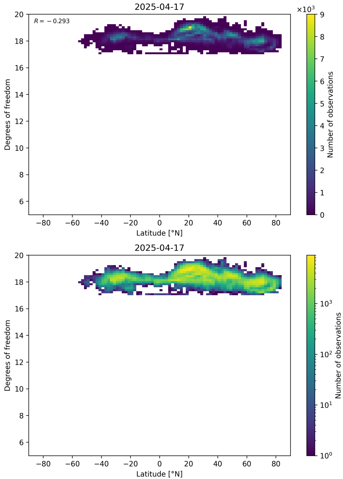
Figure 55: Scatter density plot of “Latitude” against “Degrees of freedom” for 2025-04-16 to 2025-04-18.
