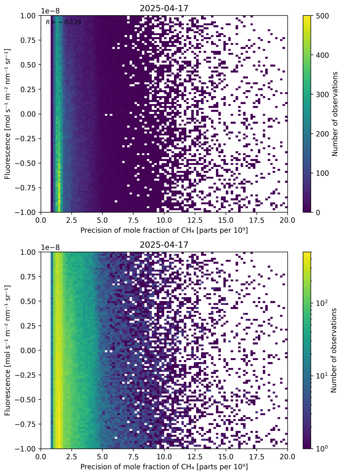
Figure 81: Scatter density plot of “Precision of mole fraction of CH 4 ” against “Fluorescence” for 2025-04-16 to 2025-04-18.
