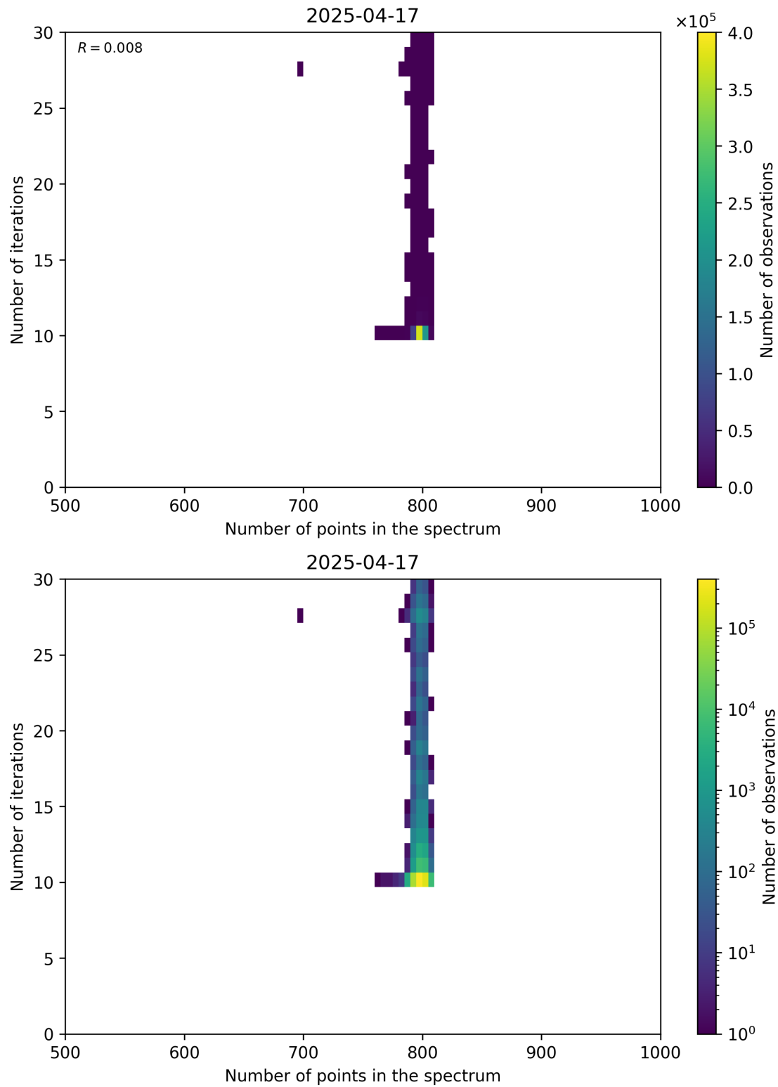
Figure 92: Scatter density plot of “Number of points in the spectrum” against “Number of iterations” for 2025-04-16 to 2025-04-18.
