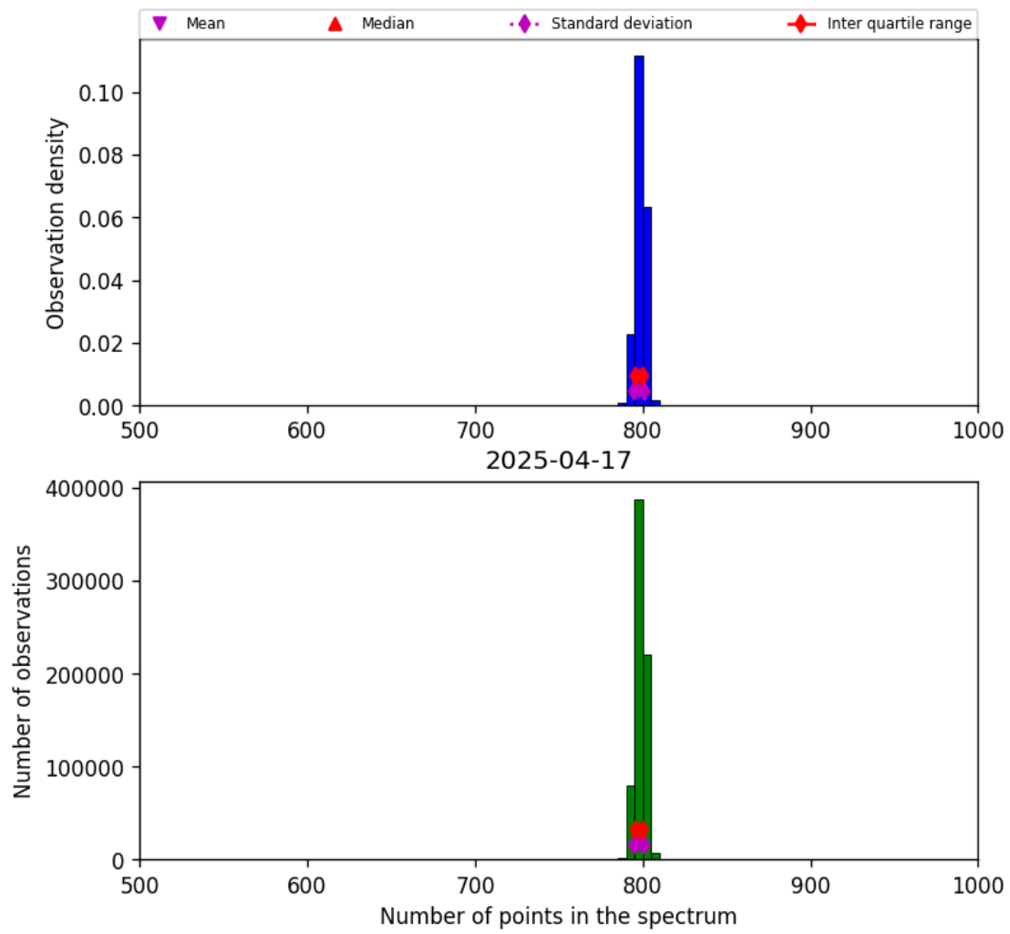
Figure 26: Histogram of “Number of points in the spectrum” for 2025-04-16 to 2025-04-18
