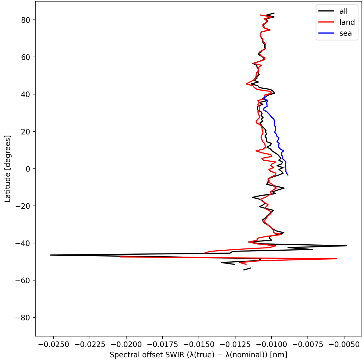
Figure 16: Zonal average of “Spectral offset SWIR ( \lambda_{\text{true}} - \lambda_{\text{nominal}} )” for 2025-04-16 to 2025-04-18.
