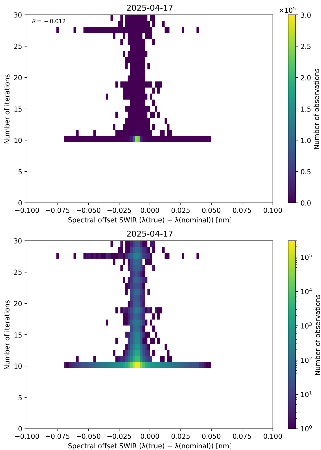
Figure 121: Scatter density plot of “Spectral offset SWIR ( \lambda_{\text{true}} - \lambda_{\text{nominal}} )” against “Number of iterations” for 2025-04-16 to 2025-04-18.
