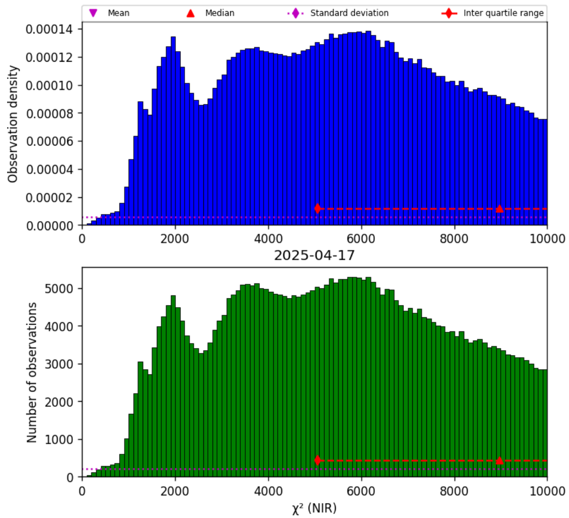
Figure 29: Histogram of “ \chi^2 (NIR)” for 2025-04-16 to 2025-04-18
