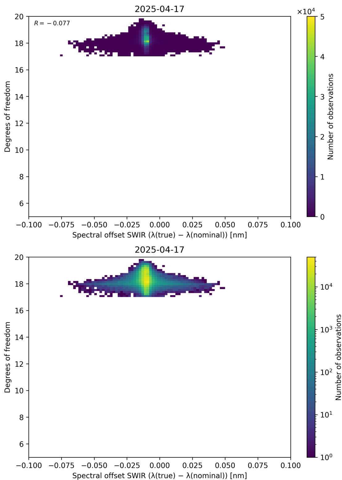
Figure 119: Scatter density plot of “Spectral offset SWIR ( \lambda_{\text{true}} - \lambda_{\text{nominal}} )” against “Degrees of freedom” for 2025-04-16 to 2025-04-18.
