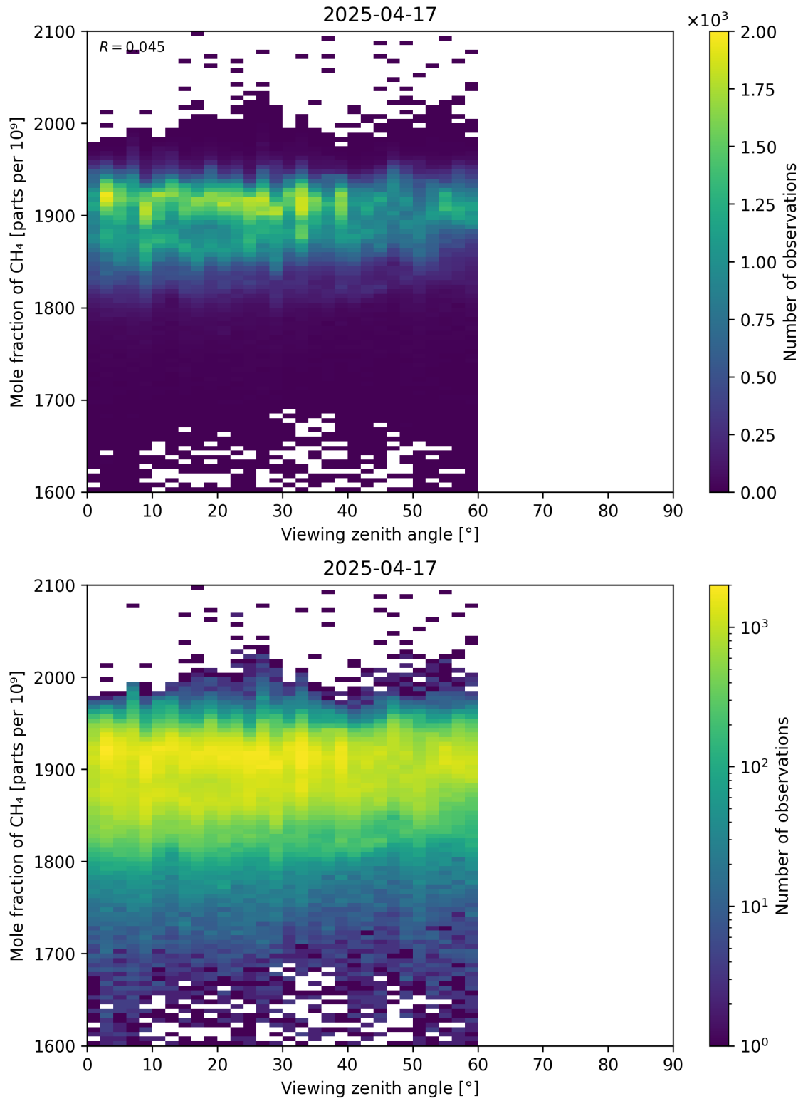
Figure 110: Scatter density plot of “Viewing zenith angle” against “Mole fraction of \text{CH}_4 ” for 2025-04-16 to 2025-04-18.
