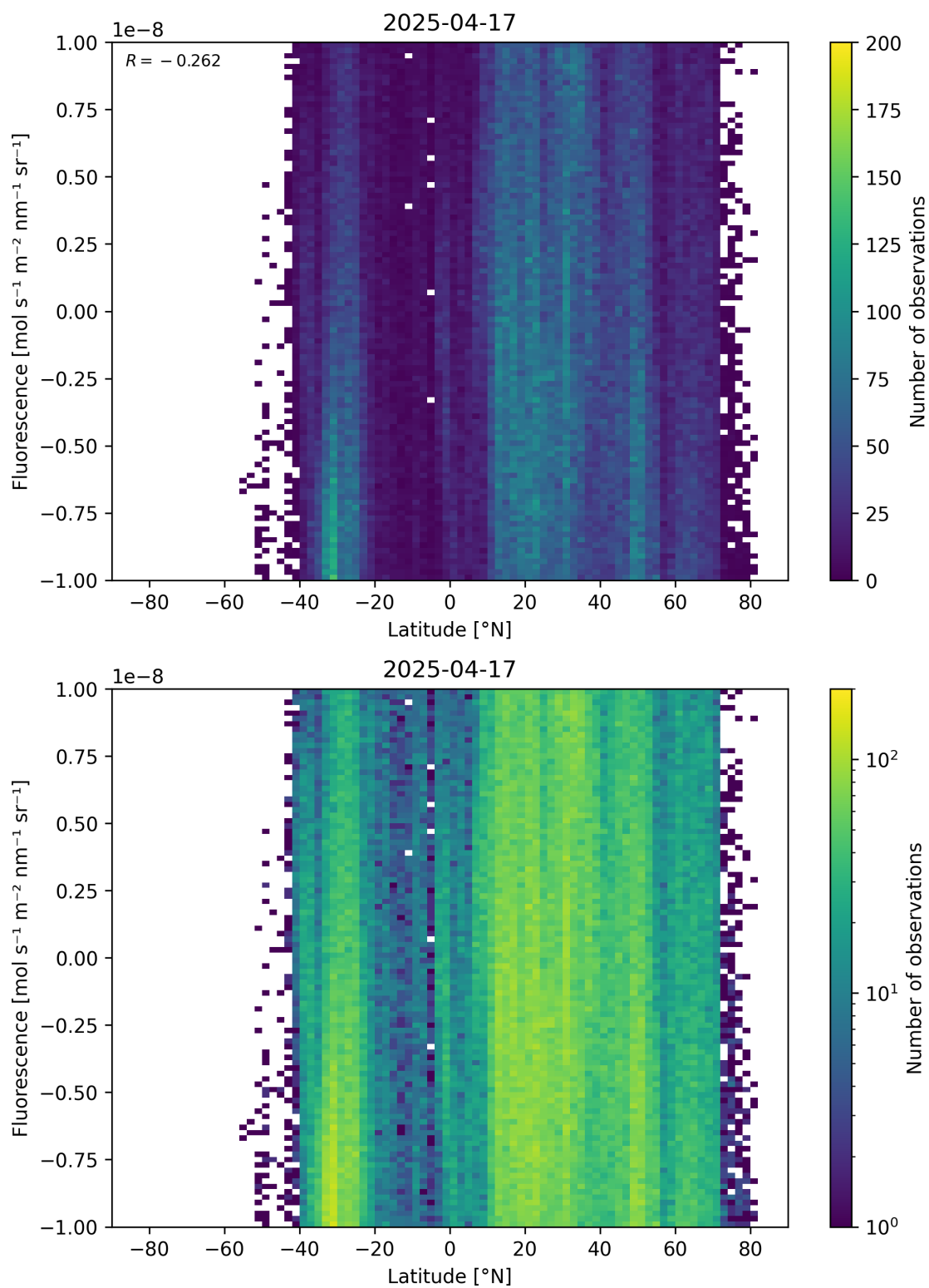
Figure 56: Scatter density plot of “Latitude” against “Fluorescence” for 2025-04-16 to 2025-04-18.
