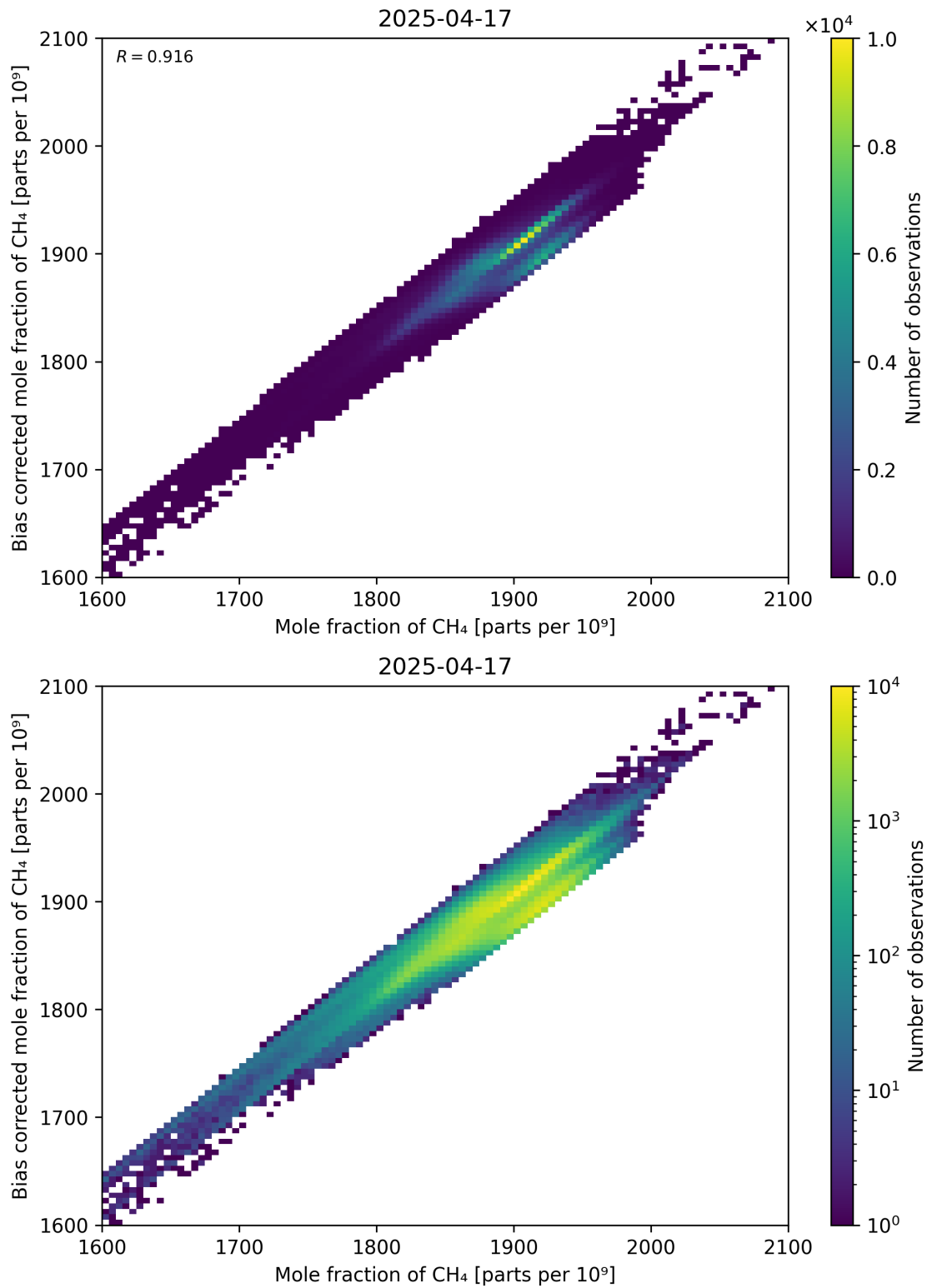
Figure 74: Scatter density plot of “Mole fraction of CH 4 ” against “Bias corrected mole fraction of CH 4 ” for 2025-04-16 to 2025-04-18.
