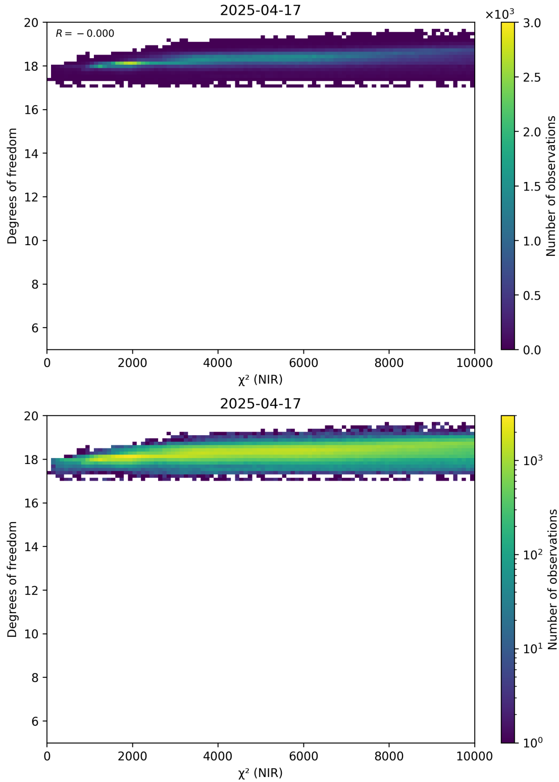
Figure 44: Scatter density plot of “ \chi^2 (NIR)” against “Degrees of freedom” for 2025-04-16 to 2025-04-18.
