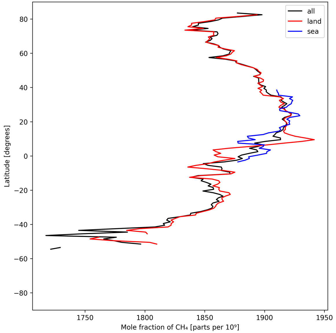
Figure 12: Zonal average of “Mole fraction of \text{CH}_4 ” for 2025-04-16 to 2025-04-18.
