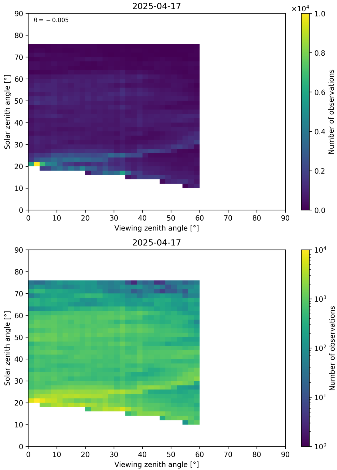
Figure 115: Scatter density plot of “Viewing zenith angle” against “Solar zenith angle” for 2025-04-16 to 2025-04-18.
