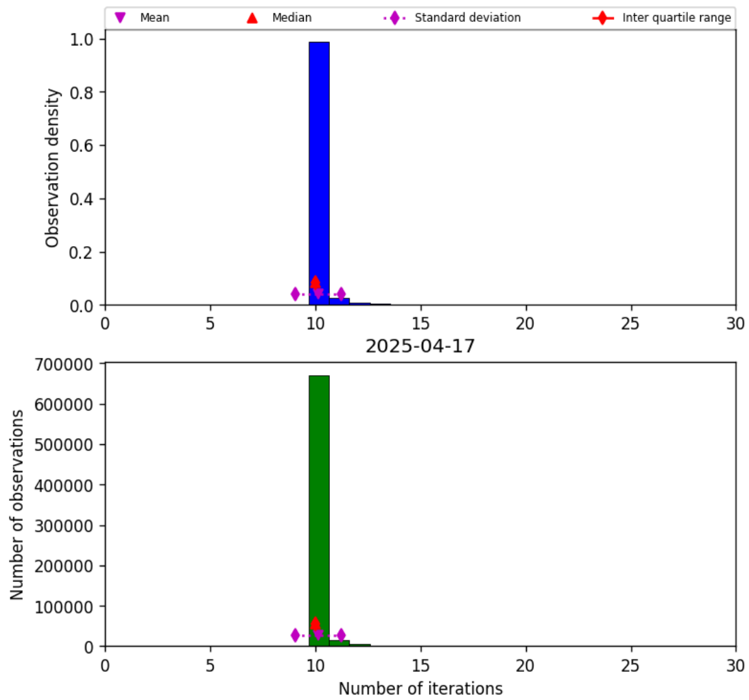
Figure 31: Histogram of “Number of iterations” for 2025-04-16 to 2025-04-18
