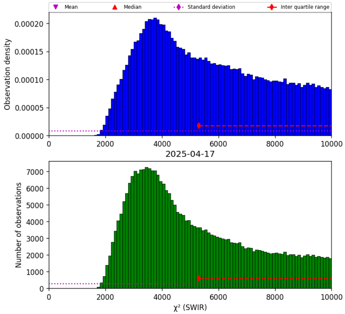
Figure 28: Histogram of “ \chi^2 (SWIR)” for 2025-04-16 to 2025-04-18
