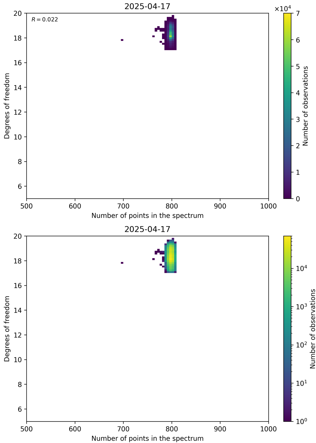
Figure 90: Scatter density plot of “Number of points in the spectrum” against “Degrees of freedom” for 2025-04-16 to 2025-04-18.
