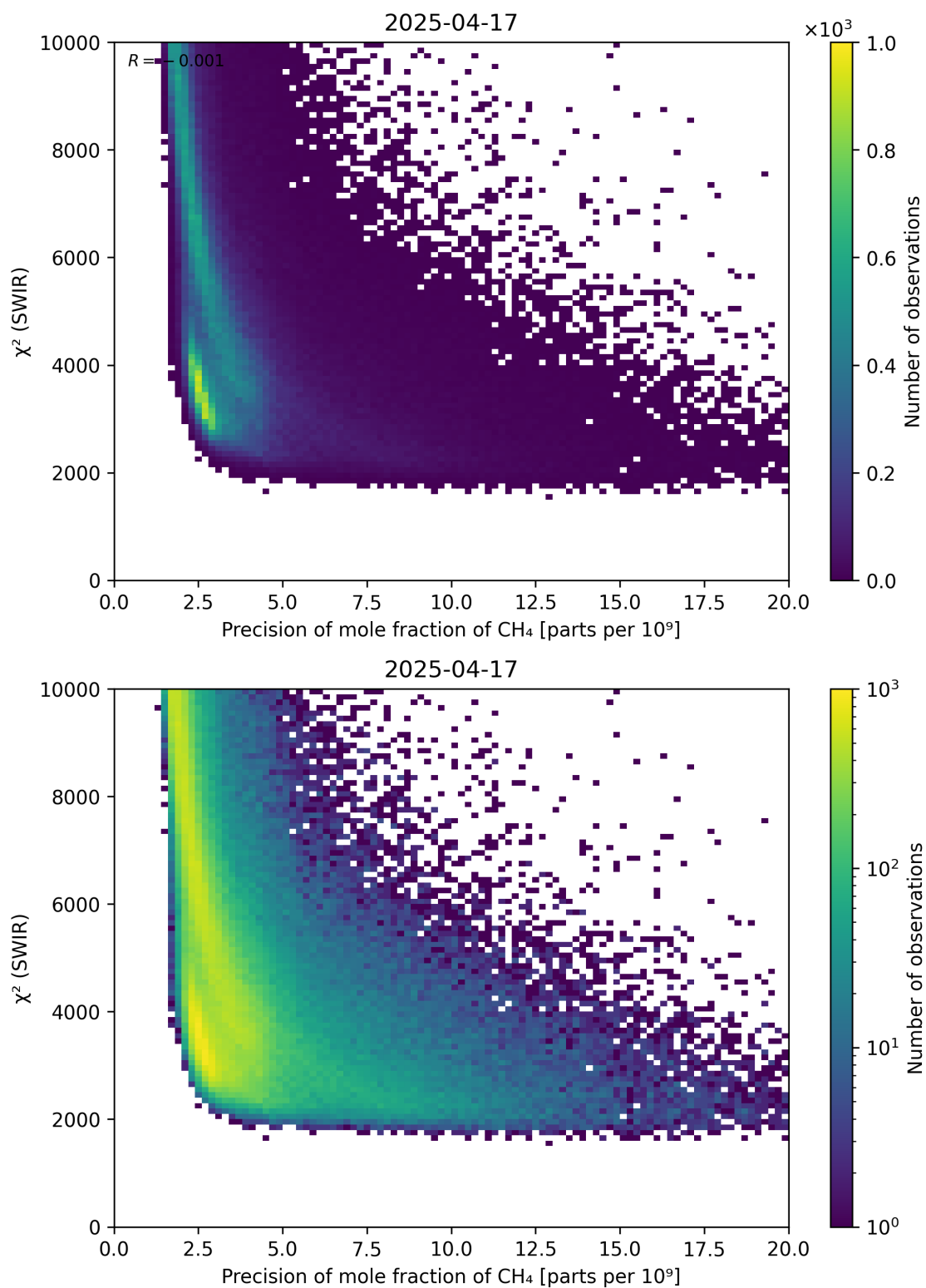
Figure 79: Scatter density plot of “Precision of mole fraction of \text{CH}_4 ” against “ \chi^2 (SWIR)” for 2025-04-16 to 2025-04-18.
