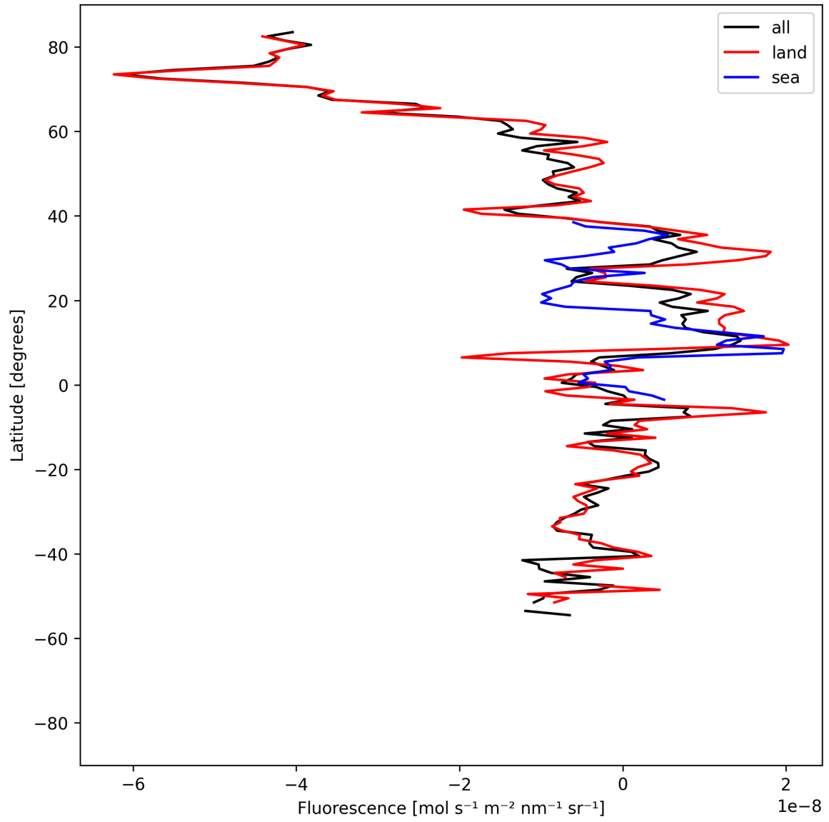
Figure 21: Zonal average of “Fluorescence” for 2025-04-16 to 2025-04-18.
