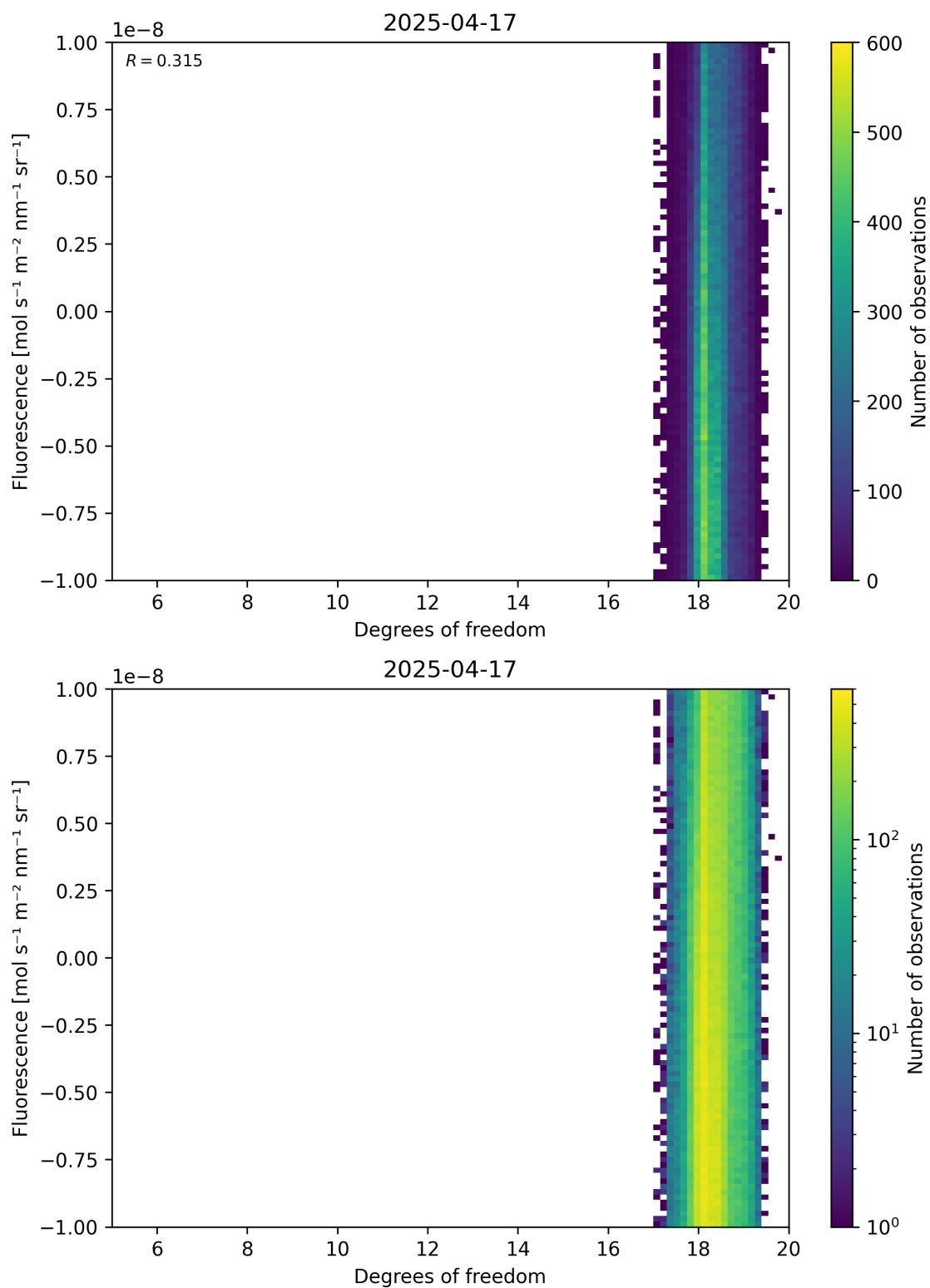
Figure 51: Scatter density plot of “Degrees of freedom” against “Fluorescence” for 2025-04-16 to 2025-04-18.
