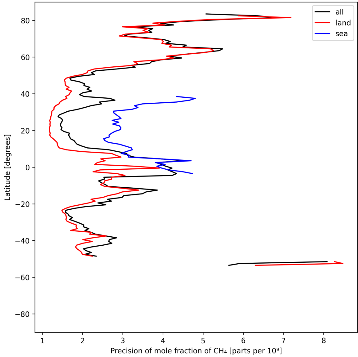
Figure 13: Zonal average of “Precision of mole fraction of CH 4 ” for 2025-04-18 to 2025-04-19.
