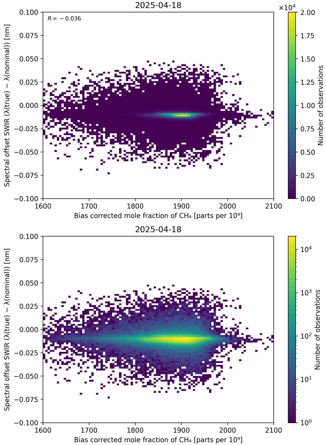
Figure 69: Scatter density plot of “Bias corrected mole fraction of CH 4 ” against “Spectral offset SWIR ( \lambda_{\text{true}} - \lambda_{\text{nominal}} )” for 2025-04-18 to 2025-04-19.
