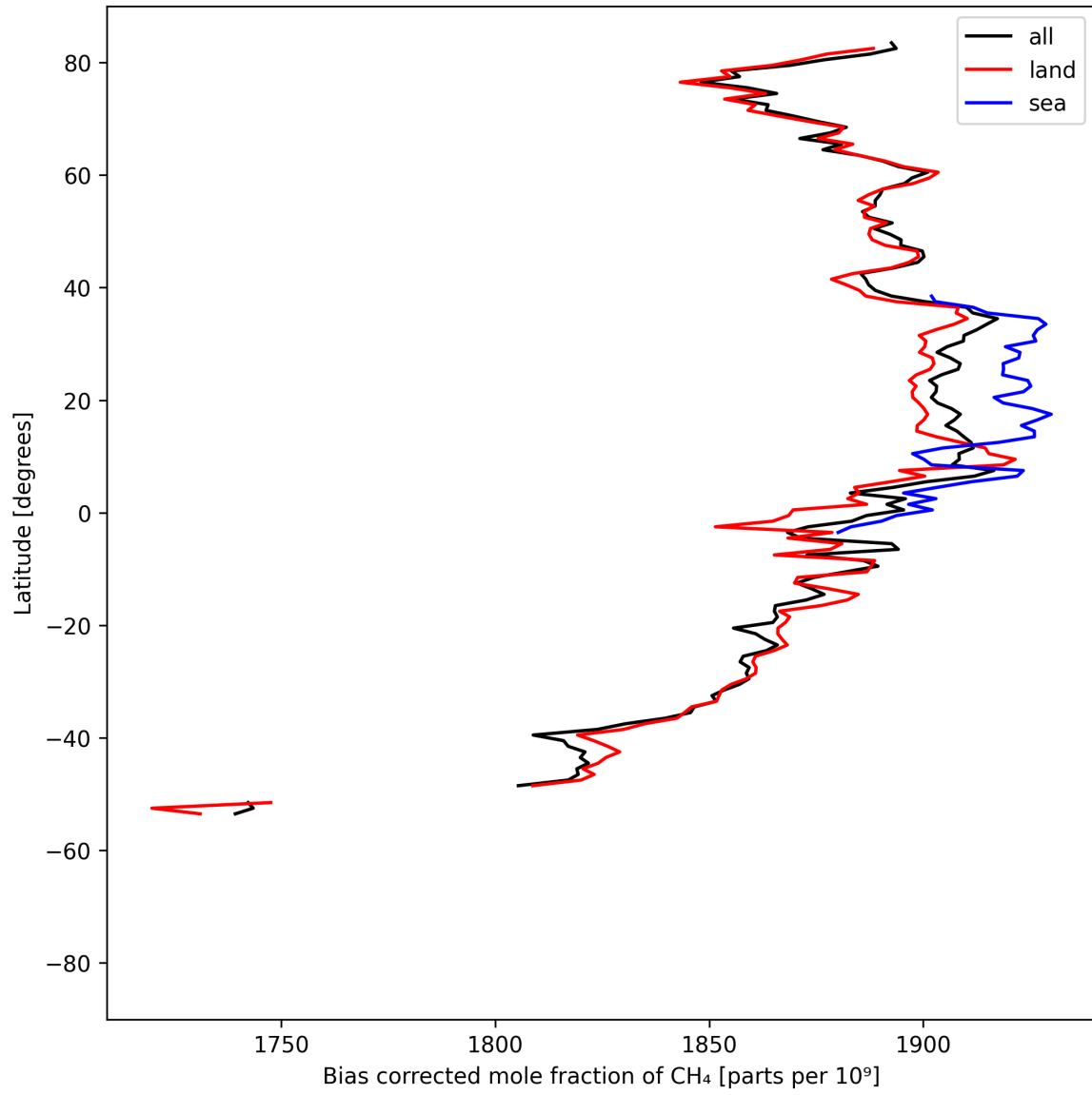
Figure 14: Zonal average of “Bias corrected mole fraction of \text{CH}_4 ” for 2025-04-18 to 2025-04-19.
