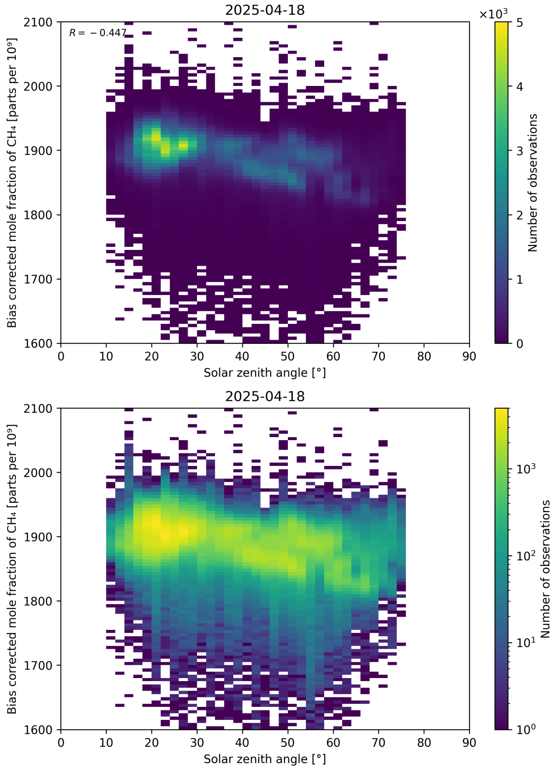
Figure 100: Scatter density plot of “Solar zenith angle” against “Bias corrected mole fraction of CH 4 ” for 2025-04-18 to 2025-04-19.
