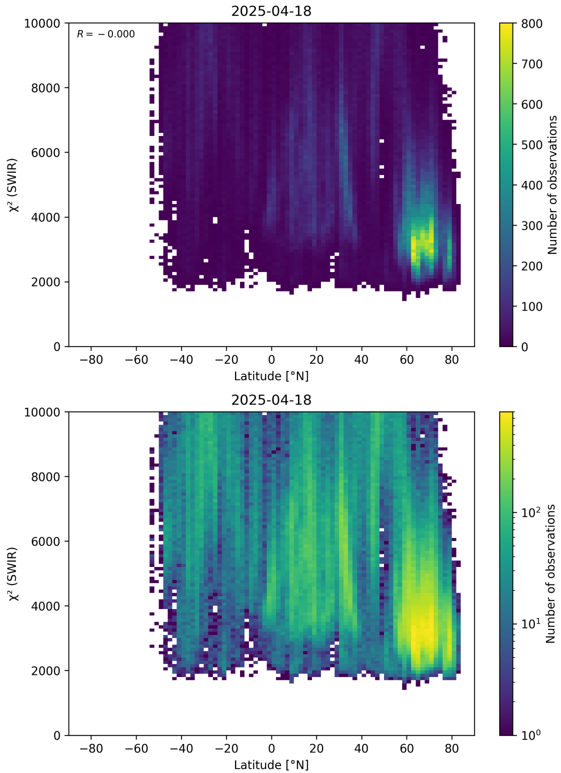
Figure 54: Scatter density plot of “Latitude” against “ \chi^2 (SWIR)” for 2025-04-18 to 2025-04-19.
