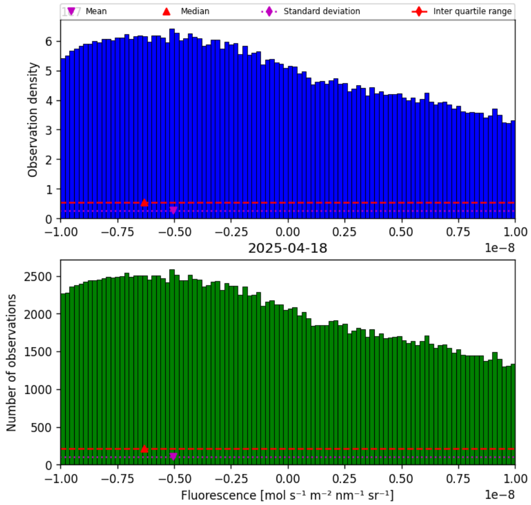
Figure 32: Histogram of “Fluorescence” for 2025-04-18 to 2025-04-19
