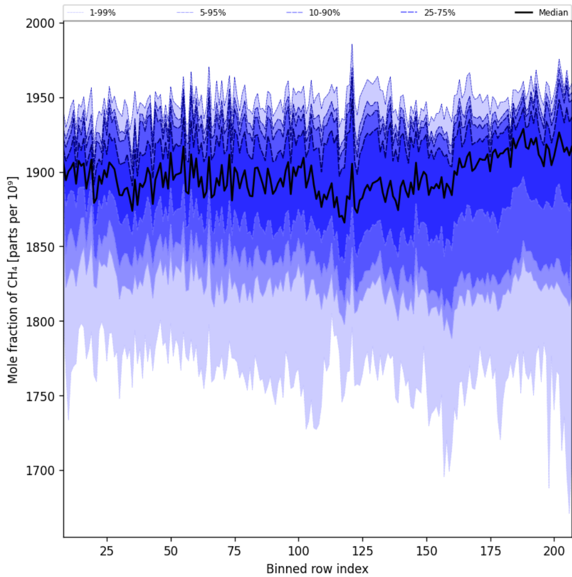
Figure 34: Along track statistics of “Mole fraction of CH 4 ” for 2025-04-18 to 2025-04-19
