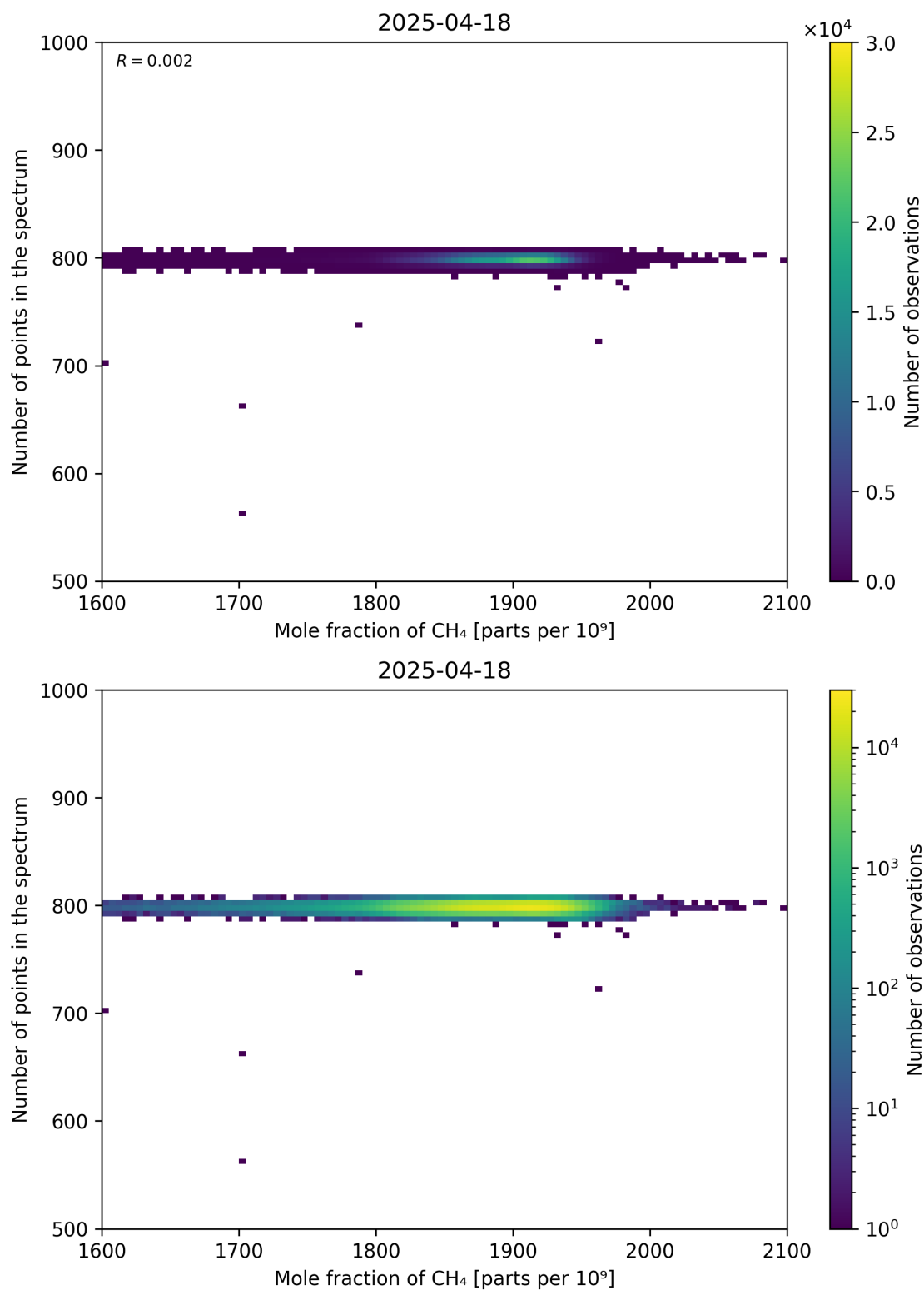
Figure 77: Scatter density plot of “Mole fraction of CH 4 ” against “Number of points in the spectrum” for 2025-04-18 to 2025-04-19.
