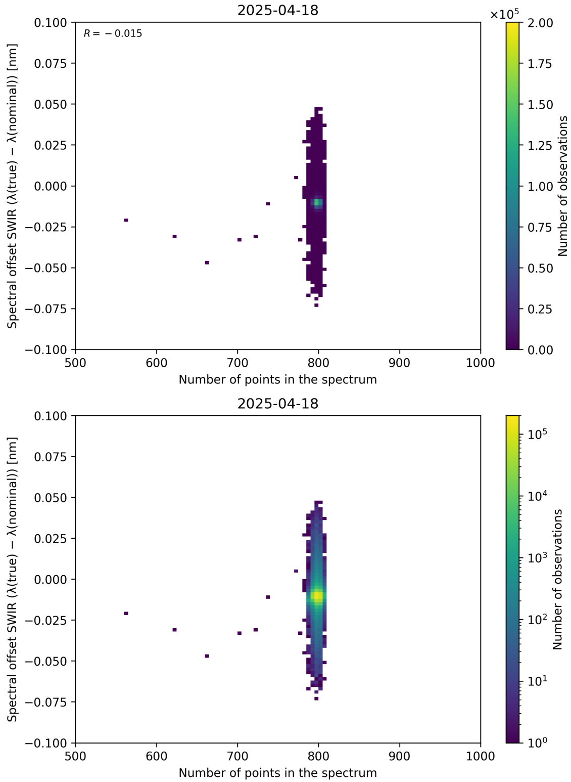
Figure 93: Scatter density plot of “Number of points in the spectrum” against “Spectral offset SWIR ( \lambda_{\text{true}} - \lambda_{\text{nominal}} )” for 2025-04-18 to 2025-04-19.
