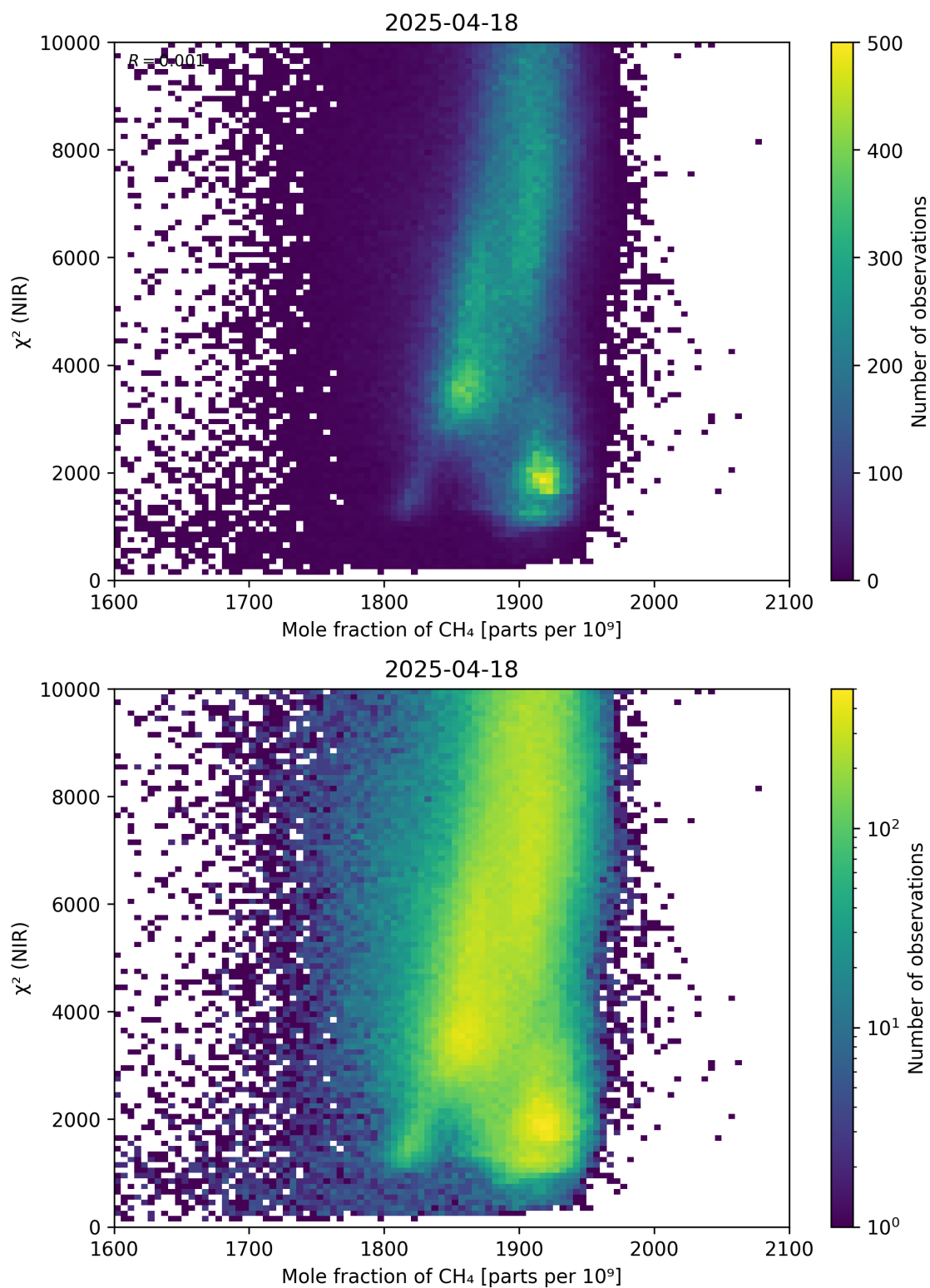
Figure 70: Scatter density plot of “Mole fraction of \text{CH}_4 ” against “ \chi^2 (NIR)” for 2025-04-18 to 2025-04-19.
