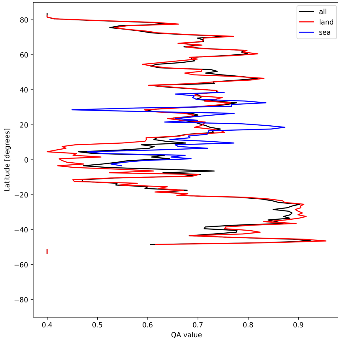
Figure 11: Zonal average of “QA value” for 2025-04-18 to 2025-04-19.
