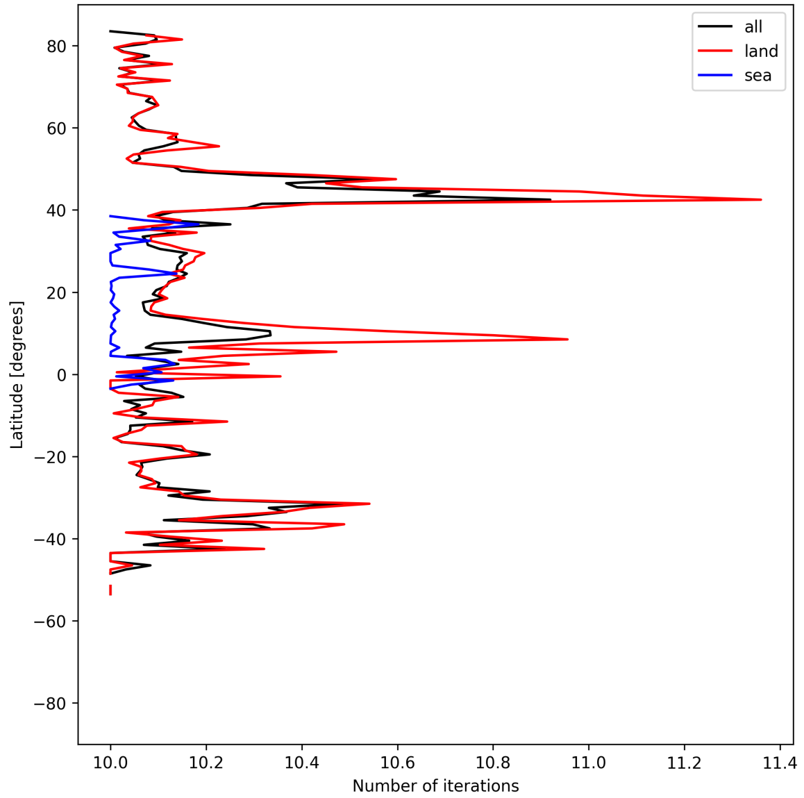
Figure 20: Zonal average of “Number of iterations” for 2025-04-18 to 2025-04-19.
