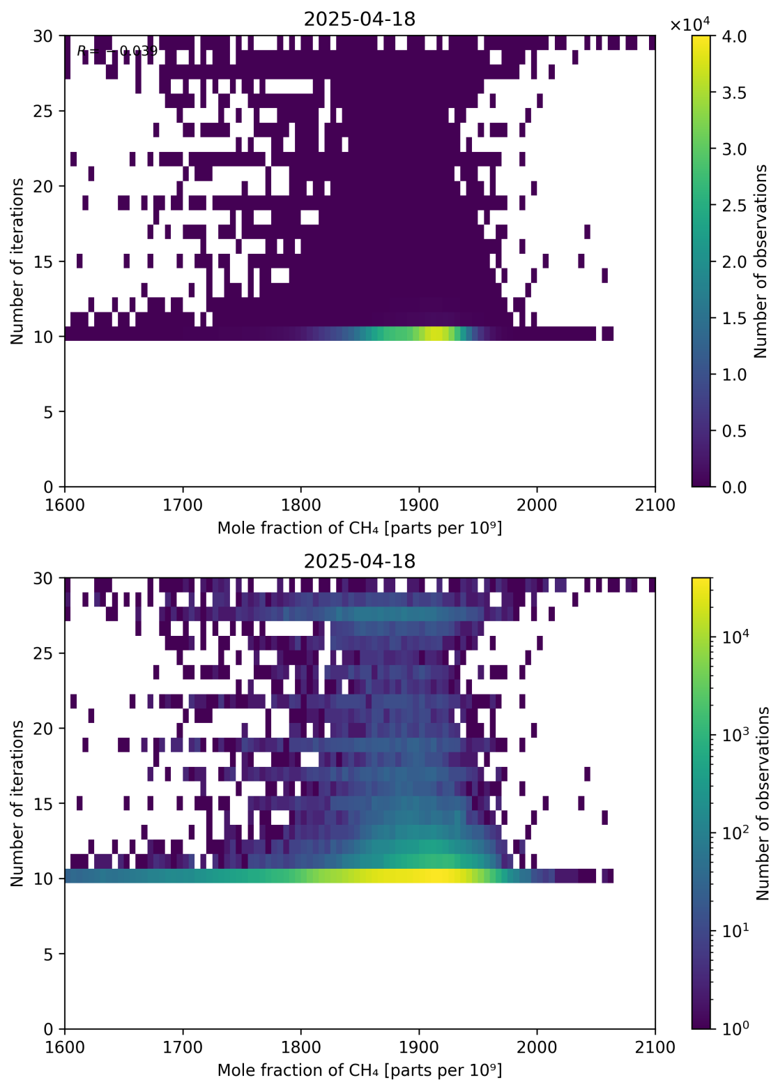
Figure 76: Scatter density plot of “Mole fraction of CH 4 ” against “Number of iterations” for 2025-04-18 to 2025-04-19.
