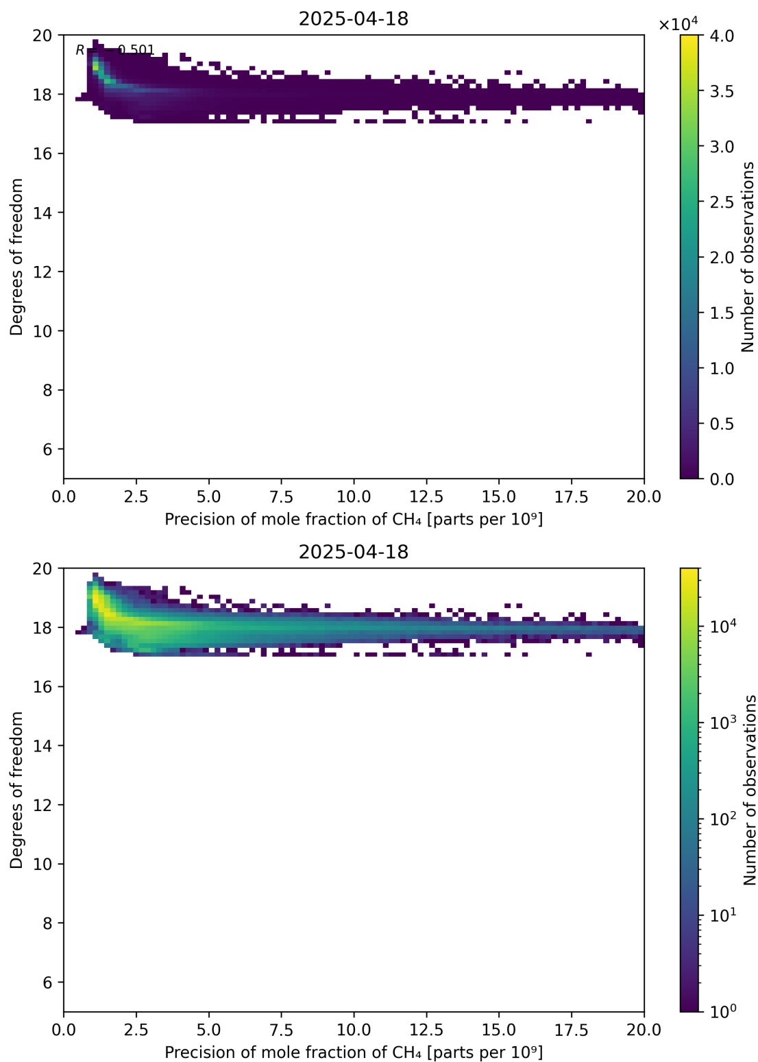
Figure 80: Scatter density plot of “Precision of mole fraction of CH 4 ” against “Degrees of freedom” for 2025-04-18 to 2025-04-19.
