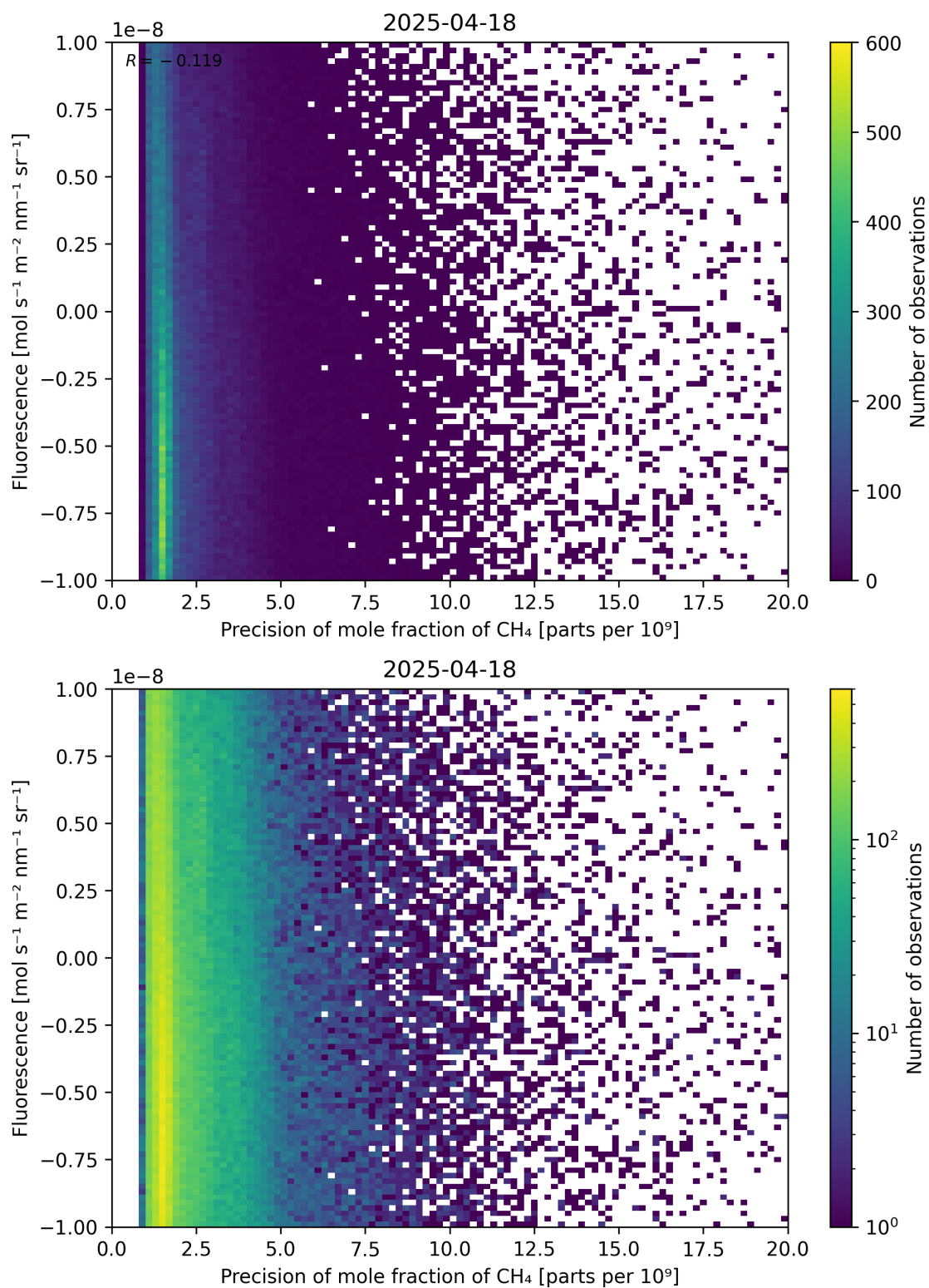
Figure 81: Scatter density plot of “Precision of mole fraction of \text{CH}_4 ” against “Fluorescence” for 2025-04-18 to 2025-04-19.
