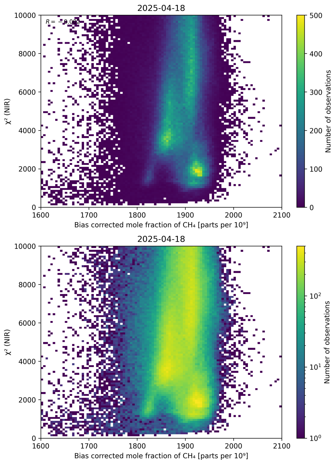
Figure 63: Scatter density plot of “Bias corrected mole fraction of CH 4 ” against “ \chi^2 (NIR)” for 2025-04-18 to 2025-04-19.
