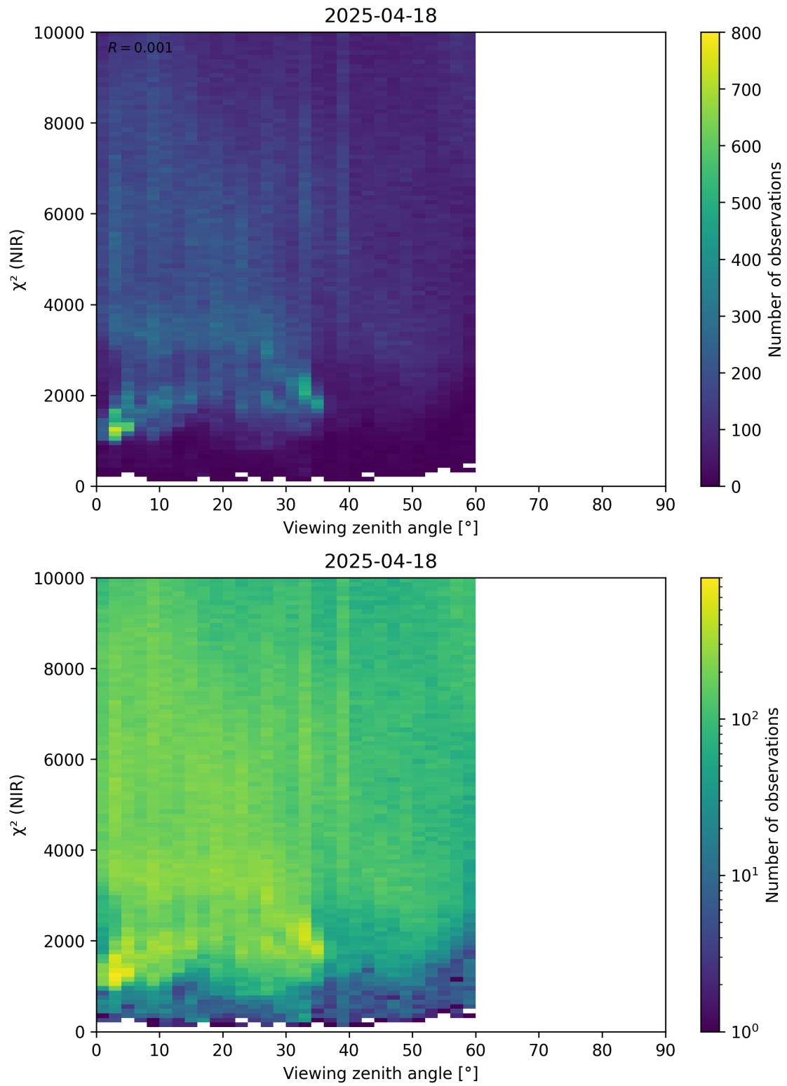
Figure 105: Scatter density plot of “Viewing zenith angle” against “ \chi^2 (NIR)” for 2025-04-18 to 2025-04-19.
