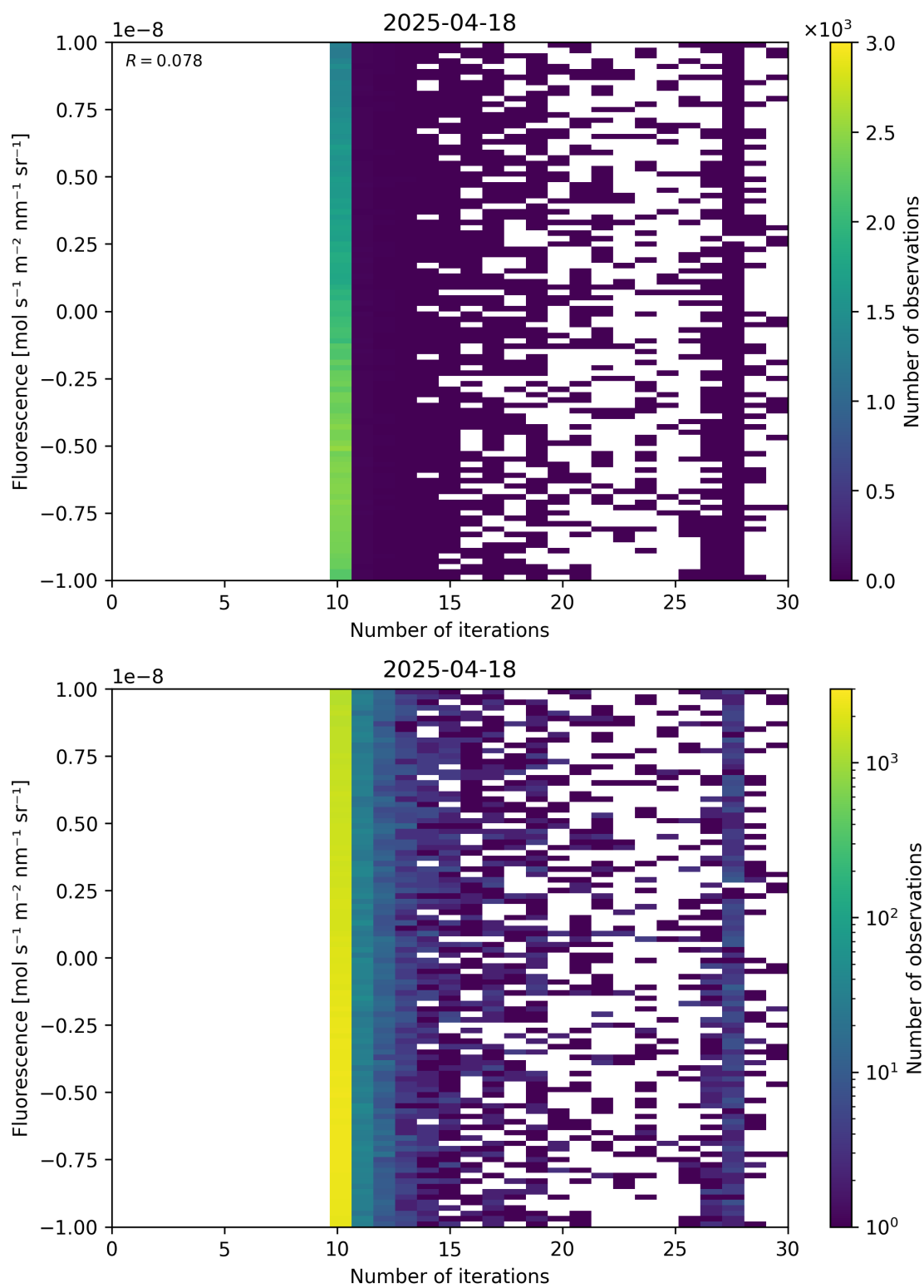
Figure 87: Scatter density plot of “Number of iterations” against “Fluorescence” for 2025-04-18 to 2025-04-19.
