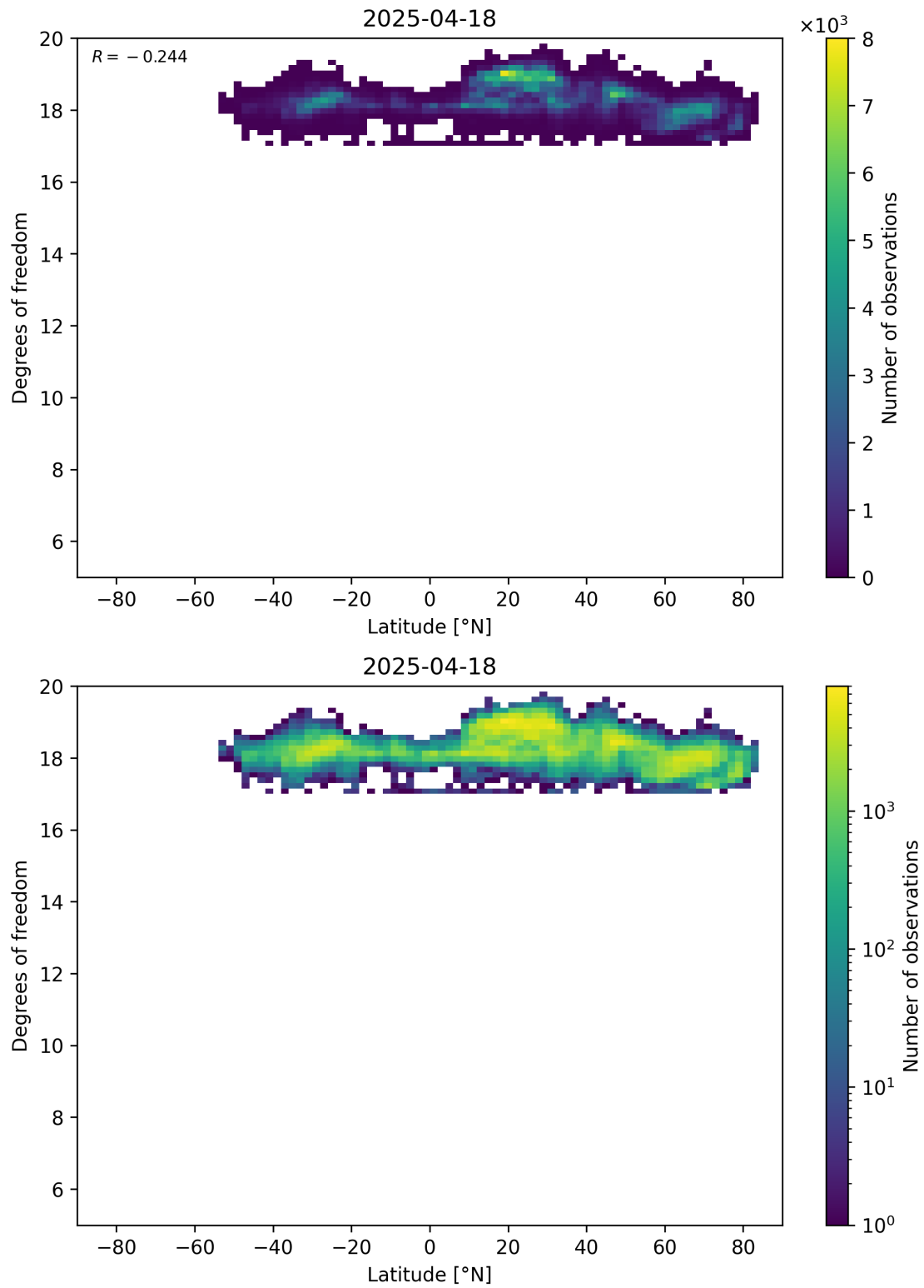
Figure 55: Scatter density plot of “Latitude” against “Degrees of freedom” for 2025-04-18 to 2025-04-19.
