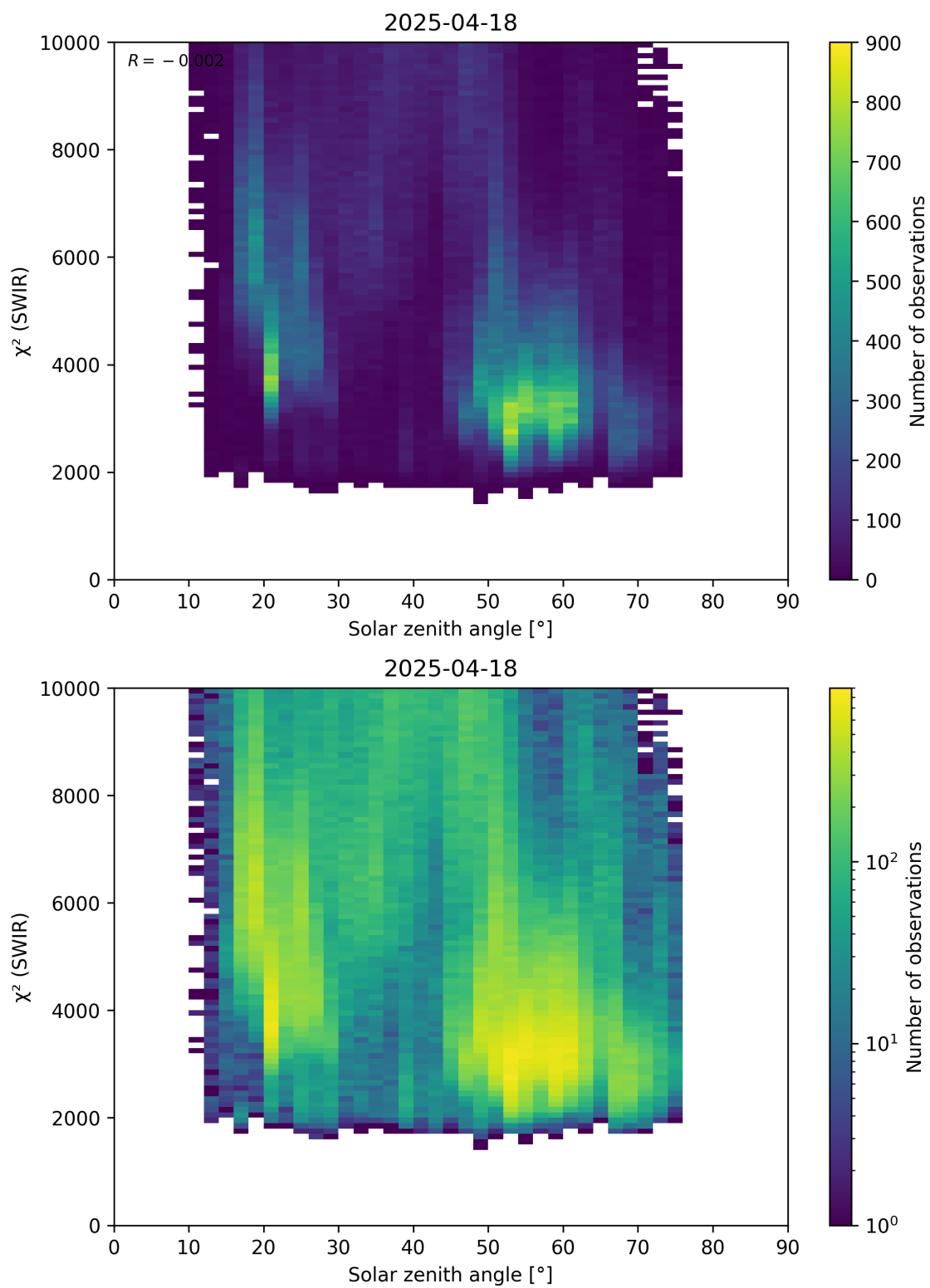
Figure 95: Scatter density plot of “Solar zenith angle” against “ \chi^2 (SWIR)” for 2025-04-18 to 2025-04-19.
