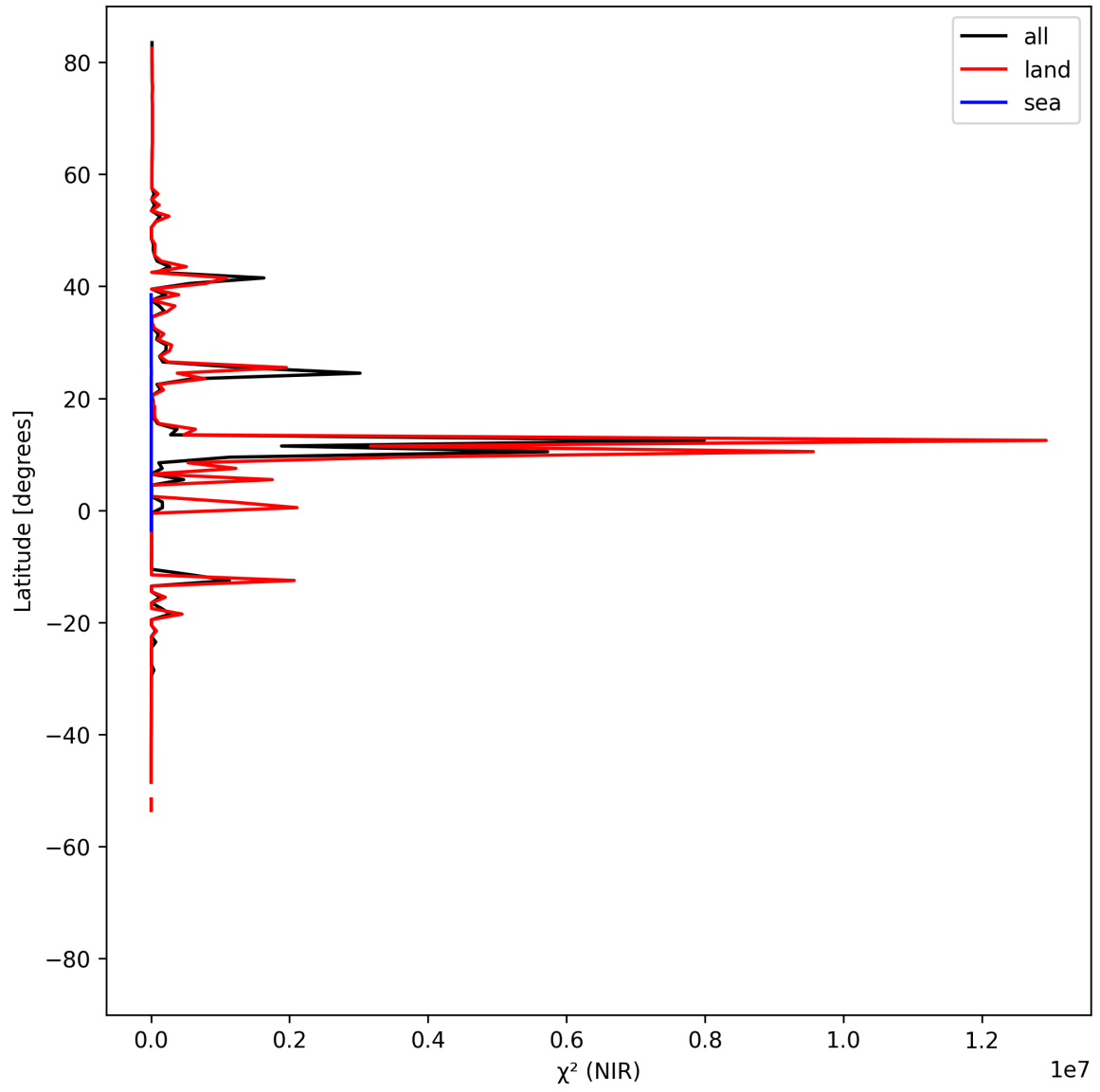
Figure 18: Zonal average of “ \chi^2 (NIR)” for 2025-04-18 to 2025-04-19.
