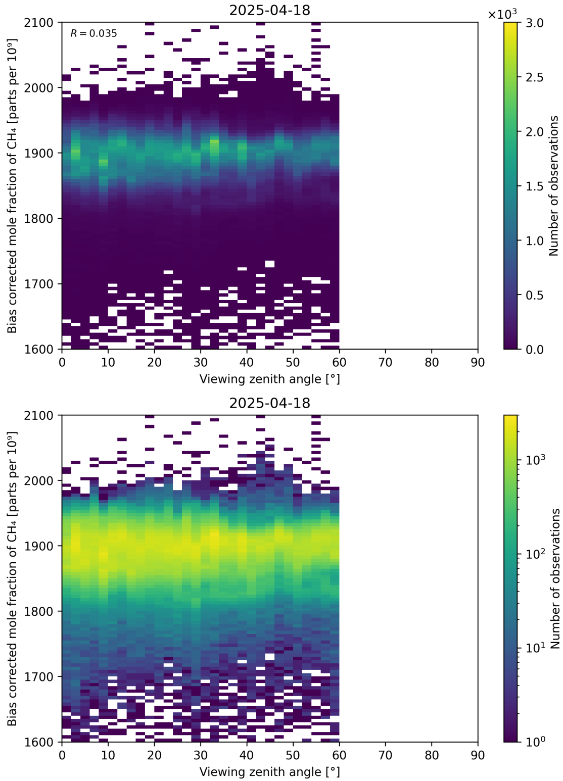
Figure 111: Scatter density plot of “Viewing zenith angle” against “Bias corrected mole fraction of CH 4 ” for 2025-04-18 to 2025-04-19.
