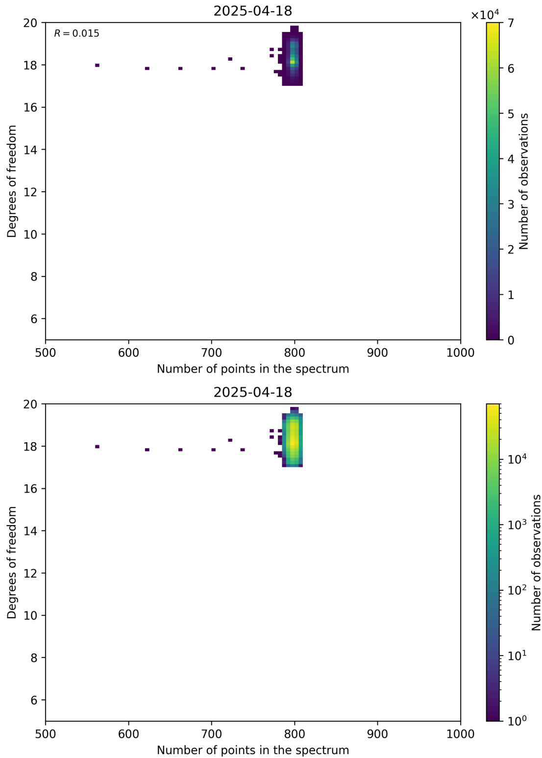
Figure 90: Scatter density plot of “Number of points in the spectrum” against “Degrees of freedom” for 2025-04-18 to 2025-04-19.
