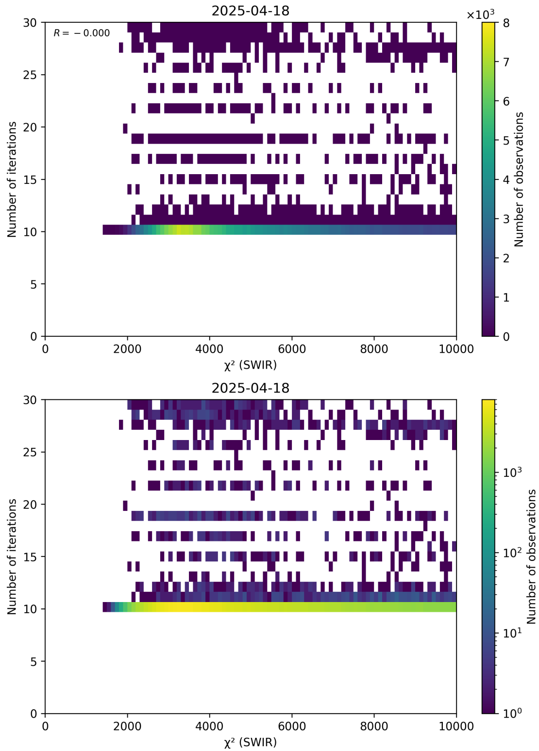
Figure 50: Scatter density plot of “ \chi^2 (SWIR)” against “Number of iterations” for 2025-04-18 to 2025-04-19.
