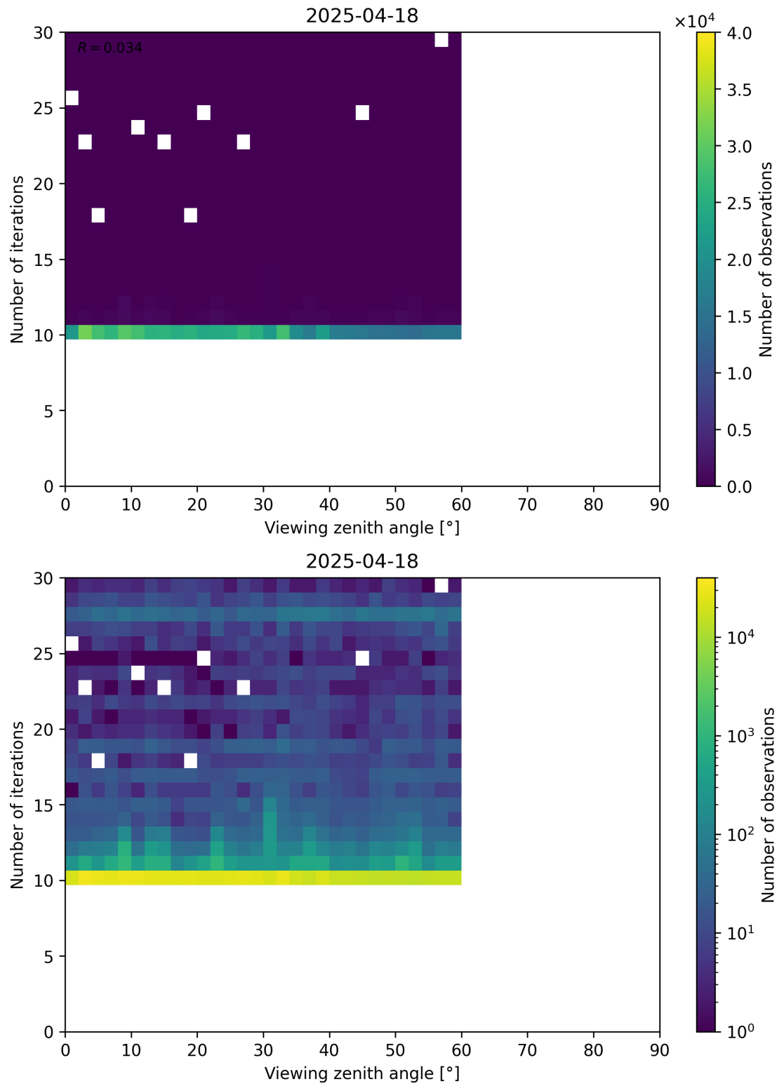
Figure 113: Scatter density plot of “Viewing zenith angle” against “Number of iterations” for 2025-04-18 to 2025-04-19.
