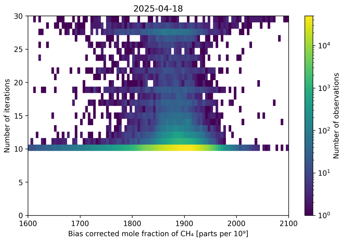
Figure 67: Scatter density plot of “Bias corrected mole fraction of CH 4 ” against “Number of iterations” for 2025-04-18 to 2025-04-19.
