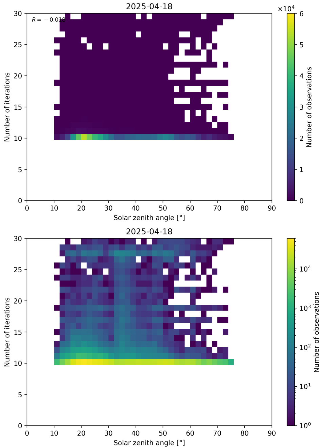
Figure 102: Scatter density plot of “Solar zenith angle” against “Number of iterations” for 2025-04-18 to 2025-04-19.
