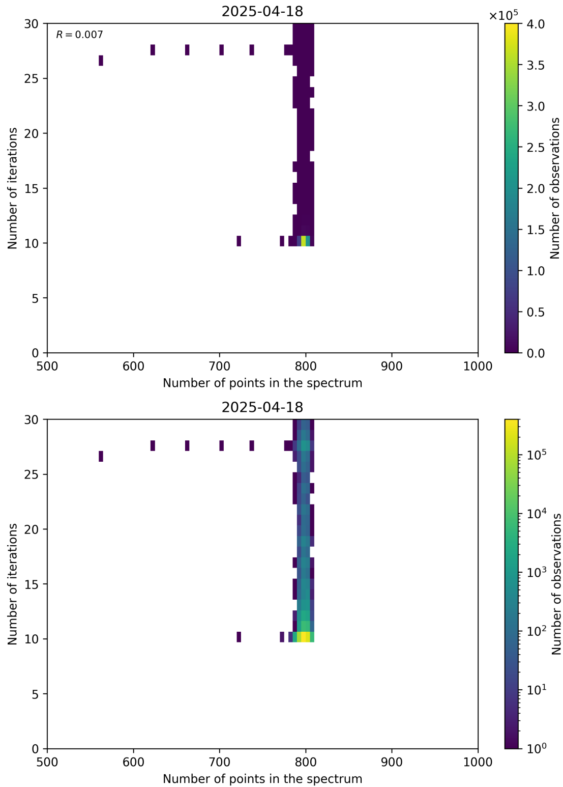
Figure 92: Scatter density plot of “Number of points in the spectrum” against “Number of iterations” for 2025-04-18 to 2025-04-19.
