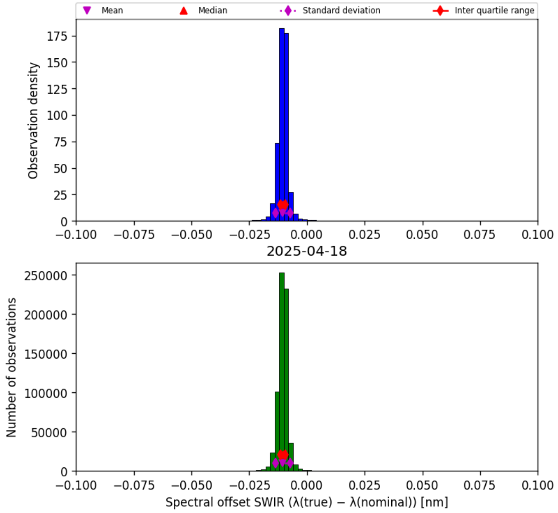
Figure 27: Histogram of “Spectral offset SWIR ( \lambda_{\text{true}} - \lambda_{\text{nominal}} )” for 2025-04-18 to 2025-04-19
