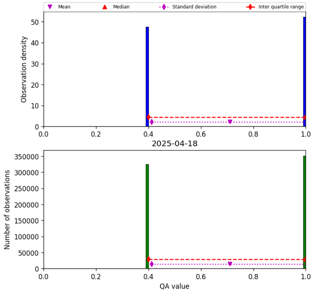
Figure 22: Histogram of “QA value” for 2025-04-18 to 2025-04-19
