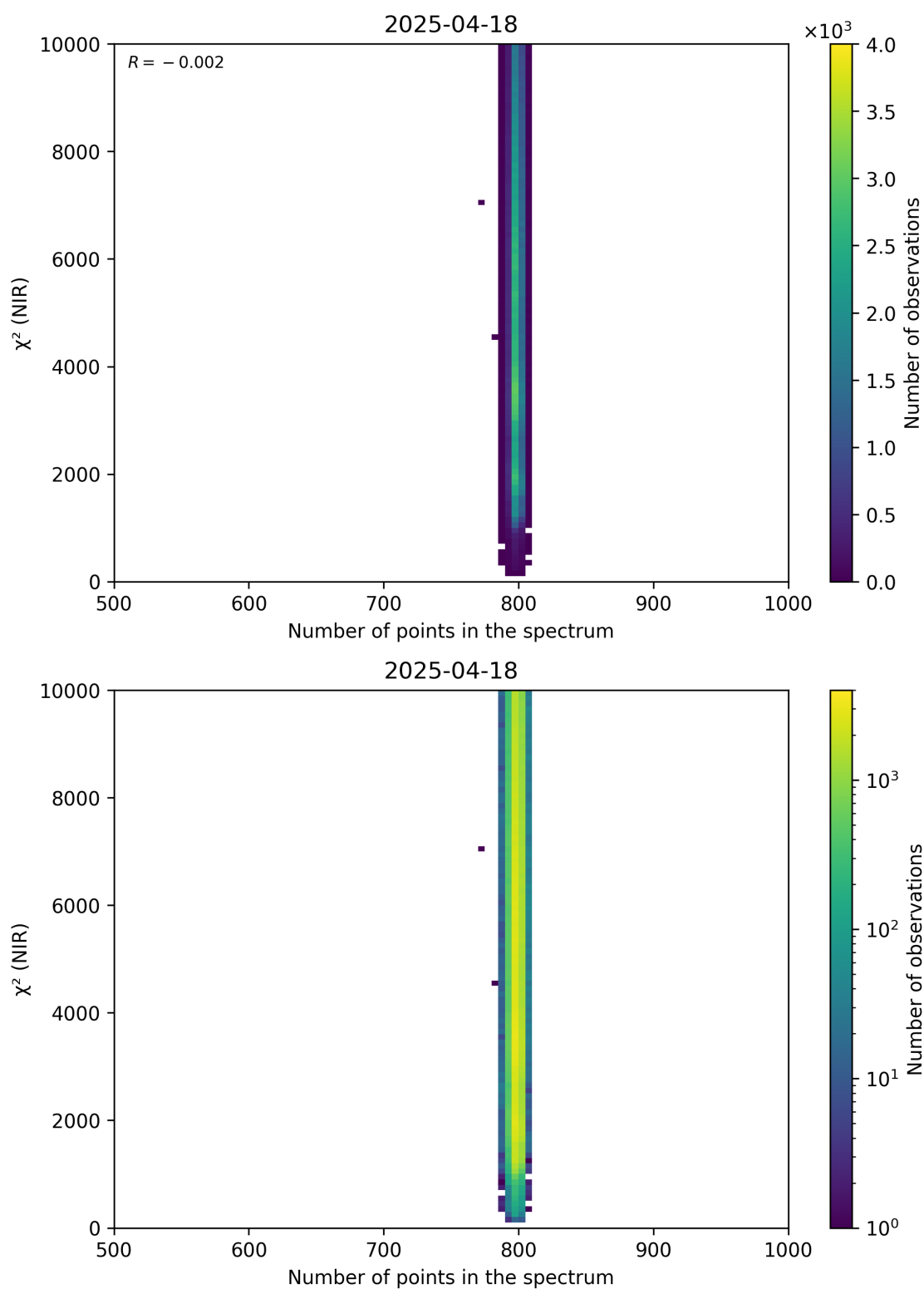
Figure 88: Scatter density plot of “Number of points in the spectrum” against “ \chi^2 (NIR)” for 2025-04-18 to 2025-04-19.
