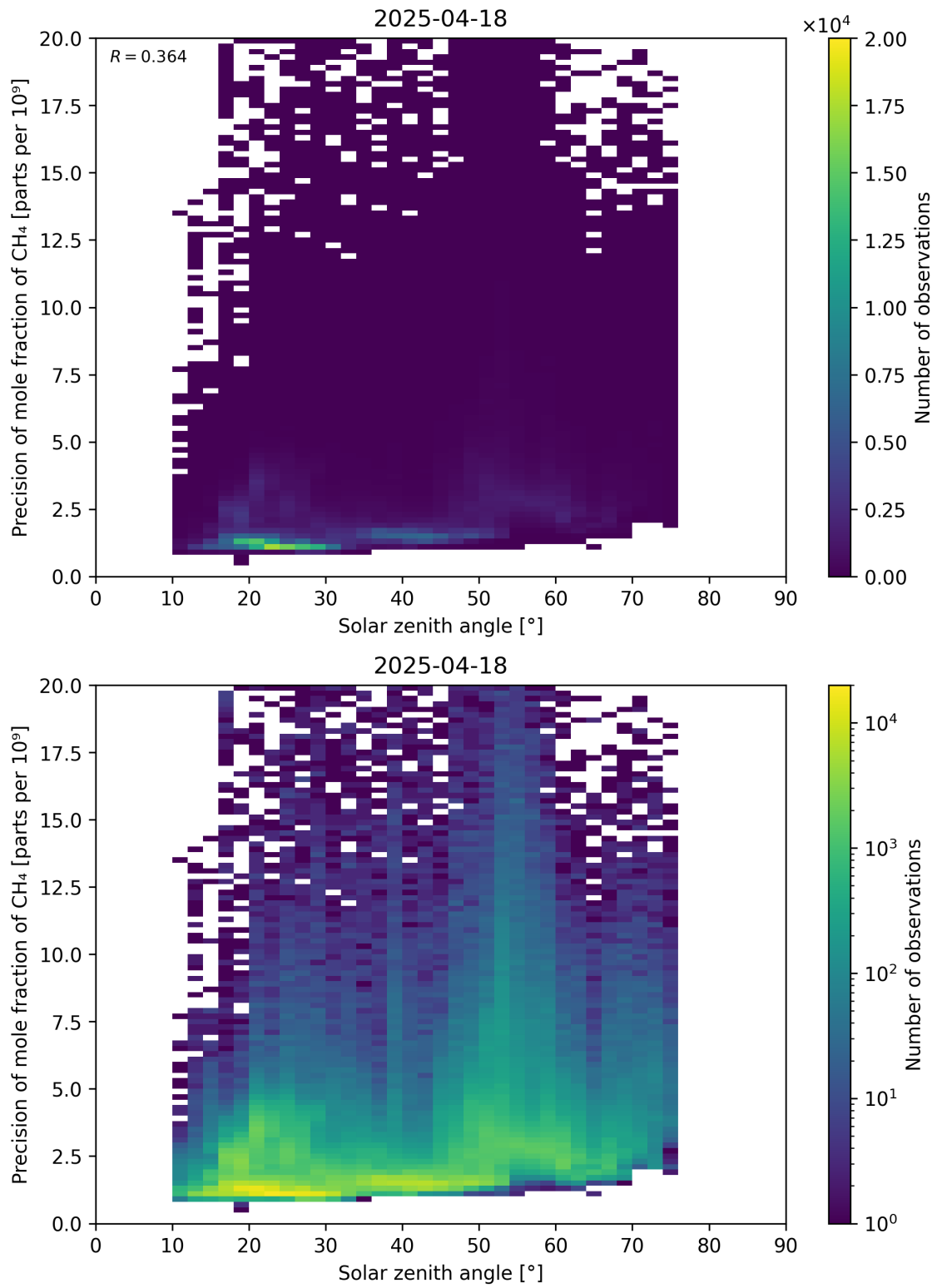
Figure 101: Scatter density plot of “Solar zenith angle” against “Precision of mole fraction of CH 4 ” for 2025-04-18 to 2025-04-19.
