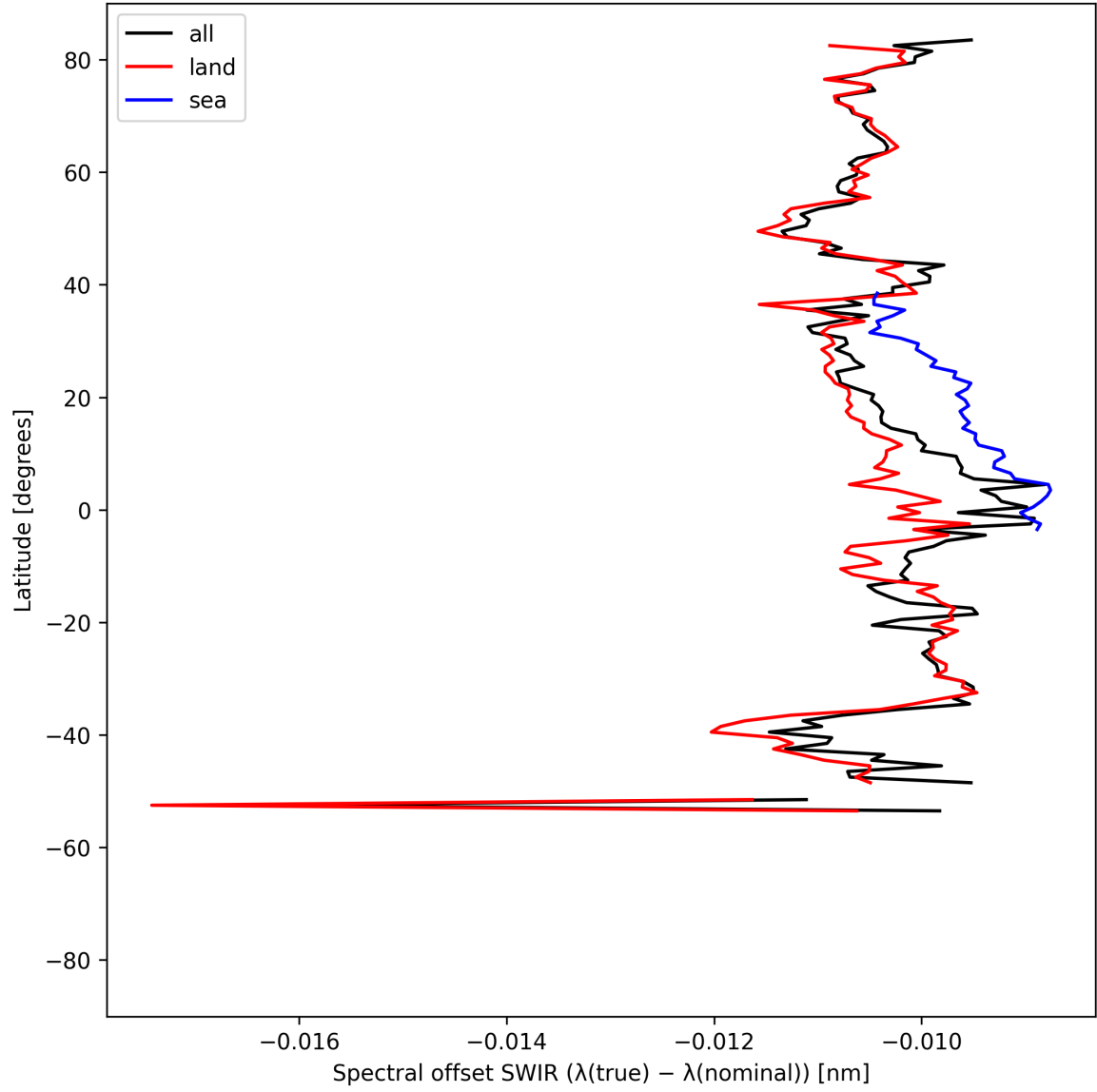
Figure 16: Zonal average of “Spectral offset SWIR ( \lambda_{\text{true}} - \lambda_{\text{nominal}} )” for 2025-04-18 to 2025-04-19.
