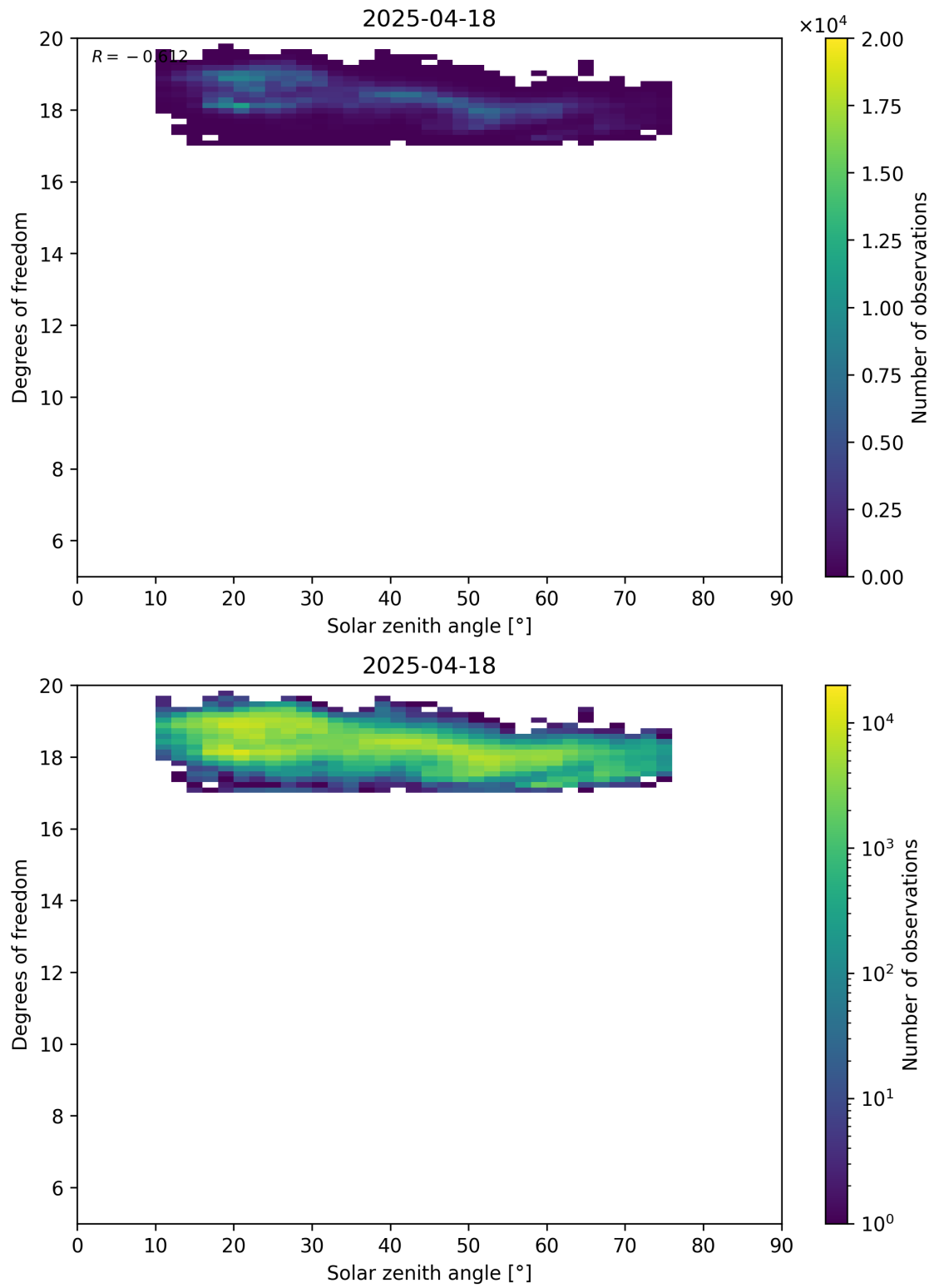
Figure 96: Scatter density plot of “Solar zenith angle” against “Degrees of freedom” for 2025-04-18 to 2025-04-19.
