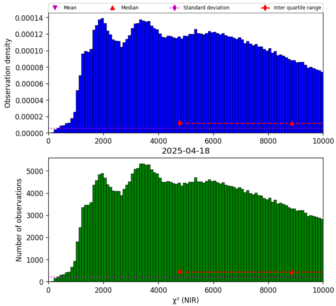
Figure 29: Histogram of “ \chi^2 (NIR)” for 2025-04-18 to 2025-04-19
