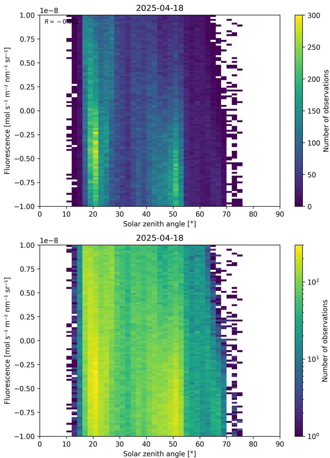
Figure 97: Scatter density plot of “Solar zenith angle” against “Fluorescence” for 2025-04-18 to 2025-04-19.
