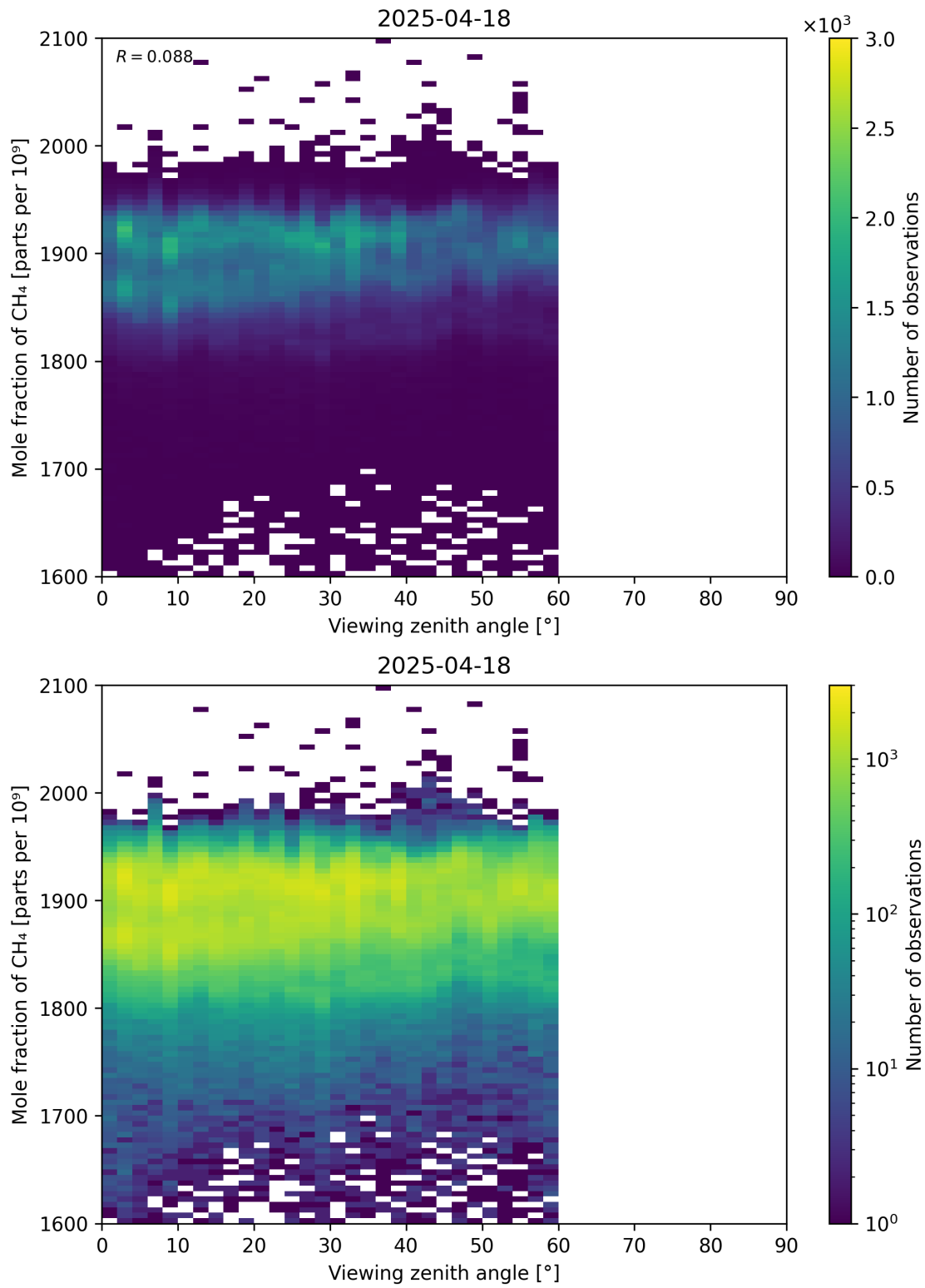
Figure 110: Scatter density plot of “Viewing zenith angle” against “Mole fraction of CH 4 ” for 2025-04-18 to 2025-04-19.
