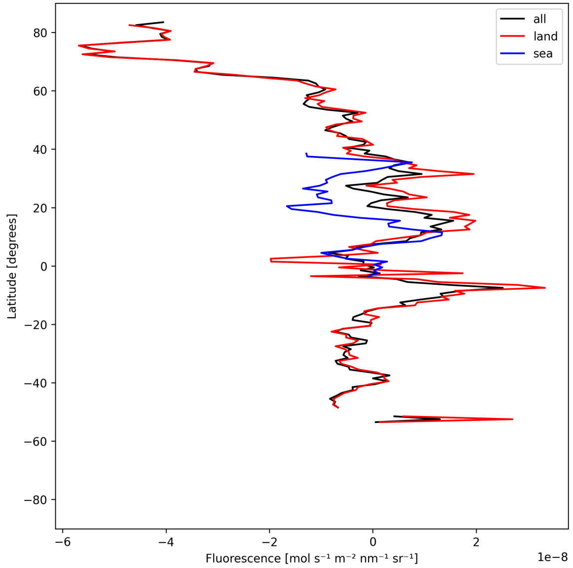
Figure 21: Zonal average of “Fluorescence” for 2025-04-18 to 2025-04-19.
