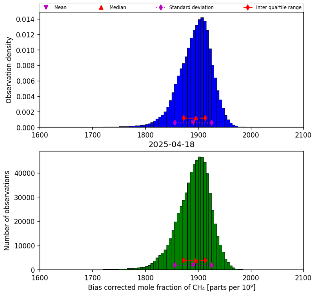
Figure 25: Histogram of “Bias corrected mole fraction of CH 4 ” for 2025-04-18 to 2025-04-19
