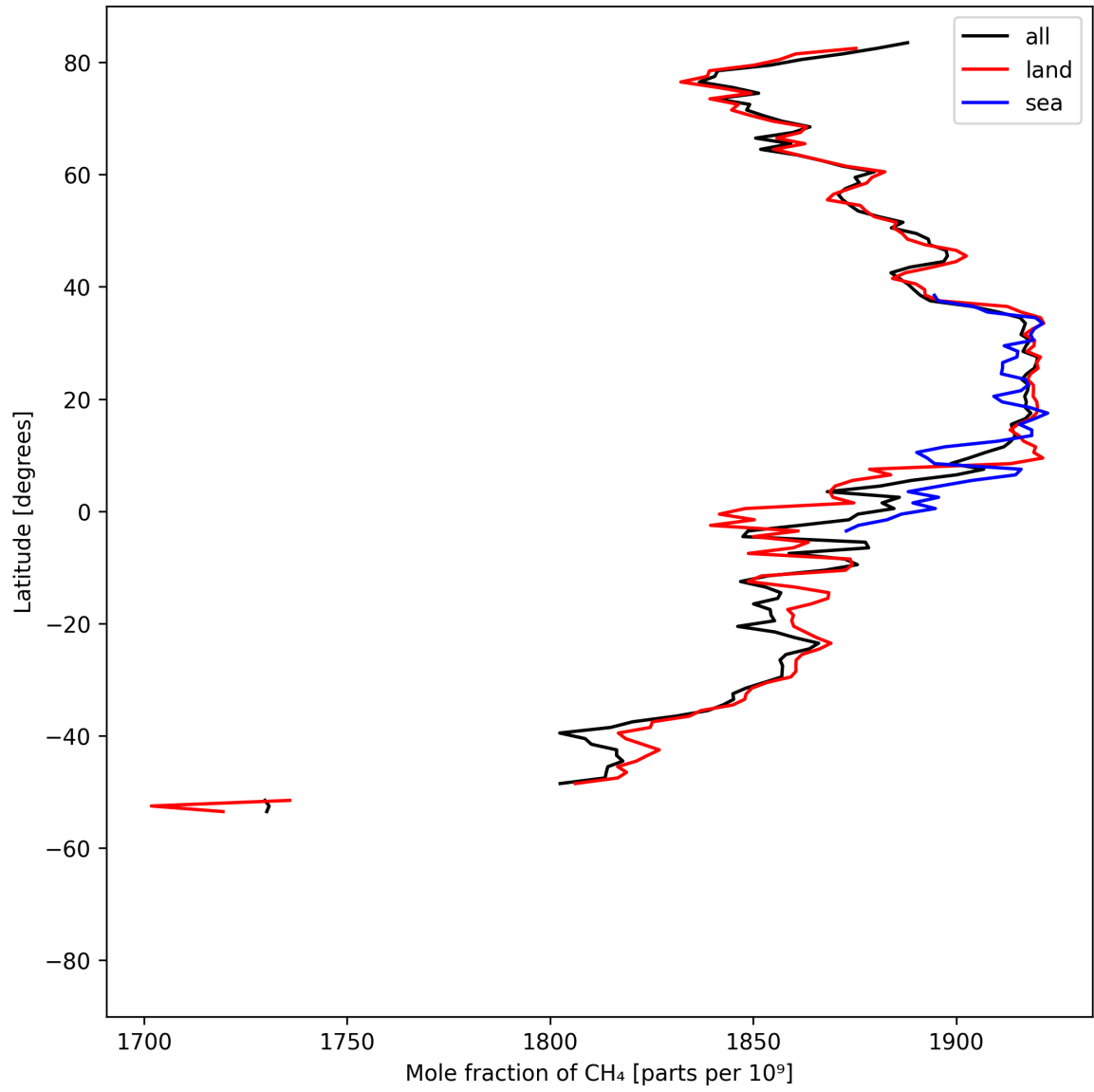
Figure 12: Zonal average of “Mole fraction of \text{CH}_4 ” for 2025-04-18 to 2025-04-19.
