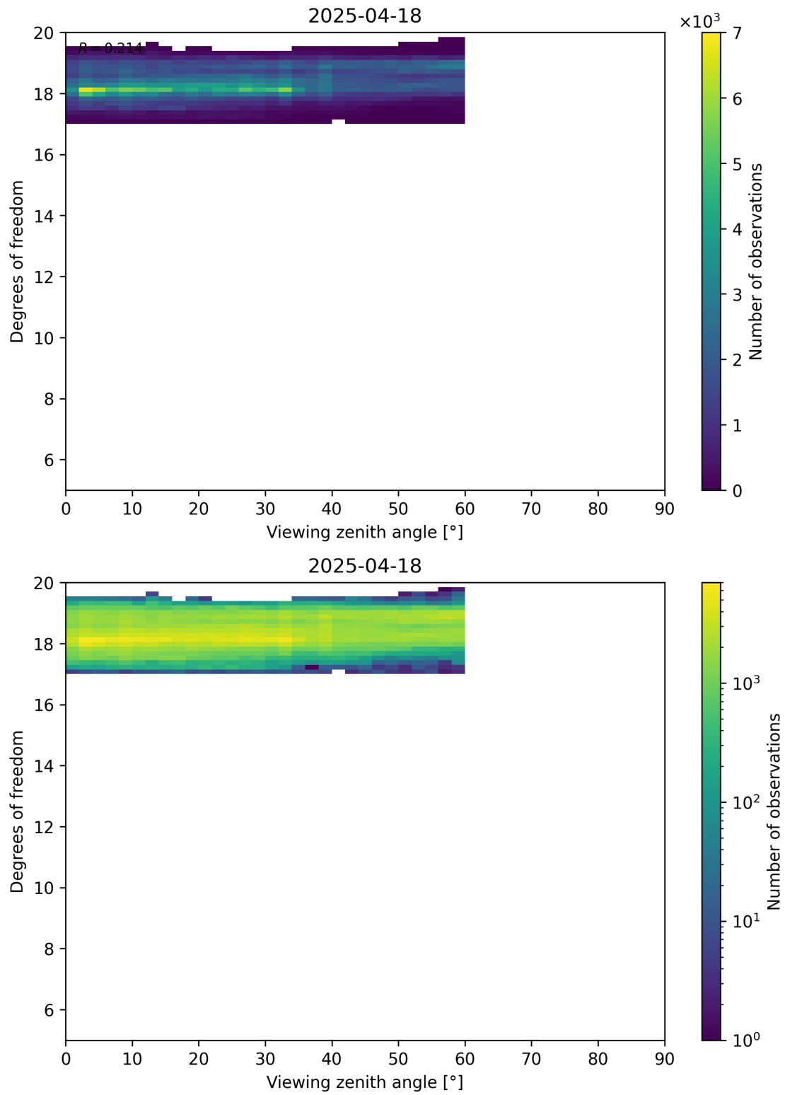
Figure 107: Scatter density plot of “Viewing zenith angle” against “Degrees of freedom” for 2025-04-18 to 2025-04-19.
