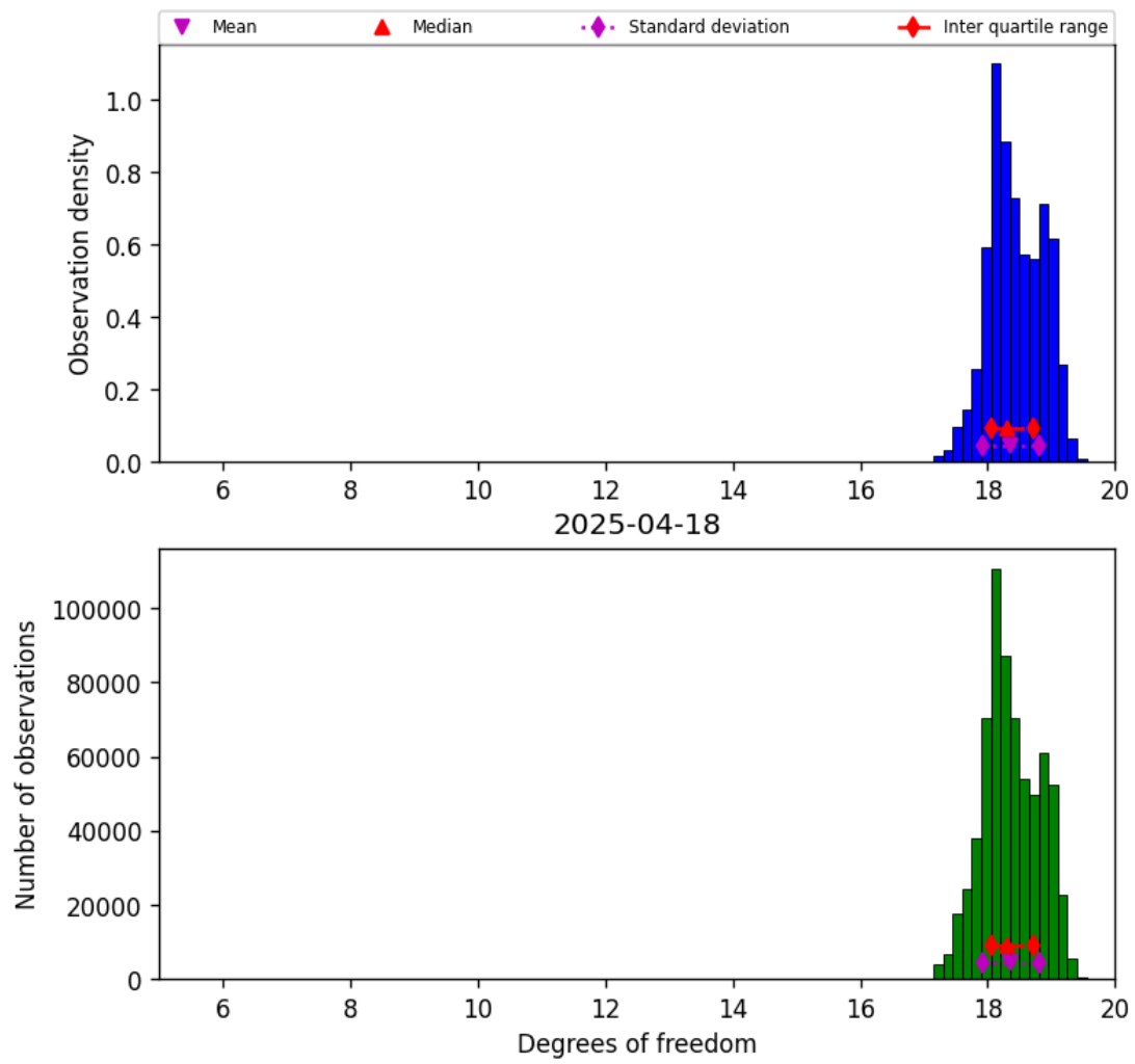
Figure 30: Histogram of “Degrees of freedom” for 2025-04-18 to 2025-04-19
