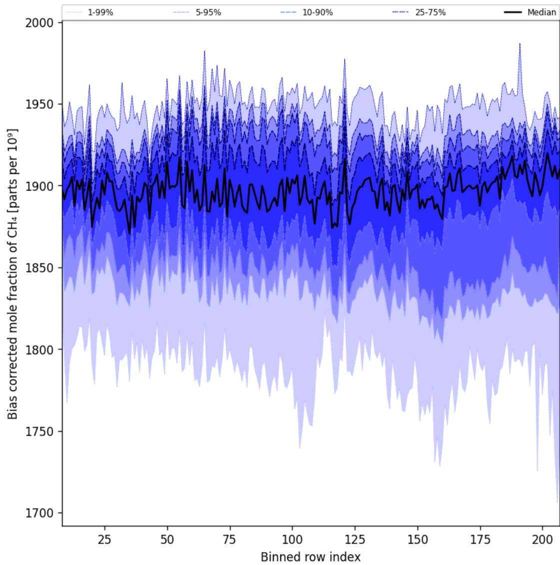
Figure 36: Along track statistics of “Bias corrected mole fraction of CH 4 ” for 2025-04-18 to 2025-04-19
