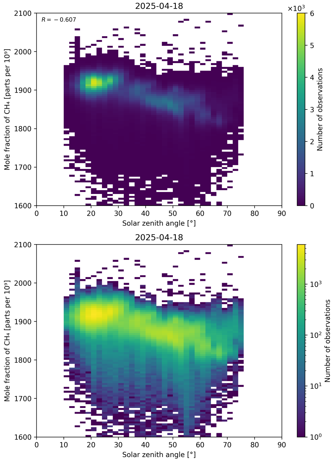
Figure 99: Scatter density plot of “Solar zenith angle” against “Mole fraction of CH 4 ” for 2025-04-18 to 2025-04-19.
