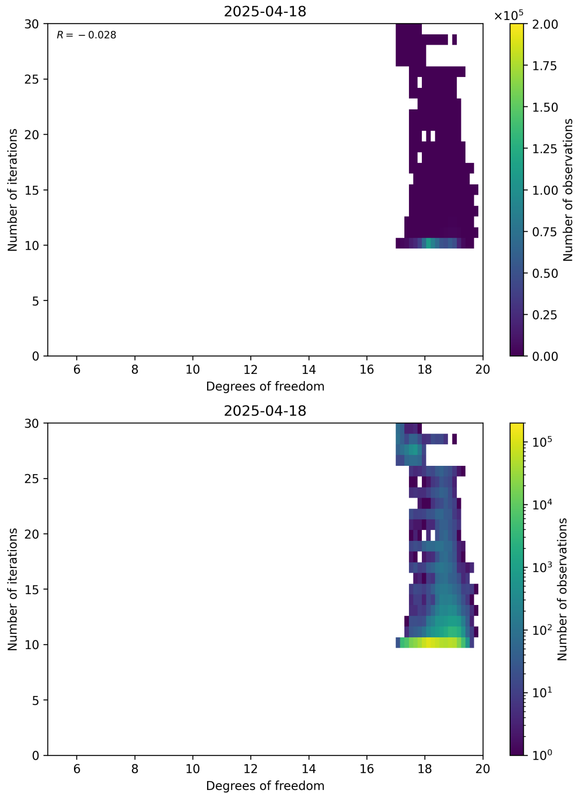
Figure 52: Scatter density plot of “Degrees of freedom” against “Number of iterations” for 2025-04-18 to 2025-04-19.
