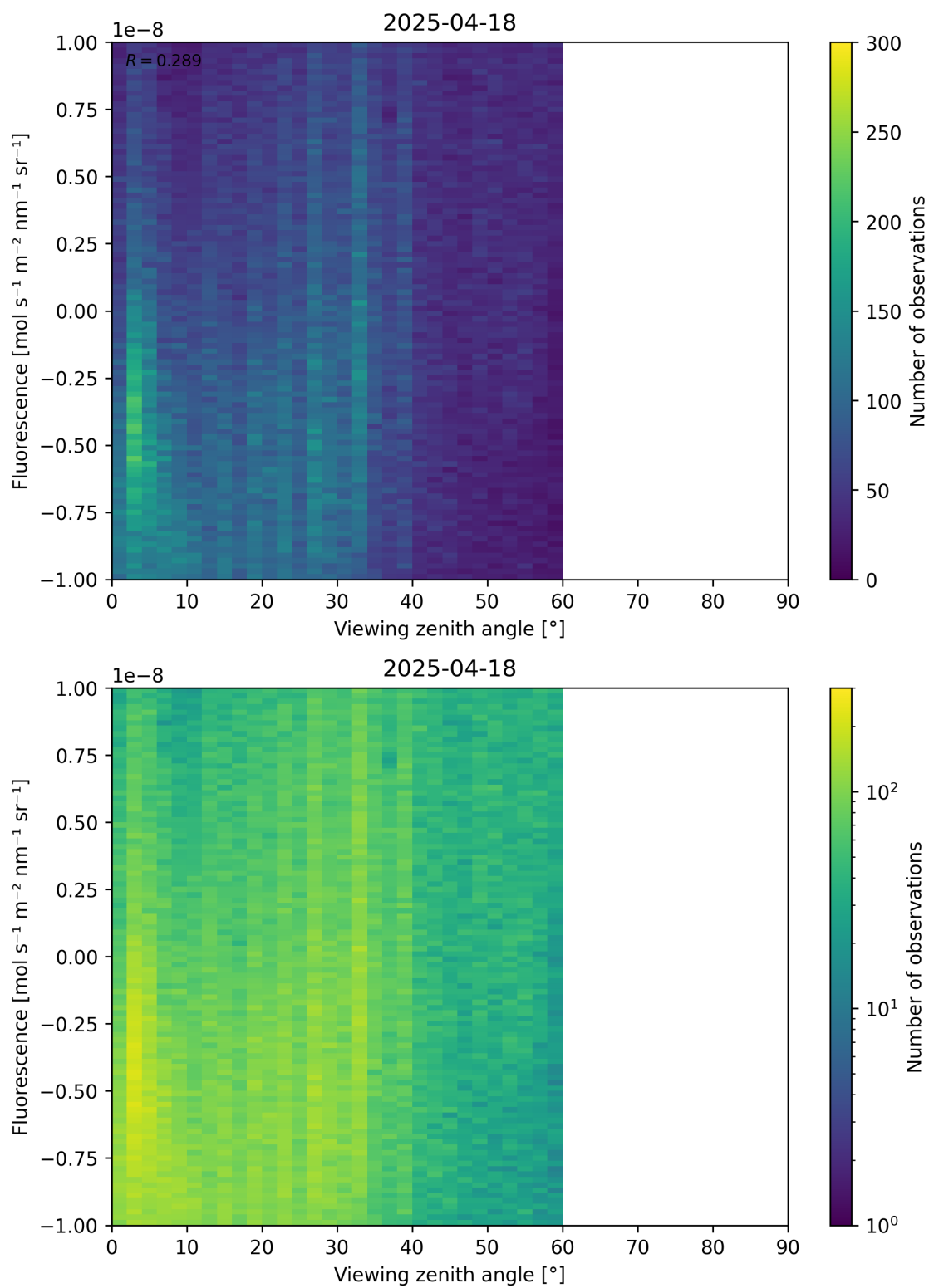
Figure 108: Scatter density plot of “Viewing zenith angle” against “Fluorescence” for 2025-04-18 to 2025-04-19.
