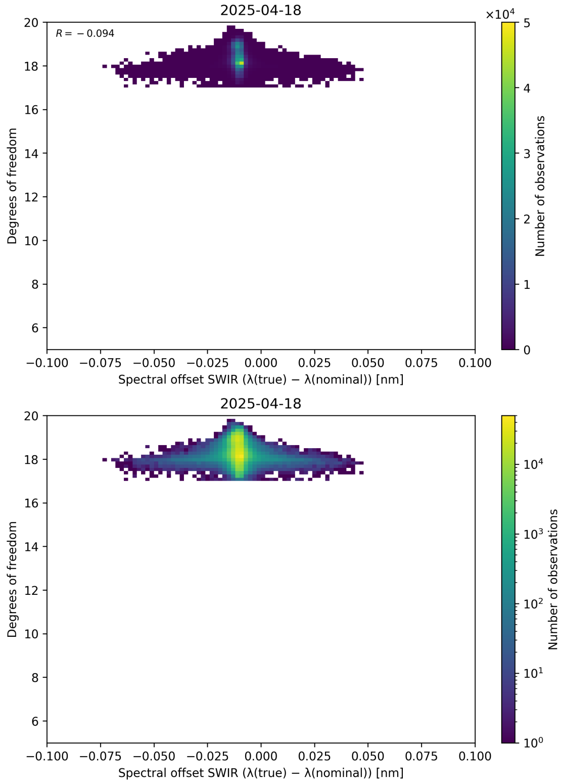
Figure 119: Scatter density plot of “Spectral offset SWIR ( \lambda_{\text{true}} - \lambda_{\text{nominal}} )” against “Degrees of freedom” for 2025-04-18 to 2025-04-19.
