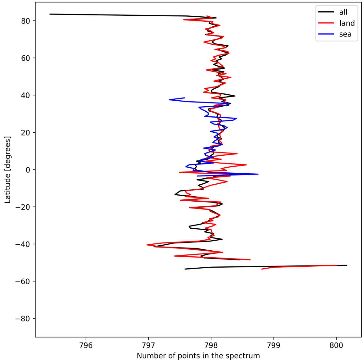
Figure 15: Zonal average of “Number of points in the spectrum” for 2025-04-18 to 2025-04-19.
