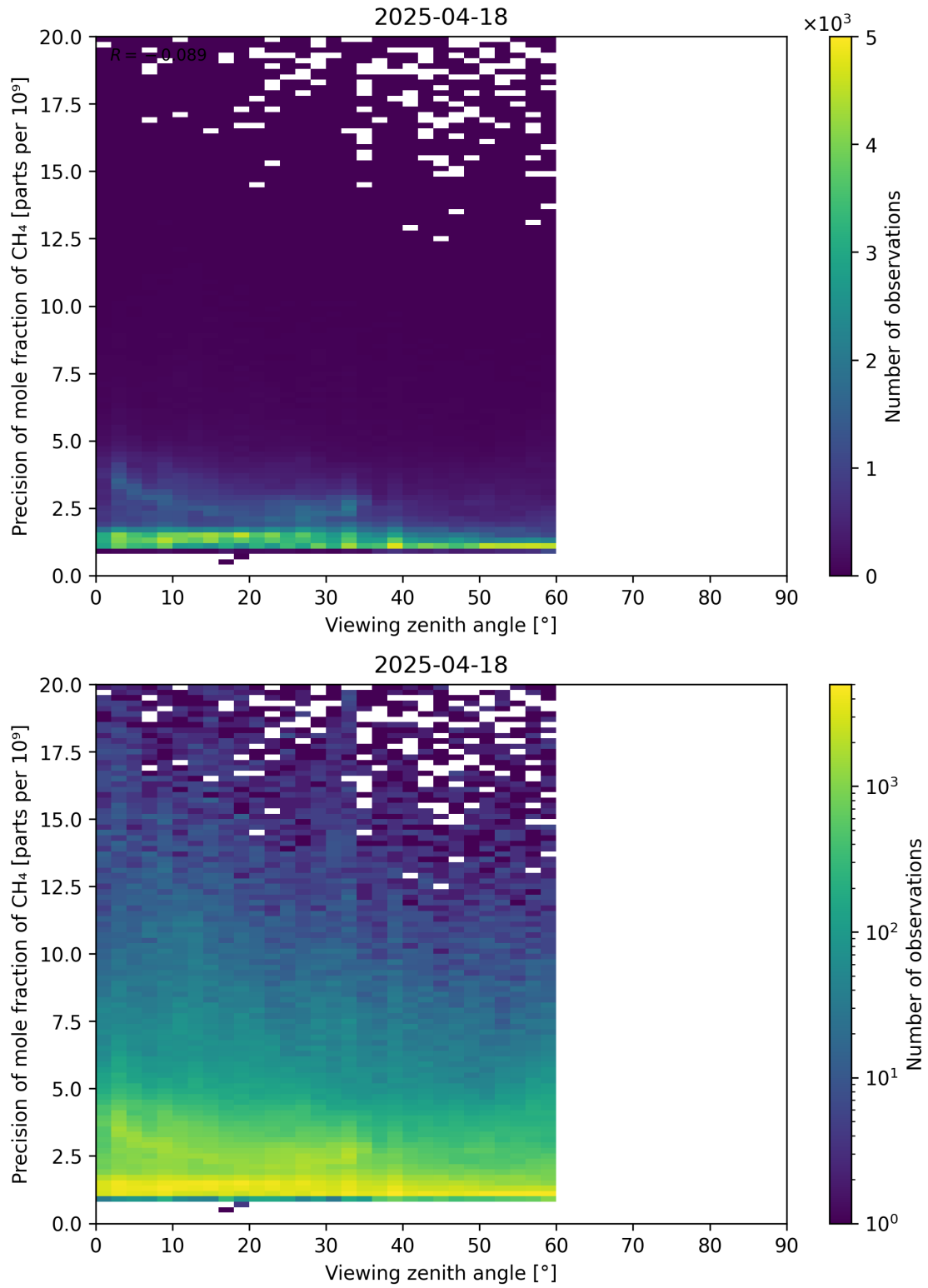
Figure 112: Scatter density plot of “Viewing zenith angle” against “Precision of mole fraction of CH 4 ” for 2025-04-18 to 2025-04-19.
