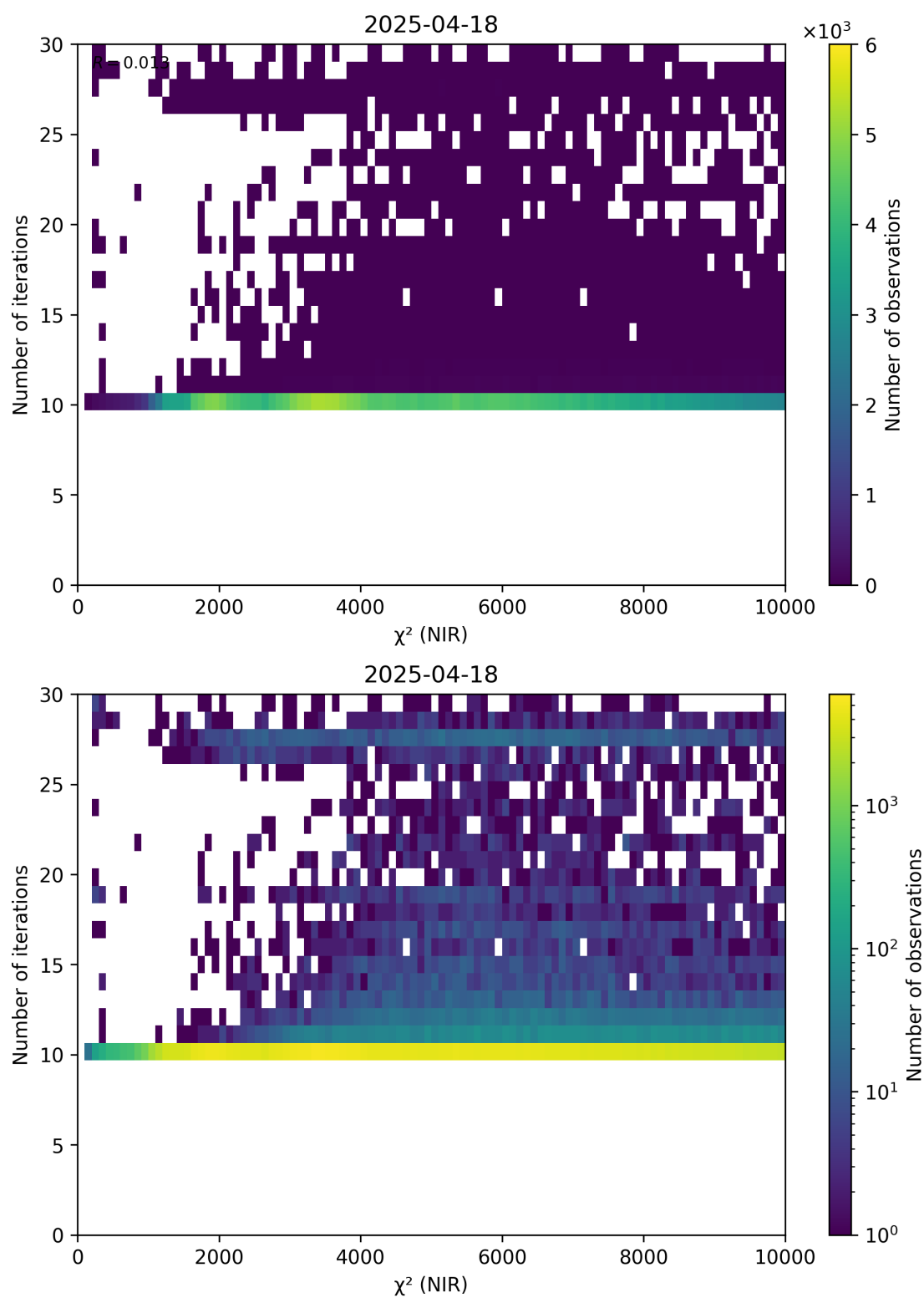
Figure 46: Scatter density plot of “ \chi^2 (NIR)” against “Number of iterations” for 2025-04-18 to 2025-04-19.
