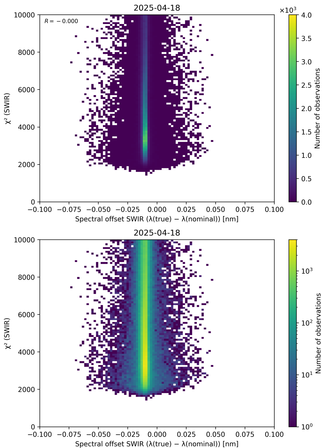
Figure 118: Scatter density plot of “Spectral offset SWIR ( \lambda_{\text{true}} - \lambda_{\text{nominal}} )” against “ \chi^2 (SWIR)” for 2025-04-18 to 2025-04-19.
