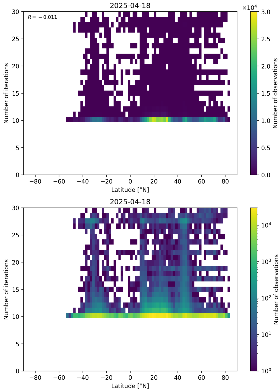
Figure 60: Scatter density plot of “Latitude” against “Number of iterations” for 2025-04-18 to 2025-04-19.
