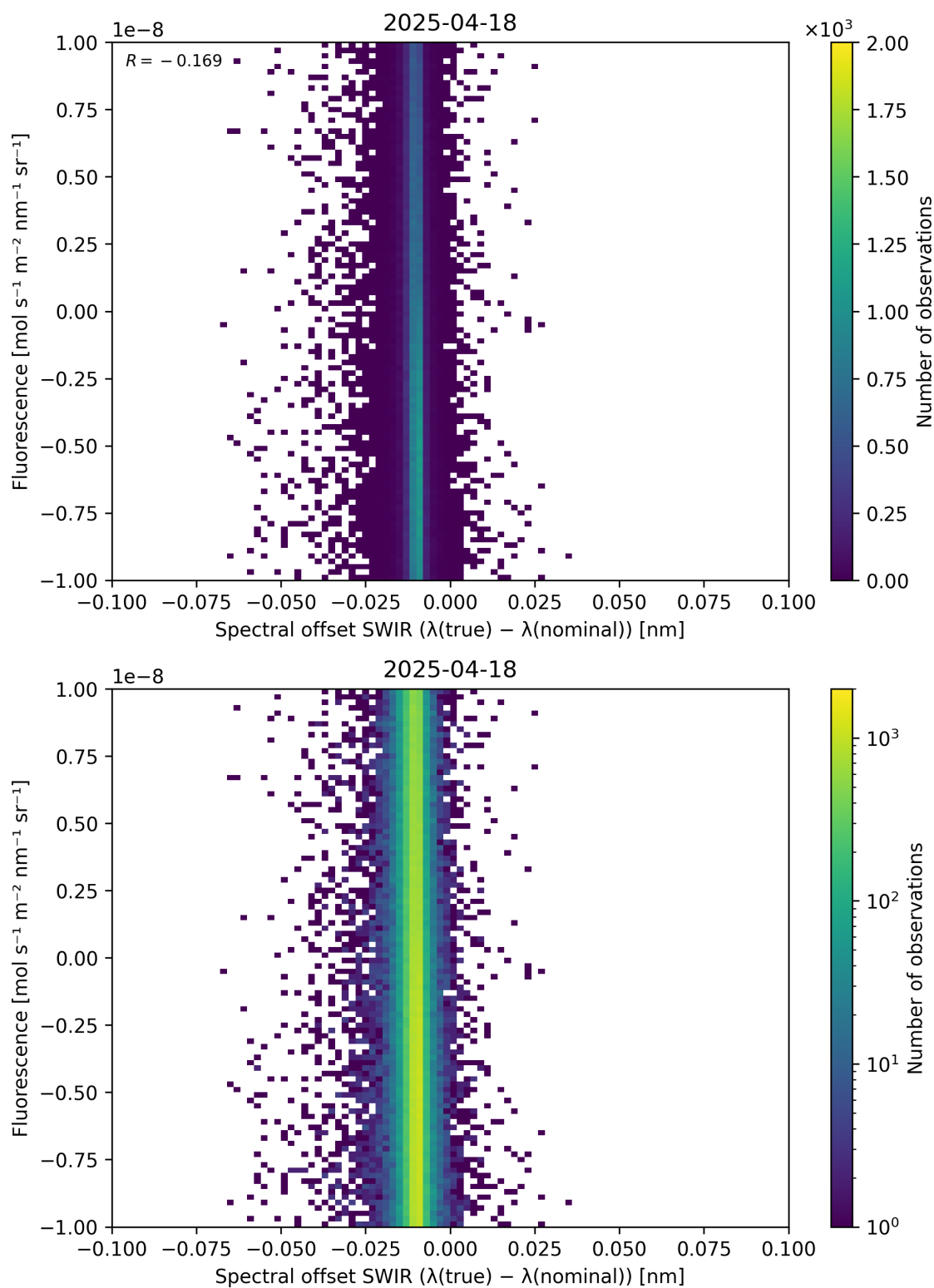
Figure 120: Scatter density plot of “Spectral offset SWIR ( \lambda_{\text{true}} - \lambda_{\text{nominal}} )” against “Fluorescence” for 2025-04-18 to 2025-04-19.
