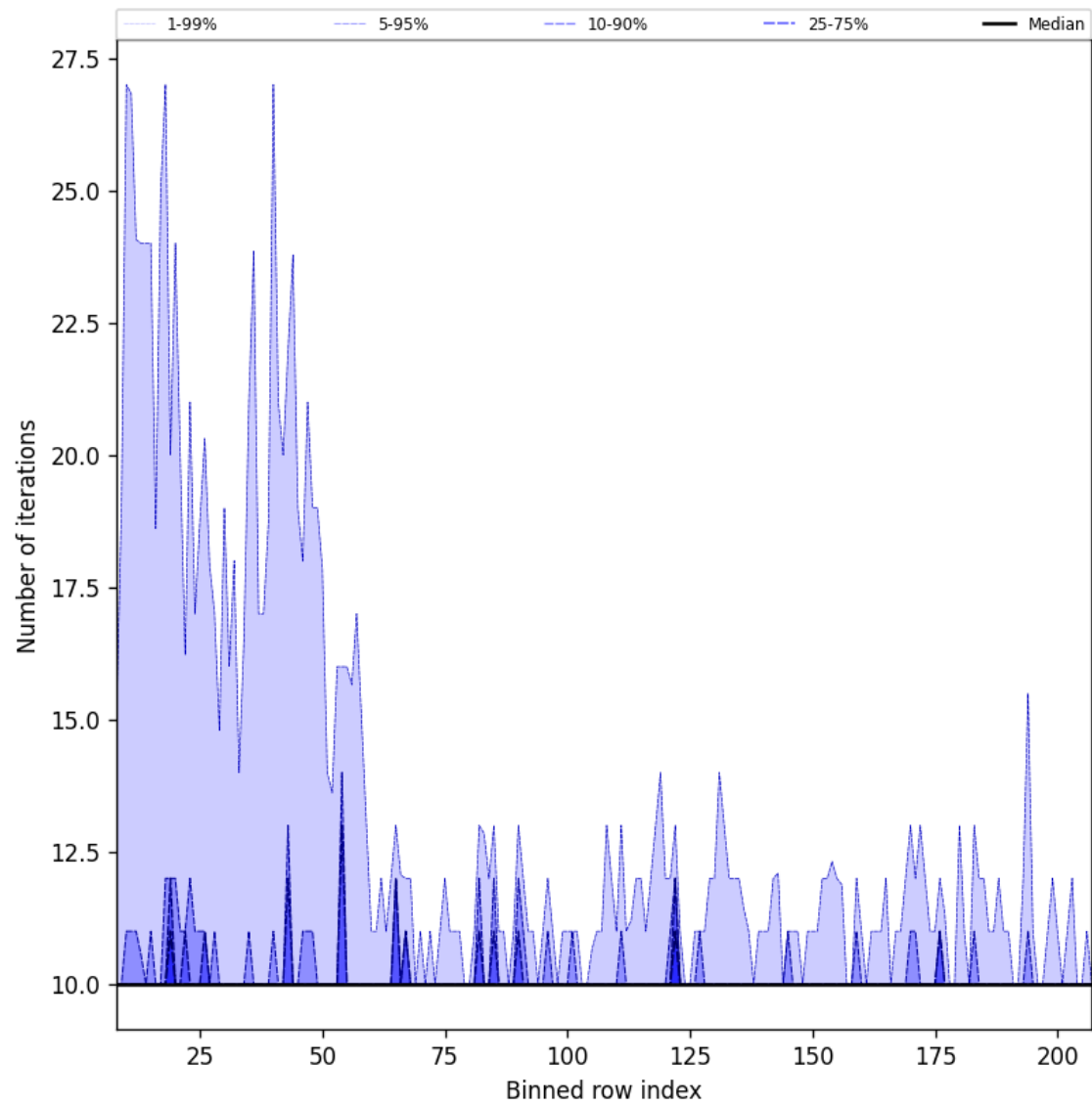
Figure 42: Along track statistics of “Number of iterations” for 2025-04-18 to 2025-04-19
