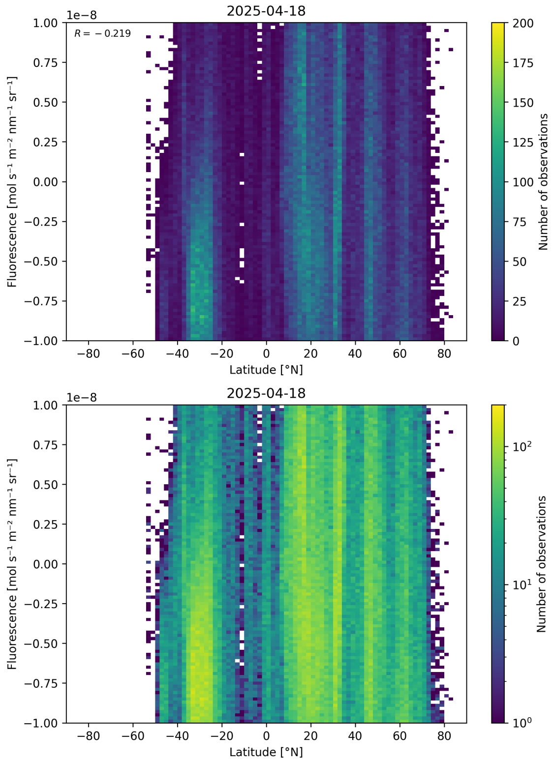
Figure 56: Scatter density plot of “Latitude” against “Fluorescence” for 2025-04-18 to 2025-04-19.
