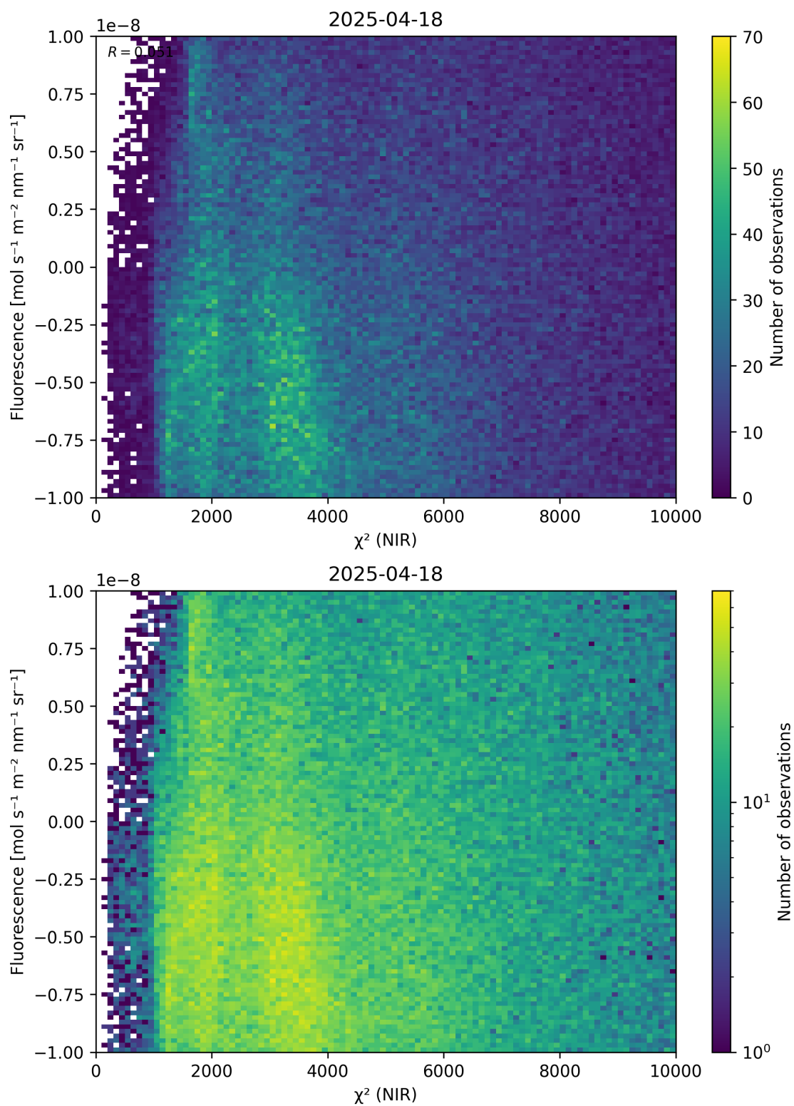
Figure 45: Scatter density plot of “ \chi^2 (NIR)” against “Fluorescence” for 2025-04-18 to 2025-04-19.
