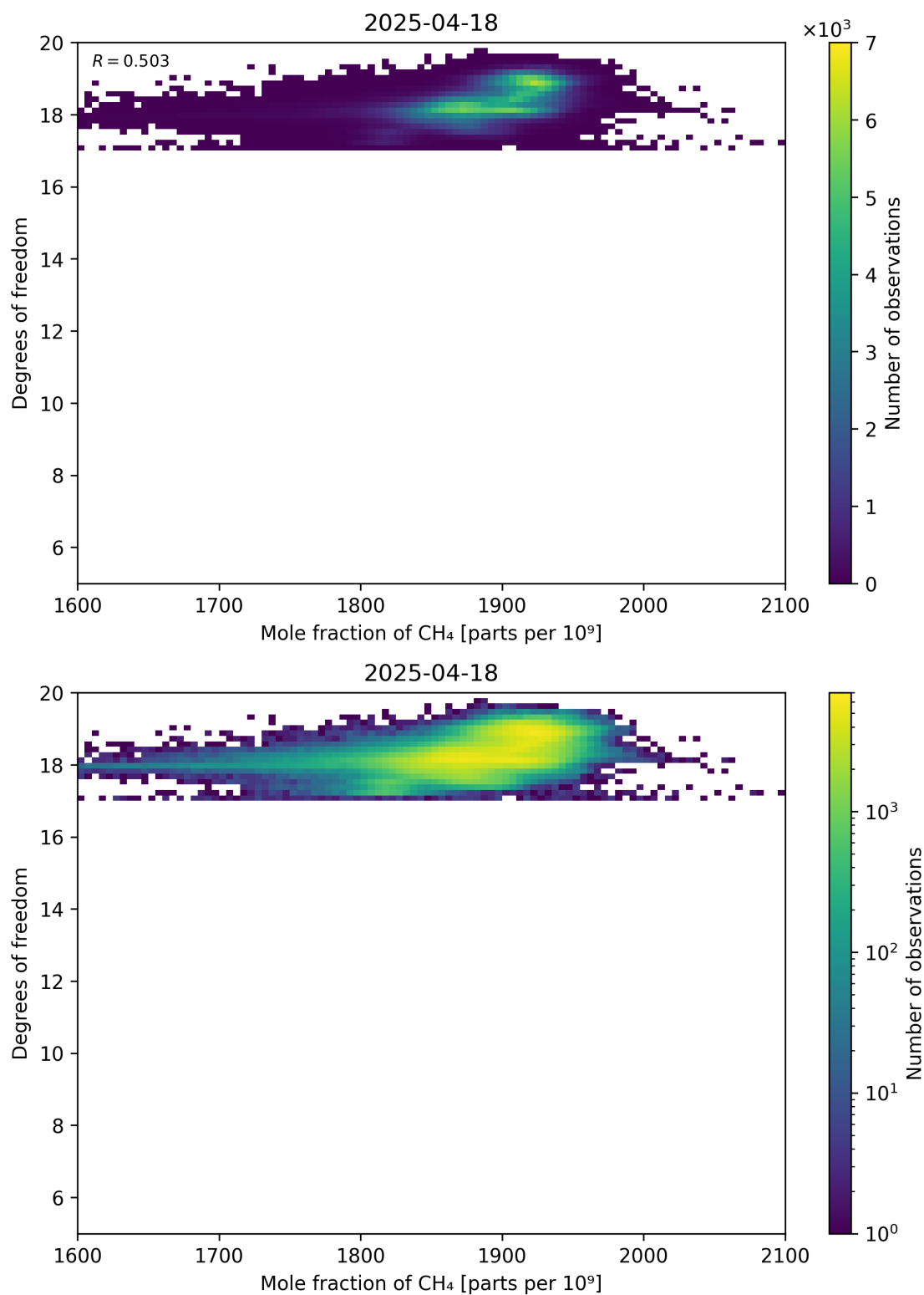
Figure 72: Scatter density plot of “Mole fraction of CH 4 ” against “Degrees of freedom” for 2025-04-18 to 2025-04-19.
