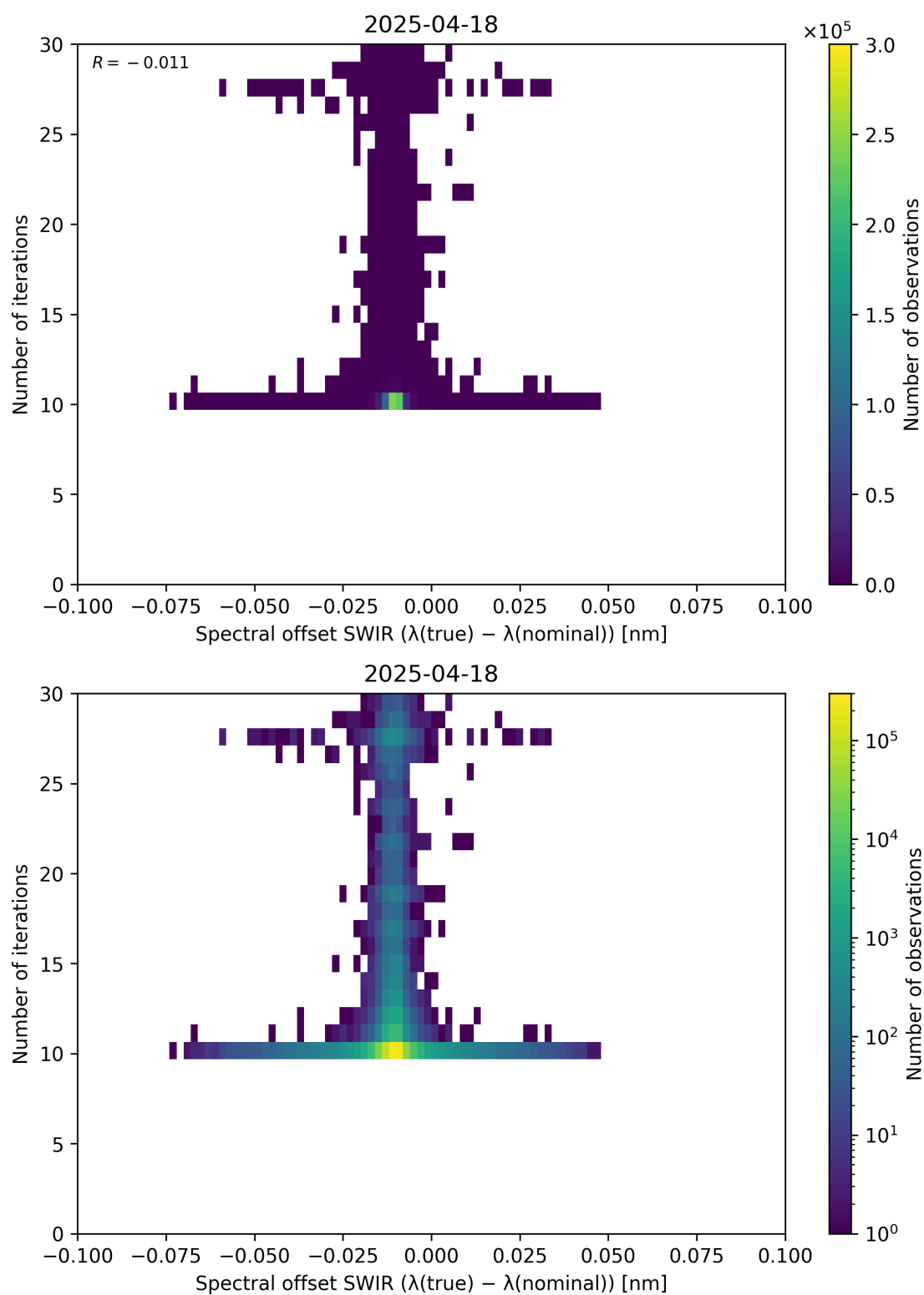
Figure 121: Scatter density plot of “Spectral offset SWIR ( \lambda_{\text{true}} - \lambda_{\text{nominal}} )” against “Number of iterations” for 2025-04-18 to 2025-04-19.
