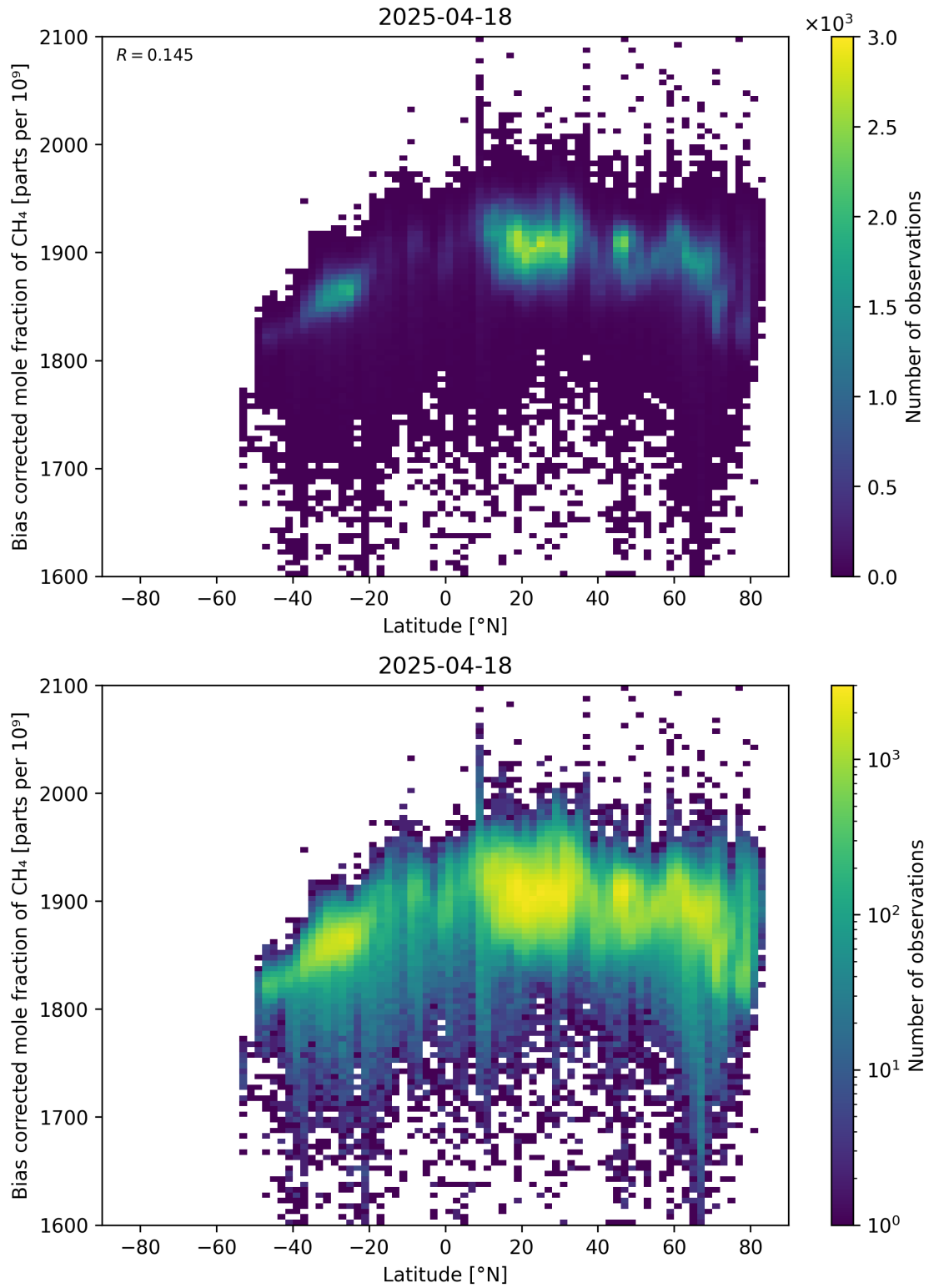
Figure 58: Scatter density plot of “Latitude” against “Bias corrected mole fraction of CH 4 ” for 2025-04-18 to 2025-04-19.
