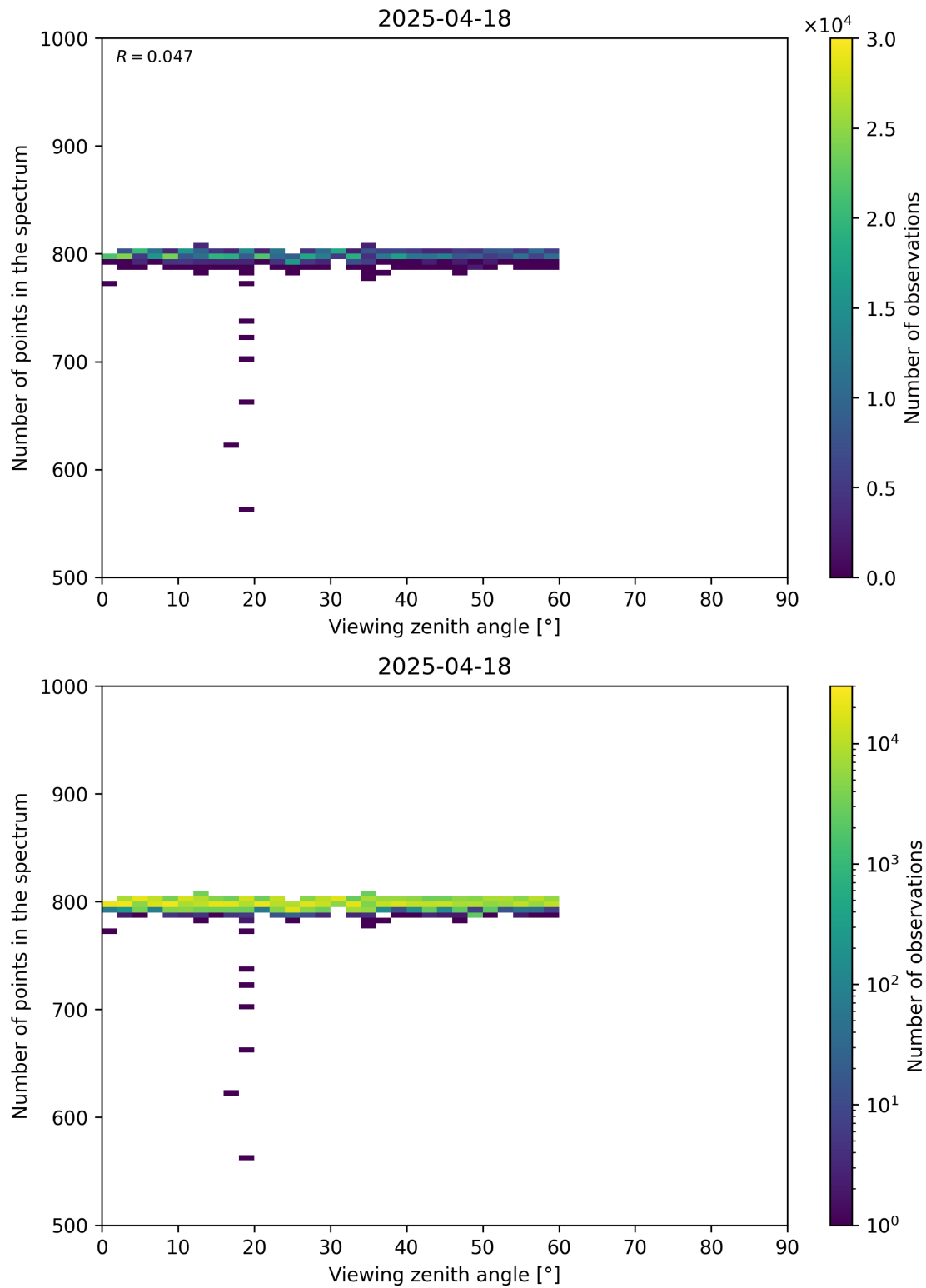
Figure 114: Scatter density plot of “Viewing zenith angle” against “Number of points in the spectrum” for 2025-04-18 to 2025-04-19.
