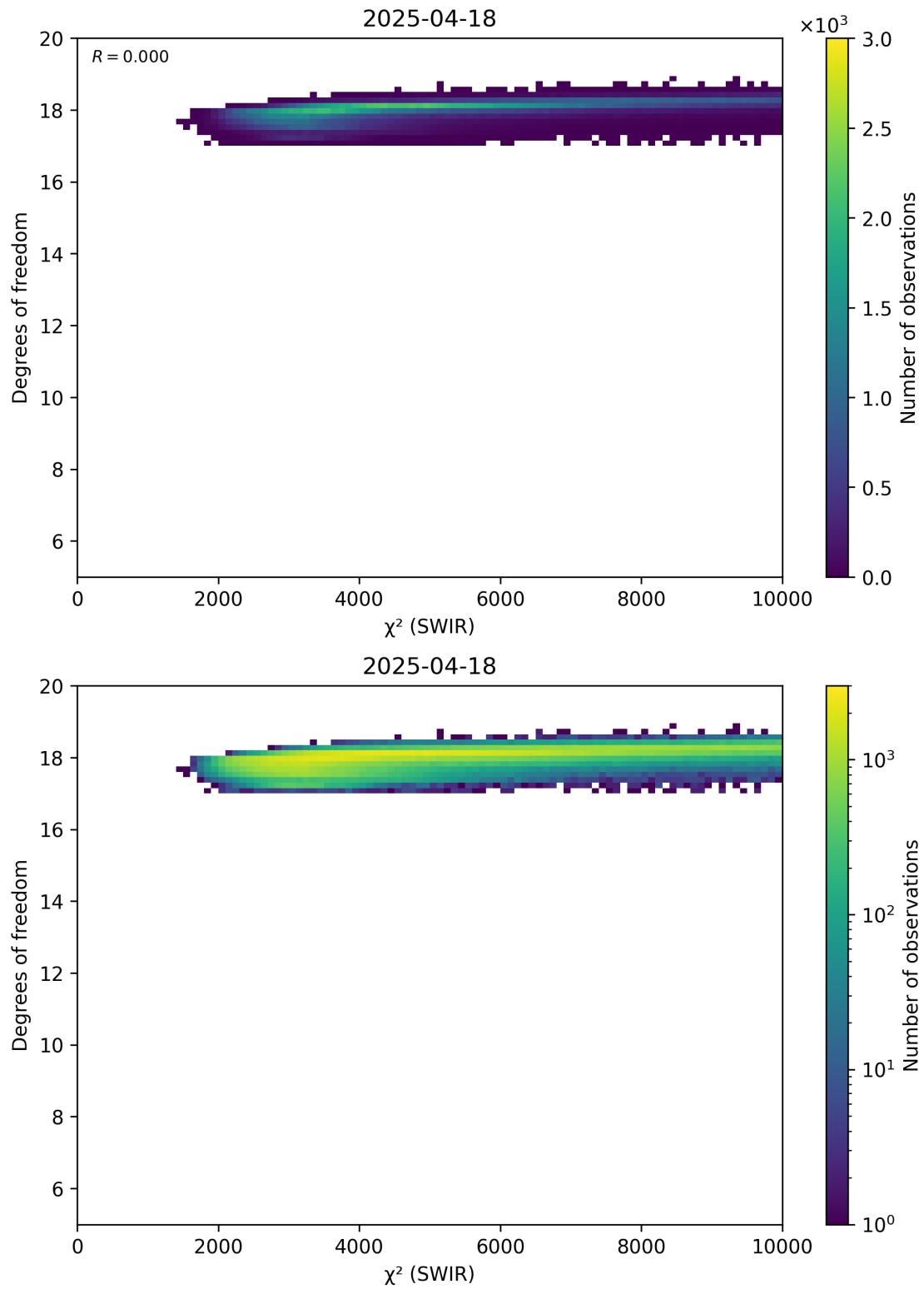
Figure 48: Scatter density plot of “ \chi^2 (SWIR)” against “Degrees of freedom” for 2025-04-18 to 2025-04-19.
