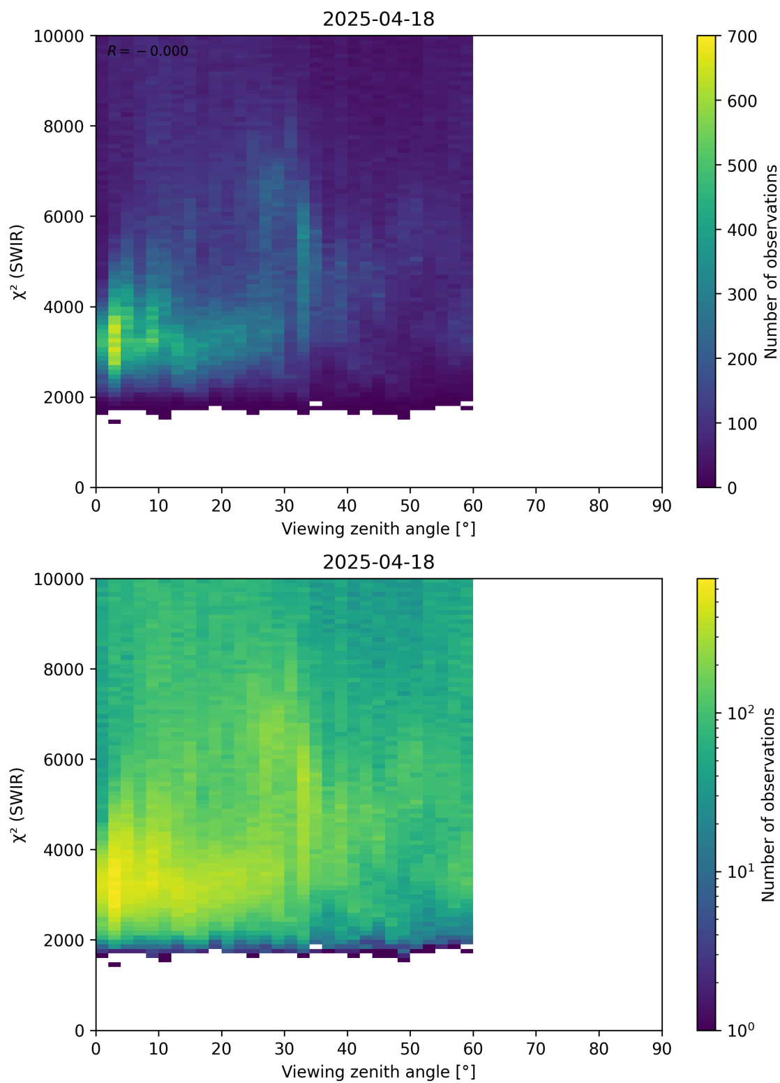
Figure 106: Scatter density plot of “Viewing zenith angle” against “ \chi^2 (SWIR)” for 2025-04-18 to 2025-04-19.
