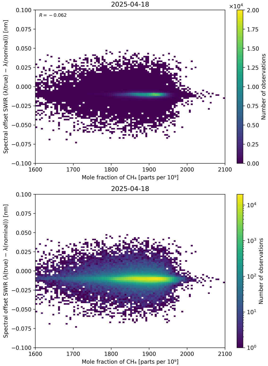
Figure 86: Scatter density plot of “Mole fraction of \text{CH}_4 ” against “Spectral offset SWIR ( \lambda_{\text{true}} - \lambda_{\text{nominal}} )” for 2025-04-18 to 2025-04-19.
