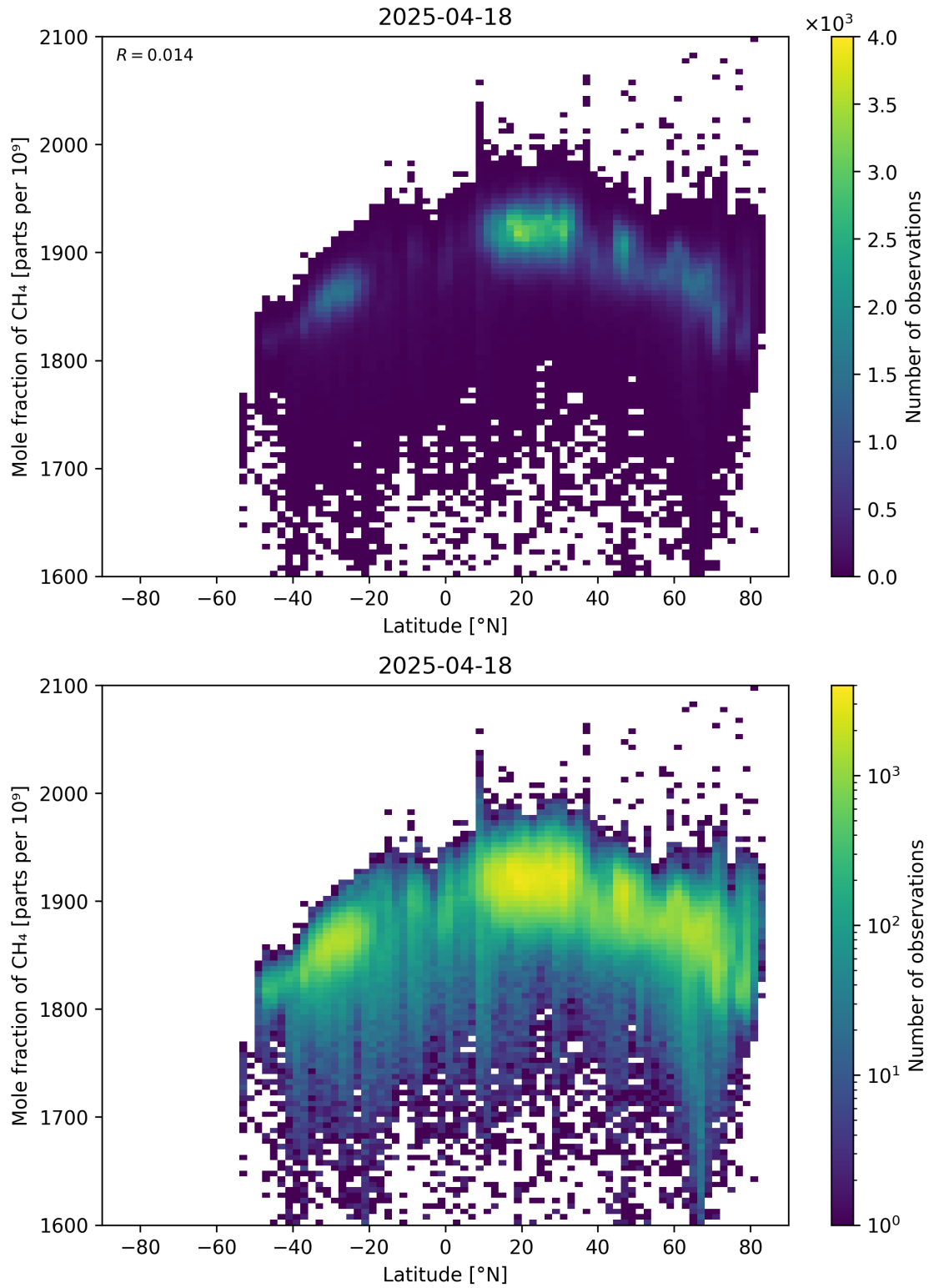
Figure 57: Scatter density plot of “Latitude” against “Mole fraction of \text{CH}_4 ” for 2025-04-18 to 2025-04-19.
