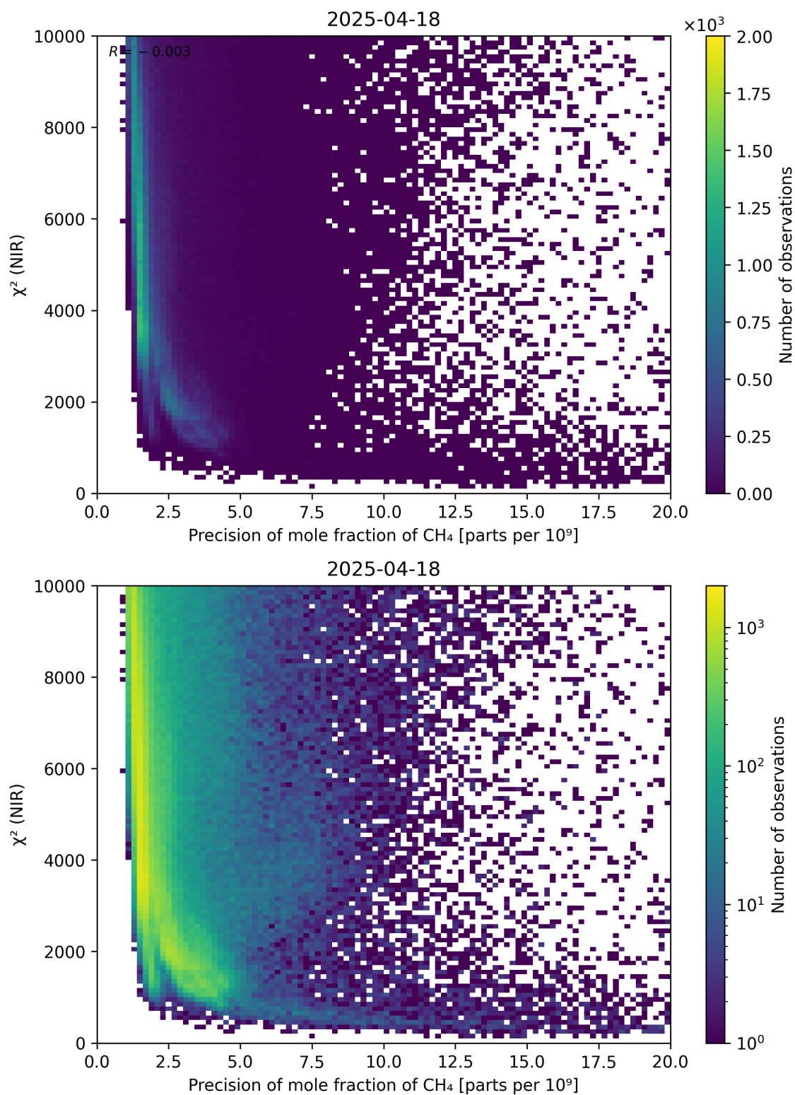
Figure 78: Scatter density plot of “Precision of mole fraction of CH 4 ” against “ \chi^2 (NIR)” for 2025-04-18 to 2025-04-19.
