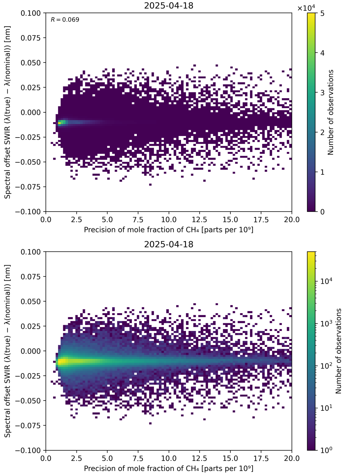
Figure 85: Scatter density plot of “Precision of mole fraction of \text{CH}_4 ” against “Spectral offset SWIR ( \lambda_{\text{true}} - \lambda_{\text{nominal}} )” for 2025-04-18 to 2025-04-19.
