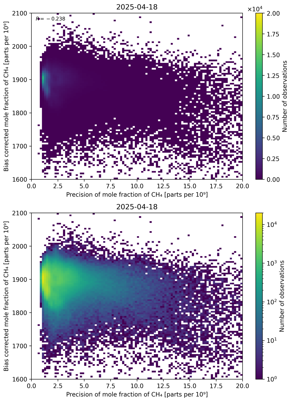
Figure 82: Scatter density plot of “Precision of mole fraction of CH 4 ” against “Bias corrected mole fraction of CH 4 ” for 2025-04-18 to 2025-04-19.
