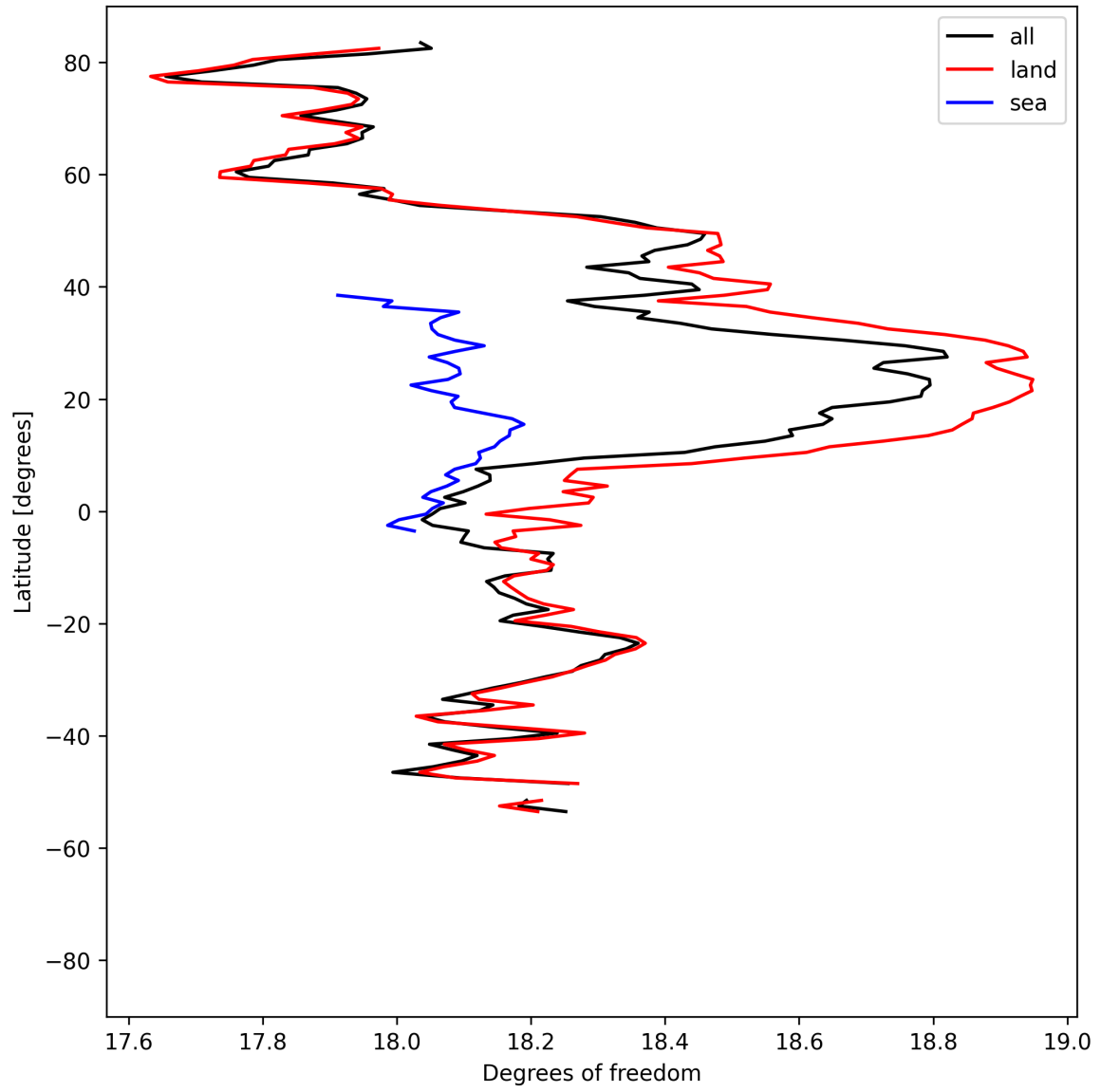
Figure 19: Zonal average of “Degrees of freedom” for 2025-04-18 to 2025-04-19.
