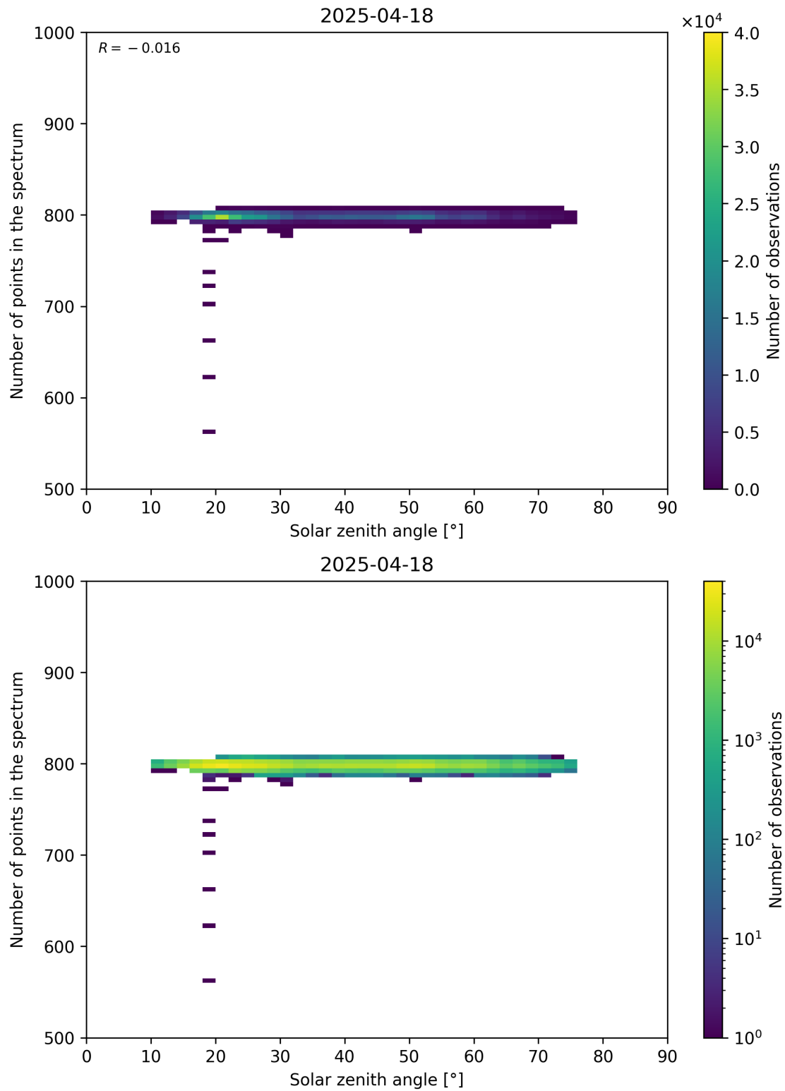
Figure 103: Scatter density plot of “Solar zenith angle” against “Number of points in the spectrum” for 2025-04-18 to 2025-04-19.
