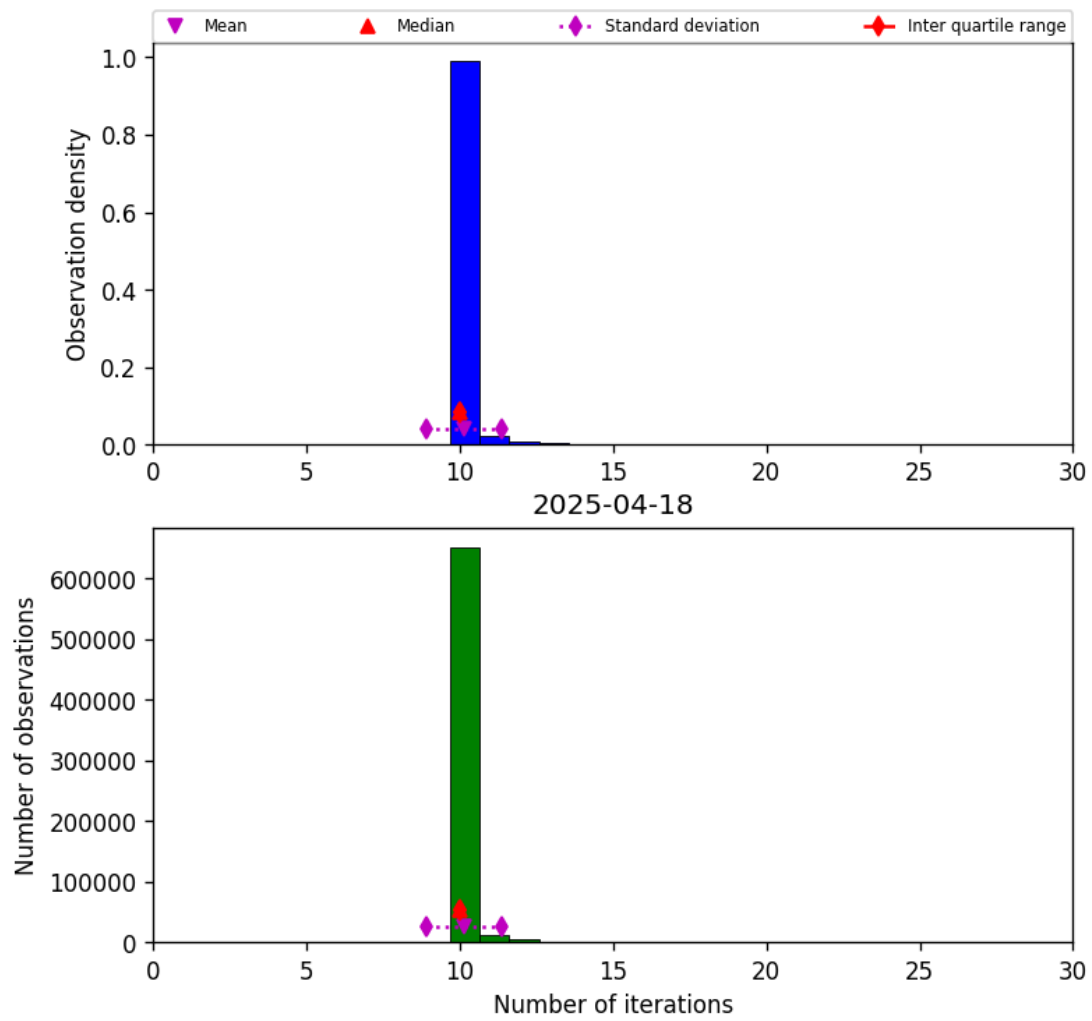
Figure 31: Histogram of “Number of iterations” for 2025-04-18 to 2025-04-19
