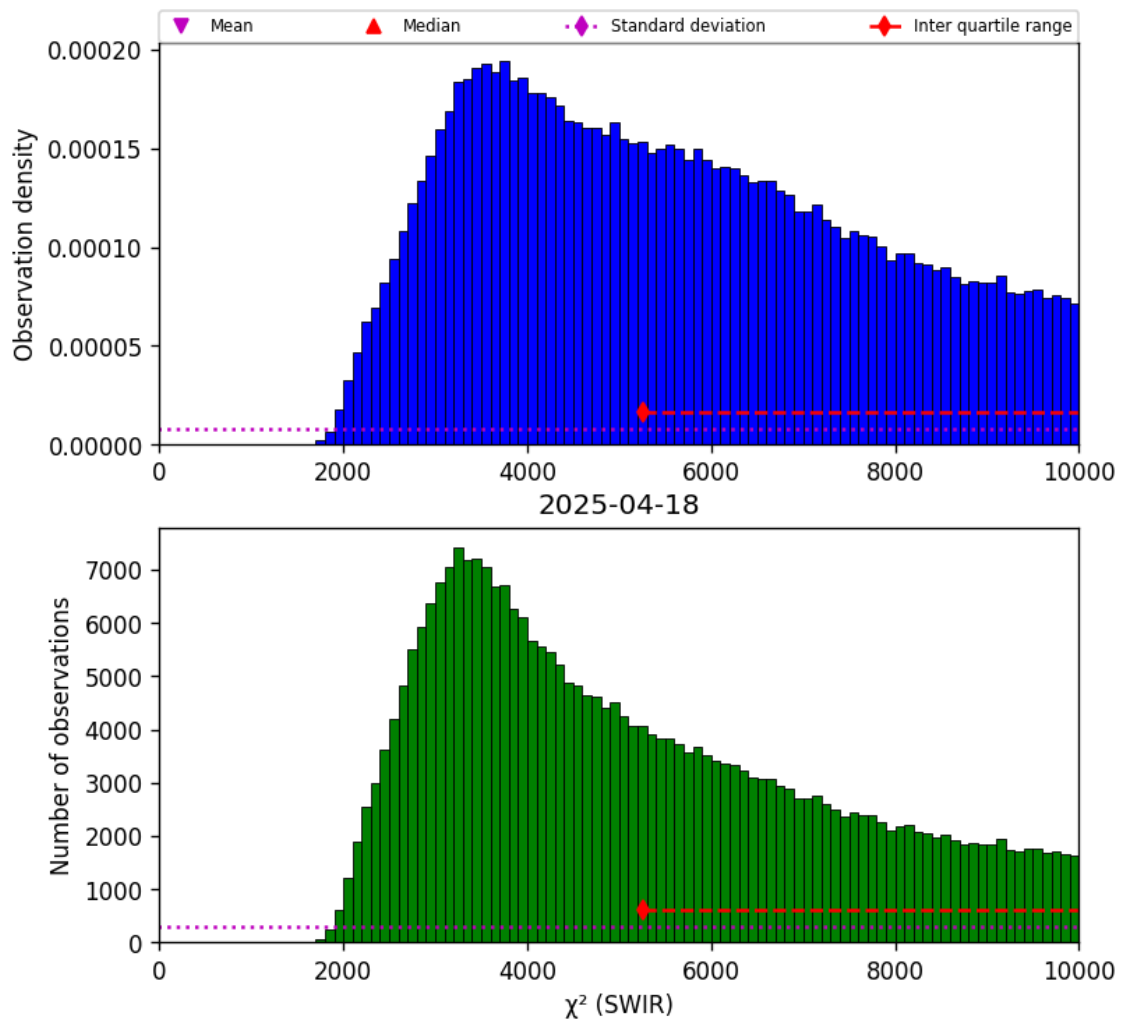
Figure 28: Histogram of " \chi^2 (SWIR)" for 2025-04-18 to 2025-04-19
