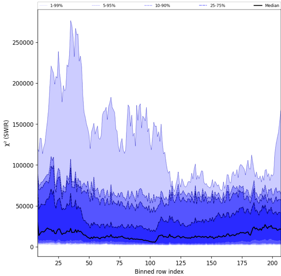
Figure 39: Along track statistics of " \chi^2 (SWIR)" for 2025-04-18 to 2025-04-19
