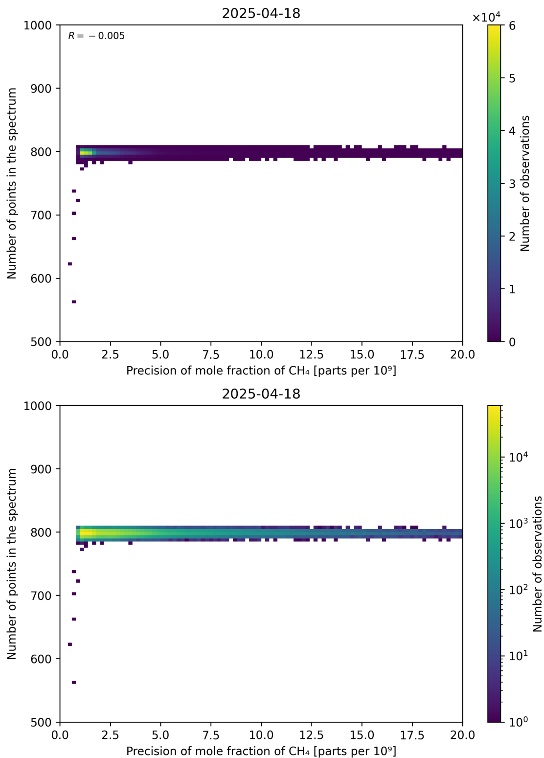
Figure 84: Scatter density plot of “Precision of mole fraction of CH 4 ” against “Number of points in the spectrum” for 2025-04-18 to 2025-04-19.
