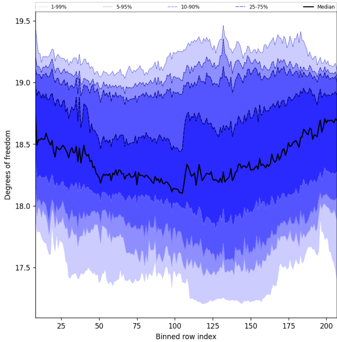
Figure 41: Along track statistics of “Degrees of freedom” for 2025-04-18 to 2025-04-19
