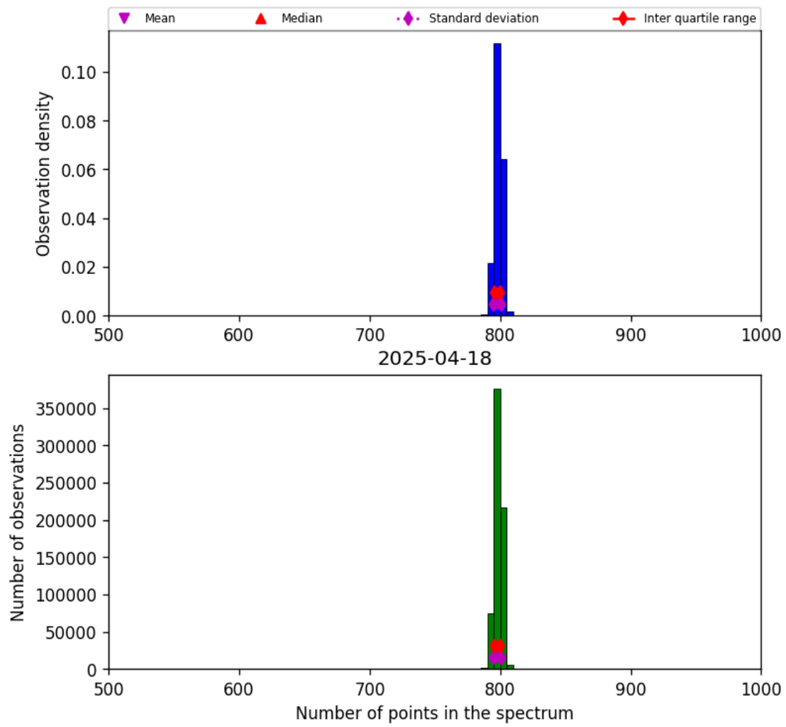
Figure 26: Histogram of “Number of points in the spectrum” for 2025-04-18 to 2025-04-19
