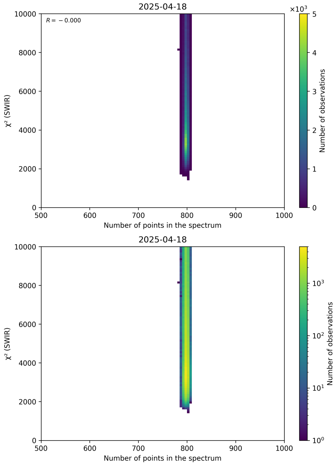
Figure 89: Scatter density plot of “Number of points in the spectrum” against “ \chi^2 (SWIR)” for 2025-04-18 to 2025-04-19.
