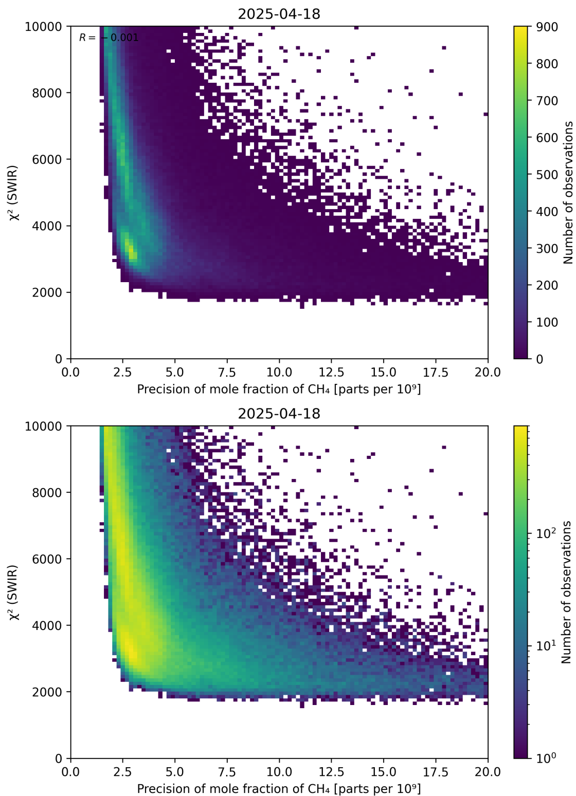
Figure 79: Scatter density plot of “Precision of mole fraction of CH 4 ” against “ \chi^2 (SWIR)” for 2025-04-18 to 2025-04-19.
