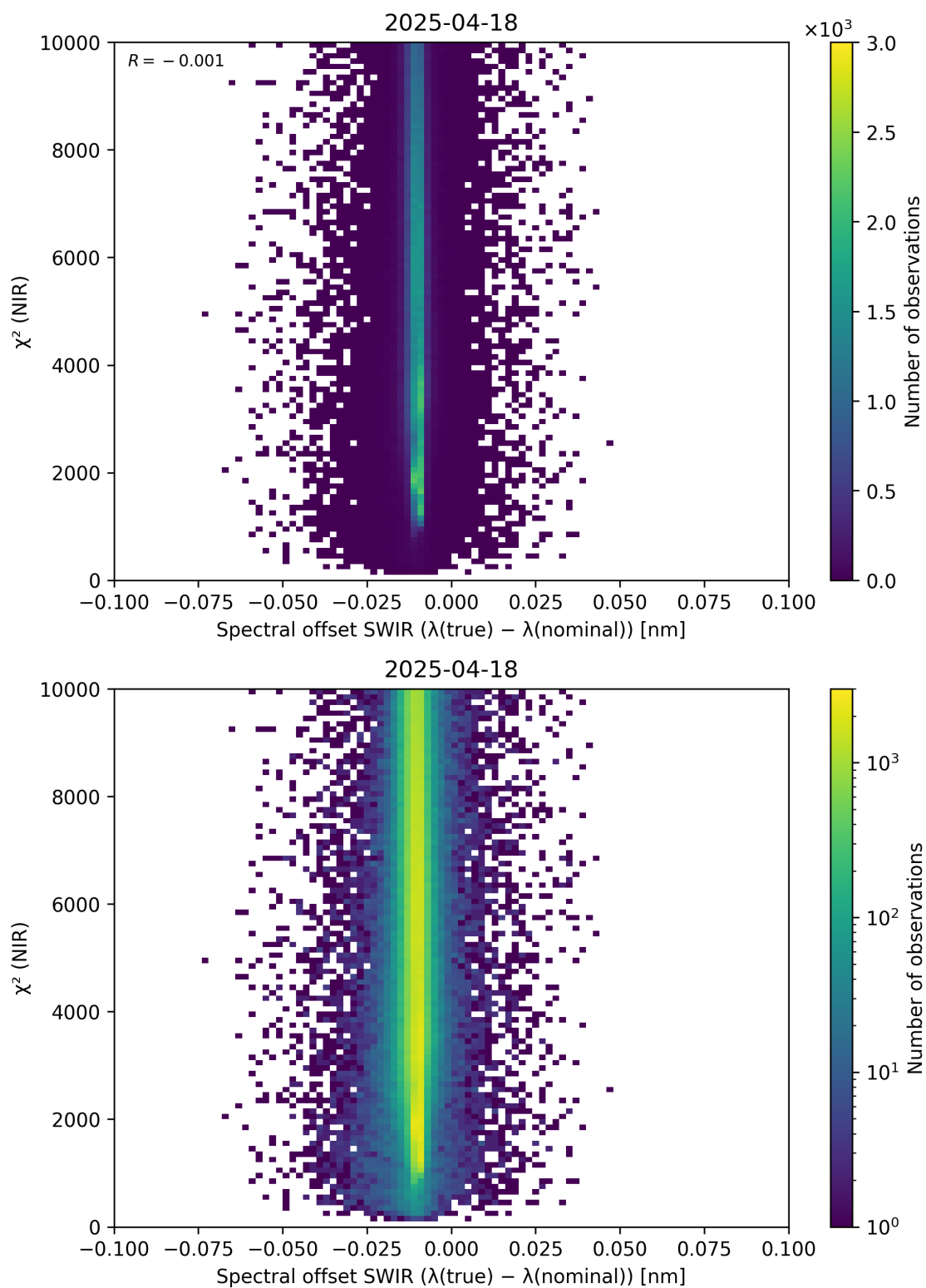
Figure 117: Scatter density plot of “Spectral offset SWIR ( \lambda_{\text{true}} - \lambda_{\text{nominal}} )” against “ \chi^2 (NIR)” for 2025-04-18 to 2025-04-19.
