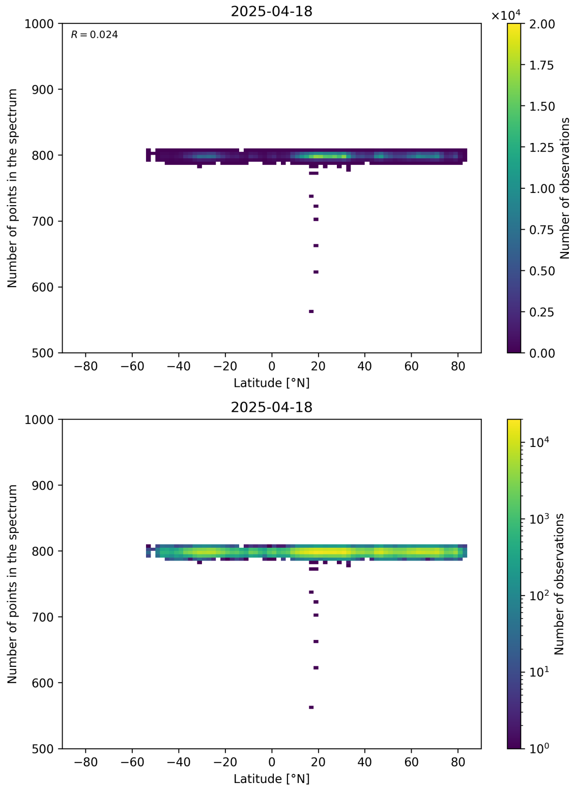
Figure 61: Scatter density plot of “Latitude” against “Number of points in the spectrum” for 2025-04-18 to 2025-04-19.
