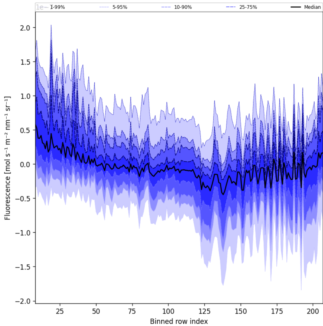
Figure 43: Along track statistics of “Fluorescence” for 2025-04-18 to 2025-04-19
