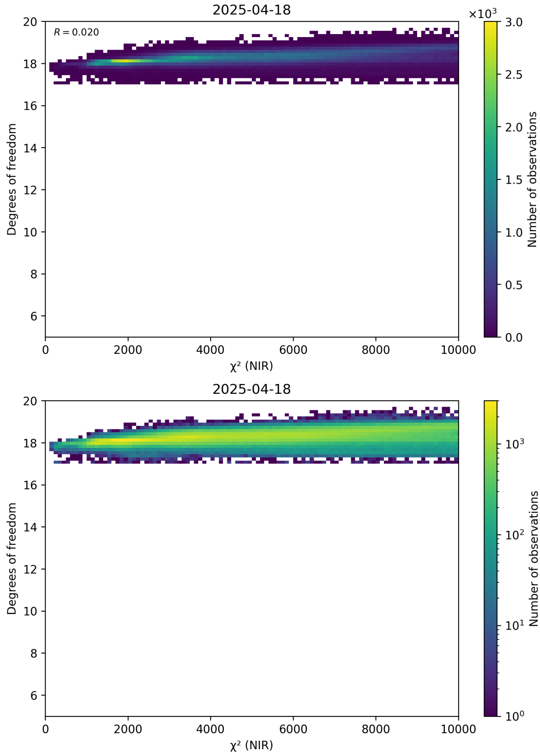
Figure 44: Scatter density plot of “ \chi^2 (NIR)” against “Degrees of freedom” for 2025-04-18 to 2025-04-19.
