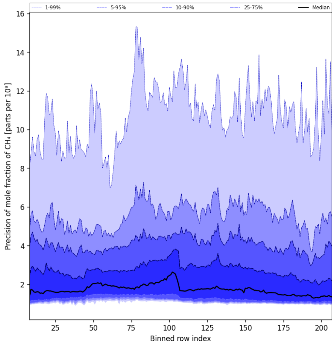
Figure 35: Along track statistics of “Precision of mole fraction of CH 4 ” for 2025-04-18 to 2025-04-19
