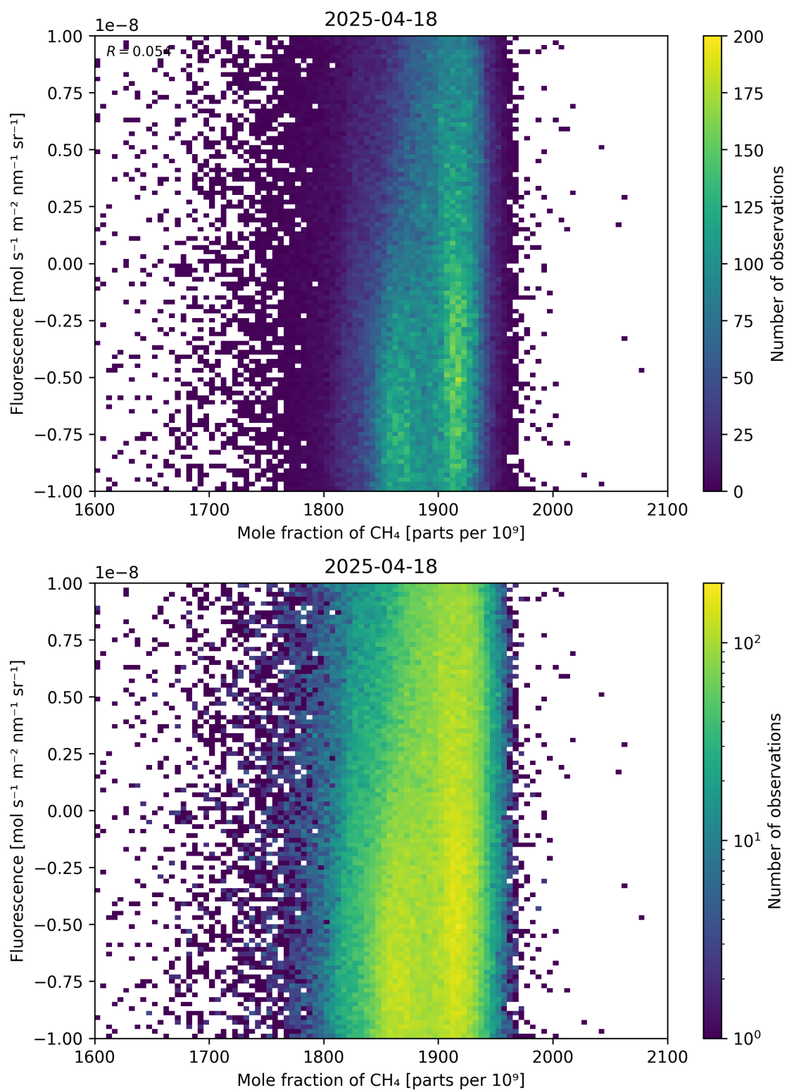
Figure 73: Scatter density plot of “Mole fraction of \text{CH}_4 ” against “Fluorescence” for 2025-04-18 to 2025-04-19.
