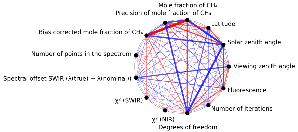
Figure 1: Map of correlation graph for 2025-04-18 to 2025-04-19.
