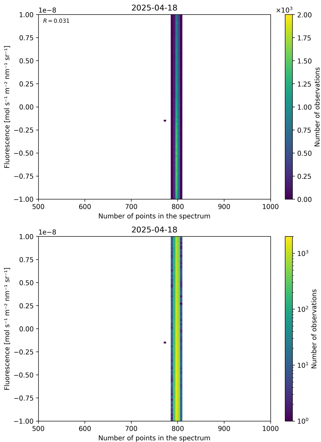
Figure 91: Scatter density plot of “Number of points in the spectrum” against “Fluorescence” for 2025-04-18 to 2025-04-19.
