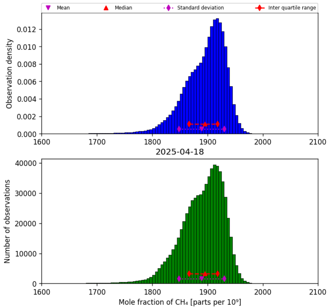
Figure 23: Histogram of “Mole fraction of CH 4 ” for 2025-04-18 to 2025-04-19
