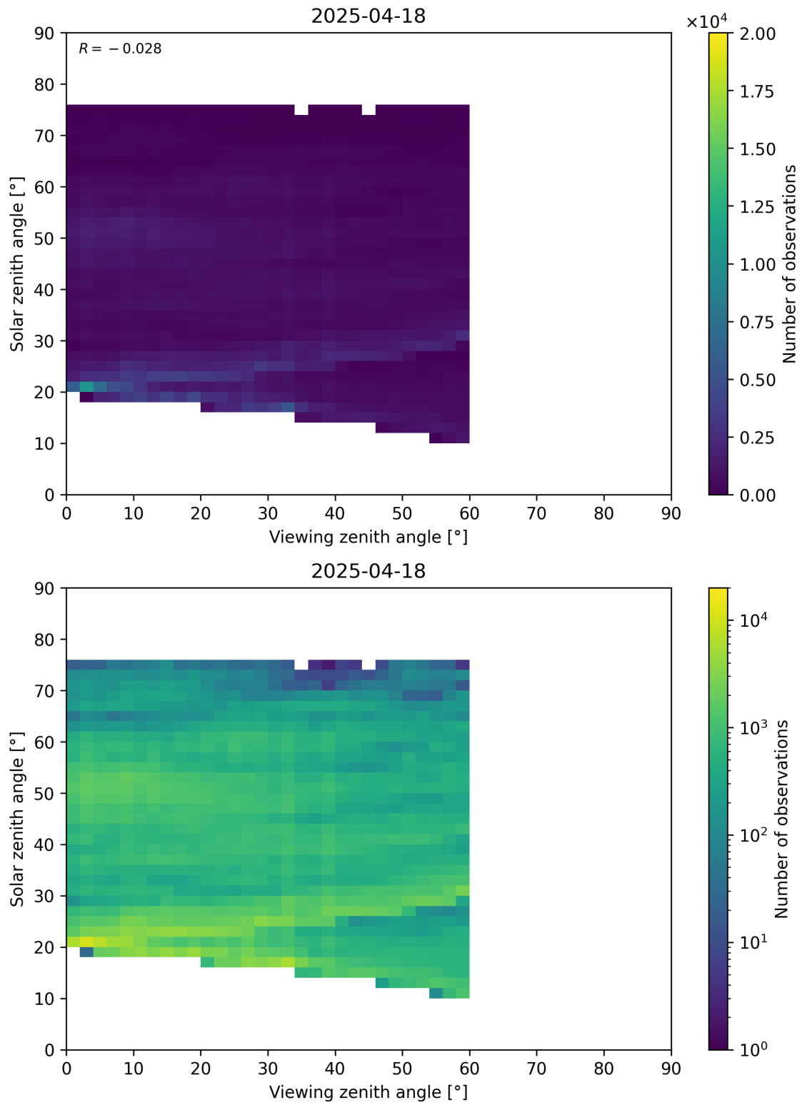
Figure 115: Scatter density plot of “Viewing zenith angle” against “Solar zenith angle” for 2025-04-18 to 2025-04-19.
