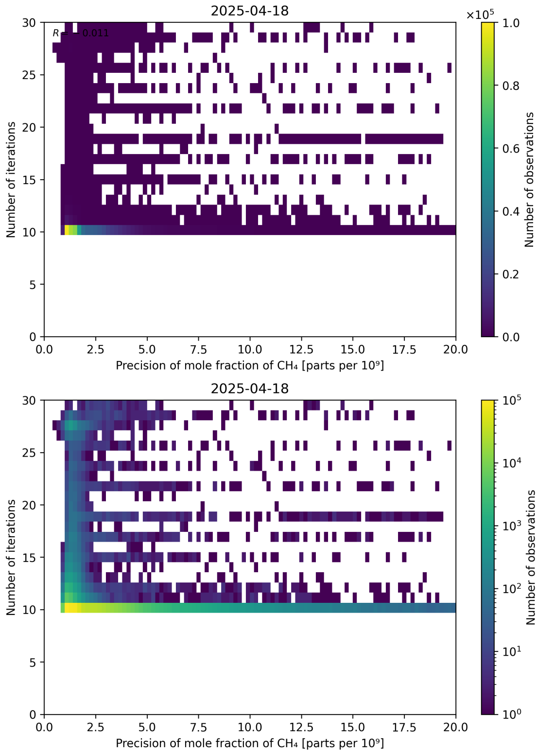
Figure 83: Scatter density plot of “Precision of mole fraction of CH 4 ” against “Number of iterations” for 2025-04-18 to 2025-04-19.
