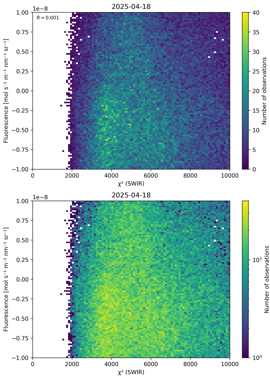
Figure 49: Scatter density plot of “ \chi^2 (SWIR)” against “Fluorescence” for 2025-04-18 to 2025-04-19.
