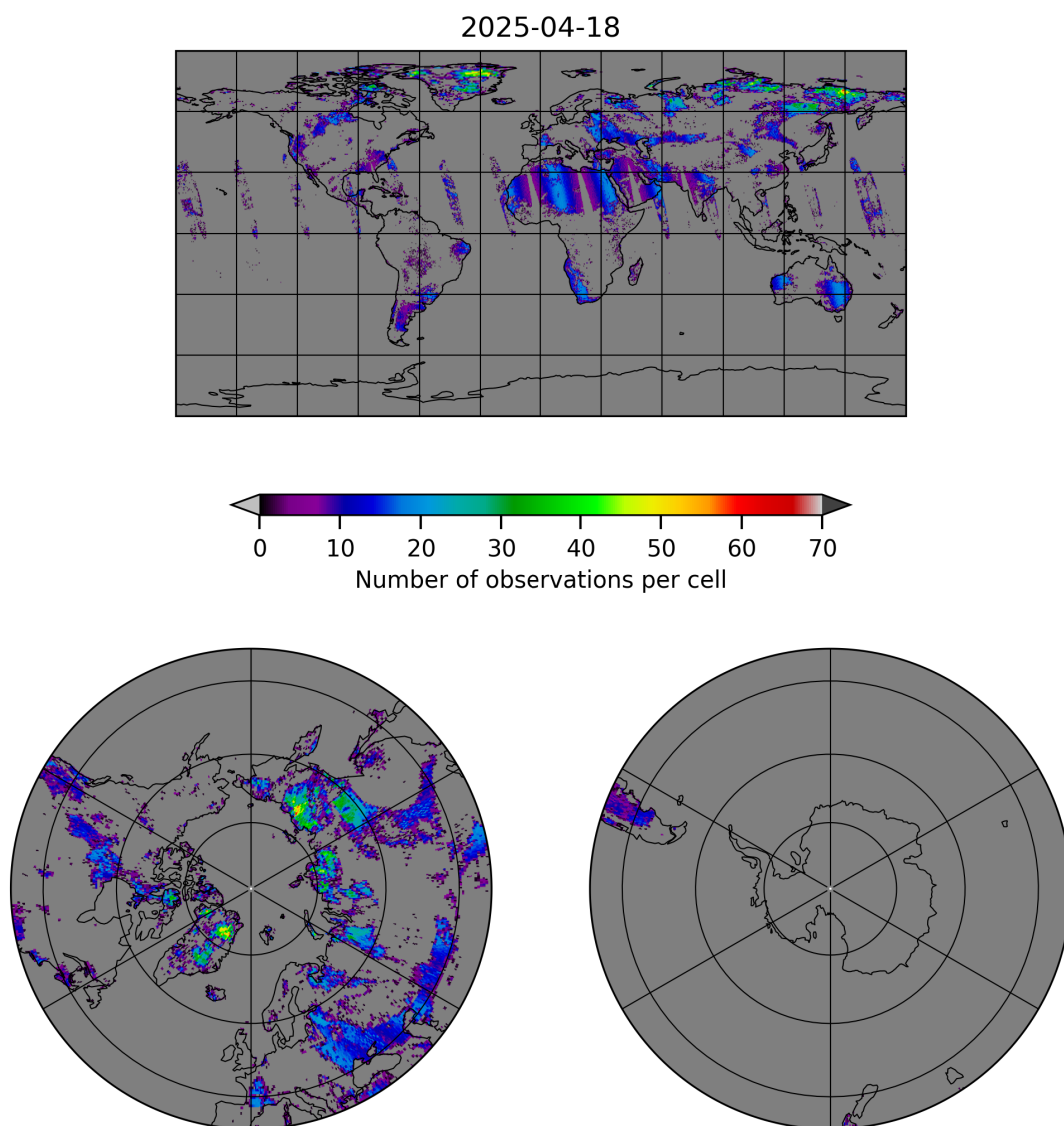
Figure 10: Map of the number of observations for 2025-04-18 to 2025-04-19
