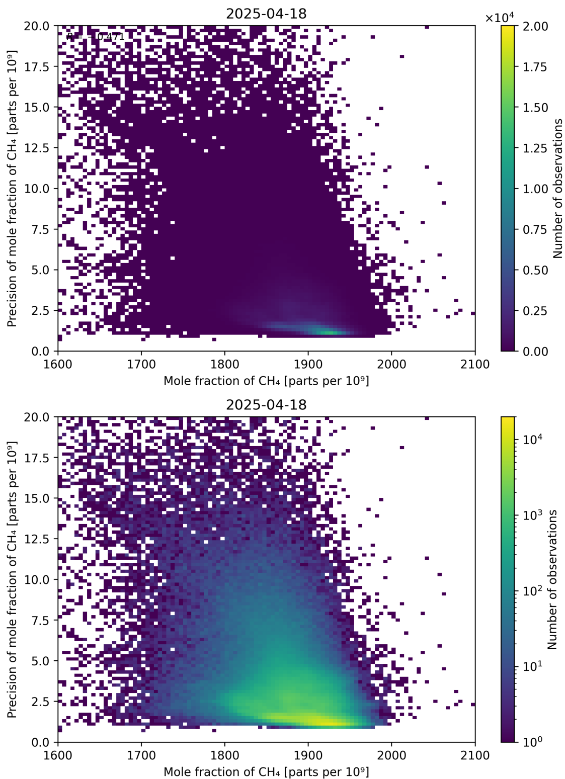
Figure 75: Scatter density plot of “Mole fraction of CH 4 ” against “Precision of mole fraction of CH 4 ” for 2025-04-18 to 2025-04-19.
