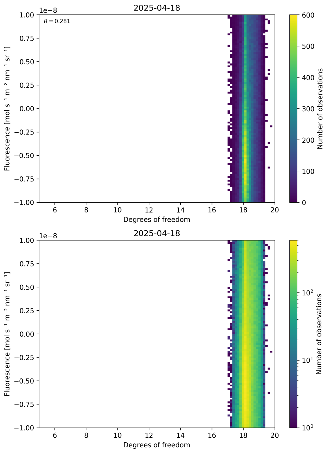
Figure 51: Scatter density plot of “Degrees of freedom” against “Fluorescence” for 2025-04-18 to 2025-04-19.
