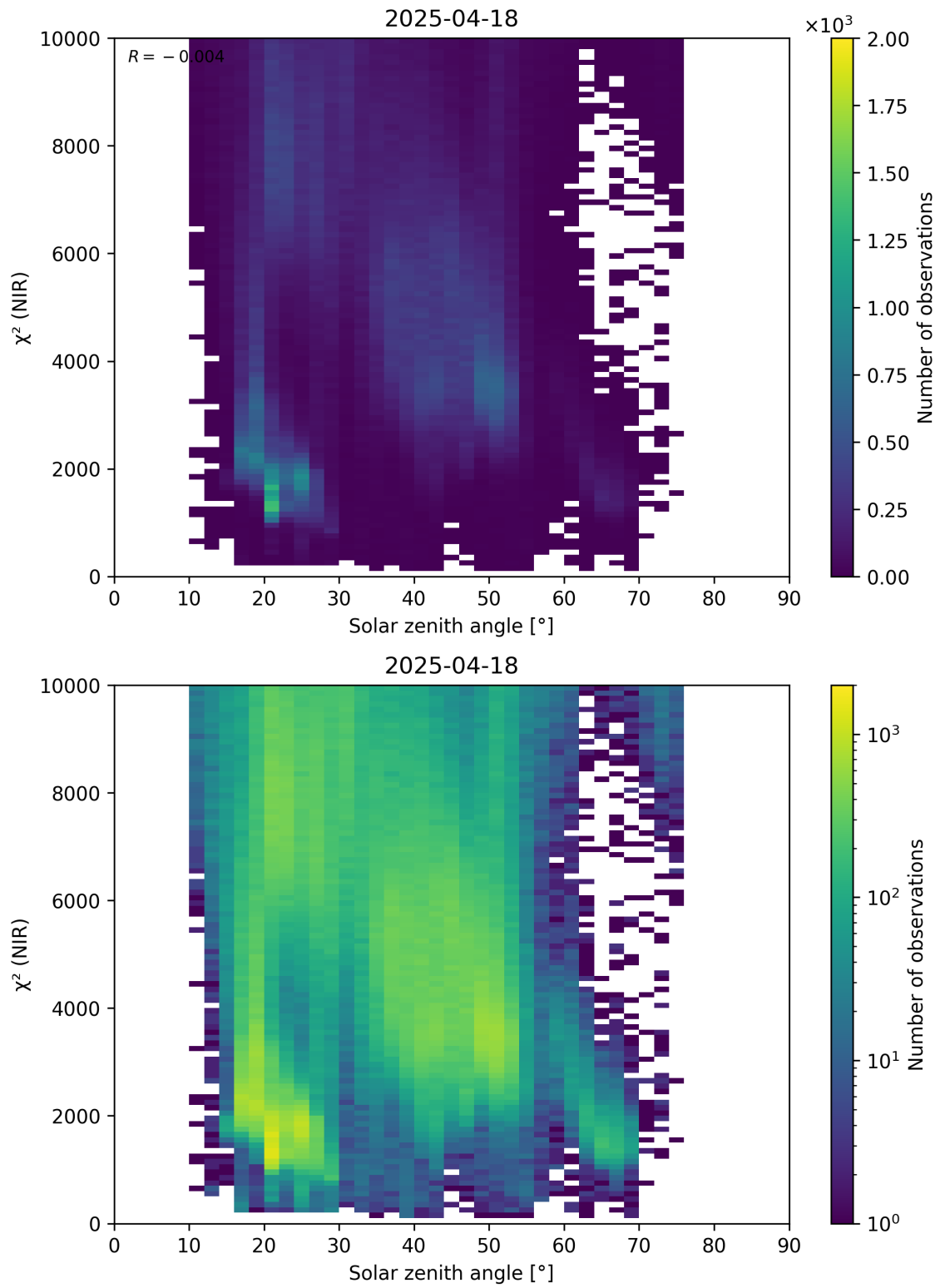
Figure 94: Scatter density plot of “Solar zenith angle” against “ \chi^2 (NIR)” for 2025-04-18 to 2025-04-19.
