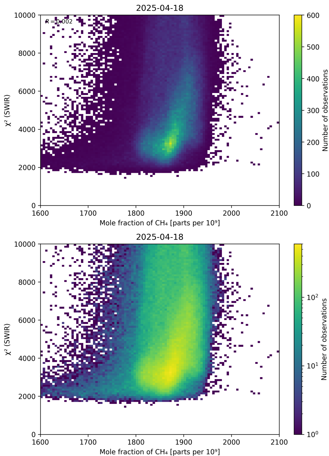
Figure 71: Scatter density plot of “Mole fraction of \text{CH}_4 ” against “ \chi^2 (SWIR)” for 2025-04-18 to 2025-04-19.
