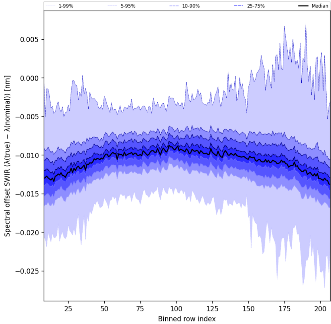
Figure 38: Along track statistics of “Spectral offset SWIR ( \lambda_{\text{true}} - \lambda_{\text{nominal}} )” for 2025-04-18 to 2025-04-19
