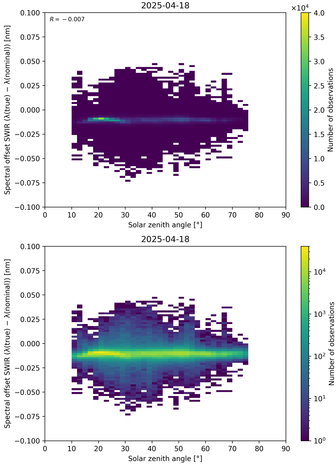
Figure 104: Scatter density plot of “Solar zenith angle” against “Spectral offset SWIR ( \lambda_{\text{true}} - \lambda_{\text{nominal}} )” for 2025-04-18 to 2025-04-19.
