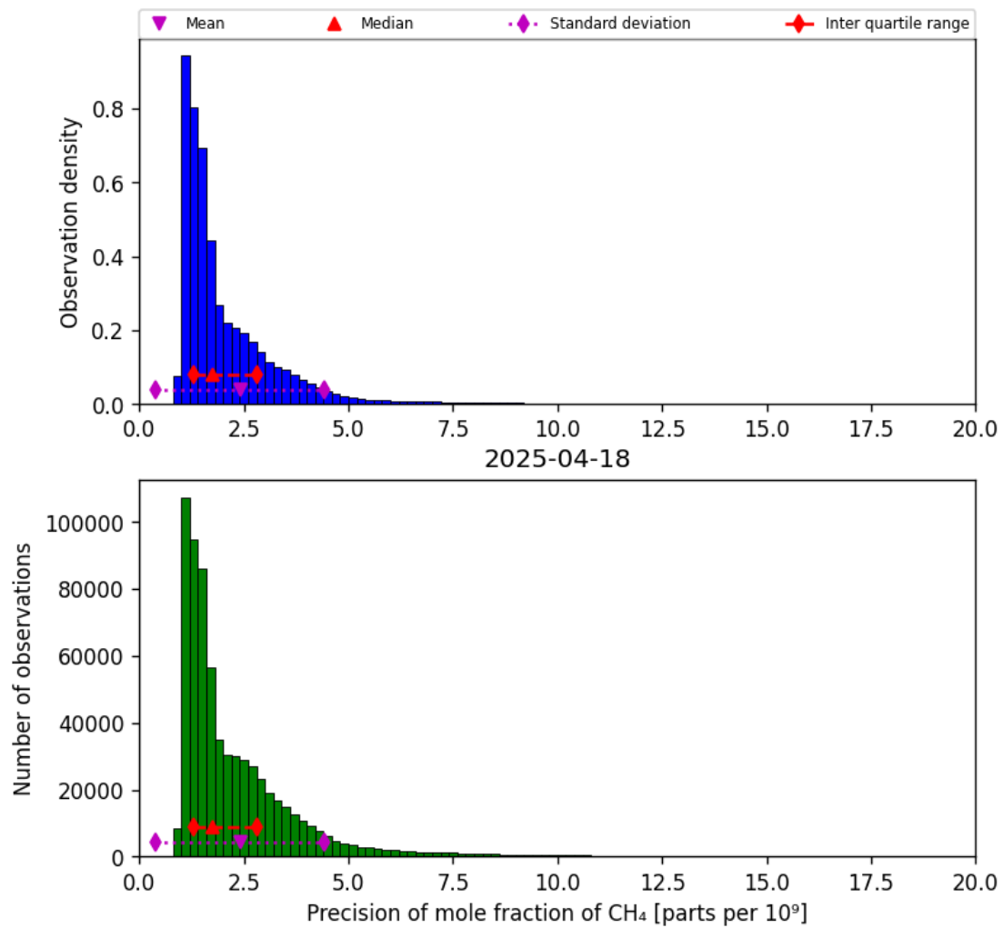
Figure 24: Histogram of “Precision of mole fraction of CH 4 ” for 2025-04-18 to 2025-04-19
