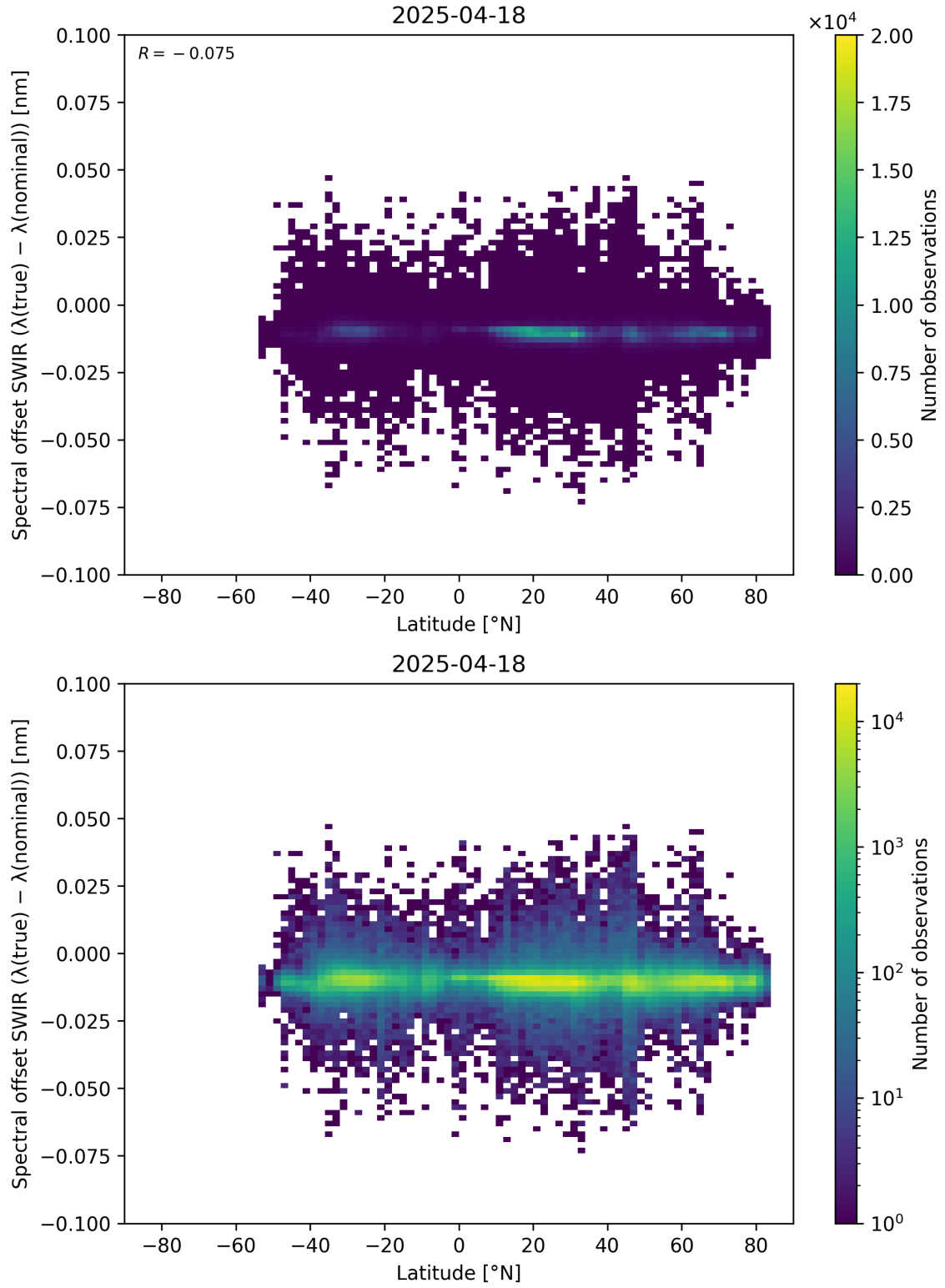
Figure 62: Scatter density plot of “Latitude” against “Spectral offset SWIR ( \lambda_{\text{true}} - \lambda_{\text{nominal}} )” for 2025-04-18 to 2025-04-19.
