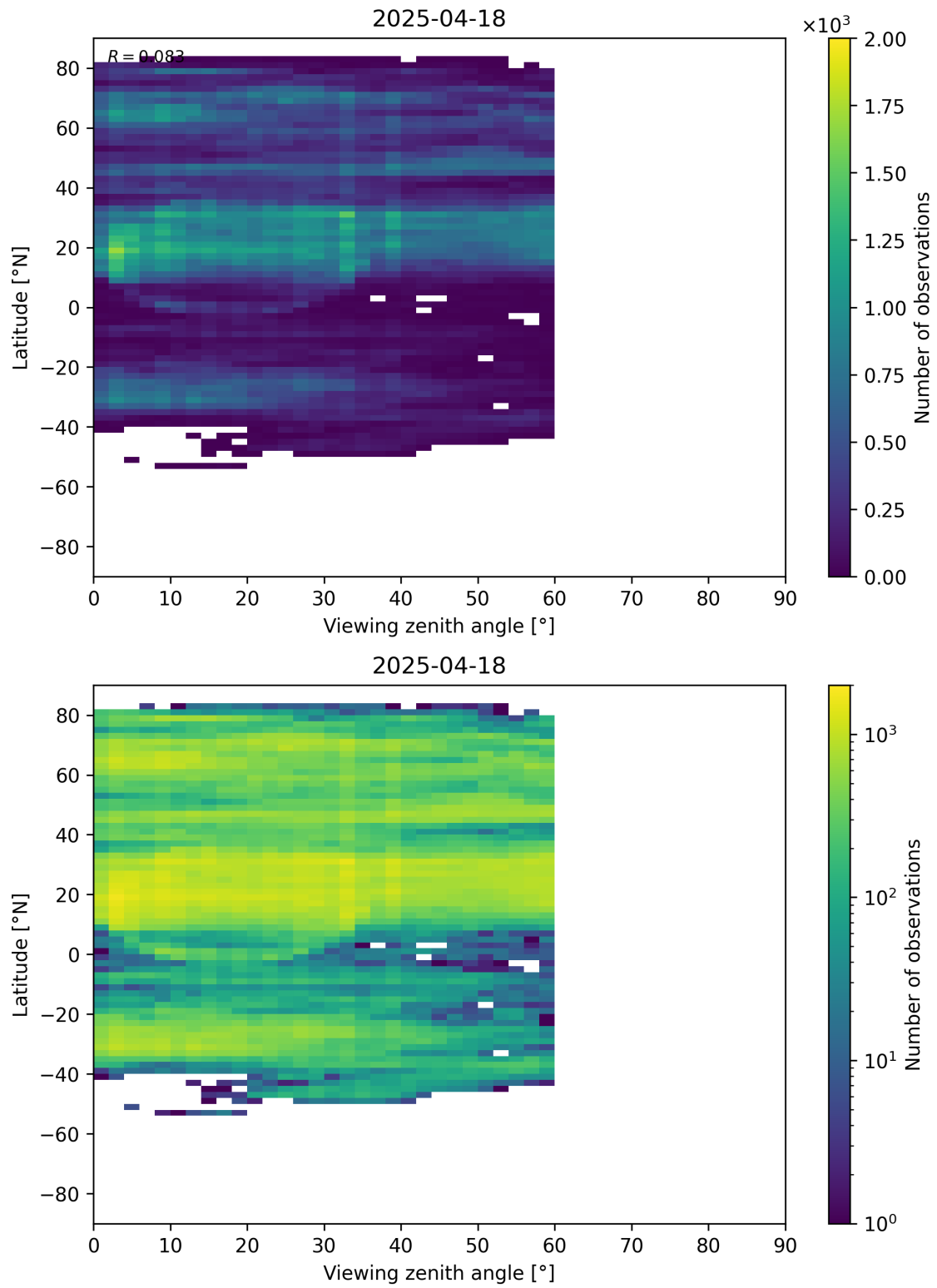
Figure 109: Scatter density plot of “Viewing zenith angle” against “Latitude” for 2025-04-18 to 2025-04-19.
