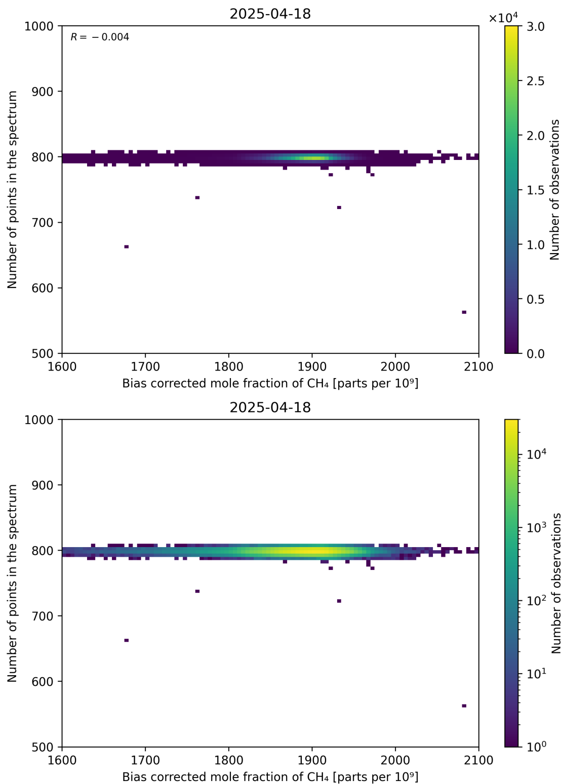
Figure 68: Scatter density plot of “Bias corrected mole fraction of CH 4 ” against “Number of points in the spectrum” for 2025-04-18 to 2025-04-19.
