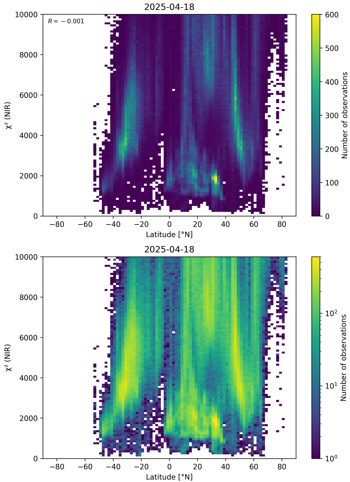
Figure 53: Scatter density plot of “Latitude” against “ \chi^2 (NIR)” for 2025-04-18 to 2025-04-19.
