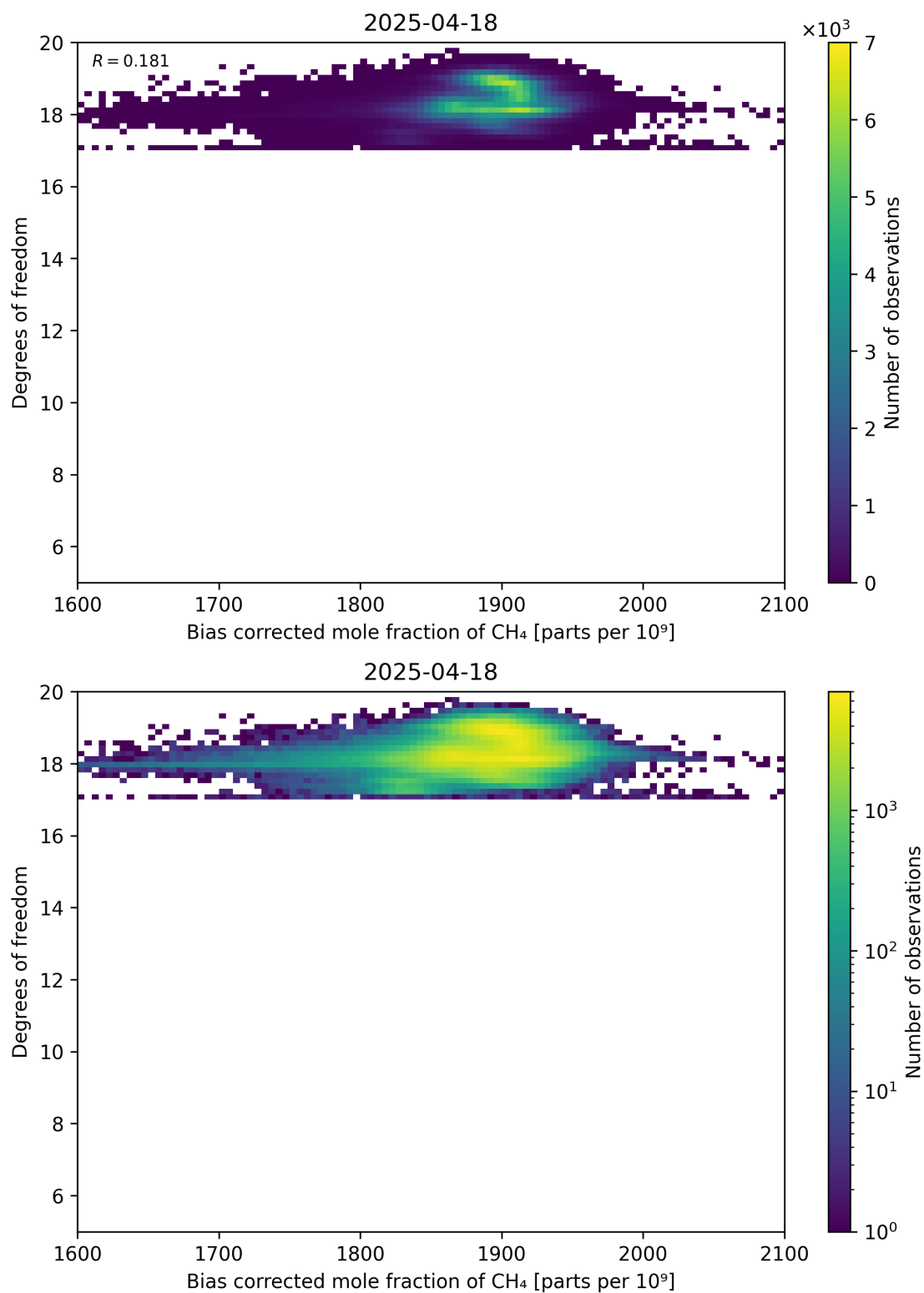
Figure 65: Scatter density plot of “Bias corrected mole fraction of CH 4 ” against “Degrees of freedom” for 2025-04-18 to 2025-04-19.
