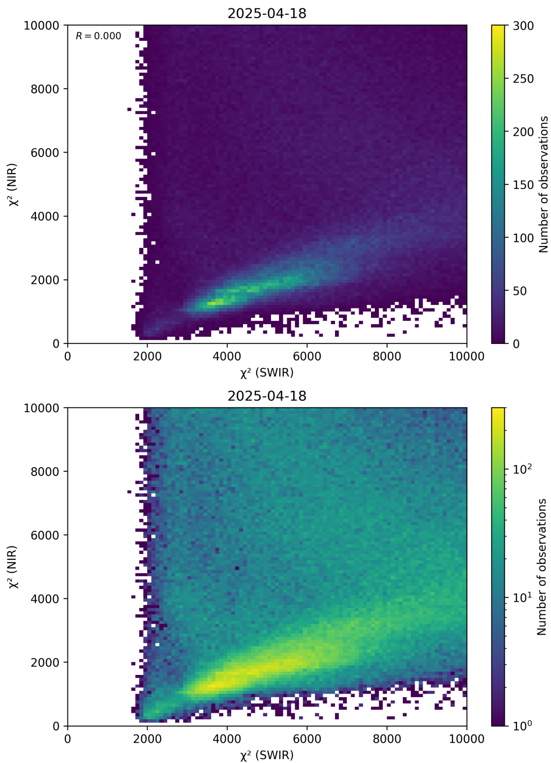
Figure 47: Scatter density plot of “ \chi^2 (SWIR)” against “ \chi^2 (NIR)” for 2025-04-18 to 2025-04-19.
