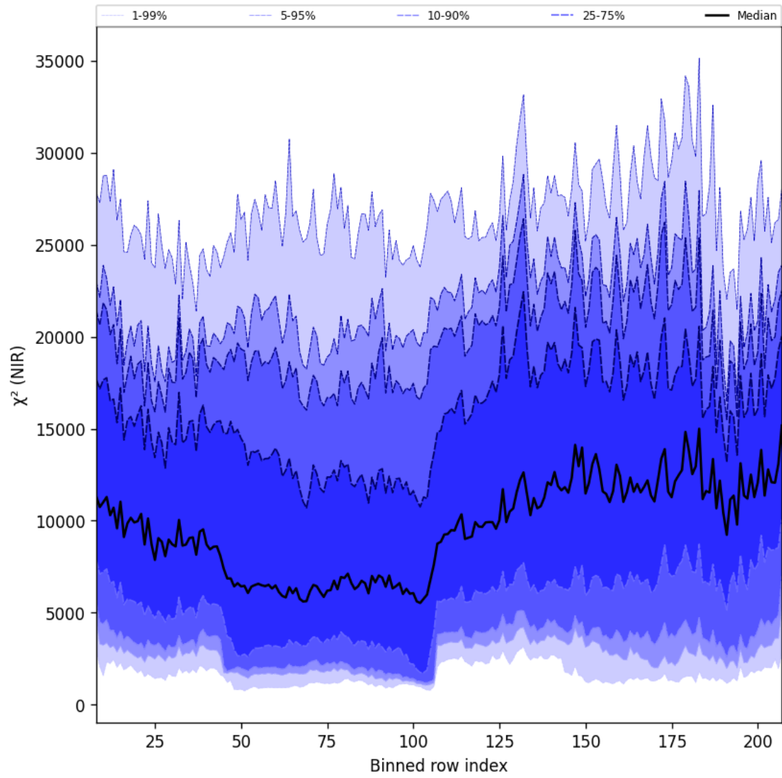
Figure 40: Along track statistics of “ \chi^2 (NIR)” for 2025-04-18 to 2025-04-19
