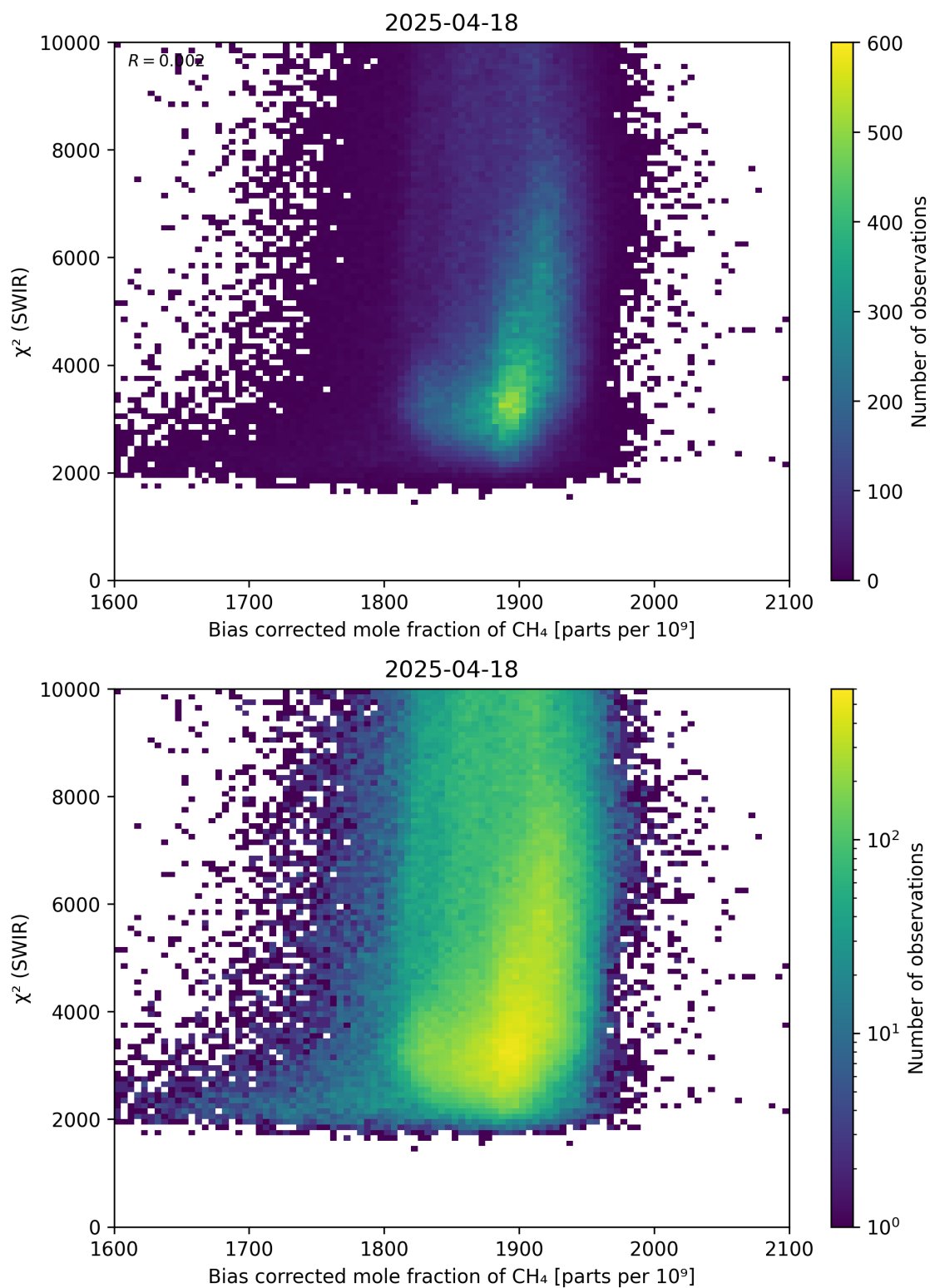
Figure 64: Scatter density plot of “Bias corrected mole fraction of \text{CH}_4 ” against “ \chi^2 (SWIR)” for 2025-04-18 to 2025-04-19.
