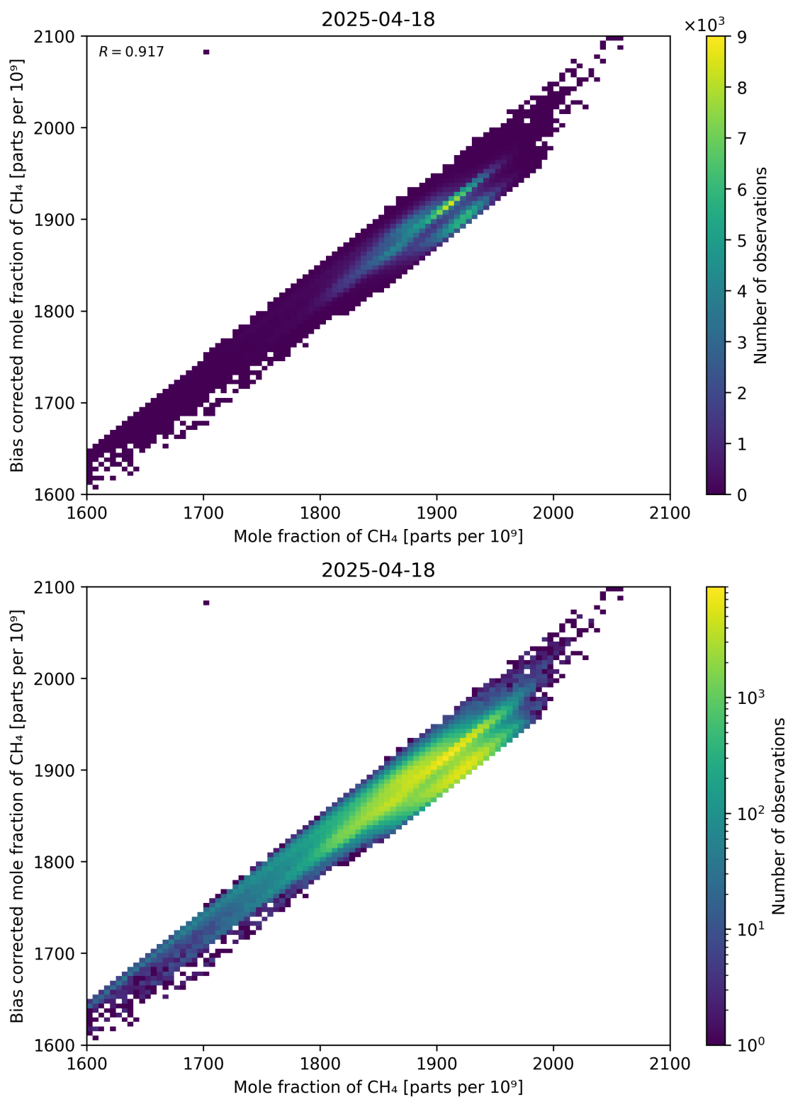
Figure 74: Scatter density plot of “Mole fraction of \text{CH}_4 ” against “Bias corrected mole fraction of \text{CH}_4 ” for 2025-04-18 to 2025-04-19.
