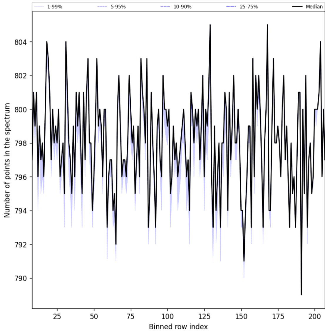
Figure 37: Along track statistics of “Number of points in the spectrum” for 2025-04-18 to 2025-04-19
