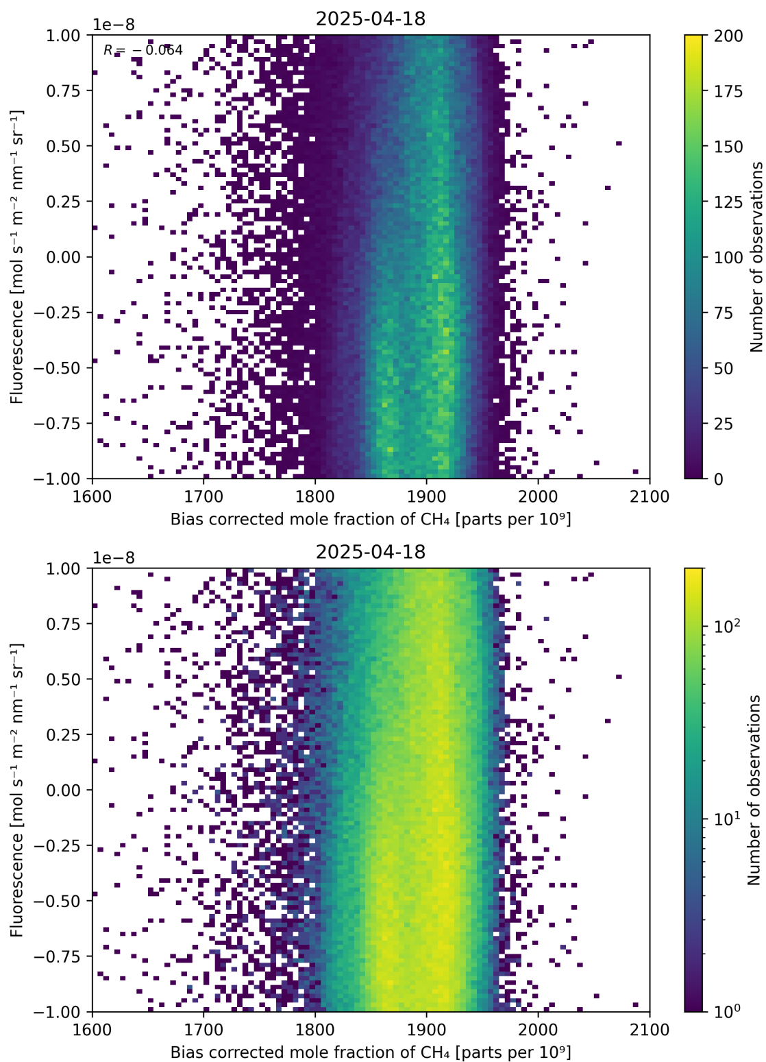
Figure 66: Scatter density plot of “Bias corrected mole fraction of \text{CH}_4 ” against “Fluorescence” for 2025-04-18 to 2025-04-19.
