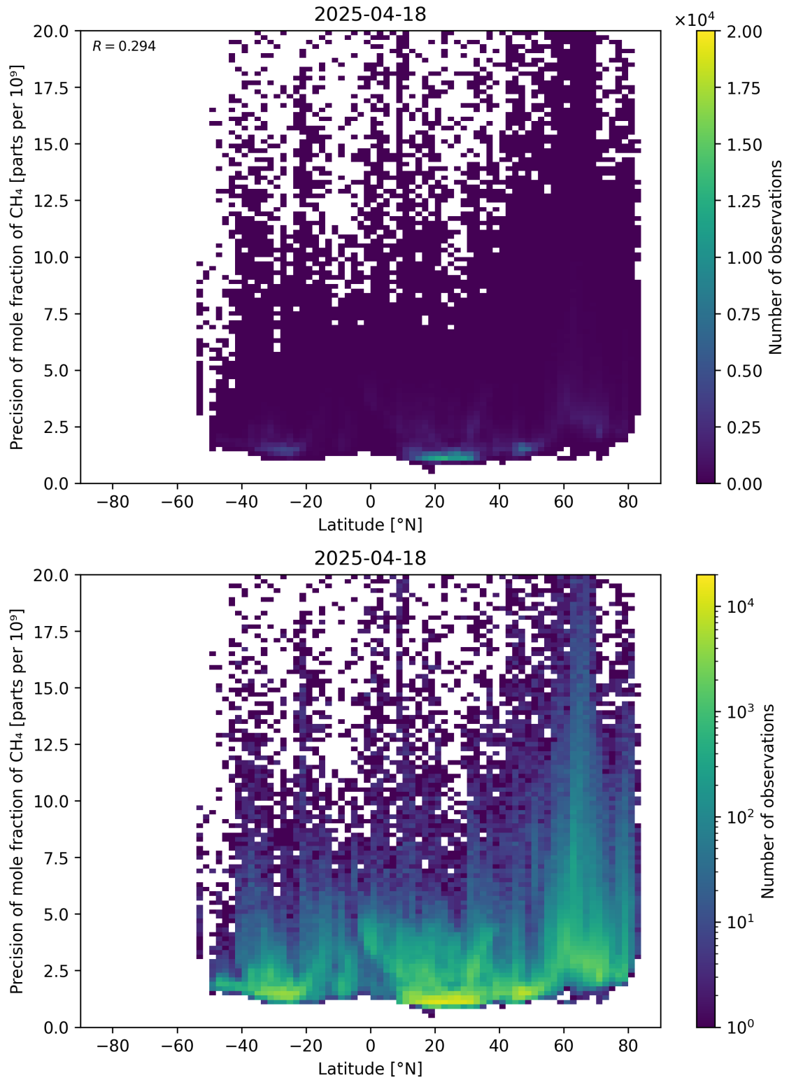
Figure 59: Scatter density plot of “Latitude” against “Precision of mole fraction of \text{CH}_4 ” for 2025-04-18 to 2025-04-19.
