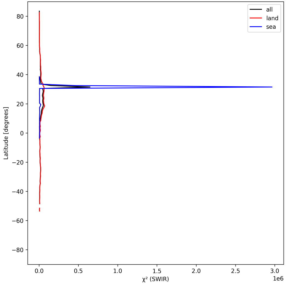
Figure 17: Zonal average of “ \chi^2 (SWIR)” for 2025-04-18 to 2025-04-19.
