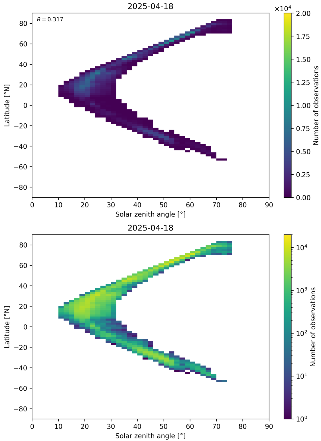
Figure 98: Scatter density plot of “Solar zenith angle” against “Latitude” for 2025-04-18 to 2025-04-19.
