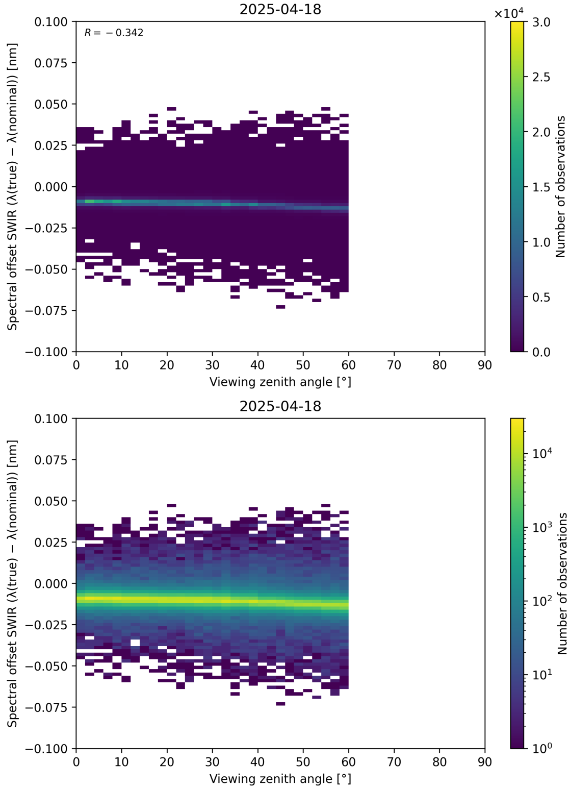
Figure 116: Scatter density plot of “Viewing zenith angle” against “Spectral offset SWIR ( \lambda_{\text{true}} - \lambda_{\text{nominal}} )” for 2025-04-18 to 2025-04-19.
