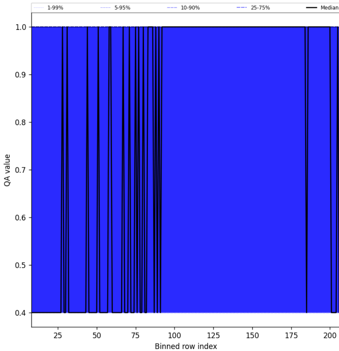
Figure 33: Along track statistics of “QA value” for 2025-04-18 to 2025-04-19
