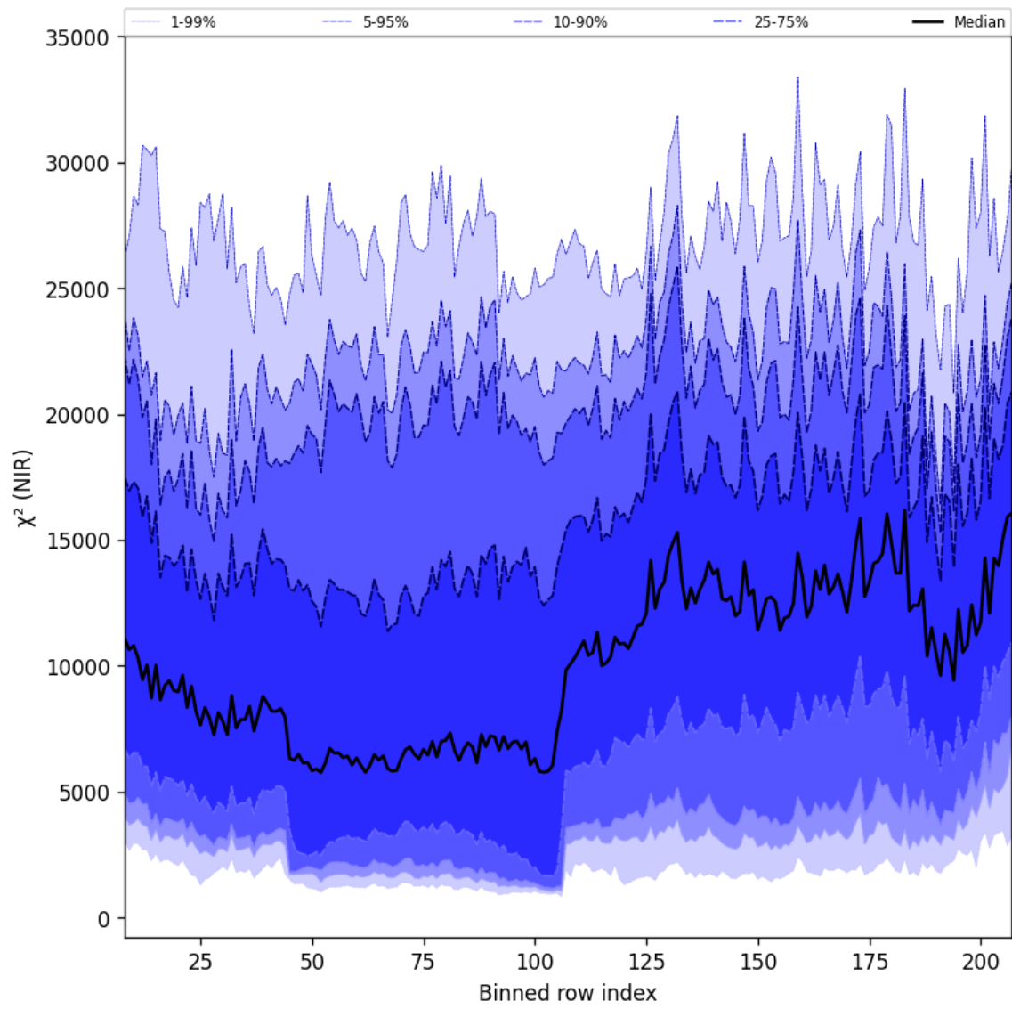
Figure 40: Along track statistics of “ \chi^2 (NIR)” for 2025-04-19 to 2025-04-20
