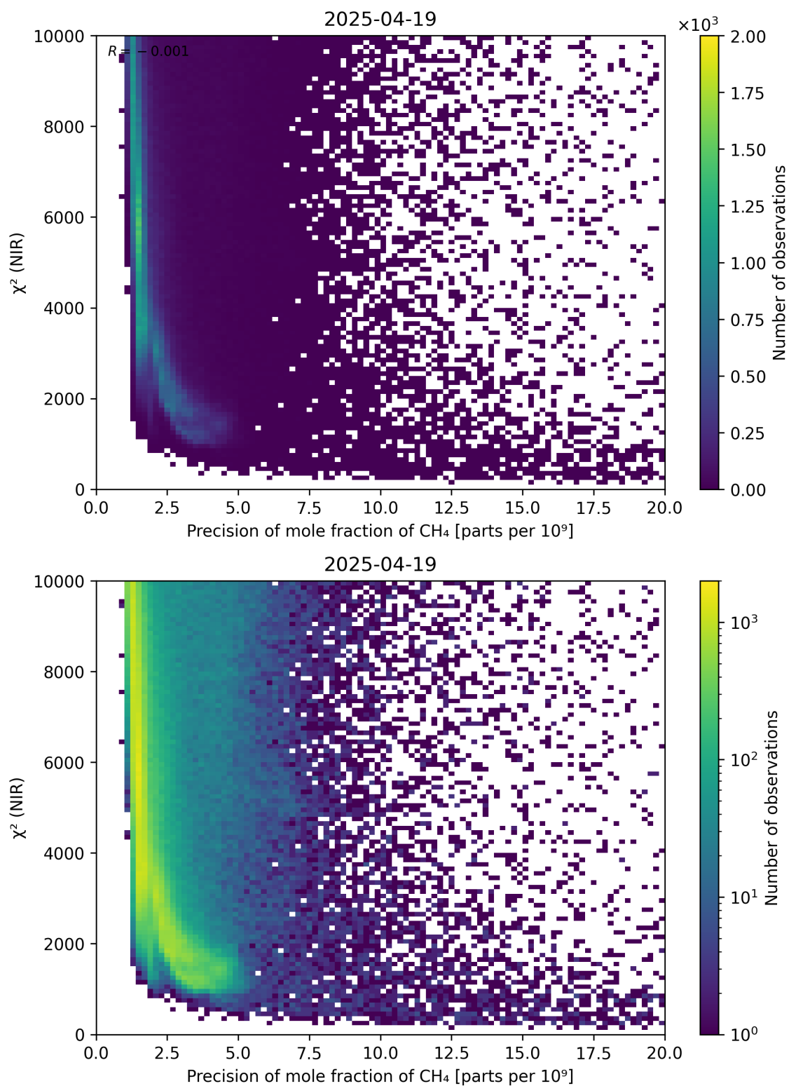
Figure 78: Scatter density plot of “Precision of mole fraction of \text{CH}_4 ” against “ \chi^2 (NIR)” for 2025-04-19 to 2025-04-20.
