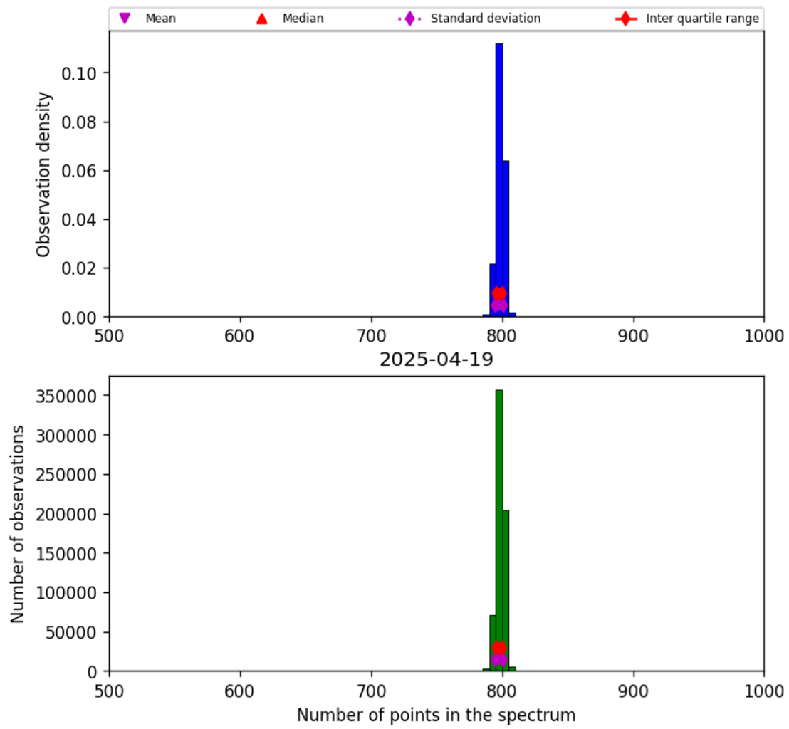
Figure 26: Histogram of “Number of points in the spectrum” for 2025-04-19 to 2025-04-20
