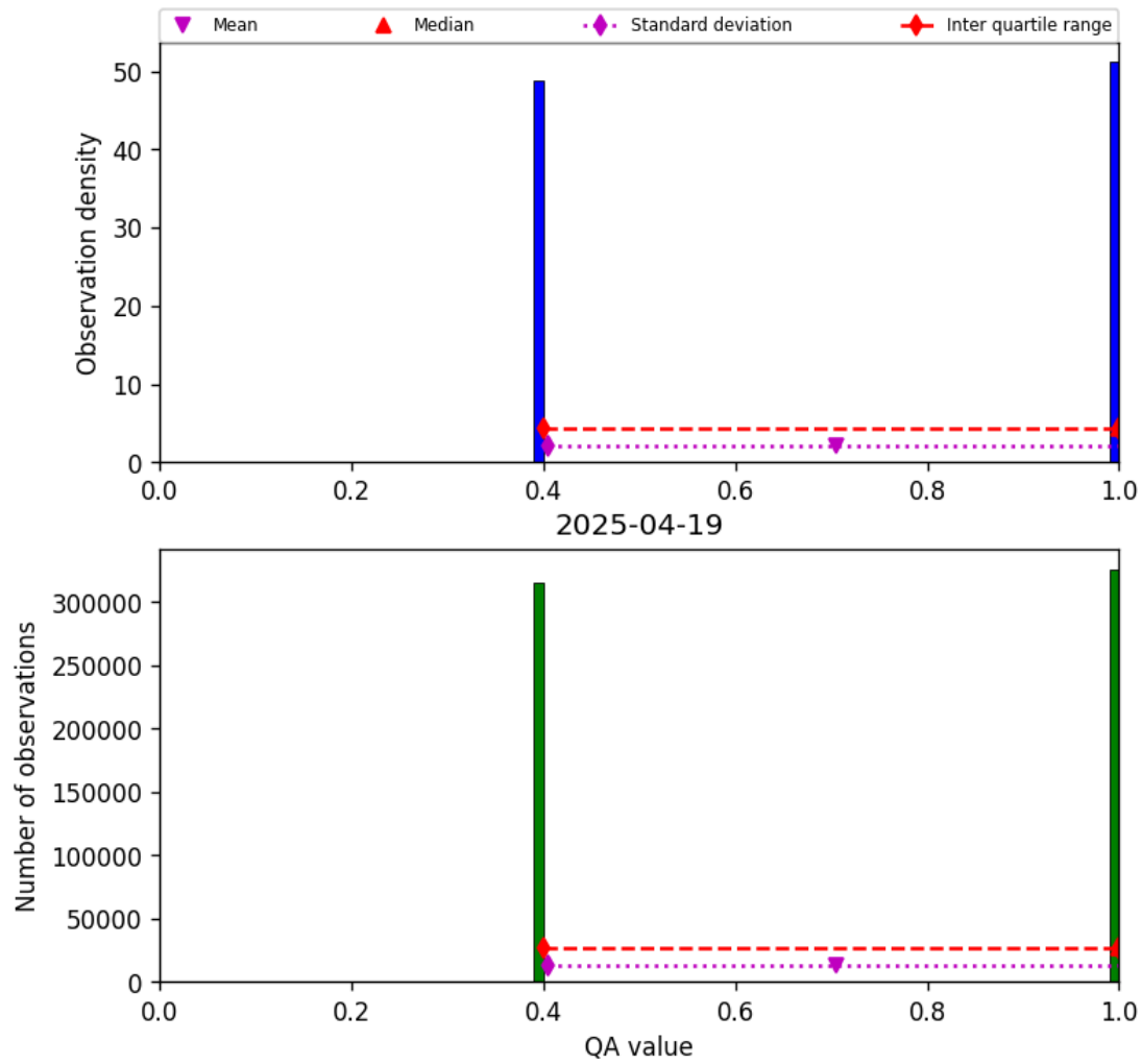
Figure 22: Histogram of “QA value” for 2025-04-19 to 2025-04-20
