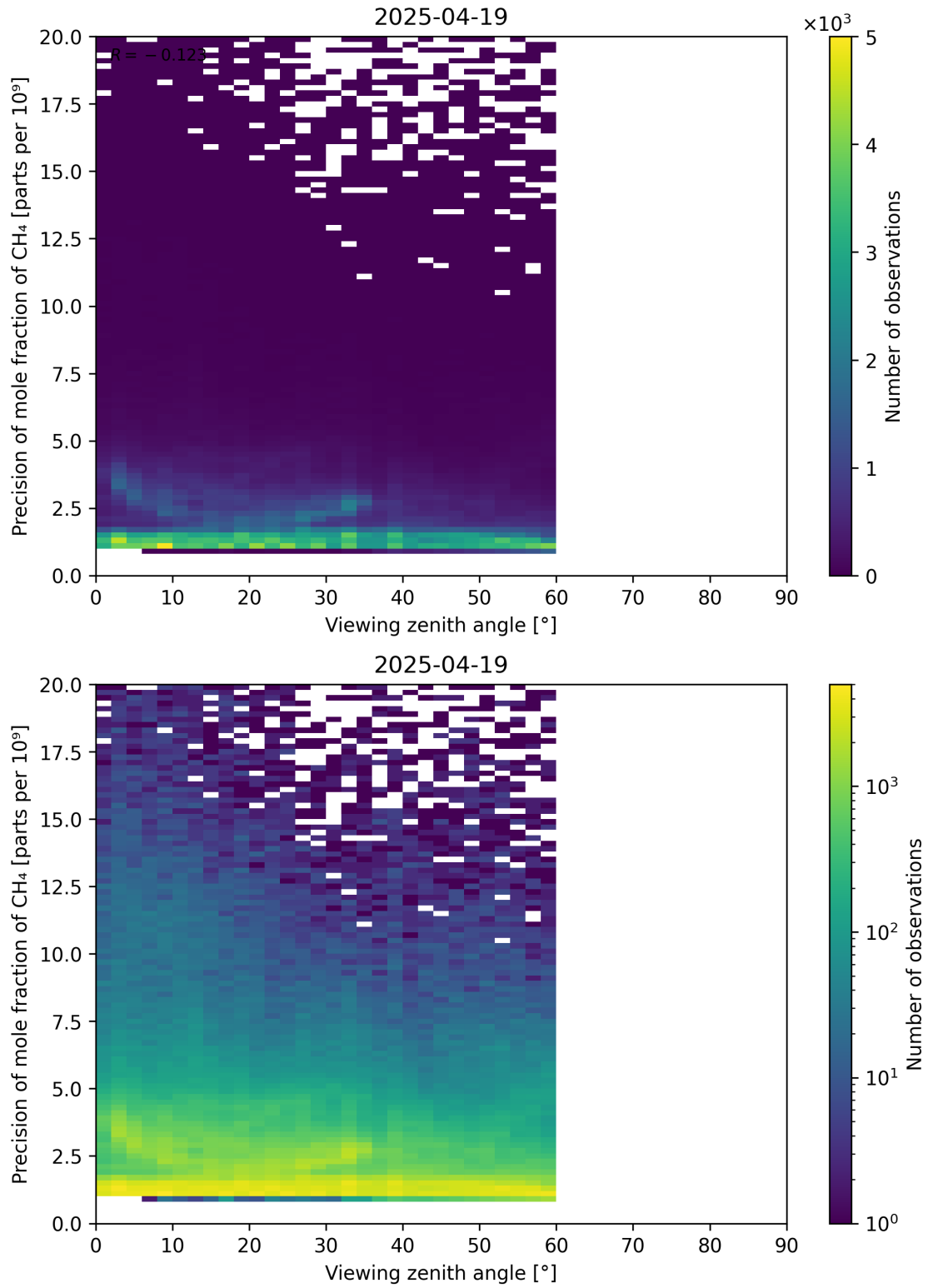
Figure 112: Scatter density plot of “Viewing zenith angle” against “Precision of mole fraction of \text{CH}_4 ” for 2025-04-19 to 2025-04-20.
