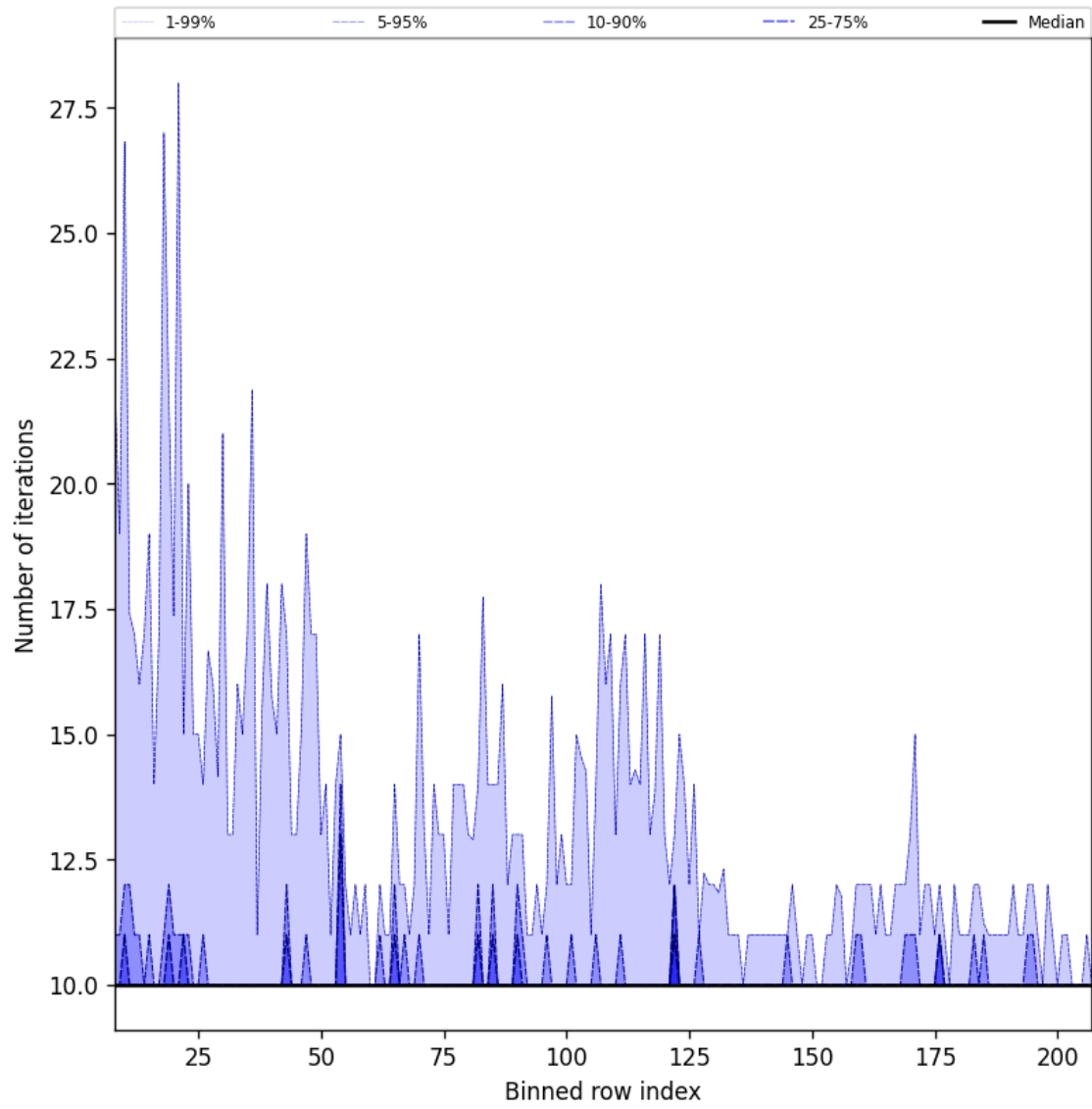
Figure 42: Along track statistics of “Number of iterations” for 2025-04-19 to 2025-04-20
