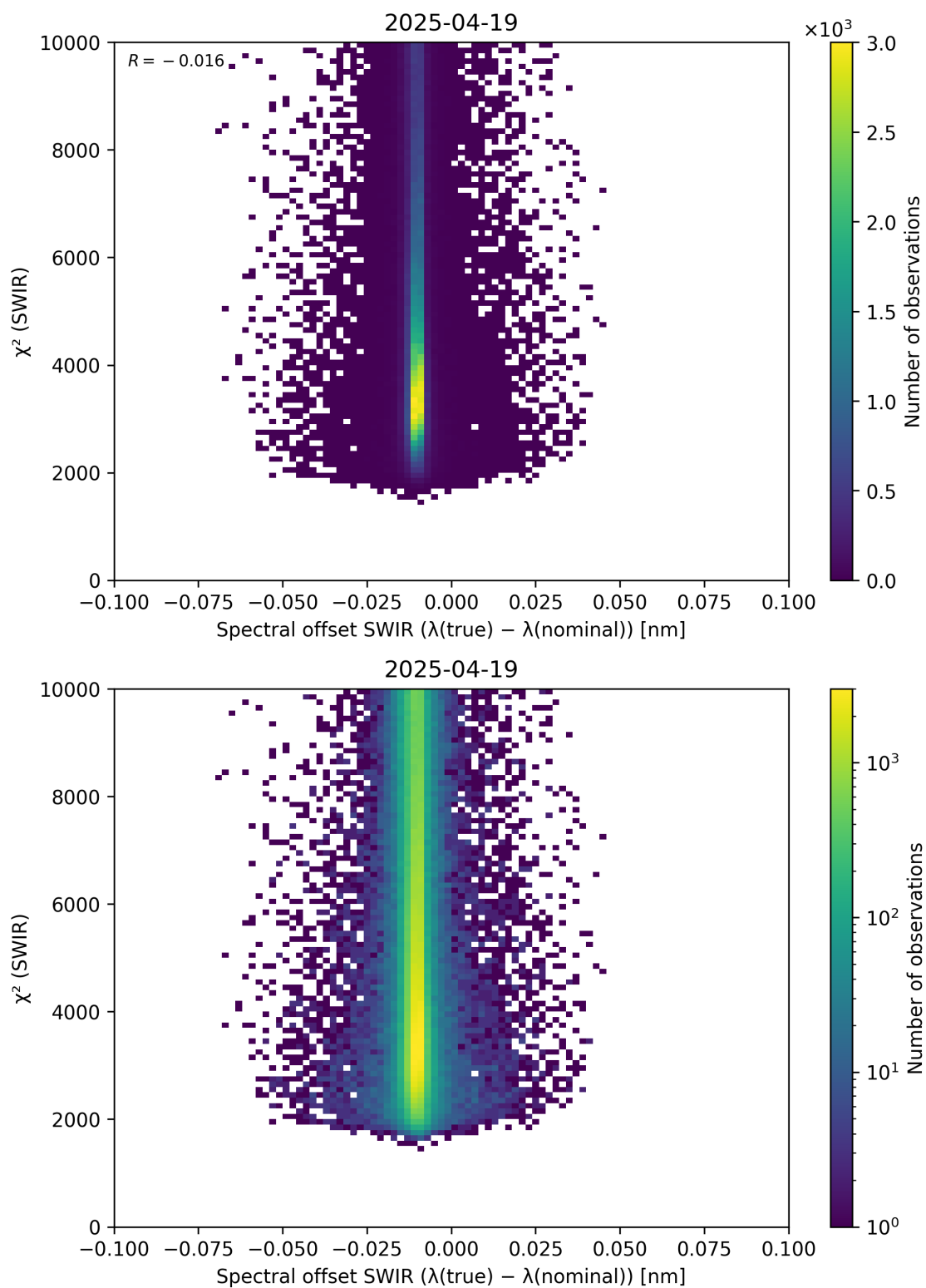
Figure 118: Scatter density plot of “Spectral offset SWIR ( \lambda_{\text{true}} - \lambda_{\text{nominal}} )” against “ \chi^2 (SWIR)” for 2025-04-19 to 2025-04-20.
