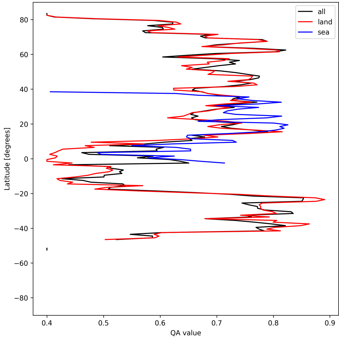
Figure 11: Zonal average of “QA value” for 2025-04-19 to 2025-04-20.
