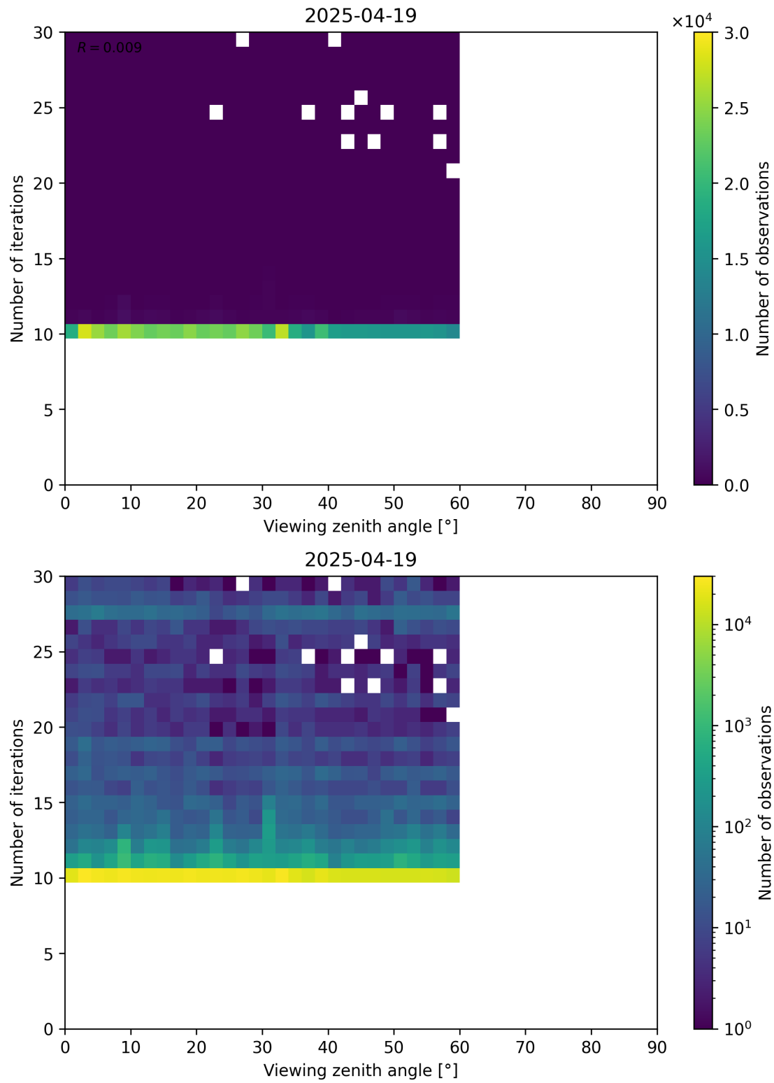
Figure 113: Scatter density plot of “Viewing zenith angle” against “Number of iterations” for 2025-04-19 to 2025-04-20.
