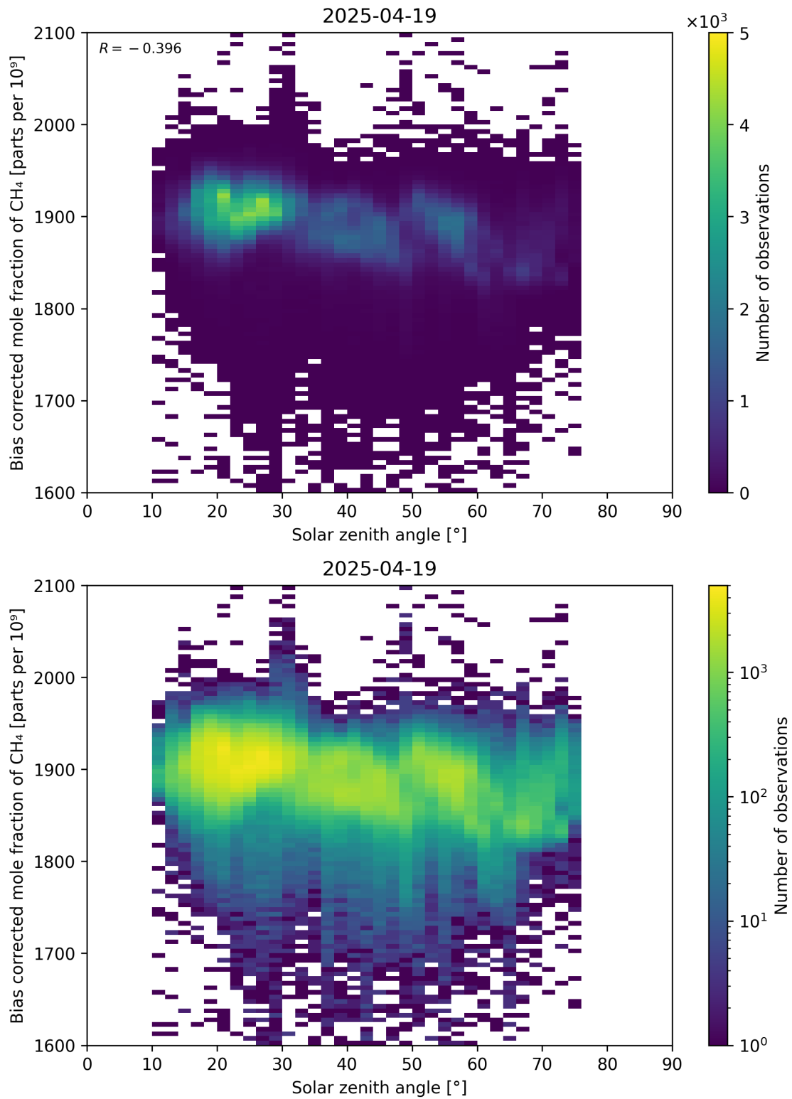
Figure 100: Scatter density plot of “Solar zenith angle” against “Bias corrected mole fraction of CH 4 ” for 2025-04-19 to 2025-04-20.
