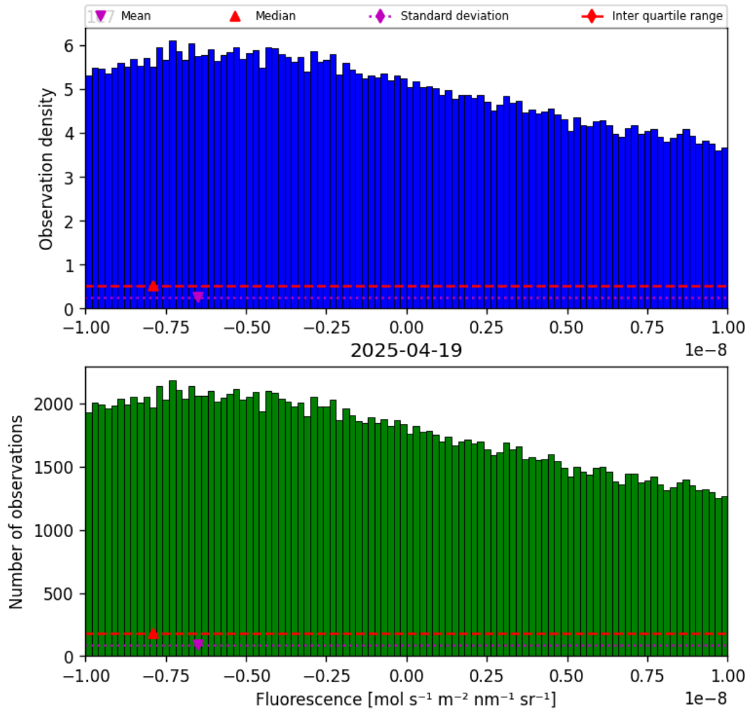
Figure 32: Histogram of “Fluorescence” for 2025-04-19 to 2025-04-20
