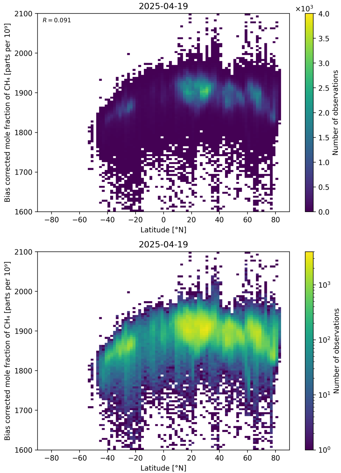
Figure 58: Scatter density plot of “Latitude” against “Bias corrected mole fraction of CH 4 ” for 2025-04-19 to 2025-04-20.
