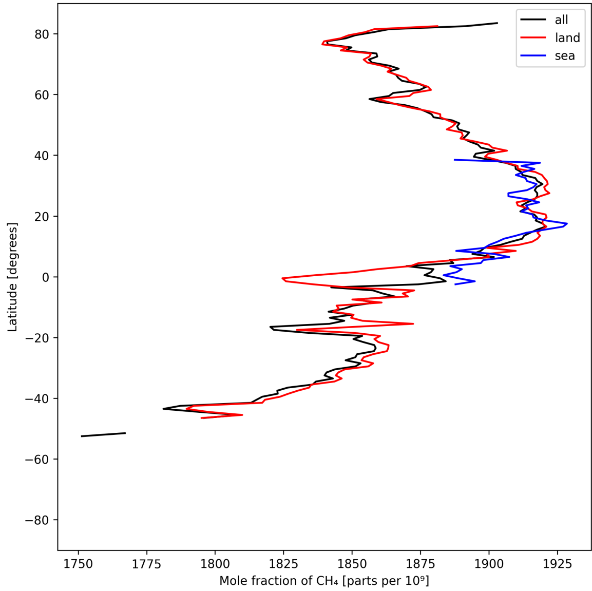
Figure 12: Zonal average of “Mole fraction of \text{CH}_4 ” for 2025-04-19 to 2025-04-20.
