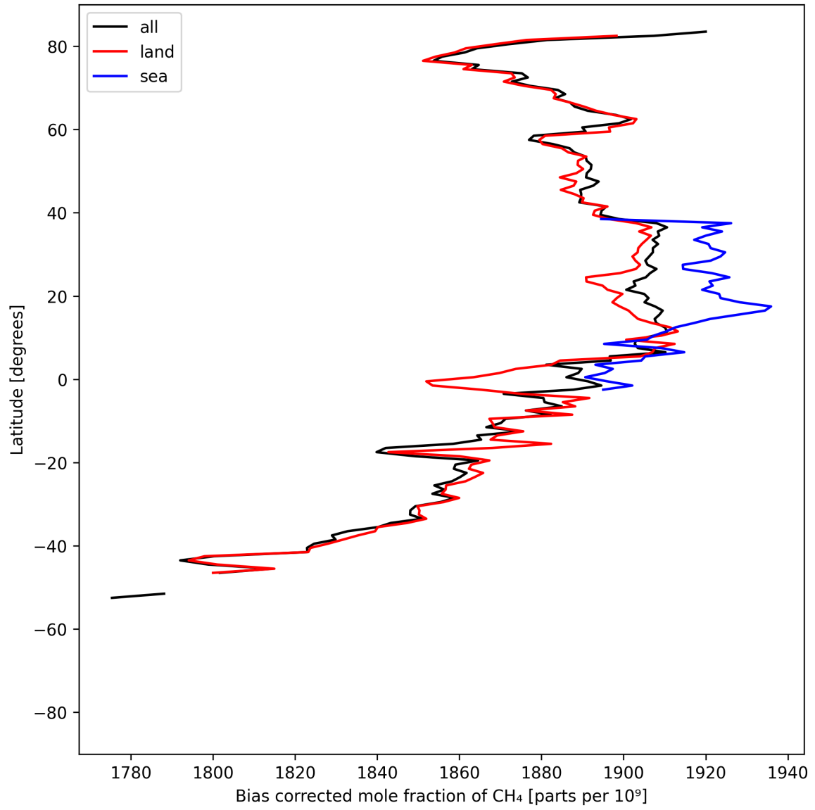
Figure 14: Zonal average of “Bias corrected mole fraction of CH 4 ” for 2025-04-19 to 2025-04-20.
