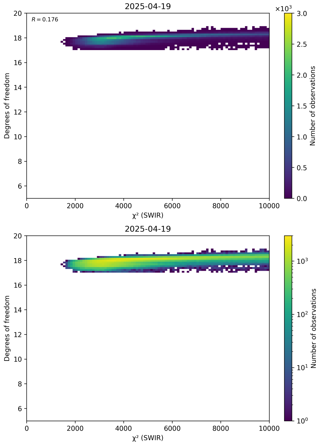
Figure 48: Scatter density plot of “ \chi^2 (SWIR)” against “Degrees of freedom” for 2025-04-19 to 2025-04-20.
