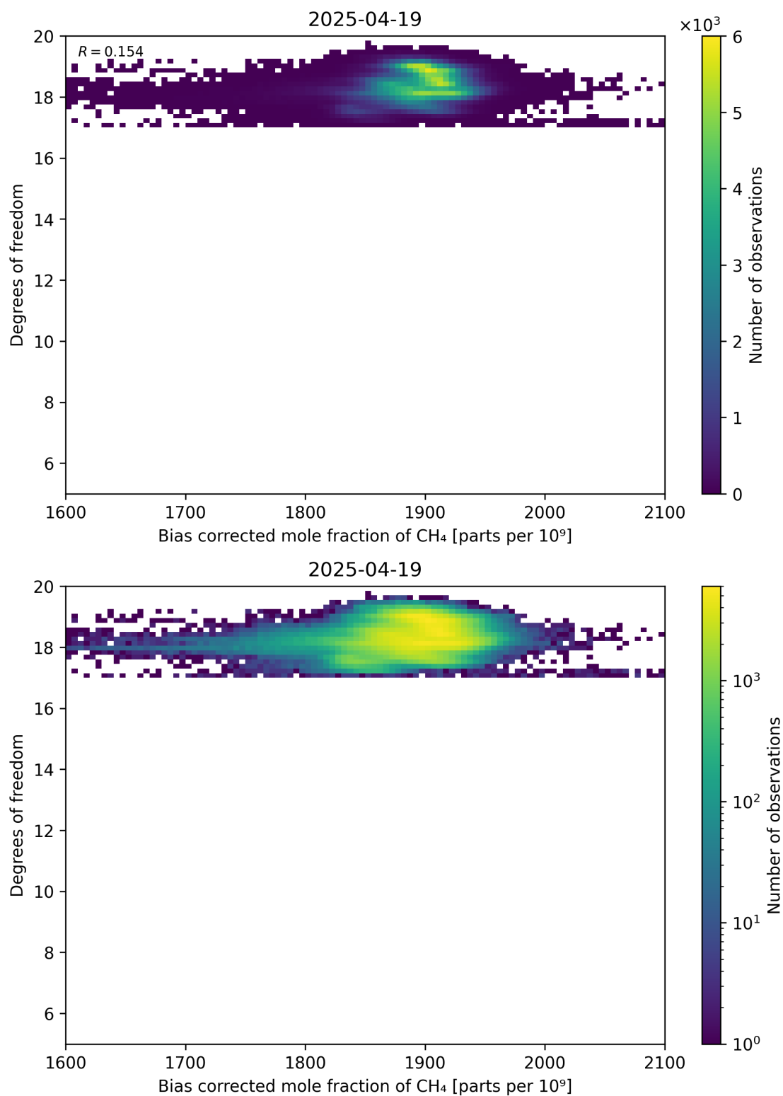
Figure 65: Scatter density plot of “Bias corrected mole fraction of CH 4 ” against “Degrees of freedom” for 2025-04-19 to 2025-04-20.
