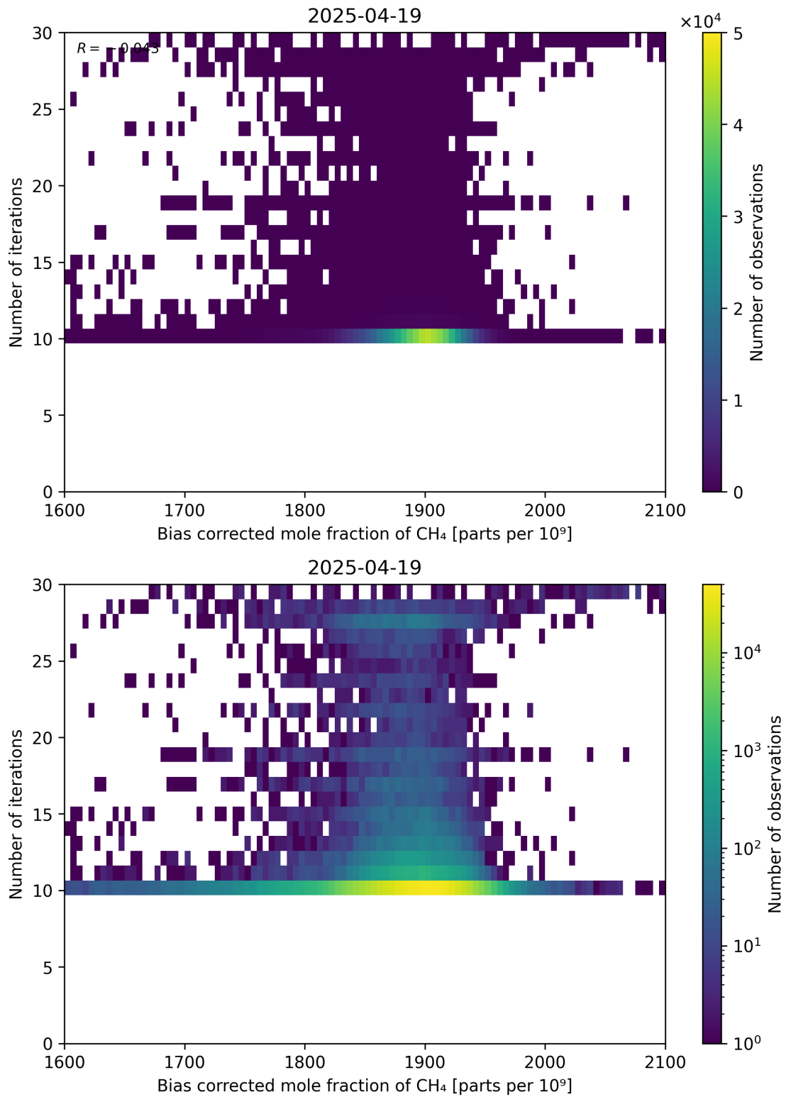
Figure 67: Scatter density plot of “Bias corrected mole fraction of CH 4 ” against “Number of iterations” for 2025-04-19 to 2025-04-20.
