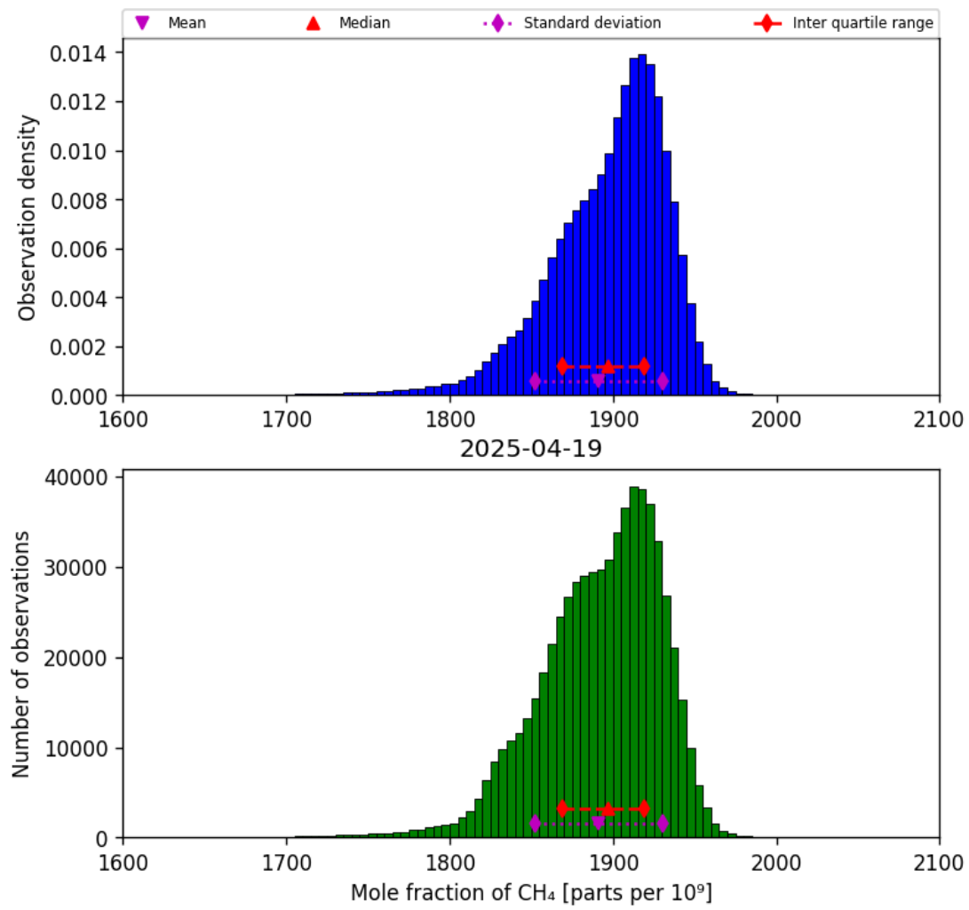
Figure 23: Histogram of “Mole fraction of CH 4 ” for 2025-04-19 to 2025-04-20
