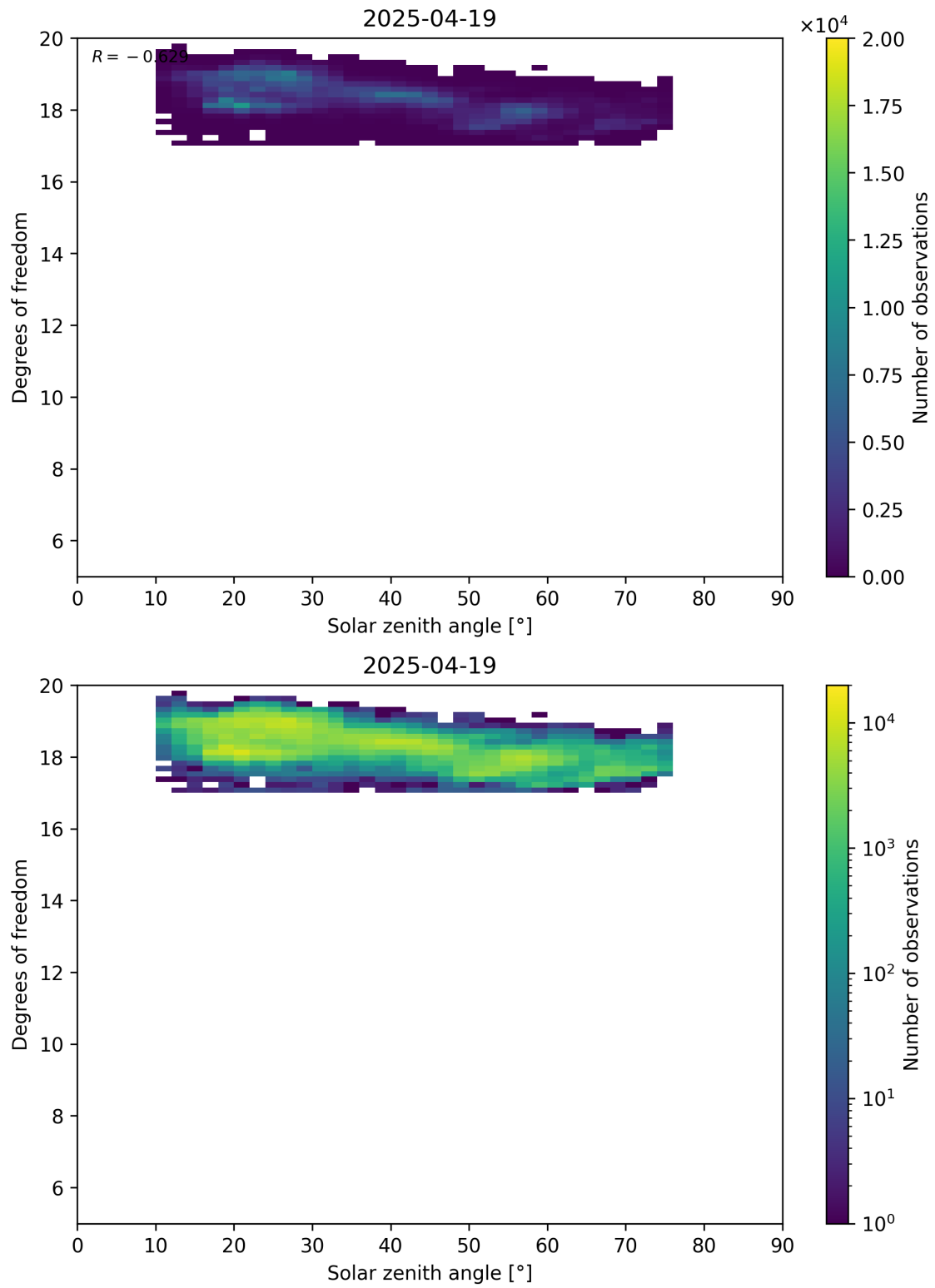
Figure 96: Scatter density plot of “Solar zenith angle” against “Degrees of freedom” for 2025-04-19 to 2025-04-20.
