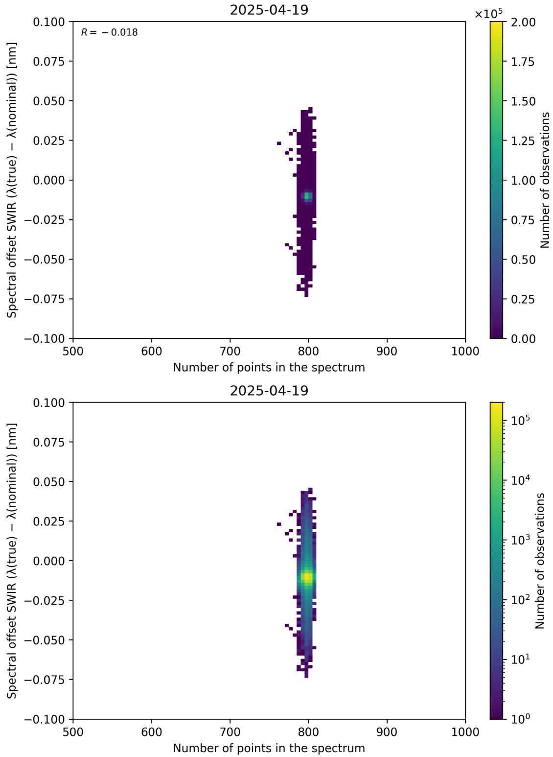
Figure 93: Scatter density plot of “Number of points in the spectrum” against “Spectral offset SWIR ( \lambda_{\text{true}} - \lambda_{\text{nominal}} )” for 2025-04-19 to 2025-04-20.
