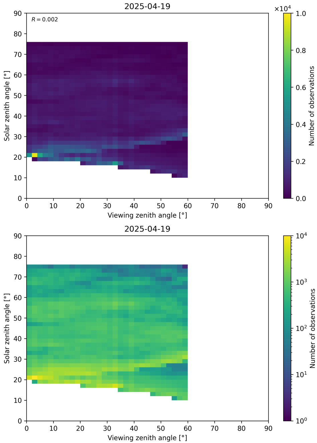
Figure 115: Scatter density plot of “Viewing zenith angle” against “Solar zenith angle” for 2025-04-19 to 2025-04-20.
