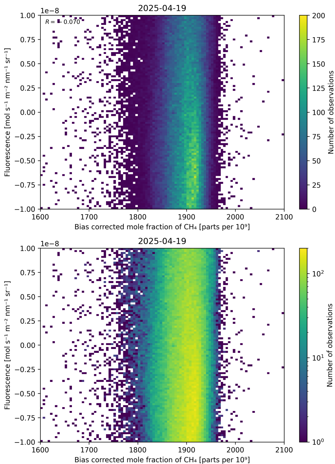
Figure 66: Scatter density plot of “Bias corrected mole fraction of \text{CH}_4 ” against “Fluorescence” for 2025-04-19 to 2025-04-20.
