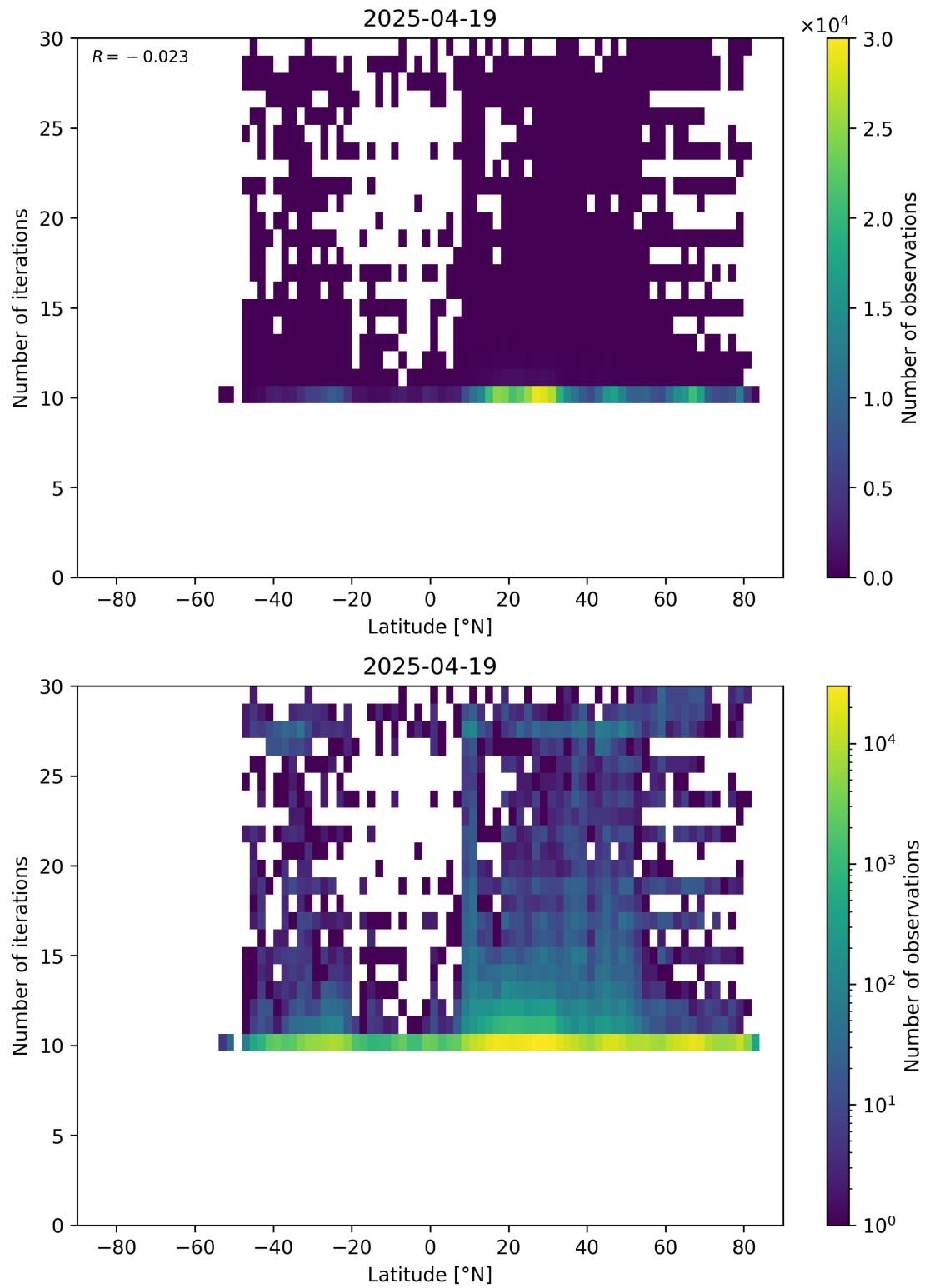
Figure 60: Scatter density plot of “Latitude” against “Number of iterations” for 2025-04-19 to 2025-04-20.
