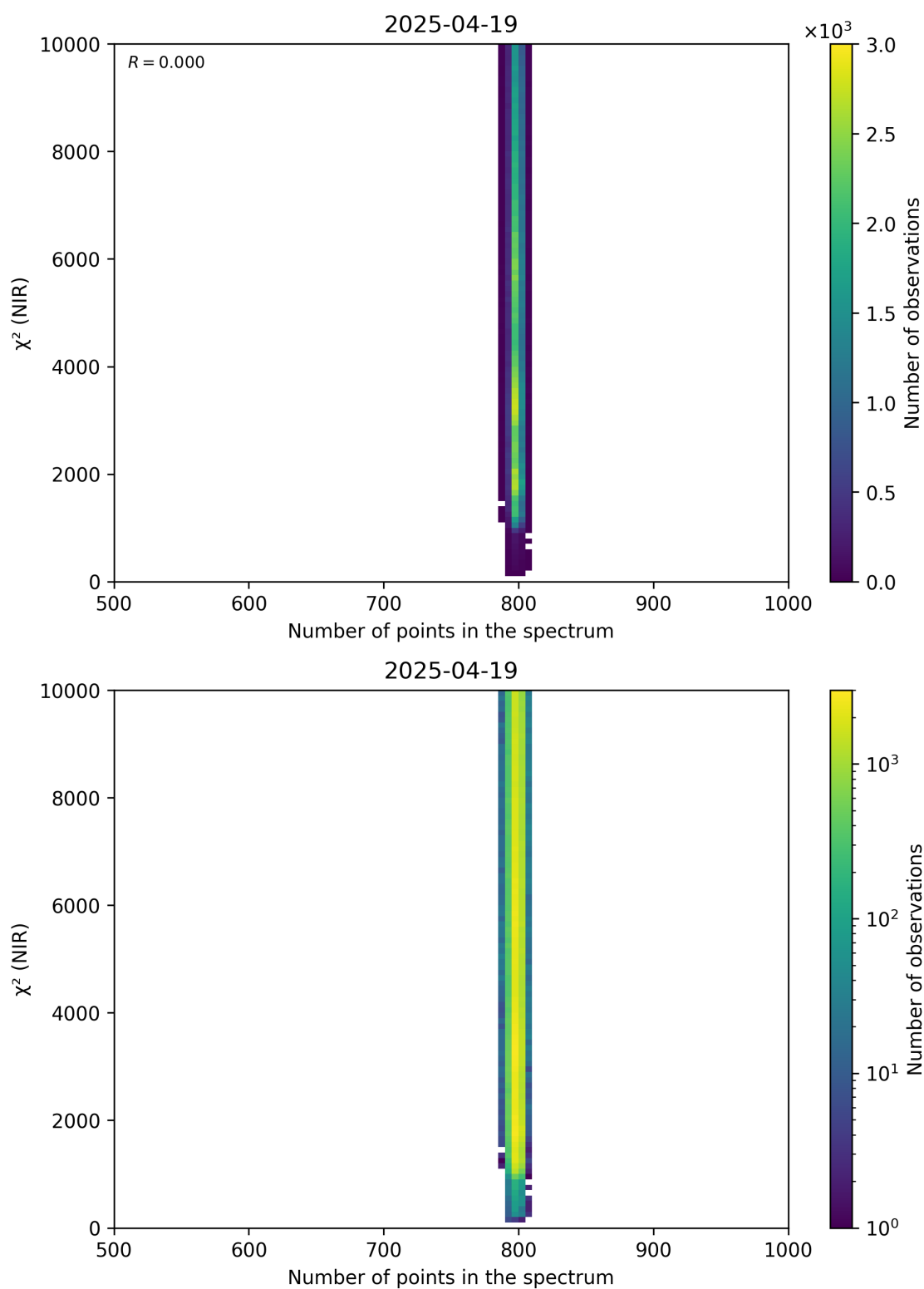
Figure 88: Scatter density plot of “Number of points in the spectrum” against “ \chi^2 (NIR)” for 2025-04-19 to 2025-04-20.
