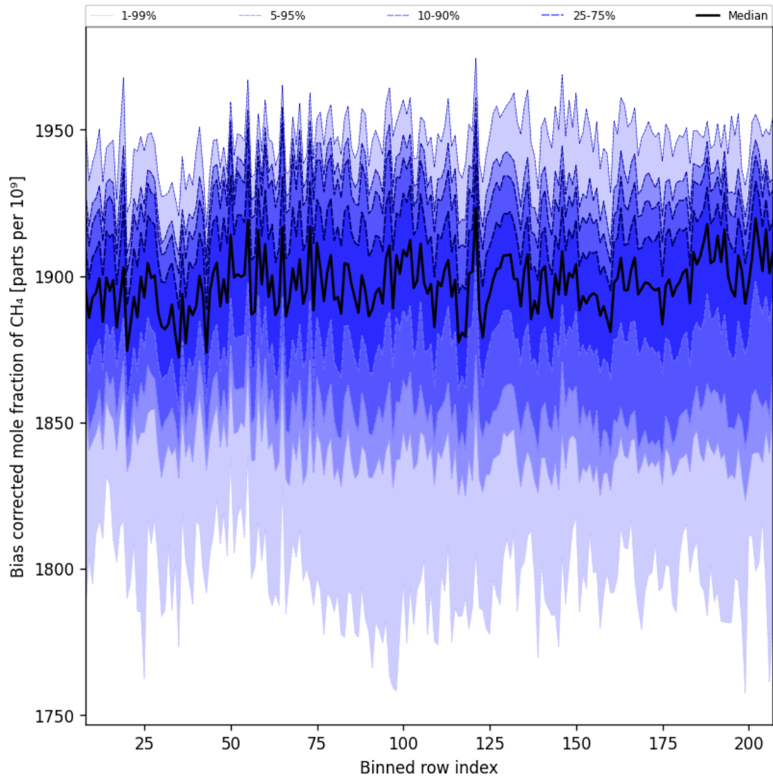
Figure 36: Along track statistics of “Bias corrected mole fraction of CH 4 ” for 2025-04-19 to 2025-04-20
