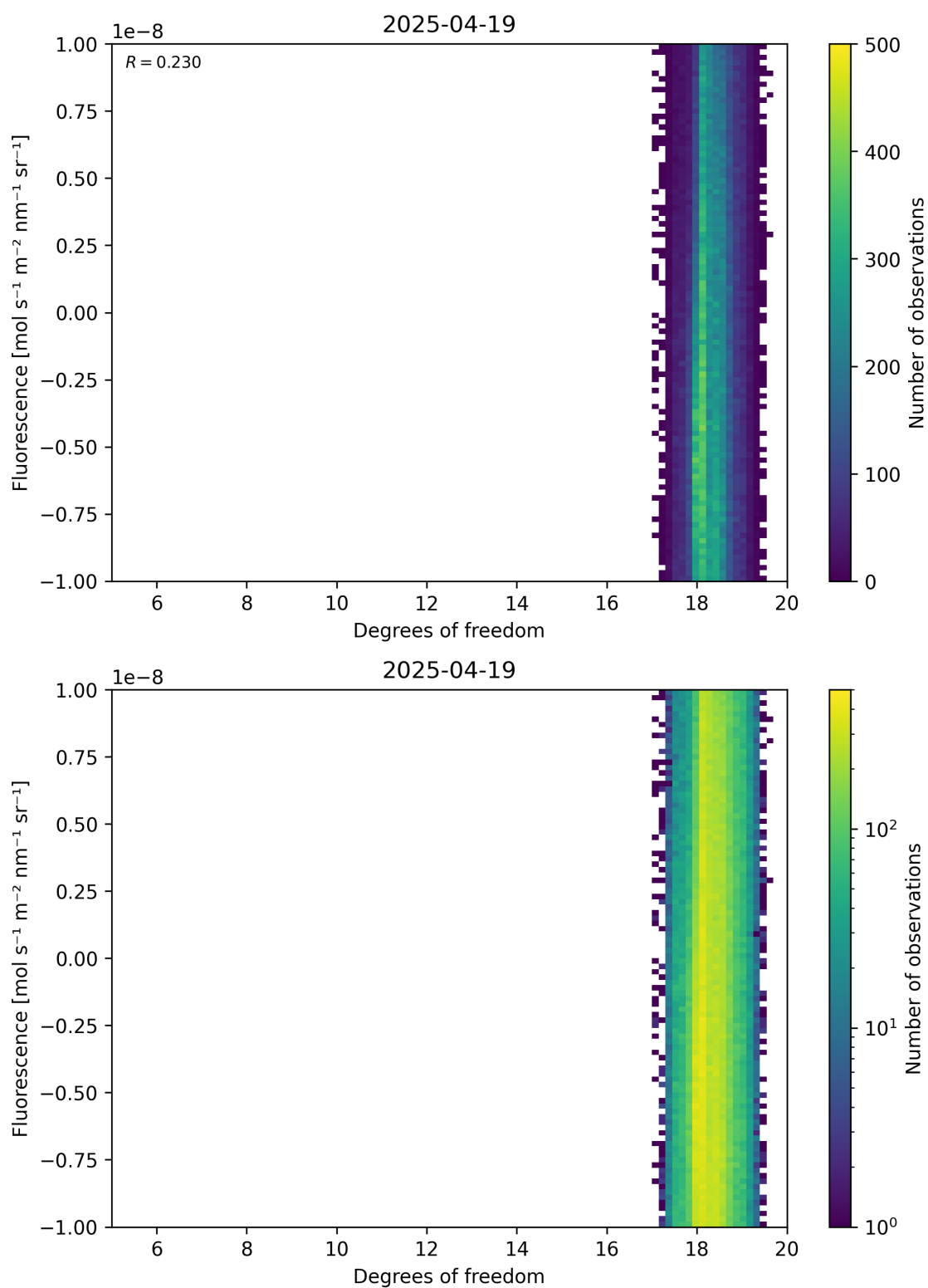
Figure 51: Scatter density plot of “Degrees of freedom” against “Fluorescence” for 2025-04-19 to 2025-04-20.
