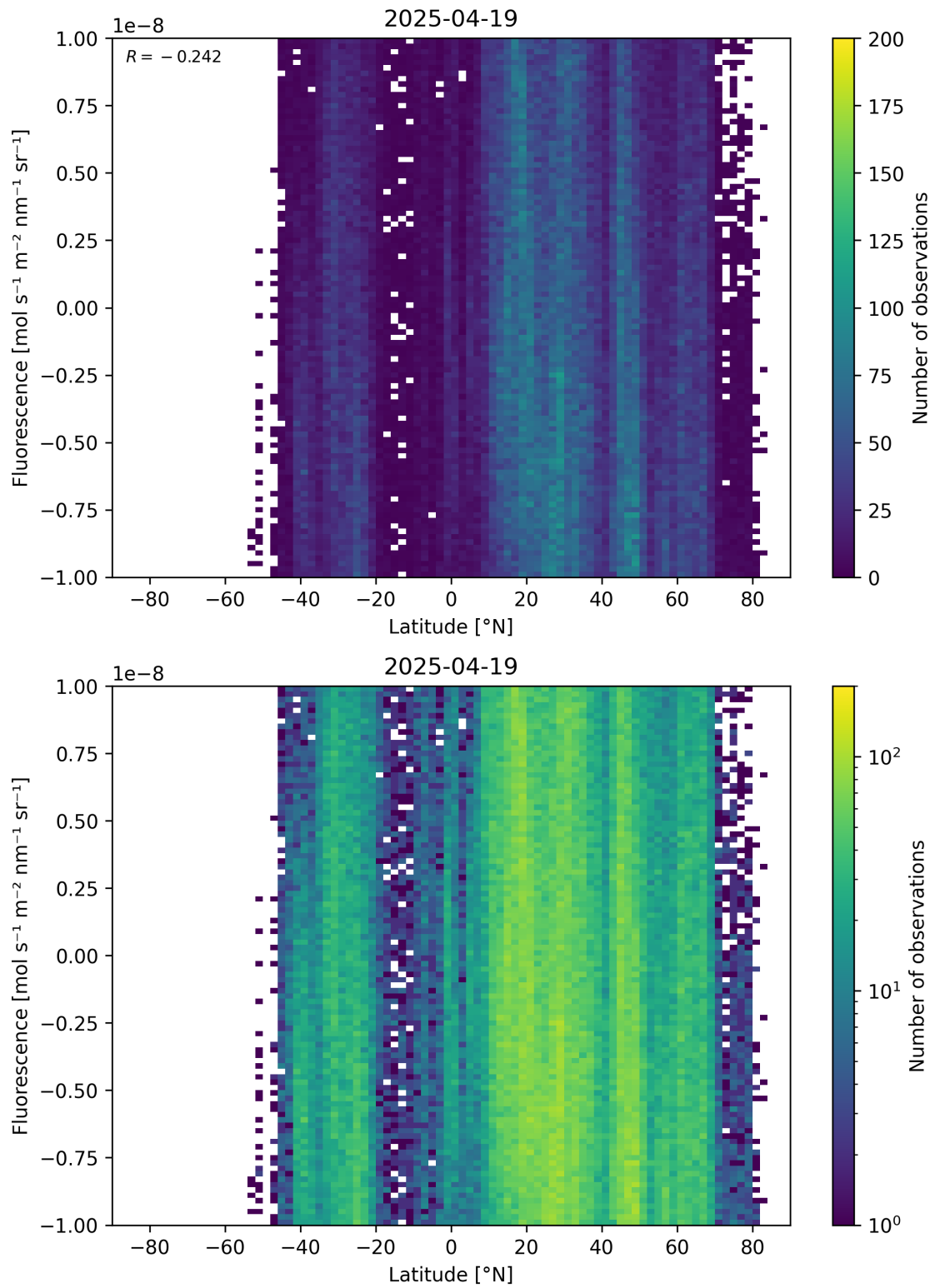
Figure 56: Scatter density plot of “Latitude” against “Fluorescence” for 2025-04-19 to 2025-04-20.
