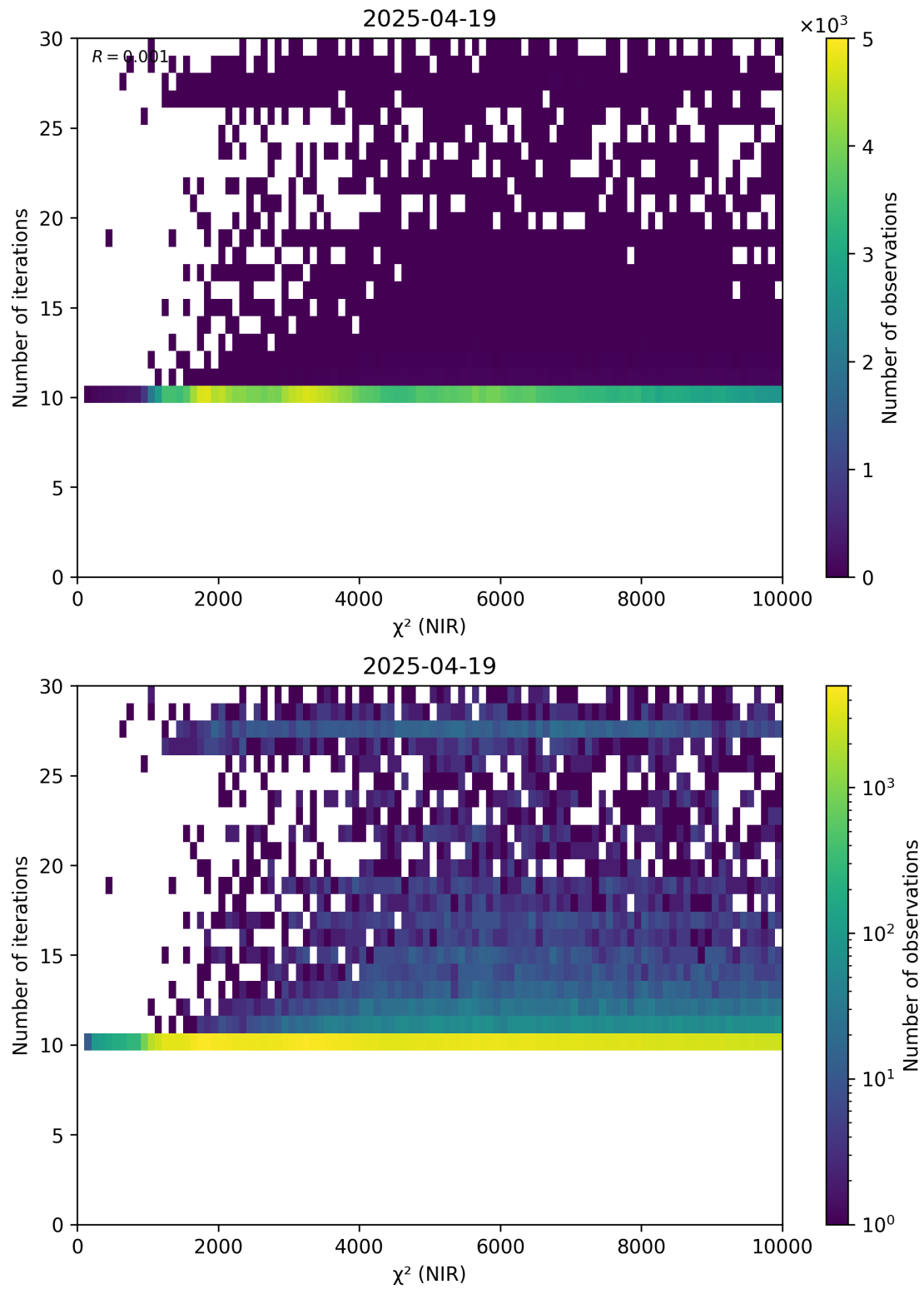
Figure 46: Scatter density plot of “ \chi^2 (NIR)” against “Number of iterations” for 2025-04-19 to 2025-04-20.
