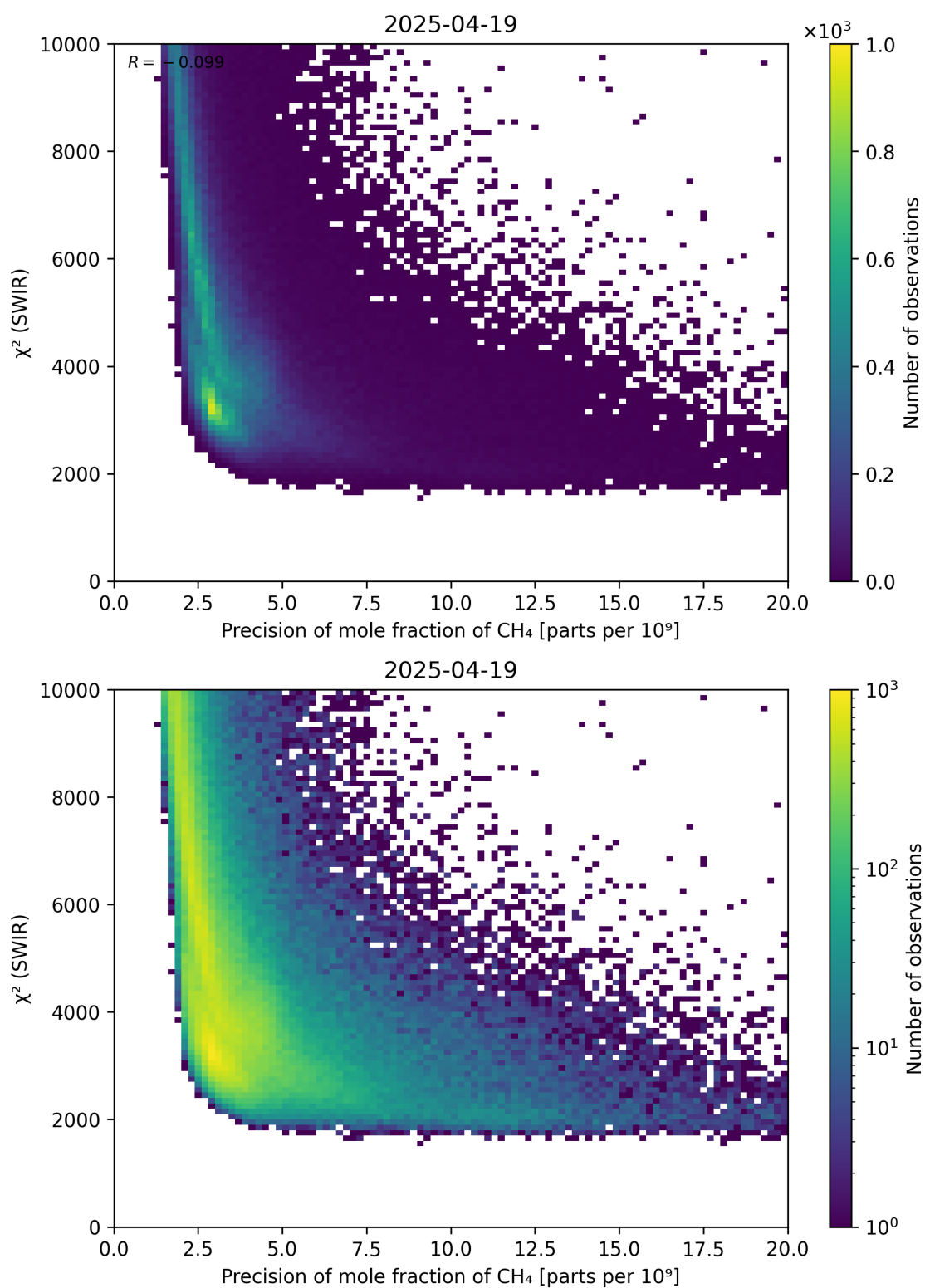
Figure 79: Scatter density plot of “Precision of mole fraction of CH 4 ” against “ \chi^2 (SWIR)” for 2025-04-19 to 2025-04-20.
