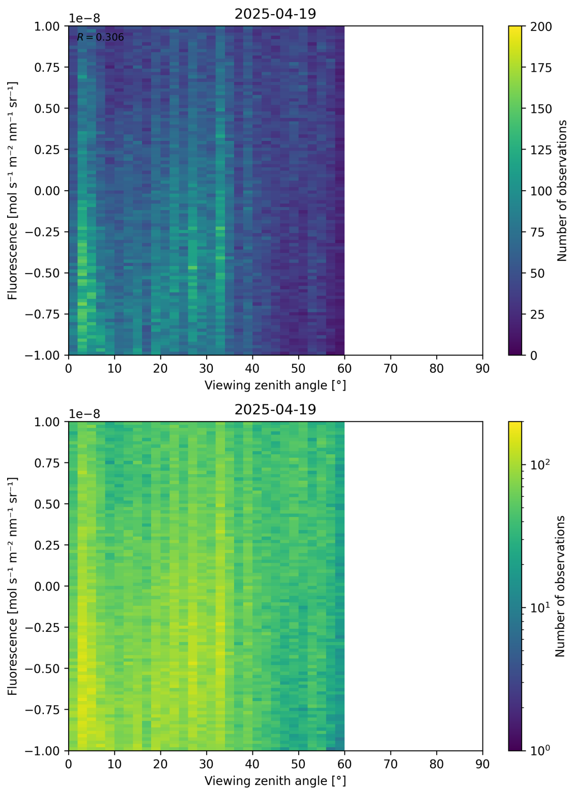
Figure 108: Scatter density plot of “Viewing zenith angle” against “Fluorescence” for 2025-04-19 to 2025-04-20.
