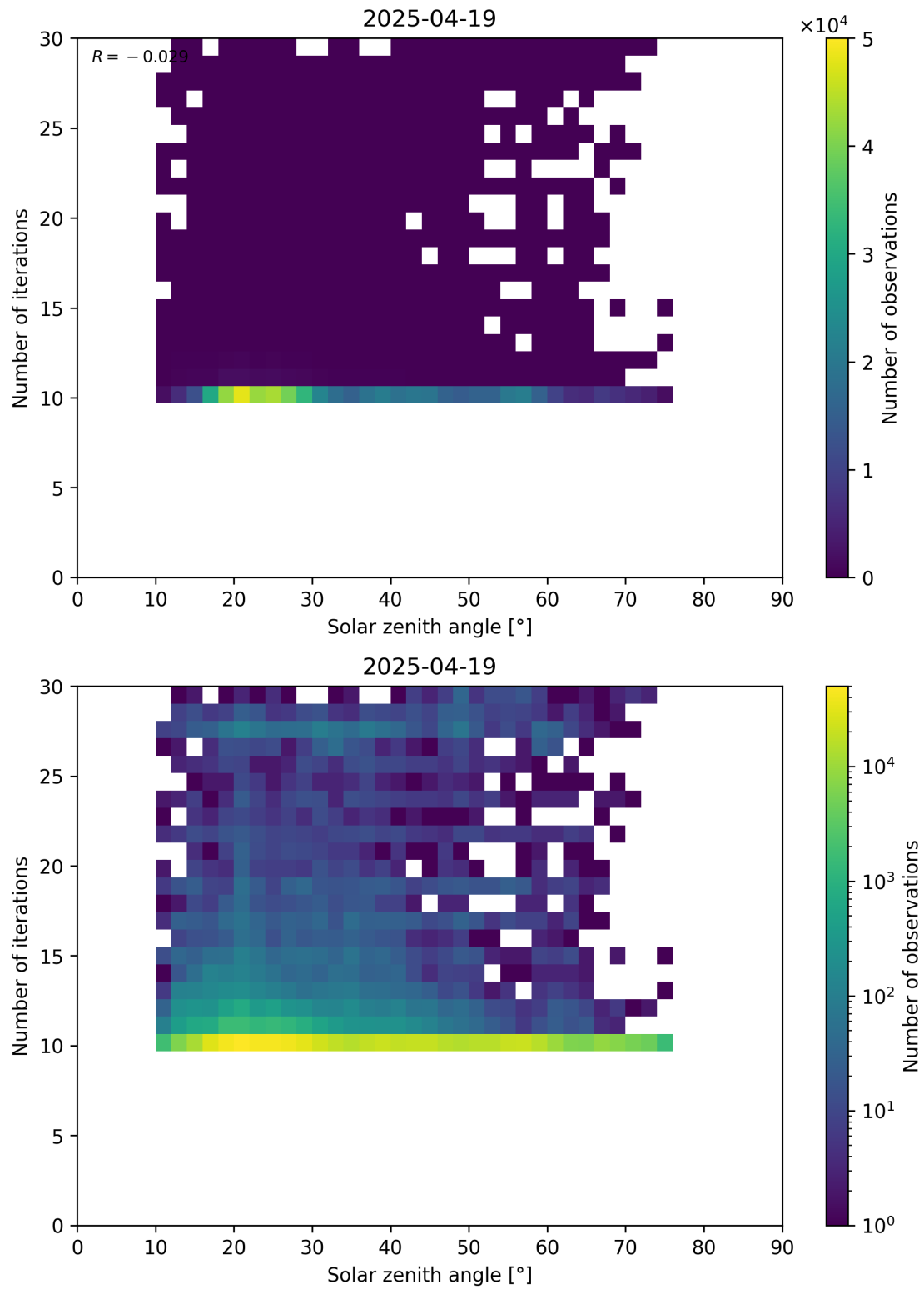
Figure 102: Scatter density plot of “Solar zenith angle” against “Number of iterations” for 2025-04-19 to 2025-04-20.
