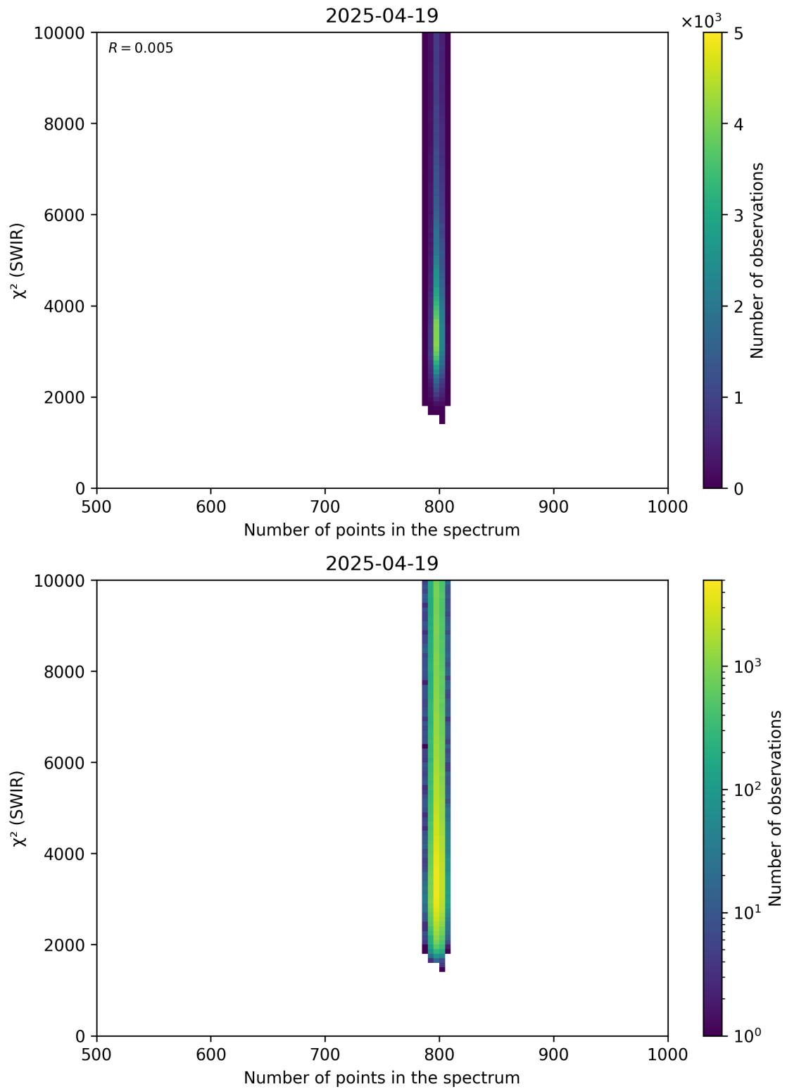
Figure 89: Scatter density plot of “Number of points in the spectrum” against “ \chi^2 (SWIR)” for 2025-04-19 to 2025-04-20.
