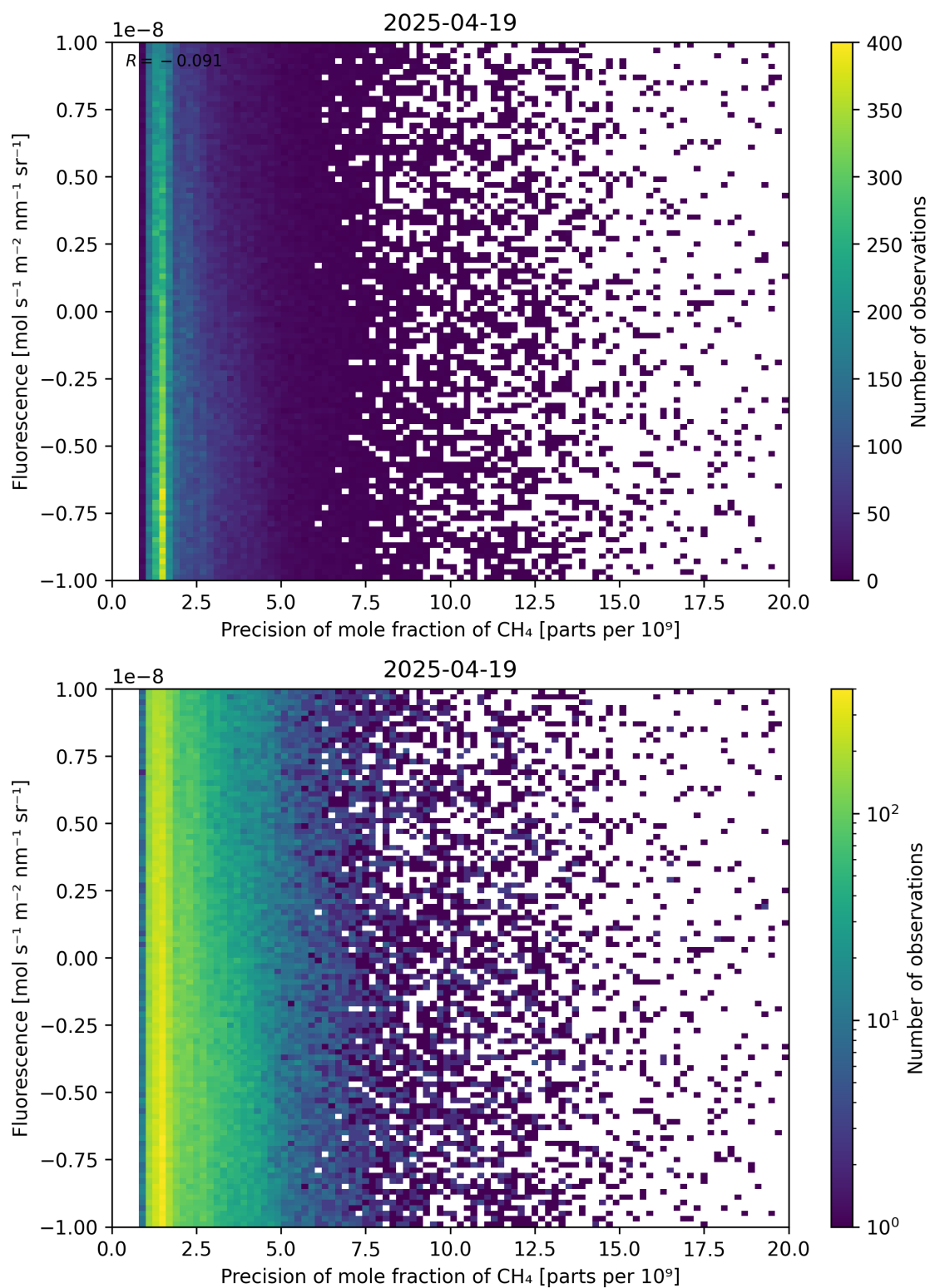
Figure 81: Scatter density plot of “Precision of mole fraction of CH 4 ” against “Fluorescence” for 2025-04-19 to 2025-04-20.
