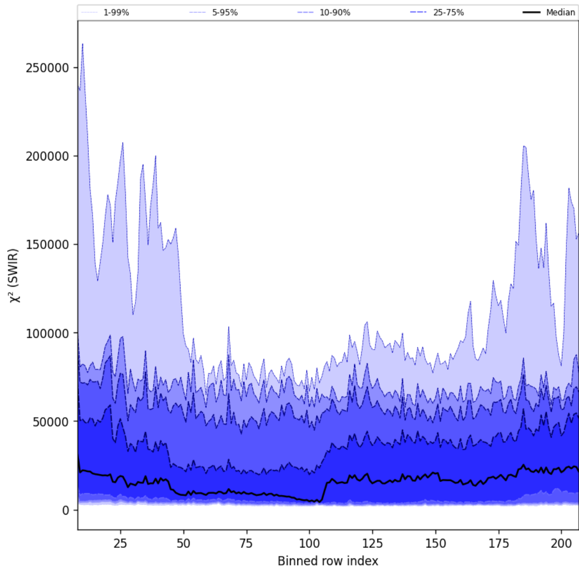
Figure 39: Along track statistics of " \chi^2 (SWIR)" for 2025-04-19 to 2025-04-20
