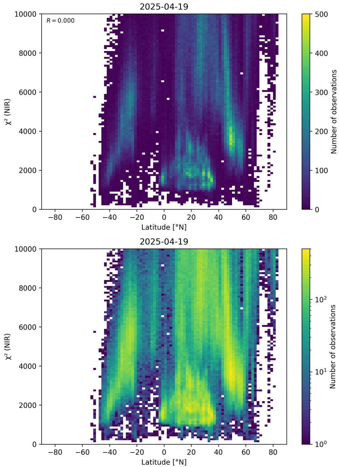
Figure 53: Scatter density plot of “Latitude” against “ \chi^2 (NIR)” for 2025-04-19 to 2025-04-20.
