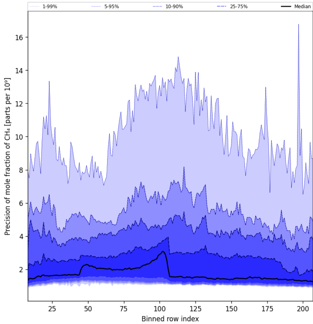
Figure 35: Along track statistics of “Precision of mole fraction of CH 4 ” for 2025-04-19 to 2025-04-20
