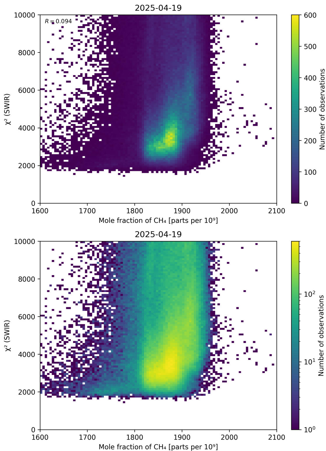
Figure 71: Scatter density plot of “Mole fraction of CH 4 ” against “ \chi^2 (SWIR)” for 2025-04-19 to 2025-04-20.
