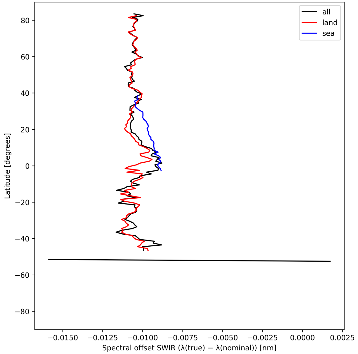
Figure 16: Zonal average of “Spectral offset SWIR ( \lambda_{\text{true}} - \lambda_{\text{nominal}} )” for 2025-04-19 to 2025-04-20.
