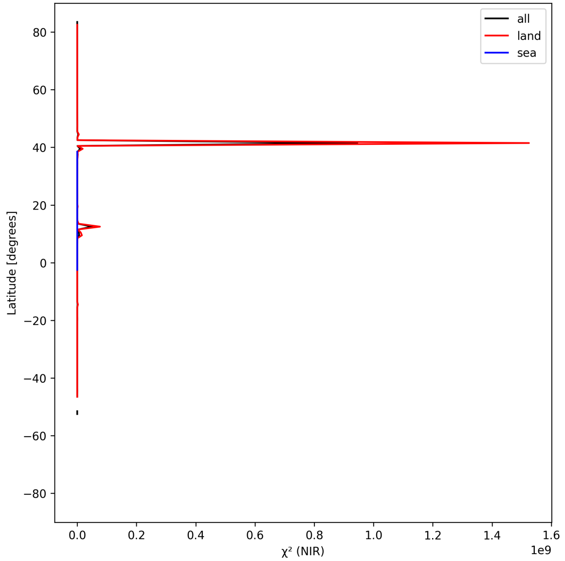
Figure 18: Zonal average of “ \chi^2 (NIR)” for 2025-04-19 to 2025-04-20.
