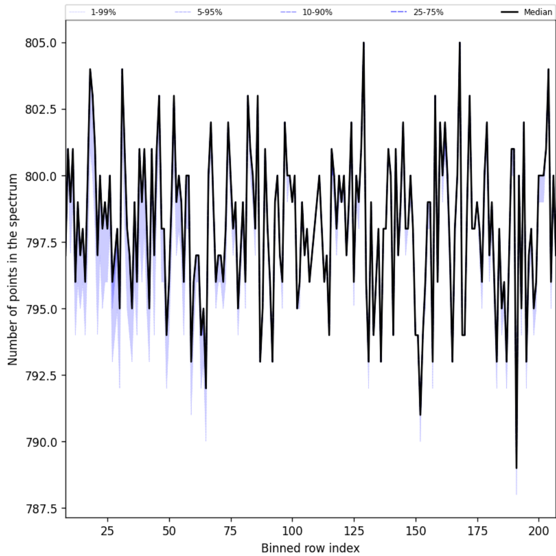
Figure 37: Along track statistics of “Number of points in the spectrum” for 2025-04-19 to 2025-04-20
