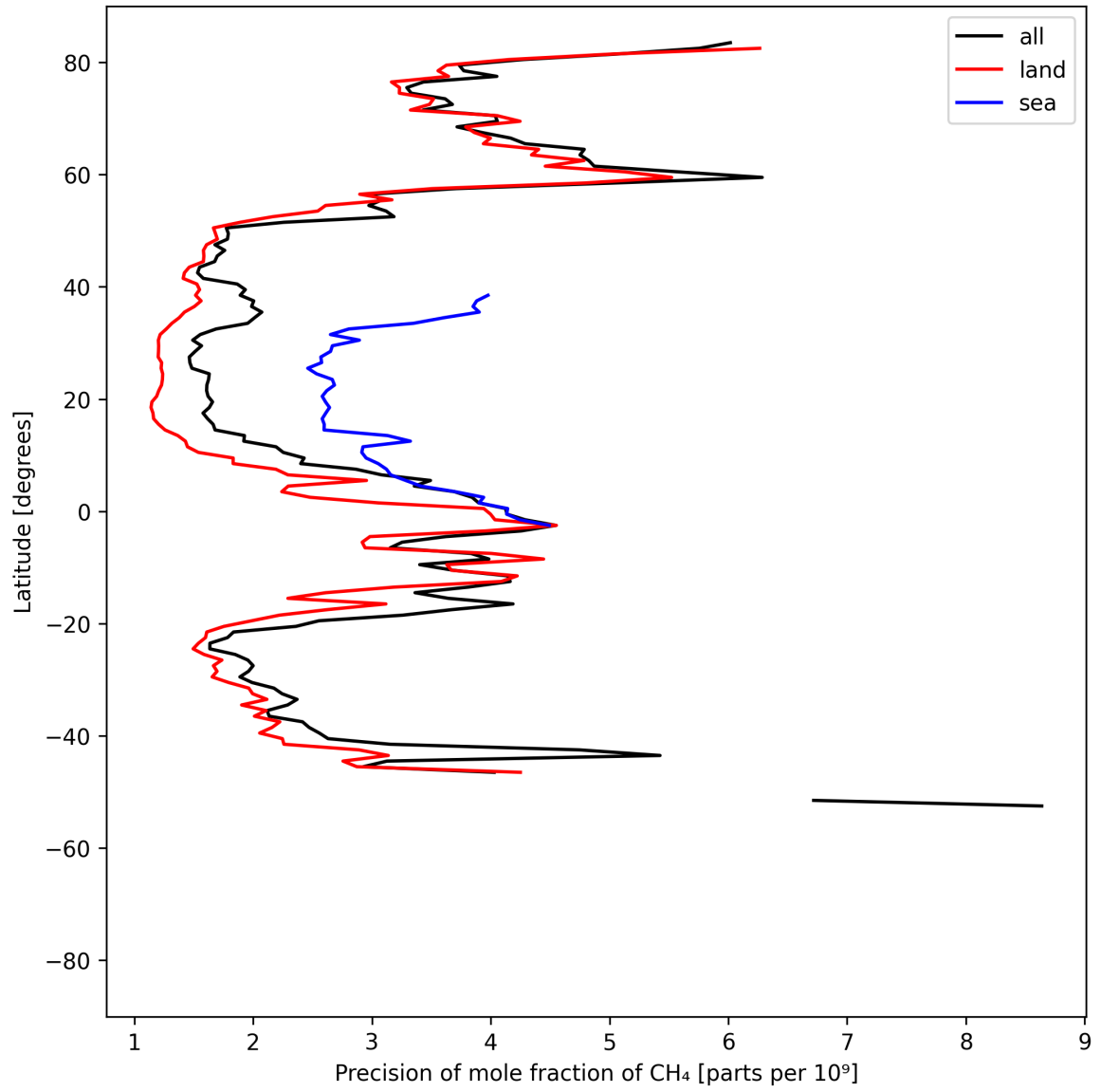
Figure 13: Zonal average of “Precision of mole fraction of CH 4 ” for 2025-04-19 to 2025-04-20.
