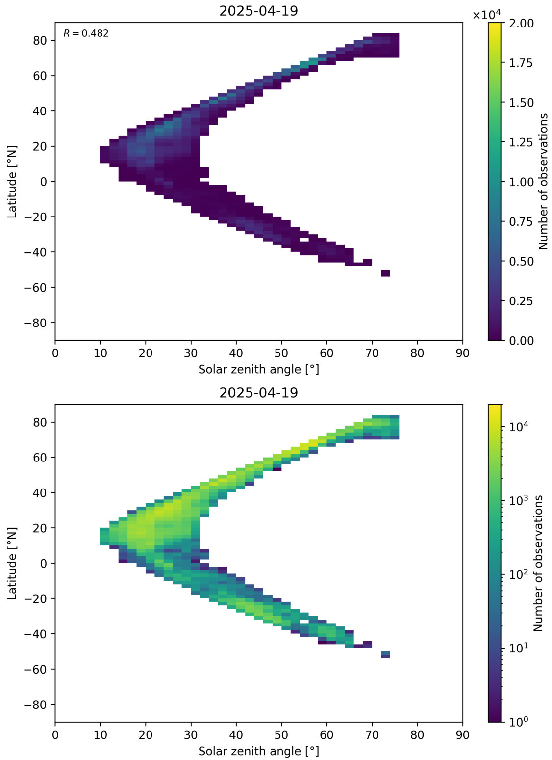
Figure 98: Scatter density plot of “Solar zenith angle” against “Latitude” for 2025-04-19 to 2025-04-20.
