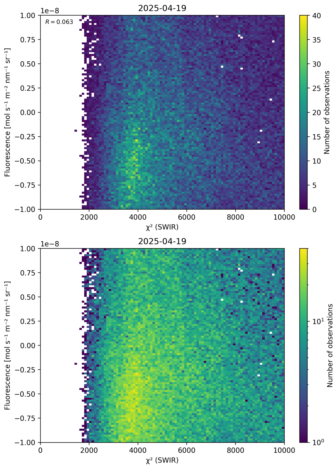
Figure 49: Scatter density plot of “ \chi^2 (SWIR)” against “Fluorescence” for 2025-04-19 to 2025-04-20.
