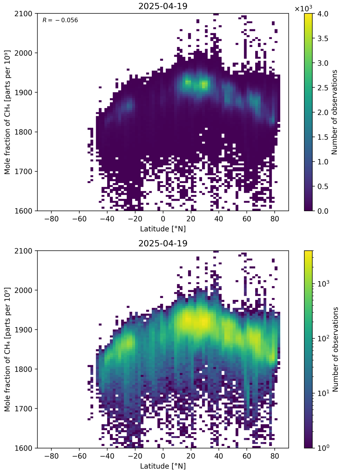
Figure 57: Scatter density plot of “Latitude” against “Mole fraction of CH 4 ” for 2025-04-19 to 2025-04-20.
