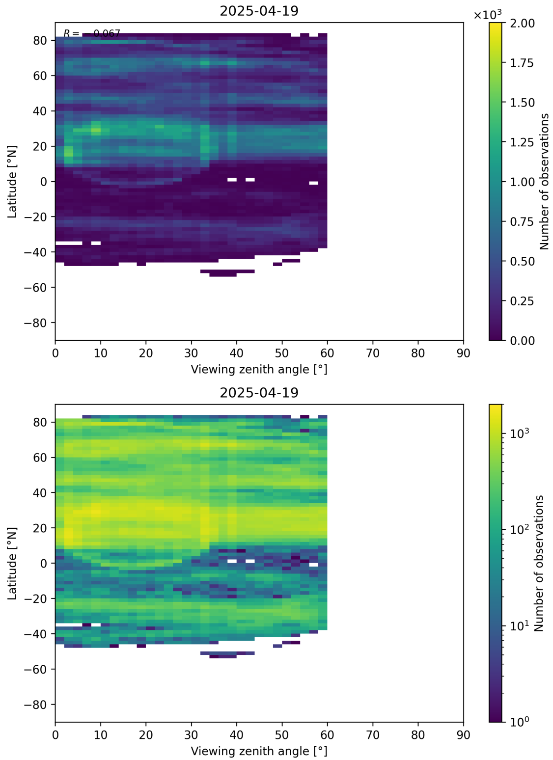
Figure 109: Scatter density plot of “Viewing zenith angle” against “Latitude” for 2025-04-19 to 2025-04-20.
