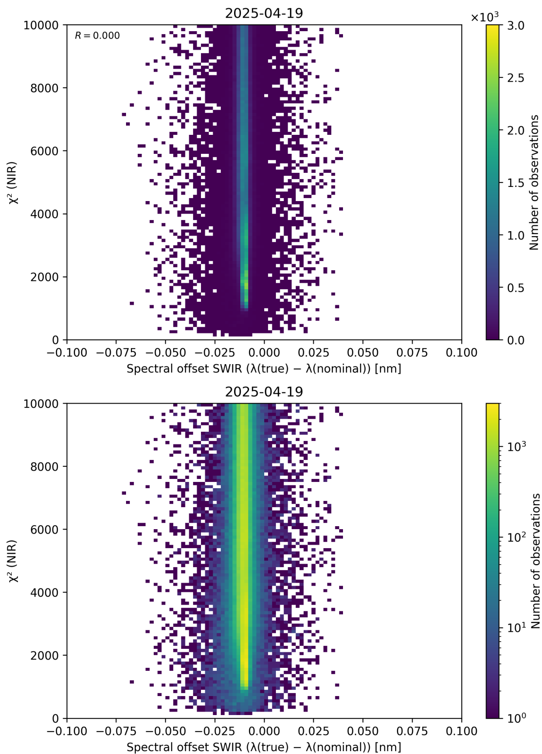
Figure 117: Scatter density plot of “Spectral offset SWIR ( \lambda_{\text{true}} - \lambda_{\text{nominal}} )” against “ \chi^2 (NIR)” for 2025-04-19 to 2025-04-20.
