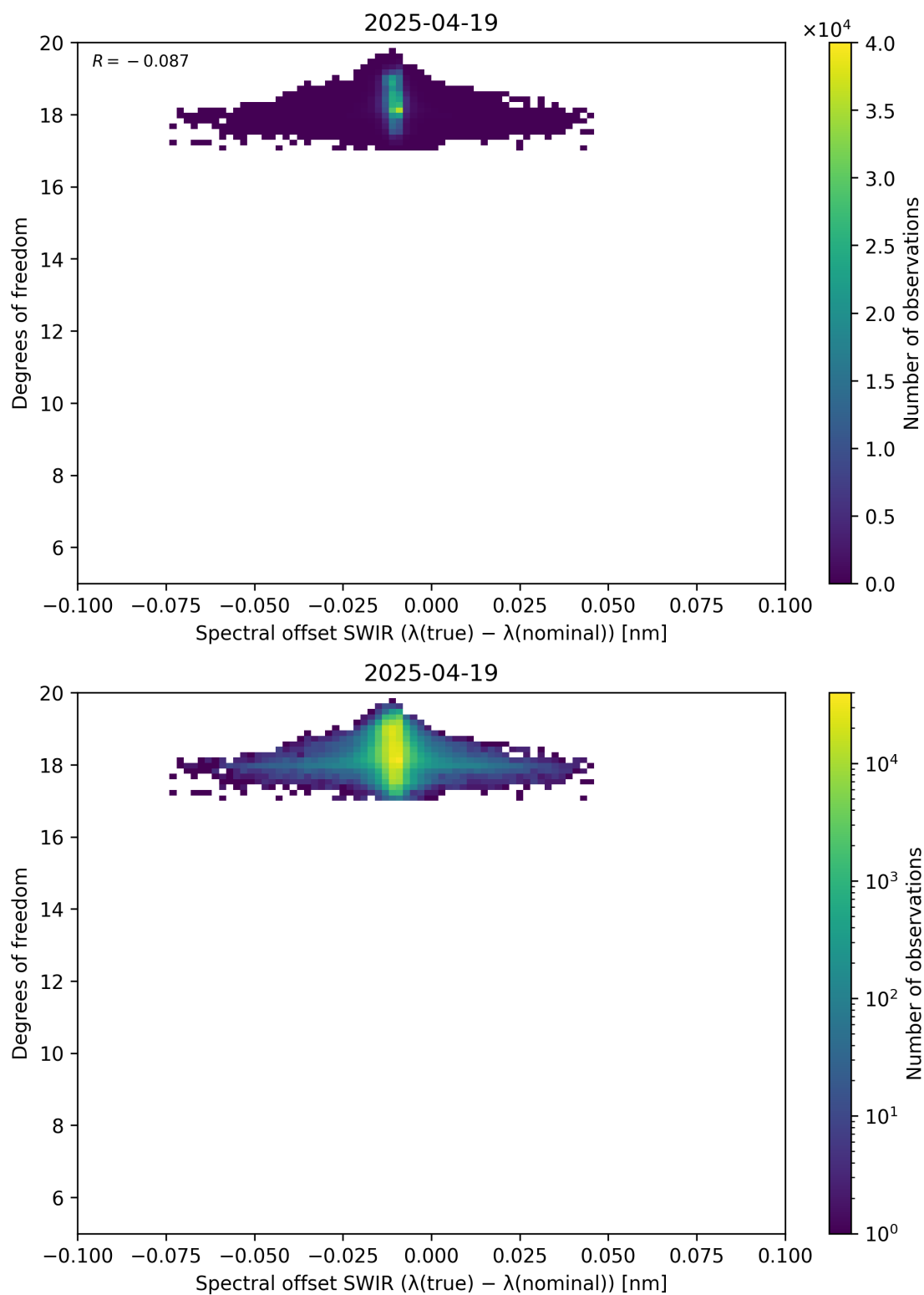
Figure 119: Scatter density plot of “Spectral offset SWIR ( \lambda_{\text{true}} - \lambda_{\text{nominal}} )” against “Degrees of freedom” for 2025-04-19 to 2025-04-20.
