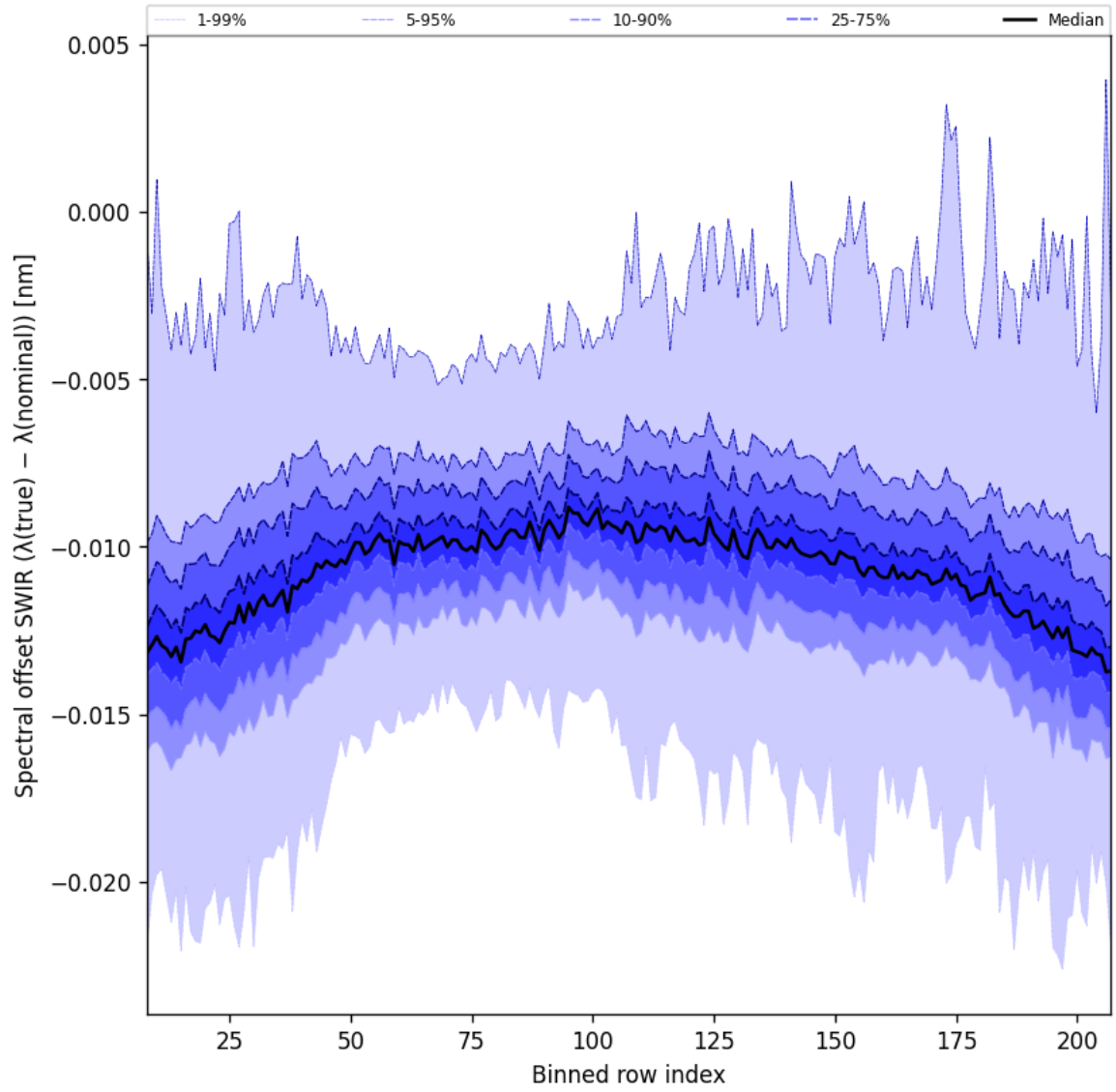
Figure 38: Along track statistics of “Spectral offset SWIR ( \lambda_{\text{true}} - \lambda_{\text{nominal}} )” for 2025-04-19 to 2025-04-20
