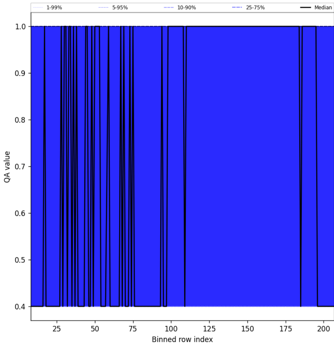
Figure 33: Along track statistics of “QA value” for 2025-04-19 to 2025-04-20
