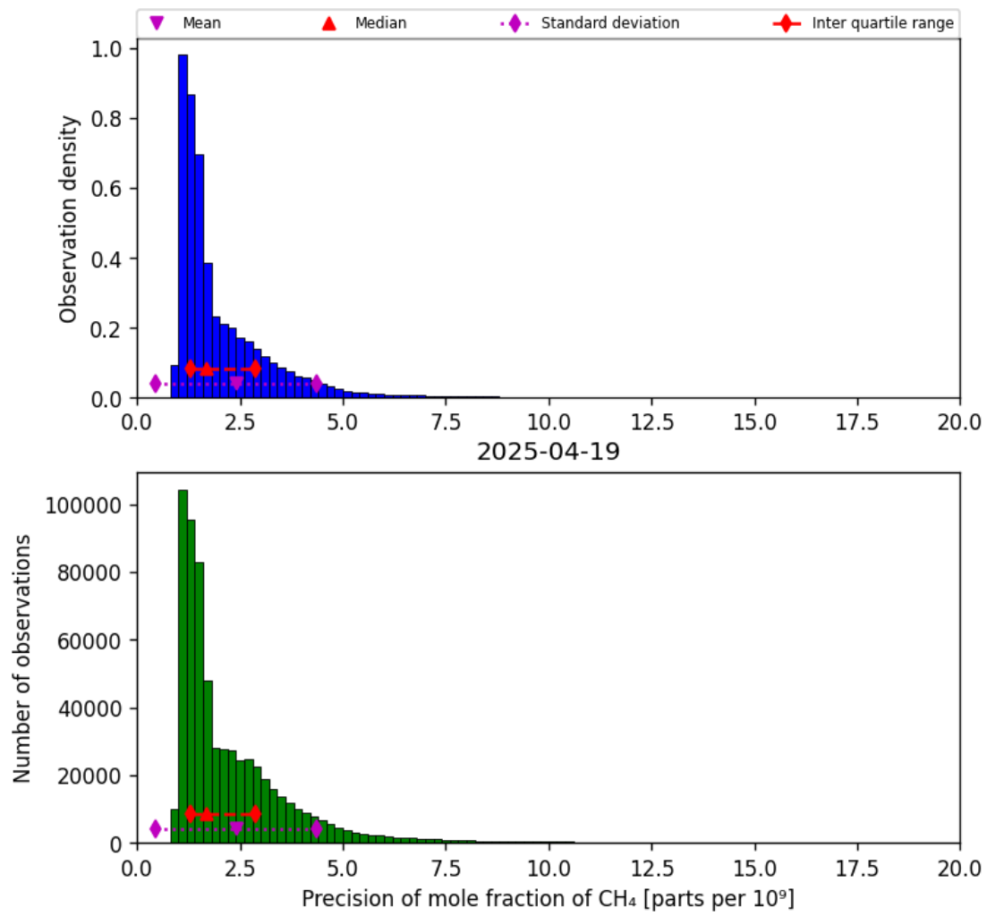
Figure 24: Histogram of “Precision of mole fraction of CH 4 ” for 2025-04-19 to 2025-04-20
