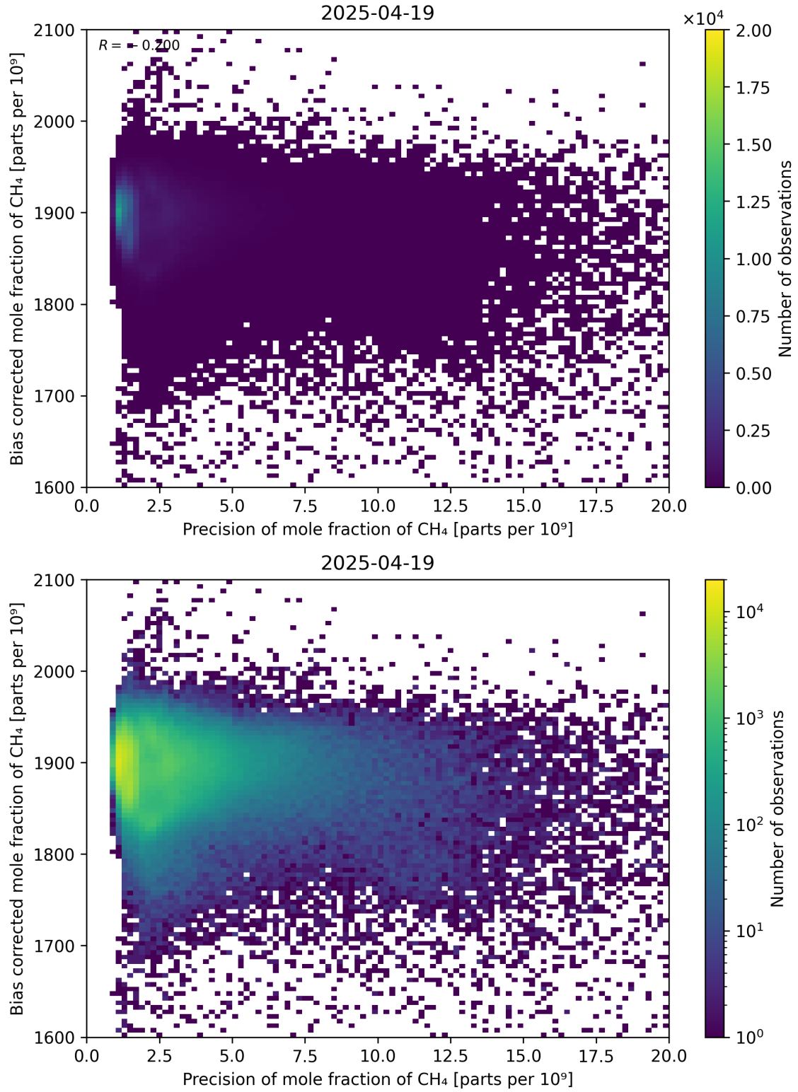
Figure 82: Scatter density plot of “Precision of mole fraction of CH 4 ” against “Bias corrected mole fraction of CH 4 ” for 2025-04-19 to 2025-04-20.
