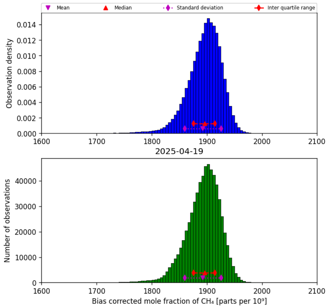
Figure 25: Histogram of “Bias corrected mole fraction of CH 4 ” for 2025-04-19 to 2025-04-20
