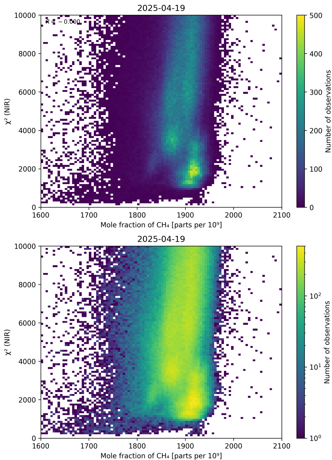
Figure 70: Scatter density plot of “Mole fraction of \text{CH}_4 ” against “ \chi^2 (NIR)” for 2025-04-19 to 2025-04-20.
