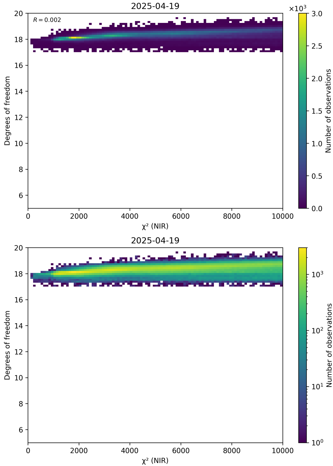
Figure 44: Scatter density plot of “ \chi^2 (NIR)” against “Degrees of freedom” for 2025-04-19 to 2025-04-20.
