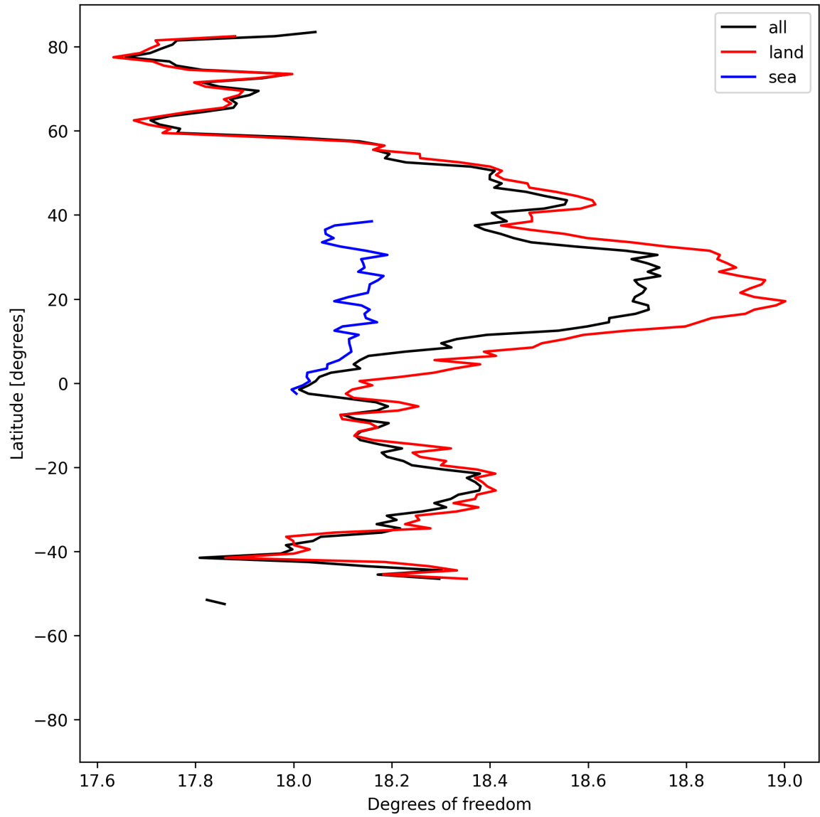
Figure 19: Zonal average of “Degrees of freedom” for 2025-04-19 to 2025-04-20.
