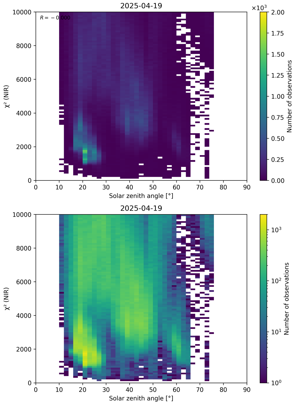
Figure 94: Scatter density plot of “Solar zenith angle” against “ \chi^2 (NIR)” for 2025-04-19 to 2025-04-20.
