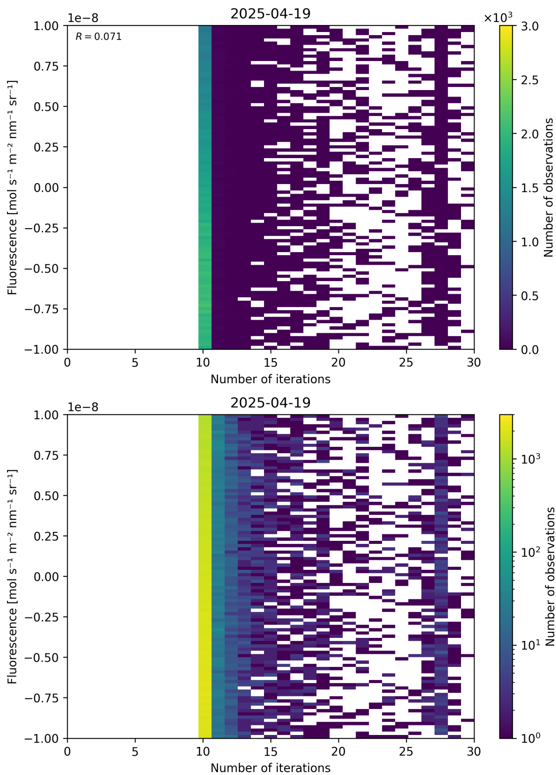
Figure 87: Scatter density plot of “Number of iterations” against “Fluorescence” for 2025-04-19 to 2025-04-20.
