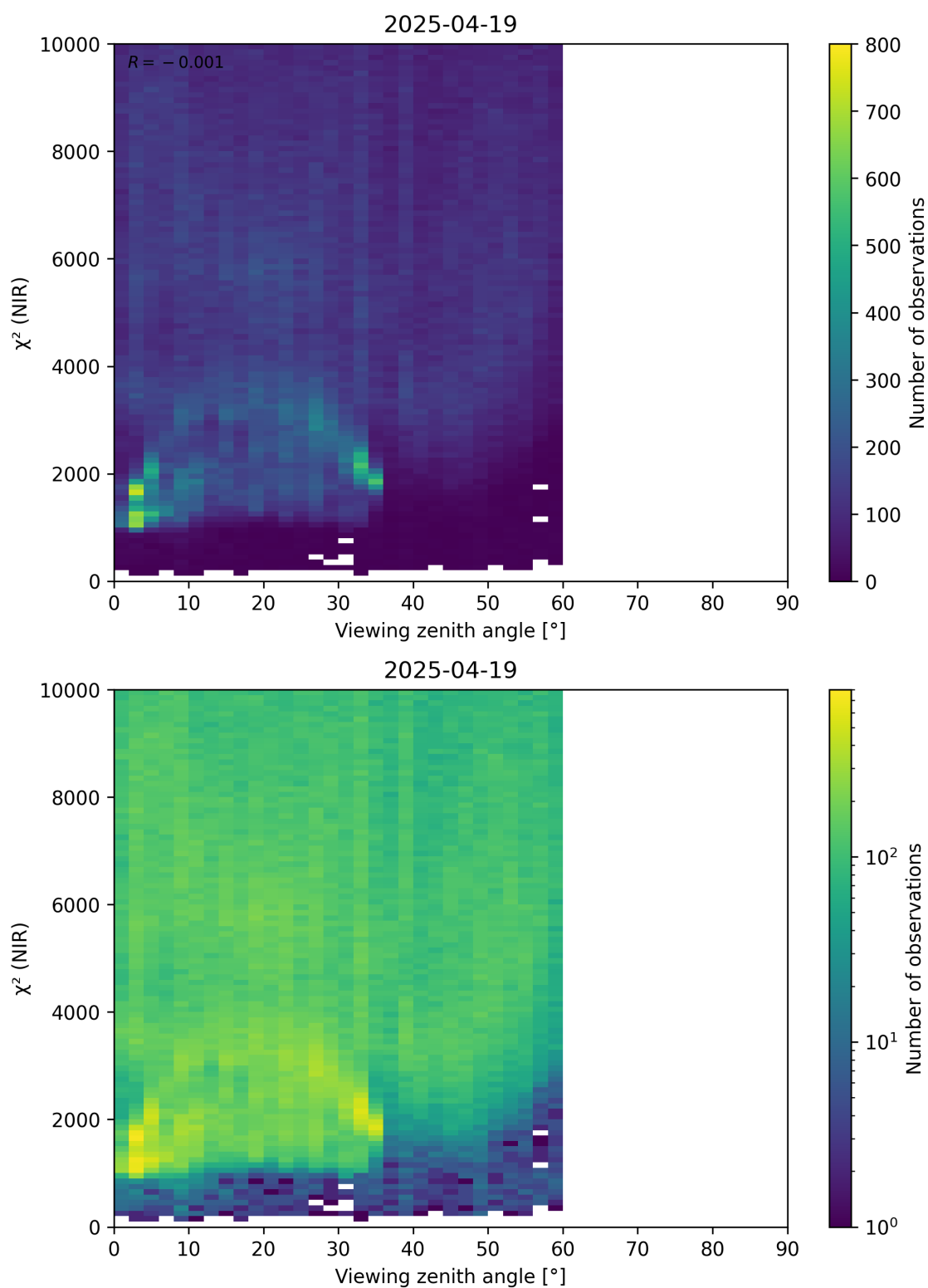
Figure 105: Scatter density plot of “Viewing zenith angle” against “ \chi^2 (NIR)” for 2025-04-19 to 2025-04-20.
