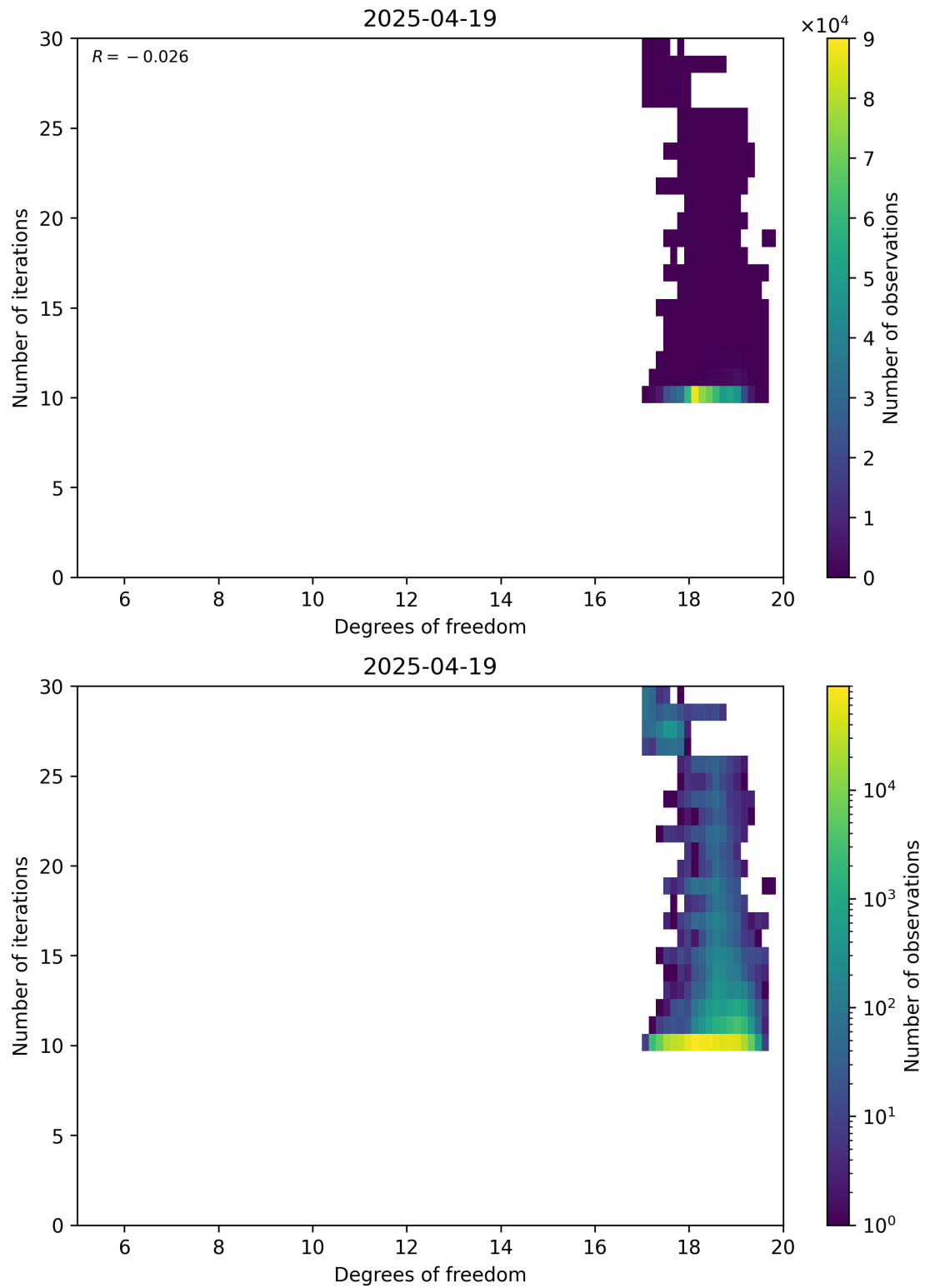
Figure 52: Scatter density plot of “Degrees of freedom” against “Number of iterations” for 2025-04-19 to 2025-04-20.
