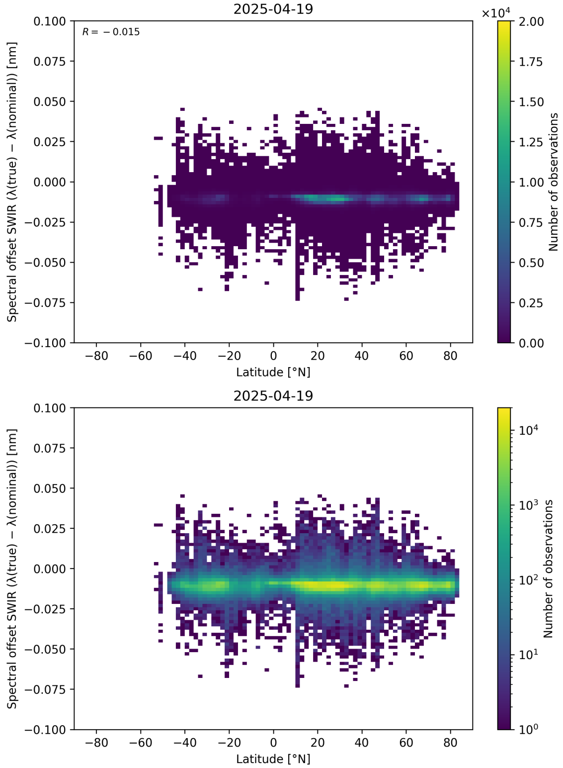
Figure 62: Scatter density plot of “Latitude” against “Spectral offset SWIR ( \lambda_{\text{true}} - \lambda_{\text{nominal}} )” for 2025-04-19 to 2025-04-20.
