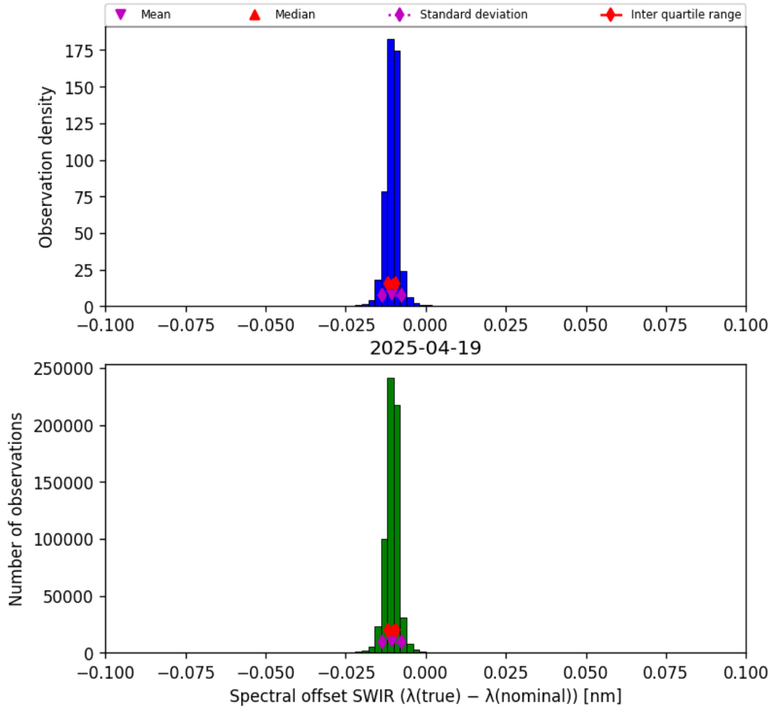
Figure 27: Histogram of “Spectral offset SWIR ( \lambda_{\text{true}} - \lambda_{\text{nominal}} )” for 2025-04-19 to 2025-04-20
