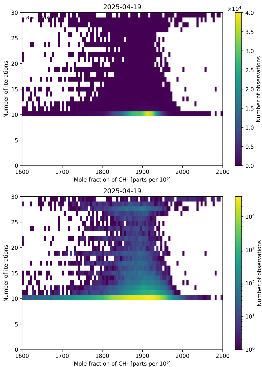
Figure 76: Scatter density plot of “Mole fraction of CH 4 ” against “Number of iterations” for 2025-04-19 to 2025-04-20.
