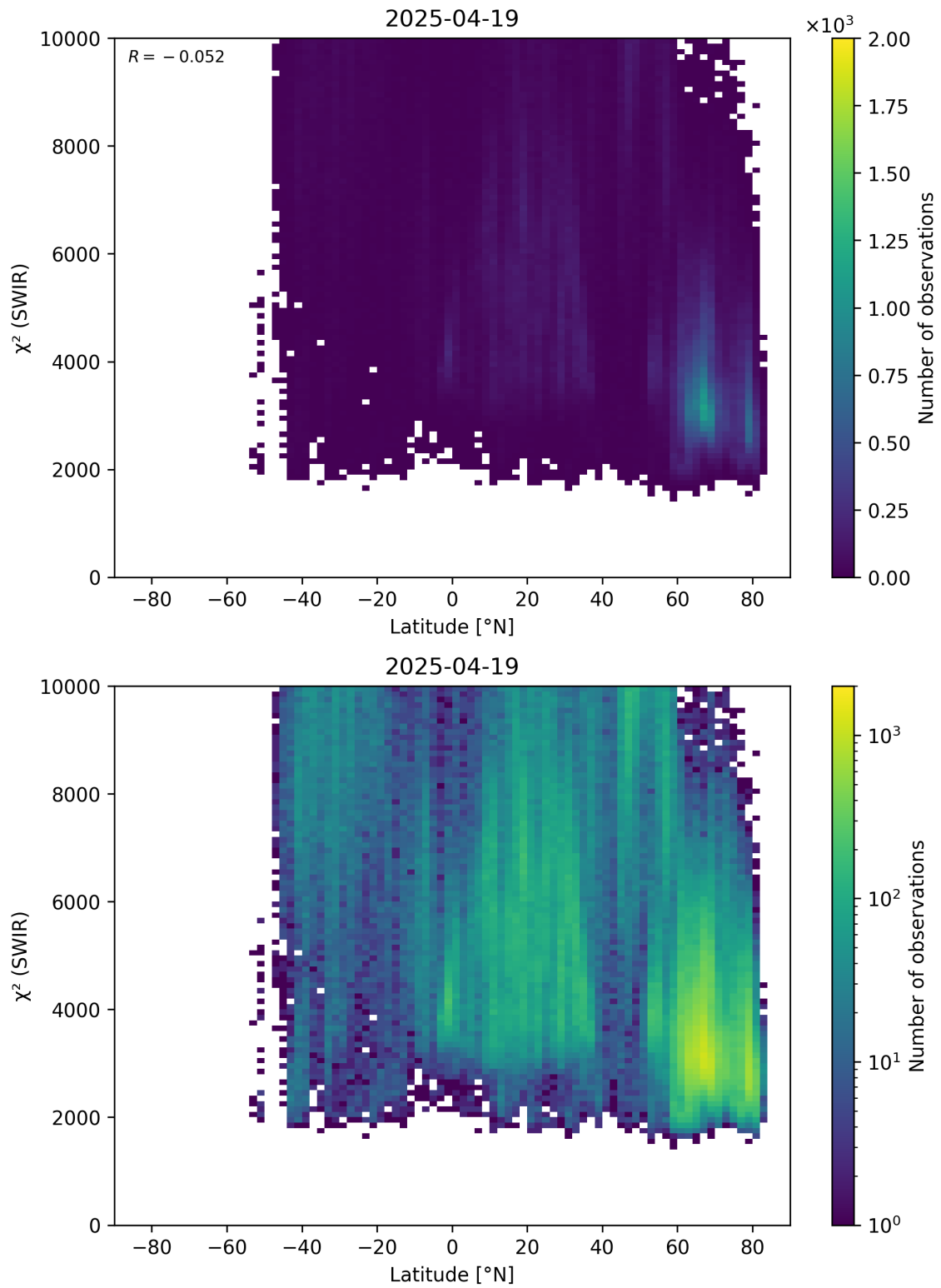
Figure 54: Scatter density plot of “Latitude” against “ \chi^2 (SWIR)” for 2025-04-19 to 2025-04-20.
