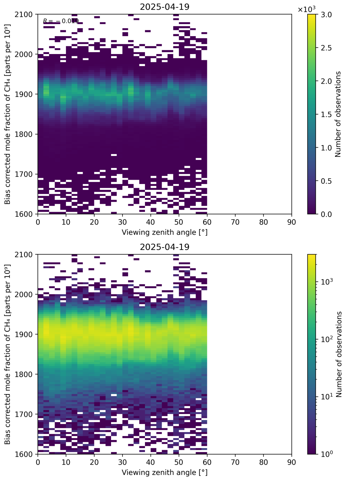
Figure 111: Scatter density plot of “Viewing zenith angle” against “Bias corrected mole fraction of CH 4 ” for 2025-04-19 to 2025-04-20.
