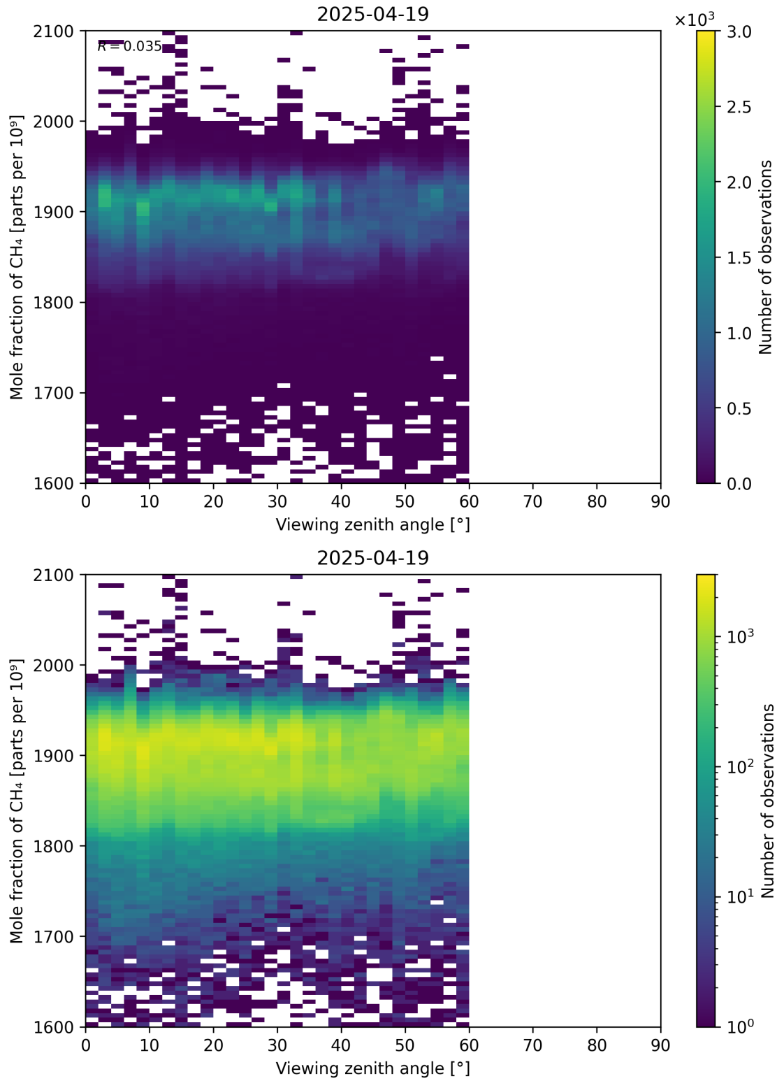
Figure 110: Scatter density plot of “Viewing zenith angle” against “Mole fraction of CH 4 ” for 2025-04-19 to 2025-04-20.
