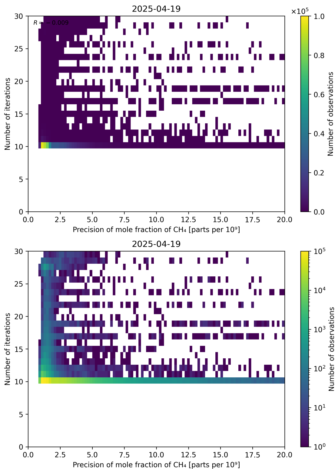
Figure 83: Scatter density plot of “Precision of mole fraction of CH 4 ” against “Number of iterations” for 2025-04-19 to 2025-04-20.
