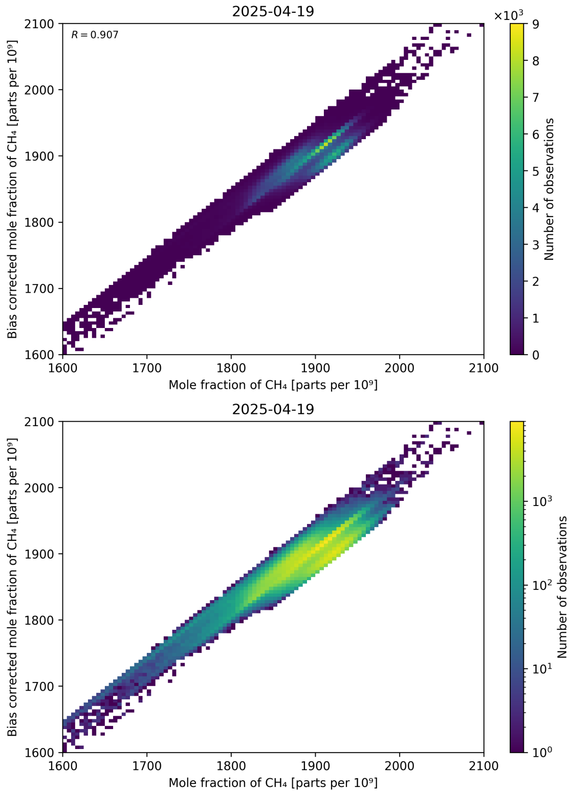
Figure 74: Scatter density plot of “Mole fraction of CH 4 ” against “Bias corrected mole fraction of CH 4 ” for 2025-04-19 to 2025-04-20.
