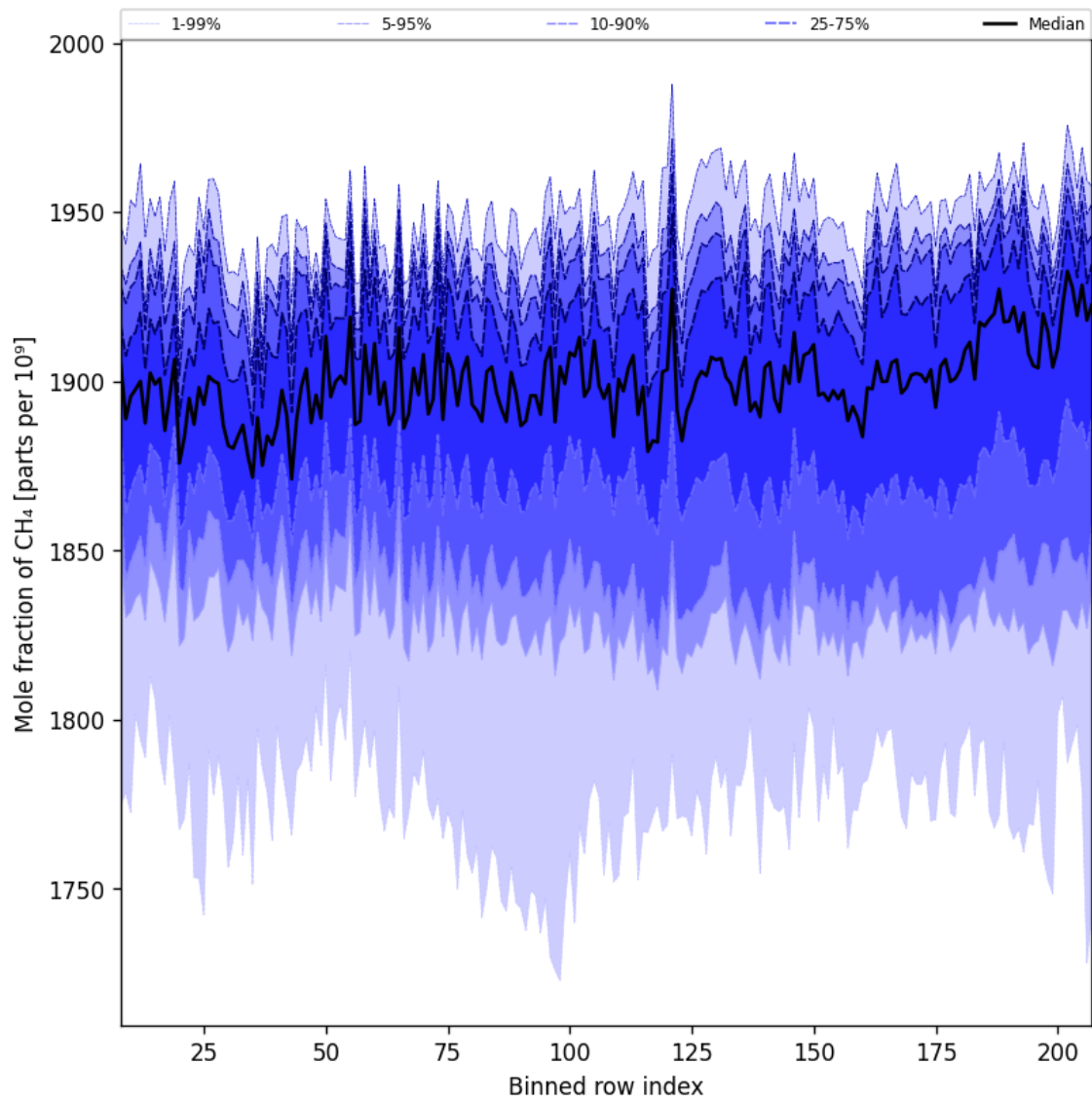
Figure 34: Along track statistics of “Mole fraction of CH 4 ” for 2025-04-19 to 2025-04-20
