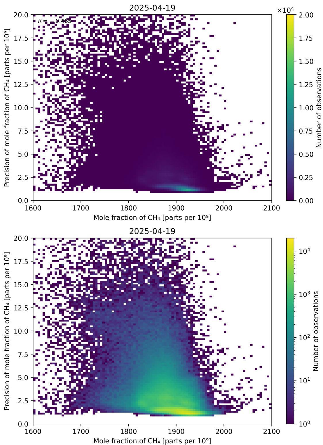
Figure 75: Scatter density plot of “Mole fraction of CH 4 ” against “Precision of mole fraction of CH 4 ” for 2025-04-19 to 2025-04-20.
