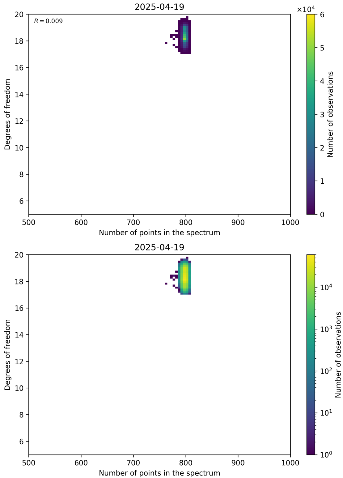
Figure 90: Scatter density plot of “Number of points in the spectrum” against “Degrees of freedom” for 2025-04-19 to 2025-04-20.
