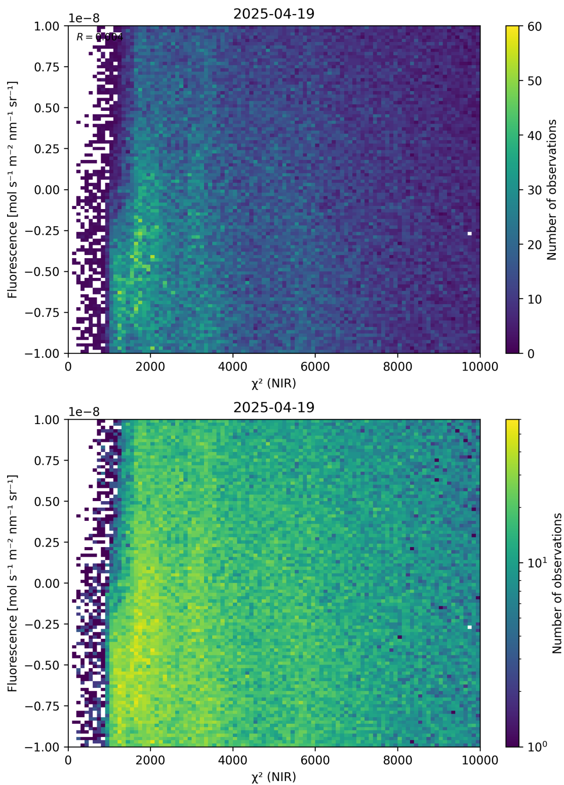
Figure 45: Scatter density plot of “ \chi^2 (NIR)” against “Fluorescence” for 2025-04-19 to 2025-04-20.
