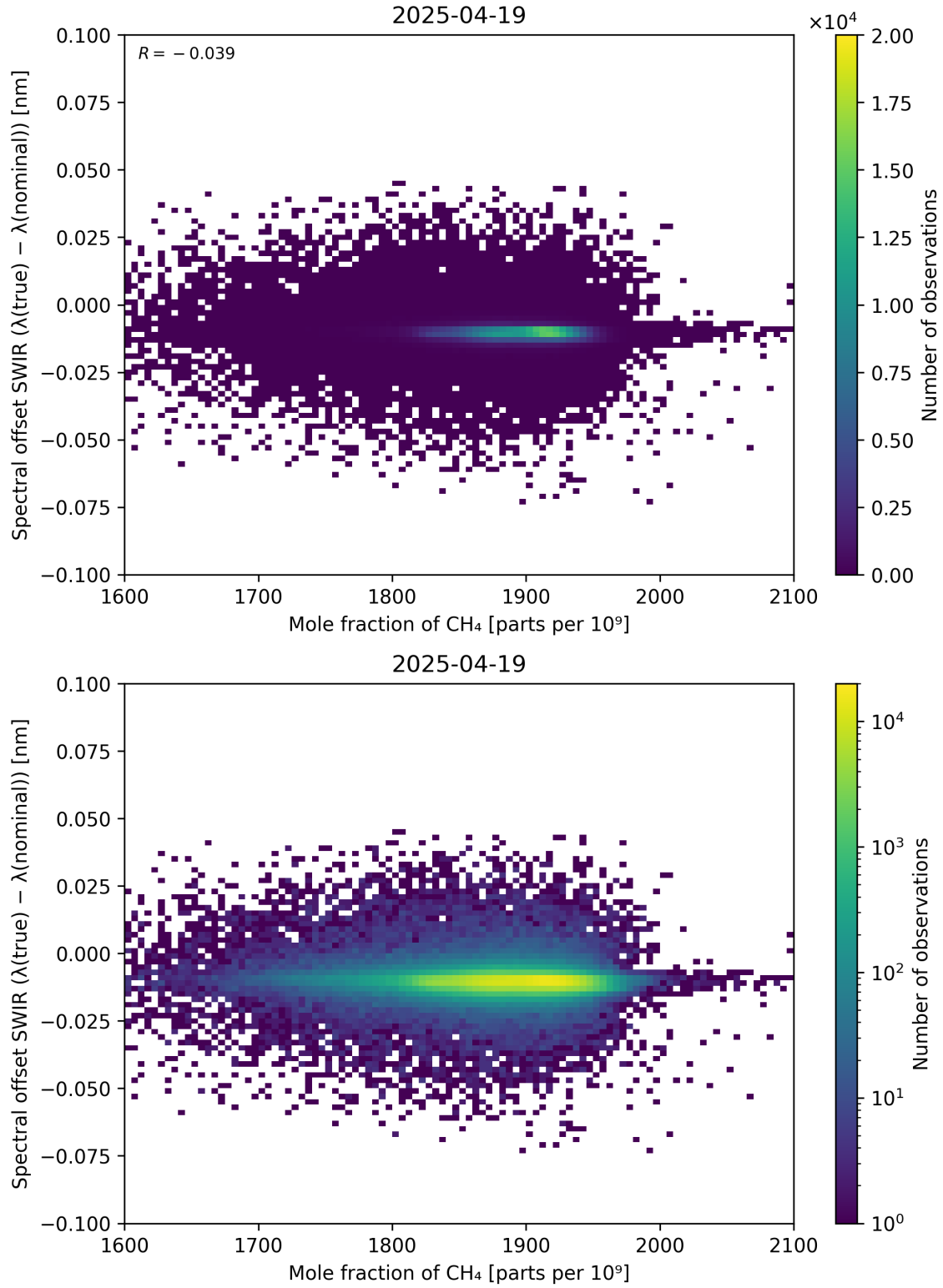
Figure 86: Scatter density plot of “Mole fraction of CH 4 ” against “Spectral offset SWIR ( \lambda_{\text{true}} - \lambda_{\text{nominal}} )” for 2025-04-19 to 2025-04-20.
