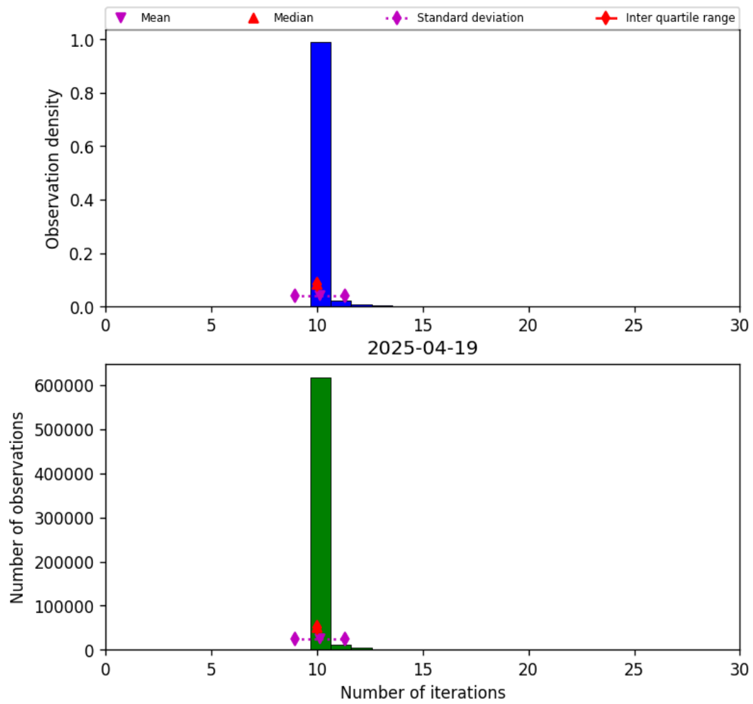
Figure 31: Histogram of “Number of iterations” for 2025-04-19 to 2025-04-20
