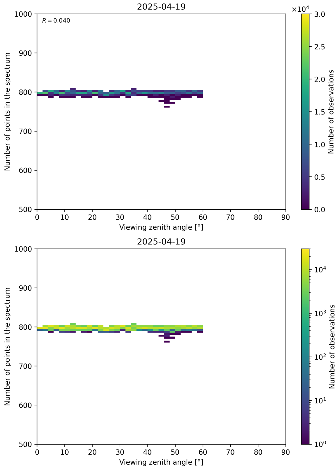
Figure 114: Scatter density plot of “Viewing zenith angle” against “Number of points in the spectrum” for 2025-04-19 to 2025-04-20.
