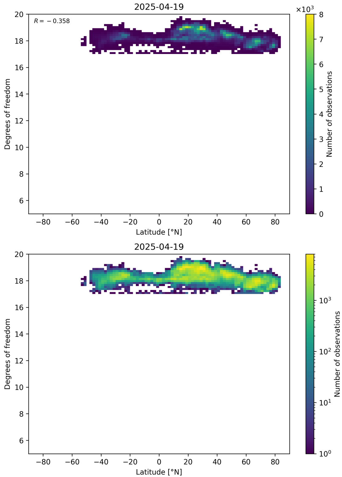
Figure 55: Scatter density plot of “Latitude” against “Degrees of freedom” for 2025-04-19 to 2025-04-20.
