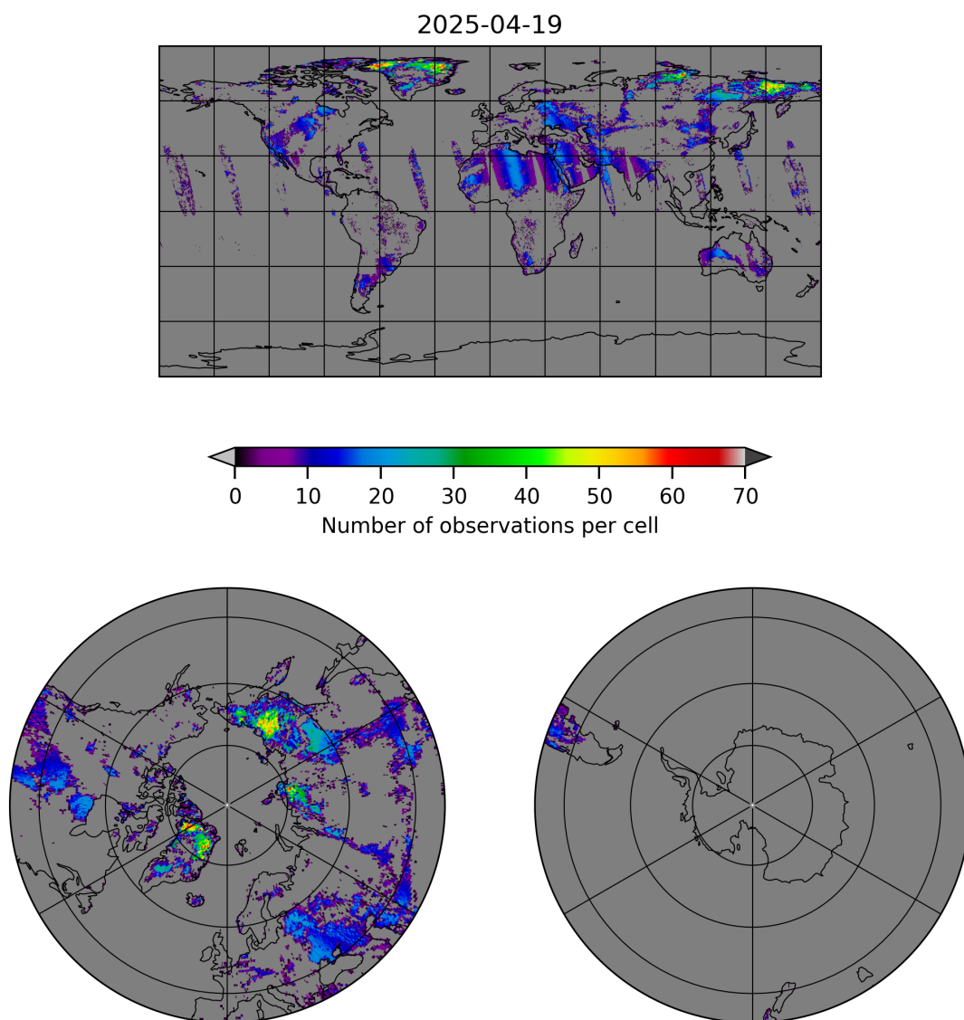
Figure 10: Map of the number of observations for 2025-04-19 to 2025-04-20
