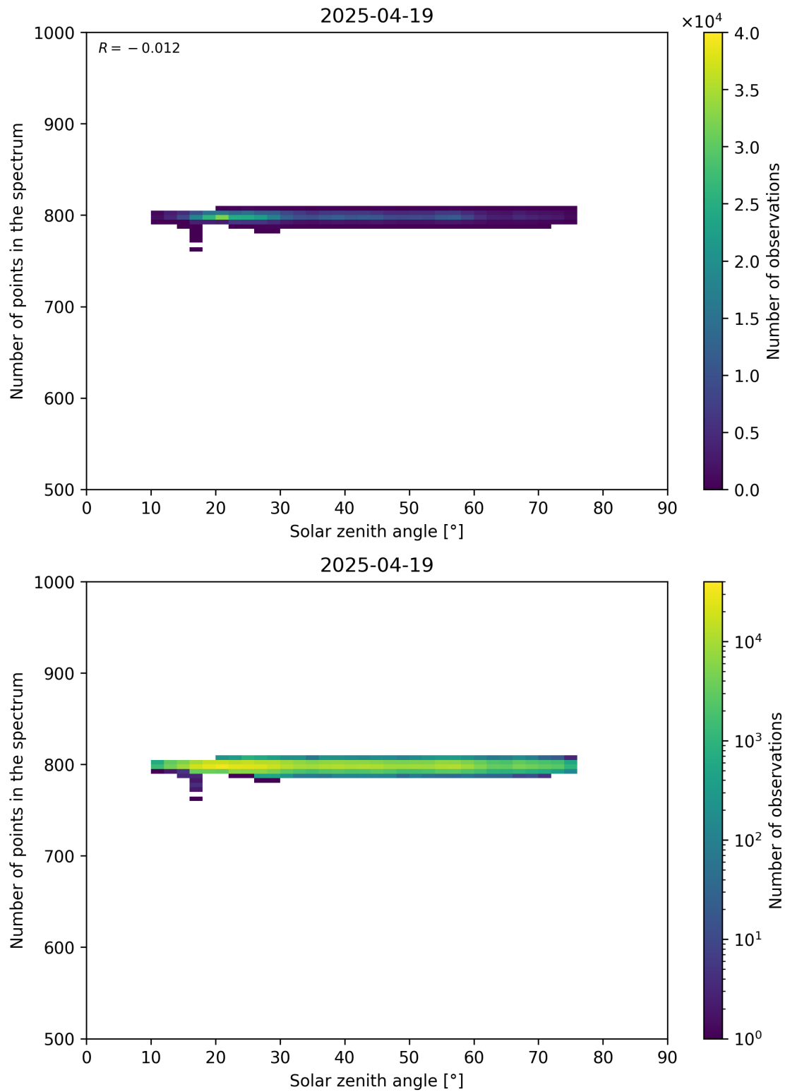
Figure 103: Scatter density plot of “Solar zenith angle” against “Number of points in the spectrum” for 2025-04-19 to 2025-04-20.
