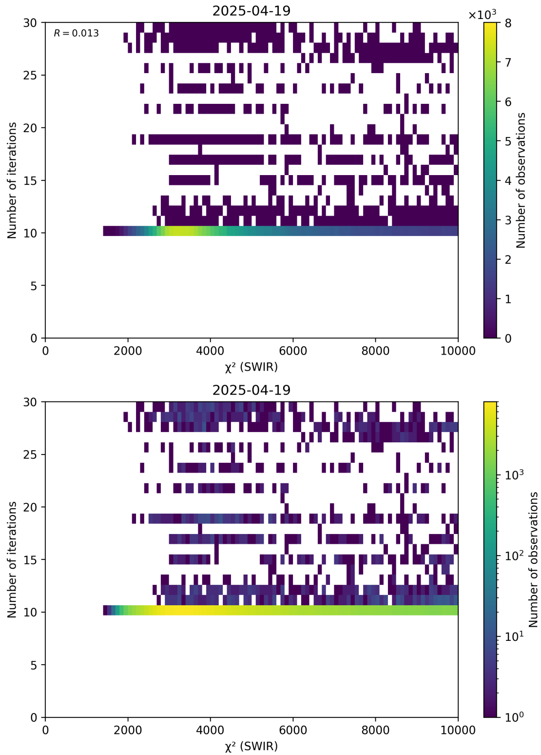
Figure 50: Scatter density plot of “ \chi^2 (SWIR)” against “Number of iterations” for 2025-04-19 to 2025-04-20.
