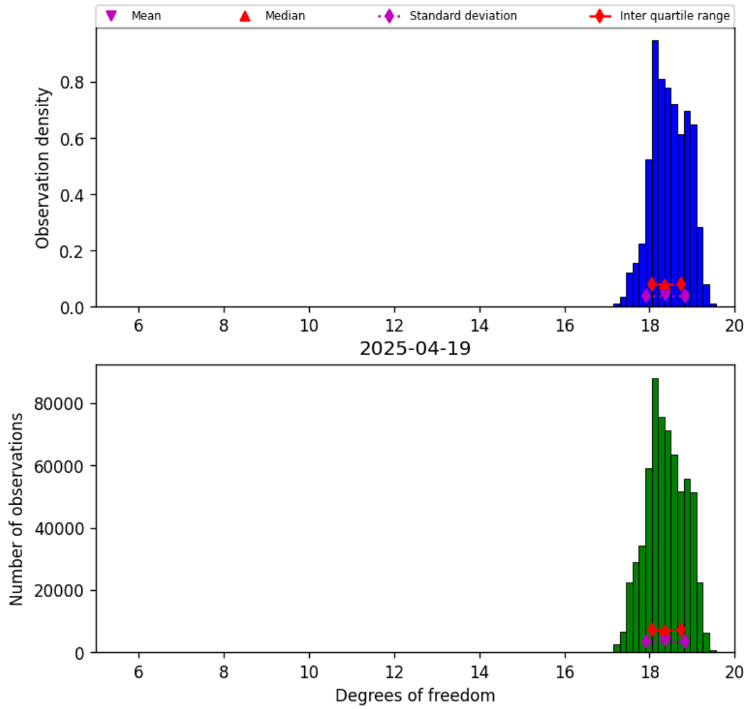
Figure 30: Histogram of “Degrees of freedom” for 2025-04-19 to 2025-04-20
