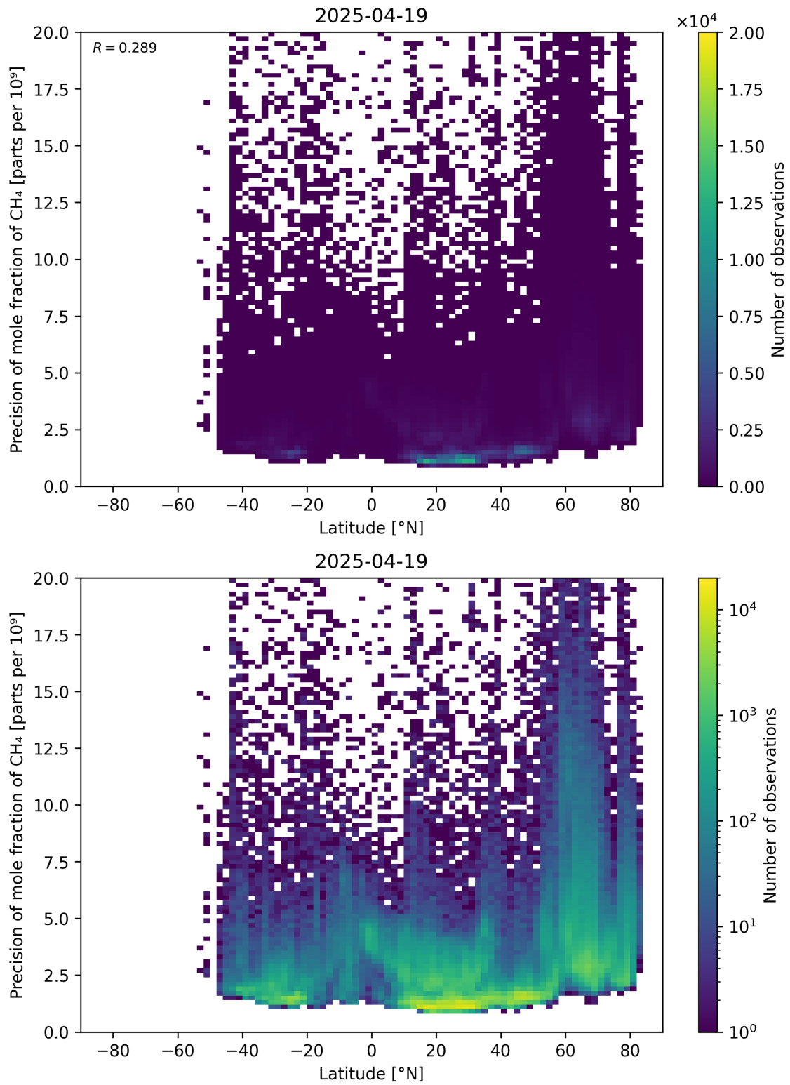
Figure 59: Scatter density plot of “Latitude” against “Precision of mole fraction of CH 4 ” for 2025-04-19 to 2025-04-20.
