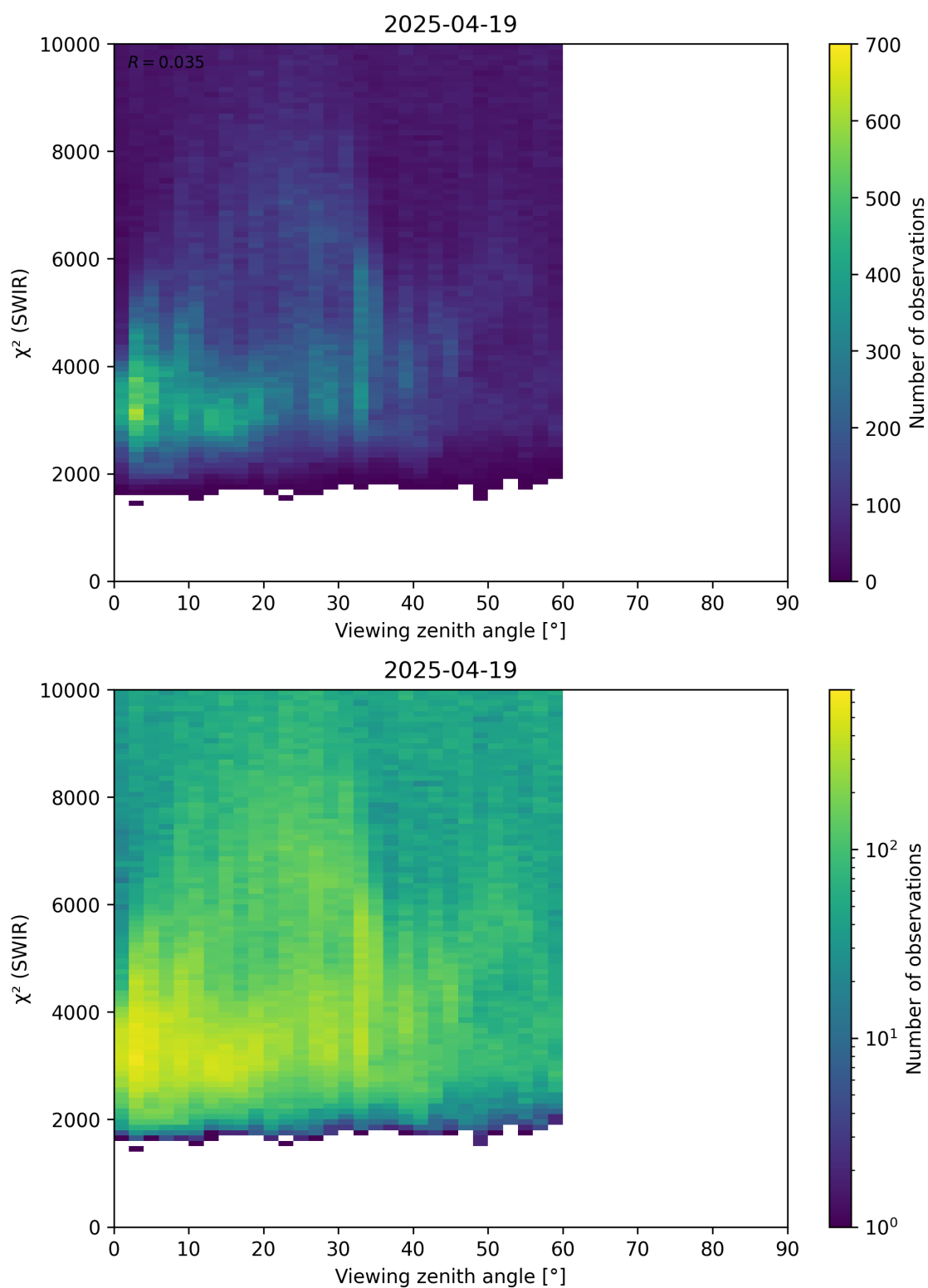
Figure 106: Scatter density plot of “Viewing zenith angle” against “ \chi^2 (SWIR)” for 2025-04-19 to 2025-04-20.
