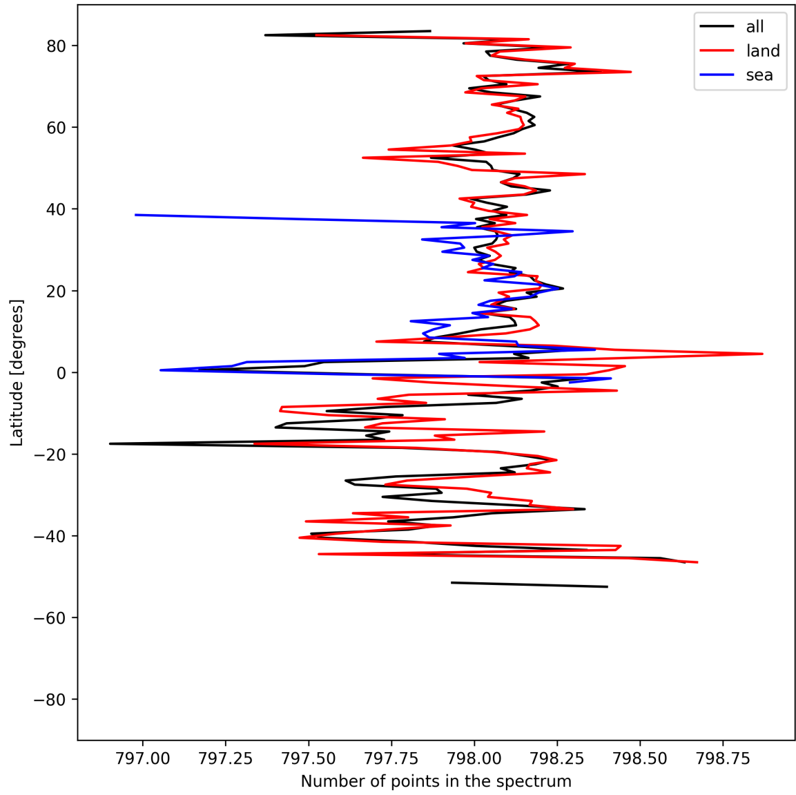
Figure 15: Zonal average of “Number of points in the spectrum” for 2025-04-19 to 2025-04-20.
