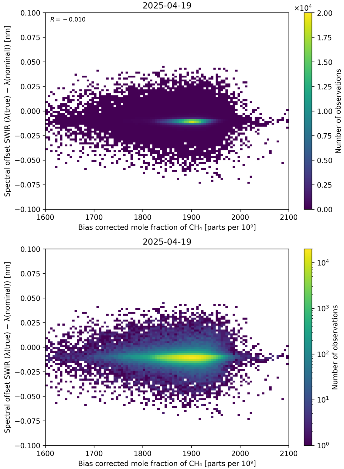
Figure 69: Scatter density plot of “Bias corrected mole fraction of \text{CH}_4 ” against “Spectral offset SWIR ( \lambda_{\text{true}} - \lambda_{\text{nominal}} )” for 2025-04-19 to 2025-04-20.
