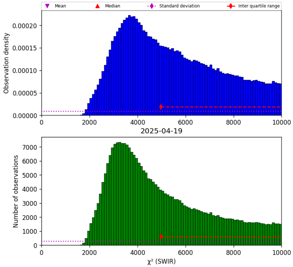
Figure 28: Histogram of “ \chi^2 (SWIR)” for 2025-04-19 to 2025-04-20
