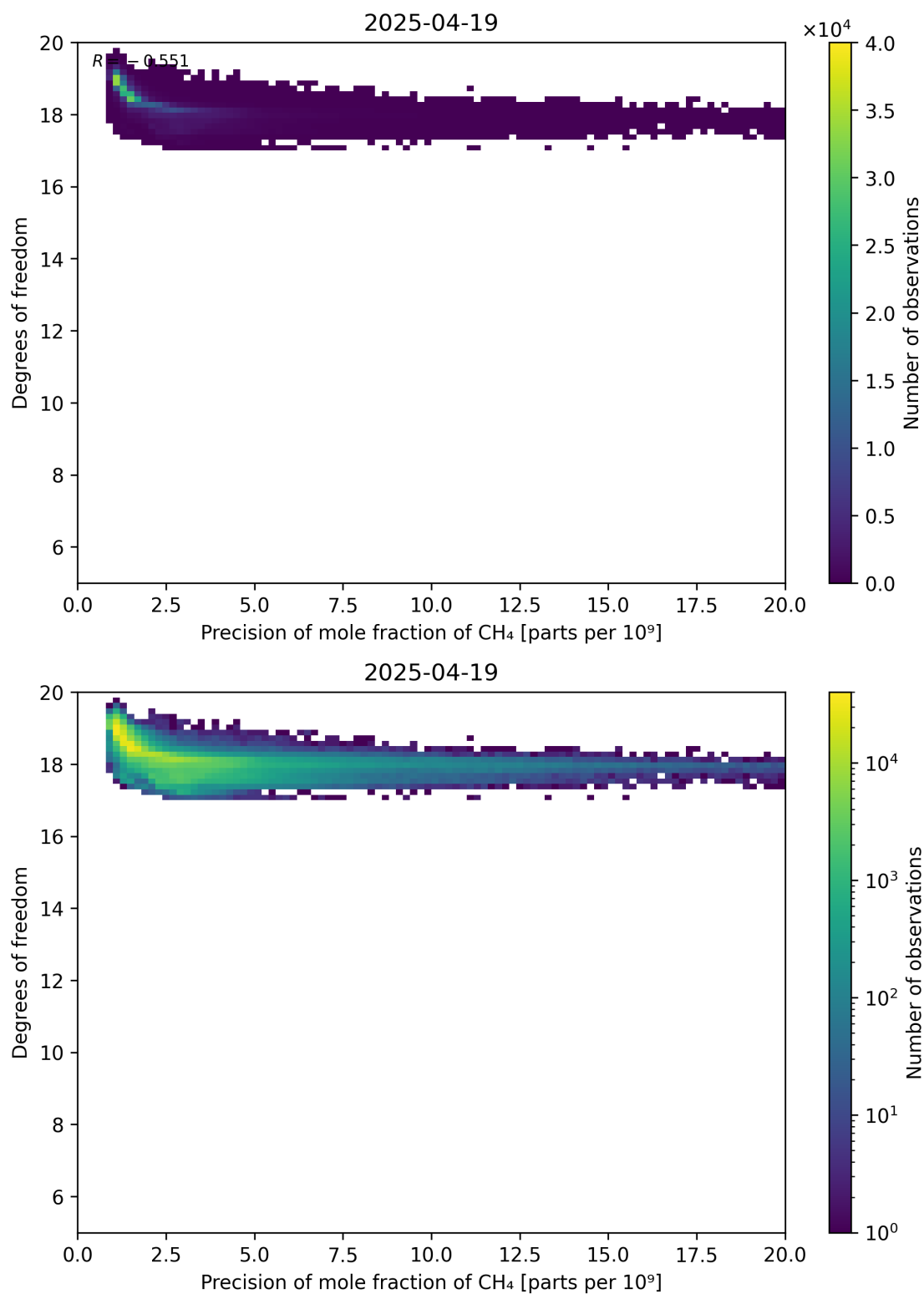
Figure 80: Scatter density plot of “Precision of mole fraction of CH 4 ” against “Degrees of freedom” for 2025-04-19 to 2025-04-20.
