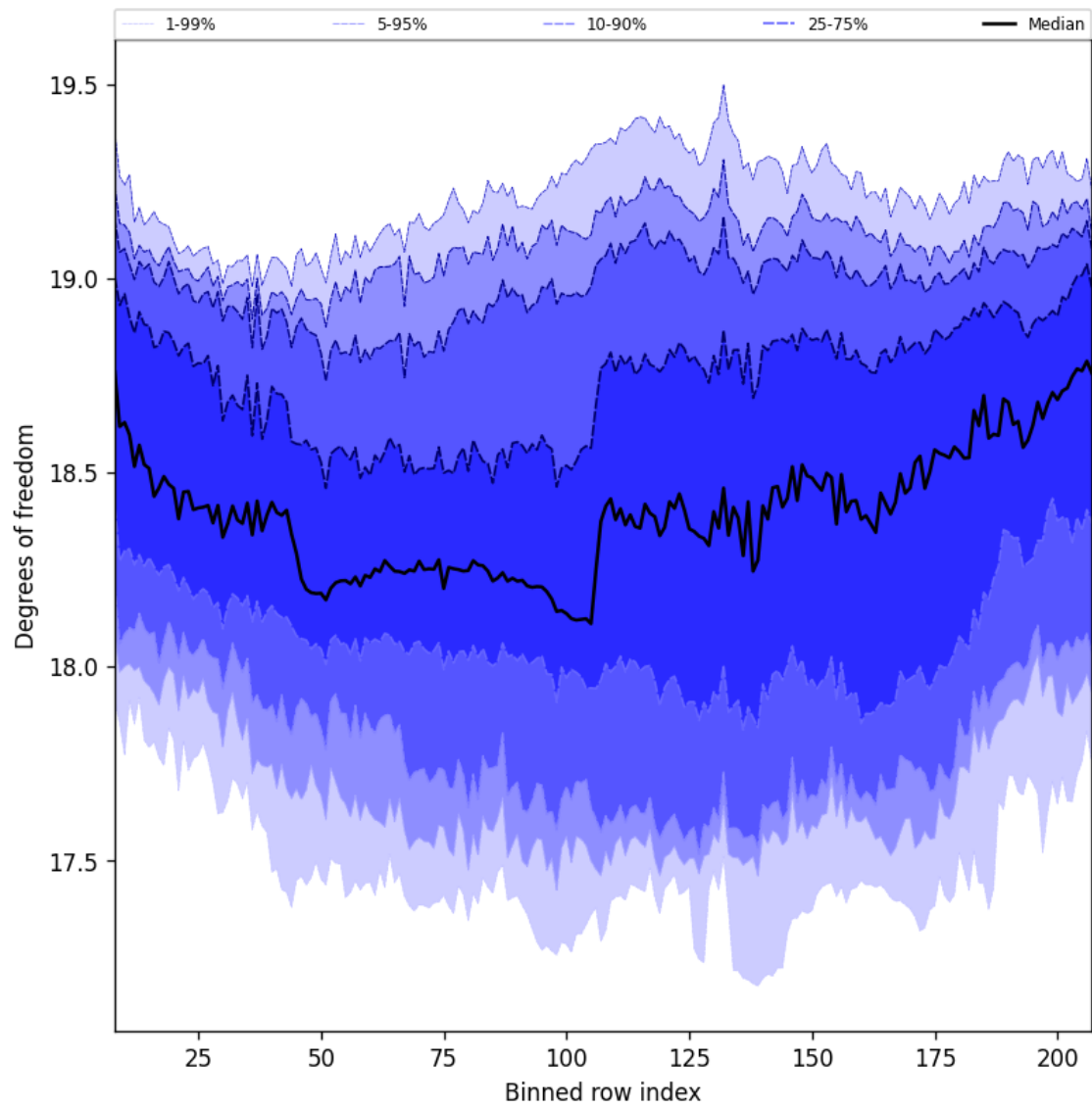
Figure 41: Along track statistics of “Degrees of freedom” for 2025-04-19 to 2025-04-20
