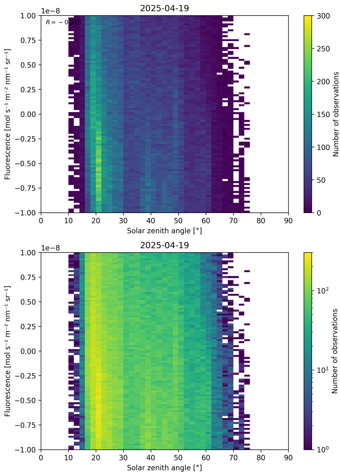
Figure 97: Scatter density plot of “Solar zenith angle” against “Fluorescence” for 2025-04-19 to 2025-04-20.
