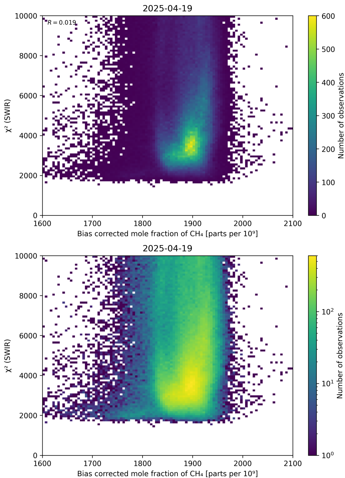
Figure 64: Scatter density plot of “Bias corrected mole fraction of \text{CH}_4 ” against “ \chi^2 (SWIR)” for 2025-04-19 to 2025-04-20.
