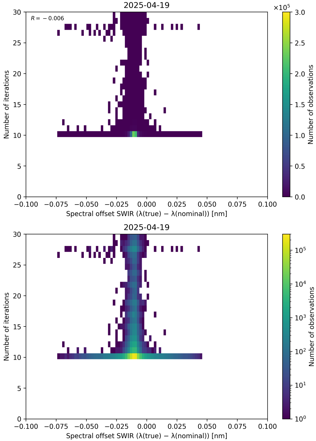
Figure 121: Scatter density plot of “Spectral offset SWIR ( \lambda_{\text{true}} - \lambda_{\text{nominal}} )” against “Number of iterations” for 2025-04-19 to 2025-04-20.
