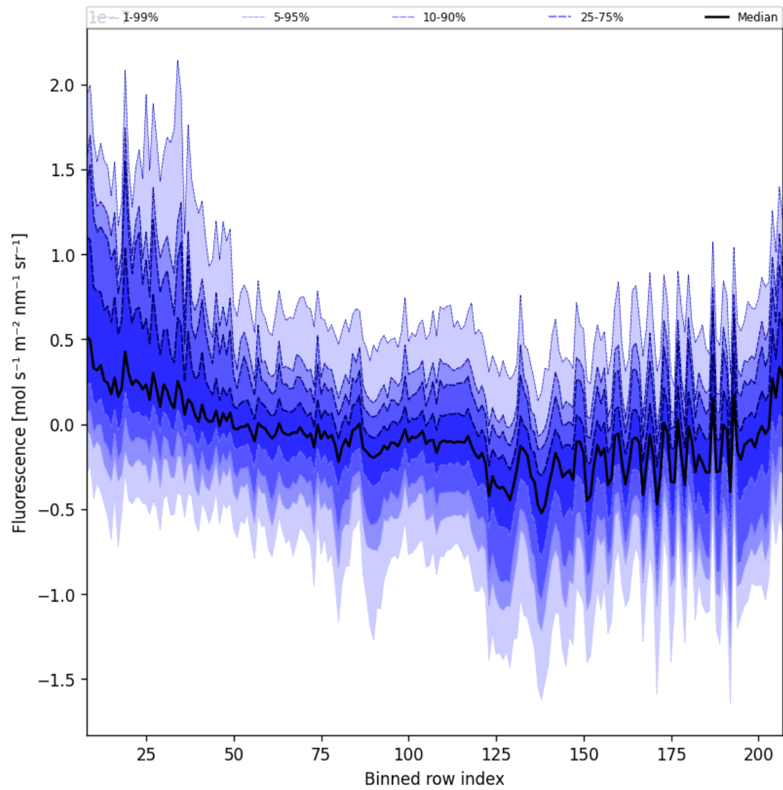
Figure 43: Along track statistics of “Fluorescence” for 2025-04-19 to 2025-04-20
