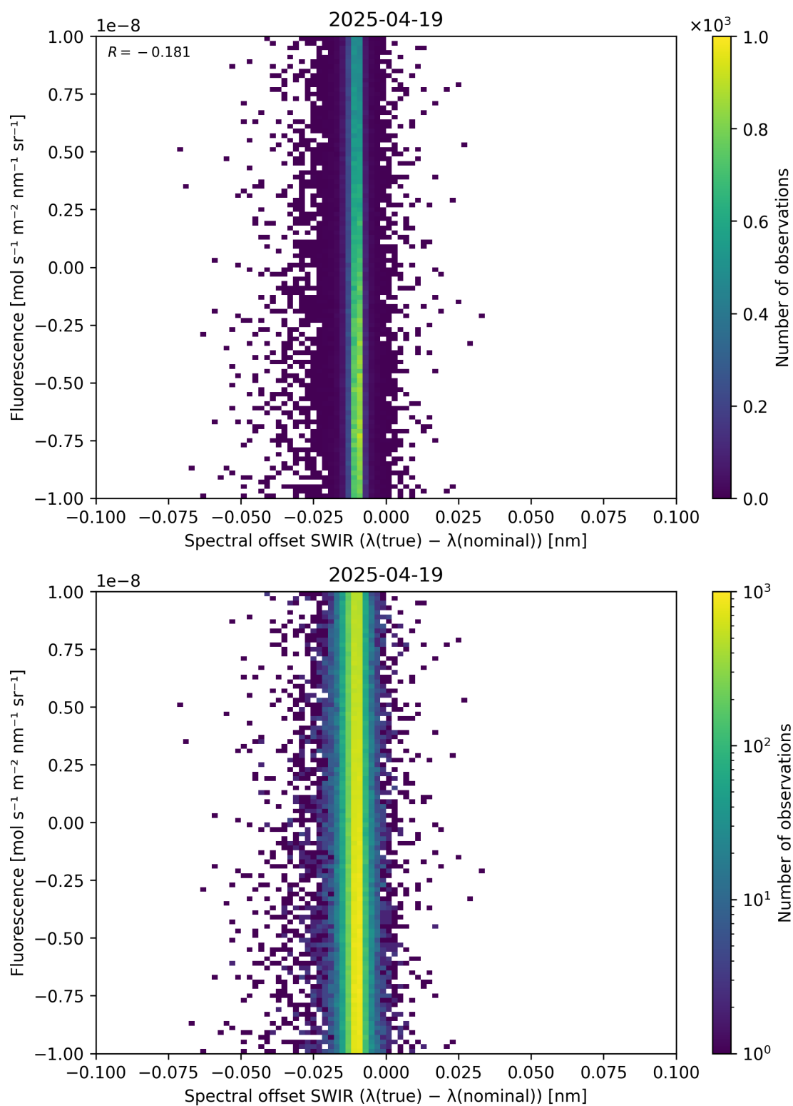
Figure 120: Scatter density plot of “Spectral offset SWIR ( \lambda_{\text{true}} - \lambda_{\text{nominal}} )” against “Fluorescence” for 2025-04-19 to 2025-04-20.
