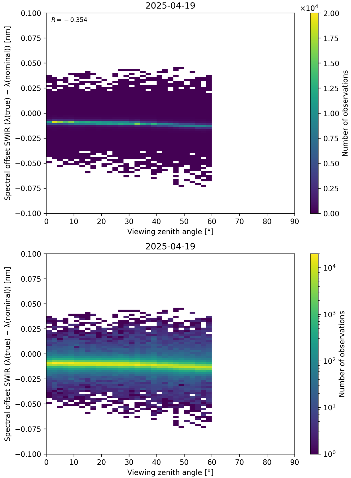
Figure 116: Scatter density plot of “Viewing zenith angle” against “Spectral offset SWIR ( \lambda_{\text{true}} - \lambda_{\text{nominal}} )” for 2025-04-19 to 2025-04-20.
