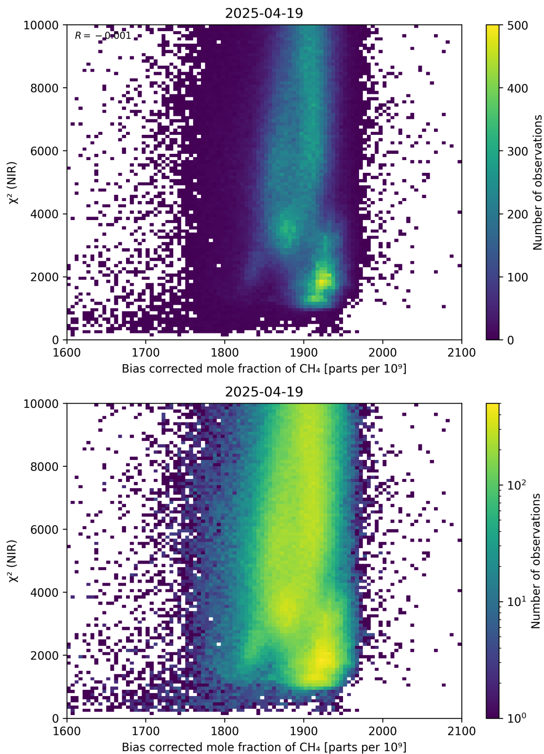
Figure 63: Scatter density plot of “Bias corrected mole fraction of CH 4 ” against “ \chi^2 (NIR)” for 2025-04-19 to 2025-04-20.
