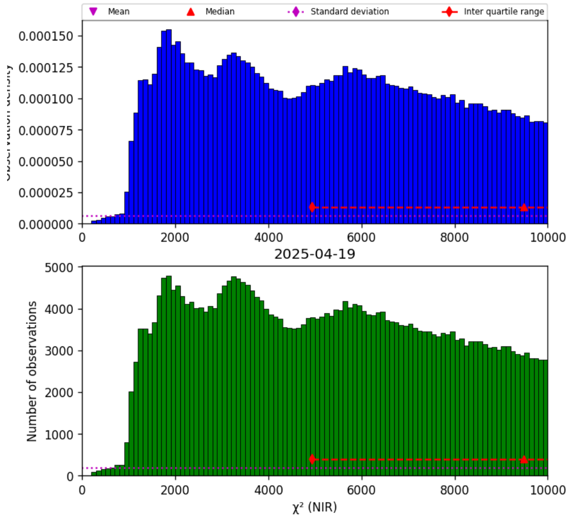
Figure 29: Histogram of “ \chi^2 (NIR)” for 2025-04-19 to 2025-04-20
