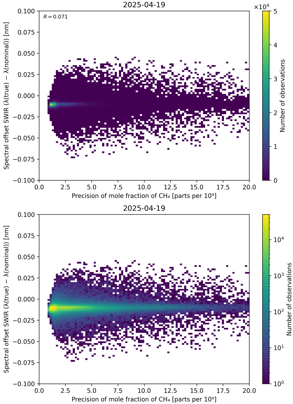
Figure 85: Scatter density plot of “Precision of mole fraction of \text{CH}_4 ” against “Spectral offset SWIR ( \lambda_{\text{true}} - \lambda_{\text{nominal}} )” for 2025-04-19 to 2025-04-20.
