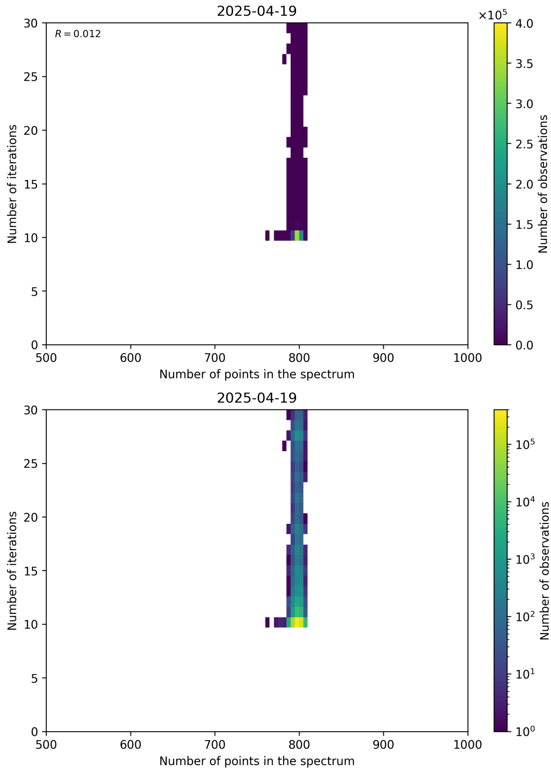
Figure 92: Scatter density plot of “Number of points in the spectrum” against “Number of iterations” for 2025-04-19 to 2025-04-20.
