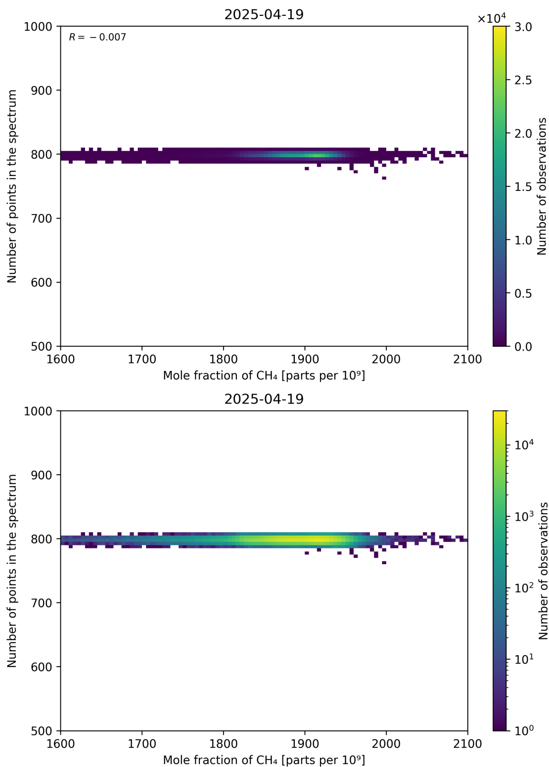
Figure 77: Scatter density plot of “Mole fraction of CH 4 ” against “Number of points in the spectrum” for 2025-04-19 to 2025-04-20.
