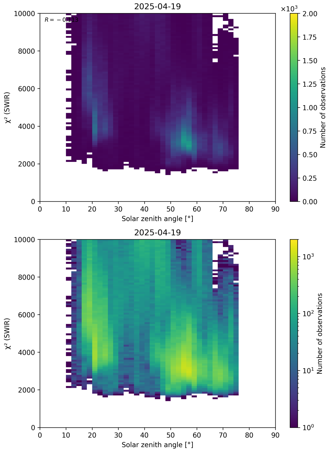
Figure 95: Scatter density plot of “Solar zenith angle” against “ \chi^2 (SWIR)” for 2025-04-19 to 2025-04-20.
