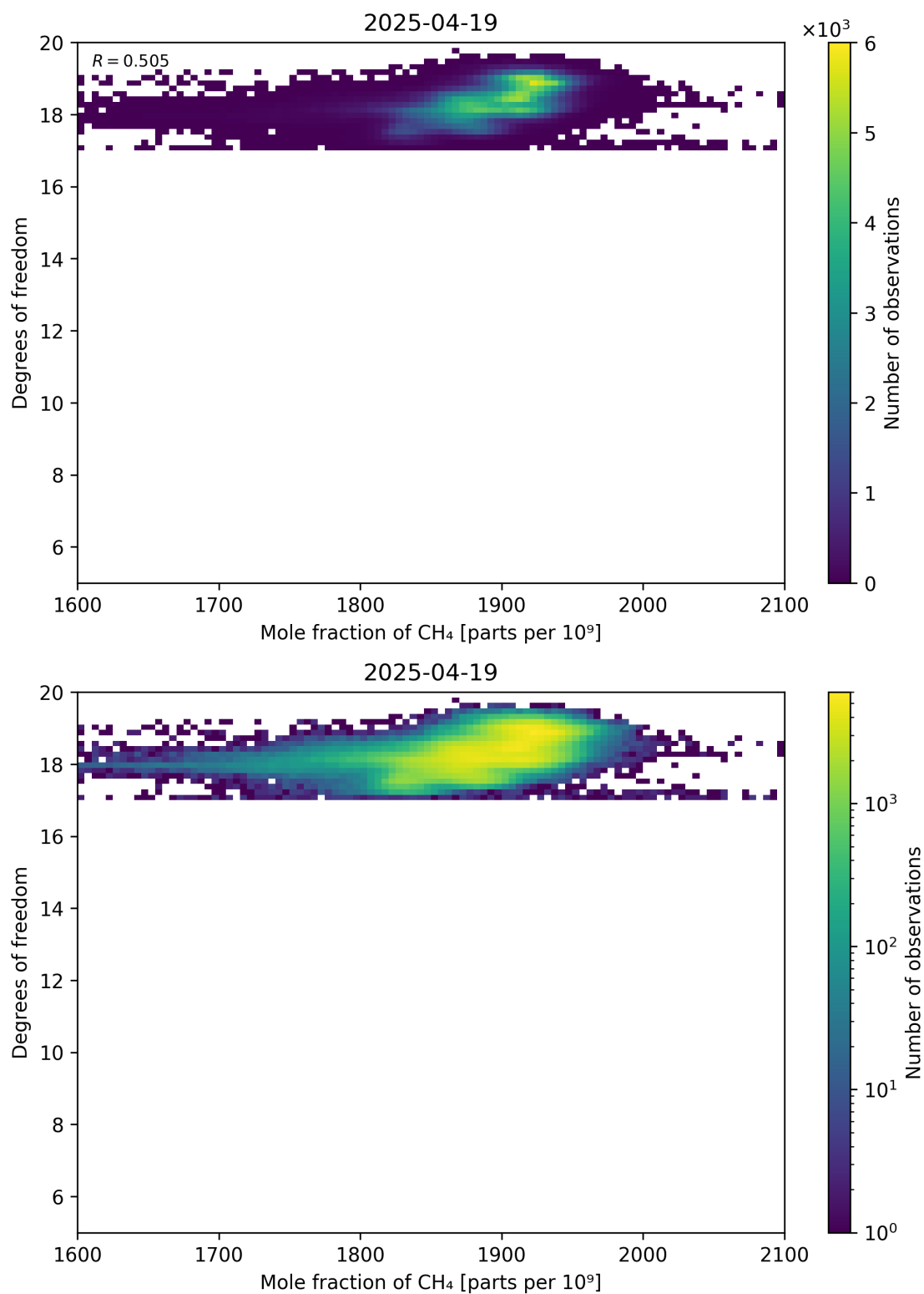
Figure 72: Scatter density plot of “Mole fraction of CH 4 ” against “Degrees of freedom” for 2025-04-19 to 2025-04-20.
