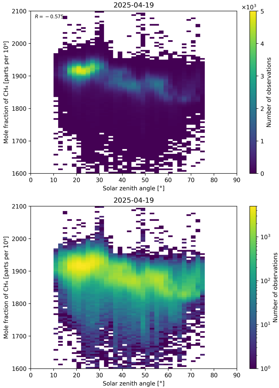
Figure 99: Scatter density plot of “Solar zenith angle” against “Mole fraction of \text{CH}_4 ” for 2025-04-19 to 2025-04-20.
