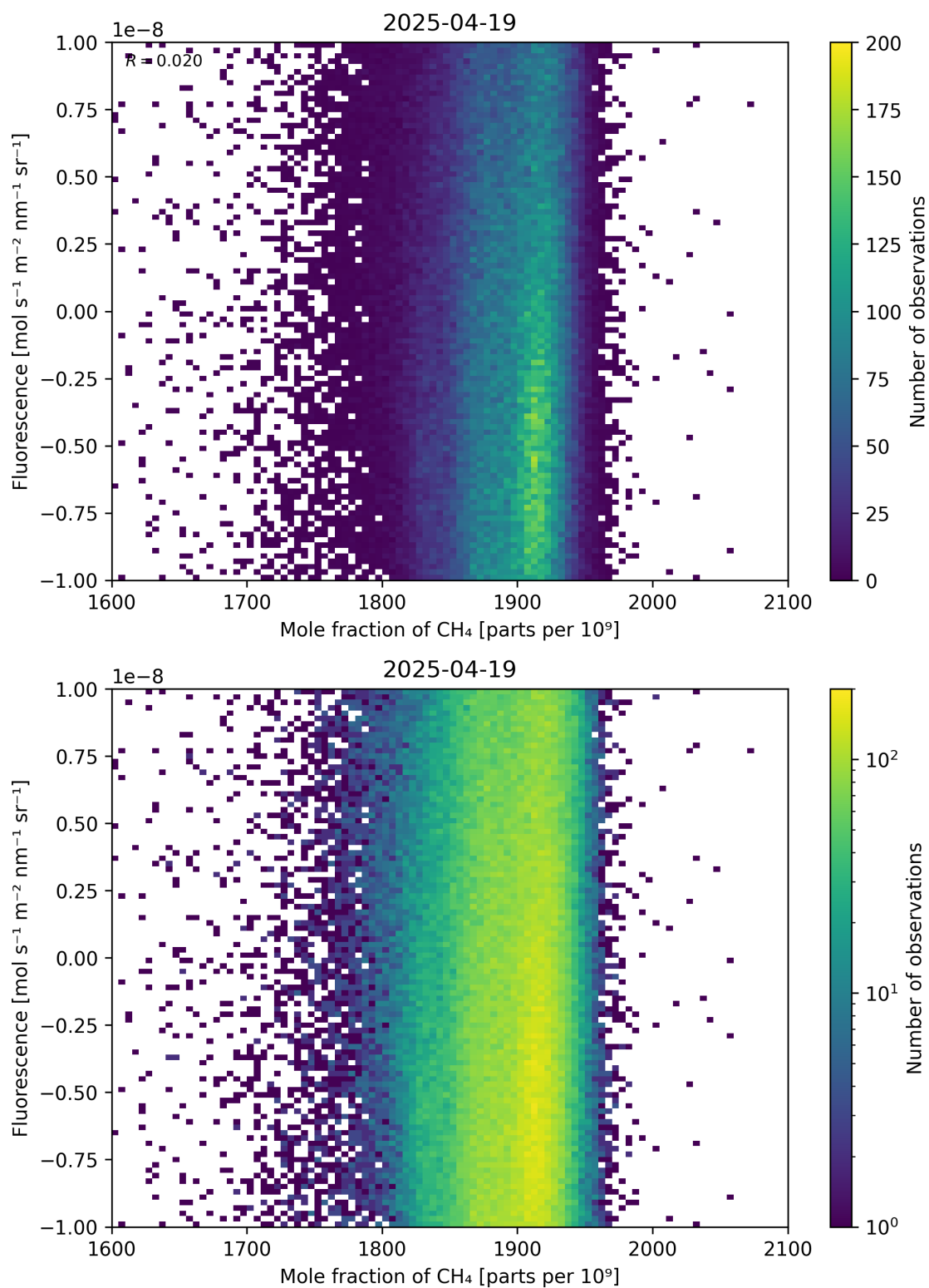
Figure 73: Scatter density plot of “Mole fraction of \text{CH}_4 ” against “Fluorescence” for 2025-04-19 to 2025-04-20.
