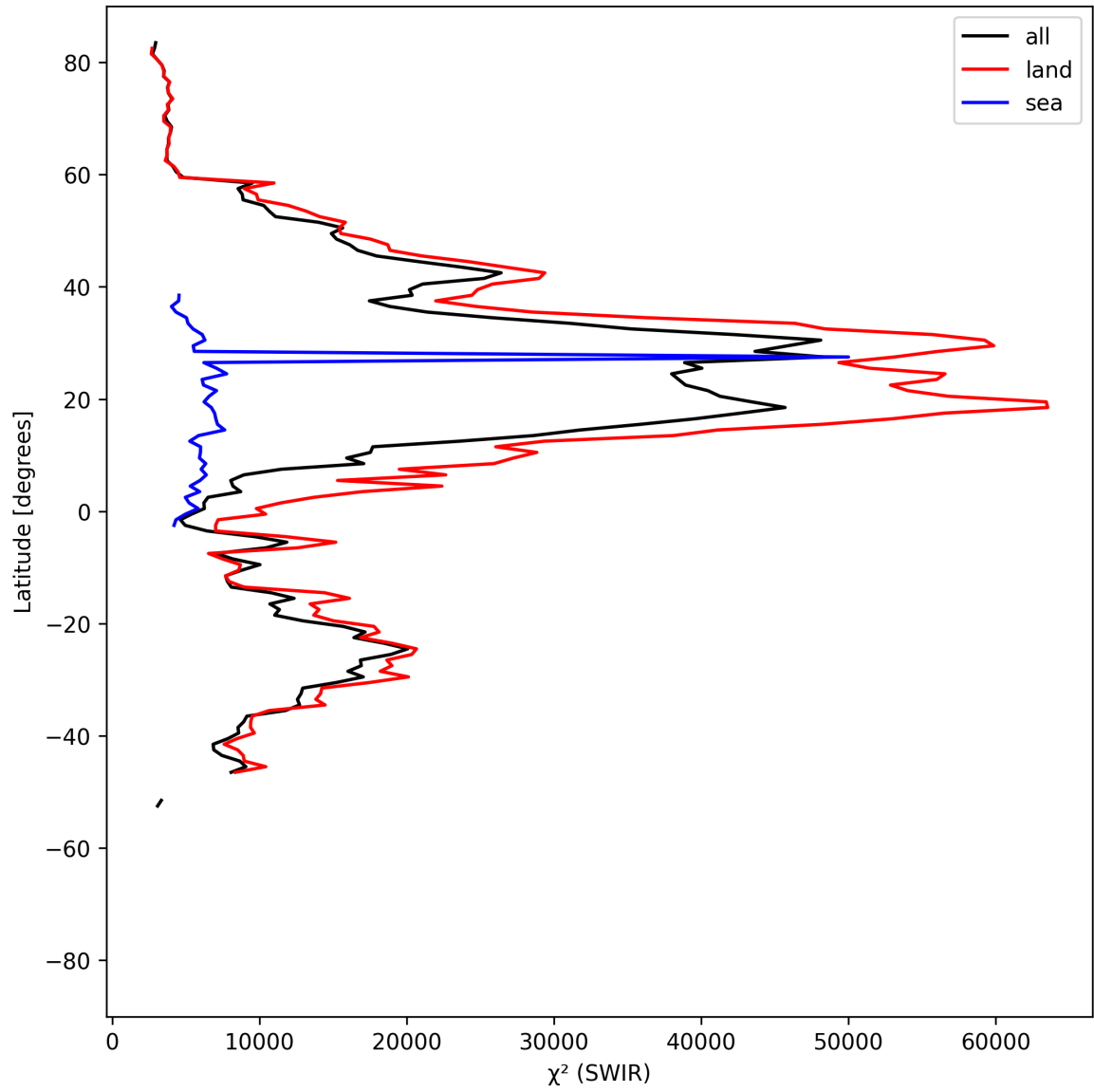
Figure 17: Zonal average of “ \chi^2 (SWIR)” for 2025-04-19 to 2025-04-20.
