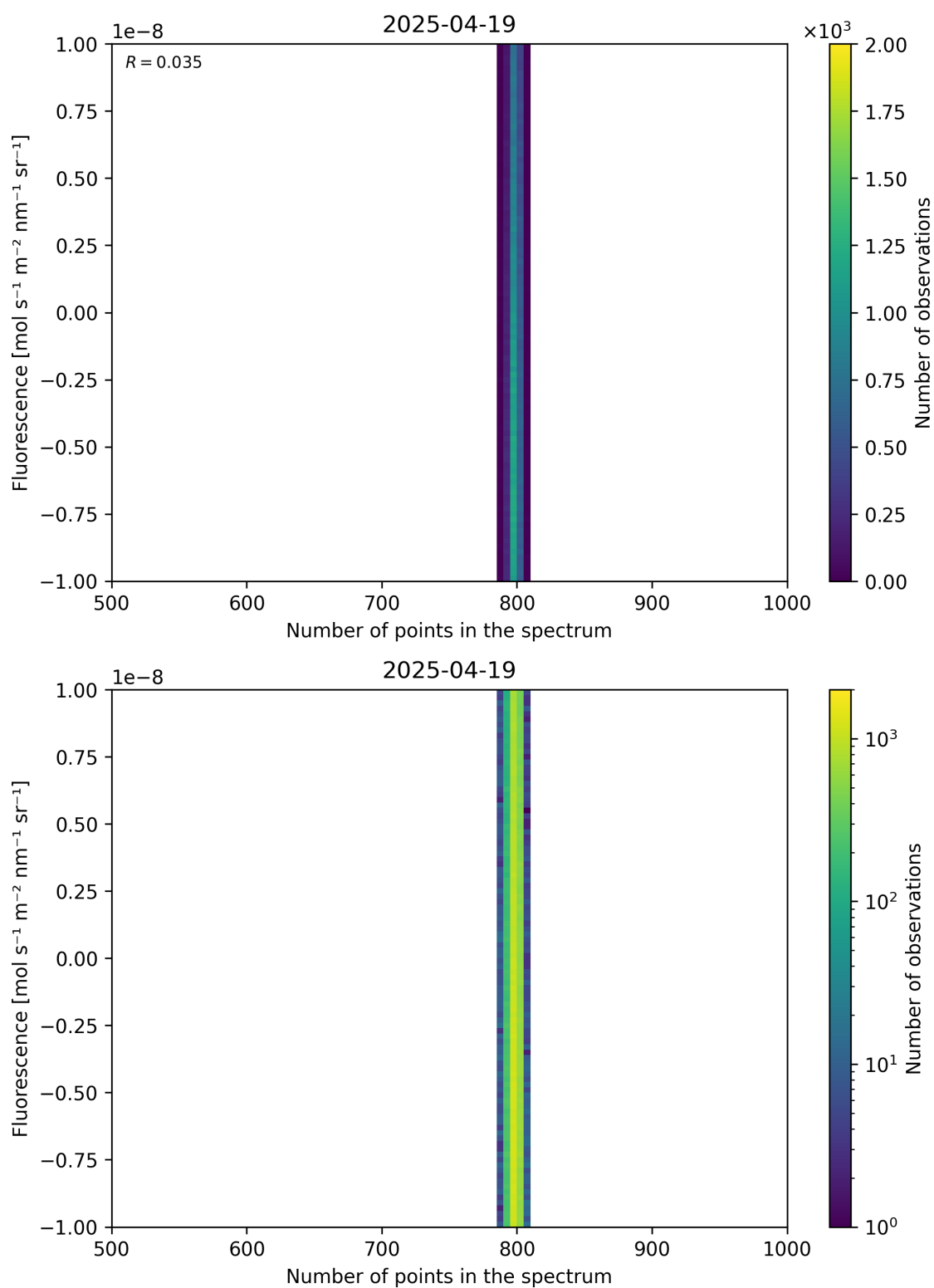
Figure 91: Scatter density plot of “Number of points in the spectrum” against “Fluorescence” for 2025-04-19 to 2025-04-20.
