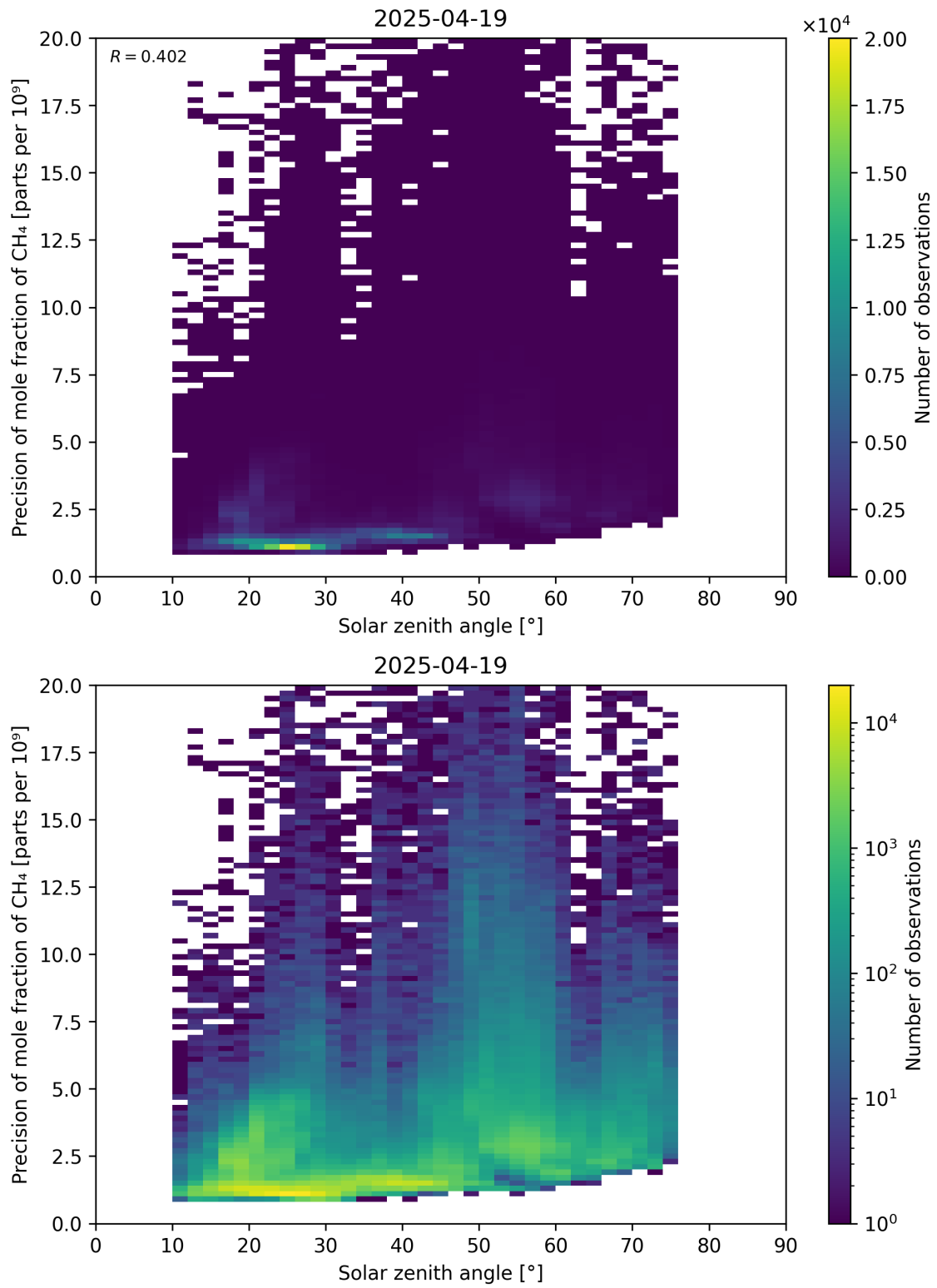
Figure 101: Scatter density plot of “Solar zenith angle” against “Precision of mole fraction of \text{CH}_4 ” for 2025-04-19 to 2025-04-20.
