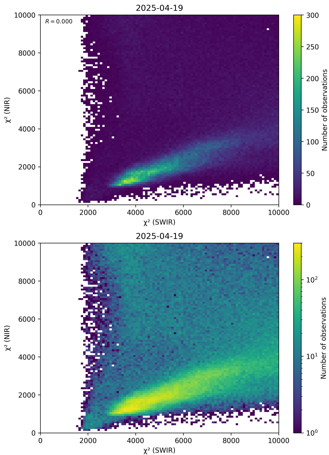
Figure 47: Scatter density plot of “ \chi^2 (SWIR)” against “ \chi^2 (NIR)” for 2025-04-19 to 2025-04-20.
