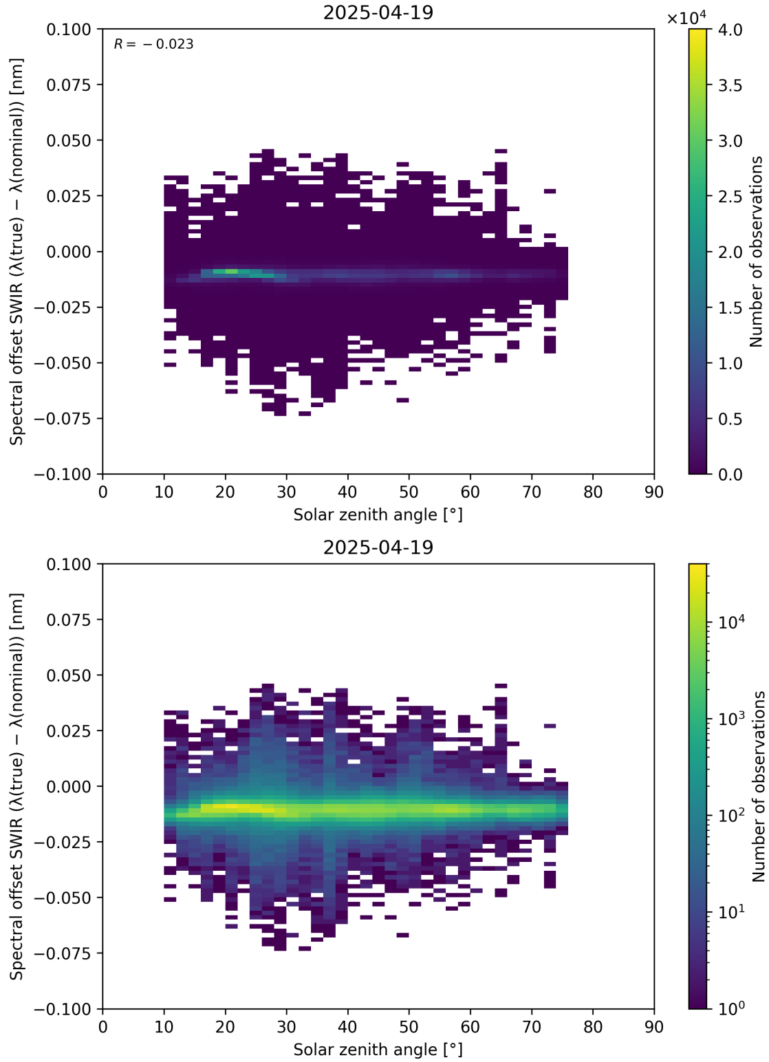
Figure 104: Scatter density plot of “Solar zenith angle” against “Spectral offset SWIR ( \lambda_{\text{true}} - \lambda_{\text{nominal}} )” for 2025-04-19 to 2025-04-20.
