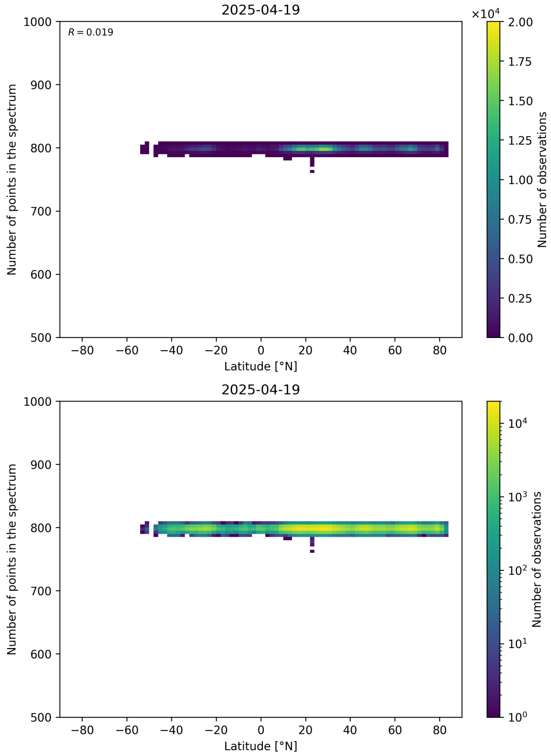
Figure 61: Scatter density plot of “Latitude” against “Number of points in the spectrum” for 2025-04-19 to 2025-04-20.
