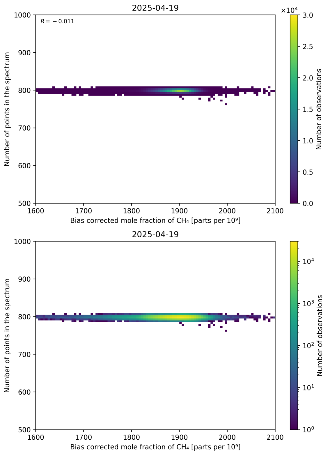
Figure 68: Scatter density plot of “Bias corrected mole fraction of CH 4 ” against “Number of points in the spectrum” for 2025-04-19 to 2025-04-20.
