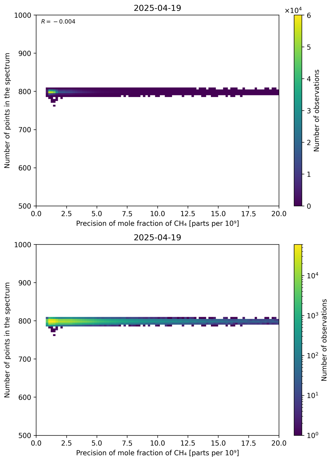
Figure 84: Scatter density plot of “Precision of mole fraction of CH 4 ” against “Number of points in the spectrum” for 2025-04-19 to 2025-04-20.
