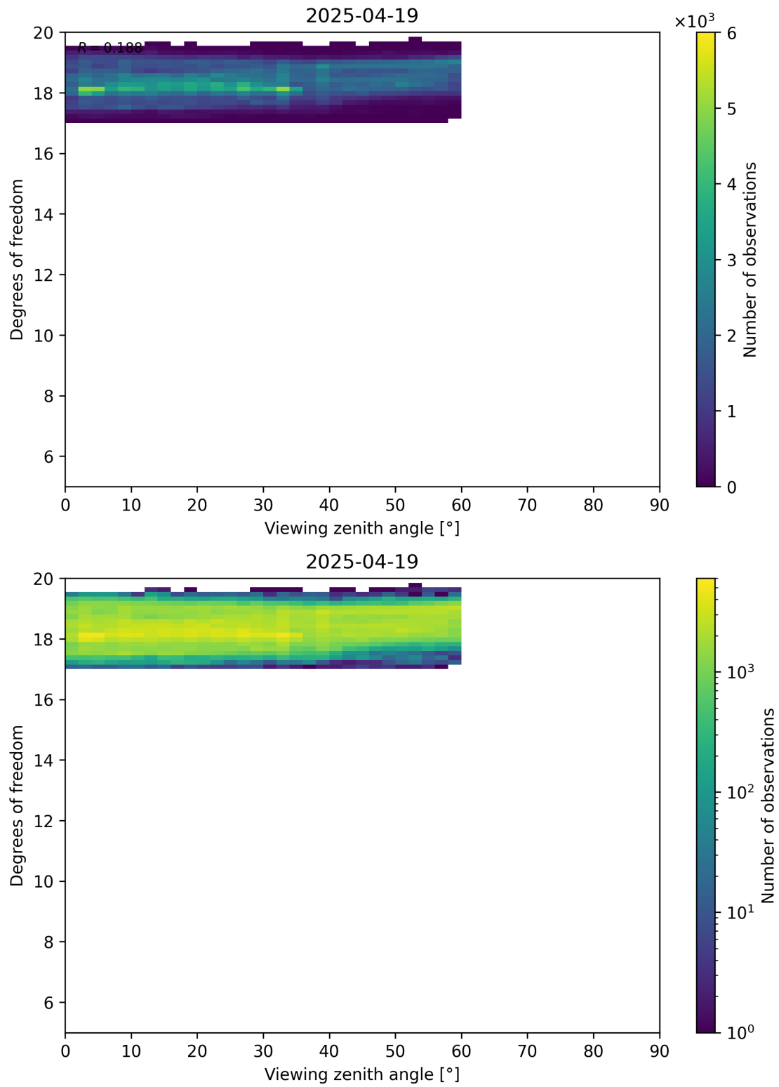
Figure 107: Scatter density plot of “Viewing zenith angle” against “Degrees of freedom” for 2025-04-19 to 2025-04-20.
