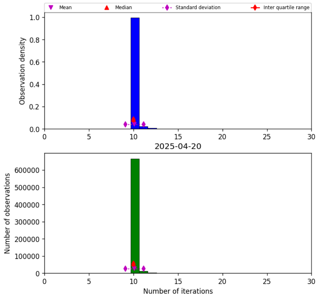
Figure 31: Histogram of “Number of iterations” for 2025-04-19 to 2025-04-21
