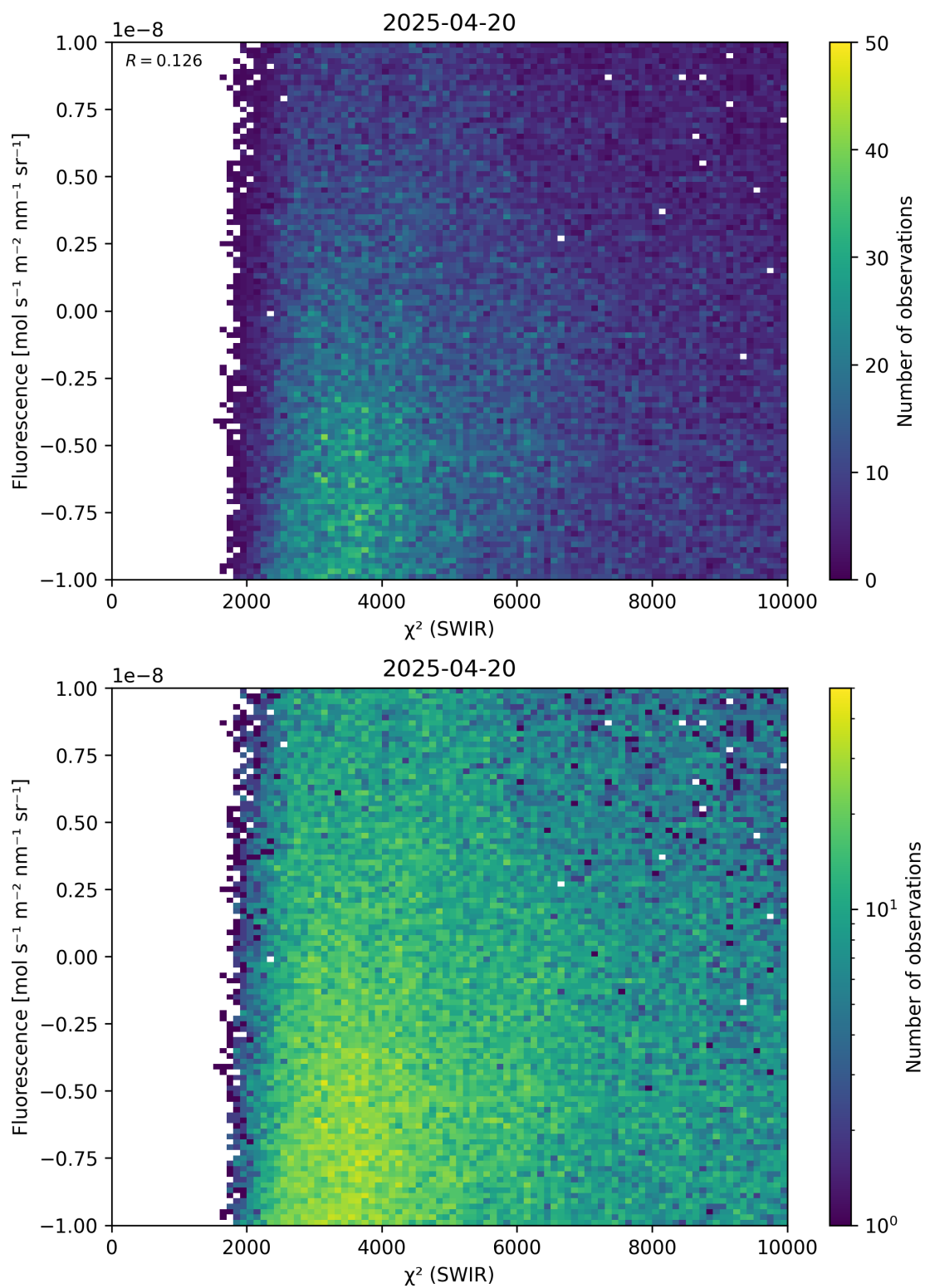
Figure 49: Scatter density plot of “ \chi^2 (SWIR)” against “Fluorescence” for 2025-04-19 to 2025-04-21.
