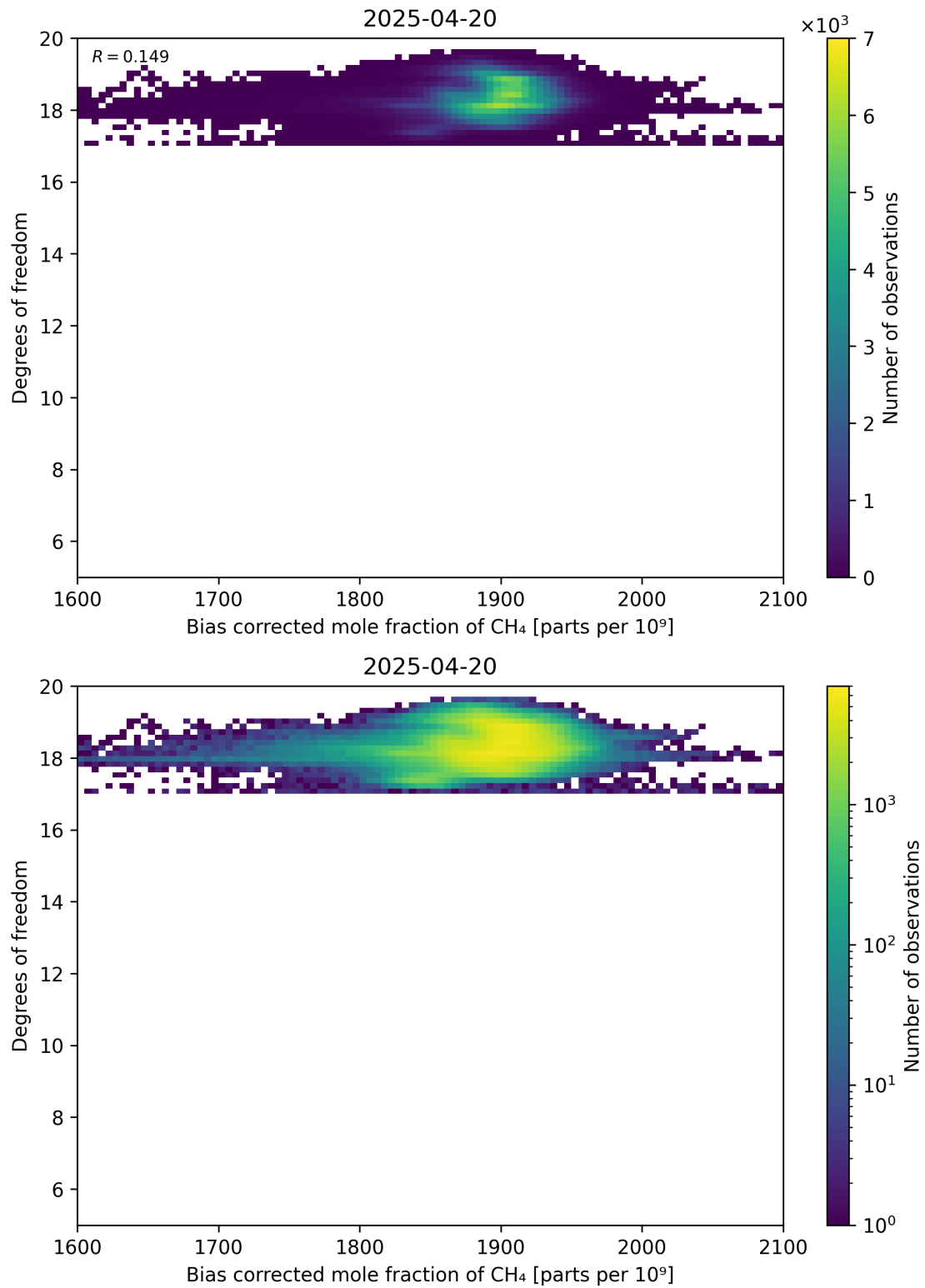
Figure 65: Scatter density plot of “Bias corrected mole fraction of CH 4 ” against “Degrees of freedom” for 2025-04-19 to 2025-04-21.
