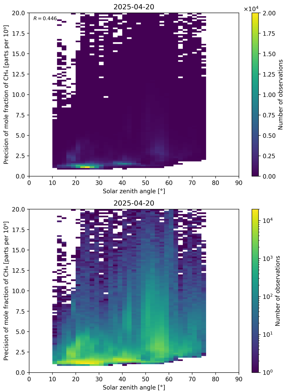
Figure 101: Scatter density plot of “Solar zenith angle” against “Precision of mole fraction of \text{CH}_4 ” for 2025-04-19 to 2025-04-21.
