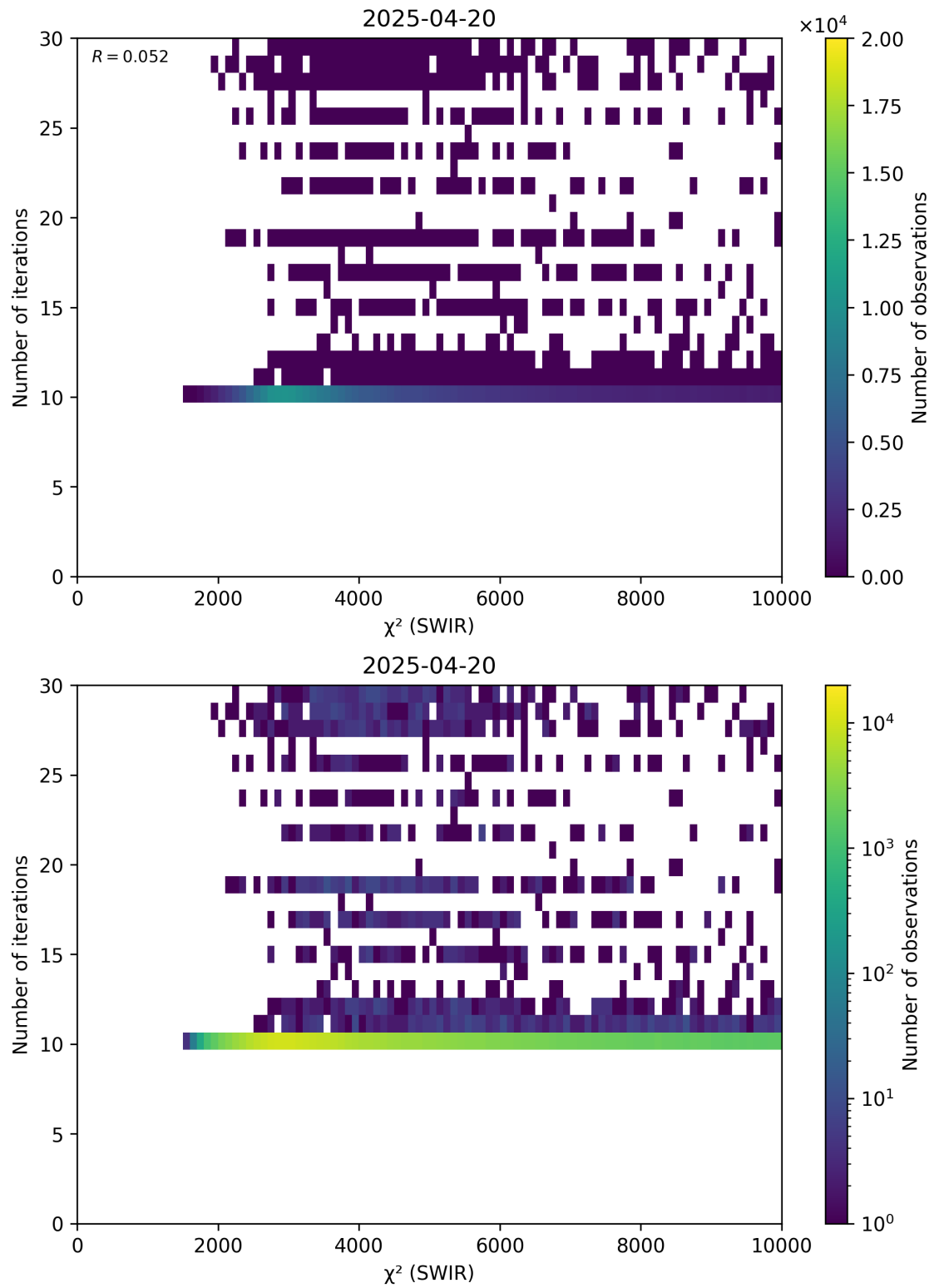
Figure 50: Scatter density plot of “ \chi^2 (SWIR)” against “Number of iterations” for 2025-04-19 to 2025-04-21.
