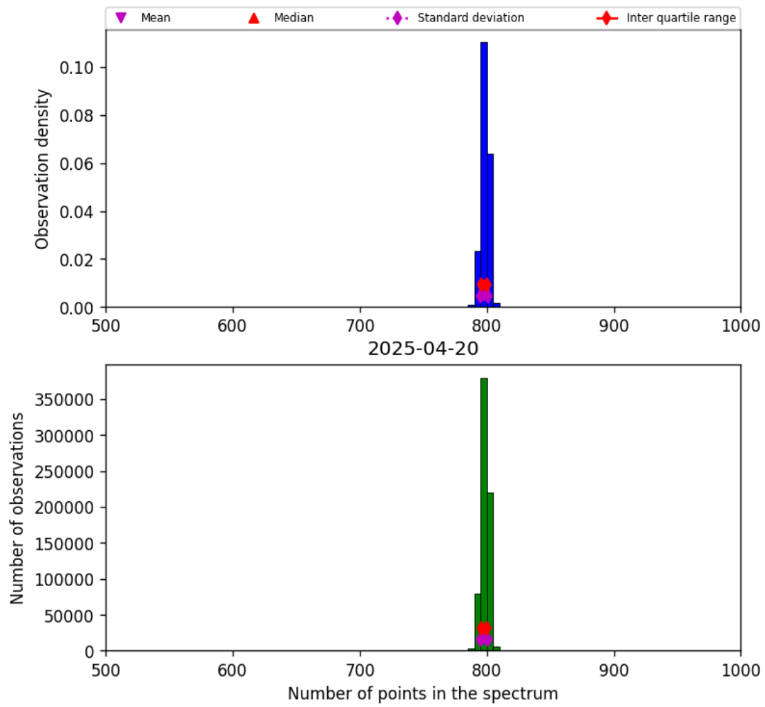
Figure 26: Histogram of “Number of points in the spectrum” for 2025-04-19 to 2025-04-21
