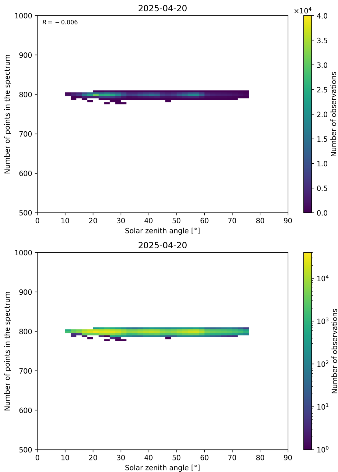
Figure 103: Scatter density plot of “Solar zenith angle” against “Number of points in the spectrum” for 2025-04-19 to 2025-04-21.
