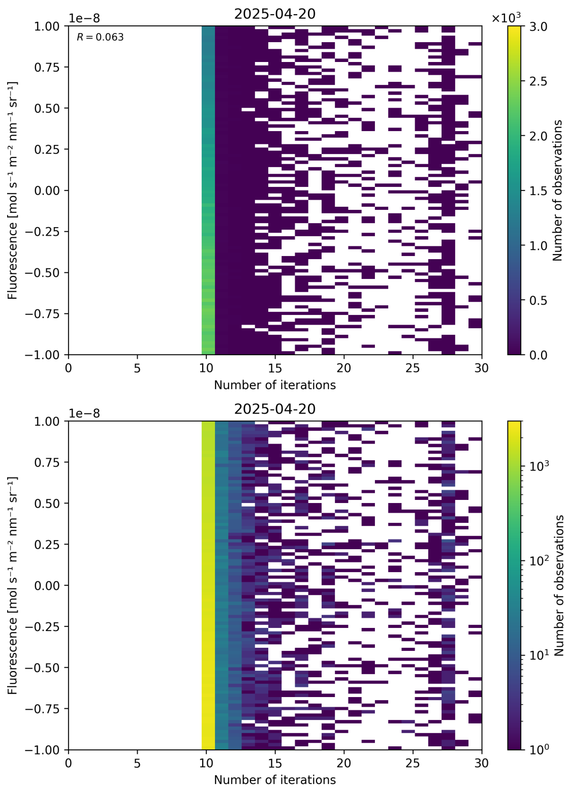
Figure 87: Scatter density plot of “Number of iterations” against “Fluorescence” for 2025-04-19 to 2025-04-21.
