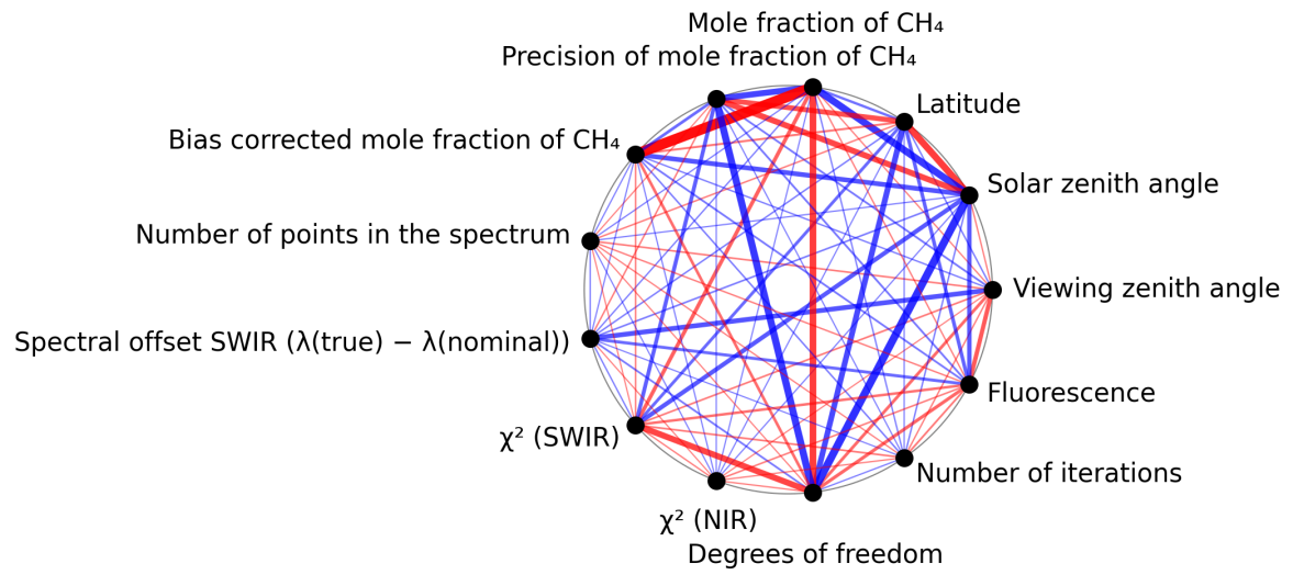
Figure 1: Map of correlation graph for 2025-04-19 to 2025-04-21.
