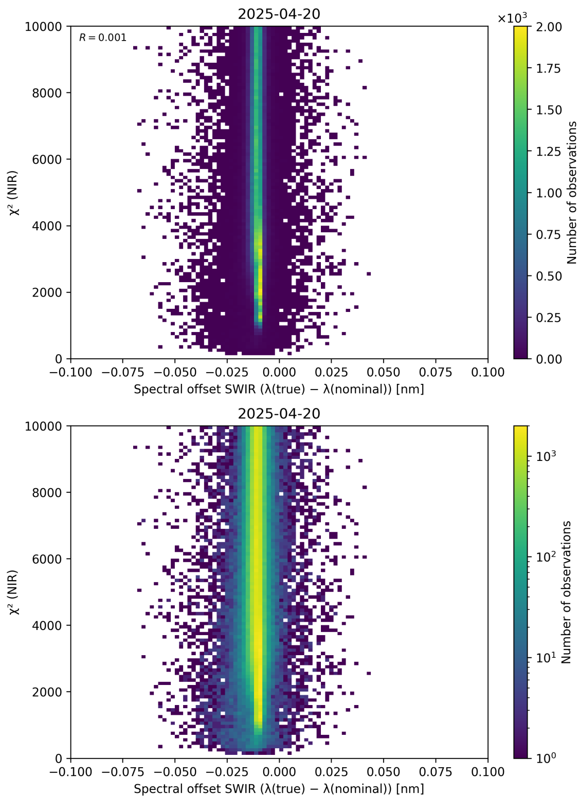
Figure 117: Scatter density plot of “Spectral offset SWIR ( \lambda_{\text{true}} - \lambda_{\text{nominal}} )” against “ \chi^2 (NIR)” for 2025-04-19 to 2025-04-21.
