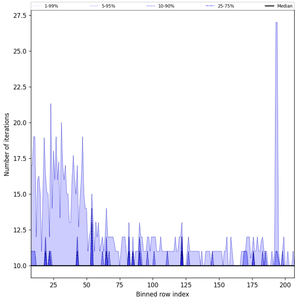
Figure 42: Along track statistics of “Number of iterations” for 2025-04-19 to 2025-04-21
