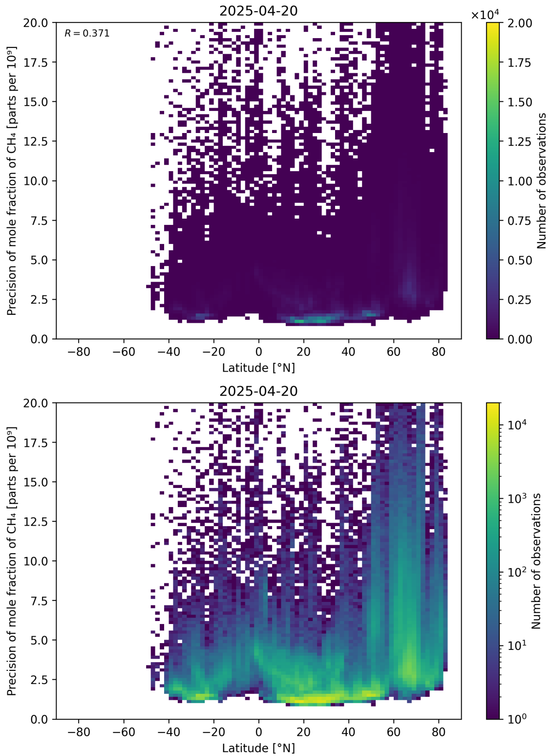
Figure 59: Scatter density plot of “Latitude” against “Precision of mole fraction of \text{CH}_4 ” for 2025-04-19 to 2025-04-21.
