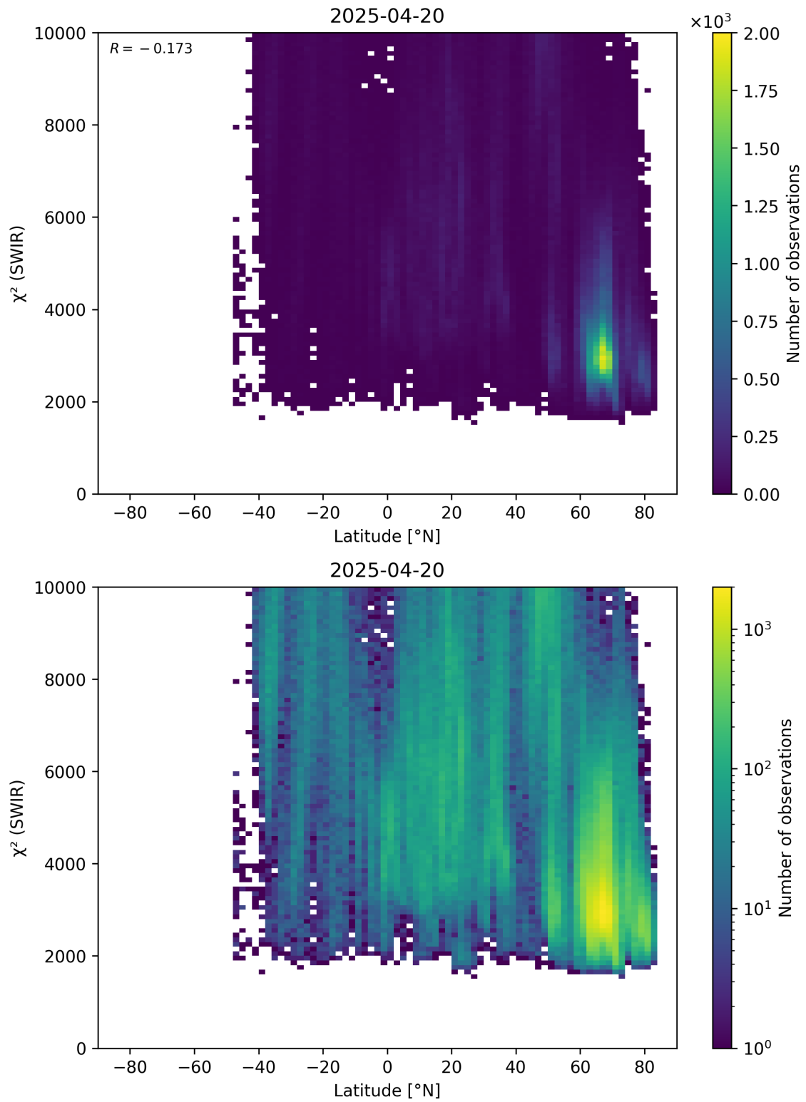
Figure 54: Scatter density plot of “Latitude” against “ \chi^2 (SWIR)” for 2025-04-19 to 2025-04-21.
