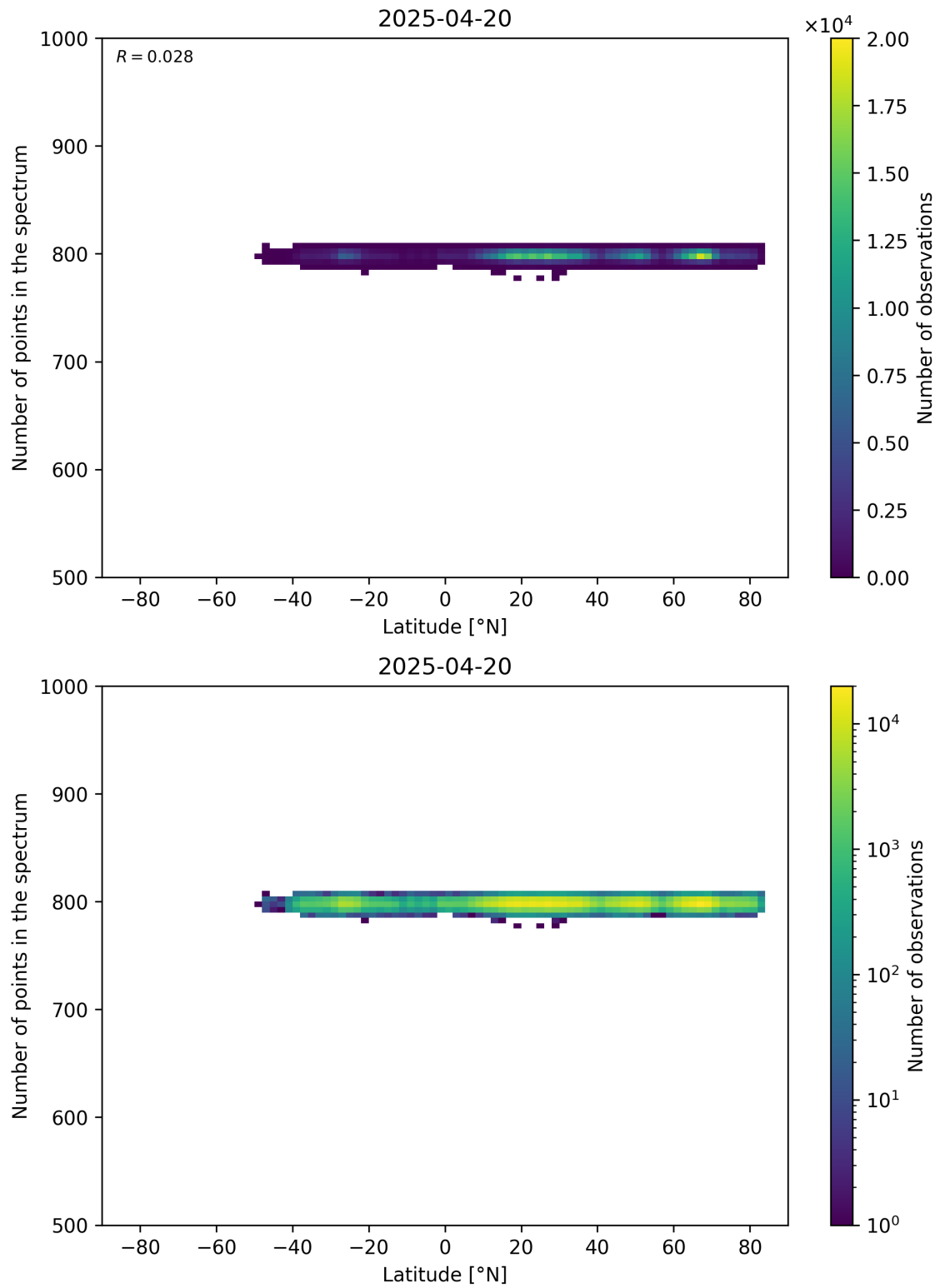
Figure 61: Scatter density plot of “Latitude” against “Number of points in the spectrum” for 2025-04-19 to 2025-04-21.
