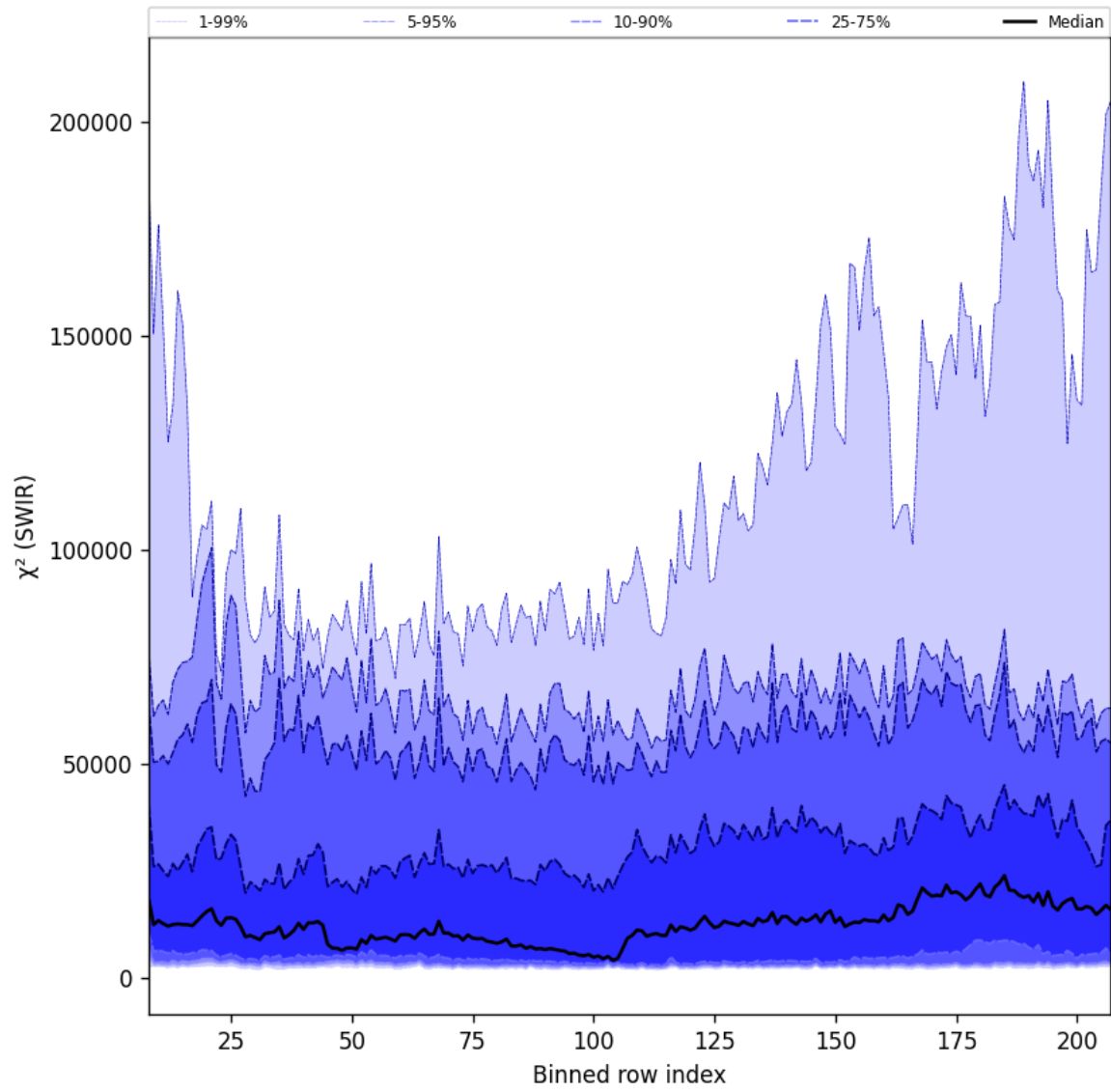
Figure 39: Along track statistics of “ \chi^2 (SWIR)” for 2025-04-19 to 2025-04-21
