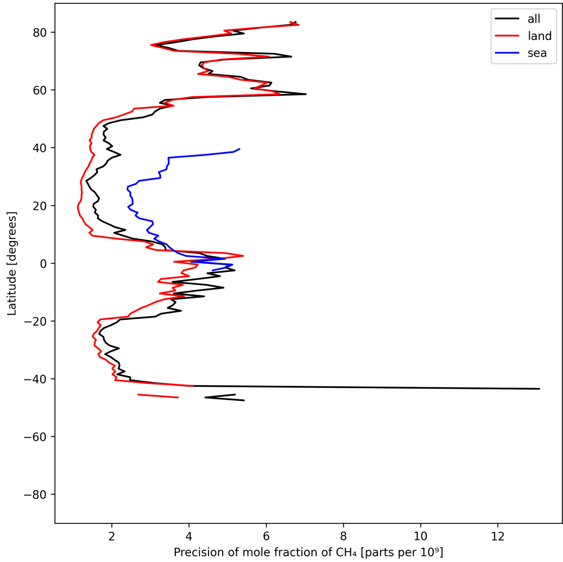
Figure 13: Zonal average of “Precision of mole fraction of CH 4 ” for 2025-04-19 to 2025-04-21.
