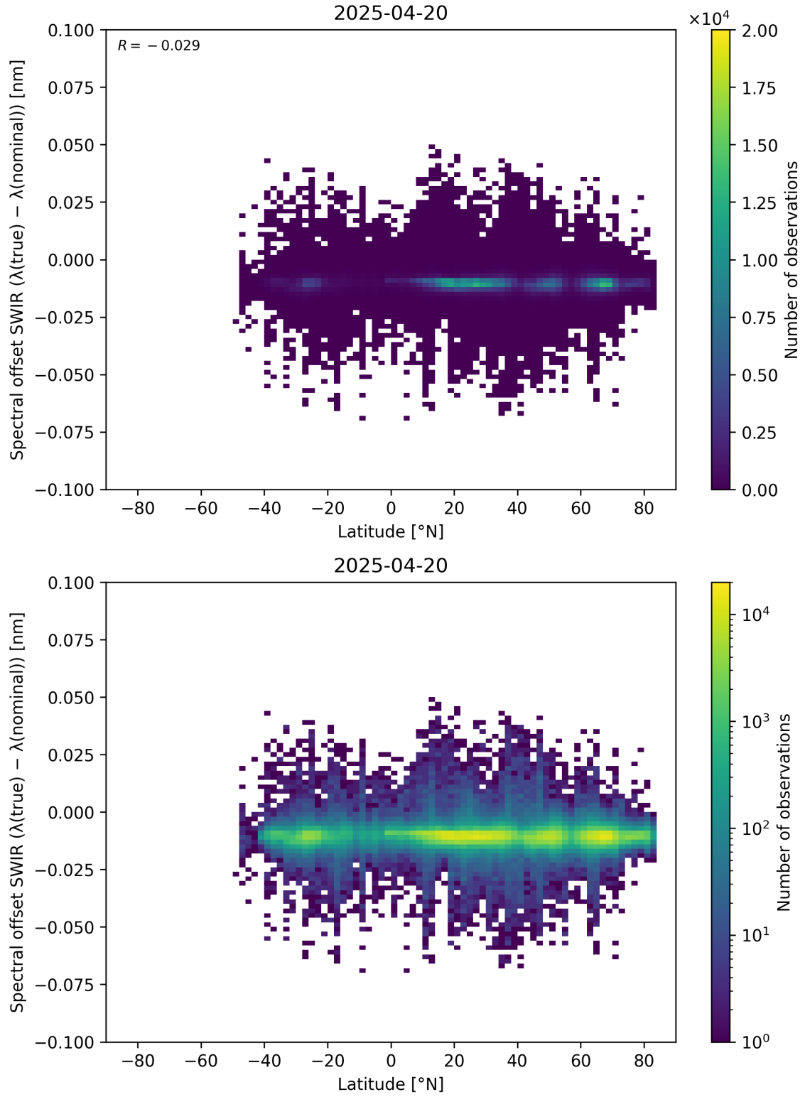
Figure 62: Scatter density plot of “Latitude” against “Spectral offset SWIR ( \lambda_{\text{true}} - \lambda_{\text{nominal}} )” for 2025-04-19 to 2025-04-21.
