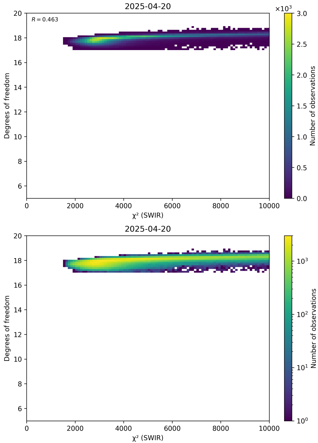
Figure 48: Scatter density plot of “ \chi^2 (SWIR)” against “Degrees of freedom” for 2025-04-19 to 2025-04-21.
