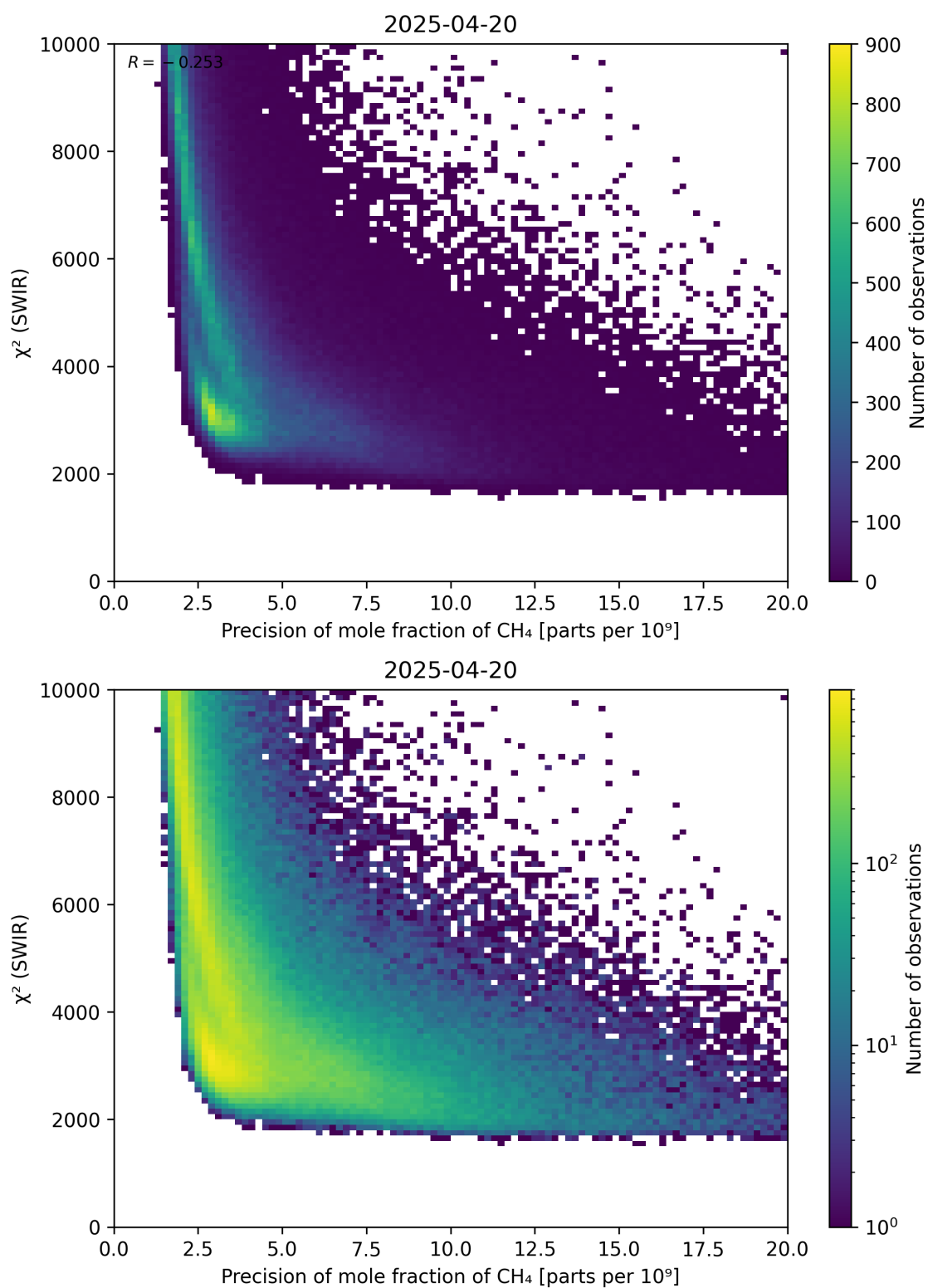
Figure 79: Scatter density plot of “Precision of mole fraction of \text{CH}_4 ” against “ \chi^2 (SWIR)” for 2025-04-19 to 2025-04-21.
