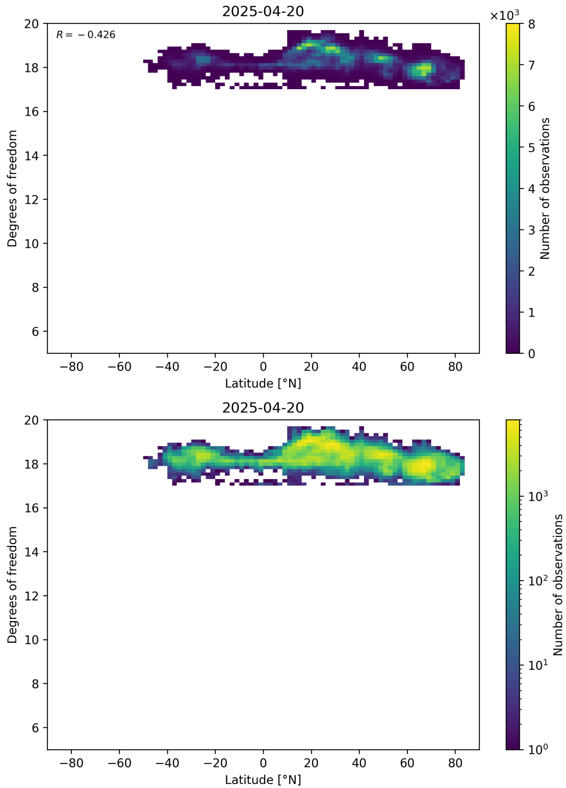
Figure 55: Scatter density plot of “Latitude” against “Degrees of freedom” for 2025-04-19 to 2025-04-21.
