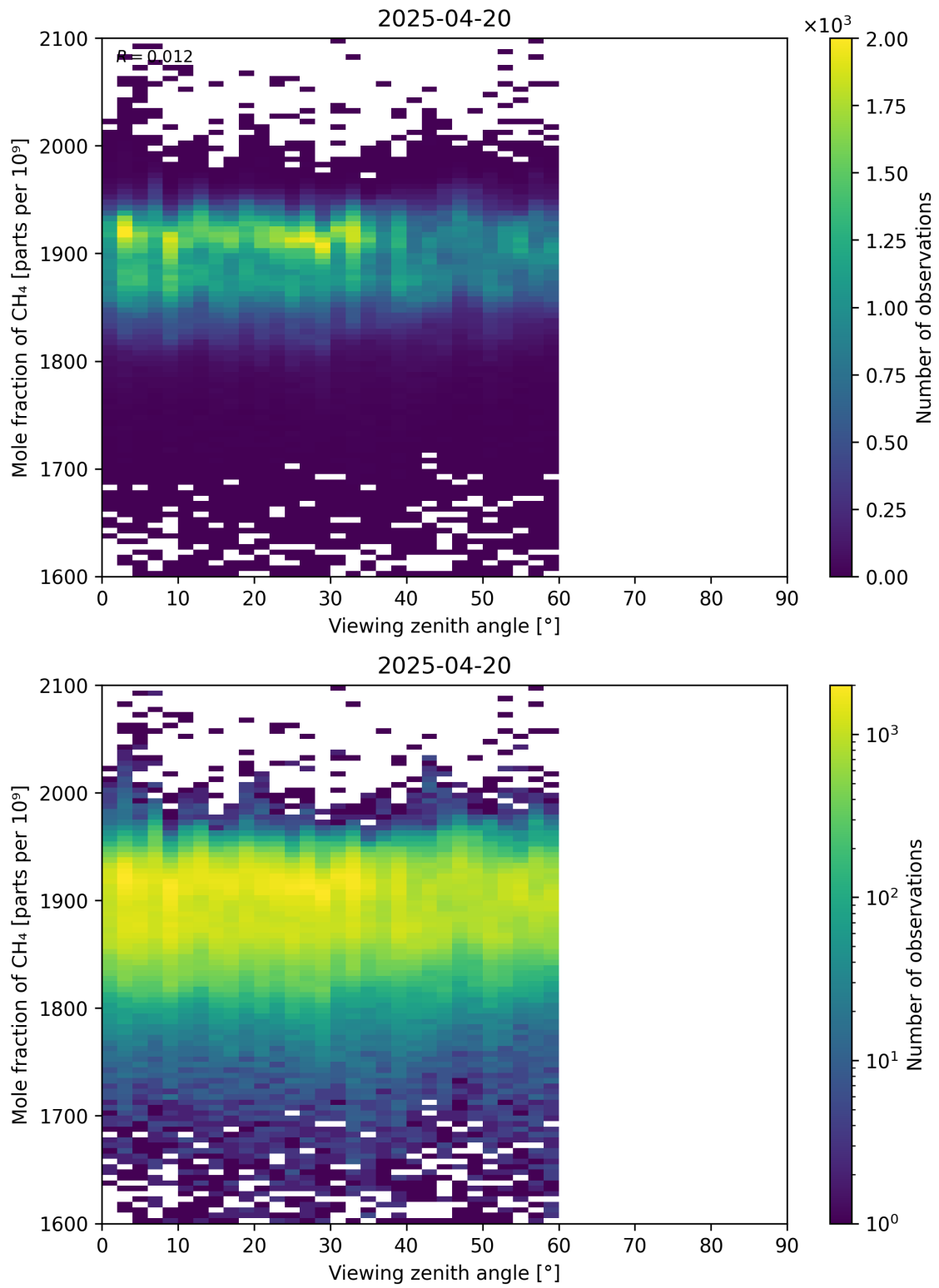
Figure 110: Scatter density plot of “Viewing zenith angle” against “Mole fraction of CH 4 ” for 2025-04-19 to 2025-04-21.
