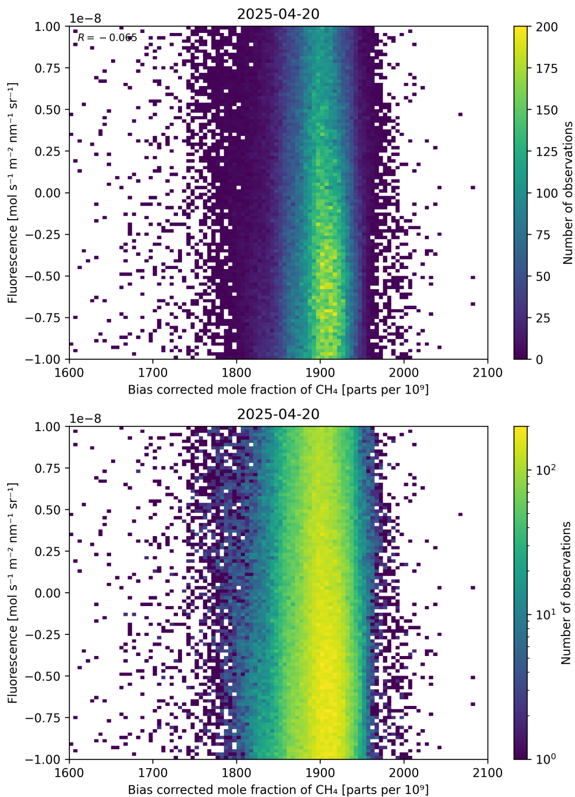
Figure 66: Scatter density plot of “Bias corrected mole fraction of \text{CH}_4 ” against “Fluorescence” for 2025-04-19 to 2025-04-21.
