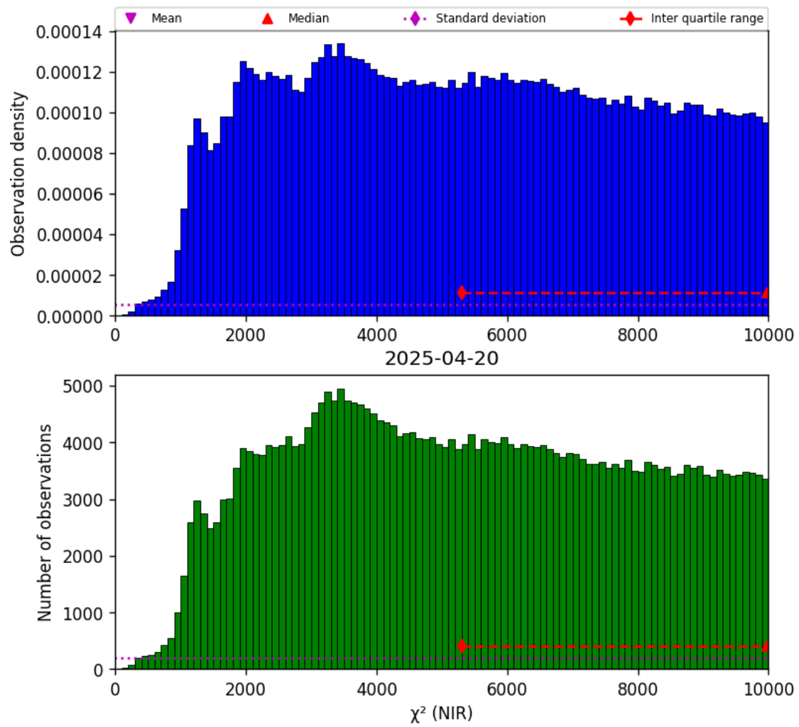
Figure 29: Histogram of “ \chi^2 (NIR)” for 2025-04-19 to 2025-04-21
