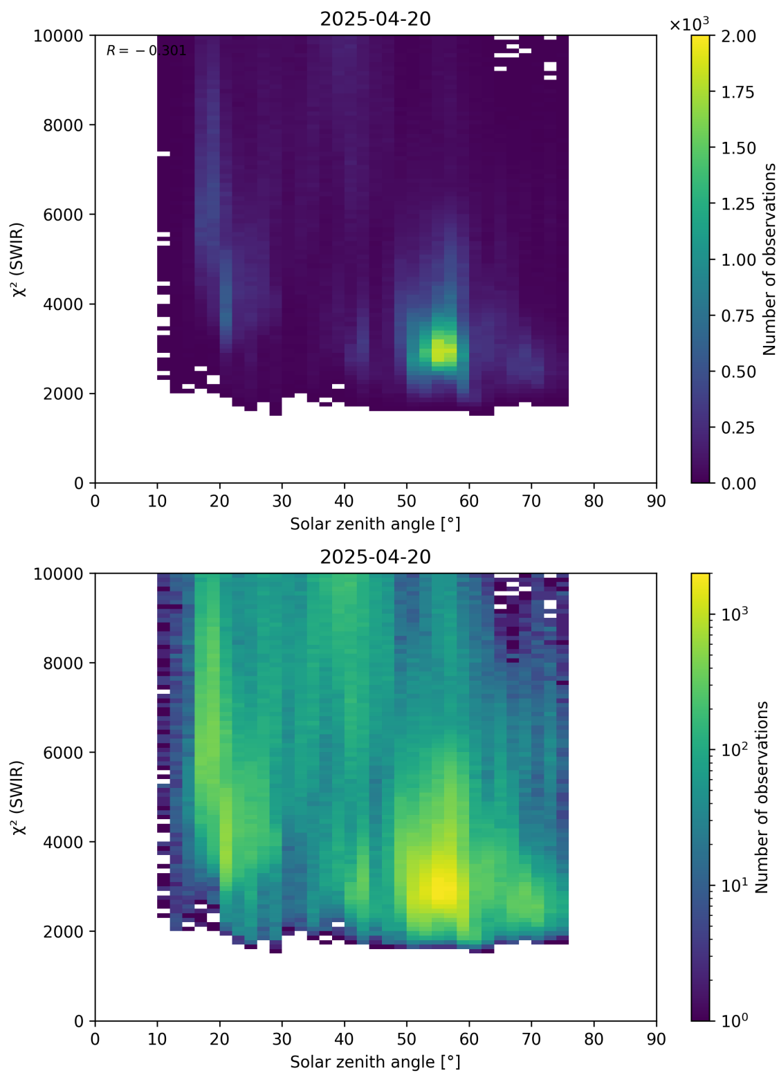
Figure 95: Scatter density plot of “Solar zenith angle” against “ \chi^2 (SWIR)” for 2025-04-19 to 2025-04-21.
