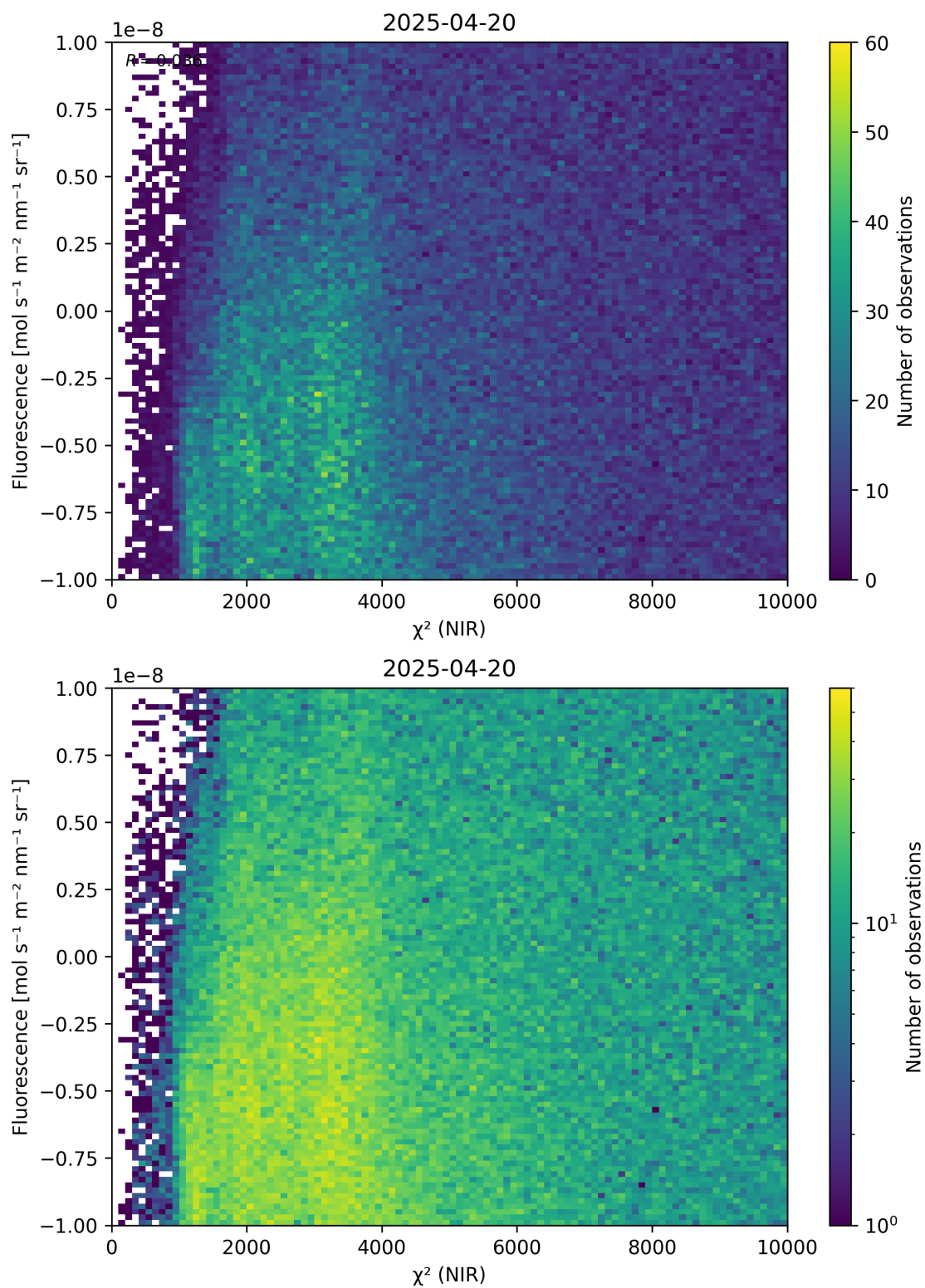
Figure 45: Scatter density plot of “ \chi^2 (NIR)” against “Fluorescence” for 2025-04-19 to 2025-04-21.
