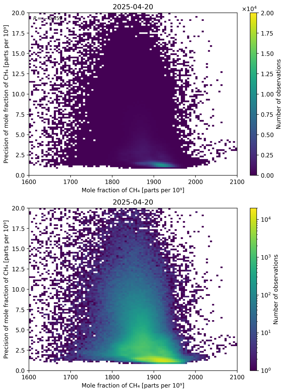
Figure 75: Scatter density plot of “Mole fraction of CH 4 ” against “Precision of mole fraction of CH 4 ” for 2025-04-19 to 2025-04-21.
