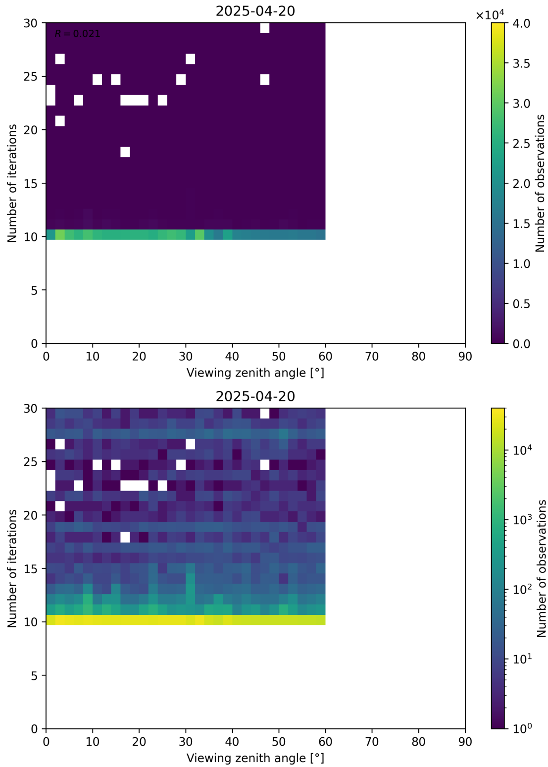
Figure 113: Scatter density plot of “Viewing zenith angle” against “Number of iterations” for 2025-04-19 to 2025-04-21.
