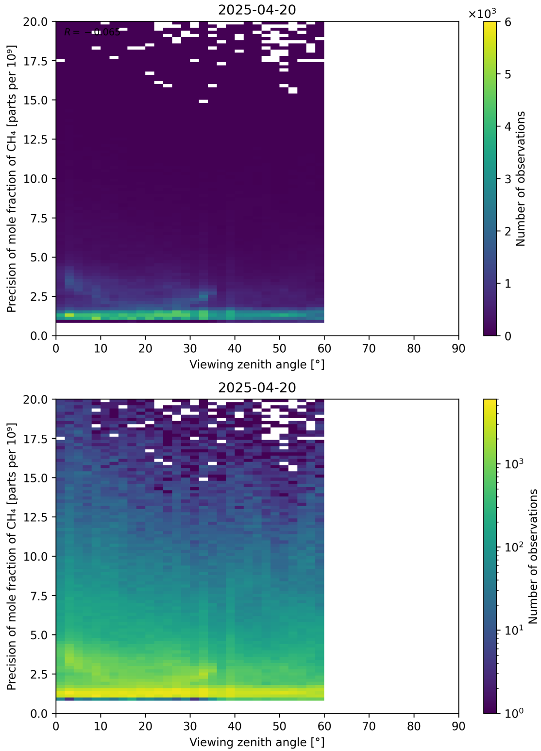
Figure 112: Scatter density plot of “Viewing zenith angle” against “Precision of mole fraction of CH 4 ” for 2025-04-19 to 2025-04-21.
