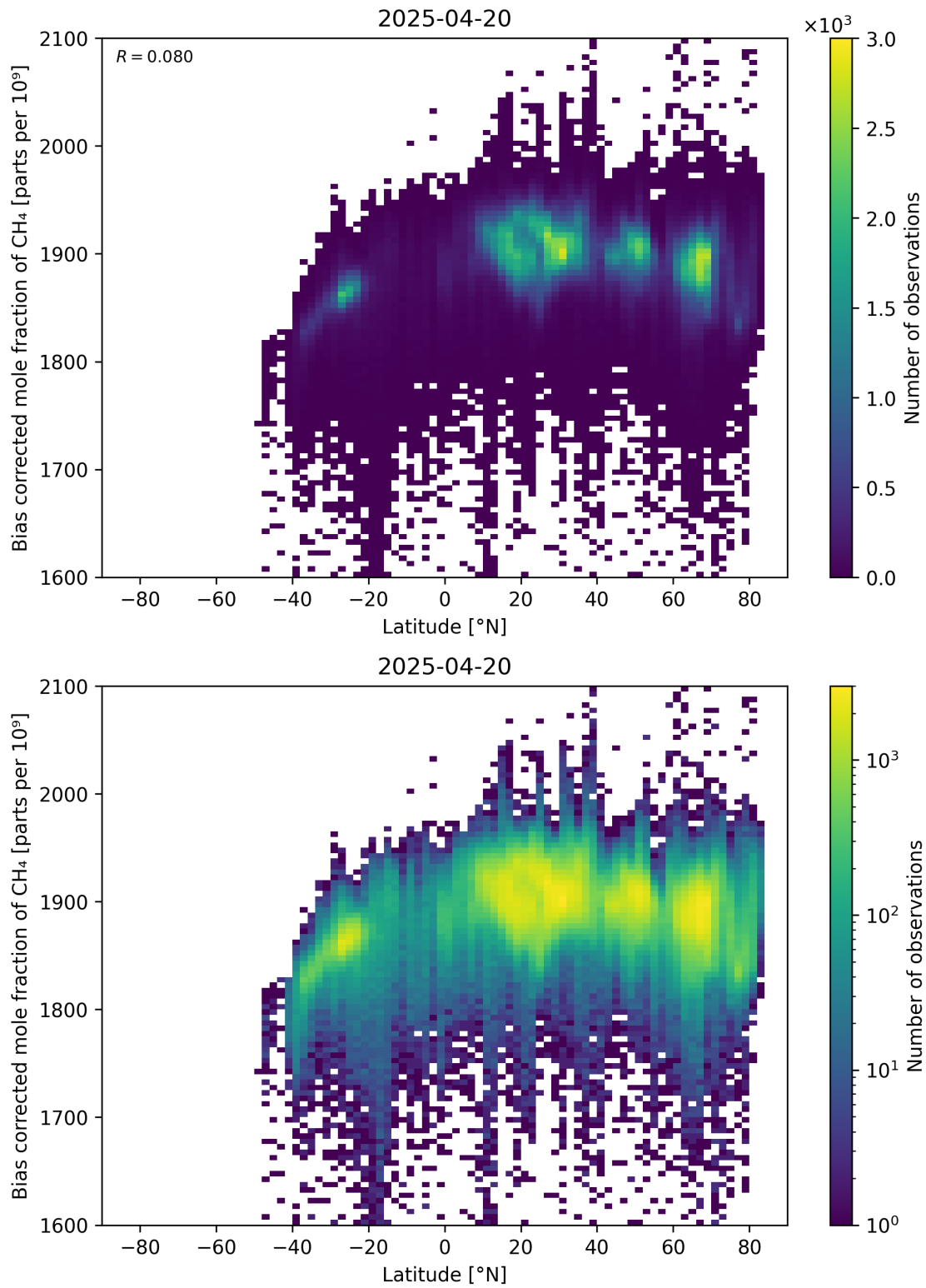
Figure 58: Scatter density plot of “Latitude” against “Bias corrected mole fraction of \text{CH}_4 ” for 2025-04-19 to 2025-04-21.
