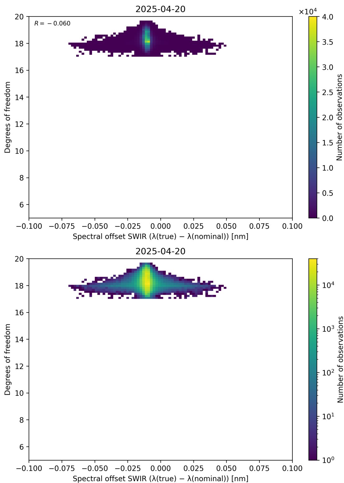
Figure 119: Scatter density plot of “Spectral offset SWIR ( \lambda_{\text{true}} - \lambda_{\text{nominal}} )” against “Degrees of freedom” for 2025-04-19 to 2025-04-21.
