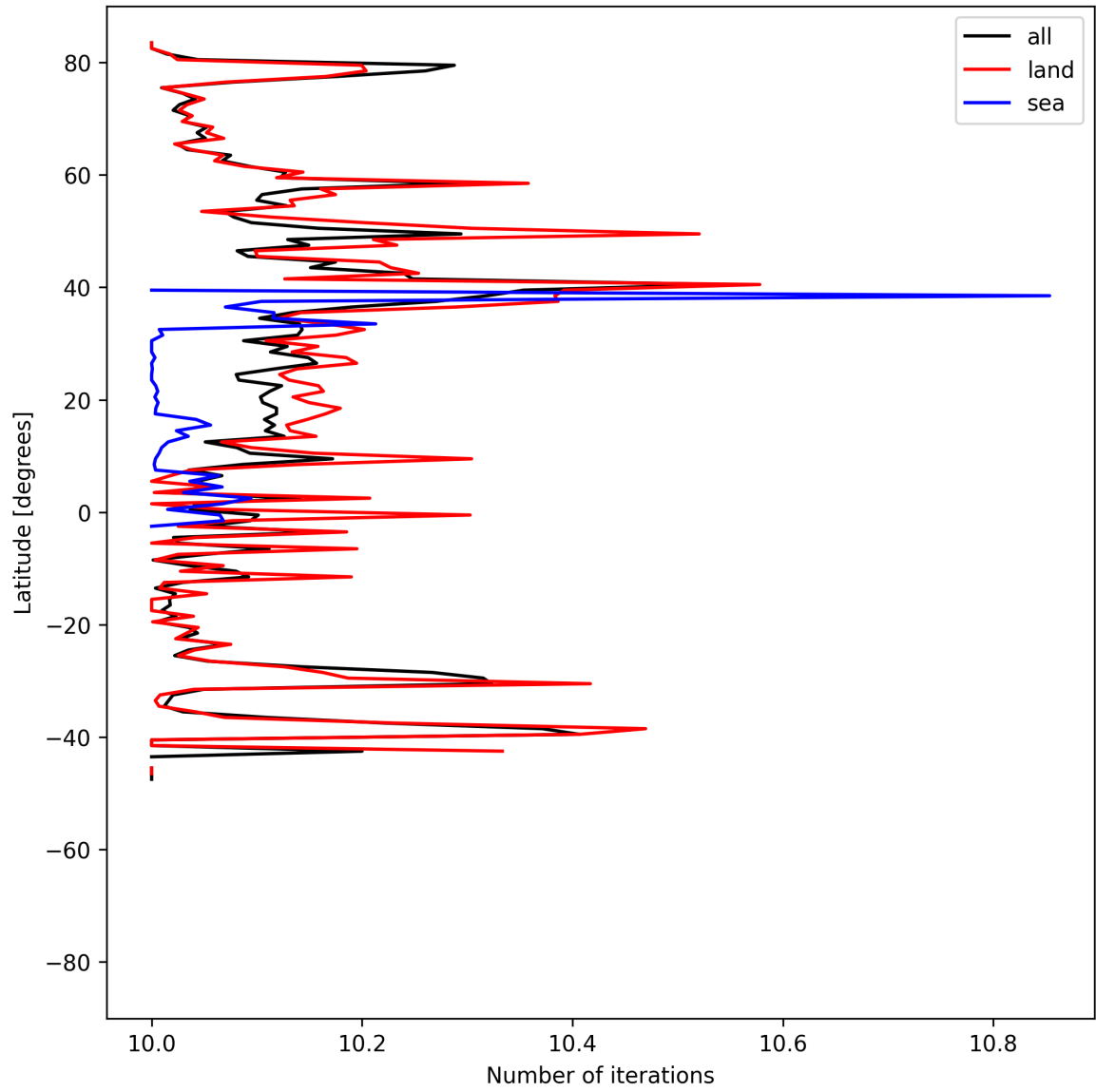
Figure 20: Zonal average of “Number of iterations” for 2025-04-19 to 2025-04-21.
