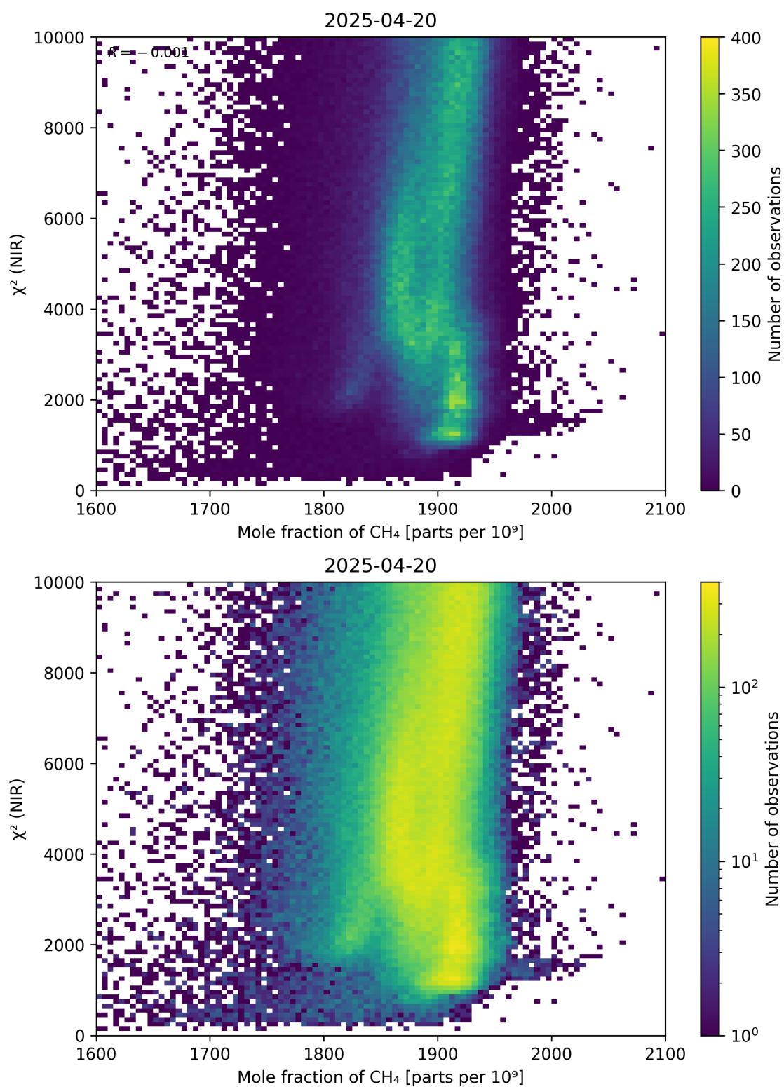
Figure 70: Scatter density plot of “Mole fraction of \text{CH}_4 ” against “ \chi^2 (NIR)” for 2025-04-19 to 2025-04-21.
