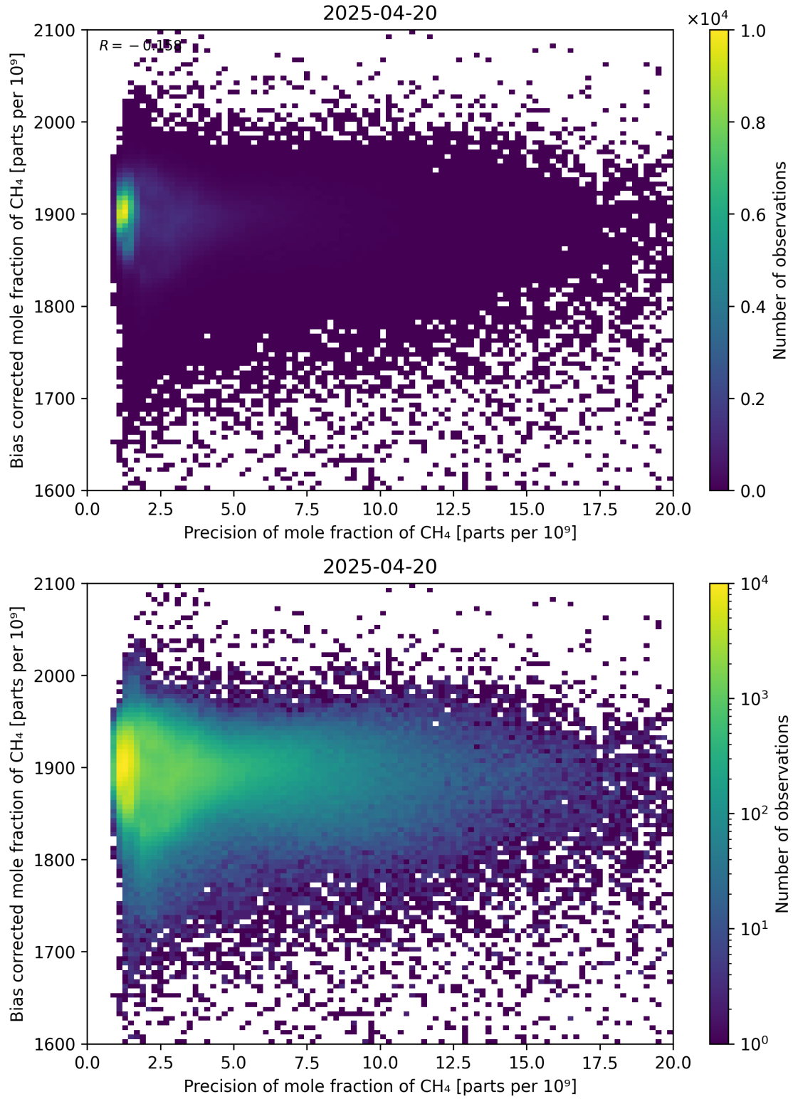
Figure 82: Scatter density plot of “Precision of mole fraction of CH 4 ” against “Bias corrected mole fraction of CH 4 ” for 2025-04-19 to 2025-04-21.
