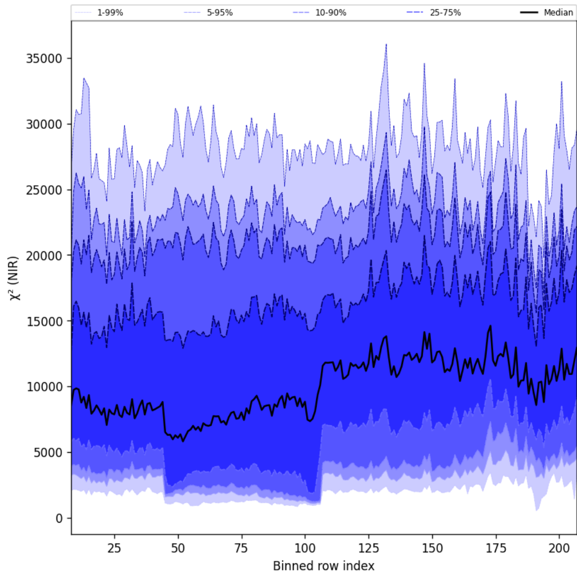
Figure 40: Along track statistics of “ \chi^2 (NIR)” for 2025-04-19 to 2025-04-21
