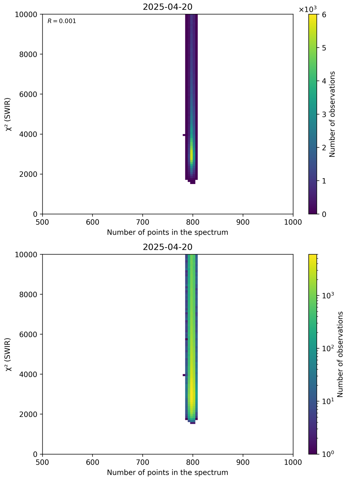
Figure 89: Scatter density plot of “Number of points in the spectrum” against “ \chi^2 (SWIR)” for 2025-04-19 to 2025-04-21.
