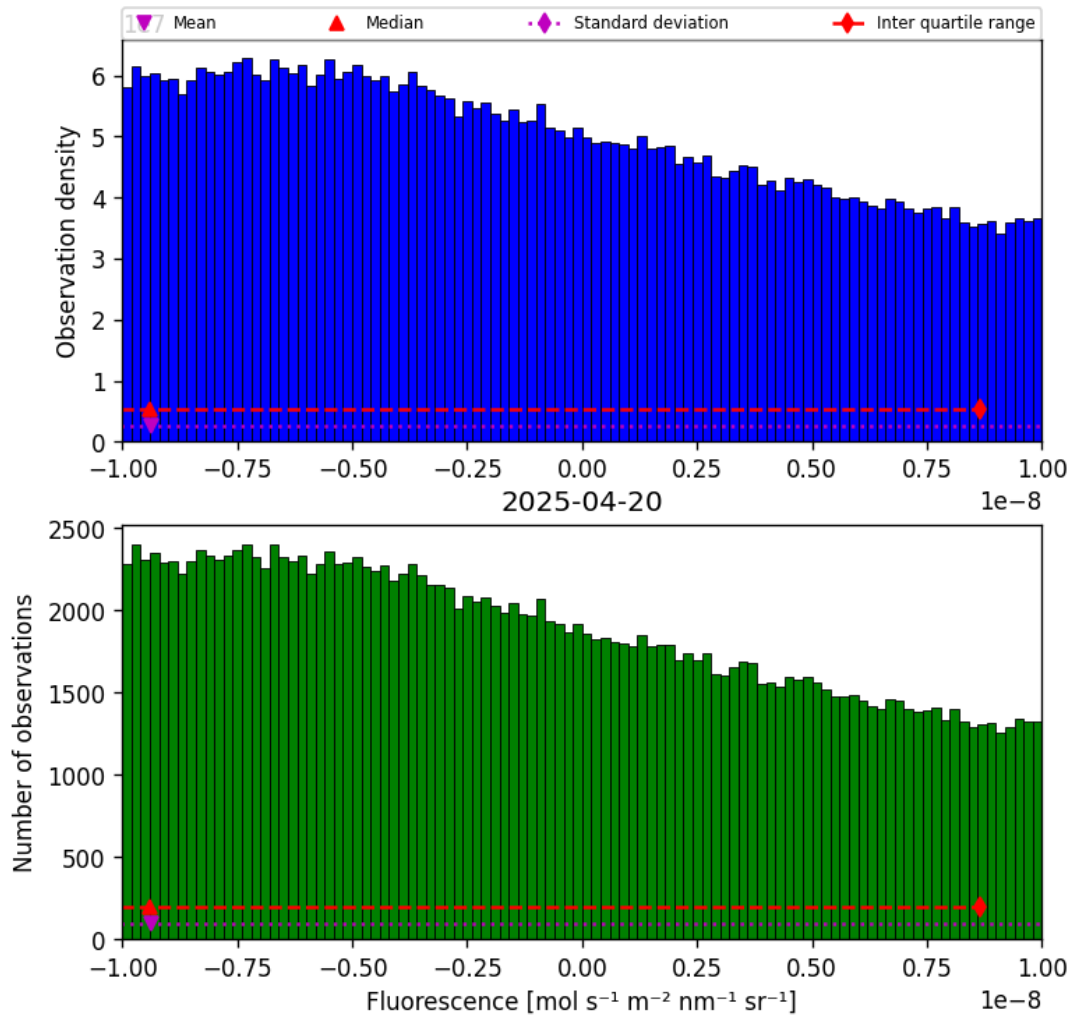
Figure 32: Histogram of “Fluorescence” for 2025-04-19 to 2025-04-21
