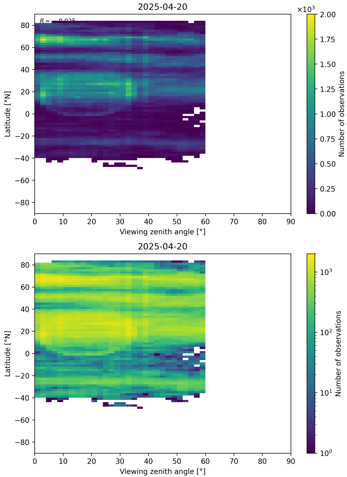
Figure 109: Scatter density plot of “Viewing zenith angle” against “Latitude” for 2025-04-19 to 2025-04-21.
