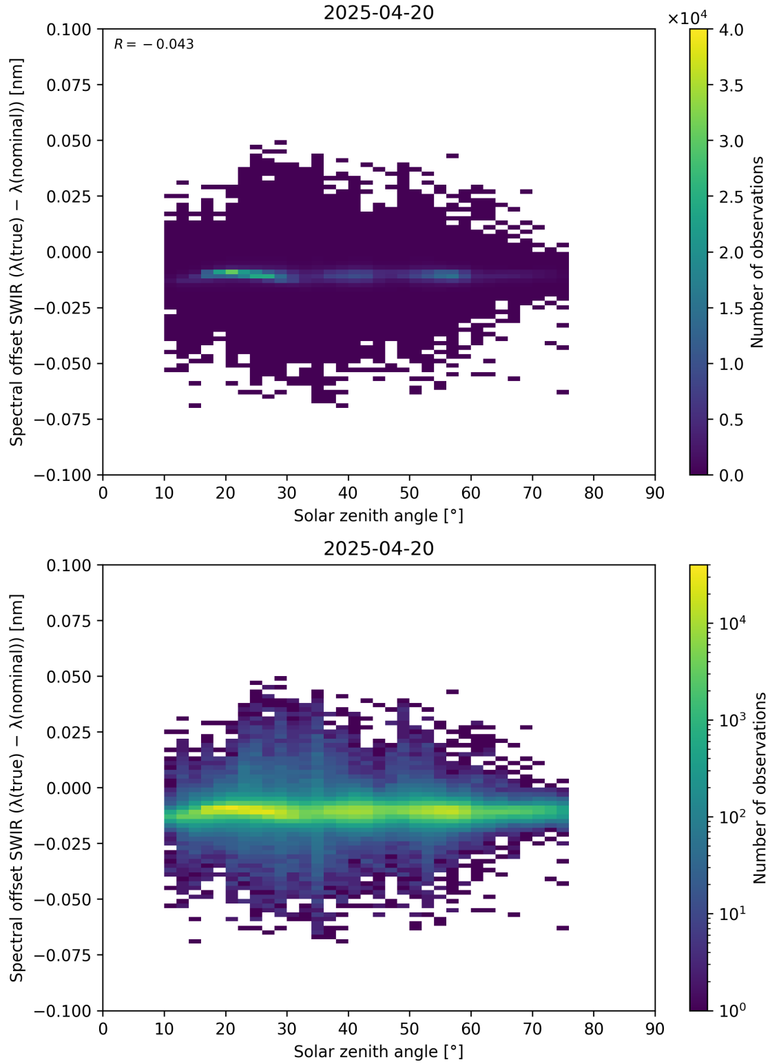
Figure 104: Scatter density plot of “Solar zenith angle” against “Spectral offset SWIR ( \lambda_{\text{true}} - \lambda_{\text{nominal}} )” for 2025-04-19 to 2025-04-21.
