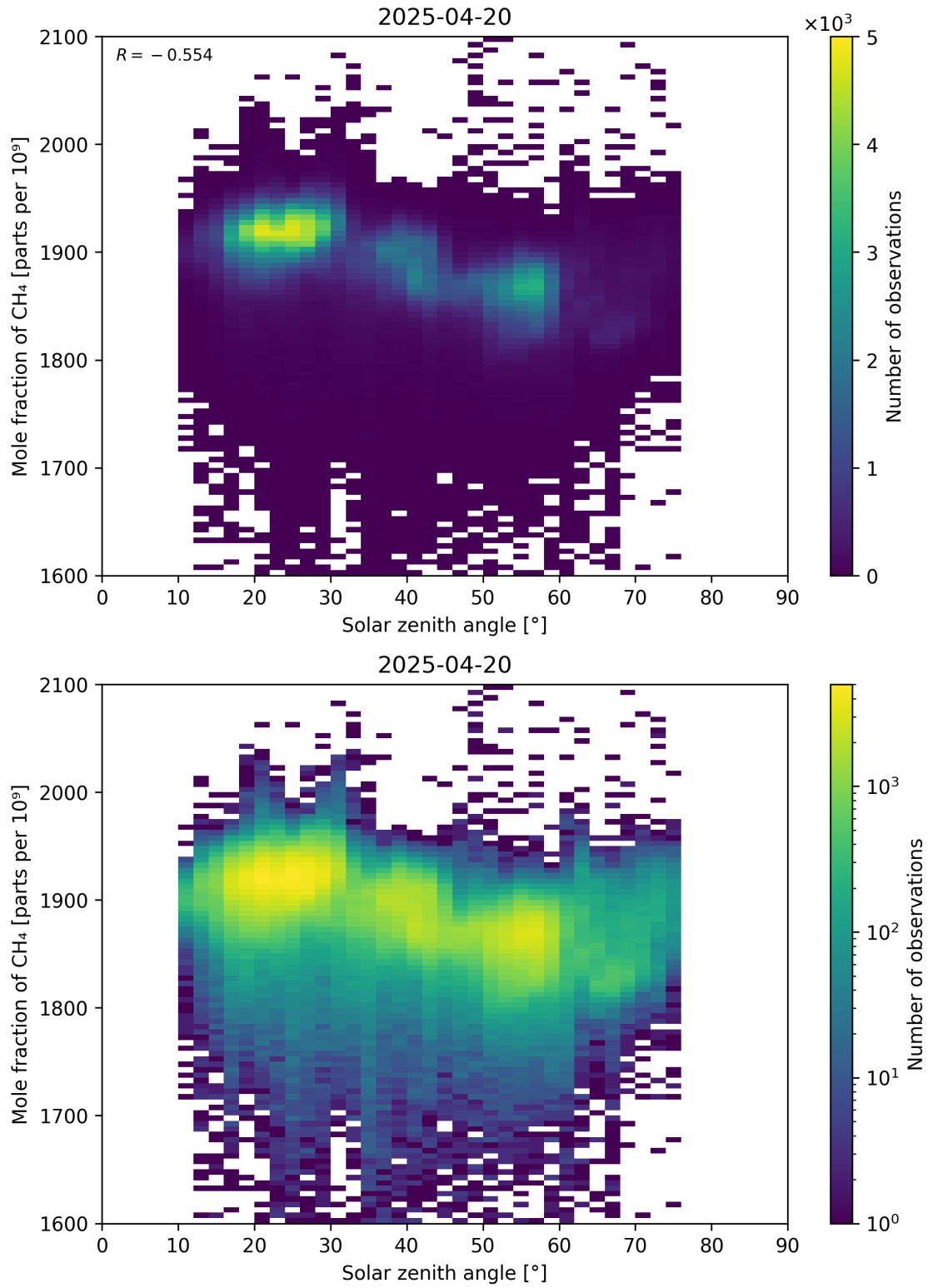
Figure 99: Scatter density plot of “Solar zenith angle” against “Mole fraction of CH 4 ” for 2025-04-19 to 2025-04-21.
