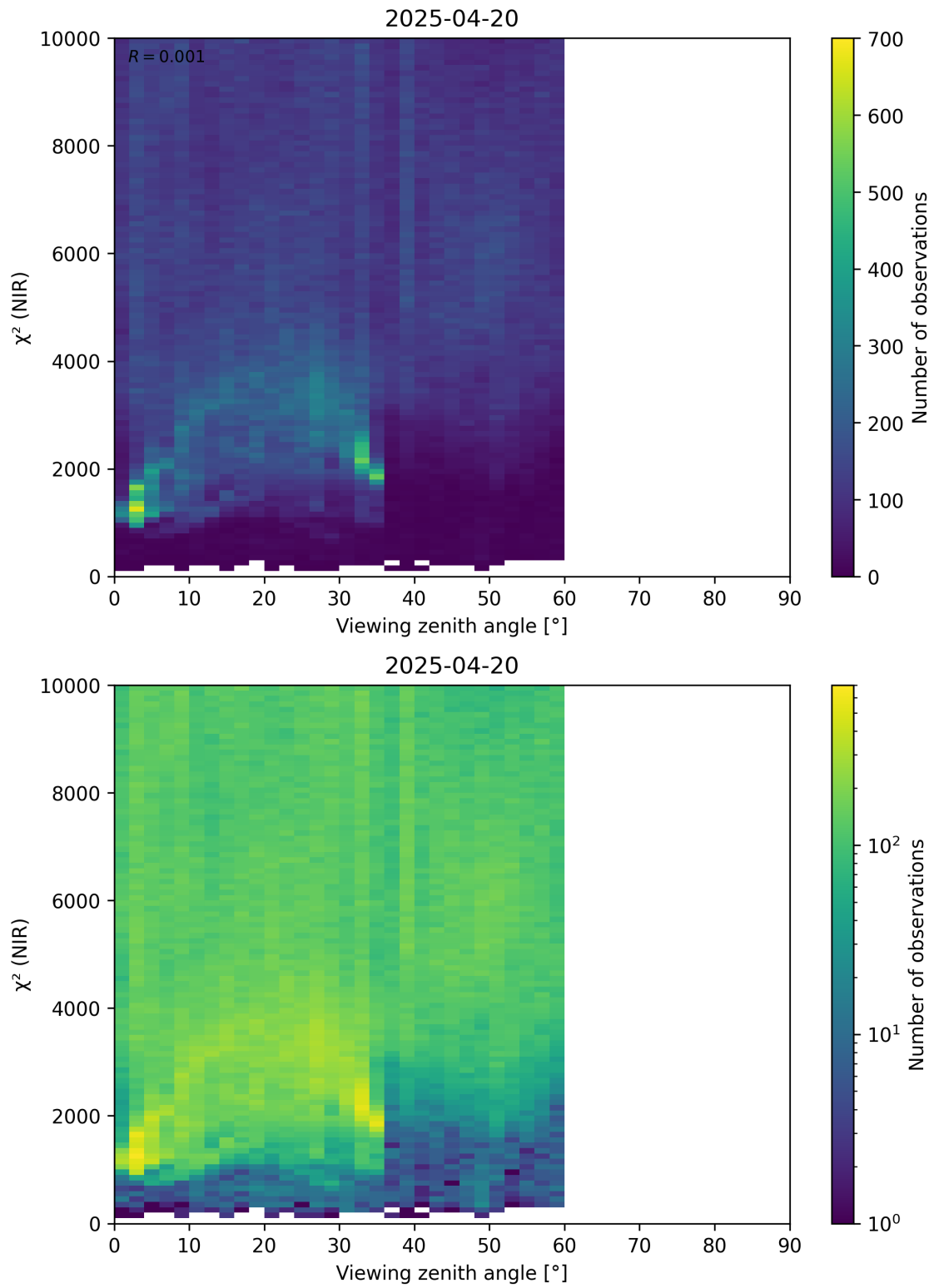
Figure 105: Scatter density plot of “Viewing zenith angle” against “ \chi^2 (NIR)” for 2025-04-19 to 2025-04-21.
