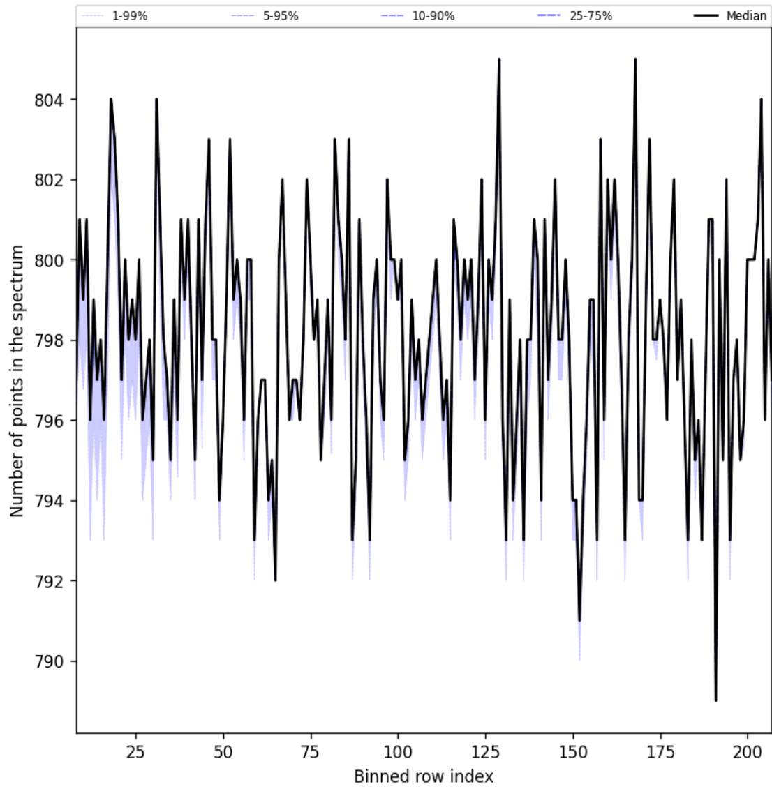
Figure 37: Along track statistics of “Number of points in the spectrum” for 2025-04-19 to 2025-04-21
