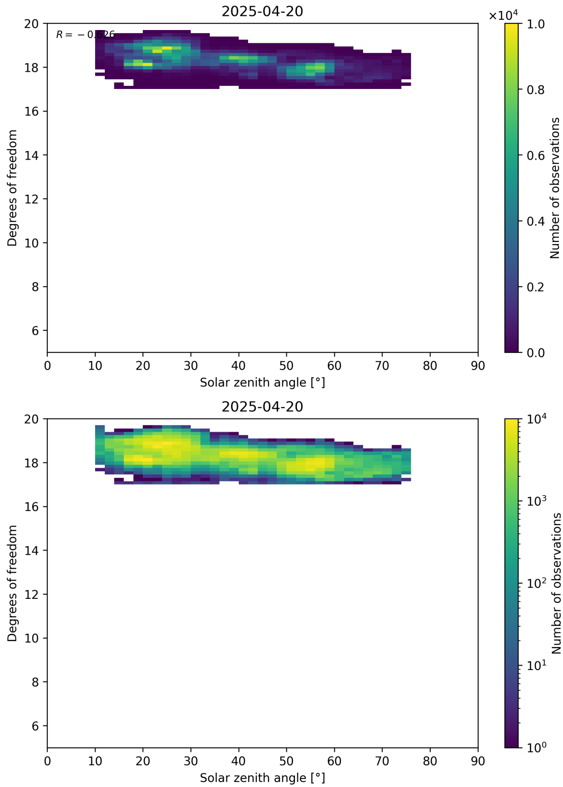
Figure 96: Scatter density plot of “Solar zenith angle” against “Degrees of freedom” for 2025-04-19 to 2025-04-21.
