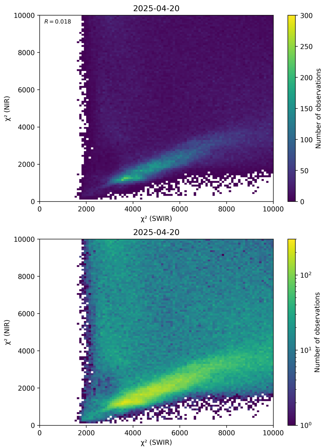
Figure 47: Scatter density plot of “ \chi^2 (SWIR)” against “ \chi^2 (NIR)” for 2025-04-19 to 2025-04-21.
