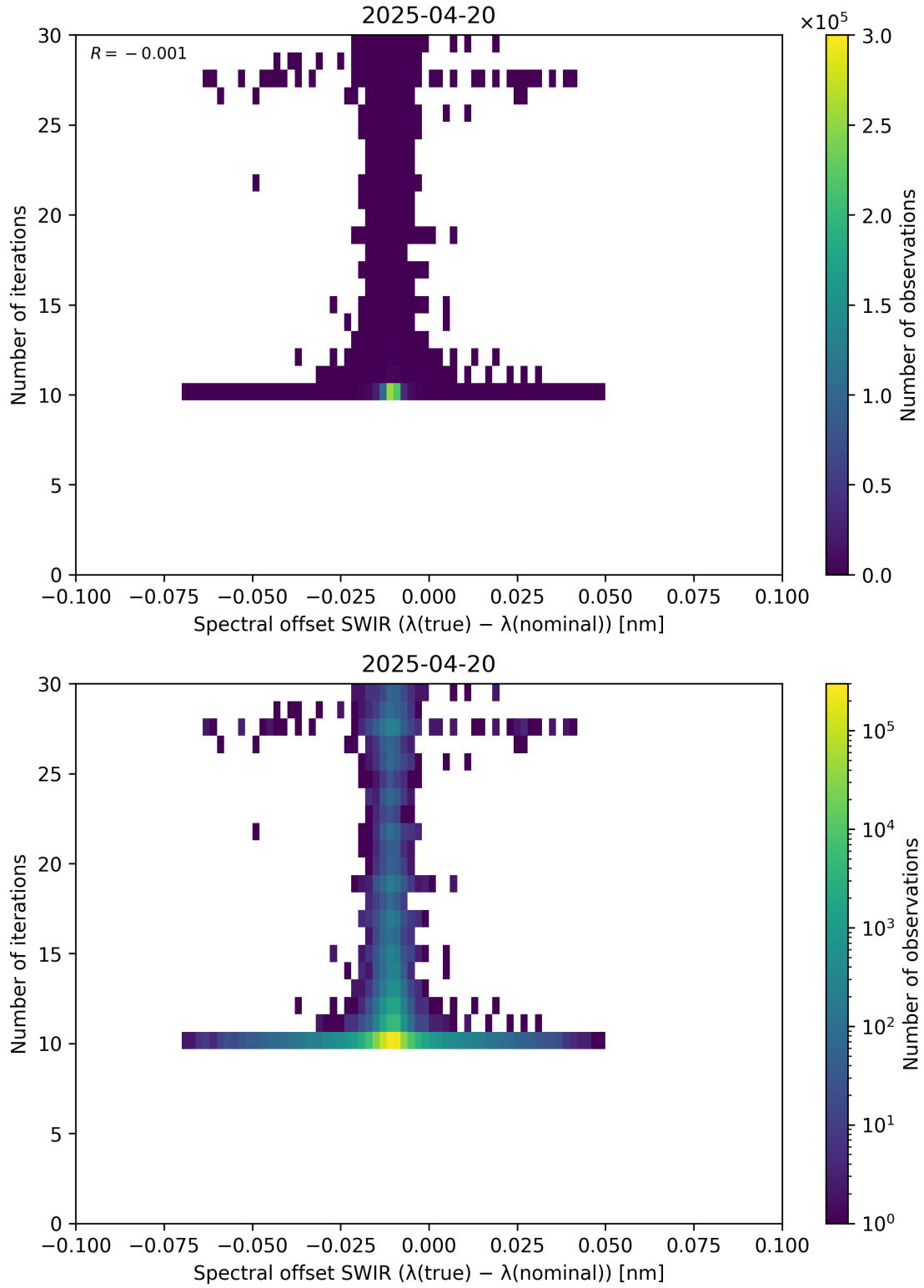
Figure 121: Scatter density plot of “Spectral offset SWIR ( \lambda_{\text{true}} - \lambda_{\text{nominal}} )” against “Number of iterations” for 2025-04-19 to 2025-04-21.
