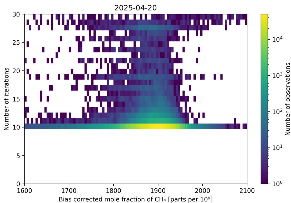
Figure 67: Scatter density plot of “Bias corrected mole fraction of \text{CH}_4 ” against “Number of iterations” for 2025-04-19 to 2025-04-21.
