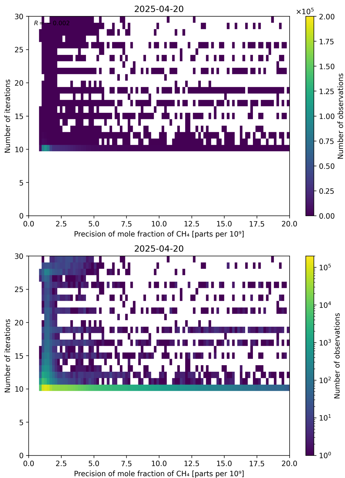
Figure 83: Scatter density plot of “Precision of mole fraction of CH 4 ” against “Number of iterations” for 2025-04-19 to 2025-04-21.
