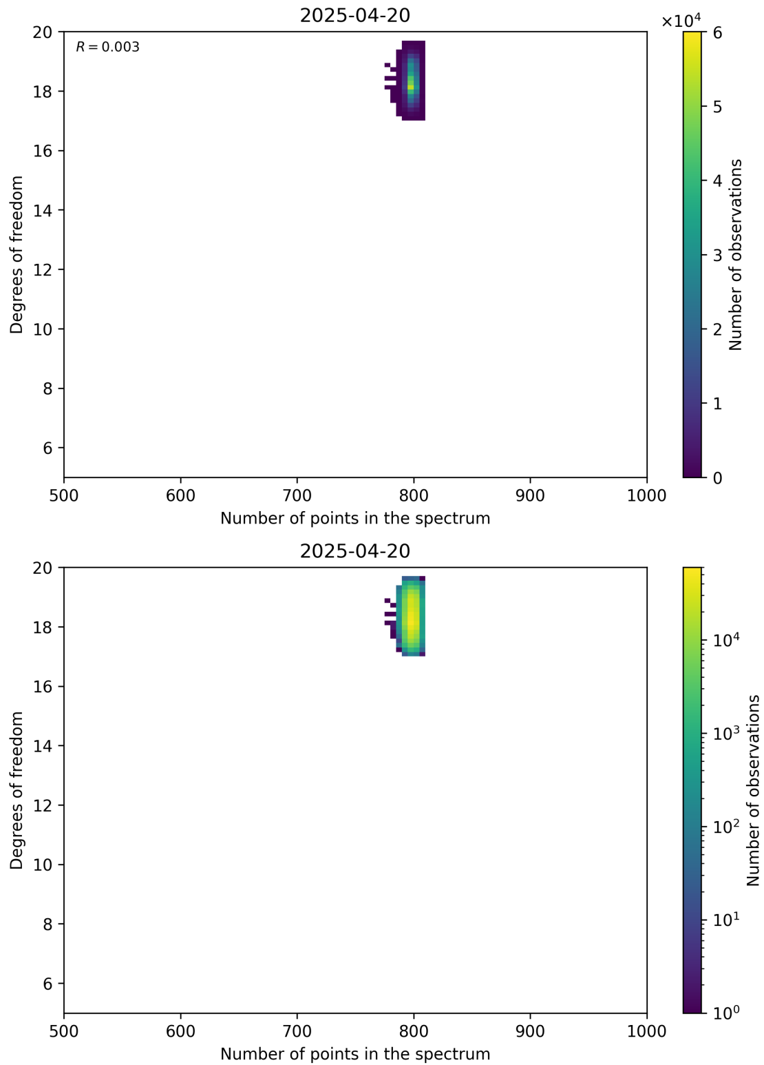
Figure 90: Scatter density plot of “Number of points in the spectrum” against “Degrees of freedom” for 2025-04-19 to 2025-04-21.
