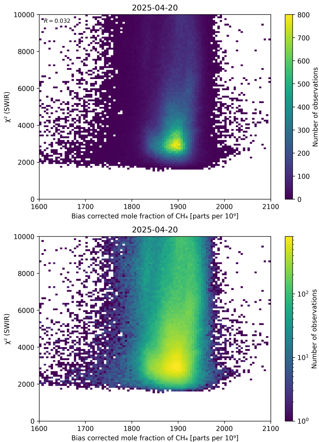
Figure 64: Scatter density plot of “Bias corrected mole fraction of CH 4 ” against “ \chi^2 (SWIR)” for 2025-04-19 to 2025-04-21.
