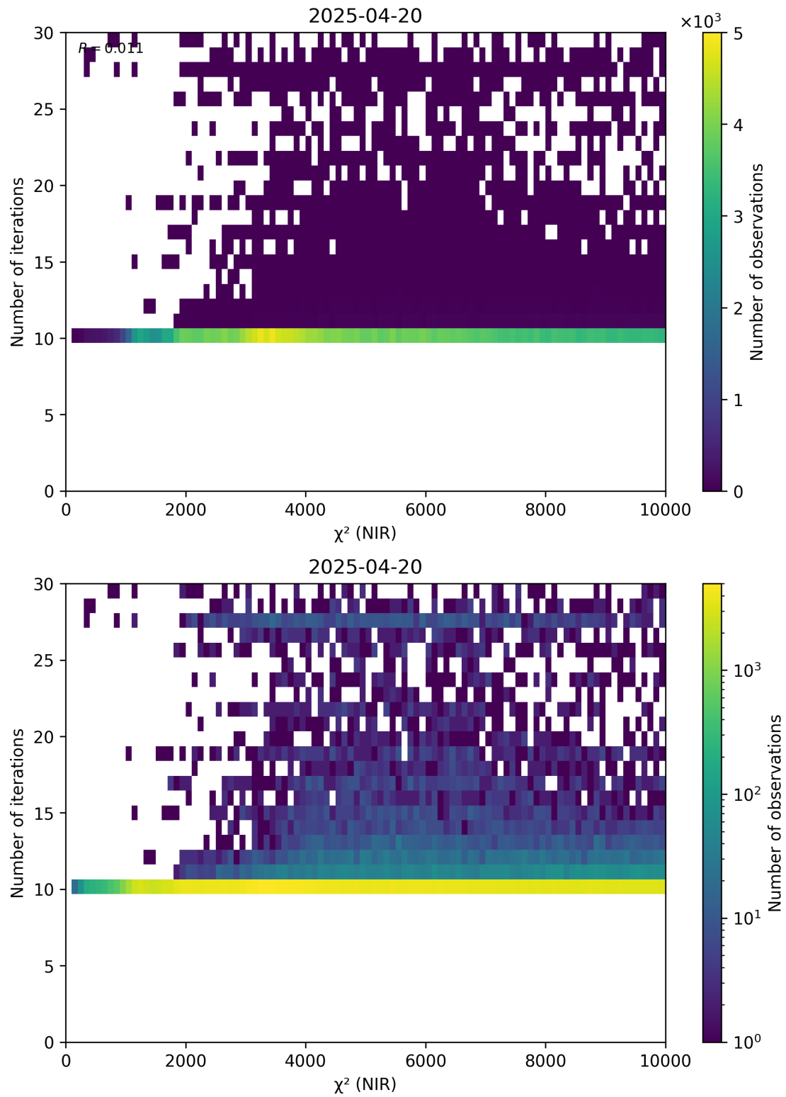
Figure 46: Scatter density plot of “ \chi^2 (NIR)” against “Number of iterations” for 2025-04-19 to 2025-04-21.
