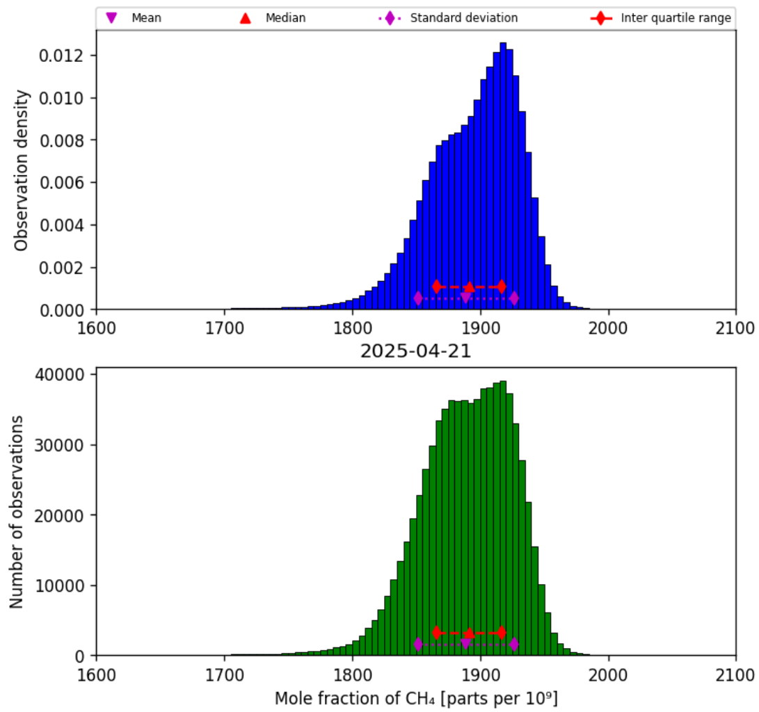
Figure 23: Histogram of “Mole fraction of CH 4 ” for 2025-04-20 to 2025-04-22
