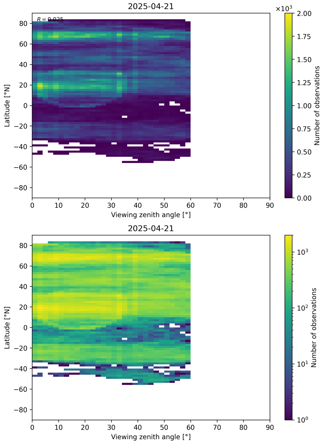
Figure 109: Scatter density plot of “Viewing zenith angle” against “Latitude” for 2025-04-20 to 2025-04-22.
