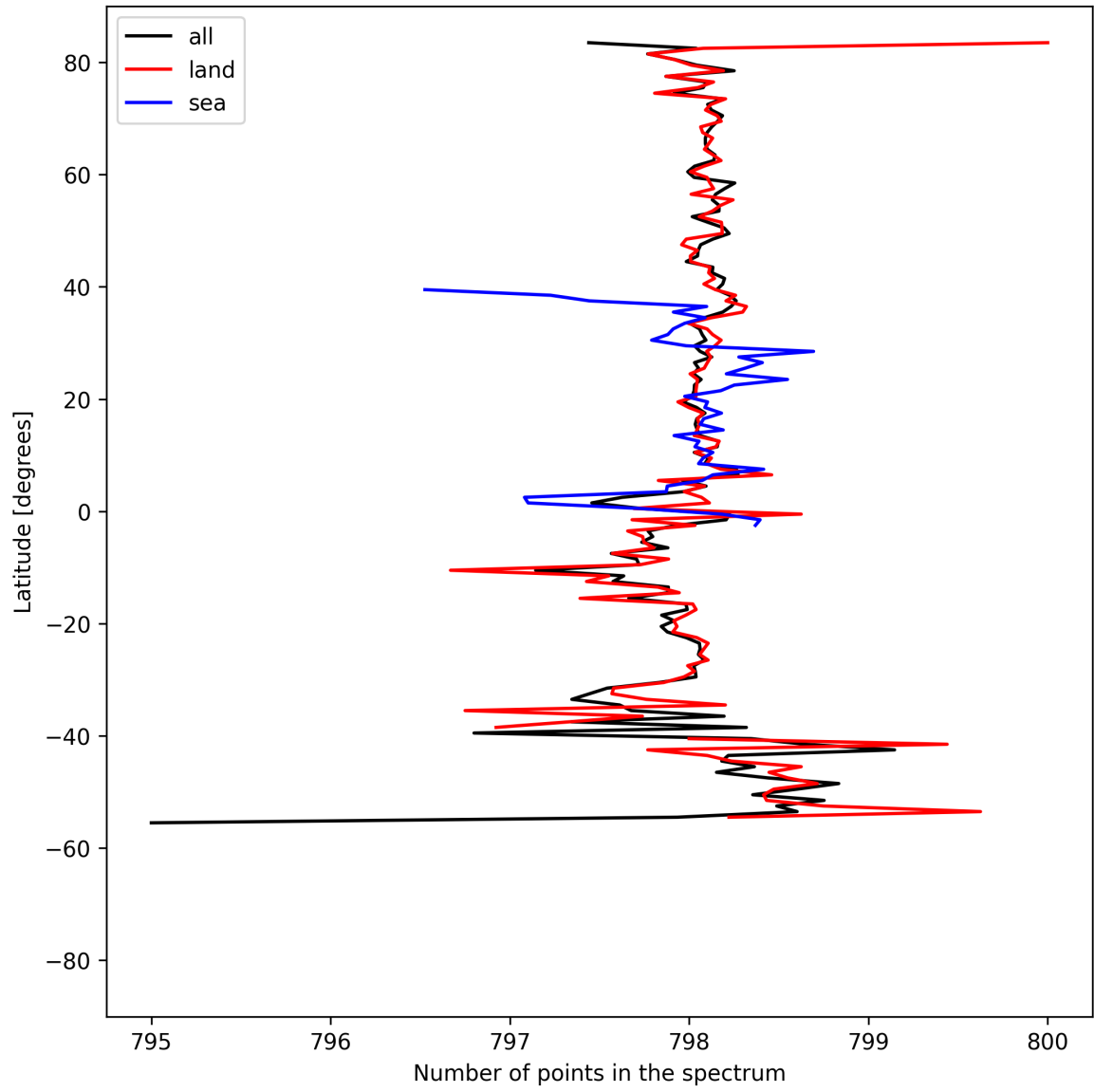
Figure 15: Zonal average of “Number of points in the spectrum” for 2025-04-20 to 2025-04-22.
