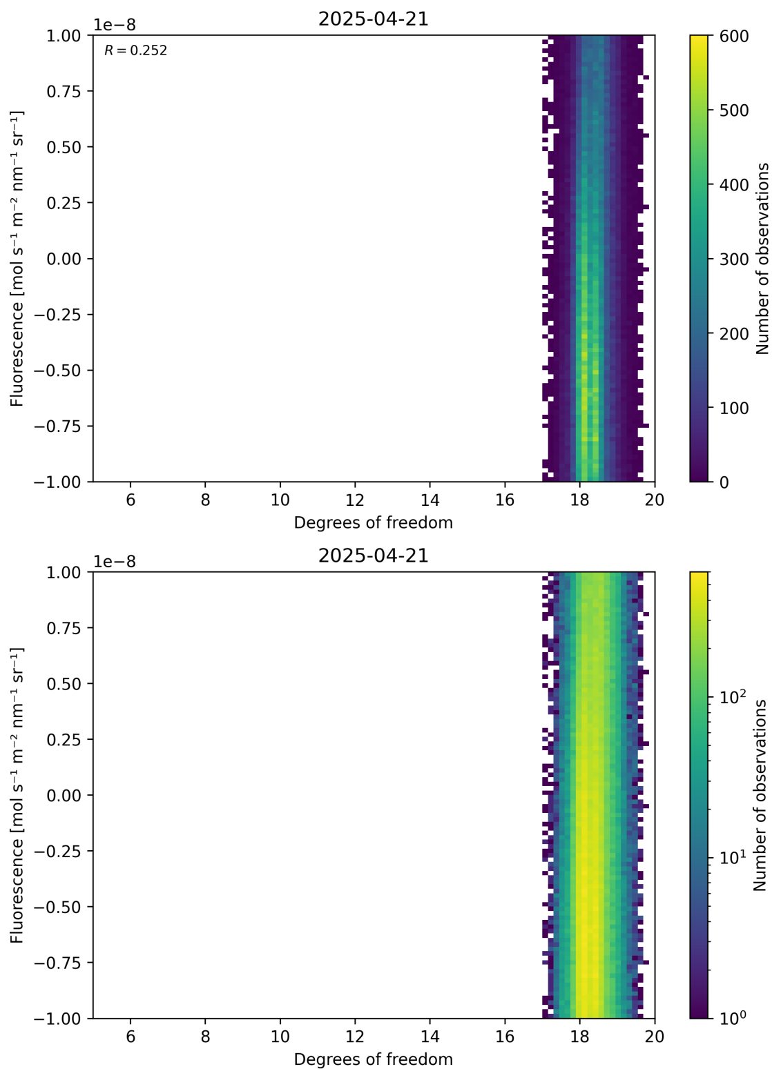
Figure 51: Scatter density plot of “Degrees of freedom” against “Fluorescence” for 2025-04-20 to 2025-04-22.
