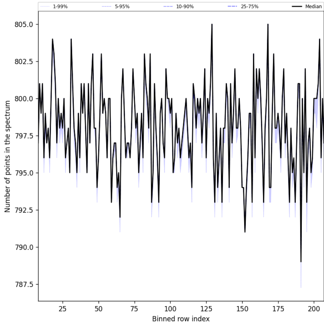
Figure 37: Along track statistics of “Number of points in the spectrum” for 2025-04-20 to 2025-04-22
