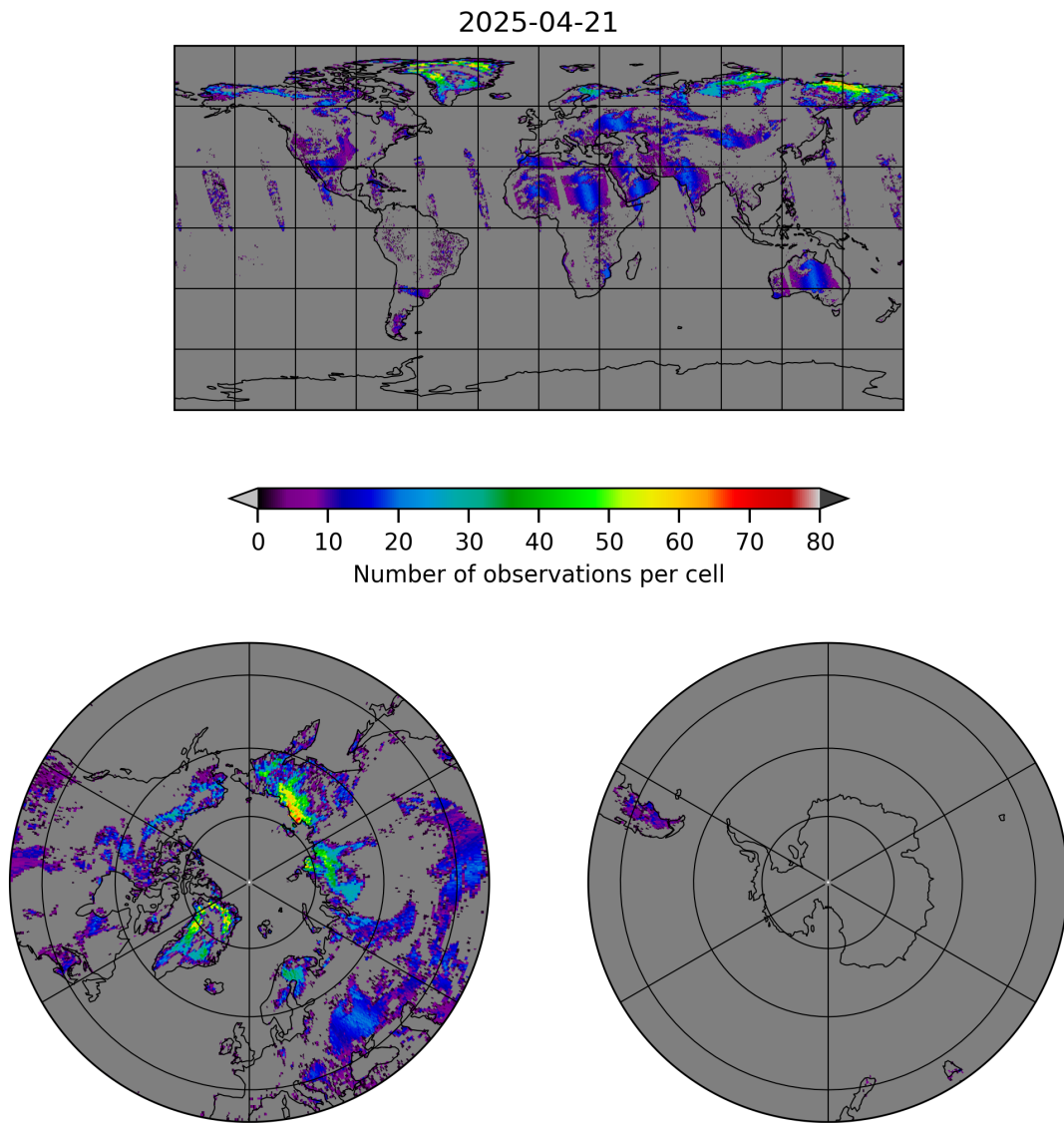
Figure 10: Map of the number of observations for 2025-04-20 to 2025-04-22
