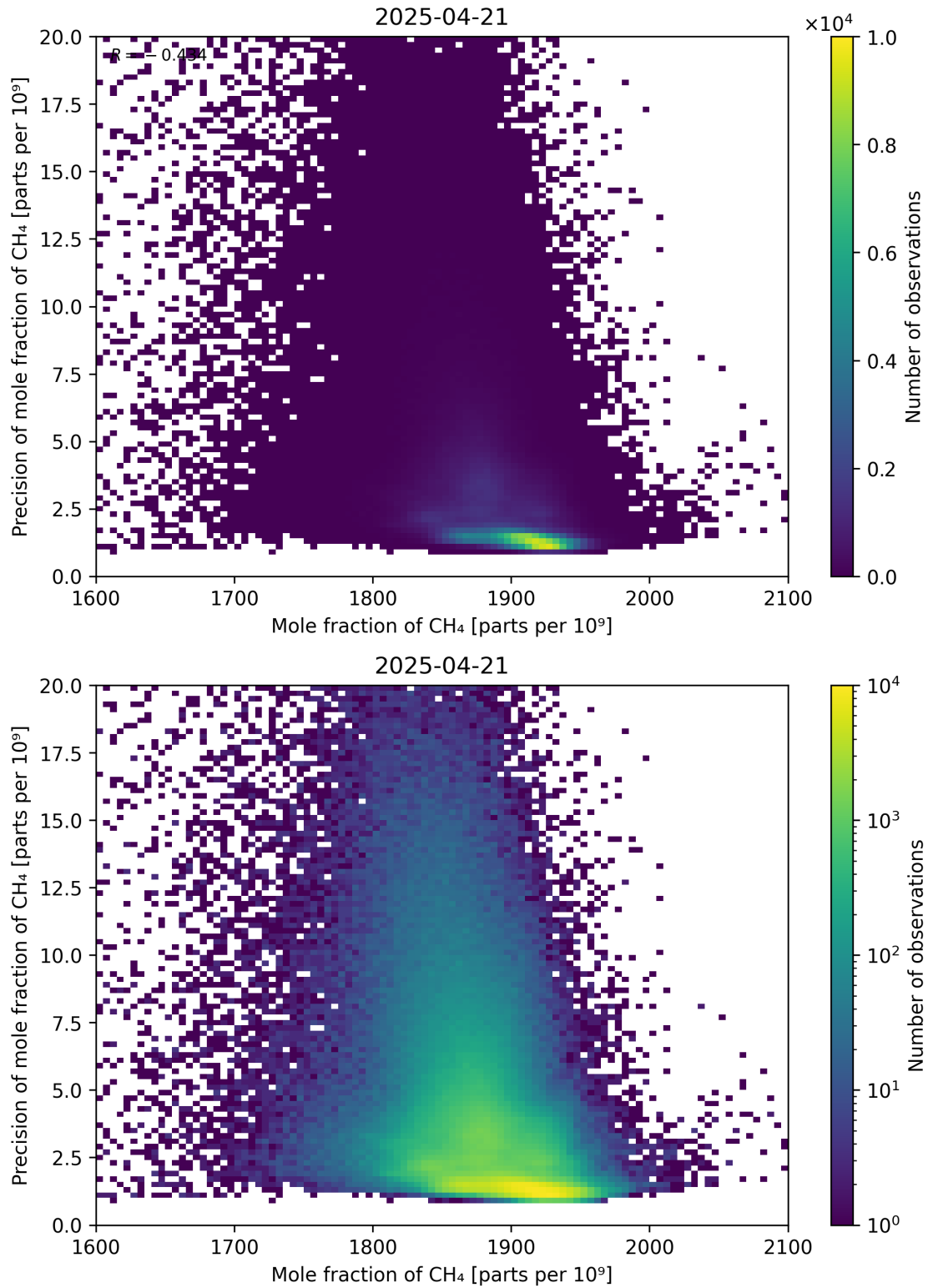
Figure 75: Scatter density plot of “Mole fraction of CH 4 ” against “Precision of mole fraction of CH 4 ” for 2025-04-20 to 2025-04-22.
