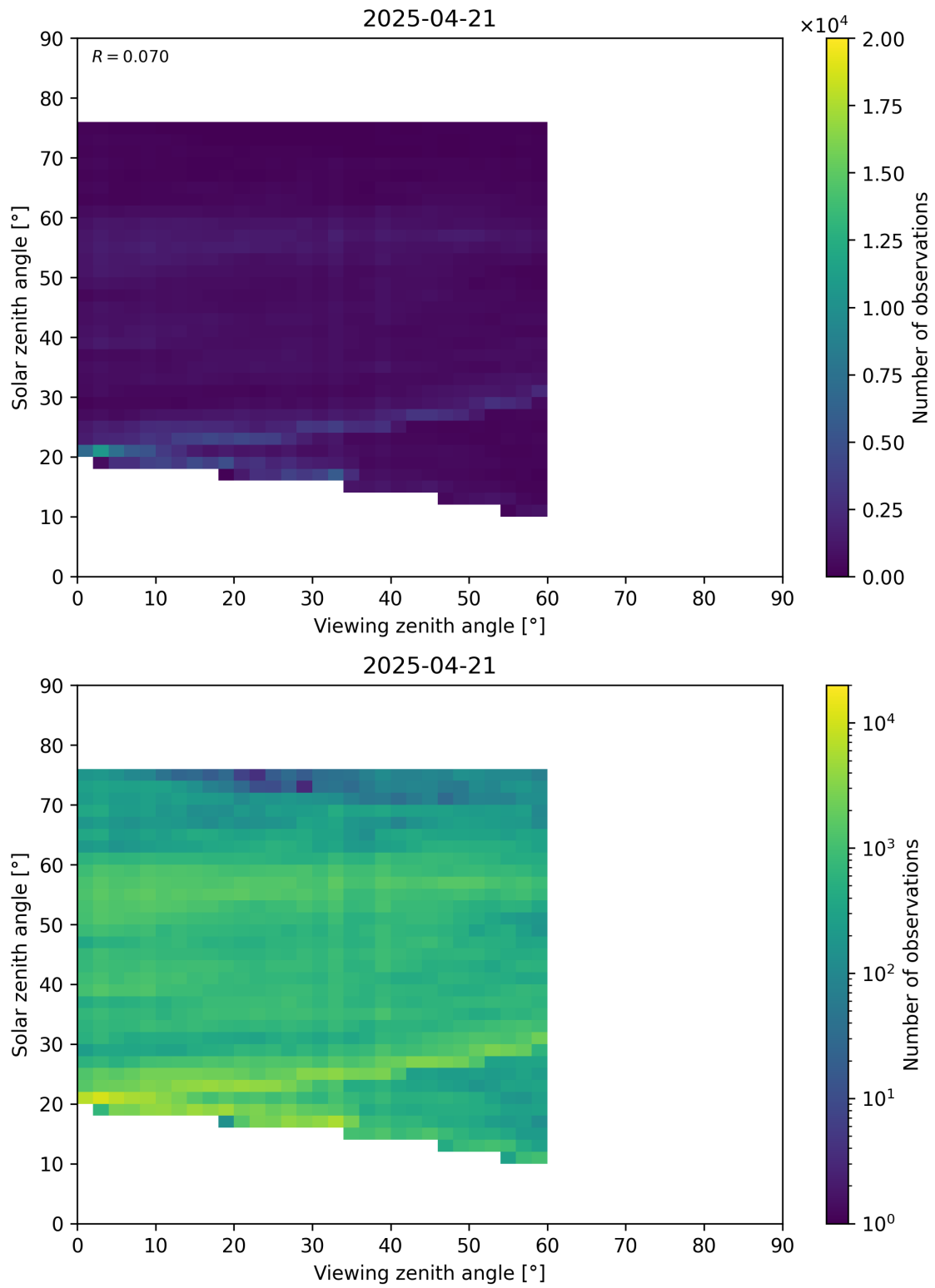
Figure 115: Scatter density plot of “Viewing zenith angle” against “Solar zenith angle” for 2025-04-20 to 2025-04-22.
