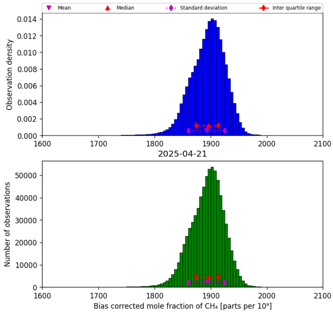
Figure 25: Histogram of “Bias corrected mole fraction of CH 4 ” for 2025-04-20 to 2025-04-22
