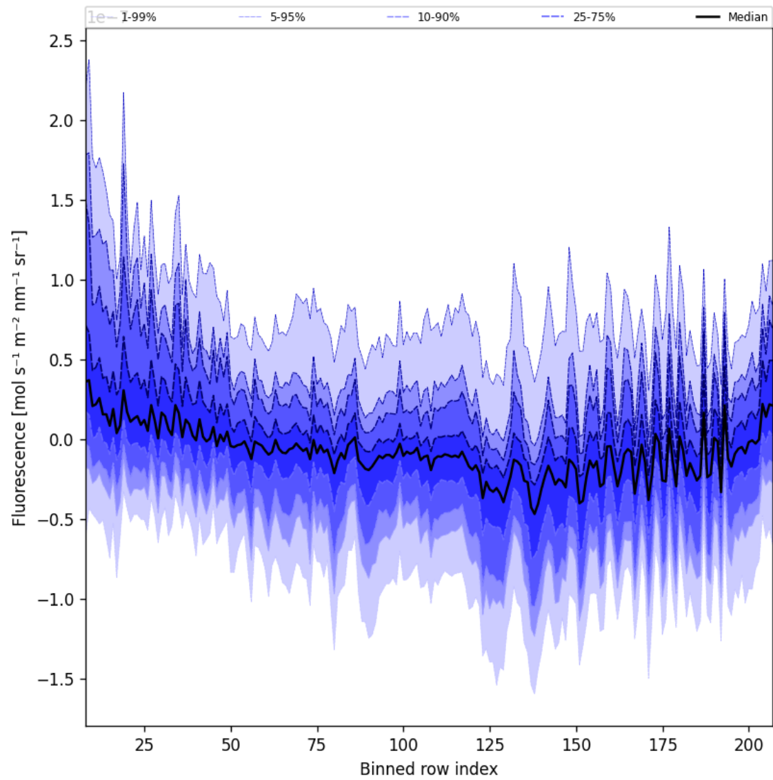
Figure 43: Along track statistics of “Fluorescence” for 2025-04-20 to 2025-04-22
