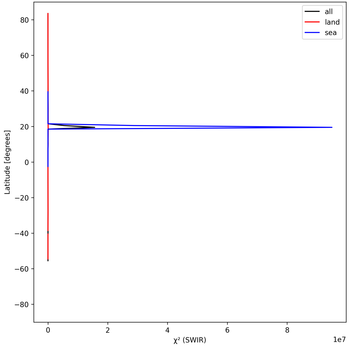
Figure 17: Zonal average of “ \chi^2 (SWIR)” for 2025-04-20 to 2025-04-22.
