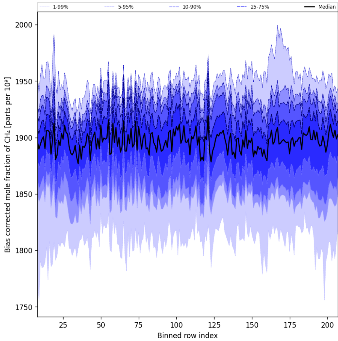
Figure 36: Along track statistics of “Bias corrected mole fraction of CH 4 ” for 2025-04-20 to 2025-04-22
