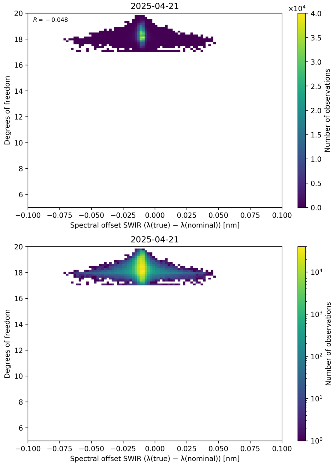
Figure 119: Scatter density plot of “Spectral offset SWIR ( \lambda_{\text{true}} - \lambda_{\text{nominal}} )” against “Degrees of freedom” for 2025-04-20 to 2025-04-22.
