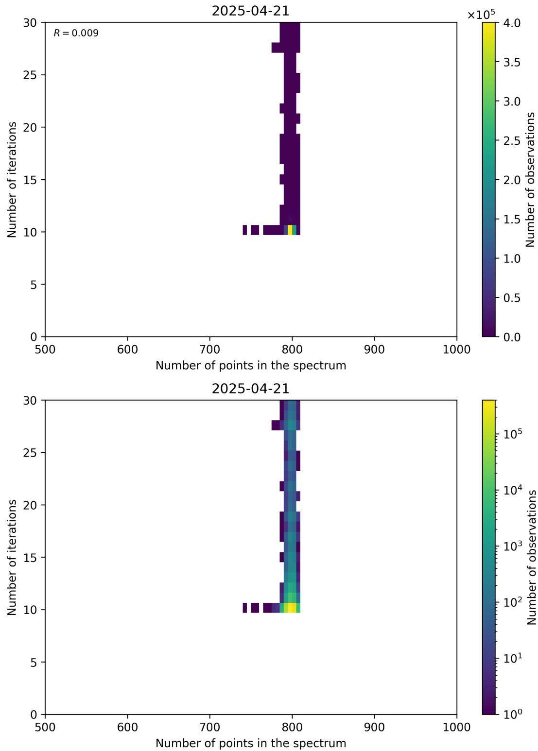
Figure 92: Scatter density plot of “Number of points in the spectrum” against “Number of iterations” for 2025-04-20 to 2025-04-22.
