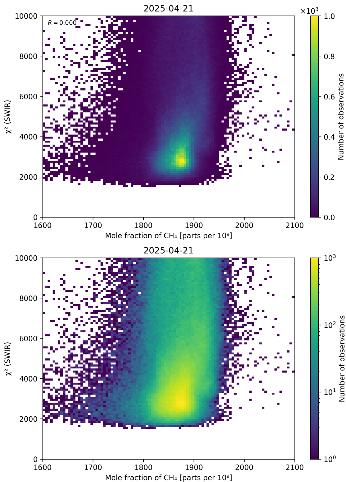
Figure 71: Scatter density plot of “Mole fraction of \text{CH}_4 ” against “ \chi^2 (SWIR)” for 2025-04-20 to 2025-04-22.
