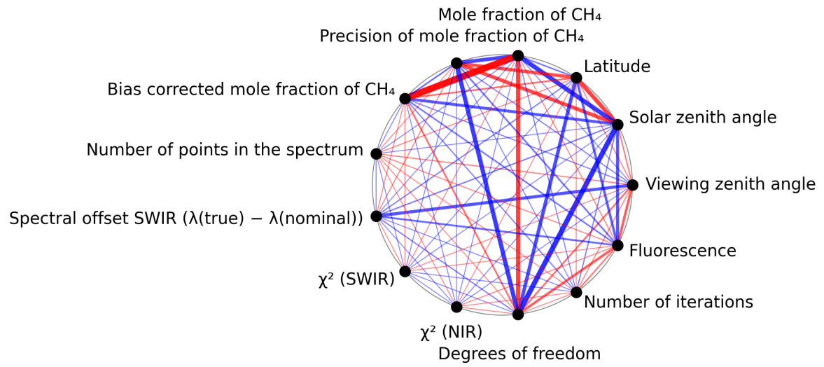
Figure 1: Map of correlation graph for 2025-04-20 to 2025-04-22.
