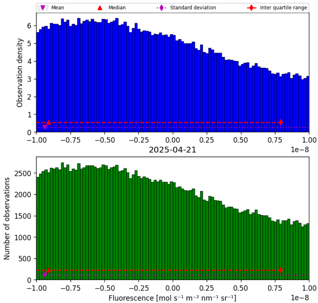
Figure 32: Histogram of “Fluorescence” for 2025-04-20 to 2025-04-22
