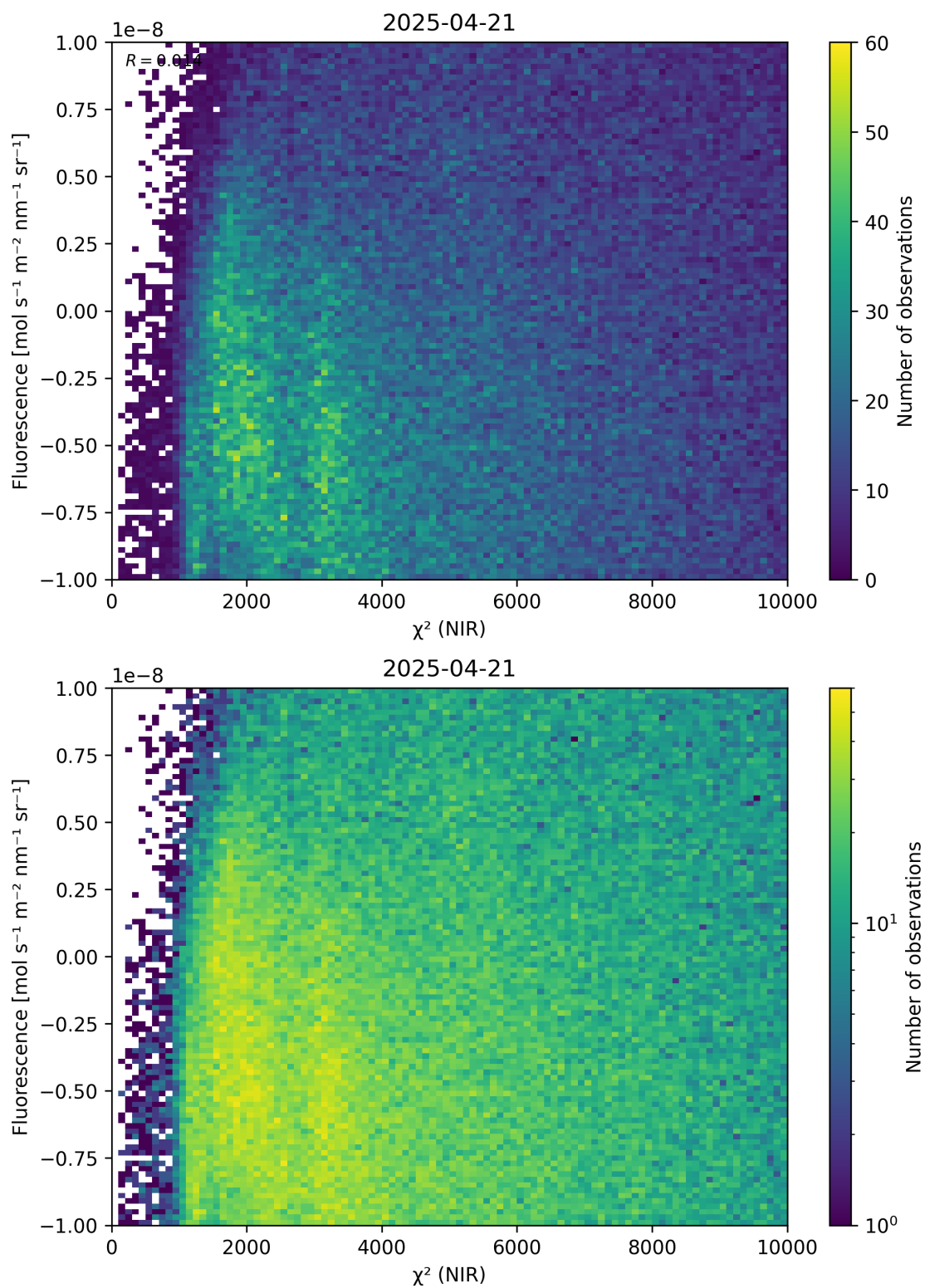
Figure 45: Scatter density plot of “ \chi^2 (NIR)” against “Fluorescence” for 2025-04-20 to 2025-04-22.
