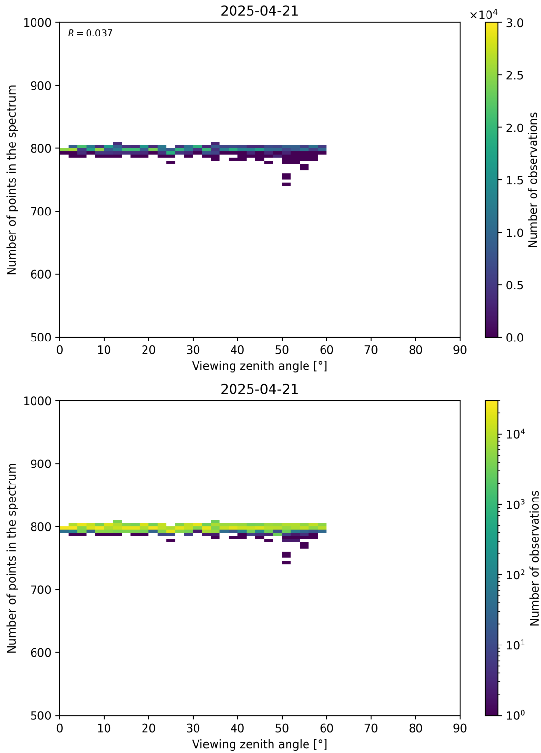
Figure 114: Scatter density plot of “Viewing zenith angle” against “Number of points in the spectrum” for 2025-04-20 to 2025-04-22.
