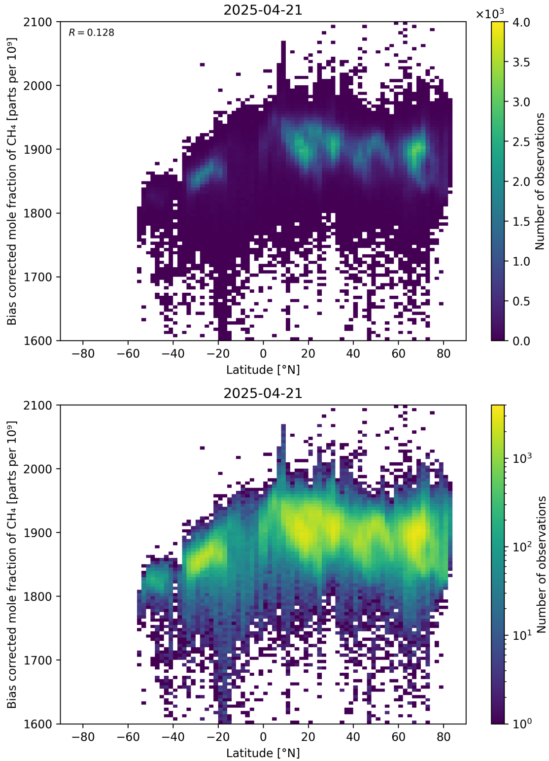
Figure 58: Scatter density plot of “Latitude” against “Bias corrected mole fraction of \text{CH}_4 ” for 2025-04-20 to 2025-04-22.
