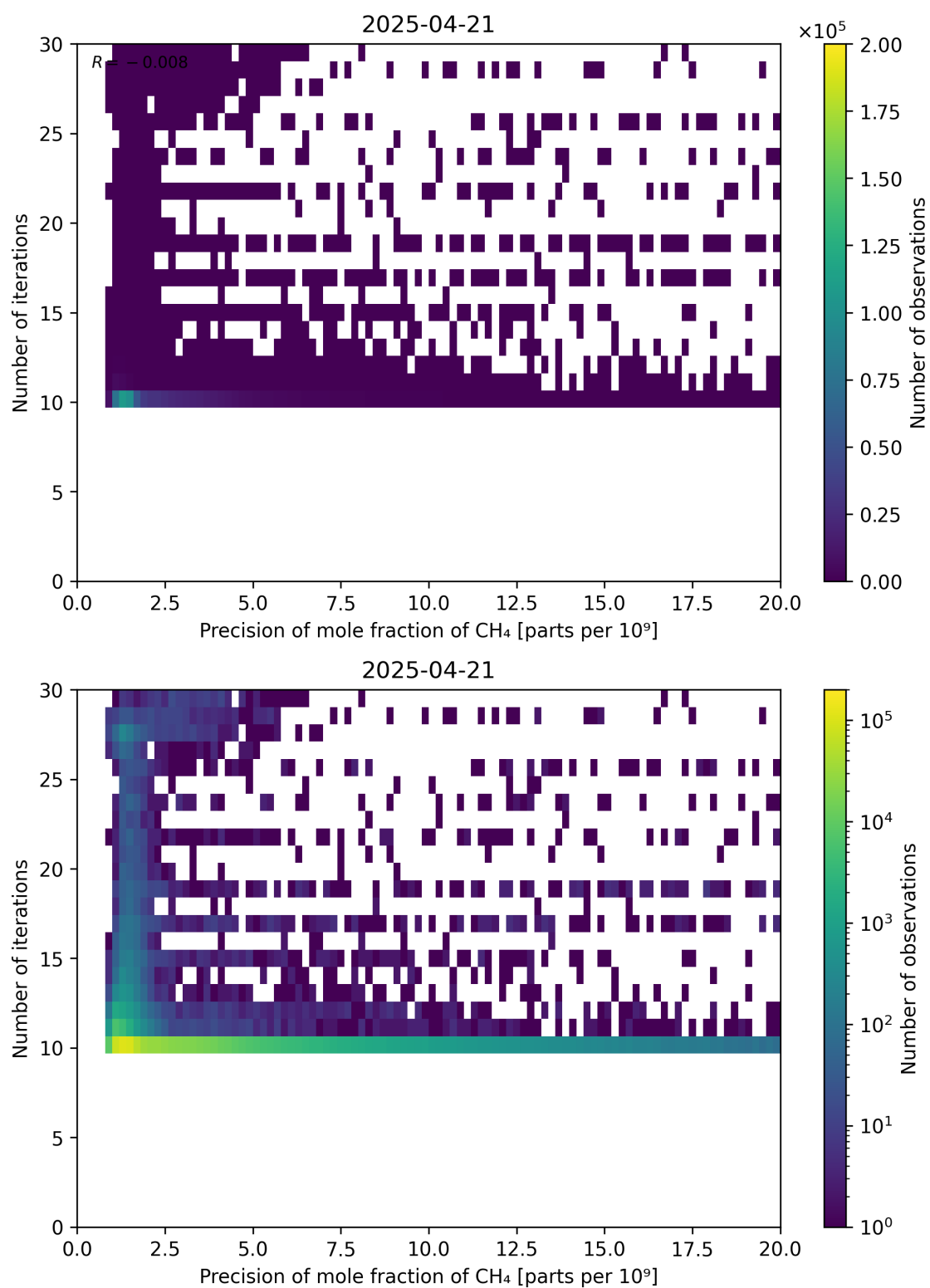
Figure 83: Scatter density plot of “Precision of mole fraction of CH 4 ” against “Number of iterations” for 2025-04-20 to 2025-04-22.
