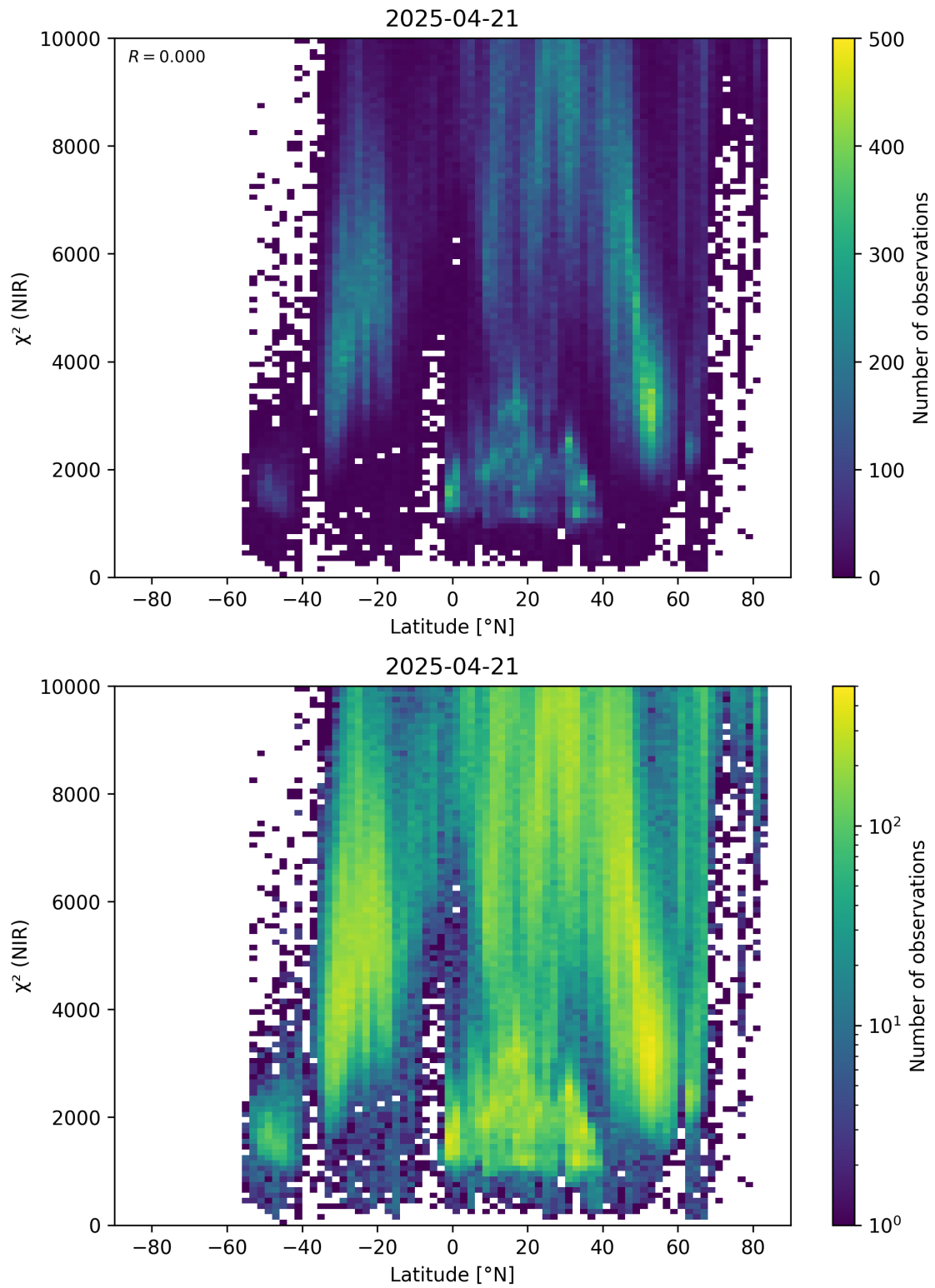
Figure 53: Scatter density plot of “Latitude” against “ \chi^2 (NIR)” for 2025-04-20 to 2025-04-22.
