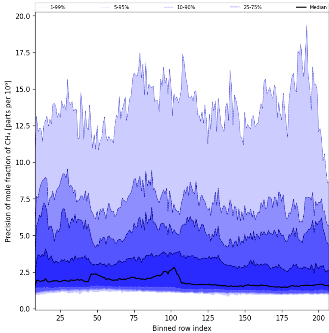
Figure 35: Along track statistics of “Precision of mole fraction of CH 4 ” for 2025-04-20 to 2025-04-22
