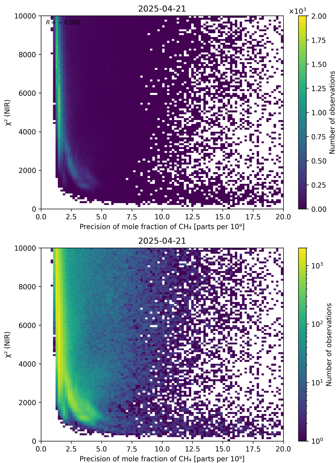
Figure 78: Scatter density plot of “Precision of mole fraction of CH 4 ” against “ \chi^2 (NIR)” for 2025-04-20 to 2025-04-22.
