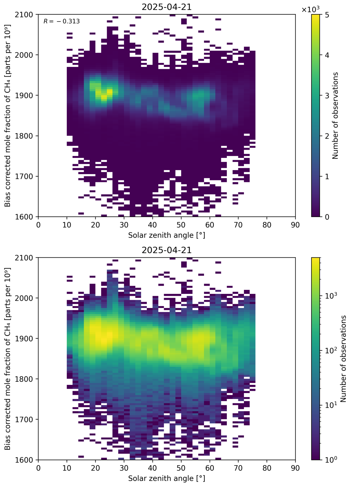
Figure 100: Scatter density plot of “Solar zenith angle” against “Bias corrected mole fraction of \text{CH}_4 ” for 2025-04-20 to 2025-04-22.
