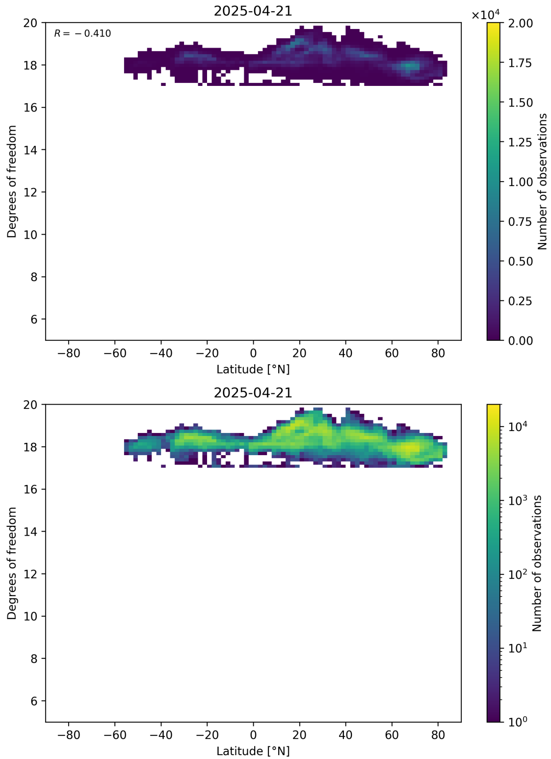
Figure 55: Scatter density plot of “Latitude” against “Degrees of freedom” for 2025-04-20 to 2025-04-22.
