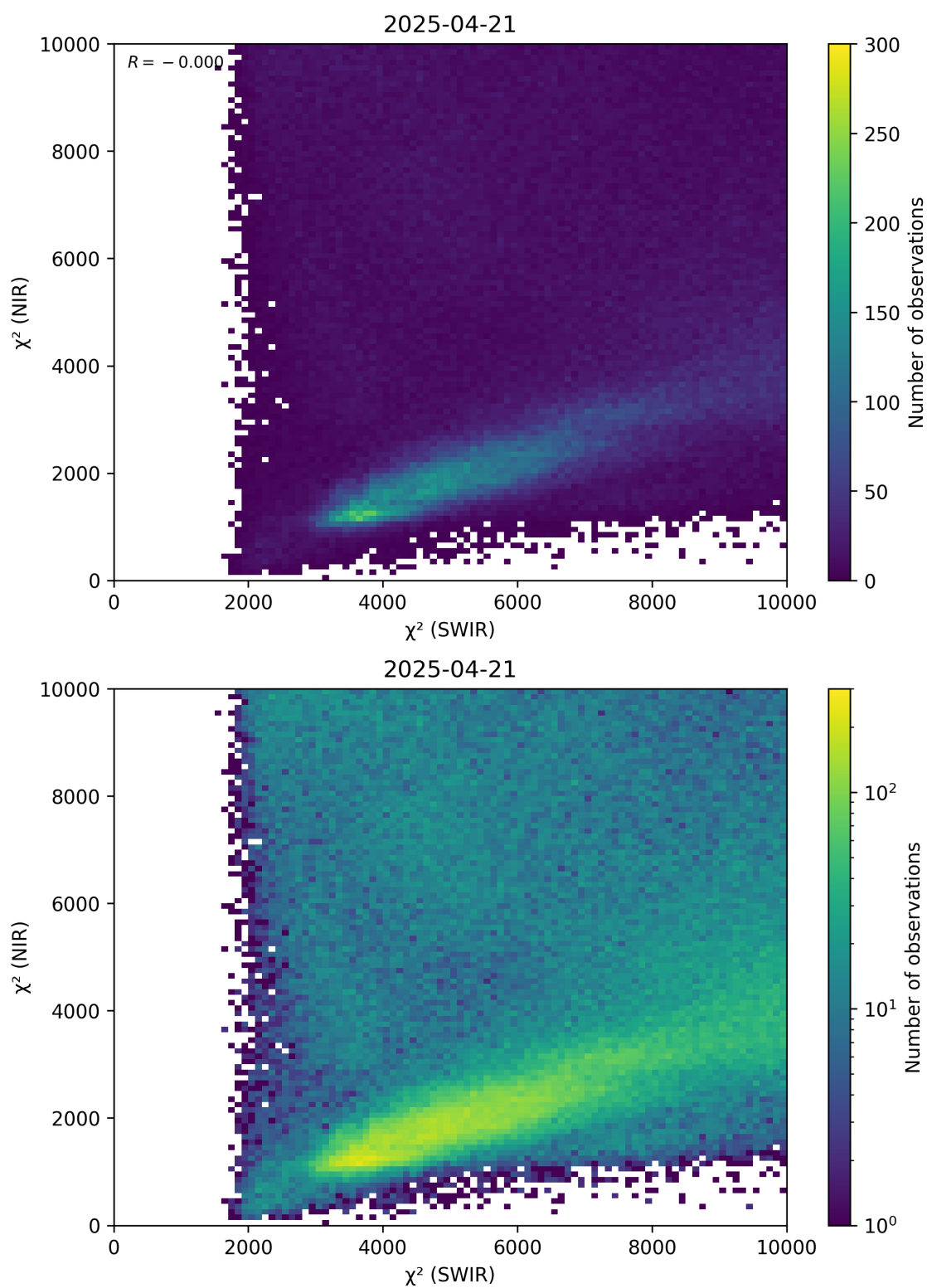
Figure 47: Scatter density plot of “ \chi^2 (SWIR)” against “ \chi^2 (NIR)” for 2025-04-20 to 2025-04-22.
