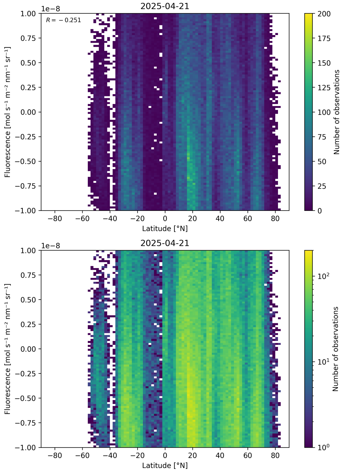
Figure 56: Scatter density plot of “Latitude” against “Fluorescence” for 2025-04-20 to 2025-04-22.
