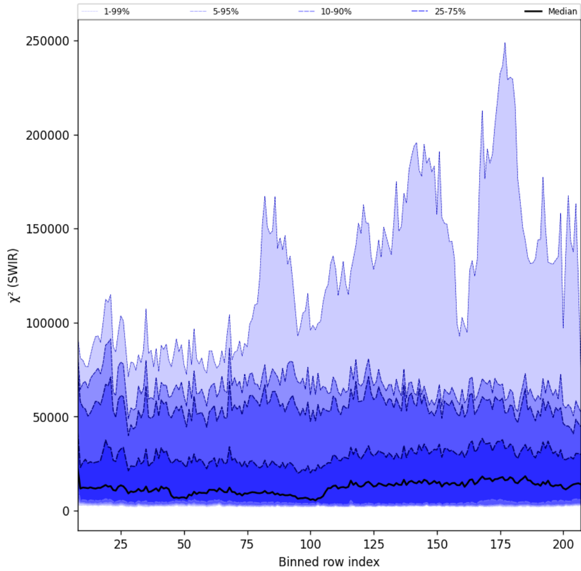
Figure 39: Along track statistics of " \chi^2 (SWIR)" for 2025-04-20 to 2025-04-22
