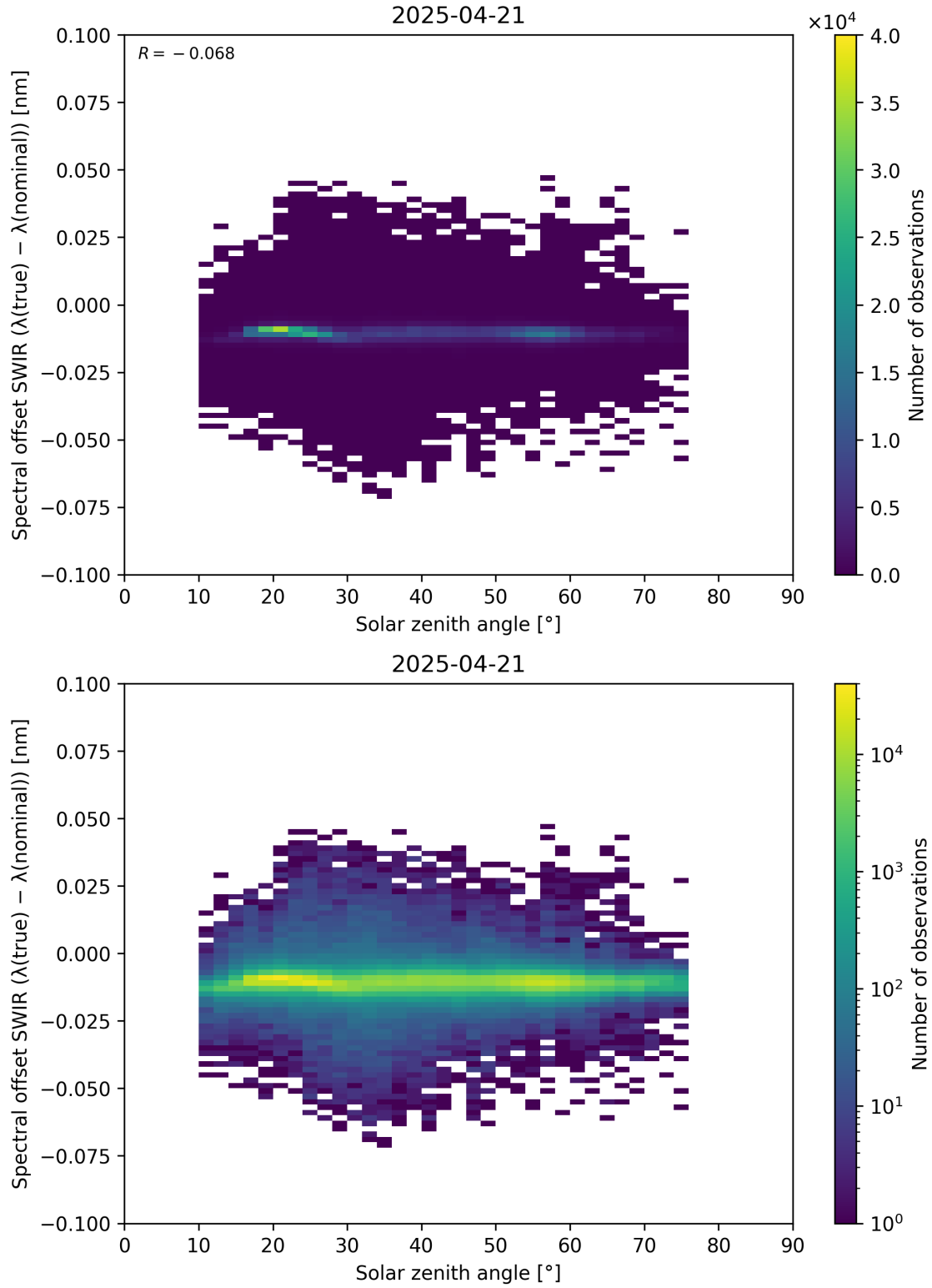
Figure 104: Scatter density plot of “Solar zenith angle” against “Spectral offset SWIR ( \lambda_{\text{true}} - \lambda_{\text{nominal}} )” for 2025-04-20 to 2025-04-22.
