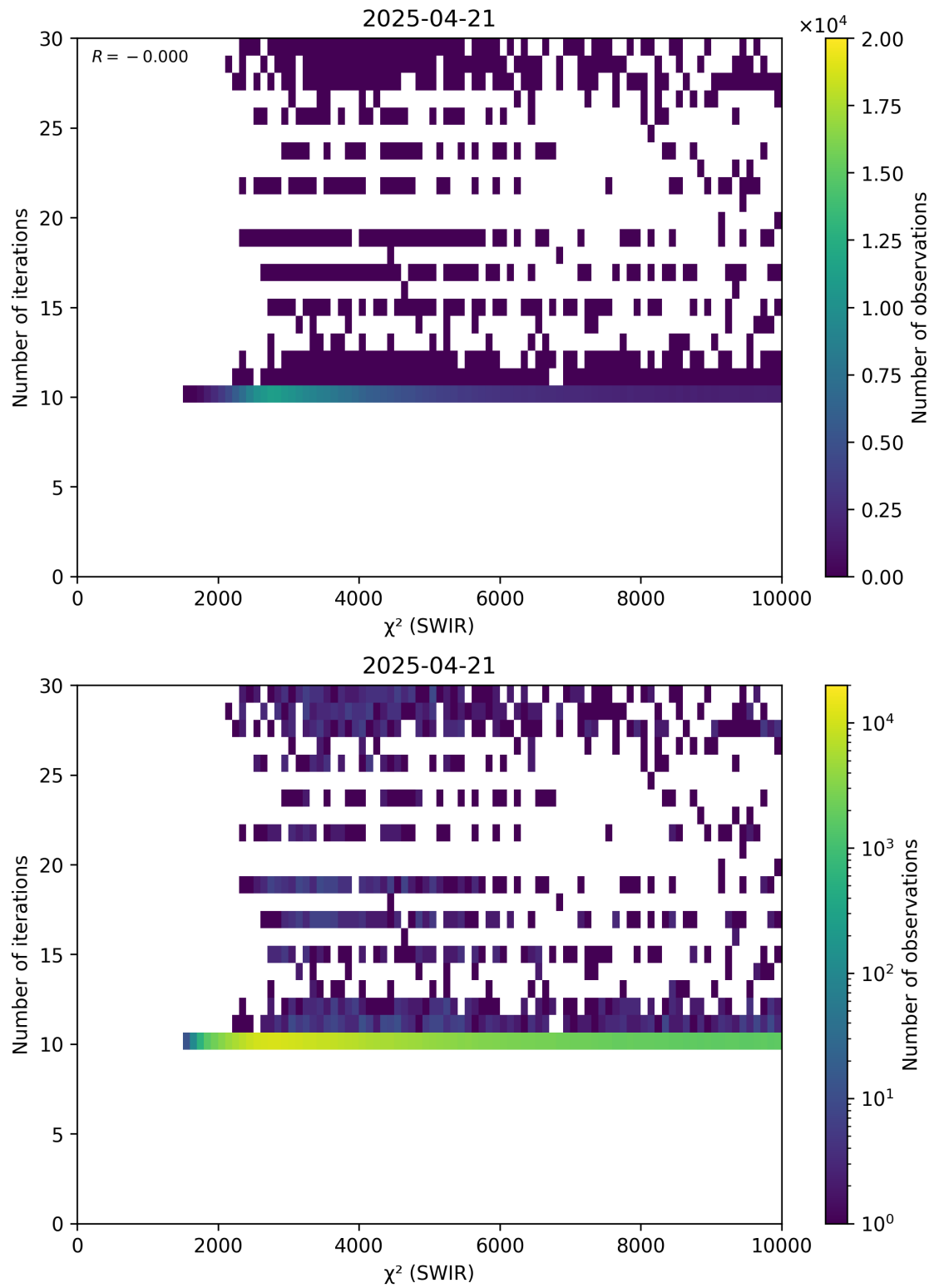
Figure 50: Scatter density plot of “ \chi^2 (SWIR)” against “Number of iterations” for 2025-04-20 to 2025-04-22.
