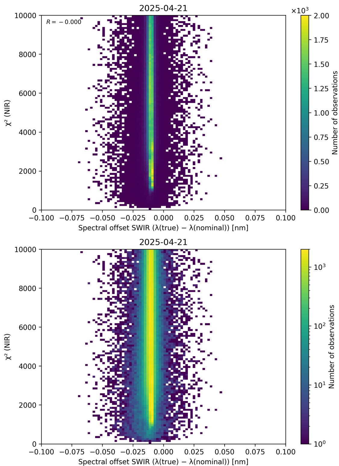
Figure 117: Scatter density plot of “Spectral offset SWIR ( \lambda_{\text{true}} - \lambda_{\text{nominal}} )” against “ \chi^2 (NIR)” for 2025-04-20 to 2025-04-22.
