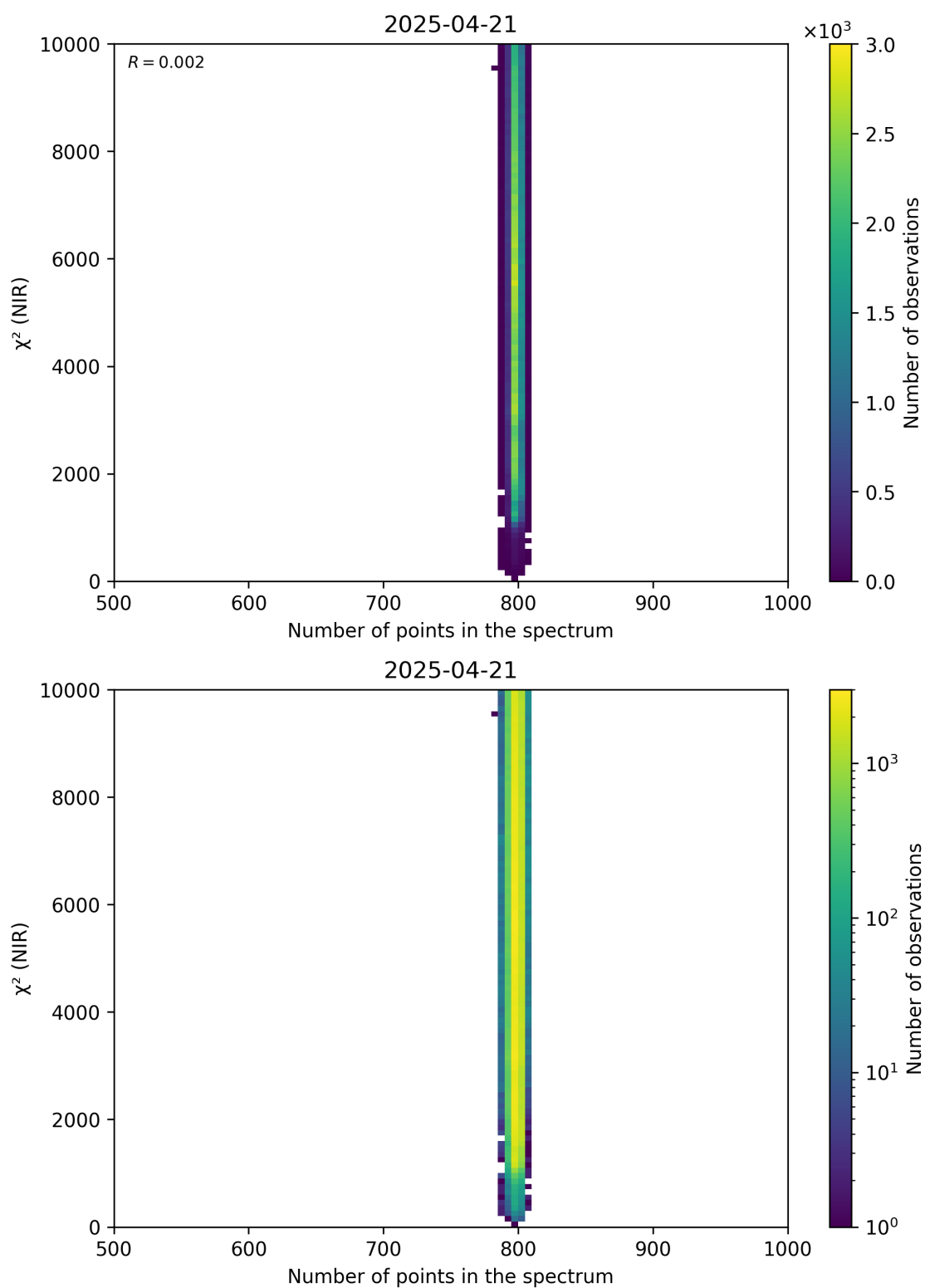
Figure 88: Scatter density plot of “Number of points in the spectrum” against “ \chi^2 (NIR)” for 2025-04-20 to 2025-04-22.
