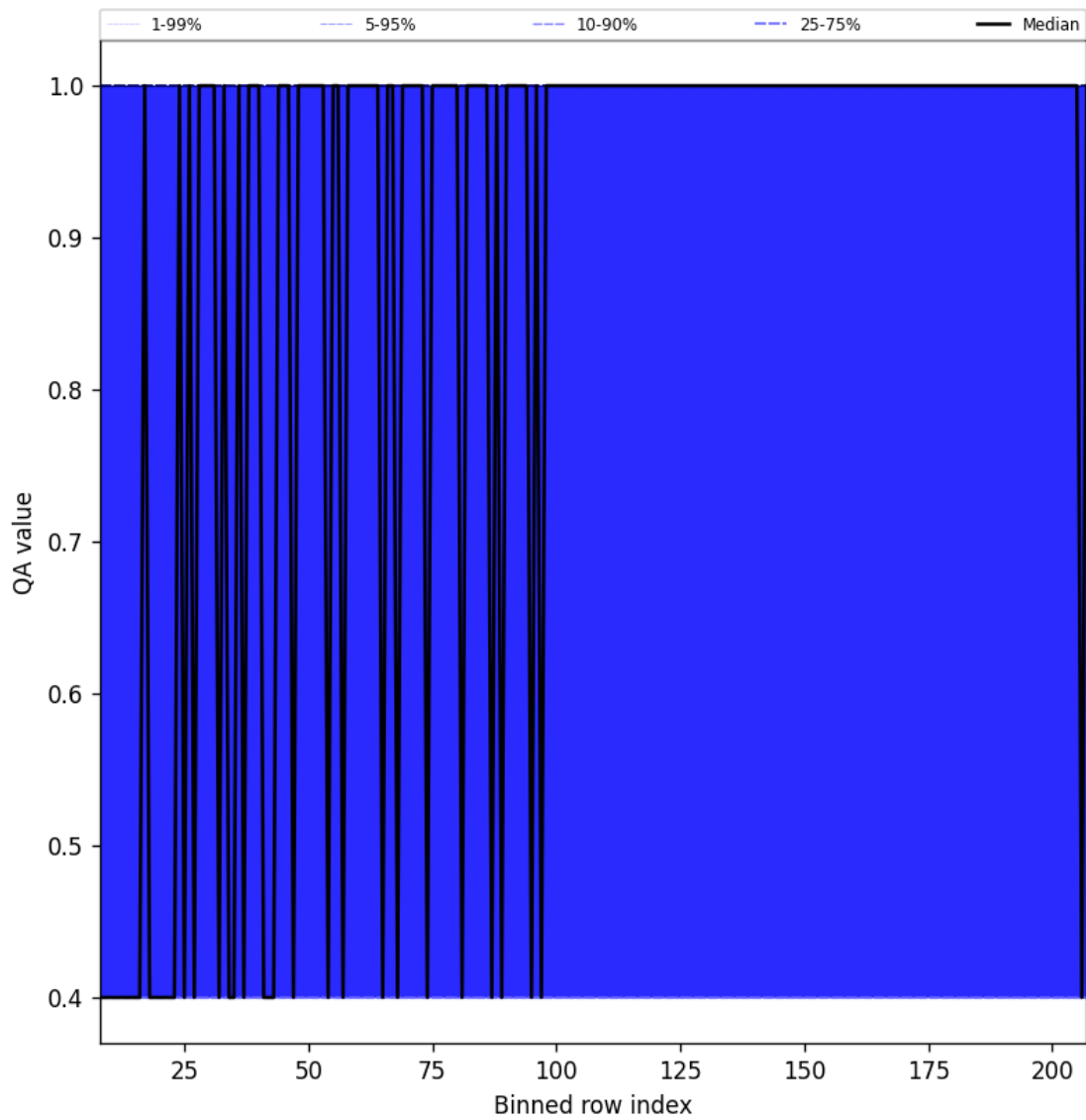
Figure 33: Along track statistics of “QA value” for 2025-04-20 to 2025-04-22
