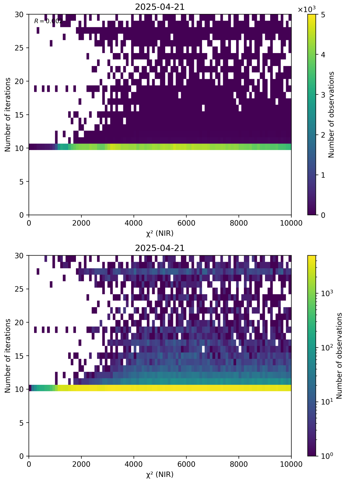
Figure 46: Scatter density plot of “ \chi^2 (NIR)” against “Number of iterations” for 2025-04-20 to 2025-04-22.
