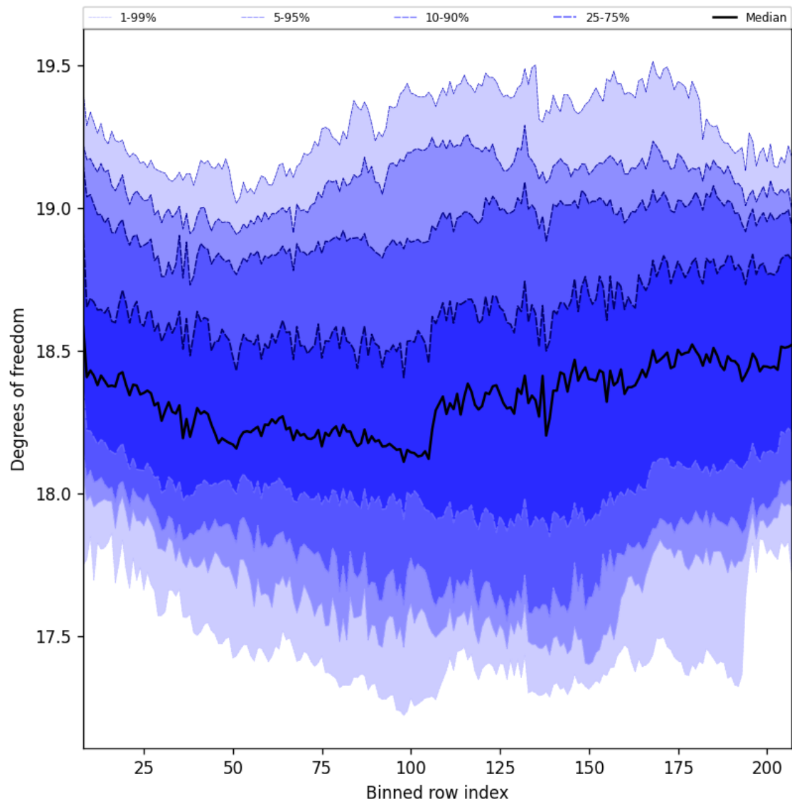
Figure 41: Along track statistics of “Degrees of freedom” for 2025-04-20 to 2025-04-22
