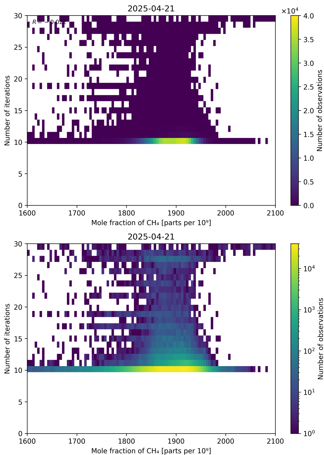
Figure 76: Scatter density plot of “Mole fraction of CH 4 ” against “Number of iterations” for 2025-04-20 to 2025-04-22.
