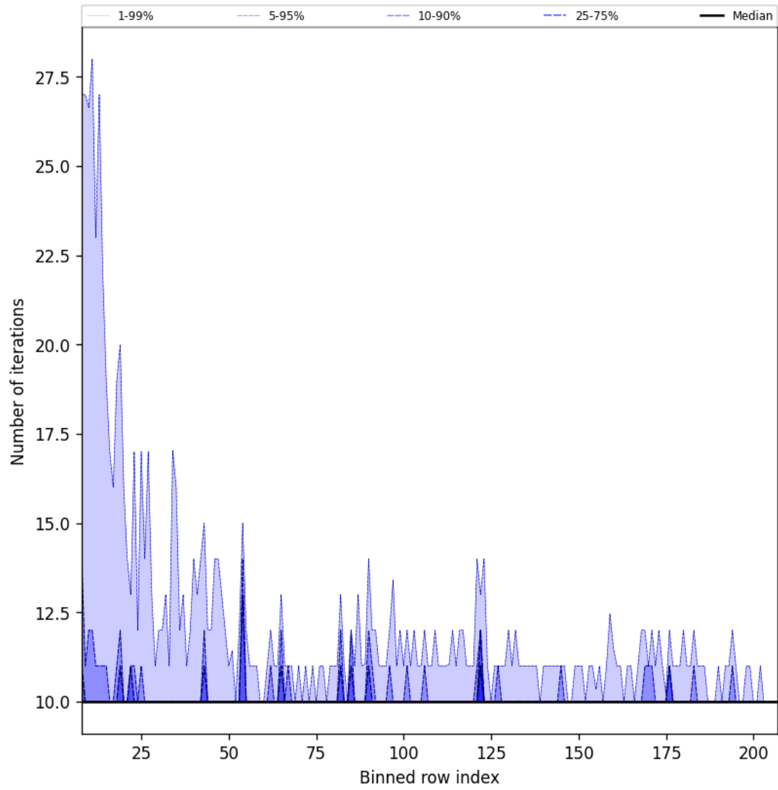
Figure 42: Along track statistics of “Number of iterations” for 2025-04-20 to 2025-04-22
