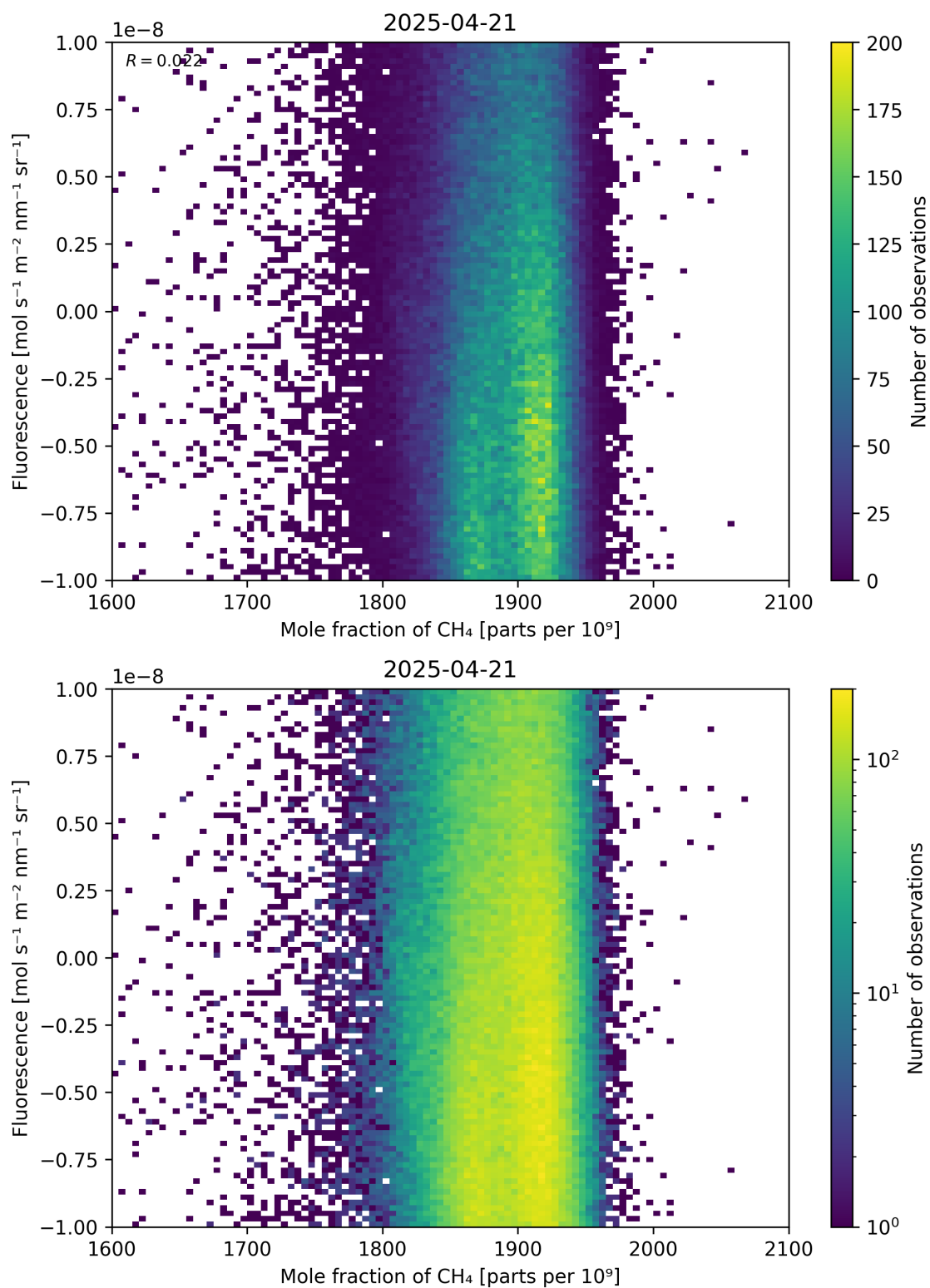
Figure 73: Scatter density plot of “Mole fraction of CH 4 ” against “Fluorescence” for 2025-04-20 to 2025-04-22.
