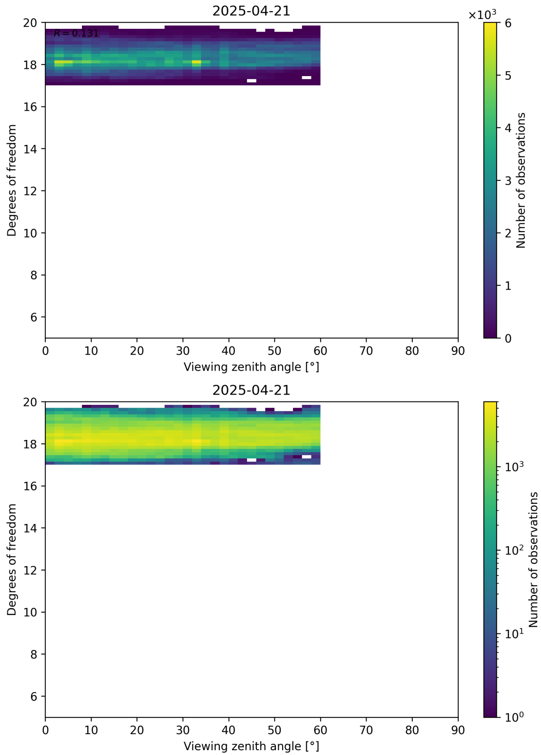
Figure 107: Scatter density plot of “Viewing zenith angle” against “Degrees of freedom” for 2025-04-20 to 2025-04-22.
