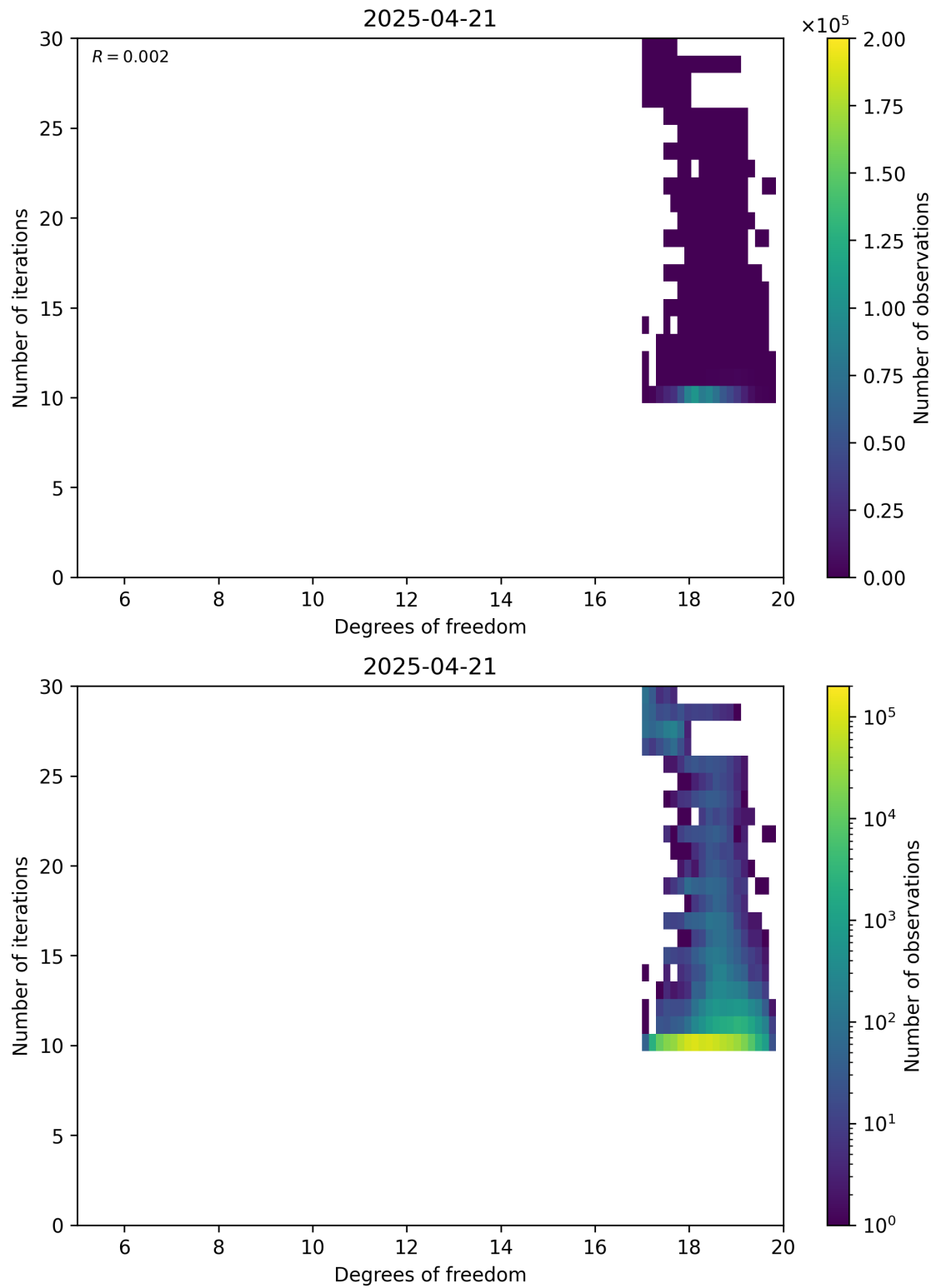
Figure 52: Scatter density plot of “Degrees of freedom” against “Number of iterations” for 2025-04-20 to 2025-04-22.
