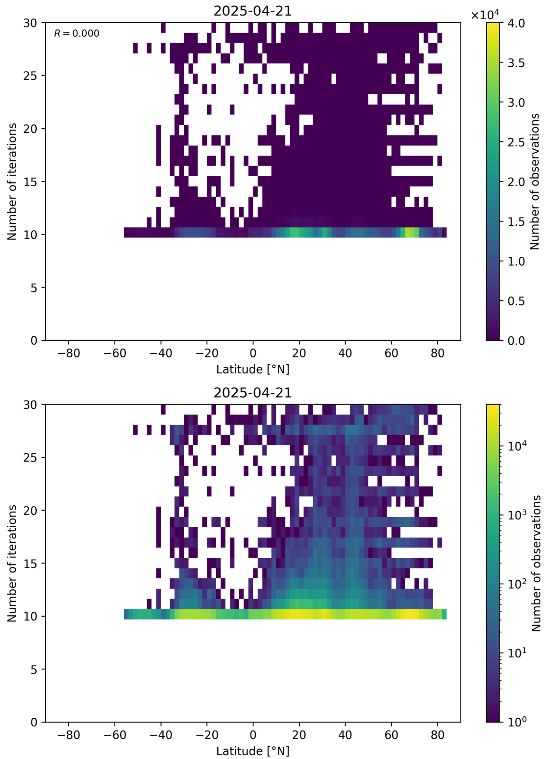
Figure 60: Scatter density plot of “Latitude” against “Number of iterations” for 2025-04-20 to 2025-04-22.
