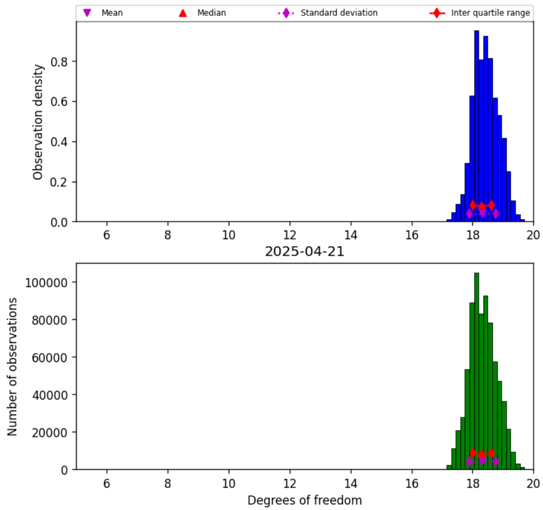
Figure 30: Histogram of “Degrees of freedom” for 2025-04-20 to 2025-04-22
