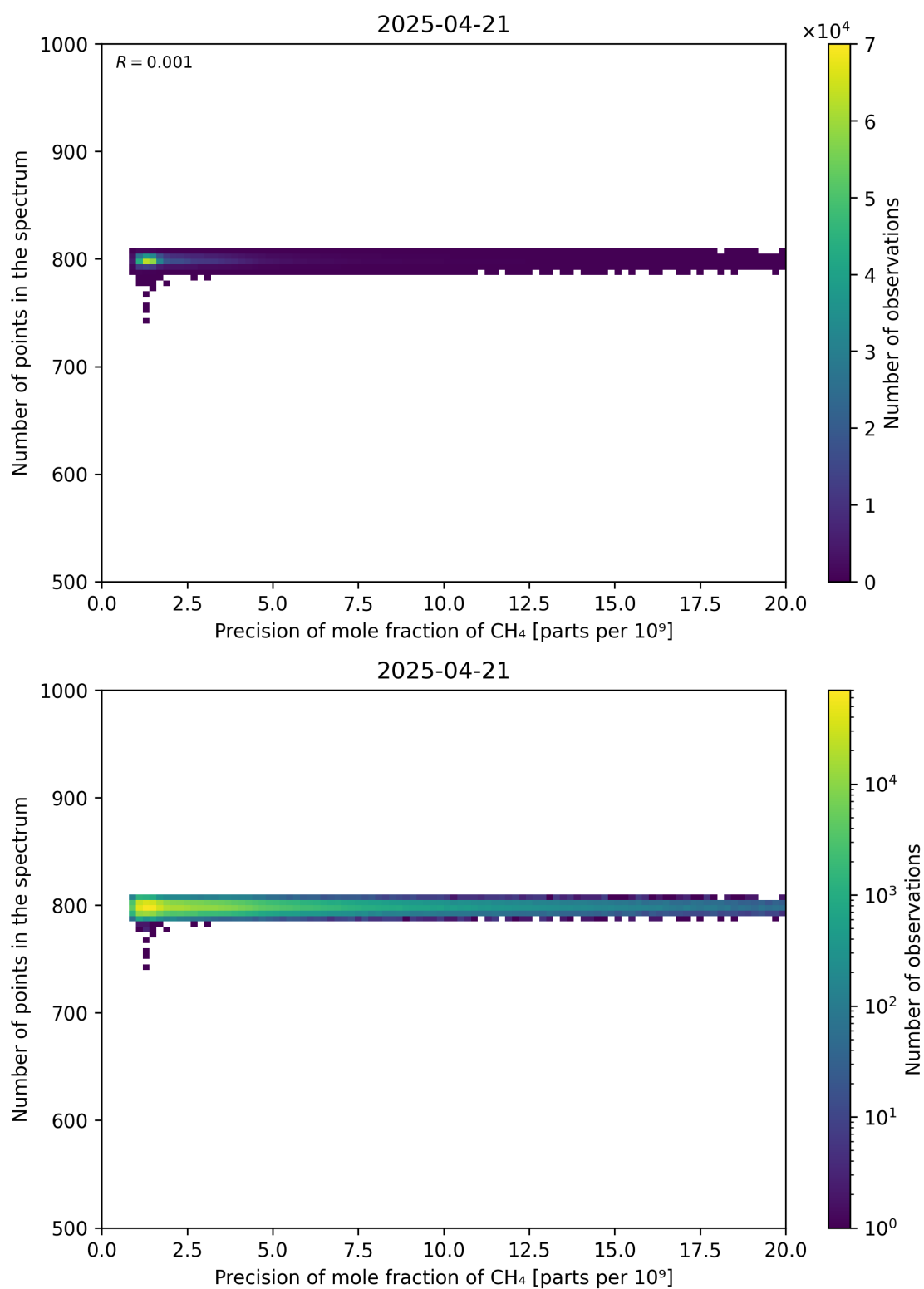
Figure 84: Scatter density plot of “Precision of mole fraction of CH 4 ” against “Number of points in the spectrum” for 2025-04-20 to 2025-04-22.
