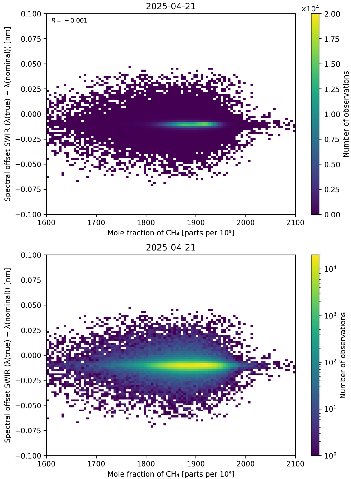
Figure 86: Scatter density plot of “Mole fraction of \text{CH}_4 ” against “Spectral offset SWIR ( \lambda_{\text{true}} - \lambda_{\text{nominal}} )” for 2025-04-20 to 2025-04-22.
