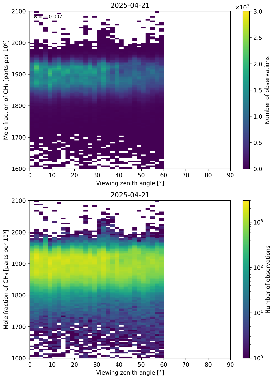
Figure 110: Scatter density plot of “Viewing zenith angle” against “Mole fraction of CH 4 ” for 2025-04-20 to 2025-04-22.
