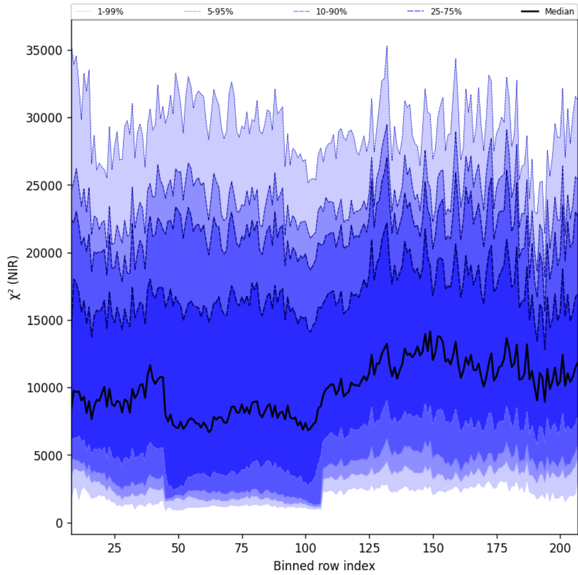
Figure 40: Along track statistics of " \chi^2 (NIR)" for 2025-04-20 to 2025-04-22
