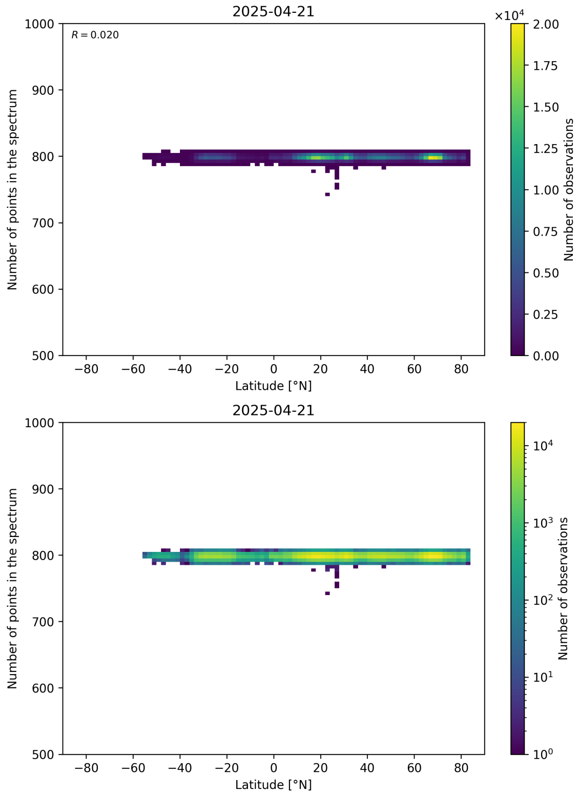
Figure 61: Scatter density plot of “Latitude” against “Number of points in the spectrum” for 2025-04-20 to 2025-04-22.
