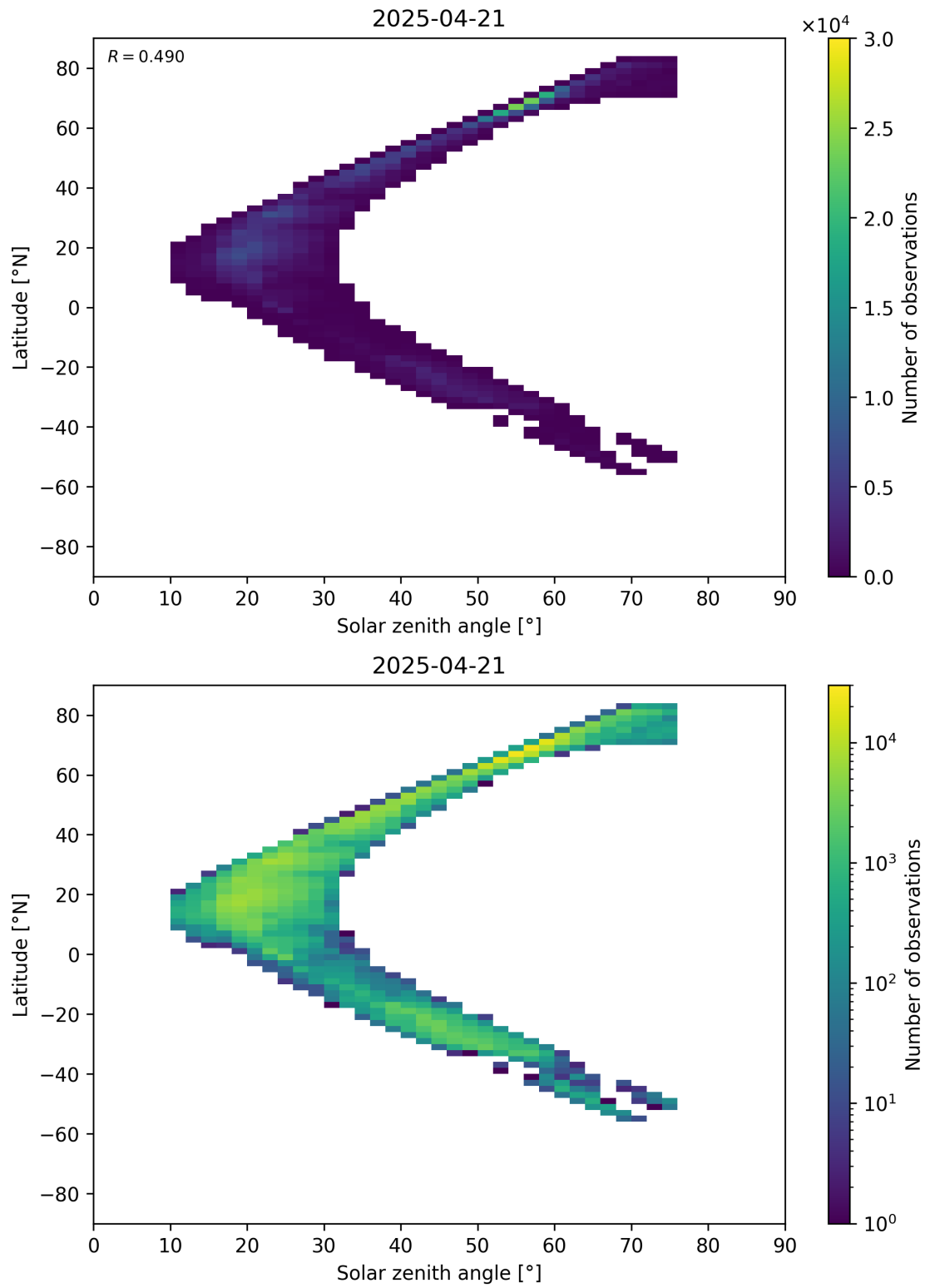
Figure 98: Scatter density plot of “Solar zenith angle” against “Latitude” for 2025-04-20 to 2025-04-22.
