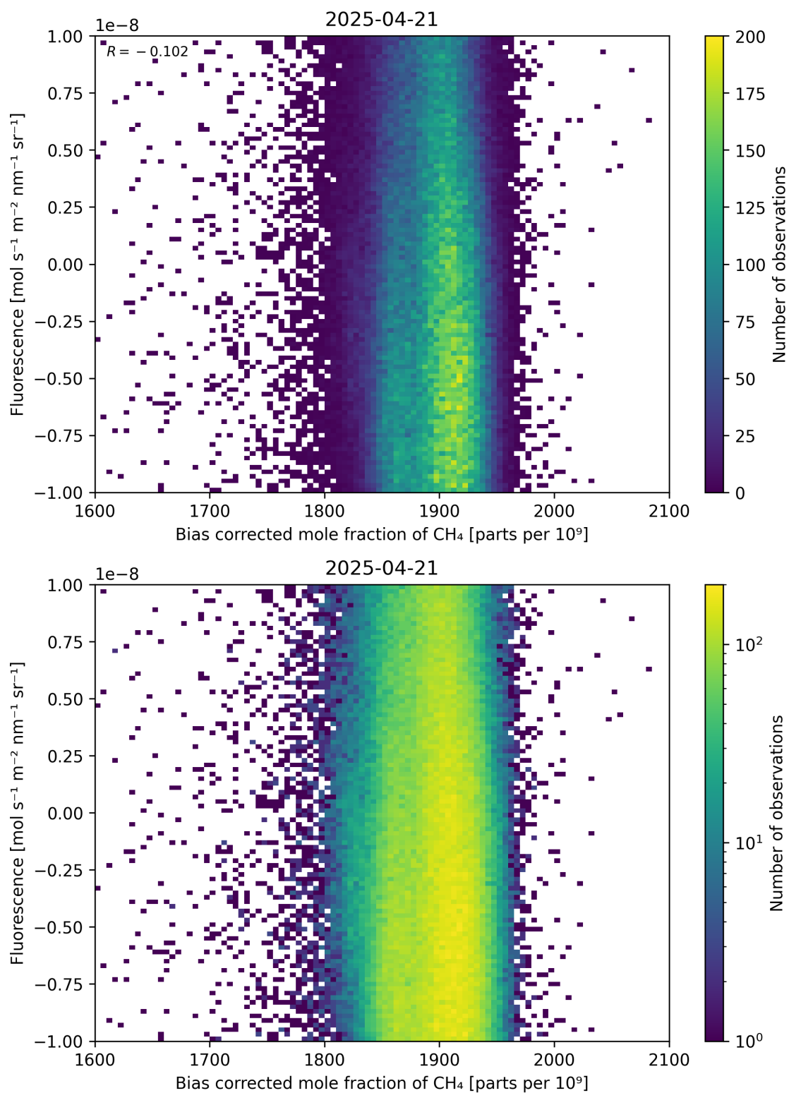
Figure 66: Scatter density plot of “Bias corrected mole fraction of \text{CH}_4 ” against “Fluorescence” for 2025-04-20 to 2025-04-22.
