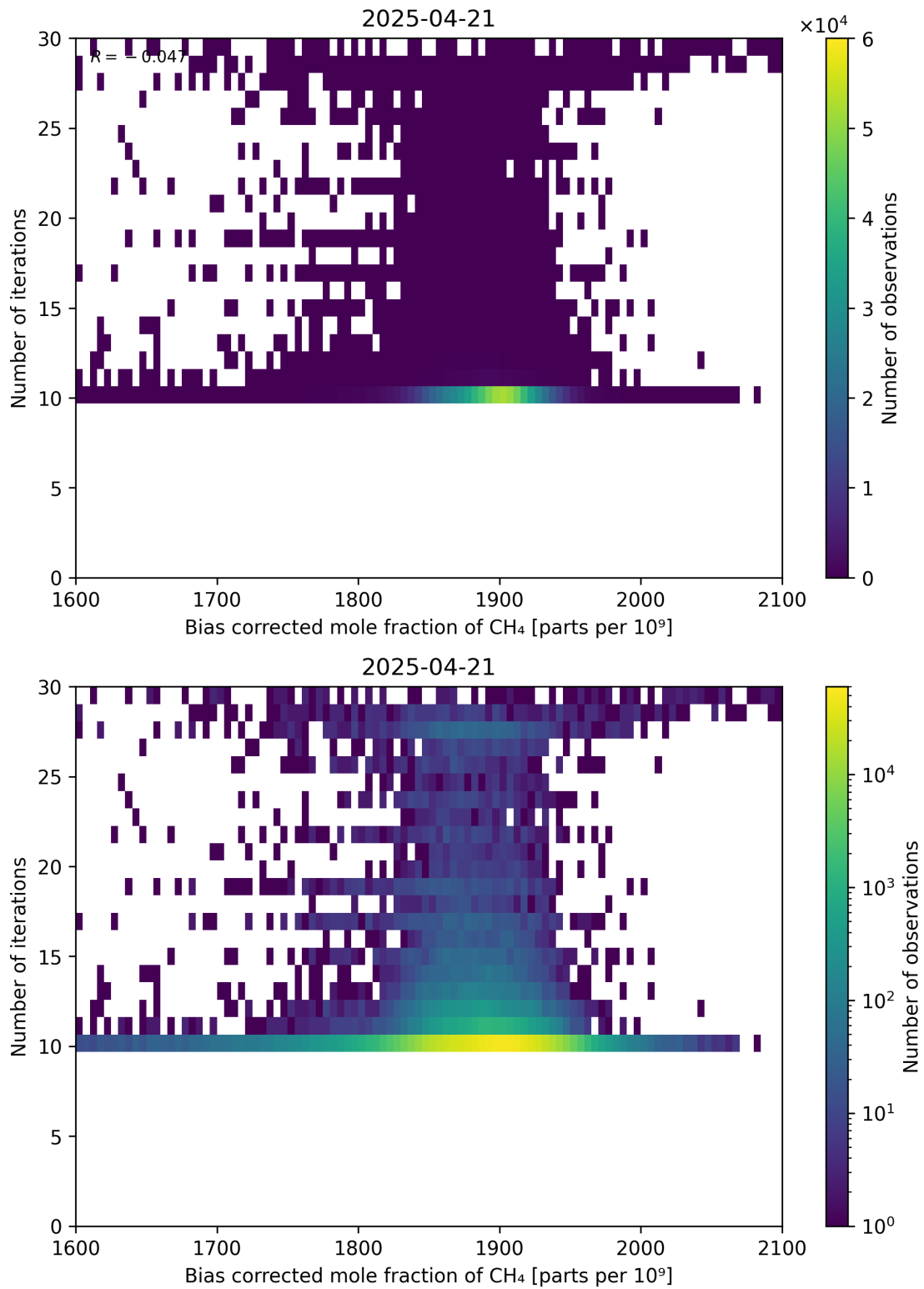
Figure 67: Scatter density plot of “Bias corrected mole fraction of \text{CH}_4 ” against “Number of iterations” for 2025-04-20 to 2025-04-22.
