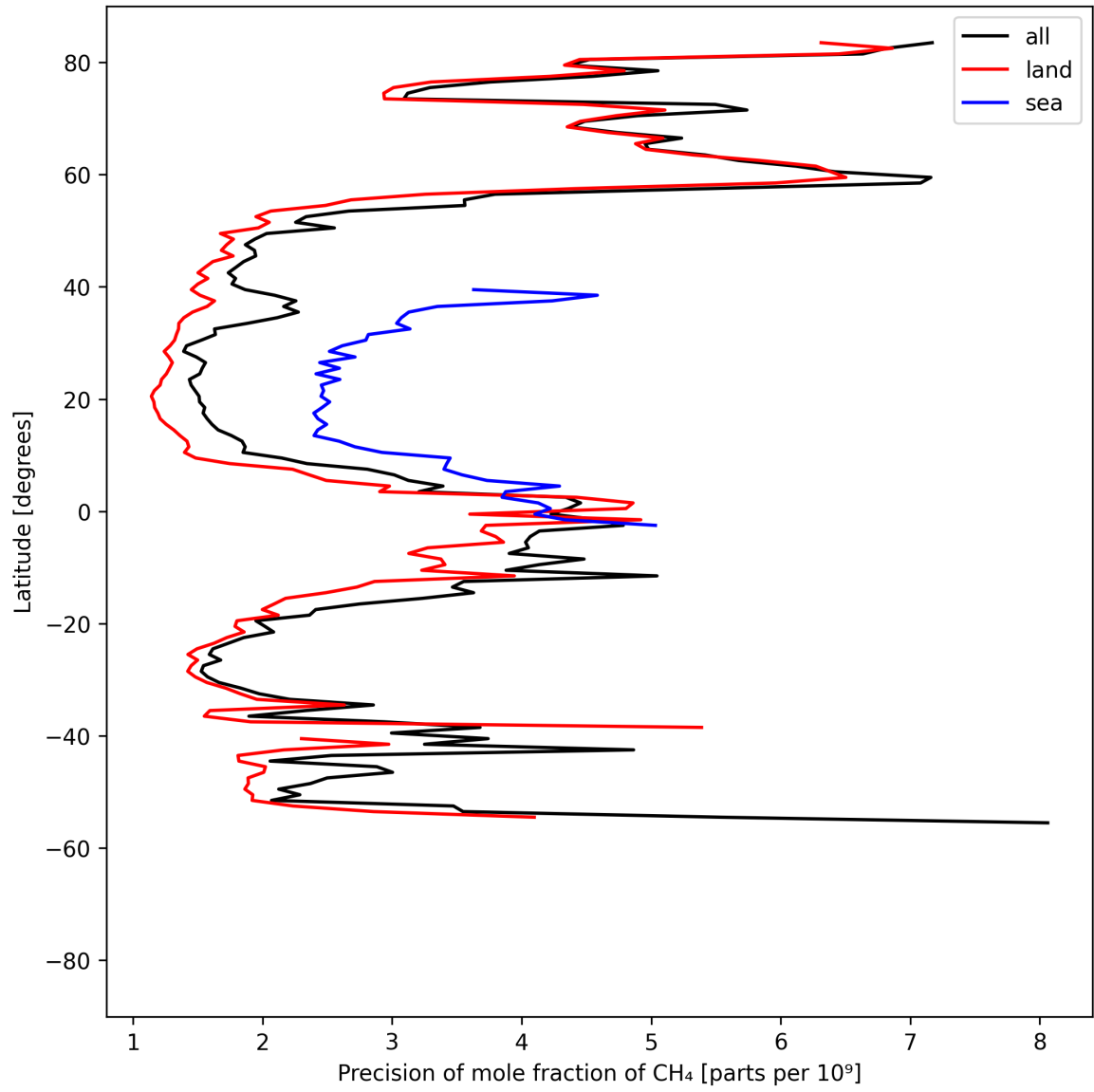
Figure 13: Zonal average of “Precision of mole fraction of CH 4 ” for 2025-04-20 to 2025-04-22.
