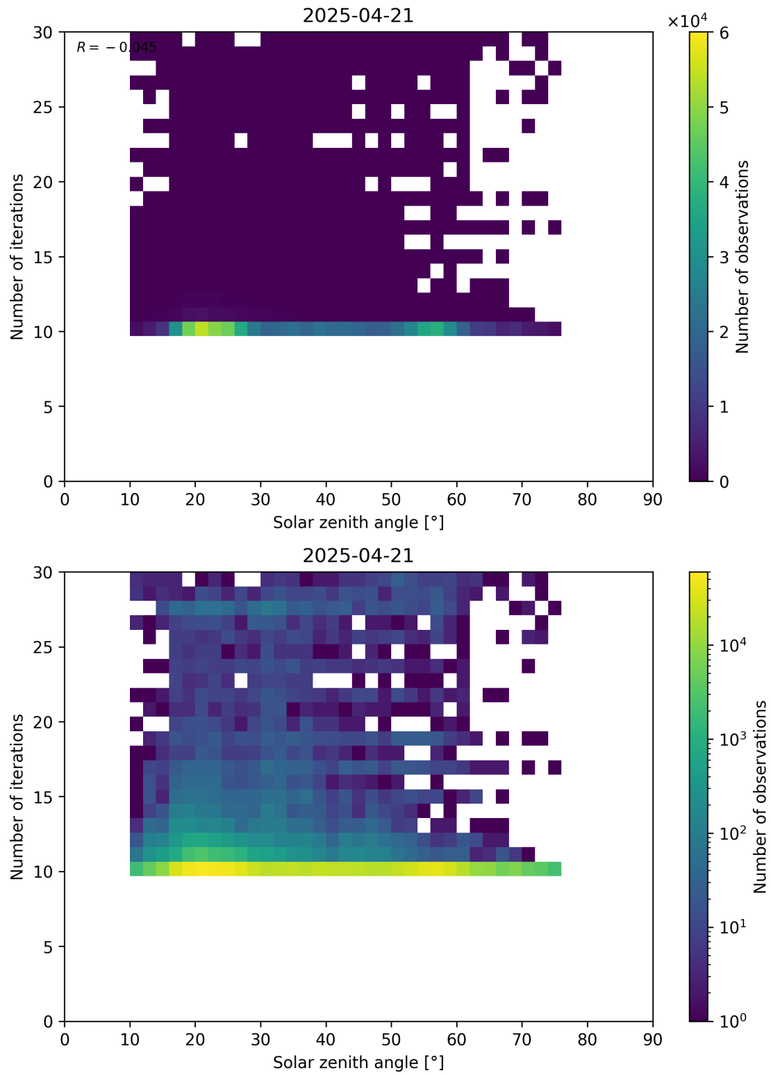
Figure 102: Scatter density plot of “Solar zenith angle” against “Number of iterations” for 2025-04-20 to 2025-04-22.
