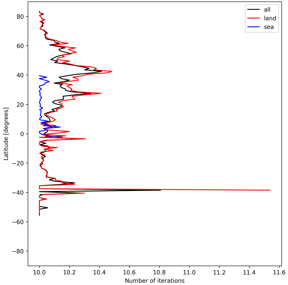
Figure 20: Zonal average of “Number of iterations” for 2025-04-20 to 2025-04-22.
