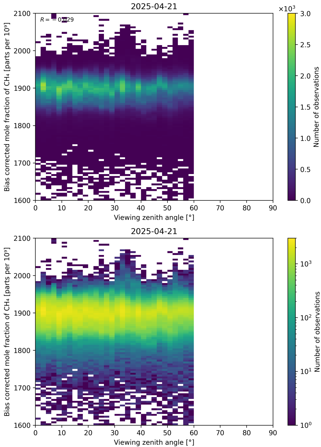
Figure 111: Scatter density plot of “Viewing zenith angle” against “Bias corrected mole fraction of CH 4 ” for 2025-04-20 to 2025-04-22.
