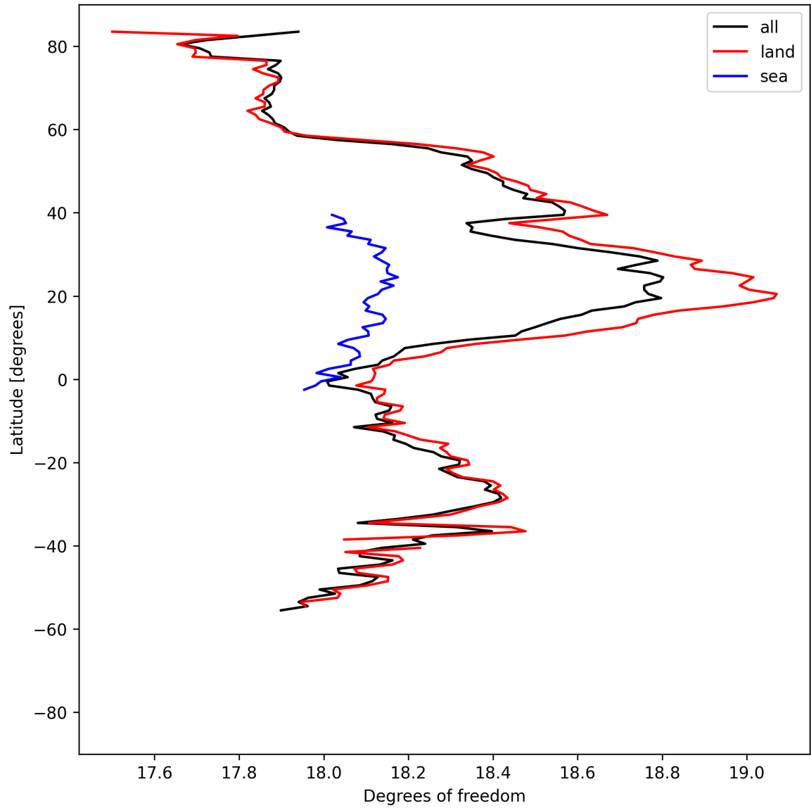
Figure 19: Zonal average of “Degrees of freedom” for 2025-04-20 to 2025-04-22.
