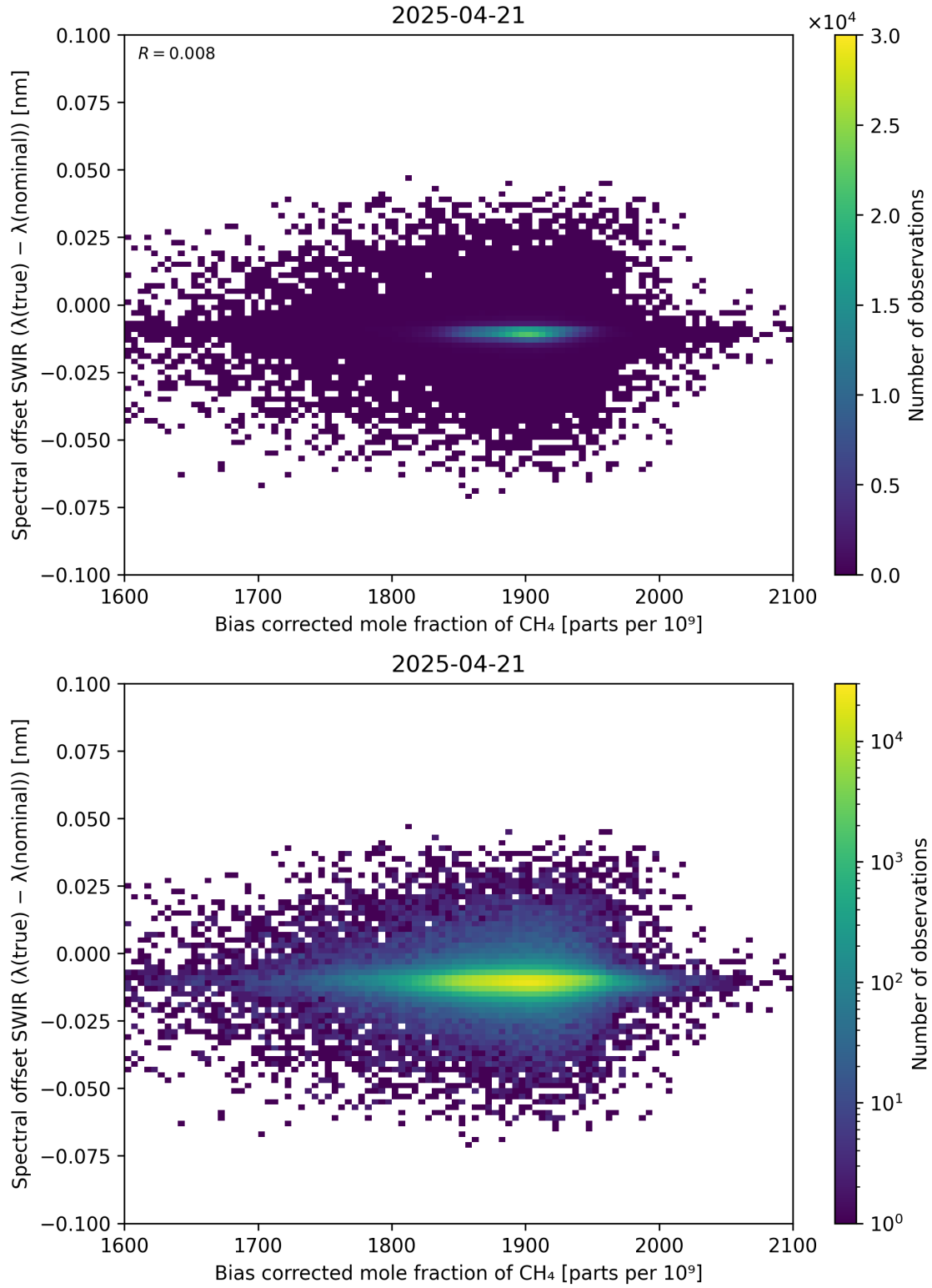
Figure 69: Scatter density plot of “Bias corrected mole fraction of \text{CH}_4 ” against “Spectral offset SWIR ( \lambda_{\text{true}} - \lambda_{\text{nominal}} )” for 2025-04-20 to 2025-04-22.
