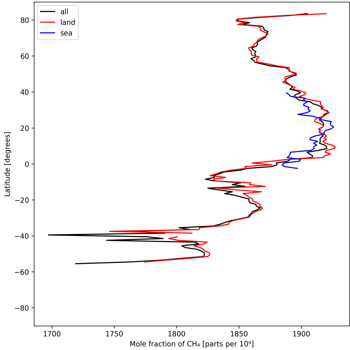
Figure 12: Zonal average of “Mole fraction of \text{CH}_4 ” for 2025-04-20 to 2025-04-22.
