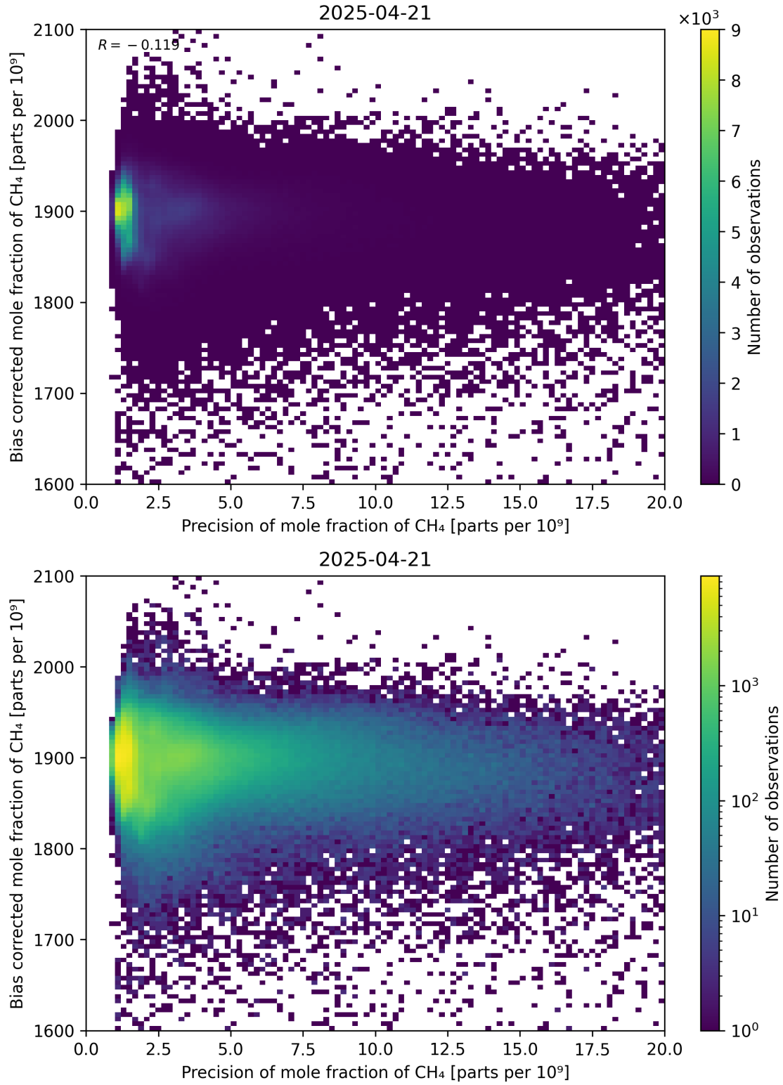
Figure 82: Scatter density plot of “Precision of mole fraction of CH 4 ” against “Bias corrected mole fraction of CH 4 ” for 2025-04-20 to 2025-04-22.
