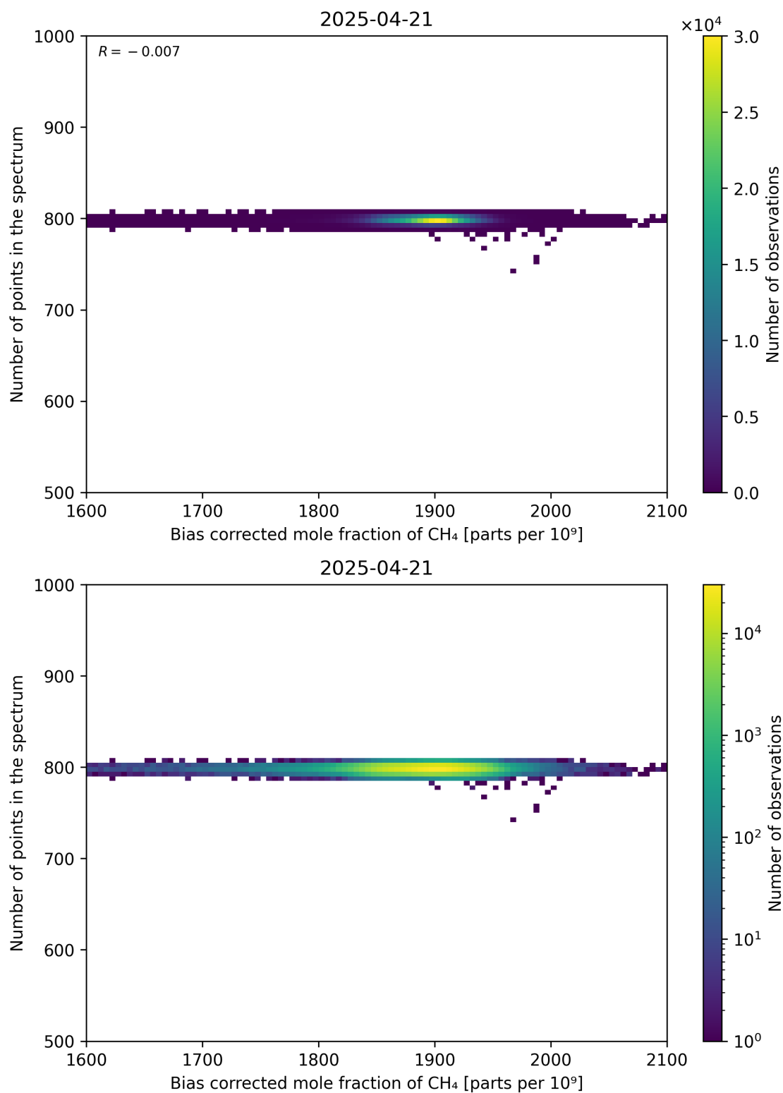
Figure 68: Scatter density plot of “Bias corrected mole fraction of CH 4 ” against “Number of points in the spectrum” for 2025-04-20 to 2025-04-22.
