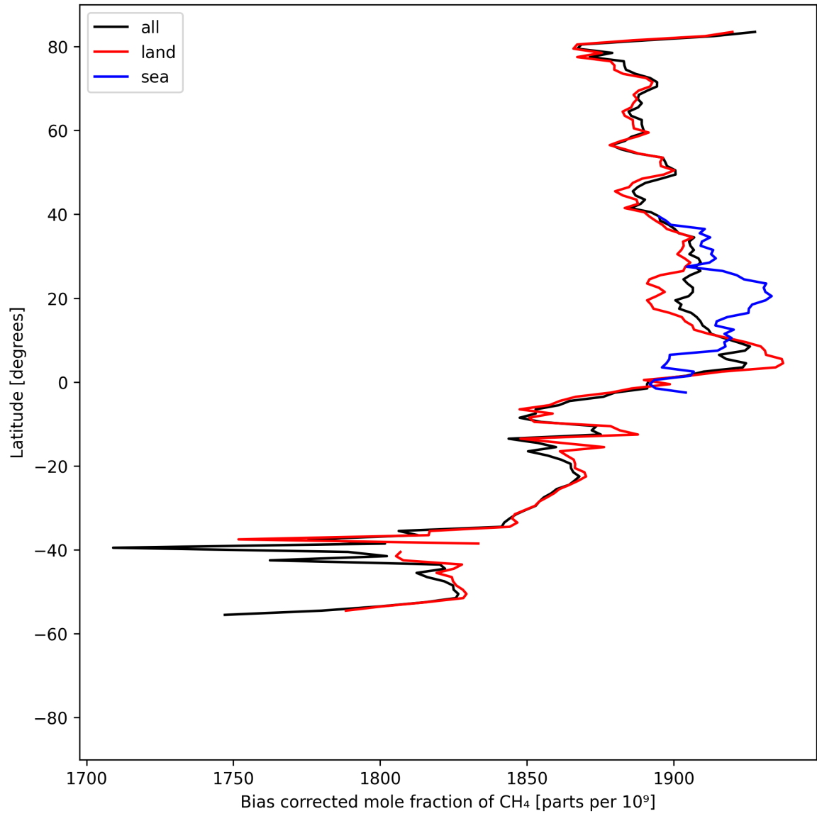
Figure 14: Zonal average of “Bias corrected mole fraction of \text{CH}_4 ” for 2025-04-20 to 2025-04-22.
