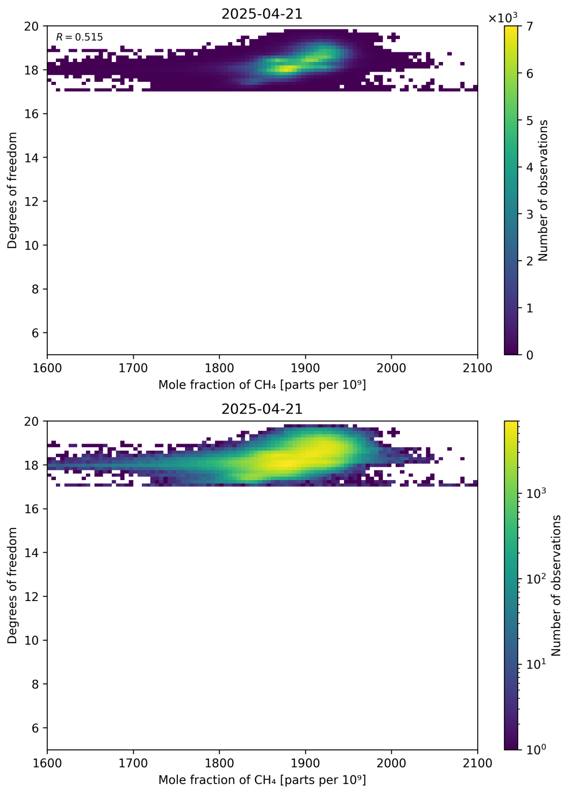
Figure 72: Scatter density plot of “Mole fraction of CH 4 ” against “Degrees of freedom” for 2025-04-20 to 2025-04-22.
