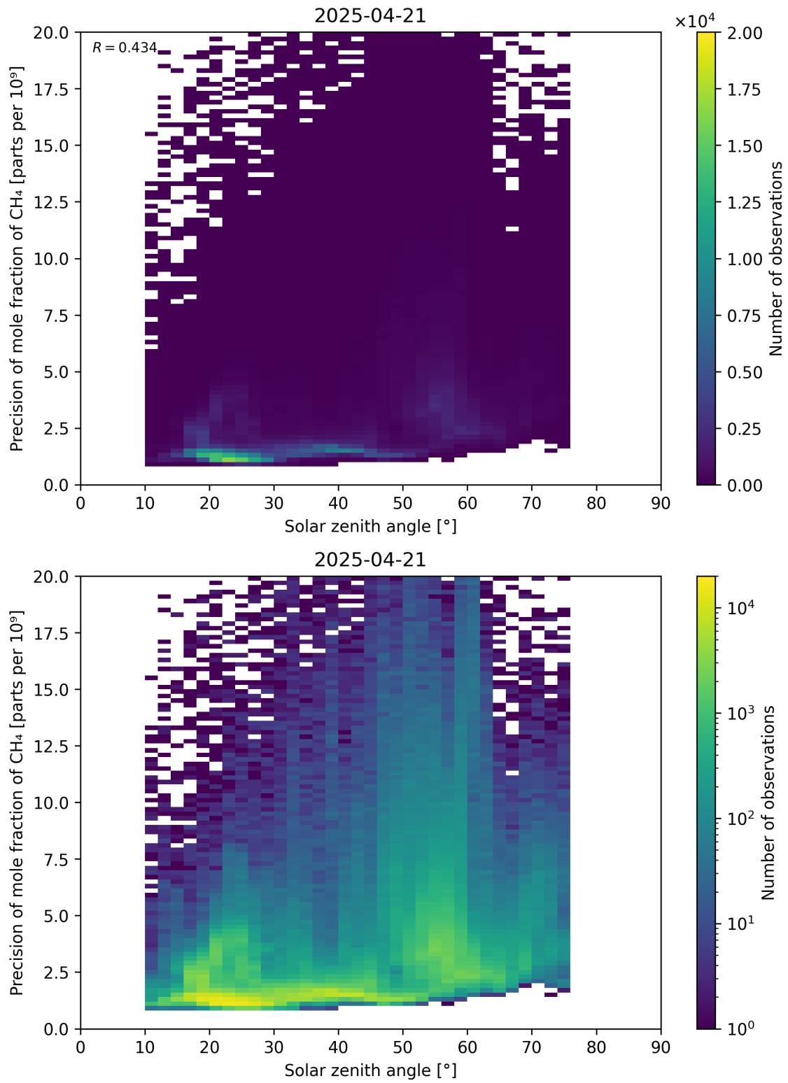
Figure 101: Scatter density plot of “Solar zenith angle” against “Precision of mole fraction of CH 4 ” for 2025-04-20 to 2025-04-22.
