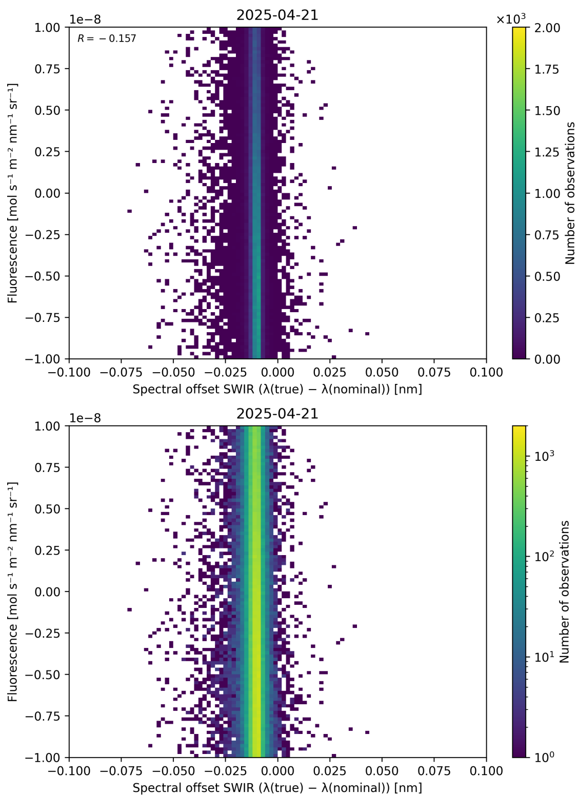
Figure 120: Scatter density plot of “Spectral offset SWIR ( \lambda_{\text{true}} - \lambda_{\text{nominal}} )” against “Fluorescence” for 2025-04-20 to 2025-04-22.
