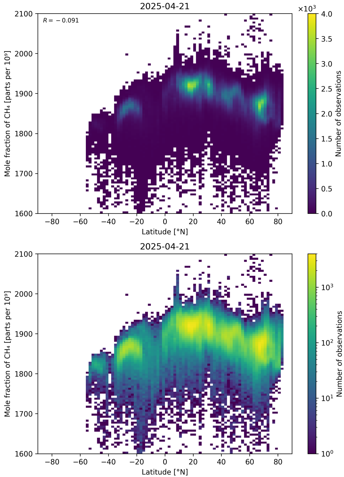
Figure 57: Scatter density plot of “Latitude” against “Mole fraction of CH 4 ” for 2025-04-20 to 2025-04-22.
