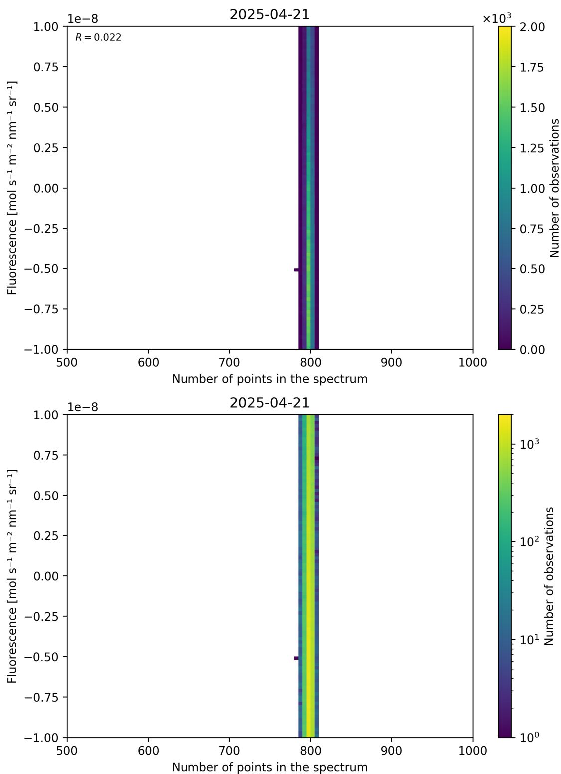
Figure 91: Scatter density plot of “Number of points in the spectrum” against “Fluorescence” for 2025-04-20 to 2025-04-22.
