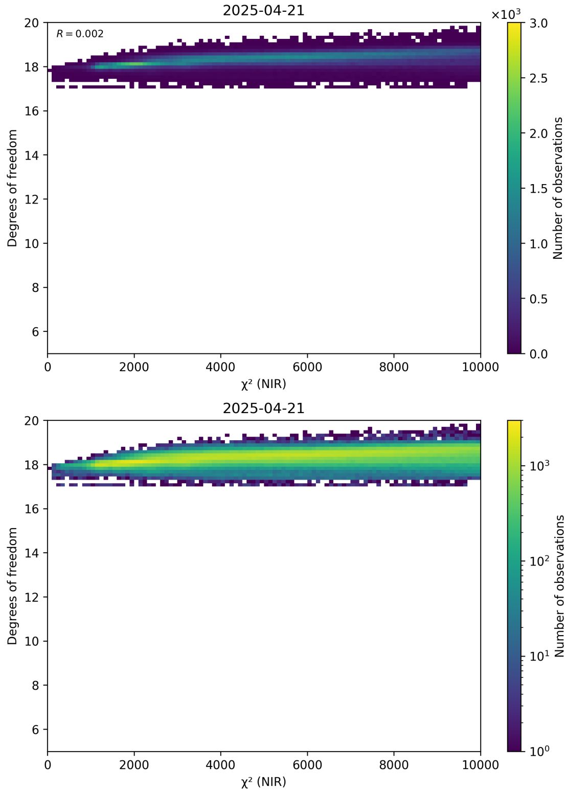
Figure 44: Scatter density plot of “ \chi^2 (NIR)” against “Degrees of freedom” for 2025-04-20 to 2025-04-22.
