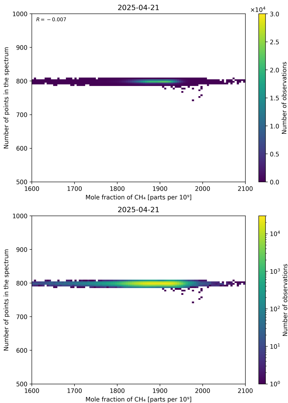
Figure 77: Scatter density plot of “Mole fraction of CH 4 ” against “Number of points in the spectrum” for 2025-04-20 to 2025-04-22.
