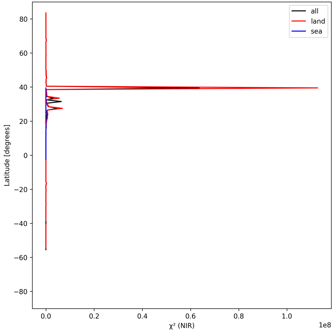
Figure 18: Zonal average of “ \chi^2 (NIR)” for 2025-04-20 to 2025-04-22.
