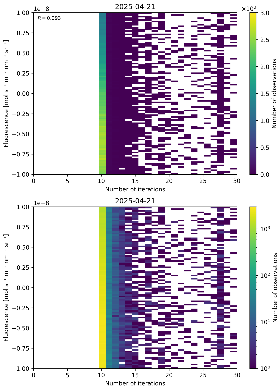
Figure 87: Scatter density plot of "Number of iterations" against "Fluorescence" for 2025-04-20 to 2025-04-22.
