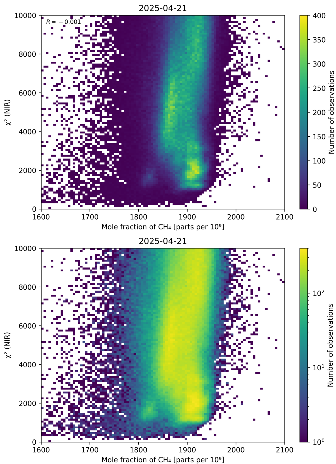
Figure 70: Scatter density plot of “Mole fraction of \text{CH}_4 ” against “ \chi^2 (NIR)” for 2025-04-20 to 2025-04-22.
