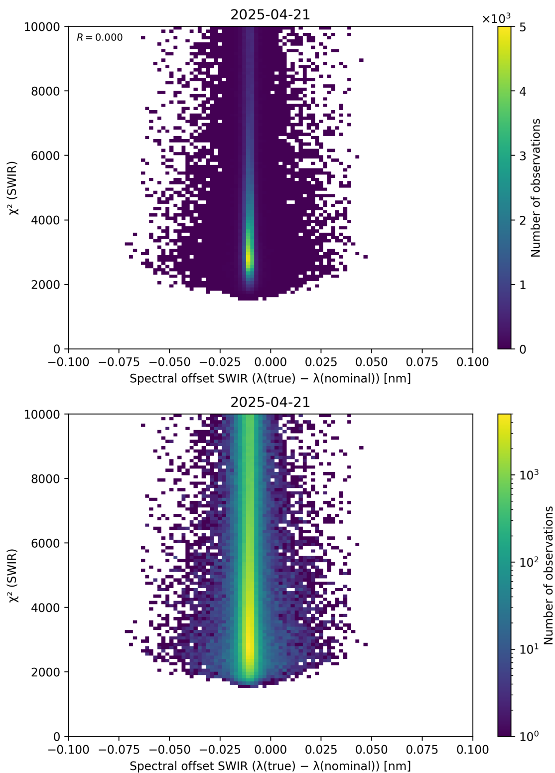
Figure 118: Scatter density plot of “Spectral offset SWIR ( \lambda_{\text{true}} - \lambda_{\text{nominal}} )” against “ \chi^2 (SWIR)” for 2025-04-20 to 2025-04-22.
