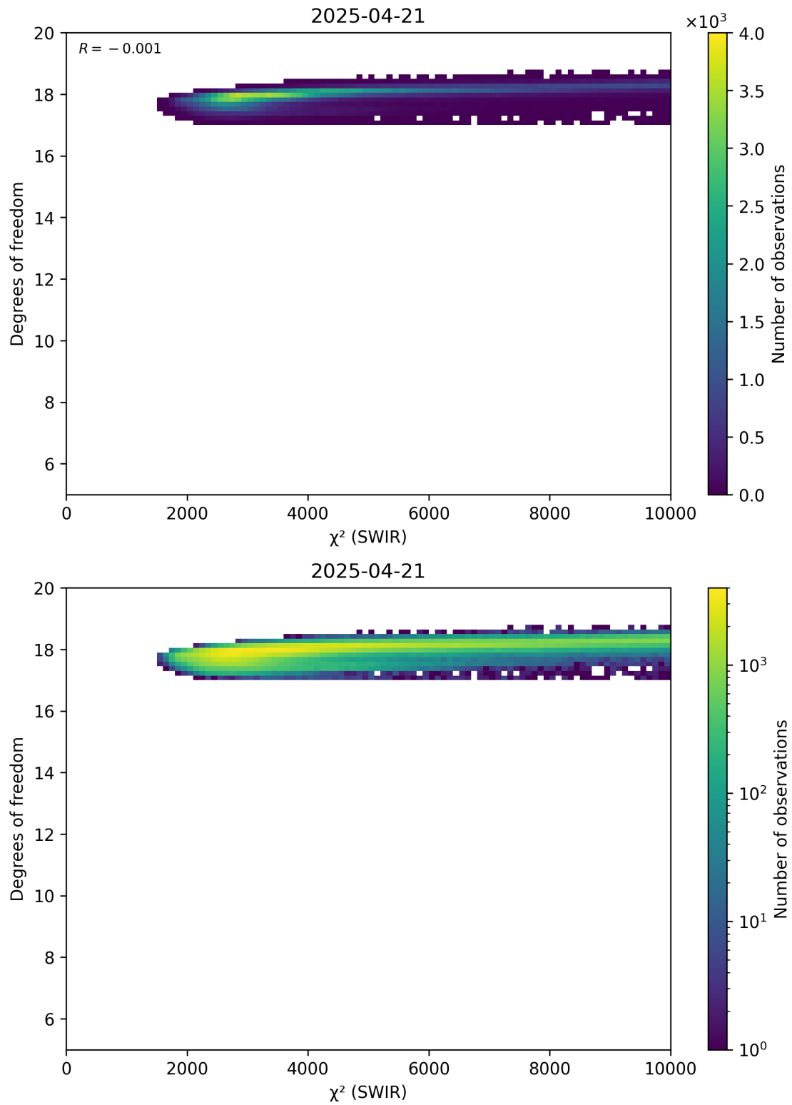
Figure 48: Scatter density plot of “ \chi^2 (SWIR)” against “Degrees of freedom” for 2025-04-20 to 2025-04-22.
