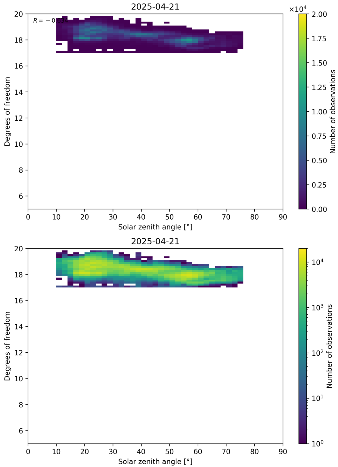
Figure 96: Scatter density plot of “Solar zenith angle” against “Degrees of freedom” for 2025-04-20 to 2025-04-22.
