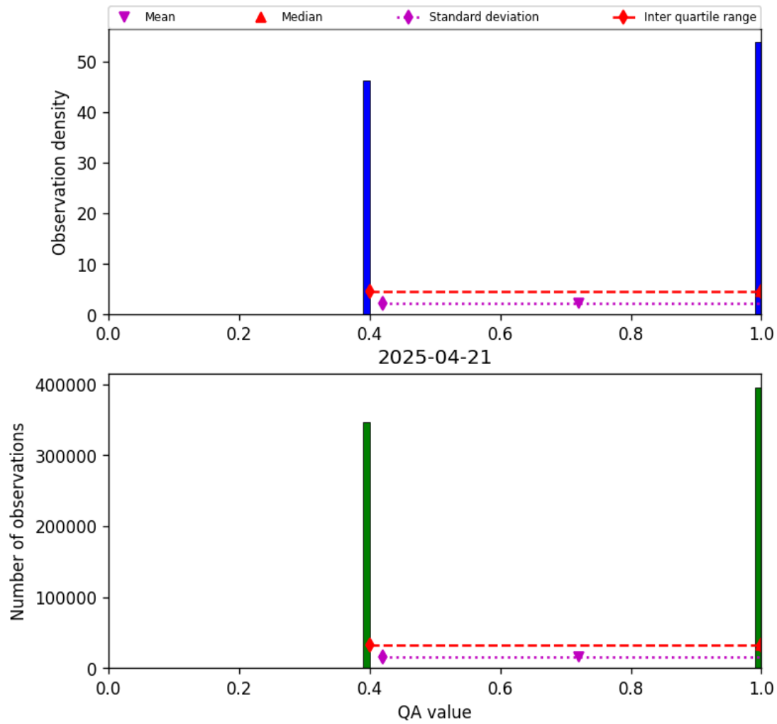
Figure 22: Histogram of “QA value” for 2025-04-20 to 2025-04-22
