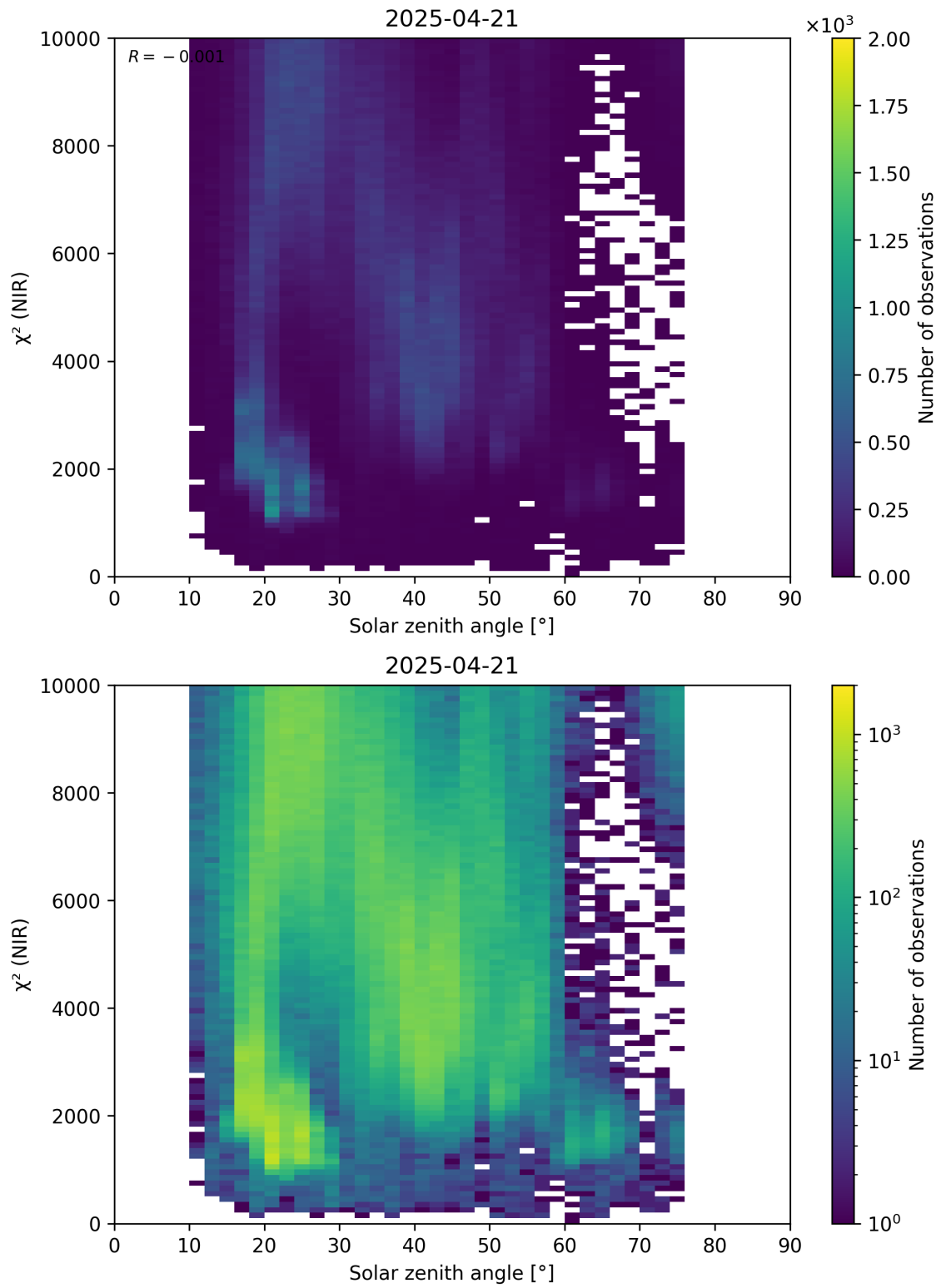
Figure 94: Scatter density plot of “Solar zenith angle” against “ \chi^2 (NIR)” for 2025-04-20 to 2025-04-22.
