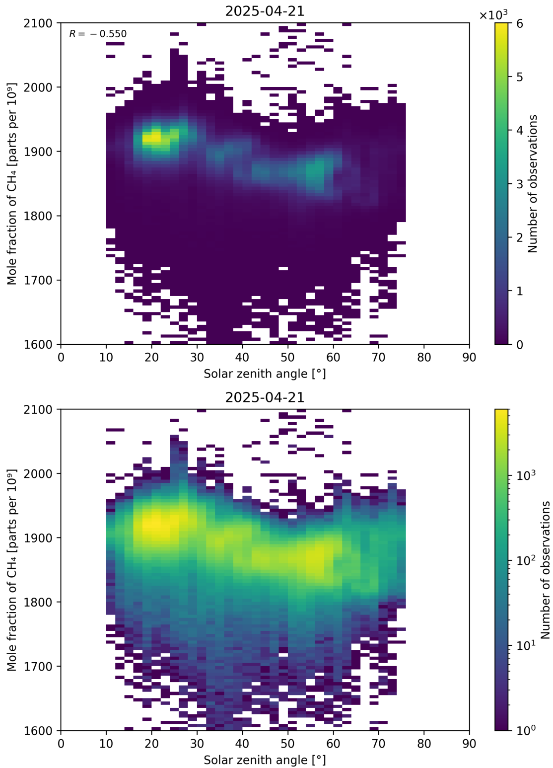
Figure 99: Scatter density plot of “Solar zenith angle” against “Mole fraction of \text{CH}_4 ” for 2025-04-20 to 2025-04-22.
