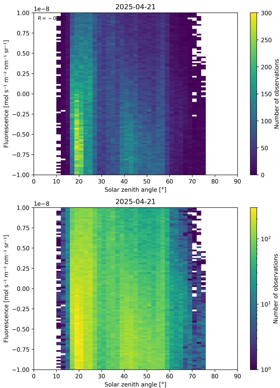
Figure 97: Scatter density plot of “Solar zenith angle” against “Fluorescence” for 2025-04-20 to 2025-04-22.
