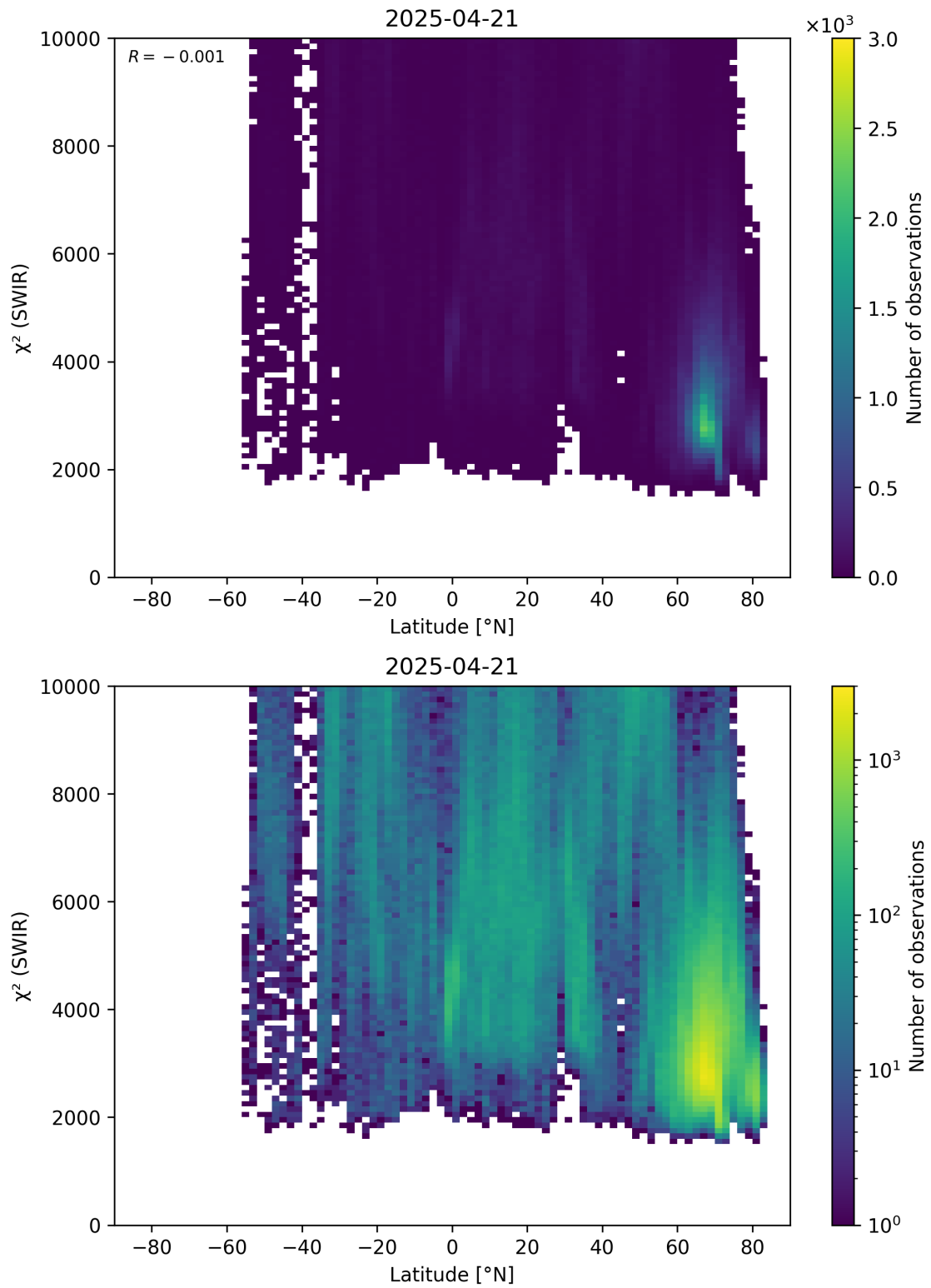
Figure 54: Scatter density plot of “Latitude” against “ \chi^2 (SWIR)” for 2025-04-20 to 2025-04-22.
