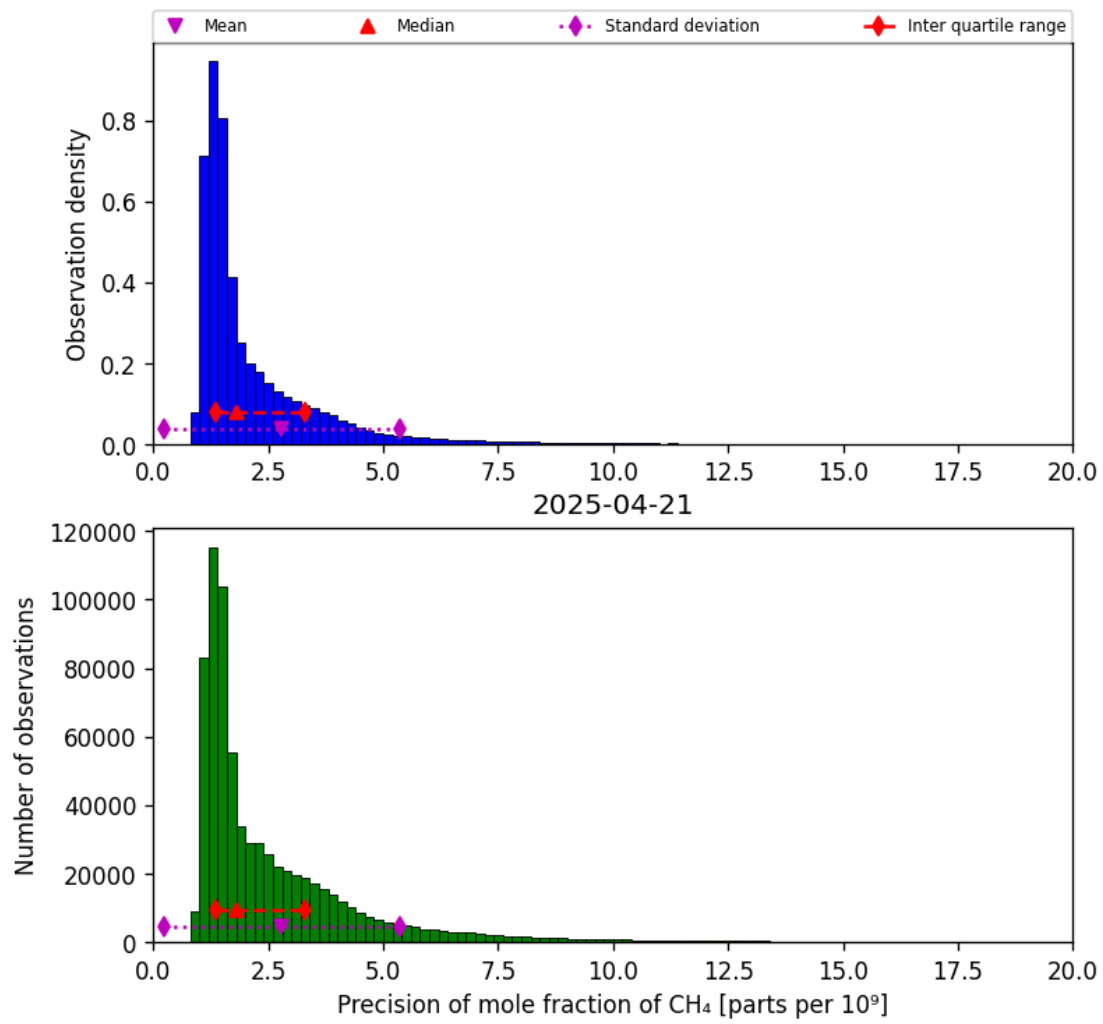
Figure 24: Histogram of “Precision of mole fraction of CH 4 ” for 2025-04-20 to 2025-04-22
