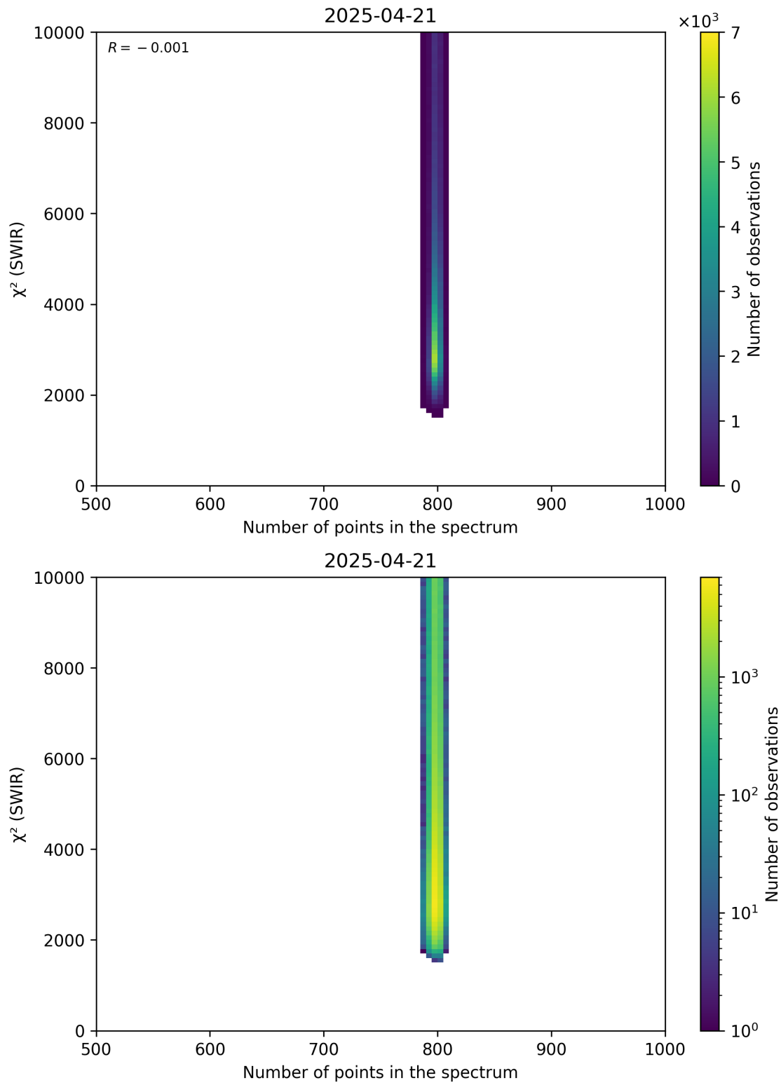
Figure 89: Scatter density plot of “Number of points in the spectrum” against “ \chi^2 (SWIR)” for 2025-04-20 to 2025-04-22.
