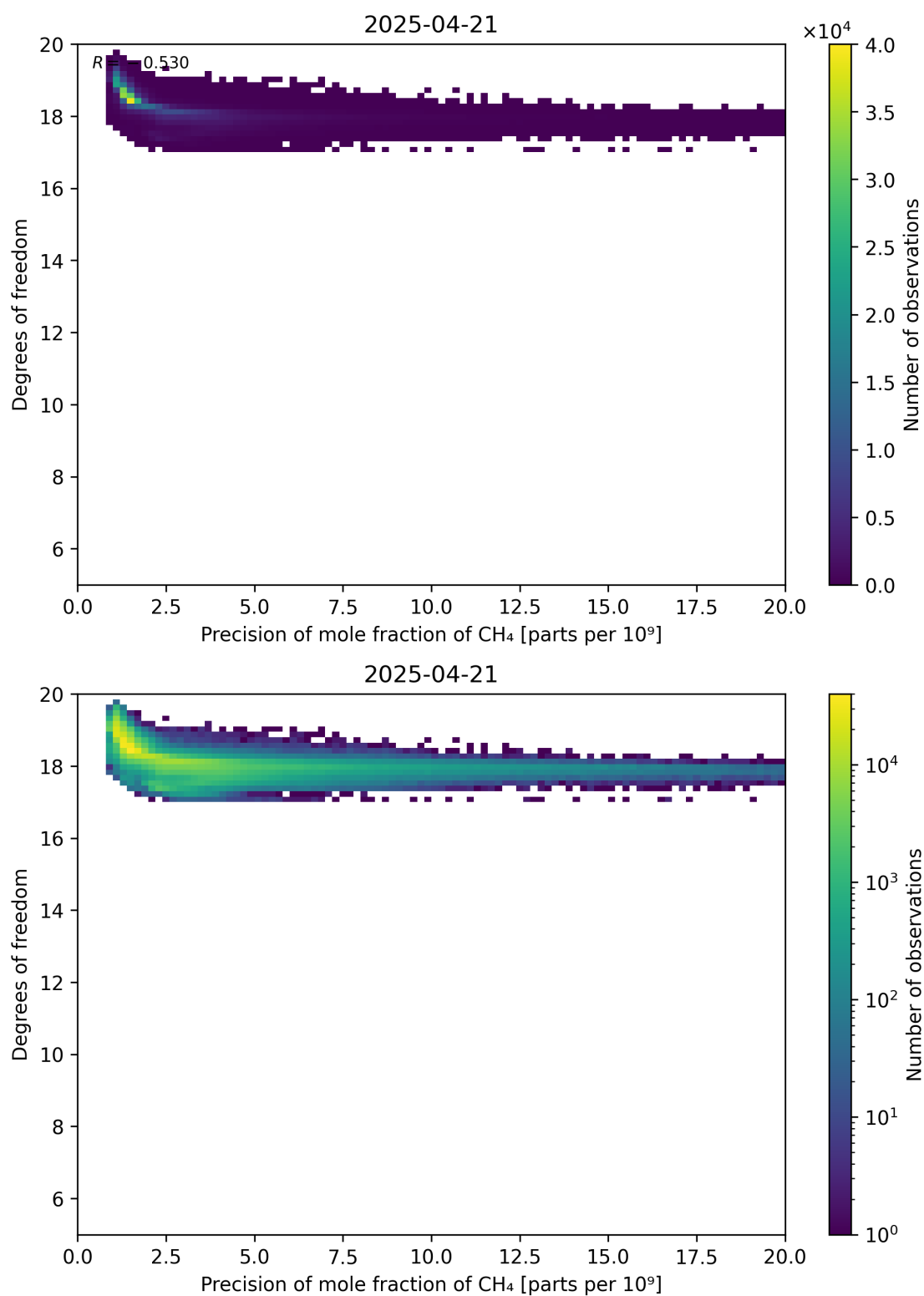
Figure 80: Scatter density plot of “Precision of mole fraction of CH 4 ” against “Degrees of freedom” for 2025-04-20 to 2025-04-22.
