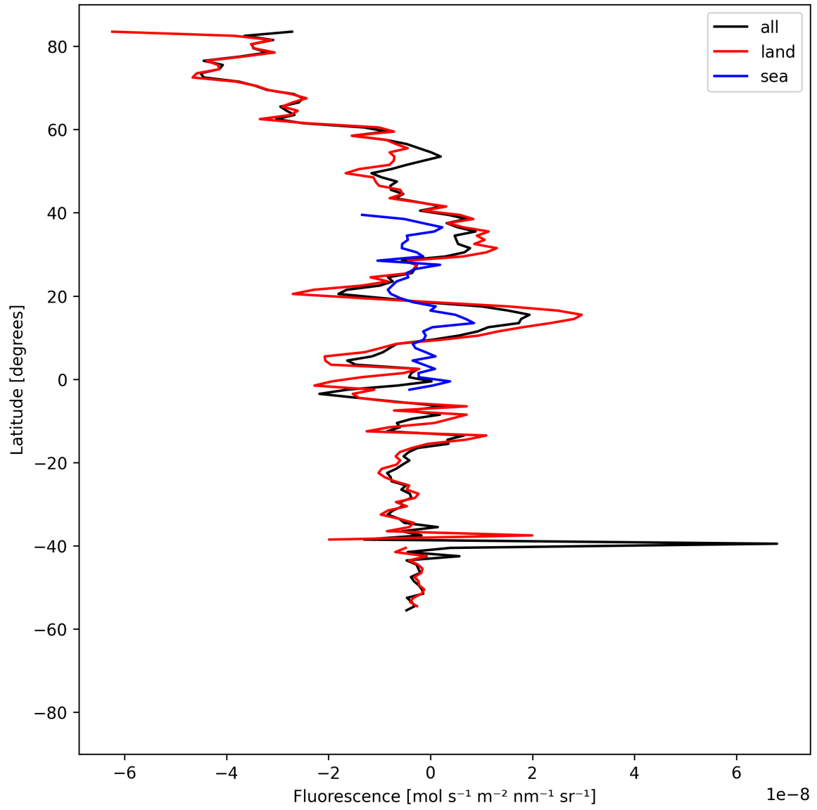
Figure 21: Zonal average of “Fluorescence” for 2025-04-20 to 2025-04-22.
