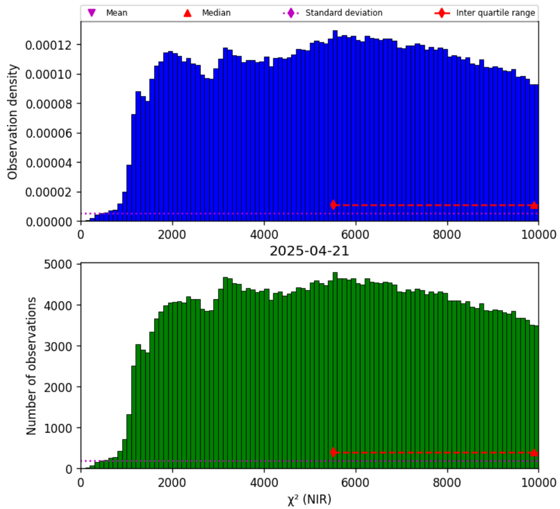
Figure 29: Histogram of “ \chi^2 (NIR)” for 2025-04-20 to 2025-04-22
