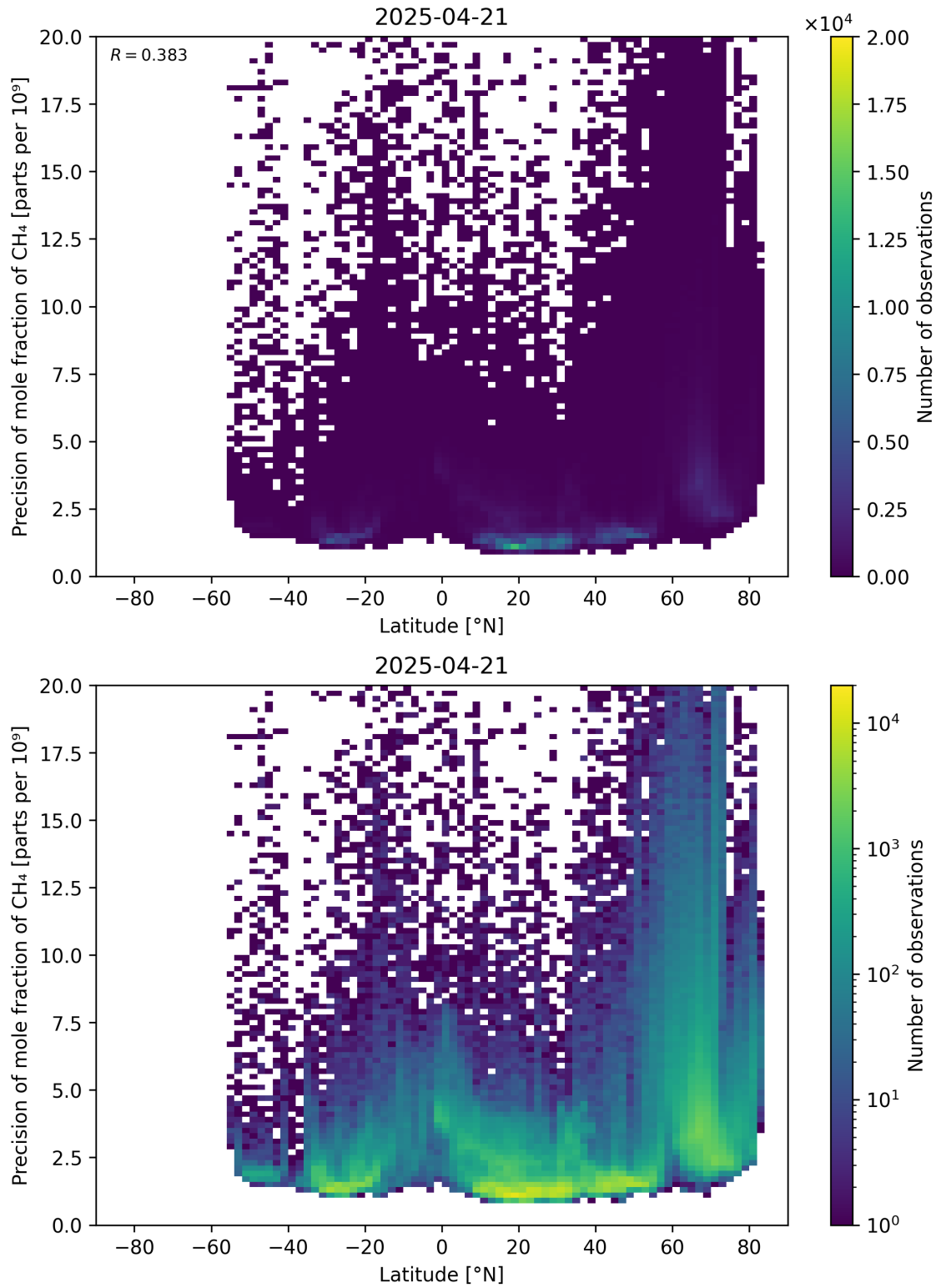
Figure 59: Scatter density plot of “Latitude” against “Precision of mole fraction of \text{CH}_4 ” for 2025-04-20 to 2025-04-22.
