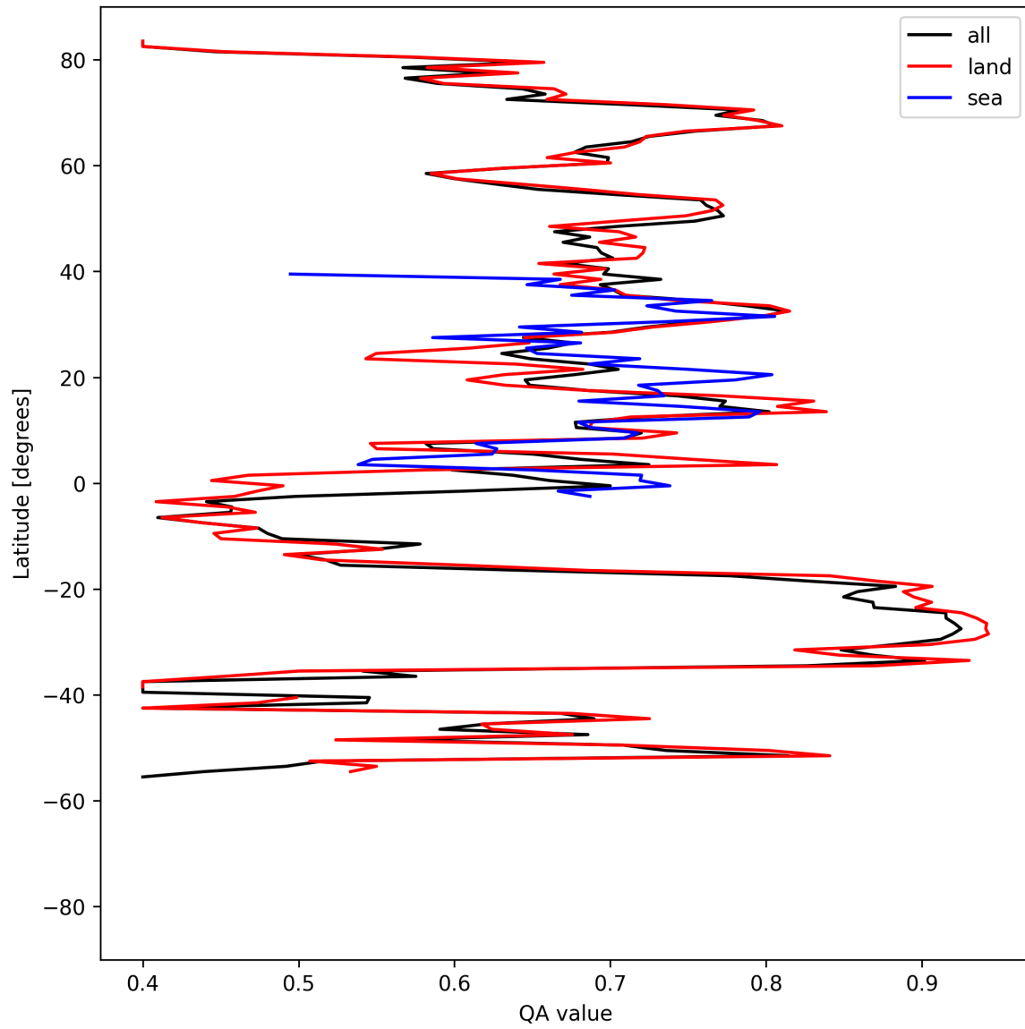
Figure 11: Zonal average of “QA value” for 2025-04-20 to 2025-04-22.
