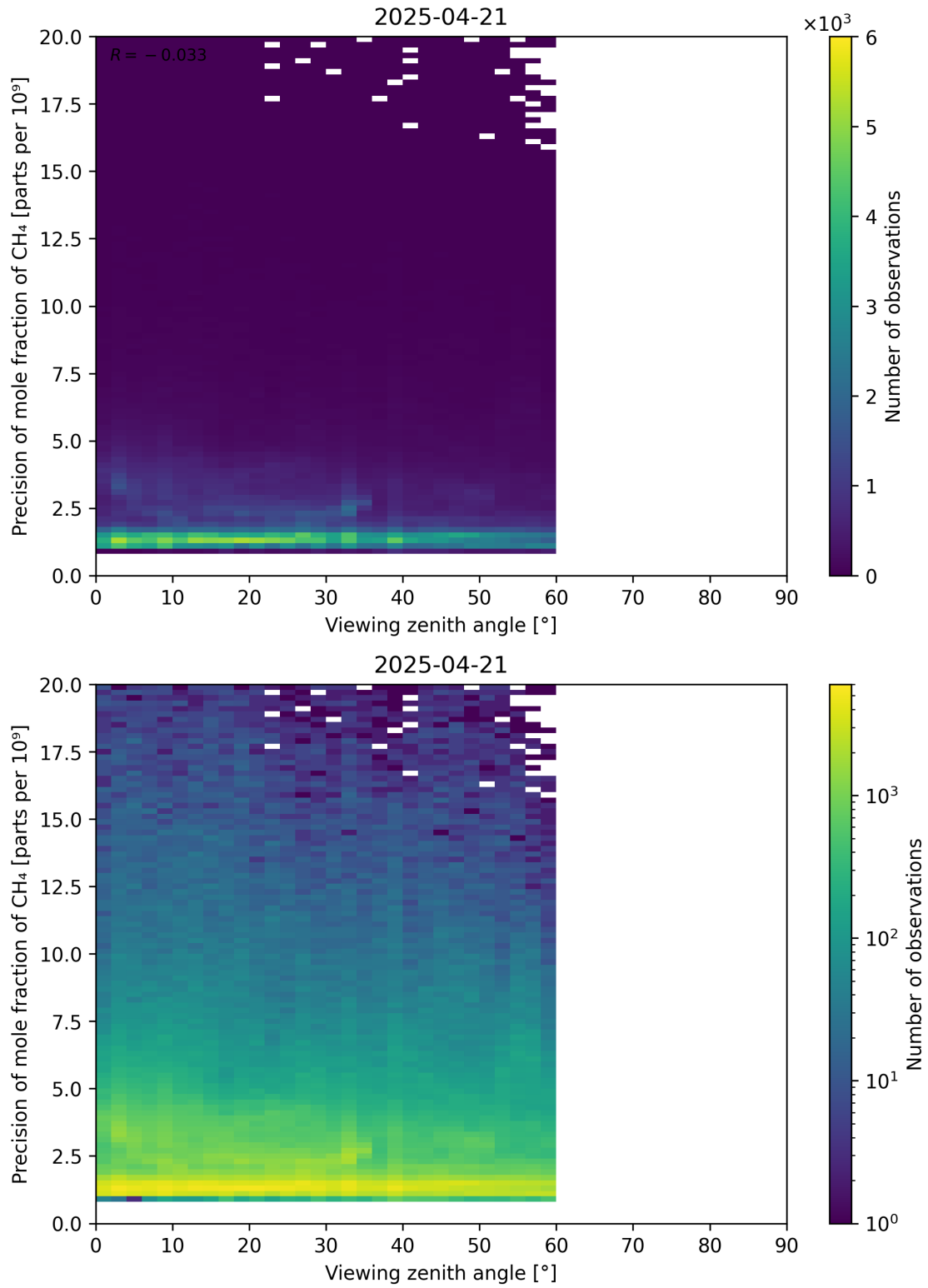
Figure 112: Scatter density plot of “Viewing zenith angle” against “Precision of mole fraction of \text{CH}_4 ” for 2025-04-20 to 2025-04-22.
