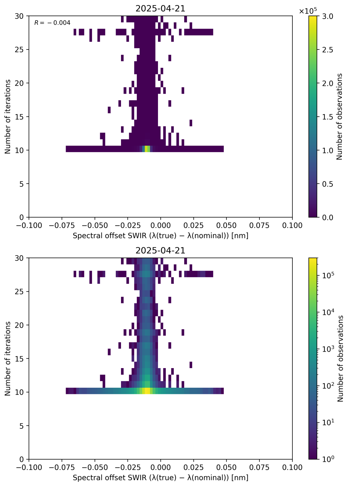
Figure 121: Scatter density plot of “Spectral offset SWIR ( \lambda_{\text{true}} - \lambda_{\text{nominal}} )” against “Number of iterations” for 2025-04-20 to 2025-04-22.
