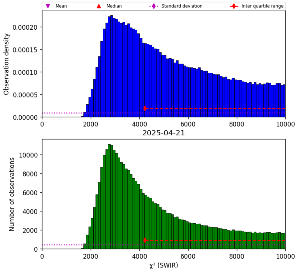
Figure 28: Histogram of “ \chi^2 (SWIR)” for 2025-04-20 to 2025-04-22
