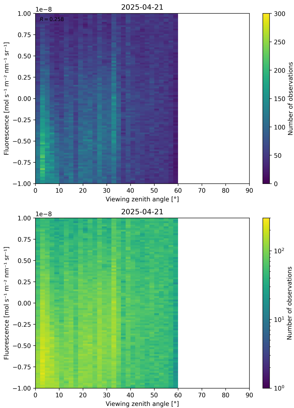
Figure 108: Scatter density plot of “Viewing zenith angle” against “Fluorescence” for 2025-04-20 to 2025-04-22.
