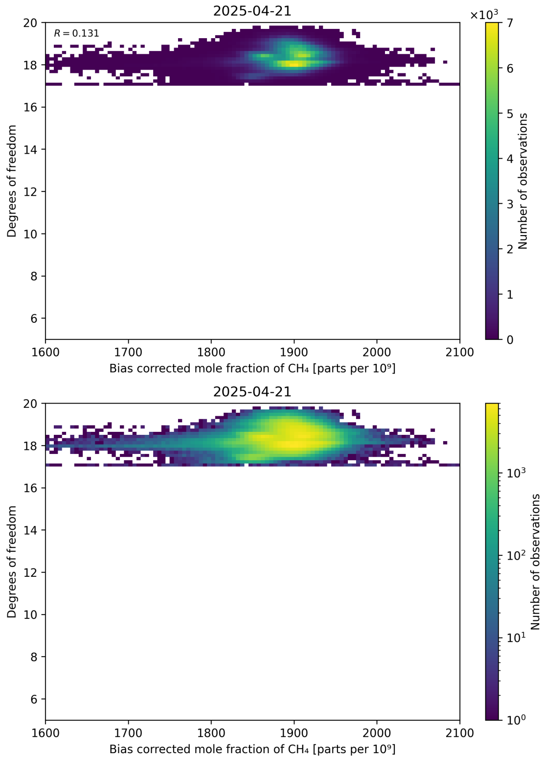
Figure 65: Scatter density plot of “Bias corrected mole fraction of CH 4 ” against “Degrees of freedom” for 2025-04-20 to 2025-04-22.
