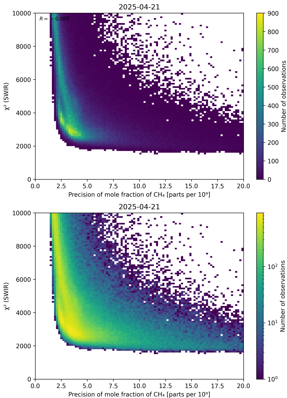
Figure 79: Scatter density plot of “Precision of mole fraction of \text{CH}_4 ” against “ \chi^2 (SWIR)” for 2025-04-20 to 2025-04-22.
