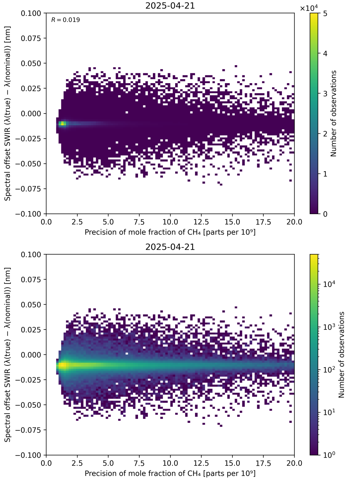
Figure 85: Scatter density plot of “Precision of mole fraction of \text{CH}_4 ” against “Spectral offset SWIR ( \lambda_{\text{true}} - \lambda_{\text{nominal}} )” for 2025-04-20 to 2025-04-22.
