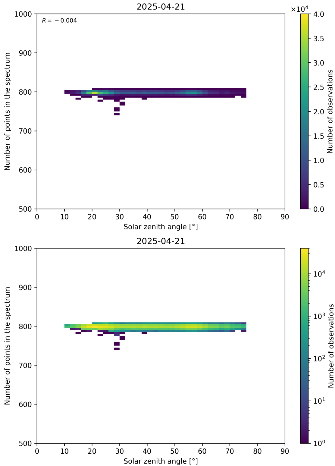
Figure 103: Scatter density plot of “Solar zenith angle” against “Number of points in the spectrum” for 2025-04-20 to 2025-04-22.
