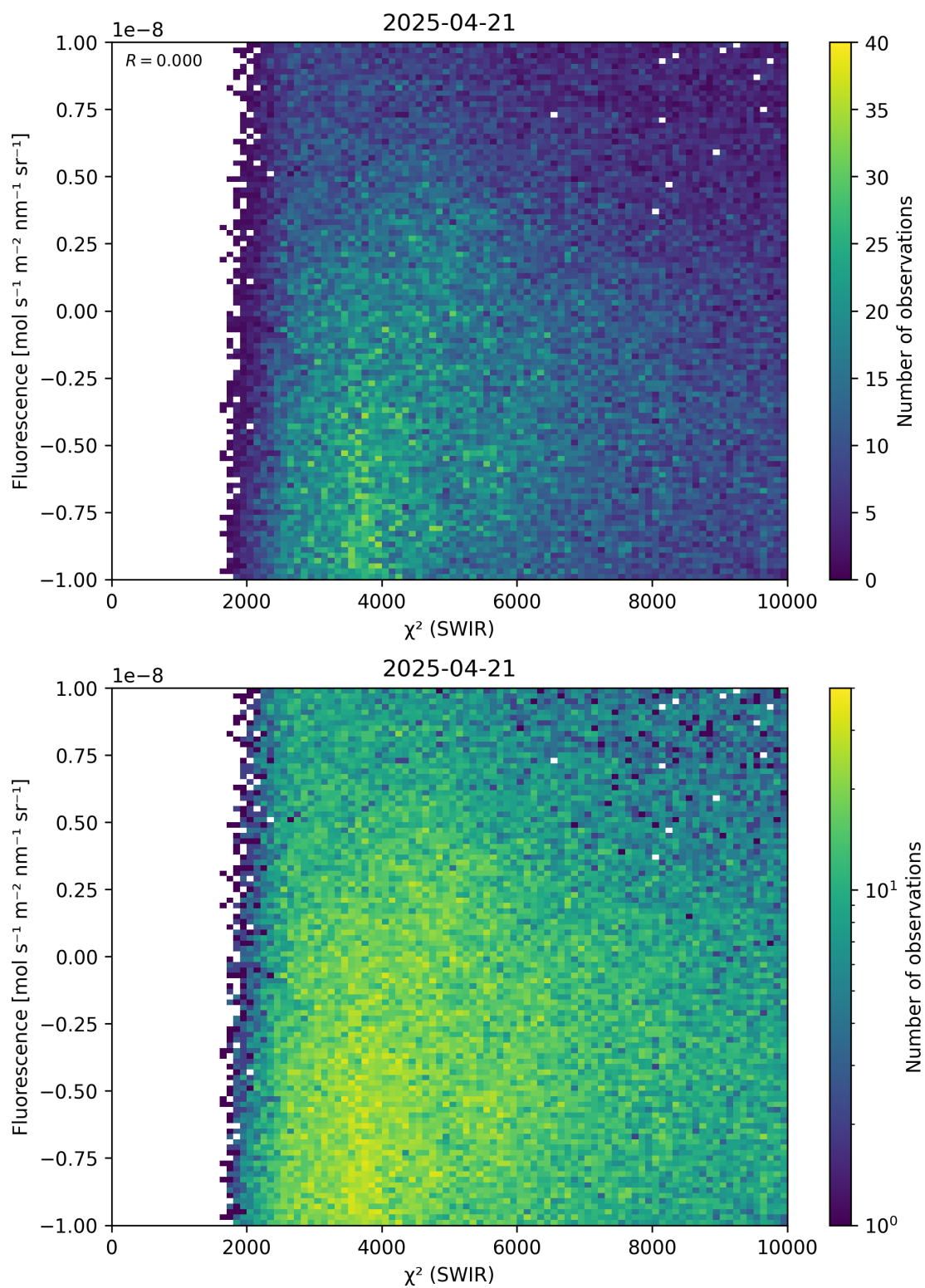
Figure 49: Scatter density plot of “ \chi^2 (SWIR)” against “Fluorescence” for 2025-04-20 to 2025-04-22.
