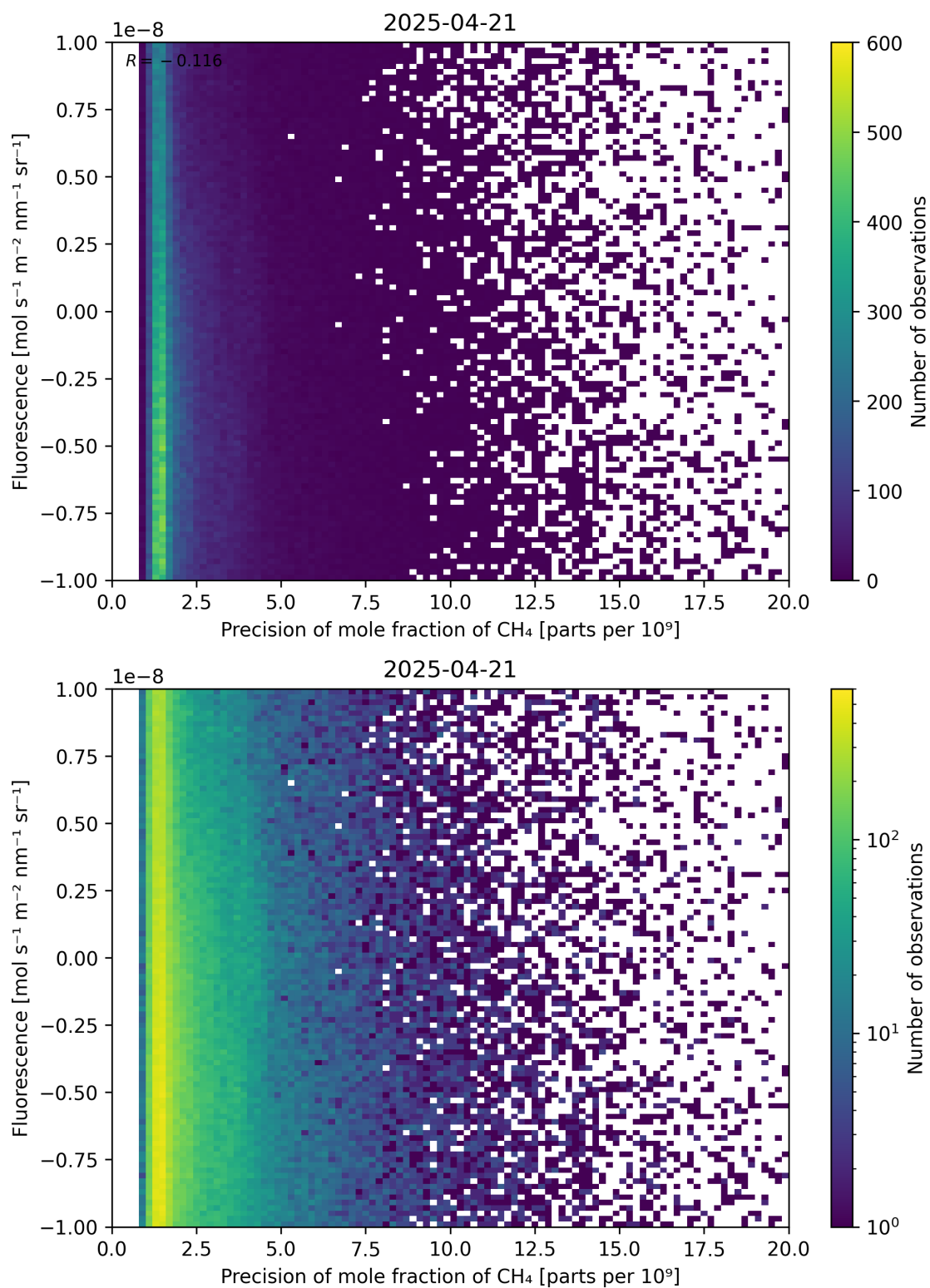
Figure 81: Scatter density plot of “Precision of mole fraction of \text{CH}_4 ” against “Fluorescence” for 2025-04-20 to 2025-04-22.
