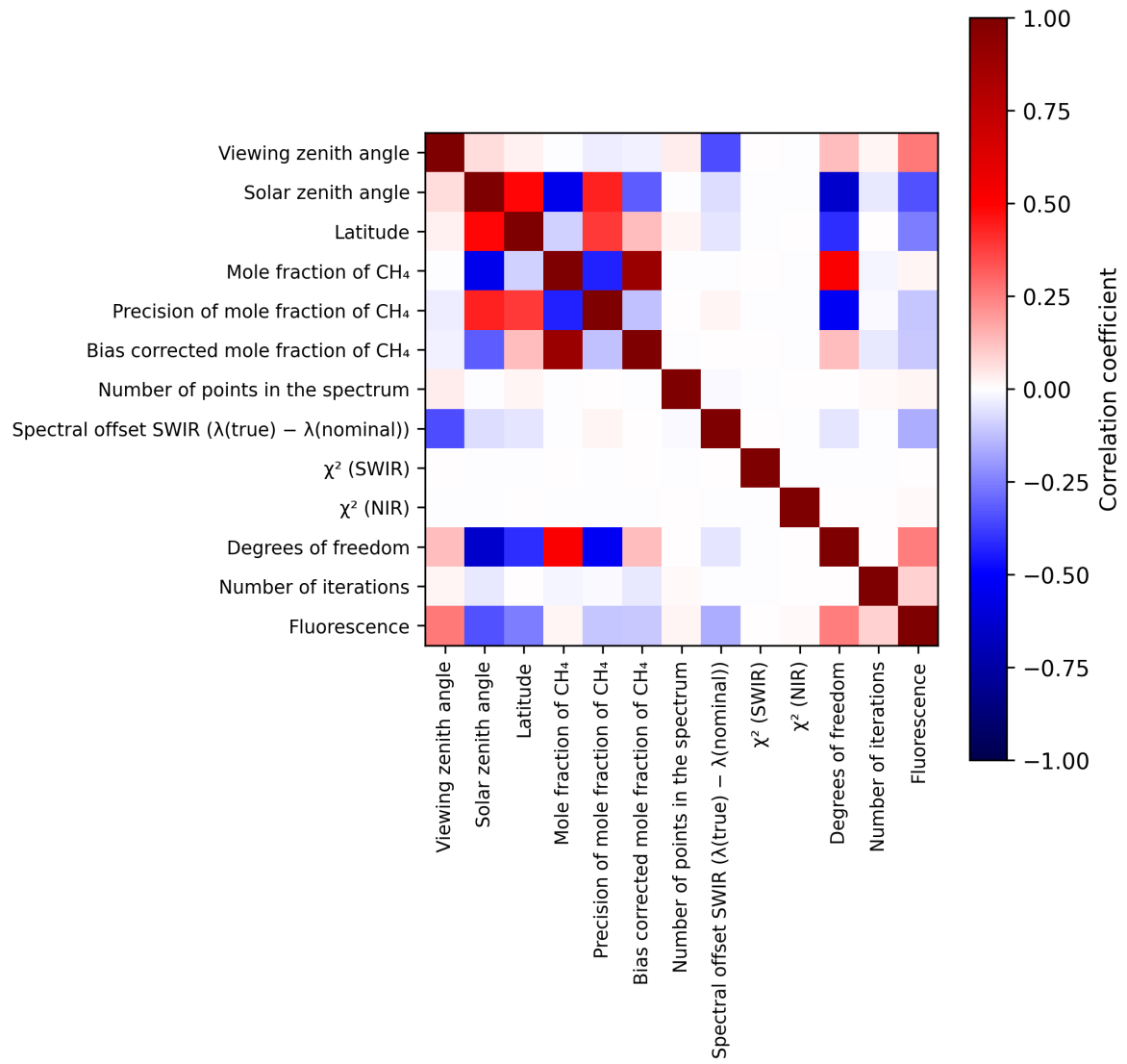
Figure 2: Map of correlation matrix for 2025-04-20 to 2025-04-22.
