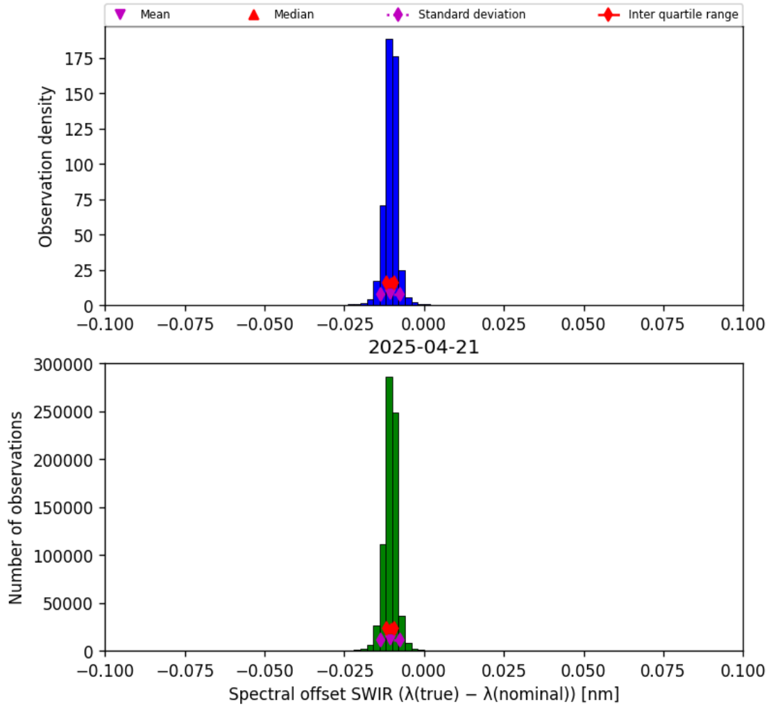
Figure 27: Histogram of “Spectral offset SWIR ( \lambda_{\text{true}} - \lambda_{\text{nominal}} )” for 2025-04-20 to 2025-04-22
