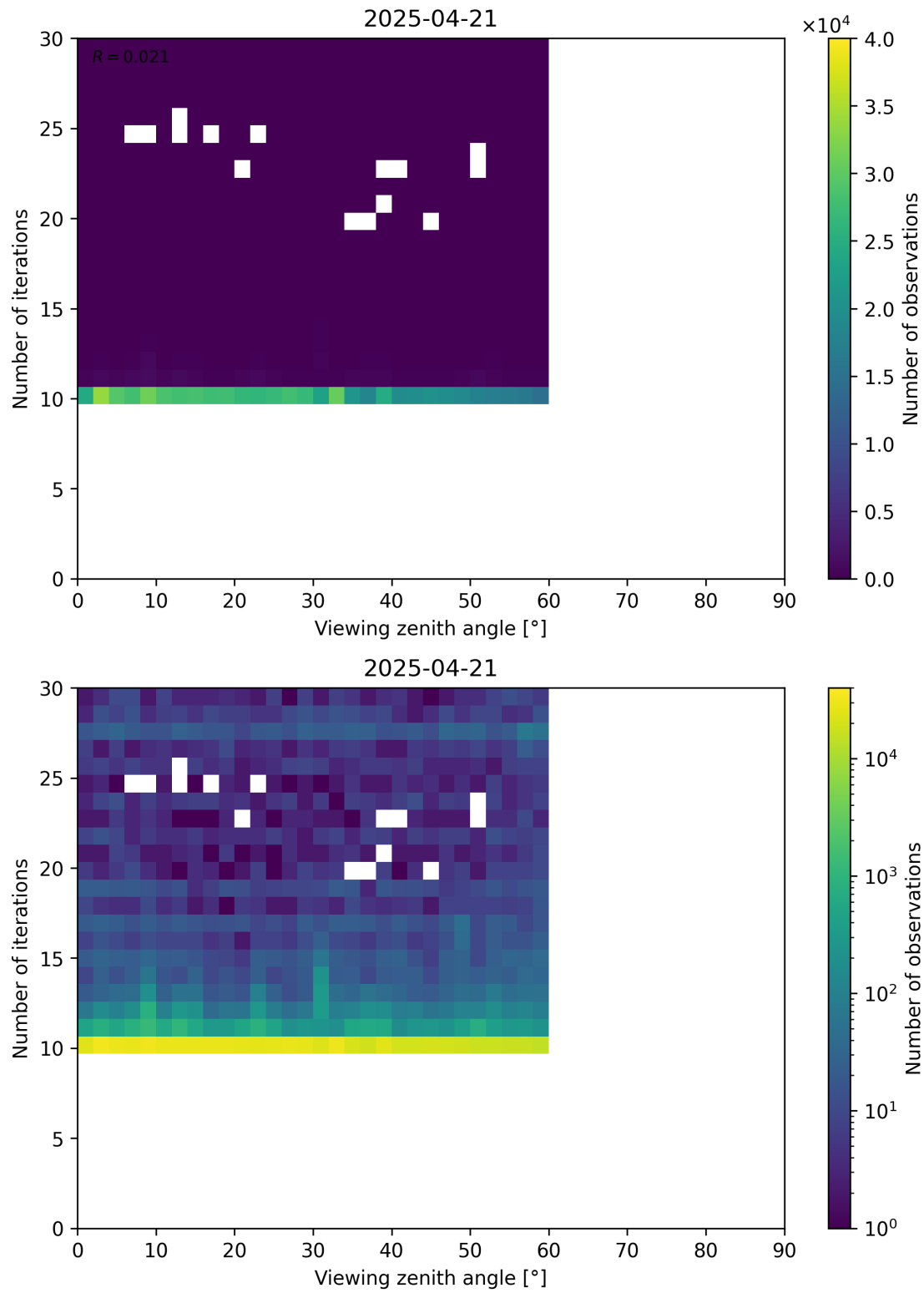
Figure 113: Scatter density plot of “Viewing zenith angle” against “Number of iterations” for 2025-04-20 to 2025-04-22.
