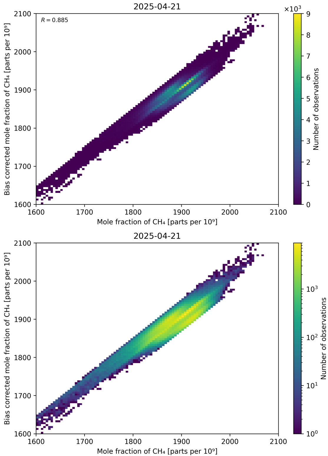
Figure 74: Scatter density plot of “Mole fraction of CH 4 ” against “Bias corrected mole fraction of CH 4 ” for 2025-04-20 to 2025-04-22.
