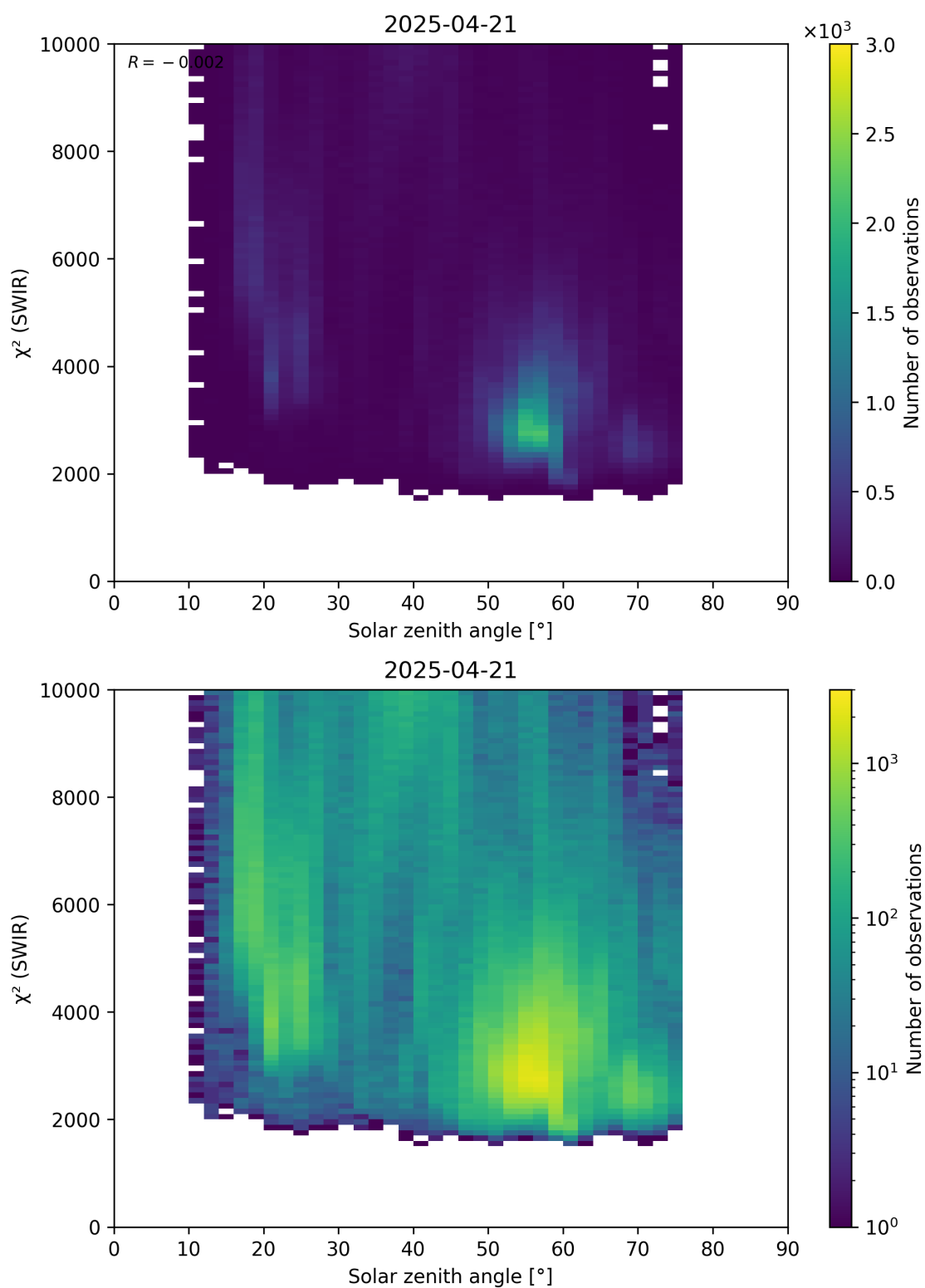
Figure 95: Scatter density plot of “Solar zenith angle” against “ \chi^2 (SWIR)” for 2025-04-20 to 2025-04-22.
