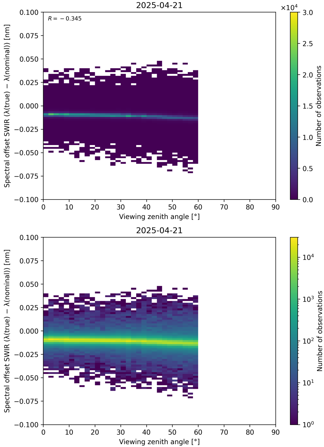
Figure 116: Scatter density plot of “Viewing zenith angle” against “Spectral offset SWIR ( \lambda_{\text{true}} - \lambda_{\text{nominal}} )” for 2025-04-20 to 2025-04-22.
