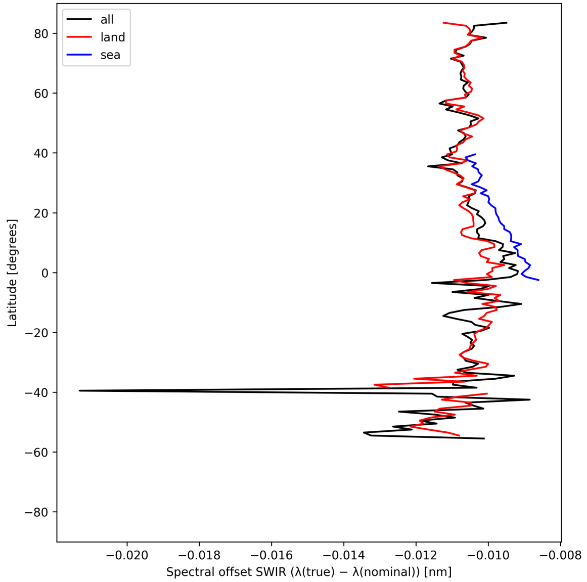
Figure 16: Zonal average of “Spectral offset SWIR ( \lambda_{\text{true}} - \lambda_{\text{nominal}} )” for 2025-04-20 to 2025-04-22.
