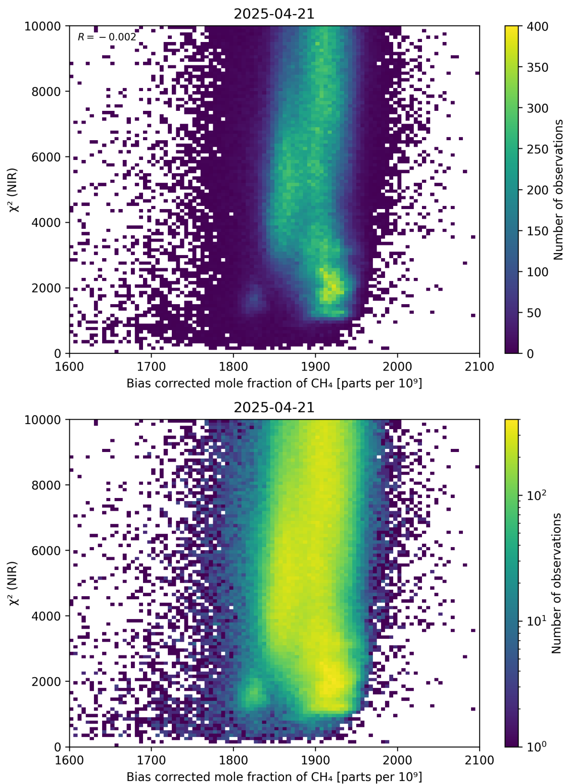
Figure 63: Scatter density plot of “Bias corrected mole fraction of CH 4 ” against “ \chi^2 (NIR)” for 2025-04-20 to 2025-04-22.
