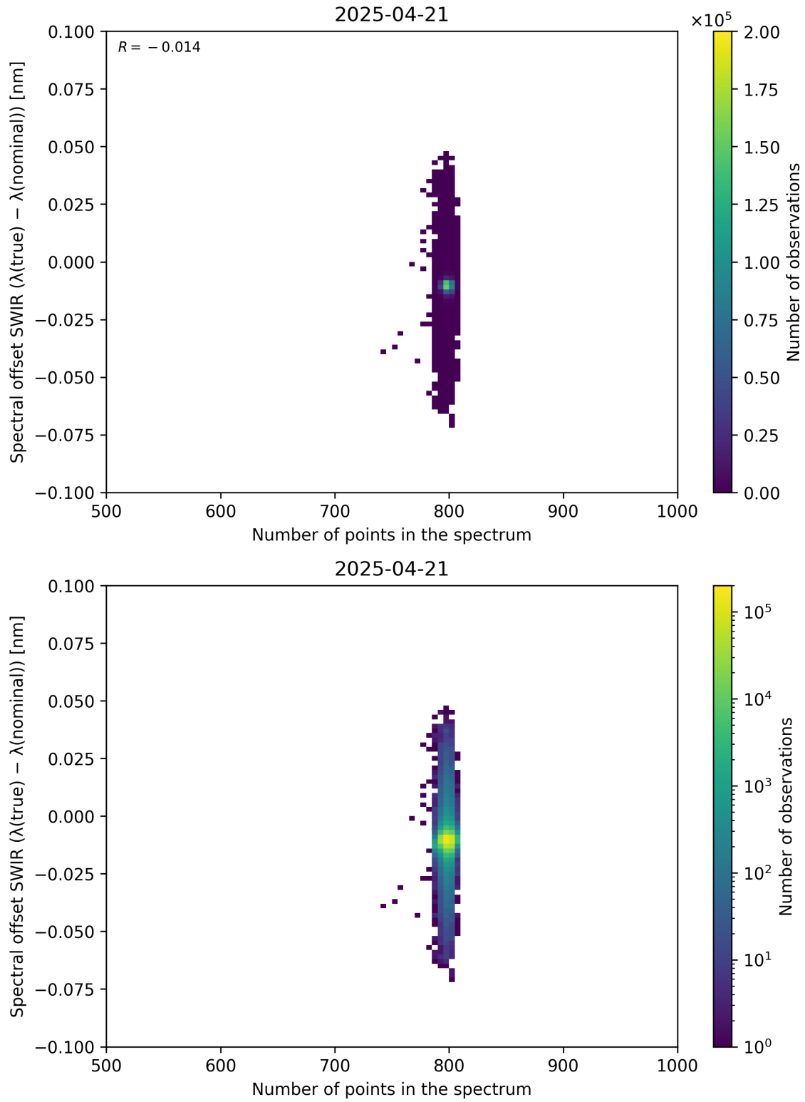
Figure 93: Scatter density plot of “Number of points in the spectrum” against “Spectral offset SWIR ( \lambda_{\text{true}} - \lambda_{\text{nominal}} )” for 2025-04-20 to 2025-04-22.
