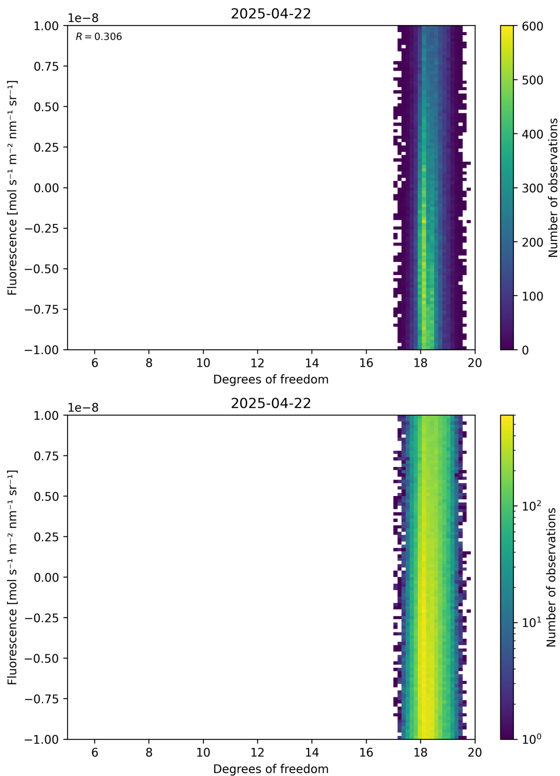
Figure 51: Scatter density plot of “Degrees of freedom” against “Fluorescence” for 2025-04-21 to 2025-04-23.
