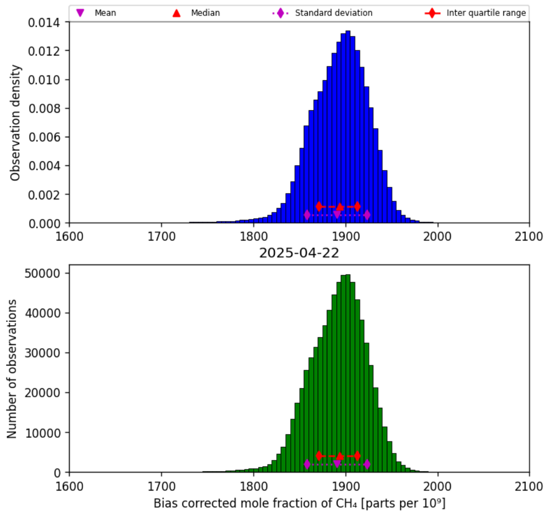
Figure 25: Histogram of “Bias corrected mole fraction of CH 4 ” for 2025-04-21 to 2025-04-23
