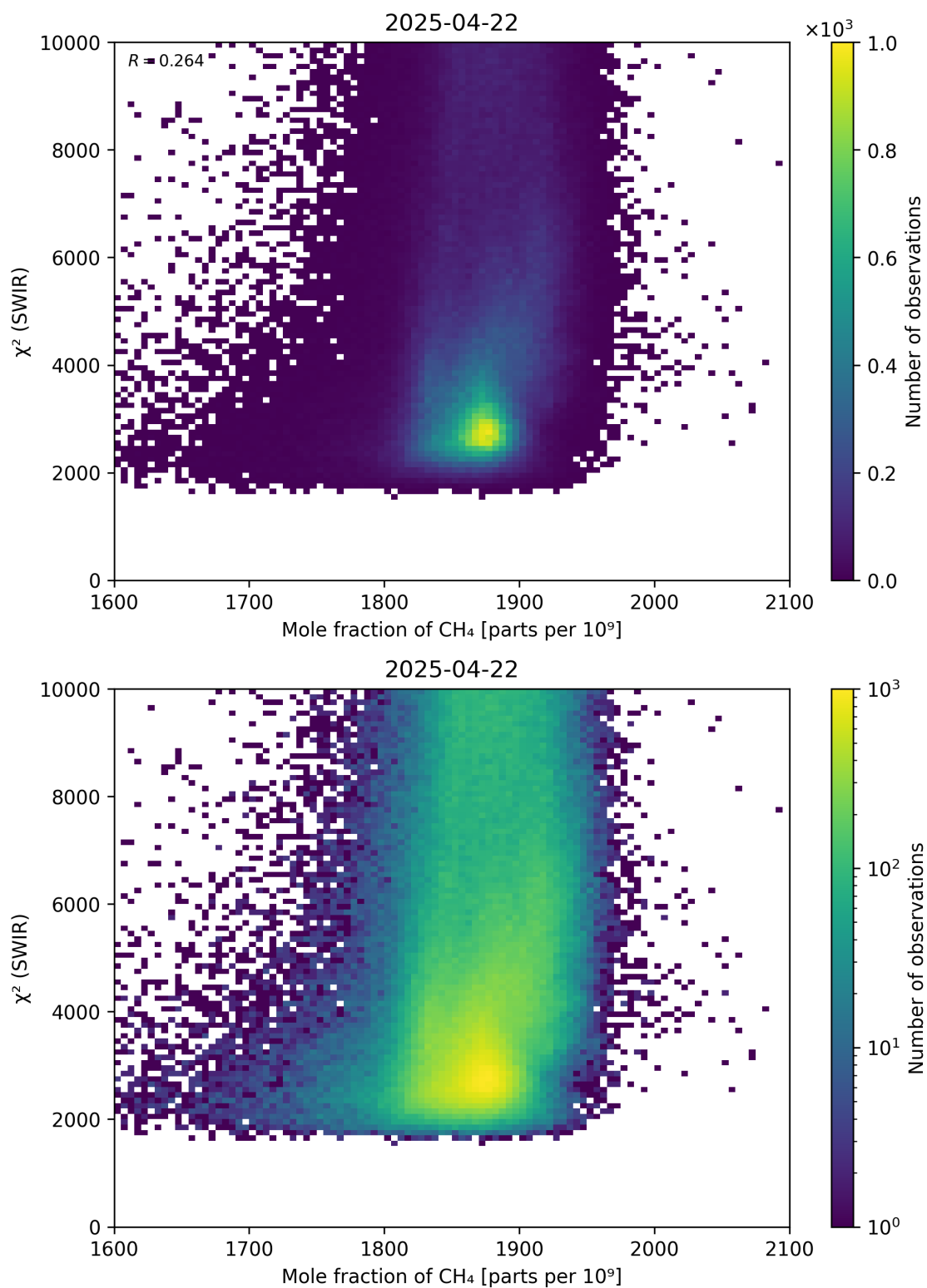
Figure 71: Scatter density plot of “Mole fraction of \text{CH}_4 ” against “ \chi^2 (SWIR)” for 2025-04-21 to 2025-04-23.
