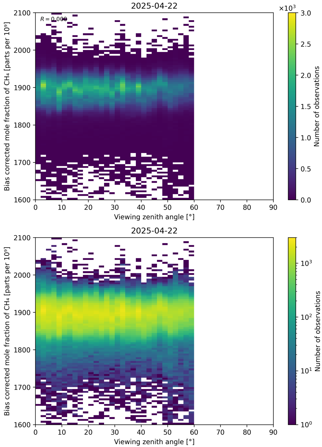
Figure 111: Scatter density plot of “Viewing zenith angle” against “Bias corrected mole fraction of CH 4 ” for 2025-04-21 to 2025-04-23.
