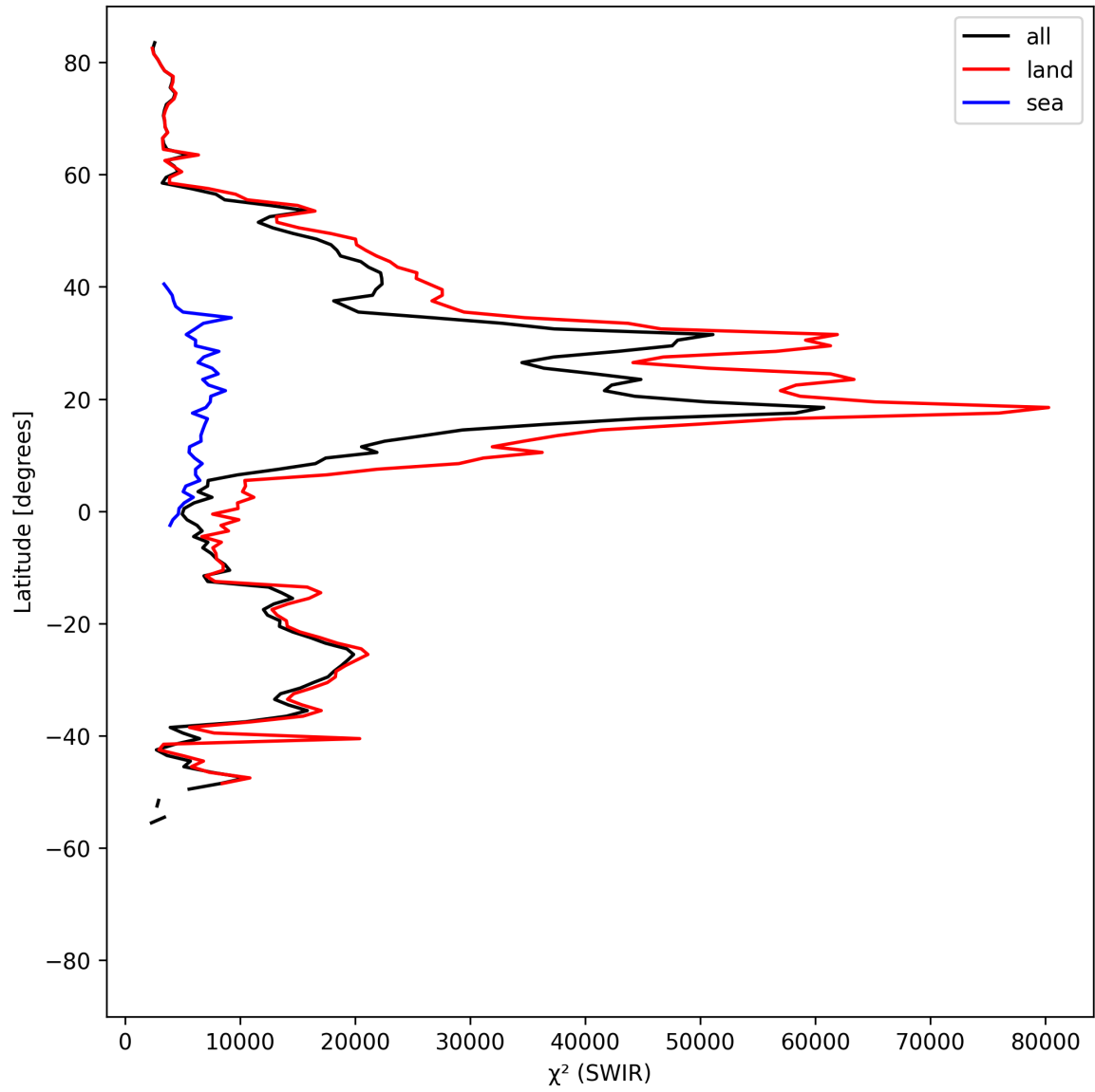
Figure 17: Zonal average of “ \chi^2 (SWIR)” for 2025-04-21 to 2025-04-23.
