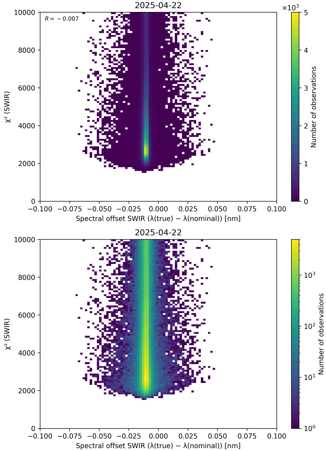
Figure 118: Scatter density plot of “Spectral offset SWIR ( \lambda_{\text{true}} - \lambda_{\text{nominal}} )” against “ \chi^2 (SWIR)” for 2025-04-21 to 2025-04-23.
