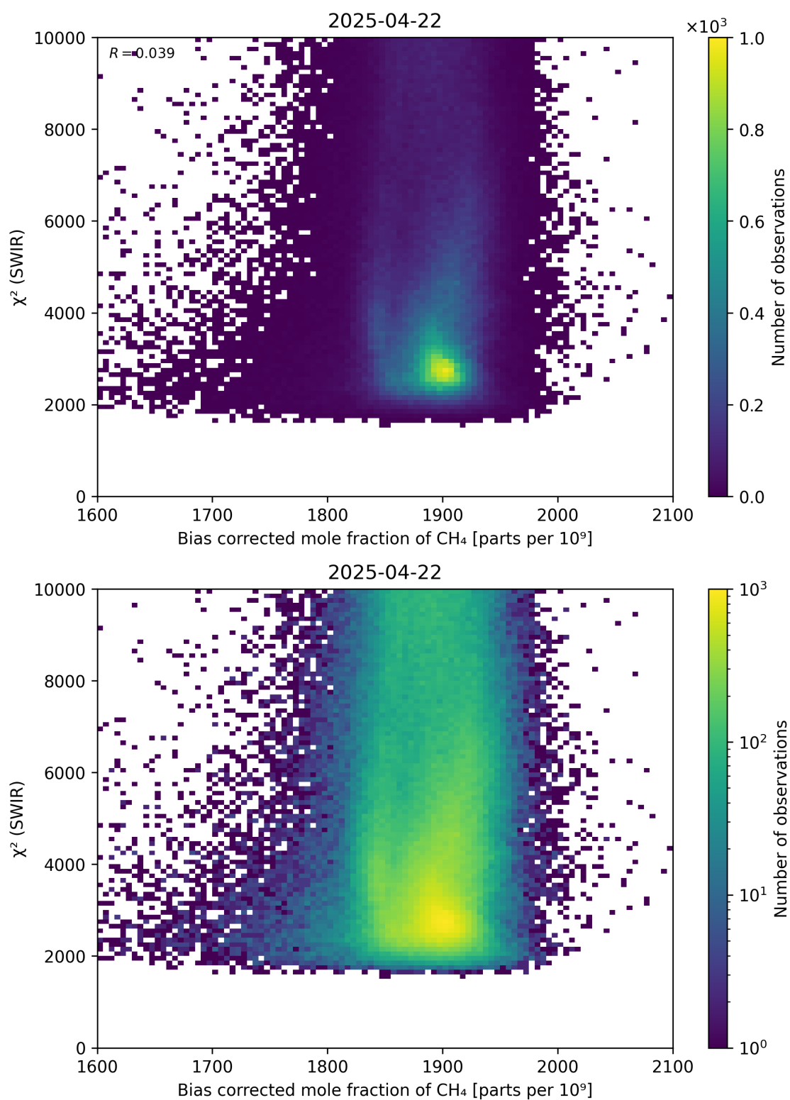
Figure 64: Scatter density plot of “Bias corrected mole fraction of \text{CH}_4 ” against “ \chi^2 (SWIR)” for 2025-04-21 to 2025-04-23.
