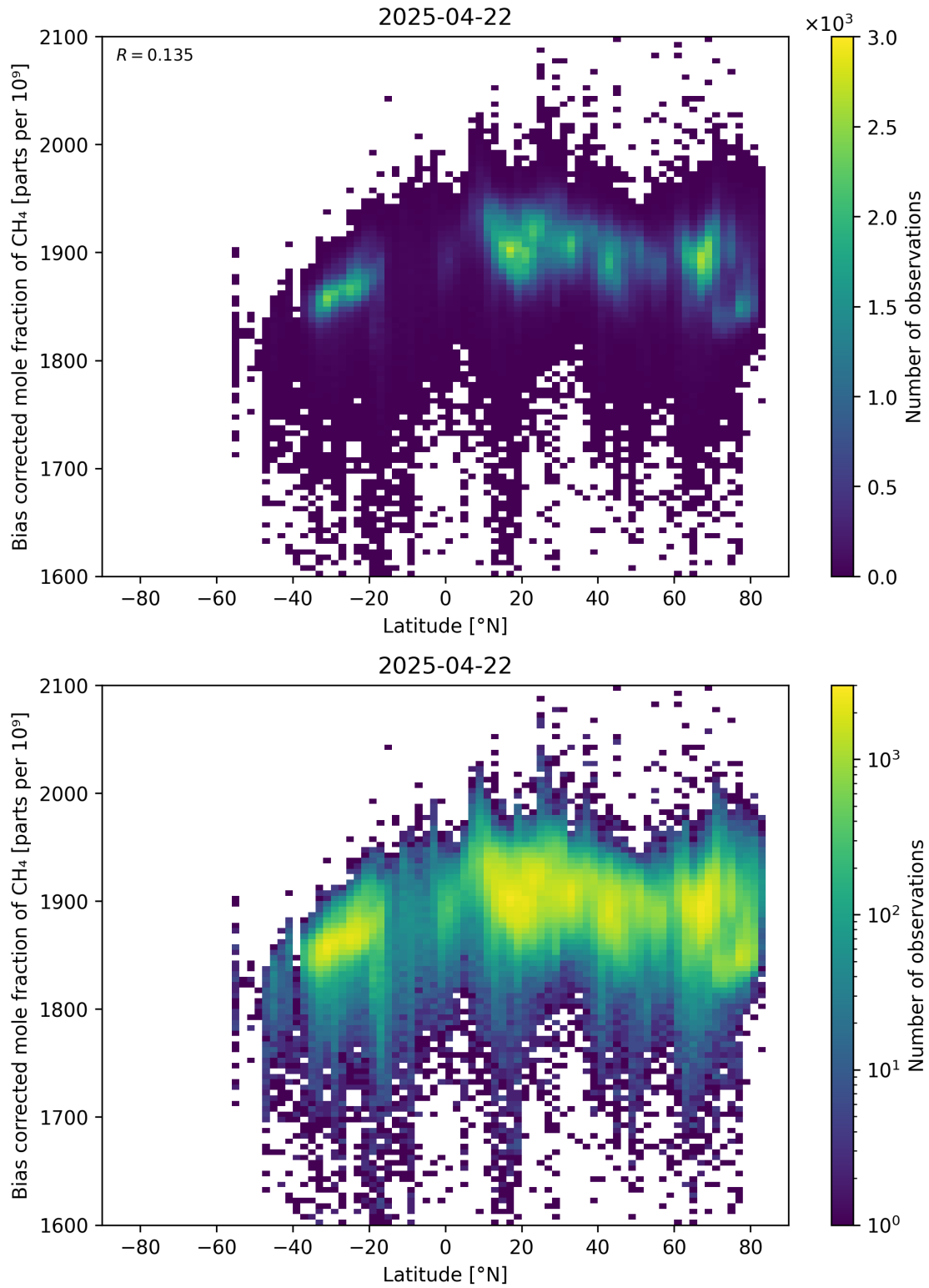
Figure 58: Scatter density plot of “Latitude” against “Bias corrected mole fraction of \text{CH}_4 ” for 2025-04-21 to 2025-04-23.
