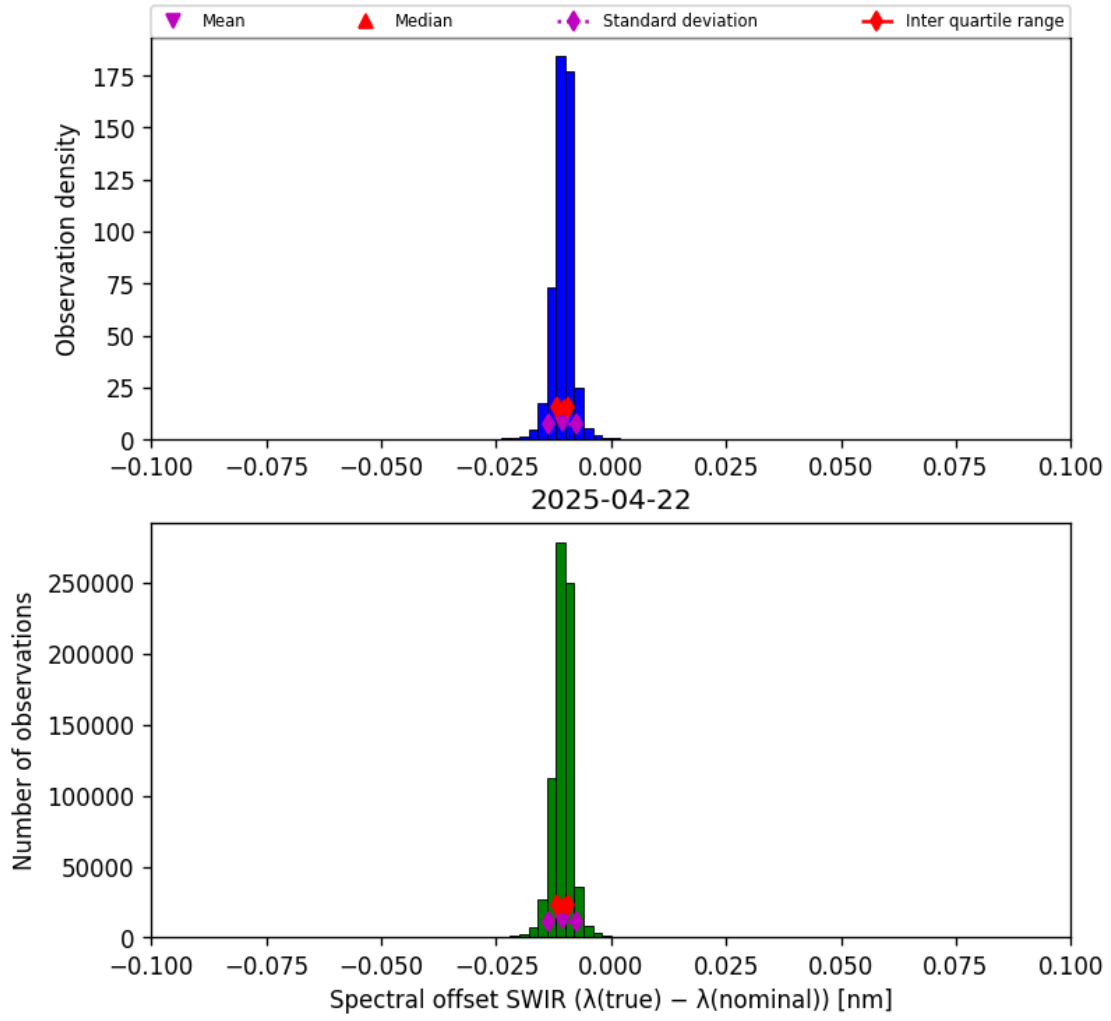
Figure 27: Histogram of “Spectral offset SWIR ( \lambda_{\text{true}} - \lambda_{\text{nominal}} )” for 2025-04-21 to 2025-04-23
