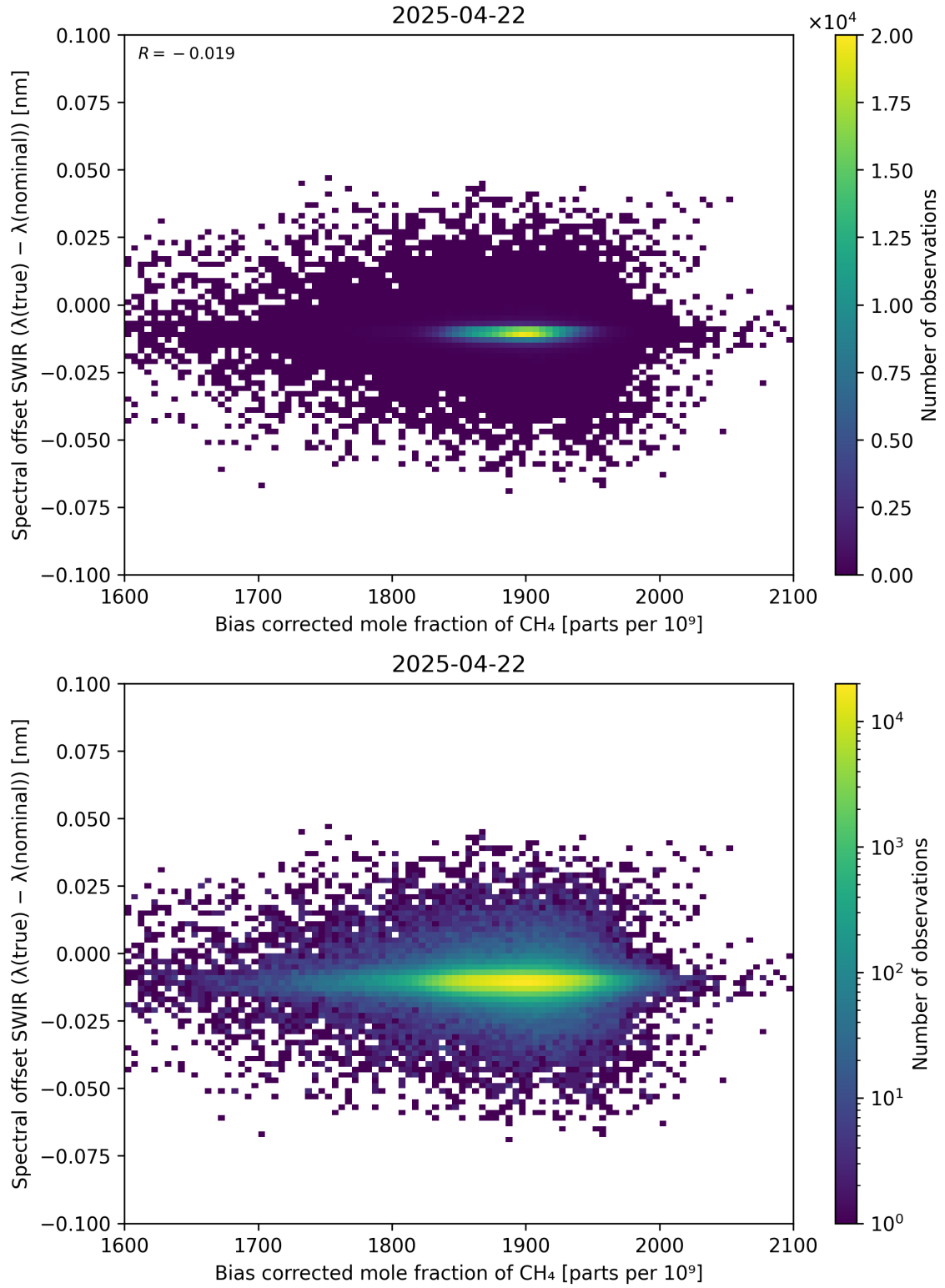
Figure 69: Scatter density plot of “Bias corrected mole fraction of \text{CH}_4 ” against “Spectral offset SWIR ( \lambda_{\text{true}} - \lambda_{\text{nominal}} )” for 2025-04-21 to 2025-04-23.
