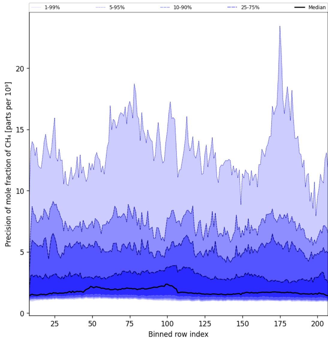
Figure 35: Along track statistics of “Precision of mole fraction of CH 4 ” for 2025-04-21 to 2025-04-23
