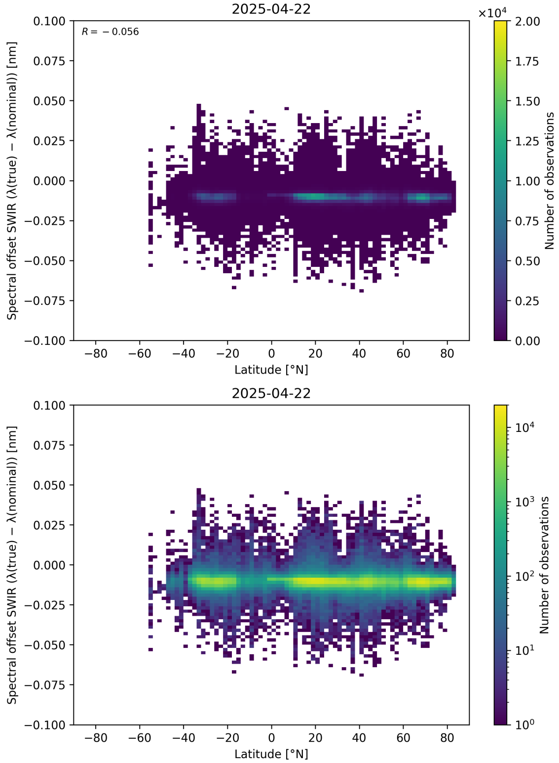
Figure 62: Scatter density plot of “Latitude” against “Spectral offset SWIR ( \lambda_{\text{true}} - \lambda_{\text{nominal}} )” for 2025-04-21 to 2025-04-23.
