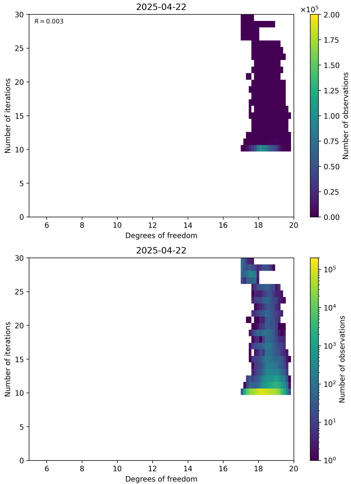
Figure 52: Scatter density plot of “Degrees of freedom” against “Number of iterations” for 2025-04-21 to 2025-04-23.
