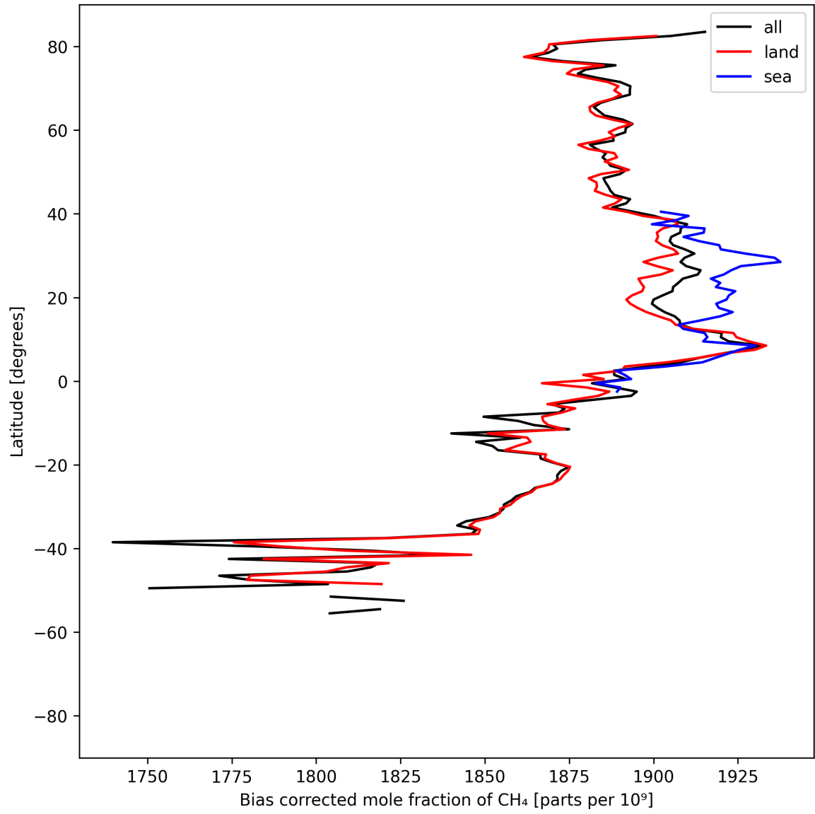
Figure 14: Zonal average of “Bias corrected mole fraction of CH 4 ” for 2025-04-21 to 2025-04-23.
