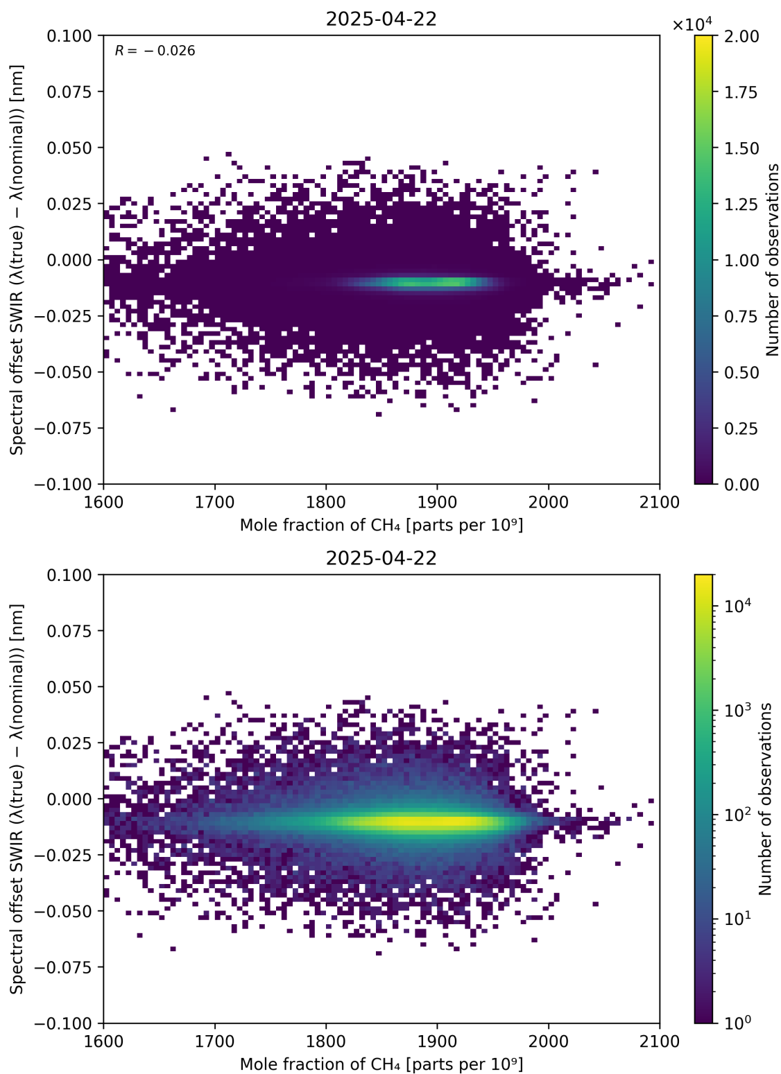
Figure 86: Scatter density plot of “Mole fraction of \text{CH}_4 ” against “Spectral offset SWIR ( \lambda_{\text{true}} - \lambda_{\text{nominal}} )” for 2025-04-21 to 2025-04-23.
