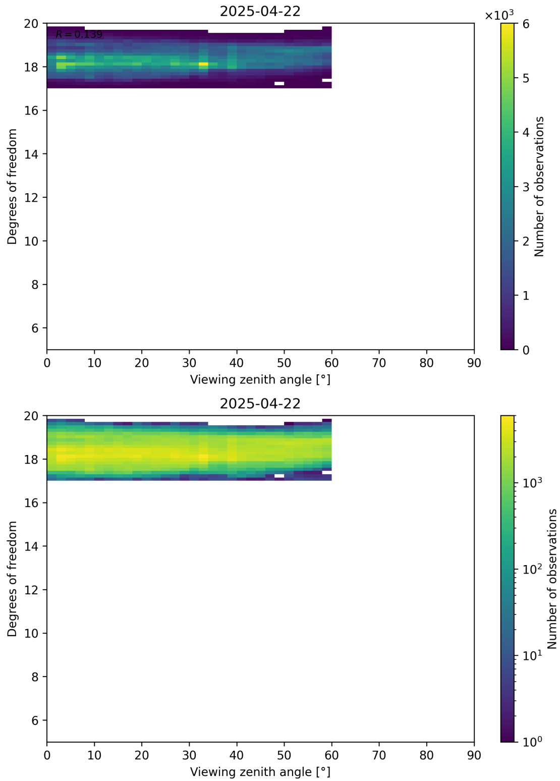
Figure 107: Scatter density plot of “Viewing zenith angle” against “Degrees of freedom” for 2025-04-21 to 2025-04-23.
