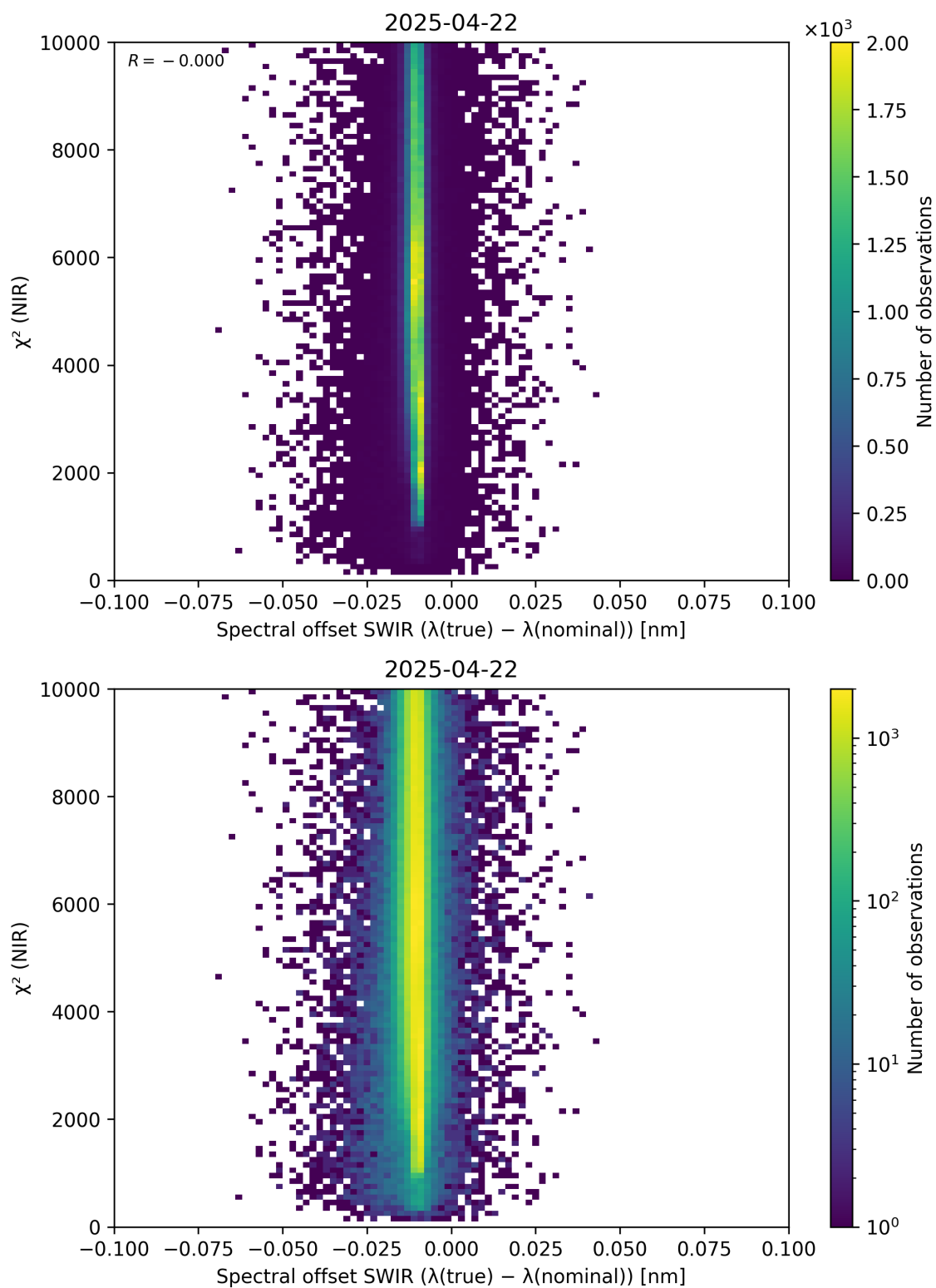
Figure 117: Scatter density plot of “Spectral offset SWIR ( \lambda_{\text{true}} - \lambda_{\text{nominal}} )” against “ \chi^2 (NIR)” for 2025-04-21 to 2025-04-23.
