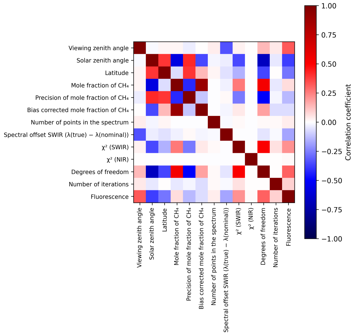
Figure 2: Map of correlation matrix for 2025-04-21 to 2025-04-23.
