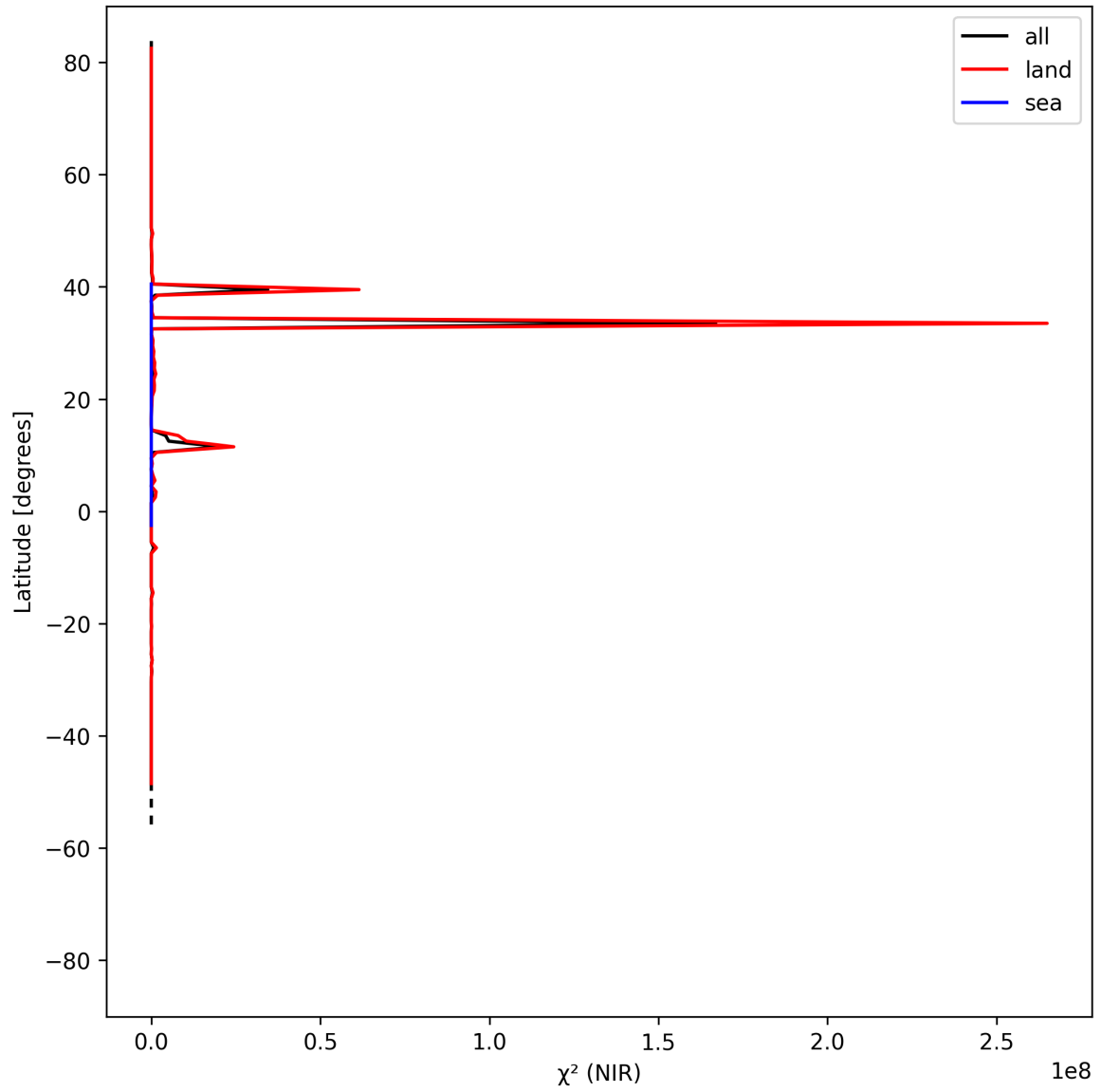
Figure 18: Zonal average of “ \chi^2 (NIR)” for 2025-04-21 to 2025-04-23.
