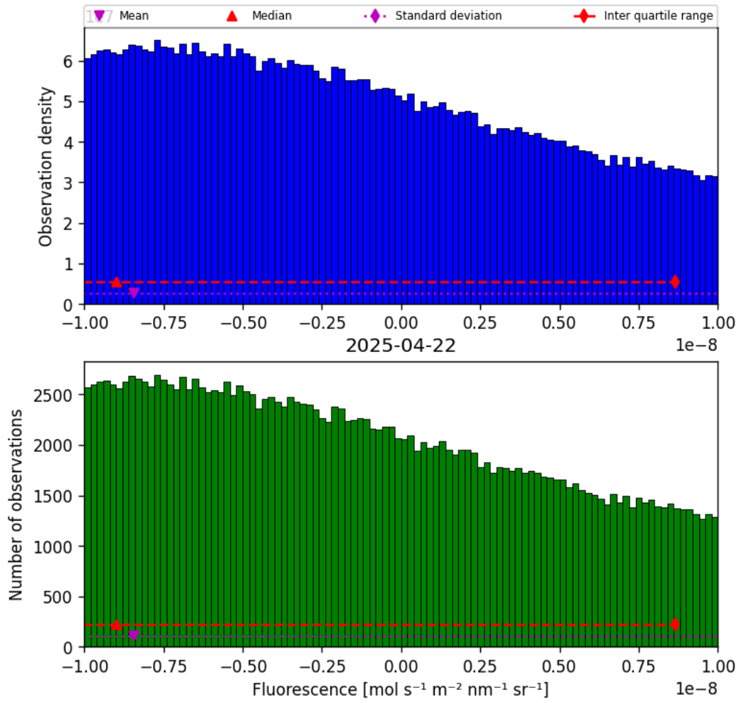
Figure 32: Histogram of “Fluorescence” for 2025-04-21 to 2025-04-23
