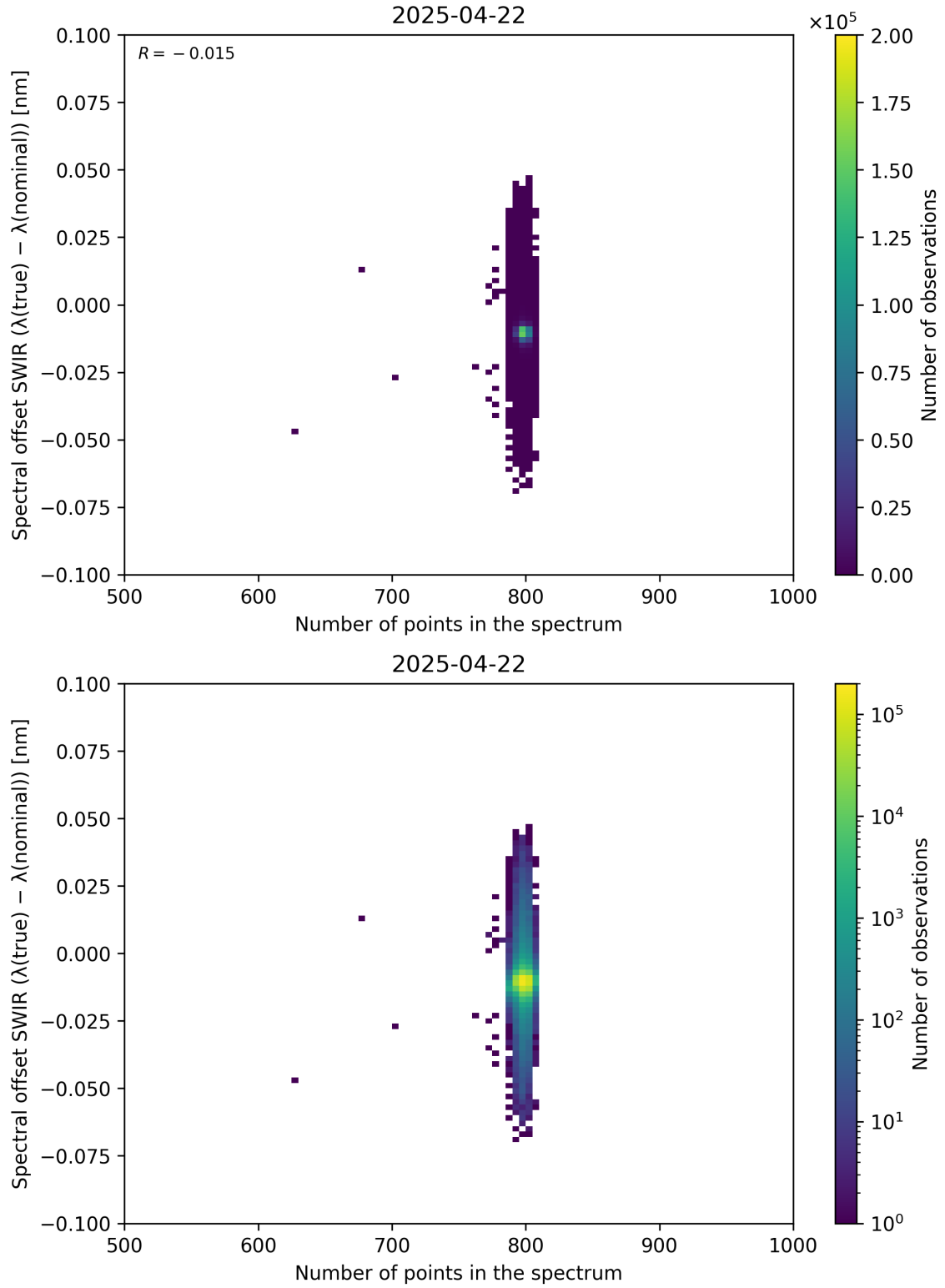
Figure 93: Scatter density plot of “Number of points in the spectrum” against “Spectral offset SWIR ( \lambda_{\text{true}} - \lambda_{\text{nominal}} )” for 2025-04-21 to 2025-04-23.
