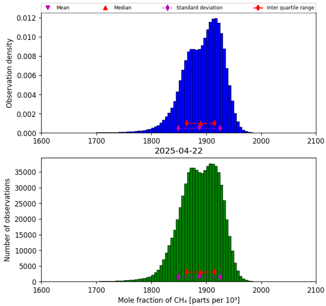
Figure 23: Histogram of “Mole fraction of CH 4 ” for 2025-04-21 to 2025-04-23
