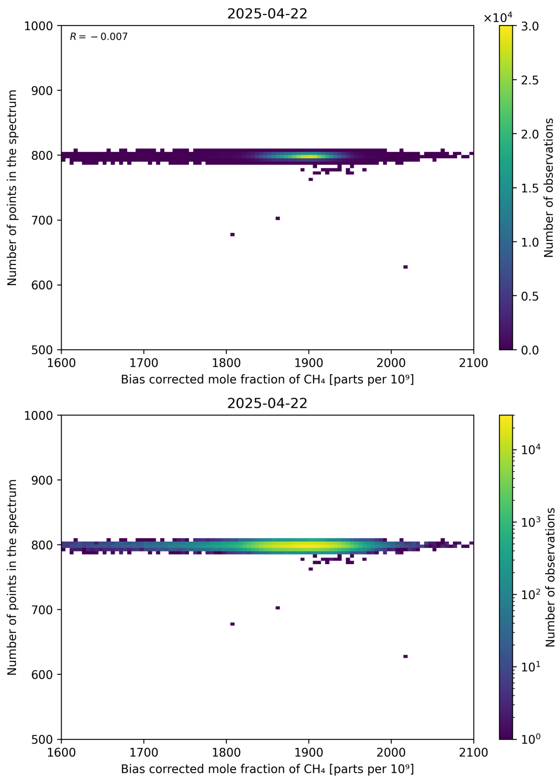
Figure 68: Scatter density plot of “Bias corrected mole fraction of CH 4 ” against “Number of points in the spectrum” for 2025-04-21 to 2025-04-23.
