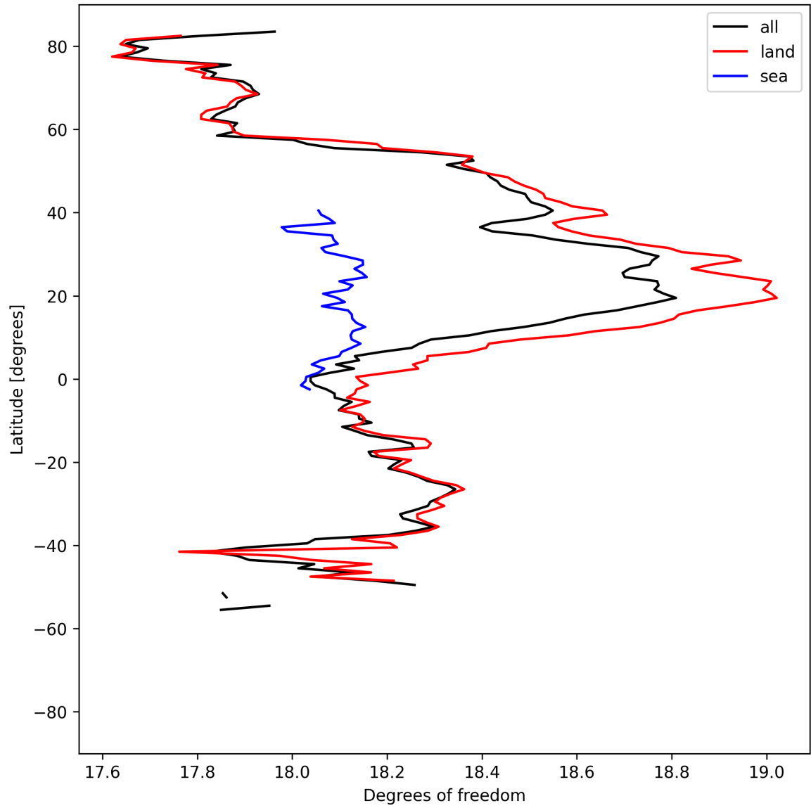
Figure 19: Zonal average of “Degrees of freedom” for 2025-04-21 to 2025-04-23.
