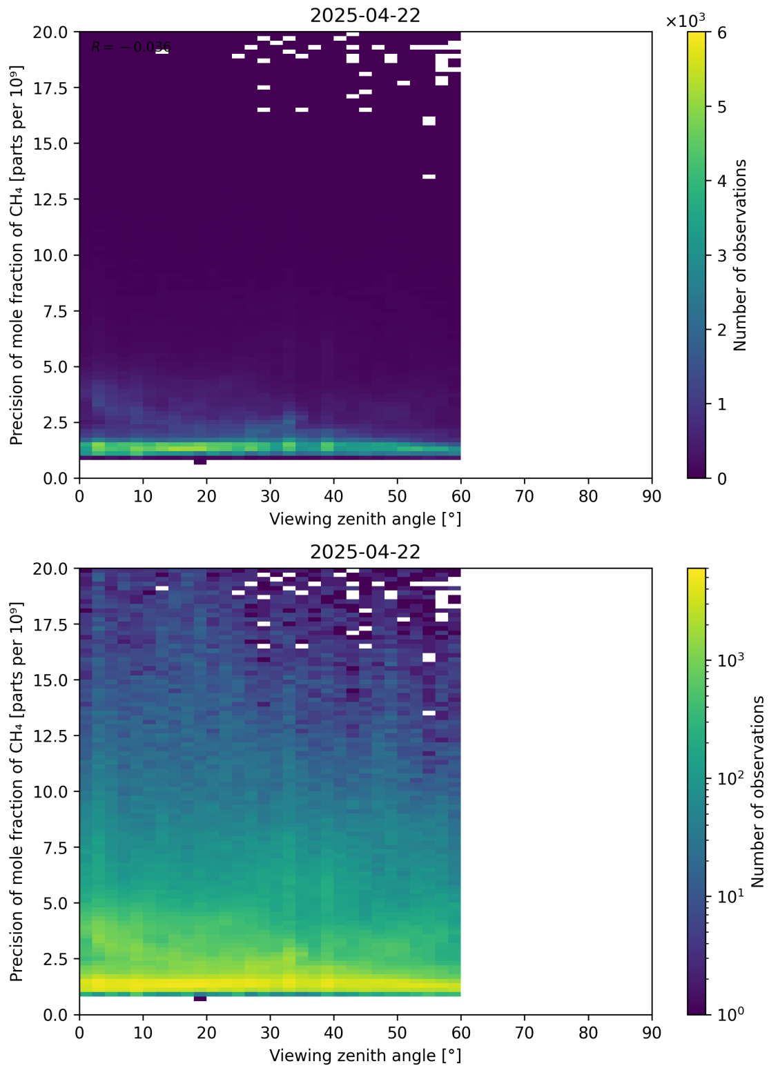
Figure 112: Scatter density plot of “Viewing zenith angle” against “Precision of mole fraction of CH 4 ” for 2025-04-21 to 2025-04-23.
