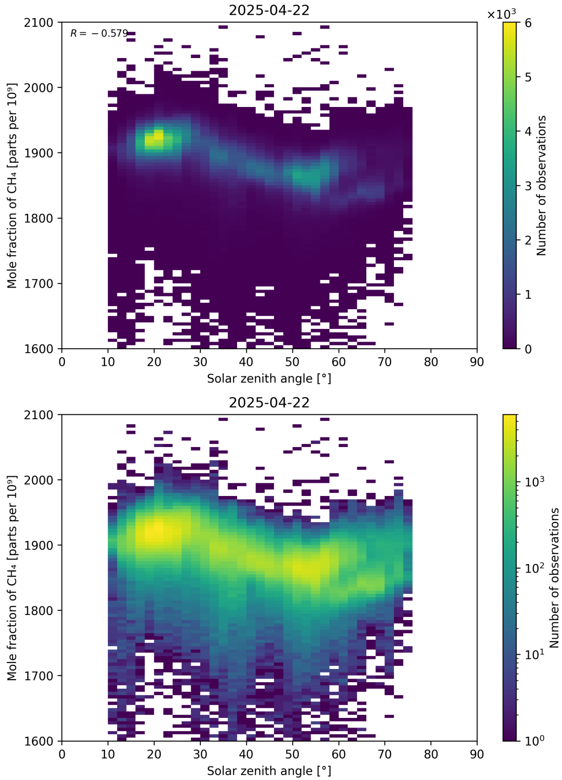
Figure 99: Scatter density plot of “Solar zenith angle” against “Mole fraction of CH 4 ” for 2025-04-21 to 2025-04-23.
