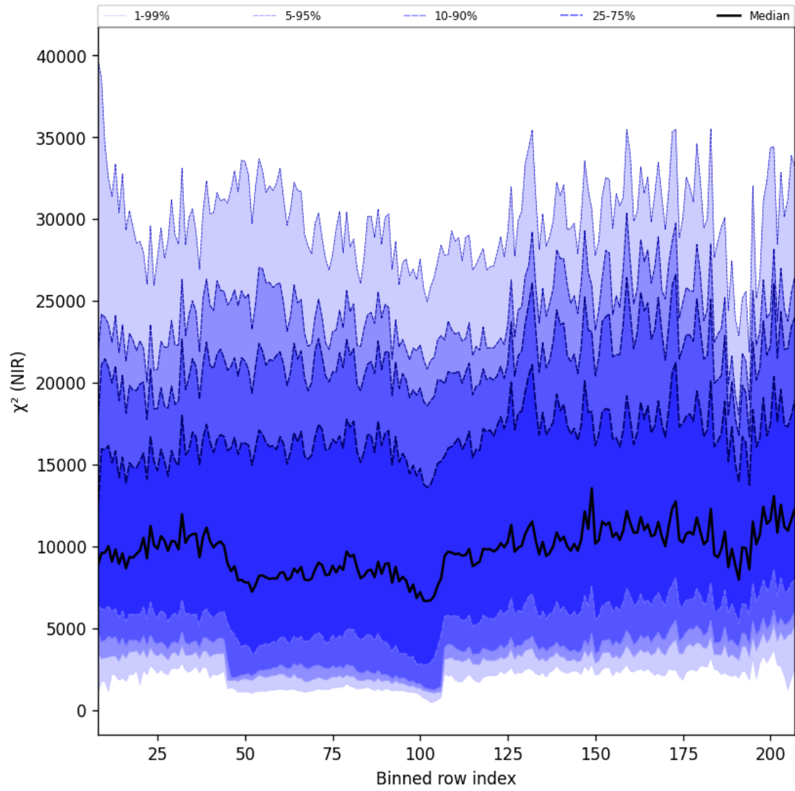
Figure 40: Along track statistics of “ \chi^2 (NIR)” for 2025-04-21 to 2025-04-23
