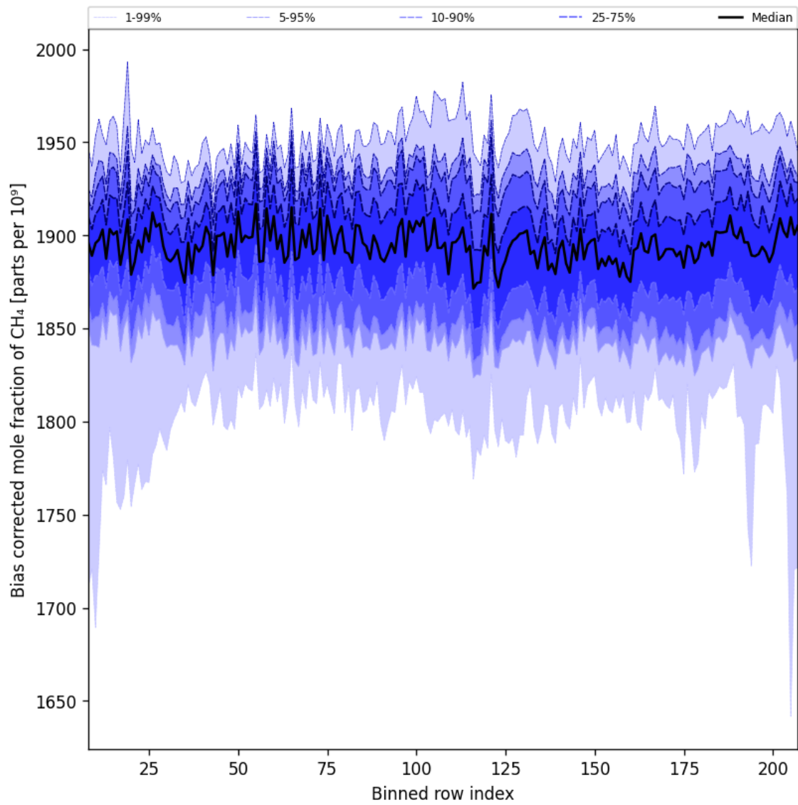
Figure 36: Along track statistics of “Bias corrected mole fraction of CH 4 ” for 2025-04-21 to 2025-04-23
