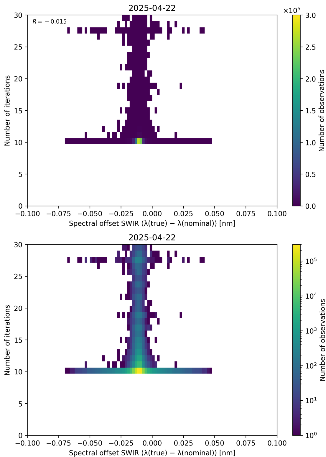
Figure 121: Scatter density plot of “Spectral offset SWIR ( \lambda_{\text{true}} - \lambda_{\text{nominal}} )” against “Number of iterations” for 2025-04-21 to 2025-04-23.
