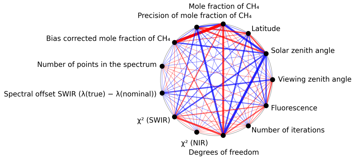
Figure 1: Map of correlation graph for 2025-04-21 to 2025-04-23.
