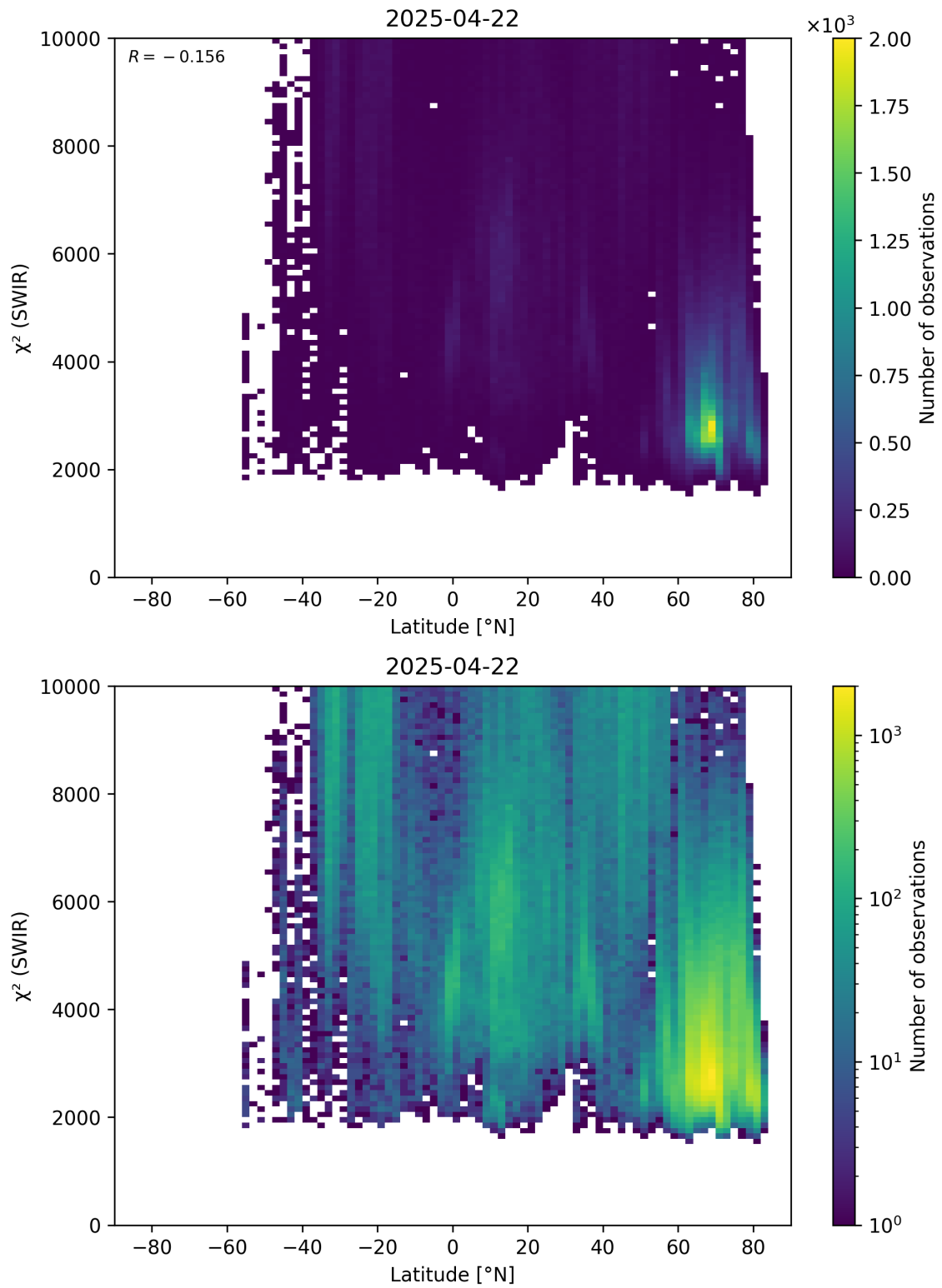
Figure 54: Scatter density plot of “Latitude” against “ \chi^2 (SWIR)” for 2025-04-21 to 2025-04-23.
