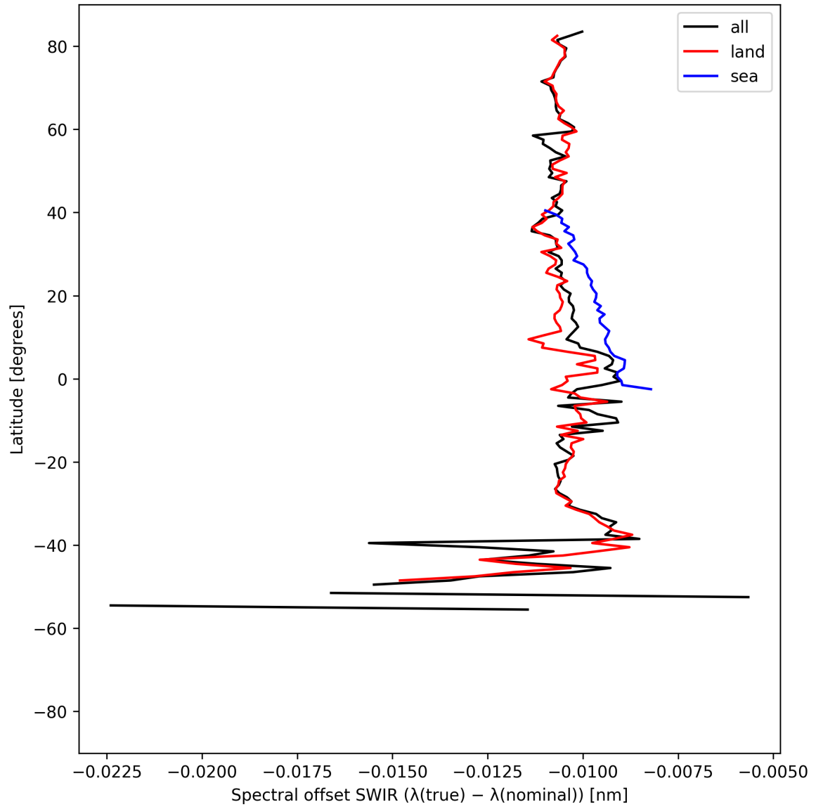
Figure 16: Zonal average of “Spectral offset SWIR ( \lambda_{\text{true}} - \lambda_{\text{nominal}} )” for 2025-04-21 to 2025-04-23.
