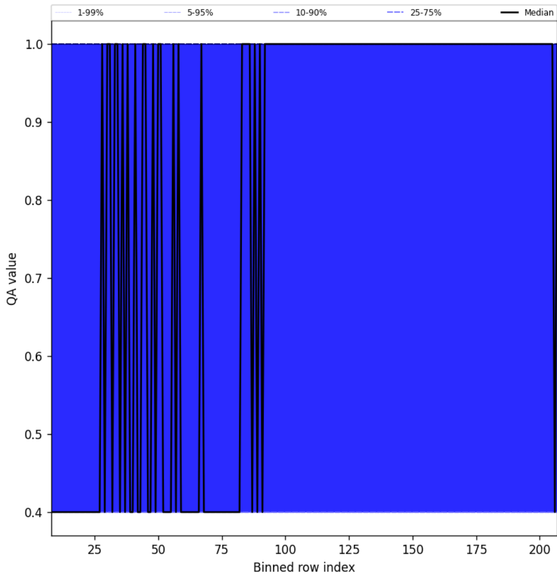
Figure 33: Along track statistics of “QA value” for 2025-04-21 to 2025-04-23
