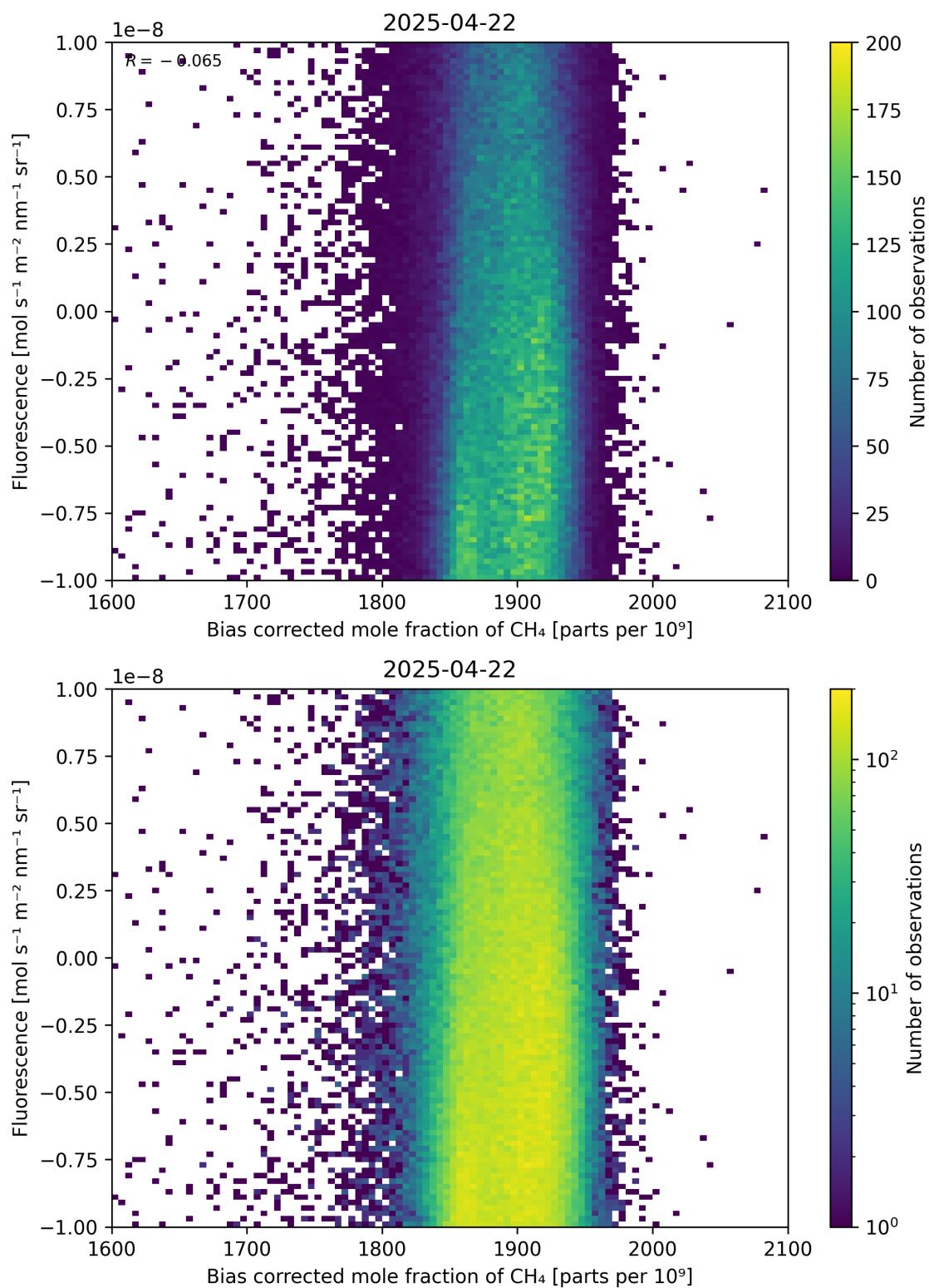
Figure 66: Scatter density plot of “Bias corrected mole fraction of CH 4 ” against “Fluorescence” for 2025-04-21 to 2025-04-23.
