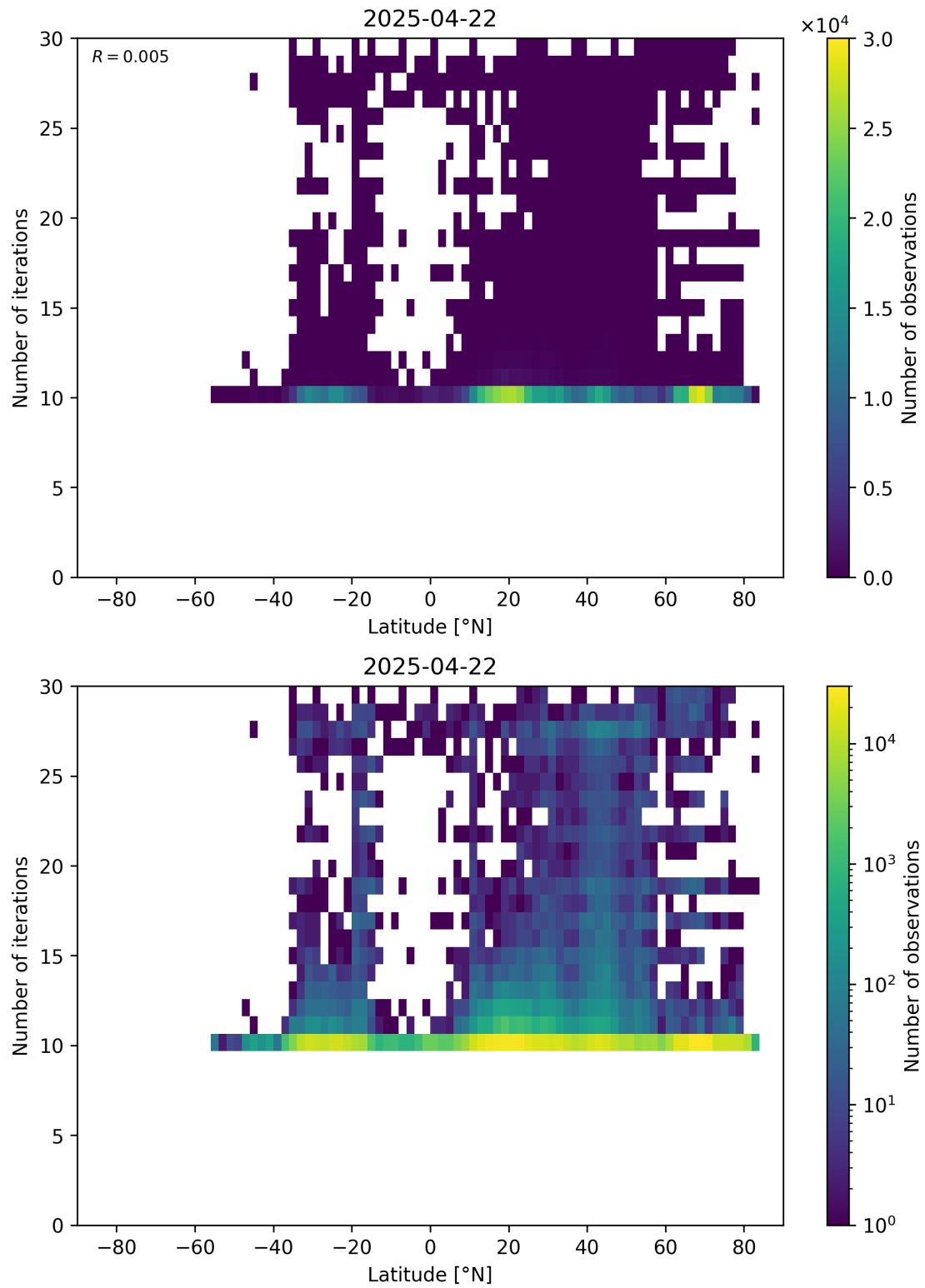
Figure 60: Scatter density plot of “Latitude” against “Number of iterations” for 2025-04-21 to 2025-04-23.
