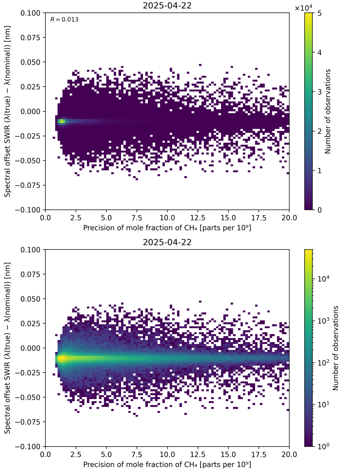
Figure 85: Scatter density plot of “Precision of mole fraction of CH 4 ” against “Spectral offset SWIR ( \lambda_{\text{true}} - \lambda_{\text{nominal}} )” for 2025-04-21 to 2025-04-23.
