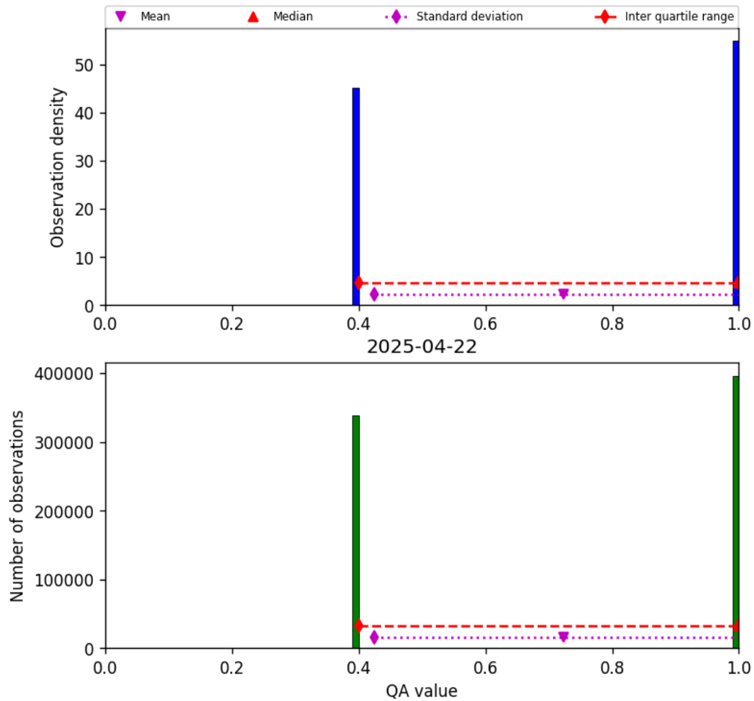
Figure 22: Histogram of “QA value” for 2025-04-21 to 2025-04-23
