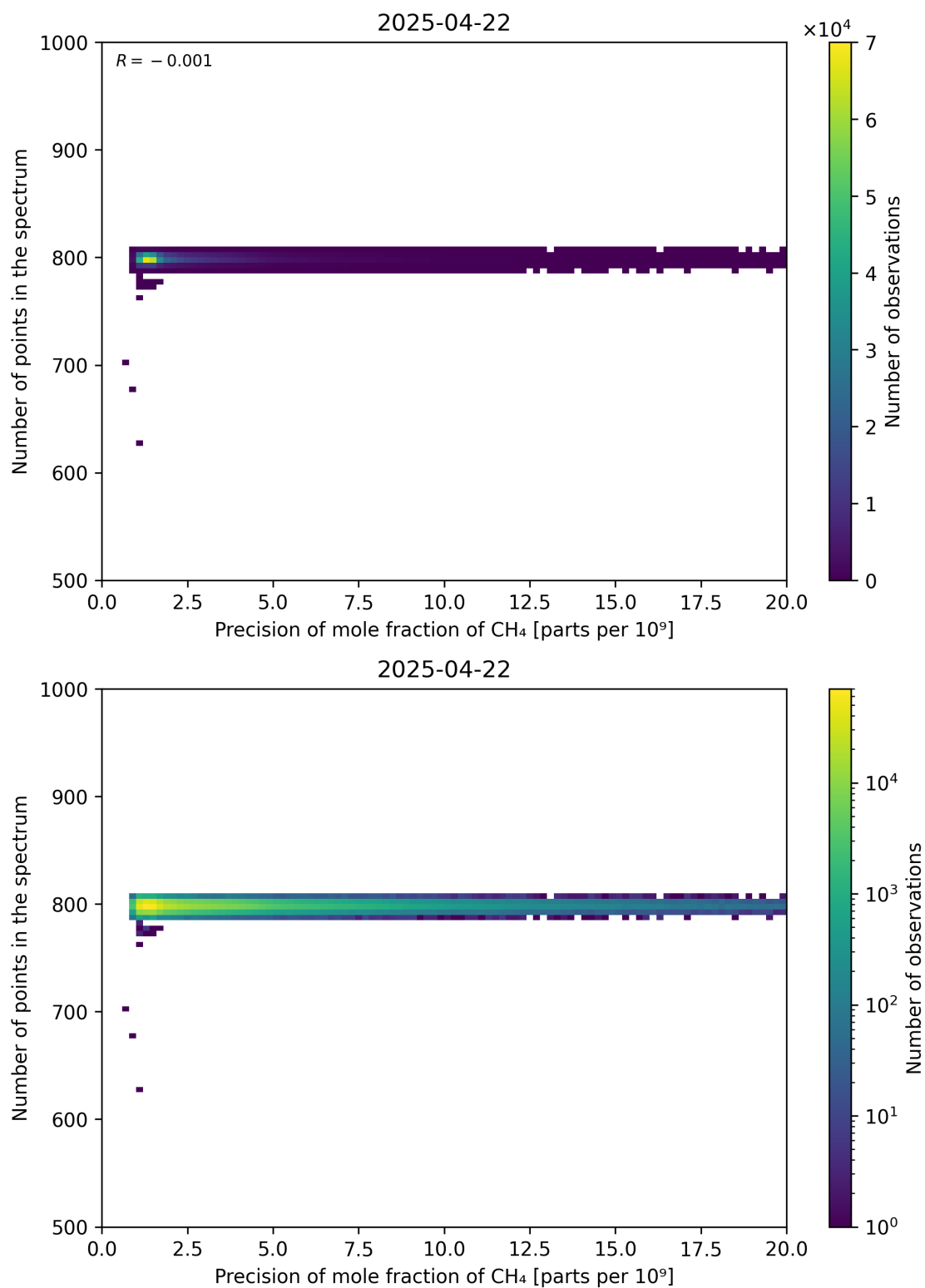
Figure 84: Scatter density plot of “Precision of mole fraction of CH 4 ” against “Number of points in the spectrum” for 2025-04-21 to 2025-04-23.
