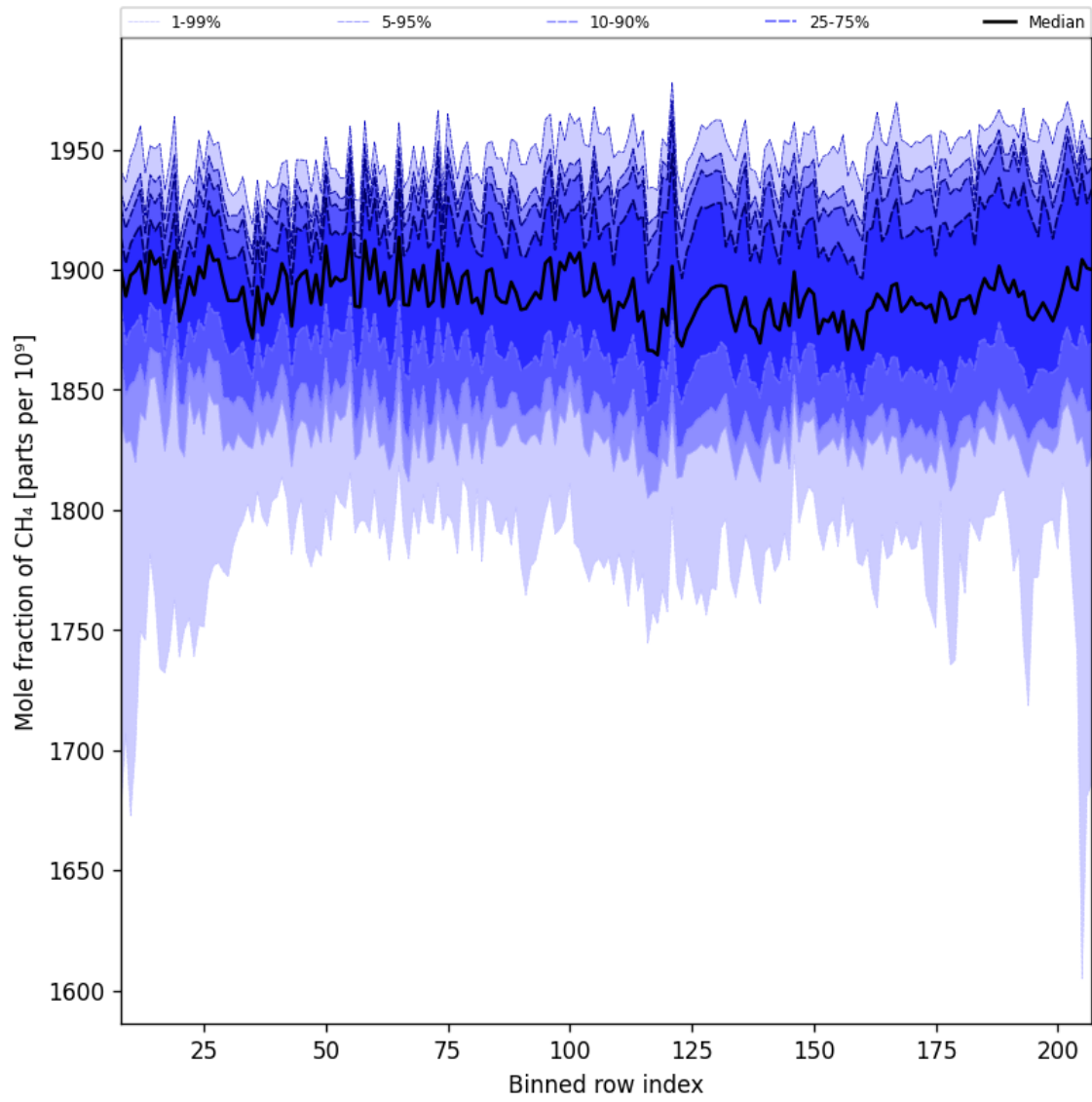
Figure 34: Along track statistics of “Mole fraction of CH 4 ” for 2025-04-21 to 2025-04-23
