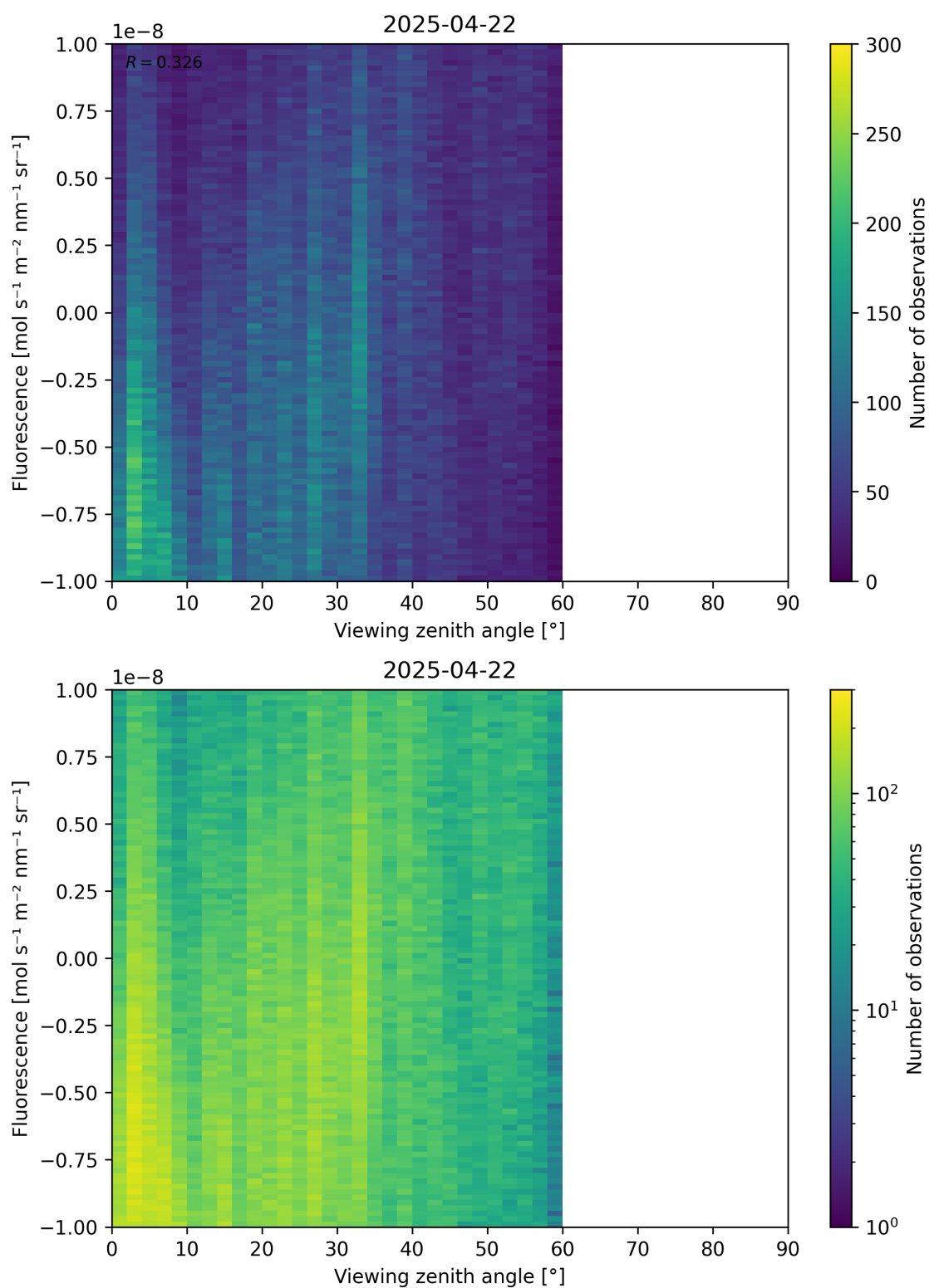
Figure 108: Scatter density plot of “Viewing zenith angle” against “Fluorescence” for 2025-04-21 to 2025-04-23.
