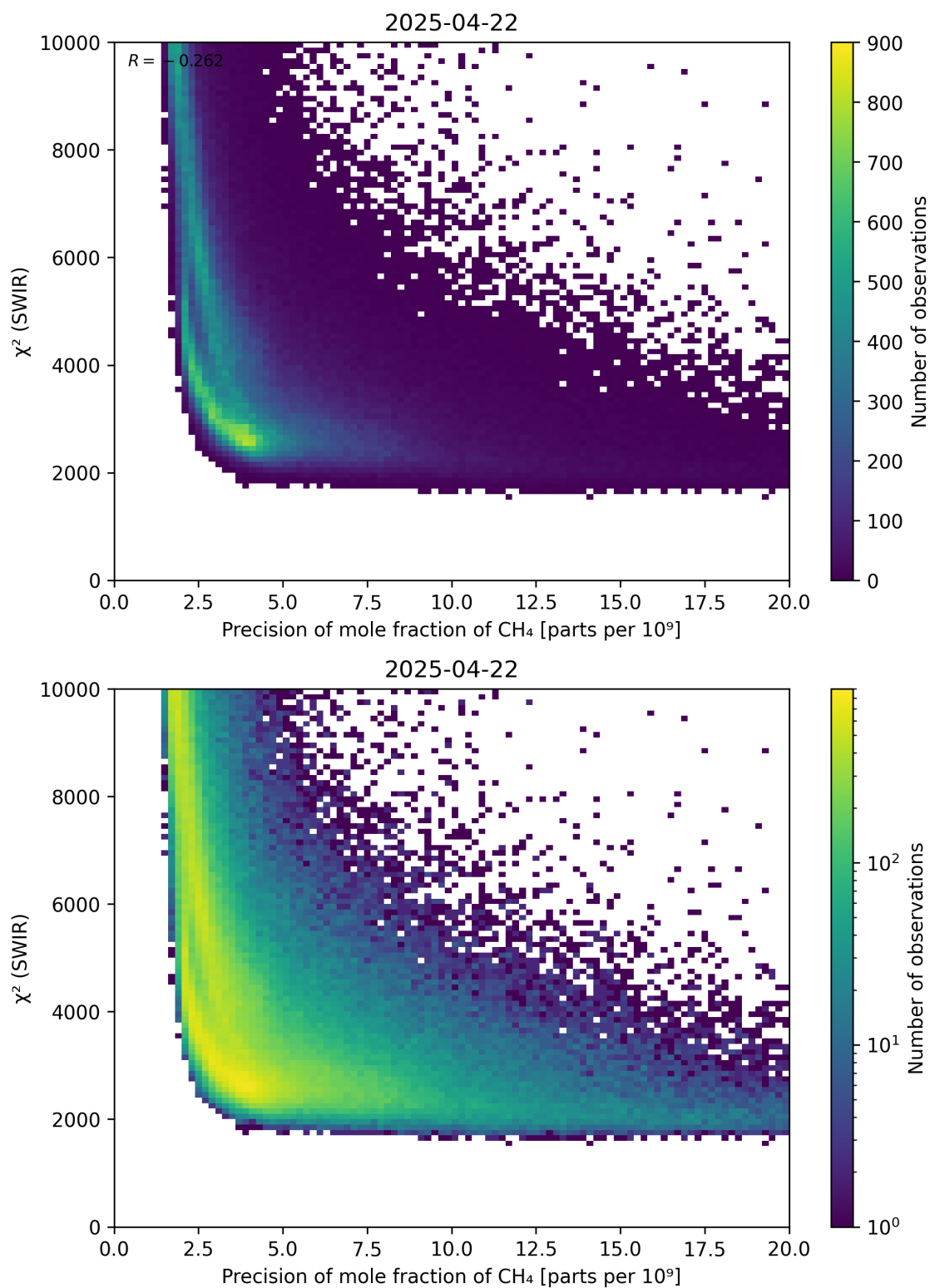
Figure 79: Scatter density plot of “Precision of mole fraction of \text{CH}_4 ” against “ \chi^2 (SWIR)” for 2025-04-21 to 2025-04-23.
