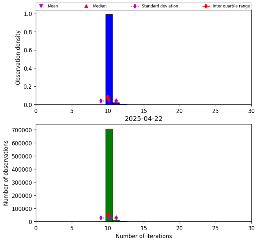
Figure 31: Histogram of “Number of iterations” for 2025-04-21 to 2025-04-23
