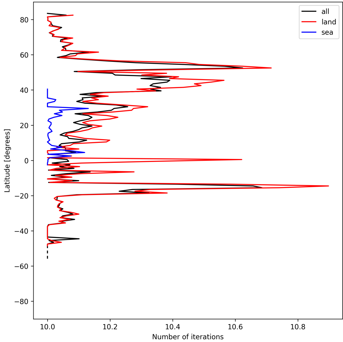
Figure 20: Zonal average of “Number of iterations” for 2025-04-21 to 2025-04-23.
