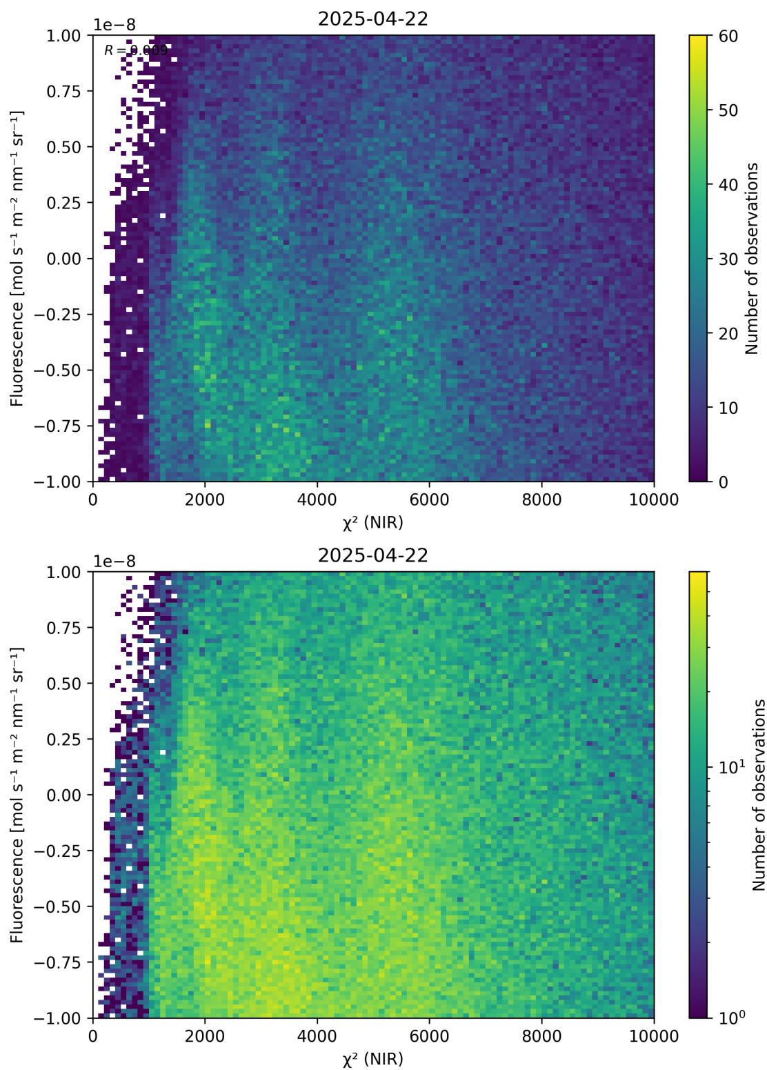
Figure 45: Scatter density plot of “ \chi^2 (NIR)” against “Fluorescence” for 2025-04-21 to 2025-04-23.
