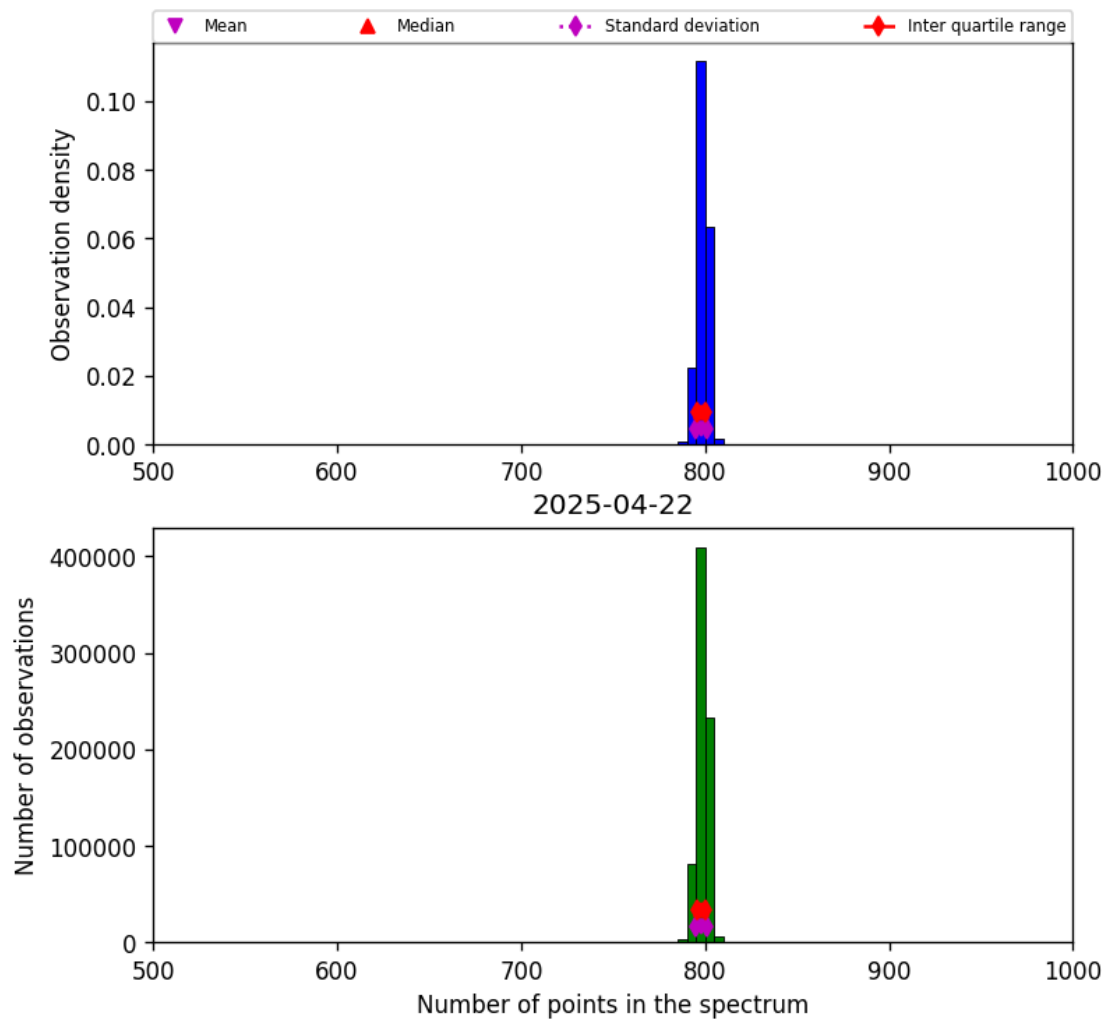
Figure 26: Histogram of “Number of points in the spectrum” for 2025-04-21 to 2025-04-23
