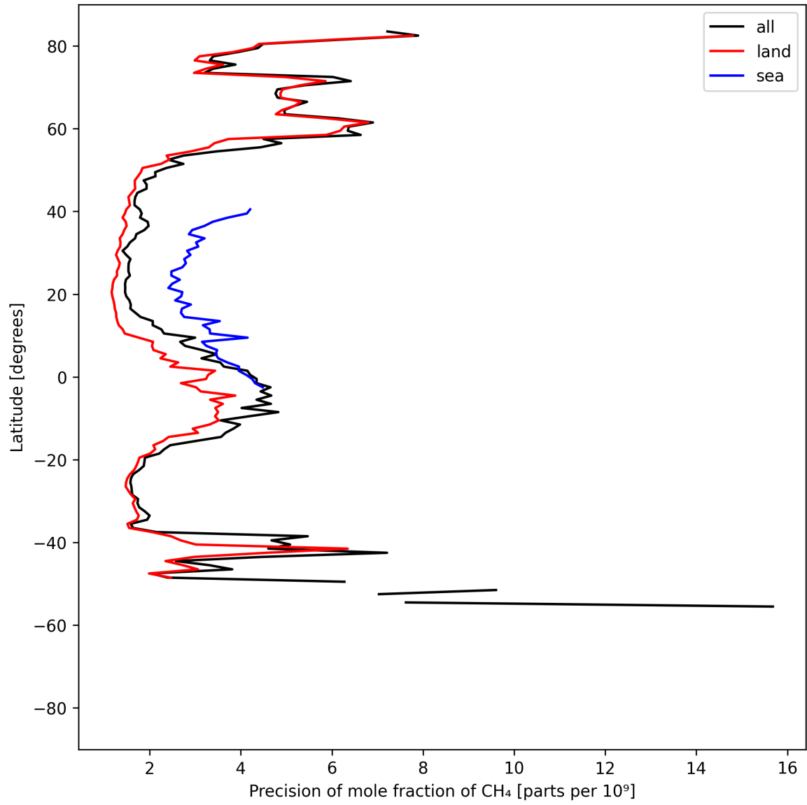
Figure 13: Zonal average of “Precision of mole fraction of CH 4 ” for 2025-04-21 to 2025-04-23.
