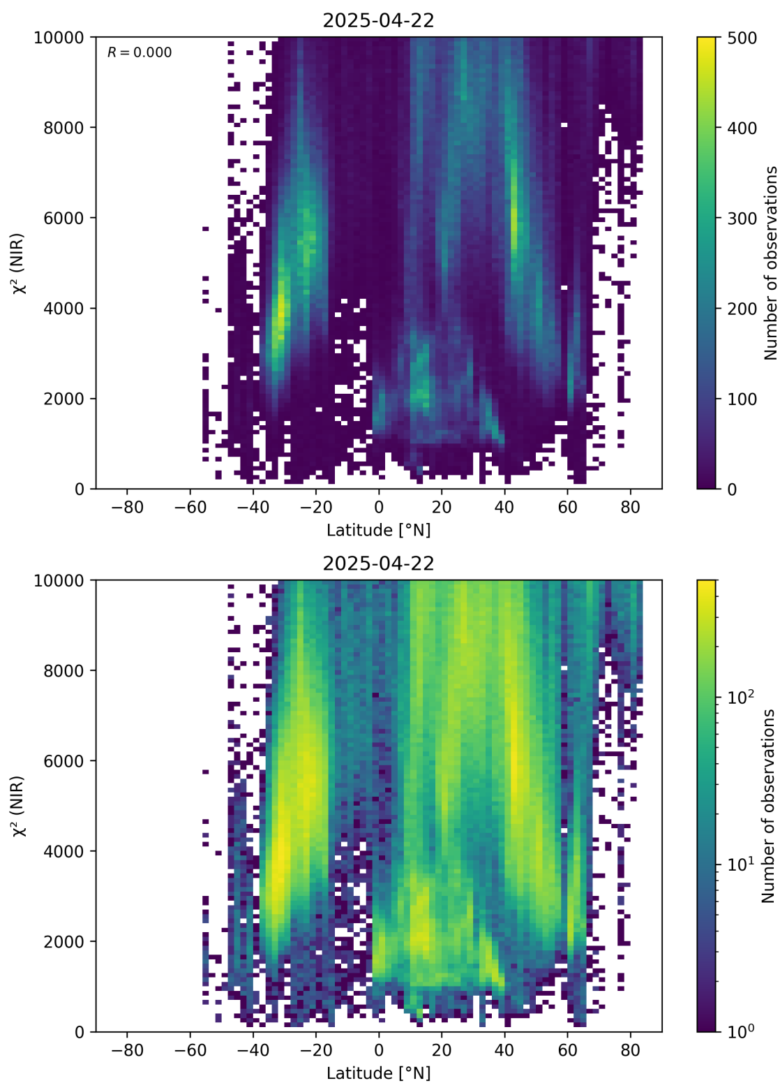
Figure 53: Scatter density plot of “Latitude” against “ \chi^2 (NIR)” for 2025-04-21 to 2025-04-23.
