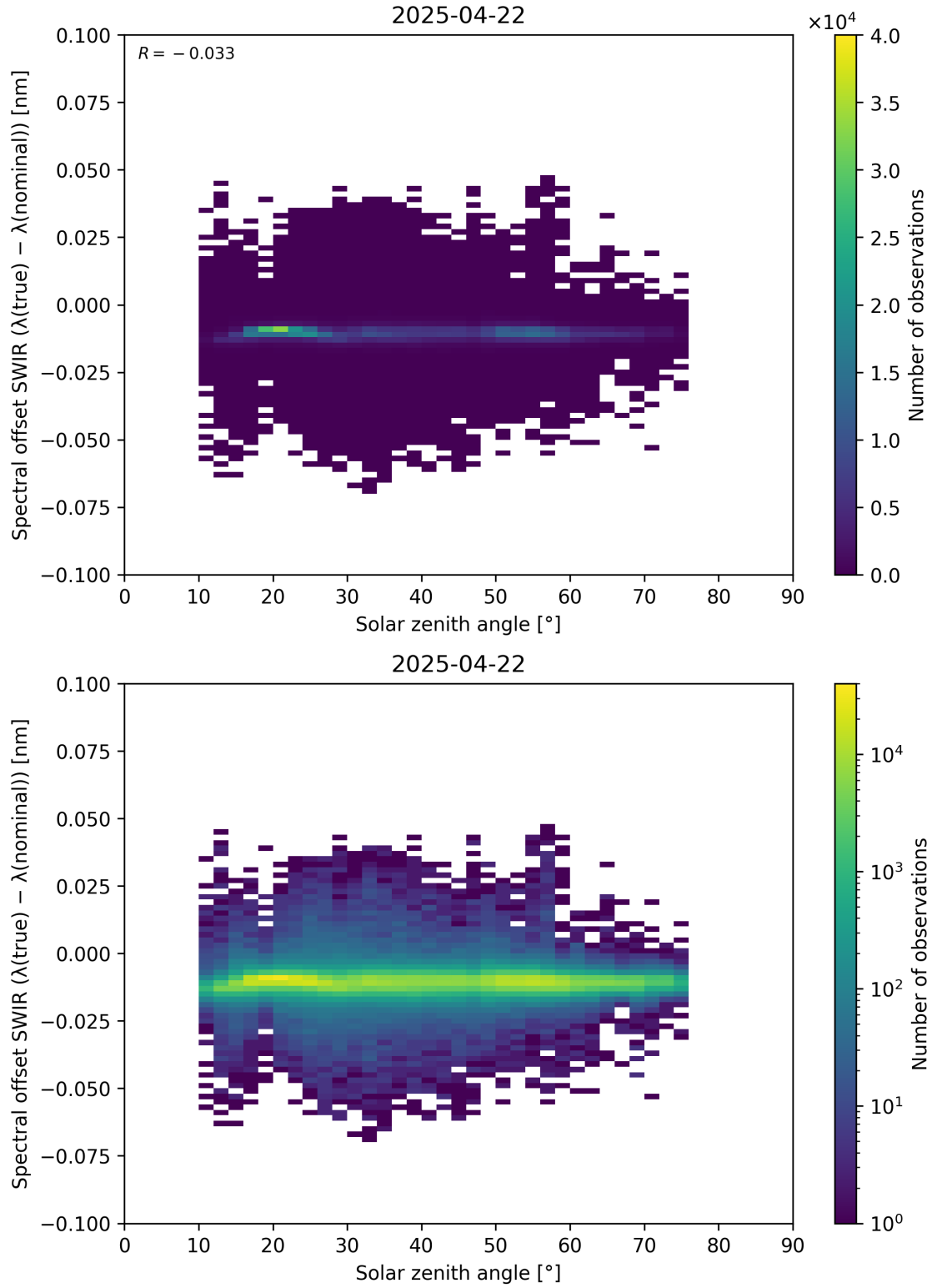
Figure 104: Scatter density plot of “Solar zenith angle” against “Spectral offset SWIR ( \lambda_{\text{true}} - \lambda_{\text{nominal}} )” for 2025-04-21 to 2025-04-23.
