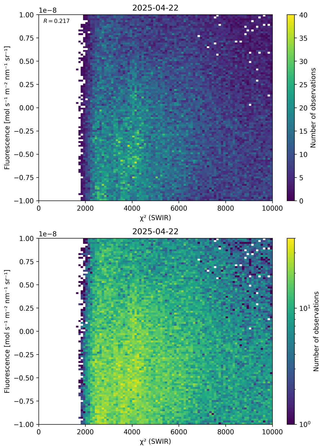
Figure 49: Scatter density plot of “ \chi^2 (SWIR)” against “Fluorescence” for 2025-04-21 to 2025-04-23.
