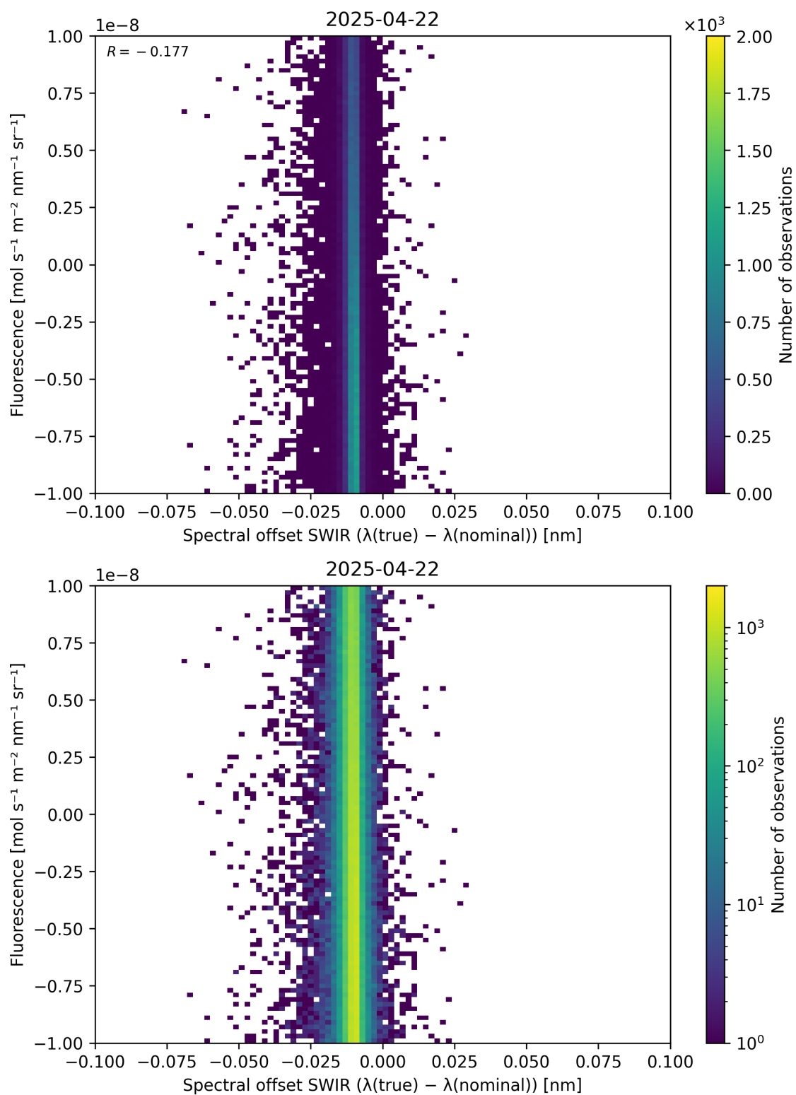
Figure 120: Scatter density plot of “Spectral offset SWIR ( \lambda_{\text{true}} - \lambda_{\text{nominal}} )” against “Fluorescence” for 2025-04-21 to 2025-04-23.
