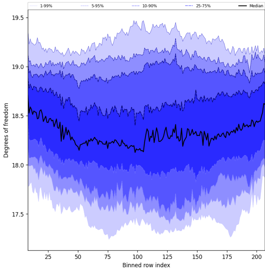
Figure 41: Along track statistics of “Degrees of freedom” for 2025-04-21 to 2025-04-23
