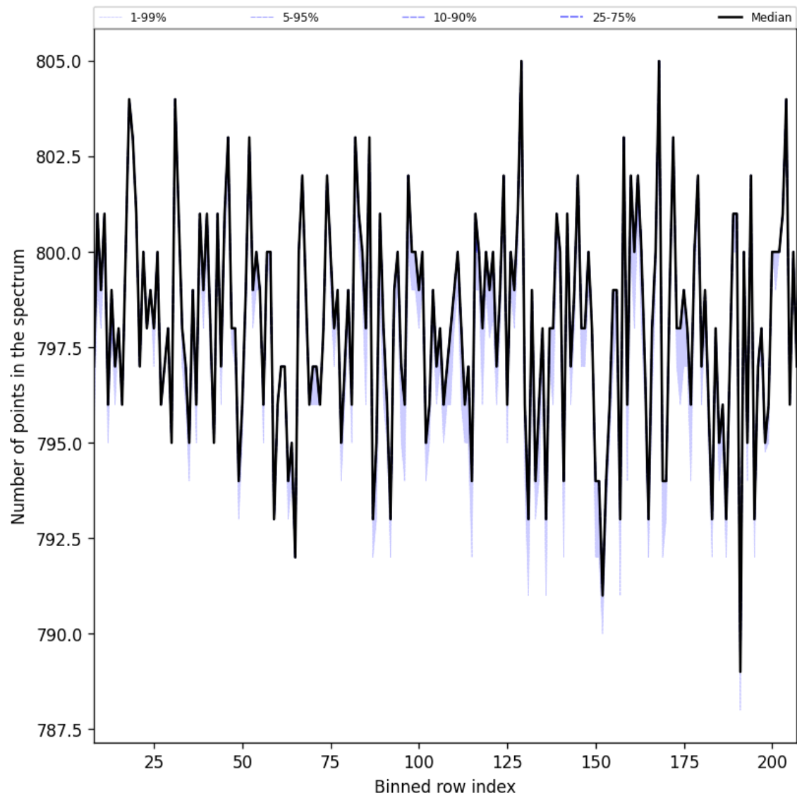
Figure 37: Along track statistics of “Number of points in the spectrum” for 2025-04-21 to 2025-04-23
