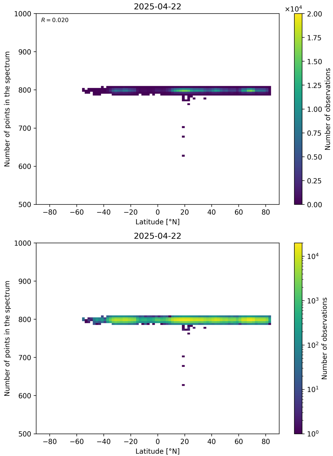
Figure 61: Scatter density plot of “Latitude” against “Number of points in the spectrum” for 2025-04-21 to 2025-04-23.
