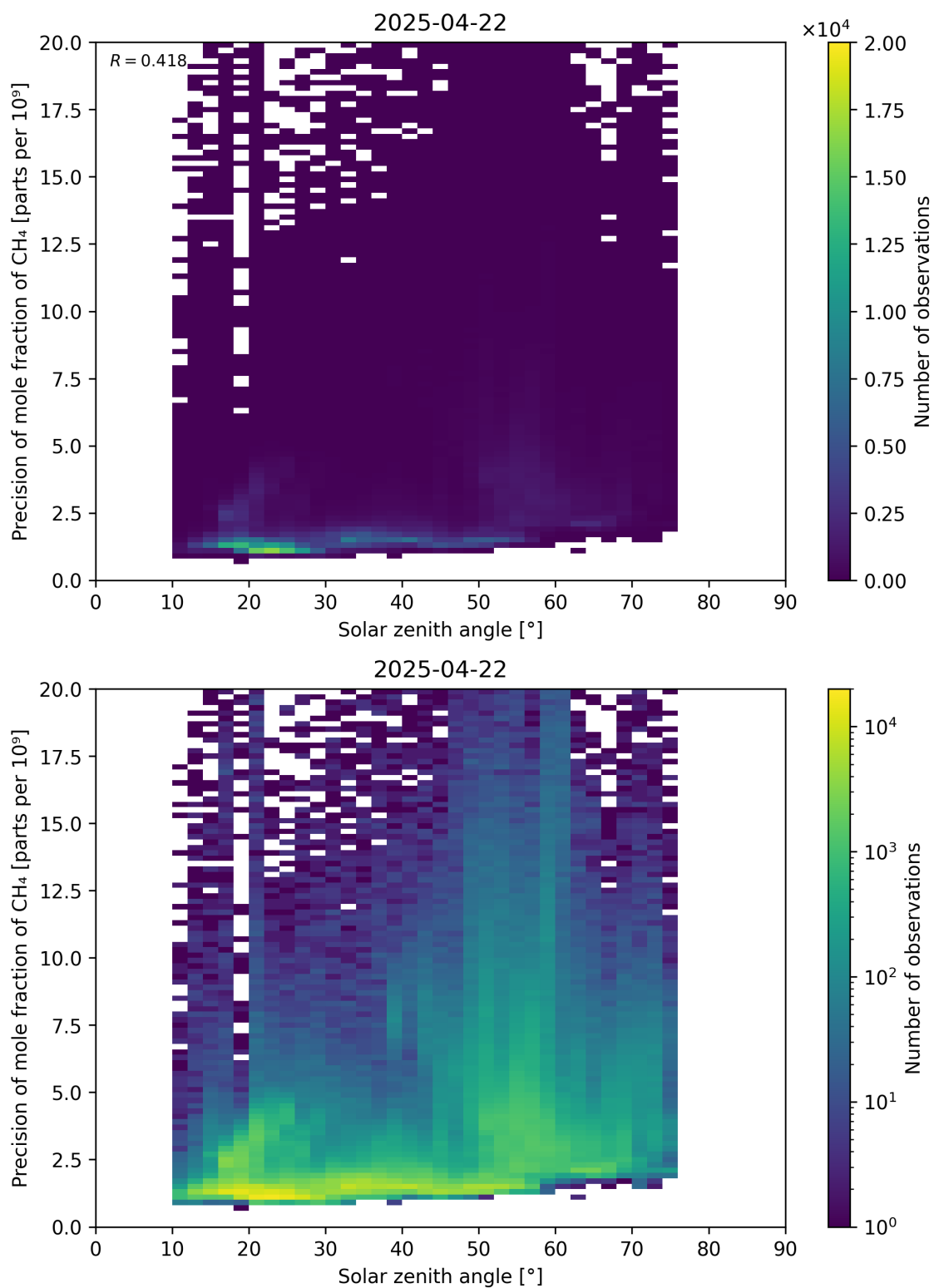
Figure 101: Scatter density plot of “Solar zenith angle” against “Precision of mole fraction of CH 4 ” for 2025-04-21 to 2025-04-23.
