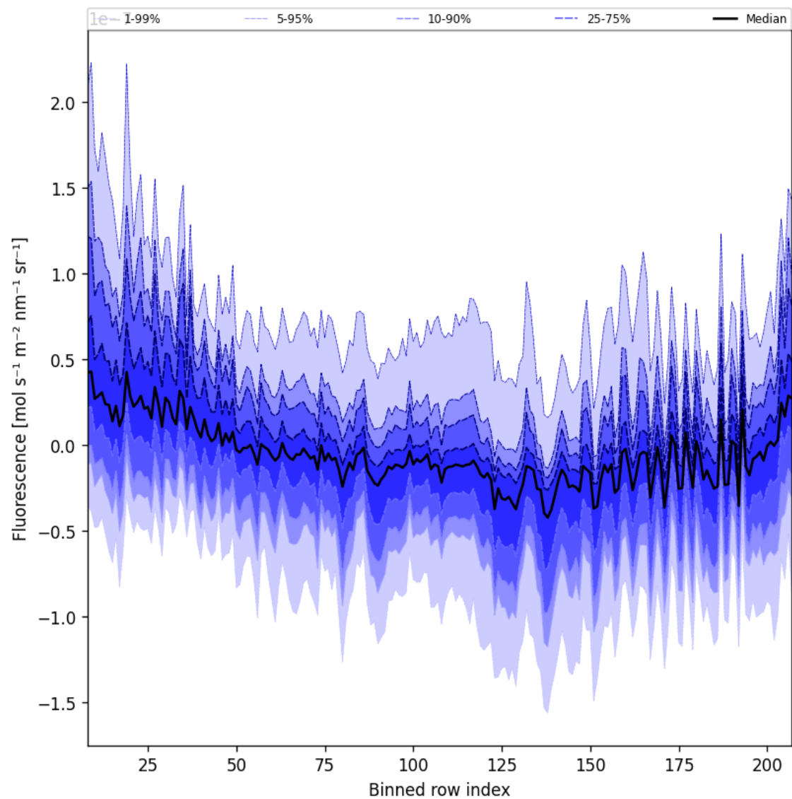
Figure 43: Along track statistics of “Fluorescence” for 2025-04-21 to 2025-04-23
