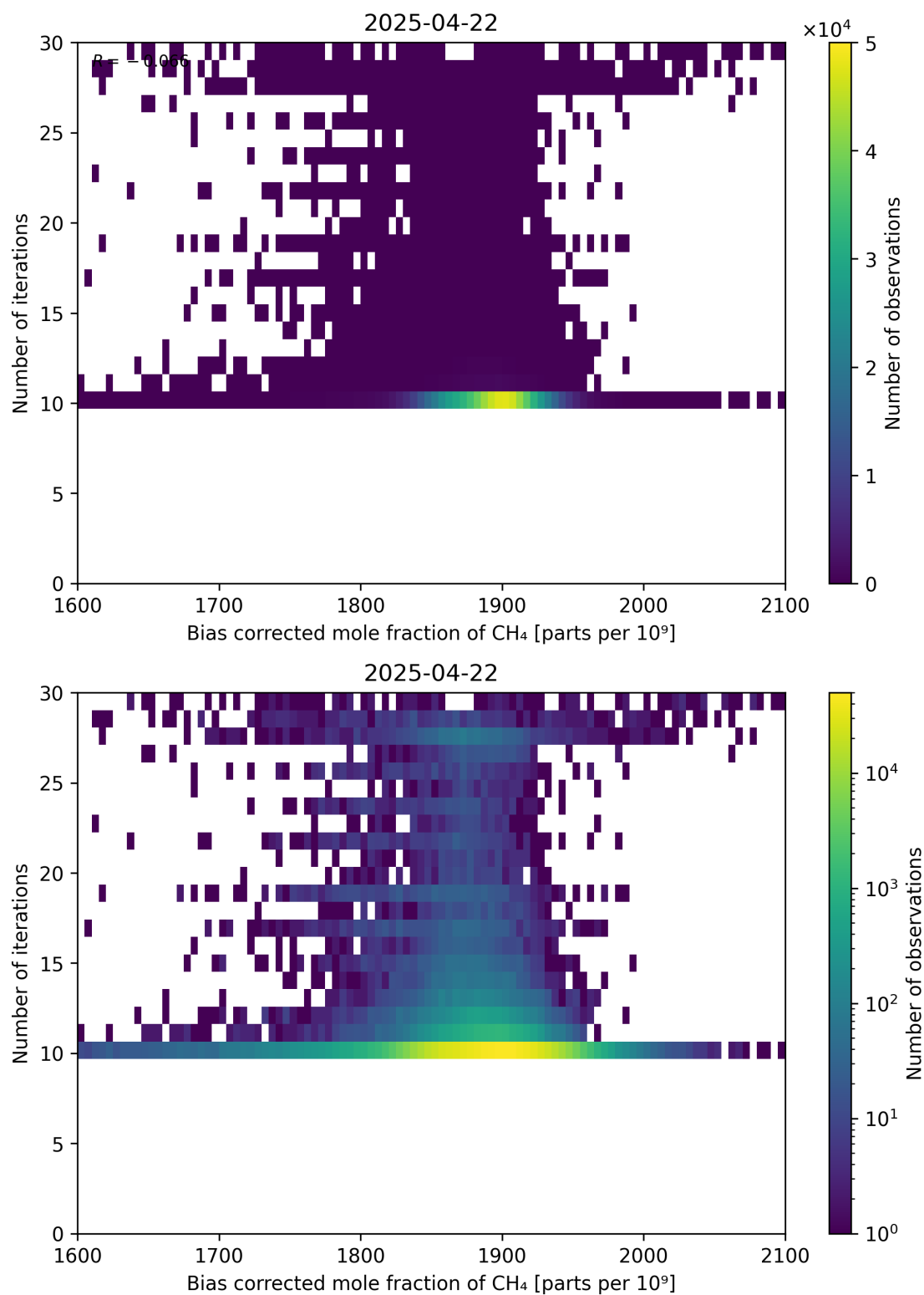
Figure 67: Scatter density plot of “Bias corrected mole fraction of CH 4 ” against “Number of iterations” for 2025-04-21 to 2025-04-23.
