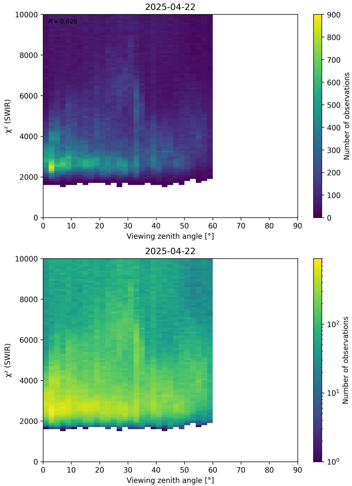
Figure 106: Scatter density plot of “Viewing zenith angle” against “ \chi^2 (SWIR)” for 2025-04-21 to 2025-04-23.
