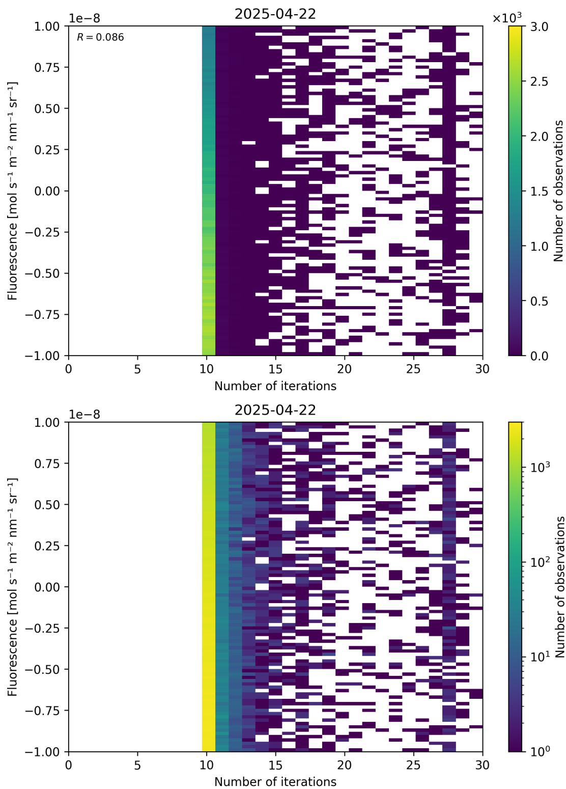
Figure 87: Scatter density plot of “Number of iterations” against “Fluorescence” for 2025-04-21 to 2025-04-23.
