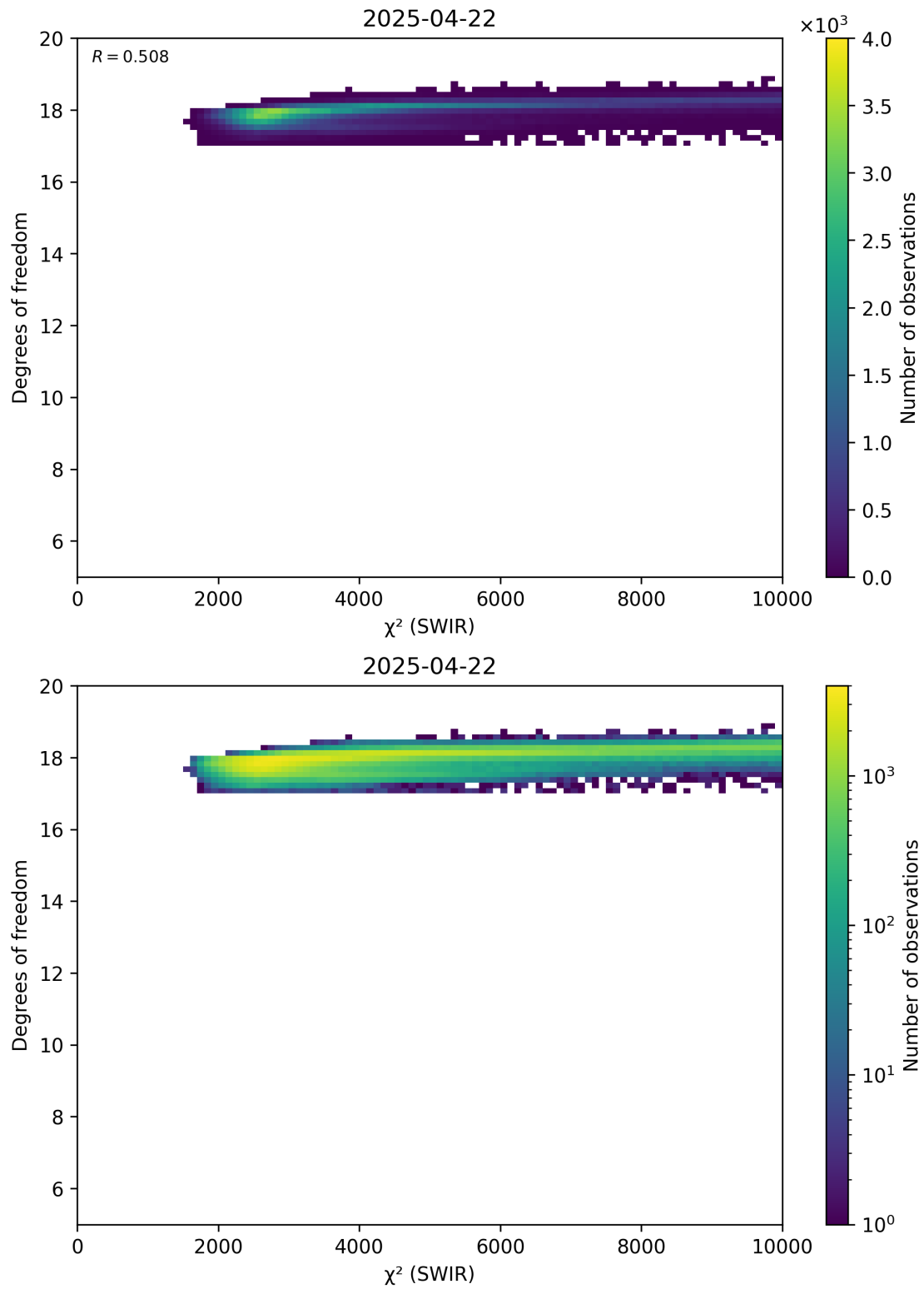
Figure 48: Scatter density plot of “ \chi^2 (SWIR)” against “Degrees of freedom” for 2025-04-21 to 2025-04-23.
