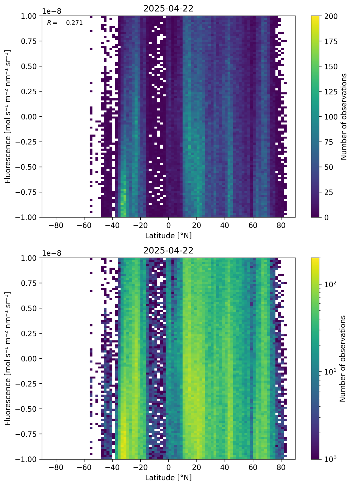
Figure 56: Scatter density plot of “Latitude” against “Fluorescence” for 2025-04-21 to 2025-04-23.
