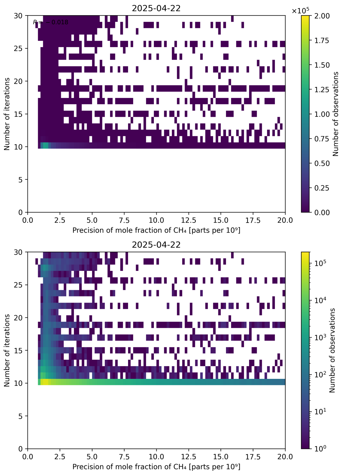
Figure 83: Scatter density plot of “Precision of mole fraction of CH 4 ” against “Number of iterations” for 2025-04-21 to 2025-04-23.
