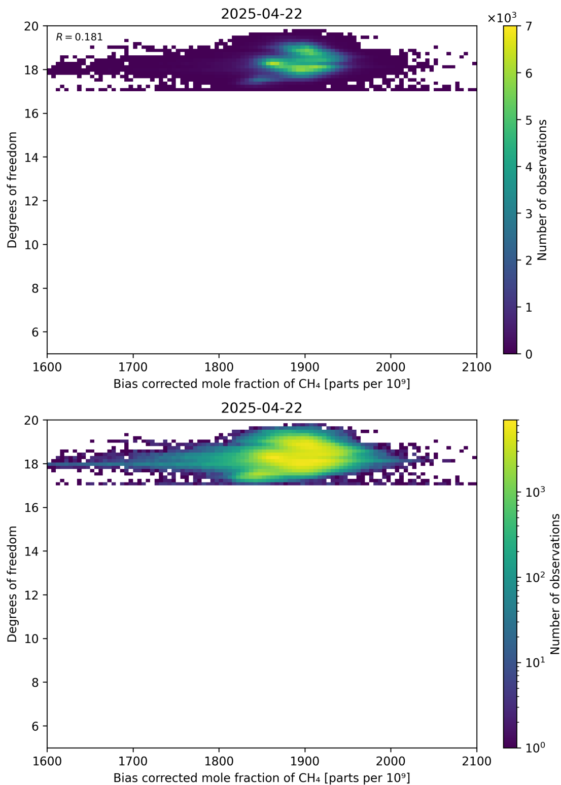
Figure 65: Scatter density plot of “Bias corrected mole fraction of CH 4 ” against “Degrees of freedom” for 2025-04-21 to 2025-04-23.
