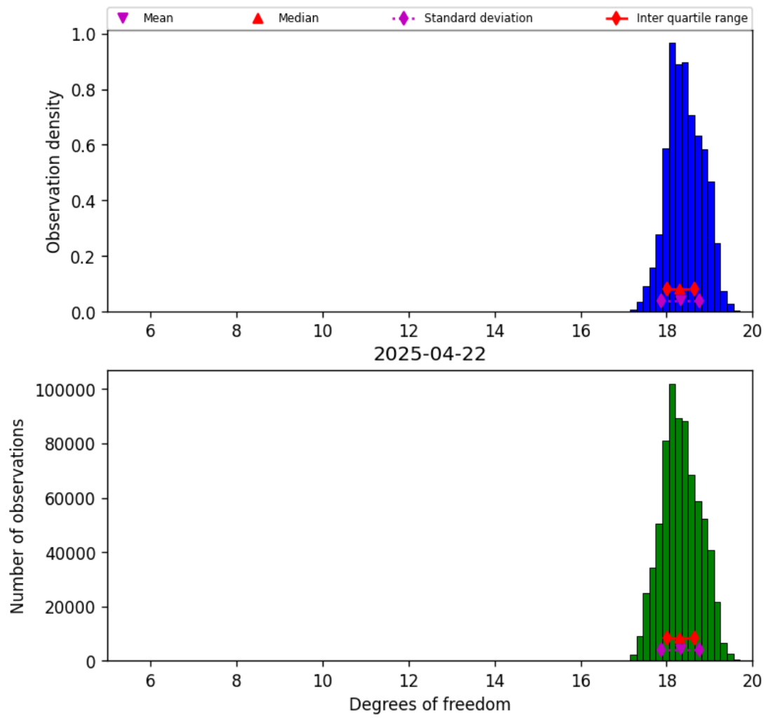
Figure 30: Histogram of “Degrees of freedom” for 2025-04-21 to 2025-04-23
