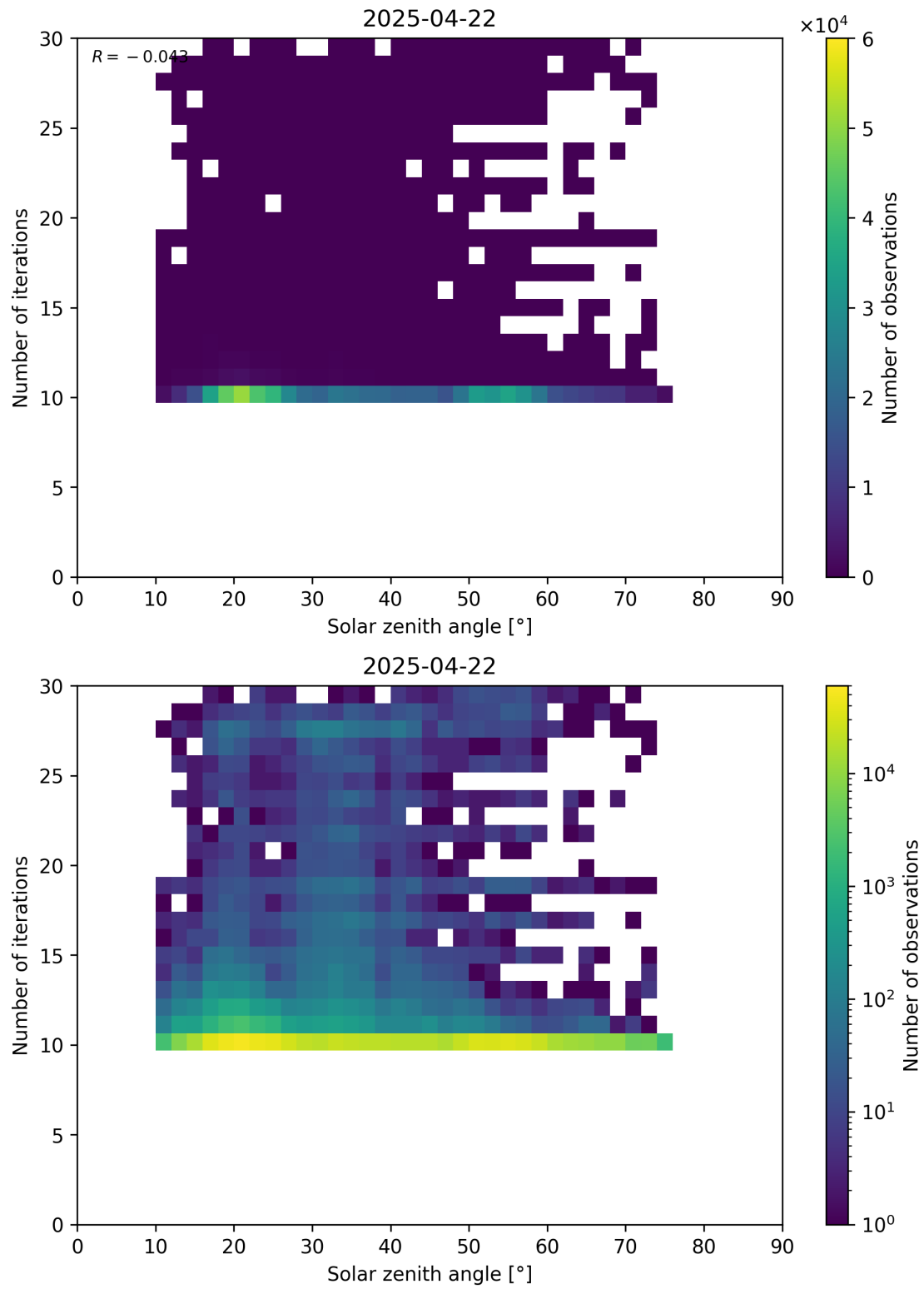
Figure 102: Scatter density plot of “Solar zenith angle” against “Number of iterations” for 2025-04-21 to 2025-04-23.
