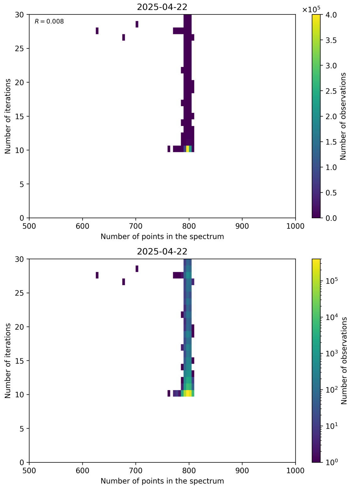
Figure 92: Scatter density plot of “Number of points in the spectrum” against “Number of iterations” for 2025-04-21 to 2025-04-23.
