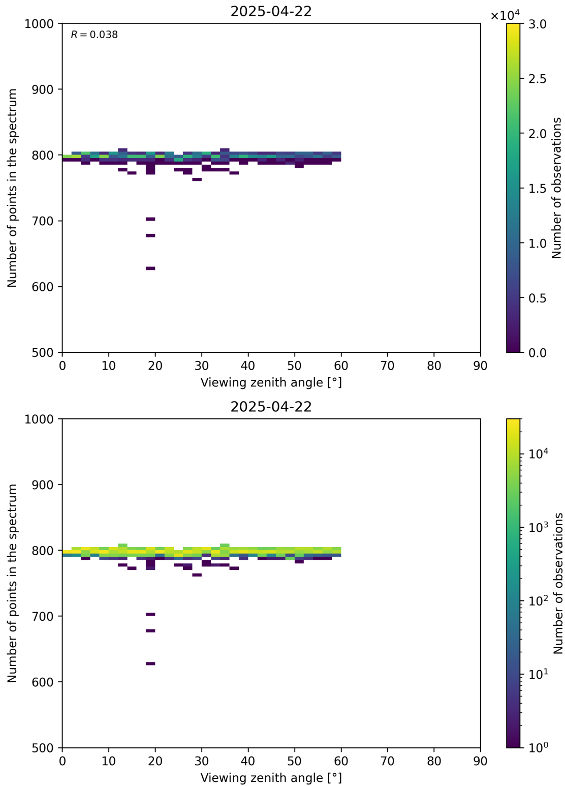
Figure 114: Scatter density plot of “Viewing zenith angle” against “Number of points in the spectrum” for 2025-04-21 to 2025-04-23.
