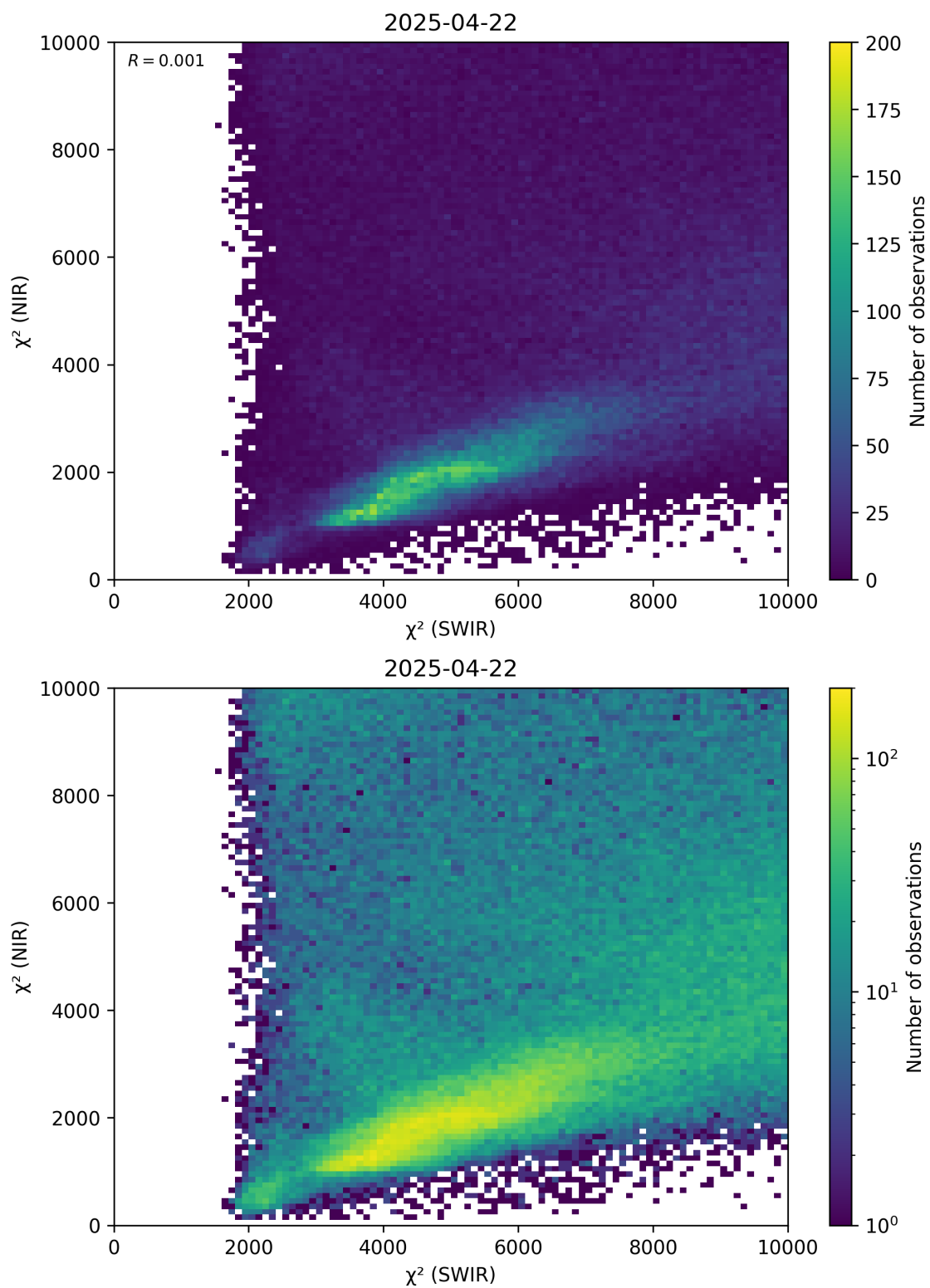
Figure 47: Scatter density plot of “ \chi^2 (SWIR)” against “ \chi^2 (NIR)” for 2025-04-21 to 2025-04-23.
