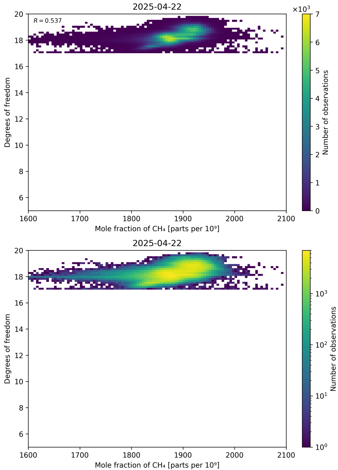
Figure 72: Scatter density plot of “Mole fraction of CH 4 ” against “Degrees of freedom” for 2025-04-21 to 2025-04-23.
