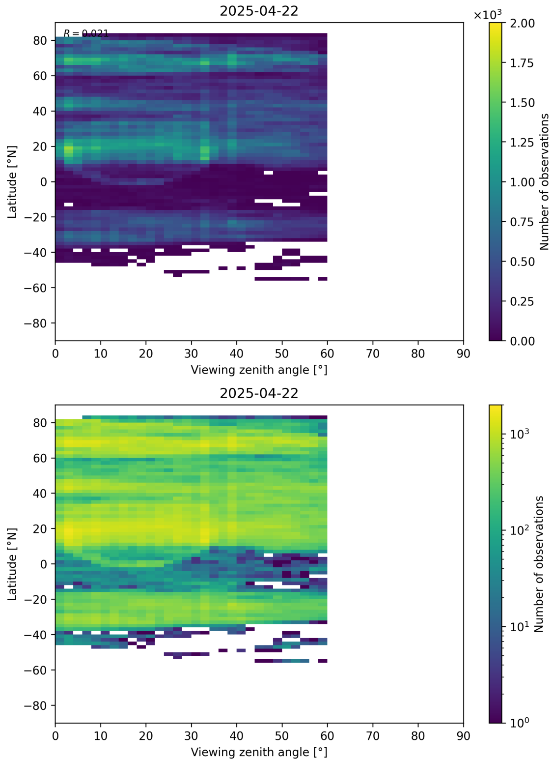
Figure 109: Scatter density plot of “Viewing zenith angle” against “Latitude” for 2025-04-21 to 2025-04-23.
