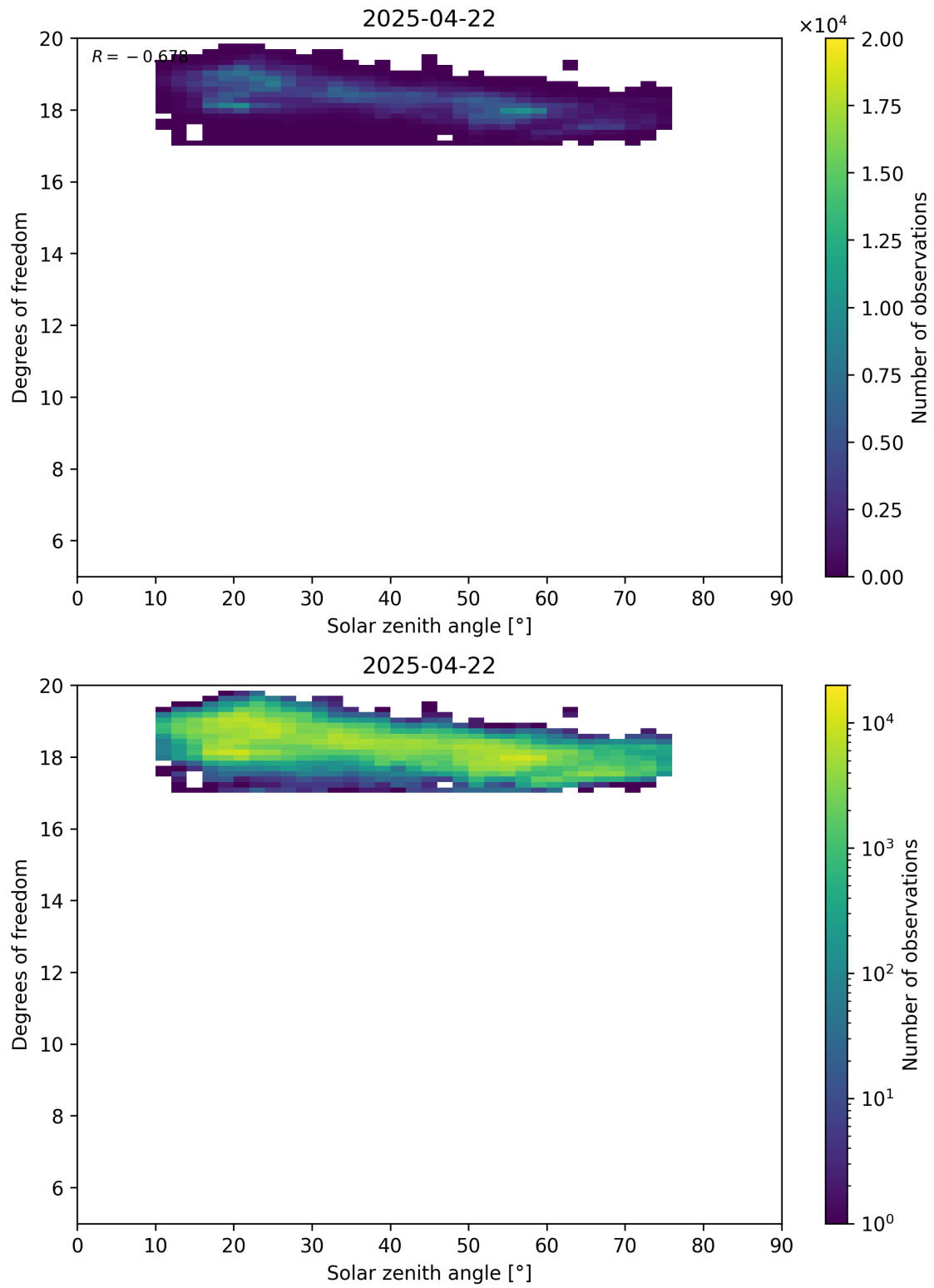
Figure 96: Scatter density plot of “Solar zenith angle” against “Degrees of freedom” for 2025-04-21 to 2025-04-23.
