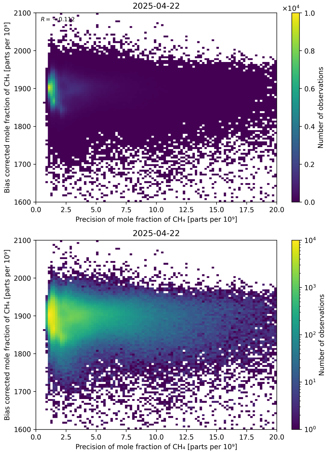
Figure 82: Scatter density plot of “Precision of mole fraction of CH 4 ” against “Bias corrected mole fraction of CH 4 ” for 2025-04-21 to 2025-04-23.
