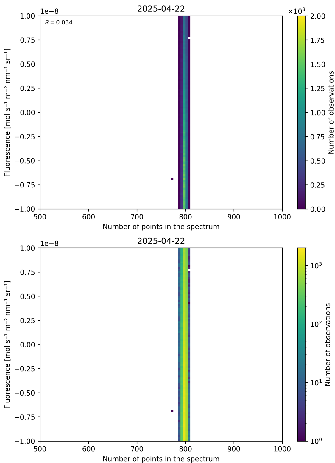
Figure 91: Scatter density plot of “Number of points in the spectrum” against “Fluorescence” for 2025-04-21 to 2025-04-23.
