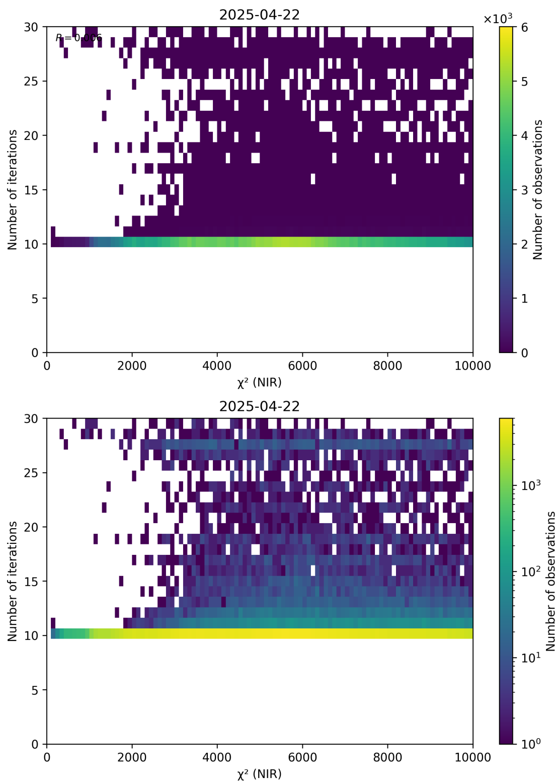
Figure 46: Scatter density plot of “ \chi^2 (NIR)” against “Number of iterations” for 2025-04-21 to 2025-04-23.
