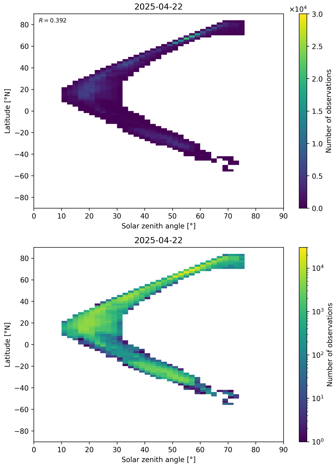
Figure 98: Scatter density plot of “Solar zenith angle” against “Latitude” for 2025-04-21 to 2025-04-23.
