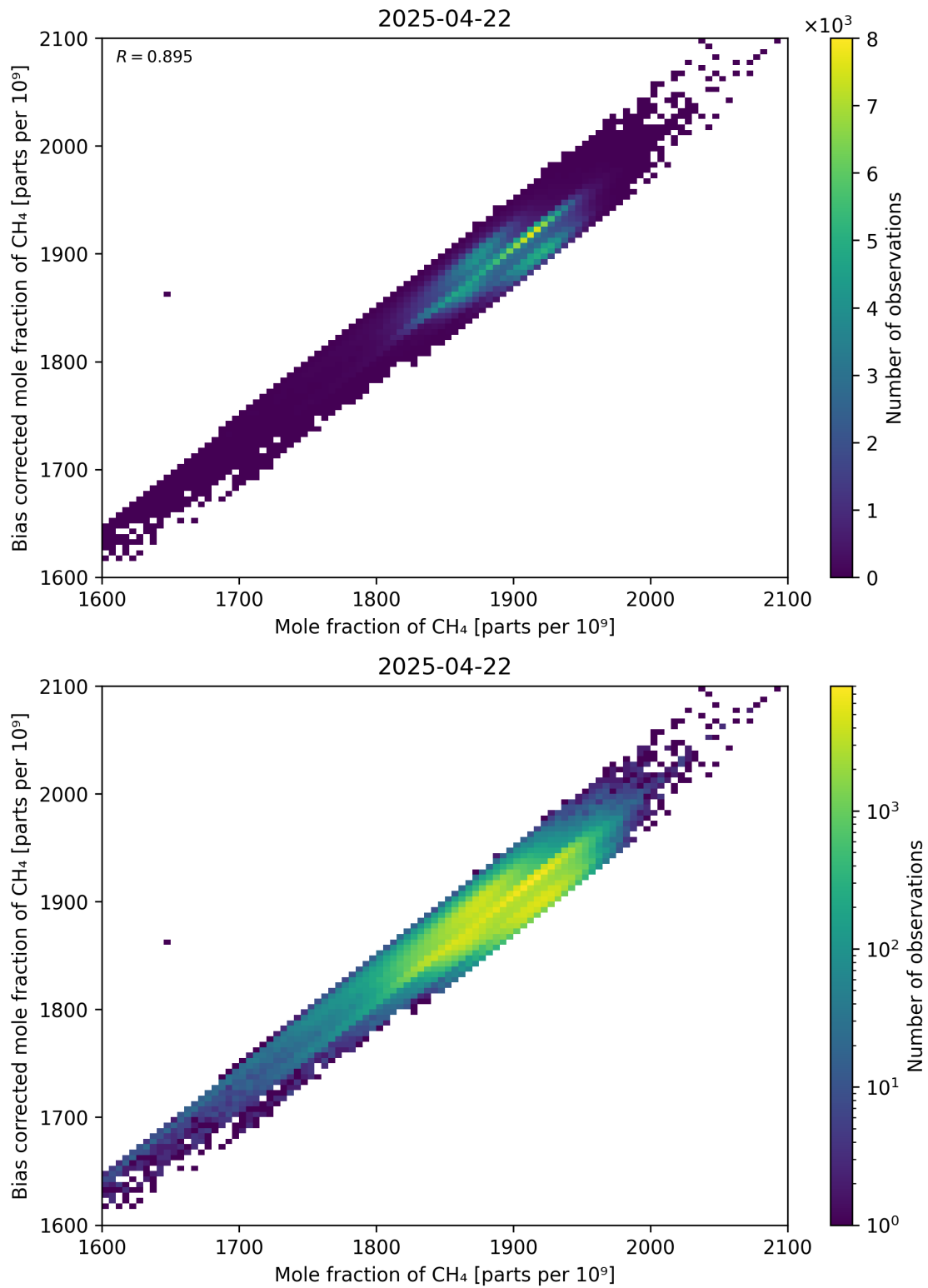
Figure 74: Scatter density plot of “Mole fraction of CH 4 ” against “Bias corrected mole fraction of CH 4 ” for 2025-04-21 to 2025-04-23.
