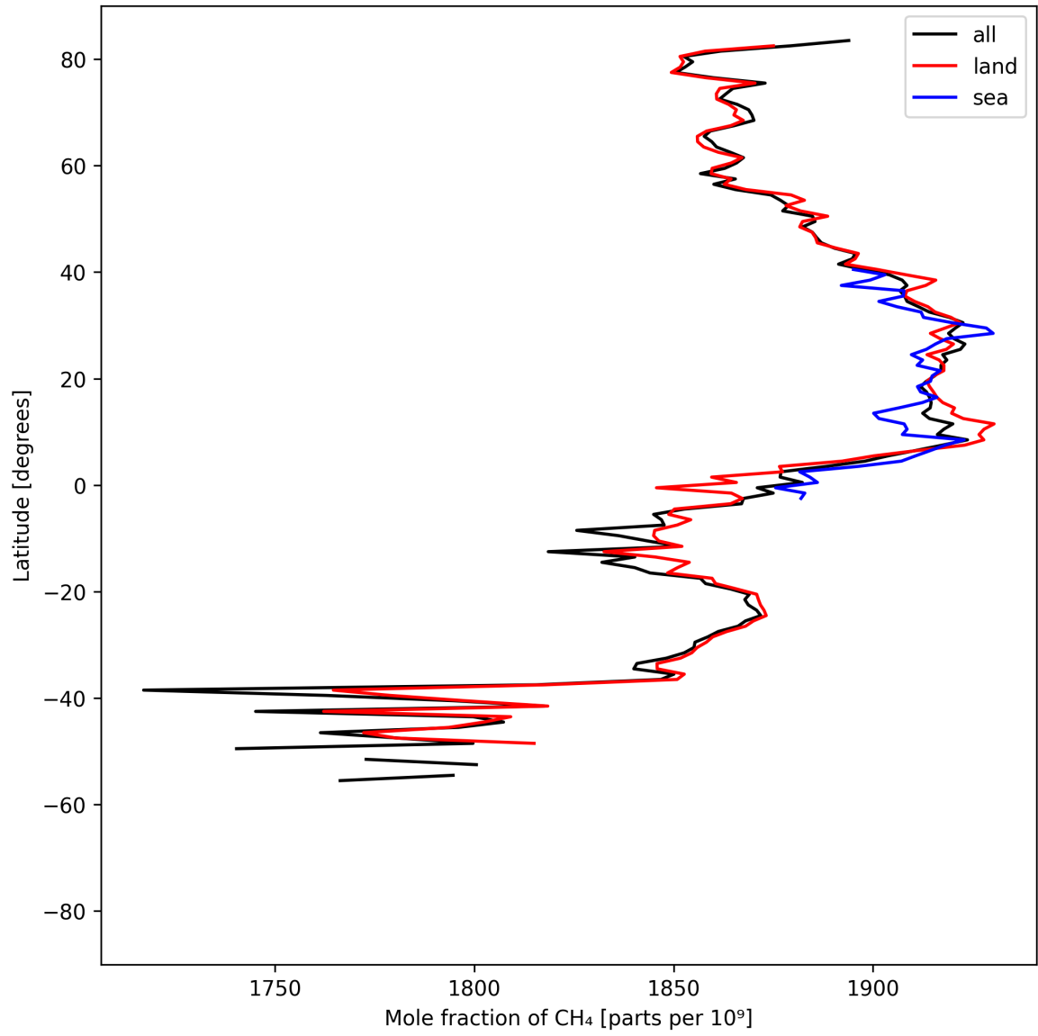
Figure 12: Zonal average of “Mole fraction of \text{CH}_4 ” for 2025-04-21 to 2025-04-23.
