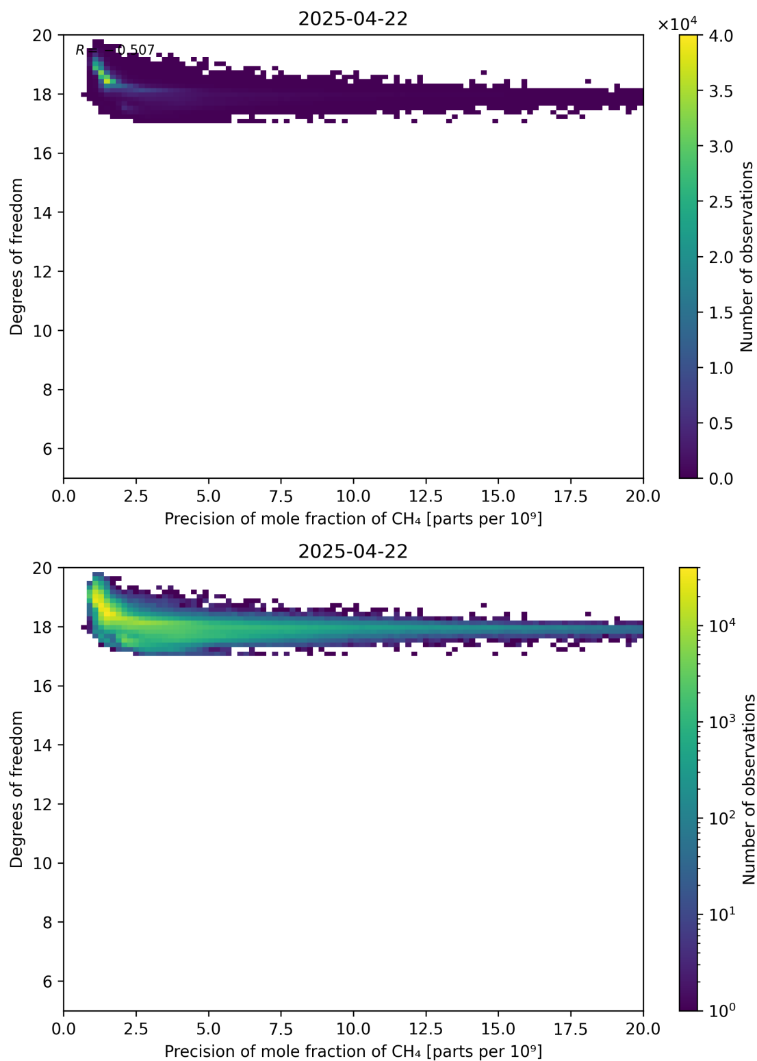
Figure 80: Scatter density plot of “Precision of mole fraction of CH 4 ” against “Degrees of freedom” for 2025-04-21 to 2025-04-23.
