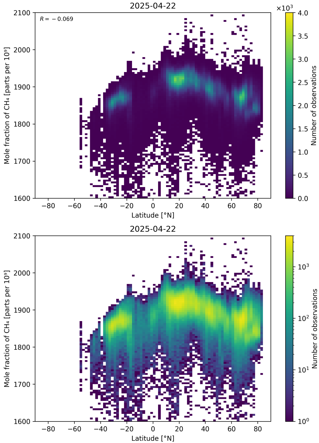
Figure 57: Scatter density plot of “Latitude” against “Mole fraction of CH 4 ” for 2025-04-21 to 2025-04-23.
