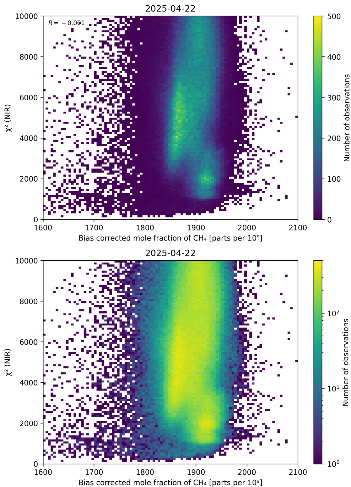
Figure 63: Scatter density plot of “Bias corrected mole fraction of CH 4 ” against “ \chi^2 (NIR)” for 2025-04-21 to 2025-04-23.
