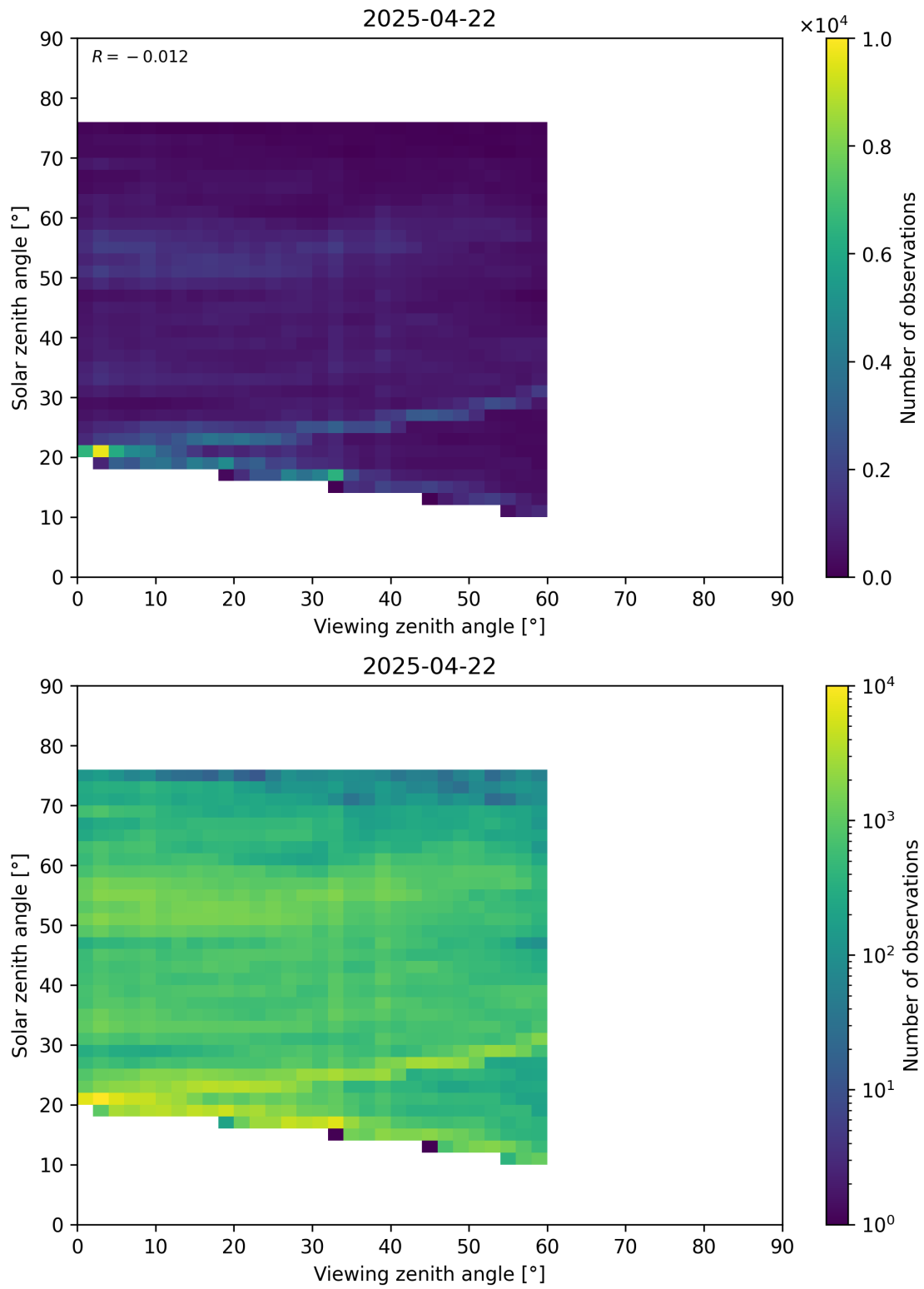
Figure 115: Scatter density plot of “Viewing zenith angle” against “Solar zenith angle” for 2025-04-21 to 2025-04-23.
