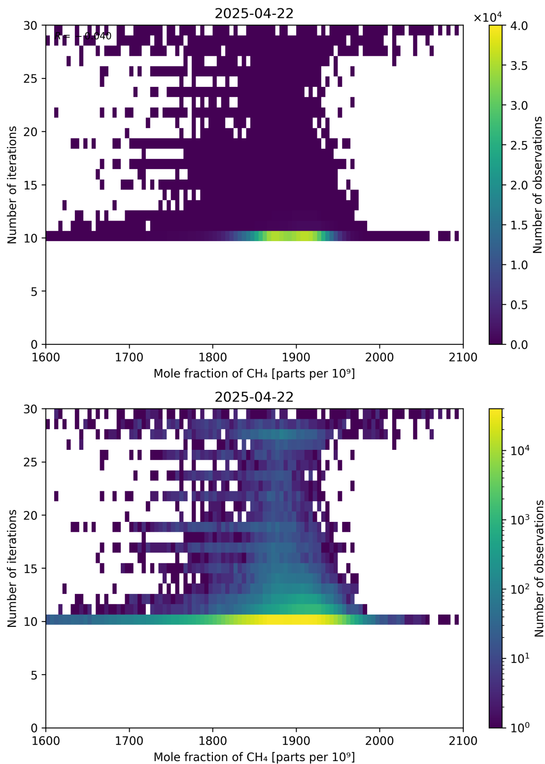
Figure 76: Scatter density plot of “Mole fraction of CH 4 ” against “Number of iterations” for 2025-04-21 to 2025-04-23.
