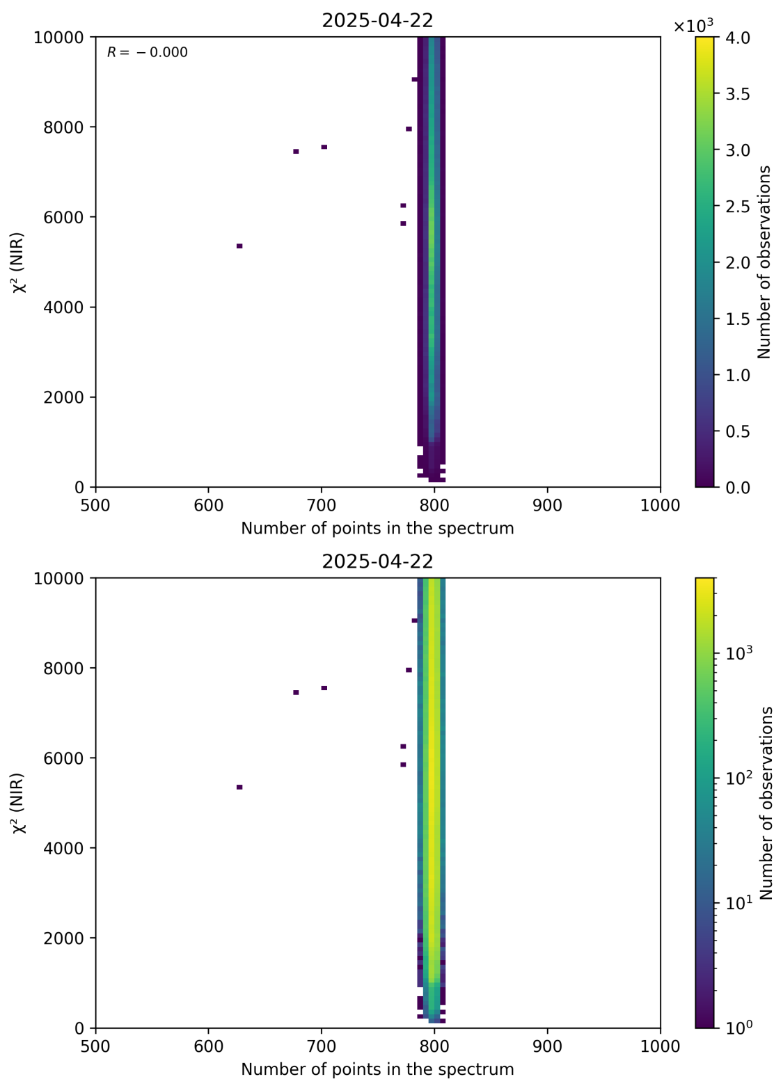
Figure 88: Scatter density plot of “Number of points in the spectrum” against “ \chi^2 (NIR)” for 2025-04-21 to 2025-04-23.
