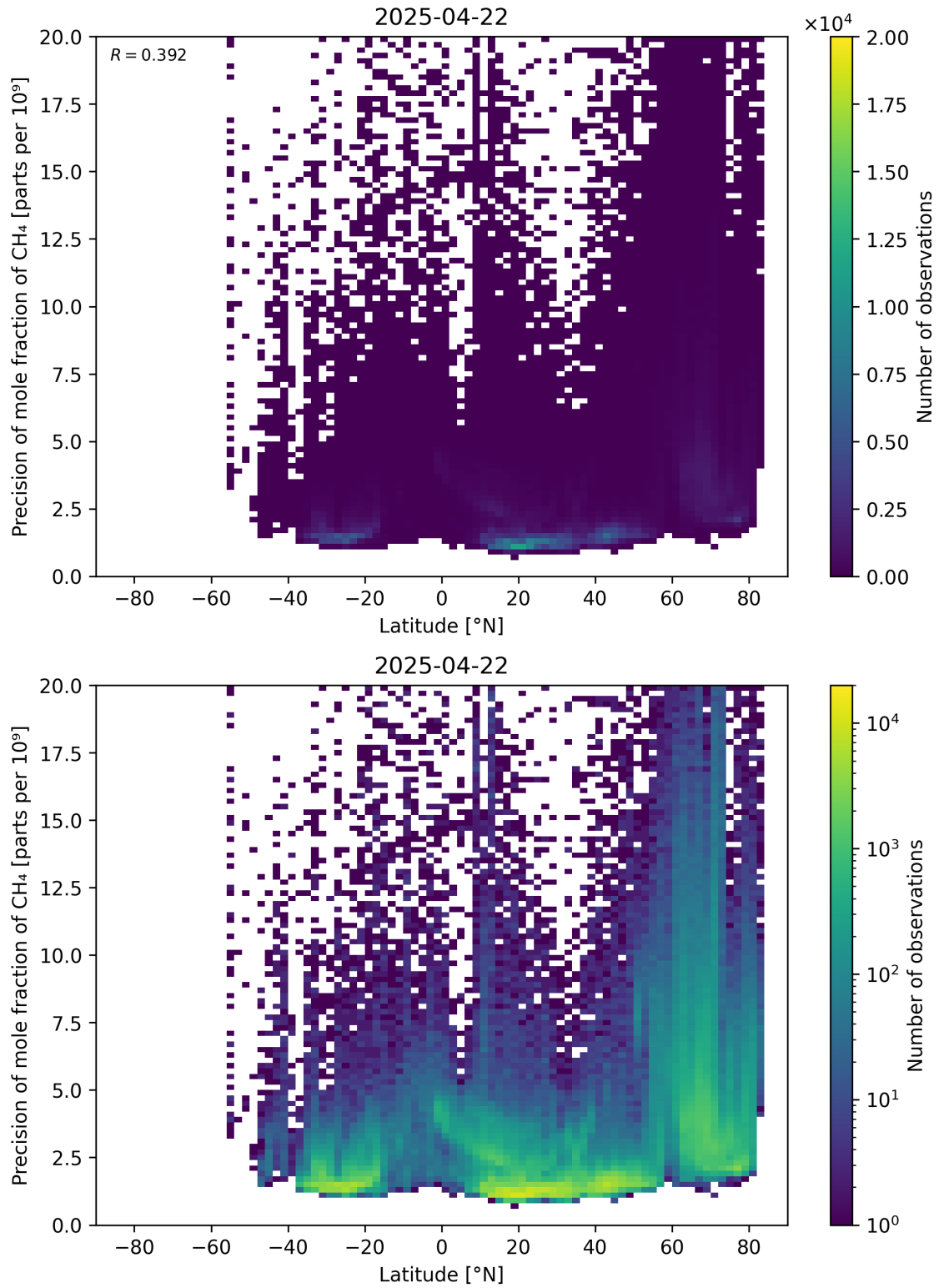
Figure 59: Scatter density plot of “Latitude” against “Precision of mole fraction of \text{CH}_4 ” for 2025-04-21 to 2025-04-23.
