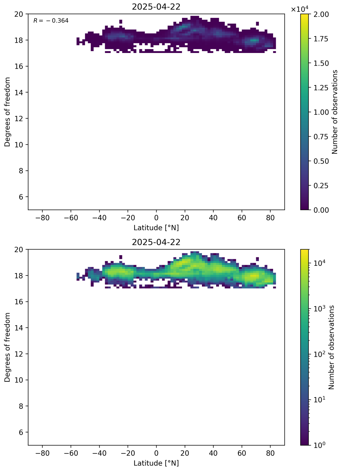
Figure 55: Scatter density plot of “Latitude” against “Degrees of freedom” for 2025-04-21 to 2025-04-23.
