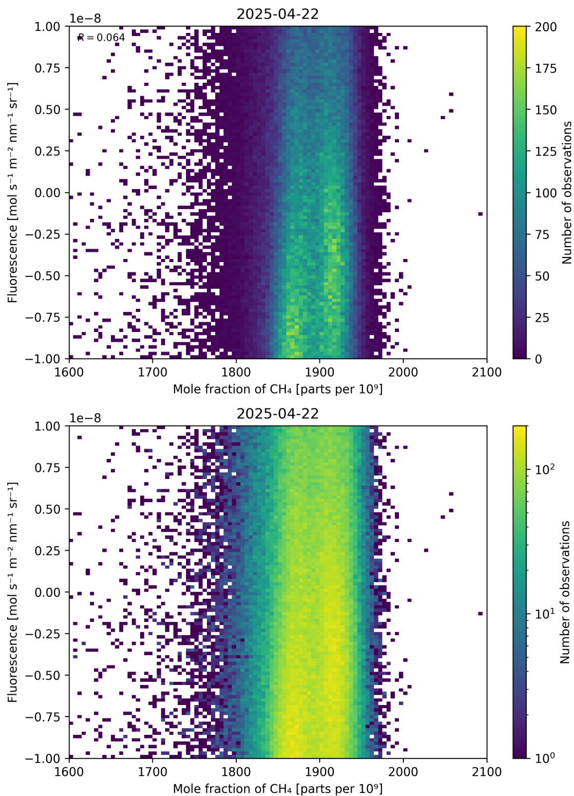
Figure 73: Scatter density plot of “Mole fraction of \text{CH}_4 ” against “Fluorescence” for 2025-04-21 to 2025-04-23.
