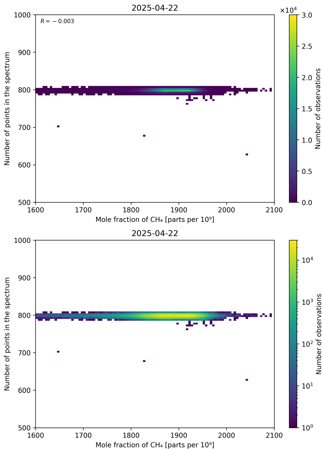
Figure 77: Scatter density plot of “Mole fraction of CH 4 ” against “Number of points in the spectrum” for 2025-04-21 to 2025-04-23.
