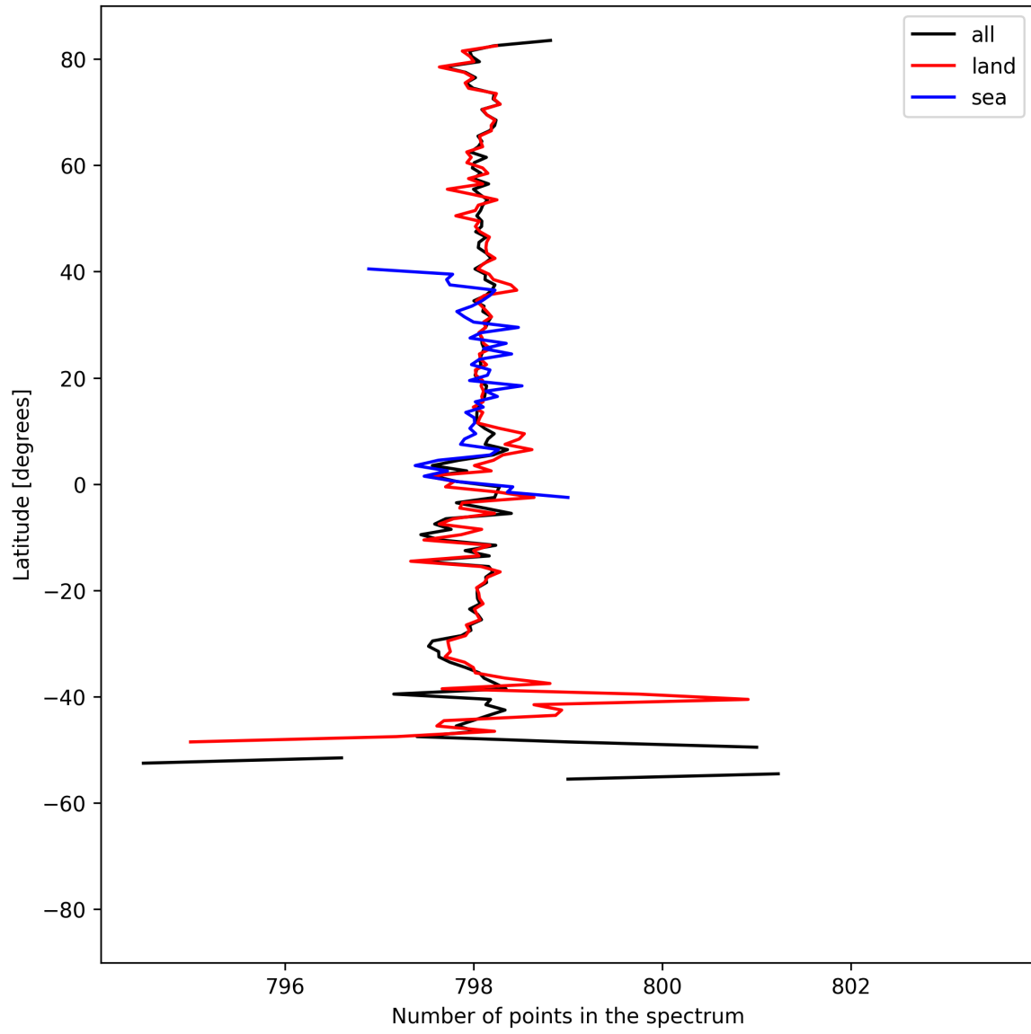
Figure 15: Zonal average of “Number of points in the spectrum” for 2025-04-21 to 2025-04-23.
