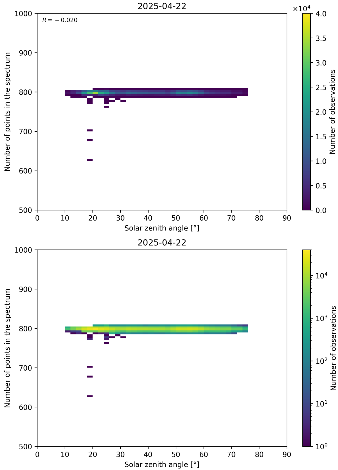
Figure 103: Scatter density plot of “Solar zenith angle” against “Number of points in the spectrum” for 2025-04-21 to 2025-04-23.
