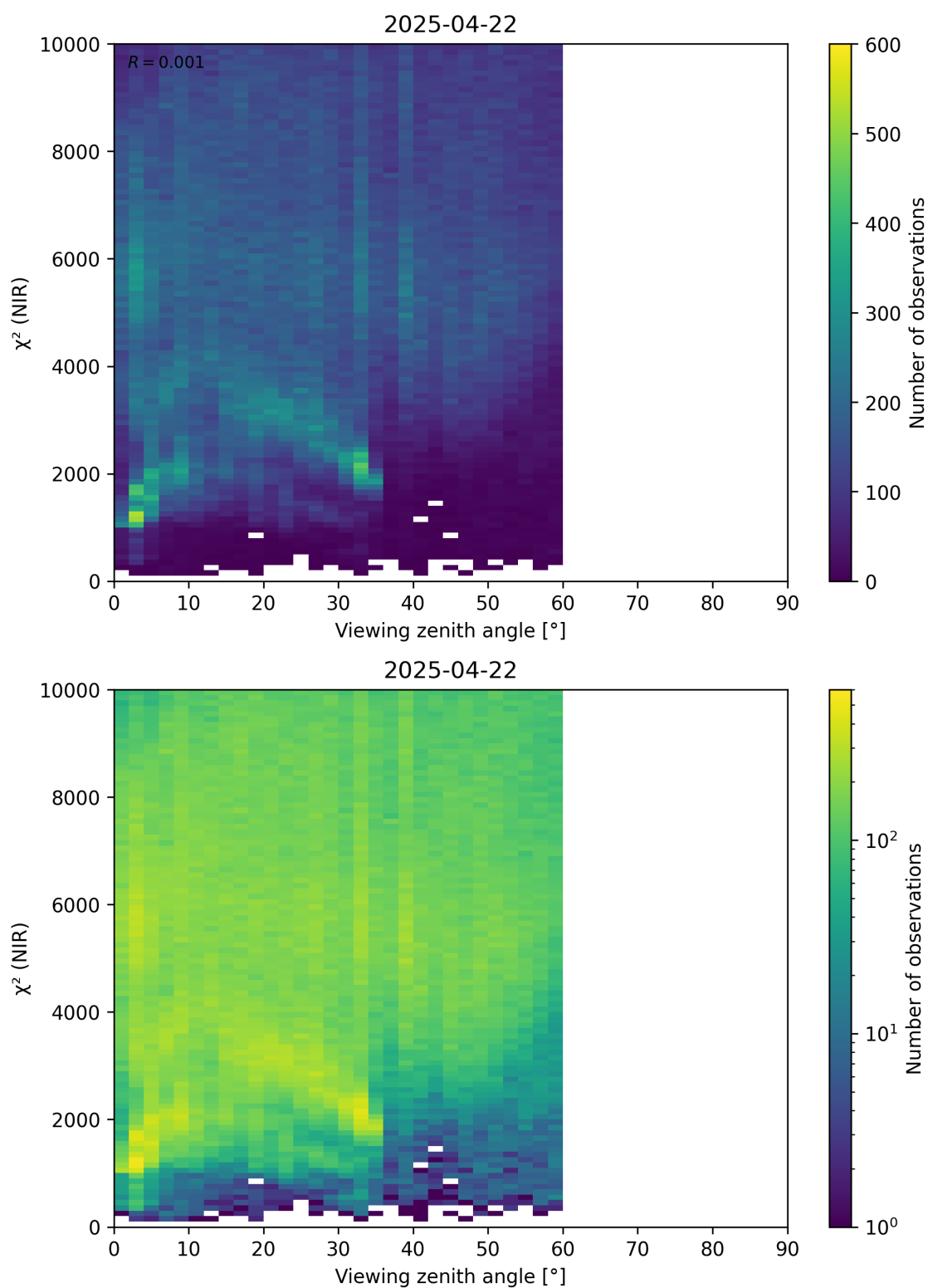
Figure 105: Scatter density plot of “Viewing zenith angle” against “ \chi^2 (NIR)” for 2025-04-21 to 2025-04-23.
