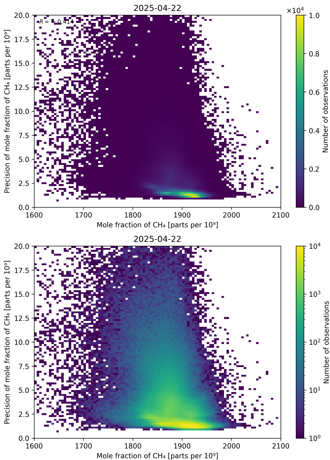
Figure 75: Scatter density plot of “Mole fraction of CH 4 ” against “Precision of mole fraction of CH 4 ” for 2025-04-21 to 2025-04-23.
