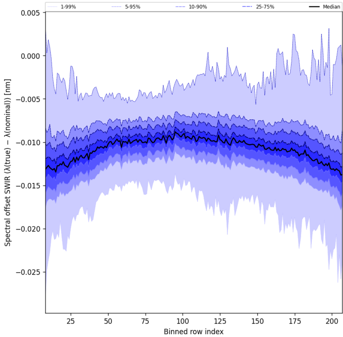
Figure 38: Along track statistics of “Spectral offset SWIR ( \lambda_{\text{true}} - \lambda_{\text{nominal}} )” for 2025-04-21 to 2025-04-23
