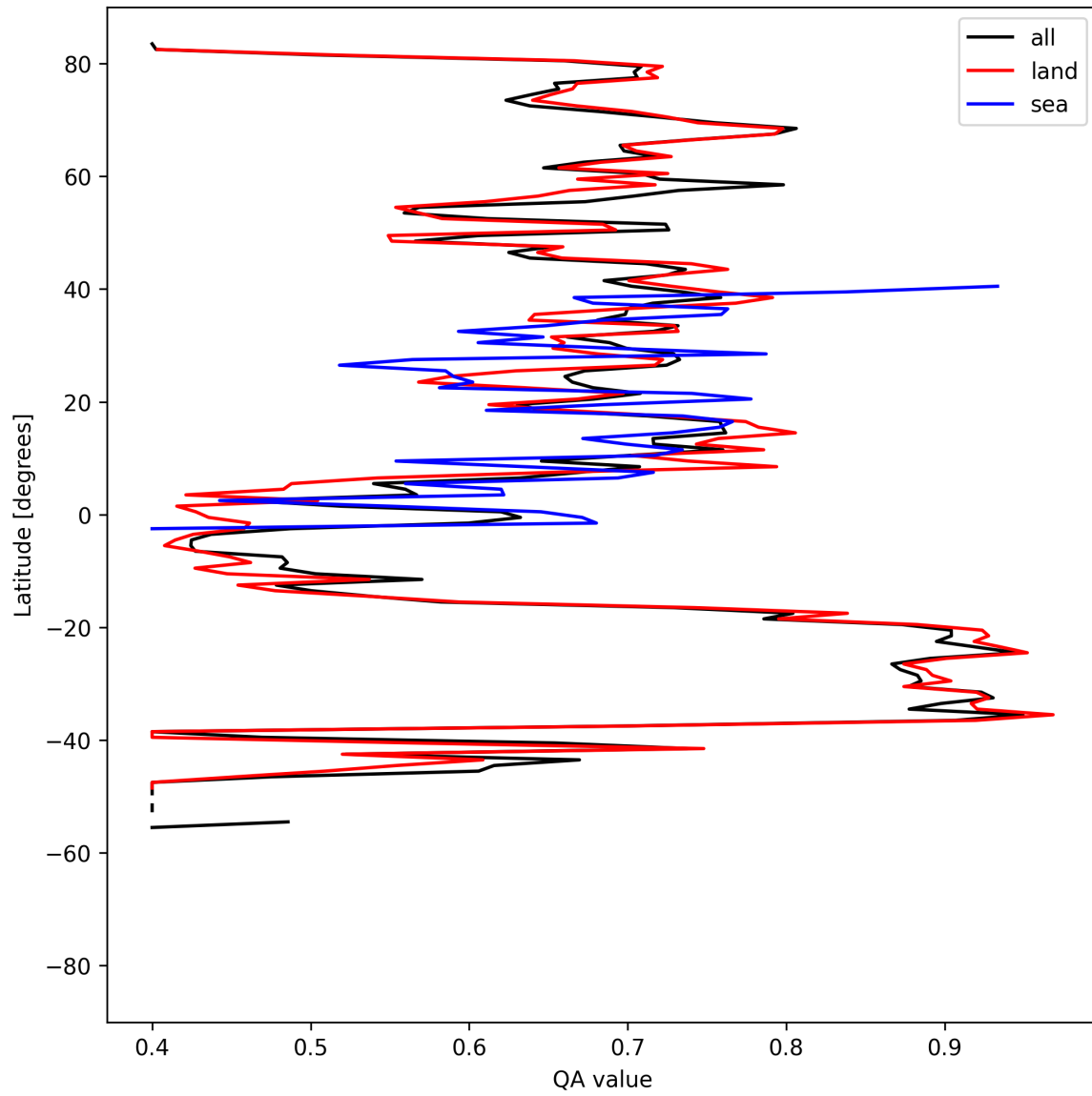
Figure 11: Zonal average of “QA value” for 2025-04-21 to 2025-04-23.
