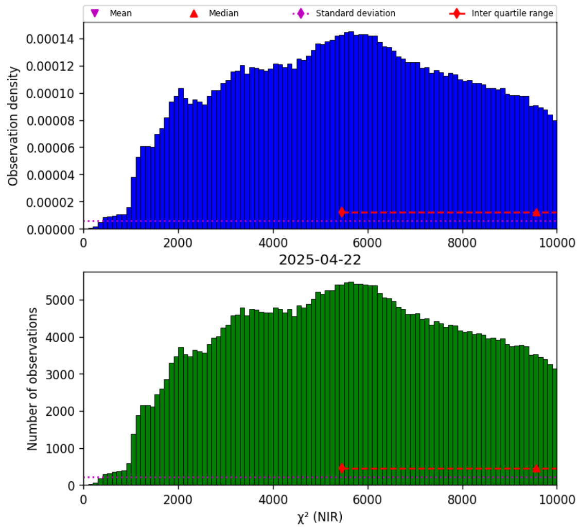
Figure 29: Histogram of " \chi^2 (NIR)" for 2025-04-21 to 2025-04-23
