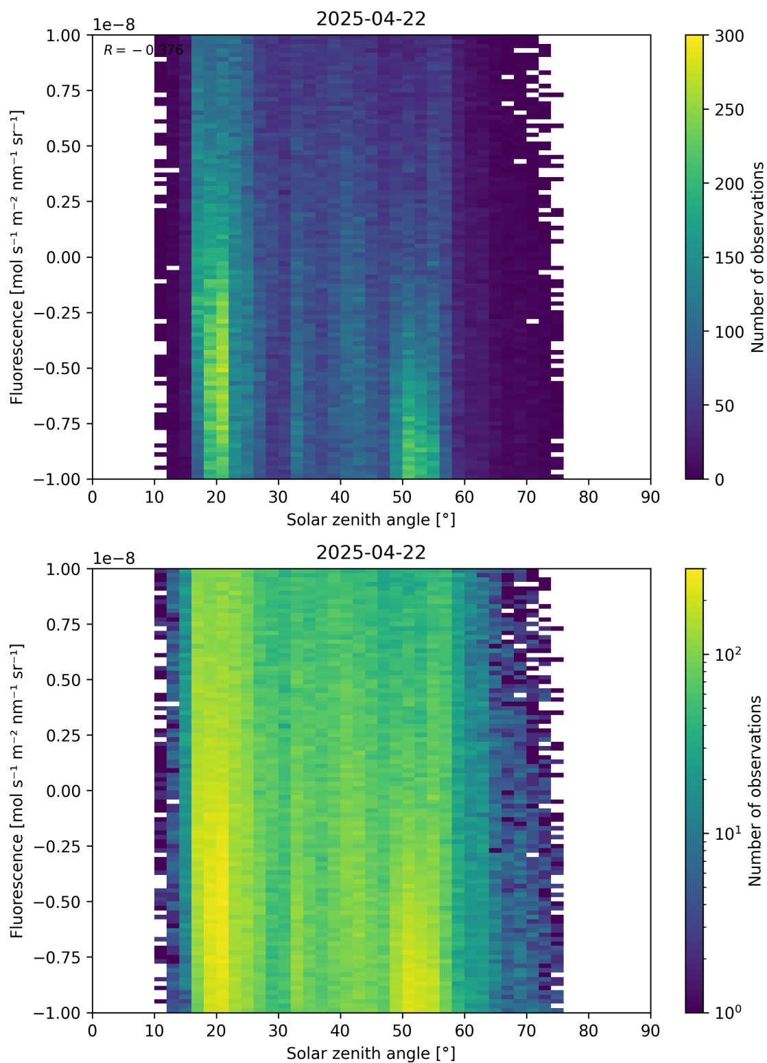
Figure 97: Scatter density plot of “Solar zenith angle” against “Fluorescence” for 2025-04-21 to 2025-04-23.
