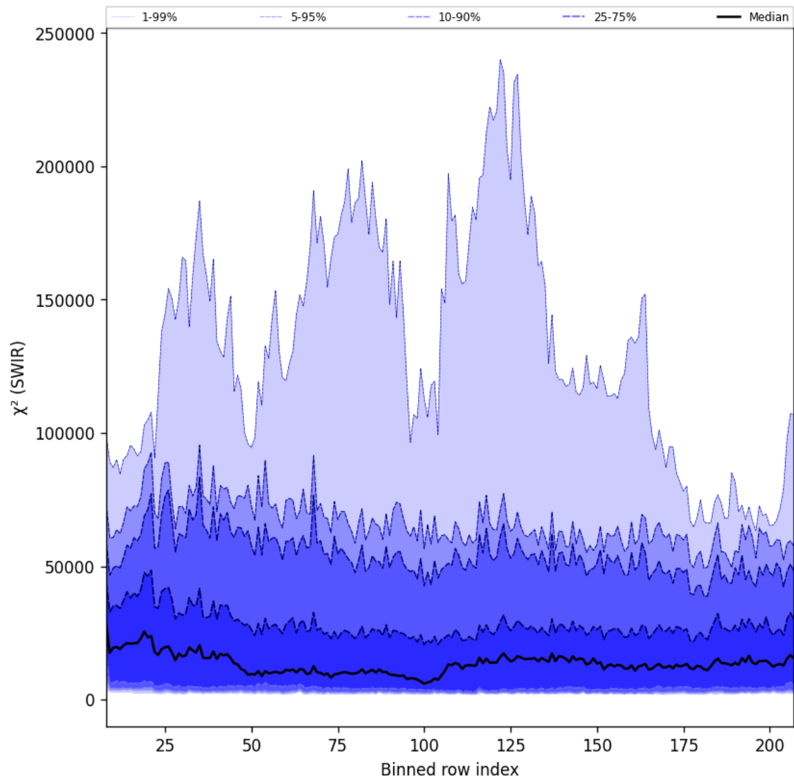
Figure 39: Along track statistics of “ \chi^2 (SWIR)” for 2025-04-21 to 2025-04-23
