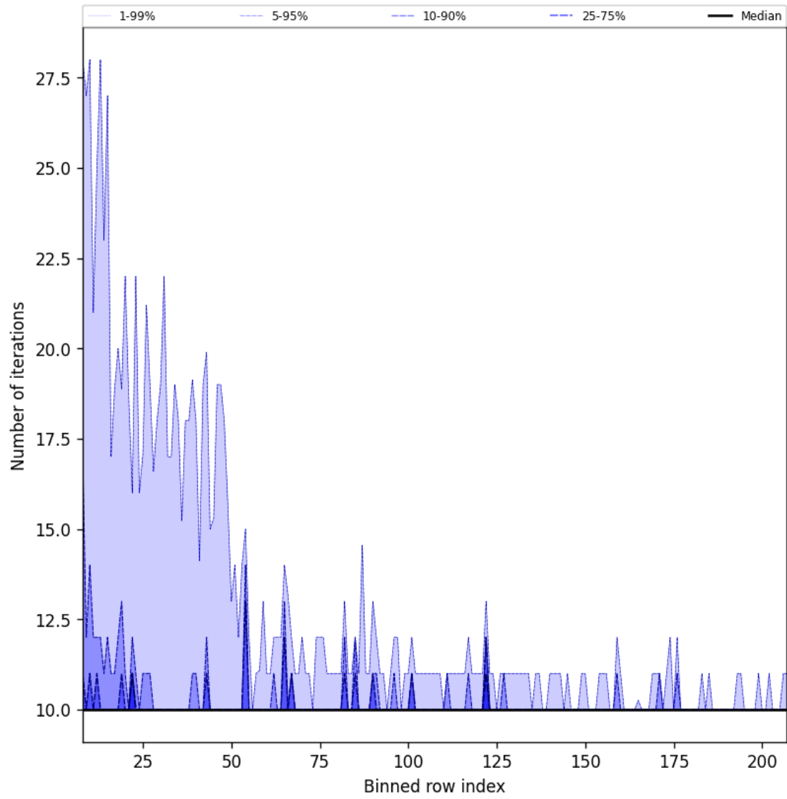
Figure 42: Along track statistics of “Number of iterations” for 2025-04-21 to 2025-04-23
