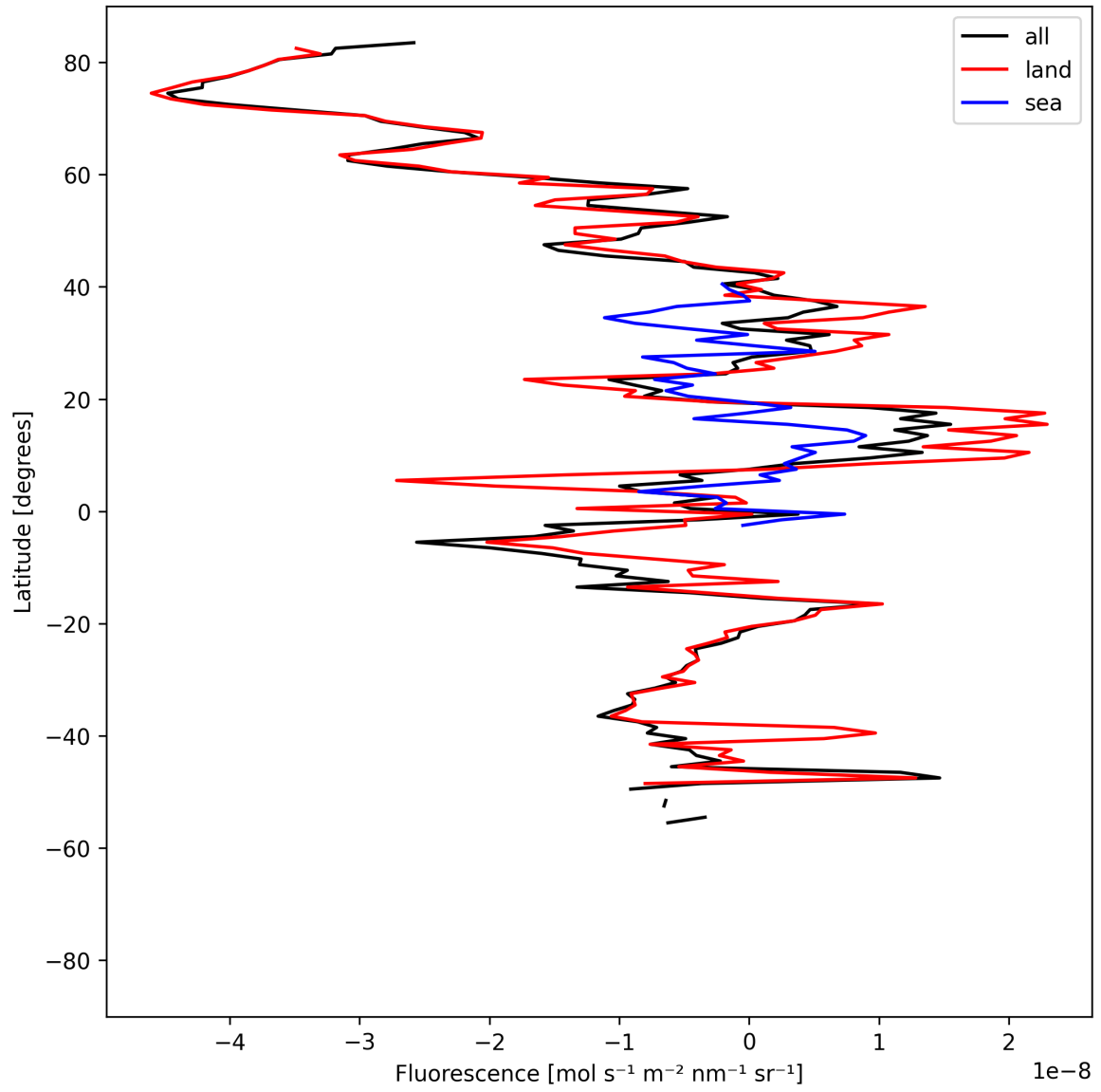
Figure 21: Zonal average of “Fluorescence” for 2025-04-21 to 2025-04-23.
