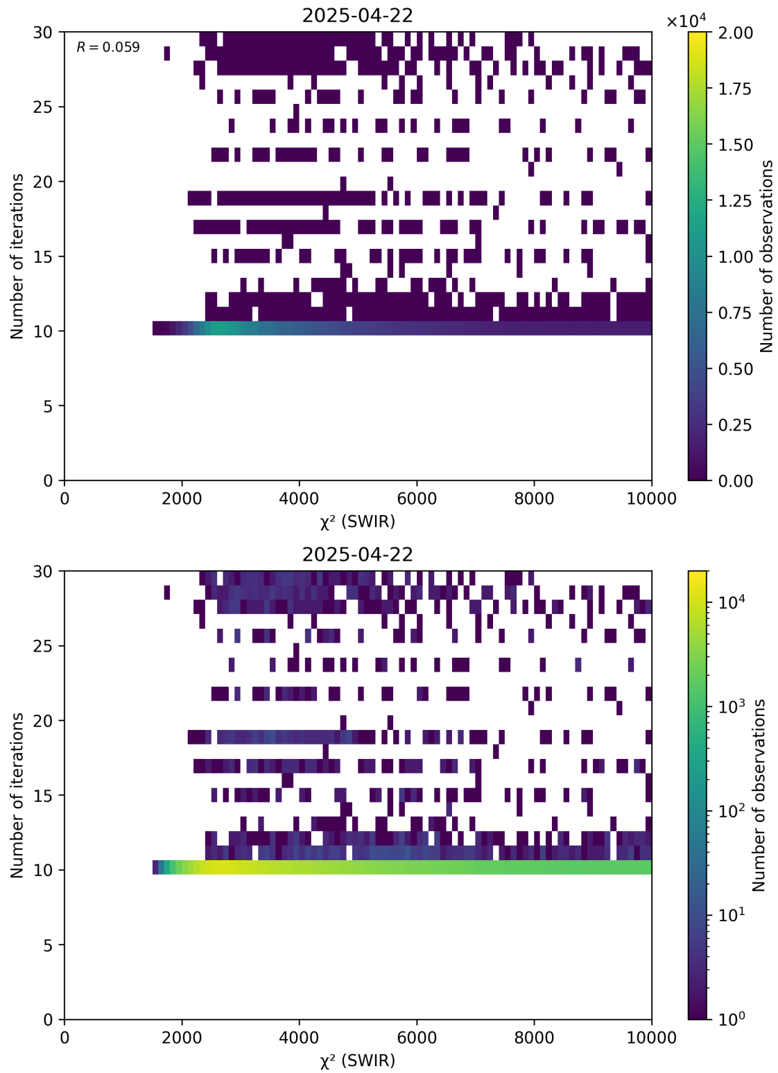
Figure 50: Scatter density plot of “ \chi^2 (SWIR)” against “Number of iterations” for 2025-04-21 to 2025-04-23.
