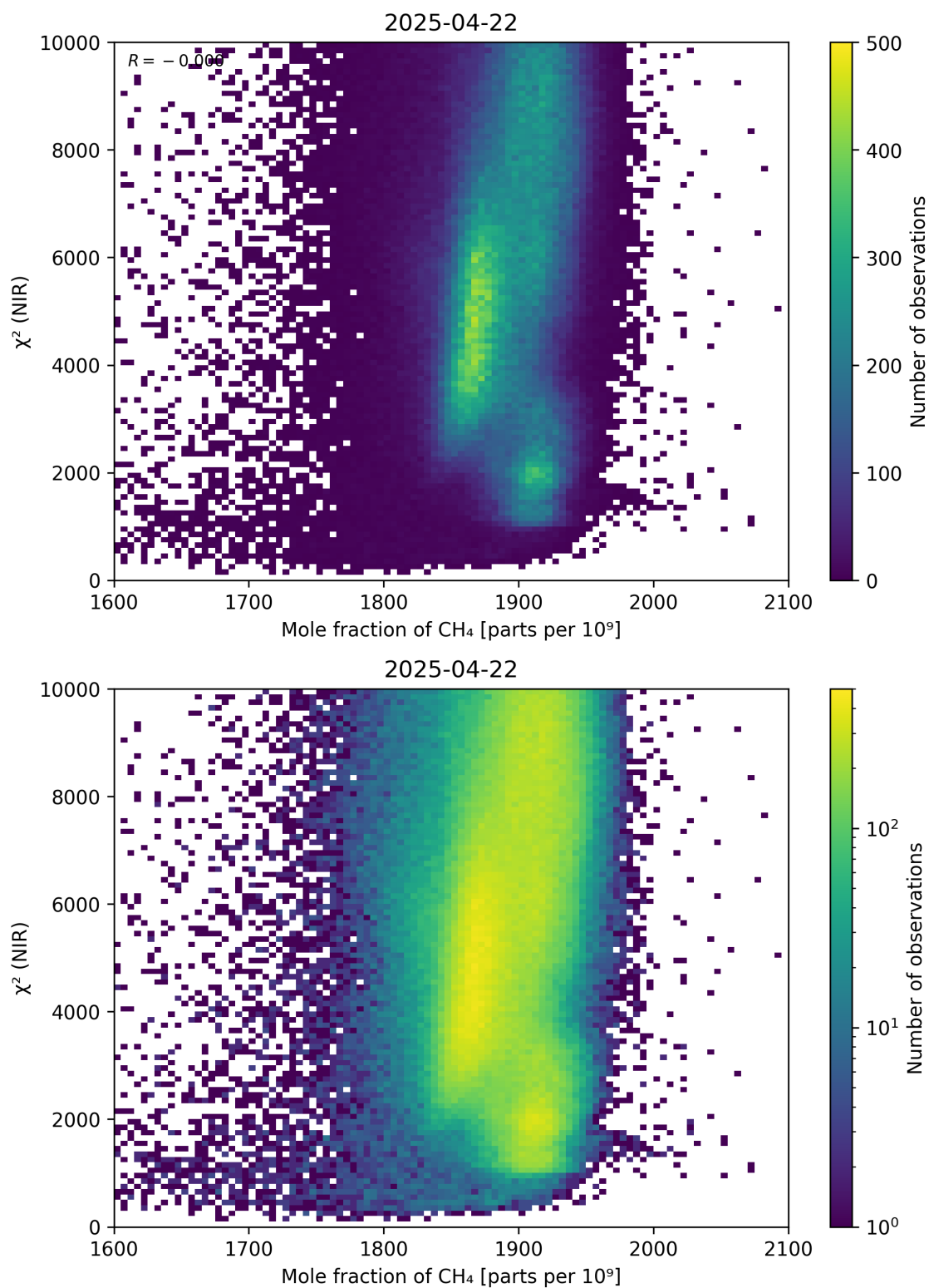
Figure 70: Scatter density plot of “Mole fraction of \text{CH}_4 ” against “ \chi^2 (NIR)” for 2025-04-21 to 2025-04-23.
