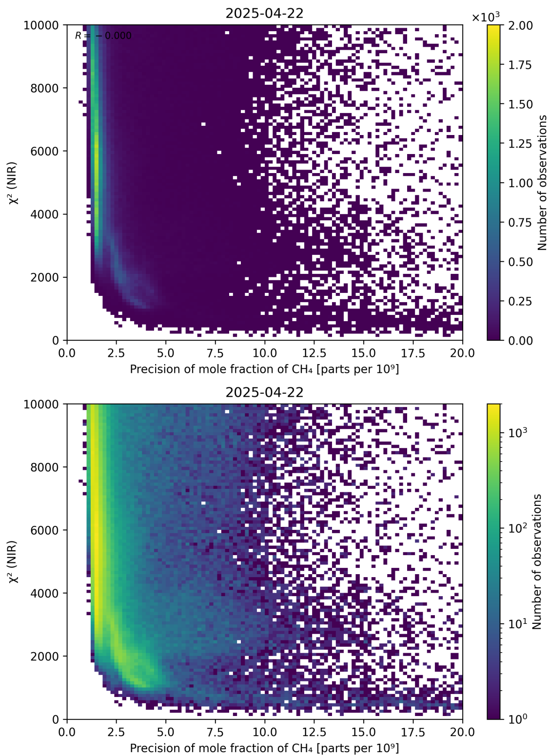
Figure 78: Scatter density plot of “Precision of mole fraction of CH 4 ” against “ \chi^2 (NIR)” for 2025-04-21 to 2025-04-23.
