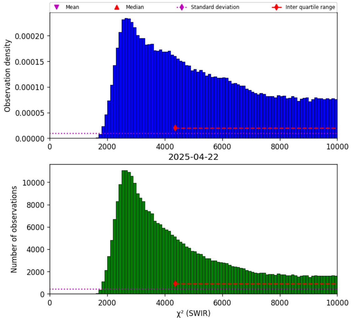
Figure 28: Histogram of “ \chi^2 (SWIR)” for 2025-04-21 to 2025-04-23
