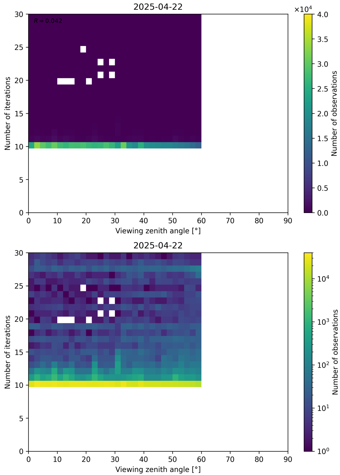
Figure 113: Scatter density plot of “Viewing zenith angle” against “Number of iterations” for 2025-04-21 to 2025-04-23.
