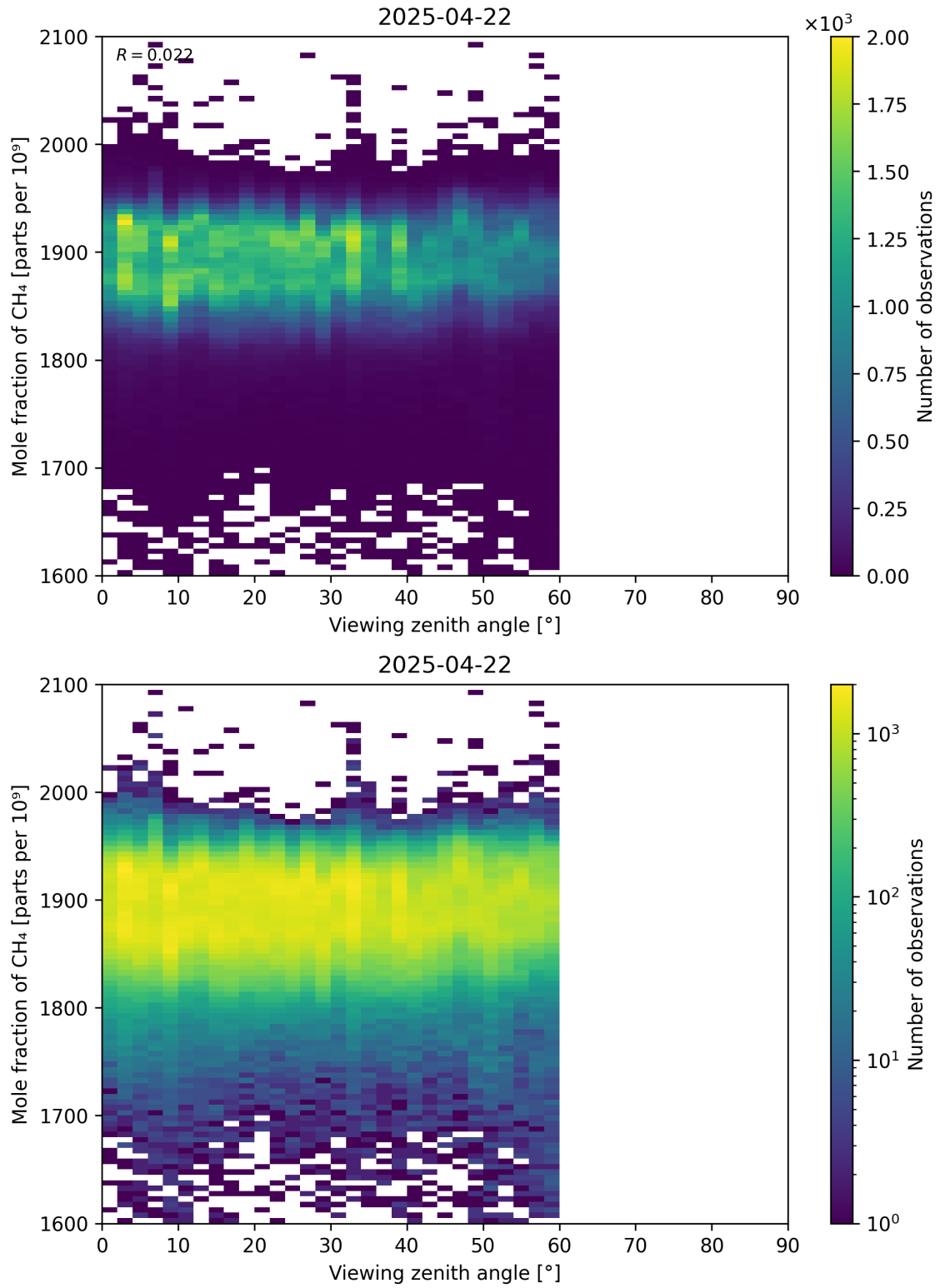
Figure 110: Scatter density plot of “Viewing zenith angle” against “Mole fraction of CH 4 ” for 2025-04-21 to 2025-04-23.
