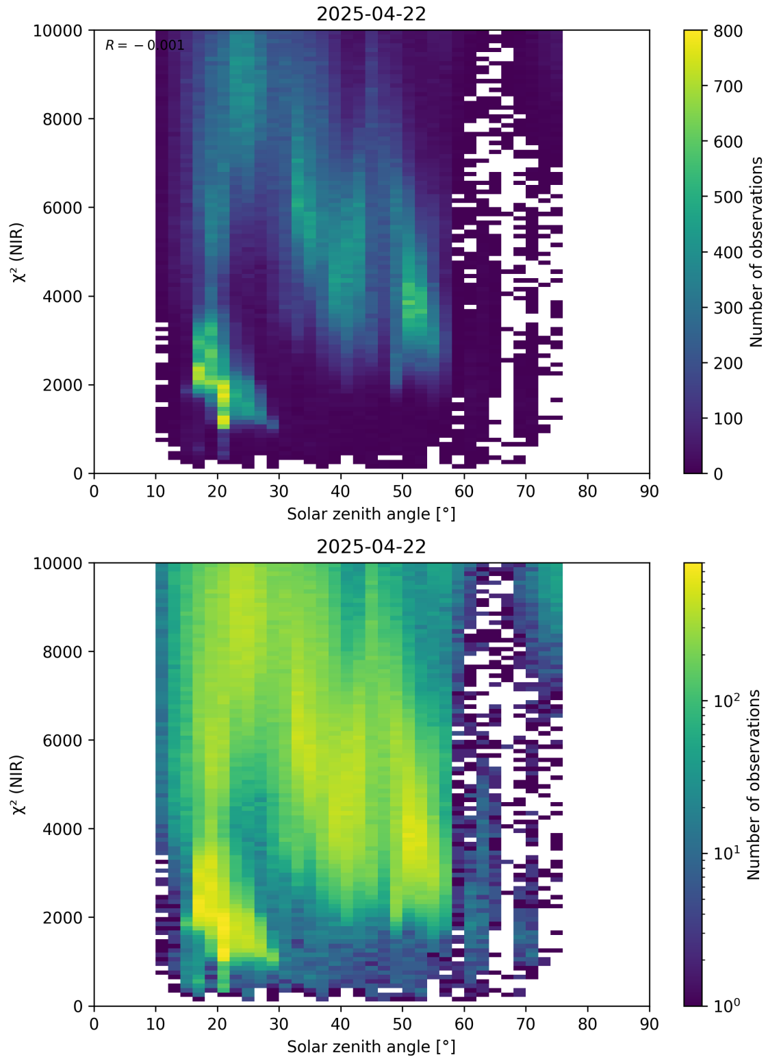
Figure 94: Scatter density plot of “Solar zenith angle” against “ \chi^2 (NIR)” for 2025-04-21 to 2025-04-23.
