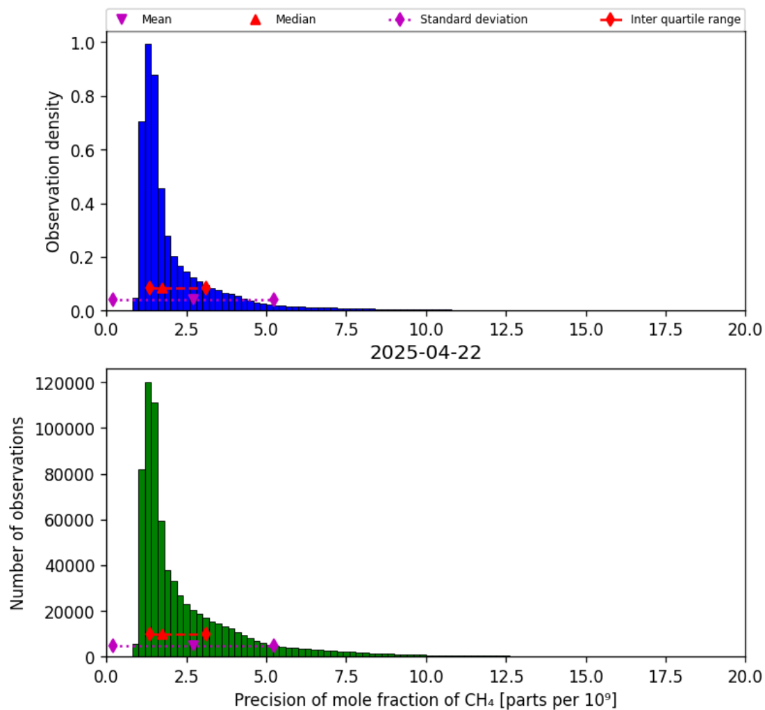
Figure 24: Histogram of “Precision of mole fraction of CH 4 ” for 2025-04-21 to 2025-04-23
