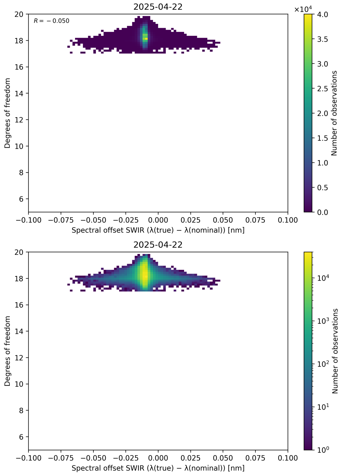
Figure 119: Scatter density plot of “Spectral offset SWIR ( \lambda_{\text{true}} - \lambda_{\text{nominal}} )” against “Degrees of freedom” for 2025-04-21 to 2025-04-23.
