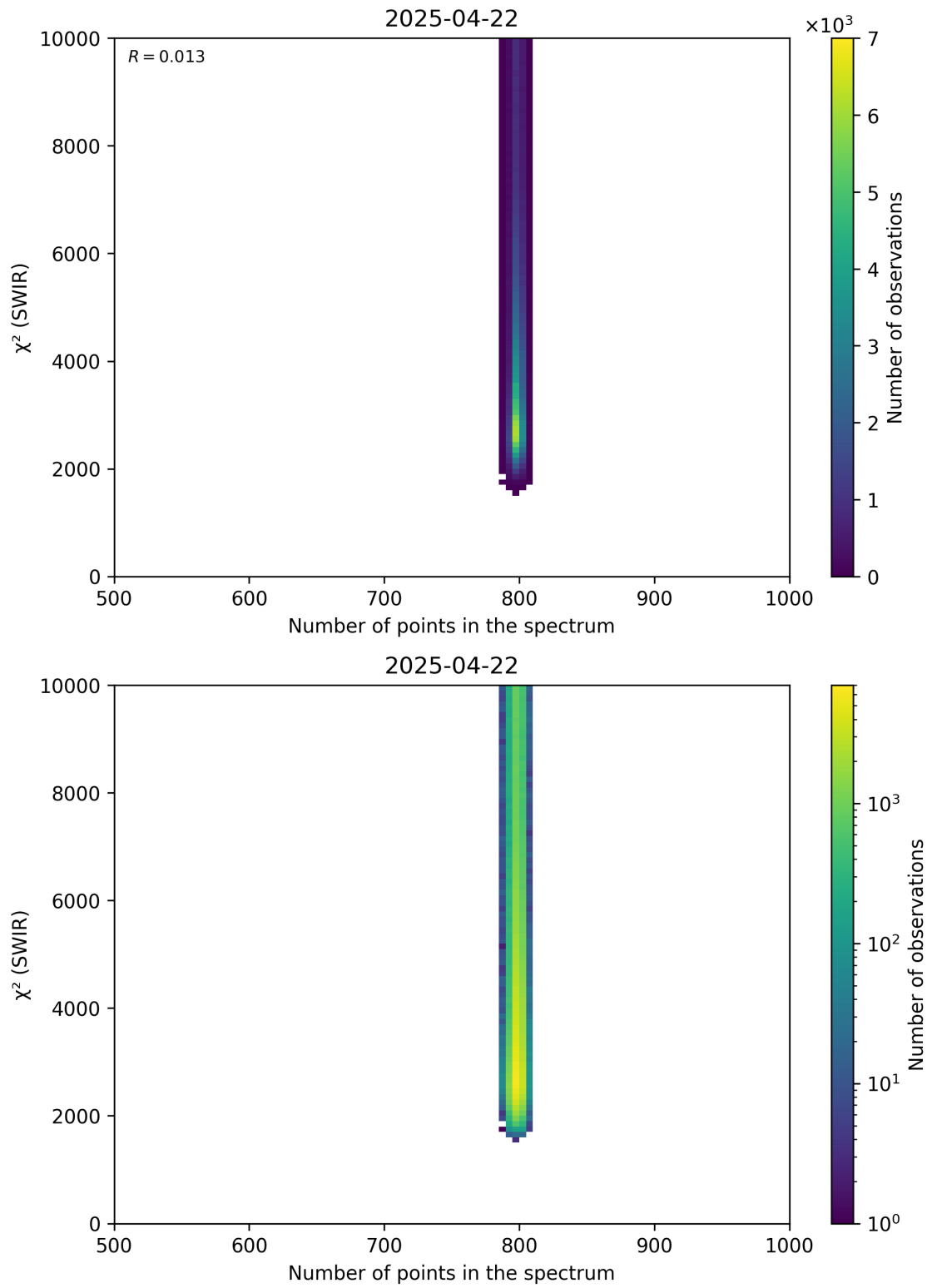
Figure 89: Scatter density plot of “Number of points in the spectrum” against “ \chi^2 (SWIR)” for 2025-04-21 to 2025-04-23.
