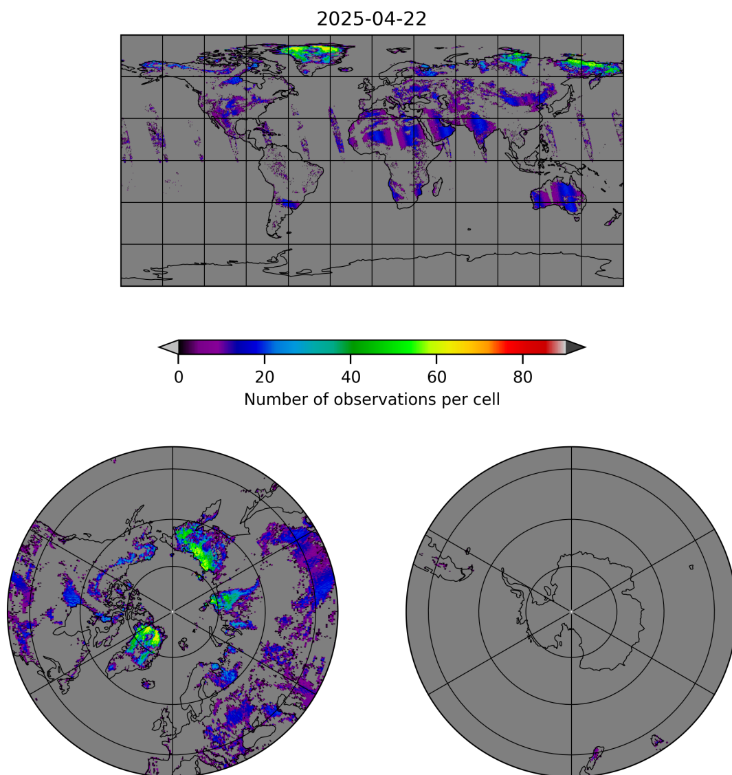
Figure 10: Map of the number of observations for 2025-04-21 to 2025-04-23
