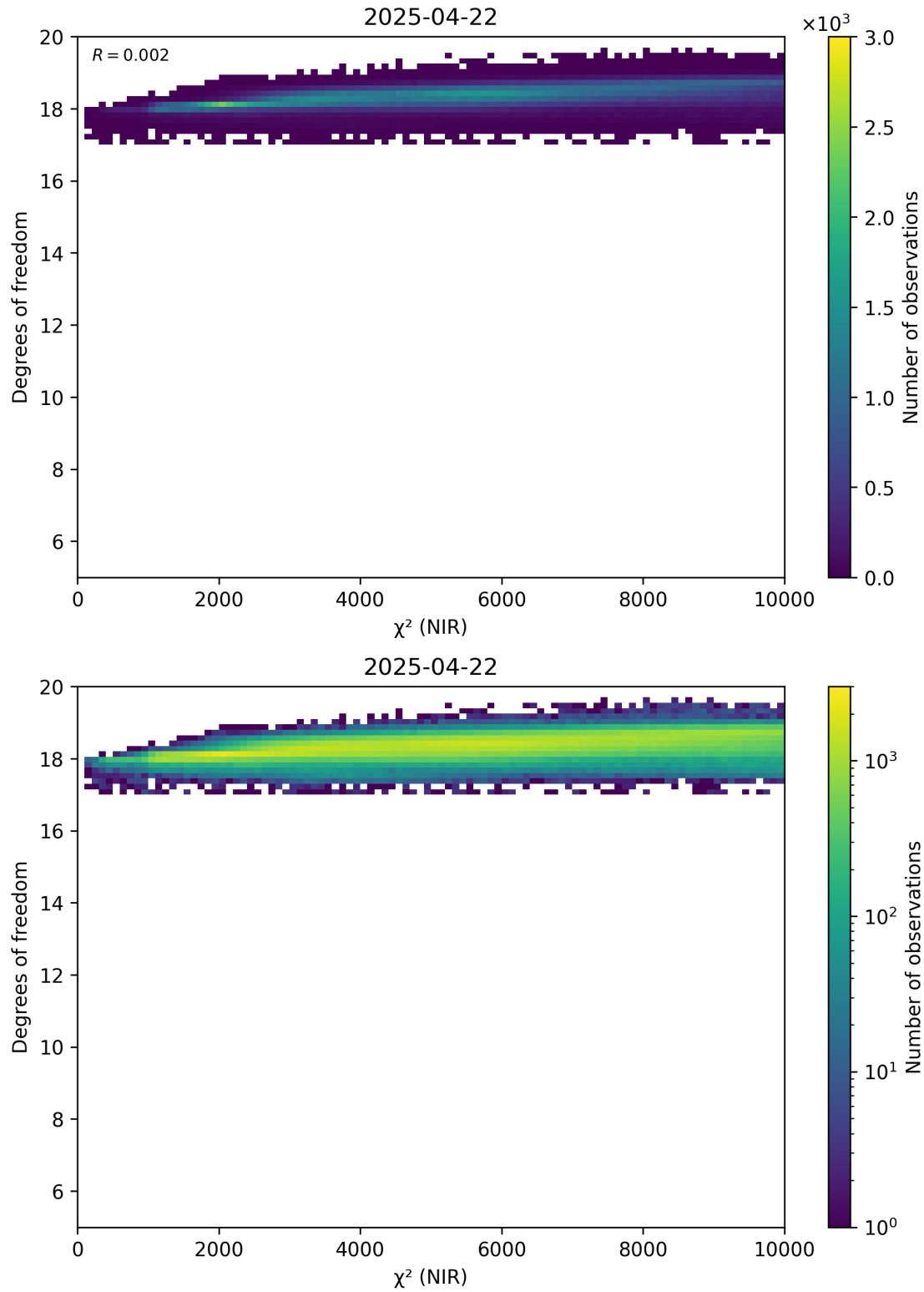
Figure 44: Scatter density plot of “ \chi^2 (NIR)” against “Degrees of freedom” for 2025-04-21 to 2025-04-23.
