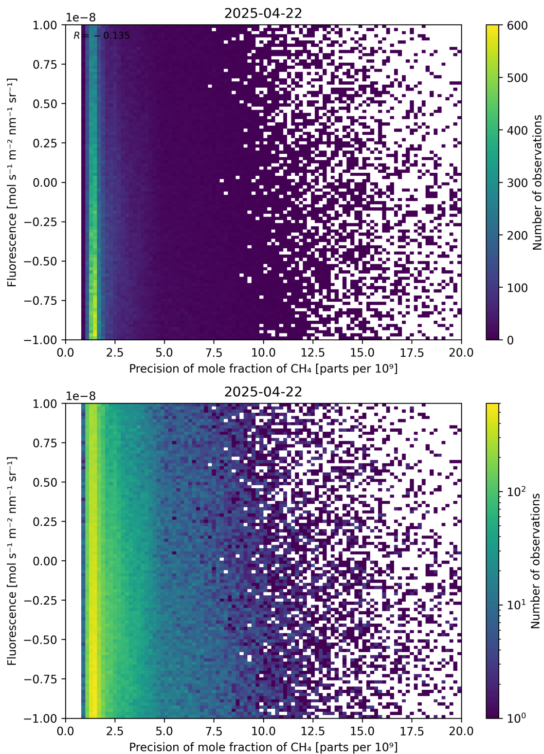
Figure 81: Scatter density plot of “Precision of mole fraction of CH 4 ” against “Fluorescence” for 2025-04-21 to 2025-04-23.
