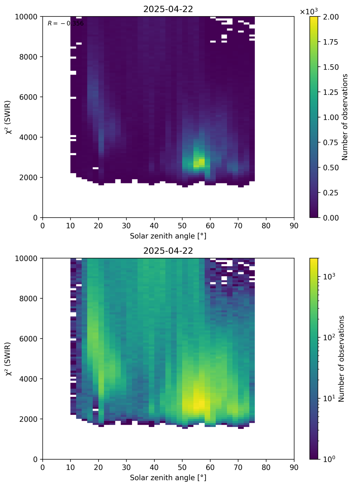
Figure 95: Scatter density plot of “Solar zenith angle” against “ \chi^2 (SWIR)” for 2025-04-21 to 2025-04-23.
