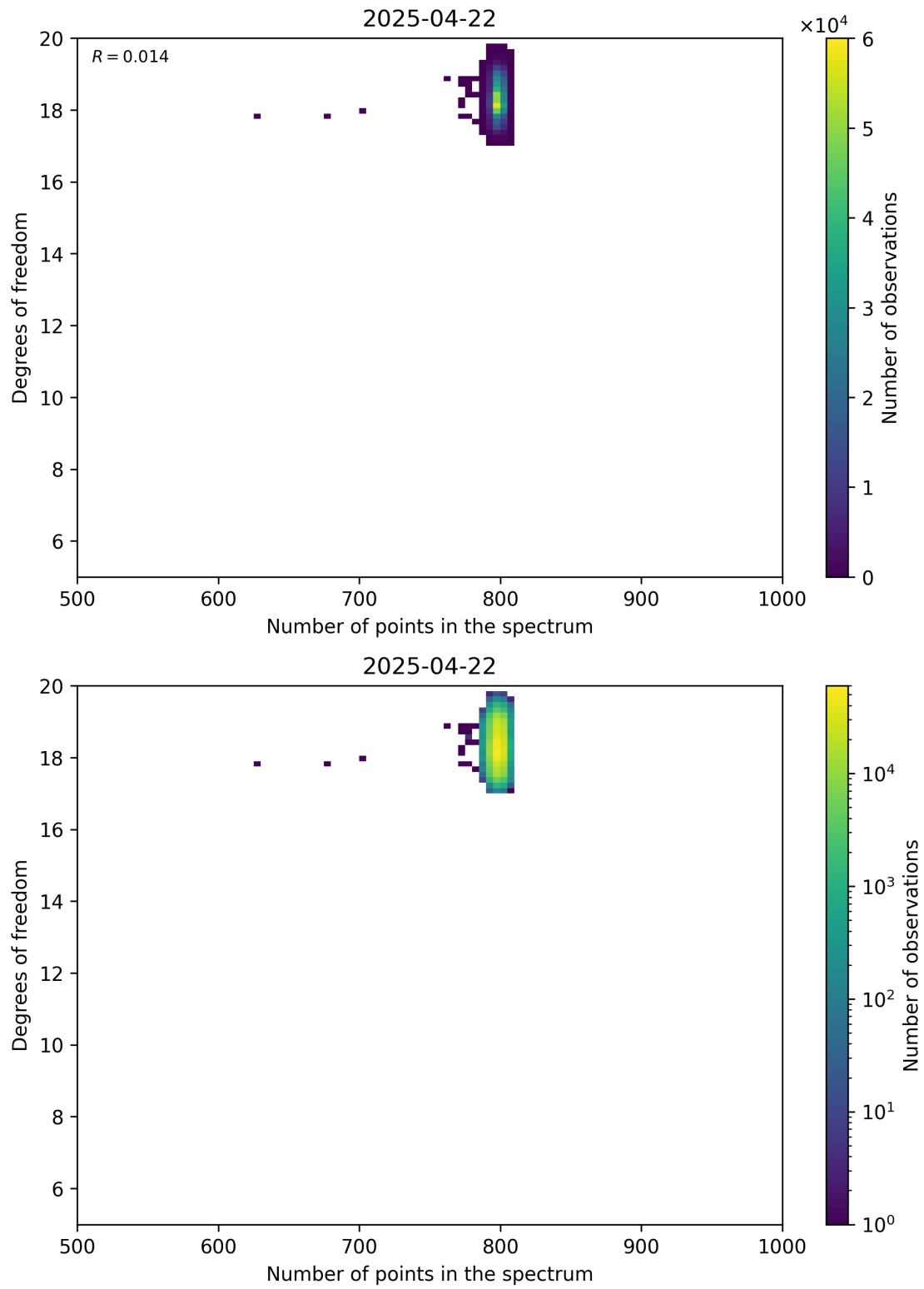
Figure 90: Scatter density plot of “Number of points in the spectrum” against “Degrees of freedom” for 2025-04-21 to 2025-04-23.
