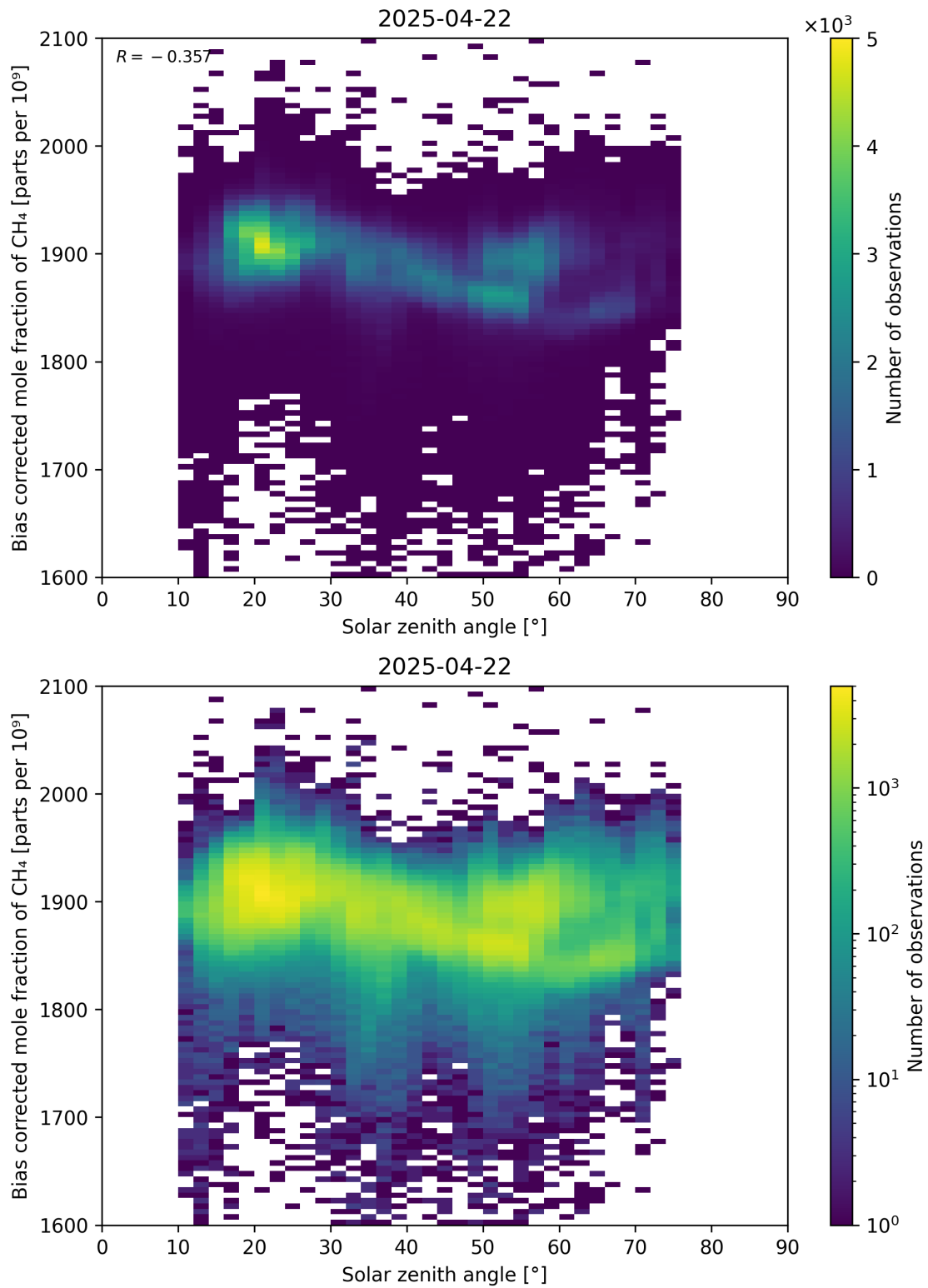
Figure 100: Scatter density plot of “Solar zenith angle” against “Bias corrected mole fraction of CH 4 ” for 2025-04-21 to 2025-04-23.
