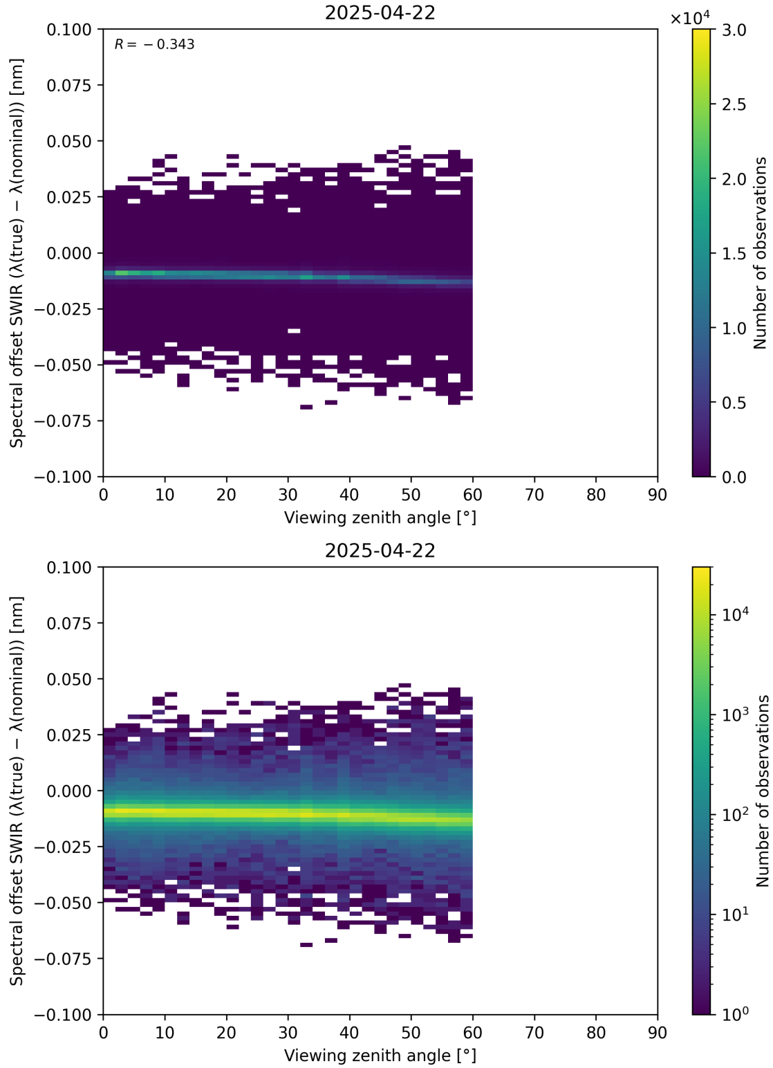
Figure 116: Scatter density plot of “Viewing zenith angle” against “Spectral offset SWIR ( \lambda_{\text{true}} - \lambda_{\text{nominal}} )” for 2025-04-21 to 2025-04-23.
