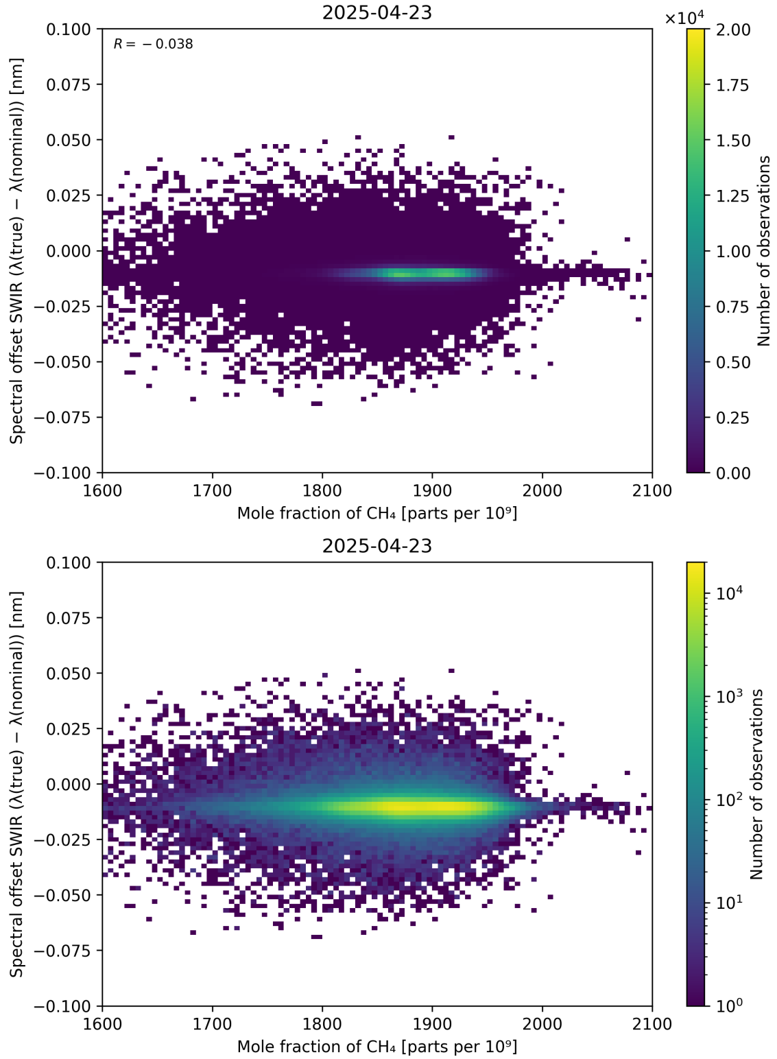
Figure 86: Scatter density plot of “Mole fraction of CH 4 ” against “Spectral offset SWIR ( \lambda_{\text{true}} - \lambda_{\text{nominal}} )” for 2025-04-22 to 2025-04-24.
