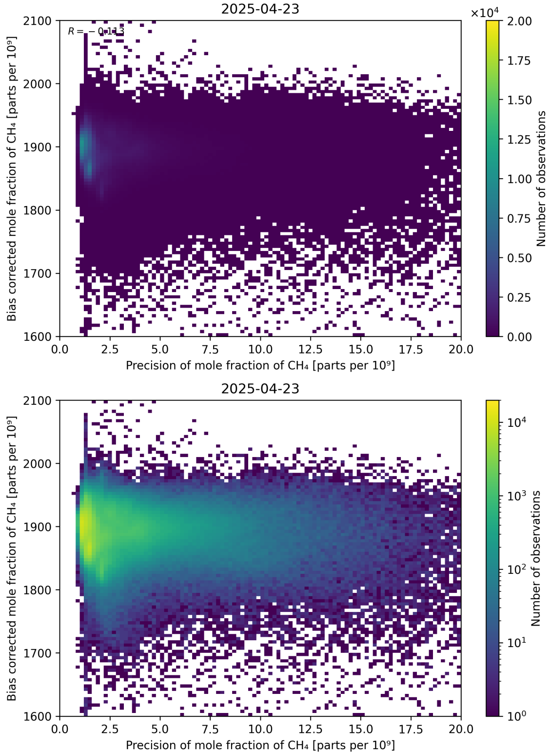
Figure 82: Scatter density plot of “Precision of mole fraction of CH 4 ” against “Bias corrected mole fraction of CH 4 ” for 2025-04-22 to 2025-04-24.
