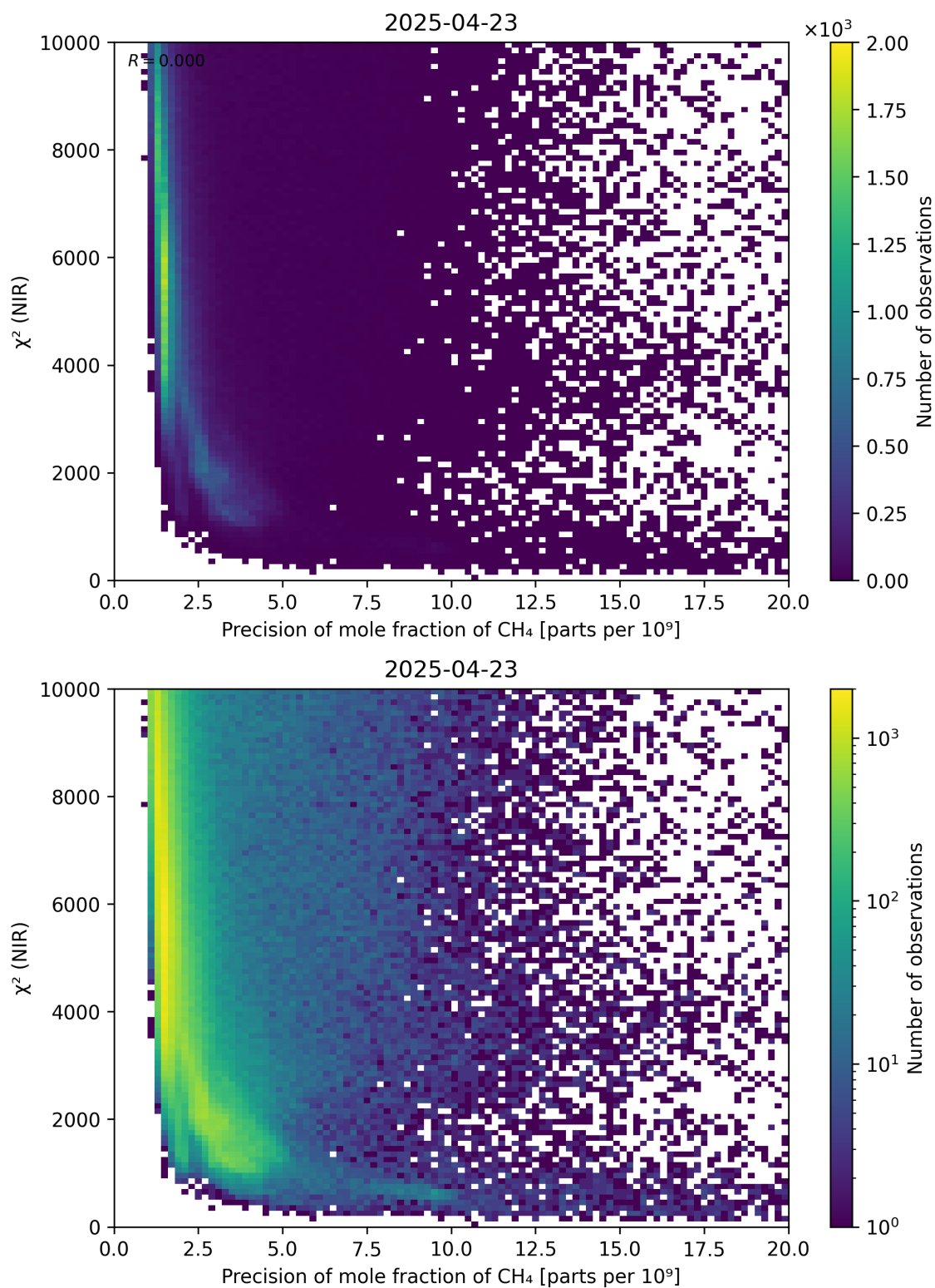
Figure 78: Scatter density plot of “Precision of mole fraction of CH 4 ” against “ \chi^2 (NIR)” for 2025-04-22 to 2025-04-24.
