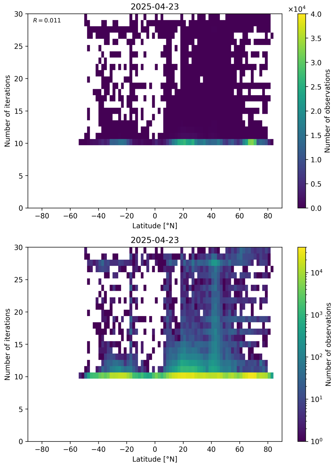
Figure 60: Scatter density plot of “Latitude” against “Number of iterations” for 2025-04-22 to 2025-04-24.
