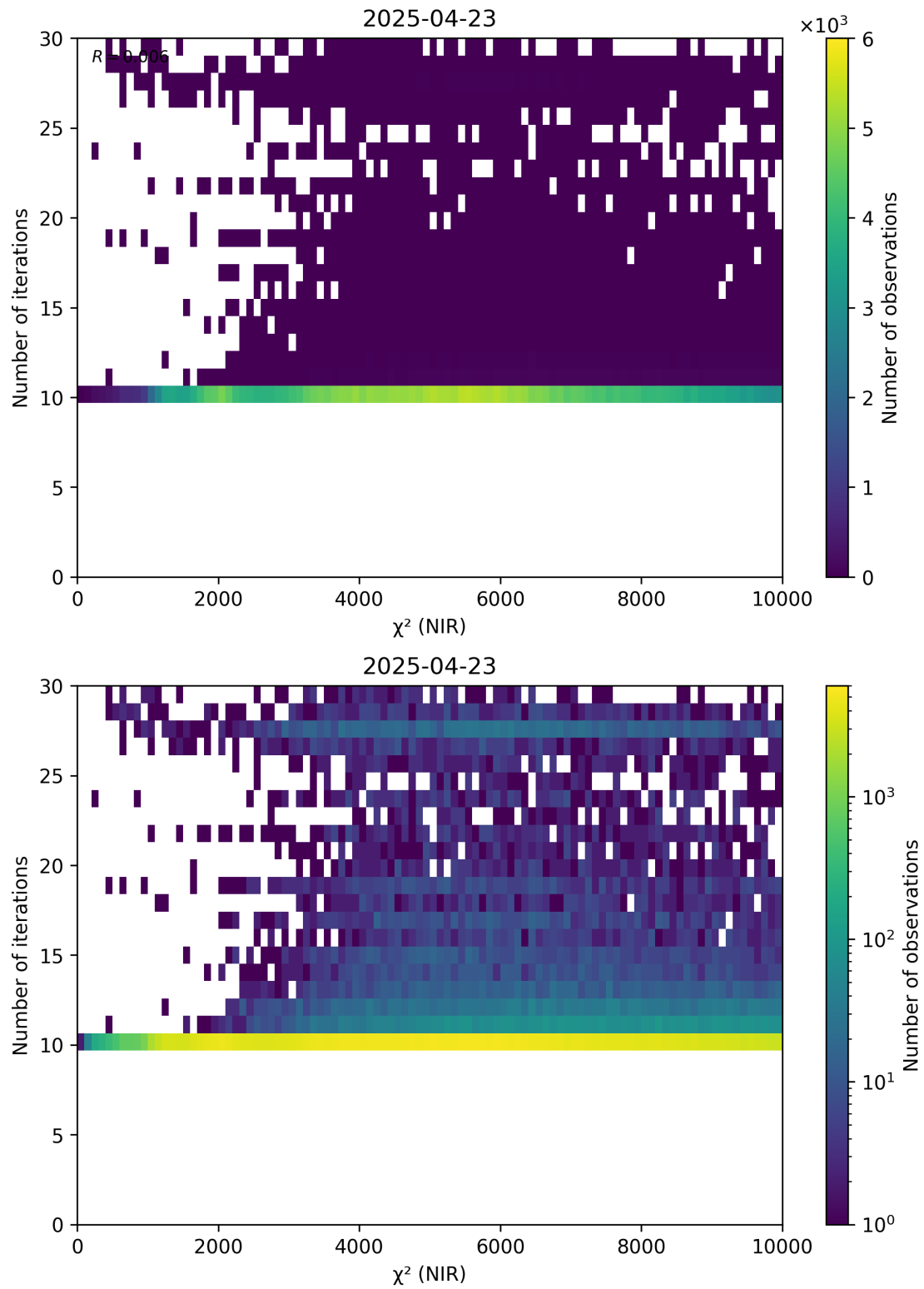
Figure 46: Scatter density plot of “ \chi^2 (NIR)” against “Number of iterations” for 2025-04-22 to 2025-04-24.
