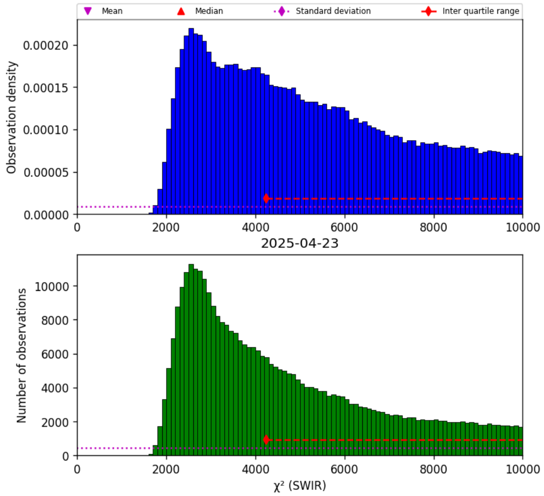
Figure 28: Histogram of “ \chi^2 (SWIR)” for 2025-04-22 to 2025-04-24
