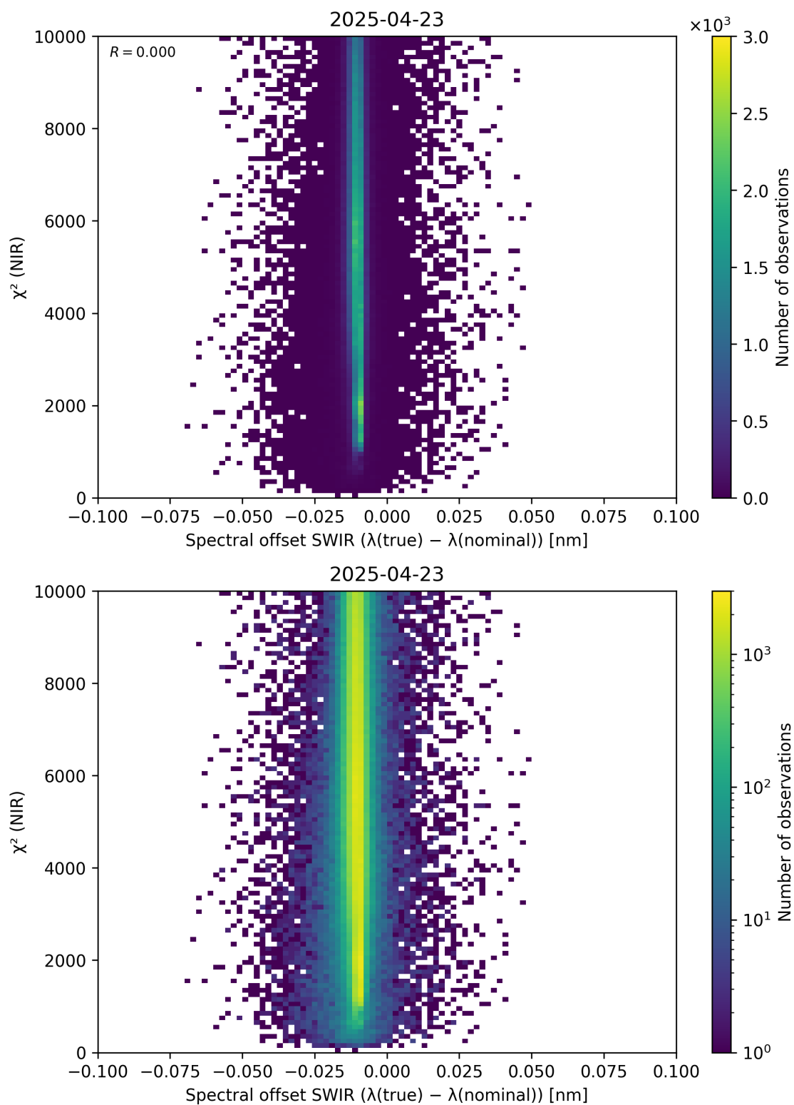
Figure 117: Scatter density plot of “Spectral offset SWIR ( \lambda_{\text{true}} - \lambda_{\text{nominal}} )” against “ \chi^2 (NIR)” for 2025-04-22 to 2025-04-24.
