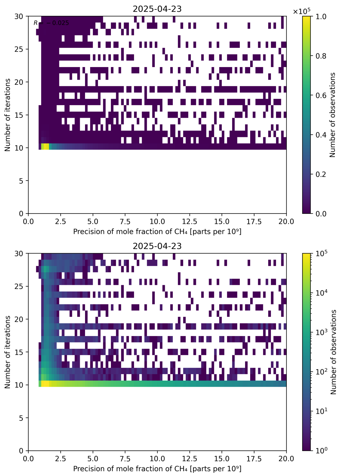
Figure 83: Scatter density plot of “Precision of mole fraction of CH 4 ” against “Number of iterations” for 2025-04-22 to 2025-04-24.
