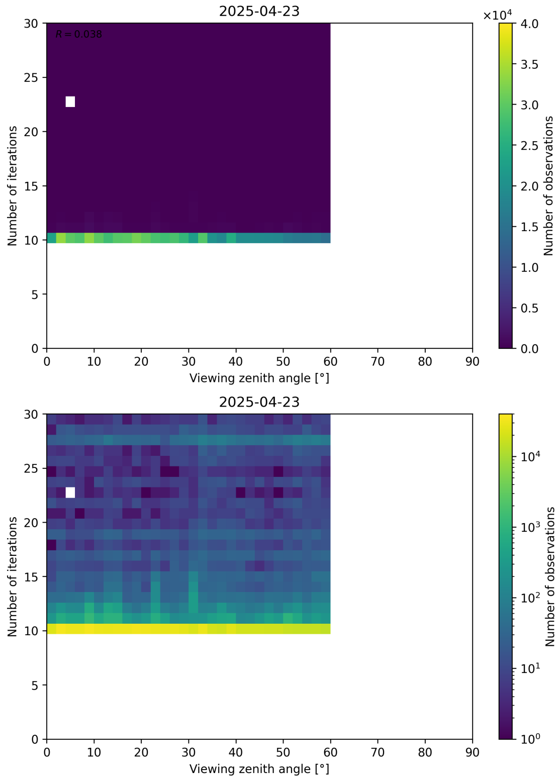
Figure 113: Scatter density plot of “Viewing zenith angle” against “Number of iterations” for 2025-04-22 to 2025-04-24.
