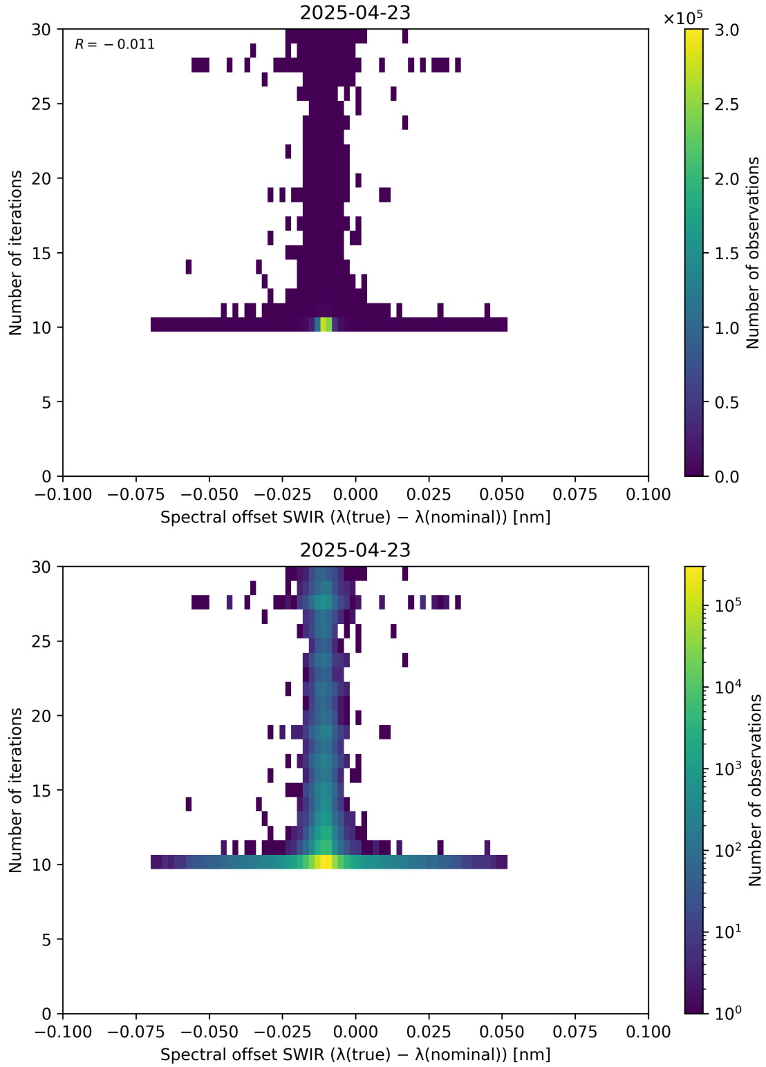
Figure 121: Scatter density plot of “Spectral offset SWIR ( \lambda_{\text{true}} - \lambda_{\text{nominal}} )” against “Number of iterations” for 2025-04-22 to 2025-04-24.
