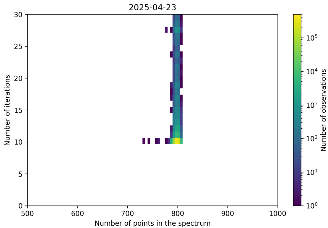
Figure 92: Scatter density plot of “Number of points in the spectrum” against “Number of iterations” for 2025-04-22 to 2025-04-24.
