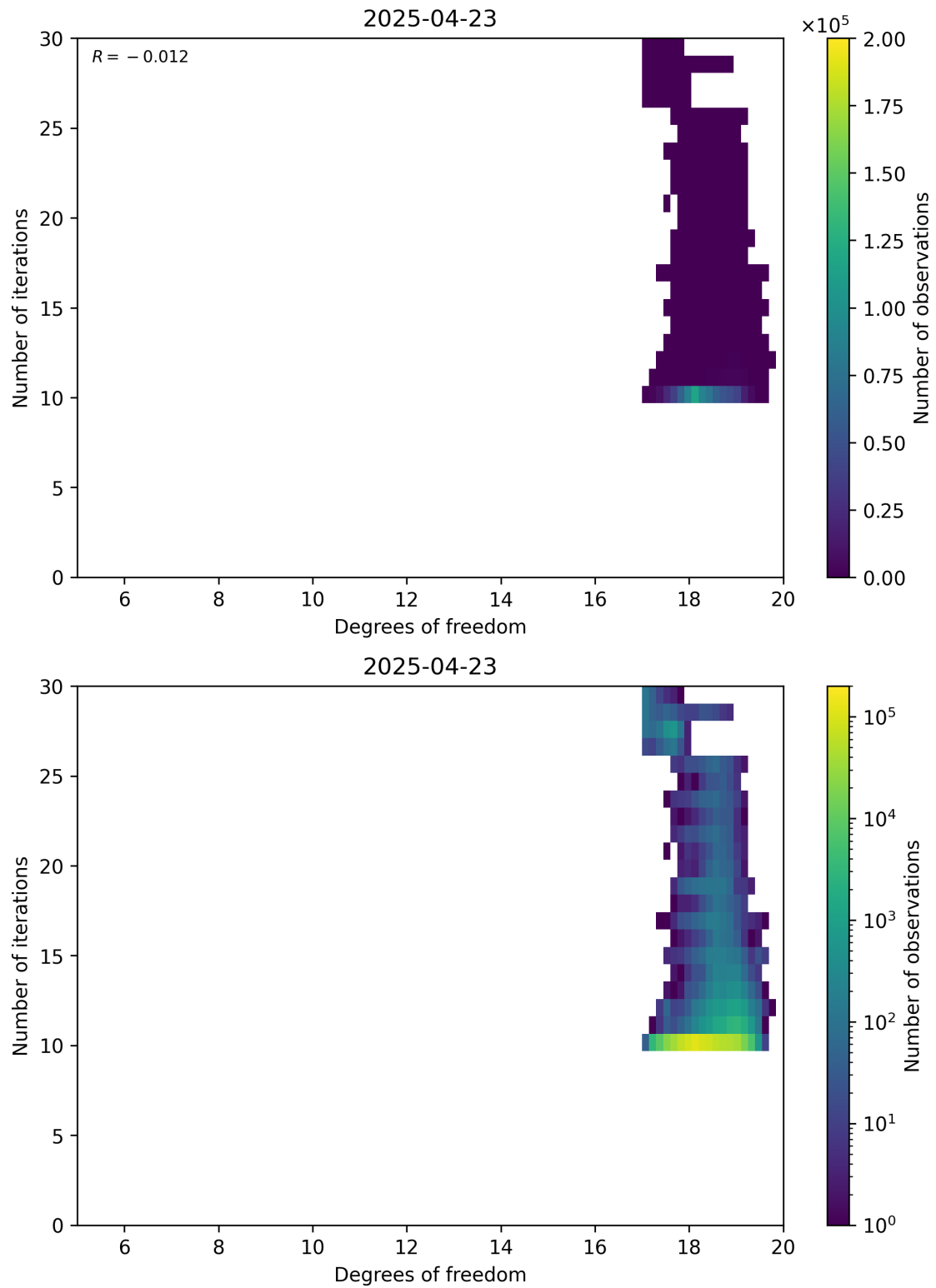
Figure 52: Scatter density plot of “Degrees of freedom” against “Number of iterations” for 2025-04-22 to 2025-04-24.
