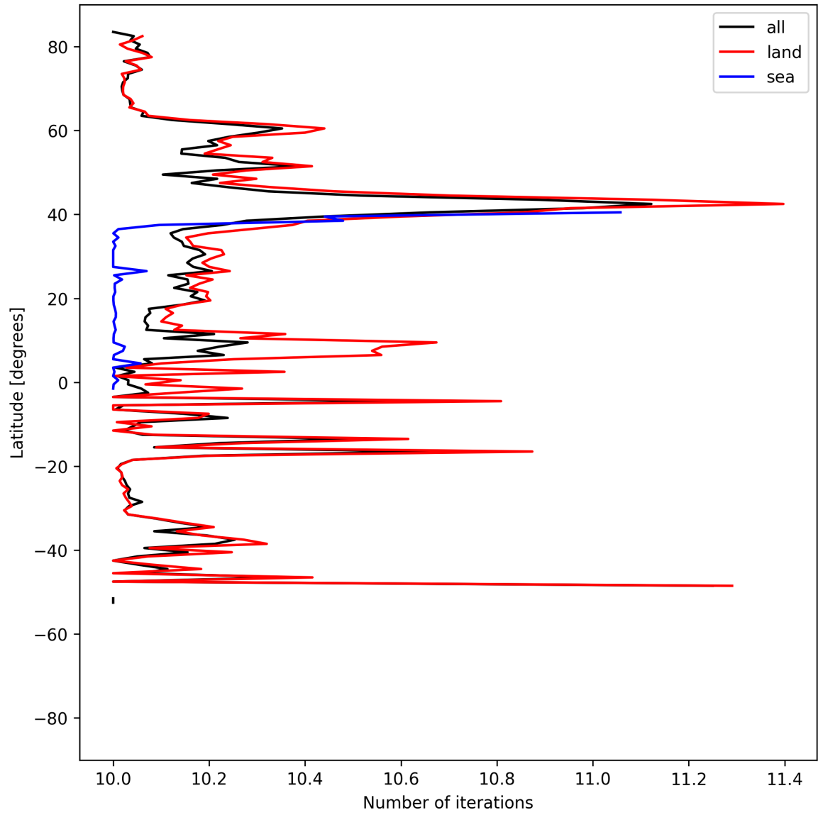
Figure 20: Zonal average of “Number of iterations” for 2025-04-22 to 2025-04-24.
