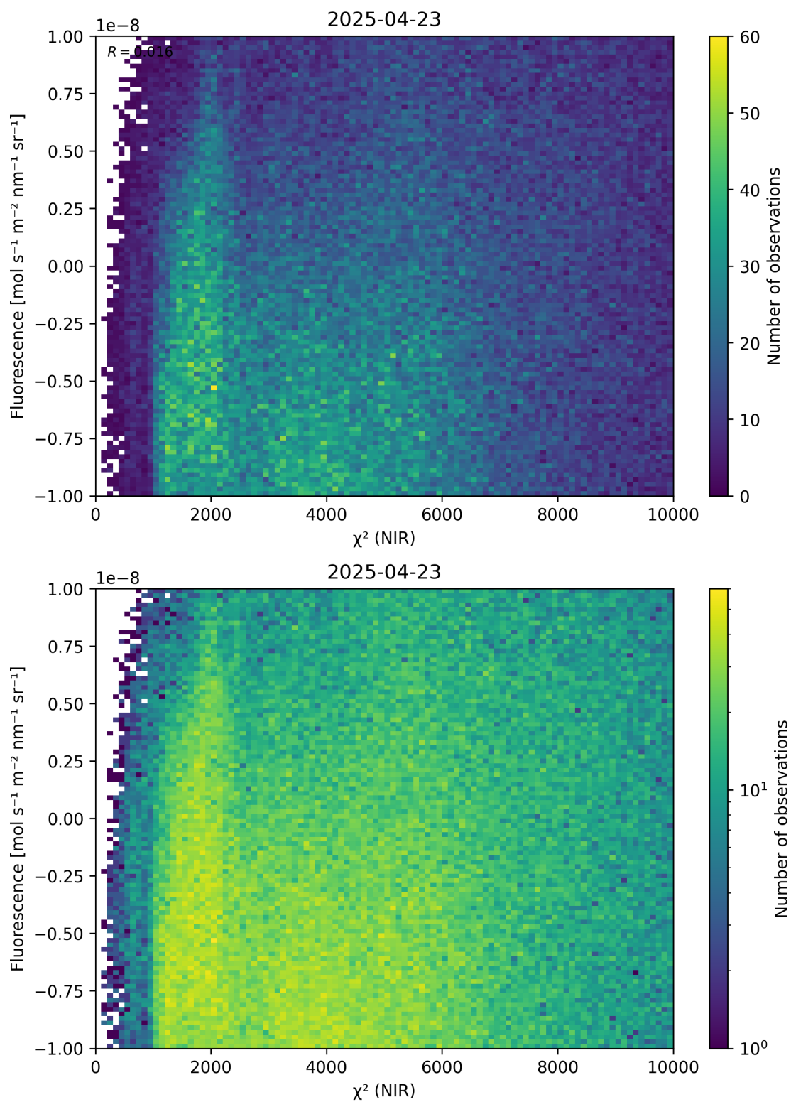
Figure 45: Scatter density plot of “ \chi^2 (NIR)” against “Fluorescence” for 2025-04-22 to 2025-04-24.
