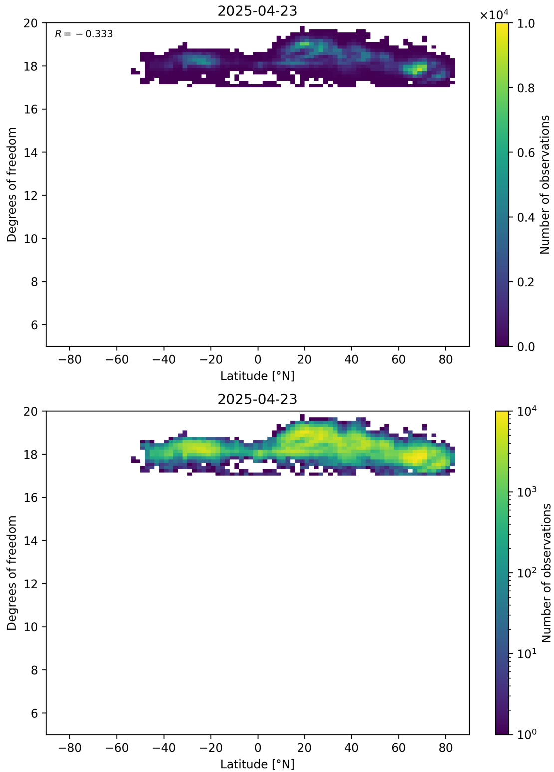
Figure 55: Scatter density plot of “Latitude” against “Degrees of freedom” for 2025-04-22 to 2025-04-24.
