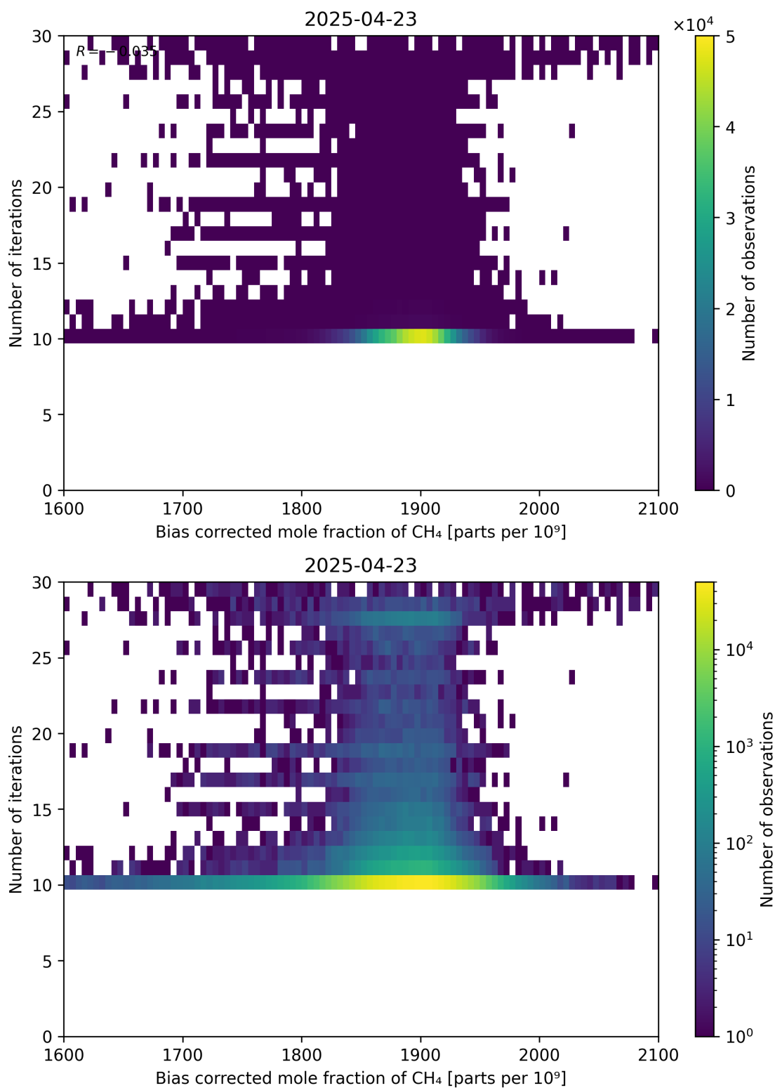
Figure 67: Scatter density plot of “Bias corrected mole fraction of CH 4 ” against “Number of iterations” for 2025-04-22 to 2025-04-24.
