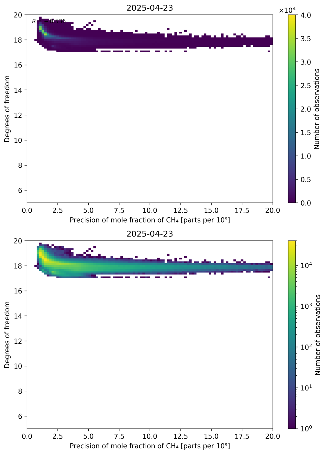
Figure 80: Scatter density plot of “Precision of mole fraction of CH 4 ” against “Degrees of freedom” for 2025-04-22 to 2025-04-24.
