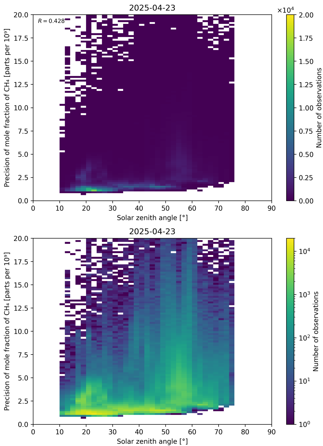
Figure 101: Scatter density plot of “Solar zenith angle” against “Precision of mole fraction of \text{CH}_4 ” for 2025-04-22 to 2025-04-24.
