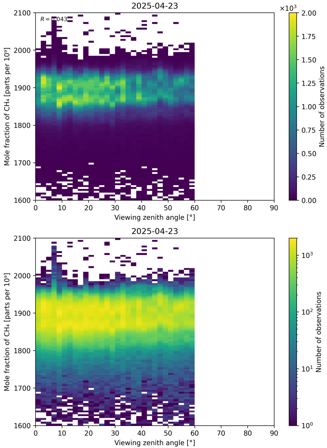
Figure 110: Scatter density plot of “Viewing zenith angle” against “Mole fraction of CH 4 ” for 2025-04-22 to 2025-04-24.
