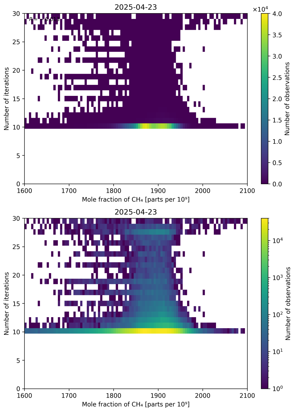
Figure 76: Scatter density plot of “Mole fraction of CH 4 ” against “Number of iterations” for 2025-04-22 to 2025-04-24.
