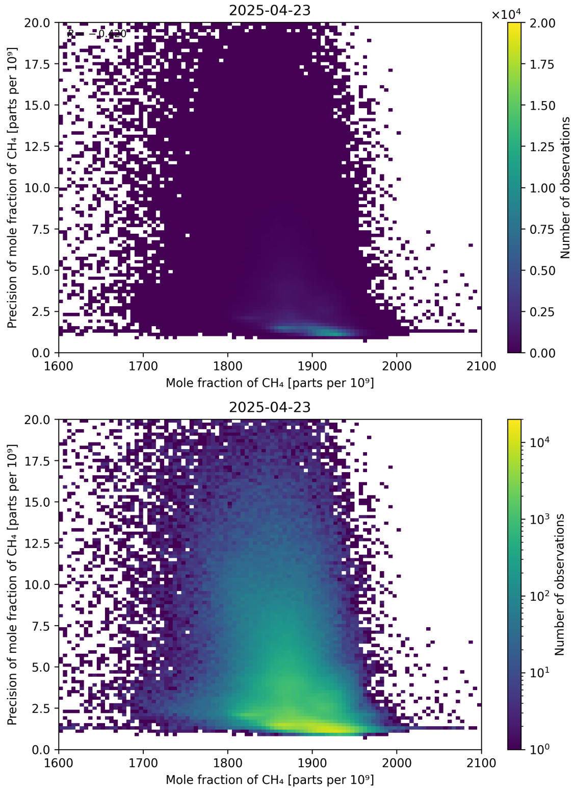
Figure 75: Scatter density plot of “Mole fraction of CH 4 ” against “Precision of mole fraction of CH 4 ” for 2025-04-22 to 2025-04-24.
