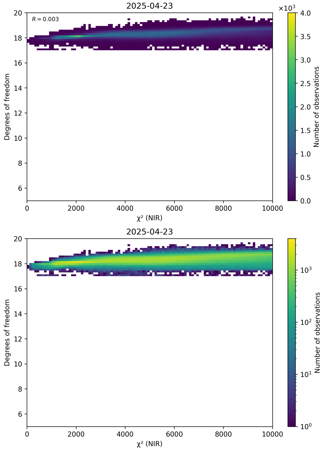
Figure 44: Scatter density plot of “ \chi^2 (NIR)” against “Degrees of freedom” for 2025-04-22 to 2025-04-24.
