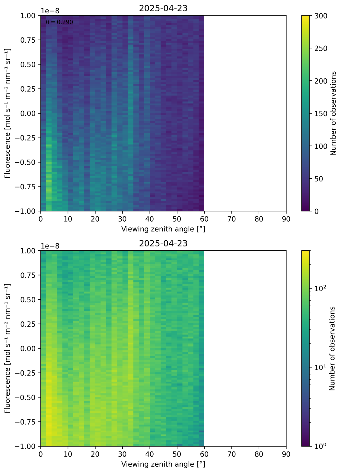
Figure 108: Scatter density plot of “Viewing zenith angle” against “Fluorescence” for 2025-04-22 to 2025-04-24.
