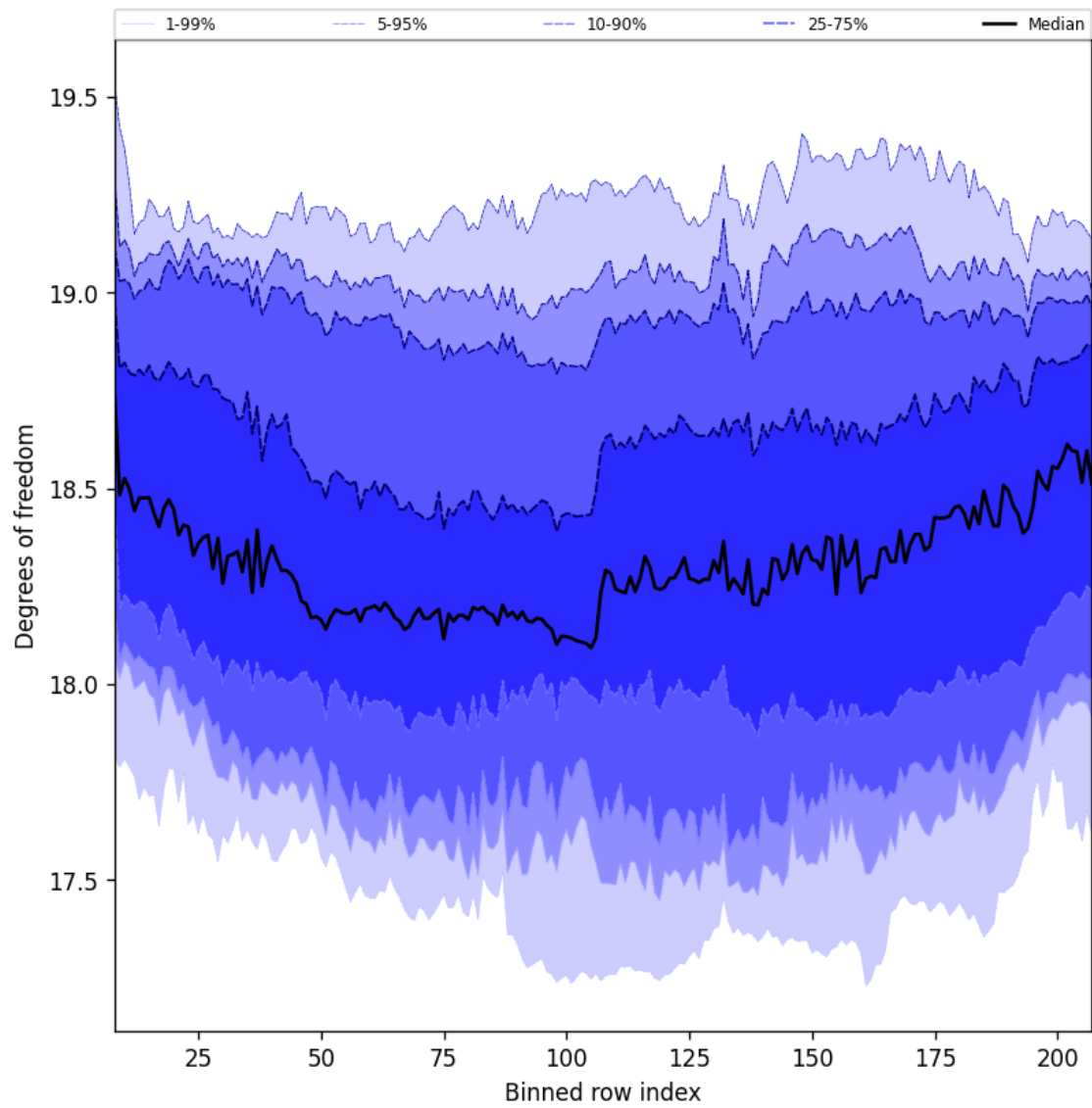
Figure 41: Along track statistics of “Degrees of freedom” for 2025-04-22 to 2025-04-24
