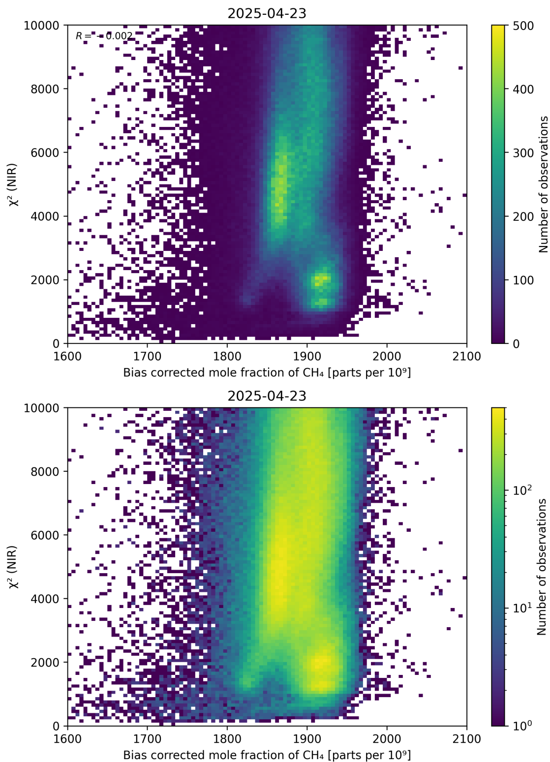
Figure 63: Scatter density plot of “Bias corrected mole fraction of CH 4 ” against “ \chi^2 (NIR)” for 2025-04-22 to 2025-04-24.
