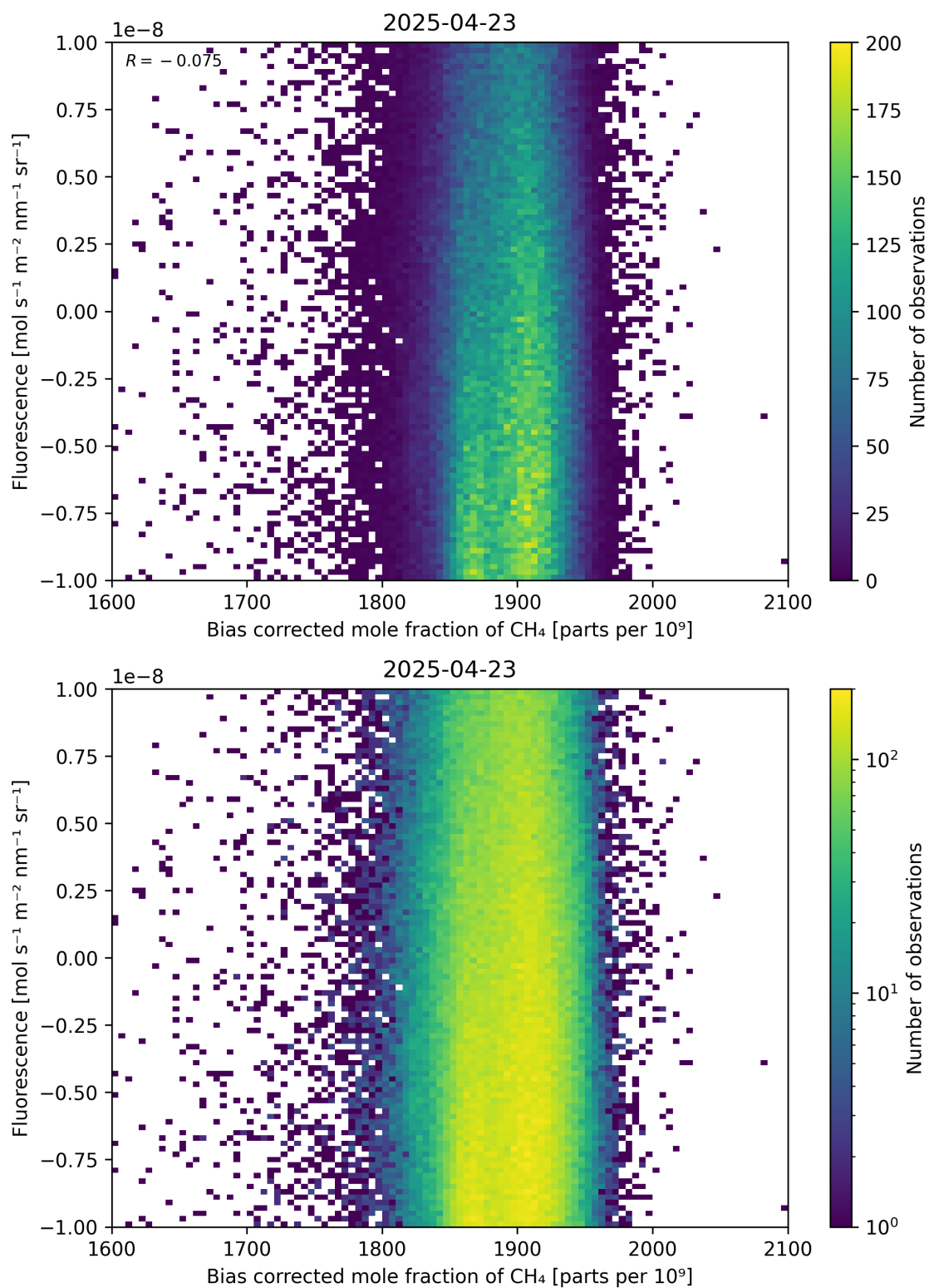
Figure 66: Scatter density plot of “Bias corrected mole fraction of \text{CH}_4 ” against “Fluorescence” for 2025-04-22 to 2025-04-24.
