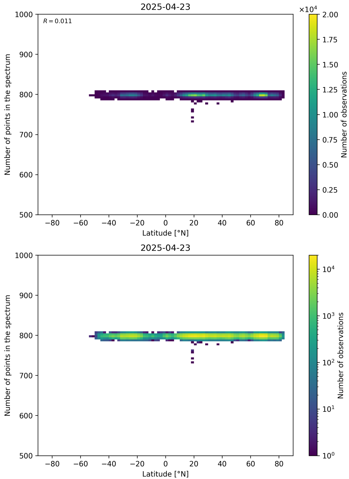
Figure 61: Scatter density plot of “Latitude” against “Number of points in the spectrum” for 2025-04-22 to 2025-04-24.
