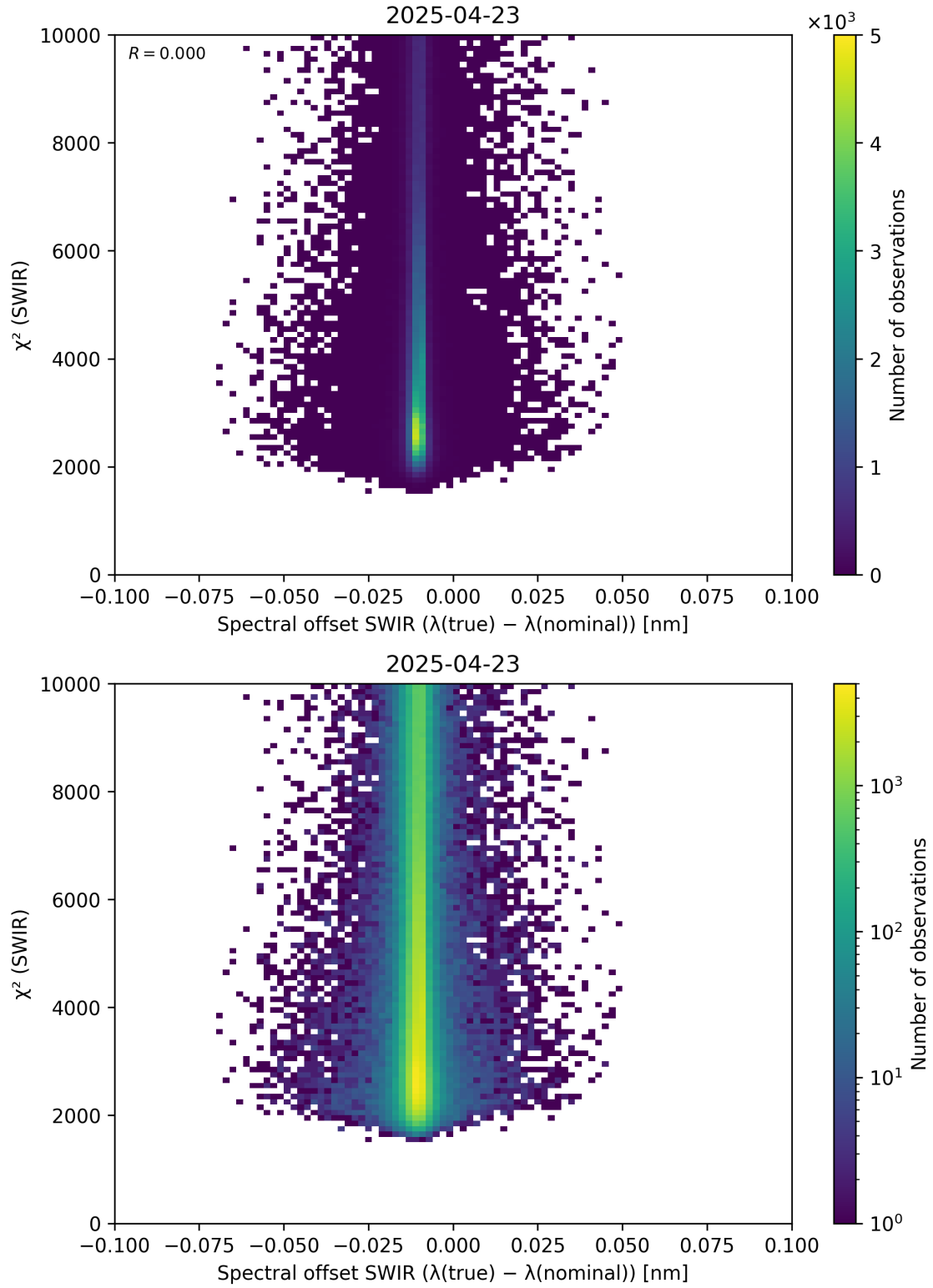
Figure 118: Scatter density plot of “Spectral offset SWIR ( \lambda_{\text{true}} - \lambda_{\text{nominal}} )” against “ \chi^2 (SWIR)” for 2025-04-22 to 2025-04-24.
