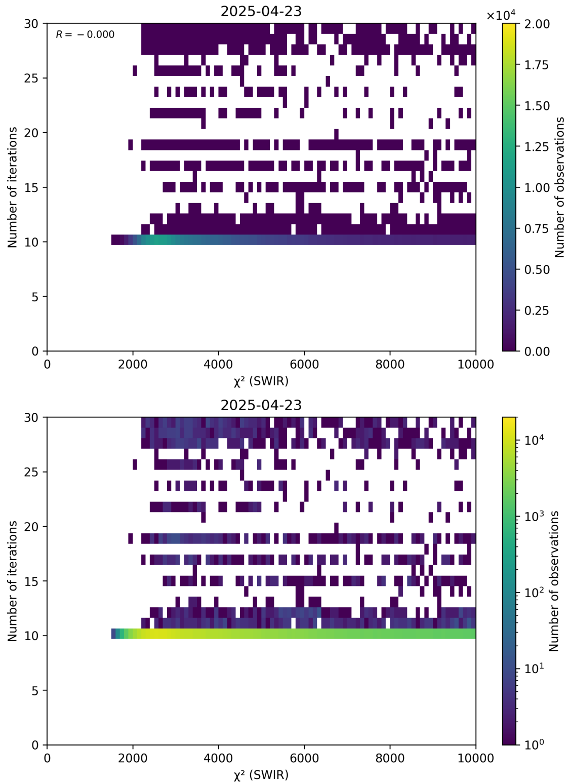
Figure 50: Scatter density plot of “ \chi^2 (SWIR)” against “Number of iterations” for 2025-04-22 to 2025-04-24.
