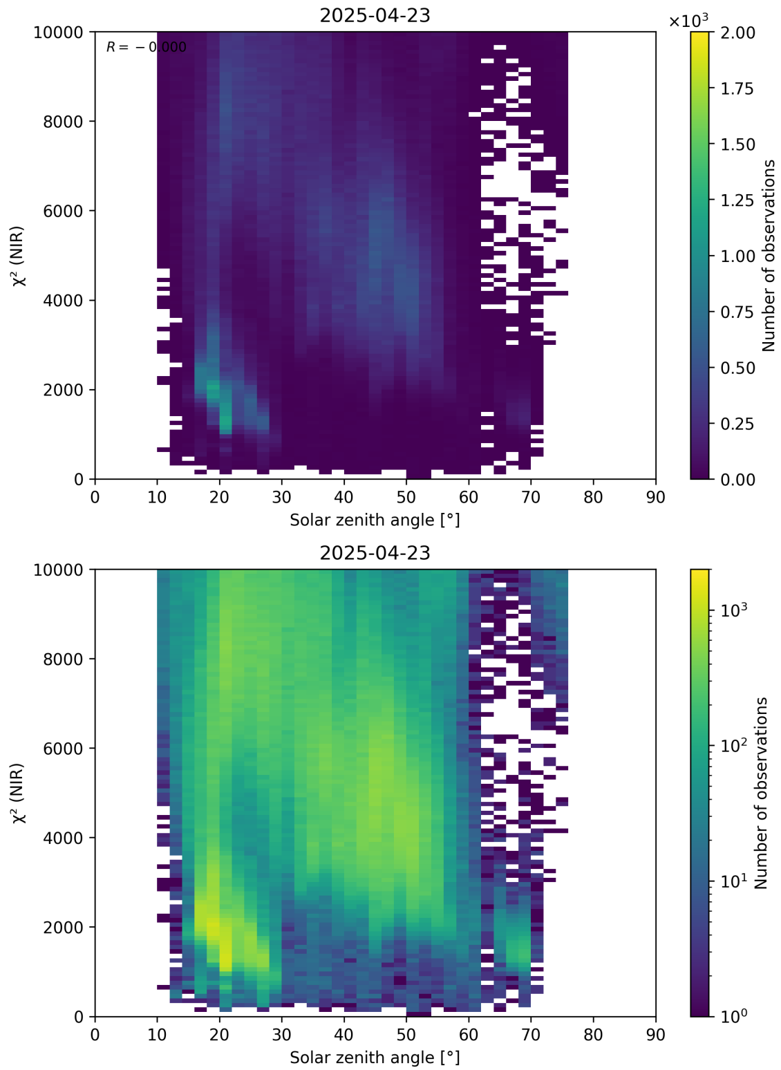
Figure 94: Scatter density plot of “Solar zenith angle” against “ \chi^2 (NIR)” for 2025-04-22 to 2025-04-24.
