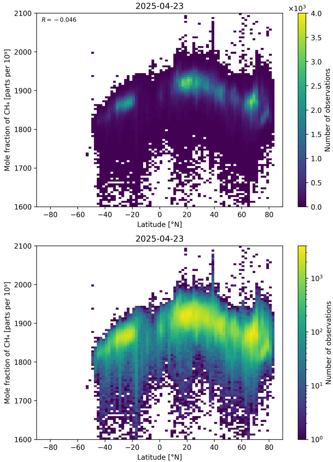
Figure 57: Scatter density plot of “Latitude” against “Mole fraction of \text{CH}_4 ” for 2025-04-22 to 2025-04-24.
