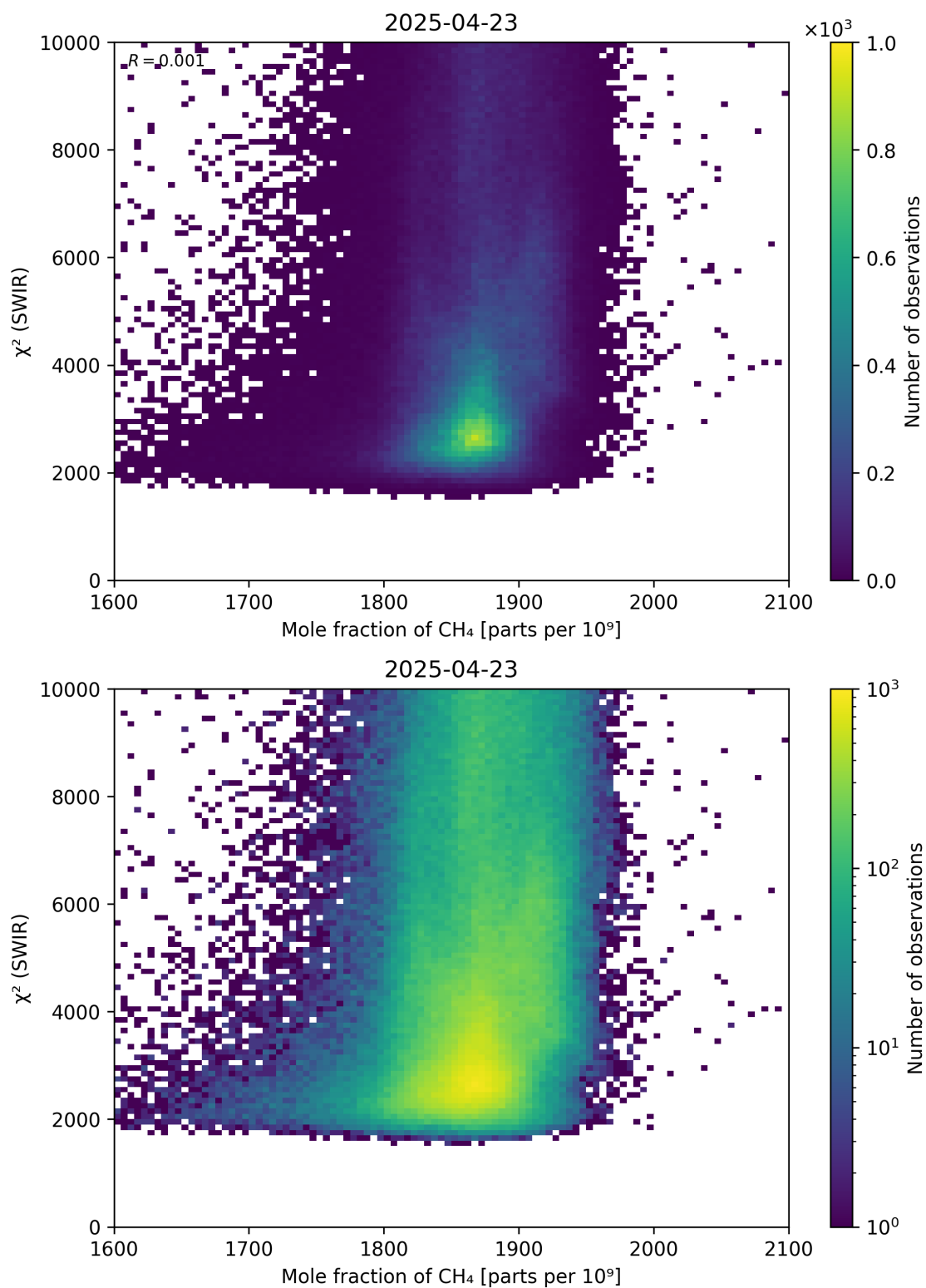
Figure 71: Scatter density plot of “Mole fraction of CH 4 ” against “ \chi^2 (SWIR)” for 2025-04-22 to 2025-04-24.
