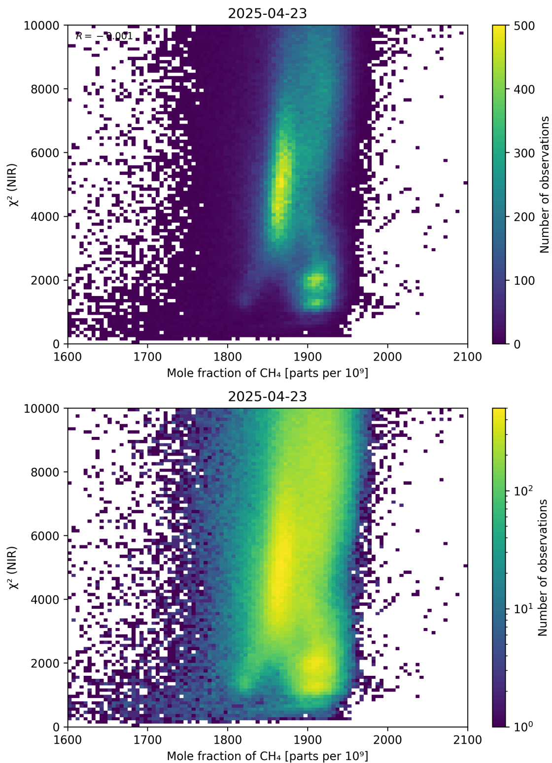
Figure 70: Scatter density plot of “Mole fraction of \text{CH}_4 ” against “ \chi^2 (NIR)” for 2025-04-22 to 2025-04-24.
