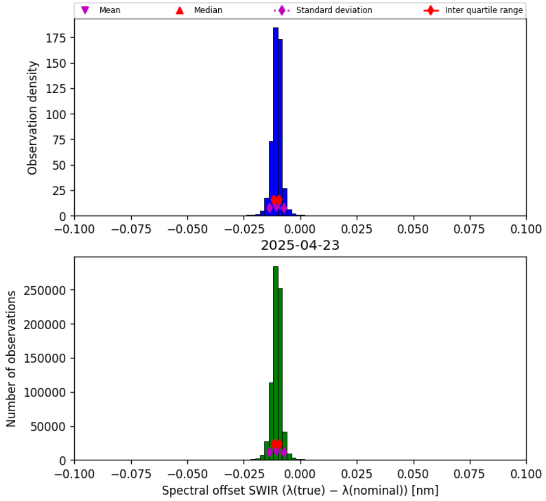
Figure 27: Histogram of “Spectral offset SWIR ( \lambda_{\text{true}} - \lambda_{\text{nominal}} )” for 2025-04-22 to 2025-04-24
