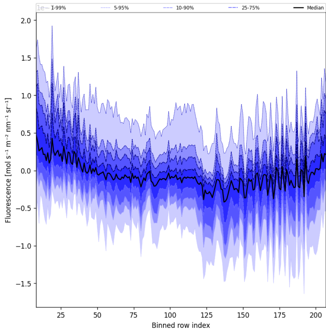
Figure 43: Along track statistics of “Fluorescence” for 2025-04-22 to 2025-04-24
