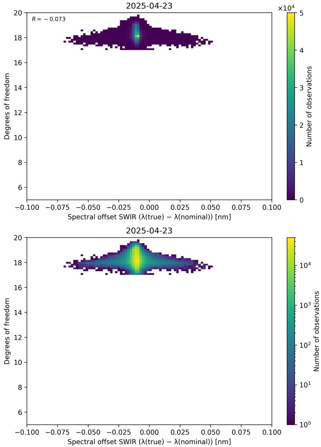
Figure 119: Scatter density plot of “Spectral offset SWIR ( \lambda_{\text{true}} - \lambda_{\text{nominal}} )” against “Degrees of freedom” for 2025-04-22 to 2025-04-24.
