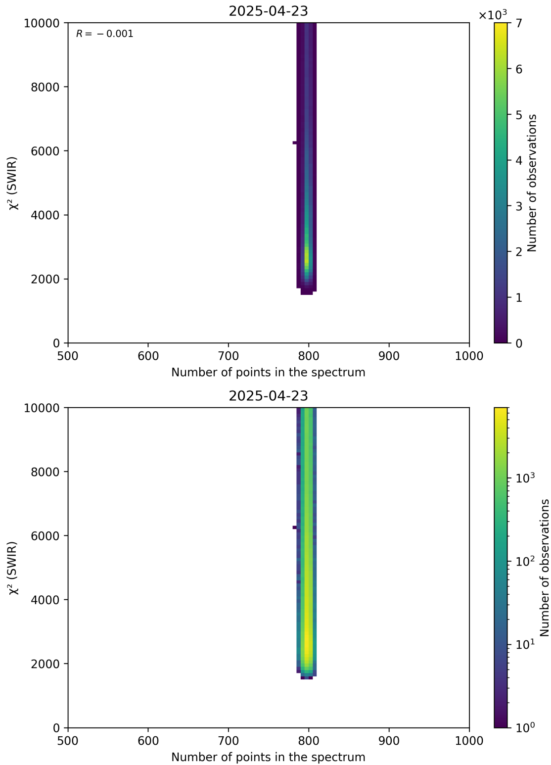
Figure 89: Scatter density plot of “Number of points in the spectrum” against “ \chi^2 (SWIR)” for 2025-04-22 to 2025-04-24.
