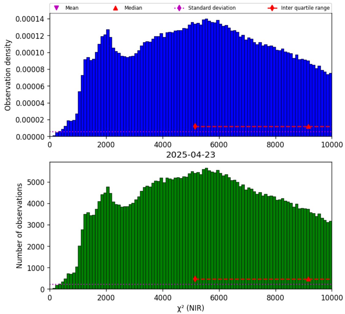
Figure 29: Histogram of " \chi^2 (NIR)" for 2025-04-22 to 2025-04-24
