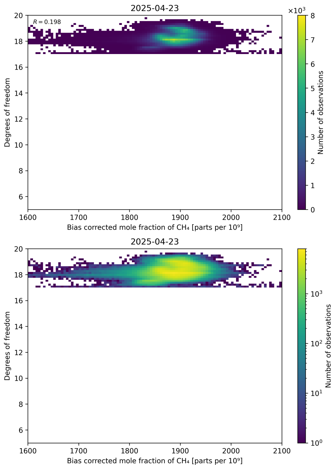
Figure 65: Scatter density plot of “Bias corrected mole fraction of CH 4 ” against “Degrees of freedom” for 2025-04-22 to 2025-04-24.
