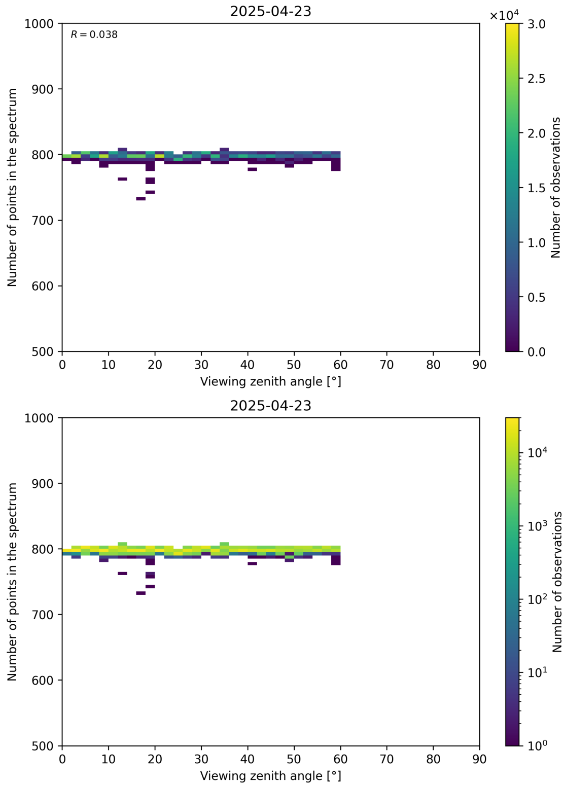
Figure 114: Scatter density plot of “Viewing zenith angle” against “Number of points in the spectrum” for 2025-04-22 to 2025-04-24.
