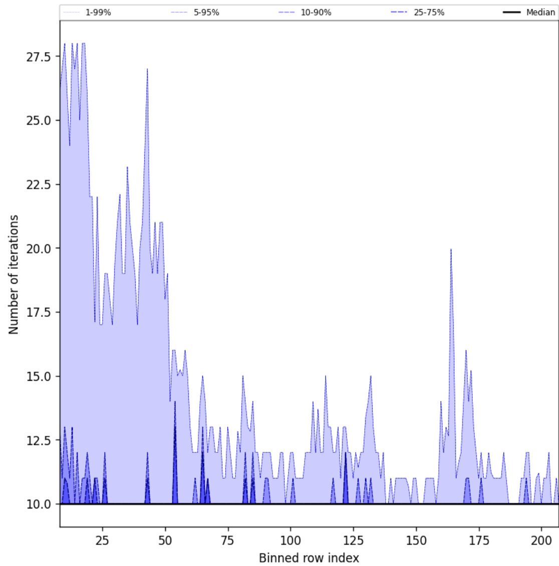
Figure 42: Along track statistics of “Number of iterations” for 2025-04-22 to 2025-04-24
