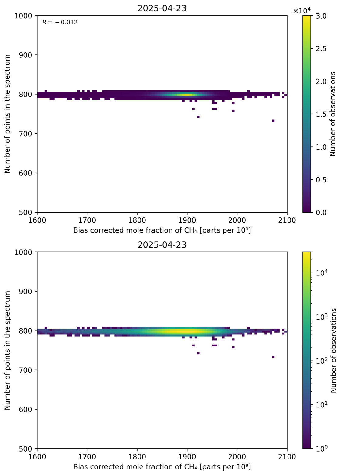
Figure 68: Scatter density plot of “Bias corrected mole fraction of CH 4 ” against “Number of points in the spectrum” for 2025-04-22 to 2025-04-24.
