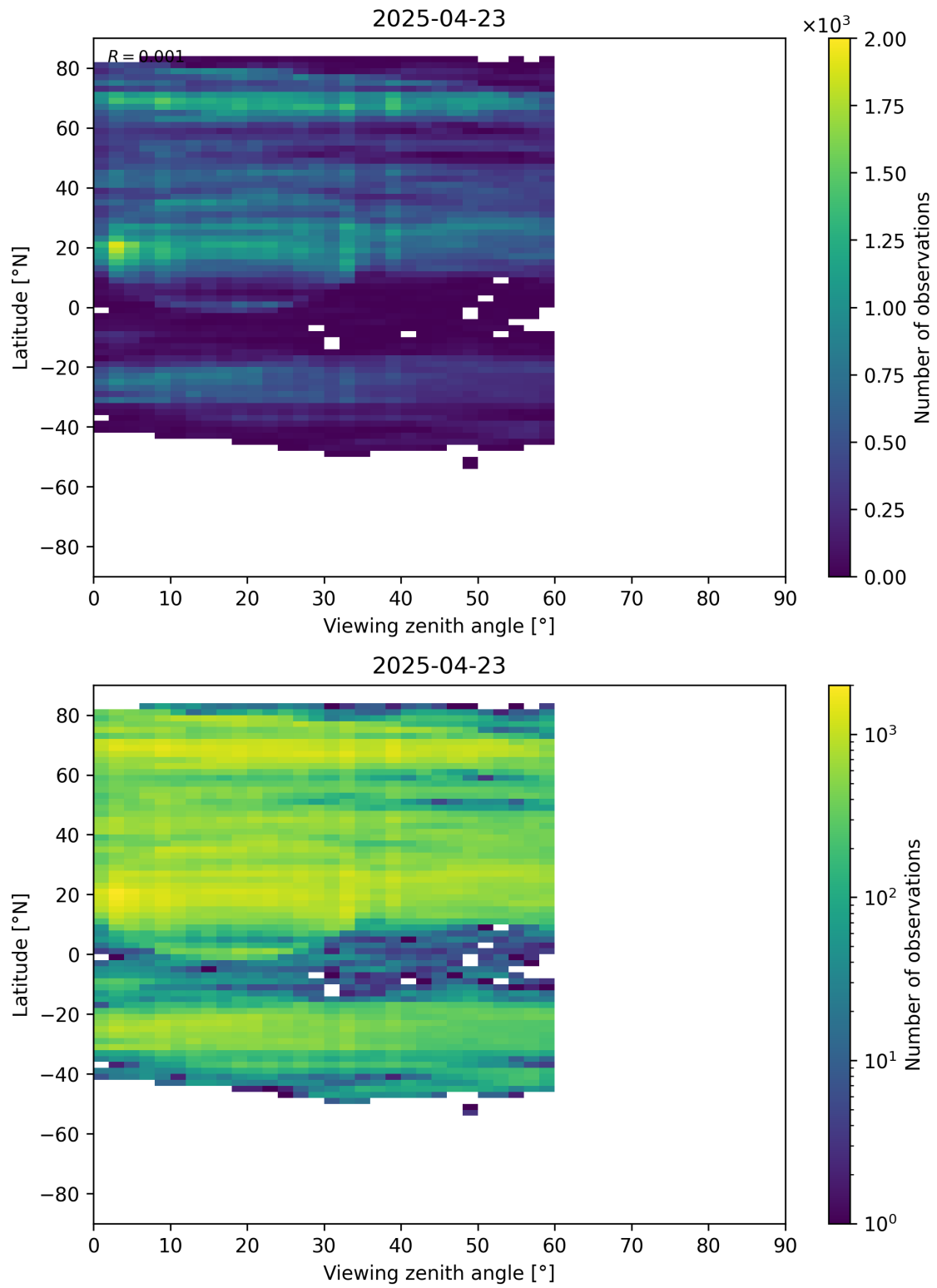
Figure 109: Scatter density plot of “Viewing zenith angle” against “Latitude” for 2025-04-22 to 2025-04-24.
