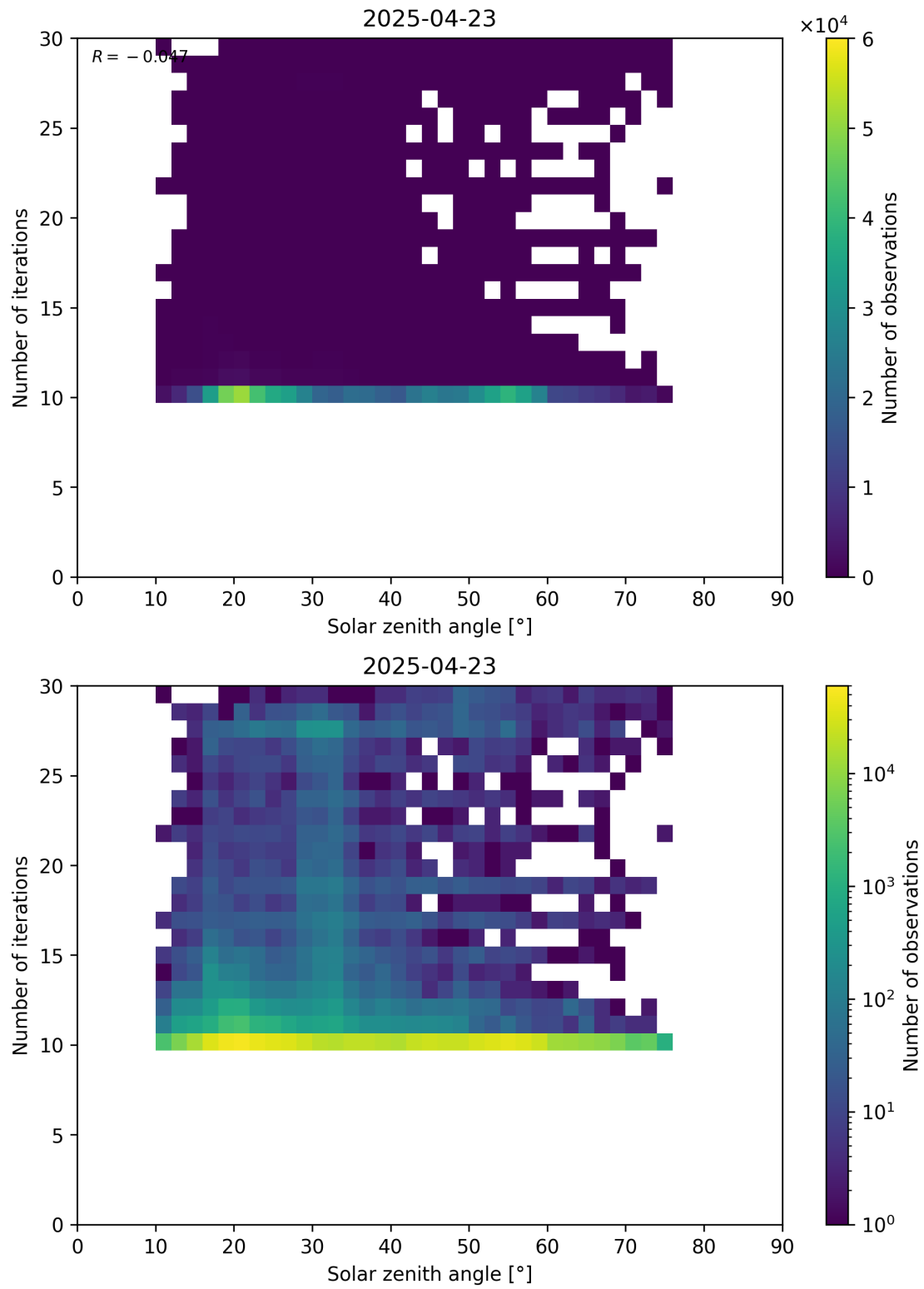
Figure 102: Scatter density plot of “Solar zenith angle” against “Number of iterations” for 2025-04-22 to 2025-04-24.
