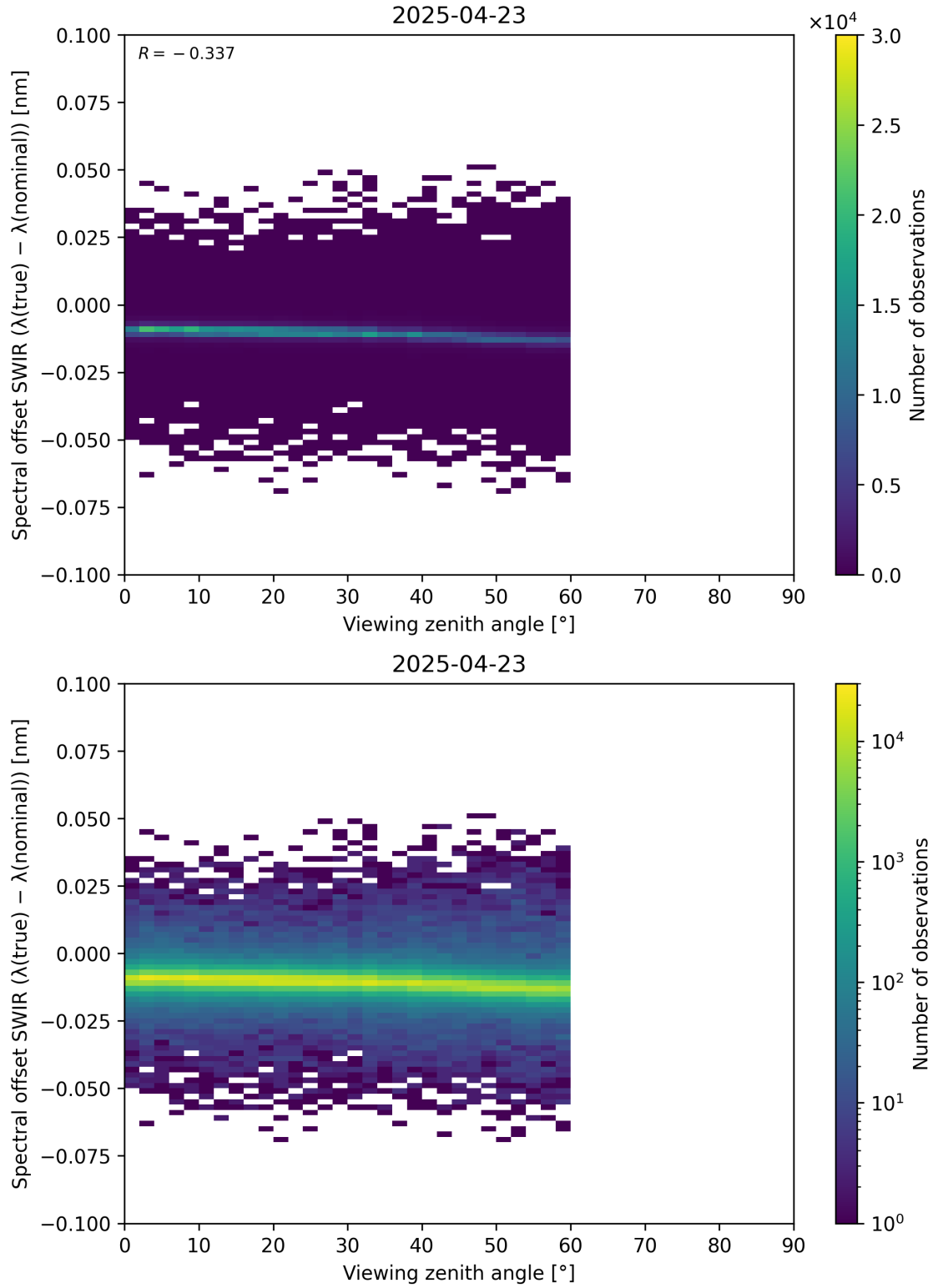
Figure 116: Scatter density plot of “Viewing zenith angle” against “Spectral offset SWIR ( \lambda_{\text{true}} - \lambda_{\text{nominal}} )” for 2025-04-22 to 2025-04-24.
