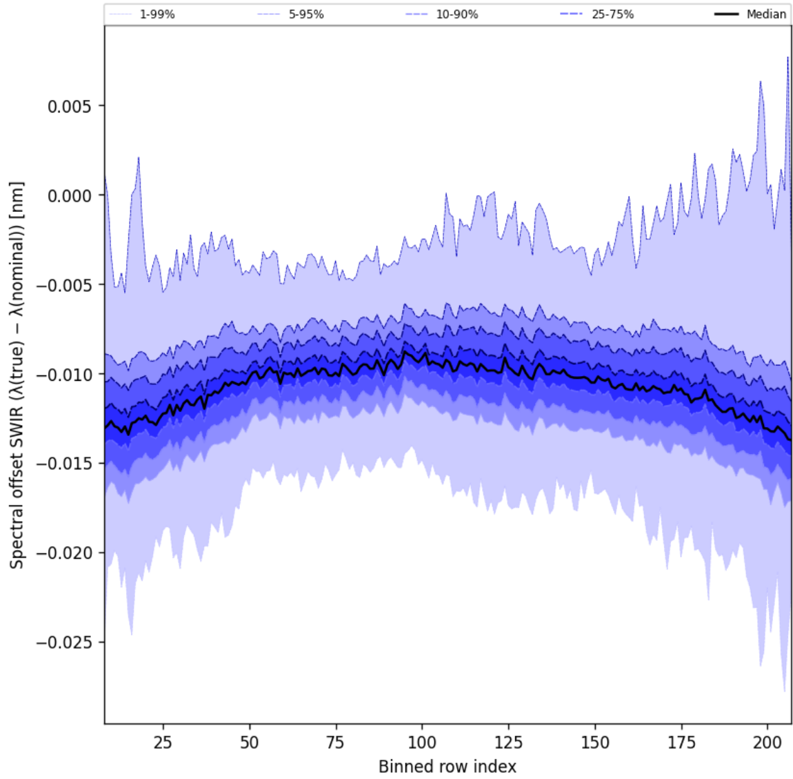
Figure 38: Along track statistics of “Spectral offset SWIR ( \lambda_{\text{true}} - \lambda_{\text{nominal}} )” for 2025-04-22 to 2025-04-24
