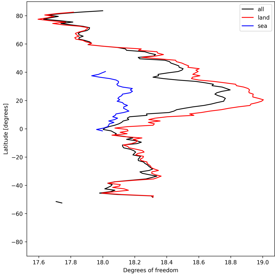
Figure 19: Zonal average of “Degrees of freedom” for 2025-04-22 to 2025-04-24.
