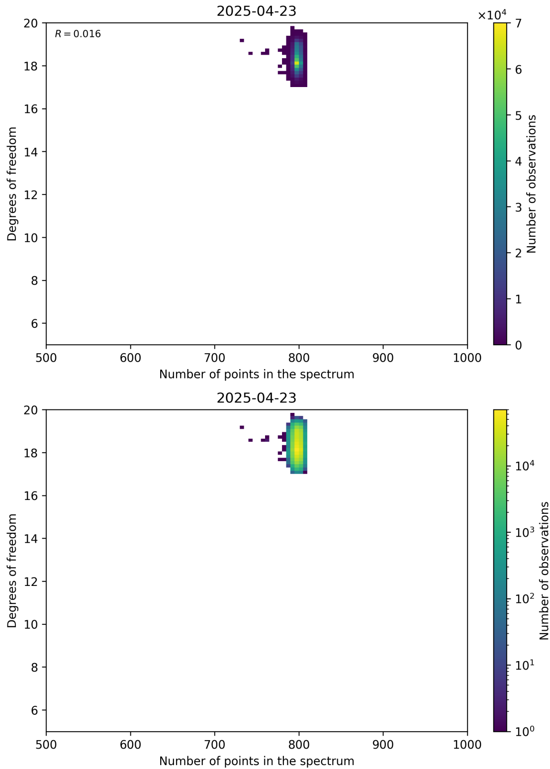
Figure 90: Scatter density plot of “Number of points in the spectrum” against “Degrees of freedom” for 2025-04-22 to 2025-04-24.
