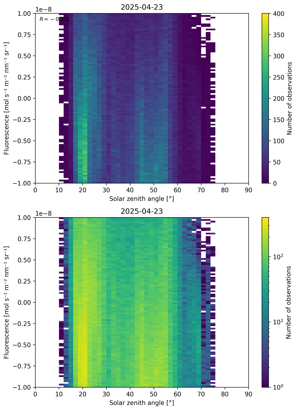
Figure 97: Scatter density plot of “Solar zenith angle” against “Fluorescence” for 2025-04-22 to 2025-04-24.
