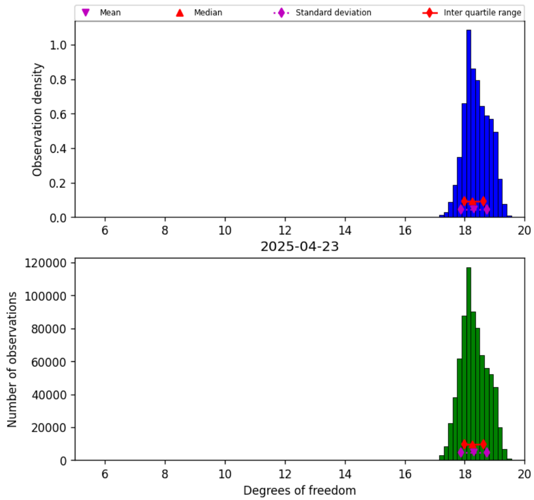
Figure 30: Histogram of “Degrees of freedom” for 2025-04-22 to 2025-04-24
