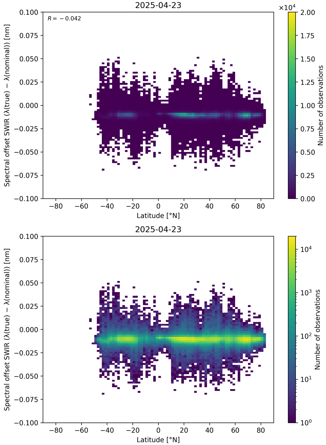
Figure 62: Scatter density plot of “Latitude” against “Spectral offset SWIR ( \lambda_{\text{true}} - \lambda_{\text{nominal}} )” for 2025-04-22 to 2025-04-24.
