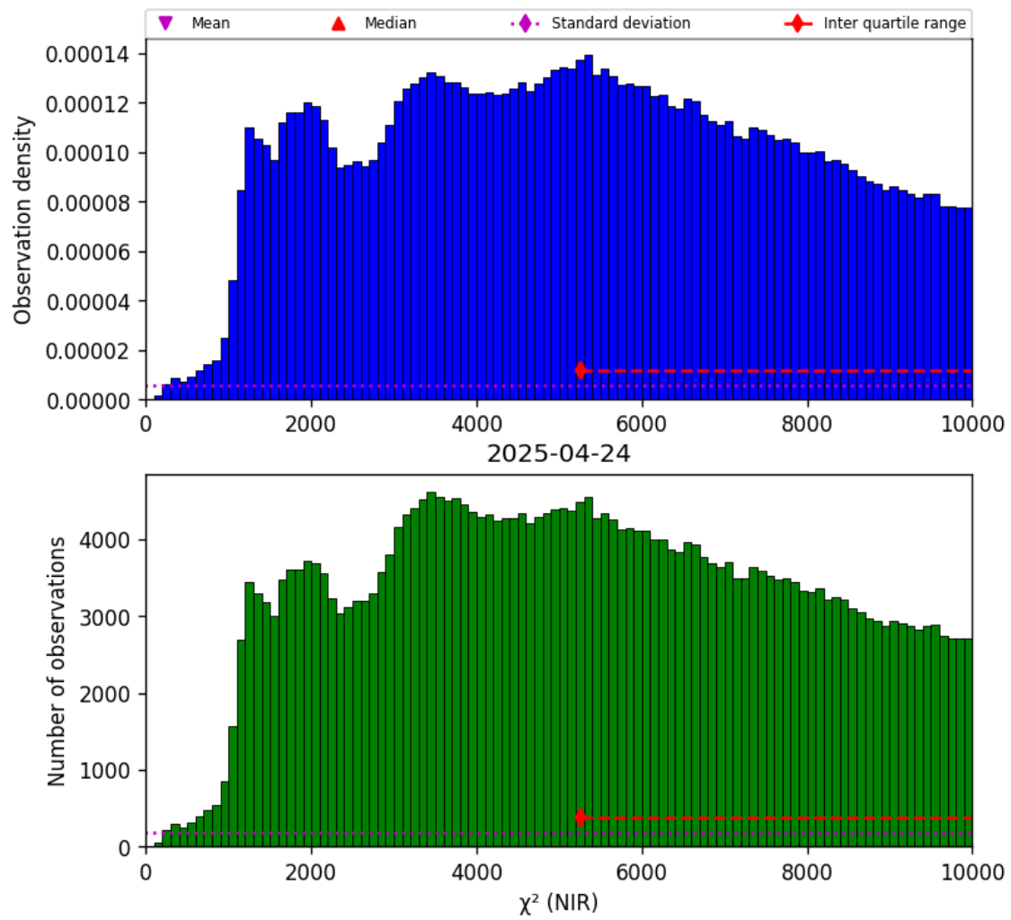
Figure 29: Histogram of “ \chi^2 (NIR)” for 2025-04-24 to 2025-04-25
