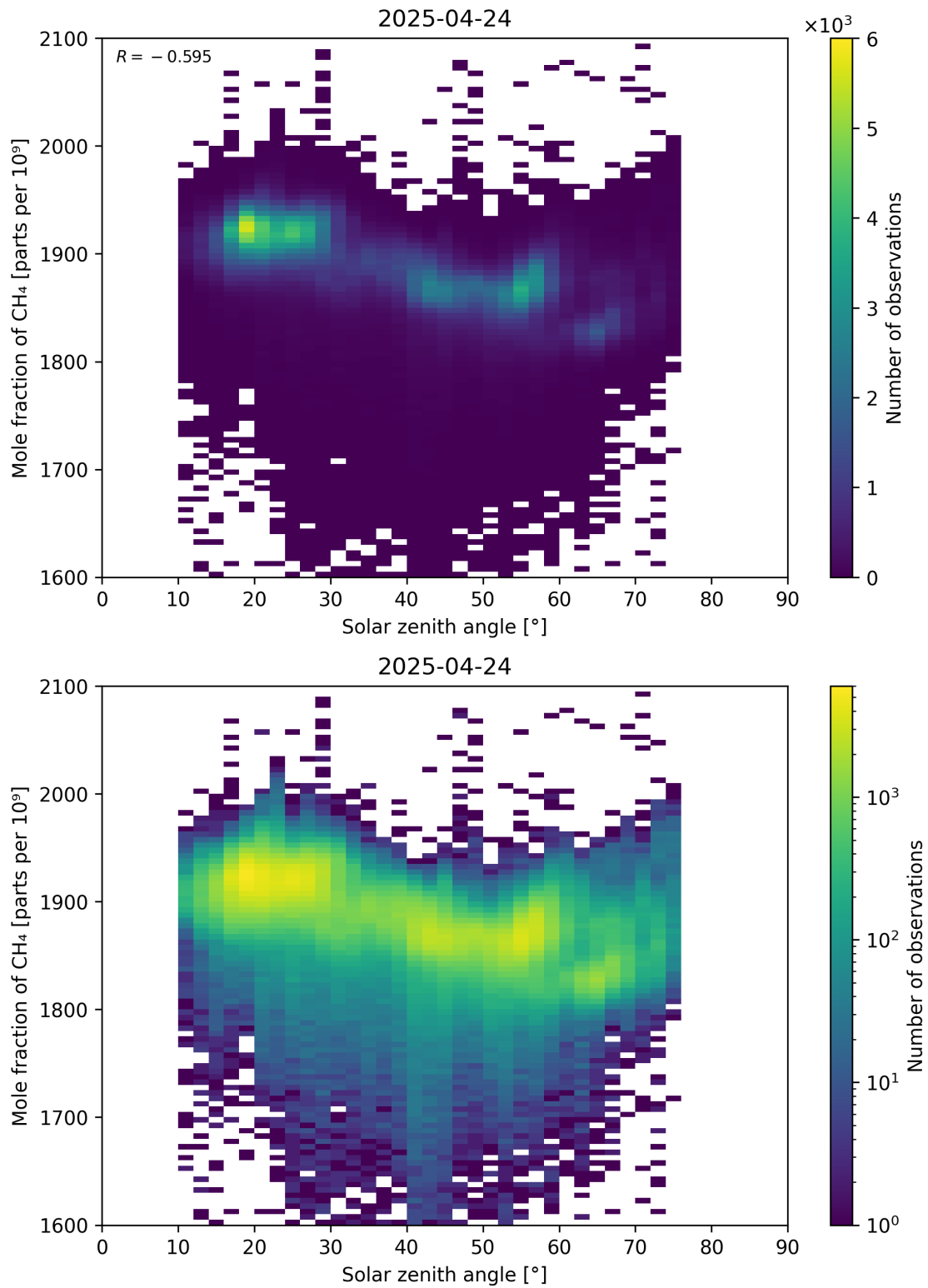
Figure 99: Scatter density plot of “Solar zenith angle” against “Mole fraction of \text{CH}_4 ” for 2025-04-24 to 2025-04-25.
