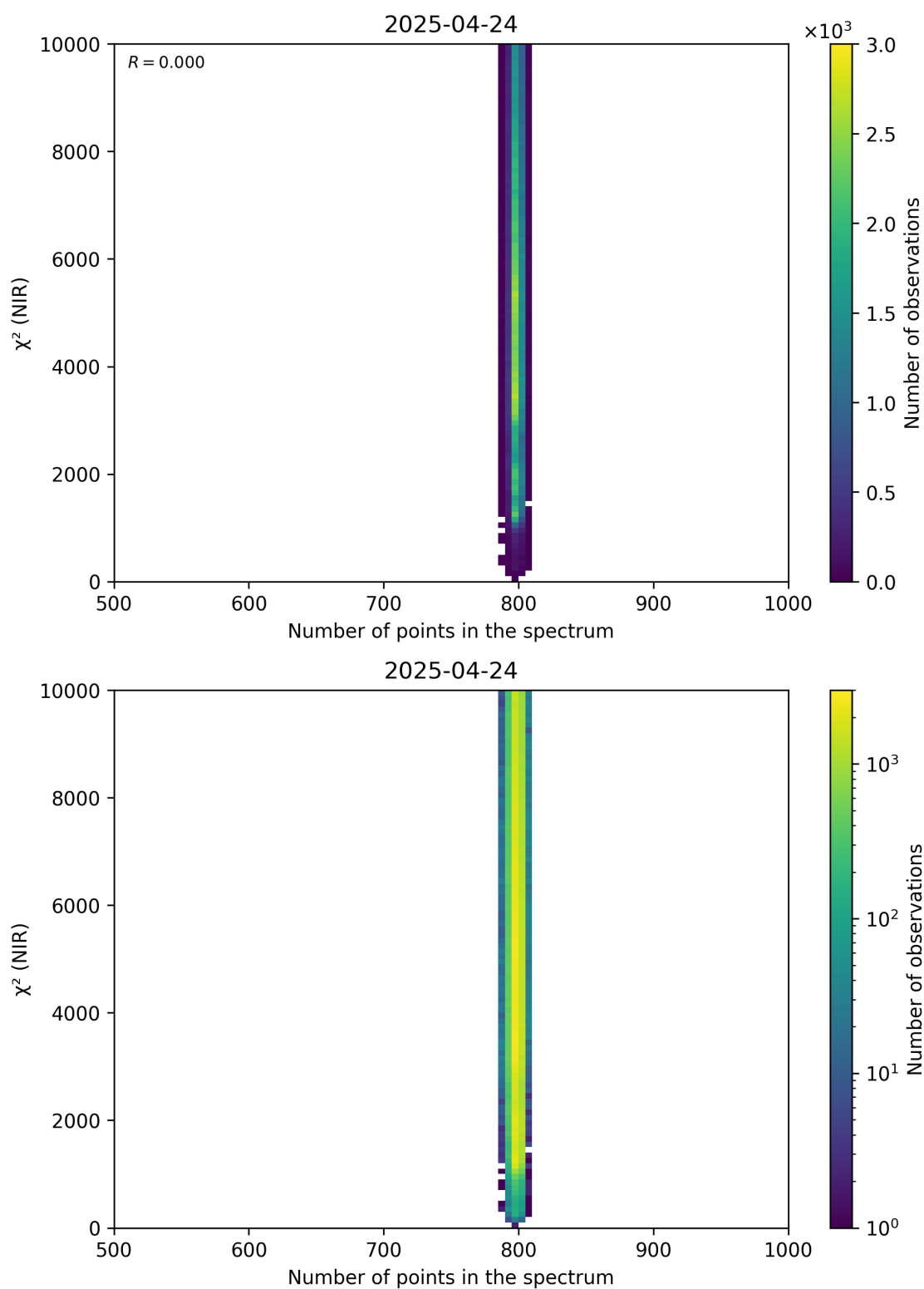
Figure 88: Scatter density plot of “Number of points in the spectrum” against “ \chi^2 (NIR)” for 2025-04-24 to 2025-04-25.
