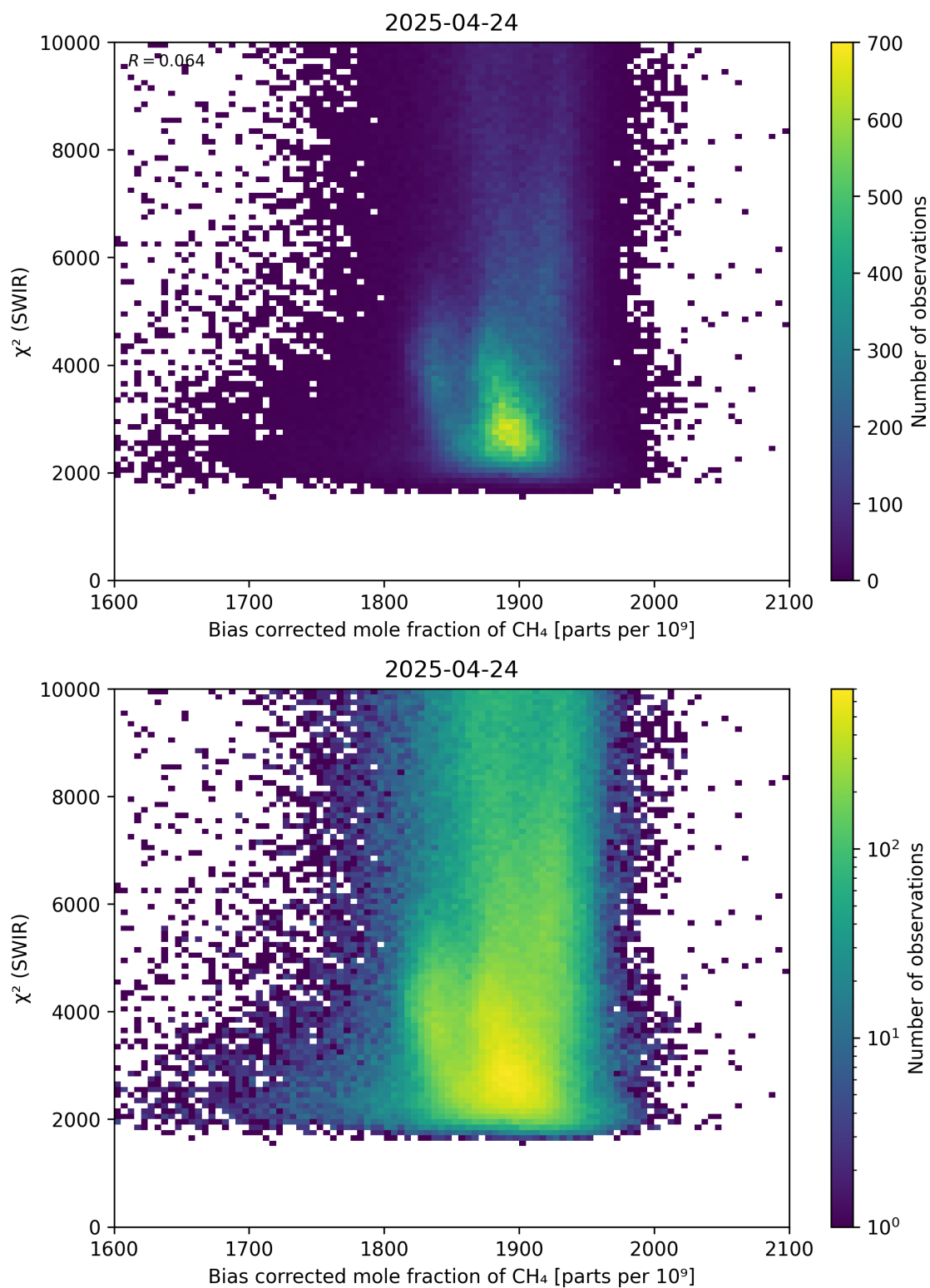
Figure 64: Scatter density plot of “Bias corrected mole fraction of \text{CH}_4 ” against “ \chi^2 (SWIR)” for 2025-04-24 to 2025-04-25.
