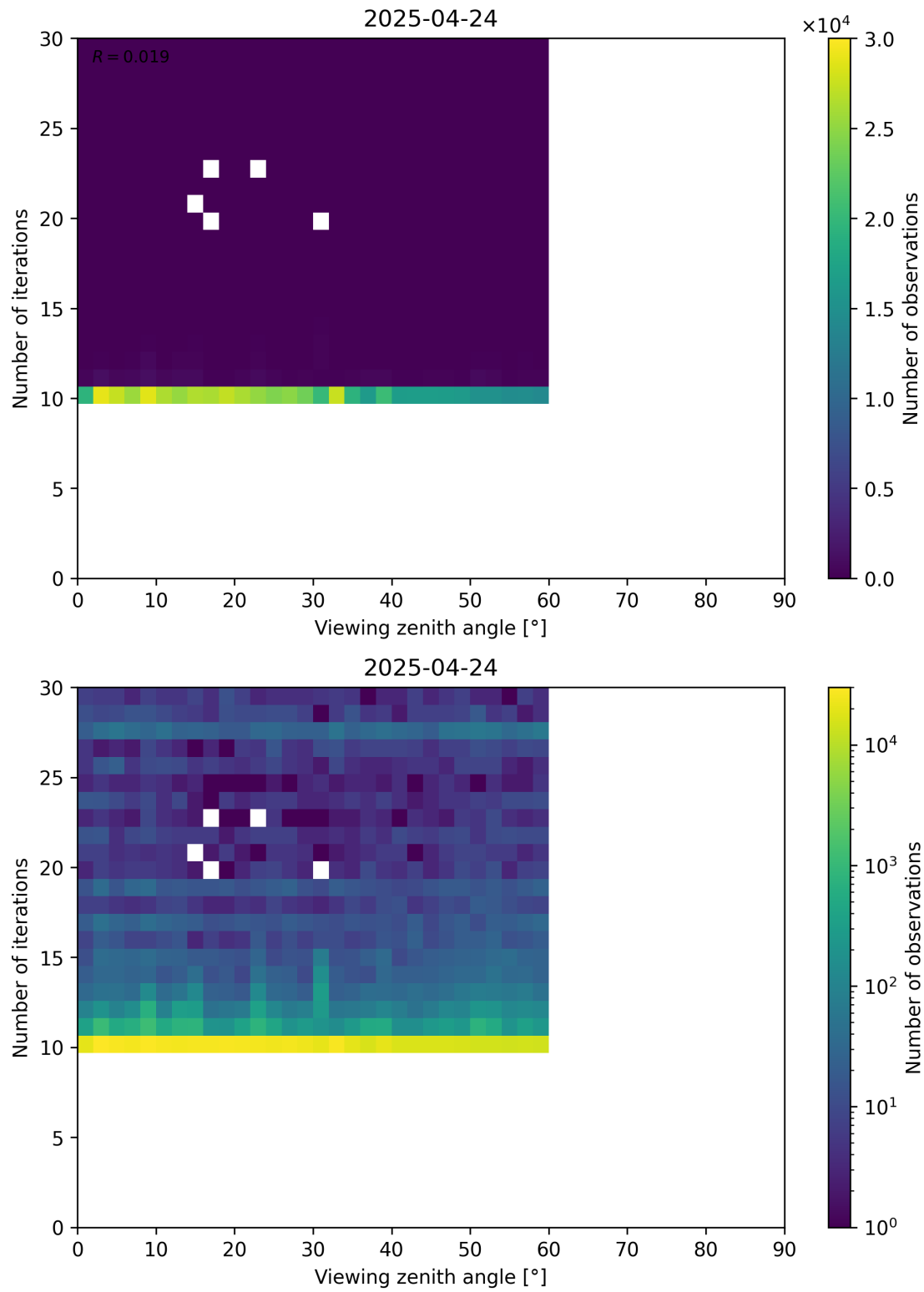
Figure 113: Scatter density plot of “Viewing zenith angle” against “Number of iterations” for 2025-04-24 to 2025-04-25.
