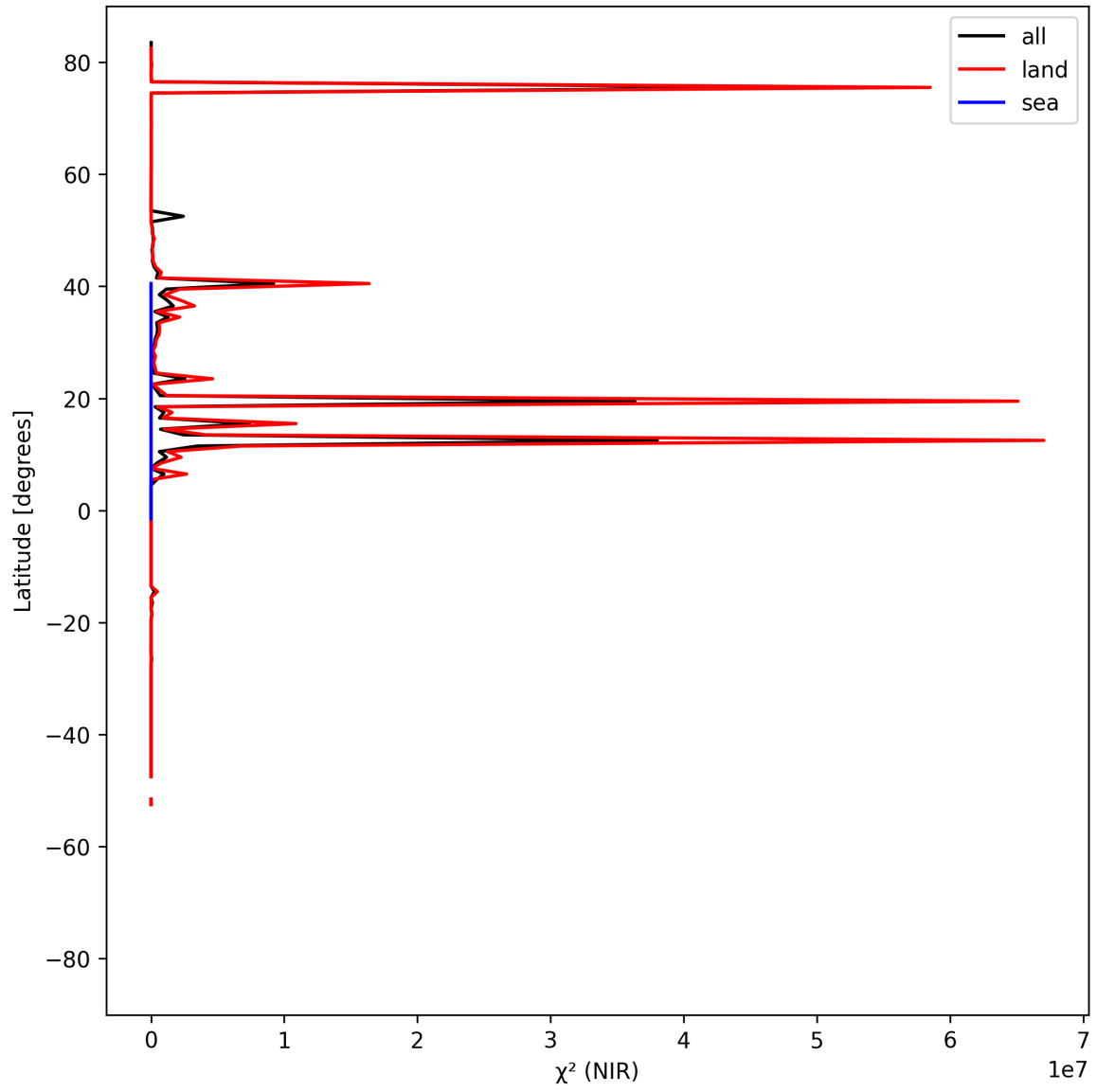
Figure 18: Zonal average of “ \chi^2 (NIR)” for 2025-04-24 to 2025-04-25.
