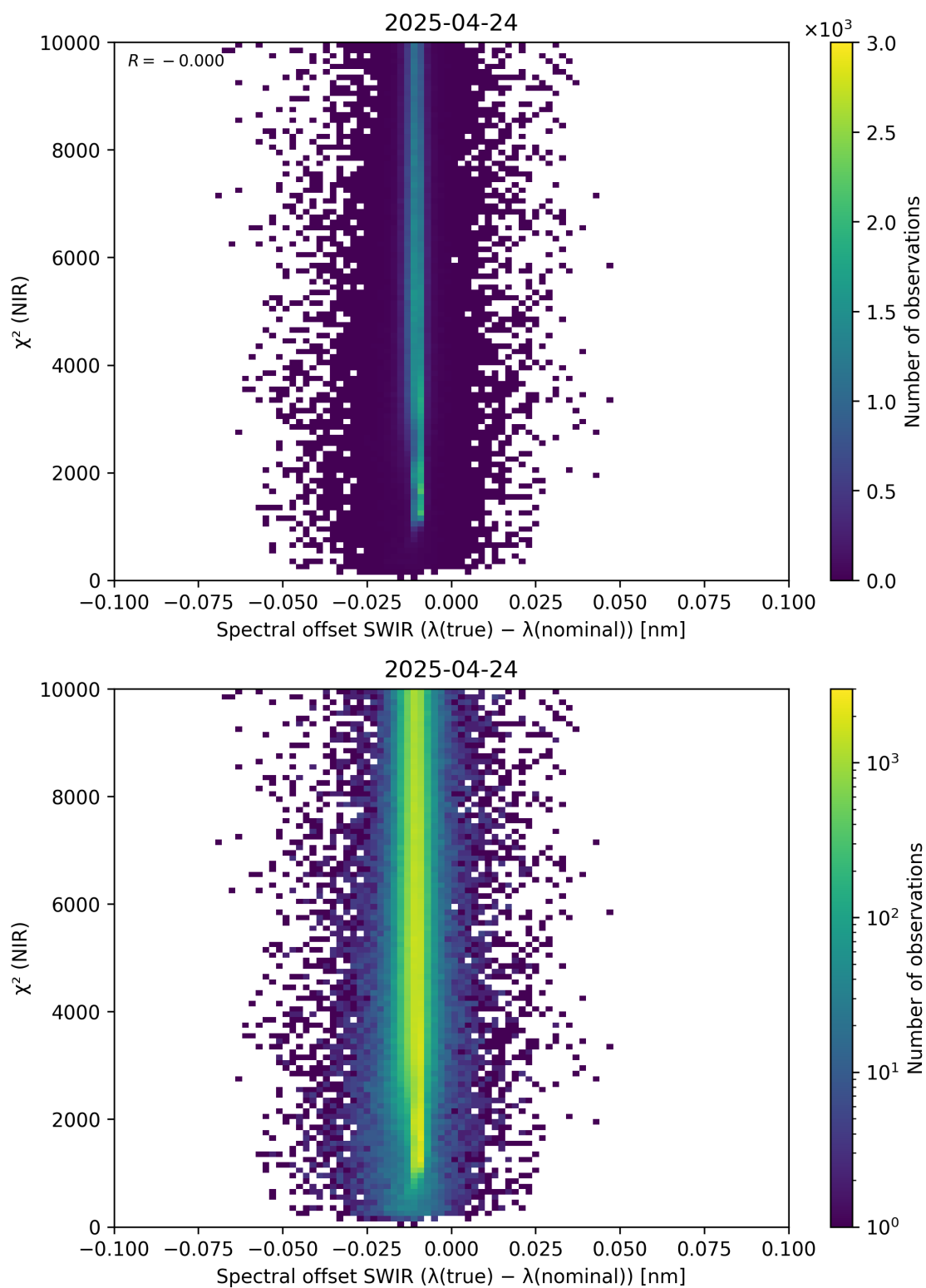
Figure 117: Scatter density plot of “Spectral offset SWIR ( \lambda_{\text{true}} - \lambda_{\text{nominal}} )” against “ \chi^2 (NIR)” for 2025-04-24 to 2025-04-25.
