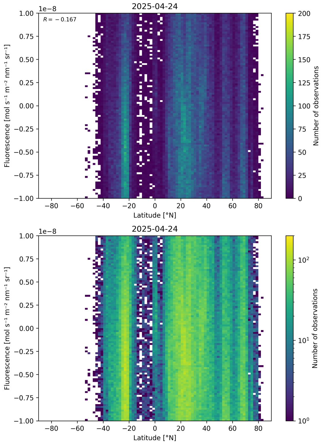
Figure 56: Scatter density plot of “Latitude” against “Fluorescence” for 2025-04-24 to 2025-04-25.
