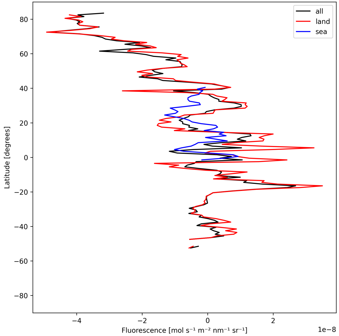
Figure 21: Zonal average of “Fluorescence” for 2025-04-24 to 2025-04-25.
