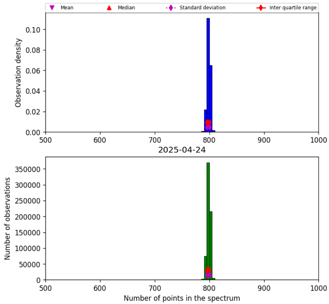
Figure 26: Histogram of “Number of points in the spectrum” for 2025-04-24 to 2025-04-25
