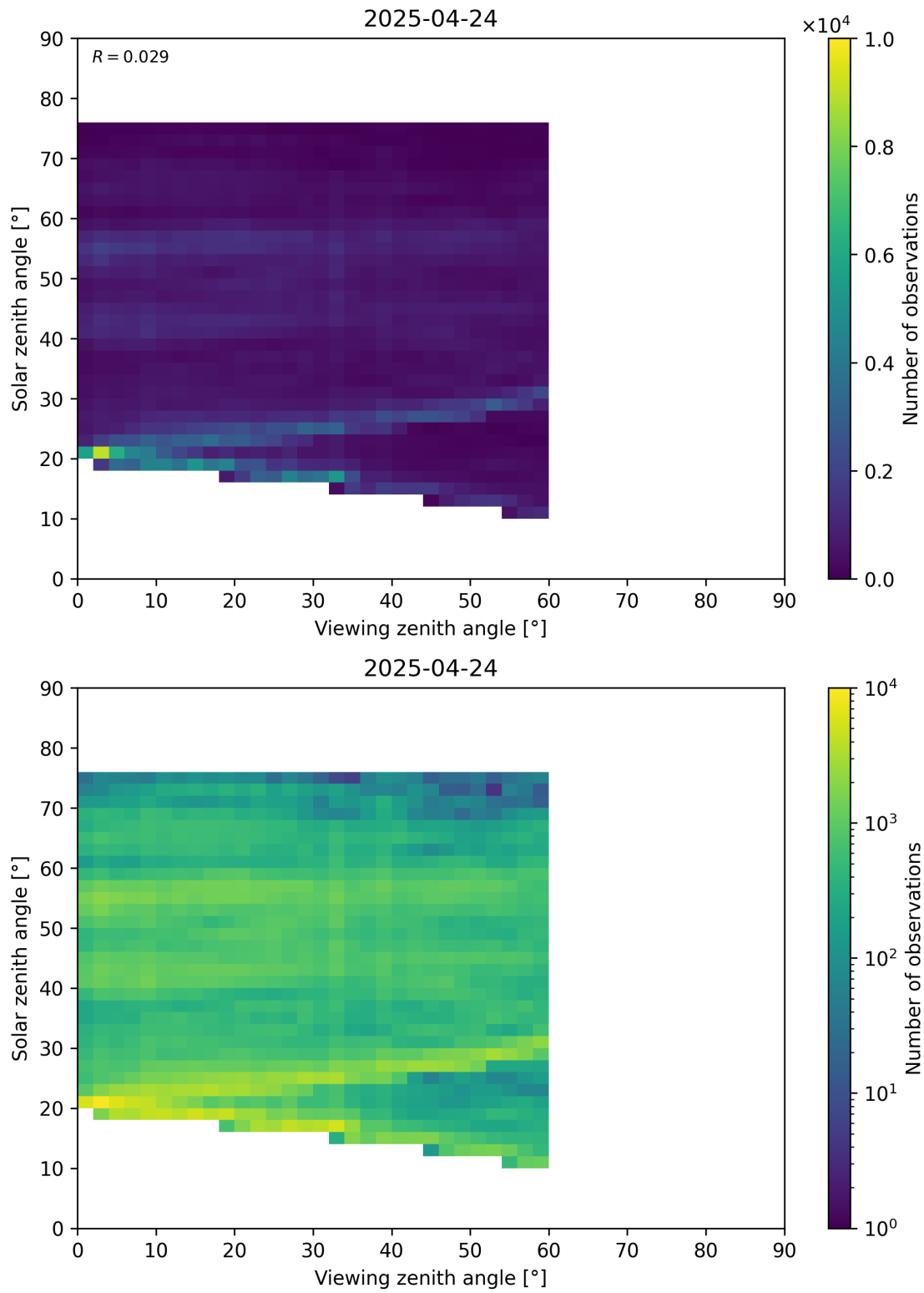
Figure 115: Scatter density plot of “Viewing zenith angle” against “Solar zenith angle” for 2025-04-24 to 2025-04-25.
