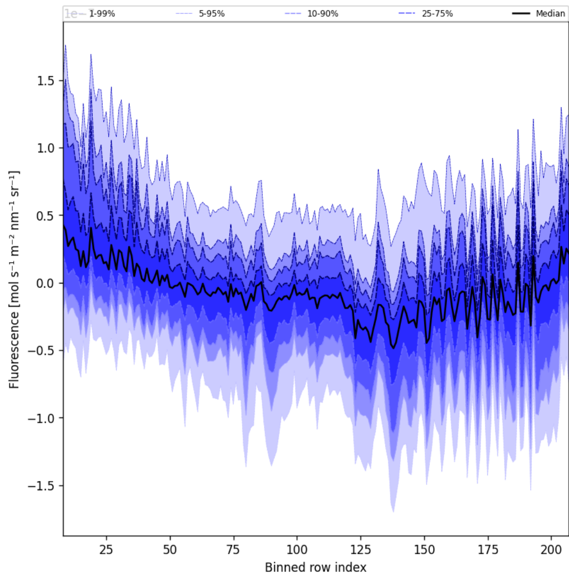
Figure 43: Along track statistics of “Fluorescence” for 2025-04-24 to 2025-04-25
