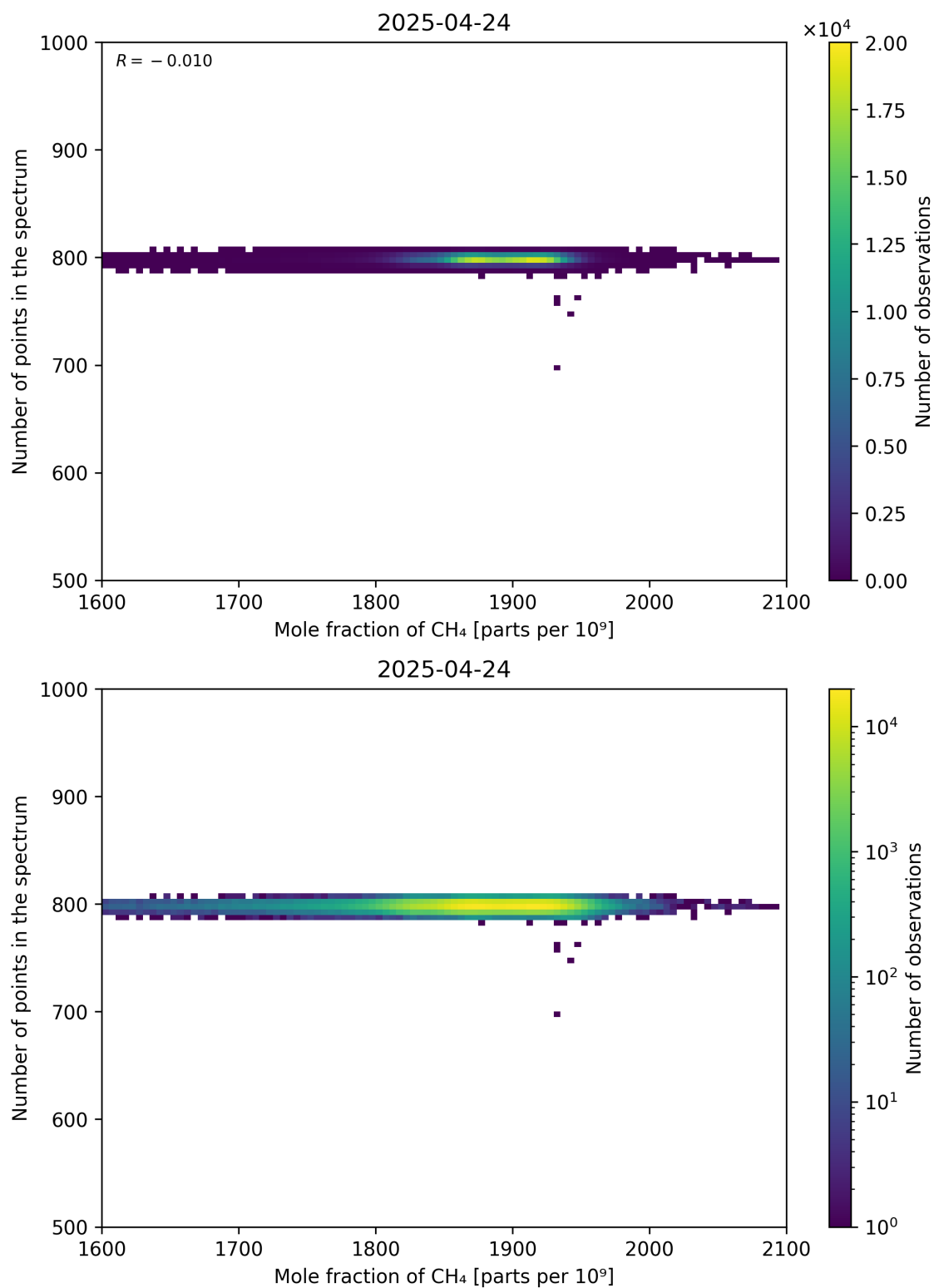
Figure 77: Scatter density plot of “Mole fraction of CH 4 ” against “Number of points in the spectrum” for 2025-04-24 to 2025-04-25.
