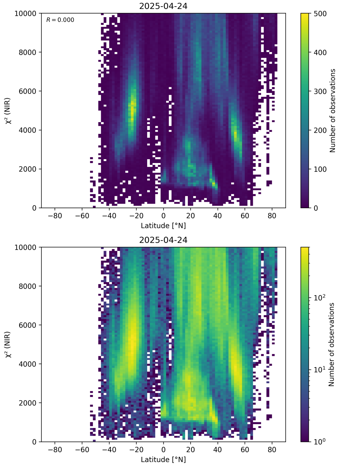
Figure 53: Scatter density plot of “Latitude” against “ \chi^2 (NIR)” for 2025-04-24 to 2025-04-25.
