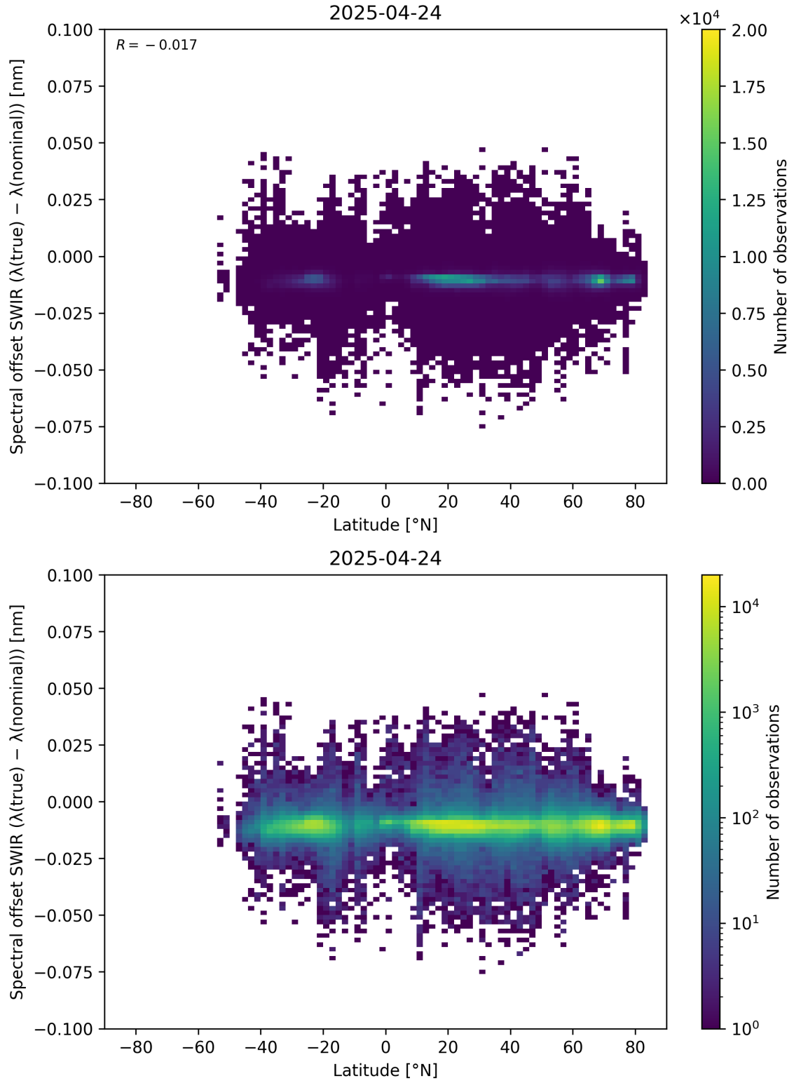
Figure 62: Scatter density plot of “Latitude” against “Spectral offset SWIR ( \lambda_{\text{true}} - \lambda_{\text{nominal}} )” for 2025-04-24 to 2025-04-25.
