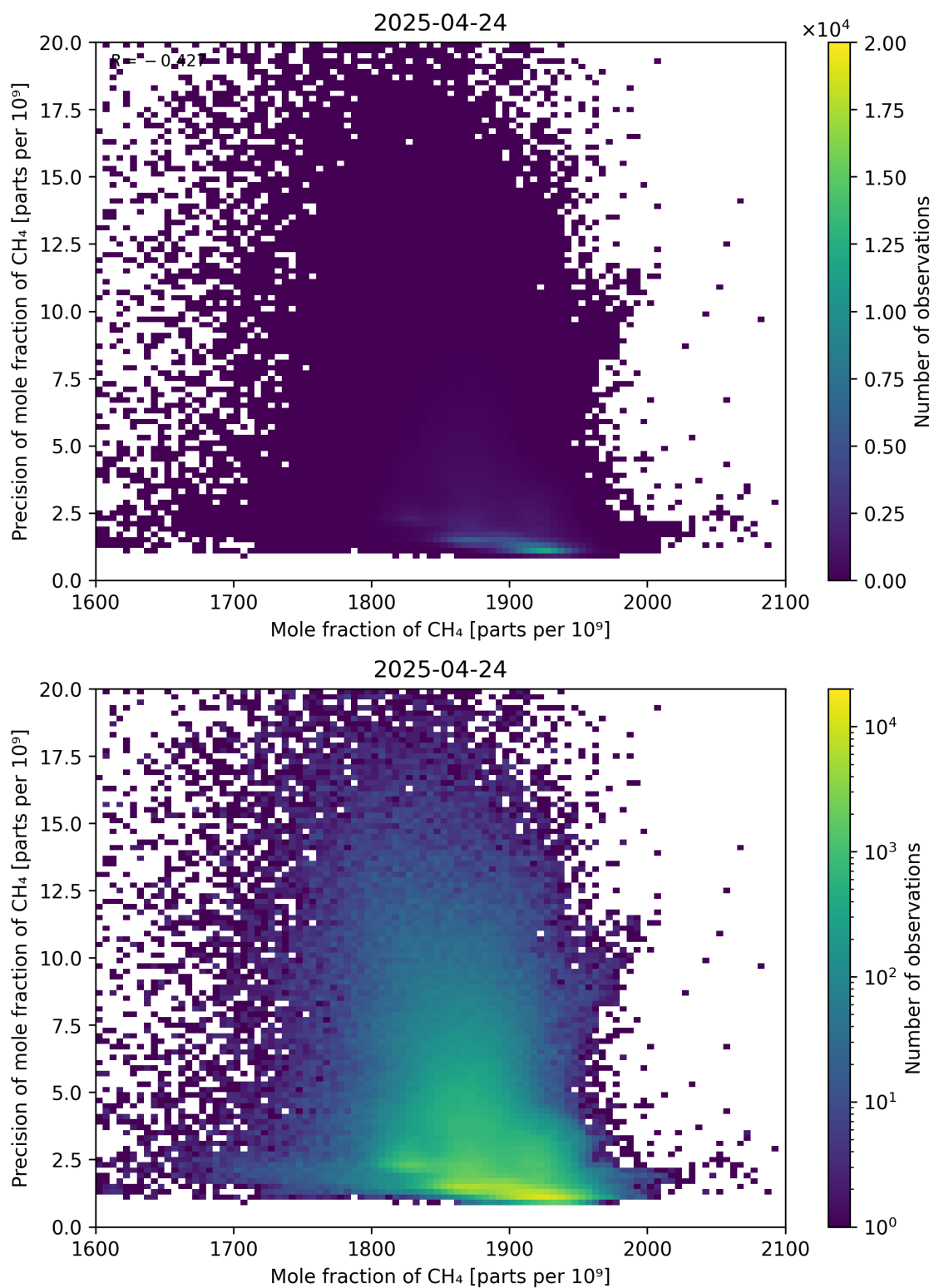
Figure 75: Scatter density plot of “Mole fraction of CH 4 ” against “Precision of mole fraction of CH 4 ” for 2025-04-24 to 2025-04-25.
