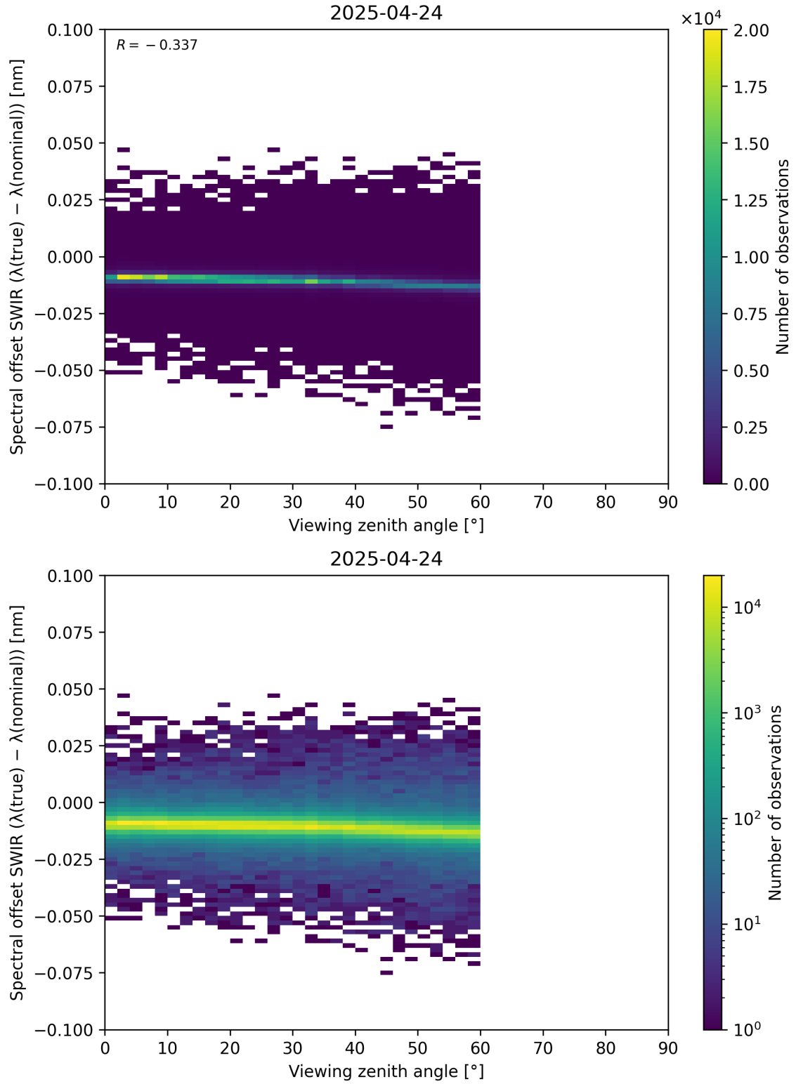
Figure 116: Scatter density plot of “Viewing zenith angle” against “Spectral offset SWIR ( \lambda_{\text{true}} - \lambda_{\text{nominal}} )” for 2025-04-24 to 2025-04-25.
