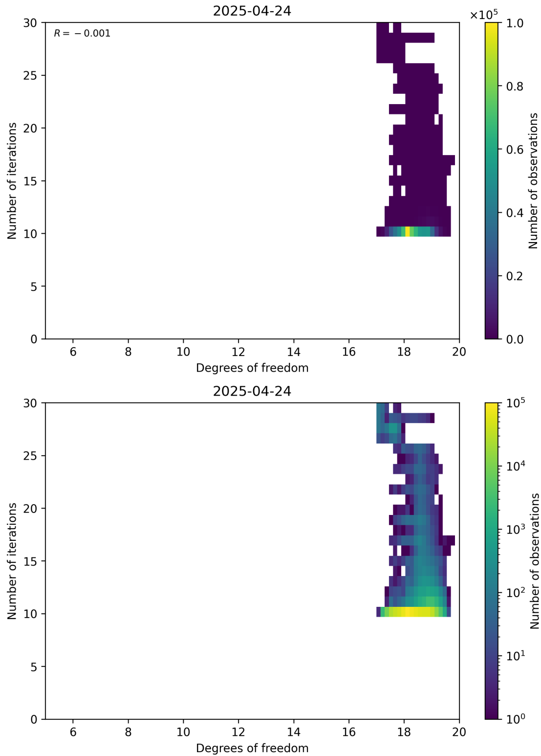
Figure 52: Scatter density plot of “Degrees of freedom” against “Number of iterations” for 2025-04-24 to 2025-04-25.
