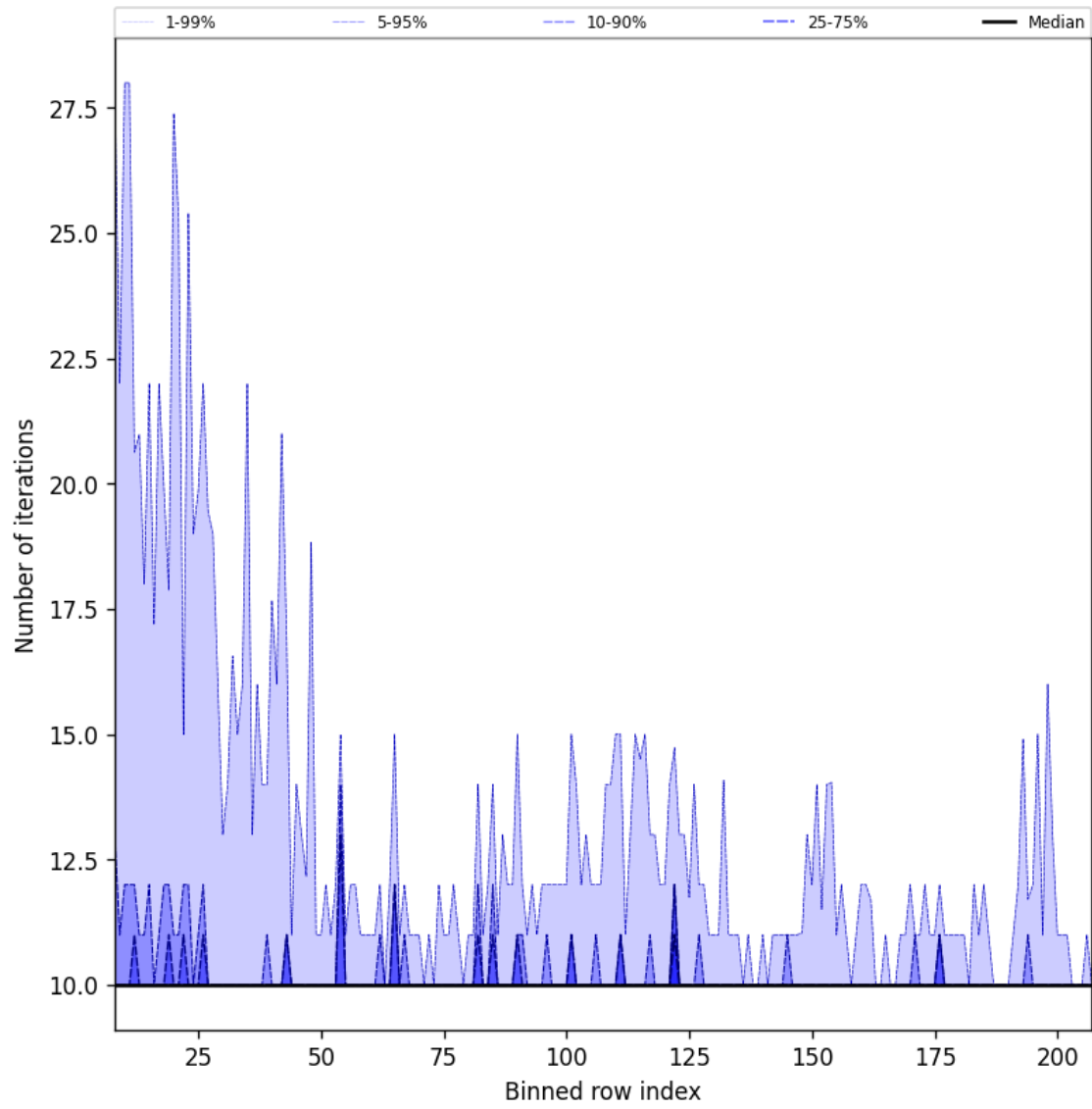
Figure 42: Along track statistics of “Number of iterations” for 2025-04-24 to 2025-04-25
