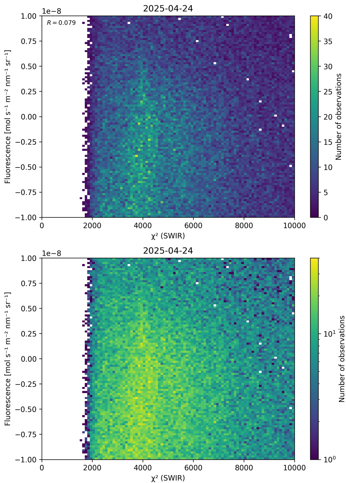
Figure 49: Scatter density plot of “ \chi^2 (SWIR)” against “Fluorescence” for 2025-04-24 to 2025-04-25.
