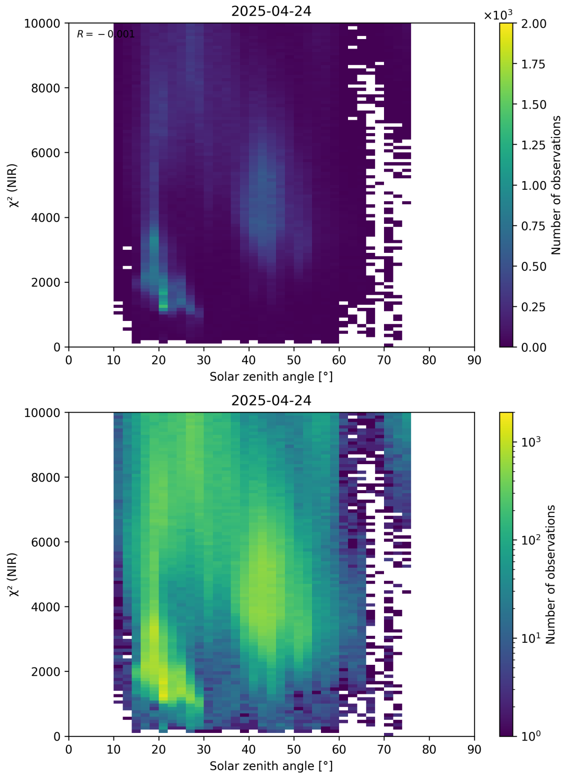
Figure 94: Scatter density plot of “Solar zenith angle” against “ \chi^2 (NIR)” for 2025-04-24 to 2025-04-25.
