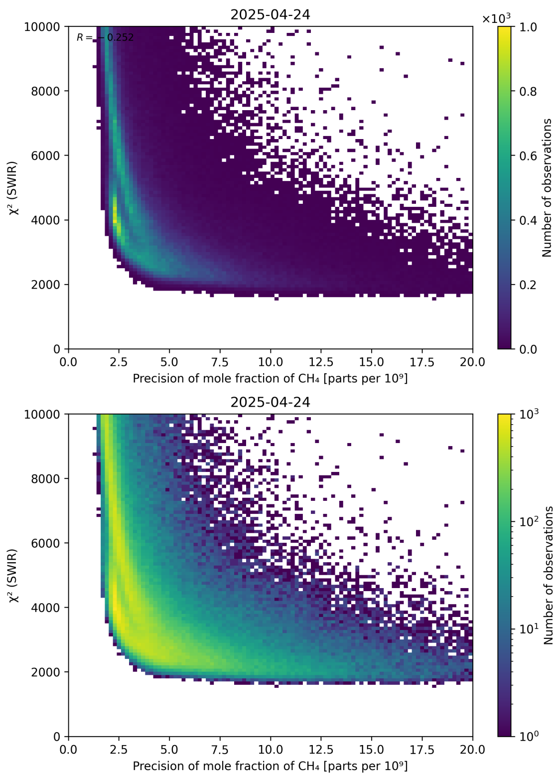
Figure 79: Scatter density plot of “Precision of mole fraction of \text{CH}_4 ” against “ \chi^2 (SWIR)” for 2025-04-24 to 2025-04-25.
