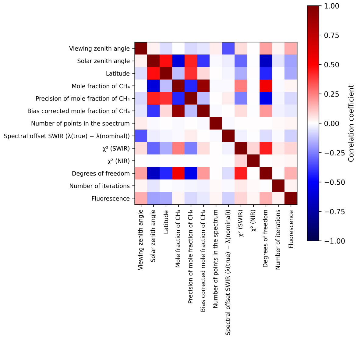
Figure 2: Map of correlation matrix for 2025-04-24 to 2025-04-25.
