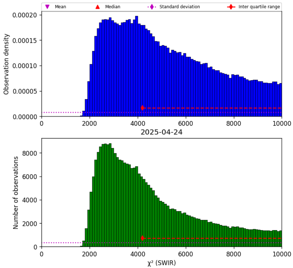
Figure 28: Histogram of “ \chi^2 (SWIR)” for 2025-04-24 to 2025-04-25
