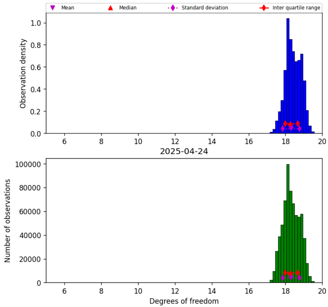
Figure 30: Histogram of “Degrees of freedom” for 2025-04-24 to 2025-04-25
