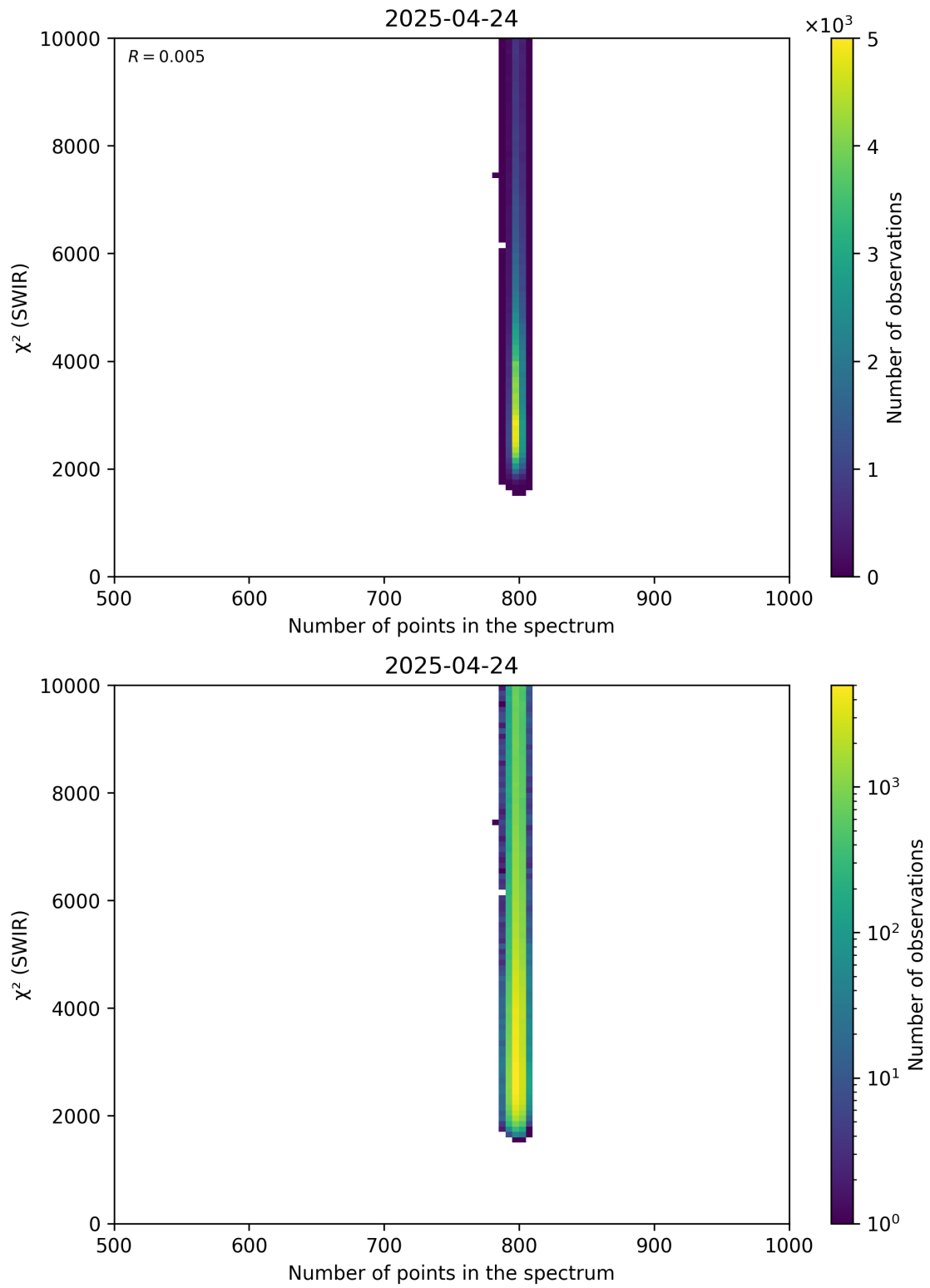
Figure 89: Scatter density plot of “Number of points in the spectrum” against “ \chi^2 (SWIR)” for 2025-04-24 to 2025-04-25.
