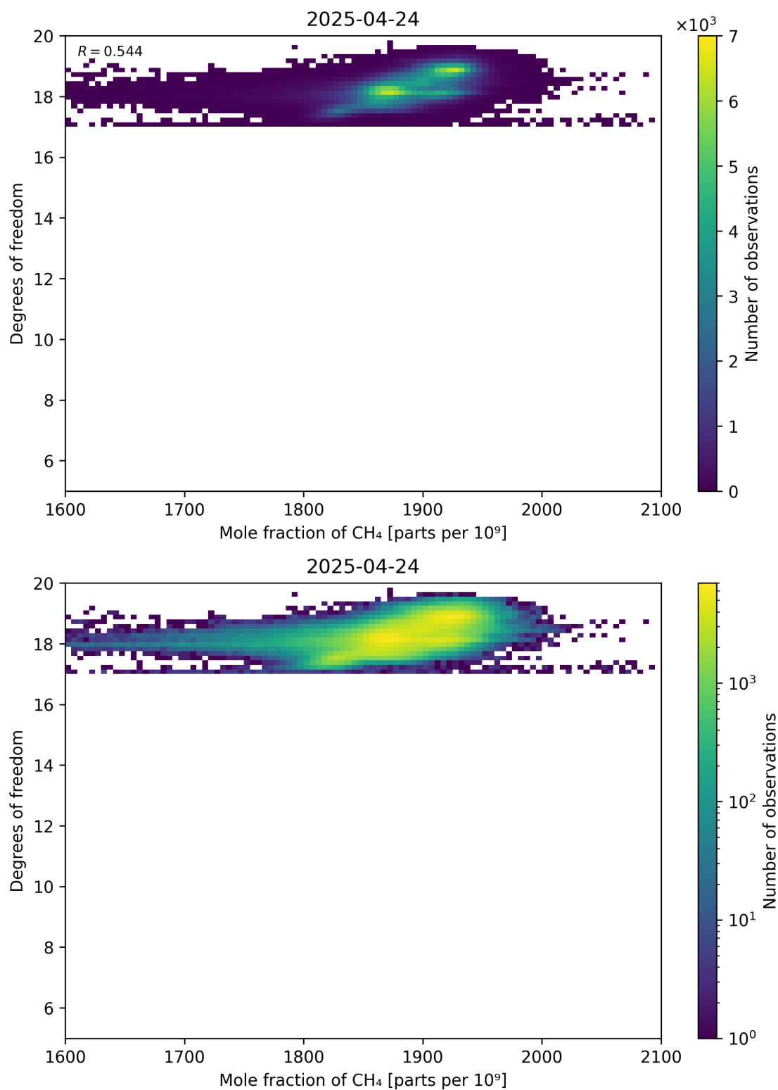
Figure 72: Scatter density plot of “Mole fraction of CH 4 ” against “Degrees of freedom” for 2025-04-24 to 2025-04-25.
