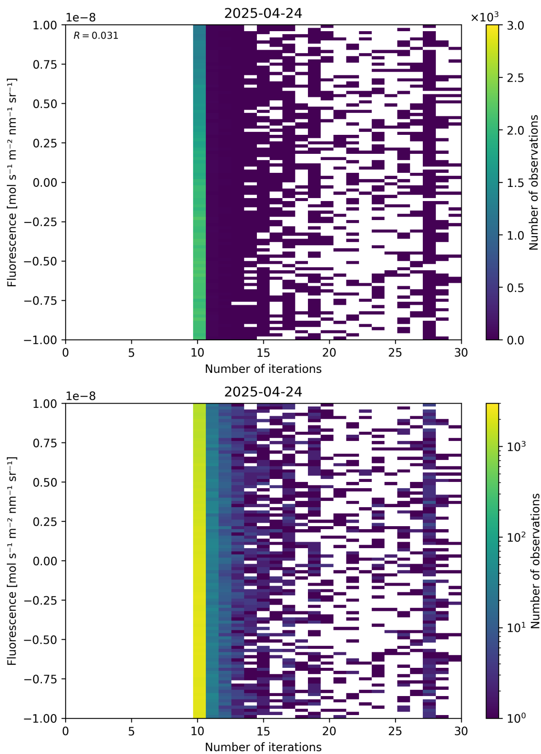
Figure 87: Scatter density plot of “Number of iterations” against “Fluorescence” for 2025-04-24 to 2025-04-25.
