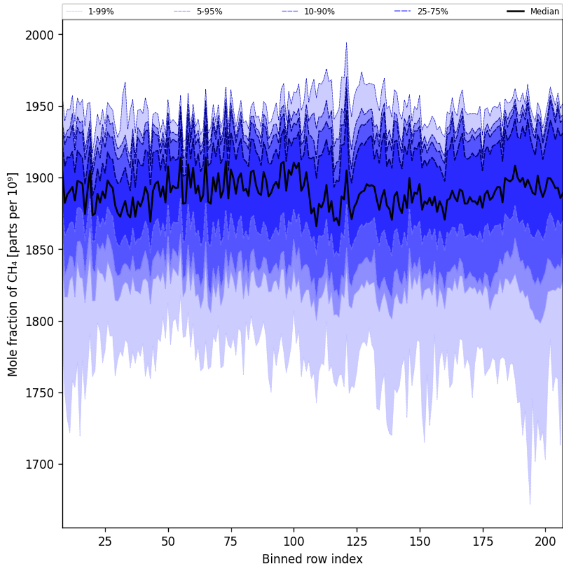
Figure 34: Along track statistics of “Mole fraction of CH 4 ” for 2025-04-24 to 2025-04-25
