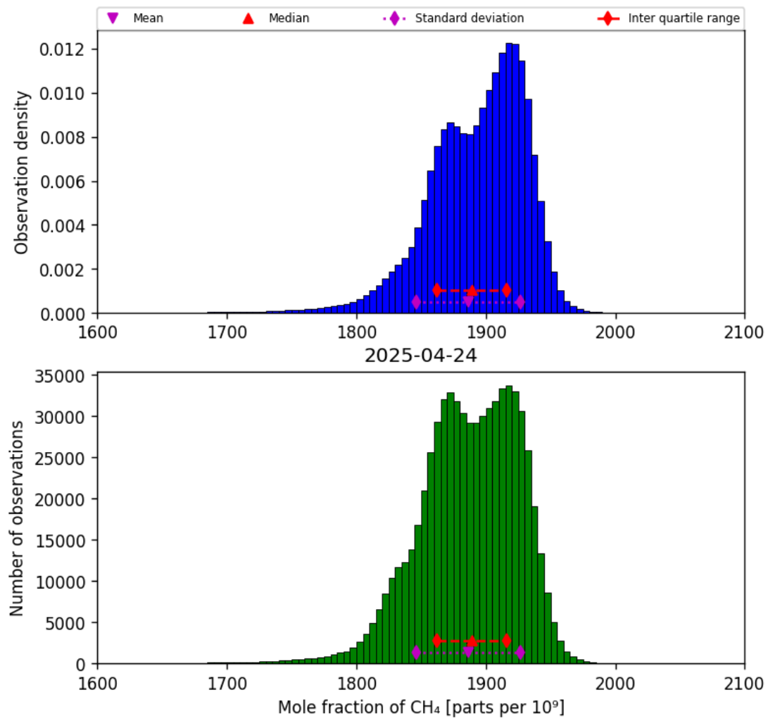
Figure 23: Histogram of “Mole fraction of CH 4 ” for 2025-04-24 to 2025-04-25
