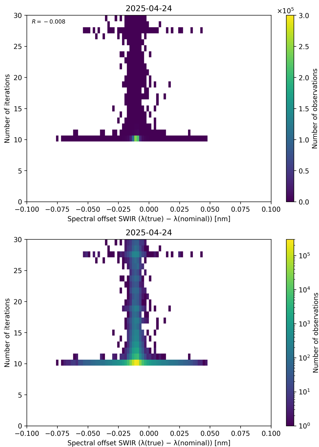
Figure 121: Scatter density plot of “Spectral offset SWIR ( \lambda_{\text{true}} - \lambda_{\text{nominal}} )” against “Number of iterations” for 2025-04-24 to 2025-04-25.
