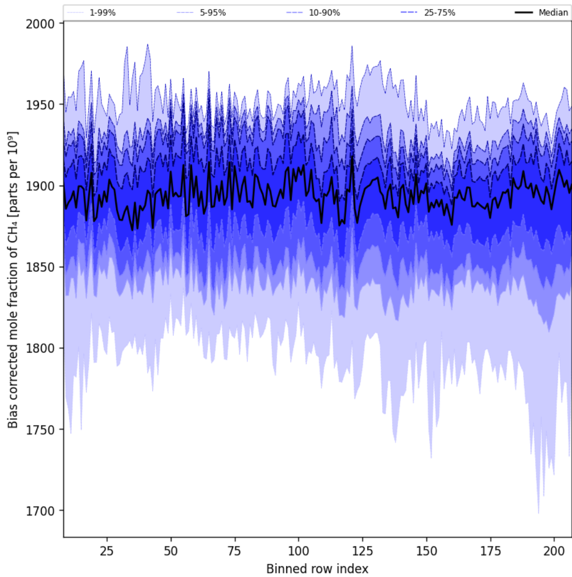
Figure 36: Along track statistics of “Bias corrected mole fraction of CH 4 ” for 2025-04-24 to 2025-04-25
