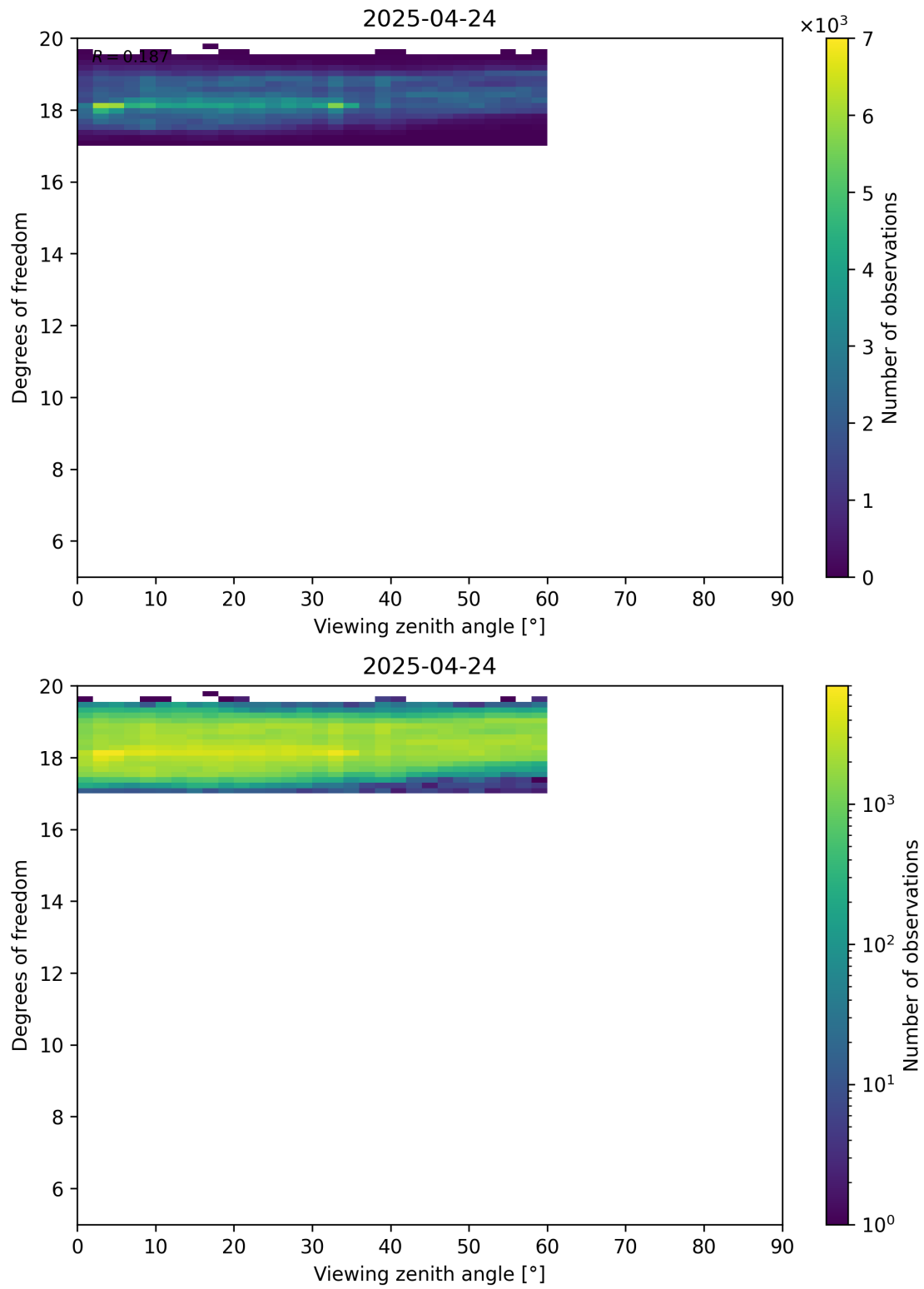
Figure 107: Scatter density plot of “Viewing zenith angle” against “Degrees of freedom” for 2025-04-24 to 2025-04-25.
