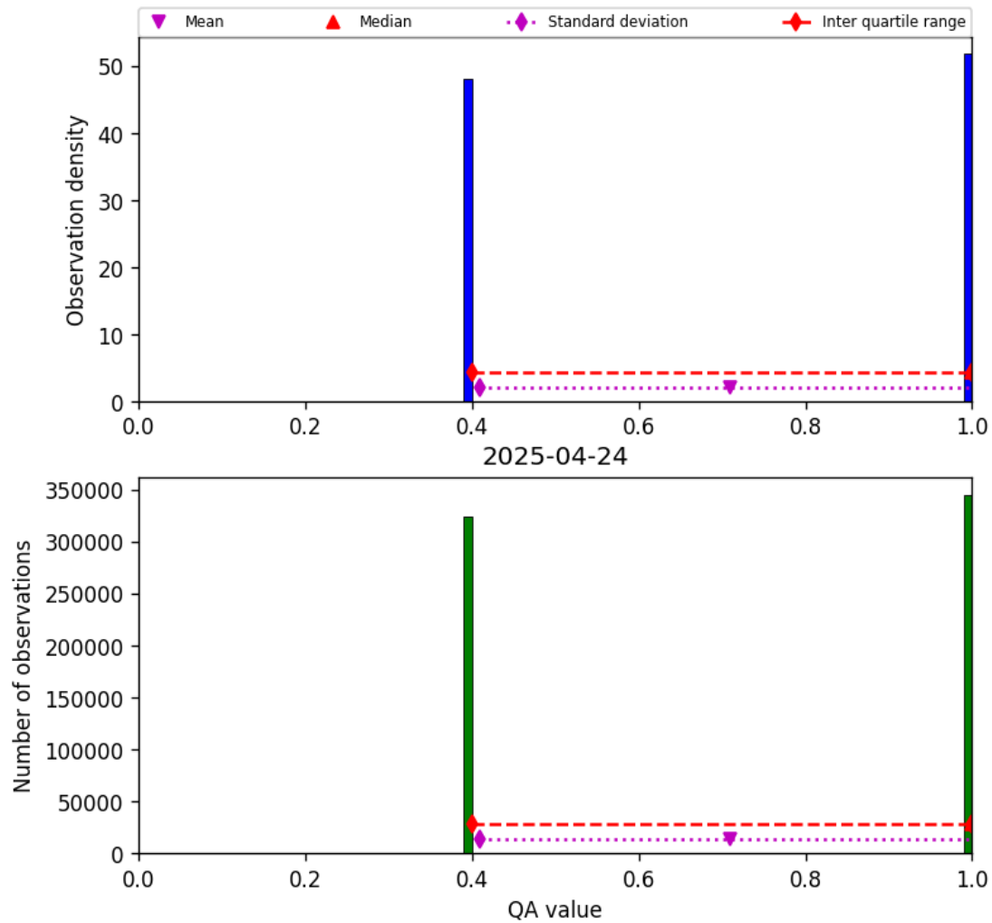
Figure 22: Histogram of “QA value” for 2025-04-24 to 2025-04-25
