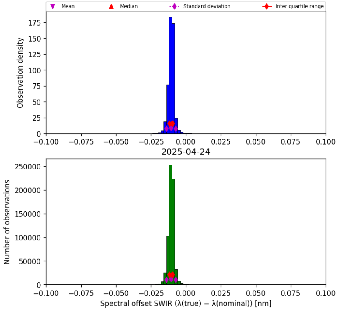
Figure 27: Histogram of “Spectral offset SWIR ( \lambda_{\text{true}} - \lambda_{\text{nominal}} )” for 2025-04-24 to 2025-04-25
