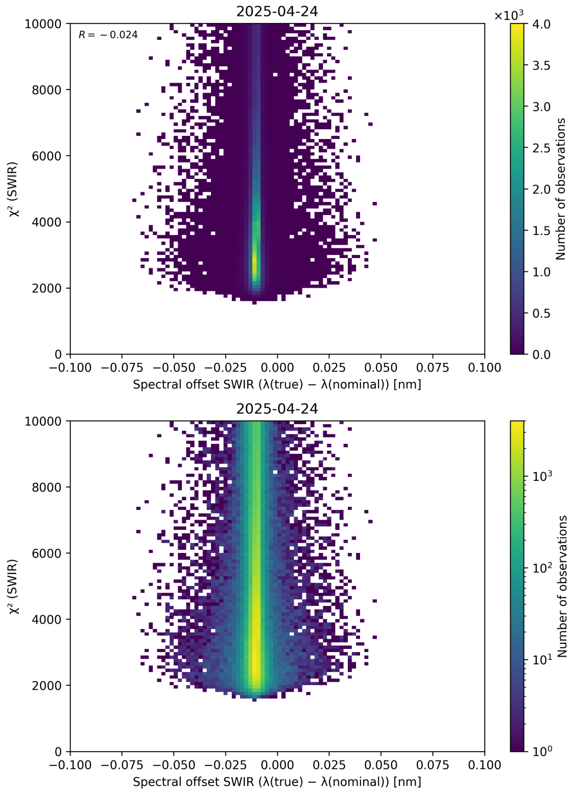
Figure 118: Scatter density plot of “Spectral offset SWIR ( \lambda_{\text{true}} - \lambda_{\text{nominal}} )” against “ \chi^2 (SWIR)” for 2025-04-24 to 2025-04-25.
