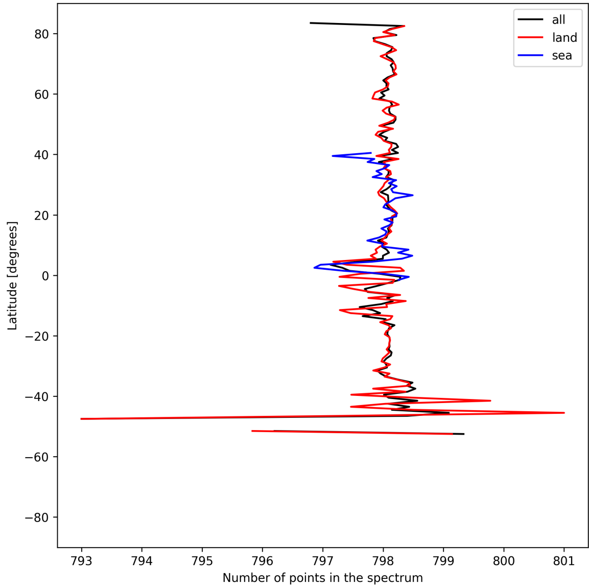
Figure 15: Zonal average of “Number of points in the spectrum” for 2025-04-24 to 2025-04-25.
