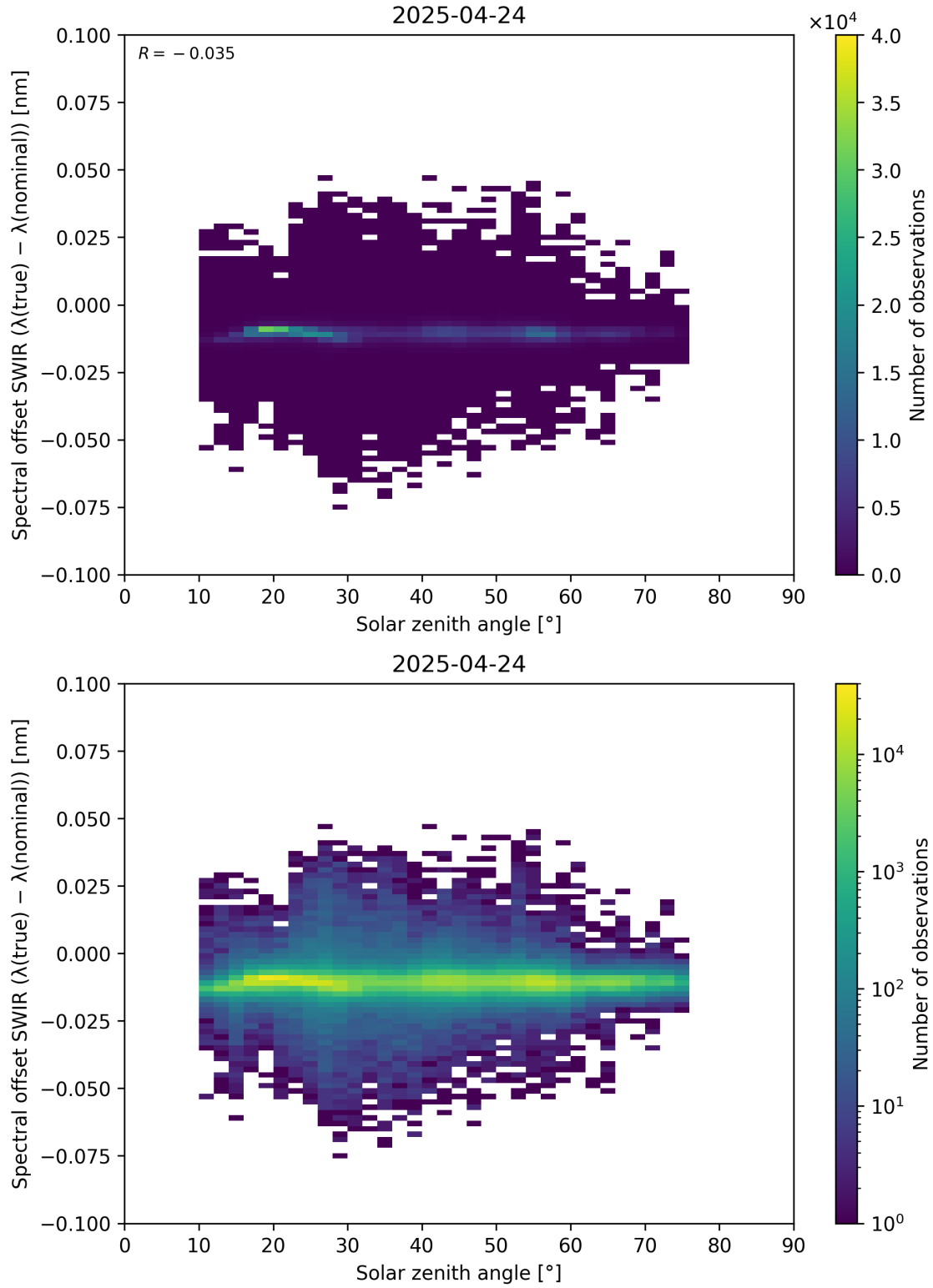
Figure 104: Scatter density plot of “Solar zenith angle” against “Spectral offset SWIR ( \lambda_{\text{true}} - \lambda_{\text{nominal}} )” for 2025-04-24 to 2025-04-25.
