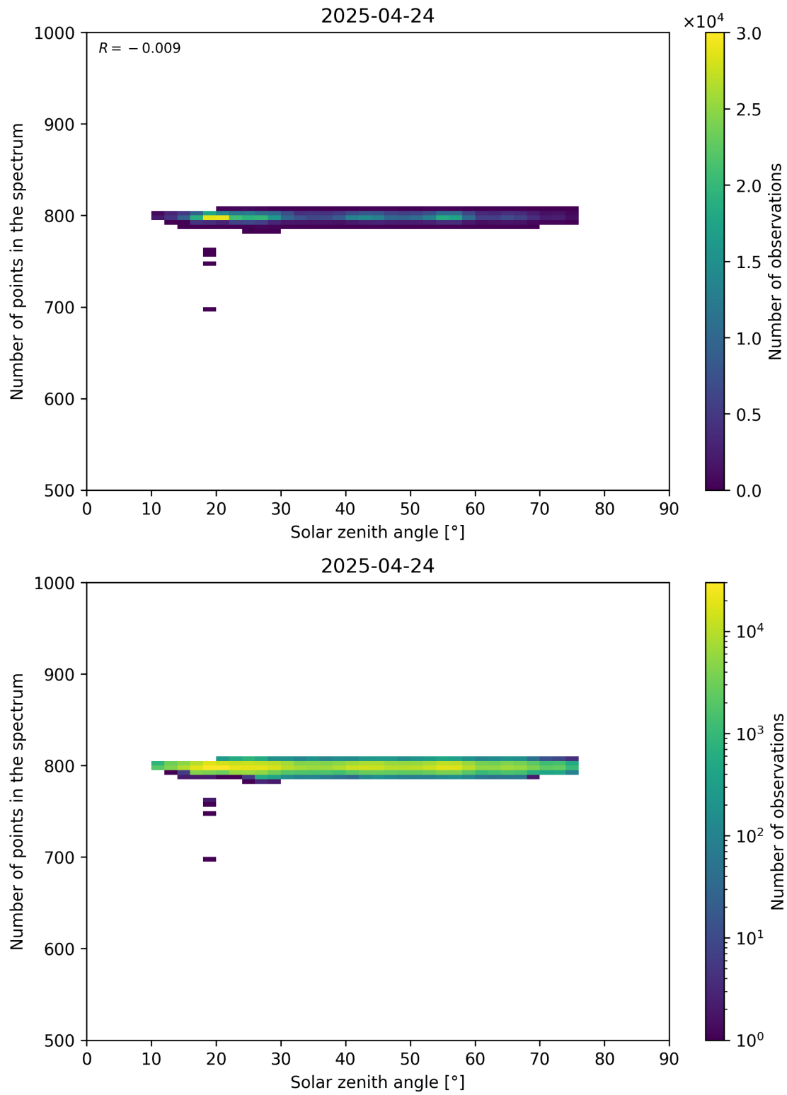
Figure 103: Scatter density plot of “Solar zenith angle” against “Number of points in the spectrum” for 2025-04-24 to 2025-04-25.
