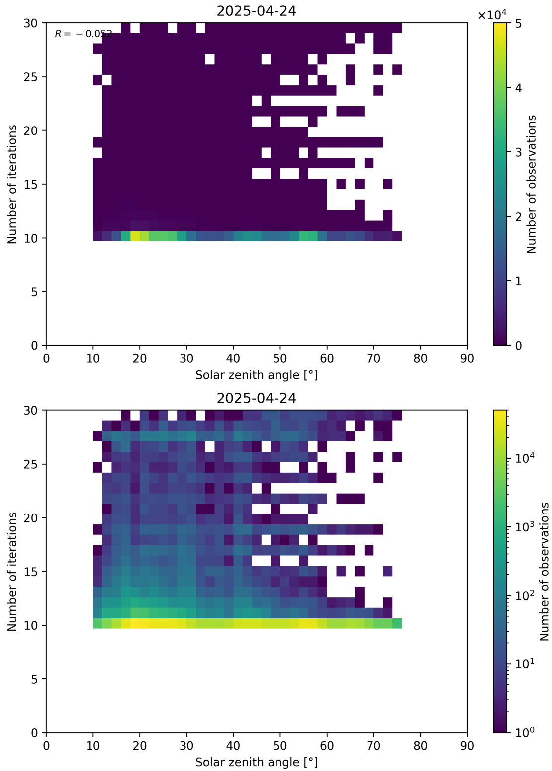
Figure 102: Scatter density plot of “Solar zenith angle” against “Number of iterations” for 2025-04-24 to 2025-04-25.
