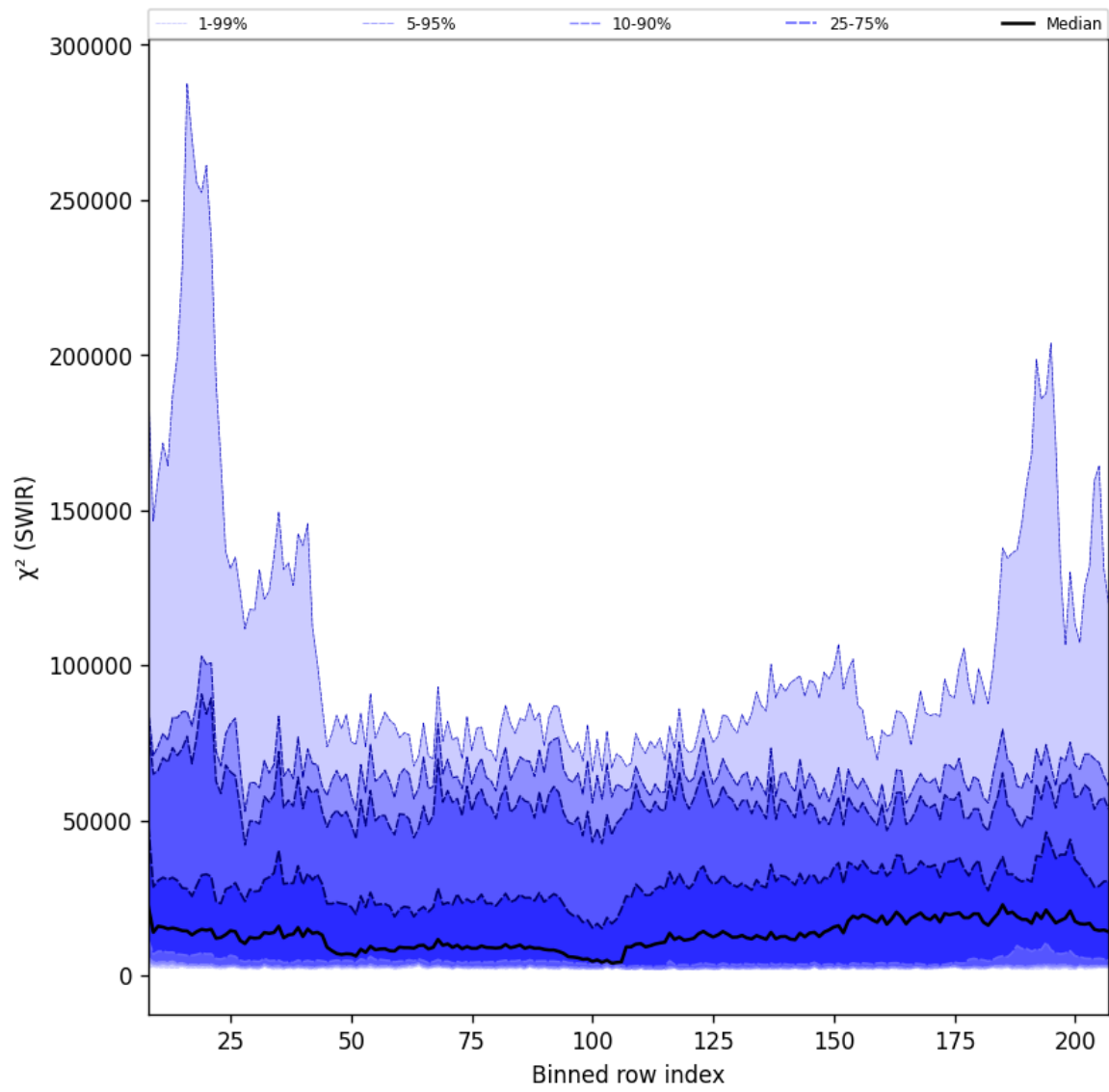
Figure 39: Along track statistics of “ \chi^2 (SWIR)” for 2025-04-24 to 2025-04-25
