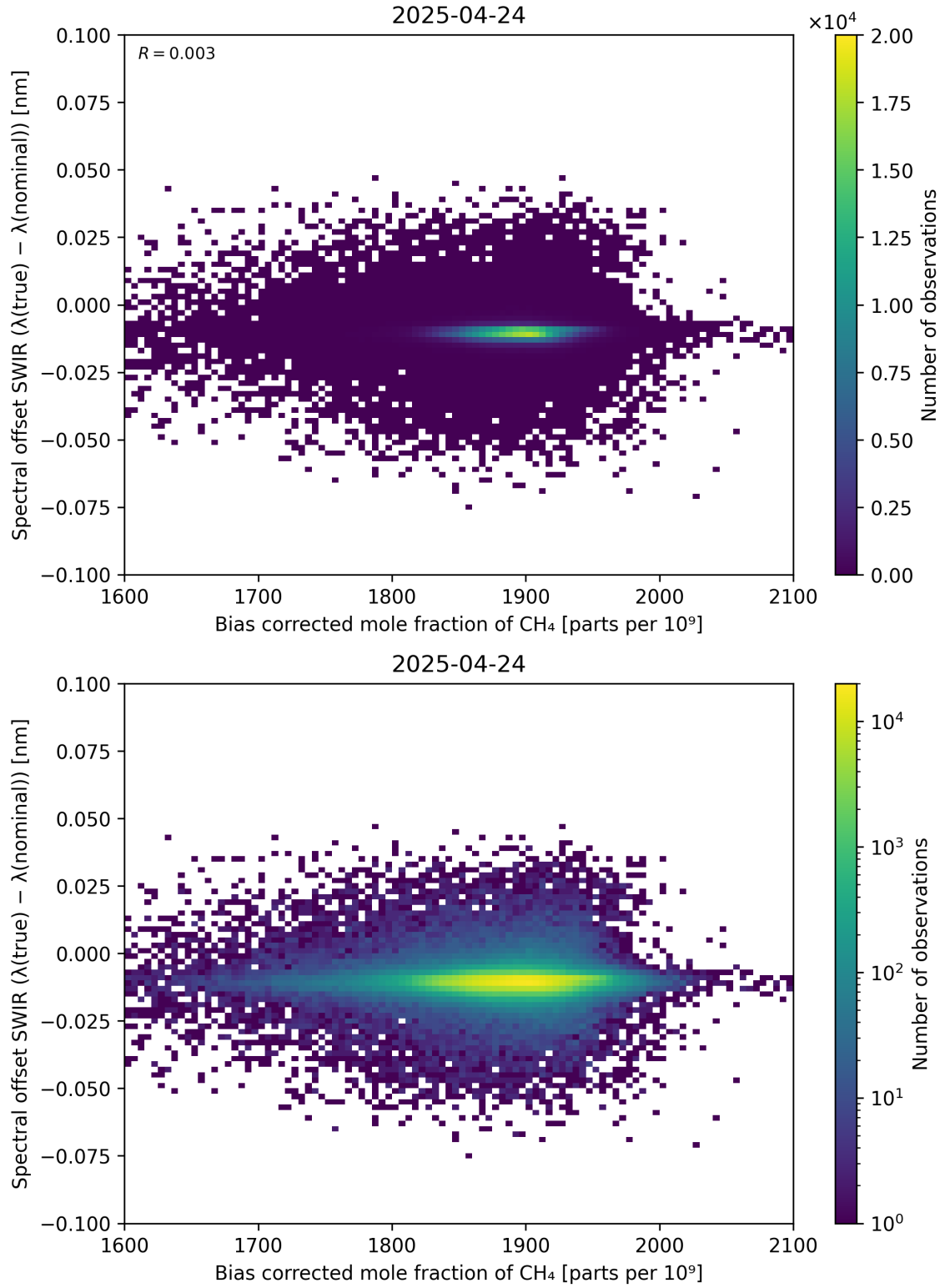
Figure 69: Scatter density plot of “Bias corrected mole fraction of \text{CH}_4 ” against “Spectral offset SWIR ( \lambda_{\text{true}} - \lambda_{\text{nominal}} )” for 2025-04-24 to 2025-04-25.
