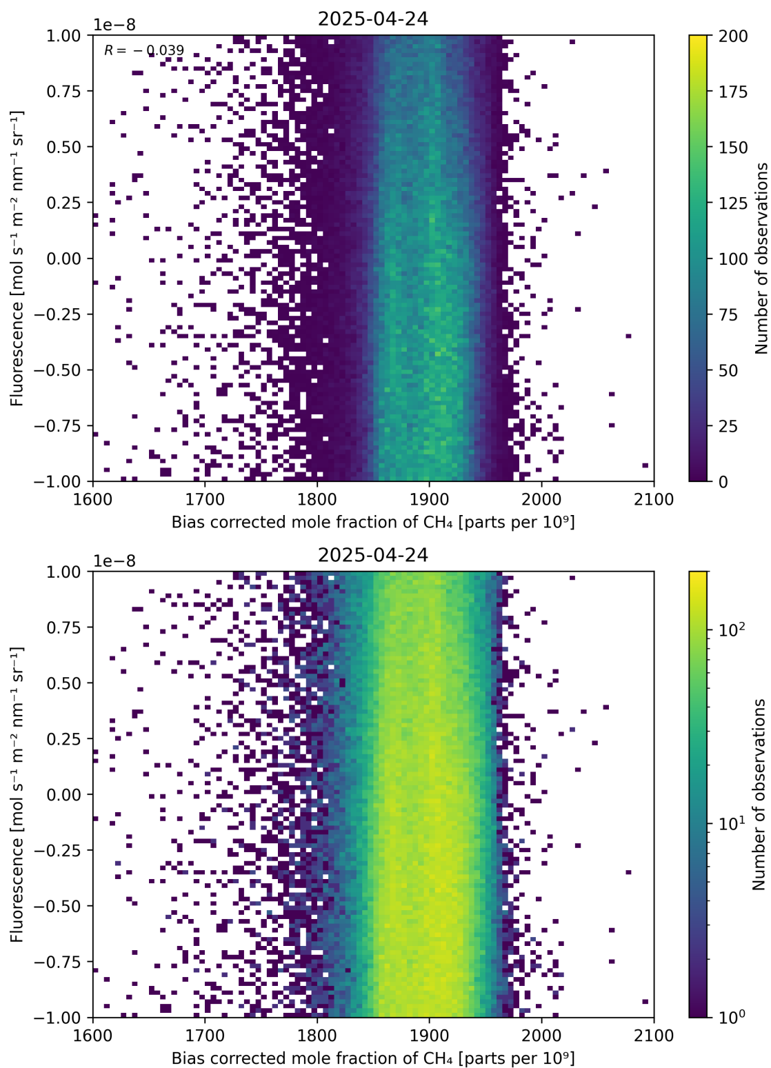
Figure 66: Scatter density plot of “Bias corrected mole fraction of \text{CH}_4 ” against “Fluorescence” for 2025-04-24 to 2025-04-25.
