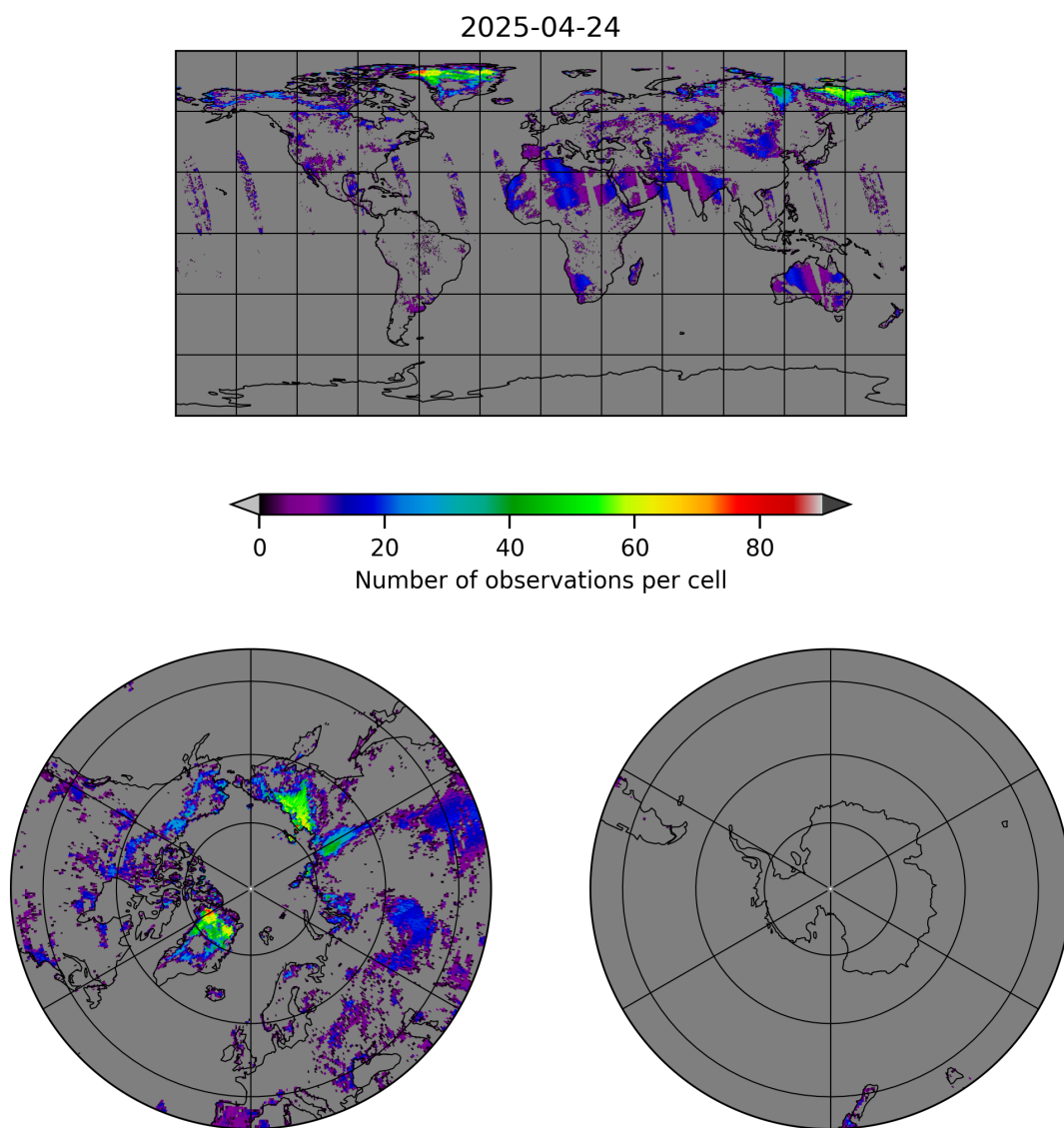
Figure 10: Map of the number of observations for 2025-04-24 to 2025-04-25
