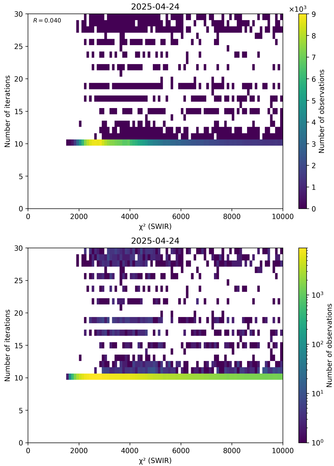
Figure 50: Scatter density plot of “ \chi^2 (SWIR)” against “Number of iterations” for 2025-04-24 to 2025-04-25.
