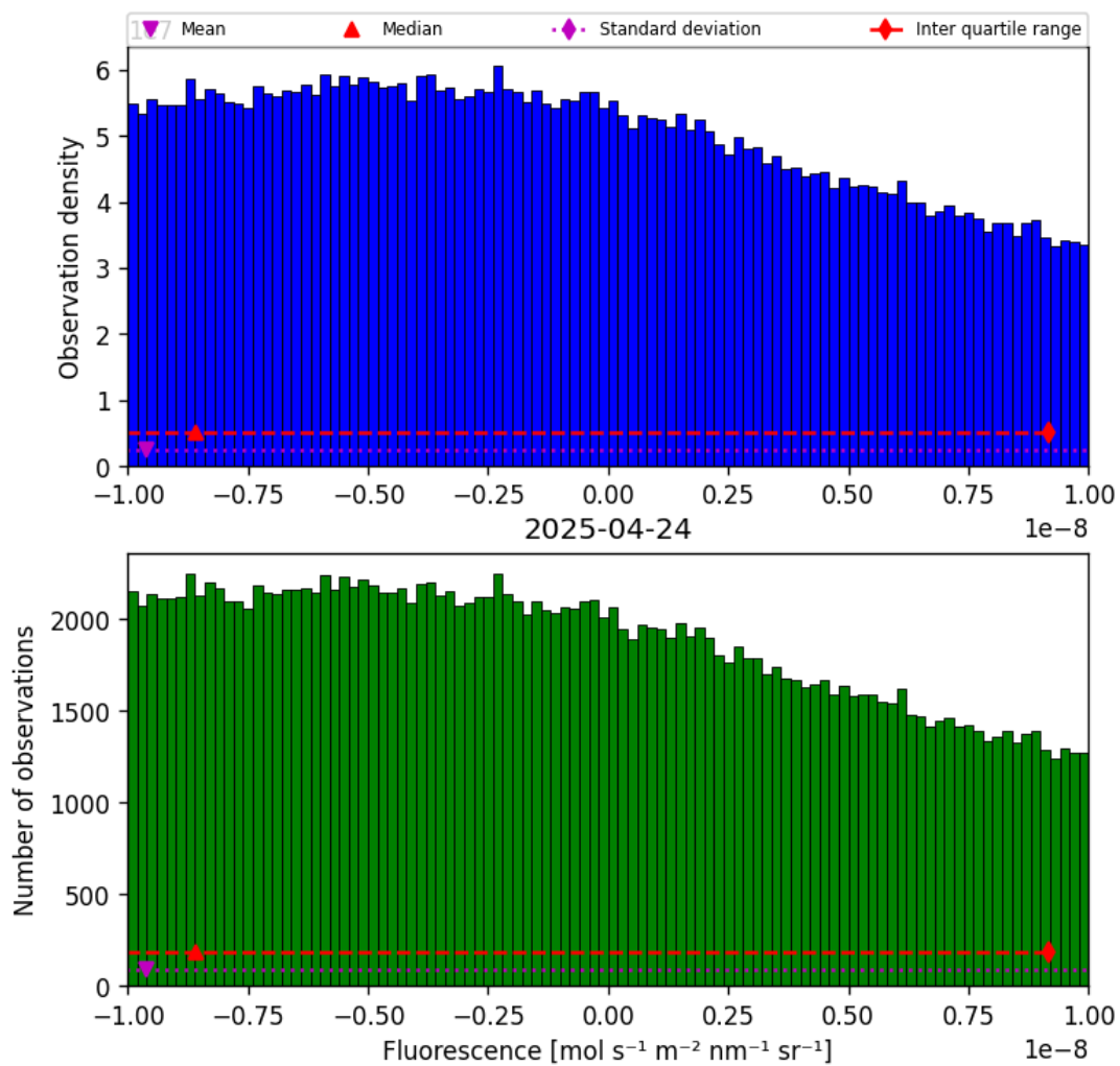
Figure 32: Histogram of “Fluorescence” for 2025-04-24 to 2025-04-25
