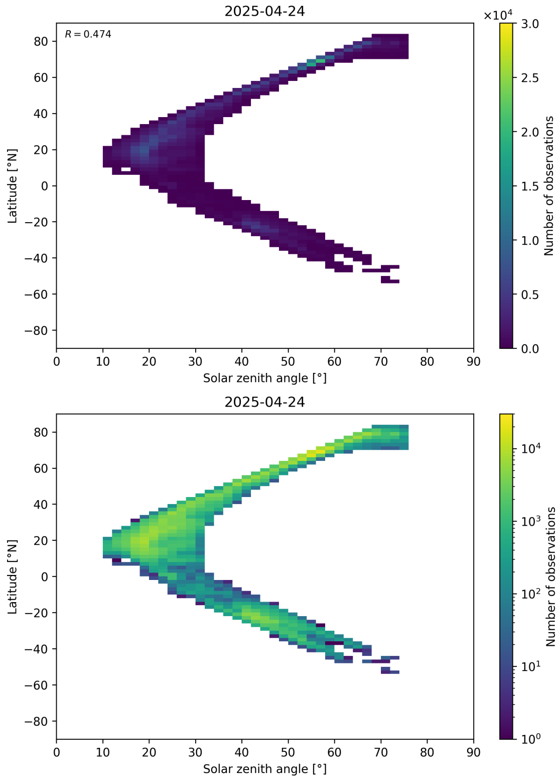
Figure 98: Scatter density plot of “Solar zenith angle” against “Latitude” for 2025-04-24 to 2025-04-25.
