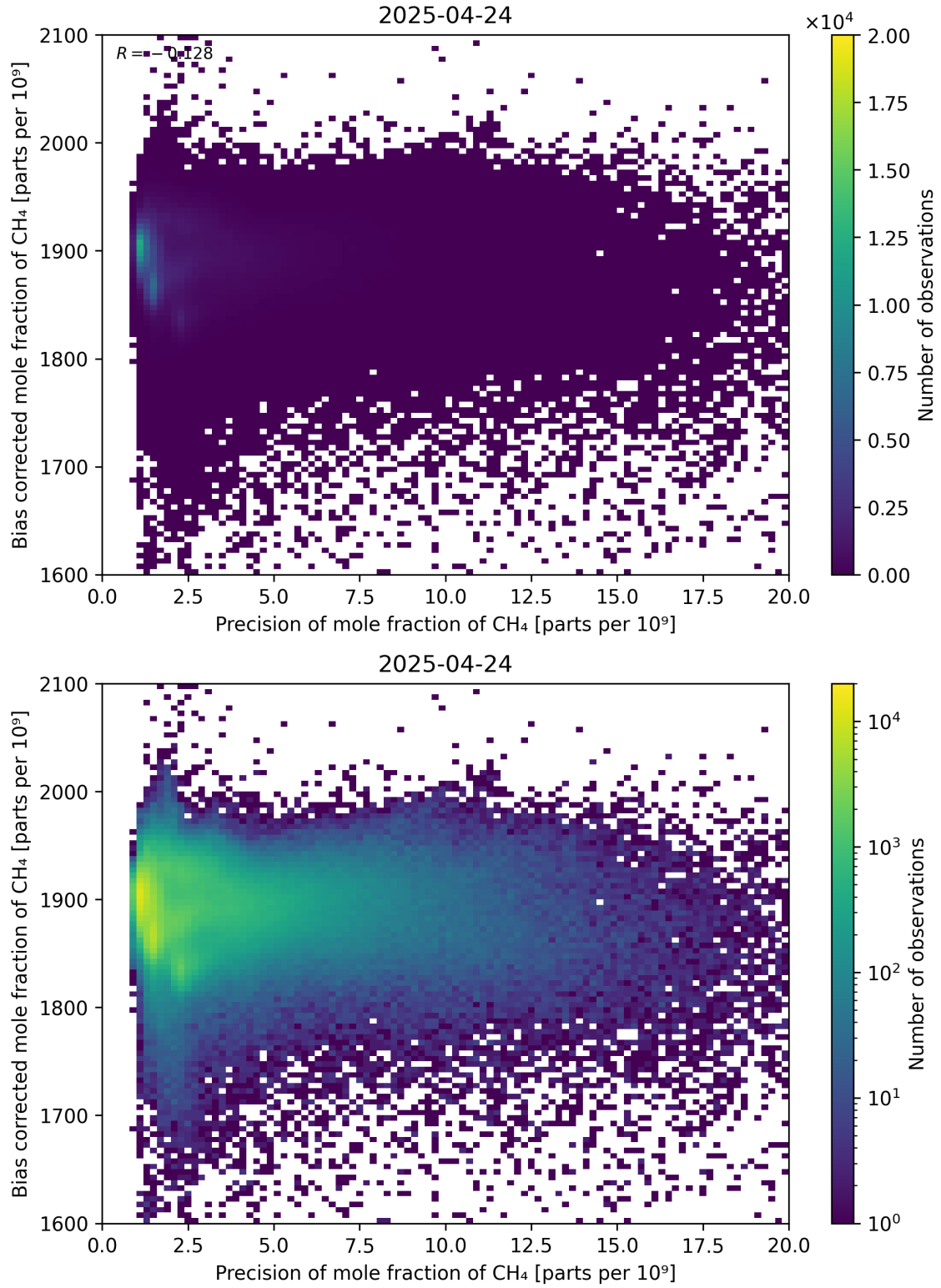
Figure 82: Scatter density plot of “Precision of mole fraction of CH 4 ” against “Bias corrected mole fraction of CH 4 ” for 2025-04-24 to 2025-04-25.
