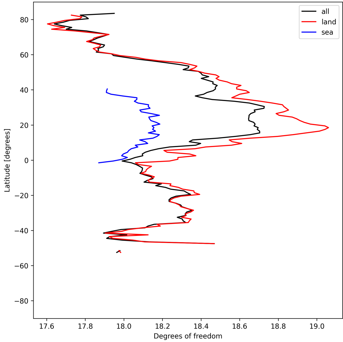
Figure 19: Zonal average of “Degrees of freedom” for 2025-04-24 to 2025-04-25.
