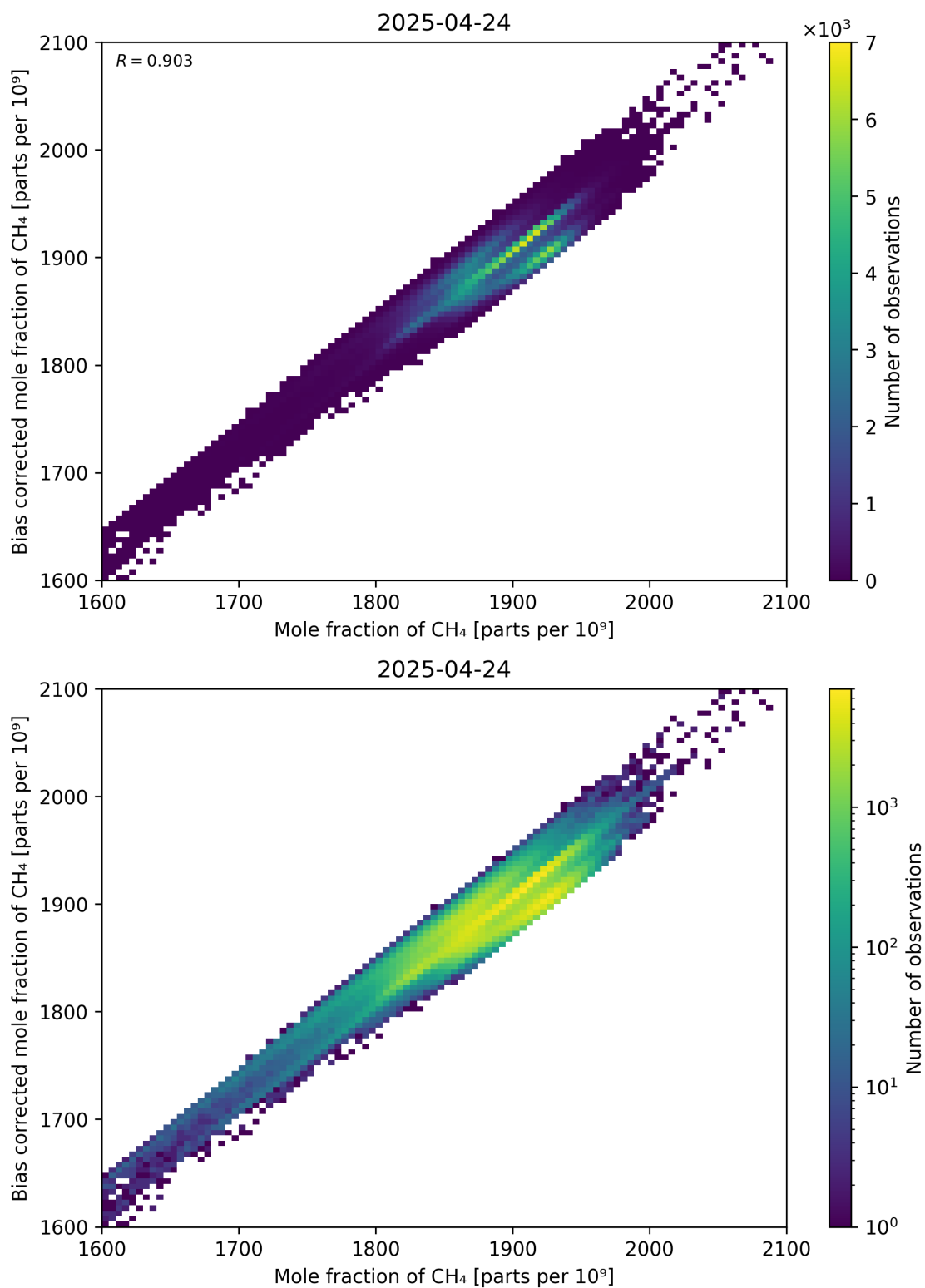
Figure 74: Scatter density plot of “Mole fraction of CH 4 ” against “Bias corrected mole fraction of CH 4 ” for 2025-04-24 to 2025-04-25.
