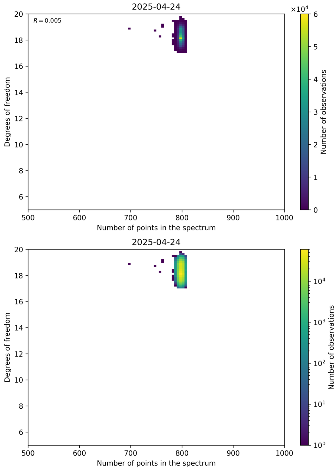
Figure 90: Scatter density plot of “Number of points in the spectrum” against “Degrees of freedom” for 2025-04-24 to 2025-04-25.
