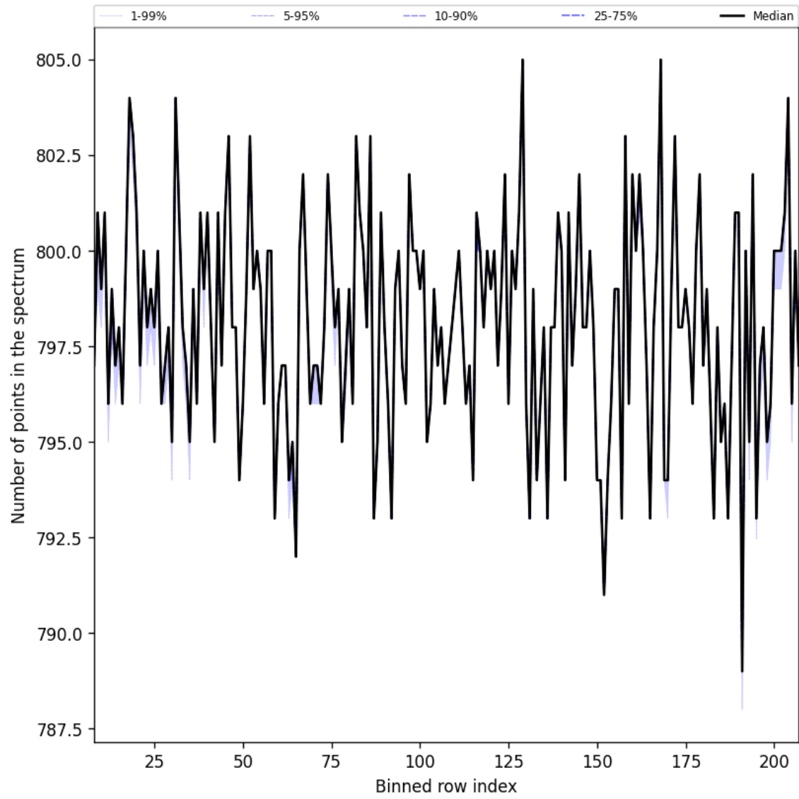
Figure 37: Along track statistics of “Number of points in the spectrum” for 2025-04-24 to 2025-04-25
