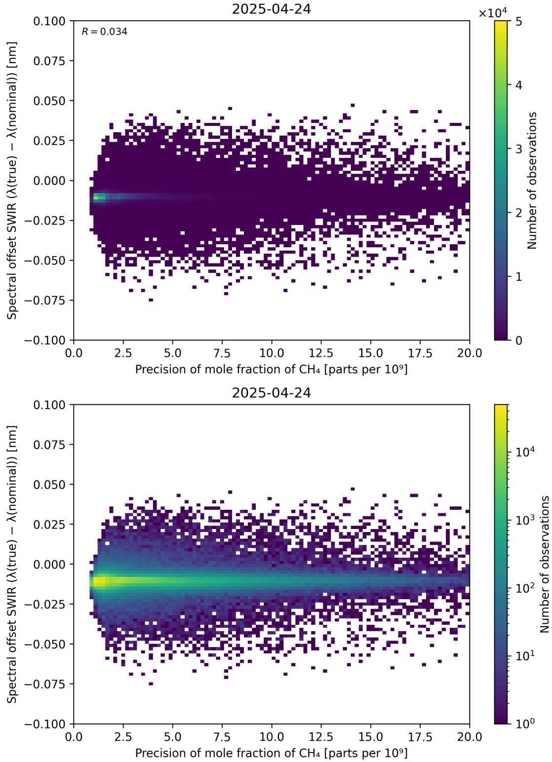
Figure 85: Scatter density plot of “Precision of mole fraction of \text{CH}_4 ” against “Spectral offset SWIR ( \lambda_{\text{true}} - \lambda_{\text{nominal}} )” for 2025-04-24 to 2025-04-25.
