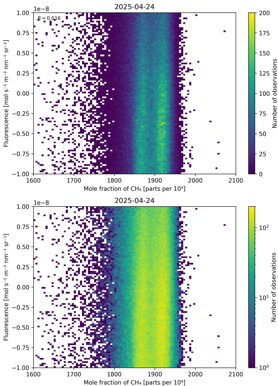
Figure 73: Scatter density plot of “Mole fraction of \text{CH}_4 ” against “Fluorescence” for 2025-04-24 to 2025-04-25.
