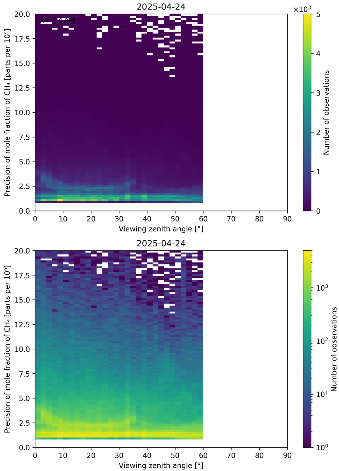
Figure 112: Scatter density plot of “Viewing zenith angle” against “Precision of mole fraction of CH 4 ” for 2025-04-24 to 2025-04-25.
