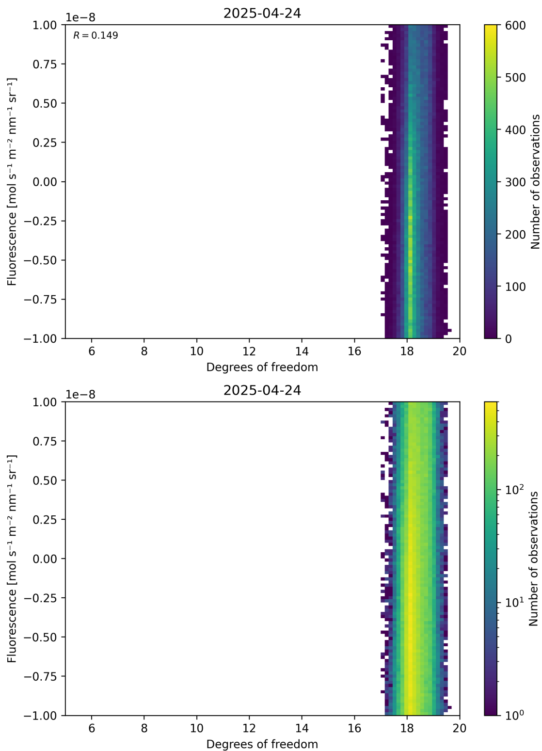
Figure 51: Scatter density plot of “Degrees of freedom” against “Fluorescence” for 2025-04-24 to 2025-04-25.
