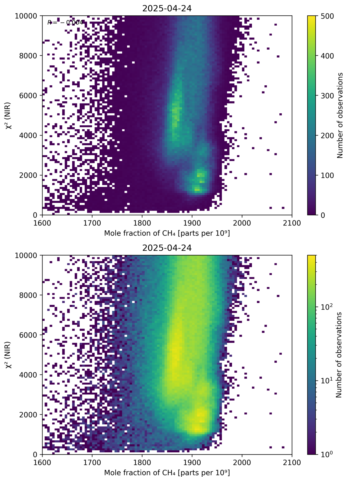
Figure 70: Scatter density plot of “Mole fraction of CH 4 ” against “ \chi^2 (NIR)” for 2025-04-24 to 2025-04-25.
