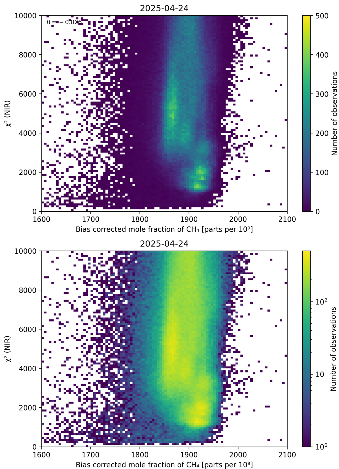
Figure 63: Scatter density plot of “Bias corrected mole fraction of CH 4 ” against “ \chi^2 (NIR)” for 2025-04-24 to 2025-04-25.
