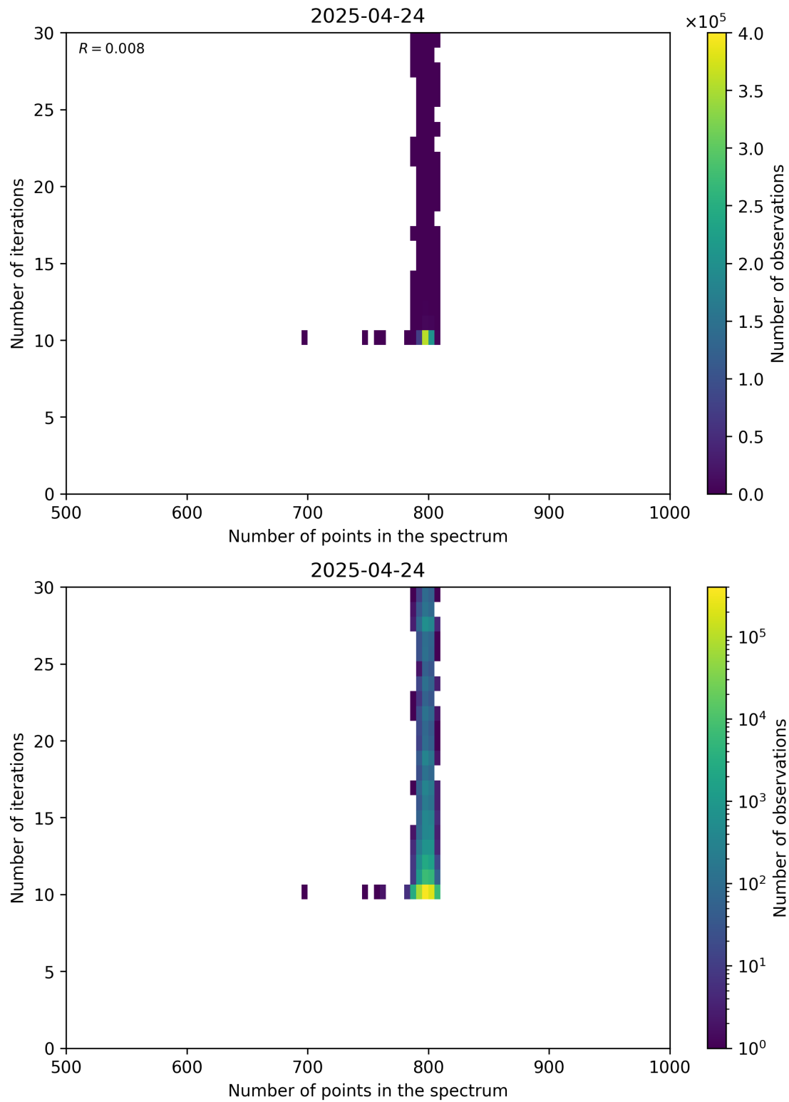
Figure 92: Scatter density plot of “Number of points in the spectrum” against “Number of iterations” for 2025-04-24 to 2025-04-25.
