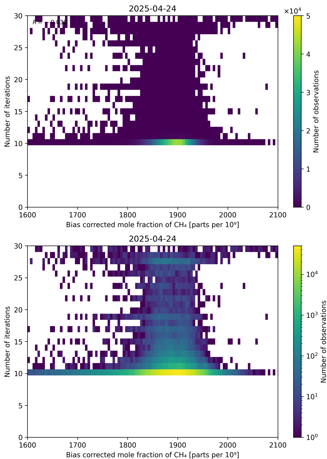
Figure 67: Scatter density plot of “Bias corrected mole fraction of \text{CH}_4 ” against “Number of iterations” for 2025-04-24 to 2025-04-25.
