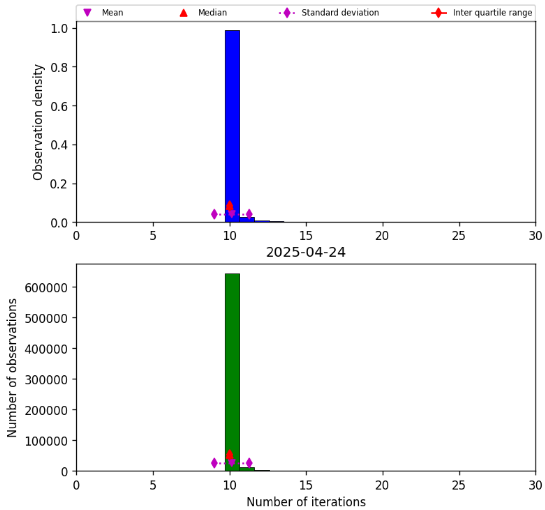
Figure 31: Histogram of “Number of iterations” for 2025-04-24 to 2025-04-25
