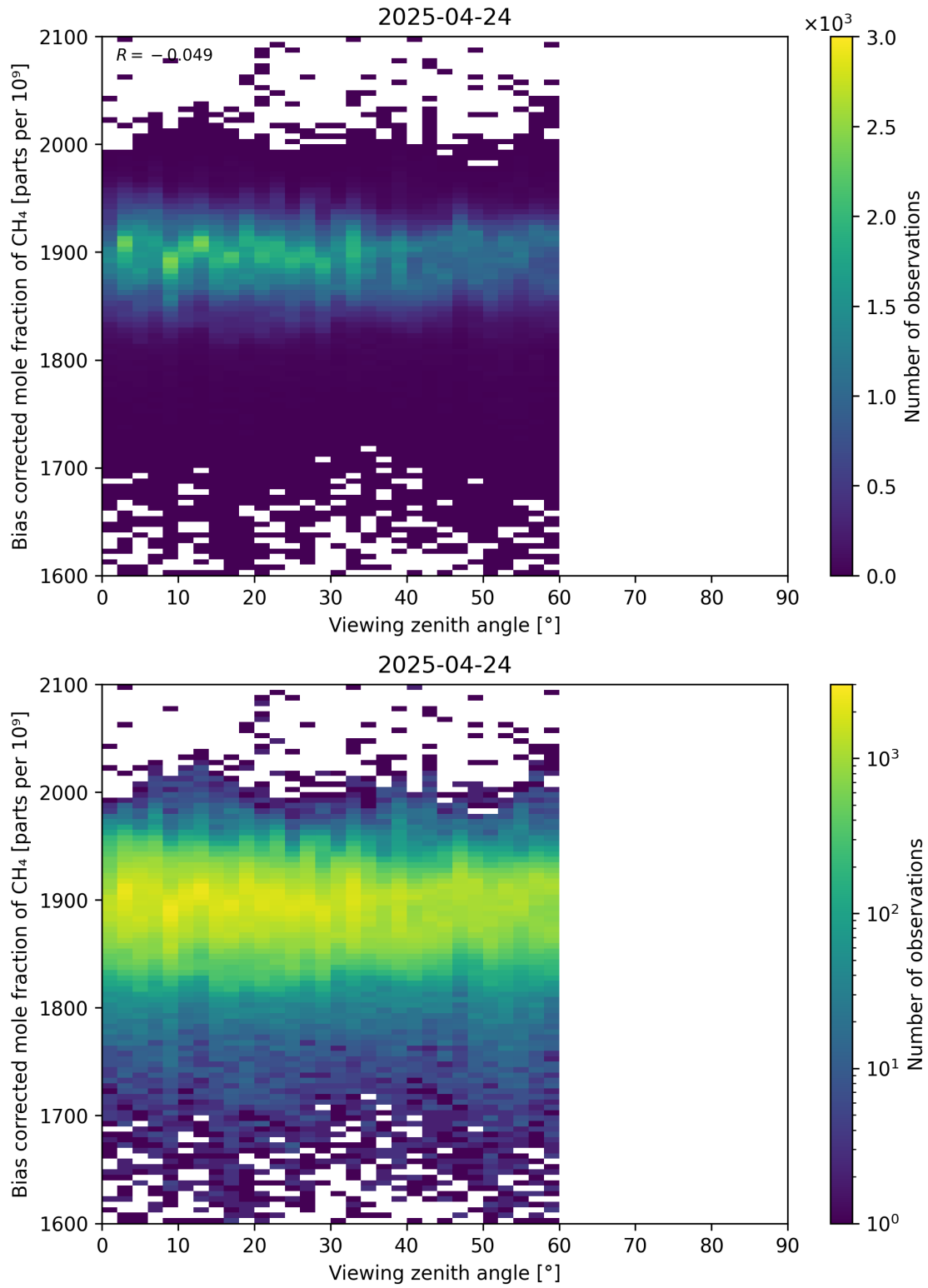
Figure 111: Scatter density plot of “Viewing zenith angle” against “Bias corrected mole fraction of CH 4 ” for 2025-04-24 to 2025-04-25.
