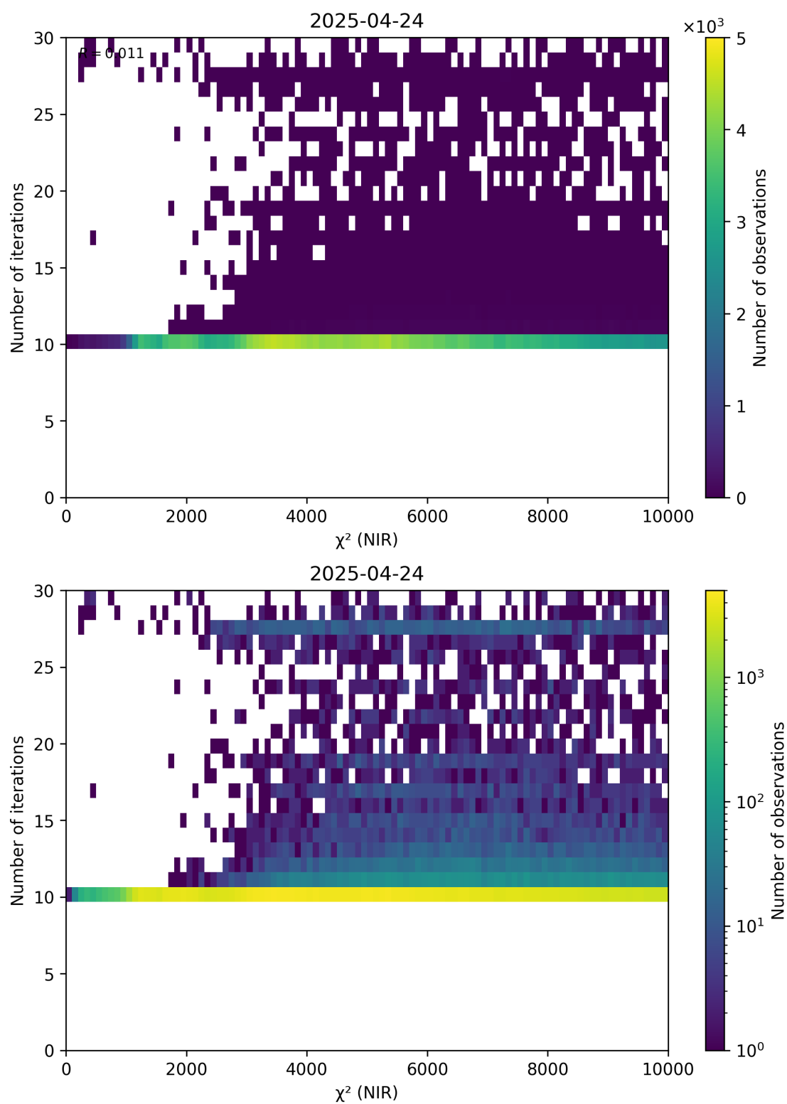
Figure 46: Scatter density plot of “ \chi^2 (NIR)” against “Number of iterations” for 2025-04-24 to 2025-04-25.
