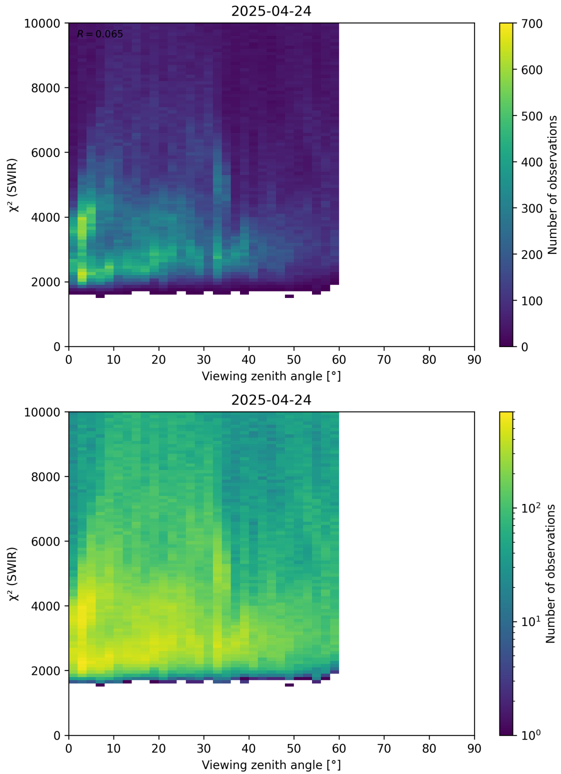
Figure 106: Scatter density plot of “Viewing zenith angle” against “ \chi^2 (SWIR)” for 2025-04-24 to 2025-04-25.
