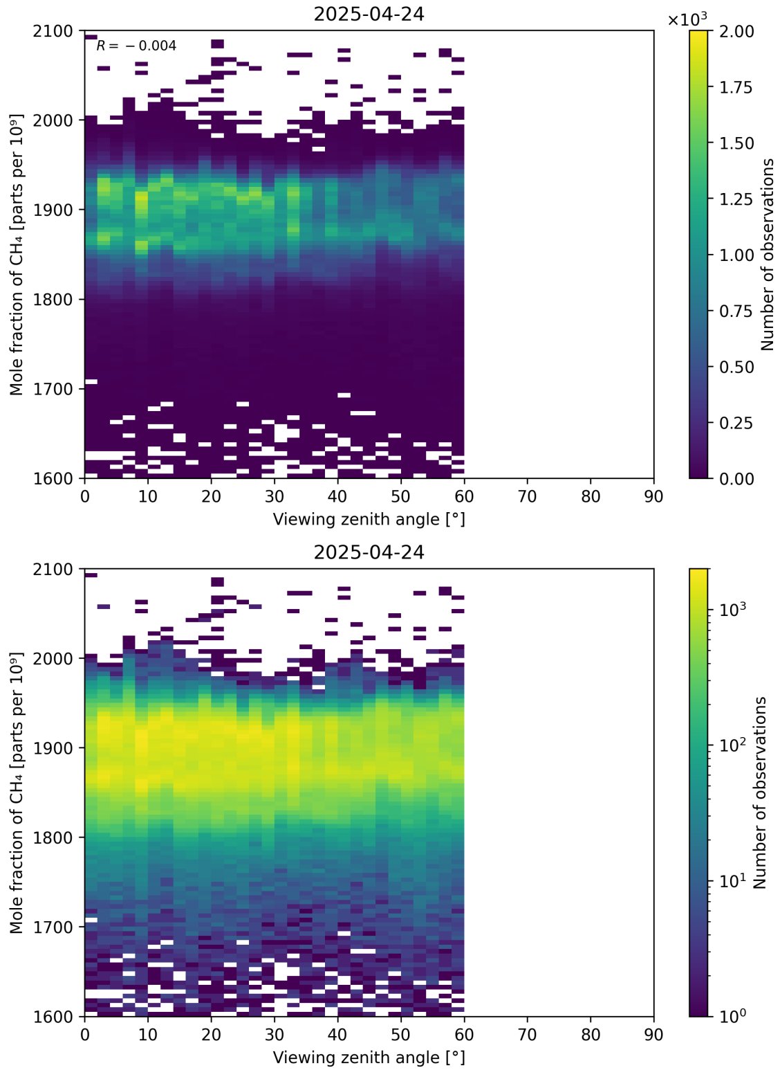
Figure 110: Scatter density plot of “Viewing zenith angle” against “Mole fraction of CH 4 ” for 2025-04-24 to 2025-04-25.
