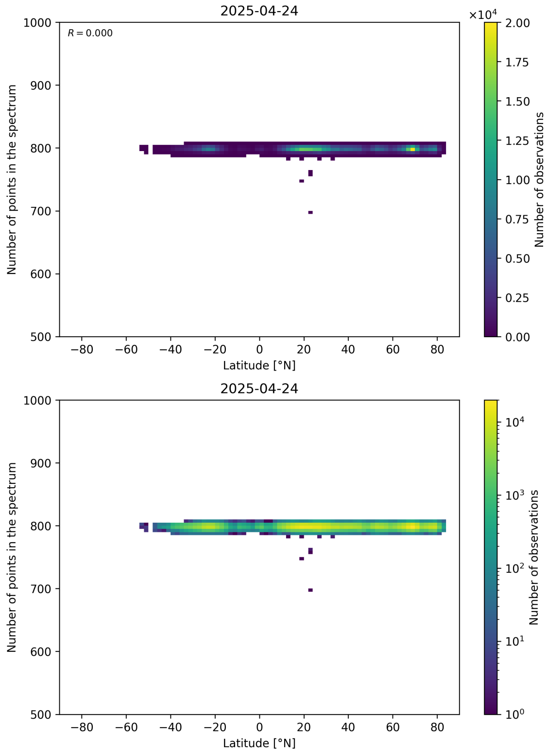
Figure 61: Scatter density plot of “Latitude” against “Number of points in the spectrum” for 2025-04-24 to 2025-04-25.
