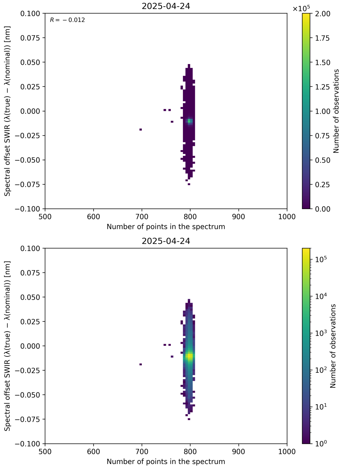
Figure 93: Scatter density plot of “Number of points in the spectrum” against “Spectral offset SWIR ( \lambda_{\text{true}} - \lambda_{\text{nominal}} )” for 2025-04-24 to 2025-04-25.
