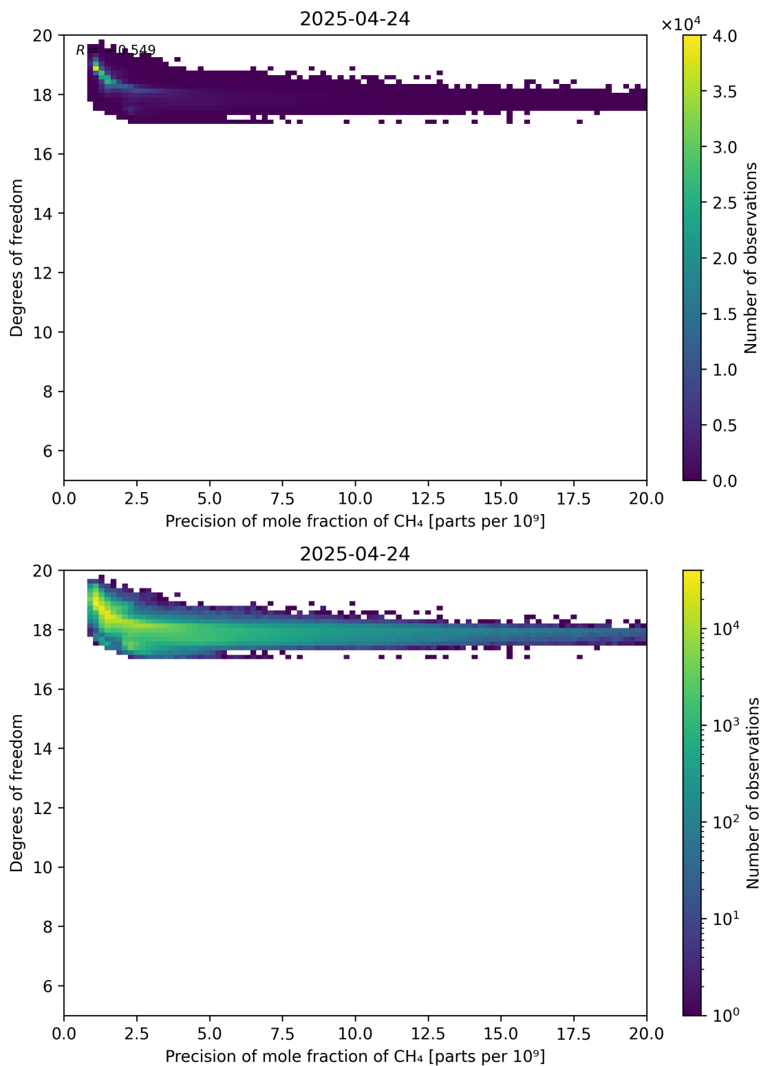
Figure 80: Scatter density plot of “Precision of mole fraction of CH 4 ” against “Degrees of freedom” for 2025-04-24 to 2025-04-25.
