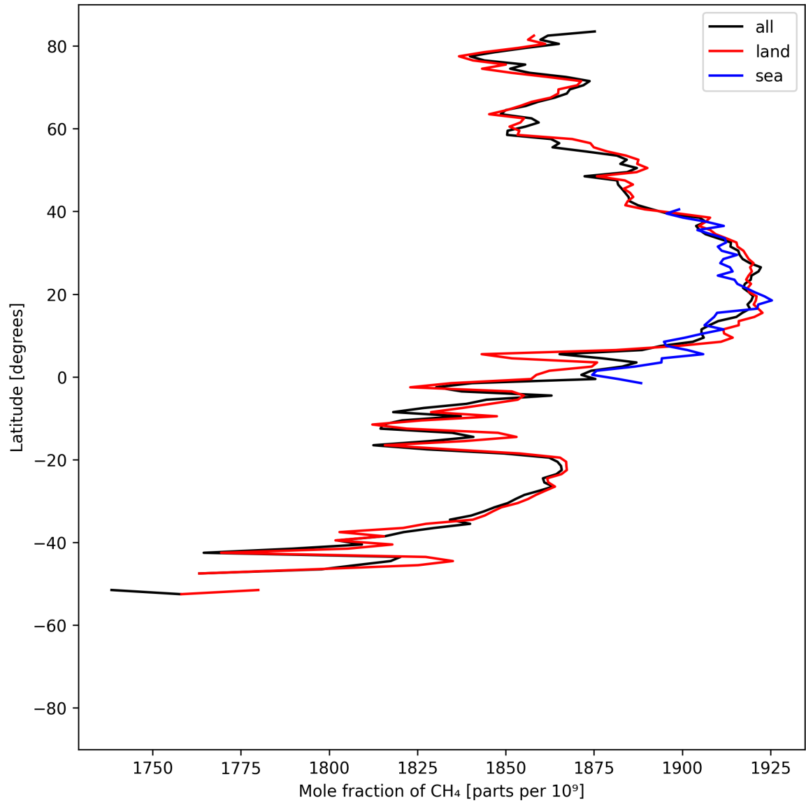
Figure 12: Zonal average of “Mole fraction of \text{CH}_4 ” for 2025-04-24 to 2025-04-25.
