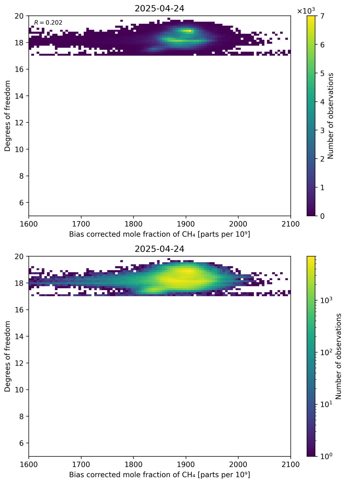
Figure 65: Scatter density plot of “Bias corrected mole fraction of CH 4 ” against “Degrees of freedom” for 2025-04-24 to 2025-04-25.
