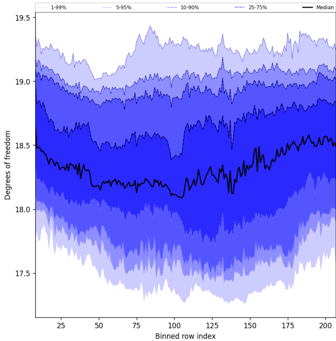
Figure 41: Along track statistics of “Degrees of freedom” for 2025-04-24 to 2025-04-25
