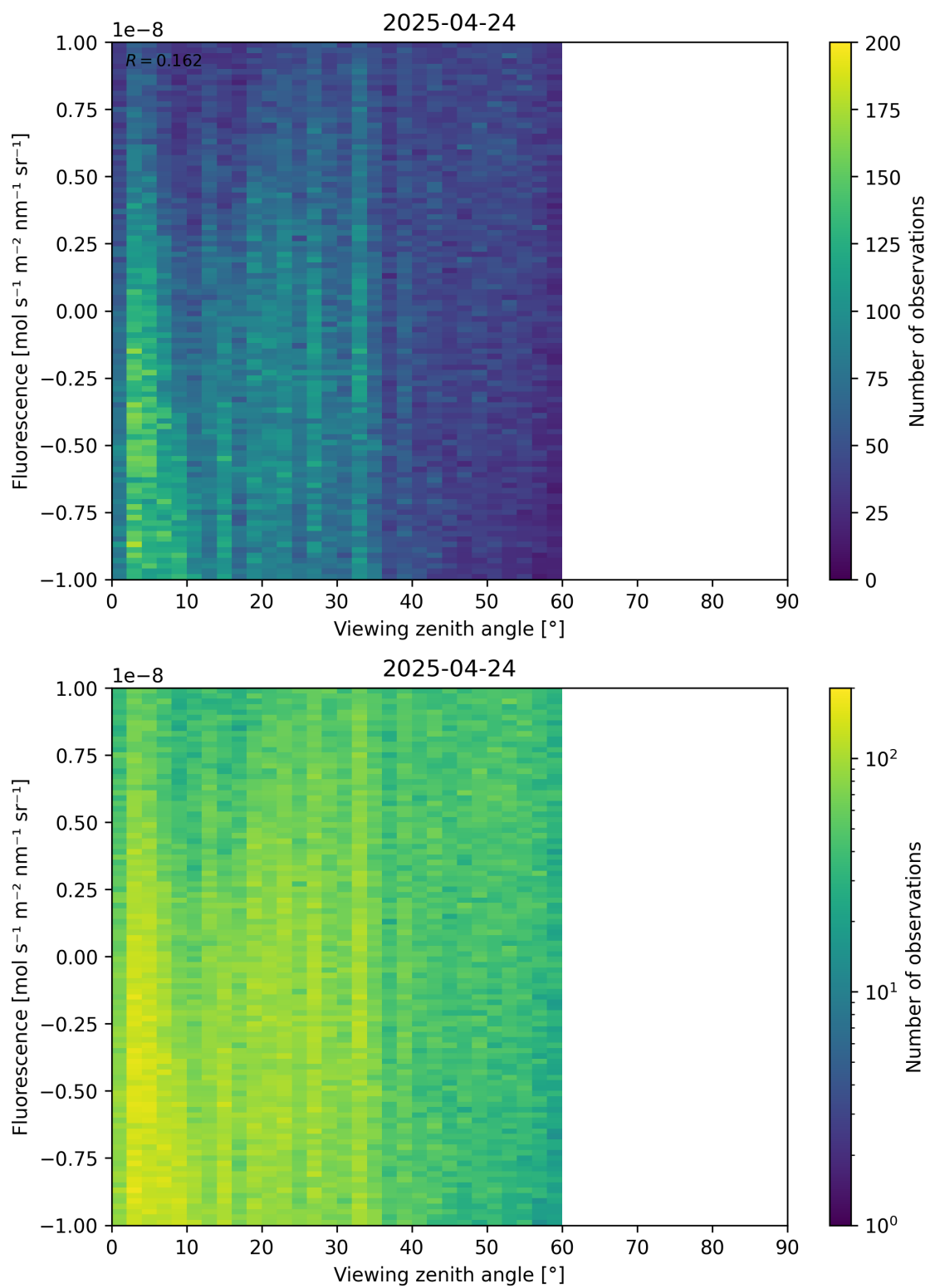
Figure 108: Scatter density plot of “Viewing zenith angle” against “Fluorescence” for 2025-04-24 to 2025-04-25.
