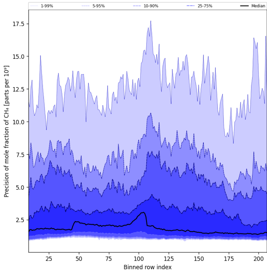
Figure 35: Along track statistics of “Precision of mole fraction of CH 4 ” for 2025-04-24 to 2025-04-25
