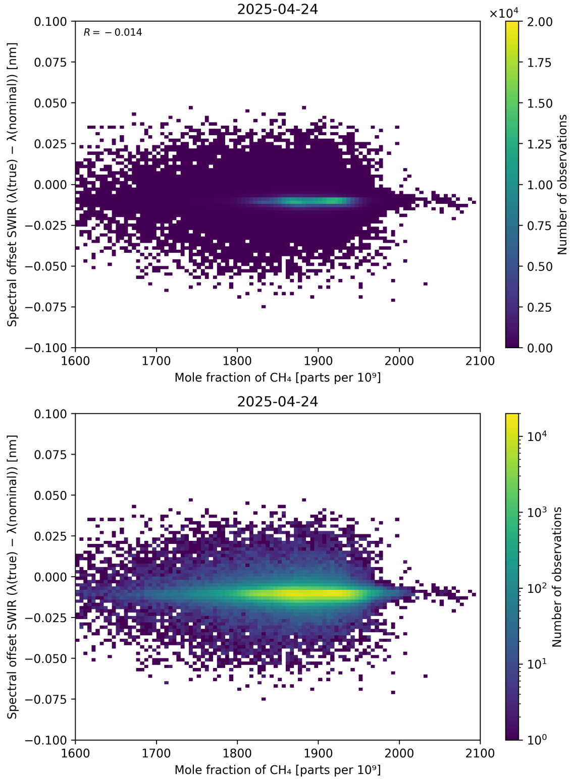
Figure 86: Scatter density plot of “Mole fraction of \text{CH}_4 ” against “Spectral offset SWIR ( \lambda_{\text{true}} - \lambda_{\text{nominal}} )” for 2025-04-24 to 2025-04-25.
