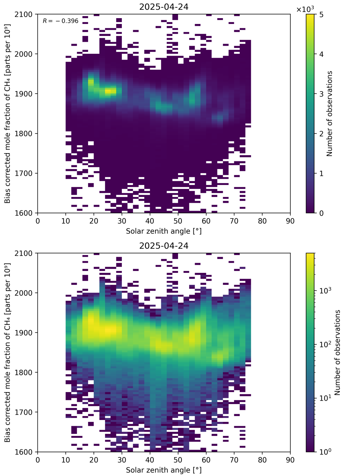
Figure 100: Scatter density plot of “Solar zenith angle” against “Bias corrected mole fraction of \text{CH}_4 ” for 2025-04-24 to 2025-04-25.
