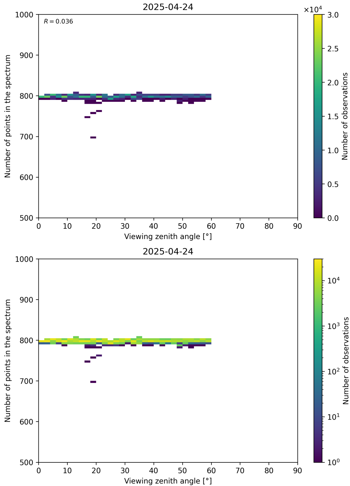
Figure 114: Scatter density plot of “Viewing zenith angle” against “Number of points in the spectrum” for 2025-04-24 to 2025-04-25.
