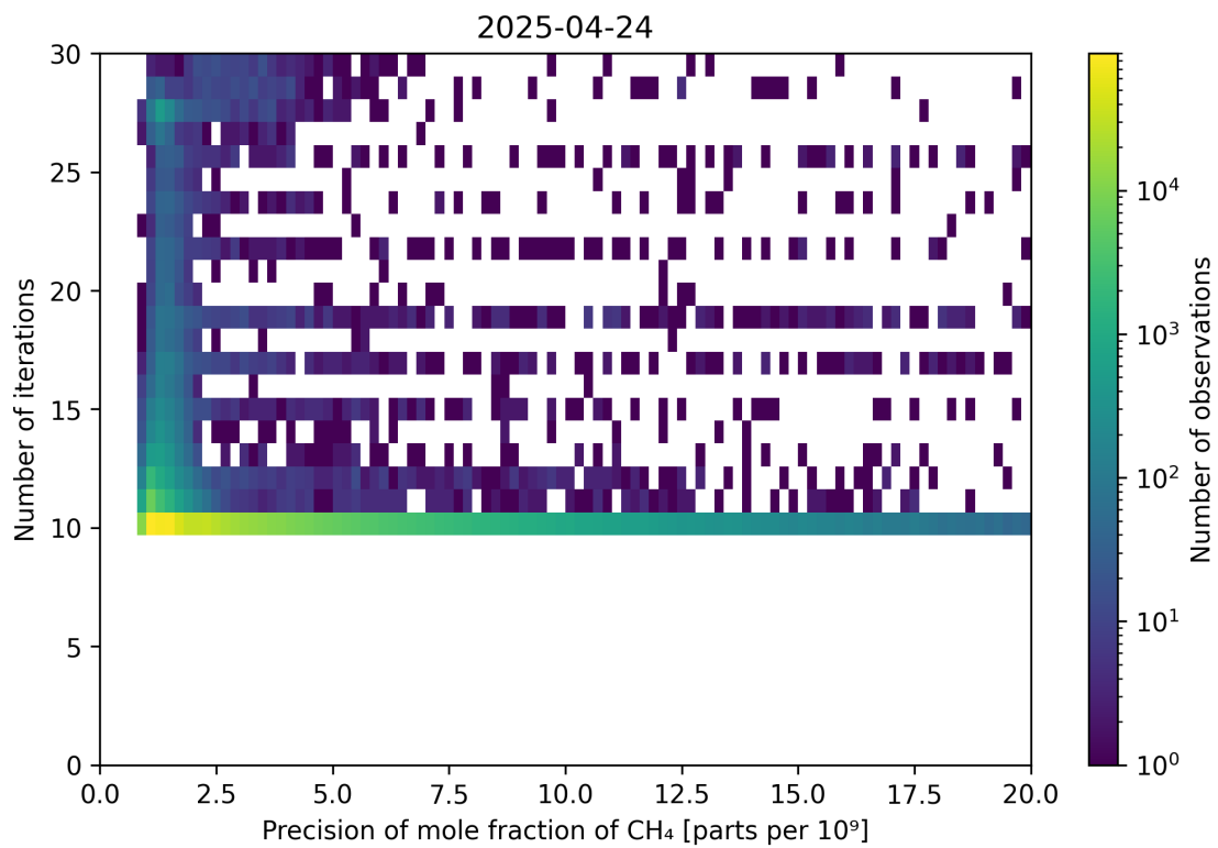
Figure 83: Scatter density plot of “Precision of mole fraction of \text{CH}_4 ” against “Number of iterations” for 2025-04-24 to 2025-04-25.
