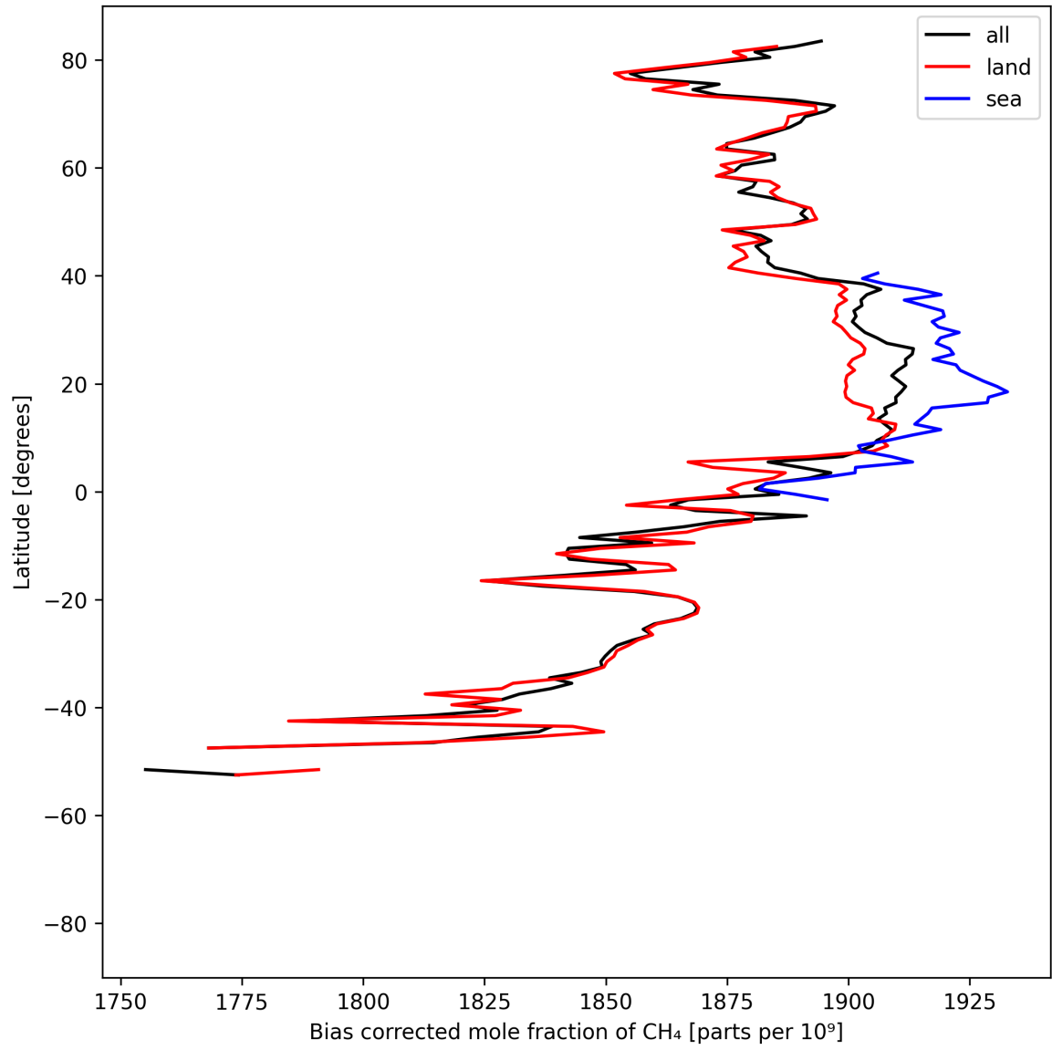
Figure 14: Zonal average of “Bias corrected mole fraction of CH 4 ” for 2025-04-24 to 2025-04-25.
