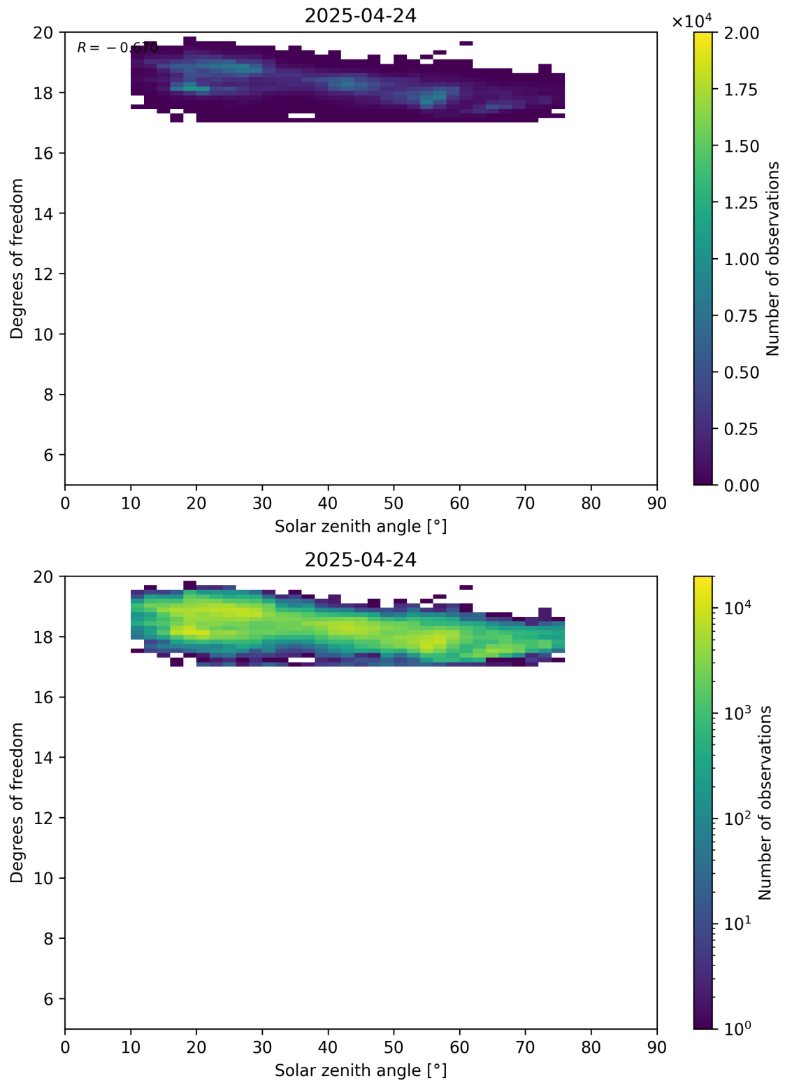
Figure 96: Scatter density plot of “Solar zenith angle” against “Degrees of freedom” for 2025-04-24 to 2025-04-25.
