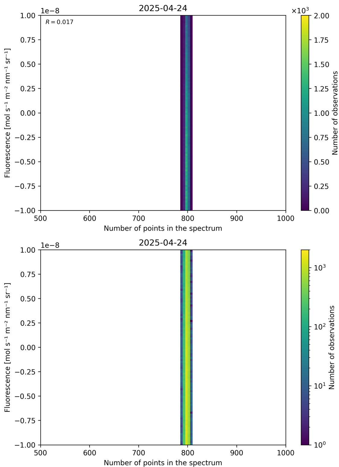
Figure 91: Scatter density plot of “Number of points in the spectrum” against “Fluorescence” for 2025-04-24 to 2025-04-25.
