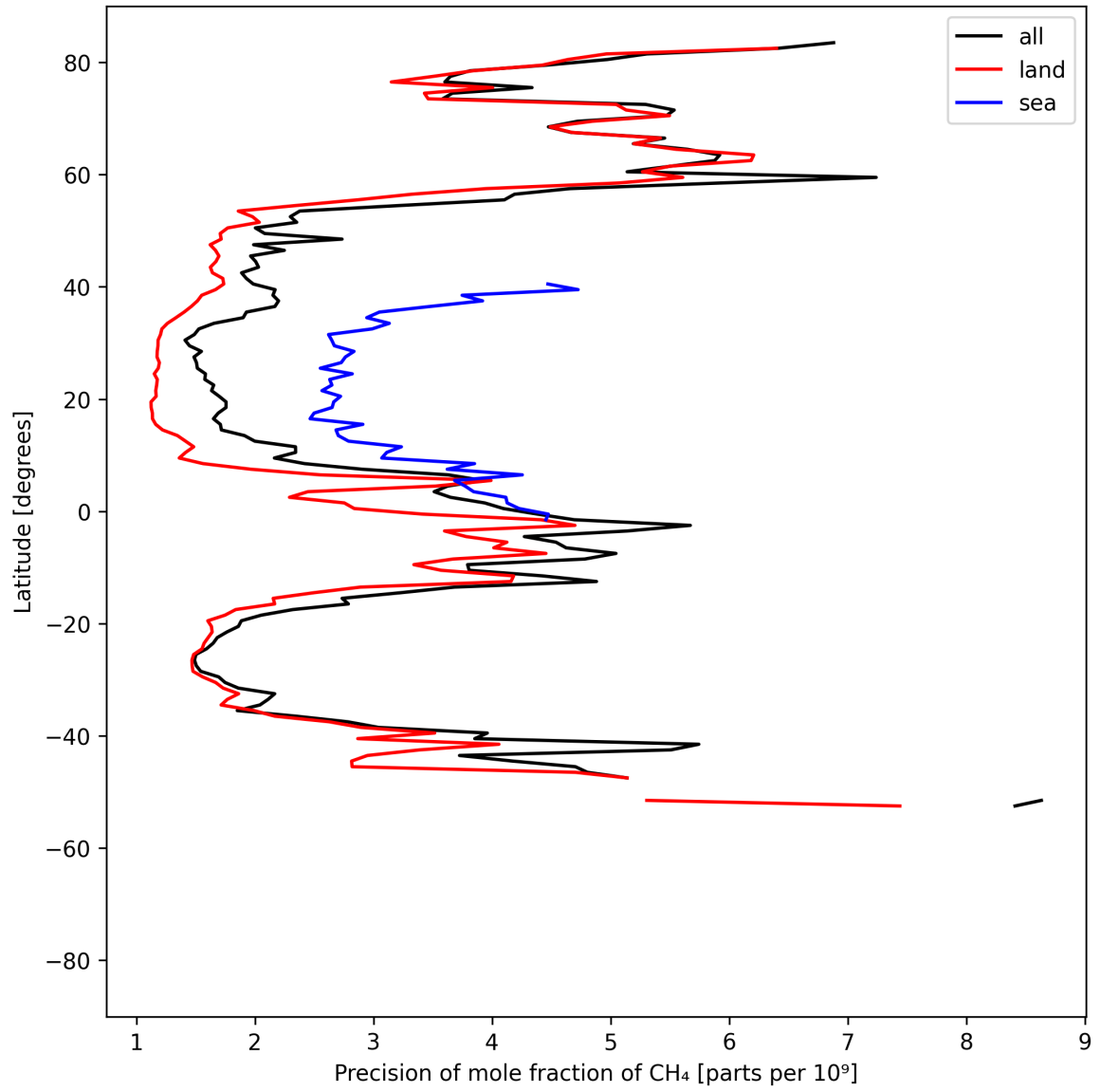
Figure 13: Zonal average of “Precision of mole fraction of CH 4 ” for 2025-04-24 to 2025-04-25.
