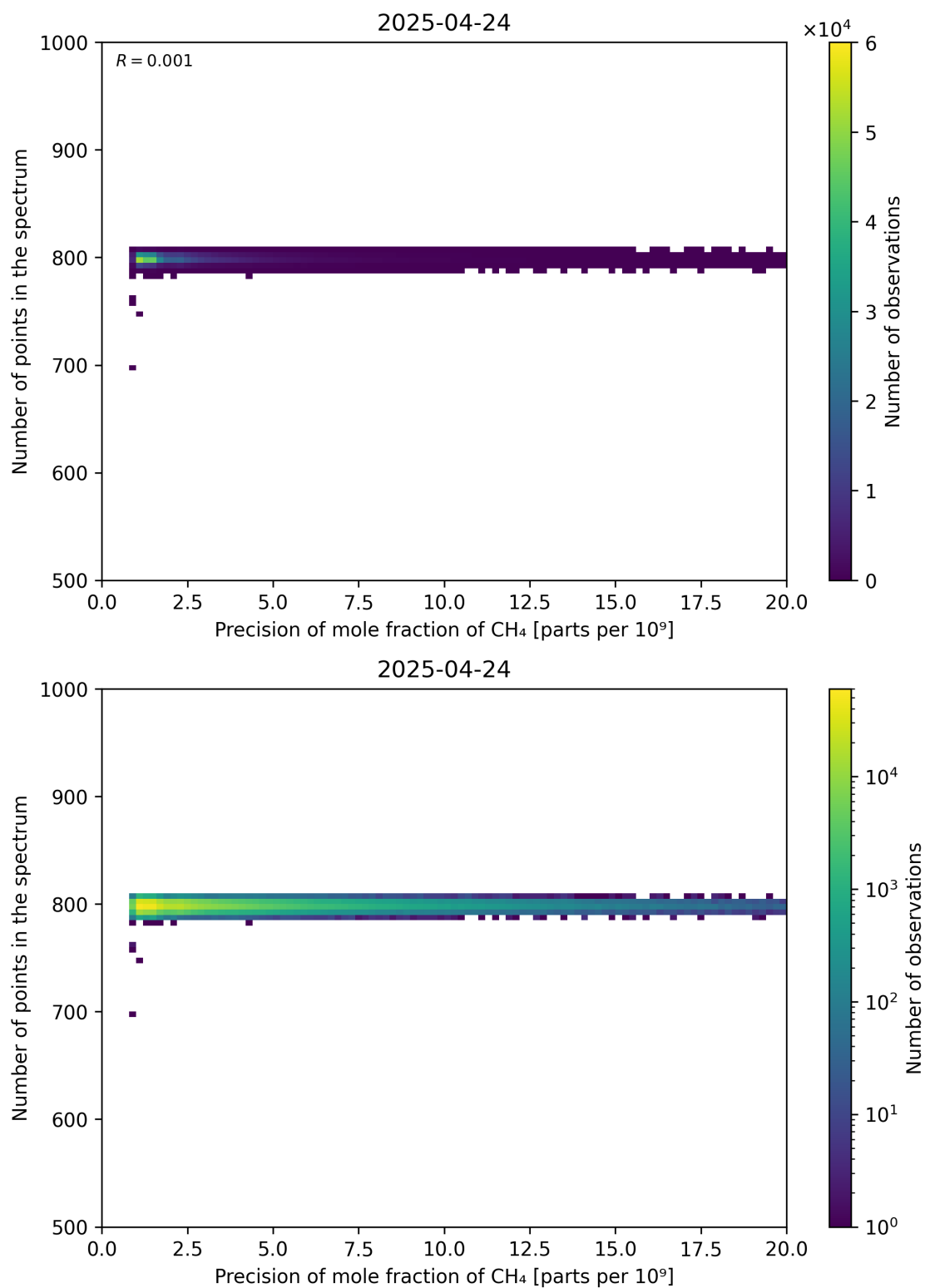
Figure 84: Scatter density plot of “Precision of mole fraction of CH 4 ” against “Number of points in the spectrum” for 2025-04-24 to 2025-04-25.
