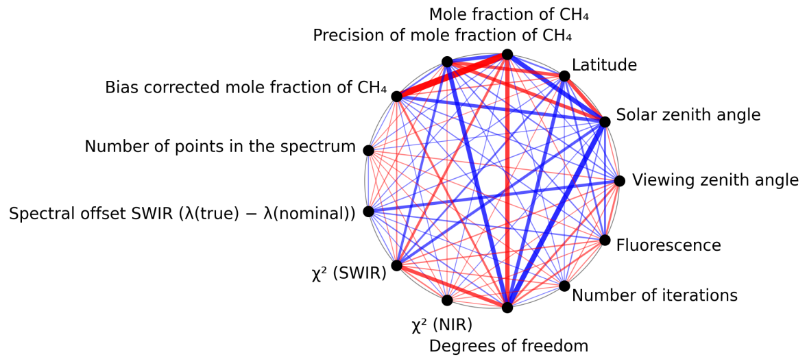
Figure 1: Map of correlation graph for 2025-04-24 to 2025-04-25.
