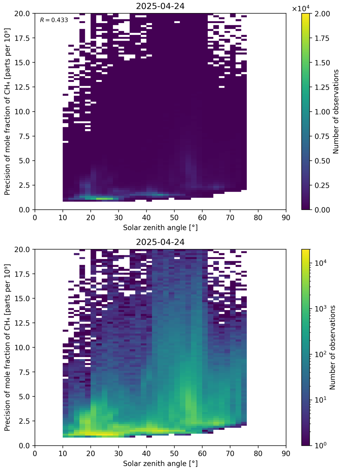
Figure 101: Scatter density plot of “Solar zenith angle” against “Precision of mole fraction of CH 4 ” for 2025-04-24 to 2025-04-25.
