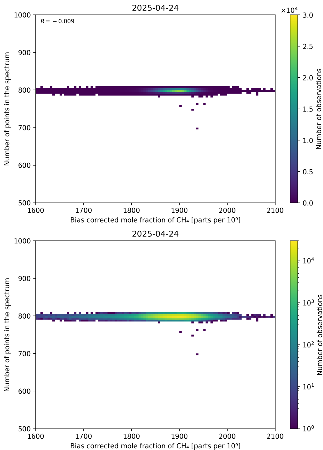
Figure 68: Scatter density plot of “Bias corrected mole fraction of CH 4 ” against “Number of points in the spectrum” for 2025-04-24 to 2025-04-25.
