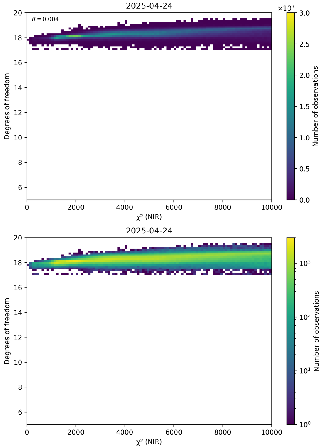
Figure 44: Scatter density plot of “ \chi^2 (NIR)” against “Degrees of freedom” for 2025-04-24 to 2025-04-25.
