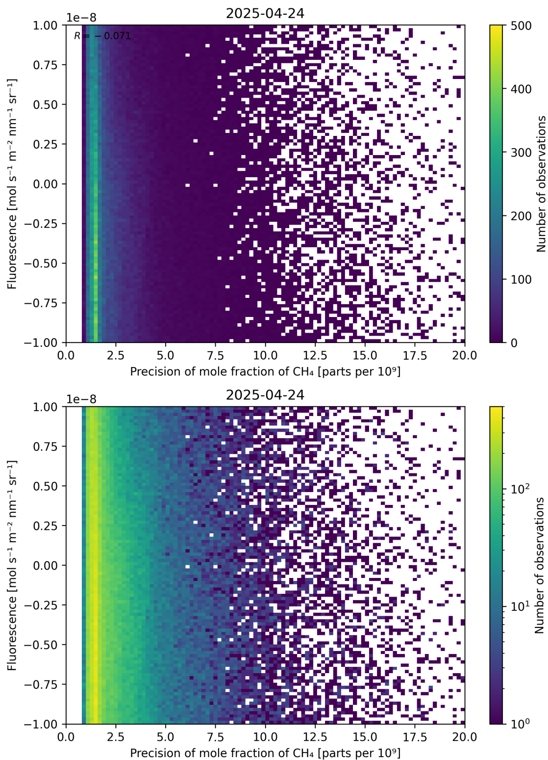
Figure 81: Scatter density plot of “Precision of mole fraction of \text{CH}_4 ” against “Fluorescence” for 2025-04-24 to 2025-04-25.
