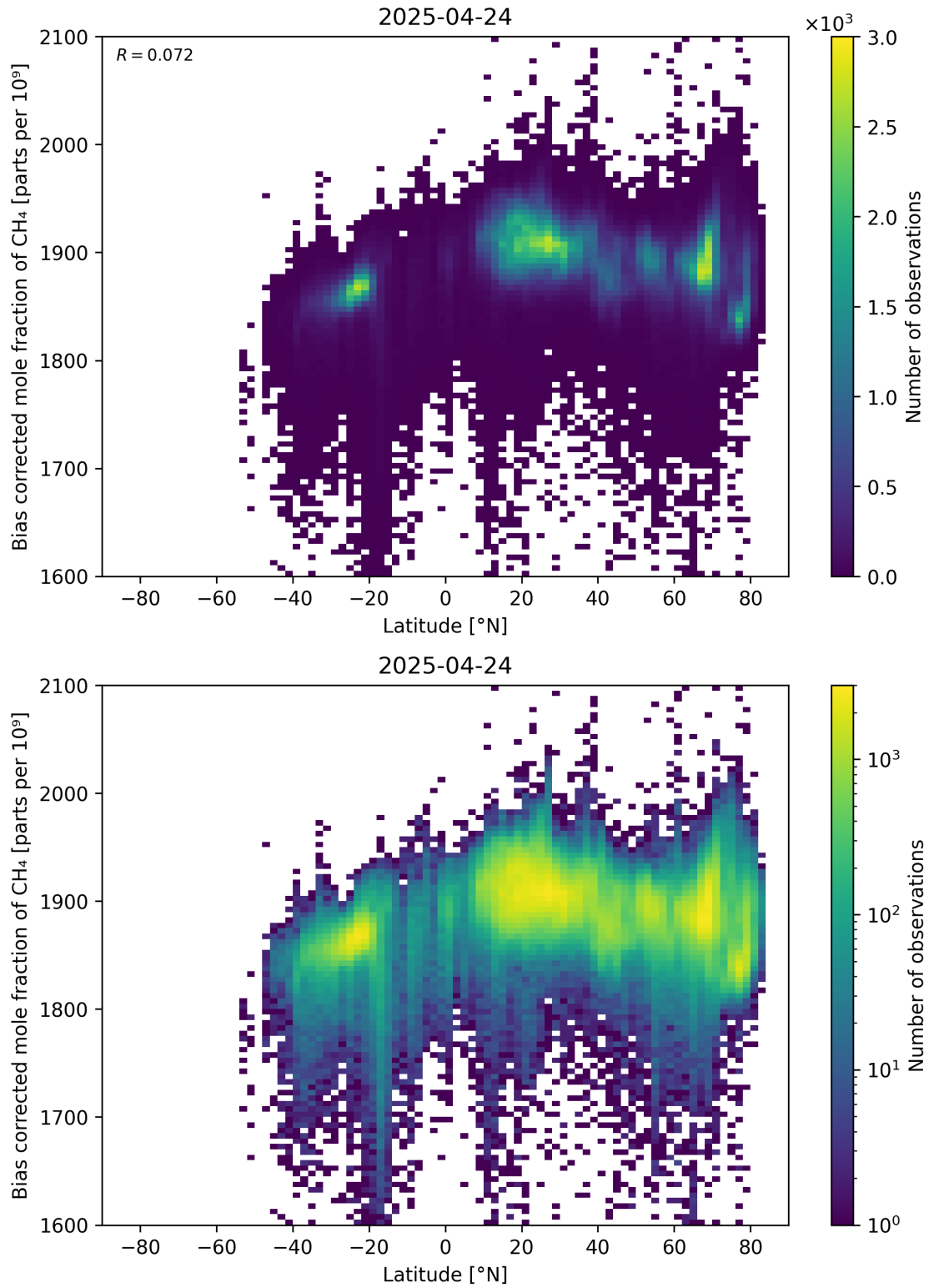
Figure 58: Scatter density plot of “Latitude” against “Bias corrected mole fraction of \text{CH}_4 ” for 2025-04-24 to 2025-04-25.
