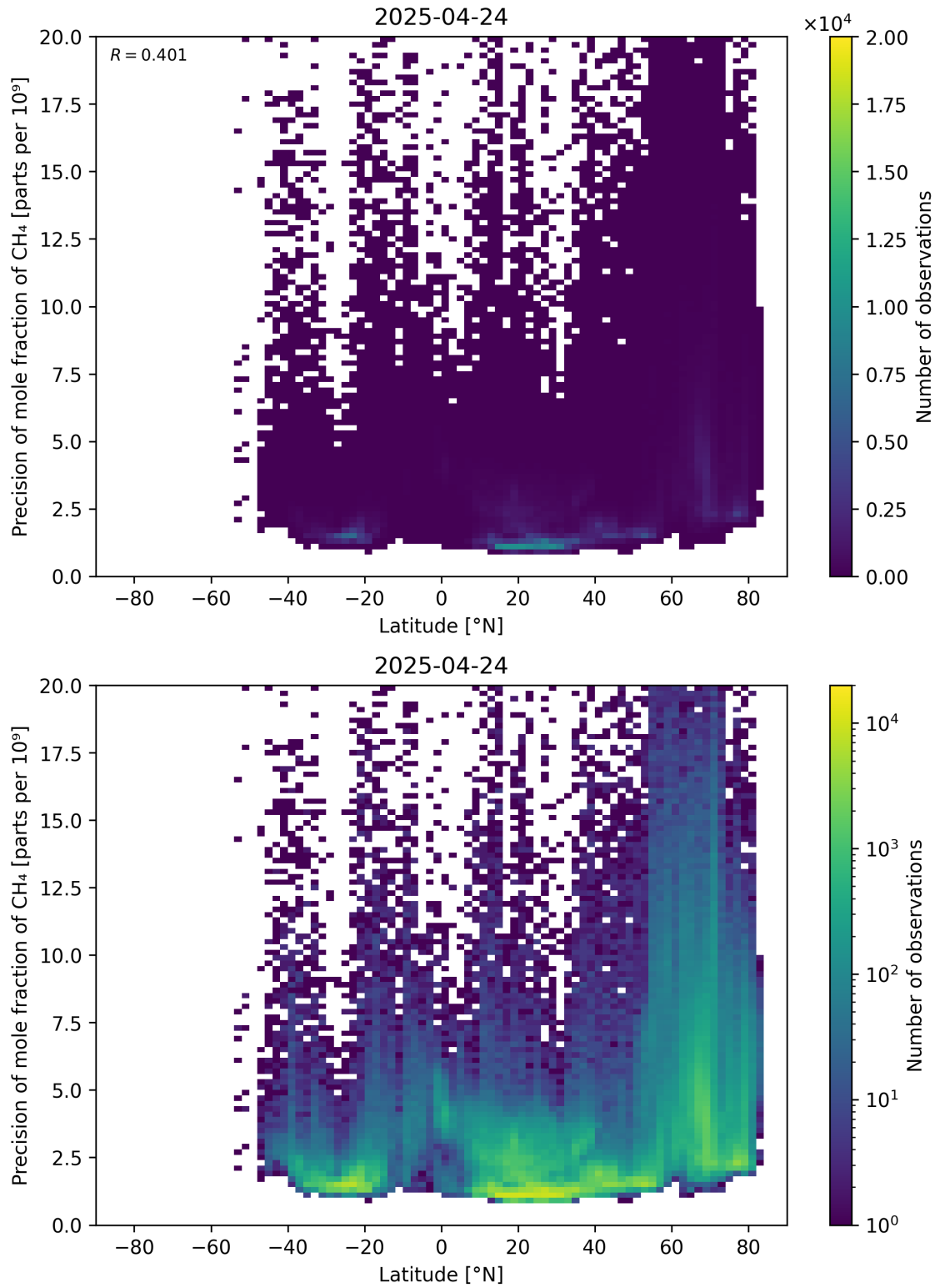
Figure 59: Scatter density plot of “Latitude” against “Precision of mole fraction of \text{CH}_4 ” for 2025-04-24 to 2025-04-25.
