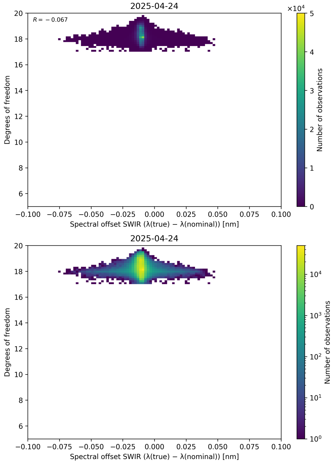
Figure 119: Scatter density plot of “Spectral offset SWIR ( \lambda_{\text{true}} - \lambda_{\text{nominal}} )” against “Degrees of freedom” for 2025-04-24 to 2025-04-25.
