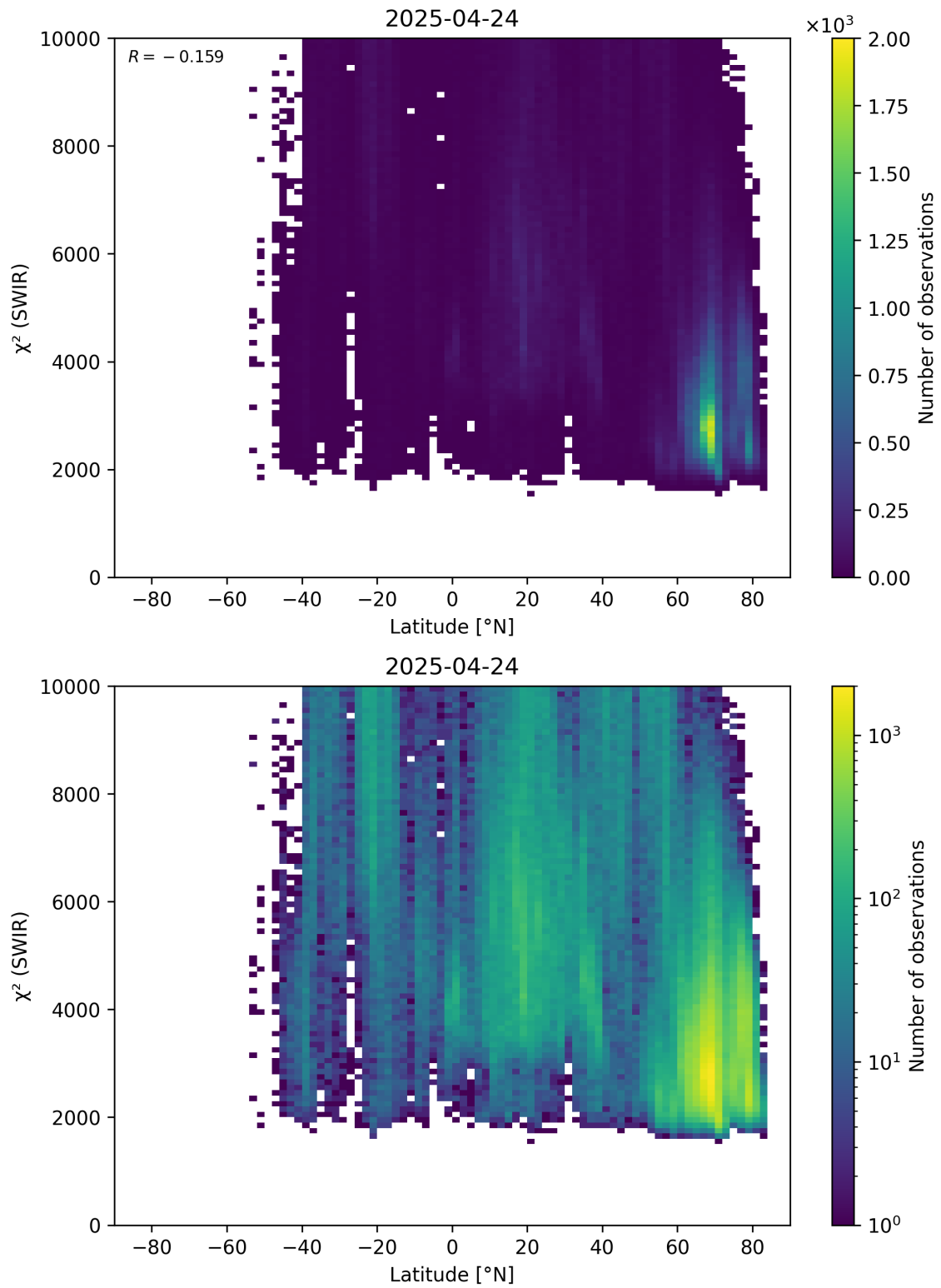
Figure 54: Scatter density plot of “Latitude” against “ \chi^2 (SWIR)” for 2025-04-24 to 2025-04-25.
