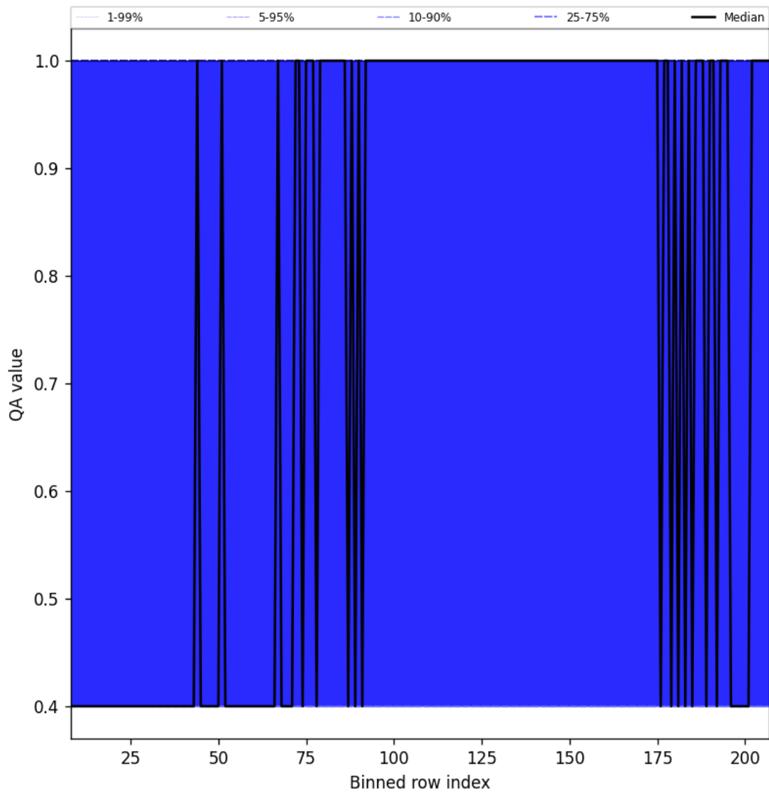
Figure 33: Along track statistics of “QA value” for 2025-04-24 to 2025-04-25
