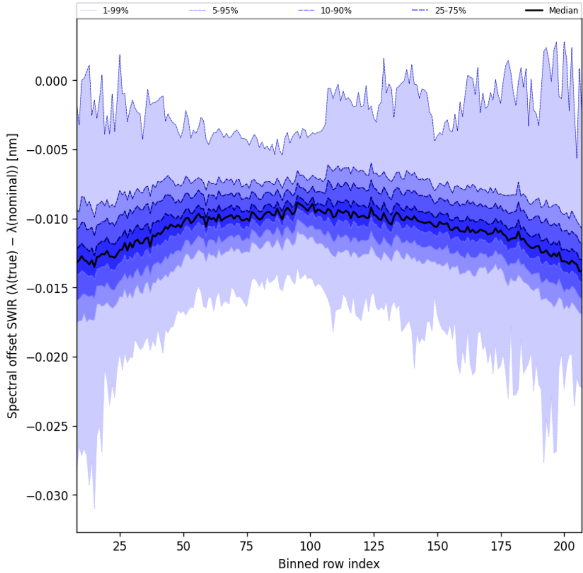
Figure 38: Along track statistics of “Spectral offset SWIR ( \lambda_{\text{true}} - \lambda_{\text{nominal}} )” for 2025-04-24 to 2025-04-25
