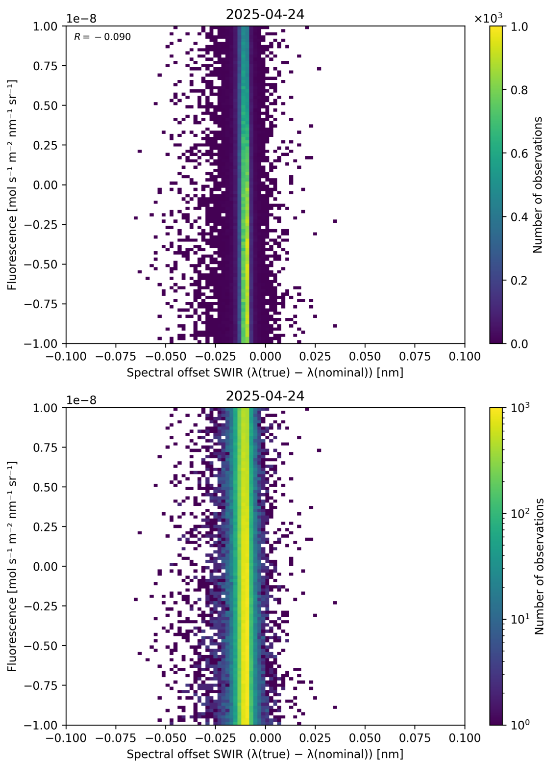
Figure 120: Scatter density plot of “Spectral offset SWIR ( \lambda_{\text{true}} - \lambda_{\text{nominal}} )” against “Fluorescence” for 2025-04-24 to 2025-04-25.
