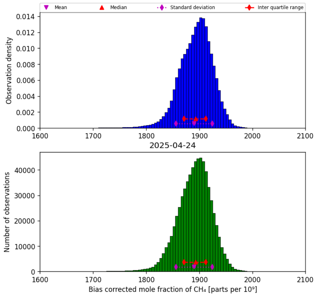
Figure 25: Histogram of “Bias corrected mole fraction of CH 4 ” for 2025-04-24 to 2025-04-25
