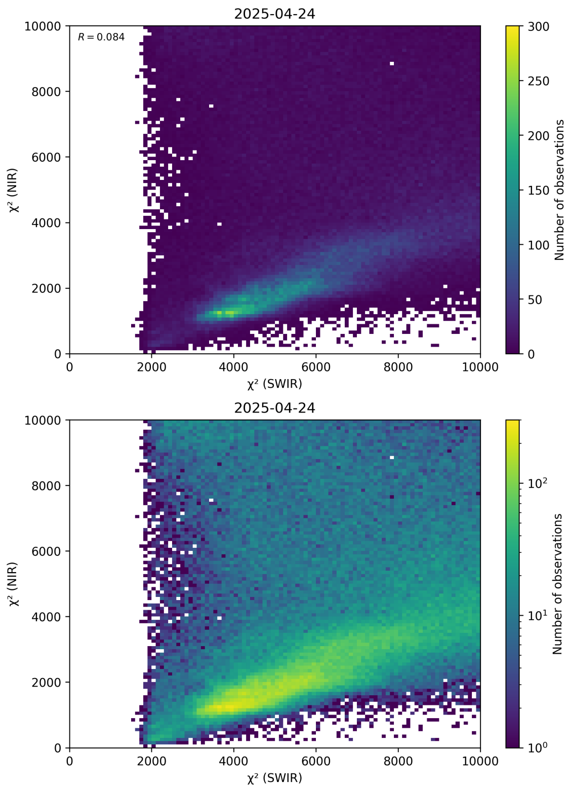
Figure 47: Scatter density plot of “ \chi^2 (SWIR)” against “ \chi^2 (NIR)” for 2025-04-24 to 2025-04-25.
