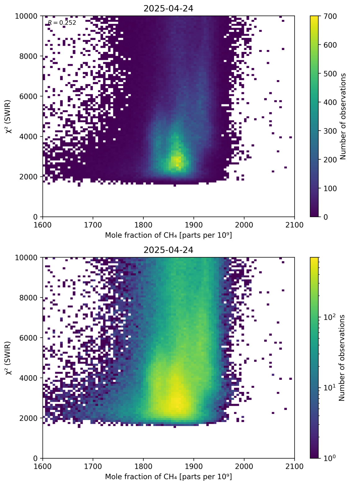
Figure 71: Scatter density plot of “Mole fraction of \text{CH}_4 ” against “ \chi^2 (SWIR)” for 2025-04-24 to 2025-04-25.
