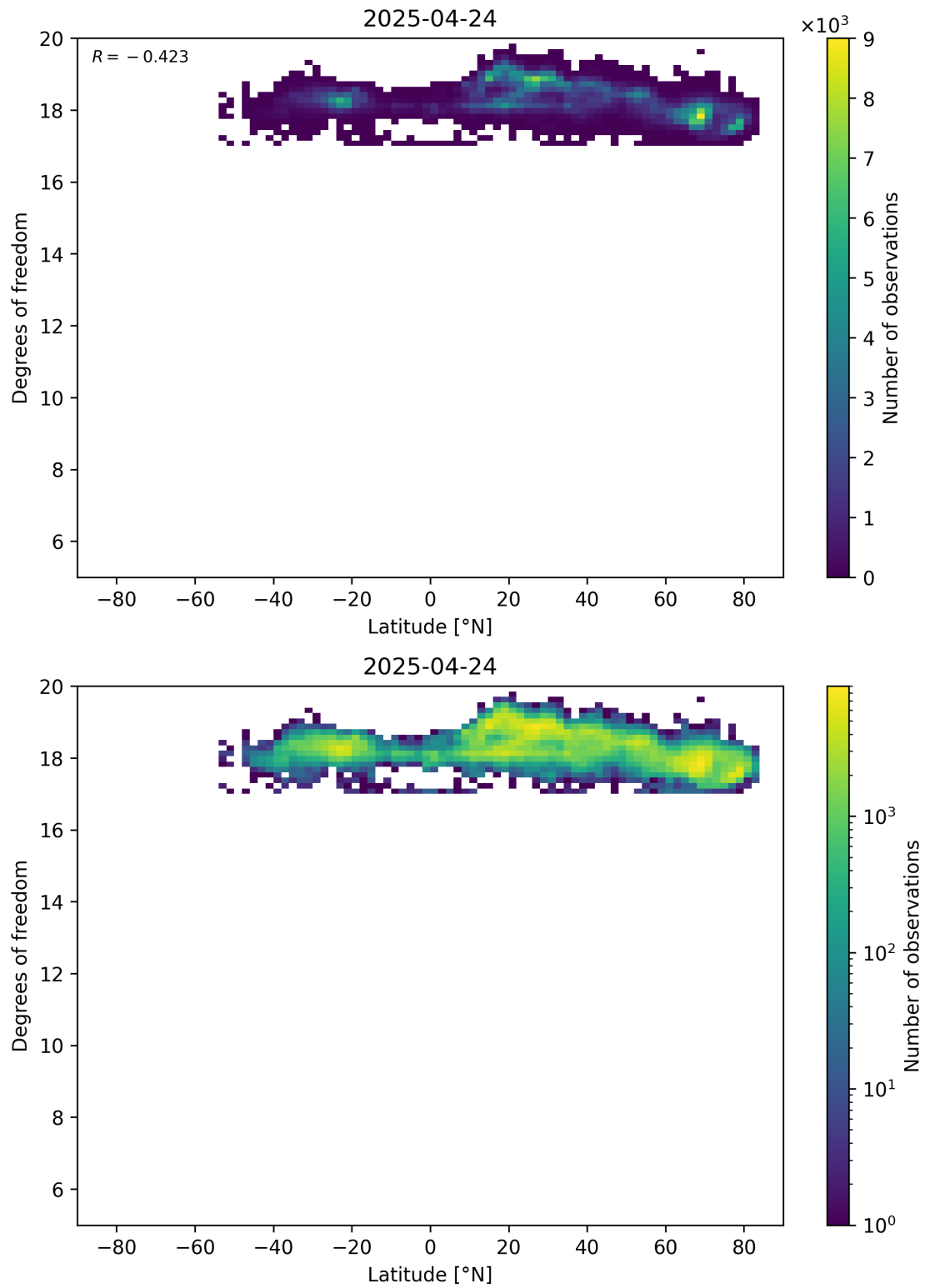
Figure 55: Scatter density plot of “Latitude” against “Degrees of freedom” for 2025-04-24 to 2025-04-25.
