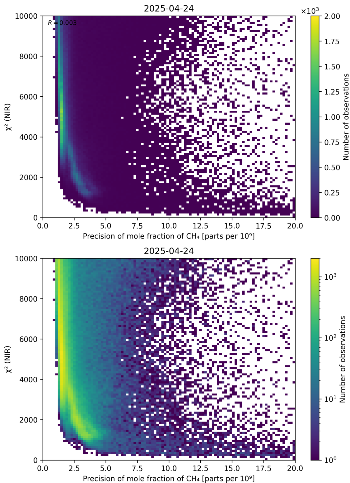
Figure 78: Scatter density plot of “Precision of mole fraction of CH 4 ” against “ \chi^2 (NIR)” for 2025-04-24 to 2025-04-25.
