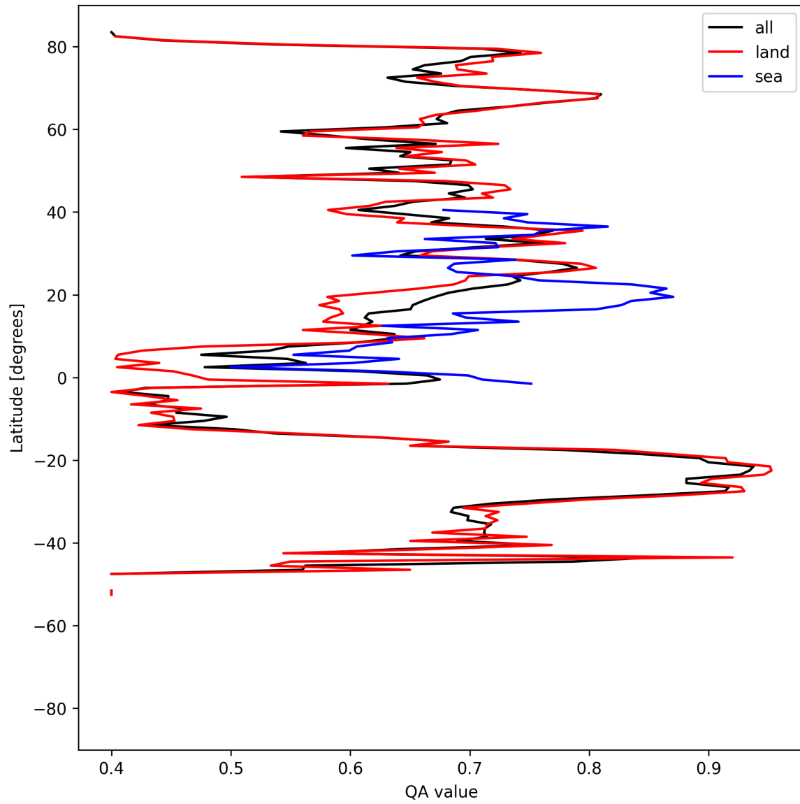
Figure 11: Zonal average of “QA value” for 2025-04-24 to 2025-04-25.
