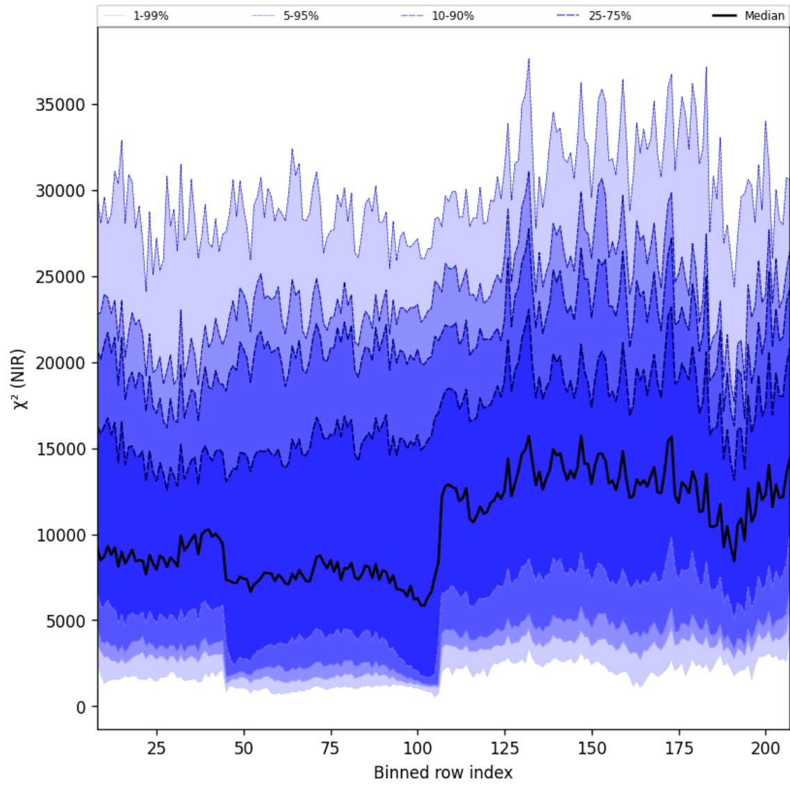
Figure 40: Along track statistics of “ \chi^2 (NIR)” for 2025-04-24 to 2025-04-25
