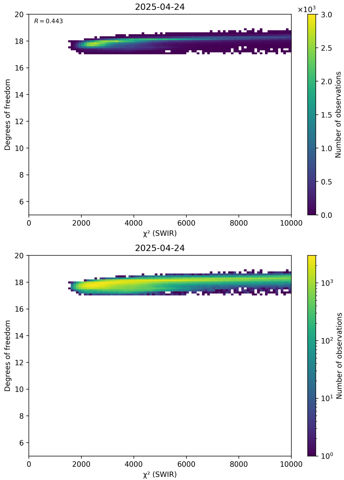
Figure 48: Scatter density plot of “ \chi^2 (SWIR)” against “Degrees of freedom” for 2025-04-24 to 2025-04-25.
