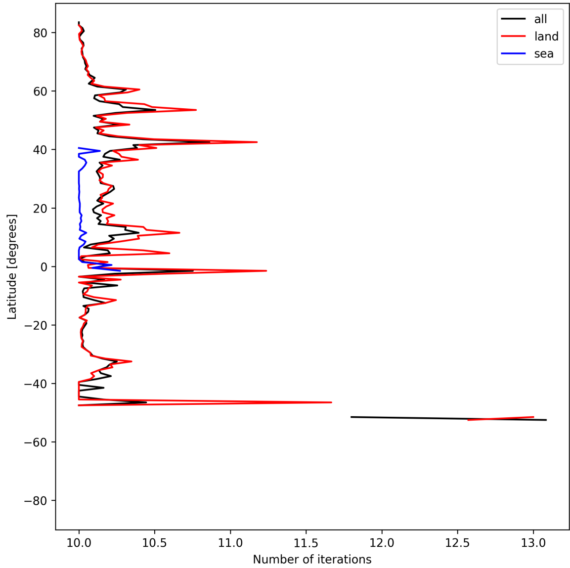
Figure 20: Zonal average of “Number of iterations” for 2025-04-24 to 2025-04-25.
