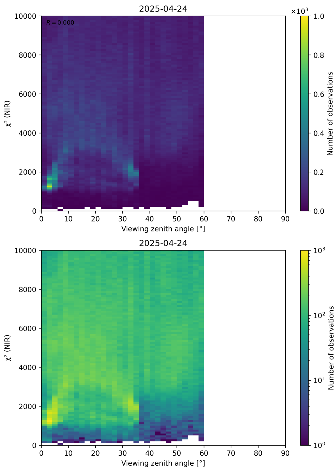
Figure 105: Scatter density plot of “Viewing zenith angle” against “ \chi^2 (NIR)” for 2025-04-24 to 2025-04-25.
