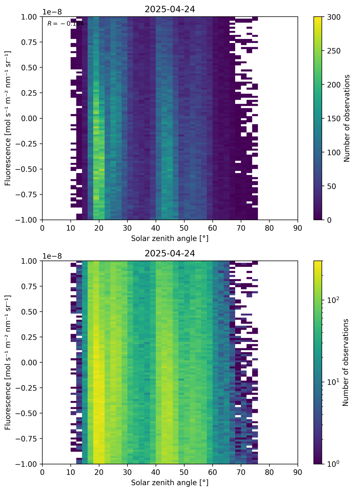
Figure 97: Scatter density plot of “Solar zenith angle” against “Fluorescence” for 2025-04-24 to 2025-04-25.
