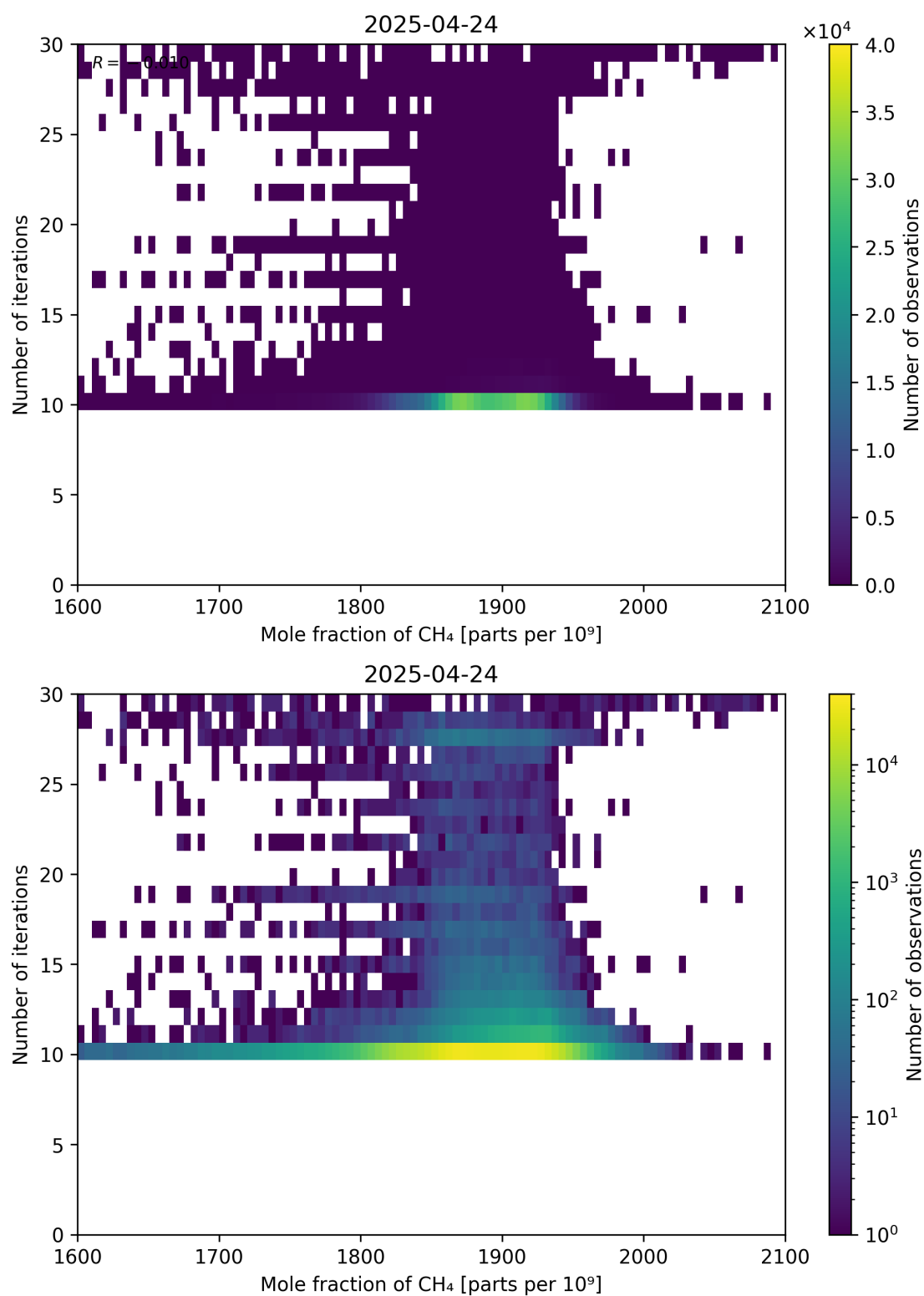
Figure 76: Scatter density plot of “Mole fraction of CH 4 ” against “Number of iterations” for 2025-04-24 to 2025-04-25.
