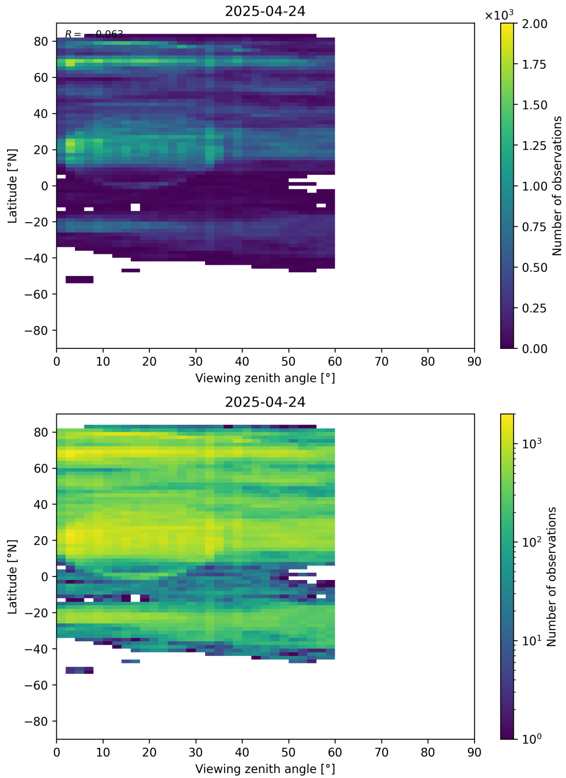
Figure 109: Scatter density plot of “Viewing zenith angle” against “Latitude” for 2025-04-24 to 2025-04-25.
