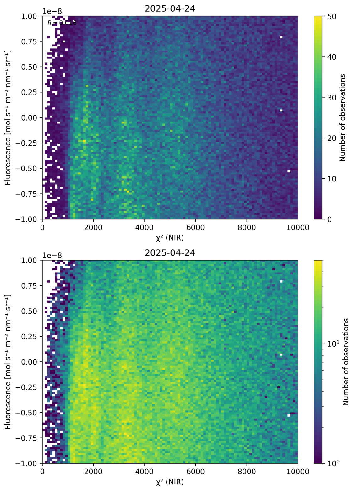
Figure 45: Scatter density plot of “ \chi^2 (NIR)” against “Fluorescence” for 2025-04-24 to 2025-04-25.
