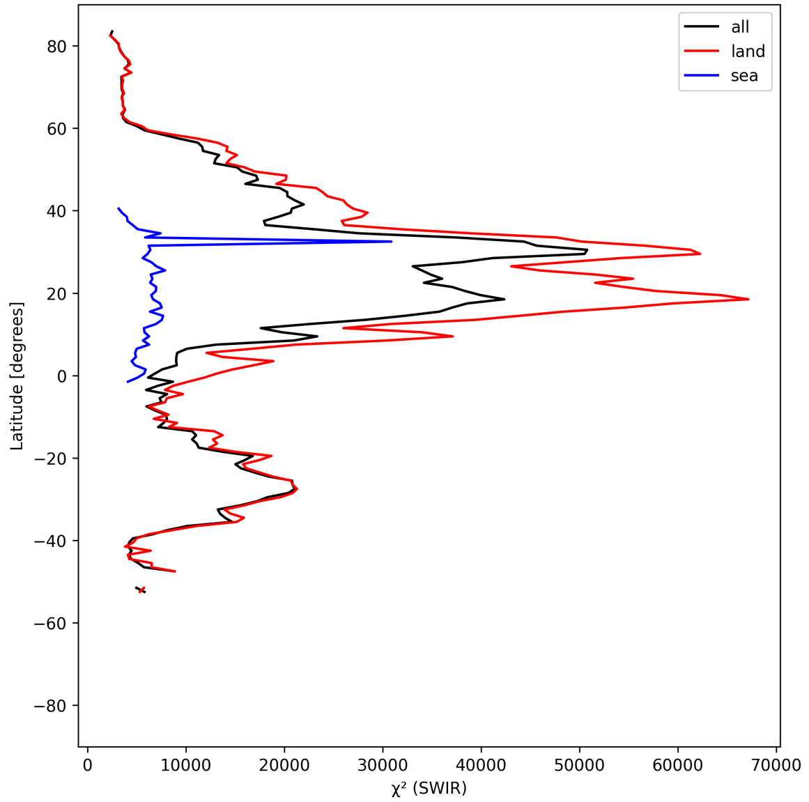
Figure 17: Zonal average of “ \chi^2 (SWIR)” for 2025-04-24 to 2025-04-25.
