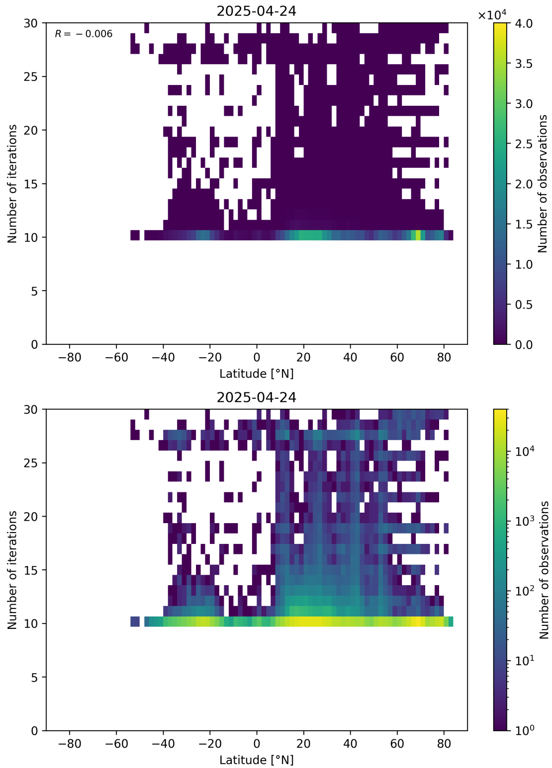
Figure 60: Scatter density plot of “Latitude” against “Number of iterations” for 2025-04-24 to 2025-04-25.
