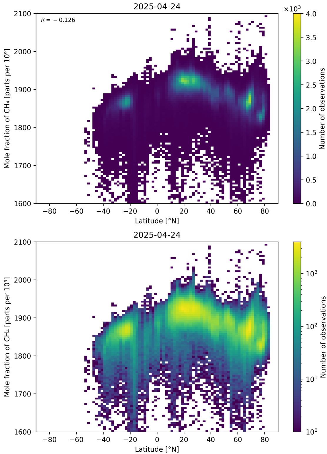
Figure 57: Scatter density plot of “Latitude” against “Mole fraction of CH 4 ” for 2025-04-24 to 2025-04-25.
