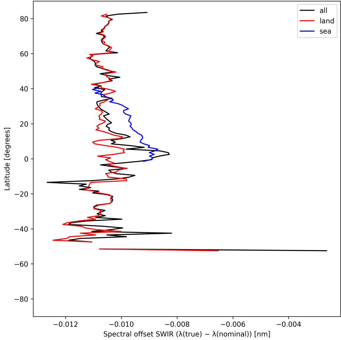
Figure 16: Zonal average of “Spectral offset SWIR ( \lambda_{\text{true}} - \lambda_{\text{nominal}} )” for 2025-04-24 to 2025-04-25.
