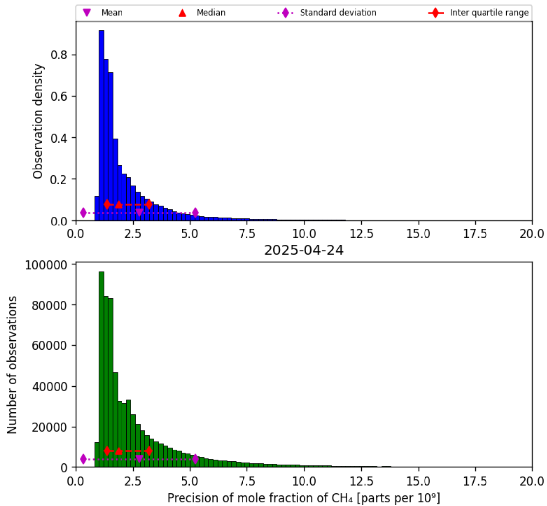
Figure 24: Histogram of “Precision of mole fraction of CH 4 ” for 2025-04-24 to 2025-04-25
