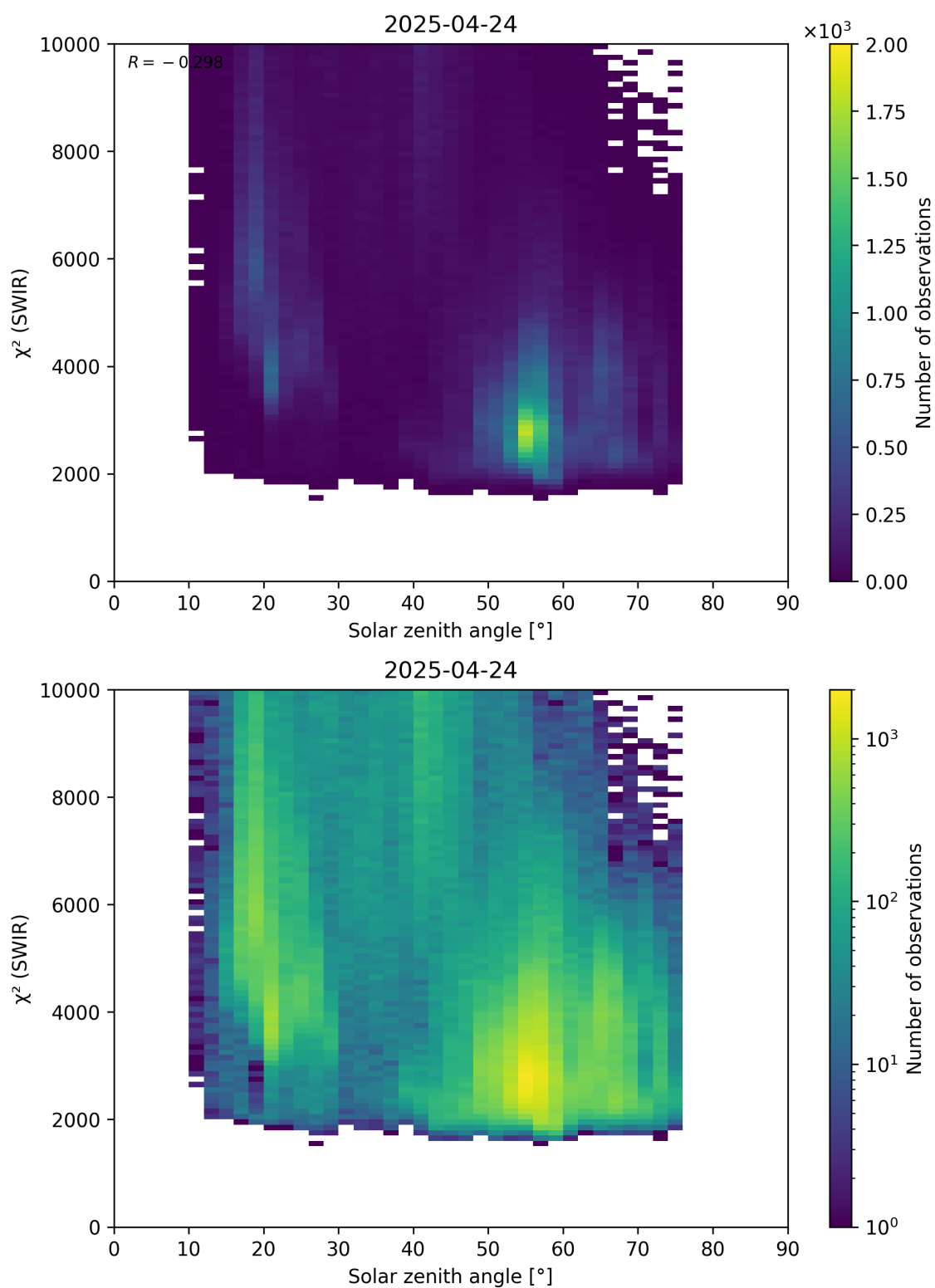
Figure 95: Scatter density plot of “Solar zenith angle” against “ \chi^2 (SWIR)” for 2025-04-24 to 2025-04-25.
