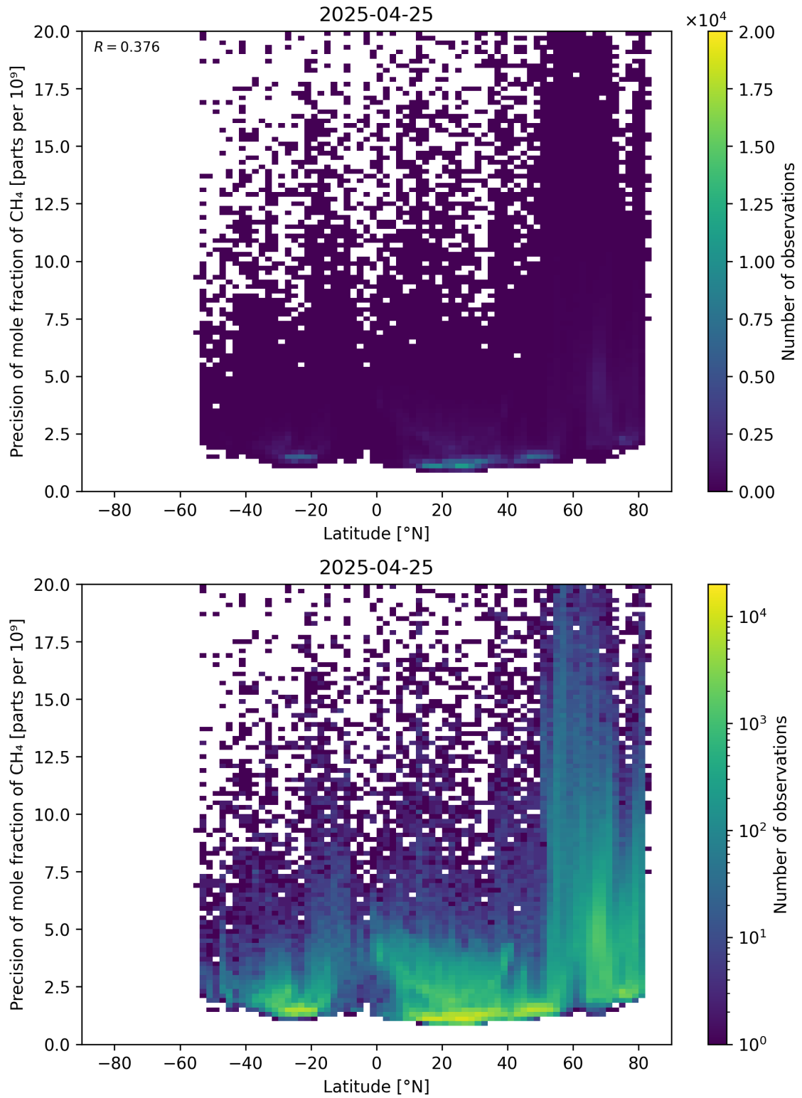
Figure 59: Scatter density plot of “Latitude” against “Precision of mole fraction of \text{CH}_4 ” for 2025-04-24 to 2025-04-26.
