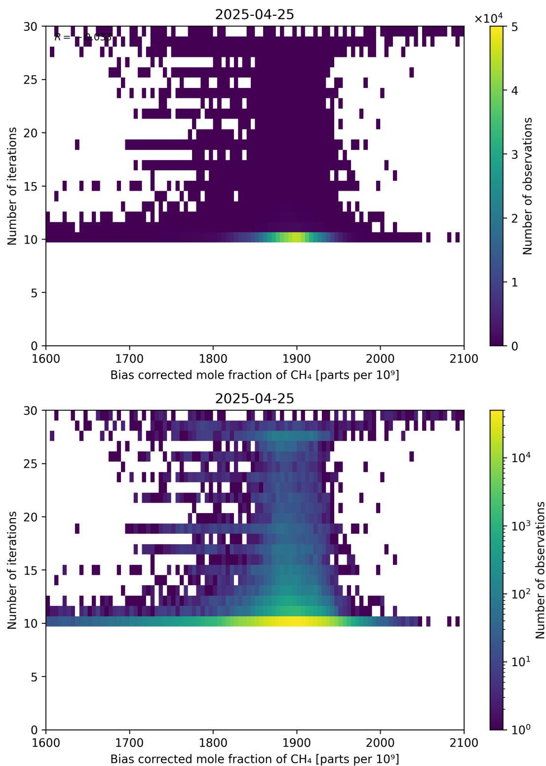
Figure 67: Scatter density plot of “Bias corrected mole fraction of \text{CH}_4 ” against “Number of iterations” for 2025-04-24 to 2025-04-26.
