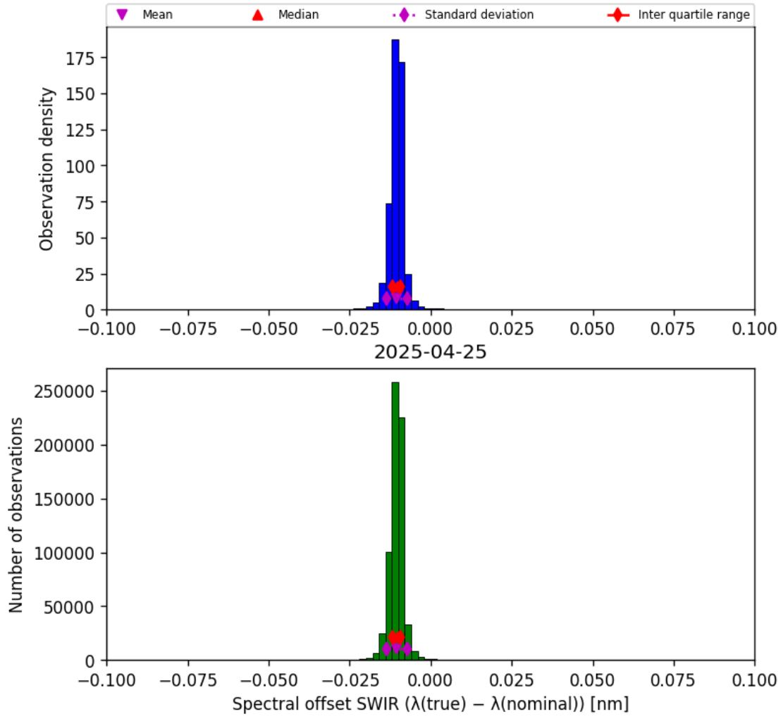
Figure 27: Histogram of “Spectral offset SWIR ( \lambda_{\text{true}} - \lambda_{\text{nominal}} )” for 2025-04-24 to 2025-04-26
