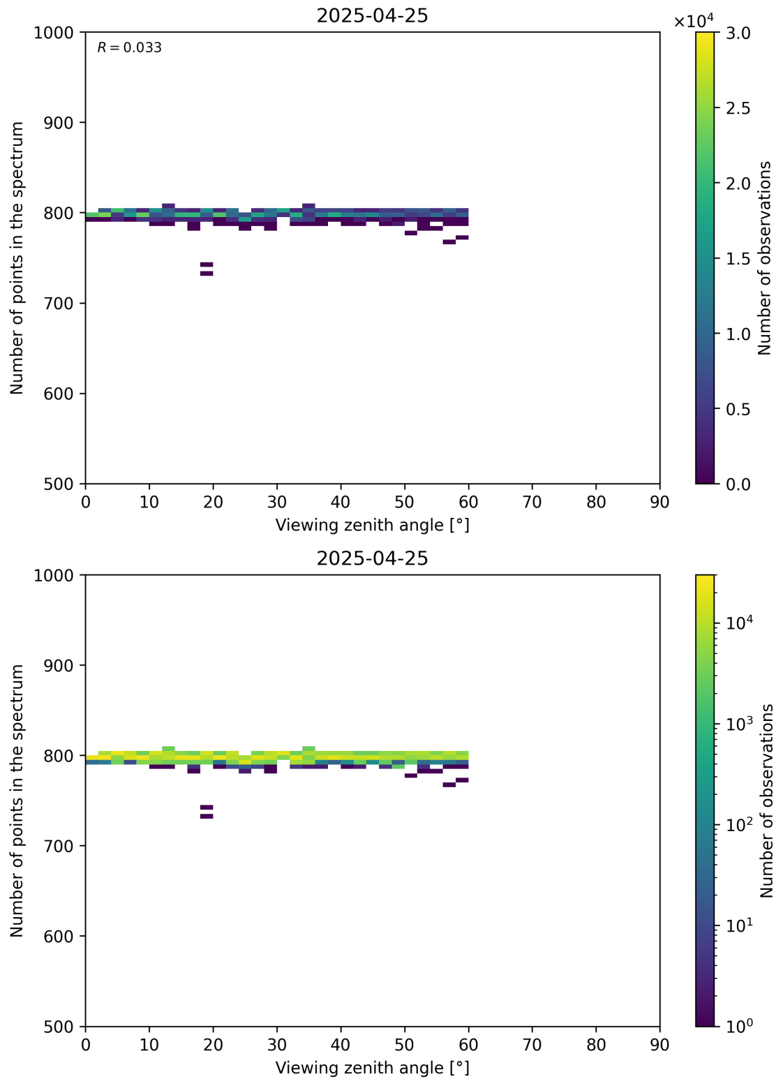
Figure 114: Scatter density plot of “Viewing zenith angle” against “Number of points in the spectrum” for 2025-04-24 to 2025-04-26.
