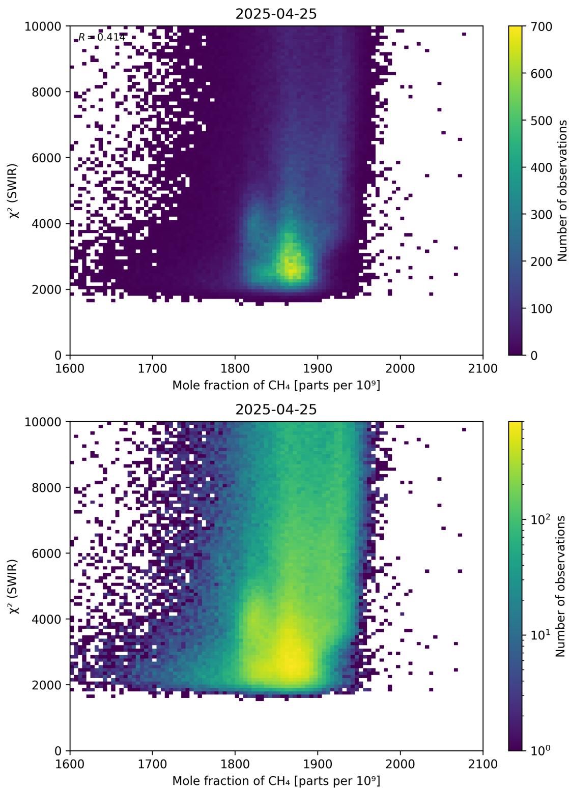
Figure 71: Scatter density plot of “Mole fraction of \text{CH}_4 ” against “ \chi^2 (SWIR)” for 2025-04-24 to 2025-04-26.
