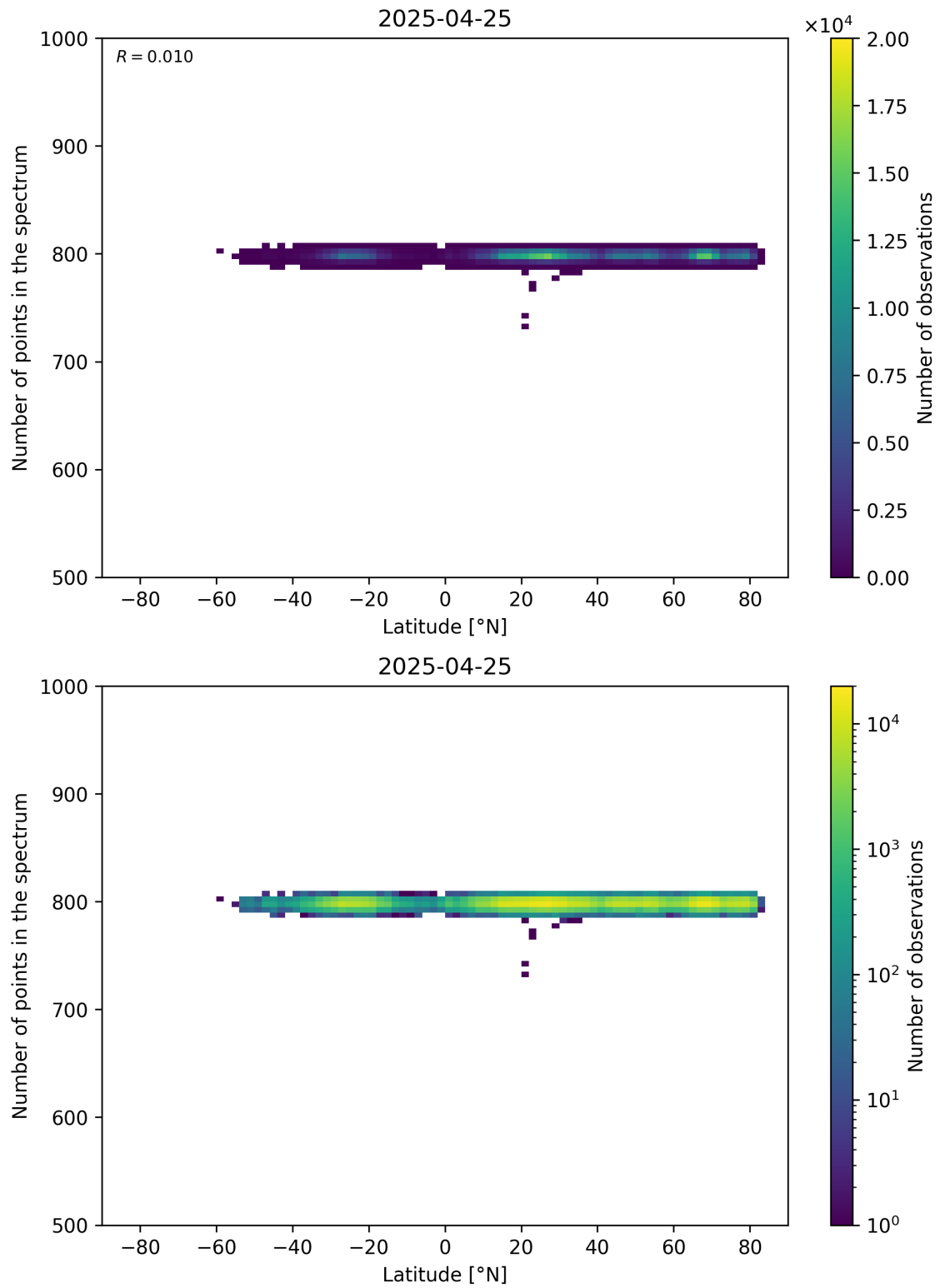
Figure 61: Scatter density plot of “Latitude” against “Number of points in the spectrum” for 2025-04-24 to 2025-04-26.
