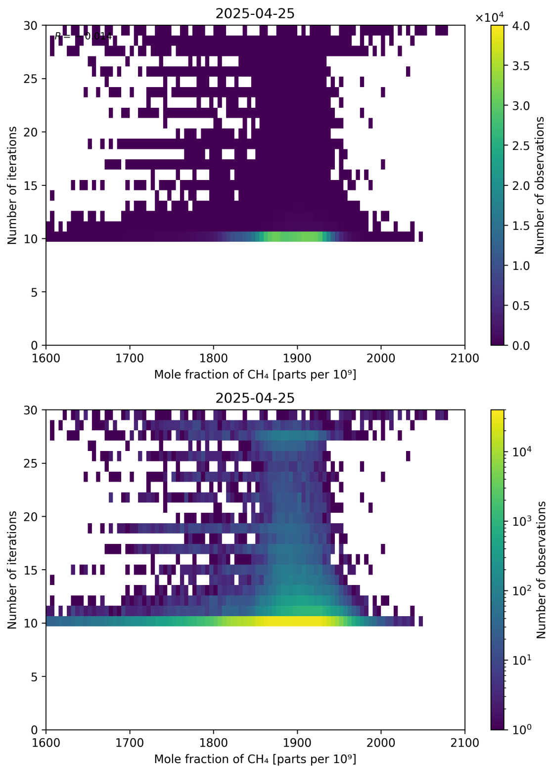
Figure 76: Scatter density plot of “Mole fraction of CH 4 ” against “Number of iterations” for 2025-04-24 to 2025-04-26.
