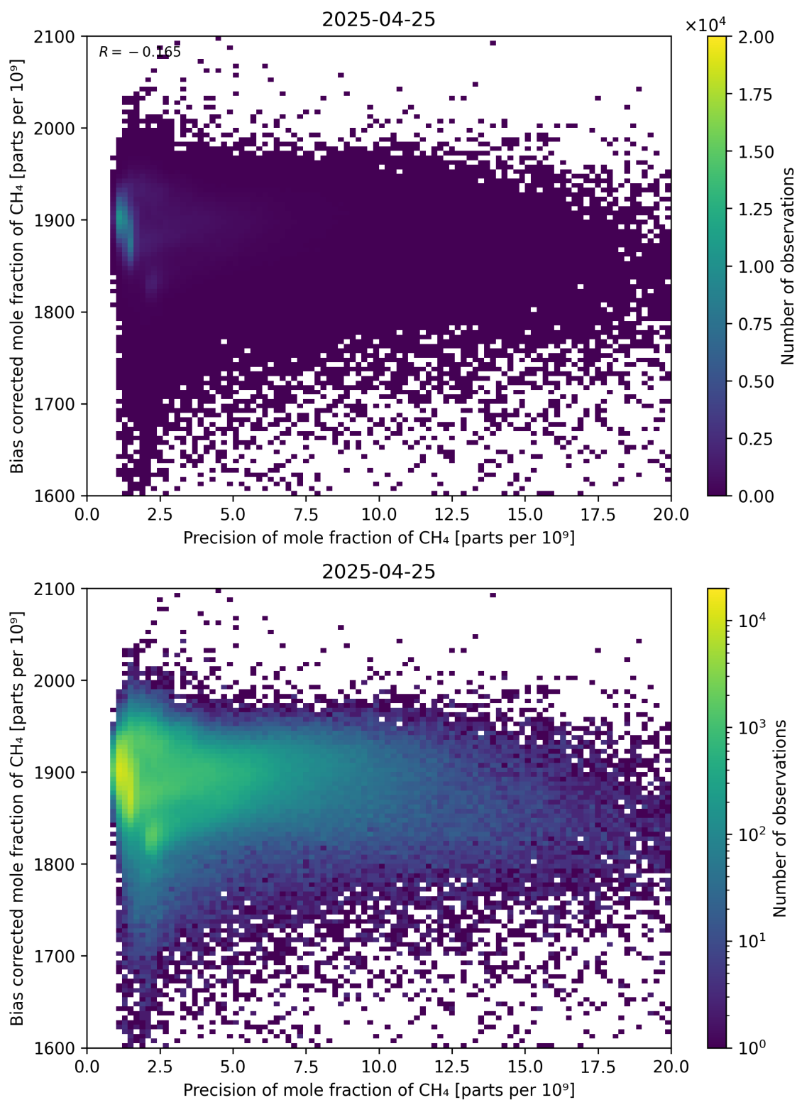
Figure 82: Scatter density plot of “Precision of mole fraction of CH 4 ” against “Bias corrected mole fraction of CH 4 ” for 2025-04-24 to 2025-04-26.
