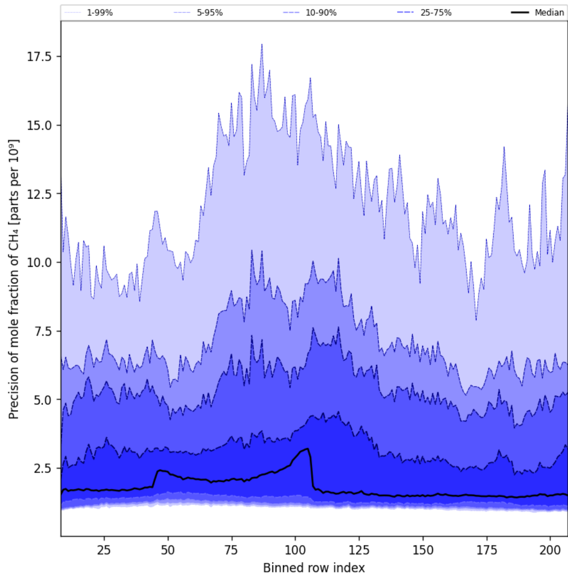
Figure 35: Along track statistics of “Precision of mole fraction of CH 4 ” for 2025-04-24 to 2025-04-26
