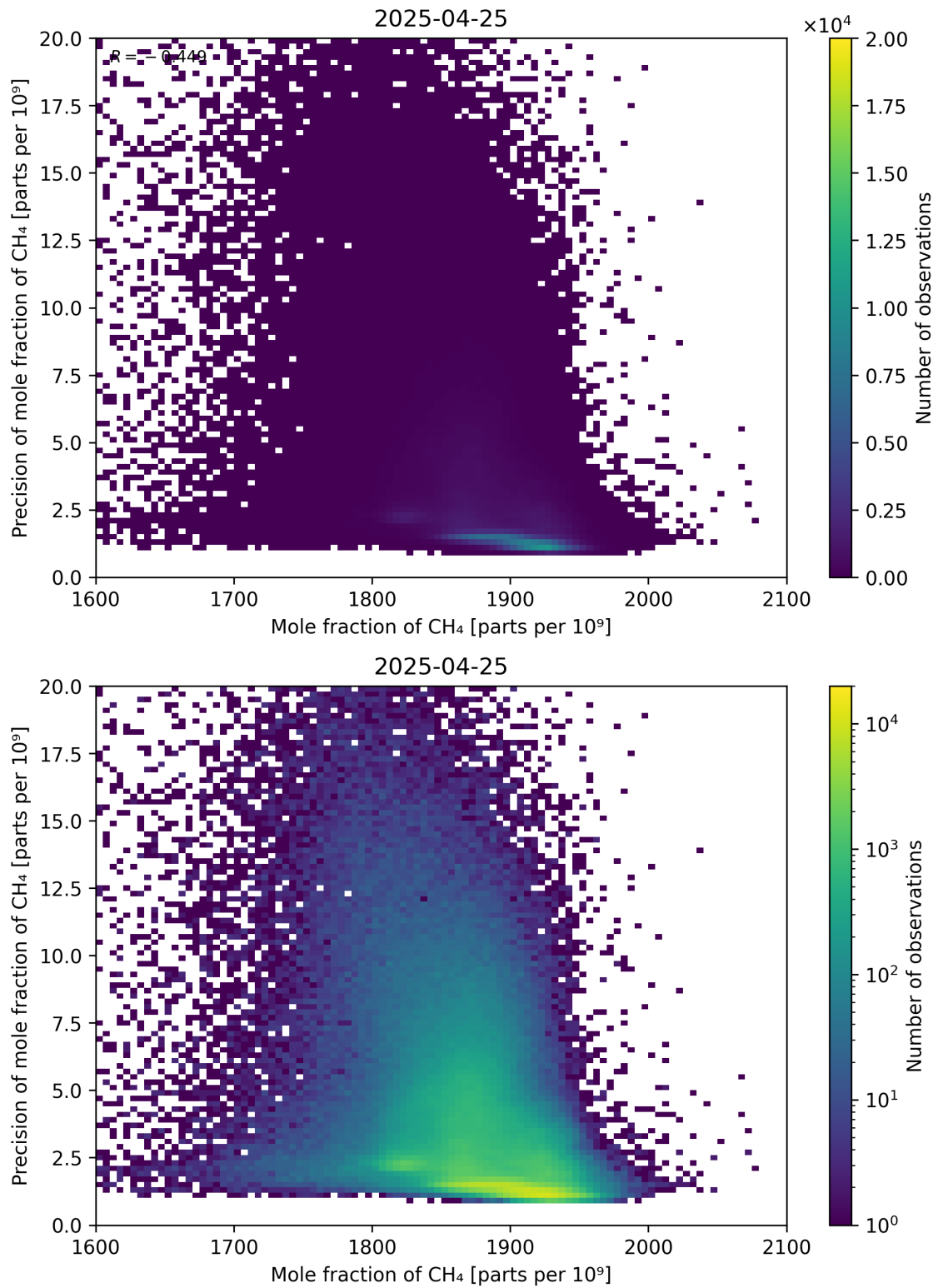
Figure 75: Scatter density plot of “Mole fraction of CH 4 ” against “Precision of mole fraction of CH 4 ” for 2025-04-24 to 2025-04-26.
