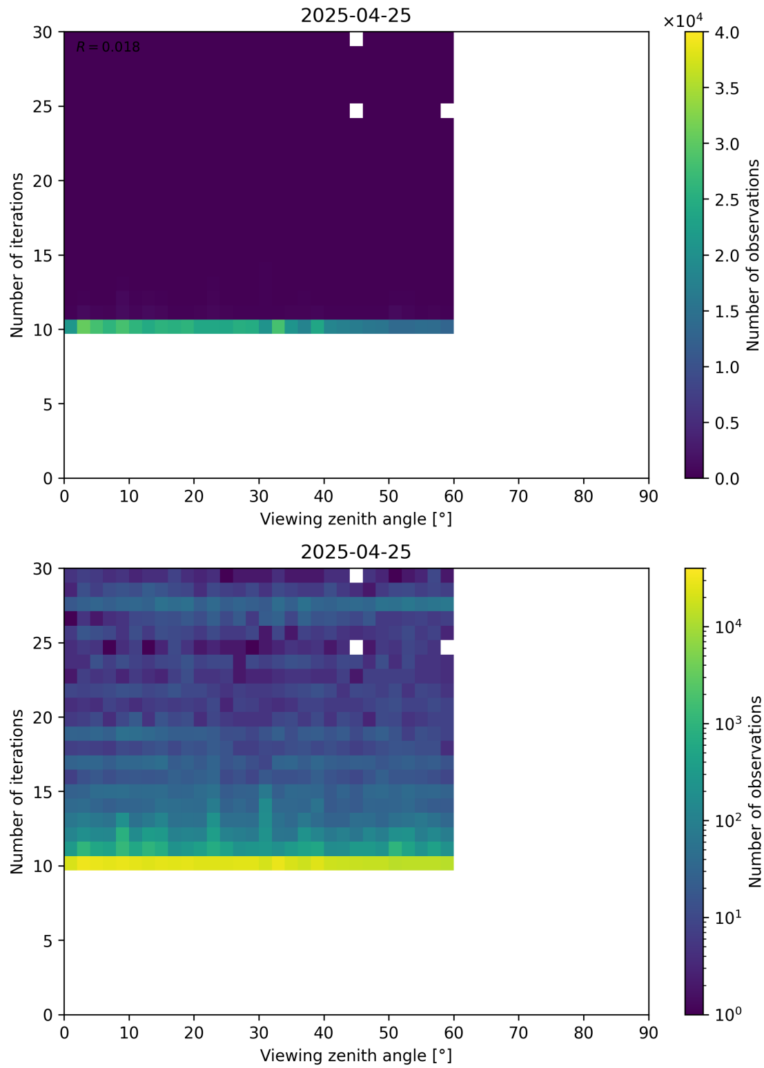
Figure 113: Scatter density plot of “Viewing zenith angle” against “Number of iterations” for 2025-04-24 to 2025-04-26.
