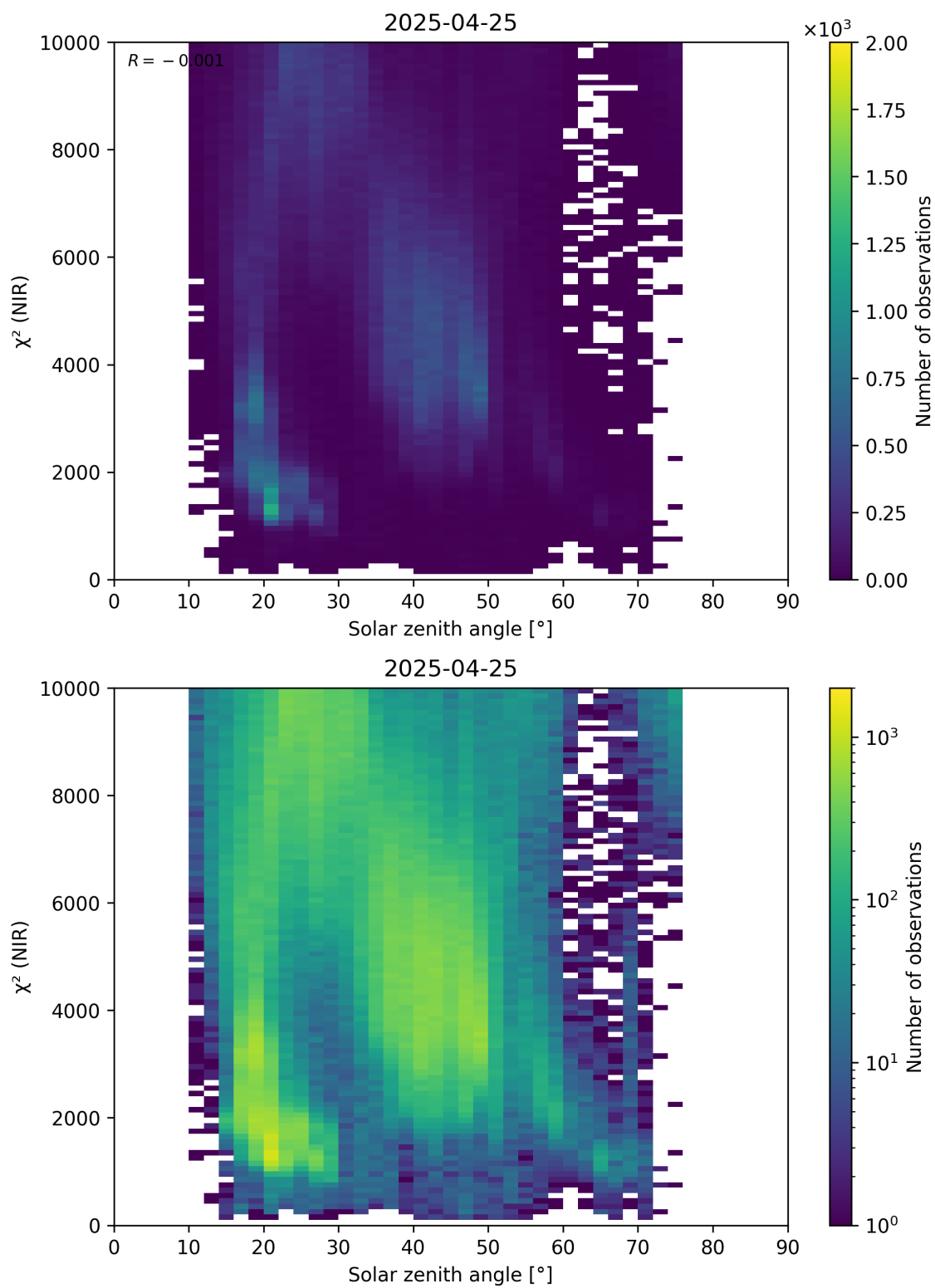
Figure 94: Scatter density plot of “Solar zenith angle” against “ \chi^2 (NIR)” for 2025-04-24 to 2025-04-26.
