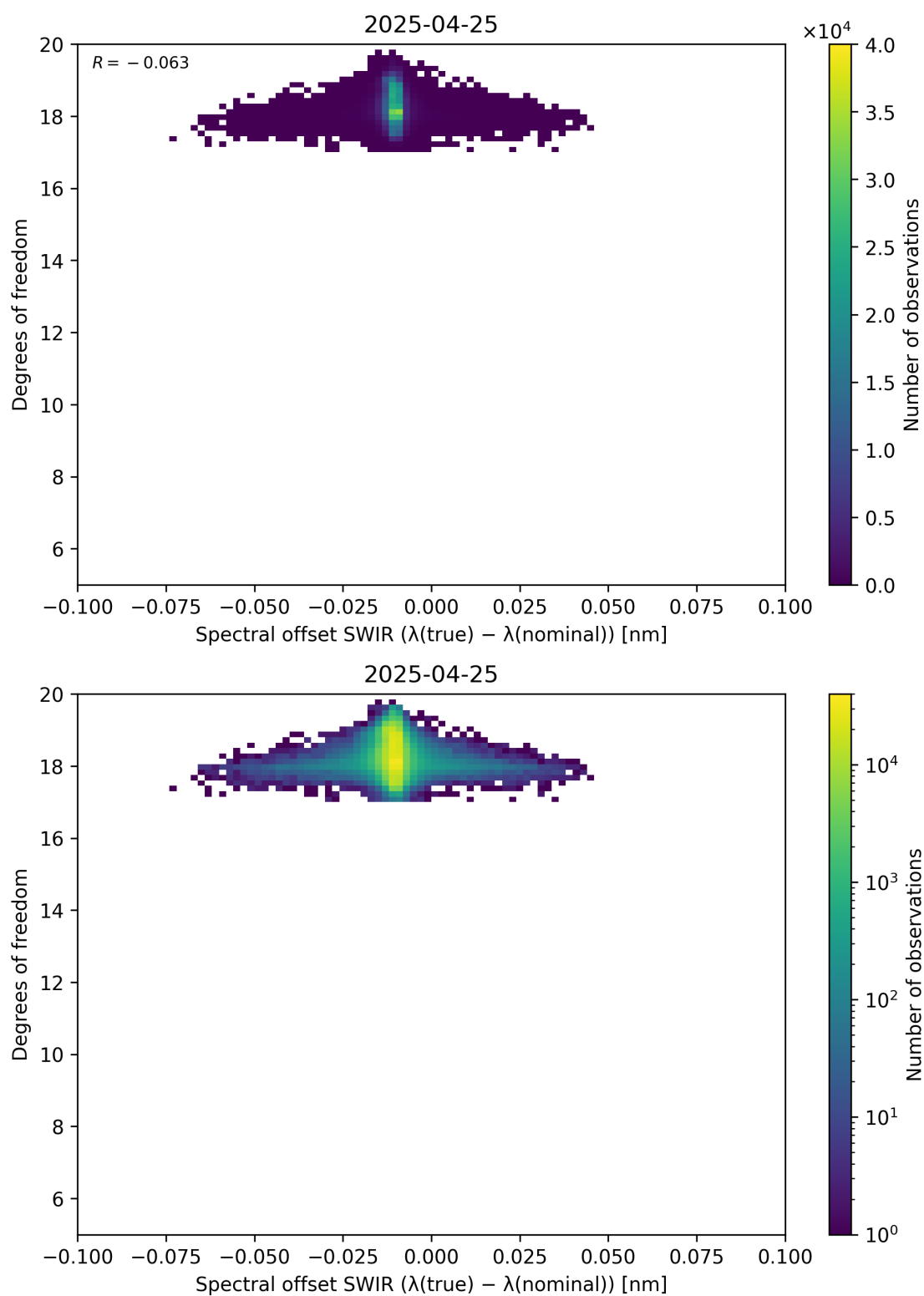
Figure 119: Scatter density plot of “Spectral offset SWIR ( \lambda_{\text{true}} - \lambda_{\text{nominal}} )” against “Degrees of freedom” for 2025-04-24 to 2025-04-26.
