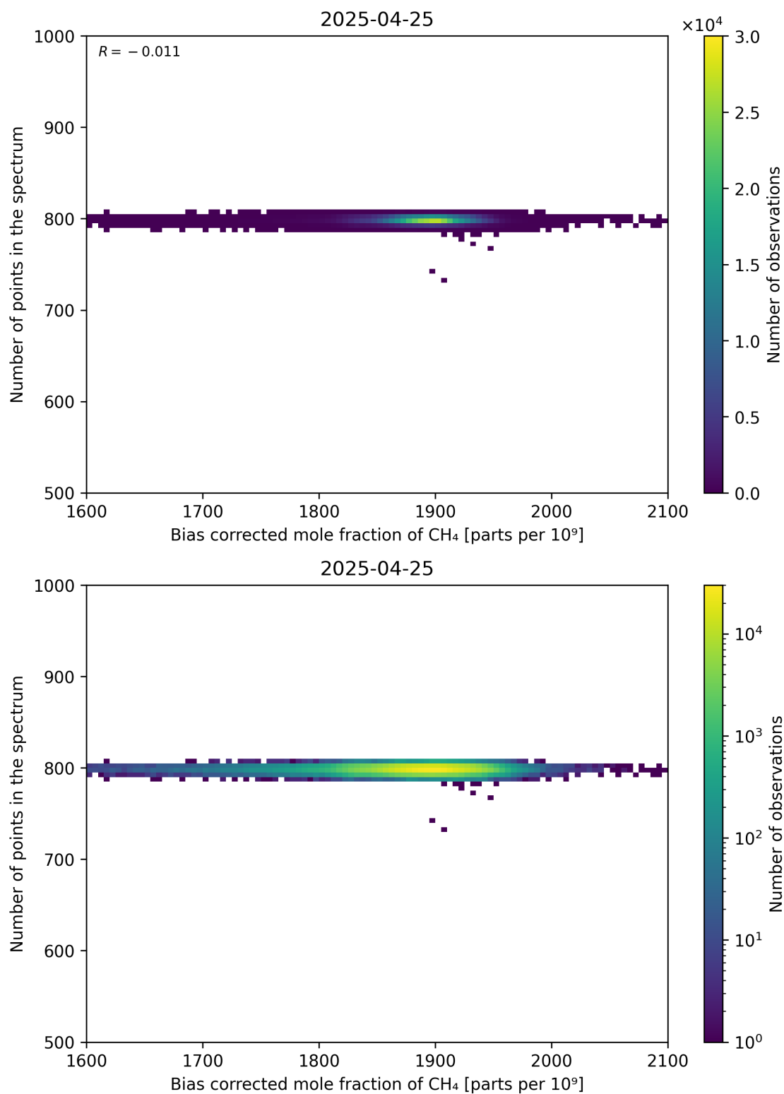
Figure 68: Scatter density plot of “Bias corrected mole fraction of CH 4 ” against “Number of points in the spectrum” for 2025-04-24 to 2025-04-26.
