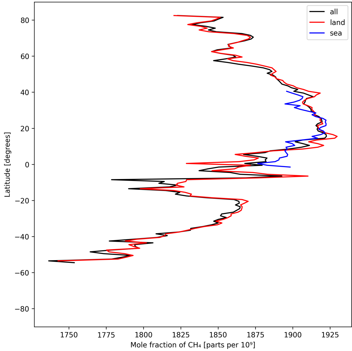
Figure 12: Zonal average of “Mole fraction of \text{CH}_4 ” for 2025-04-24 to 2025-04-26.
