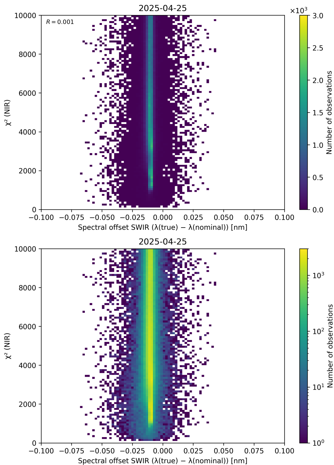
Figure 117: Scatter density plot of “Spectral offset SWIR ( \lambda_{\text{true}} - \lambda_{\text{nominal}} )” against “ \chi^2 (NIR)” for 2025-04-24 to 2025-04-26.
