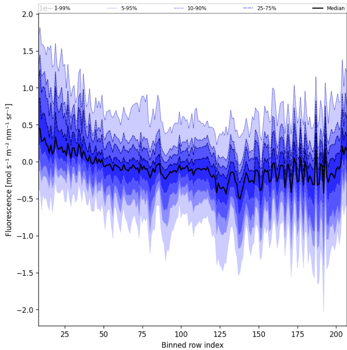
Figure 43: Along track statistics of "Fluorescence" for 2025-04-24 to 2025-04-26
