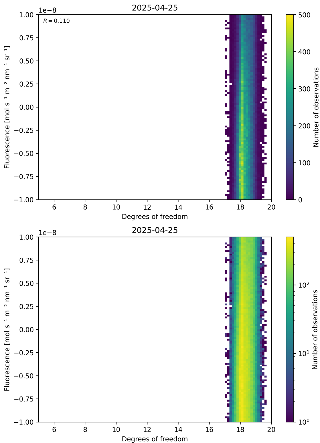
Figure 51: Scatter density plot of “Degrees of freedom” against “Fluorescence” for 2025-04-24 to 2025-04-26.
