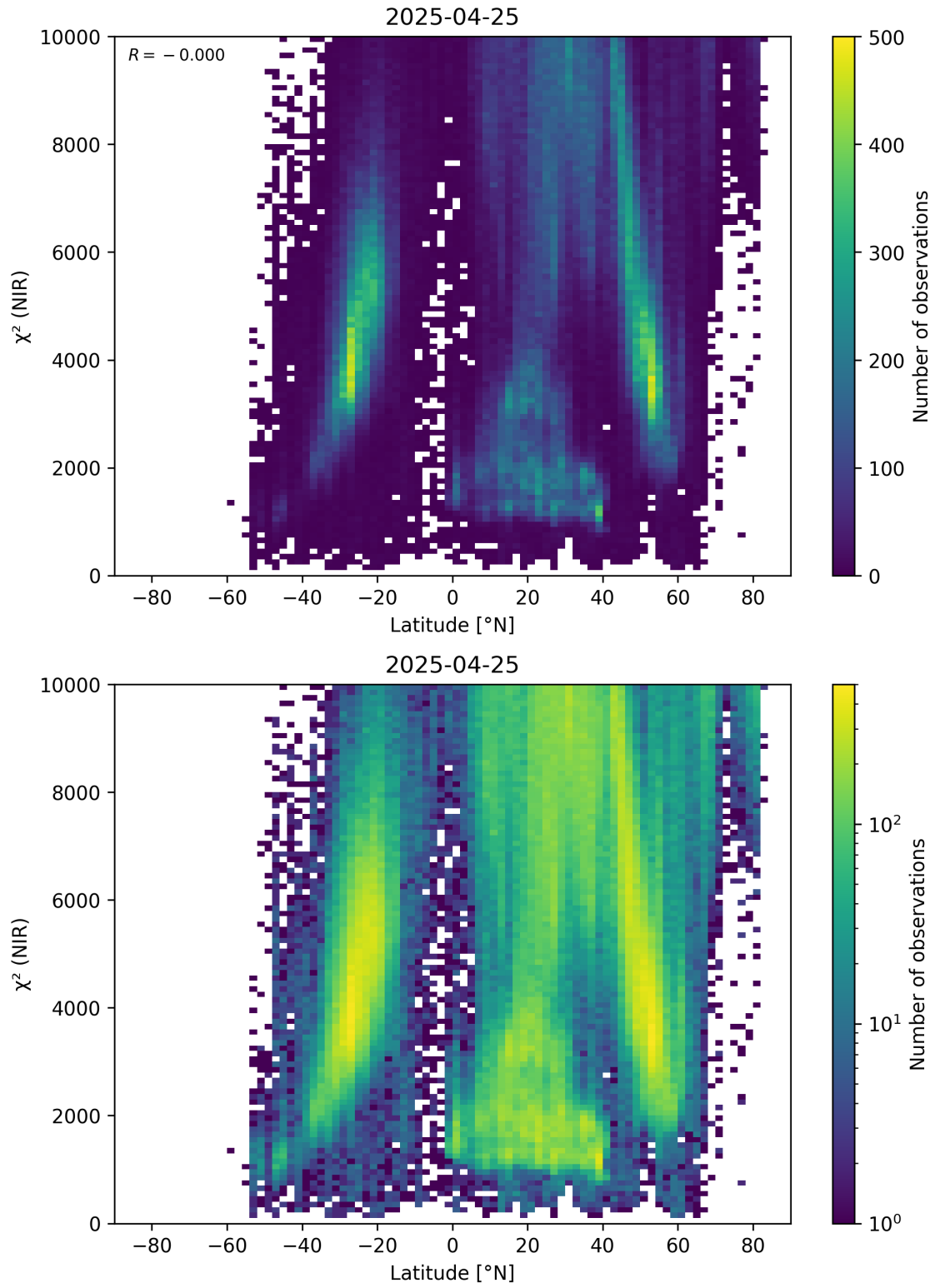
Figure 53: Scatter density plot of “Latitude” against “ \chi^2 (NIR)” for 2025-04-24 to 2025-04-26.
