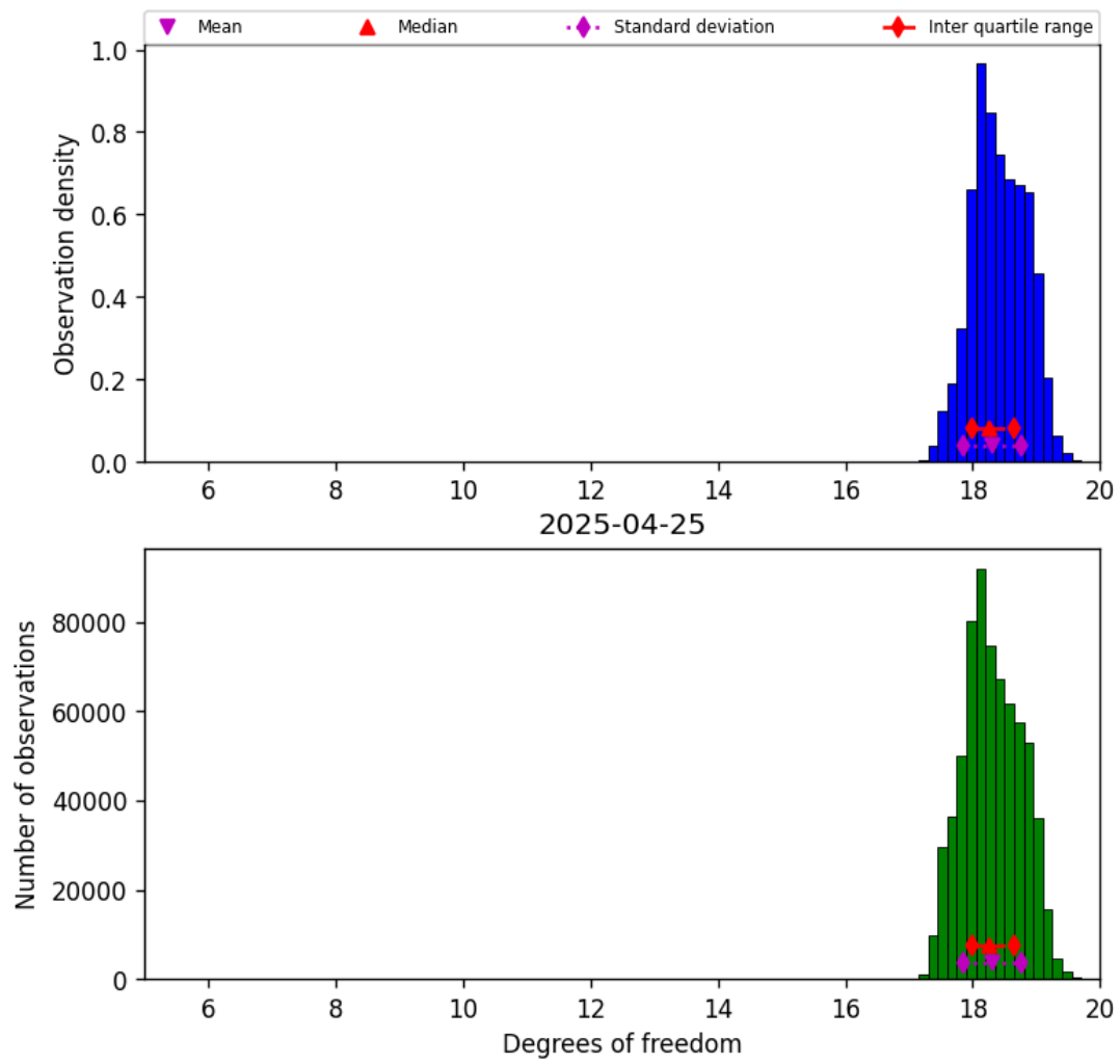
Figure 30: Histogram of “Degrees of freedom” for 2025-04-24 to 2025-04-26
