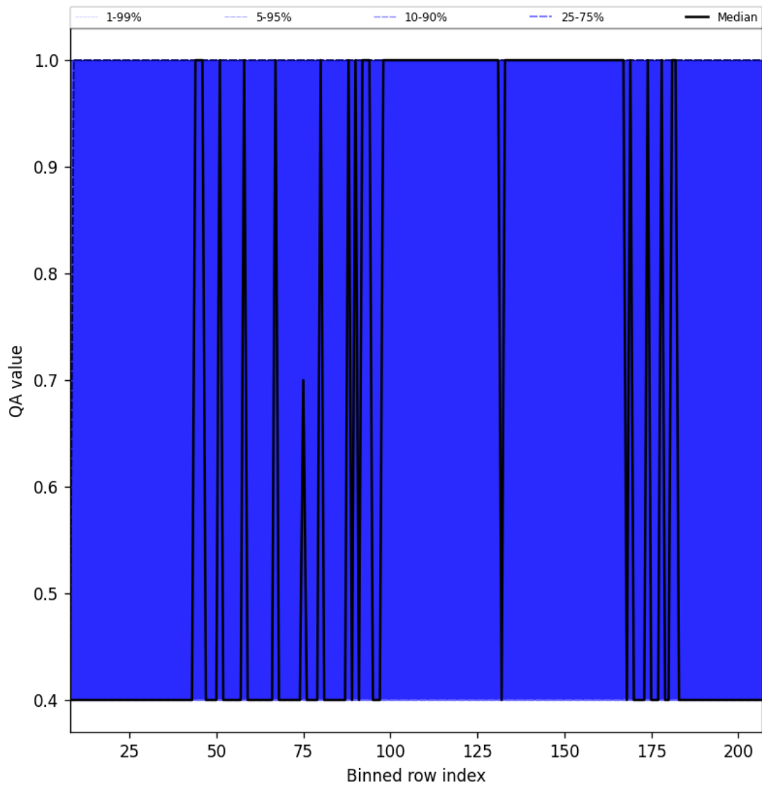
Figure 33: Along track statistics of “QA value” for 2025-04-24 to 2025-04-26
