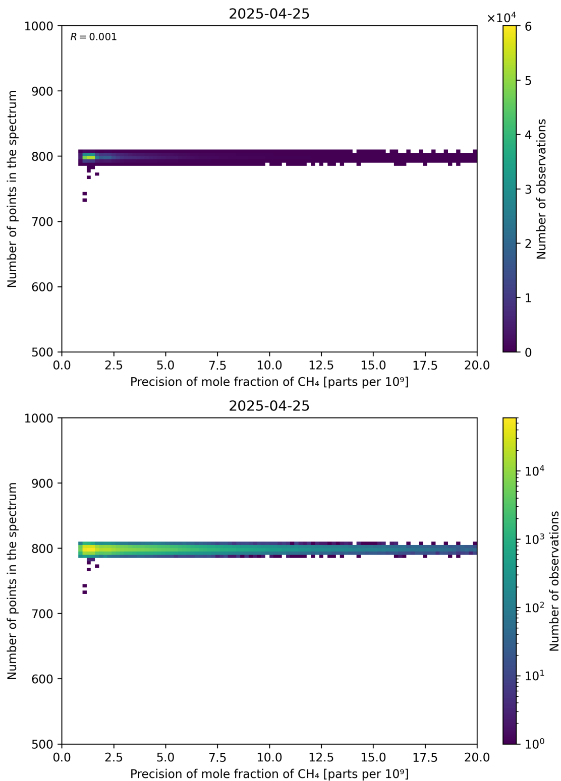
Figure 84: Scatter density plot of “Precision of mole fraction of CH 4 ” against “Number of points in the spectrum” for 2025-04-24 to 2025-04-26.
