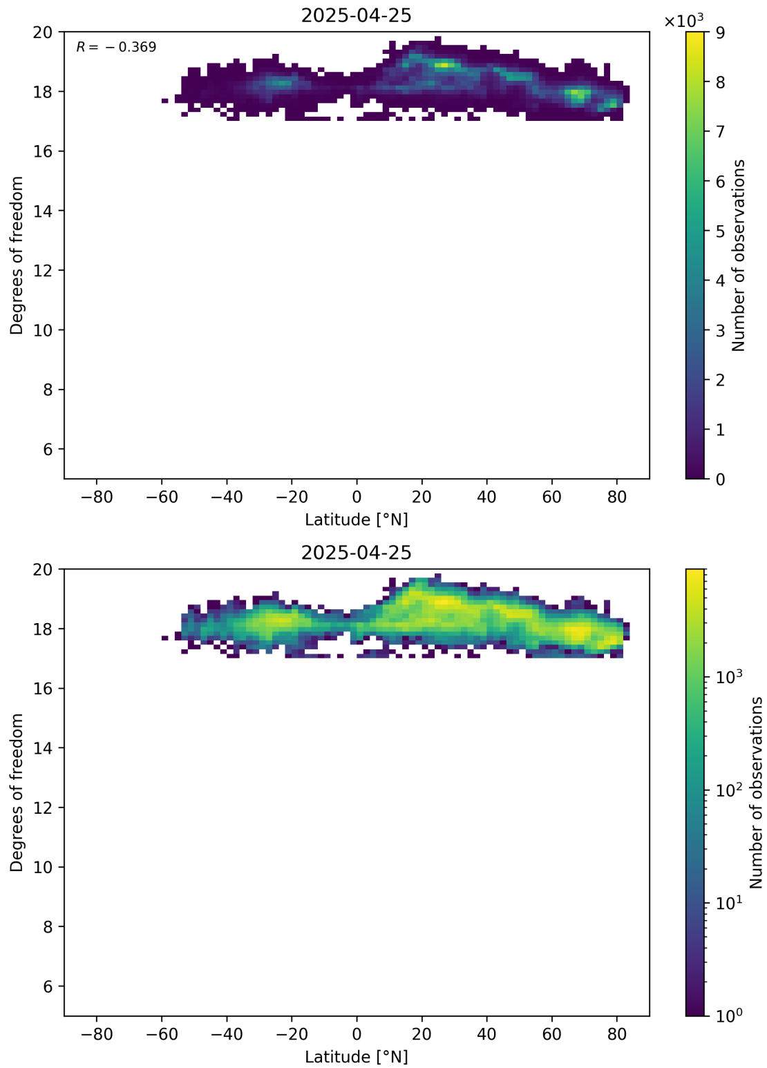
Figure 55: Scatter density plot of “Latitude” against “Degrees of freedom” for 2025-04-24 to 2025-04-26.
