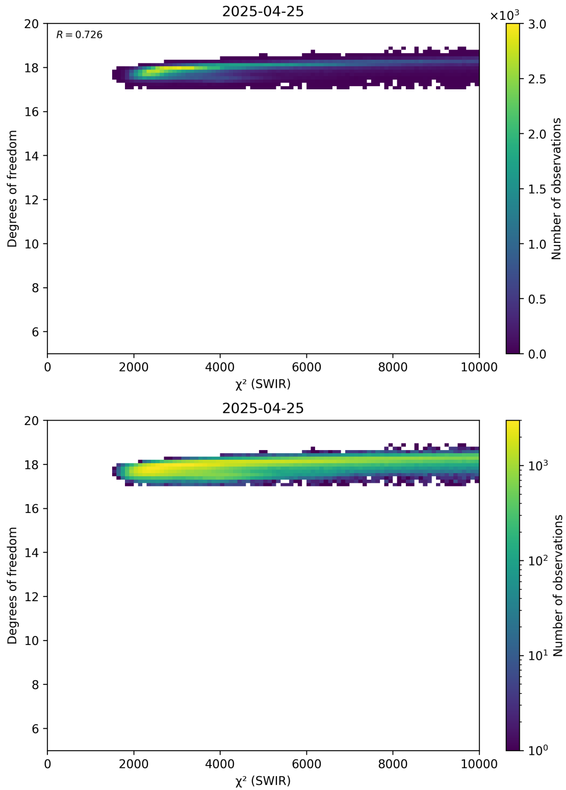
Figure 48: Scatter density plot of " \chi^2 (SWIR)" against "Degrees of freedom" for 2025-04-24 to 2025-04-26.
