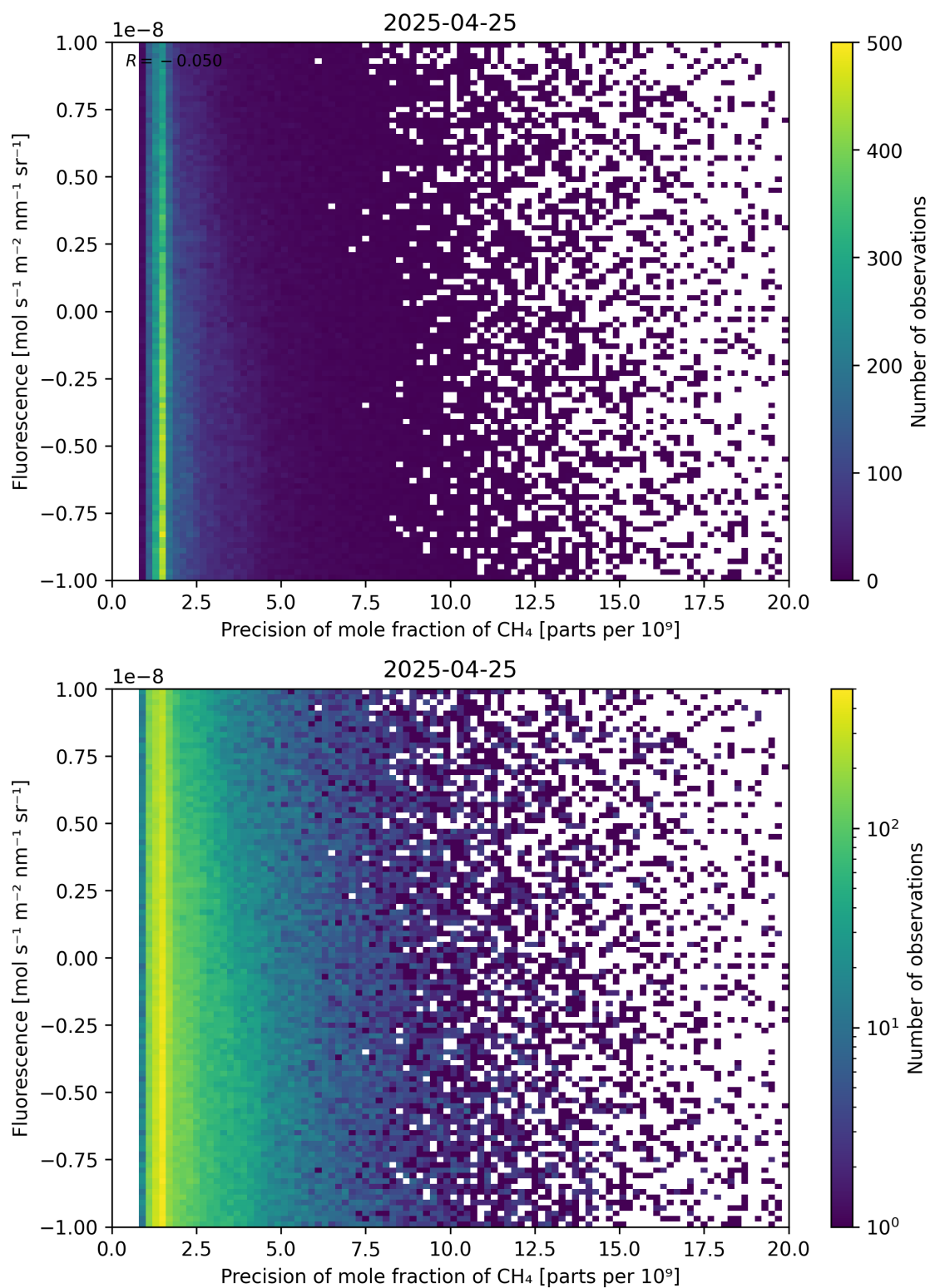
Figure 81: Scatter density plot of “Precision of mole fraction of \text{CH}_4 ” against “Fluorescence” for 2025-04-24 to 2025-04-26.
