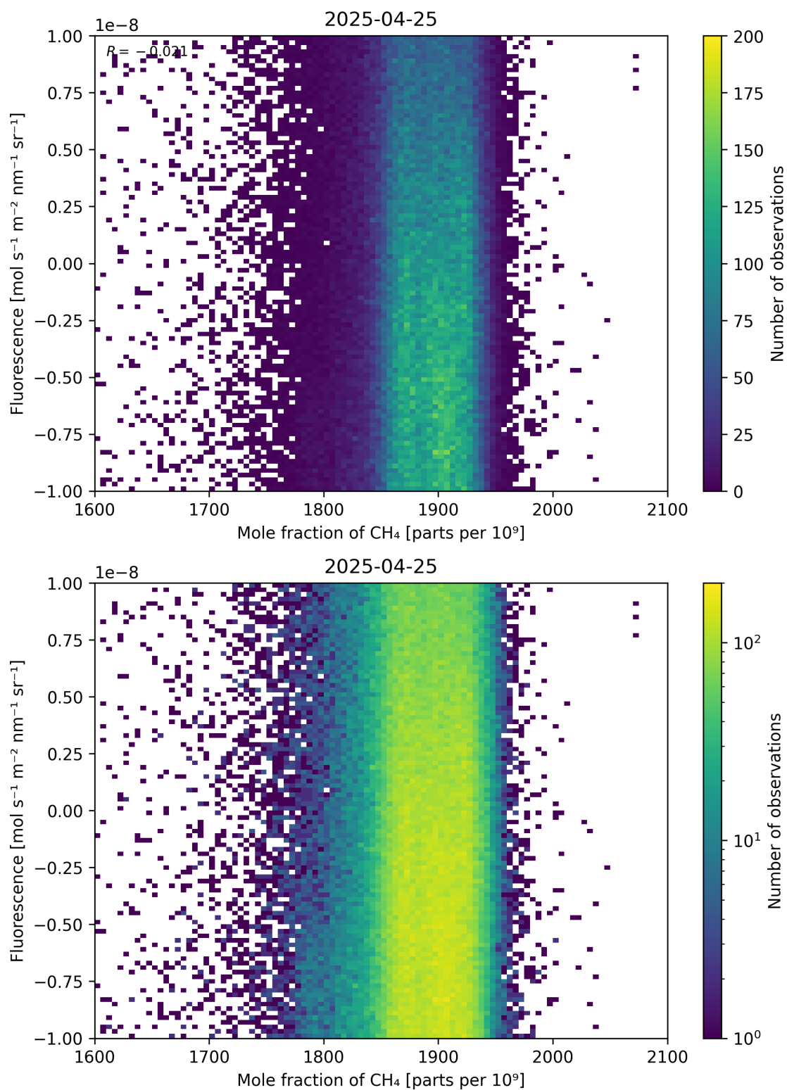
Figure 73: Scatter density plot of “Mole fraction of \text{CH}_4 ” against “Fluorescence” for 2025-04-24 to 2025-04-26.
