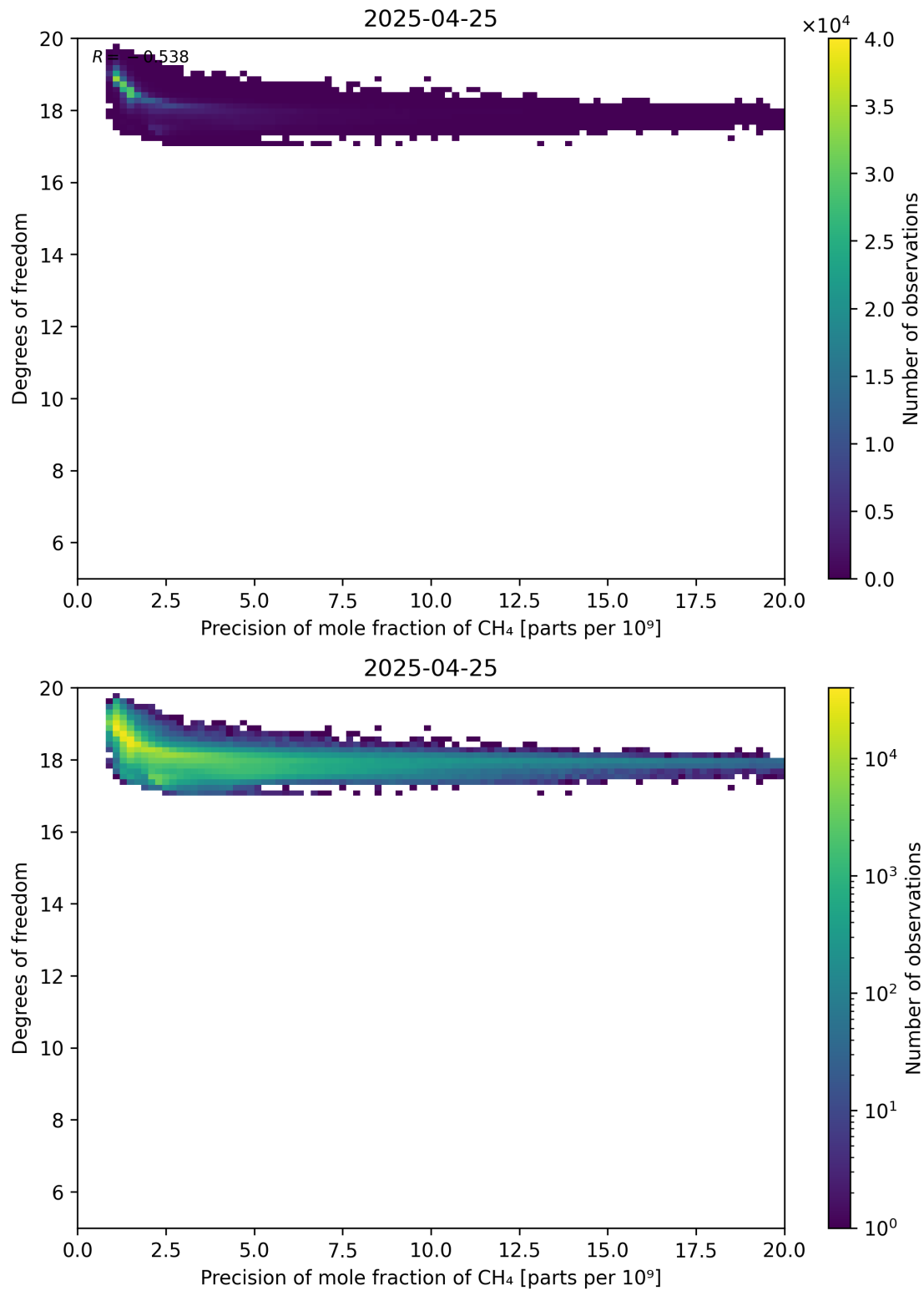
Figure 80: Scatter density plot of “Precision of mole fraction of CH 4 ” against “Degrees of freedom” for 2025-04-24 to 2025-04-26.
