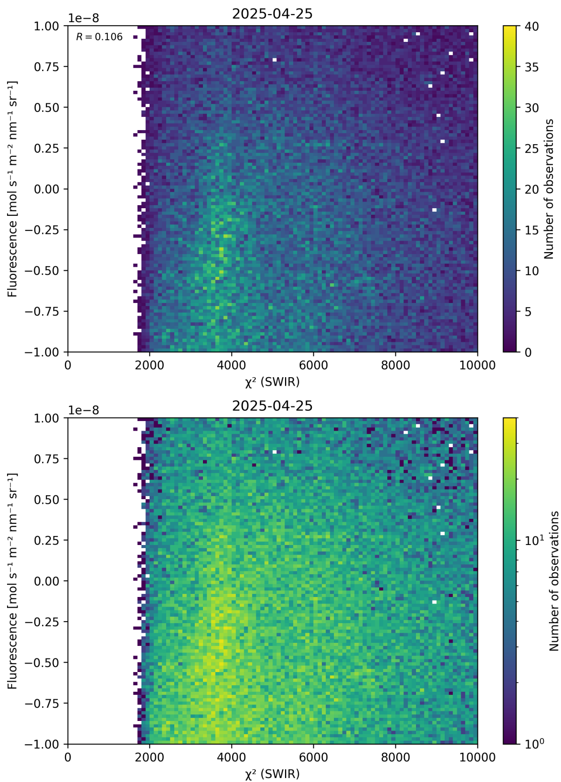
Figure 49: Scatter density plot of “ \chi^2 (SWIR)” against “Fluorescence” for 2025-04-24 to 2025-04-26.
