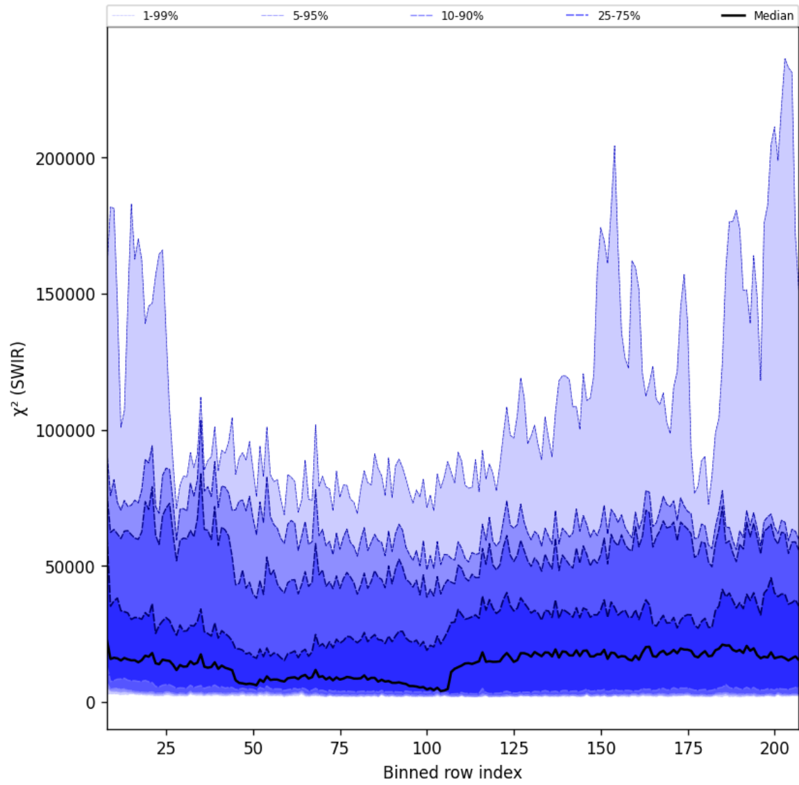
Figure 39: Along track statistics of “ \chi^2 (SWIR)” for 2025-04-24 to 2025-04-26
