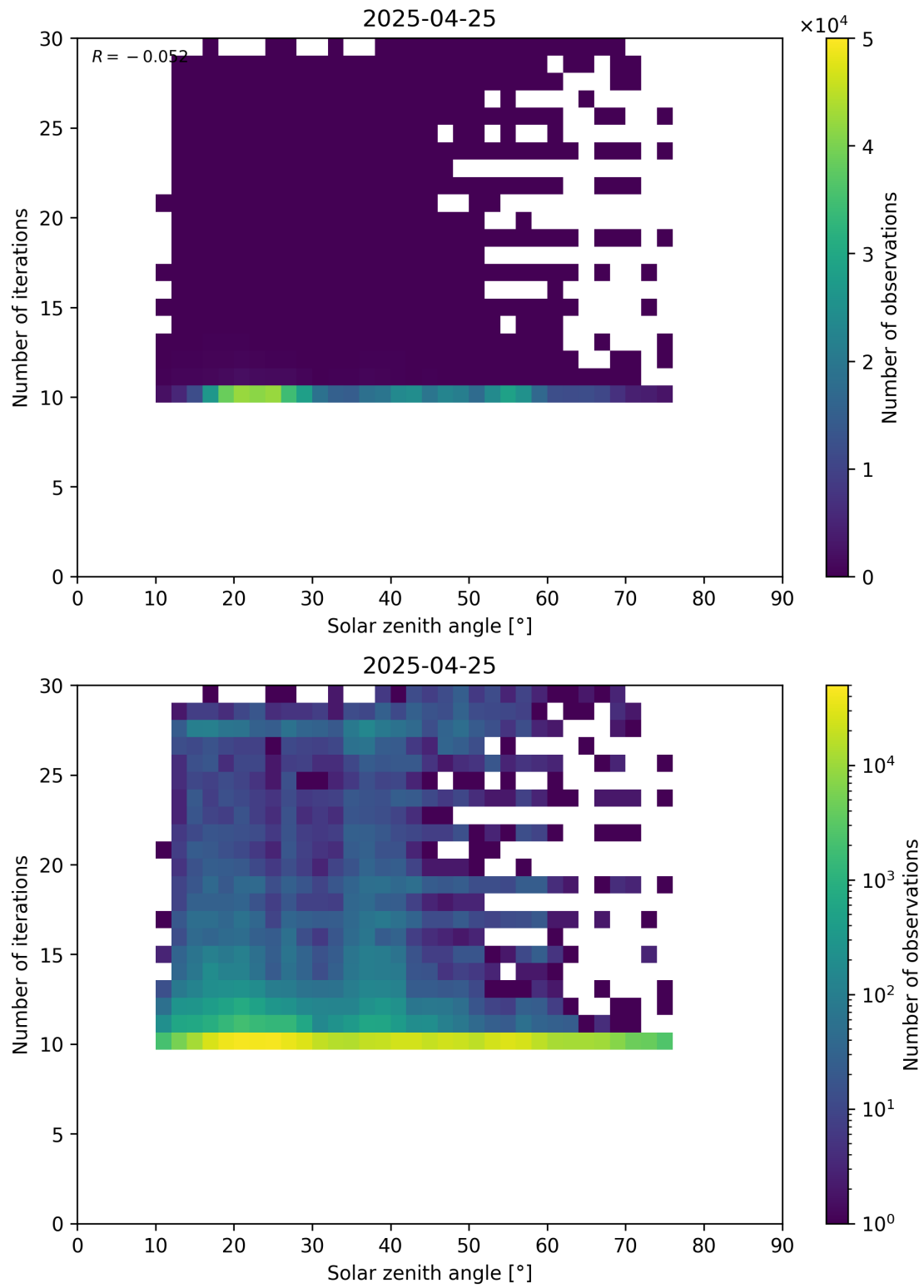
Figure 102: Scatter density plot of “Solar zenith angle” against “Number of iterations” for 2025-04-24 to 2025-04-26.
