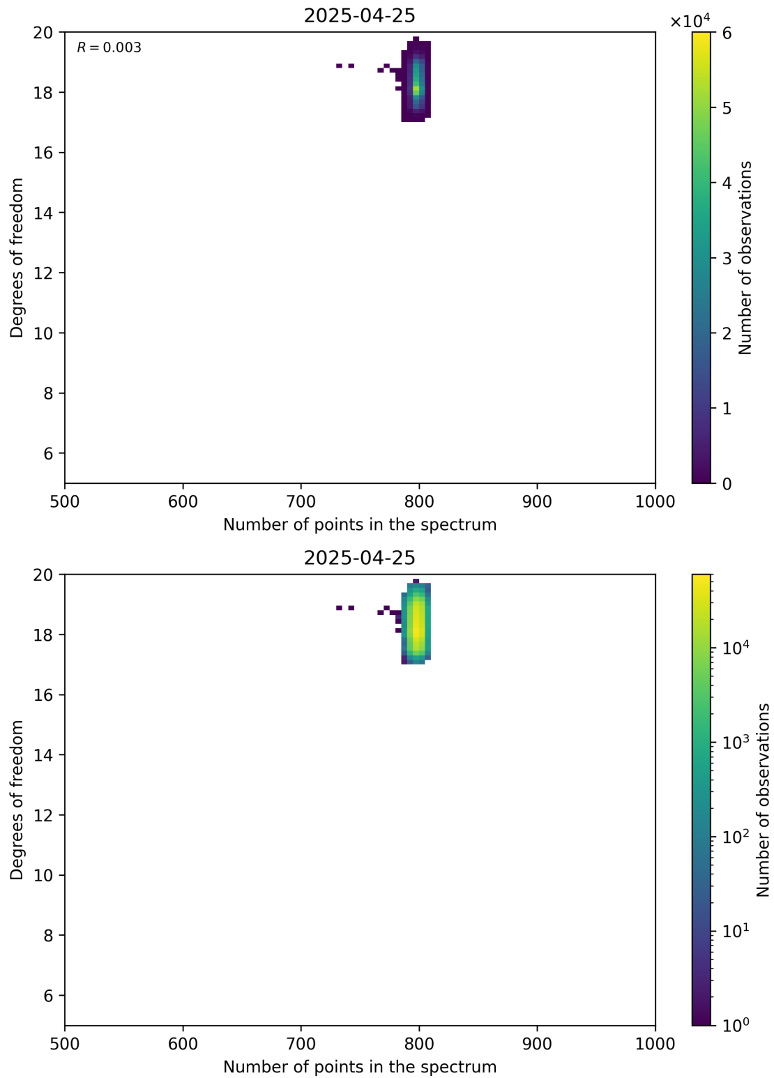
Figure 90: Scatter density plot of “Number of points in the spectrum” against “Degrees of freedom” for 2025-04-24 to 2025-04-26.
