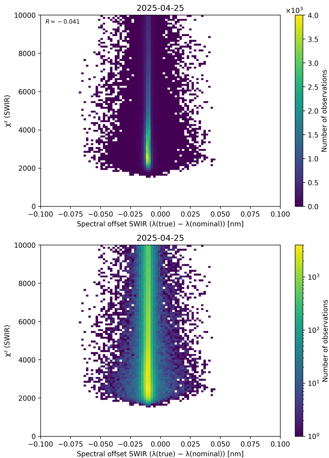
Figure 118: Scatter density plot of “Spectral offset SWIR ( \lambda_{\text{true}} - \lambda_{\text{nominal}} )” against “ \chi^2 (SWIR)” for 2025-04-24 to 2025-04-26.
