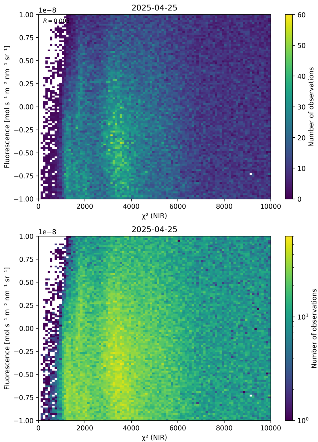
Figure 45: Scatter density plot of “ \chi^2 (NIR)” against “Fluorescence” for 2025-04-24 to 2025-04-26.
