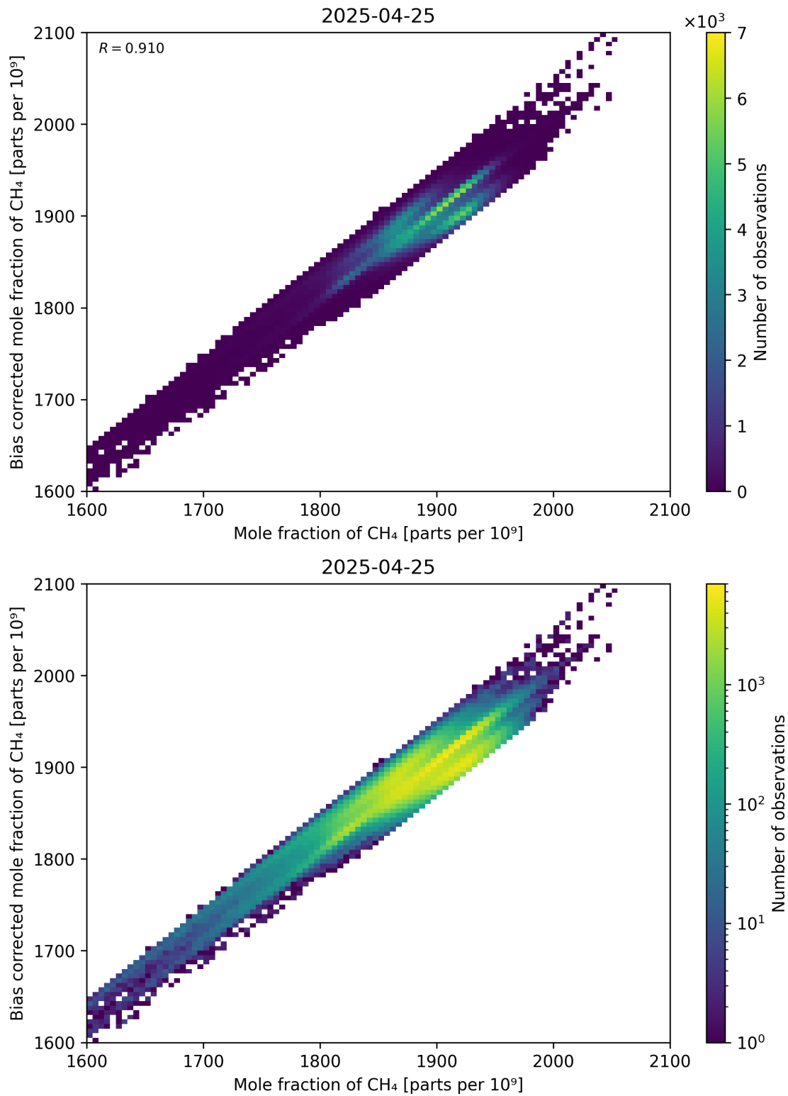
Figure 74: Scatter density plot of “Mole fraction of CH 4 ” against “Bias corrected mole fraction of CH 4 ” for 2025-04-24 to 2025-04-26.
