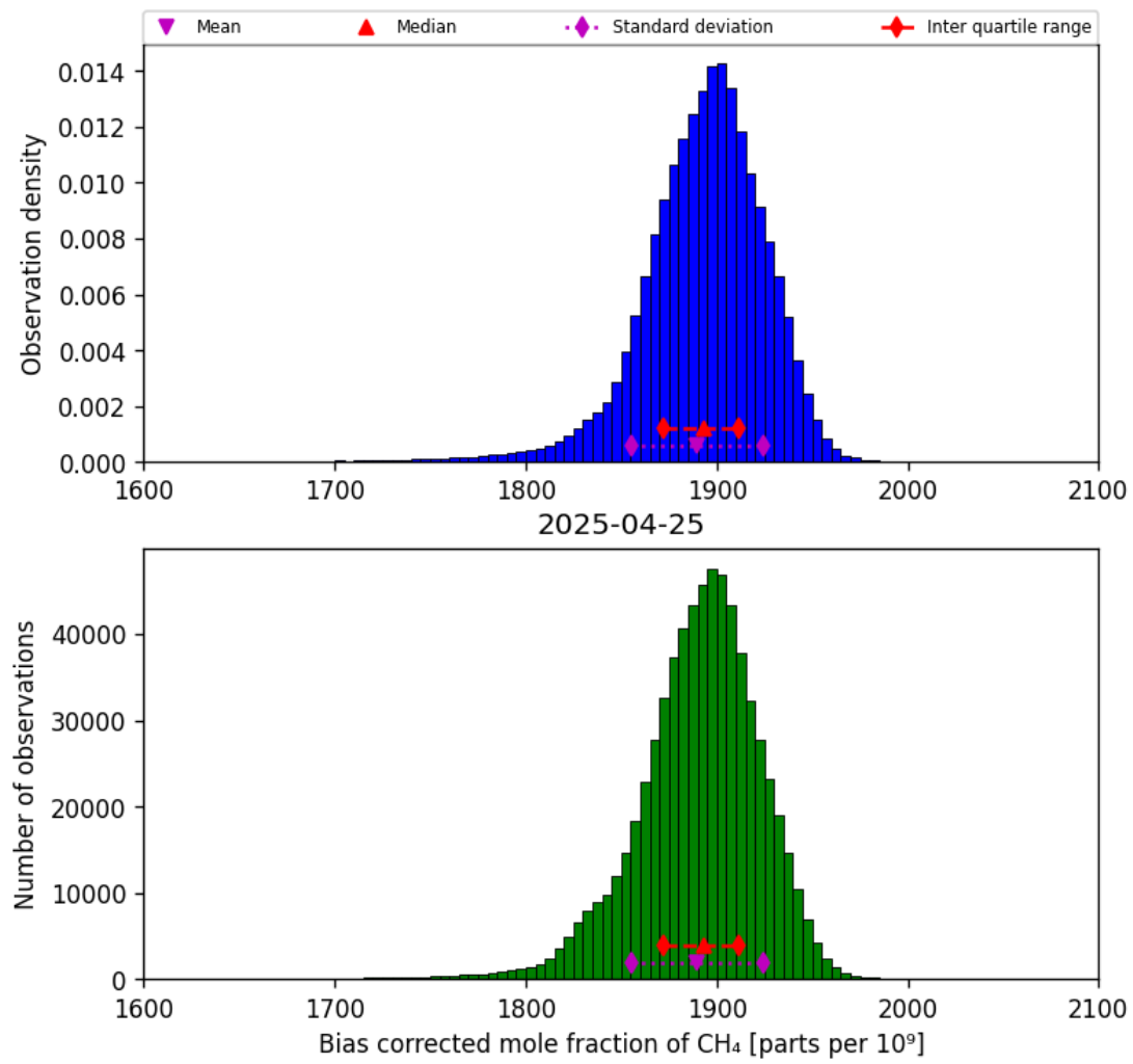
Figure 25: Histogram of “Bias corrected mole fraction of CH 4 ” for 2025-04-24 to 2025-04-26
