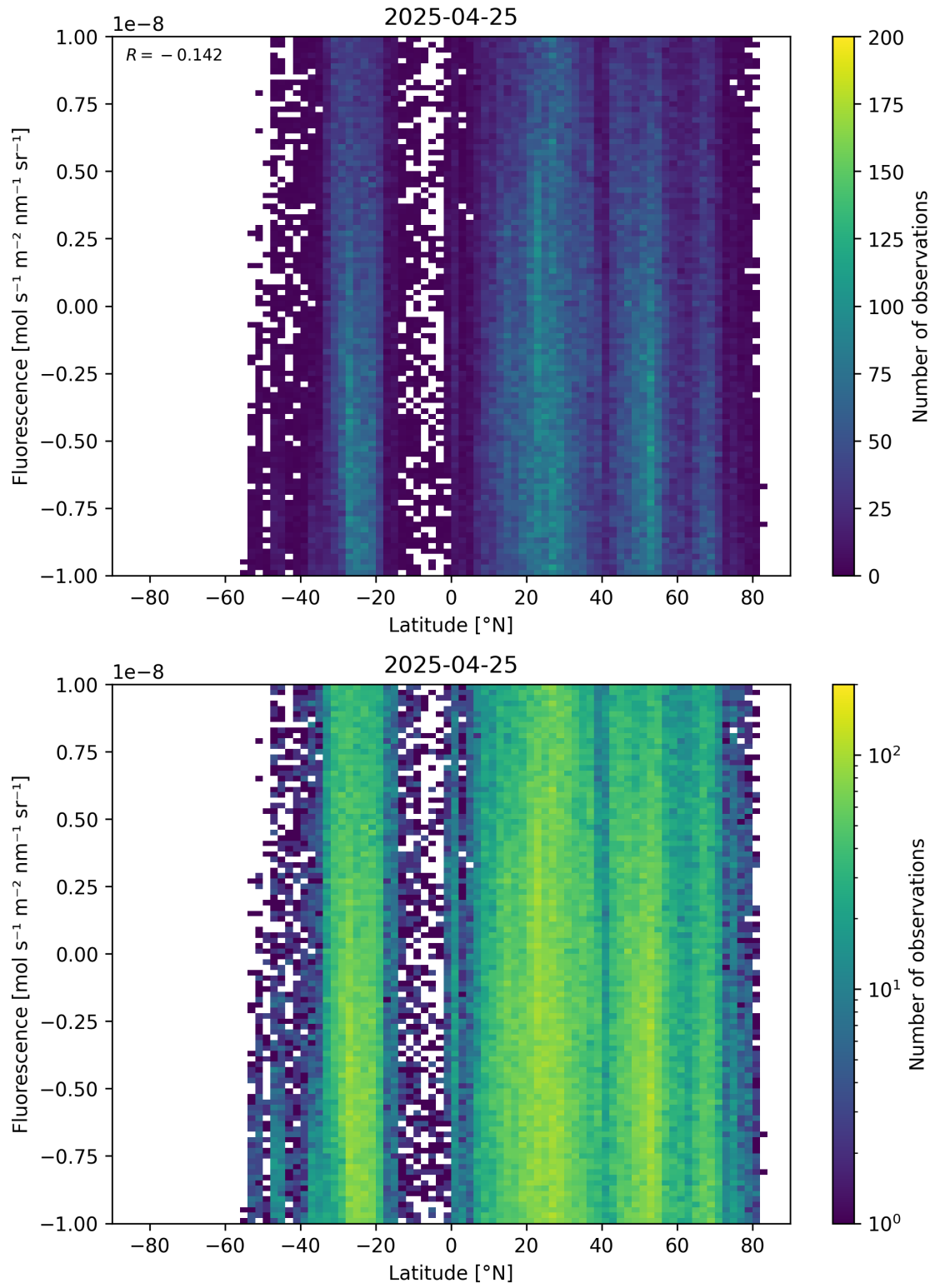
Figure 56: Scatter density plot of “Latitude” against “Fluorescence” for 2025-04-24 to 2025-04-26.
