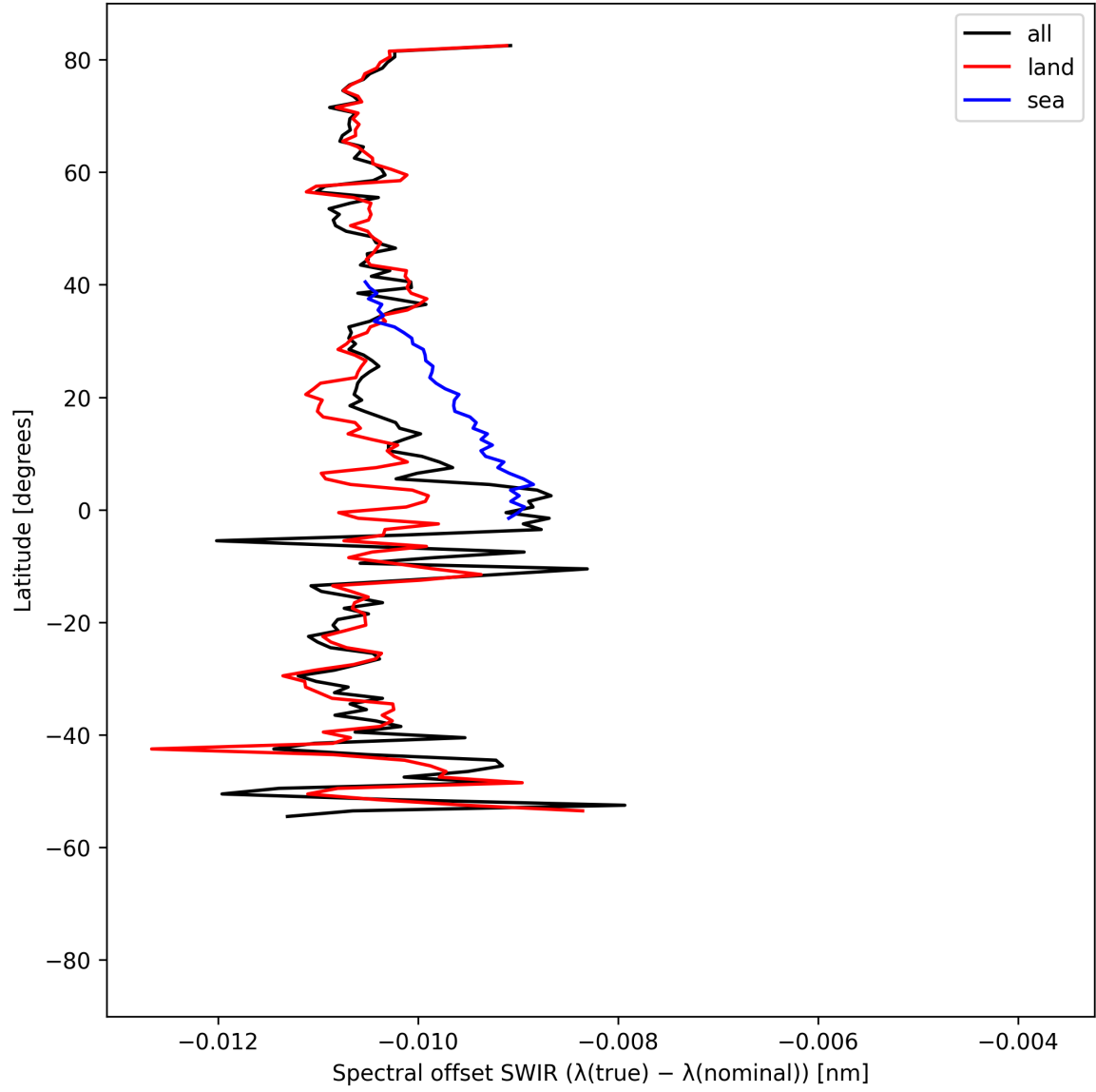
Figure 16: Zonal average of “Spectral offset SWIR ( \lambda_{\text{true}} - \lambda_{\text{nominal}} )” for 2025-04-24 to 2025-04-26.
