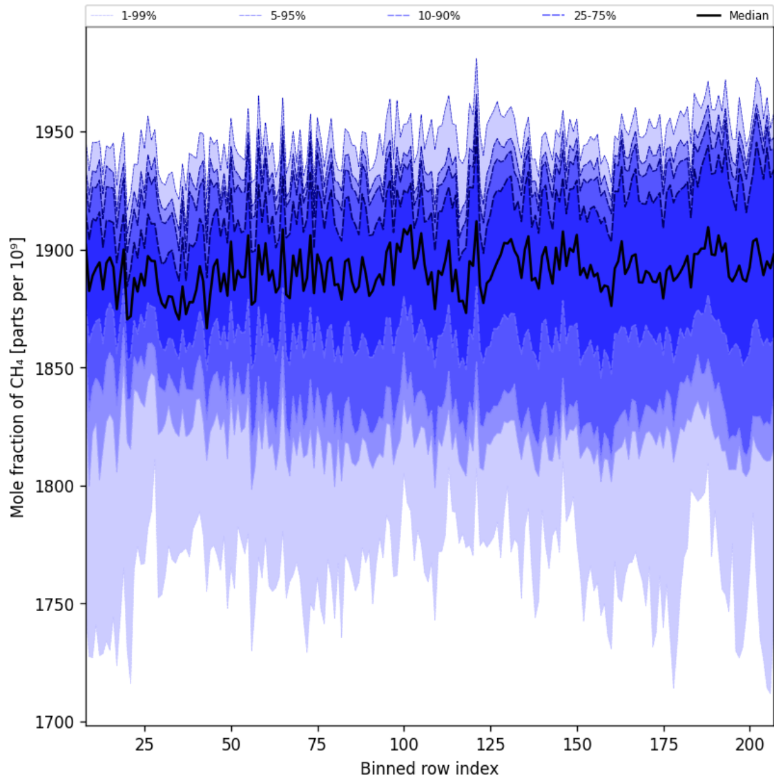
Figure 34: Along track statistics of “Mole fraction of CH 4 ” for 2025-04-24 to 2025-04-26
