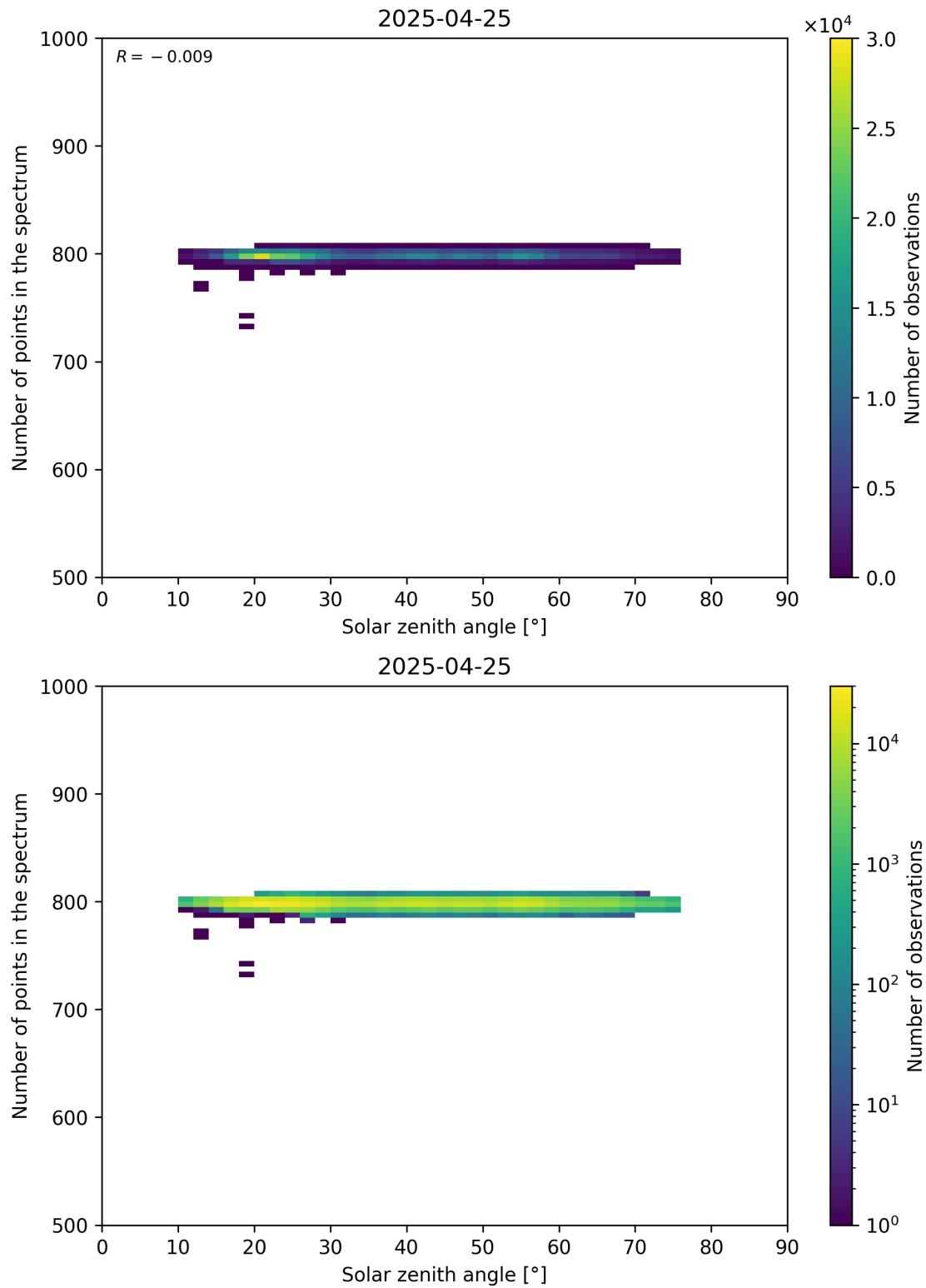
Figure 103: Scatter density plot of “Solar zenith angle” against “Number of points in the spectrum” for 2025-04-24 to 2025-04-26.
