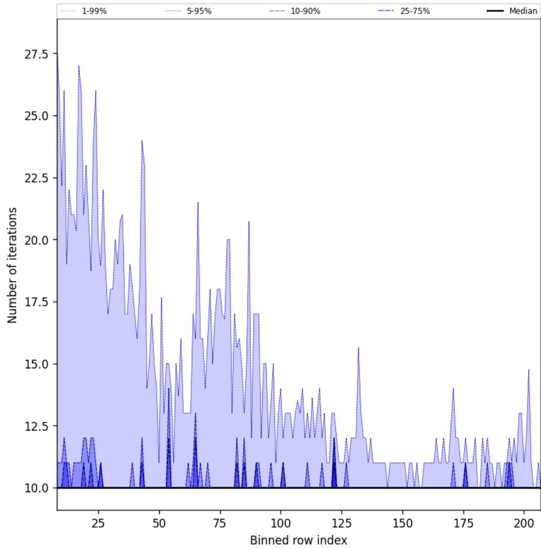
Figure 42: Along track statistics of “Number of iterations” for 2025-04-24 to 2025-04-26
