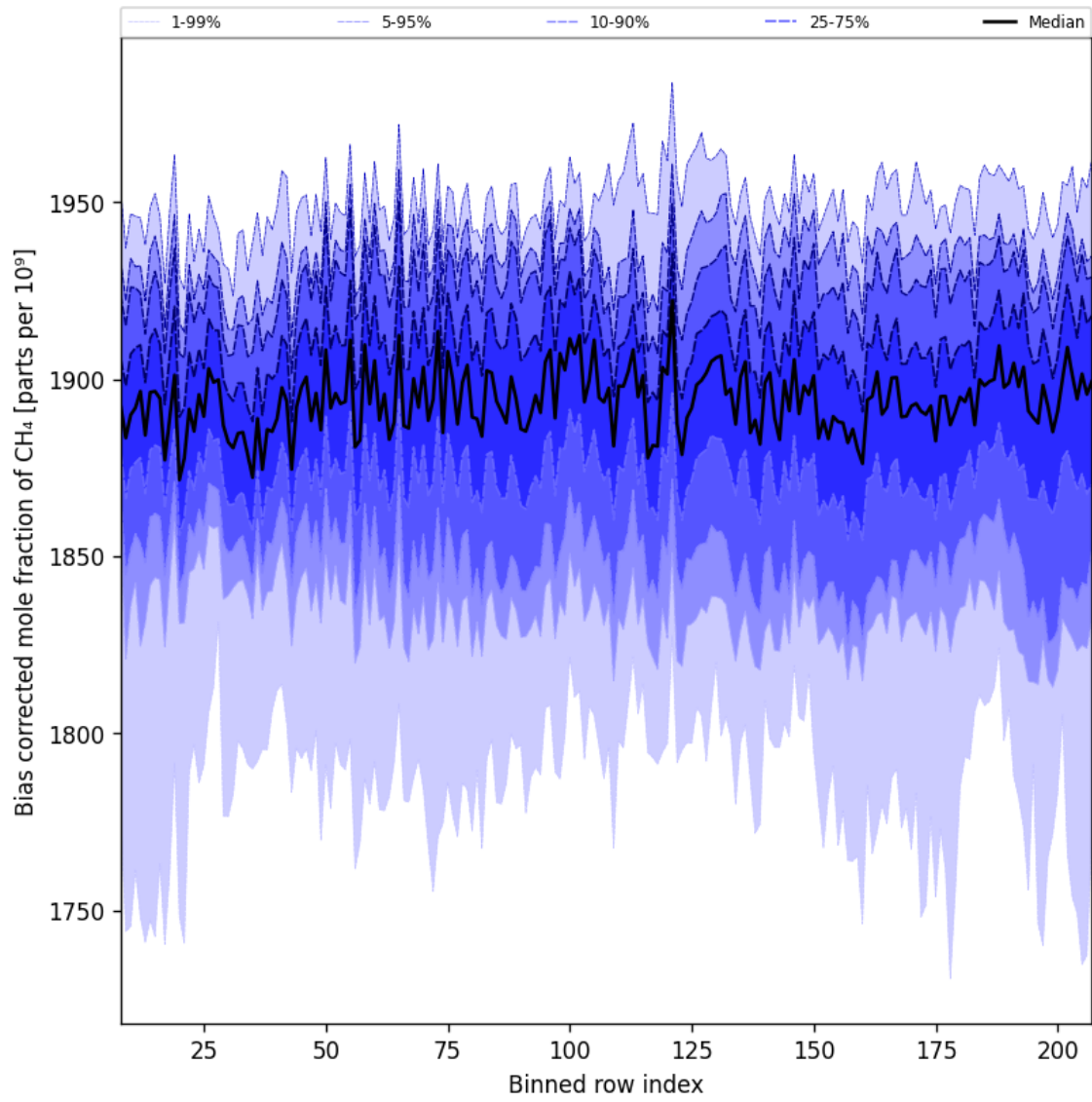
Figure 36: Along track statistics of “Bias corrected mole fraction of CH 4 ” for 2025-04-24 to 2025-04-26
