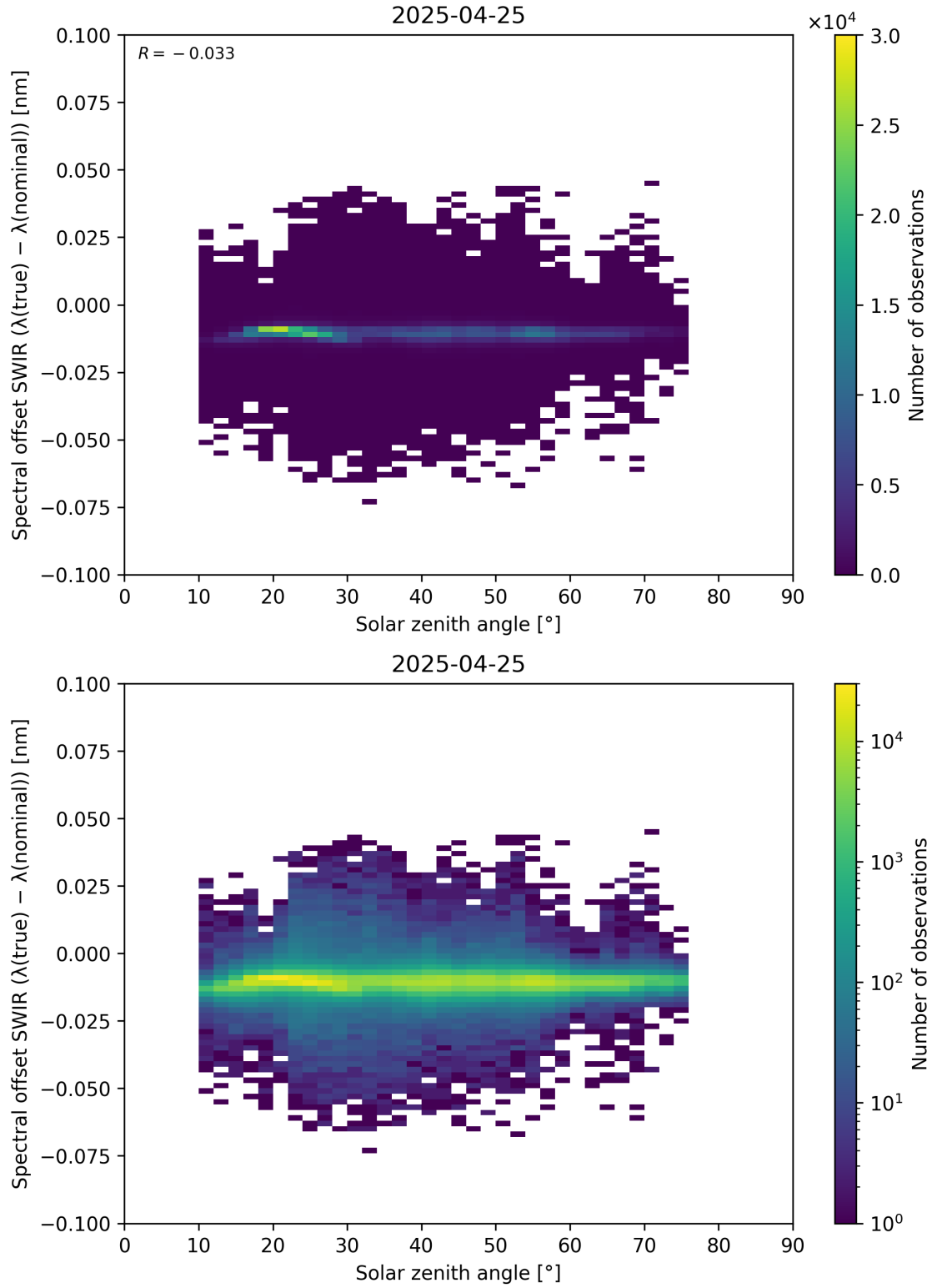
Figure 104: Scatter density plot of “Solar zenith angle” against “Spectral offset SWIR ( \lambda_{\text{true}} - \lambda_{\text{nominal}} )” for 2025-04-24 to 2025-04-26.
