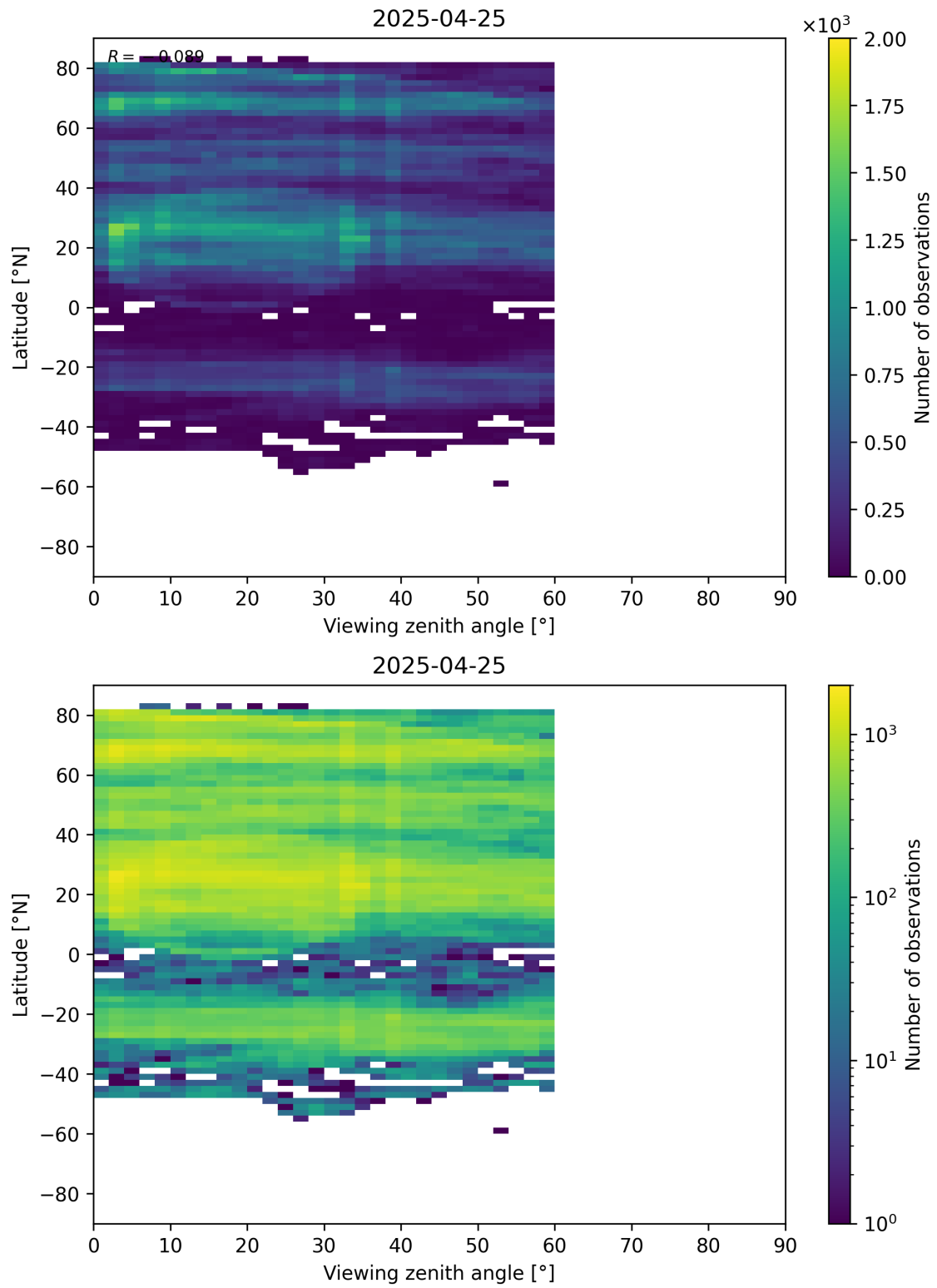
Figure 109: Scatter density plot of “Viewing zenith angle” against “Latitude” for 2025-04-24 to 2025-04-26.
