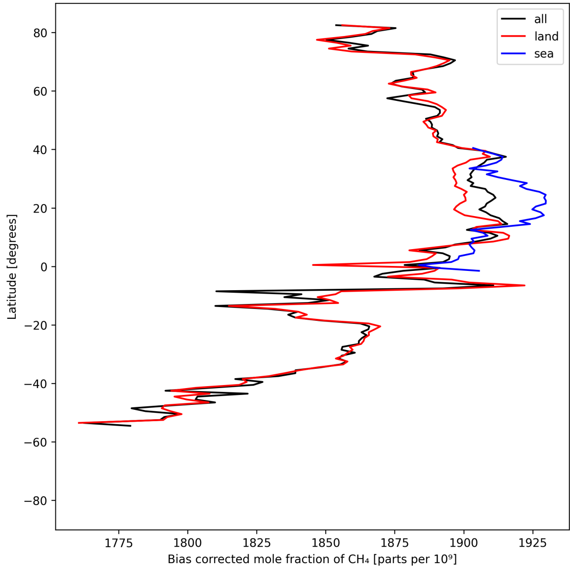
Figure 14: Zonal average of “Bias corrected mole fraction of CH 4 ” for 2025-04-24 to 2025-04-26.
