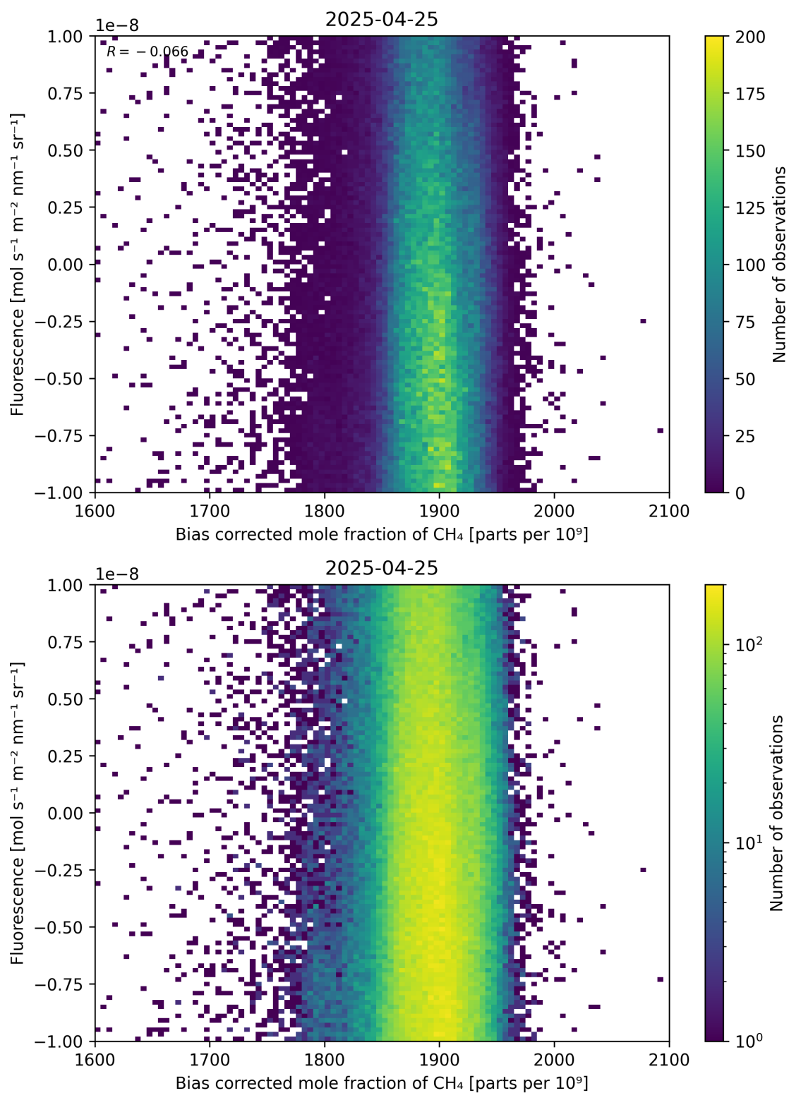
Figure 66: Scatter density plot of “Bias corrected mole fraction of \text{CH}_4 ” against “Fluorescence” for 2025-04-24 to 2025-04-26.
