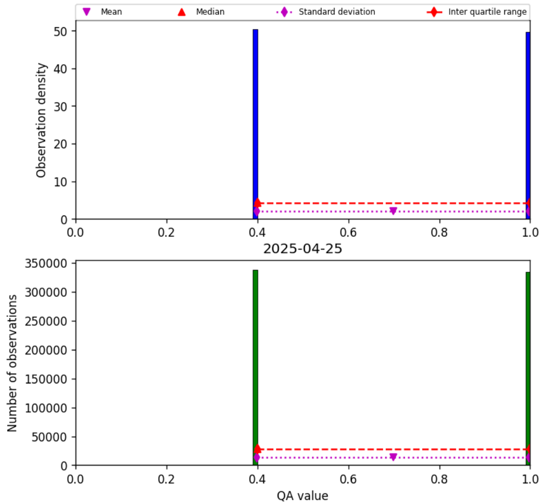
Figure 22: Histogram of “QA value” for 2025-04-24 to 2025-04-26
