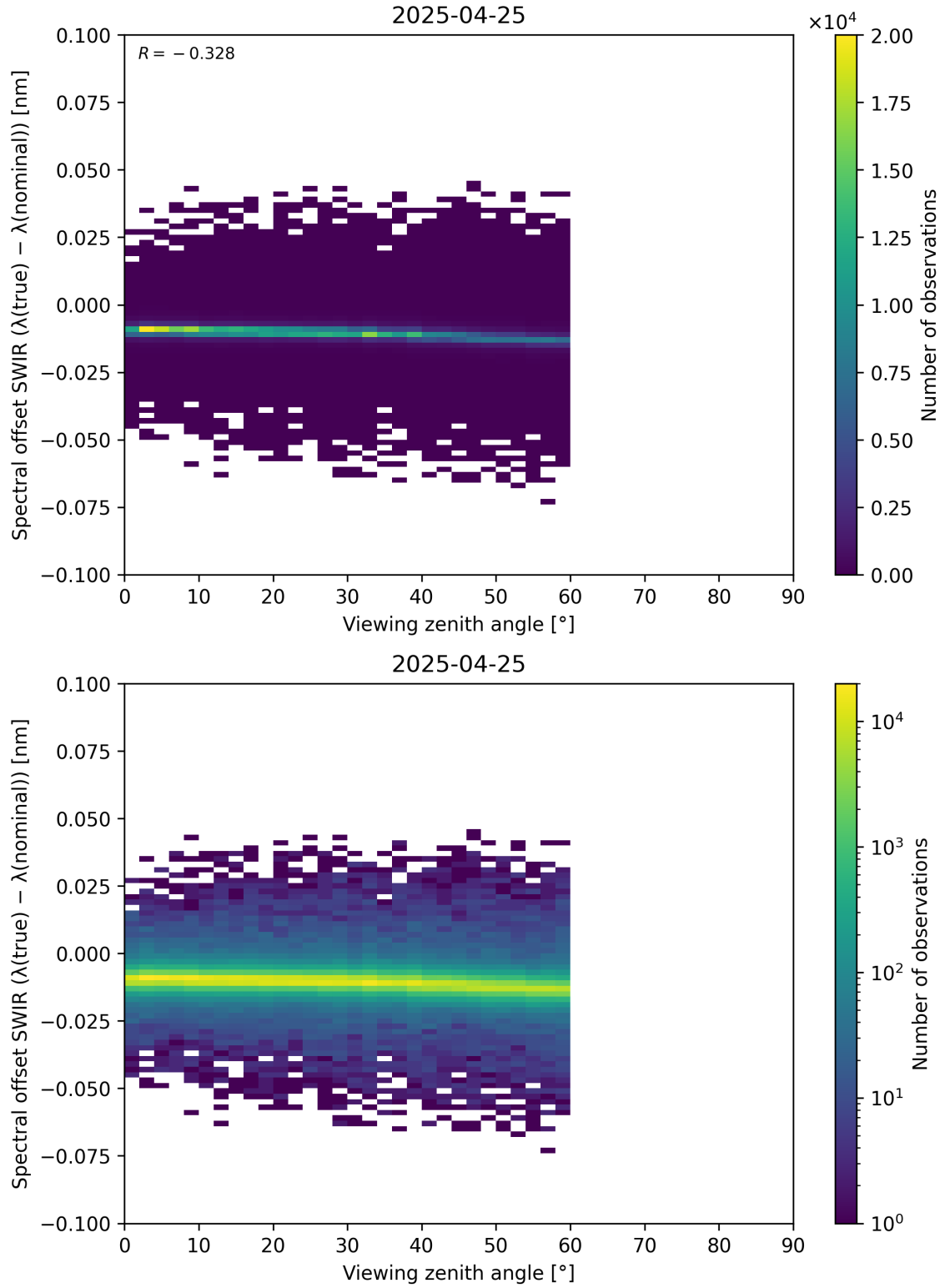
Figure 116: Scatter density plot of “Viewing zenith angle” against “Spectral offset SWIR ( \lambda_{\text{true}} - \lambda_{\text{nominal}} )” for 2025-04-24 to 2025-04-26.
