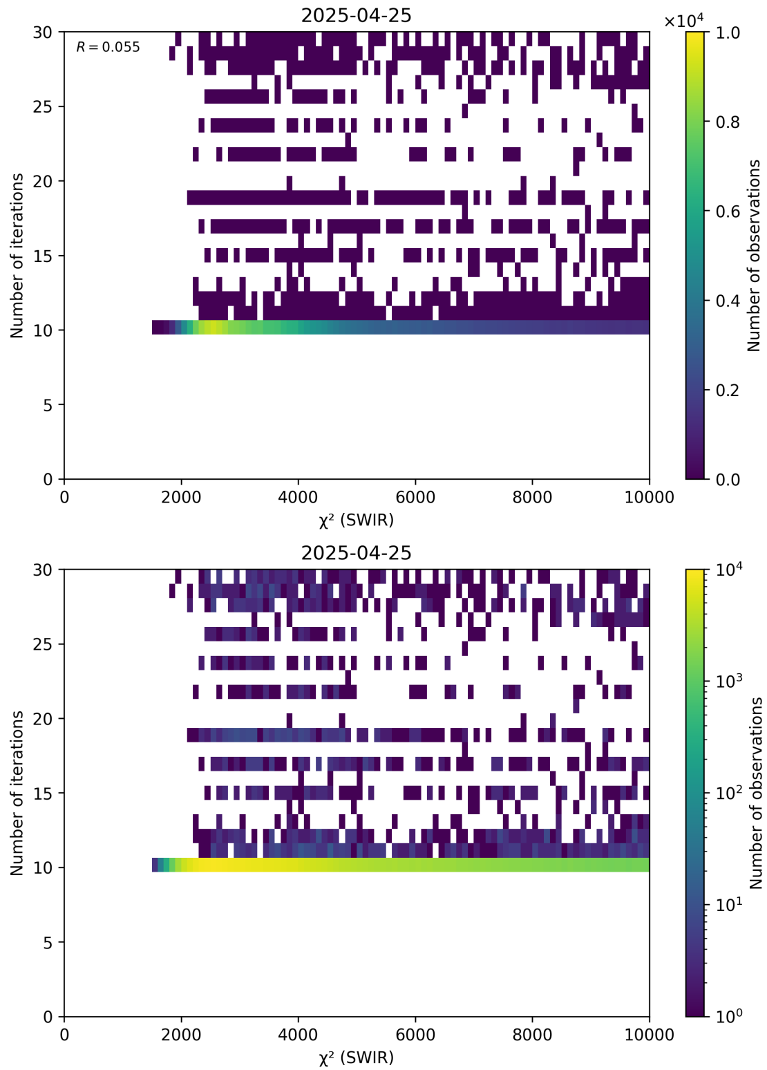
Figure 50: Scatter density plot of “ \chi^2 (SWIR)” against “Number of iterations” for 2025-04-24 to 2025-04-26.
