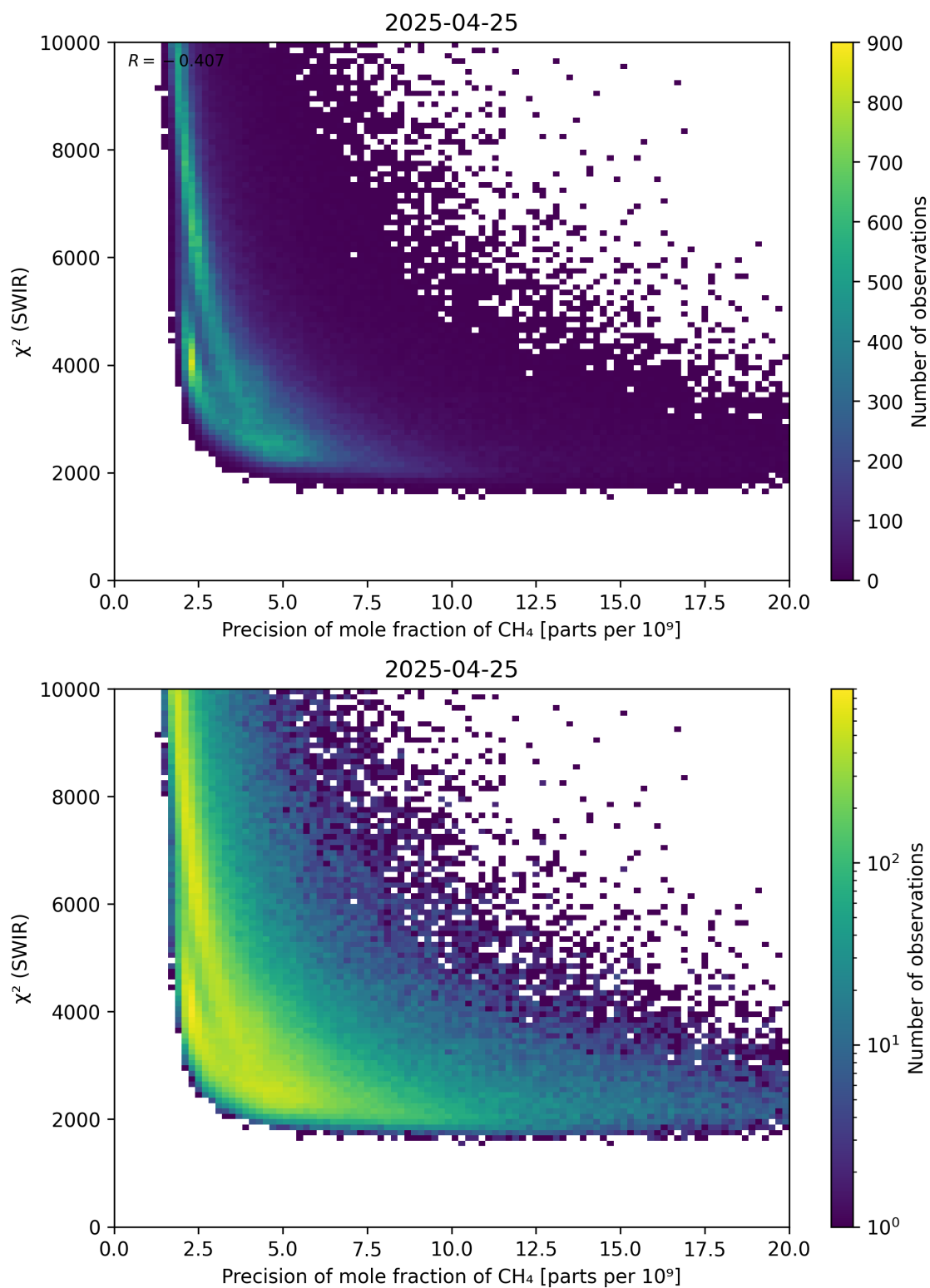
Figure 79: Scatter density plot of “Precision of mole fraction of \text{CH}_4 ” against “ \chi^2 (SWIR)” for 2025-04-24 to 2025-04-26.
