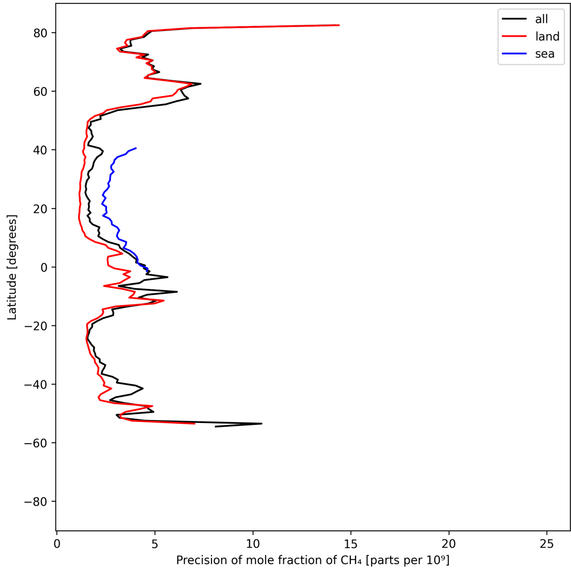
Figure 13: Zonal average of “Precision of mole fraction of CH 4 ” for 2025-04-24 to 2025-04-26.
