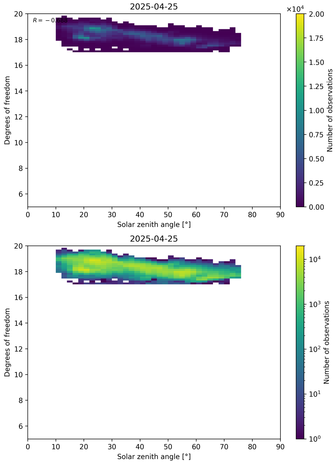
Figure 96: Scatter density plot of “Solar zenith angle” against “Degrees of freedom” for 2025-04-24 to 2025-04-26.
