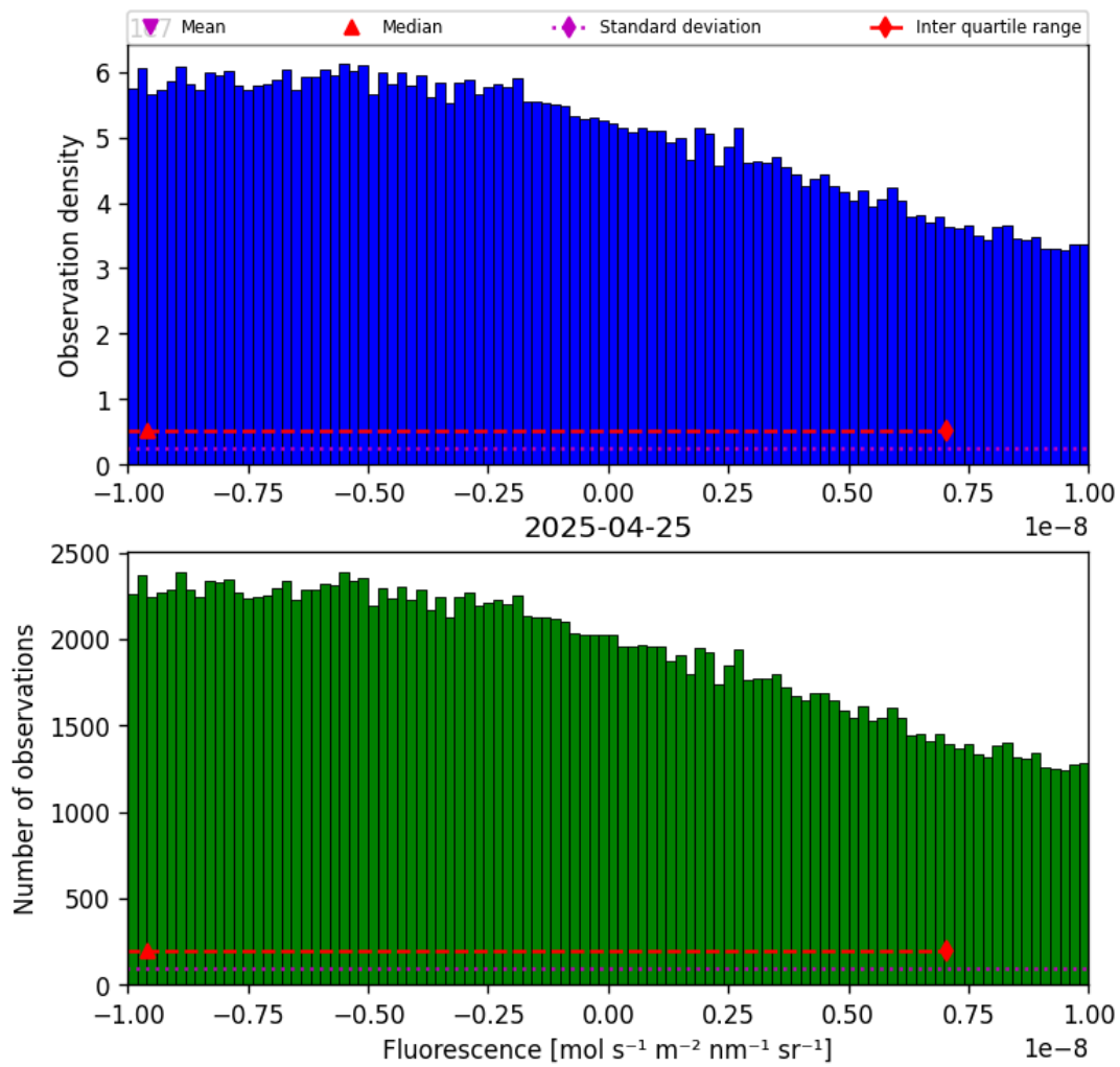
Figure 32: Histogram of “Fluorescence” for 2025-04-24 to 2025-04-26
