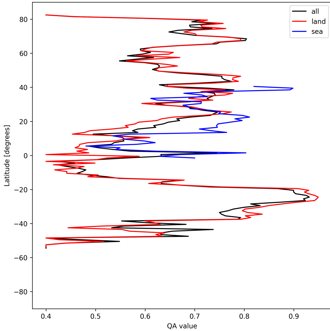
Figure 11: Zonal average of “QA value” for 2025-04-24 to 2025-04-26.
