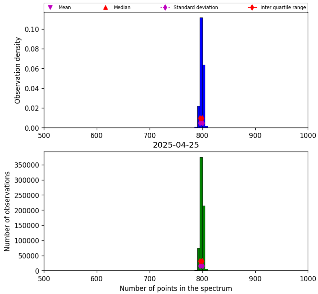
Figure 26: Histogram of “Number of points in the spectrum” for 2025-04-24 to 2025-04-26
