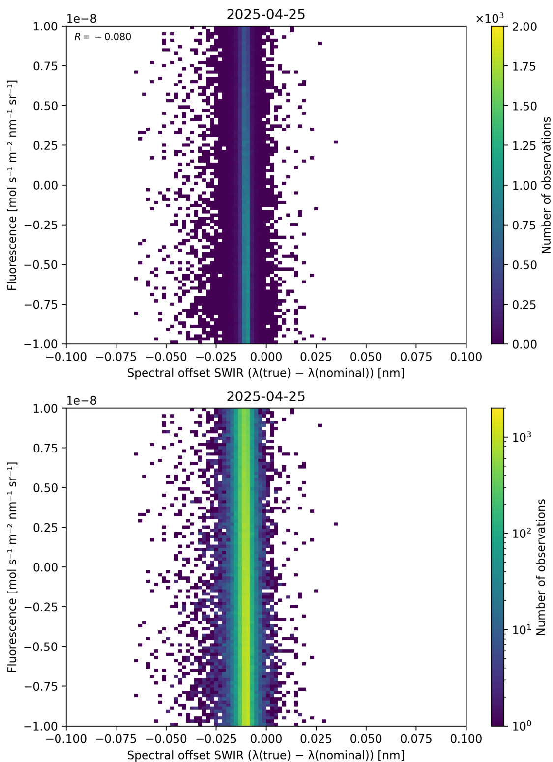
Figure 120: Scatter density plot of “Spectral offset SWIR ( \lambda_{\text{true}} - \lambda_{\text{nominal}} )” against “Fluorescence” for 2025-04-24 to 2025-04-26.
