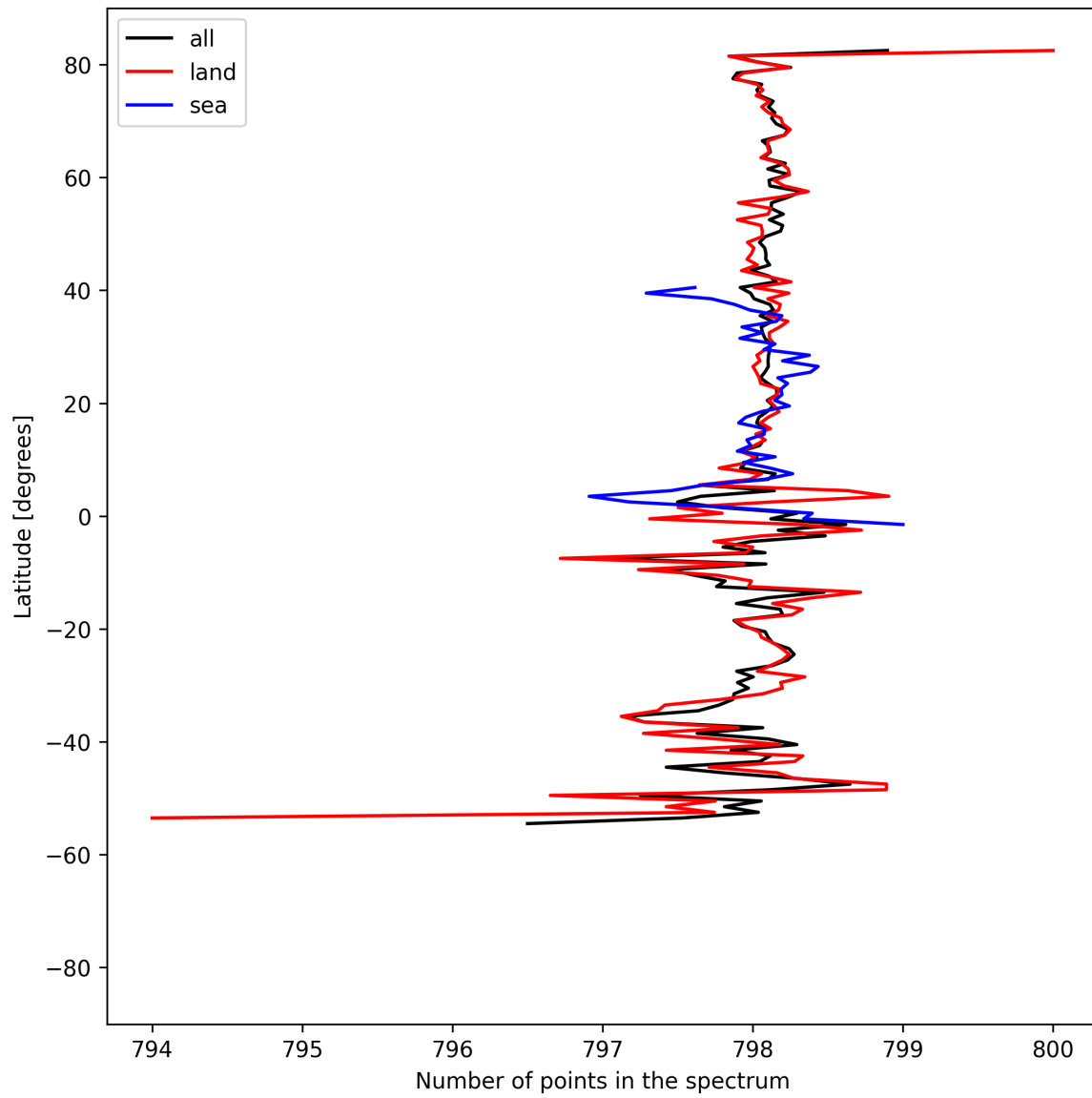
Figure 15: Zonal average of “Number of points in the spectrum” for 2025-04-24 to 2025-04-26.
