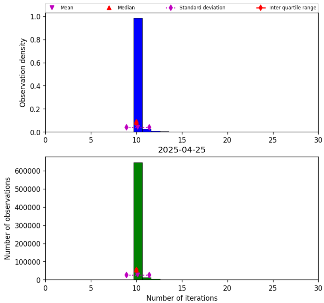
Figure 31: Histogram of “Number of iterations” for 2025-04-24 to 2025-04-26
