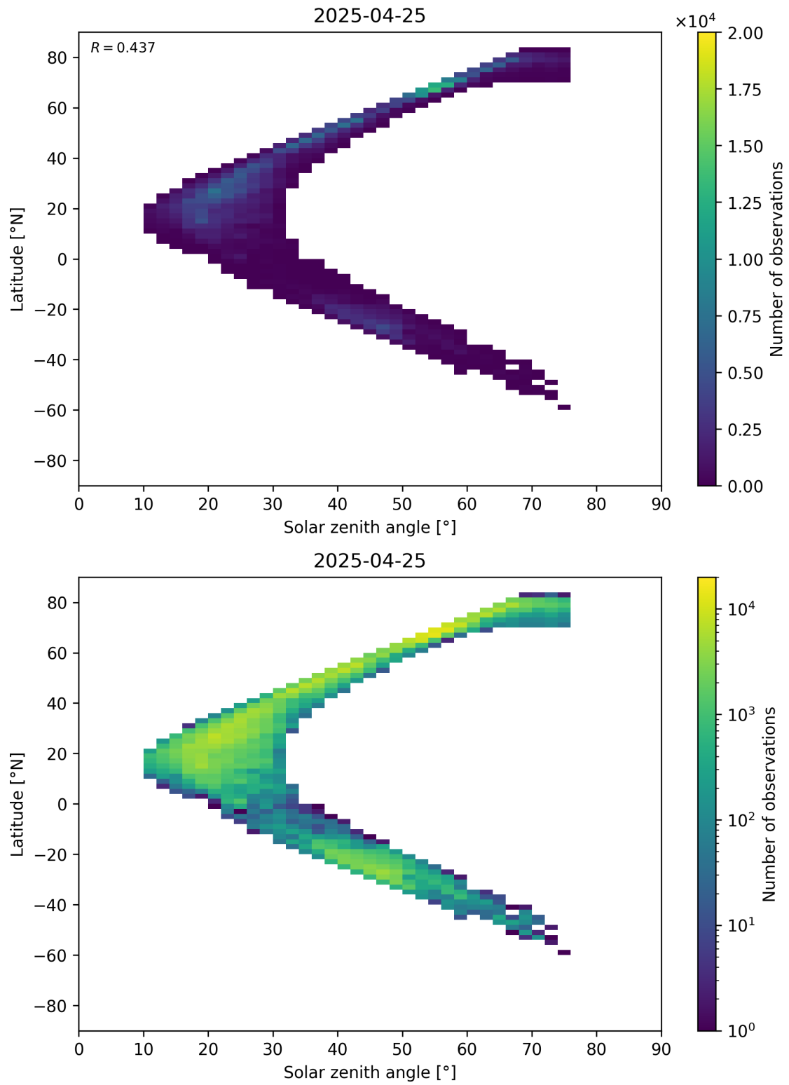
Figure 98: Scatter density plot of “Solar zenith angle” against “Latitude” for 2025-04-24 to 2025-04-26.
