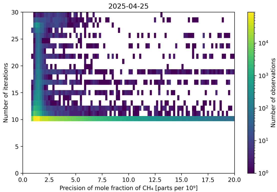
Figure 83: Scatter density plot of “Precision of mole fraction of CH 4 ” against “Number of iterations” for 2025-04-24 to 2025-04-26.
