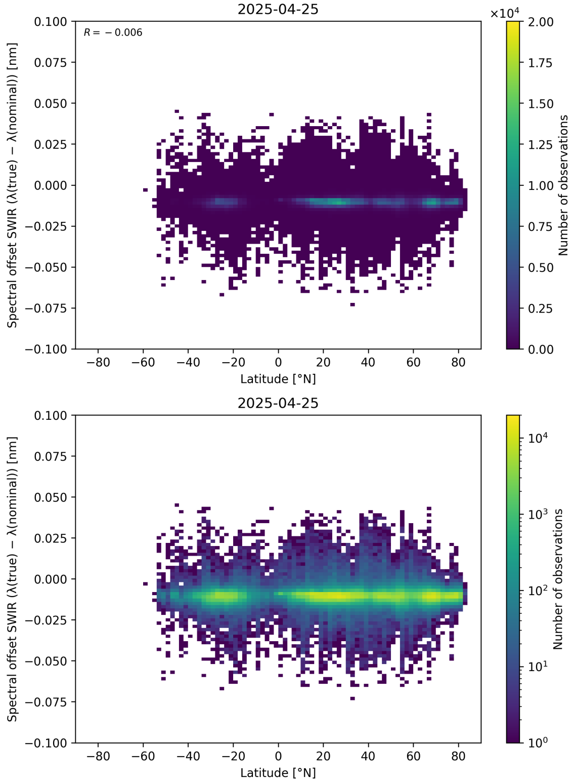
Figure 62: Scatter density plot of “Latitude” against “Spectral offset SWIR ( \lambda_{\text{true}} - \lambda_{\text{nominal}} )” for 2025-04-24 to 2025-04-26.
