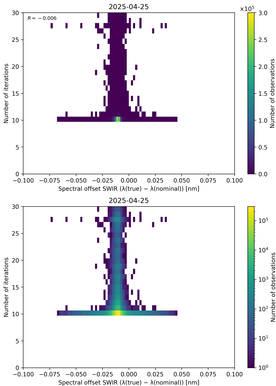
Figure 121: Scatter density plot of “Spectral offset SWIR ( \lambda_{\text{true}} - \lambda_{\text{nominal}} )” against “Number of iterations” for 2025-04-24 to 2025-04-26.
