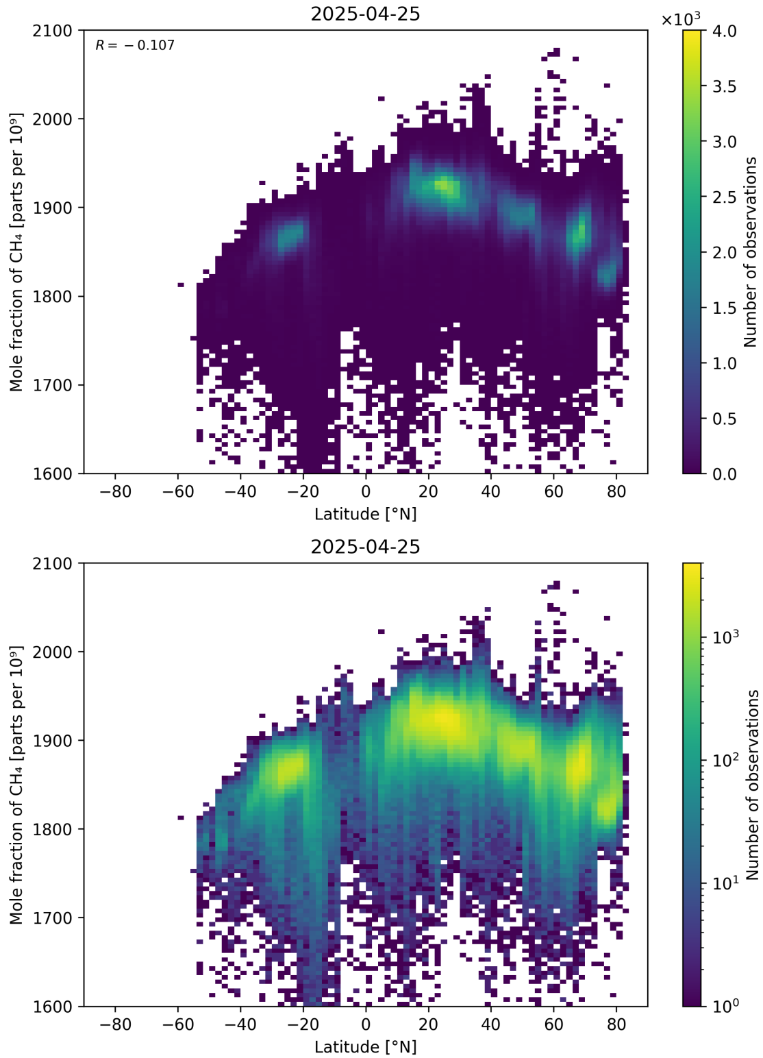
Figure 57: Scatter density plot of “Latitude” against “Mole fraction of \text{CH}_4 ” for 2025-04-24 to 2025-04-26.
