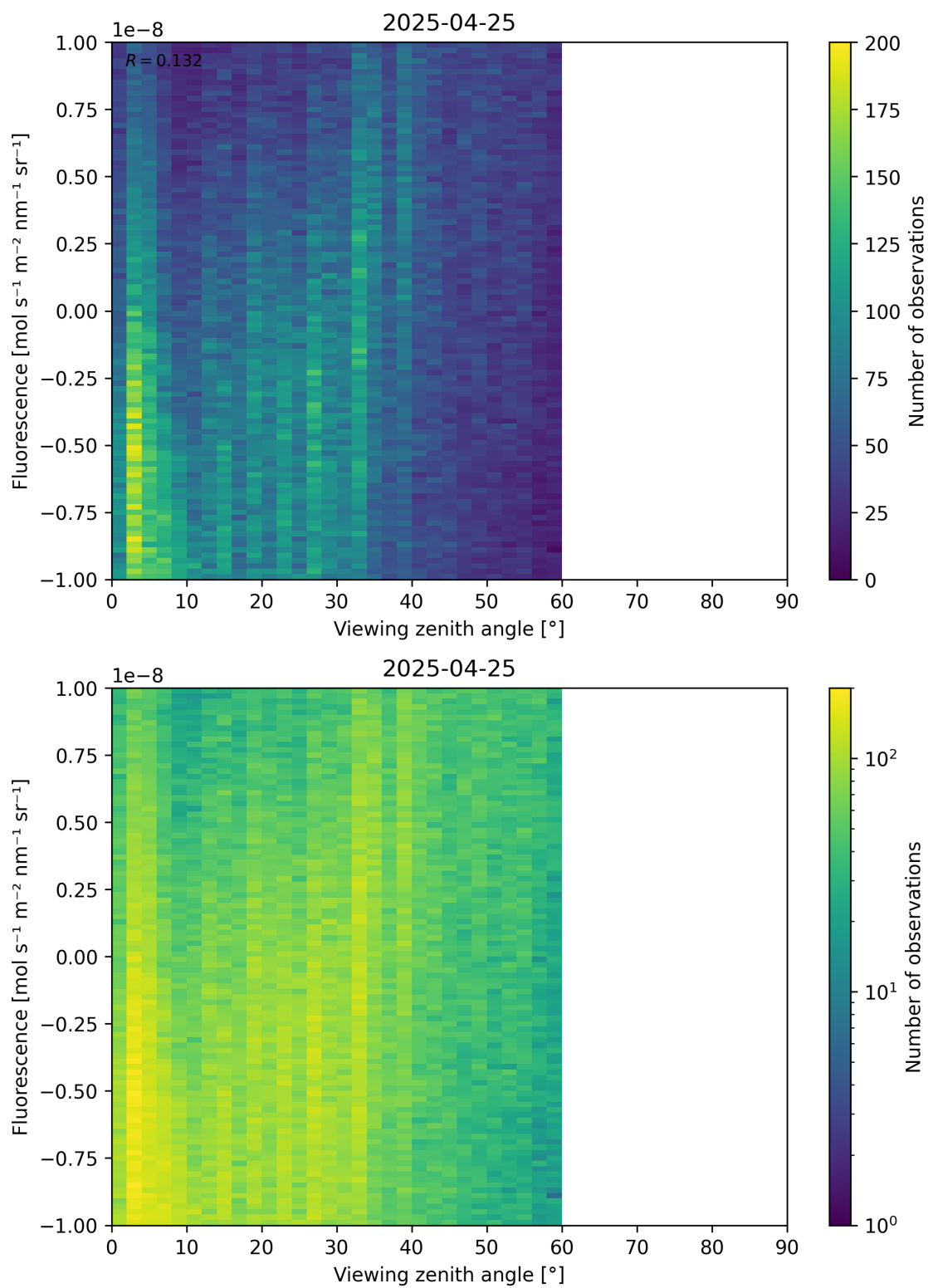
Figure 108: Scatter density plot of “Viewing zenith angle” against “Fluorescence” for 2025-04-24 to 2025-04-26.
