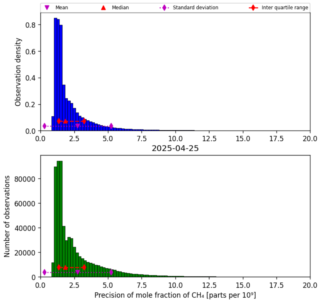
Figure 24: Histogram of “Precision of mole fraction of CH 4 ” for 2025-04-24 to 2025-04-26
