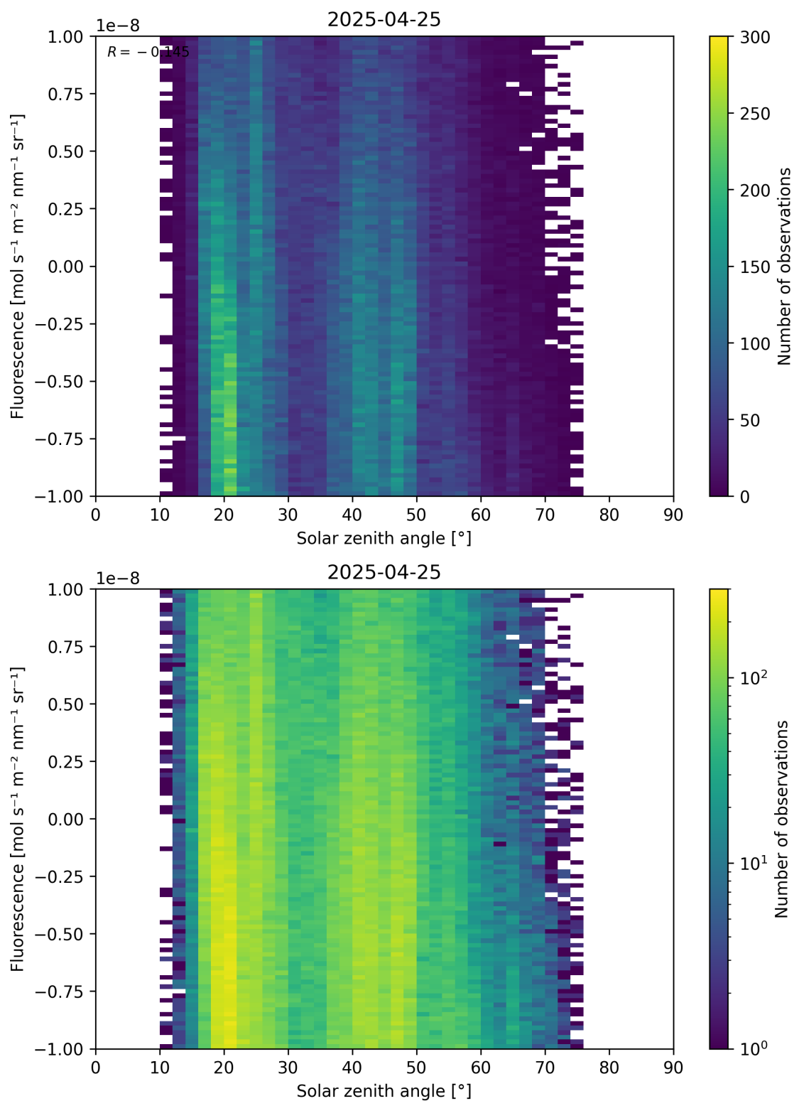
Figure 97: Scatter density plot of “Solar zenith angle” against “Fluorescence” for 2025-04-24 to 2025-04-26.
