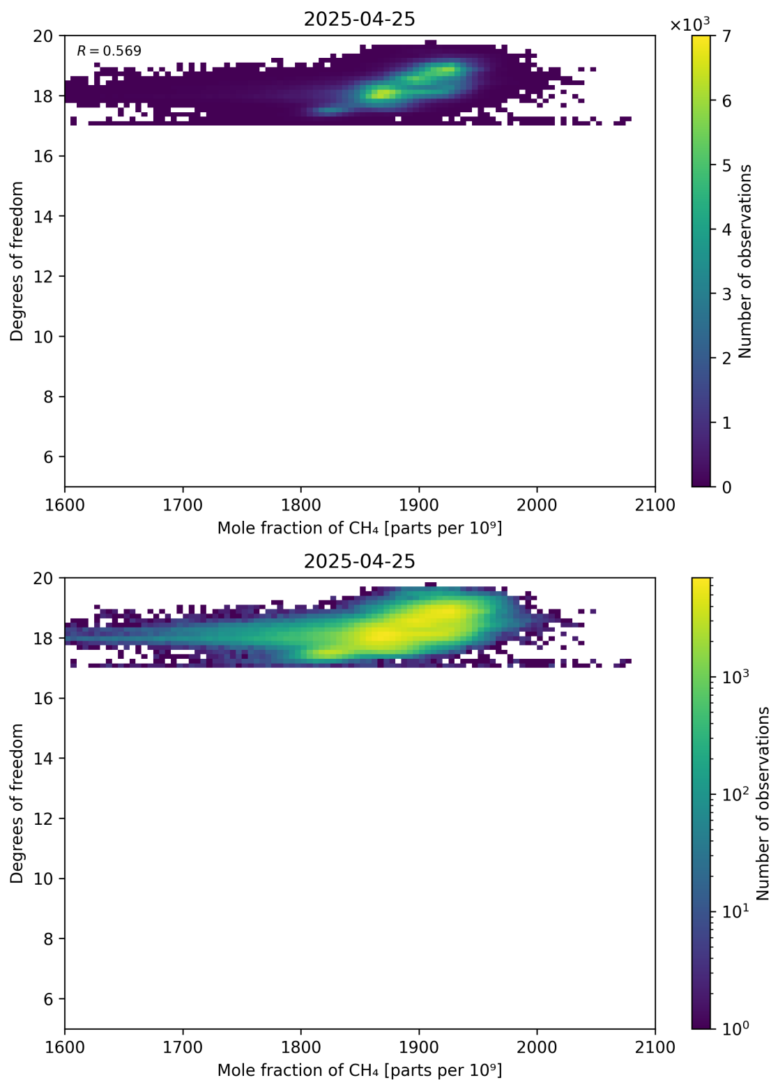
Figure 72: Scatter density plot of “Mole fraction of CH 4 ” against “Degrees of freedom” for 2025-04-24 to 2025-04-26.
