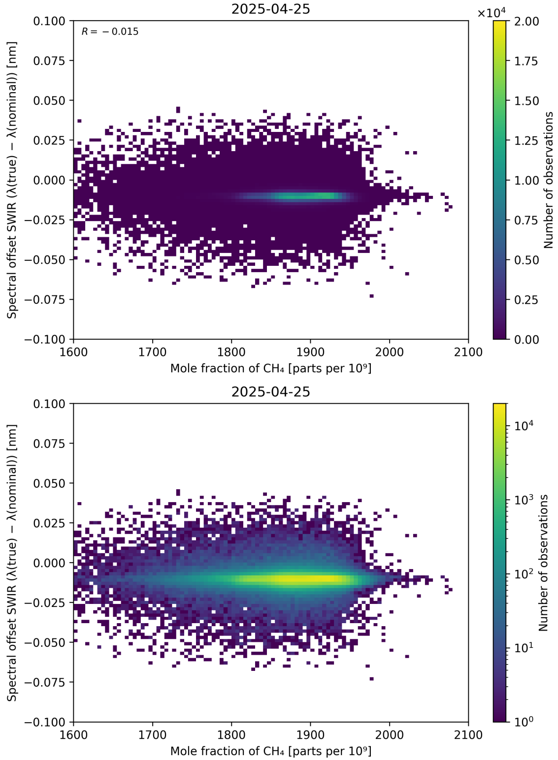
Figure 86: Scatter density plot of “Mole fraction of CH 4 ” against “Spectral offset SWIR ( \lambda_{\text{true}} - \lambda_{\text{nominal}} )” for 2025-04-24 to 2025-04-26.
