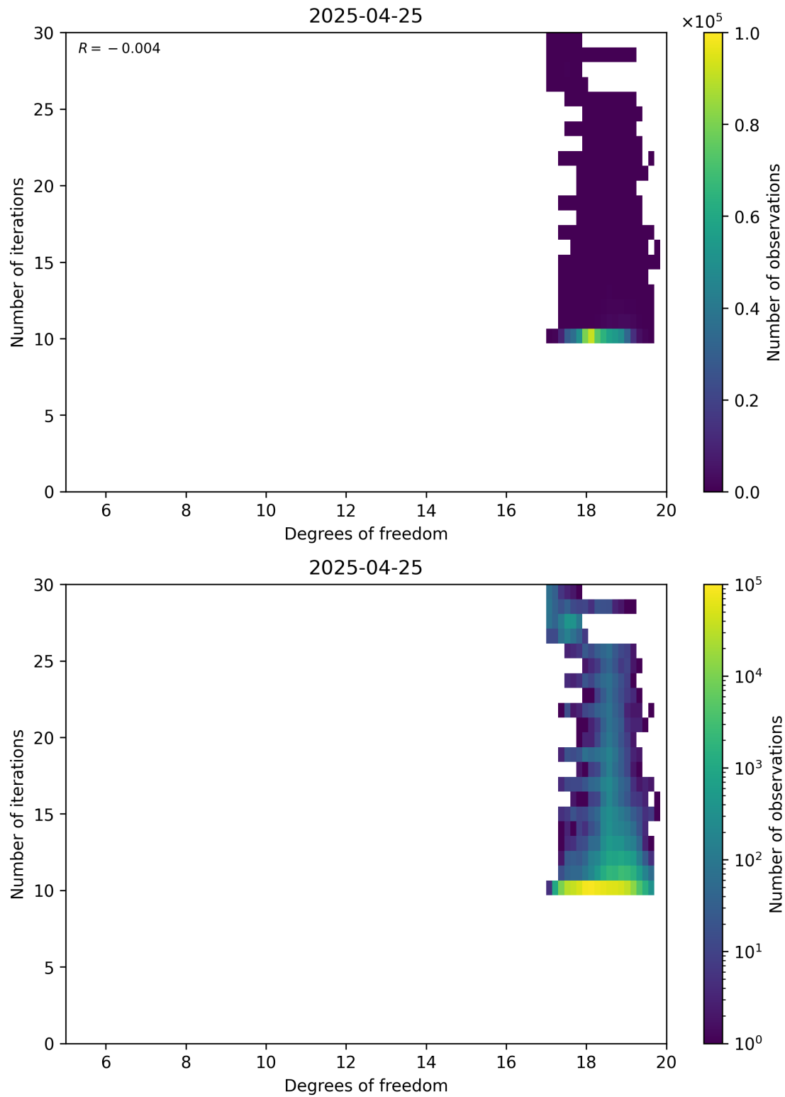
Figure 52: Scatter density plot of “Degrees of freedom” against “Number of iterations” for 2025-04-24 to 2025-04-26.
