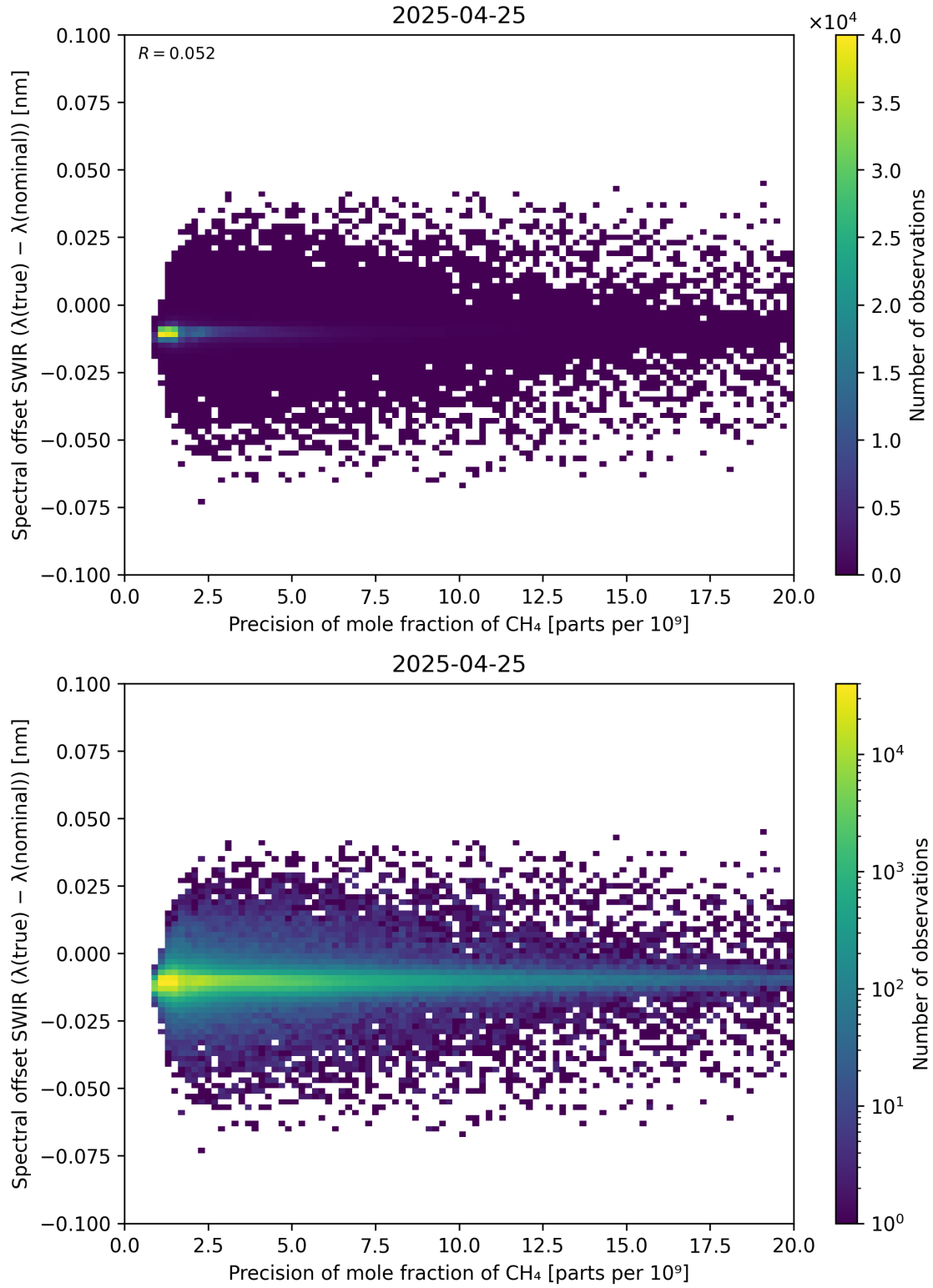
Figure 85: Scatter density plot of “Precision of mole fraction of \text{CH}_4 ” against “Spectral offset SWIR ( \lambda_{\text{true}} - \lambda_{\text{nominal}} )” for 2025-04-24 to 2025-04-26.
