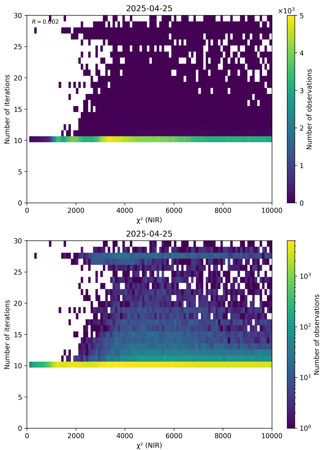
Figure 46: Scatter density plot of “ \chi^2 (NIR)” against “Number of iterations” for 2025-04-24 to 2025-04-26.
