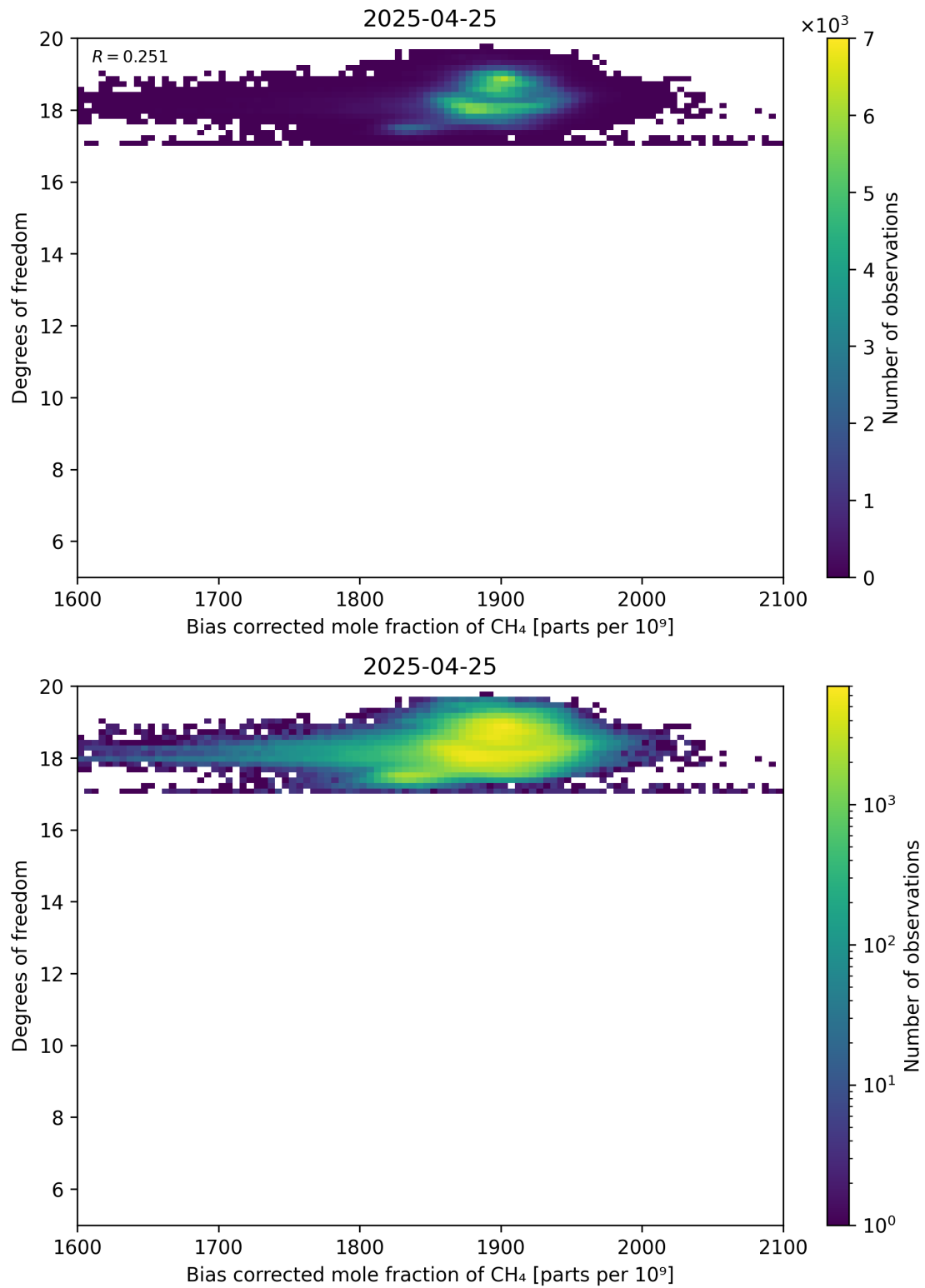
Figure 65: Scatter density plot of “Bias corrected mole fraction of CH 4 ” against “Degrees of freedom” for 2025-04-24 to 2025-04-26.
