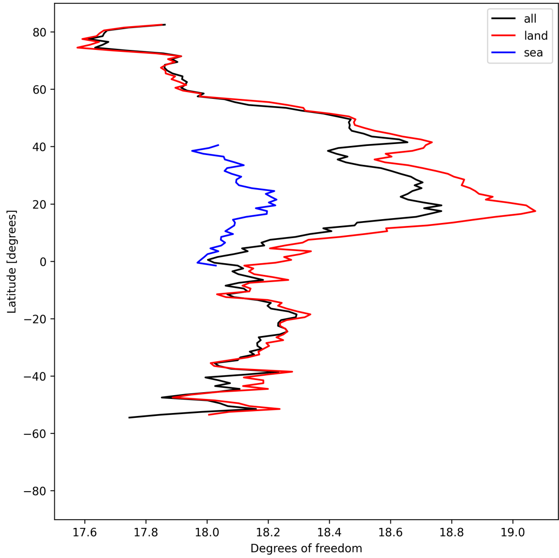
Figure 19: Zonal average of “Degrees of freedom” for 2025-04-24 to 2025-04-26.
