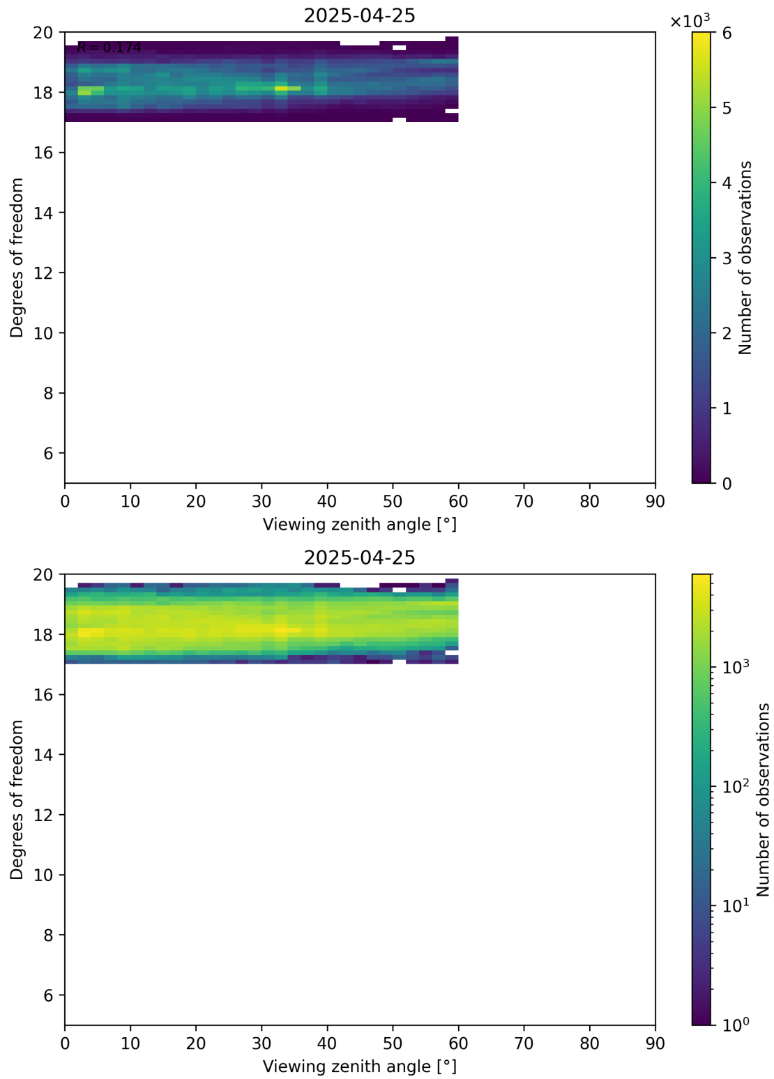
Figure 107: Scatter density plot of “Viewing zenith angle” against “Degrees of freedom” for 2025-04-24 to 2025-04-26.
