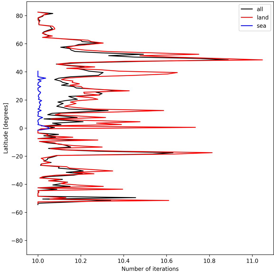
Figure 20: Zonal average of “Number of iterations” for 2025-04-24 to 2025-04-26.
