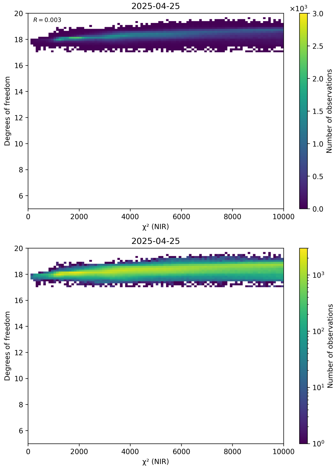
Figure 44: Scatter density plot of “ \chi^2 (NIR)” against “Degrees of freedom” for 2025-04-24 to 2025-04-26.
