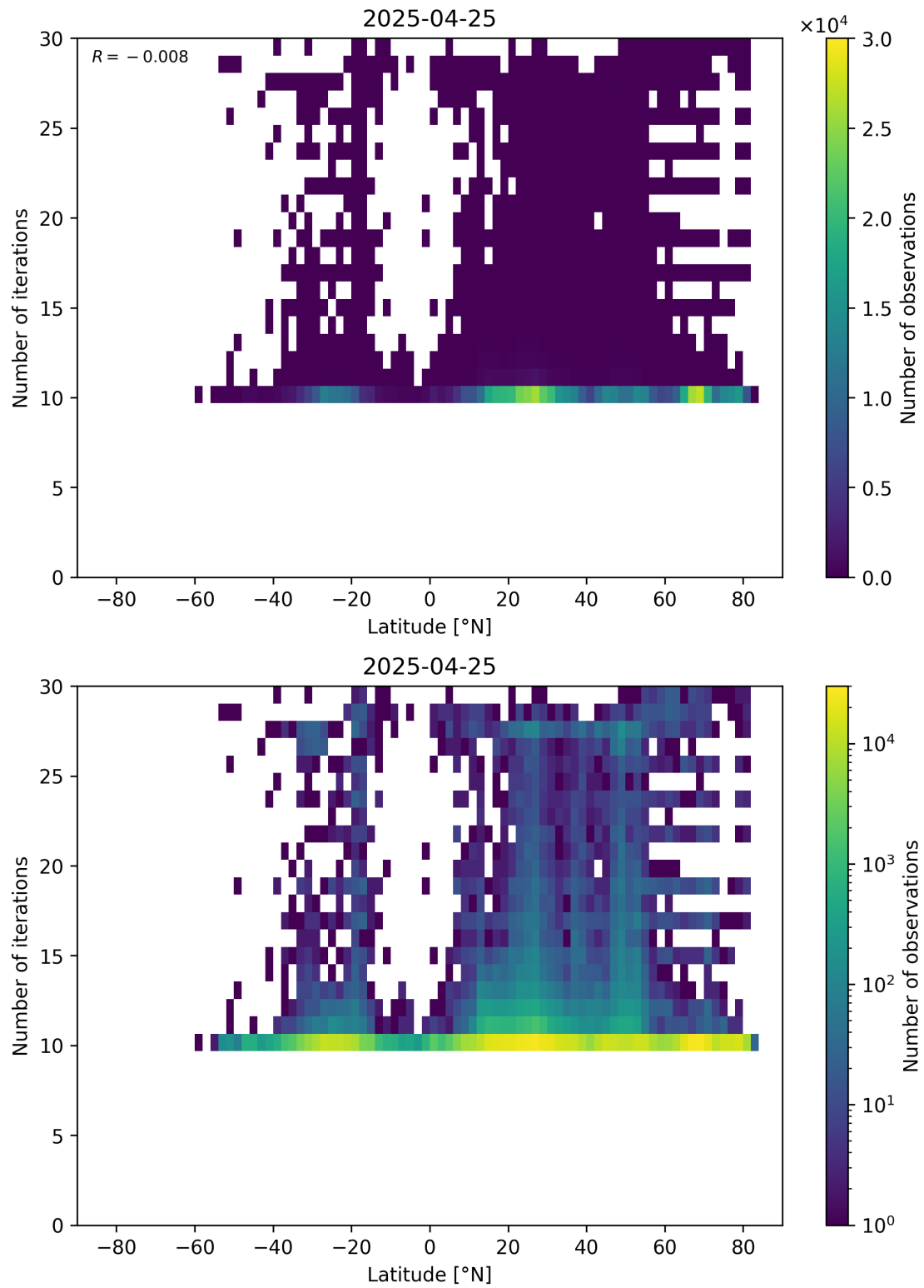
Figure 60: Scatter density plot of “Latitude” against “Number of iterations” for 2025-04-24 to 2025-04-26.
