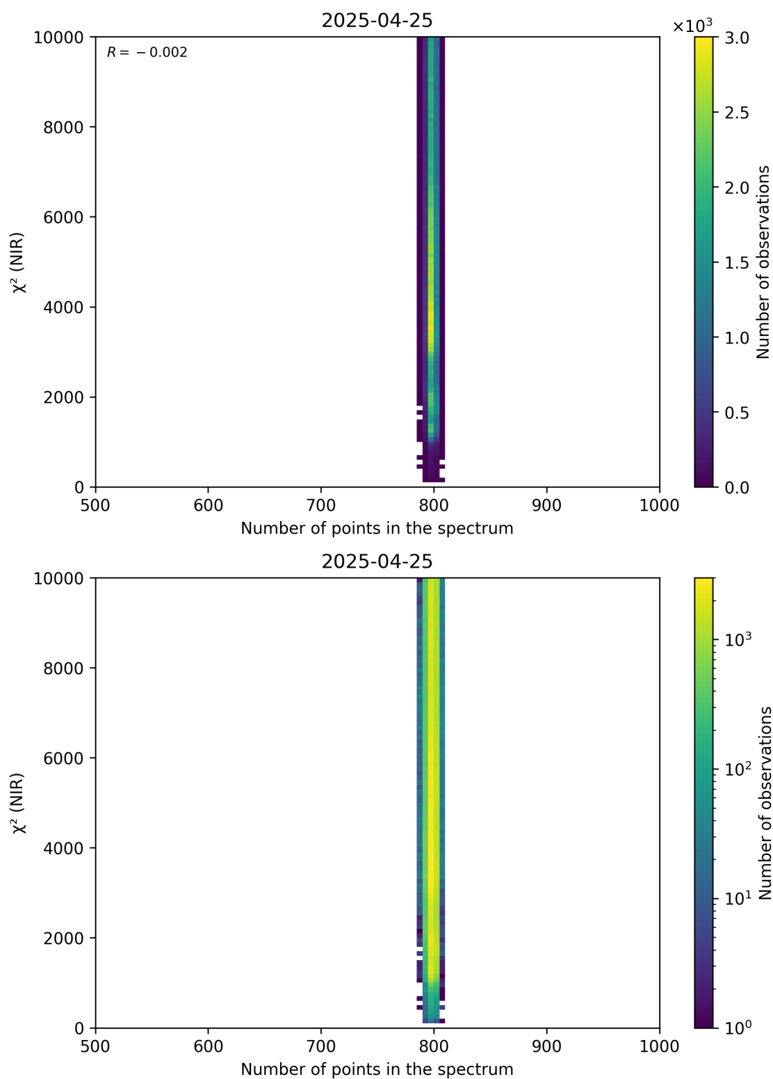
Figure 88: Scatter density plot of “Number of points in the spectrum” against “ \chi^2 (NIR)” for 2025-04-24 to 2025-04-26.
