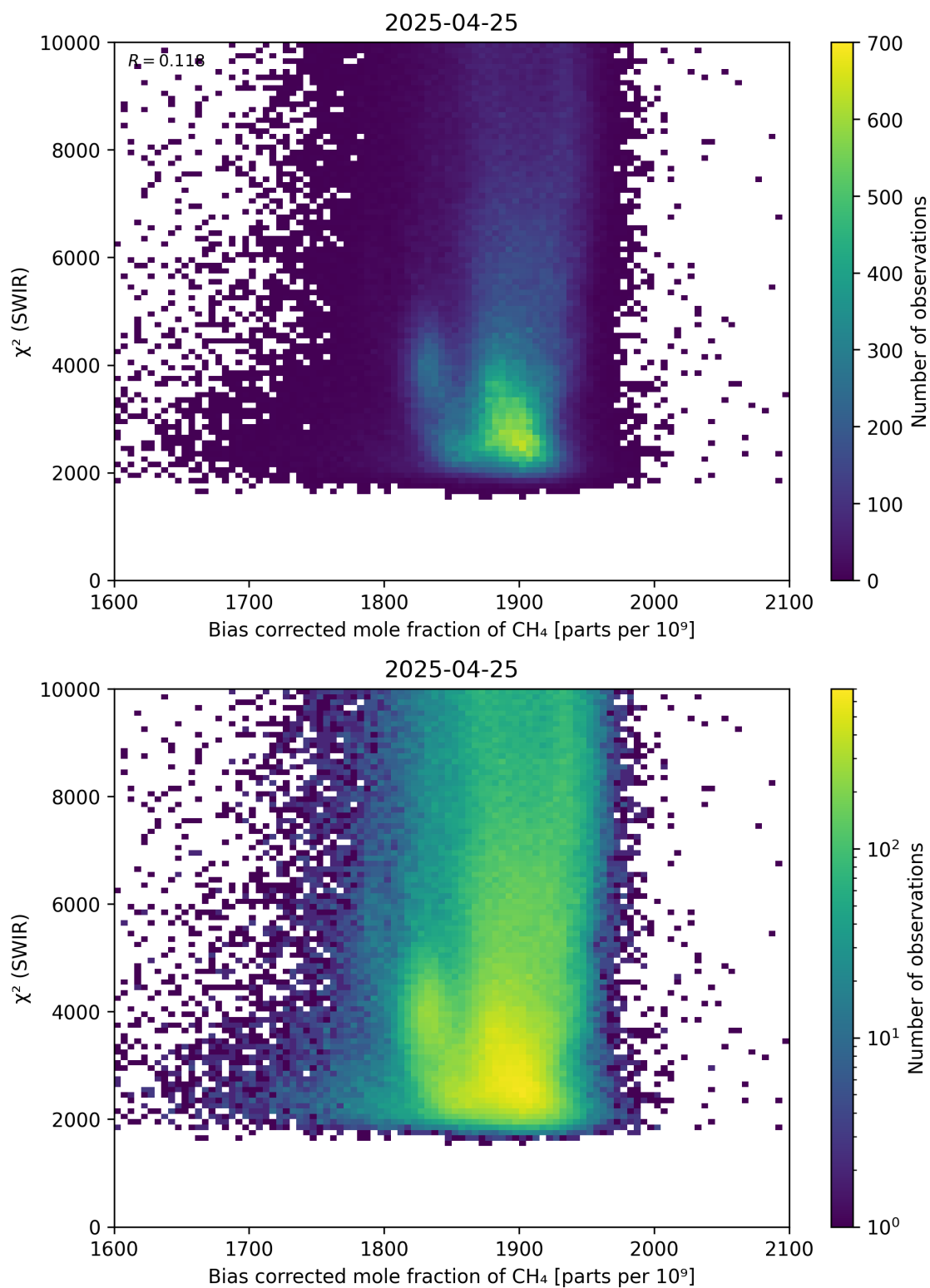
Figure 64: Scatter density plot of “Bias corrected mole fraction of \text{CH}_4 ” against “ \chi^2 (SWIR)” for 2025-04-24 to 2025-04-26.
