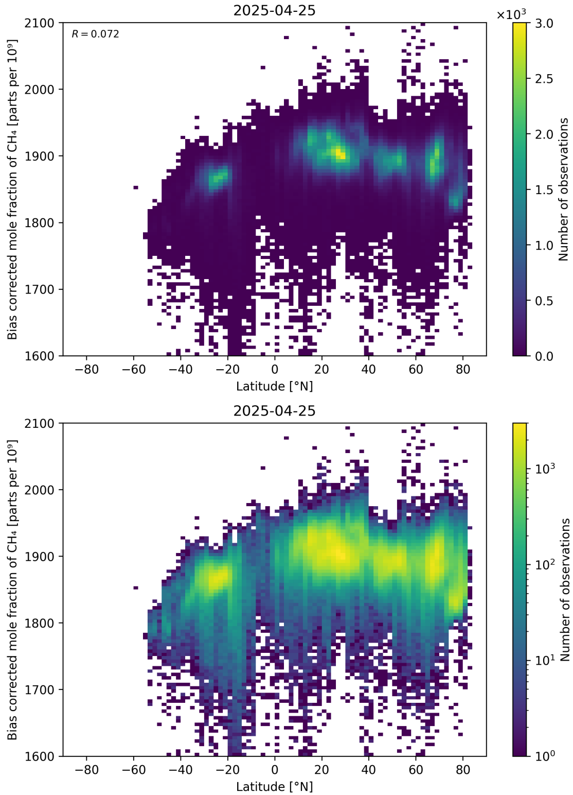
Figure 58: Scatter density plot of “Latitude” against “Bias corrected mole fraction of CH 4 ” for 2025-04-24 to 2025-04-26.
