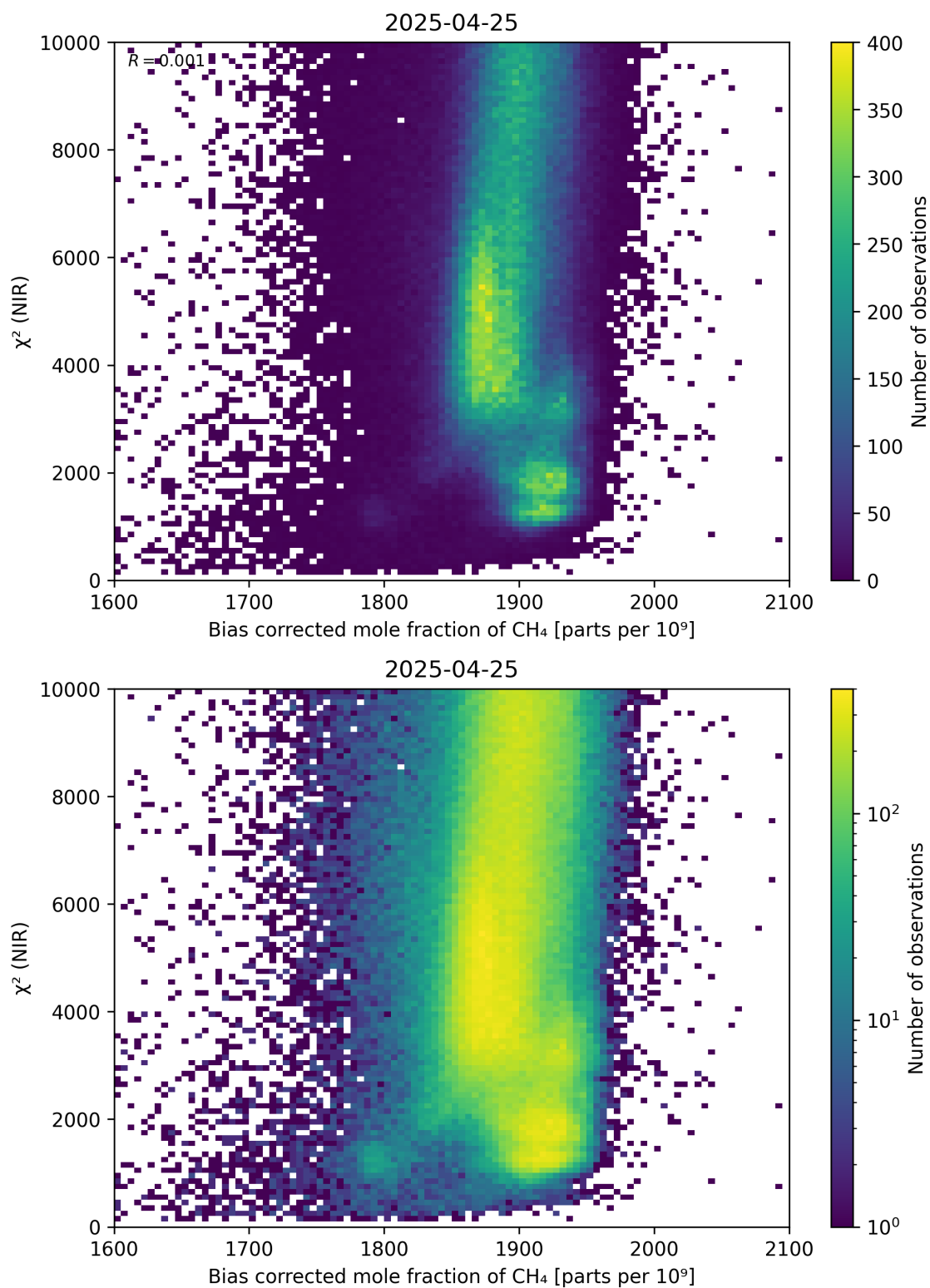
Figure 63: Scatter density plot of “Bias corrected mole fraction of CH 4 ” against “ \chi^2 (NIR)” for 2025-04-24 to 2025-04-26.
