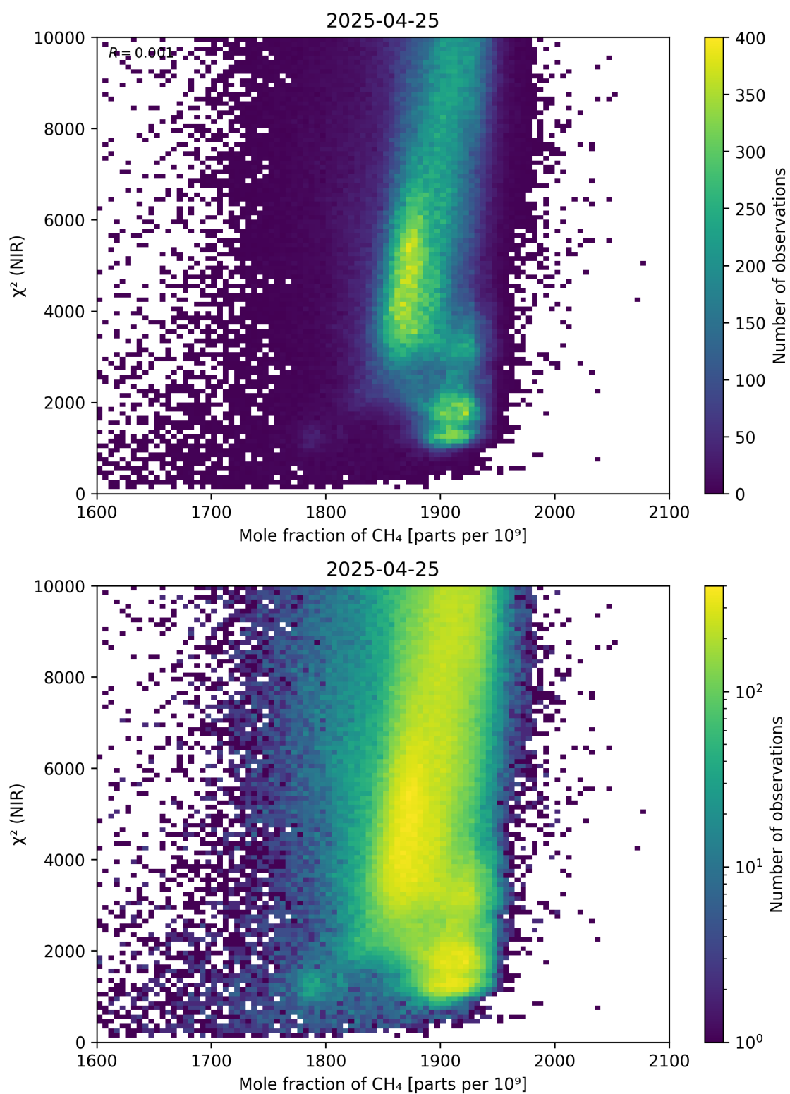
Figure 70: Scatter density plot of “Mole fraction of \text{CH}_4 ” against “ \chi^2 (NIR)” for 2025-04-24 to 2025-04-26.
