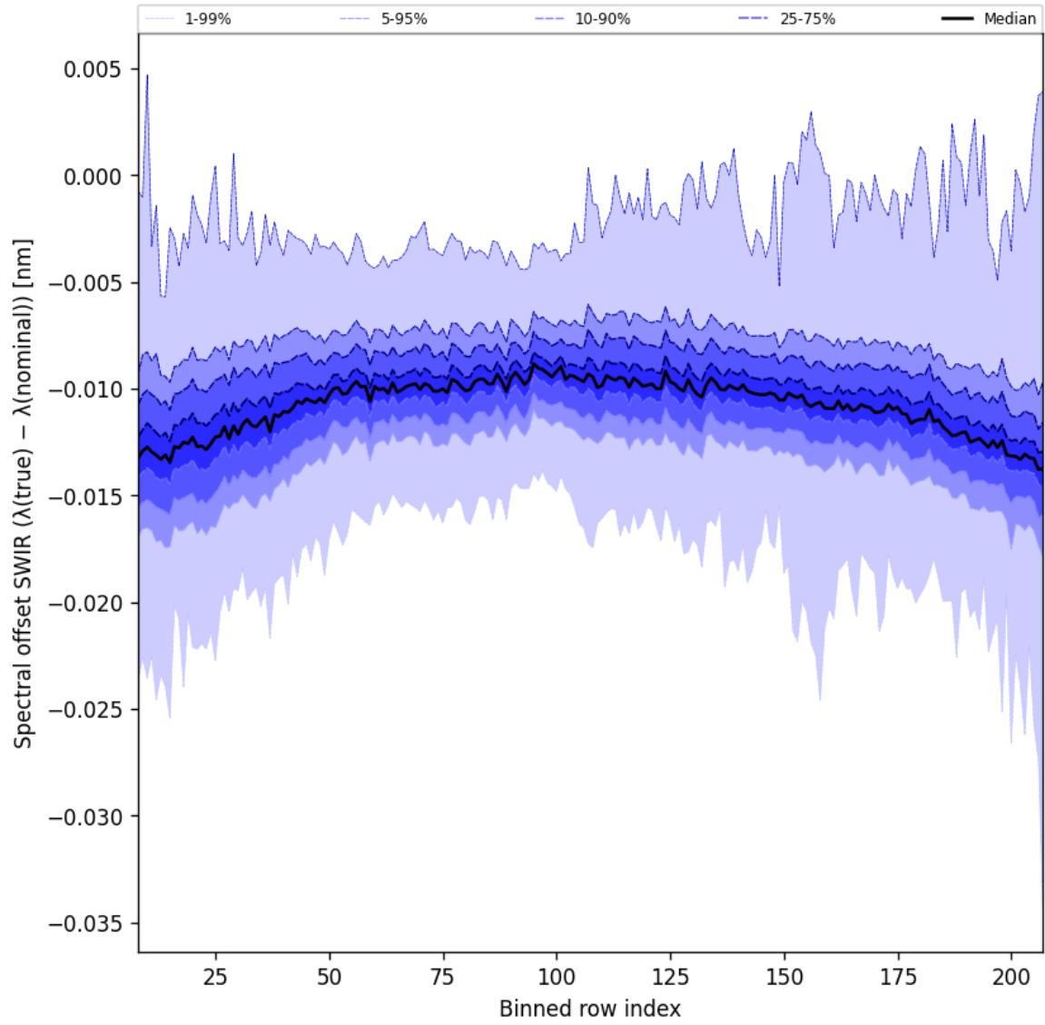
Figure 38: Along track statistics of “Spectral offset SWIR ( \lambda_{\text{true}} - \lambda_{\text{nominal}} )” for 2025-04-24 to 2025-04-26
