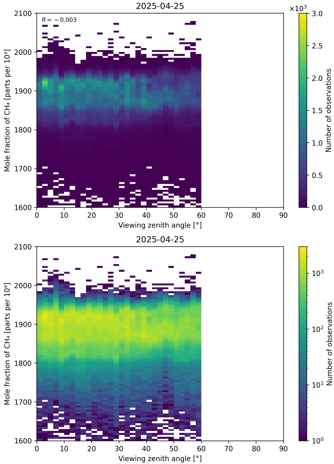
Figure 110: Scatter density plot of “Viewing zenith angle” against “Mole fraction of CH 4 ” for 2025-04-24 to 2025-04-26.
