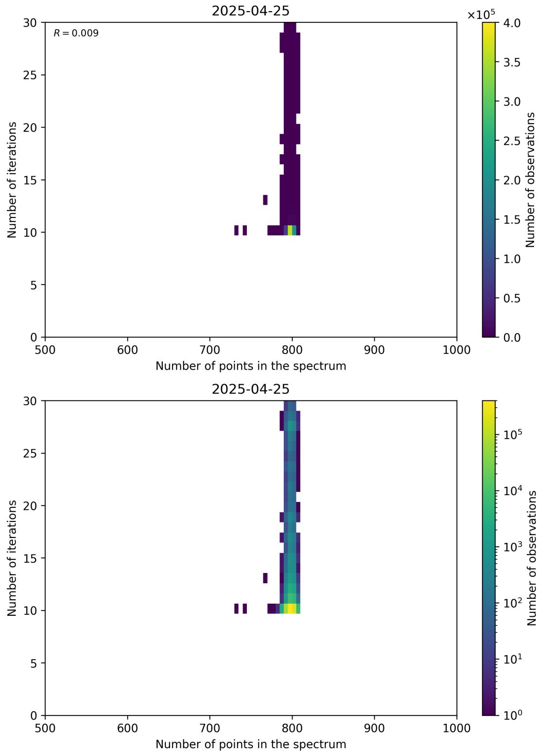
Figure 92: Scatter density plot of “Number of points in the spectrum” against “Number of iterations” for 2025-04-24 to 2025-04-26.
