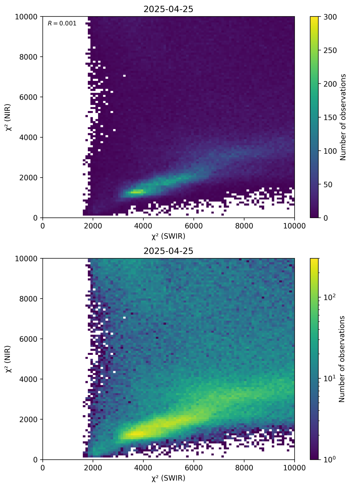
Figure 47: Scatter density plot of “ \chi^2 (SWIR)” against “ \chi^2 (NIR)” for 2025-04-24 to 2025-04-26.
