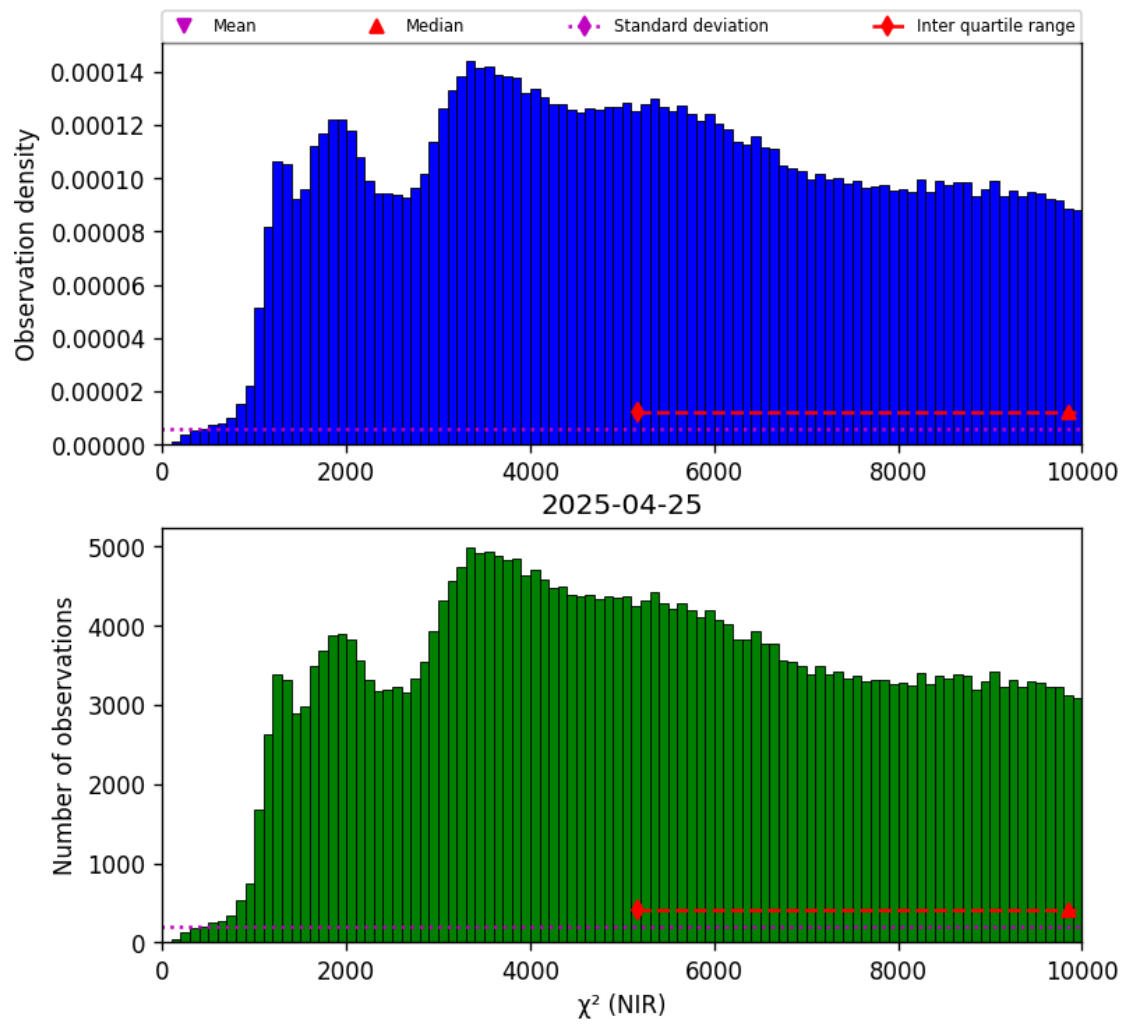
Figure 29: Histogram of “ \chi^2 (NIR)” for 2025-04-24 to 2025-04-26
