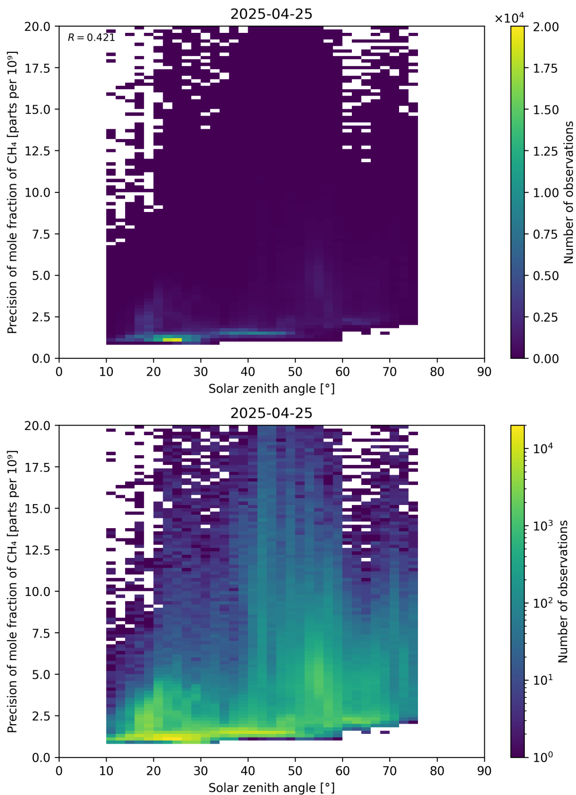
Figure 101: Scatter density plot of “Solar zenith angle” against “Precision of mole fraction of CH 4 ” for 2025-04-24 to 2025-04-26.
