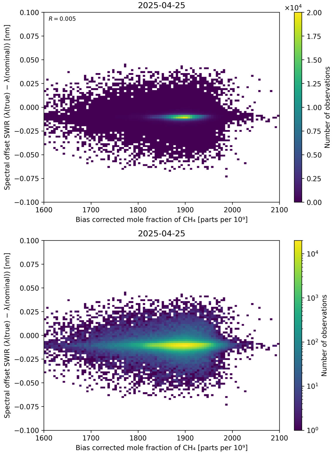
Figure 69: Scatter density plot of “Bias corrected mole fraction of \text{CH}_4 ” against “Spectral offset SWIR ( \lambda_{\text{true}} - \lambda_{\text{nominal}} )” for 2025-04-24 to 2025-04-26.
