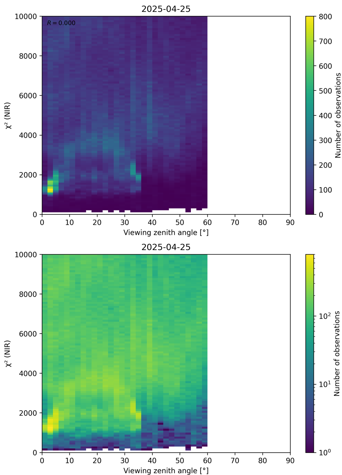
Figure 105: Scatter density plot of “Viewing zenith angle” against “ \chi^2 (NIR)” for 2025-04-24 to 2025-04-26.
