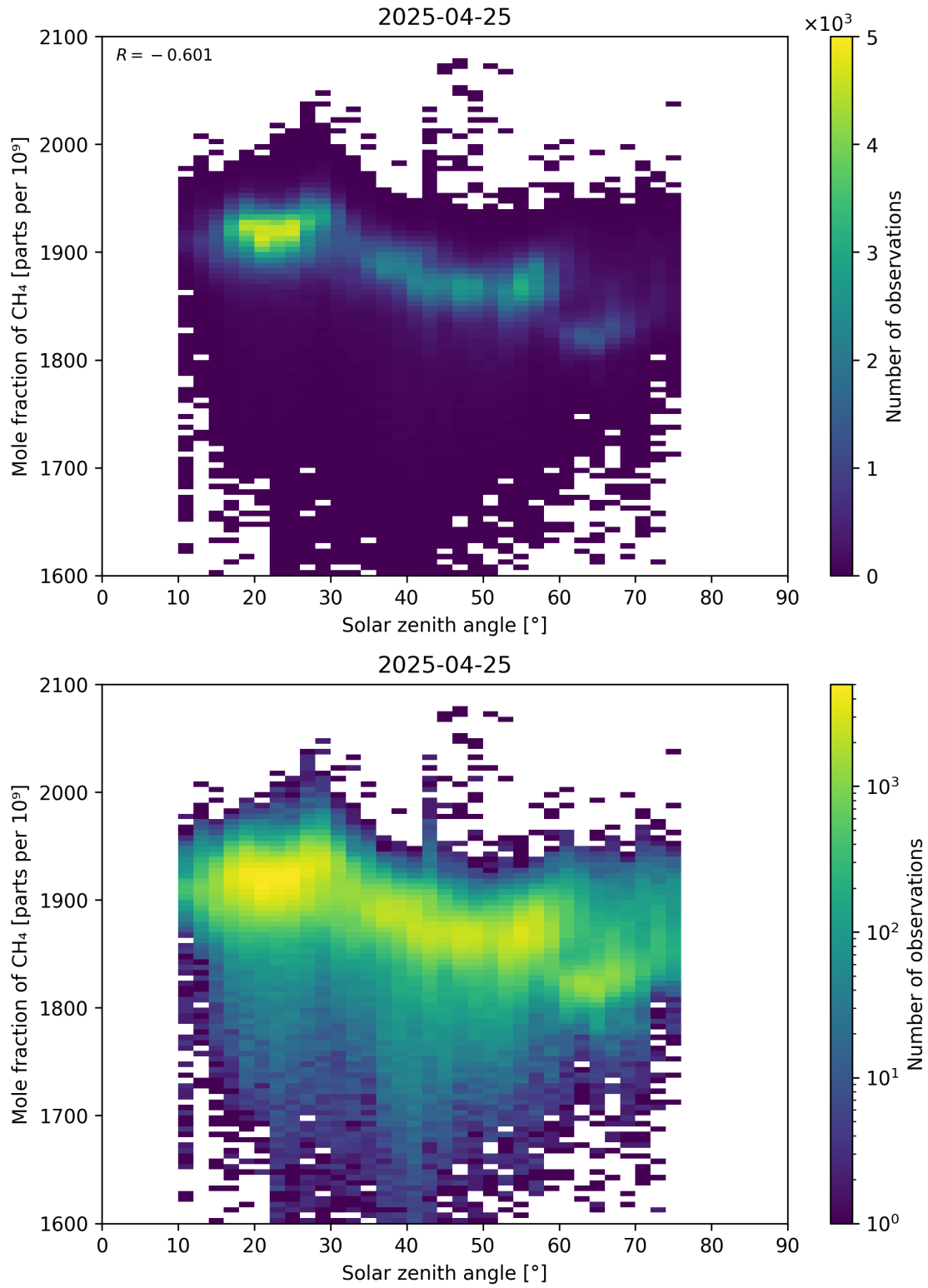
Figure 99: Scatter density plot of “Solar zenith angle” against “Mole fraction of CH 4 ” for 2025-04-24 to 2025-04-26.
