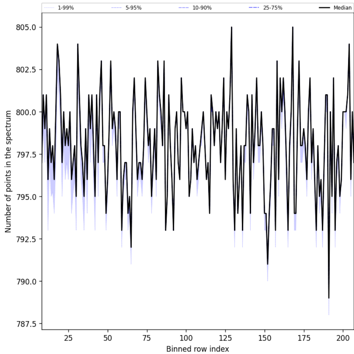
Figure 37: Along track statistics of “Number of points in the spectrum” for 2025-04-24 to 2025-04-26
