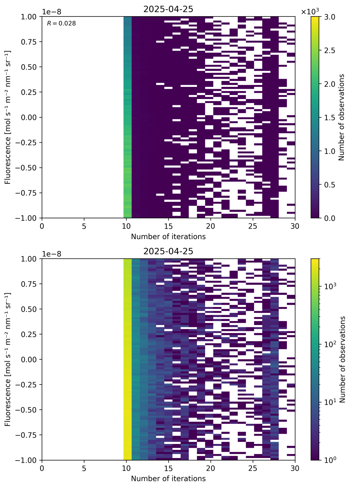
Figure 87: Scatter density plot of “Number of iterations” against “Fluorescence” for 2025-04-24 to 2025-04-26.
