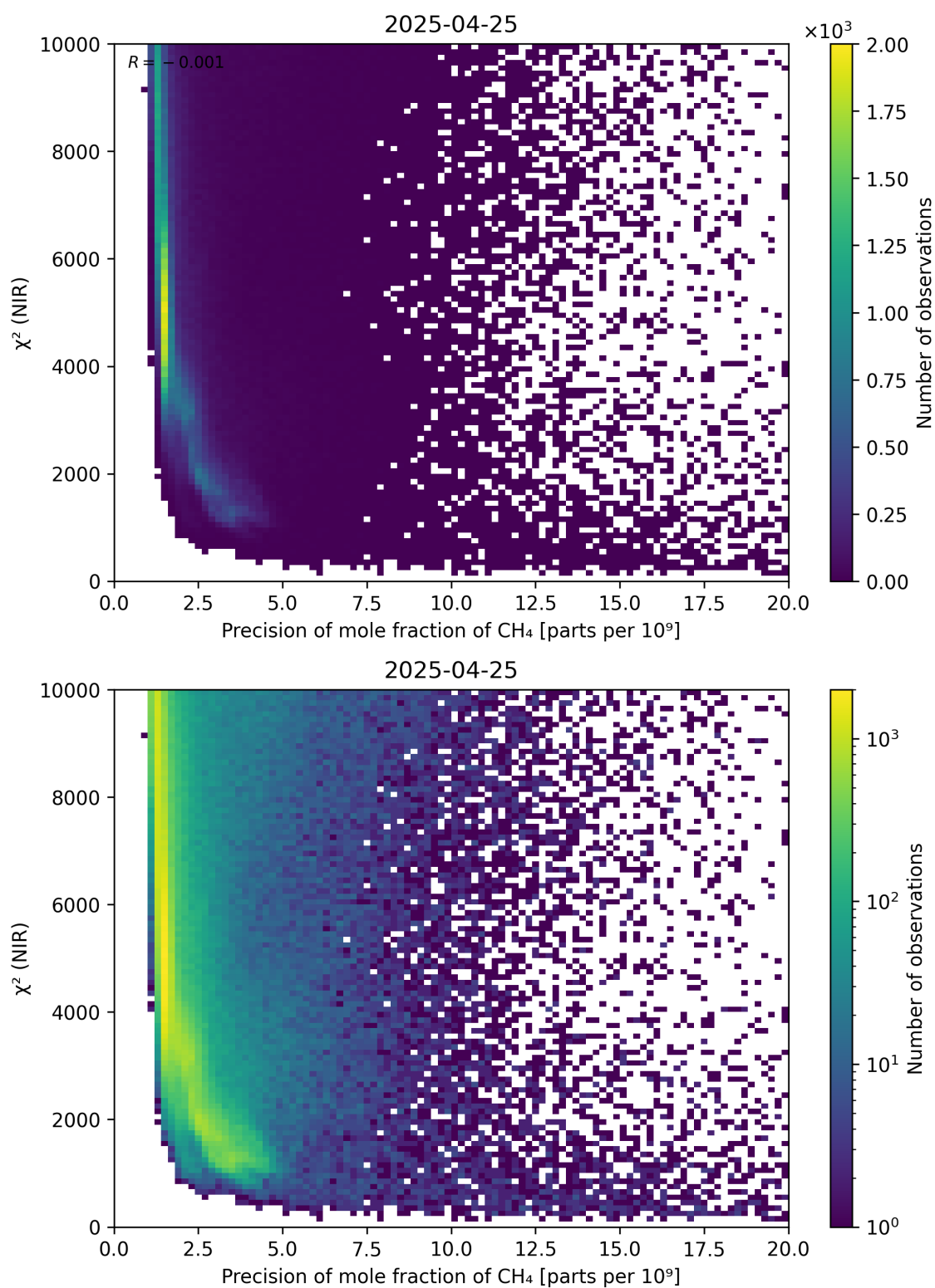
Figure 78: Scatter density plot of “Precision of mole fraction of CH 4 ” against “ \chi^2 (NIR)” for 2025-04-24 to 2025-04-26.
