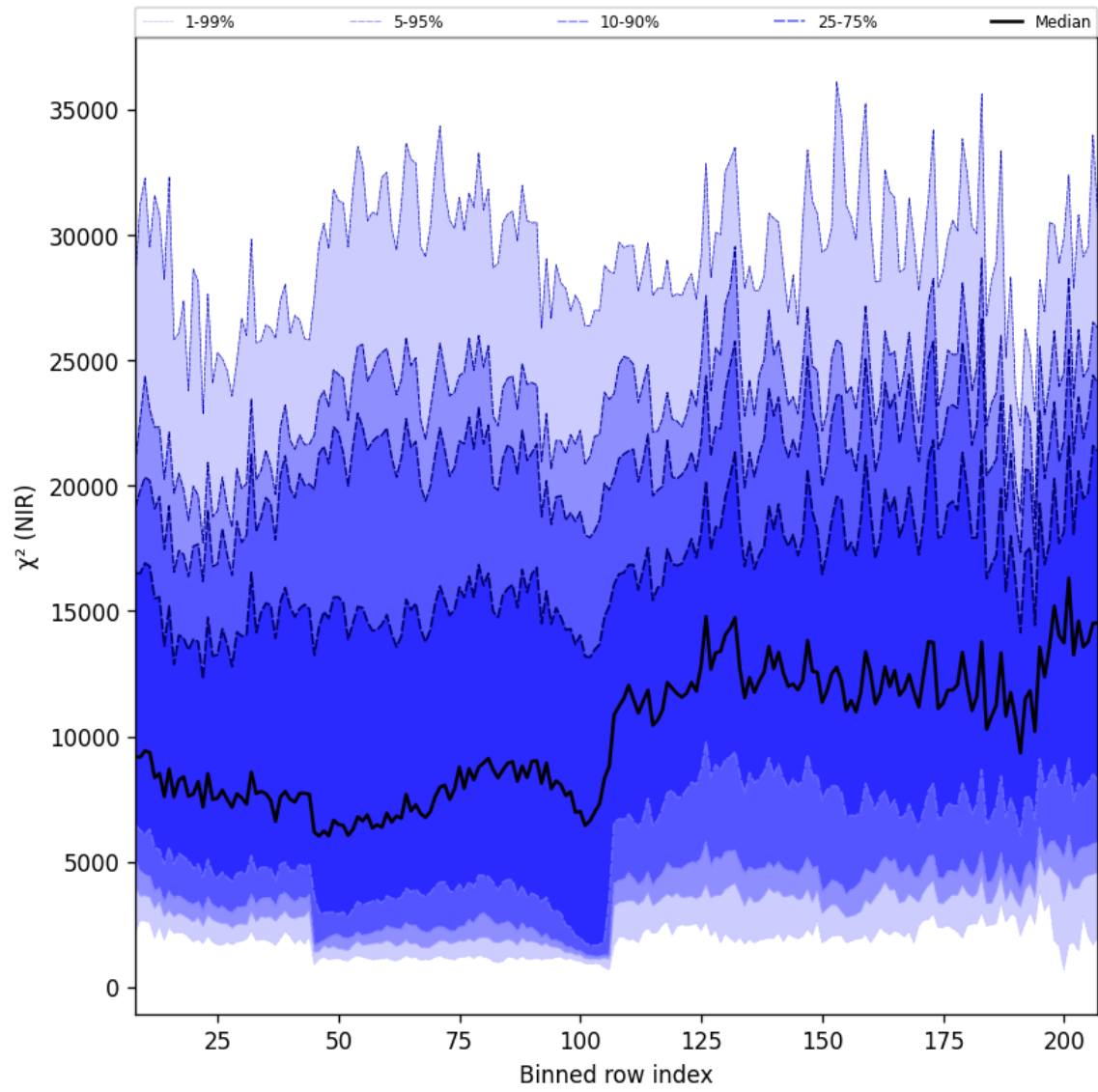
Figure 40: Along track statistics of “ \chi^2 (NIR)” for 2025-04-24 to 2025-04-26
