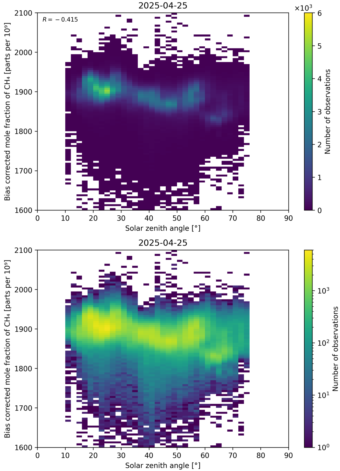
Figure 100: Scatter density plot of “Solar zenith angle” against “Bias corrected mole fraction of CH 4 ” for 2025-04-24 to 2025-04-26.
