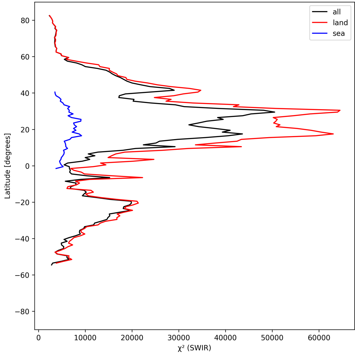
Figure 17: Zonal average of “ \chi^2 (SWIR)” for 2025-04-24 to 2025-04-26.
