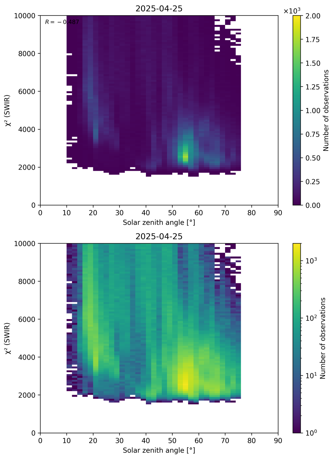
Figure 95: Scatter density plot of “Solar zenith angle” against “ \chi^2 (SWIR)” for 2025-04-24 to 2025-04-26.
