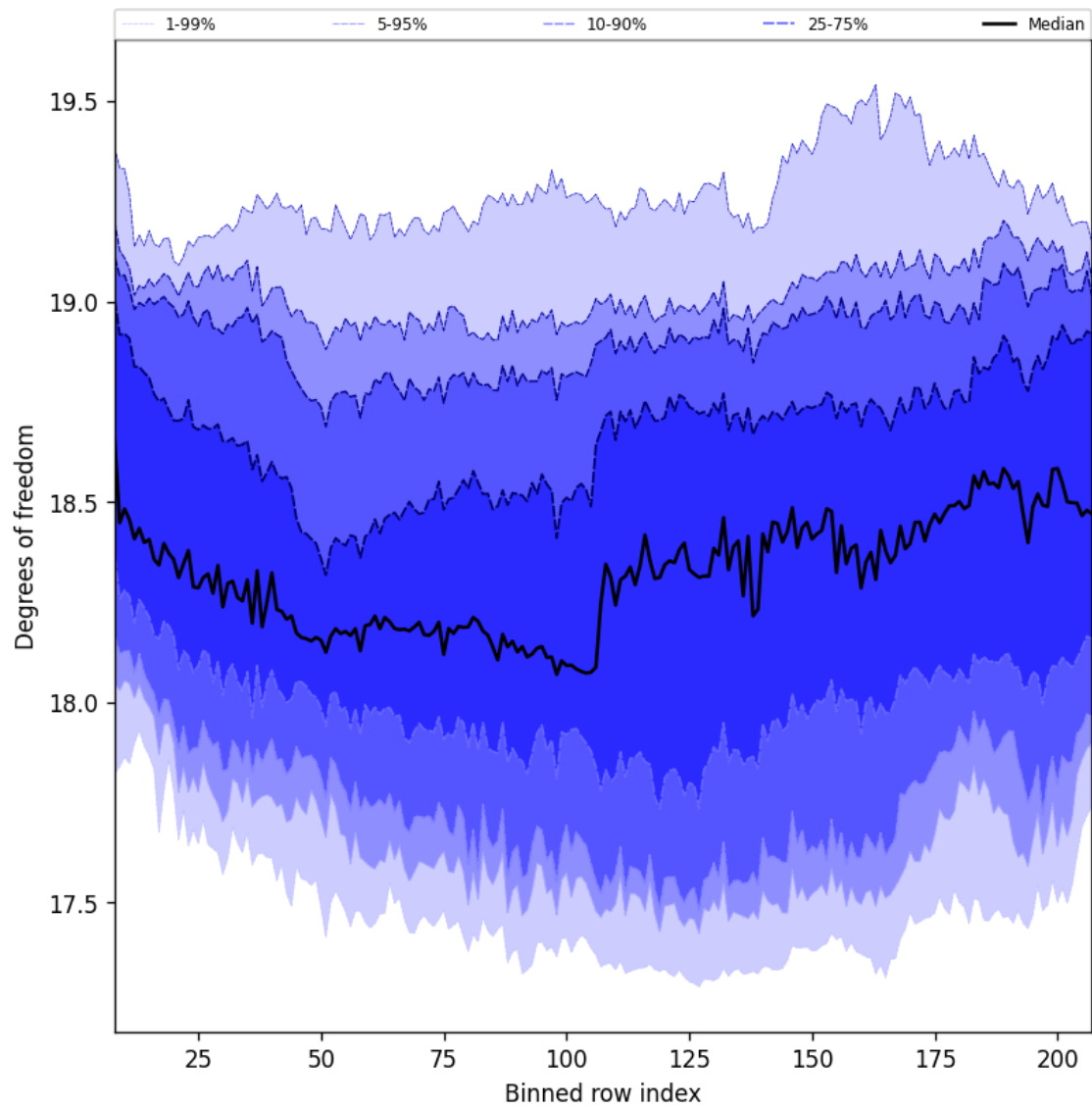
Figure 41: Along track statistics of “Degrees of freedom” for 2025-04-24 to 2025-04-26
