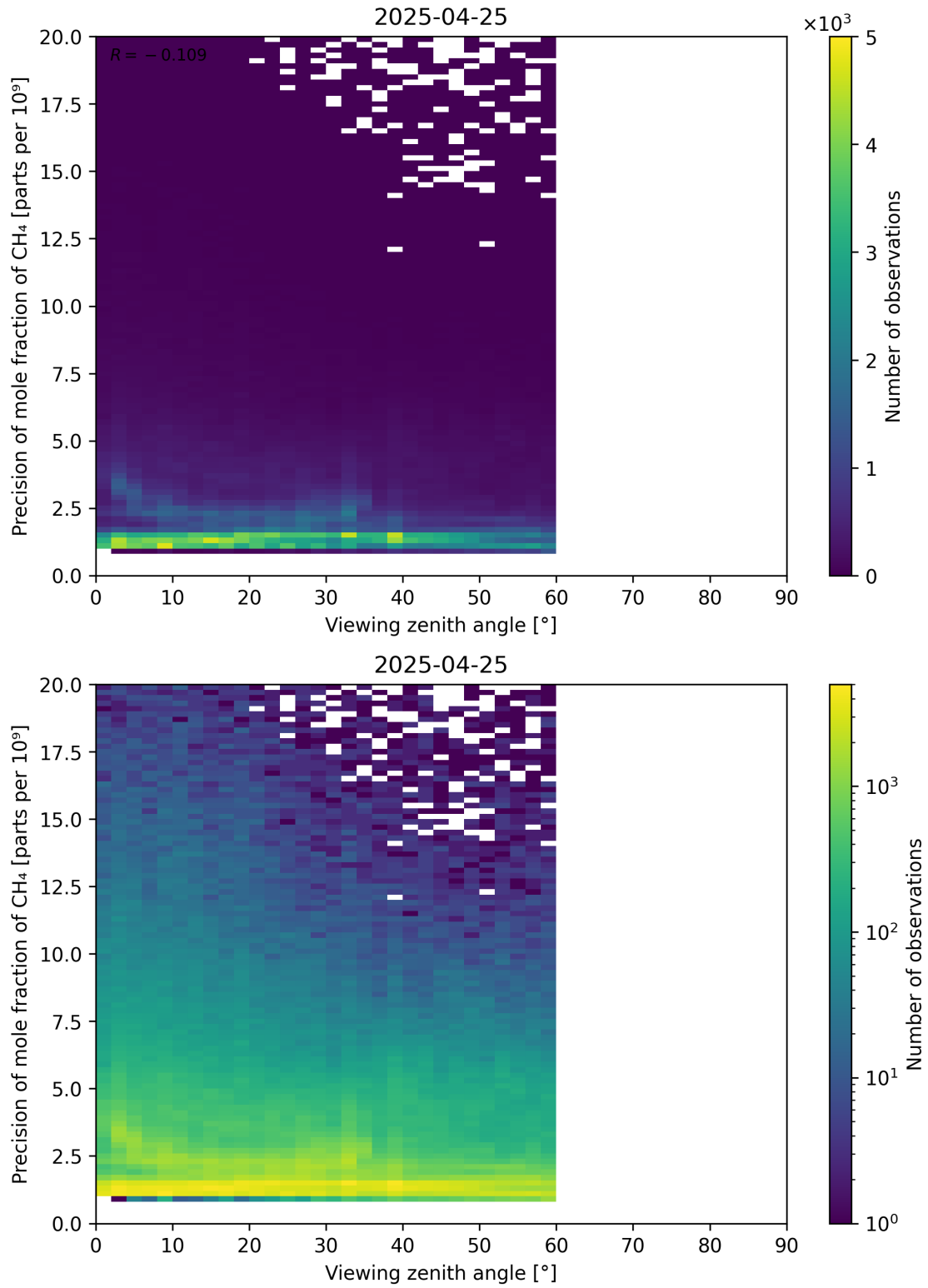
Figure 112: Scatter density plot of “Viewing zenith angle” against “Precision of mole fraction of \text{CH}_4 ” for 2025-04-24 to 2025-04-26.
