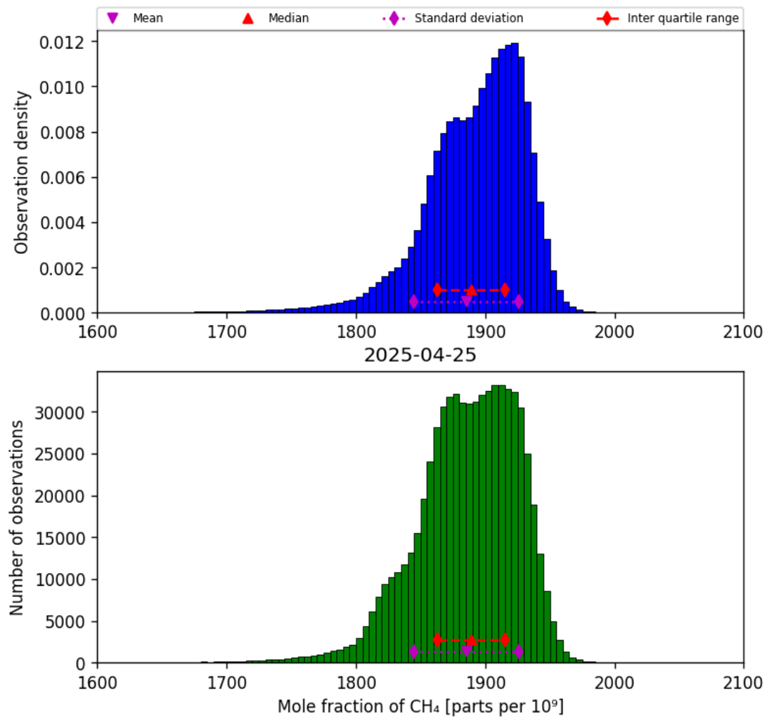
Figure 23: Histogram of “Mole fraction of CH 4 ” for 2025-04-24 to 2025-04-26
