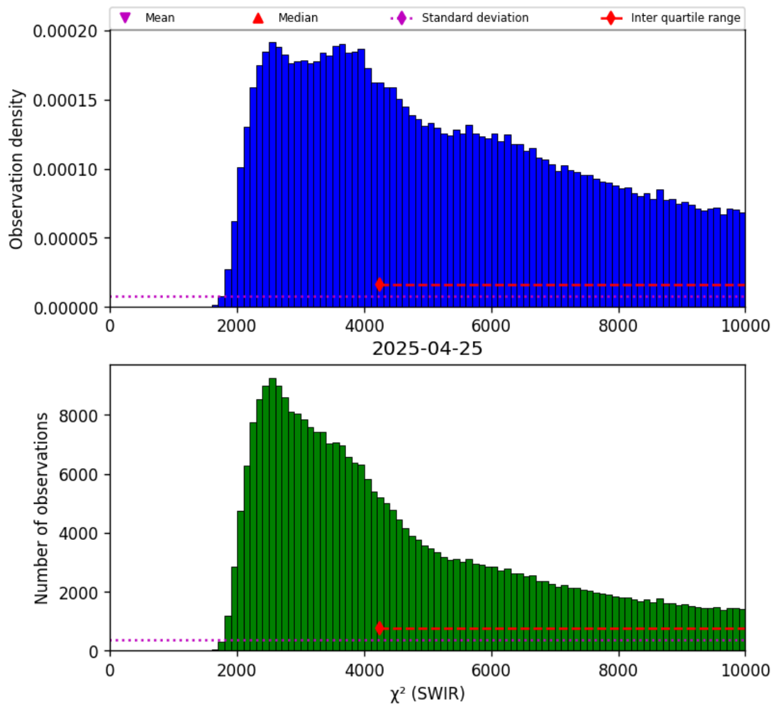
Figure 28: Histogram of " \chi^2 (SWIR)" for 2025-04-24 to 2025-04-26
