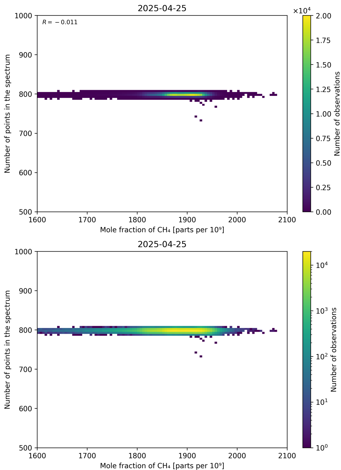
Figure 77: Scatter density plot of “Mole fraction of CH 4 ” against “Number of points in the spectrum” for 2025-04-24 to 2025-04-26.
