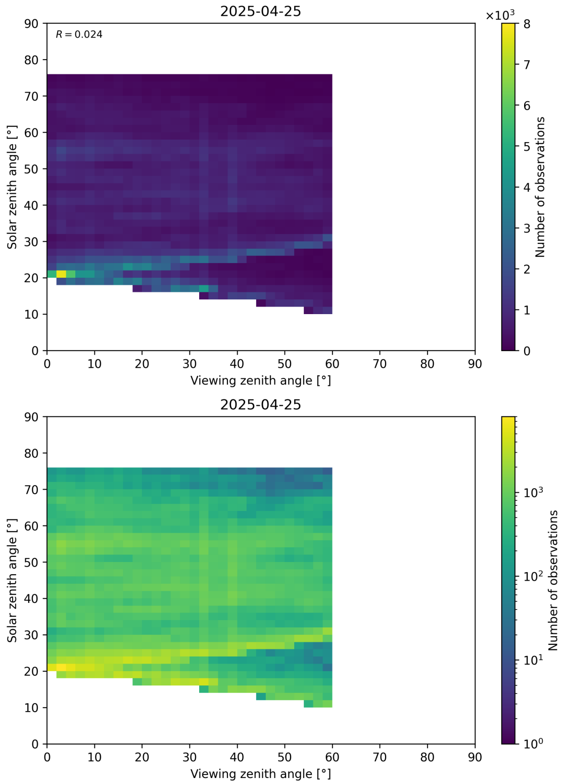
Figure 115: Scatter density plot of “Viewing zenith angle” against “Solar zenith angle” for 2025-04-24 to 2025-04-26.
