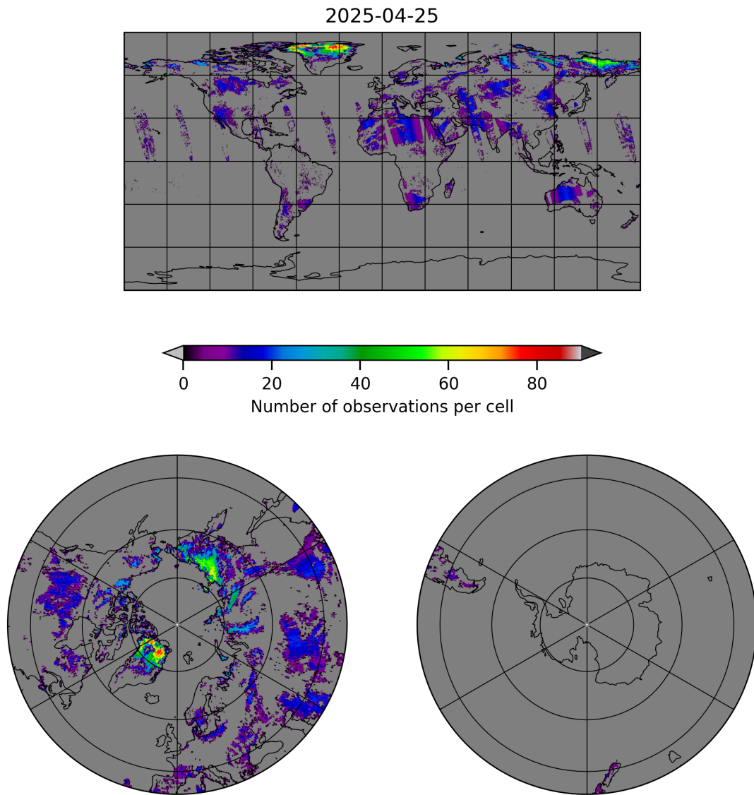
Figure 10: Map of the number of observations for 2025-04-24 to 2025-04-26
