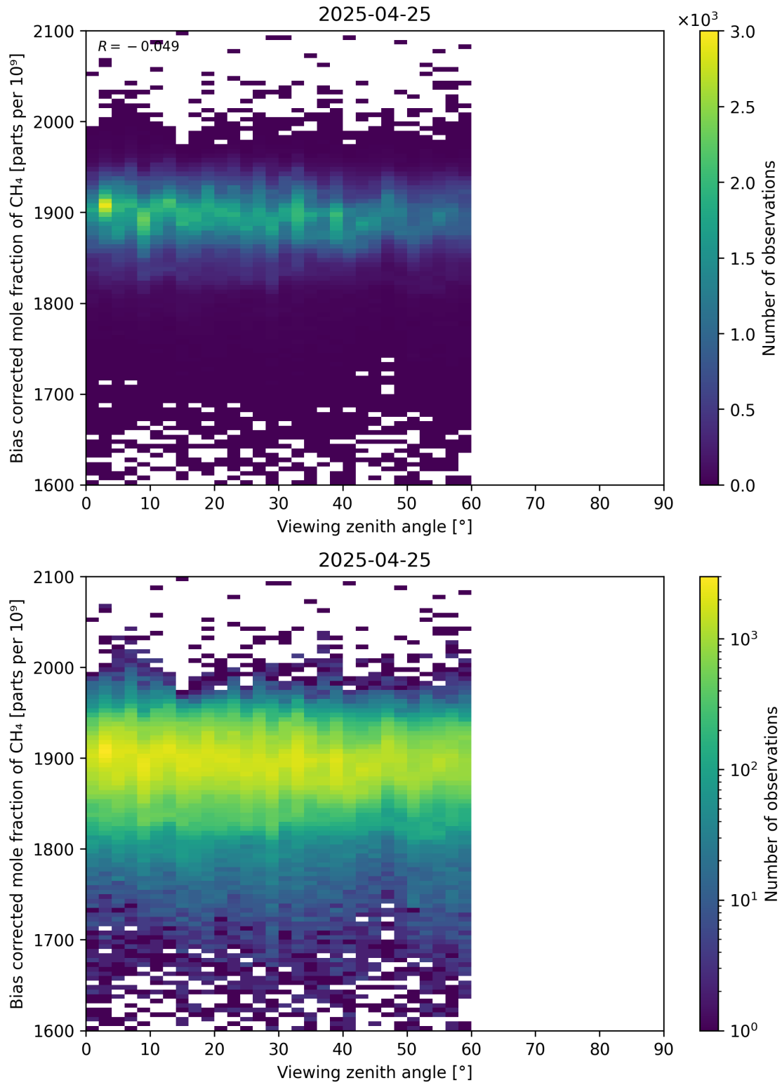
Figure 111: Scatter density plot of “Viewing zenith angle” against “Bias corrected mole fraction of CH 4 ” for 2025-04-24 to 2025-04-26.
