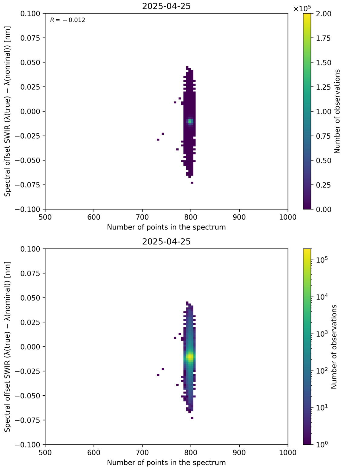
Figure 93: Scatter density plot of “Number of points in the spectrum” against “Spectral offset SWIR ( \lambda_{\text{true}} - \lambda_{\text{nominal}} )” for 2025-04-24 to 2025-04-26.
