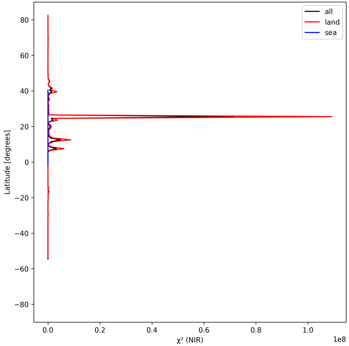
Figure 18: Zonal average of “ \chi^2 (NIR)” for 2025-04-24 to 2025-04-26.
