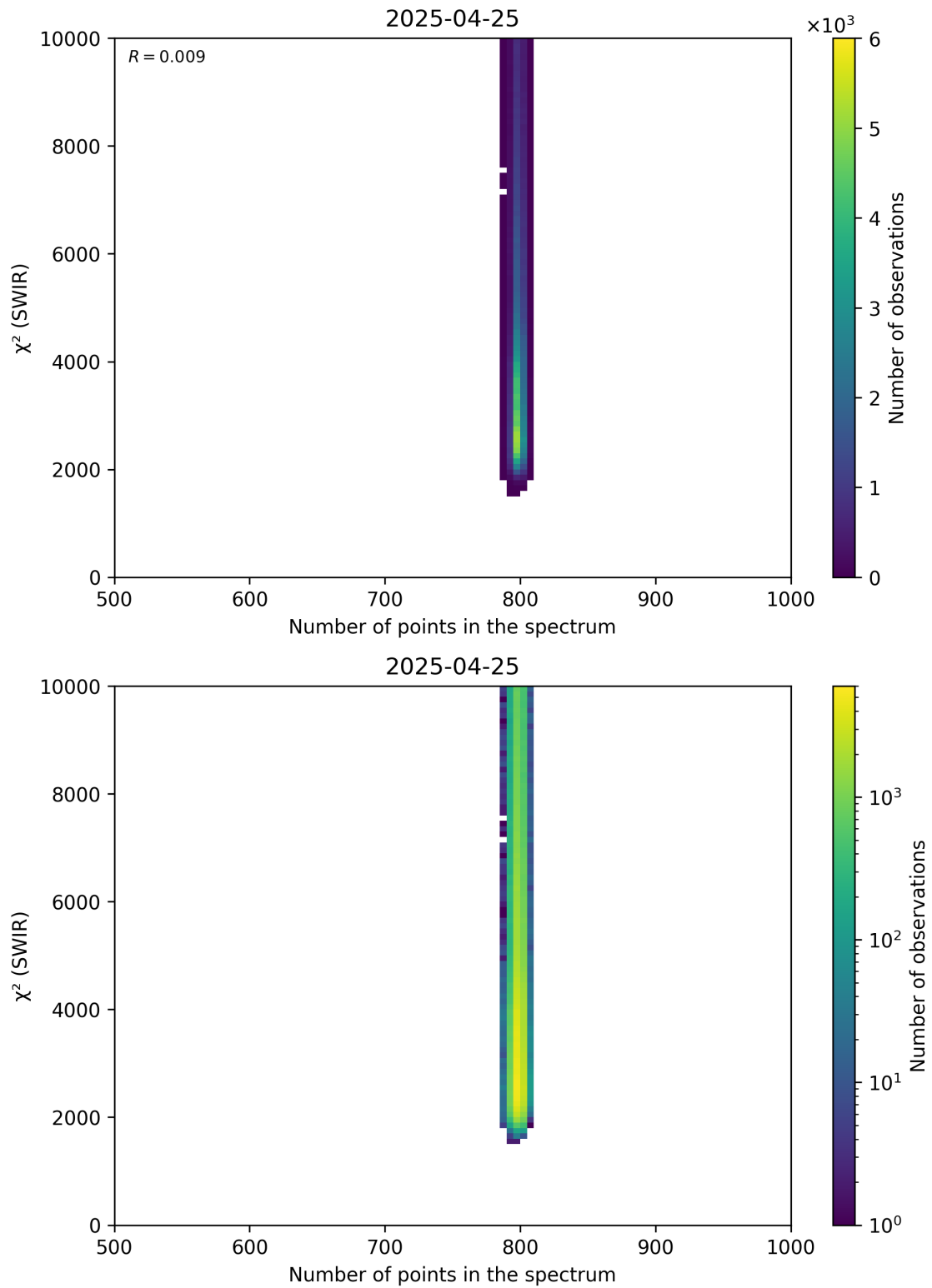
Figure 89: Scatter density plot of “Number of points in the spectrum” against “ \chi^2 (SWIR)” for 2025-04-24 to 2025-04-26.
