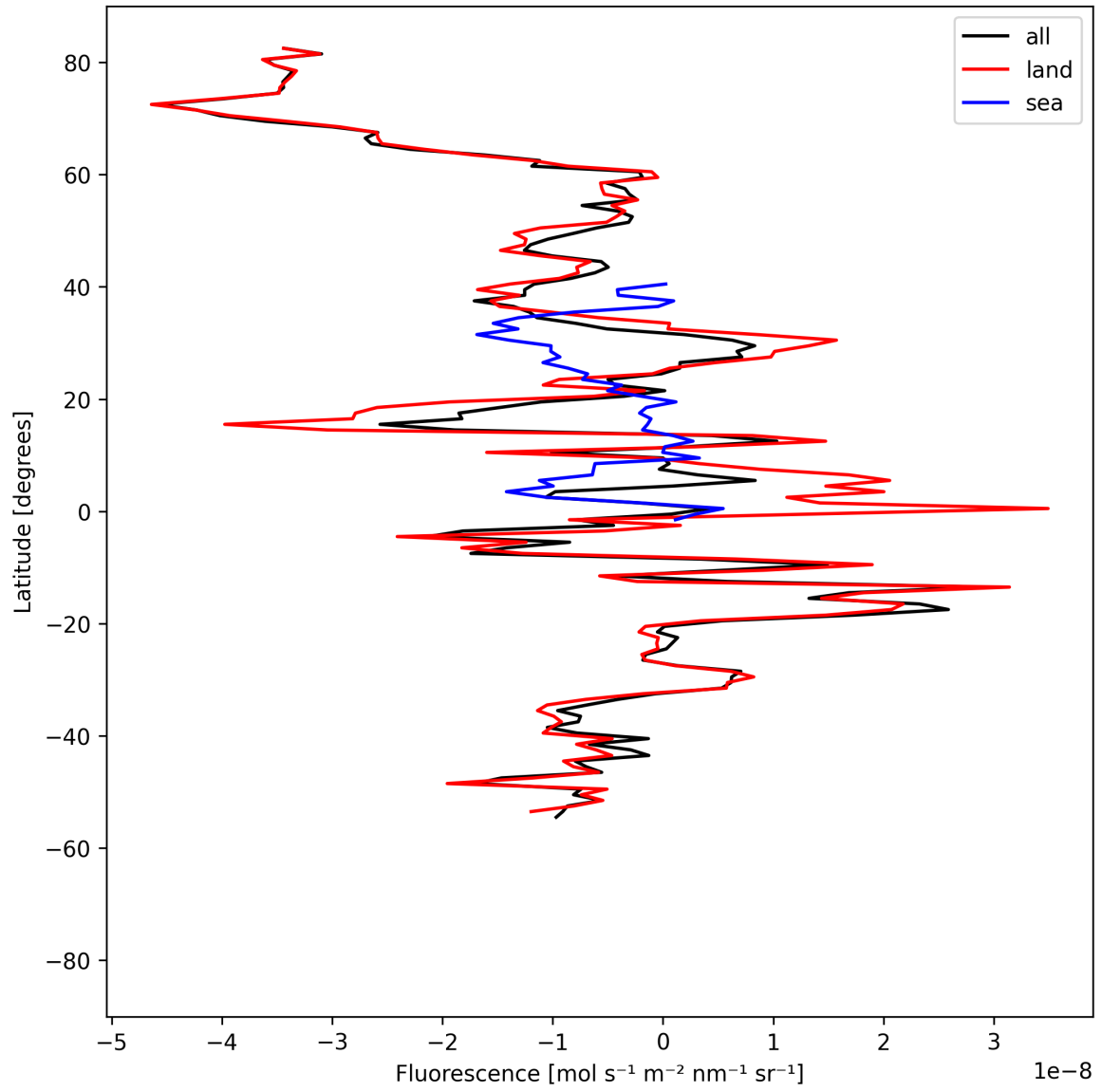
Figure 21: Zonal average of “Fluorescence” for 2025-04-24 to 2025-04-26.
