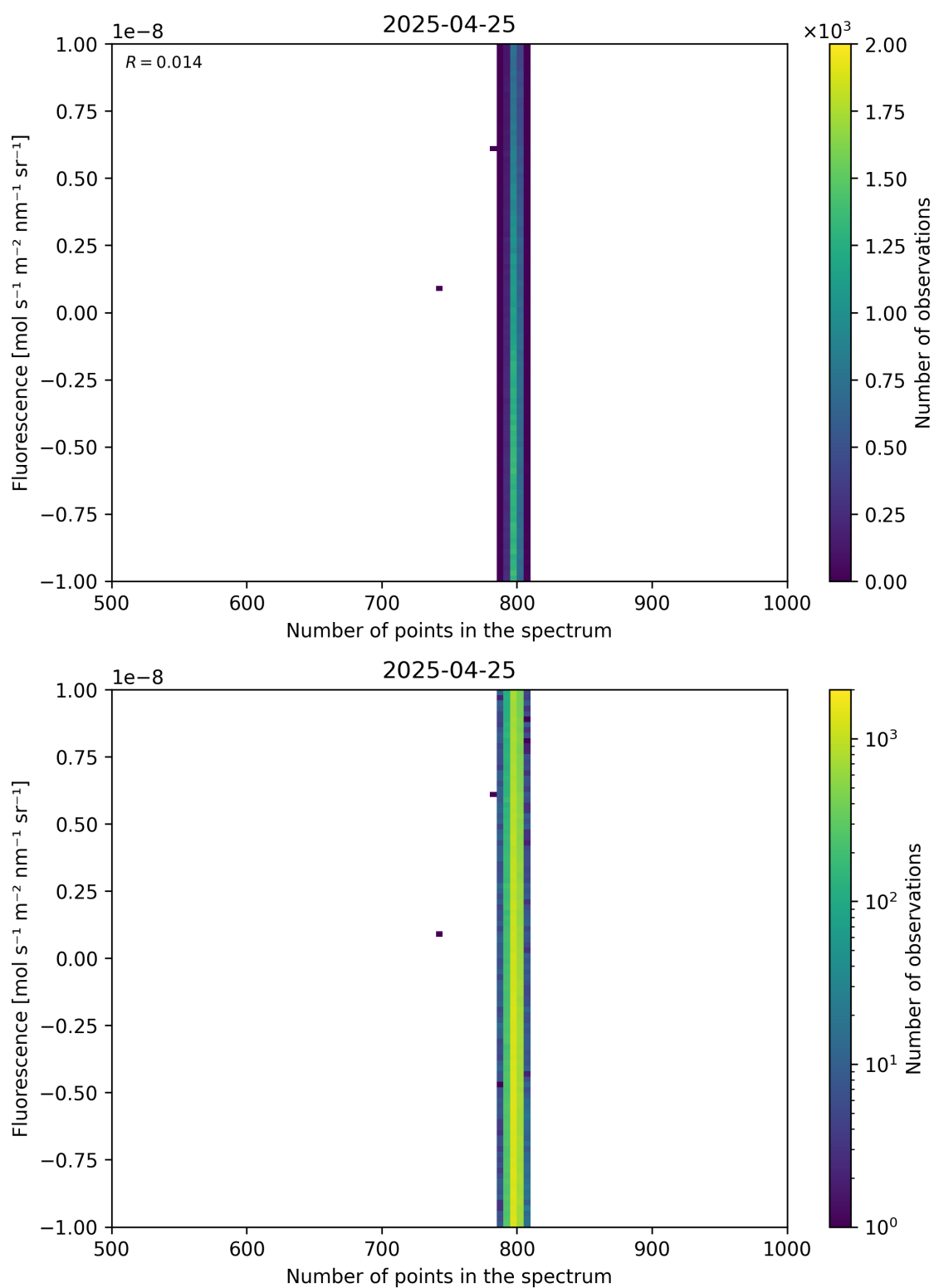
Figure 91: Scatter density plot of “Number of points in the spectrum” against “Fluorescence” for 2025-04-24 to 2025-04-26.
