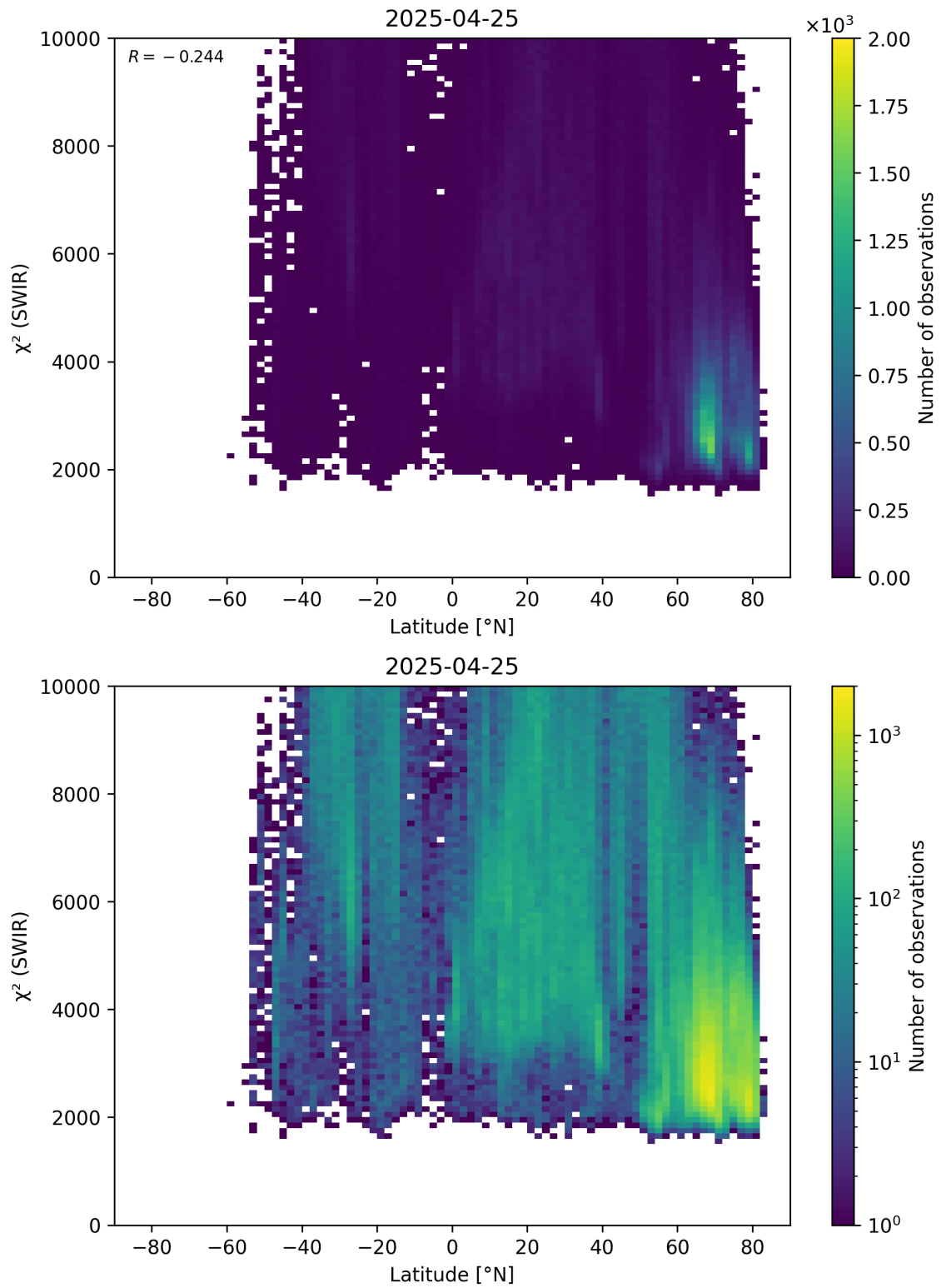
Figure 54: Scatter density plot of “Latitude” against “ \chi^2 (SWIR)” for 2025-04-24 to 2025-04-26.
