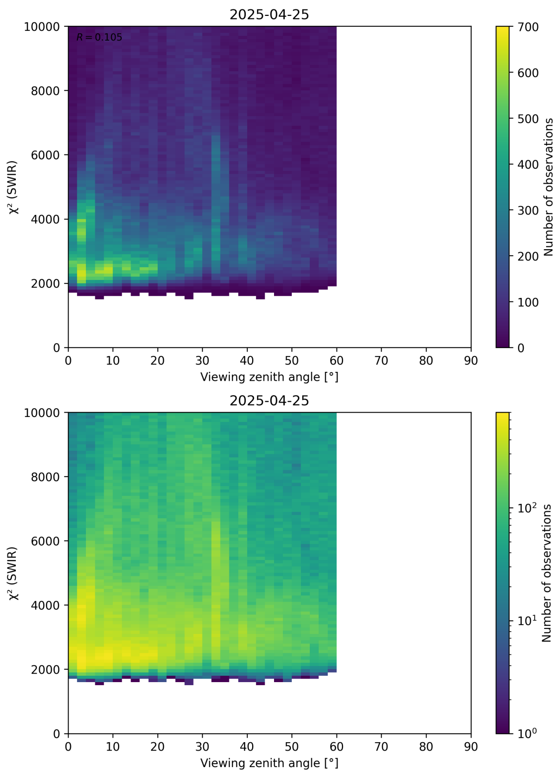
Figure 106: Scatter density plot of “Viewing zenith angle” against “ \chi^2 (SWIR)” for 2025-04-24 to 2025-04-26.
