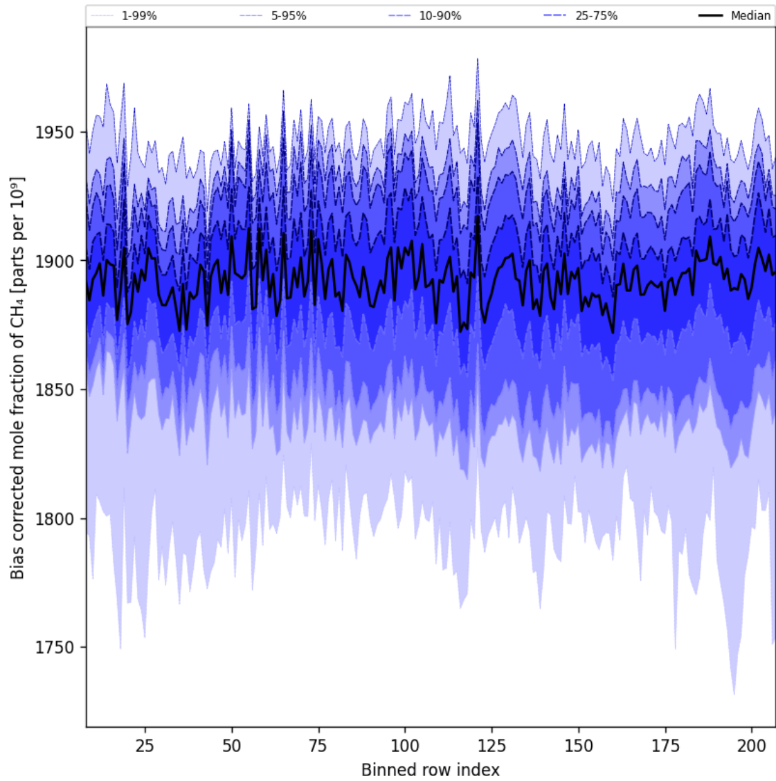
Figure 36: Along track statistics of “Bias corrected mole fraction of CH 4 ” for 2025-04-25 to 2025-04-27
