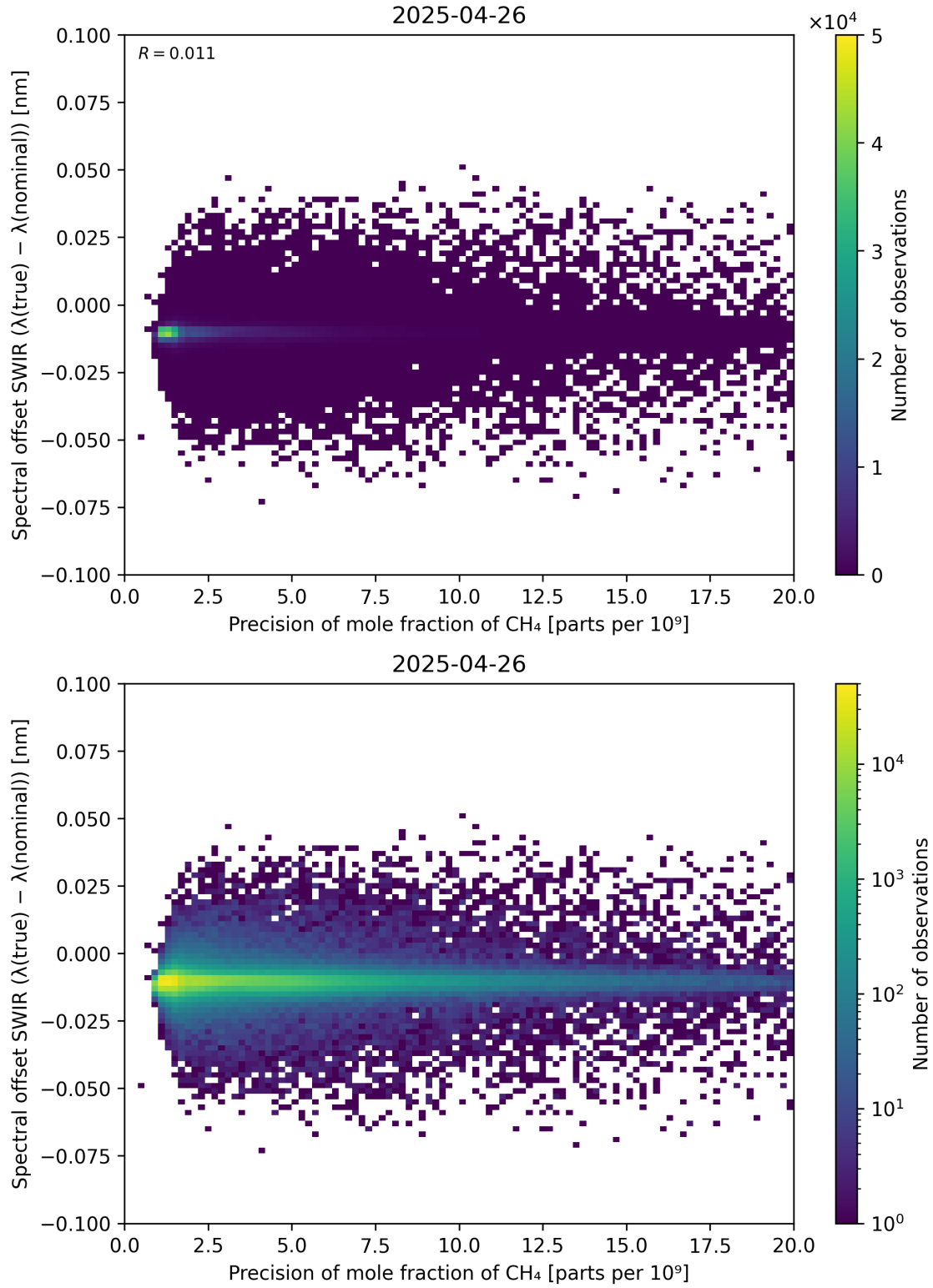
Figure 85: Scatter density plot of “Precision of mole fraction of CH 4 ” against “Spectral offset SWIR ( \lambda_{\text{true}} - \lambda_{\text{nominal}} )” for 2025-04-25 to 2025-04-27.
