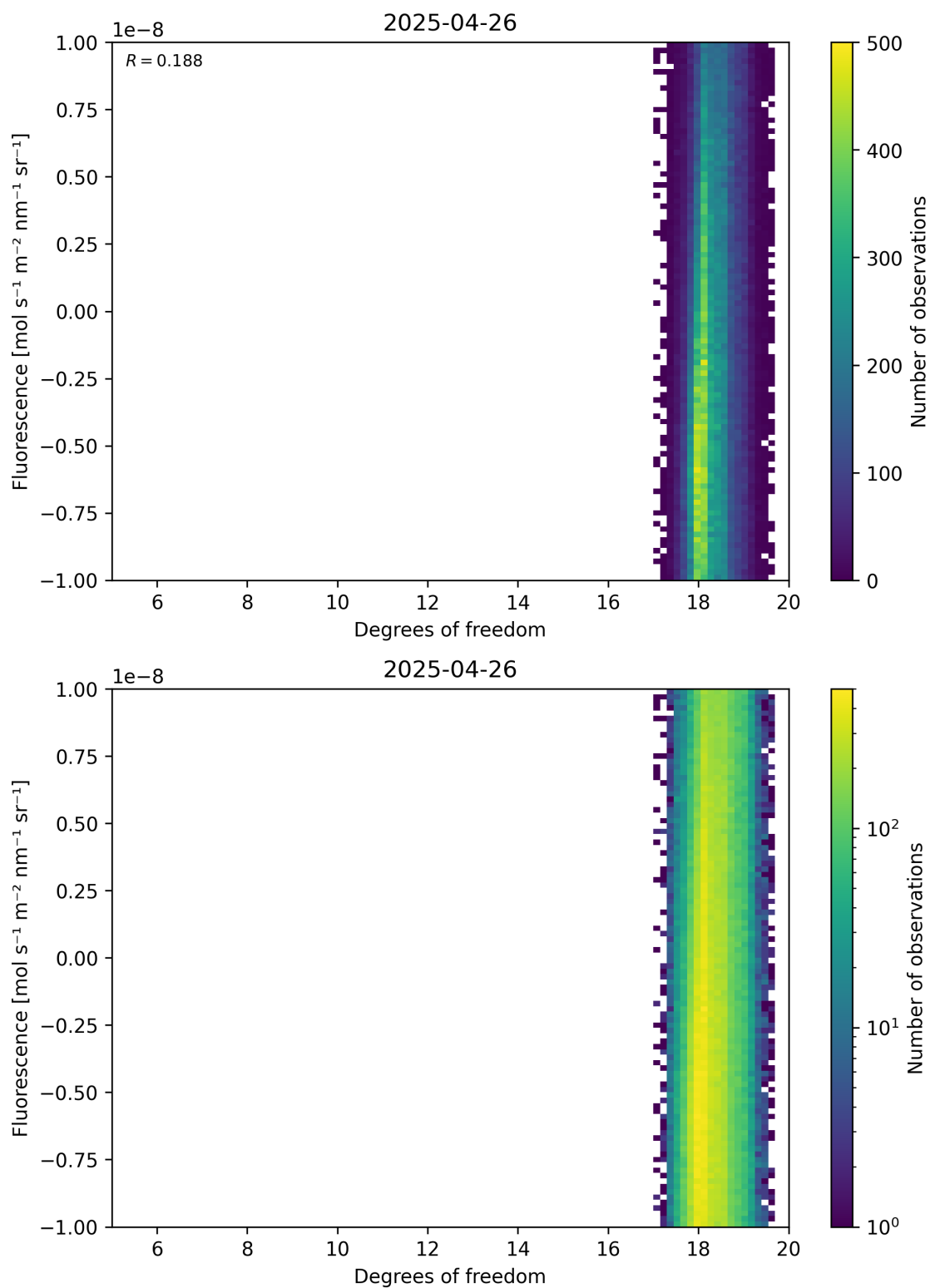
Figure 51: Scatter density plot of “Degrees of freedom” against “Fluorescence” for 2025-04-25 to 2025-04-27.
