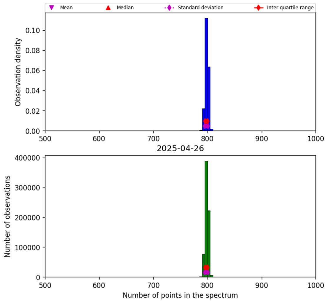
Figure 26: Histogram of “Number of points in the spectrum” for 2025-04-25 to 2025-04-27
