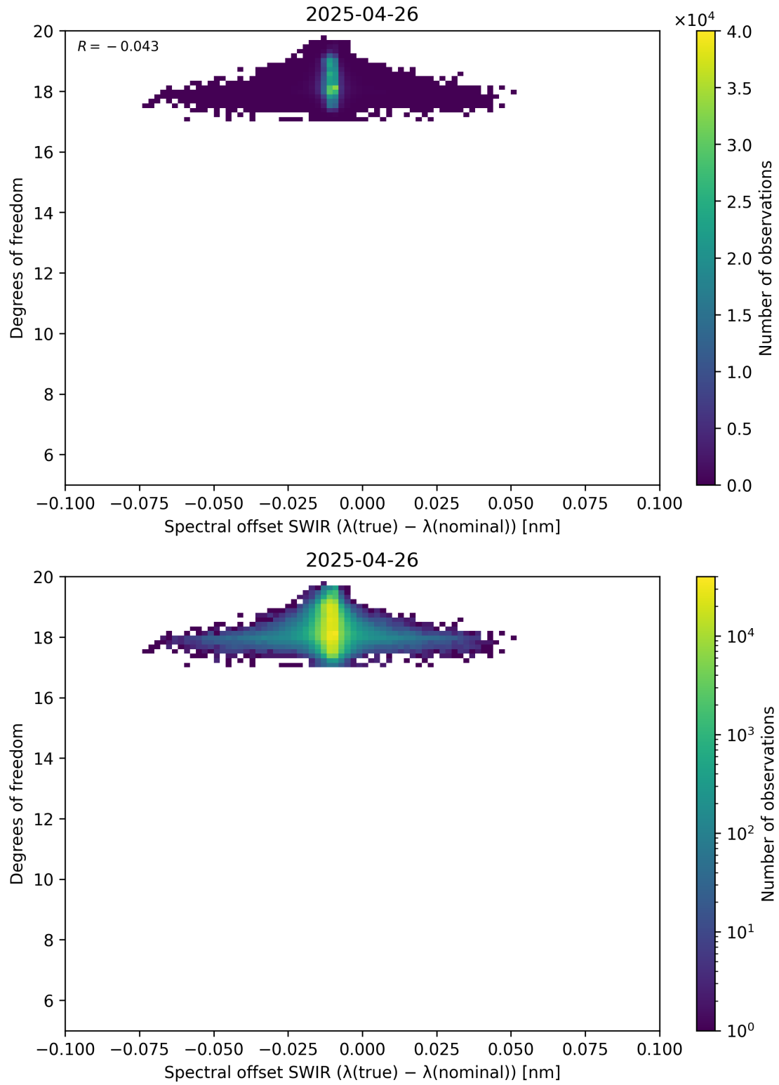
Figure 119: Scatter density plot of “Spectral offset SWIR ( \lambda_{\text{true}} - \lambda_{\text{nominal}} )” against “Degrees of freedom” for 2025-04-25 to 2025-04-27.
