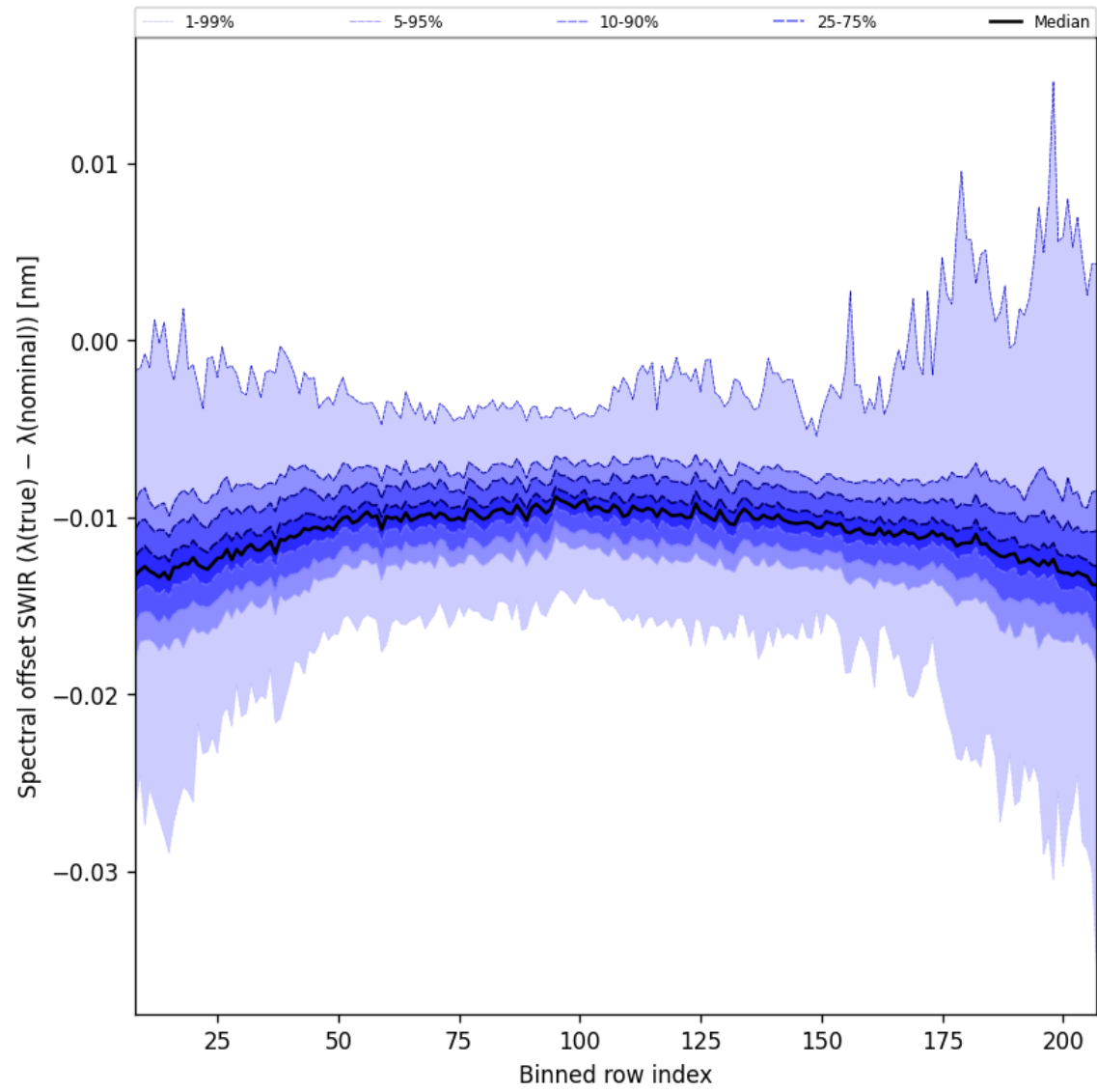
Figure 38: Along track statistics of “Spectral offset SWIR ( \lambda_{\text{true}} - \lambda_{\text{nominal}} )” for 2025-04-25 to 2025-04-27
