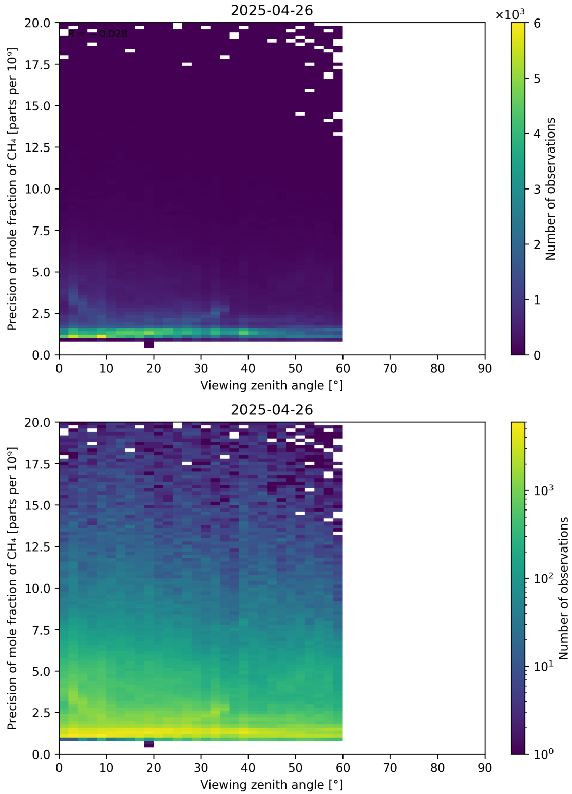
Figure 112: Scatter density plot of “Viewing zenith angle” against “Precision of mole fraction of CH 4 ” for 2025-04-25 to 2025-04-27.
