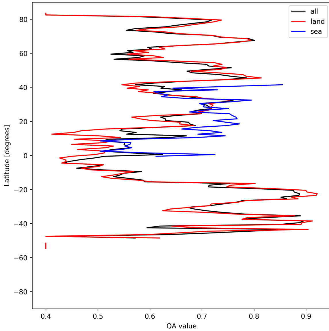
Figure 11: Zonal average of “QA value” for 2025-04-25 to 2025-04-27.
