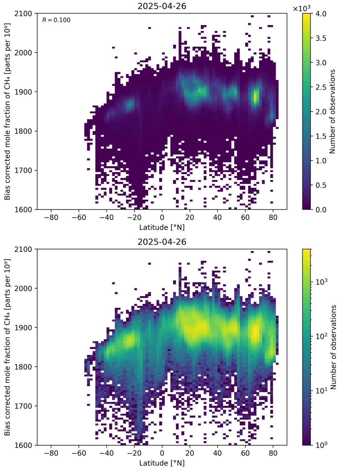
Figure 58: Scatter density plot of “Latitude” against “Bias corrected mole fraction of CH 4 ” for 2025-04-25 to 2025-04-27.
