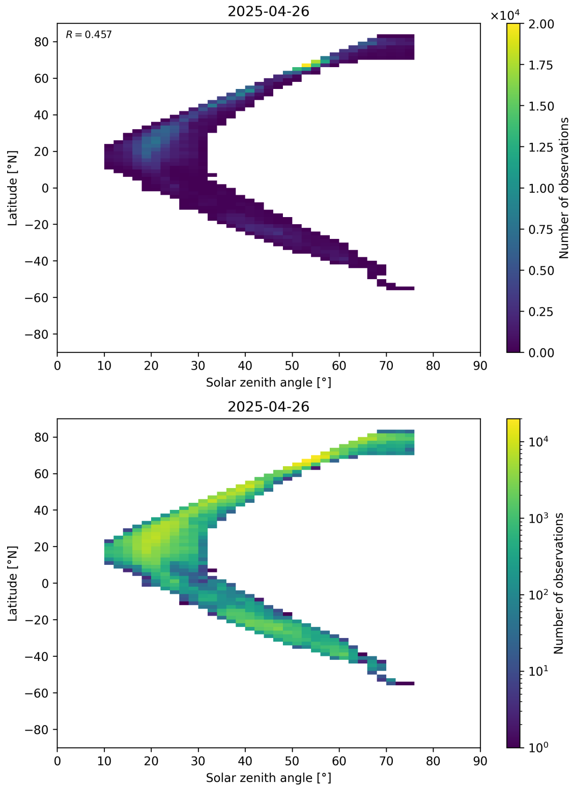
Figure 98: Scatter density plot of “Solar zenith angle” against “Latitude” for 2025-04-25 to 2025-04-27.
