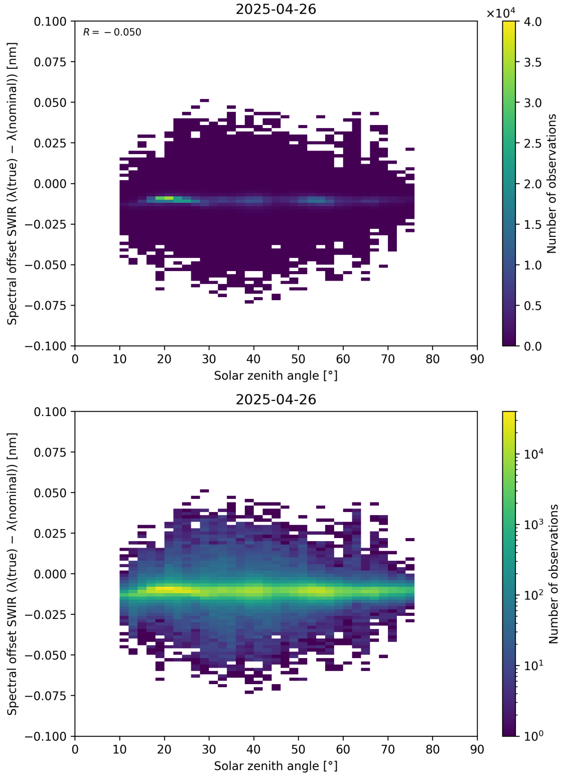
Figure 104: Scatter density plot of “Solar zenith angle” against “Spectral offset SWIR ( \lambda_{\text{true}} - \lambda_{\text{nominal}} )” for 2025-04-25 to 2025-04-27.
