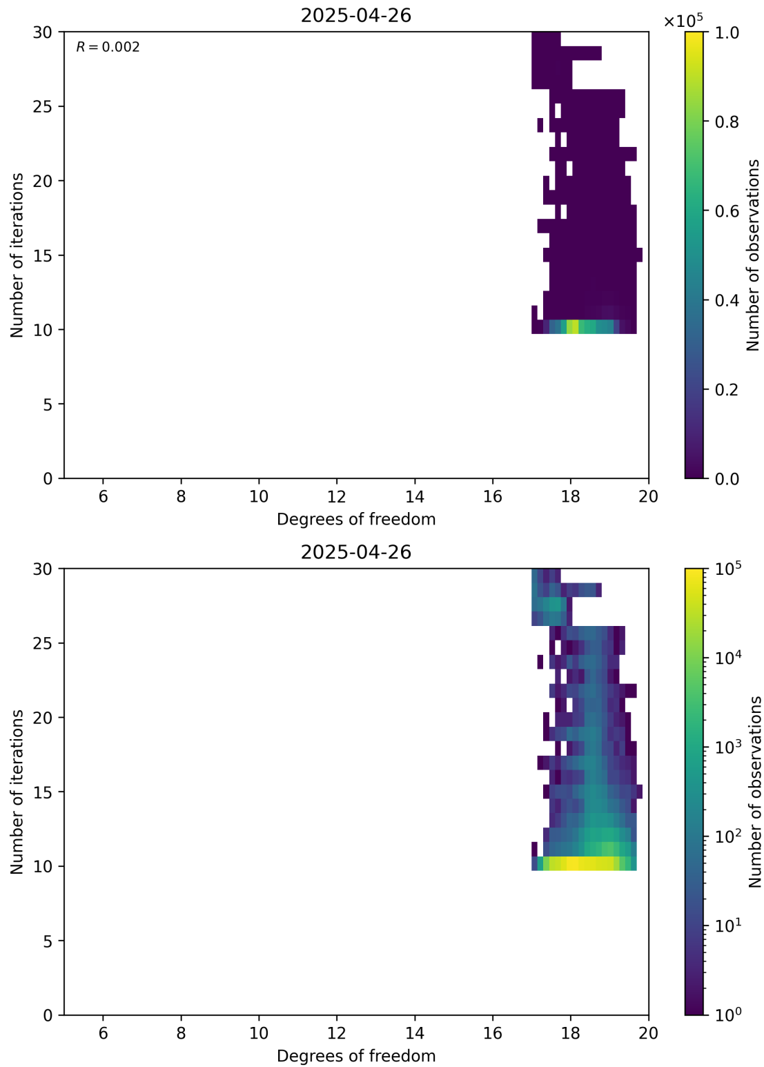
Figure 52: Scatter density plot of “Degrees of freedom” against “Number of iterations” for 2025-04-25 to 2025-04-27.
