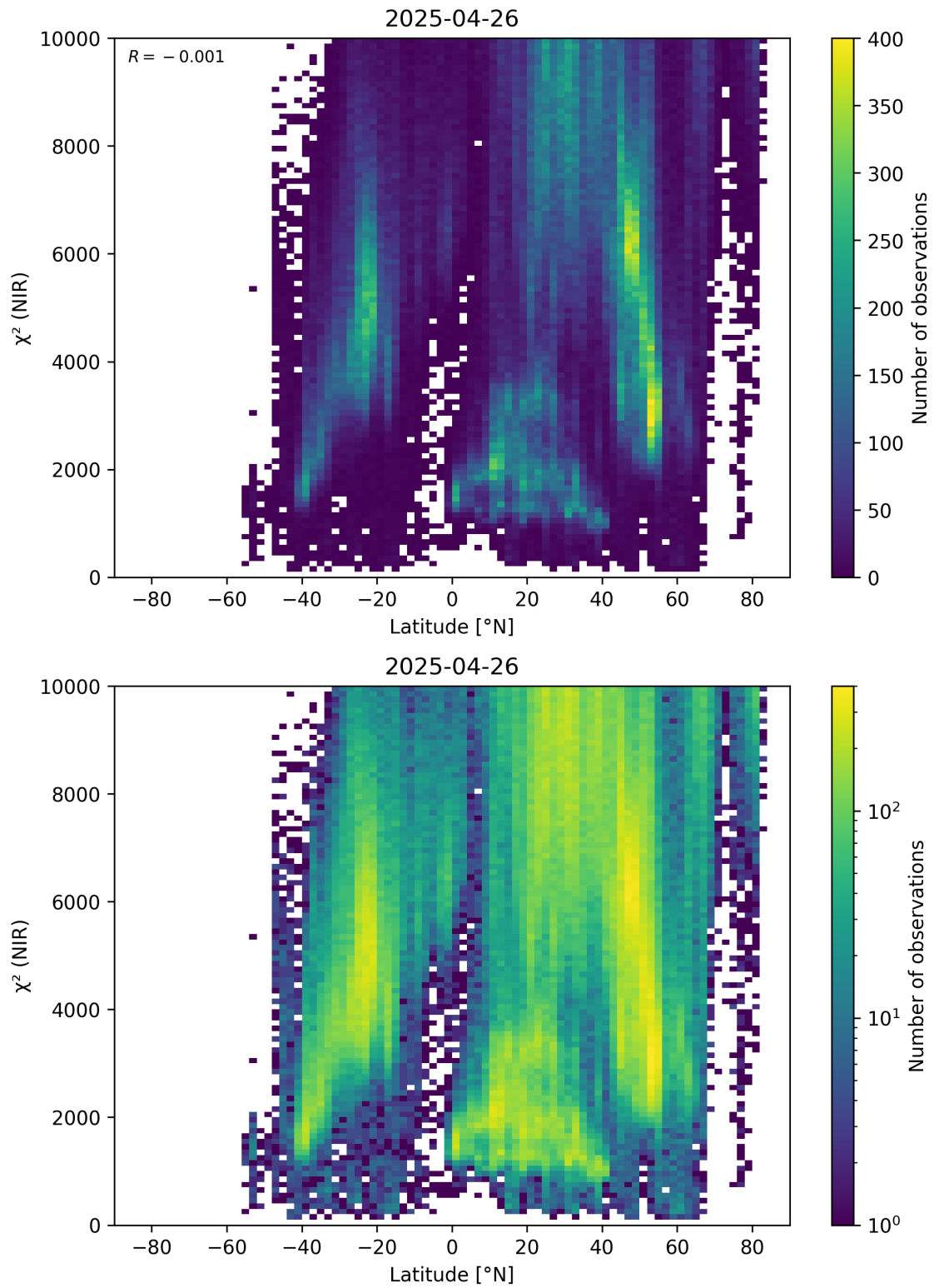
Figure 53: Scatter density plot of “Latitude” against “ \chi^2 (NIR)” for 2025-04-25 to 2025-04-27.
