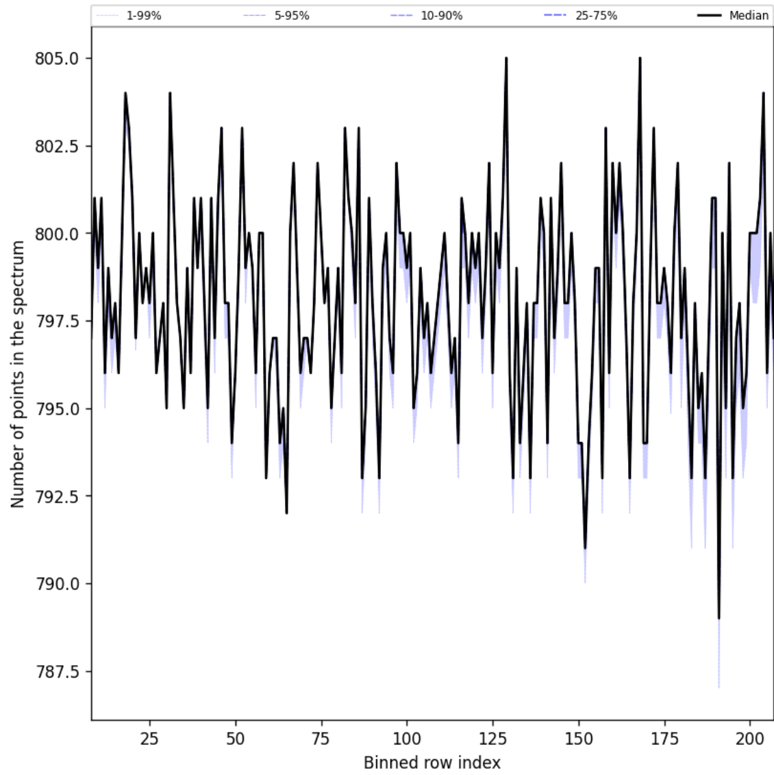
Figure 37: Along track statistics of “Number of points in the spectrum” for 2025-04-25 to 2025-04-27
