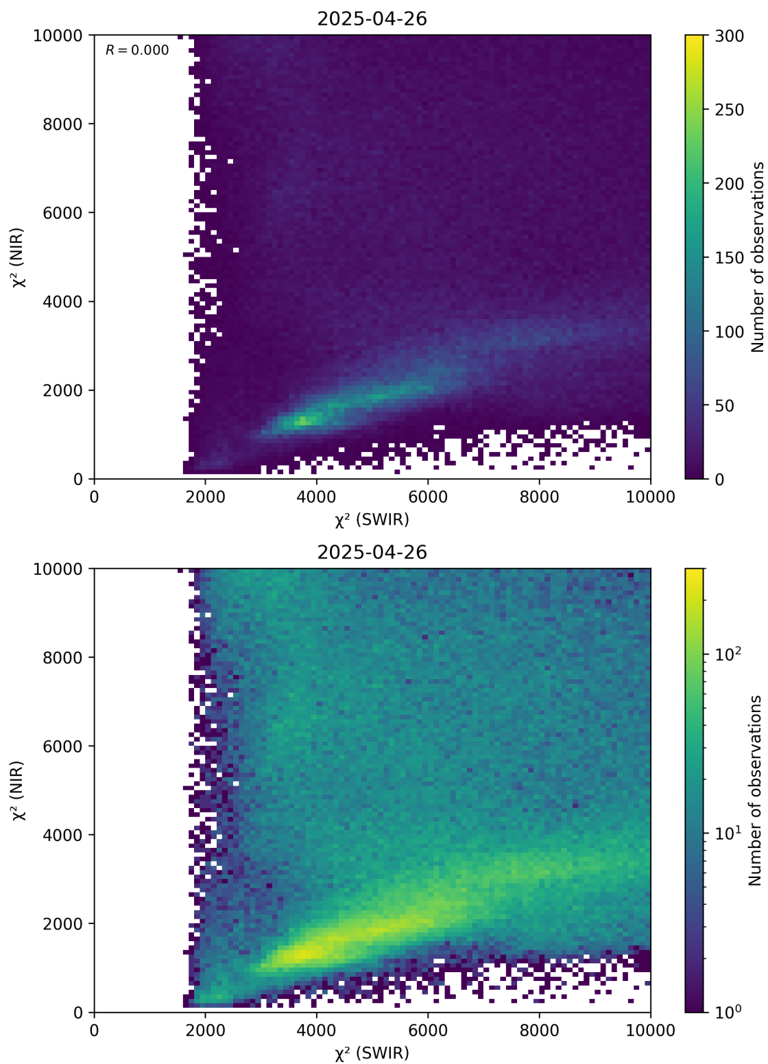
Figure 47: Scatter density plot of “ \chi^2 (SWIR)” against “ \chi^2 (NIR)” for 2025-04-25 to 2025-04-27.
