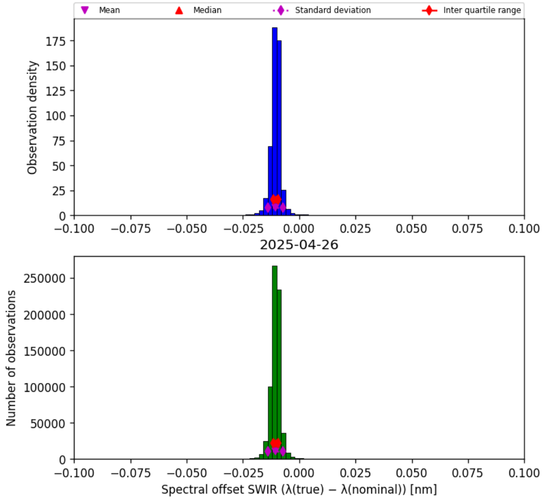
Figure 27: Histogram of “Spectral offset SWIR ( \lambda_{\text{true}} - \lambda_{\text{nominal}} )” for 2025-04-25 to 2025-04-27
