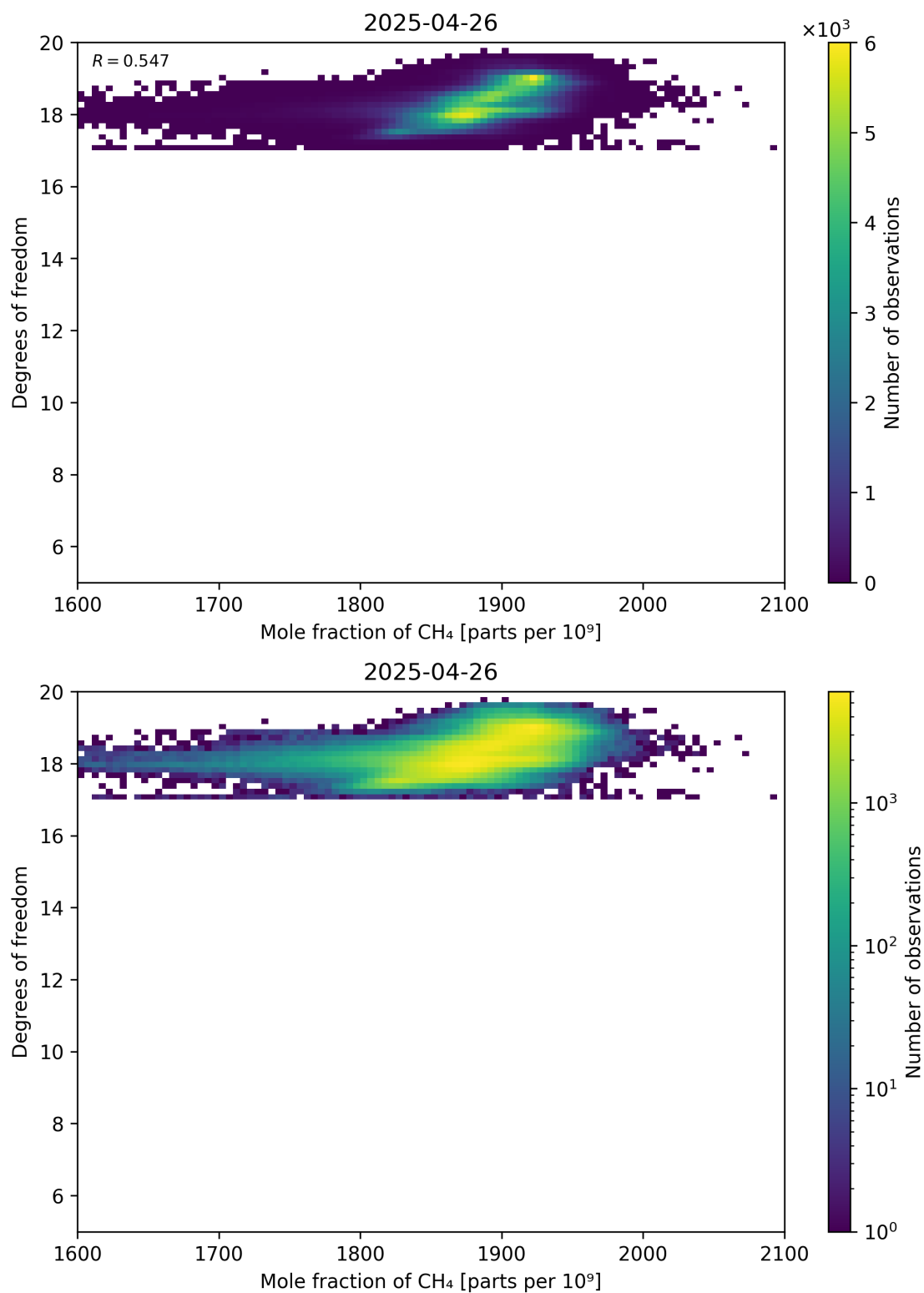
Figure 72: Scatter density plot of “Mole fraction of CH 4 ” against “Degrees of freedom” for 2025-04-25 to 2025-04-27.
