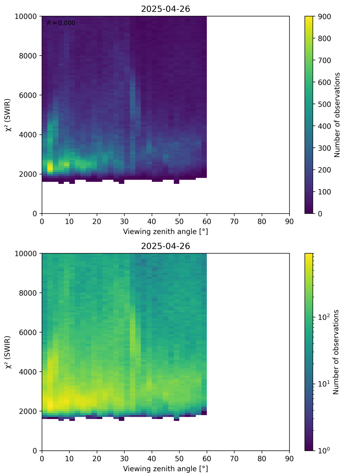
Figure 106: Scatter density plot of “Viewing zenith angle” against “ \chi^2 (SWIR)” for 2025-04-25 to 2025-04-27.
