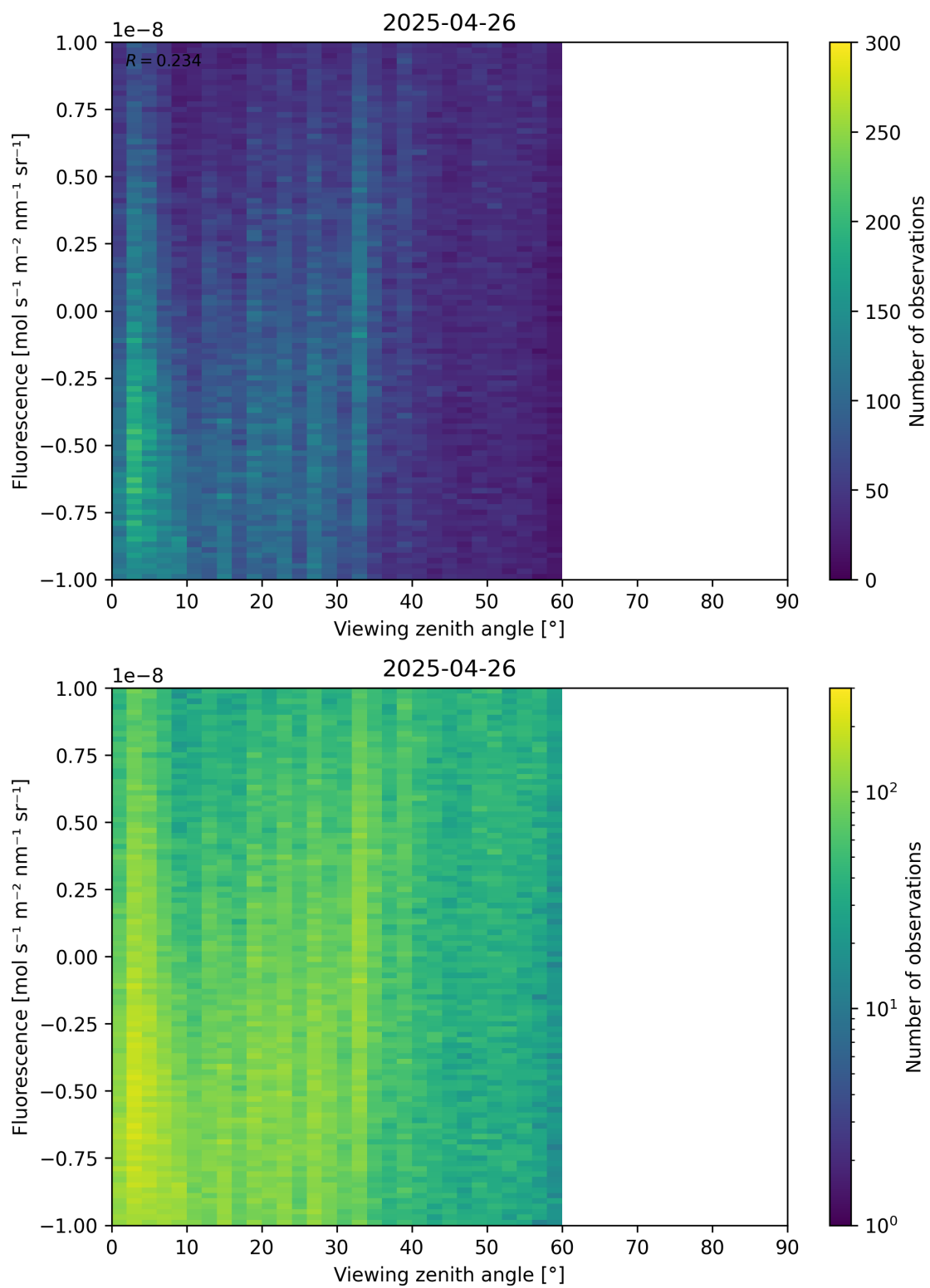
Figure 108: Scatter density plot of “Viewing zenith angle” against “Fluorescence” for 2025-04-25 to 2025-04-27.
