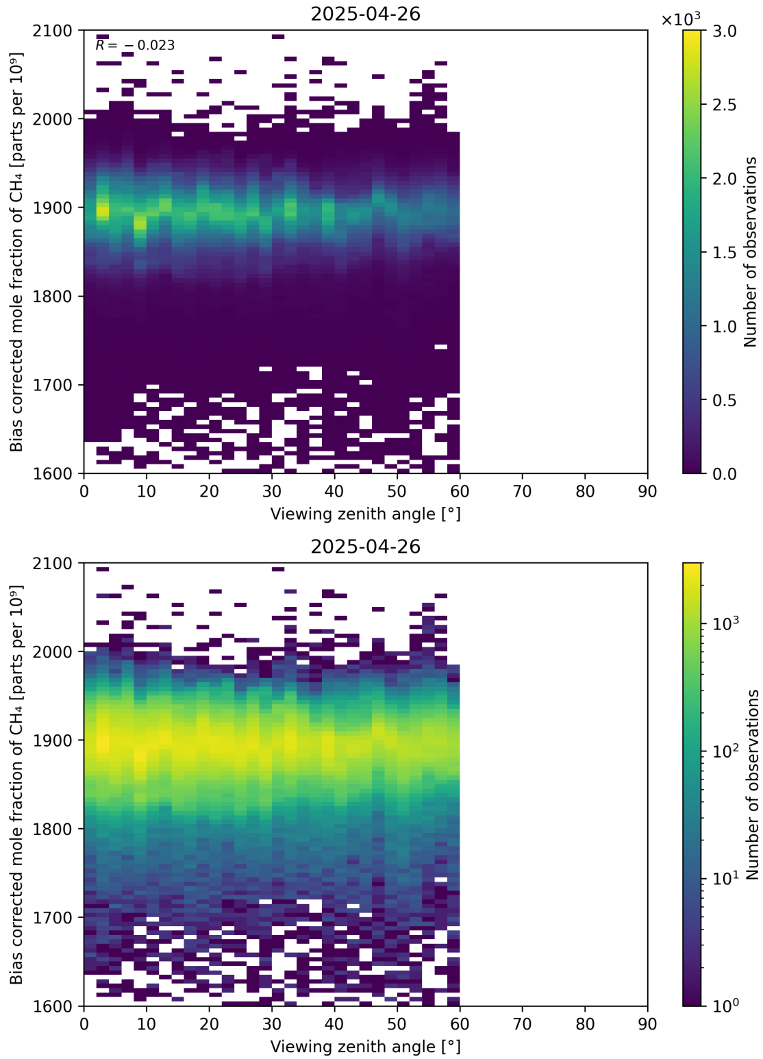
Figure 111: Scatter density plot of “Viewing zenith angle” against “Bias corrected mole fraction of CH 4 ” for 2025-04-25 to 2025-04-27.
