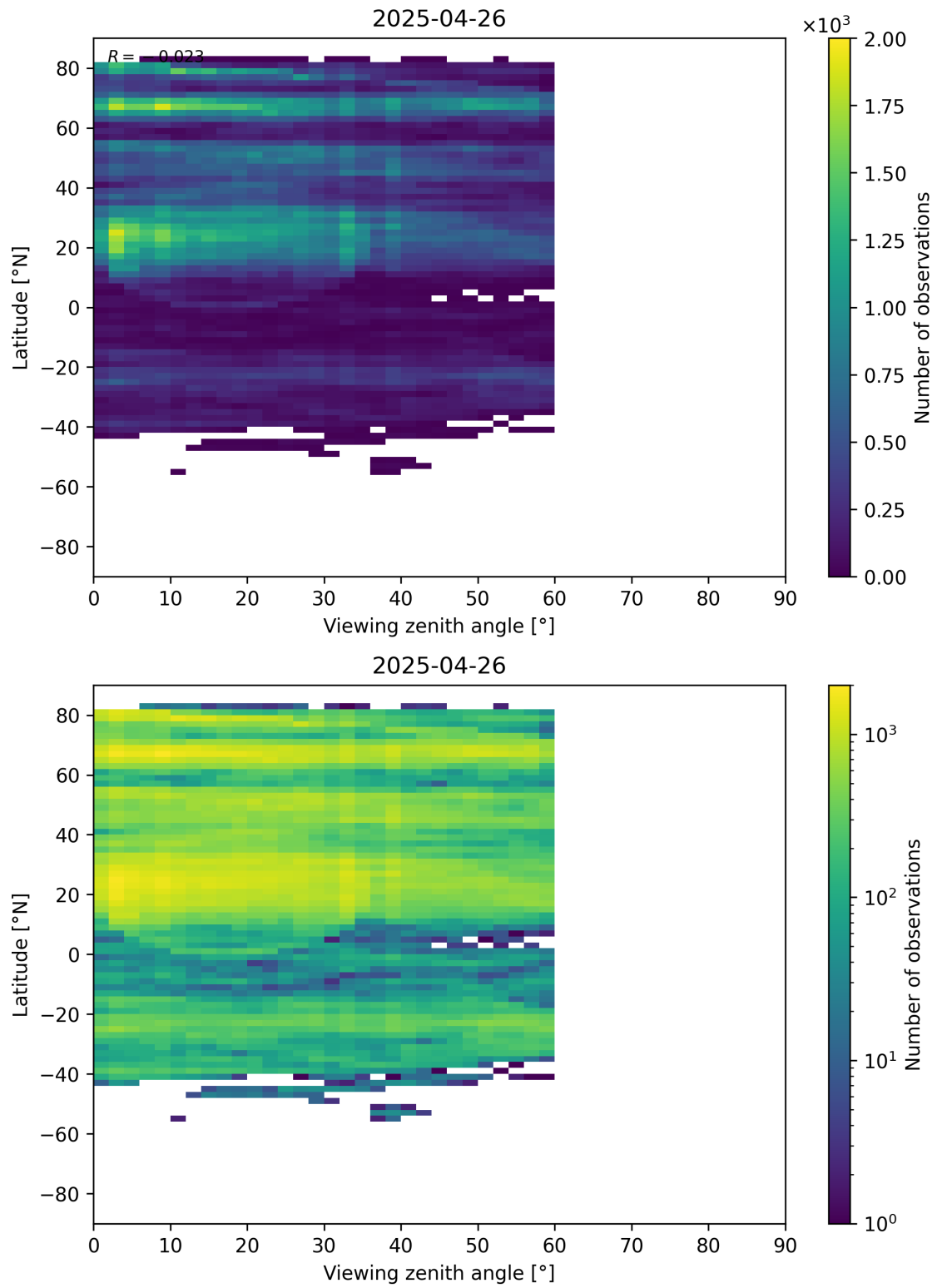
Figure 109: Scatter density plot of “Viewing zenith angle” against “Latitude” for 2025-04-25 to 2025-04-27.
