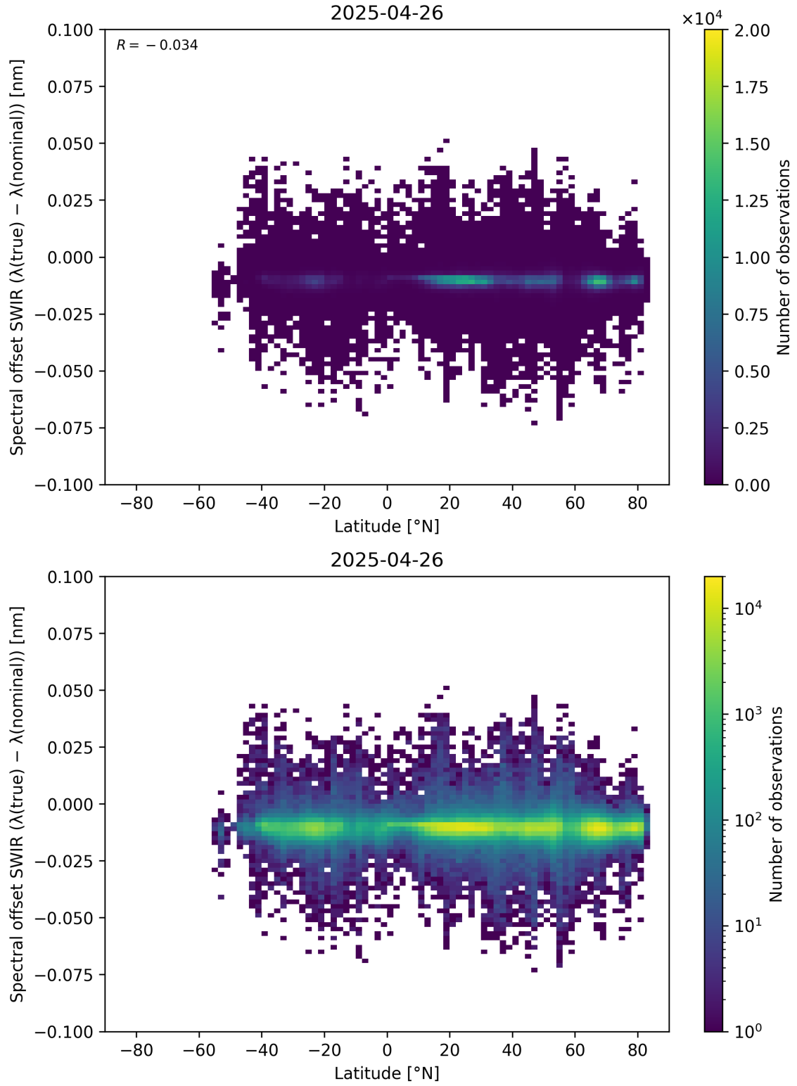
Figure 62: Scatter density plot of “Latitude” against “Spectral offset SWIR ( \lambda_{\text{true}} - \lambda_{\text{nominal}} )” for 2025-04-25 to 2025-04-27.
