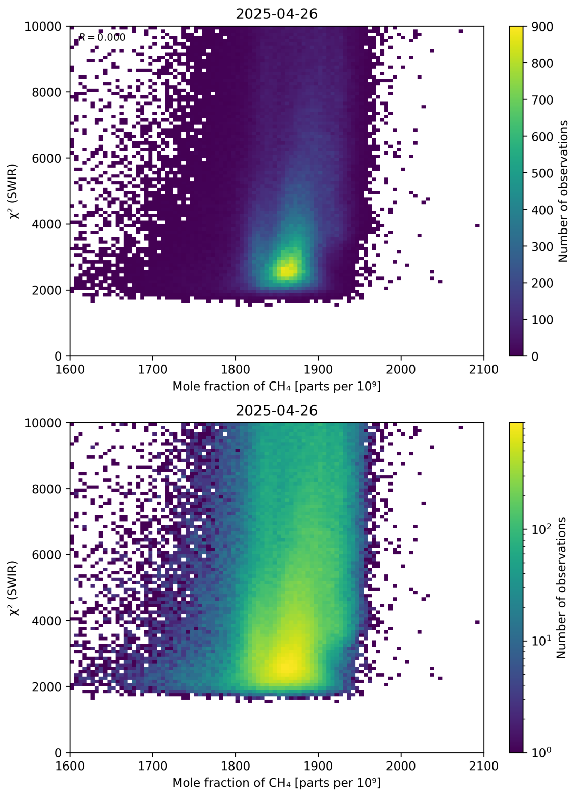
Figure 71: Scatter density plot of “Mole fraction of \text{CH}_4 ” against “ \chi^2 (SWIR)” for 2025-04-25 to 2025-04-27.
