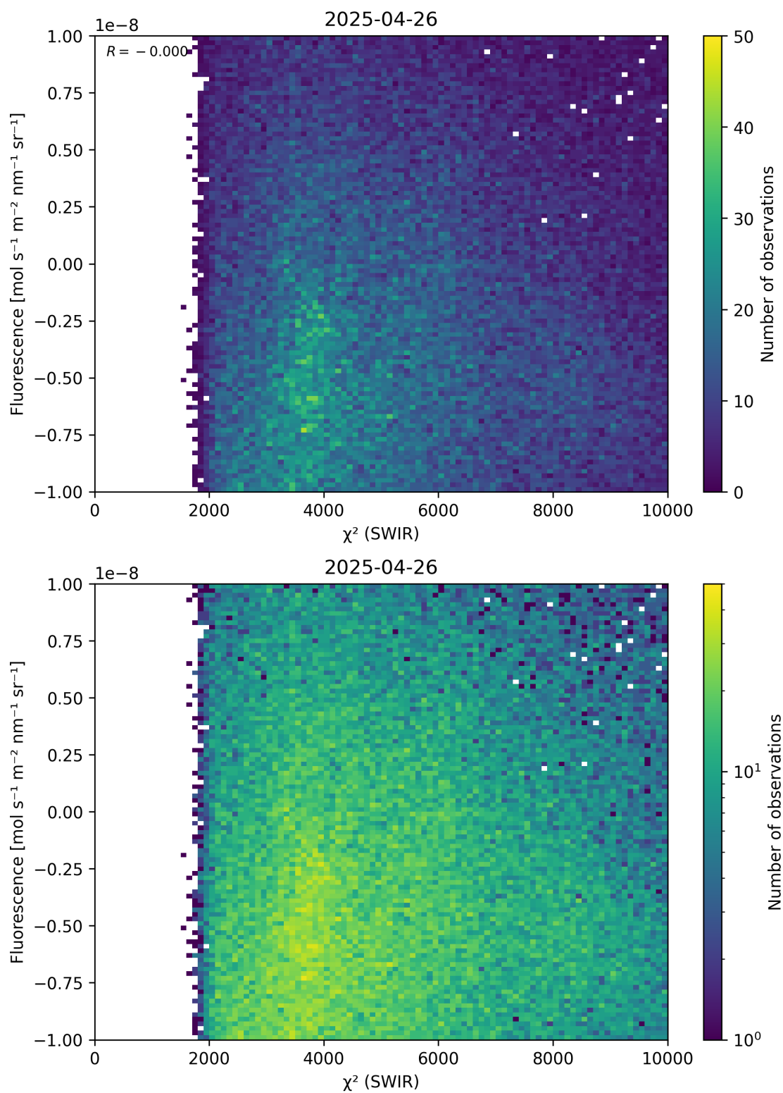
Figure 49: Scatter density plot of “ \chi^2 (SWIR)” against “Fluorescence” for 2025-04-25 to 2025-04-27.
