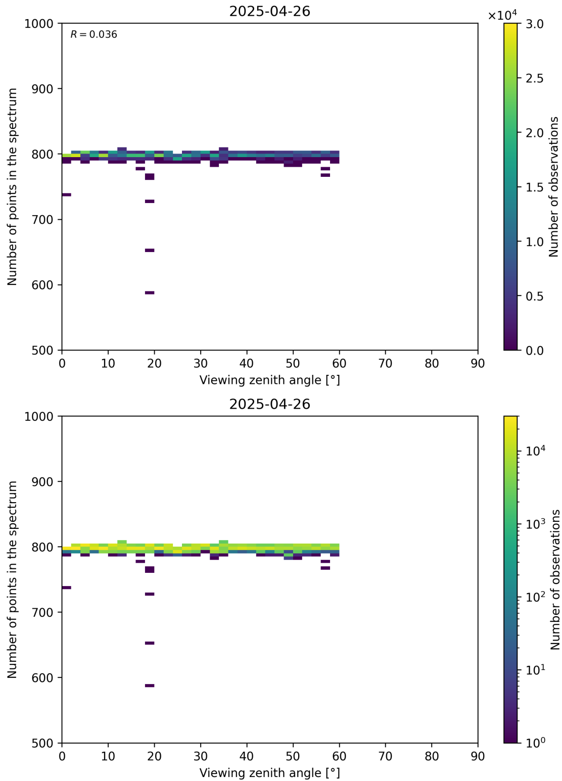
Figure 114: Scatter density plot of “Viewing zenith angle” against “Number of points in the spectrum” for 2025-04-25 to 2025-04-27.
