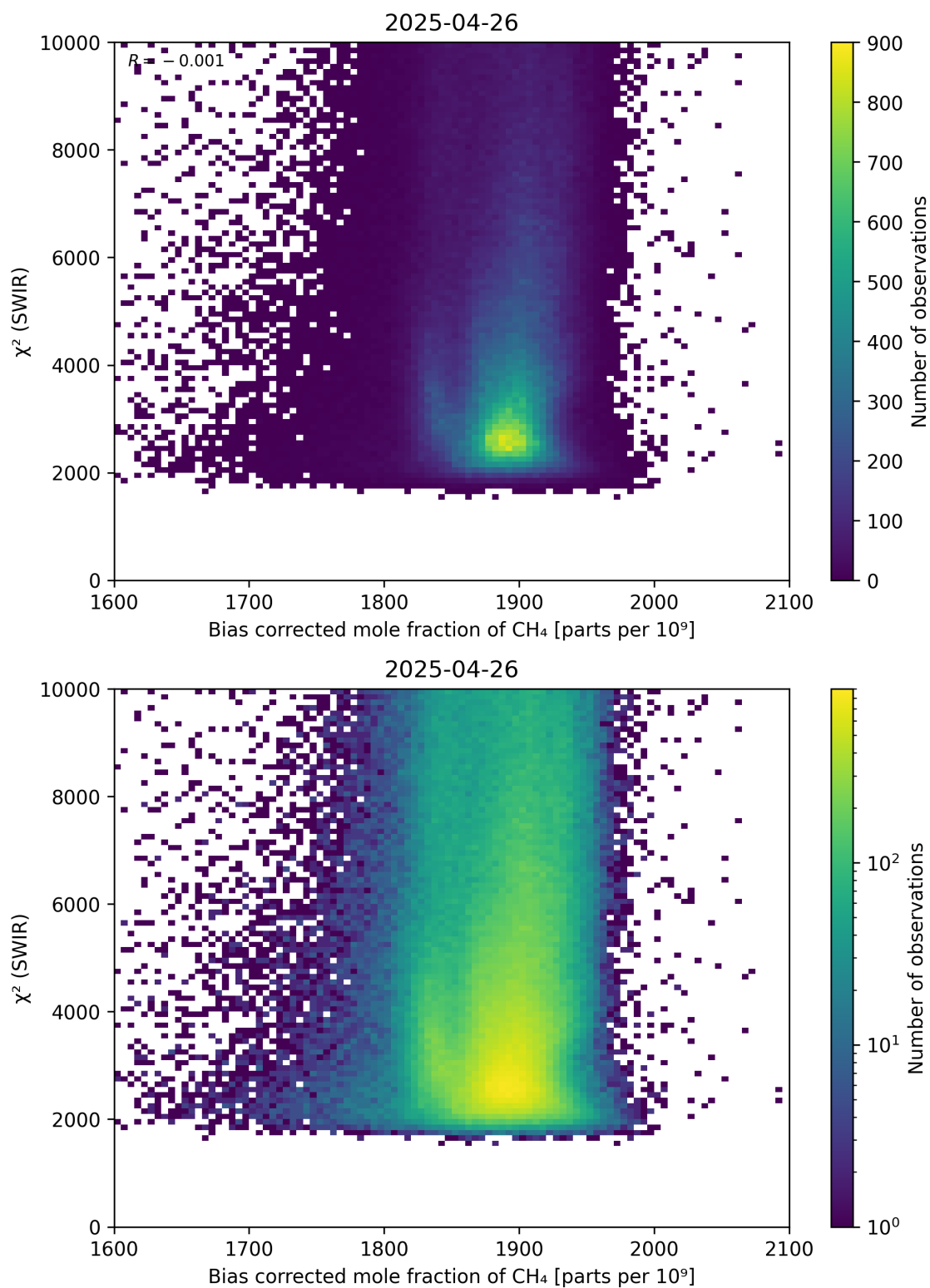
Figure 64: Scatter density plot of “Bias corrected mole fraction of \text{CH}_4 ” against “ \chi^2 (SWIR)” for 2025-04-25 to 2025-04-27.
