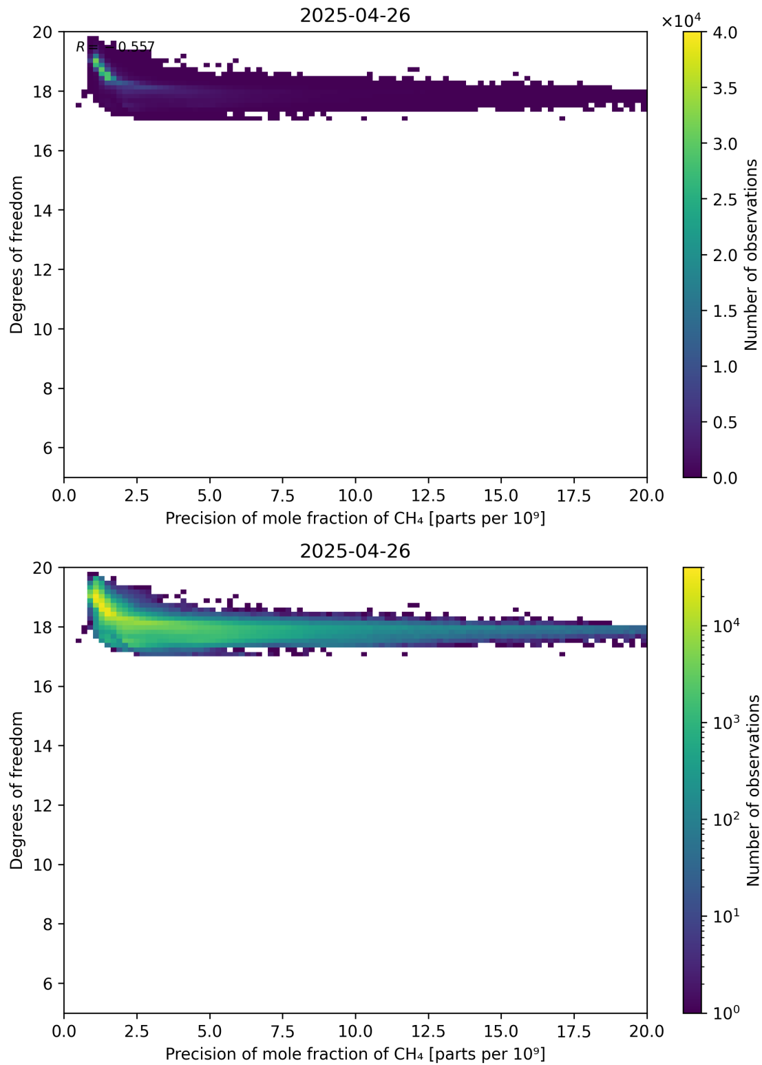
Figure 80: Scatter density plot of “Precision of mole fraction of CH 4 ” against “Degrees of freedom” for 2025-04-25 to 2025-04-27.
