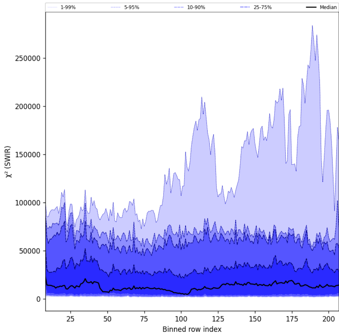
Figure 39: Along track statistics of “ \chi^2 (SWIR)” for 2025-04-25 to 2025-04-27
