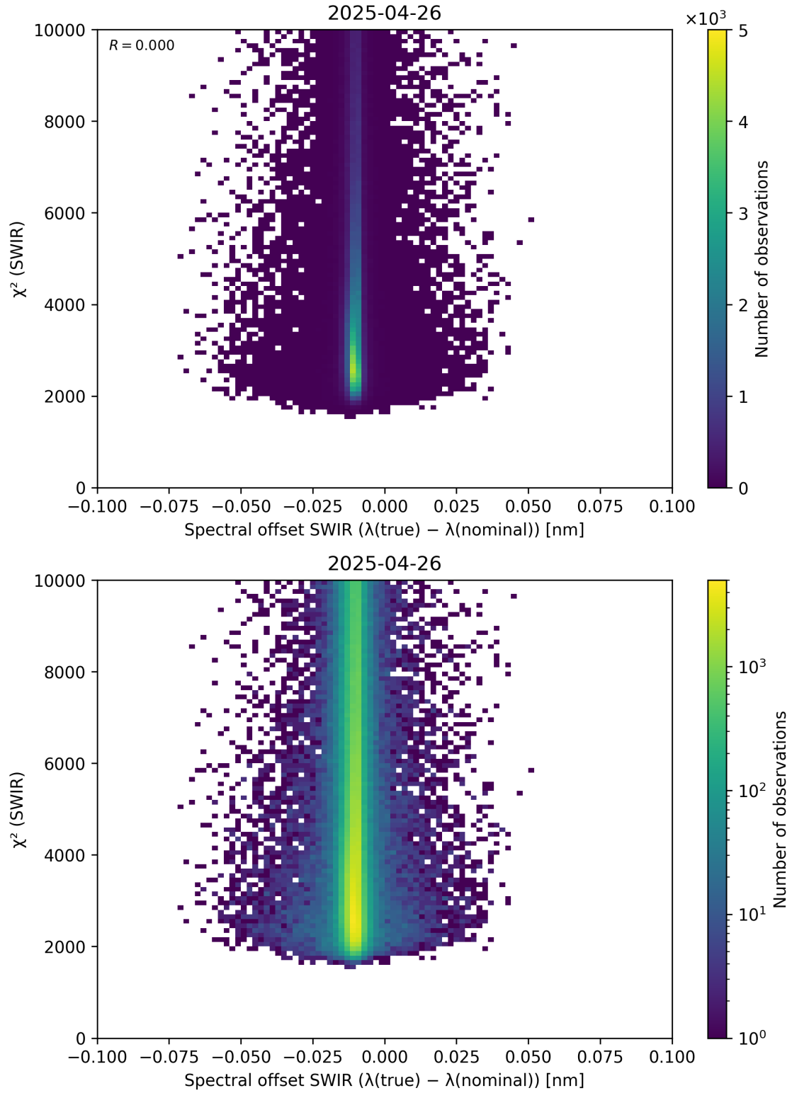
Figure 118: Scatter density plot of “Spectral offset SWIR ( \lambda_{\text{true}} - \lambda_{\text{nominal}} )” against “ \chi^2 (SWIR)” for 2025-04-25 to 2025-04-27.
