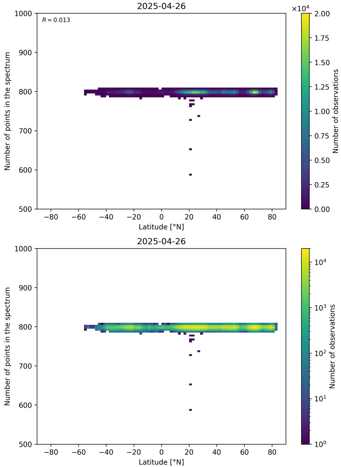
Figure 61: Scatter density plot of “Latitude” against “Number of points in the spectrum” for 2025-04-25 to 2025-04-27.
