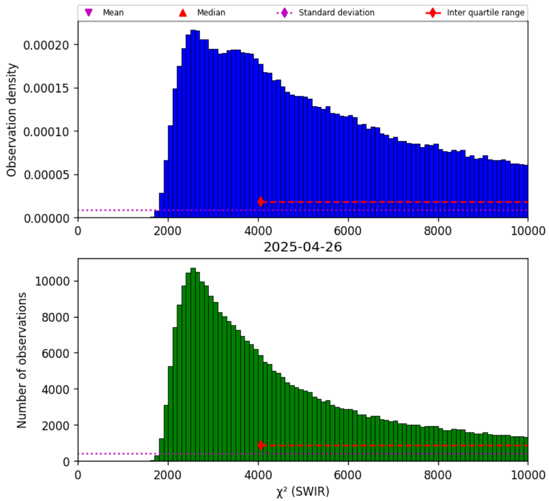
Figure 28: Histogram of " \chi^2 (SWIR)" for 2025-04-25 to 2025-04-27
