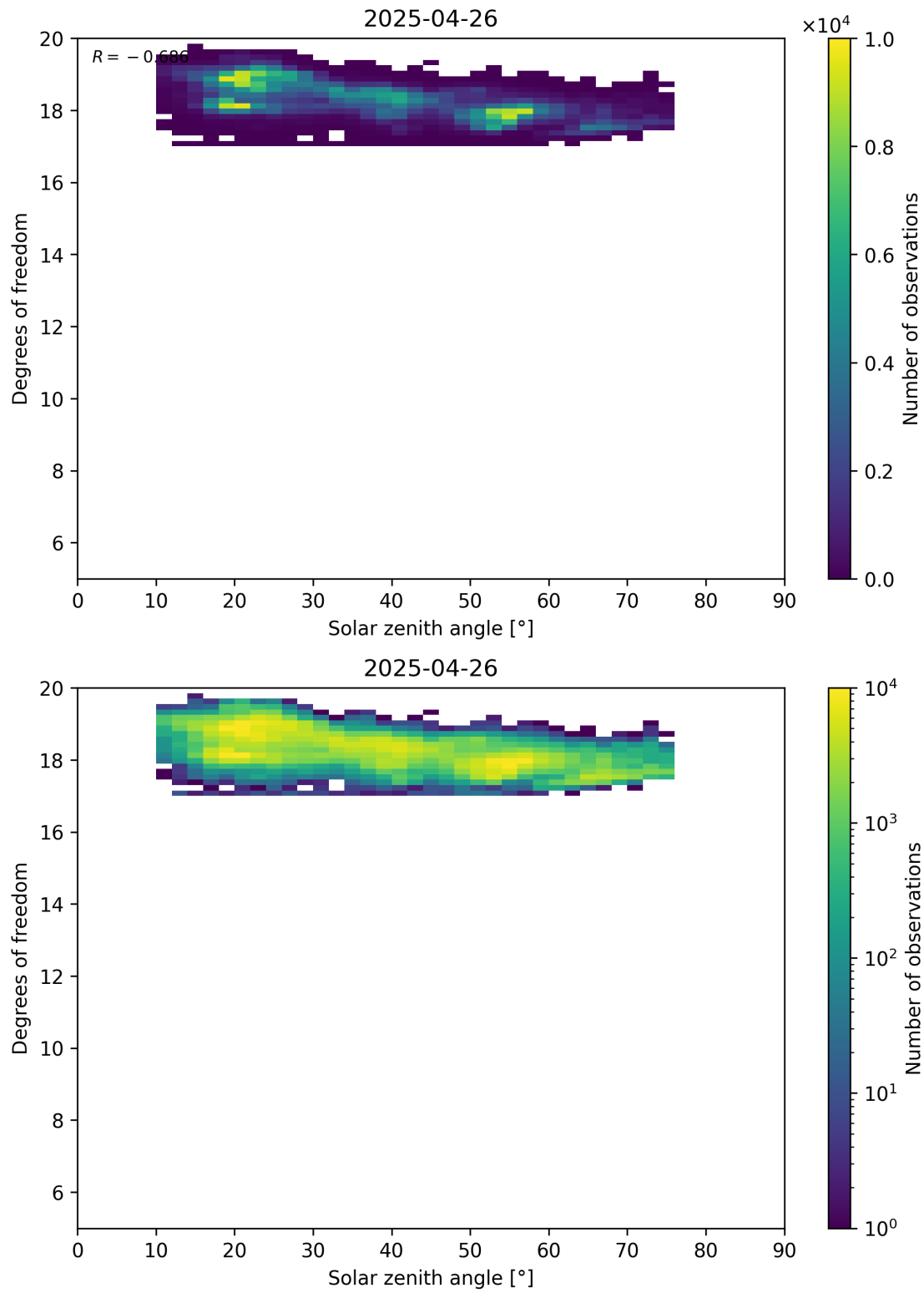
Figure 96: Scatter density plot of “Solar zenith angle” against “Degrees of freedom” for 2025-04-25 to 2025-04-27.
