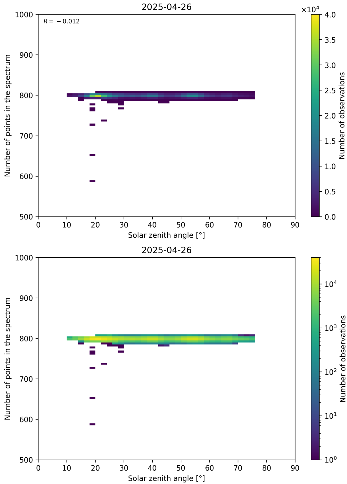
Figure 103: Scatter density plot of “Solar zenith angle” against “Number of points in the spectrum” for 2025-04-25 to 2025-04-27.
