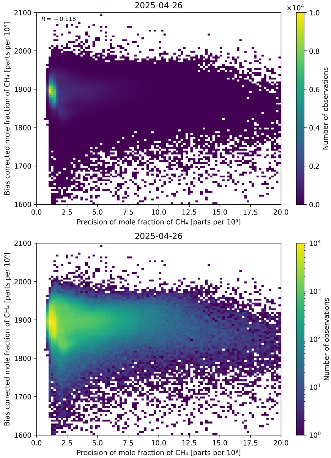
Figure 82: Scatter density plot of “Precision of mole fraction of CH 4 ” against “Bias corrected mole fraction of CH 4 ” for 2025-04-25 to 2025-04-27.
