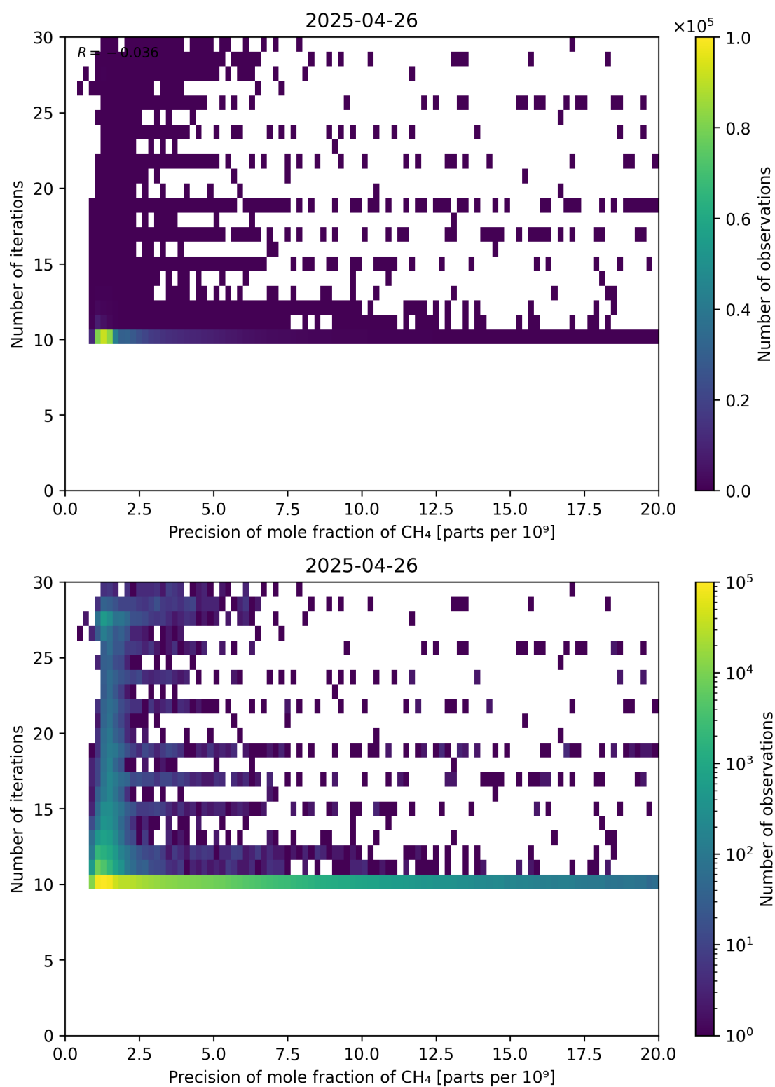
Figure 83: Scatter density plot of “Precision of mole fraction of \text{CH}_4 ” against “Number of iterations” for 2025-04-25 to 2025-04-27.
