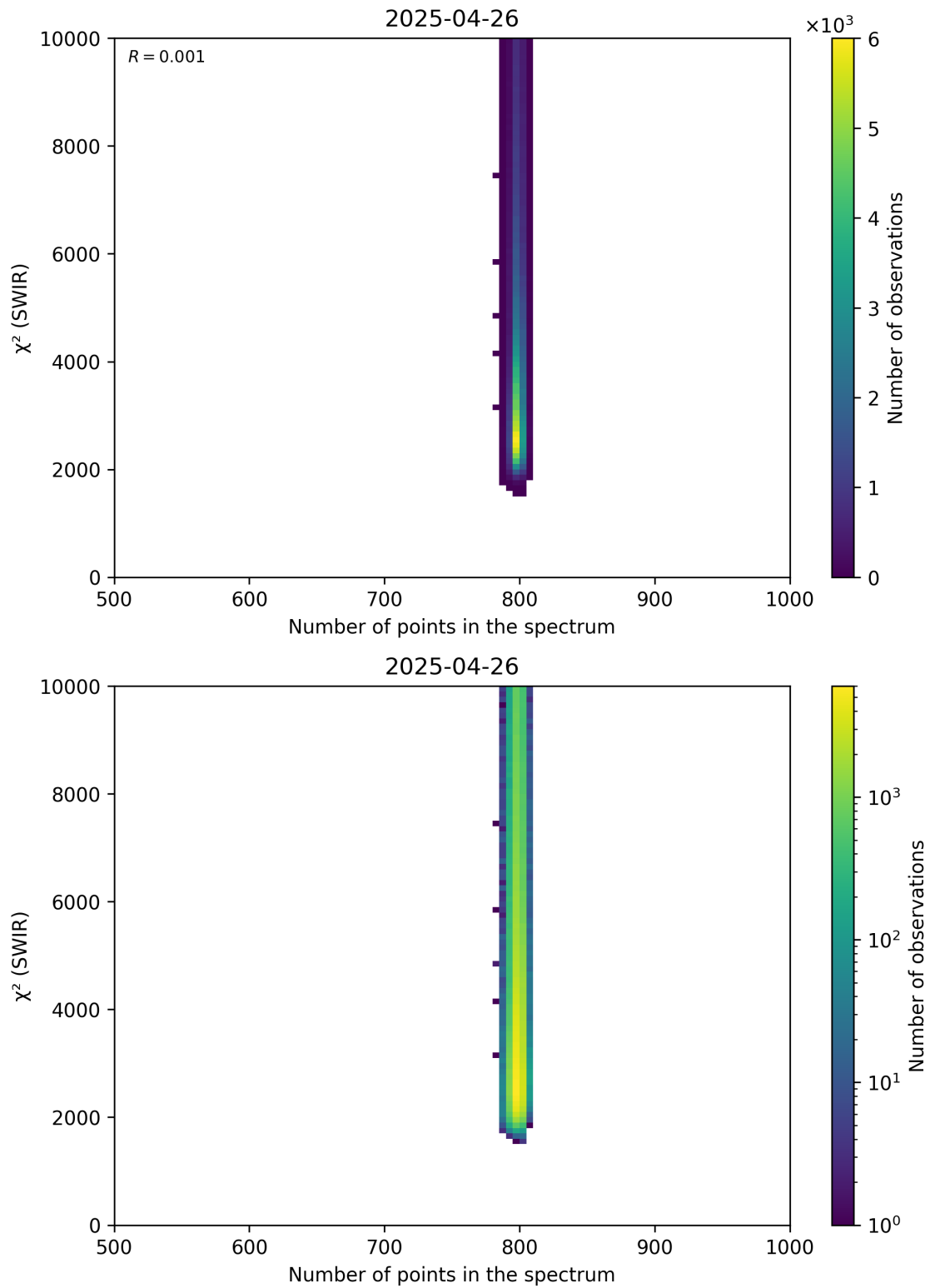
Figure 89: Scatter density plot of “Number of points in the spectrum” against “ \chi^2 (SWIR)” for 2025-04-25 to 2025-04-27.
