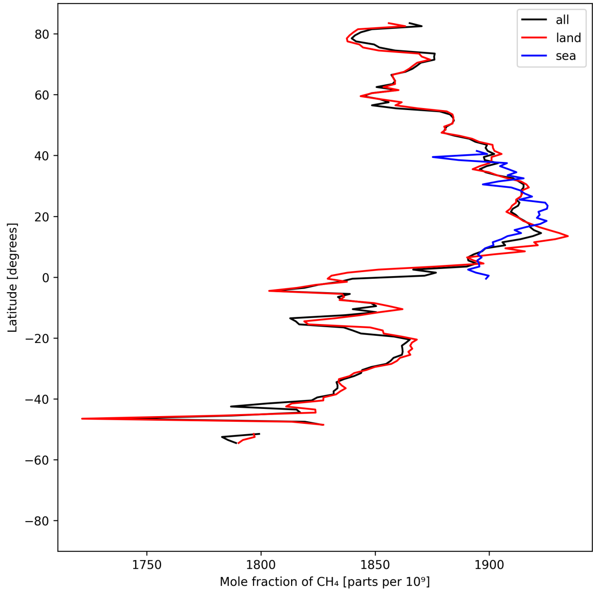
Figure 12: Zonal average of “Mole fraction of CH 4 ” for 2025-04-25 to 2025-04-27.
