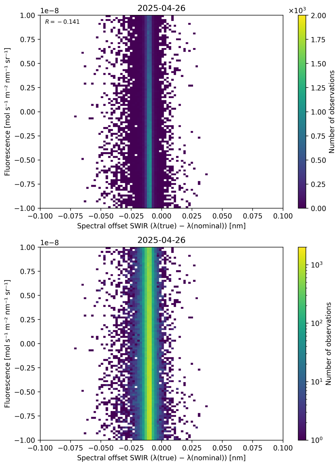
Figure 120: Scatter density plot of “Spectral offset SWIR ( \lambda_{\text{true}} - \lambda_{\text{nominal}} )” against “Fluorescence” for 2025-04-25 to 2025-04-27.
