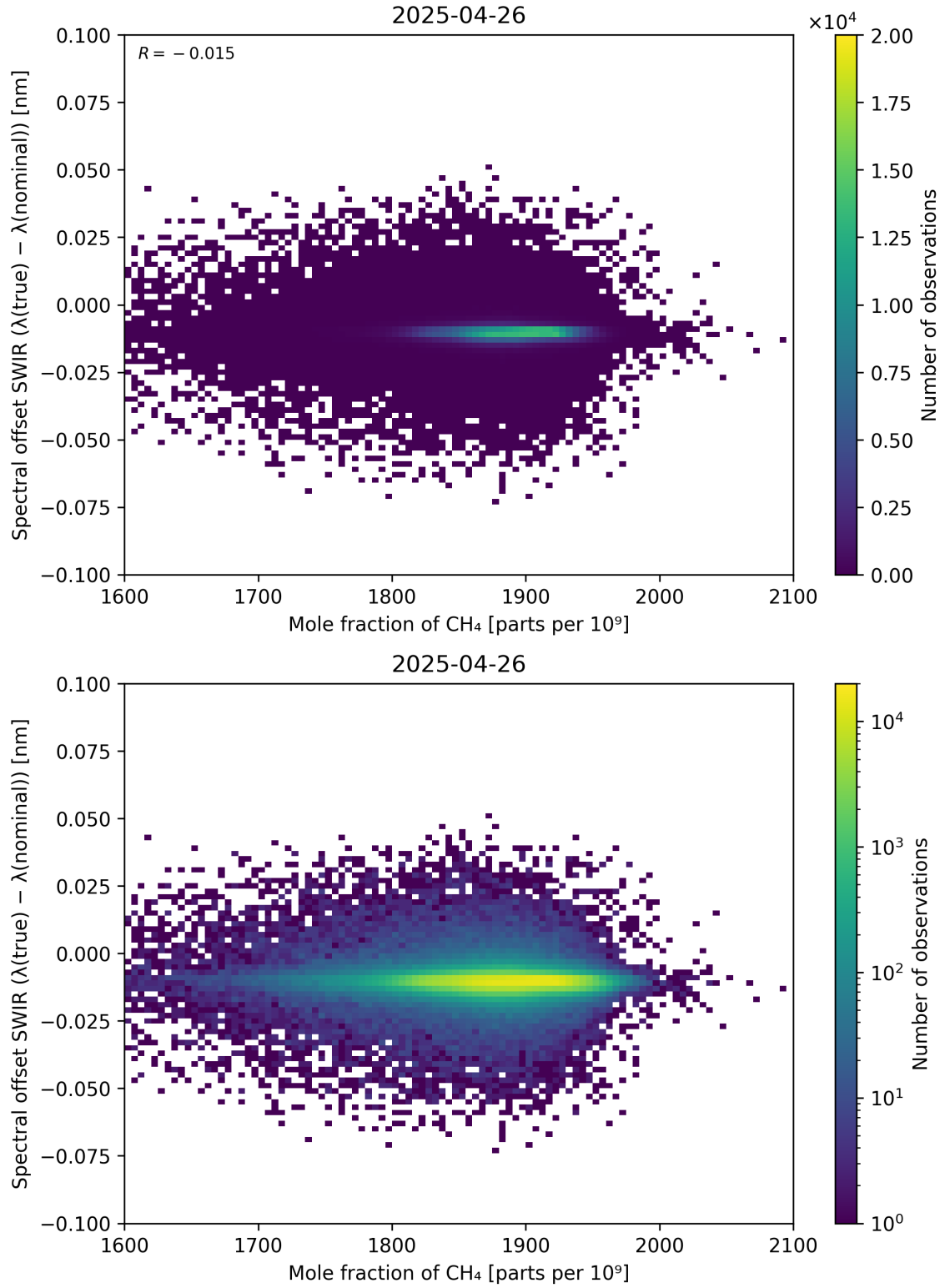
Figure 86: Scatter density plot of “Mole fraction of CH 4 ” against “Spectral offset SWIR ( \lambda_{\text{true}} - \lambda_{\text{nominal}} )” for 2025-04-25 to 2025-04-27.
