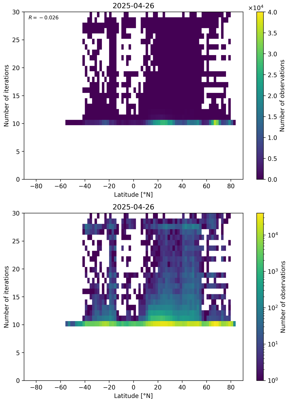
Figure 60: Scatter density plot of “Latitude” against “Number of iterations” for 2025-04-25 to 2025-04-27.
