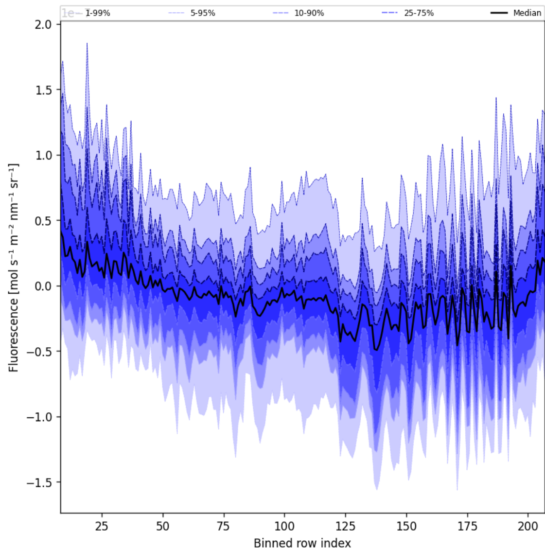
Figure 43: Along track statistics of “Fluorescence” for 2025-04-25 to 2025-04-27
