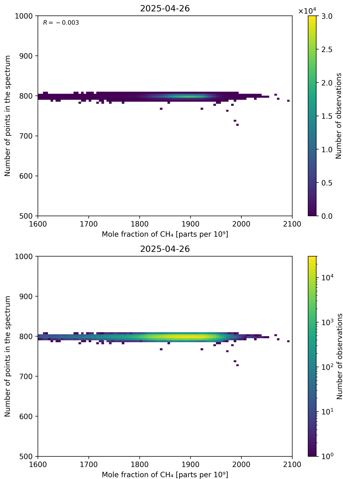
Figure 77: Scatter density plot of “Mole fraction of CH 4 ” against “Number of points in the spectrum” for 2025-04-25 to 2025-04-27.
