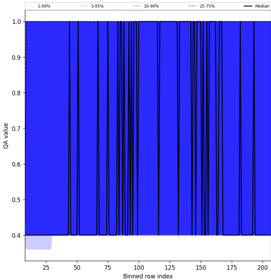
Figure 33: Along track statistics of “QA value” for 2025-04-25 to 2025-04-27
