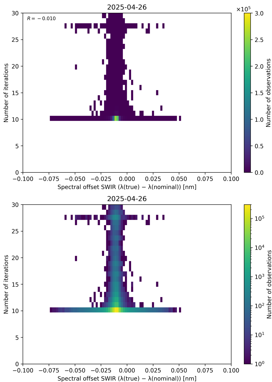
Figure 121: Scatter density plot of “Spectral offset SWIR ( \lambda_{\text{true}} - \lambda_{\text{nominal}} )” against “Number of iterations” for 2025-04-25 to 2025-04-27.
