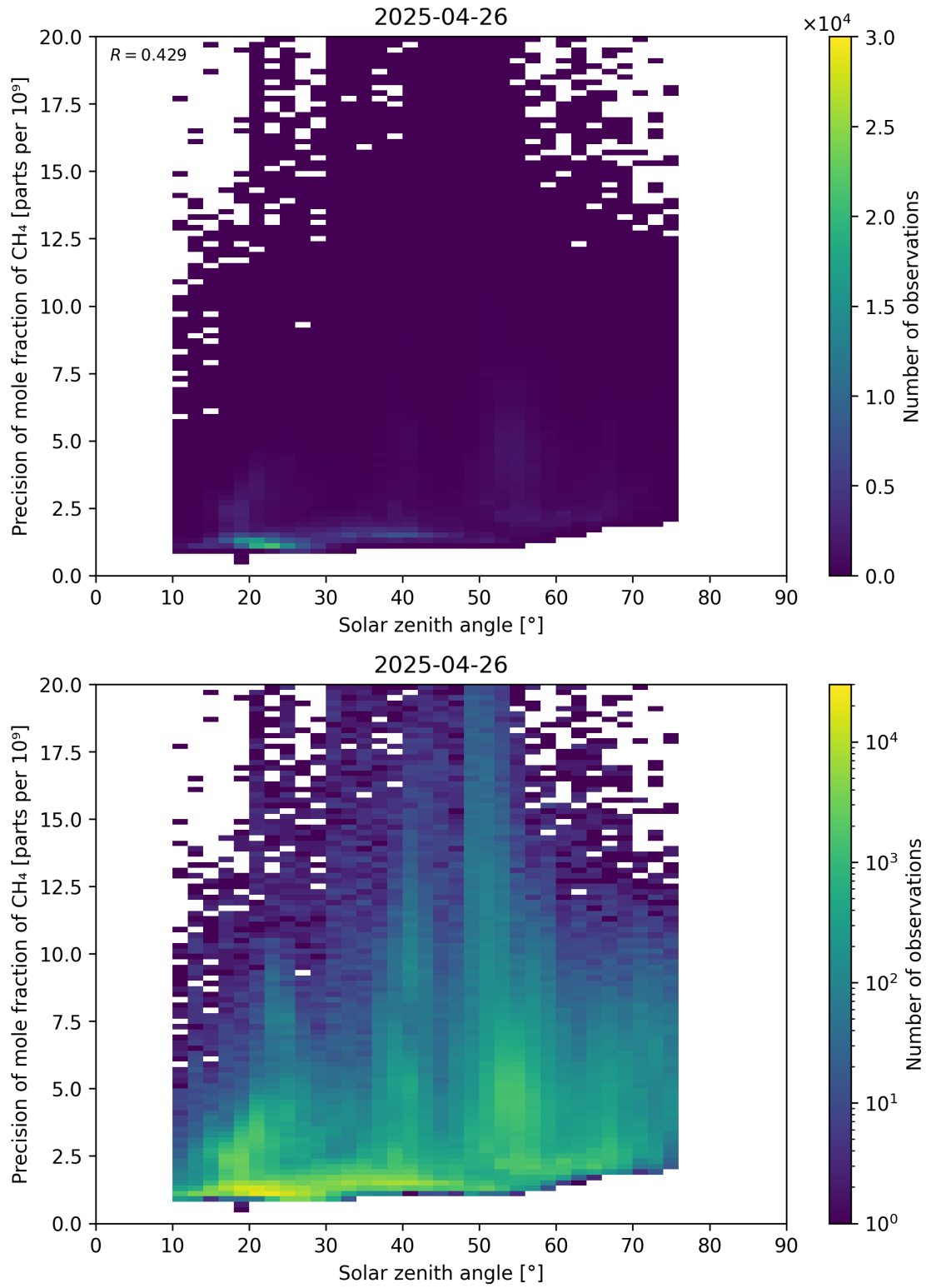
Figure 101: Scatter density plot of “Solar zenith angle” against “Precision of mole fraction of \text{CH}_4 ” for 2025-04-25 to 2025-04-27.
