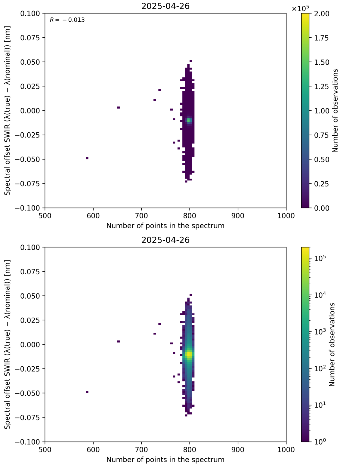
Figure 93: Scatter density plot of “Number of points in the spectrum” against “Spectral offset SWIR ( \lambda_{\text{true}} - \lambda_{\text{nominal}} )” for 2025-04-25 to 2025-04-27.
