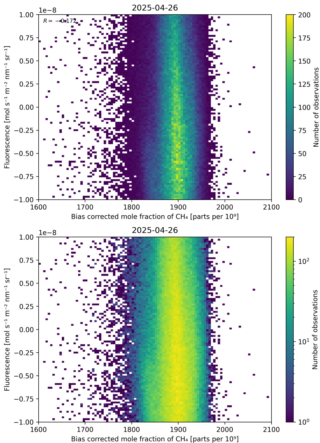
Figure 66: Scatter density plot of “Bias corrected mole fraction of \text{CH}_4 ” against “Fluorescence” for 2025-04-25 to 2025-04-27.
