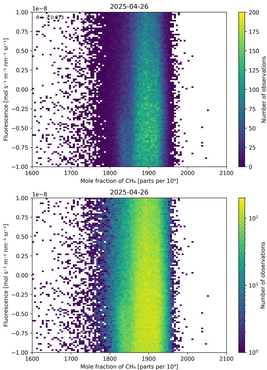
Figure 73: Scatter density plot of “Mole fraction of \text{CH}_4 ” against “Fluorescence” for 2025-04-25 to 2025-04-27.
