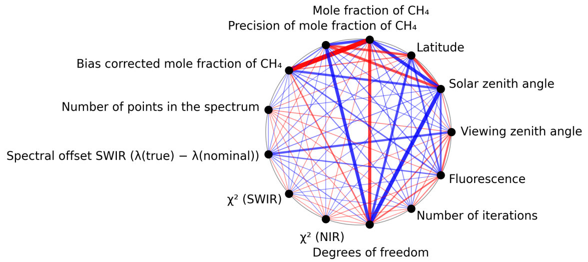
Figure 1: Map of correlation graph for 2025-04-25 to 2025-04-27.
