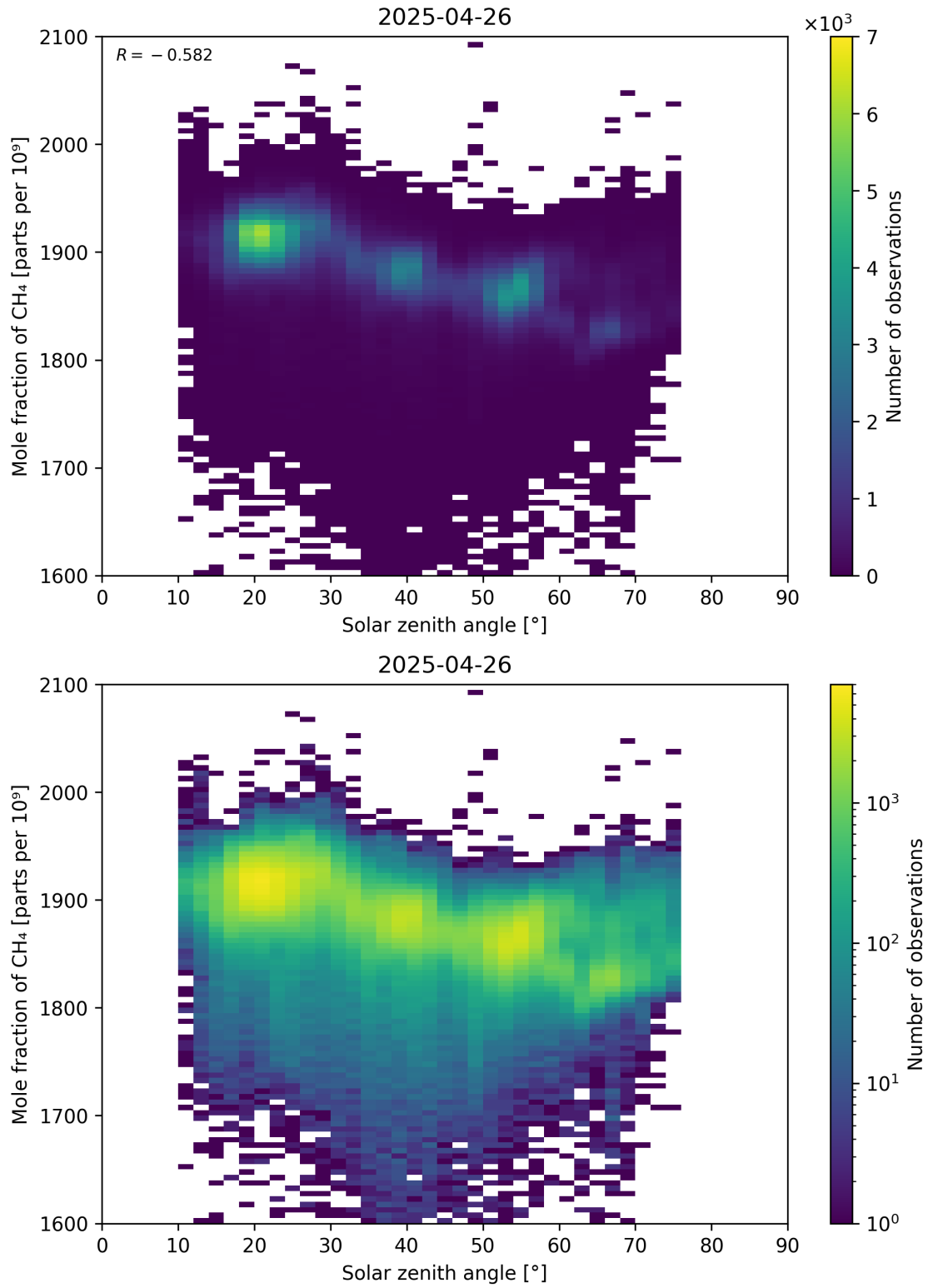
Figure 99: Scatter density plot of “Solar zenith angle” against “Mole fraction of CH 4 ” for 2025-04-25 to 2025-04-27.
