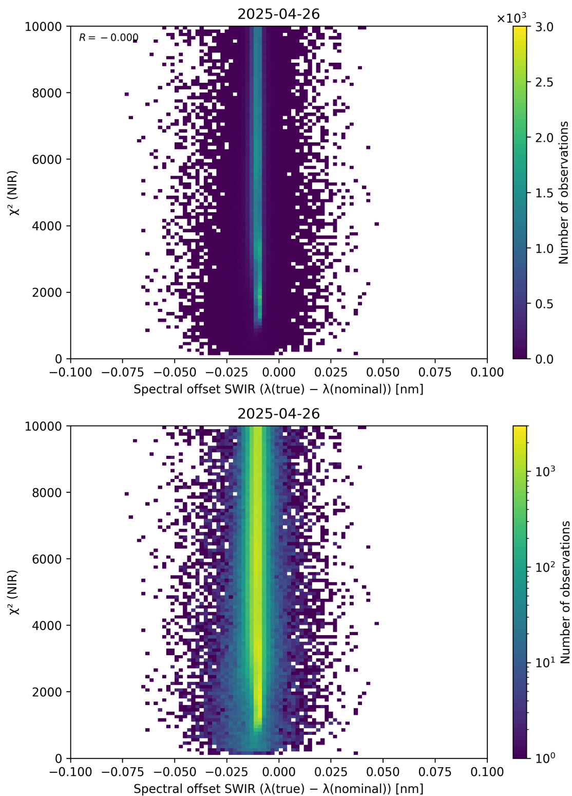
Figure 117: Scatter density plot of “Spectral offset SWIR ( \lambda_{\text{true}} - \lambda_{\text{nominal}} )” against “ \chi^2 (NIR)” for 2025-04-25 to 2025-04-27.
