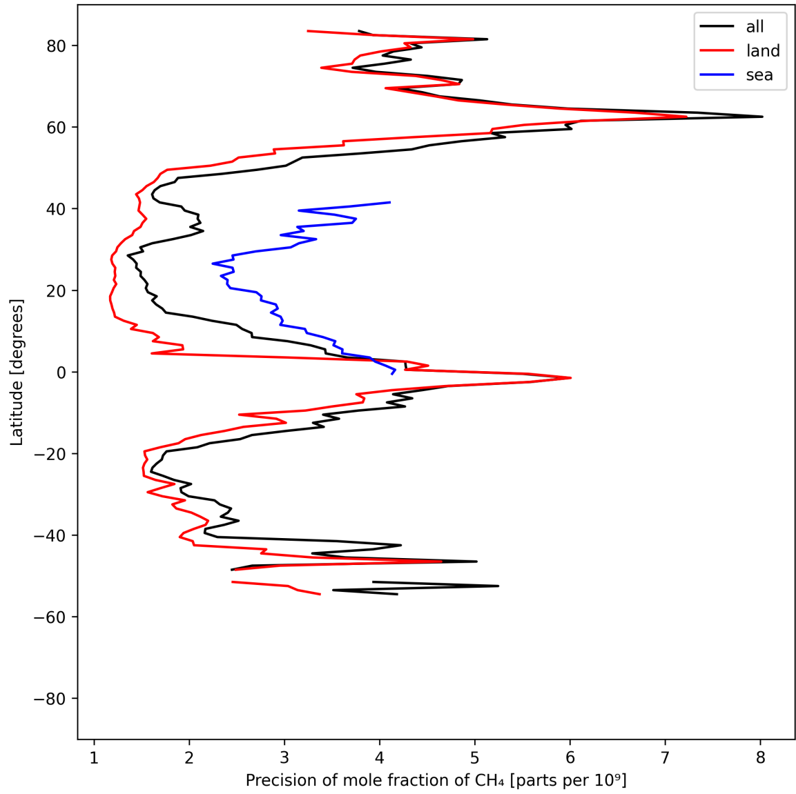
Figure 13: Zonal average of “Precision of mole fraction of CH 4 ” for 2025-04-25 to 2025-04-27.
