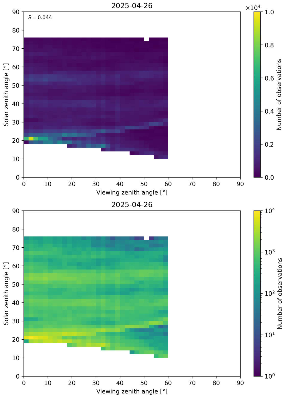
Figure 115: Scatter density plot of “Viewing zenith angle” against “Solar zenith angle” for 2025-04-25 to 2025-04-27.
