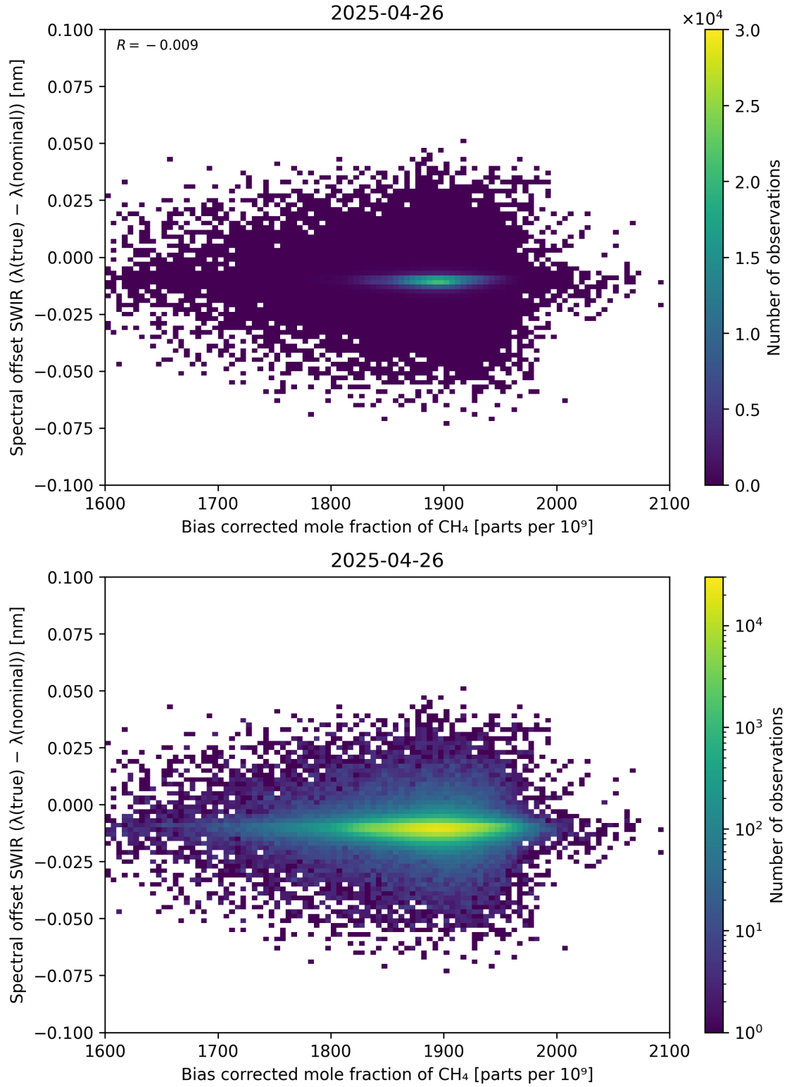
Figure 69: Scatter density plot of “Bias corrected mole fraction of \text{CH}_4 ” against “Spectral offset SWIR ( \lambda_{\text{true}} - \lambda_{\text{nominal}} )” for 2025-04-25 to 2025-04-27.
