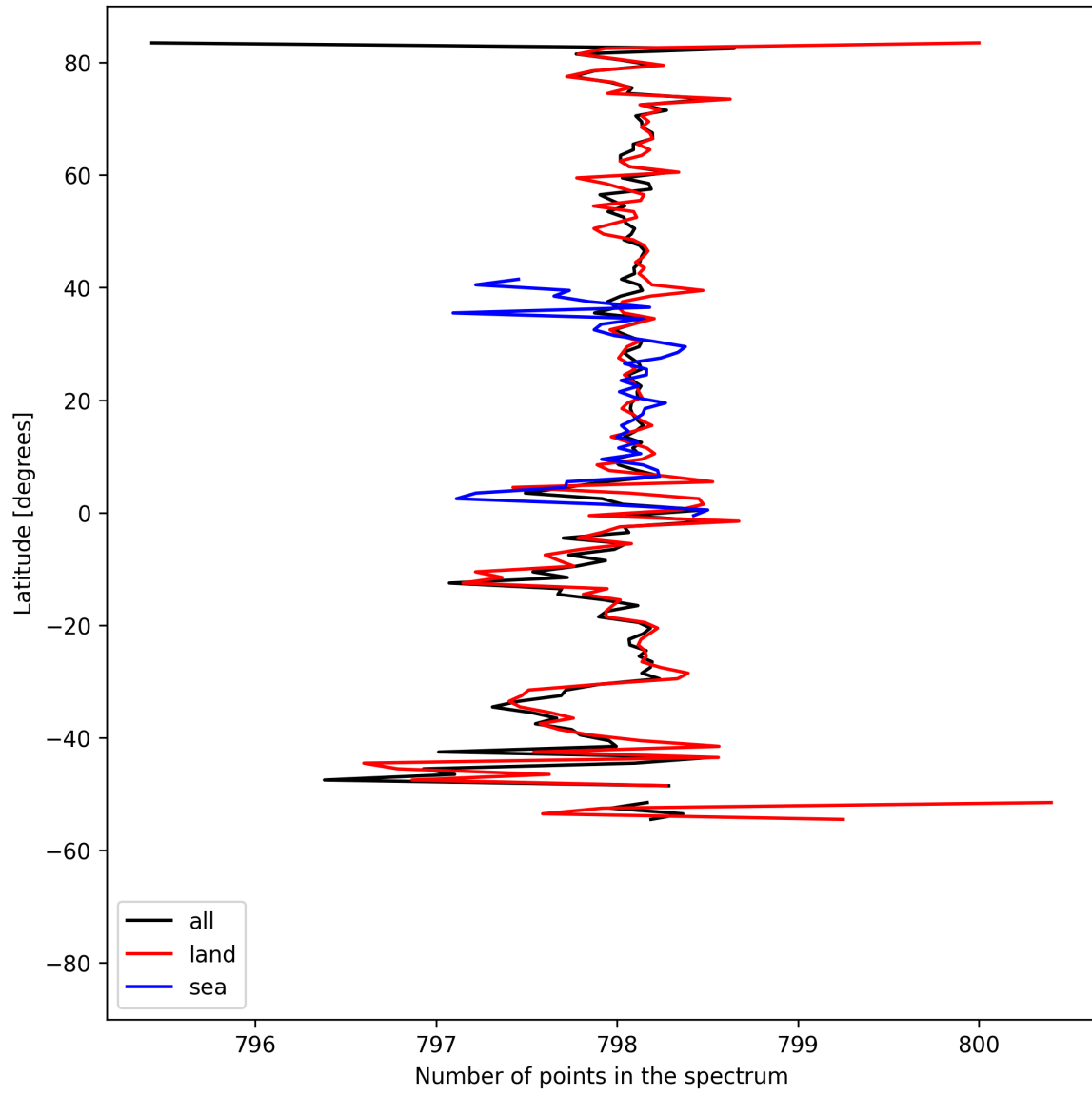
Figure 15: Zonal average of “Number of points in the spectrum” for 2025-04-25 to 2025-04-27.
