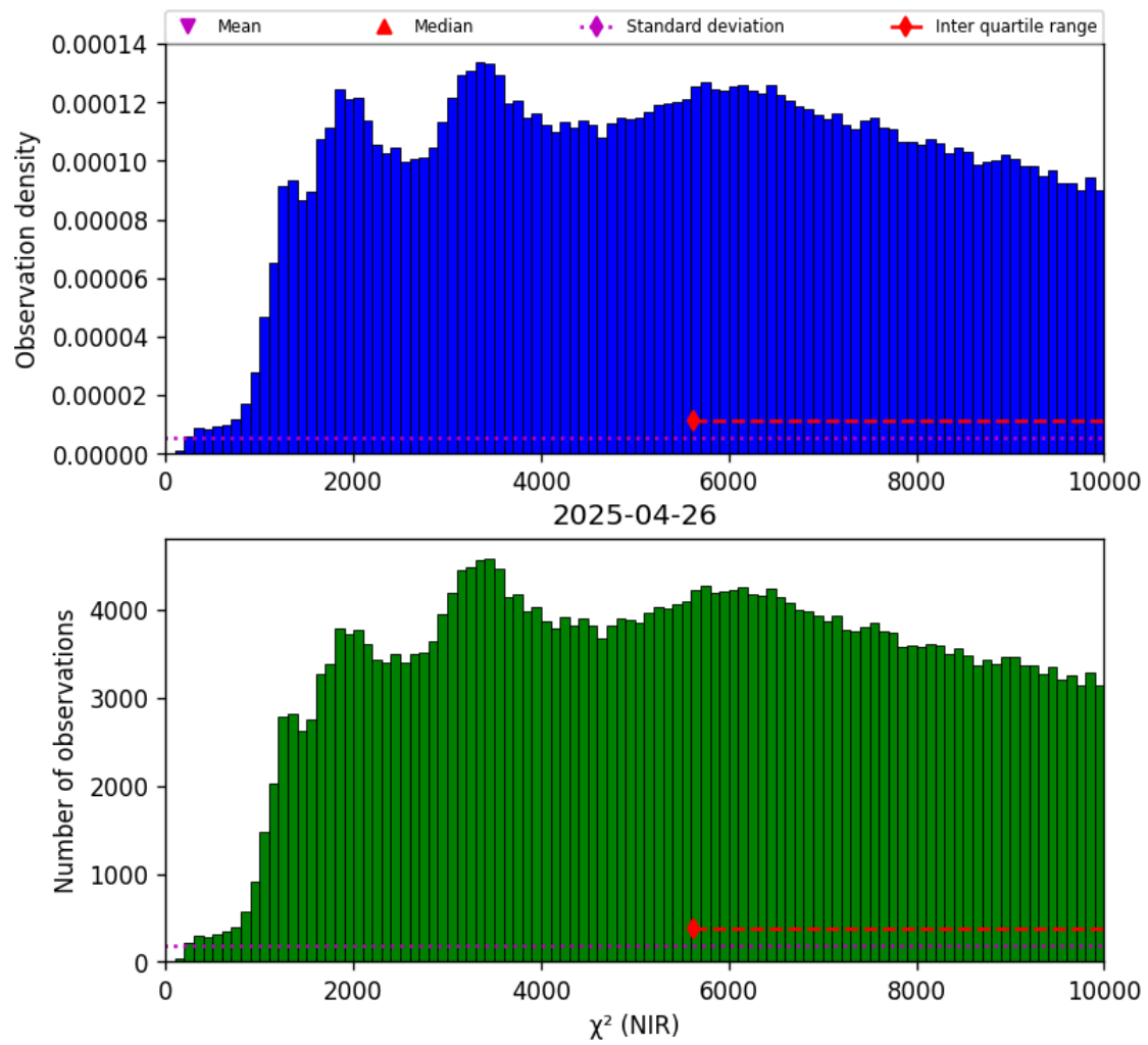
Figure 29: Histogram of “ \chi^2 (NIR)” for 2025-04-25 to 2025-04-27
