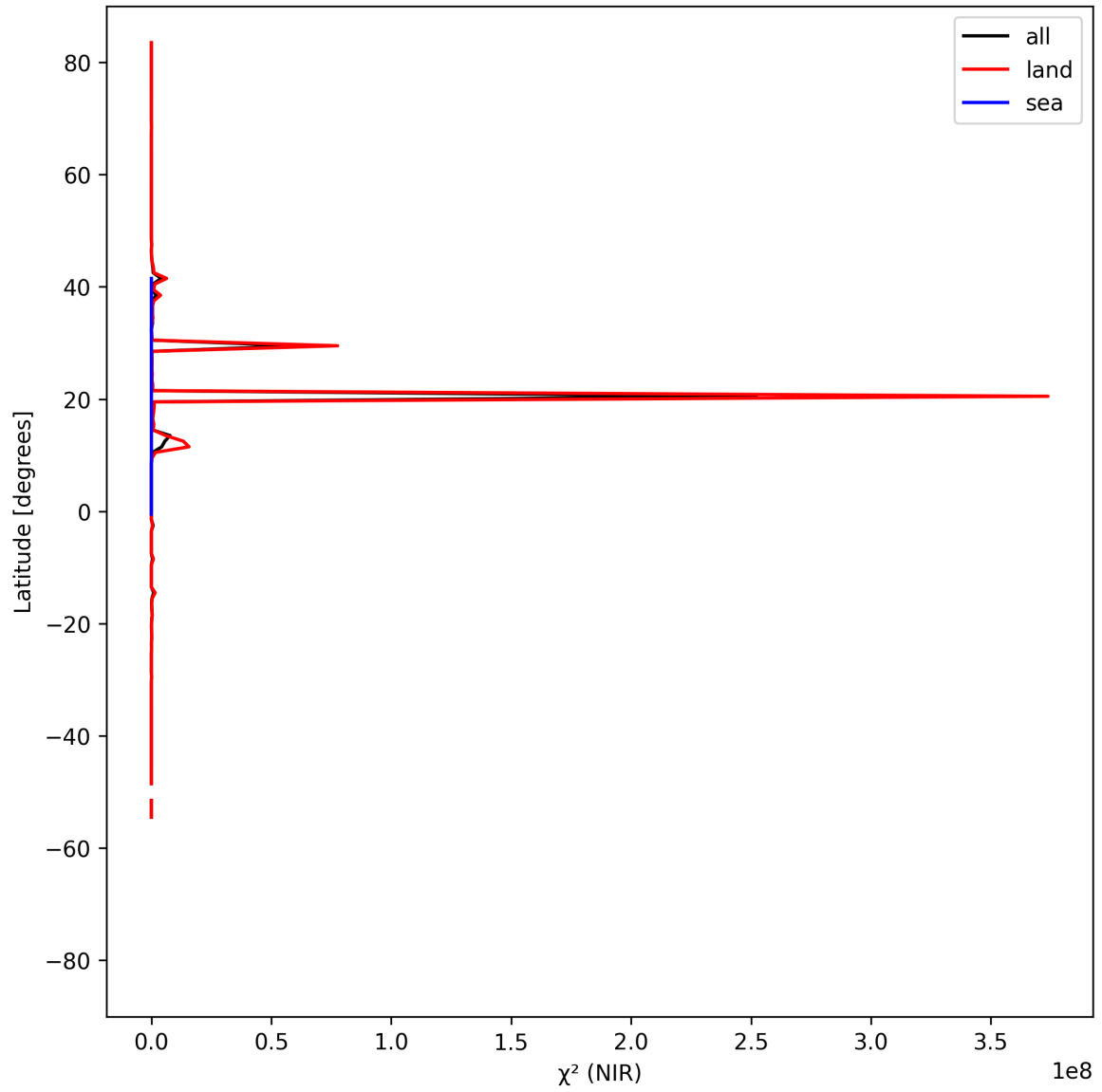
Figure 18: Zonal average of “ \chi^2 (NIR)” for 2025-04-25 to 2025-04-27.
