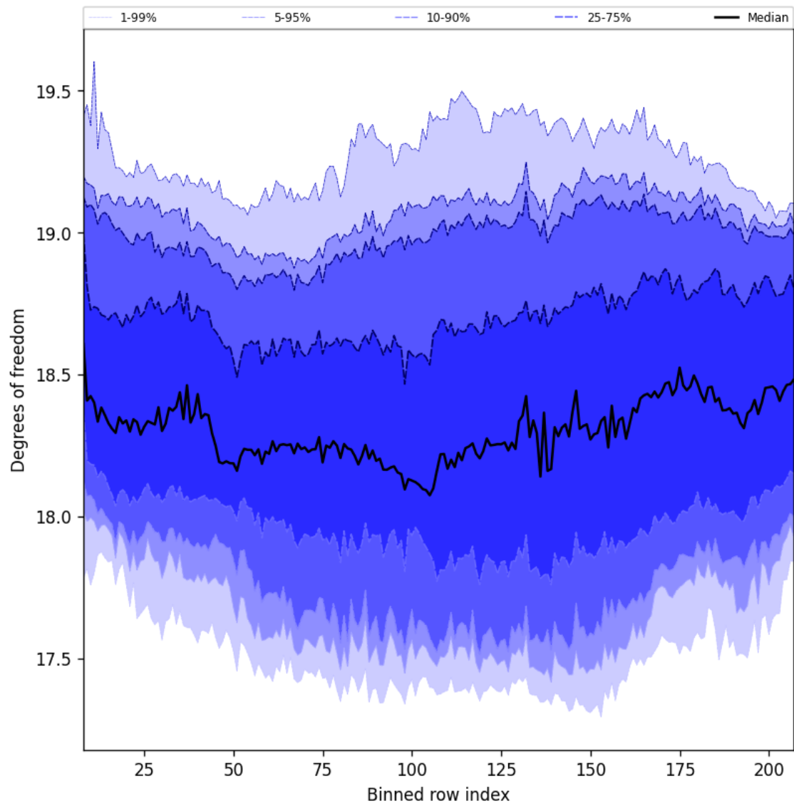
Figure 41: Along track statistics of “Degrees of freedom” for 2025-04-25 to 2025-04-27
