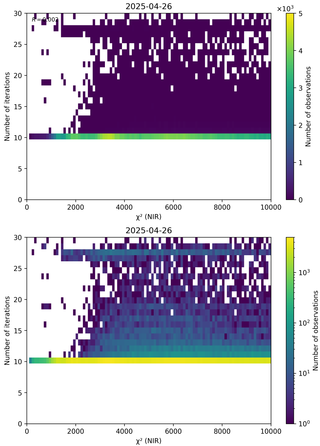
Figure 46: Scatter density plot of “ \chi^2 (NIR)” against “Number of iterations” for 2025-04-25 to 2025-04-27.
