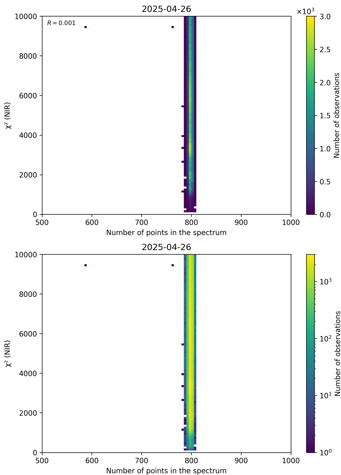
Figure 88: Scatter density plot of “Number of points in the spectrum” against “ \chi^2 (NIR)” for 2025-04-25 to 2025-04-27.
