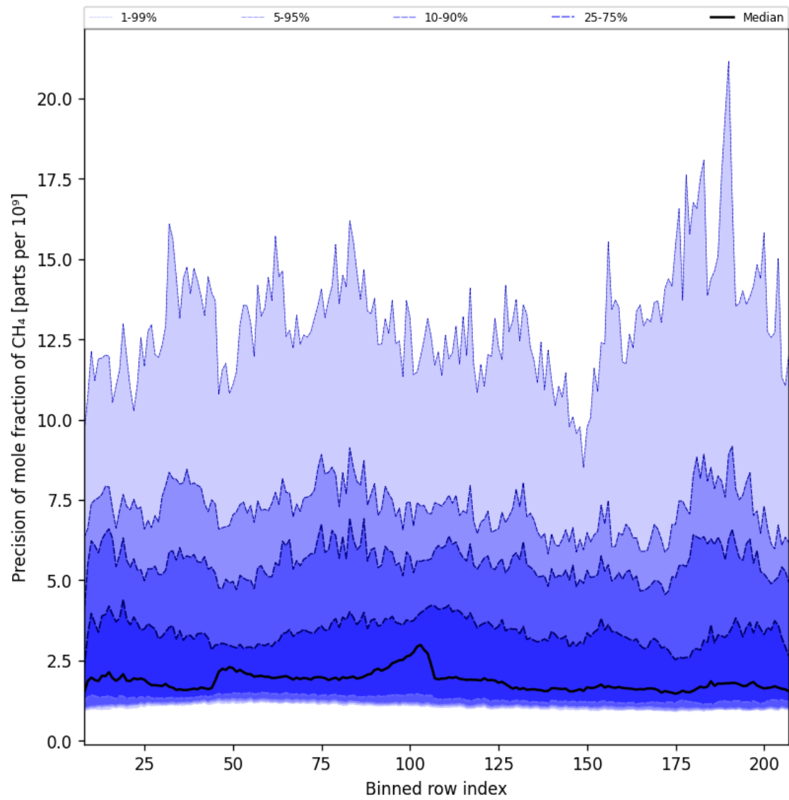
Figure 35: Along track statistics of “Precision of mole fraction of CH 4 ” for 2025-04-25 to 2025-04-27
