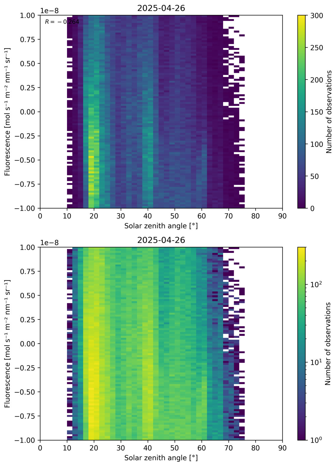
Figure 97: Scatter density plot of “Solar zenith angle” against “Fluorescence” for 2025-04-25 to 2025-04-27.
