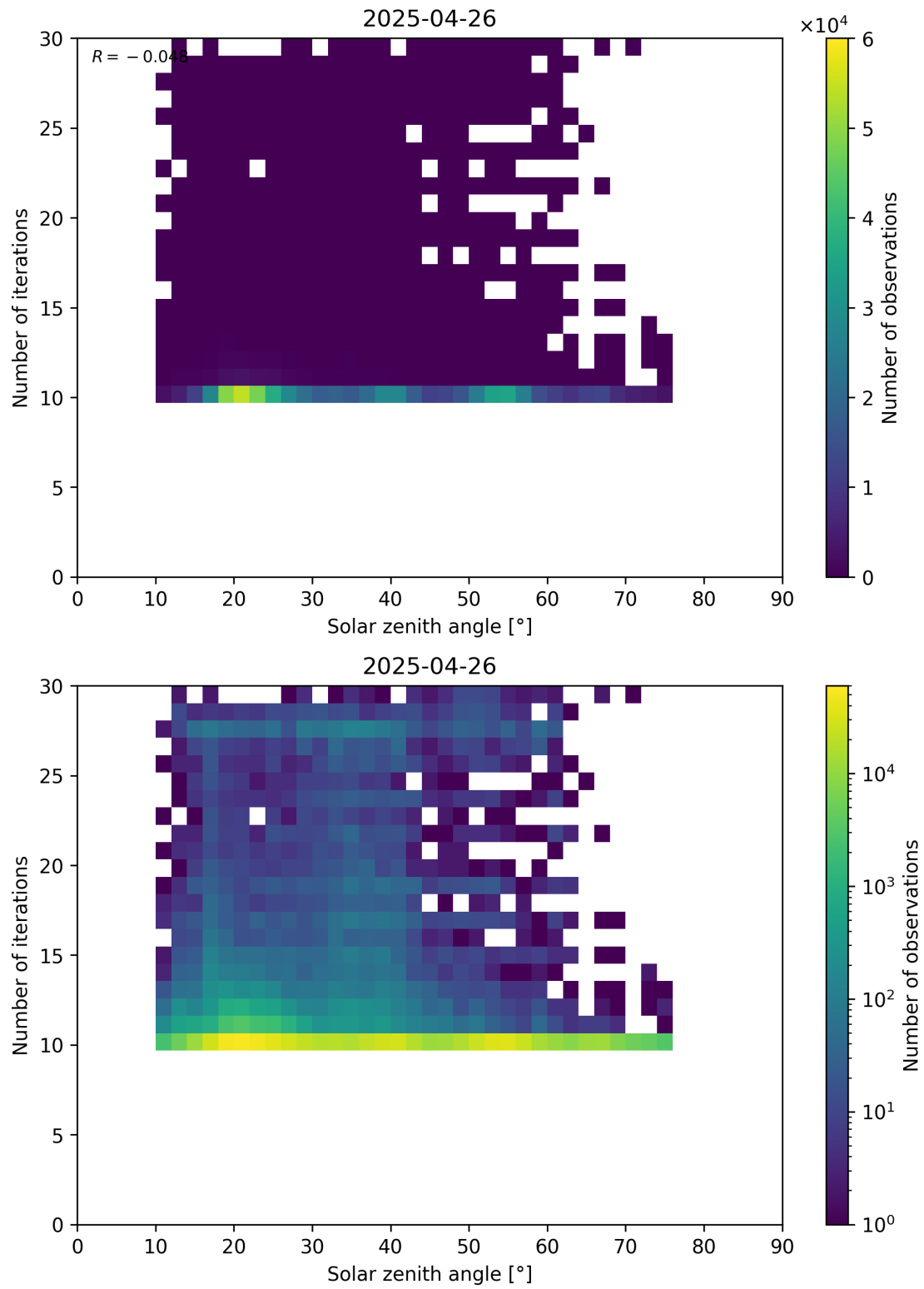
Figure 102: Scatter density plot of “Solar zenith angle” against “Number of iterations” for 2025-04-25 to 2025-04-27.
