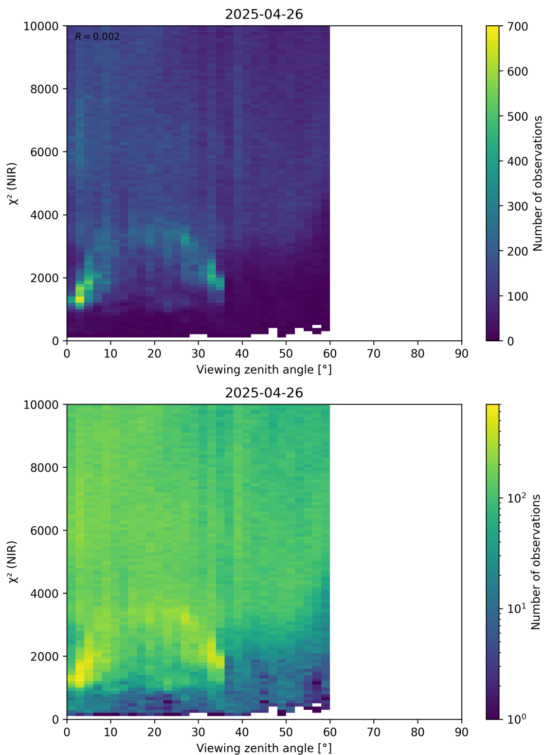
Figure 105: Scatter density plot of “Viewing zenith angle” against “ \chi^2 (NIR)” for 2025-04-25 to 2025-04-27.
