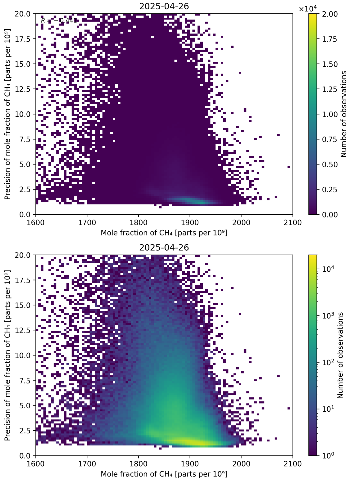
Figure 75: Scatter density plot of “Mole fraction of CH 4 ” against “Precision of mole fraction of CH 4 ” for 2025-04-25 to 2025-04-27.
