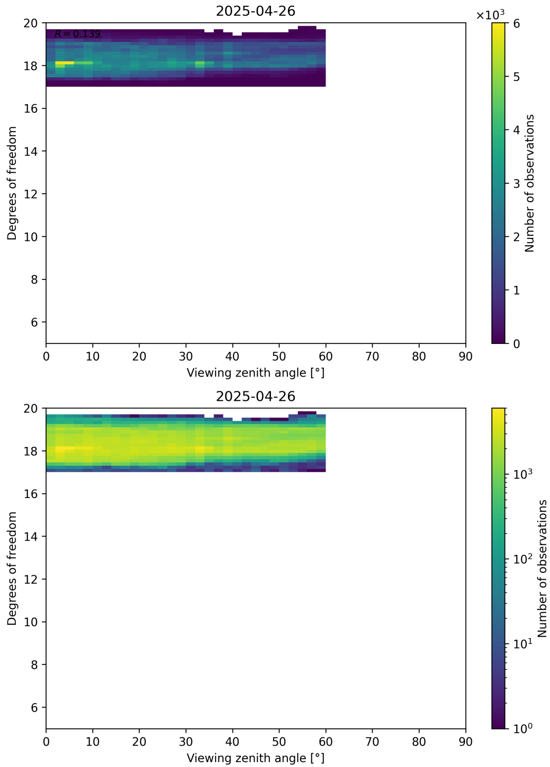
Figure 107: Scatter density plot of “Viewing zenith angle” against “Degrees of freedom” for 2025-04-25 to 2025-04-27.
