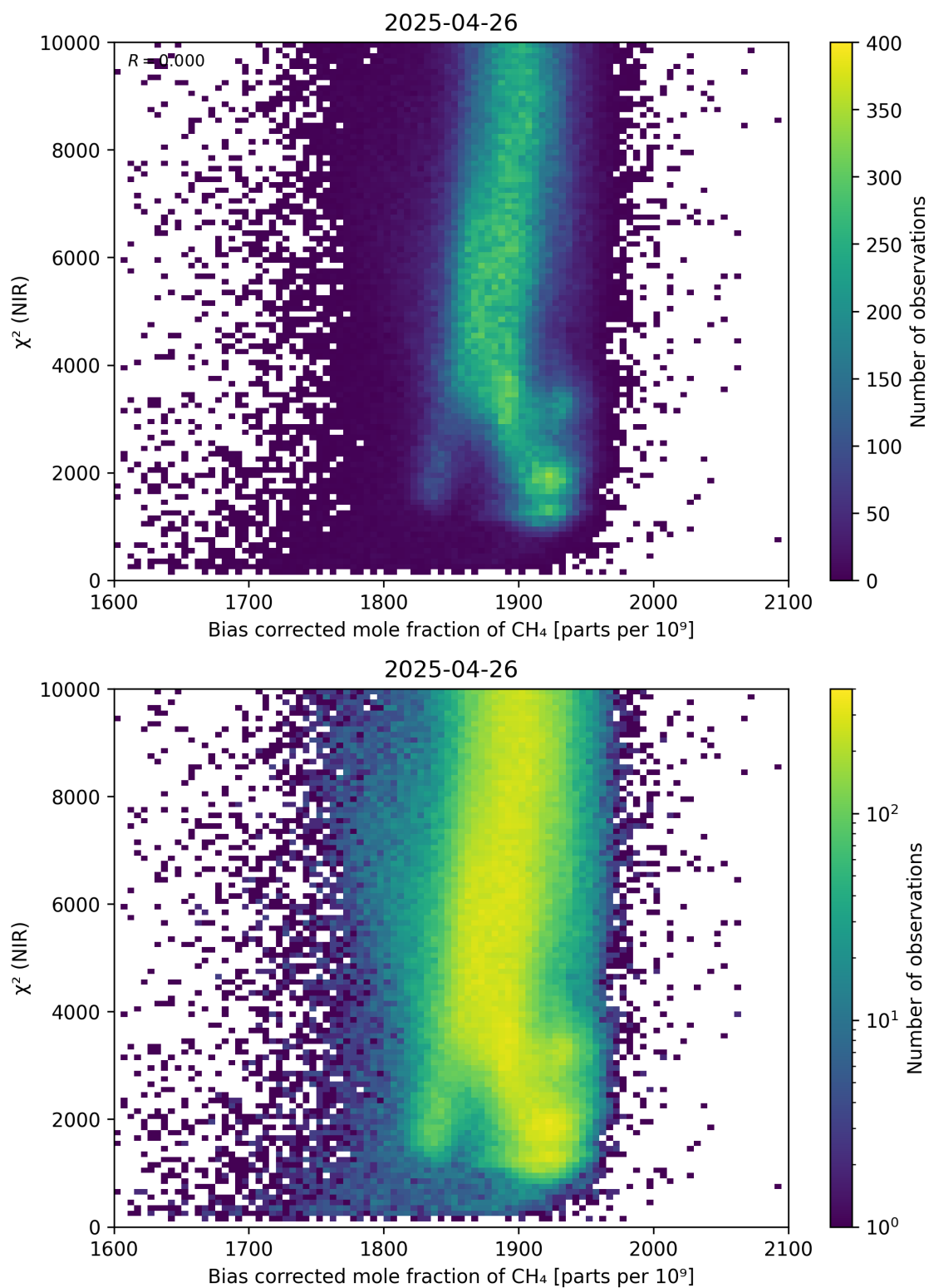
Figure 63: Scatter density plot of “Bias corrected mole fraction of \text{CH}_4 ” against “ \chi^2 (NIR)” for 2025-04-25 to 2025-04-27.
