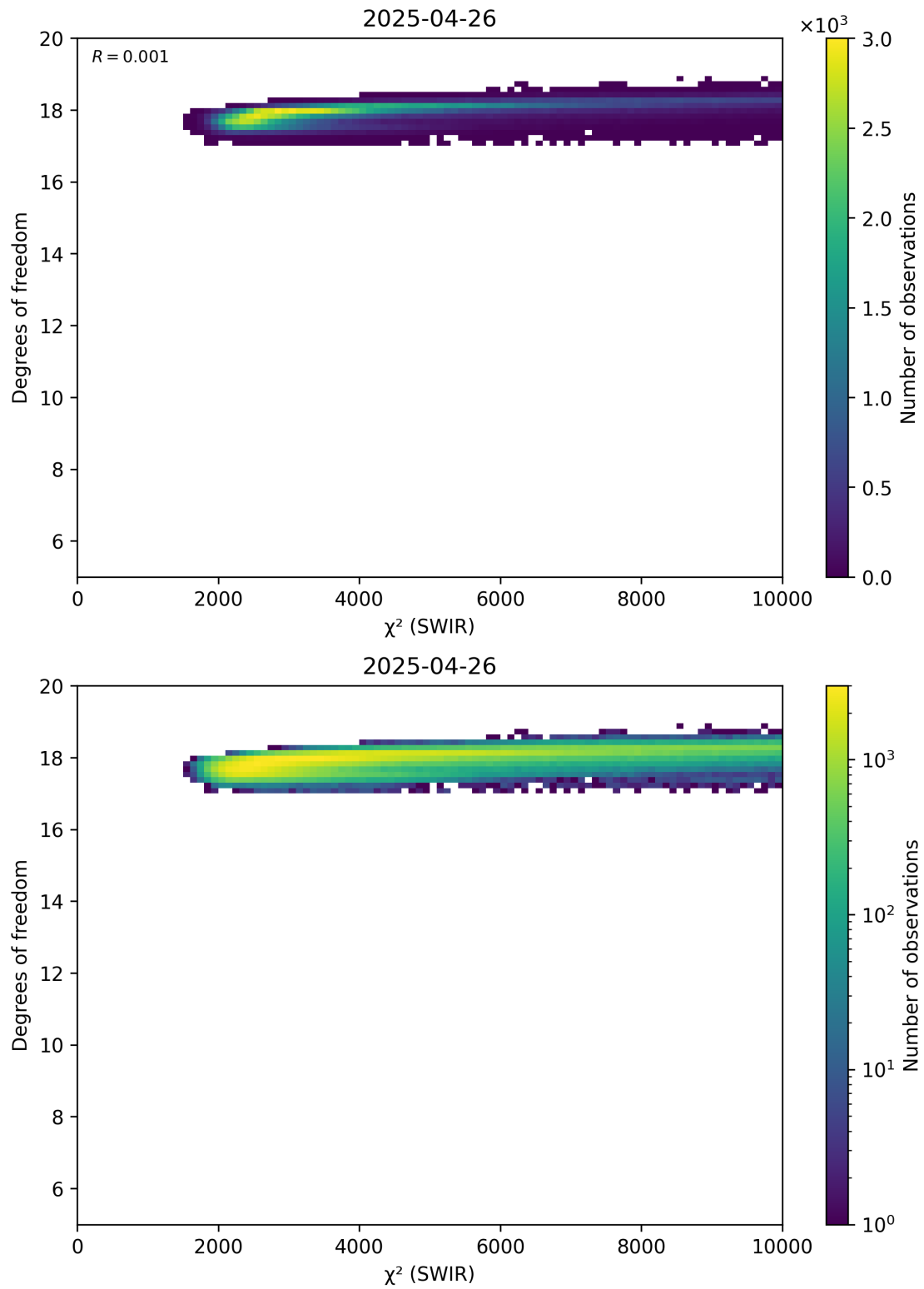
Figure 48: Scatter density plot of “ \chi^2 (SWIR)” against “Degrees of freedom” for 2025-04-25 to 2025-04-27.
