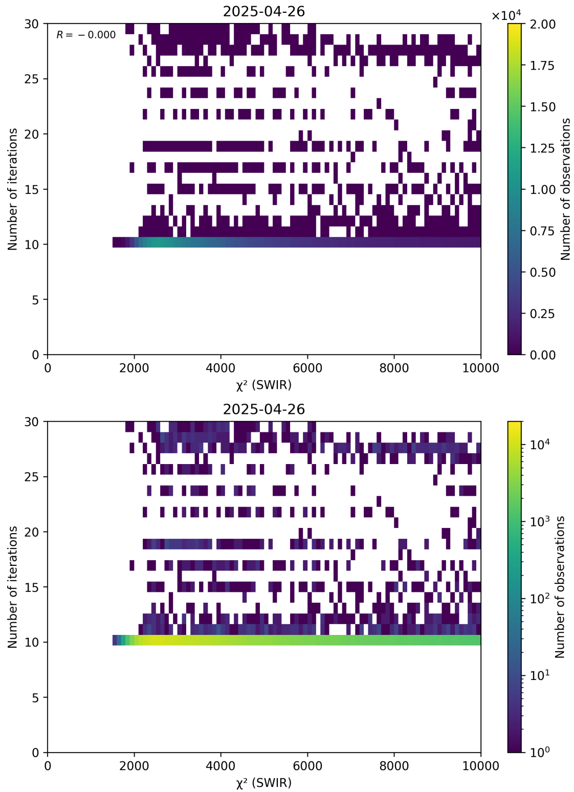
Figure 50: Scatter density plot of “ \chi^2 (SWIR)” against “Number of iterations” for 2025-04-25 to 2025-04-27.
