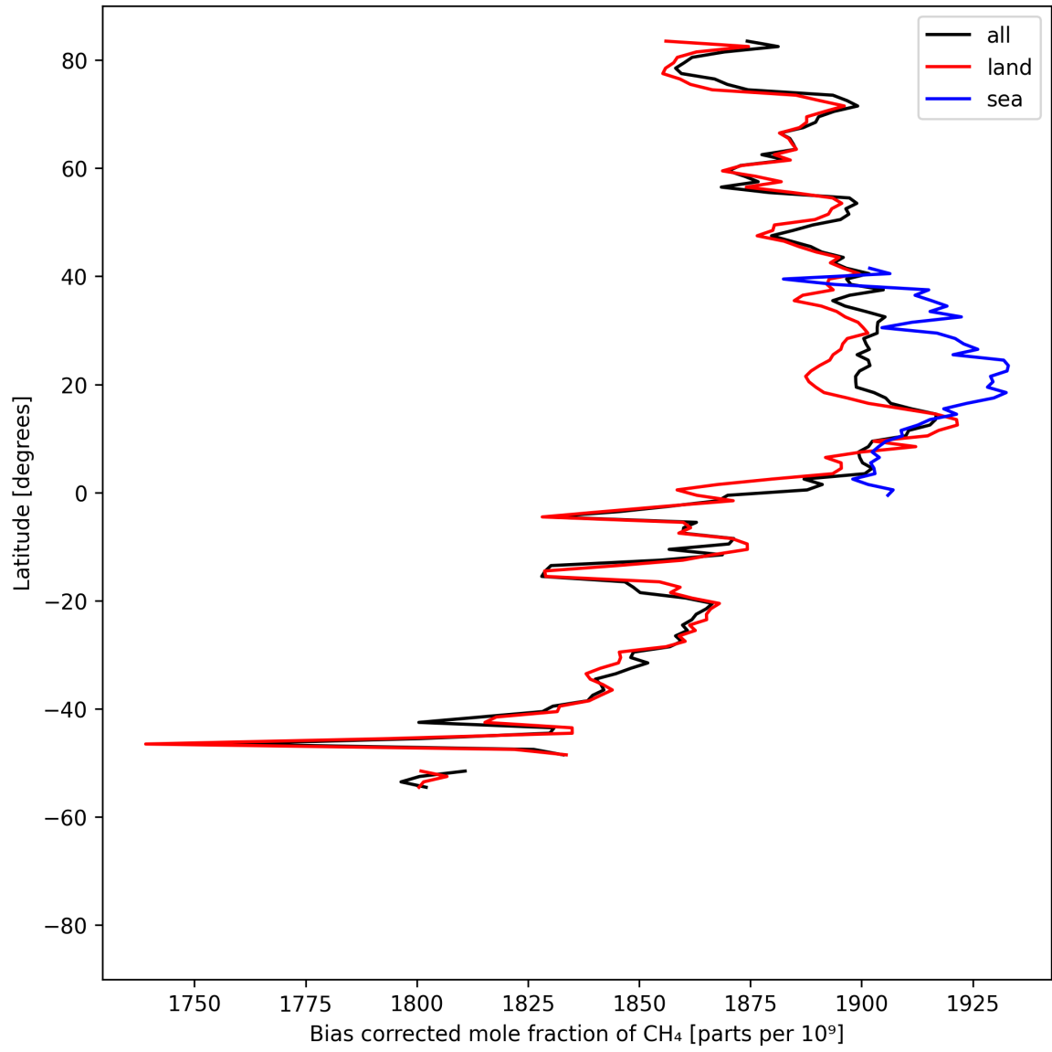
Figure 14: Zonal average of “Bias corrected mole fraction of \text{CH}_4 ” for 2025-04-25 to 2025-04-27.
