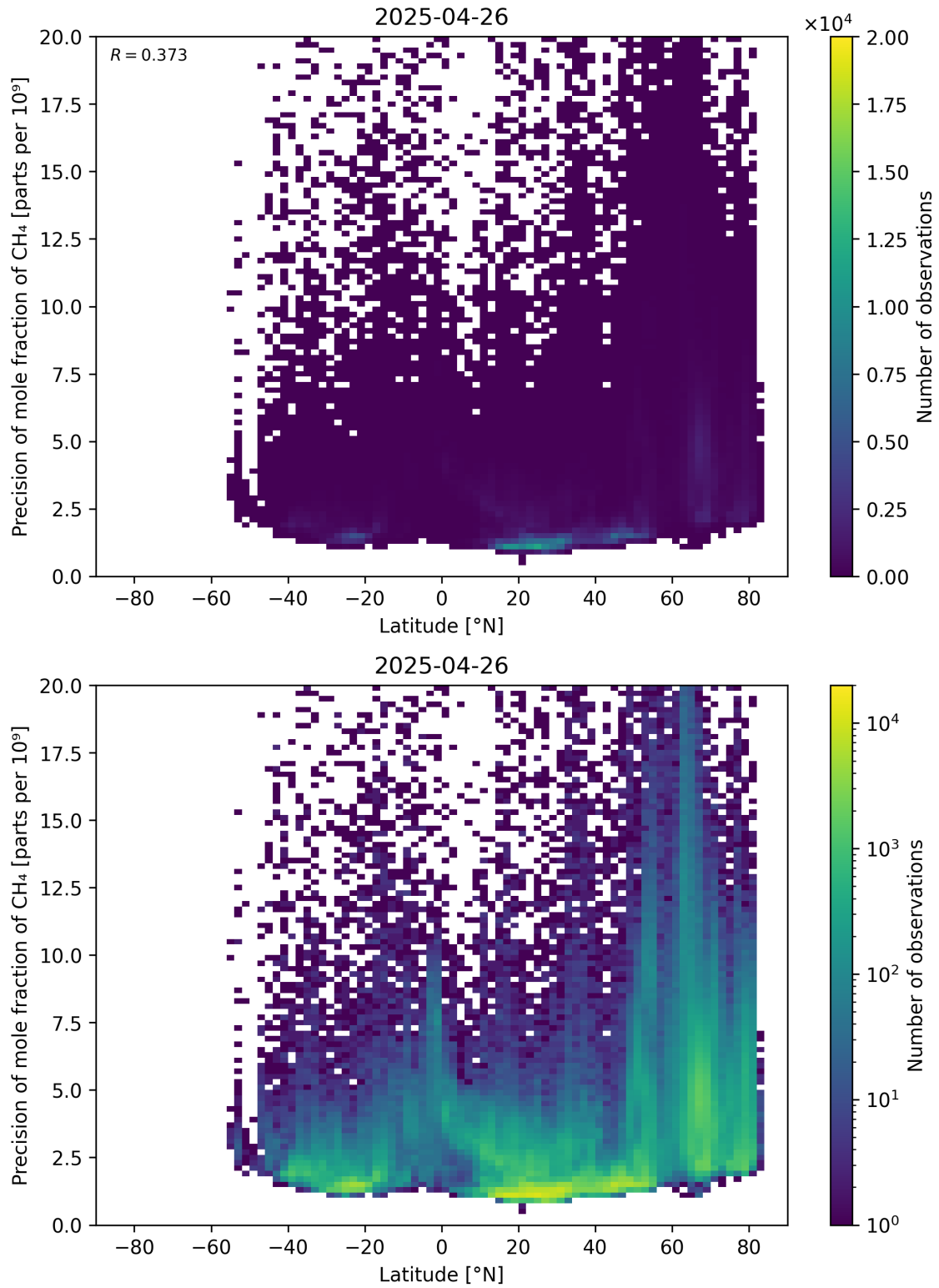
Figure 59: Scatter density plot of “Latitude” against “Precision of mole fraction of \text{CH}_4 ” for 2025-04-25 to 2025-04-27.
