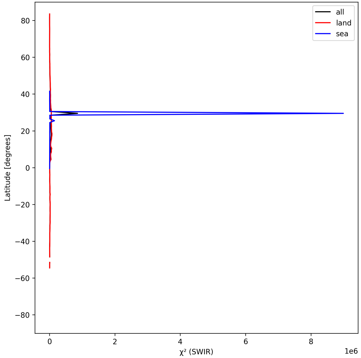
Figure 17: Zonal average of “ \chi^2 (SWIR)” for 2025-04-25 to 2025-04-27.
