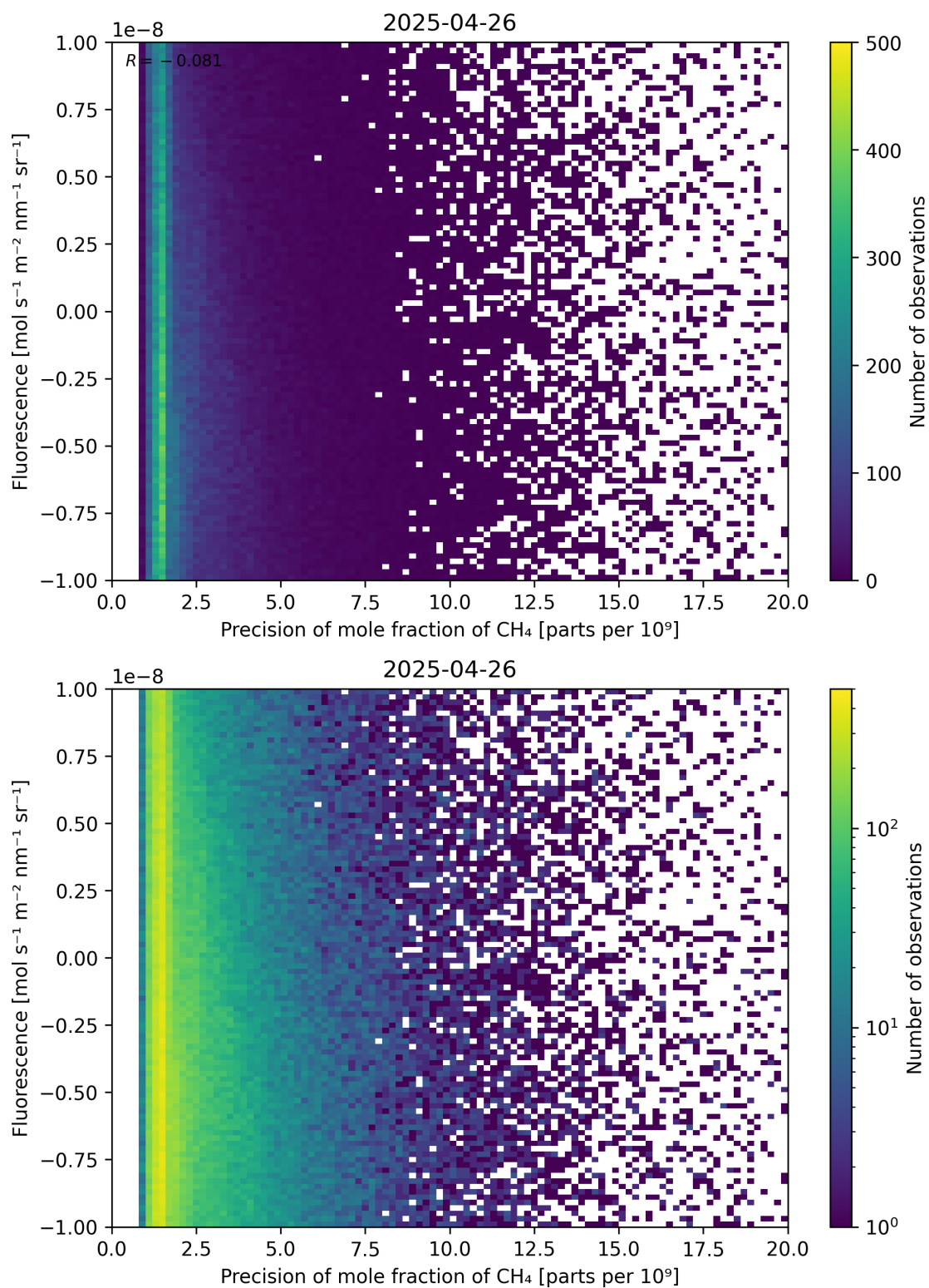
Figure 81: Scatter density plot of “Precision of mole fraction of CH 4 ” against “Fluorescence” for 2025-04-25 to 2025-04-27.
