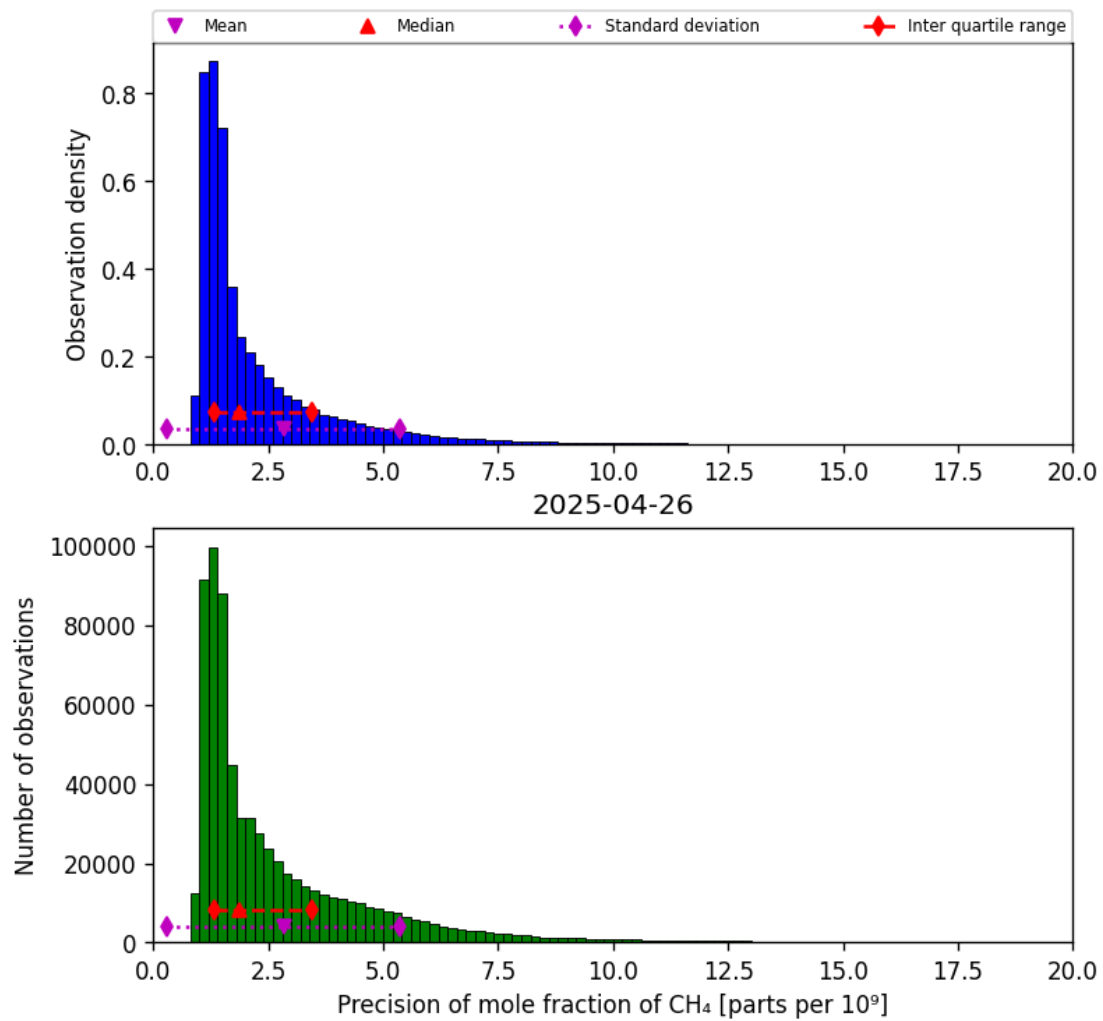
Figure 24: Histogram of “Precision of mole fraction of CH 4 ” for 2025-04-25 to 2025-04-27
