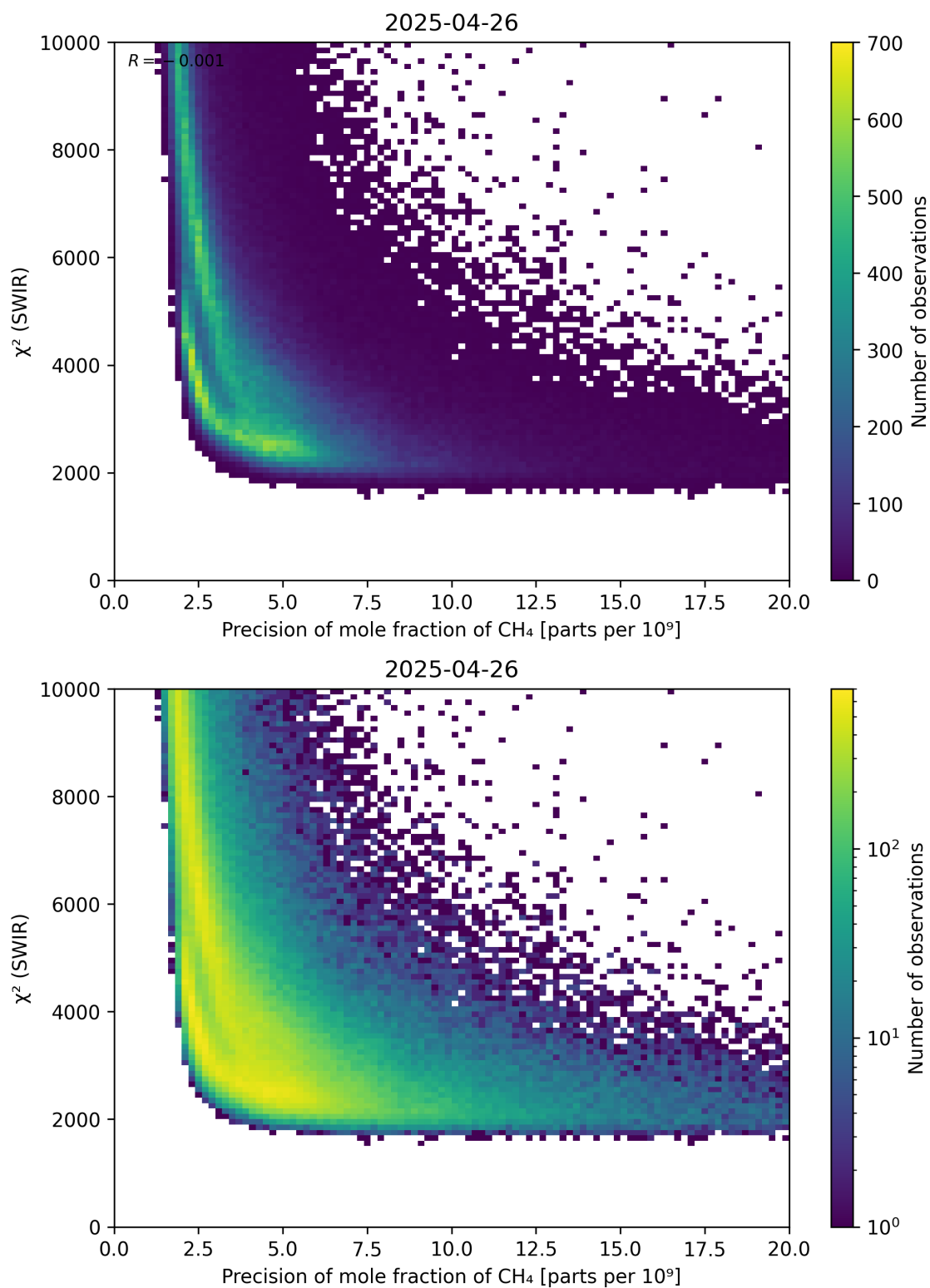
Figure 79: Scatter density plot of “Precision of mole fraction of CH 4 ” against “ \chi^2 (SWIR)” for 2025-04-25 to 2025-04-27.
