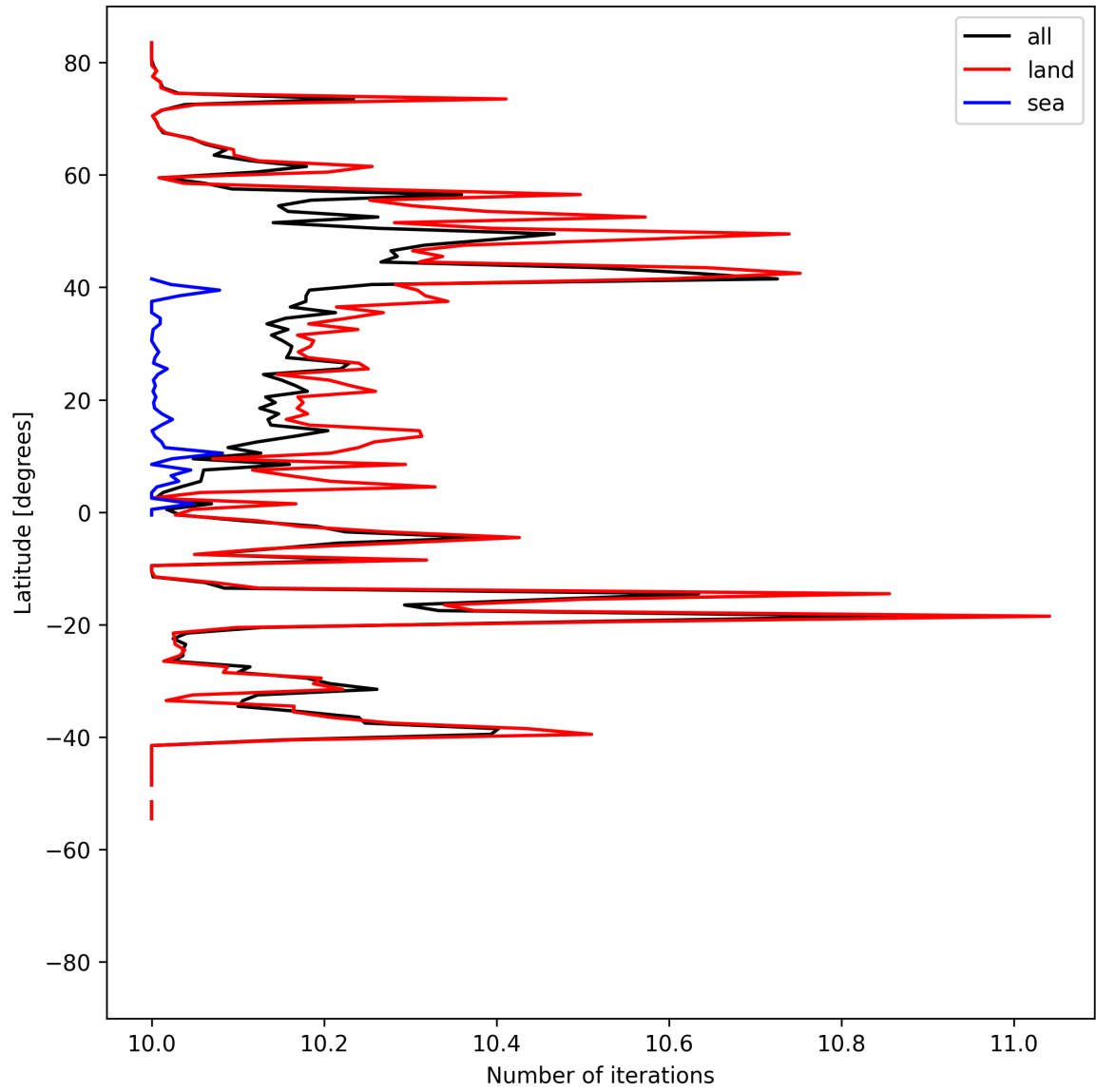
Figure 20: Zonal average of “Number of iterations” for 2025-04-25 to 2025-04-27.
