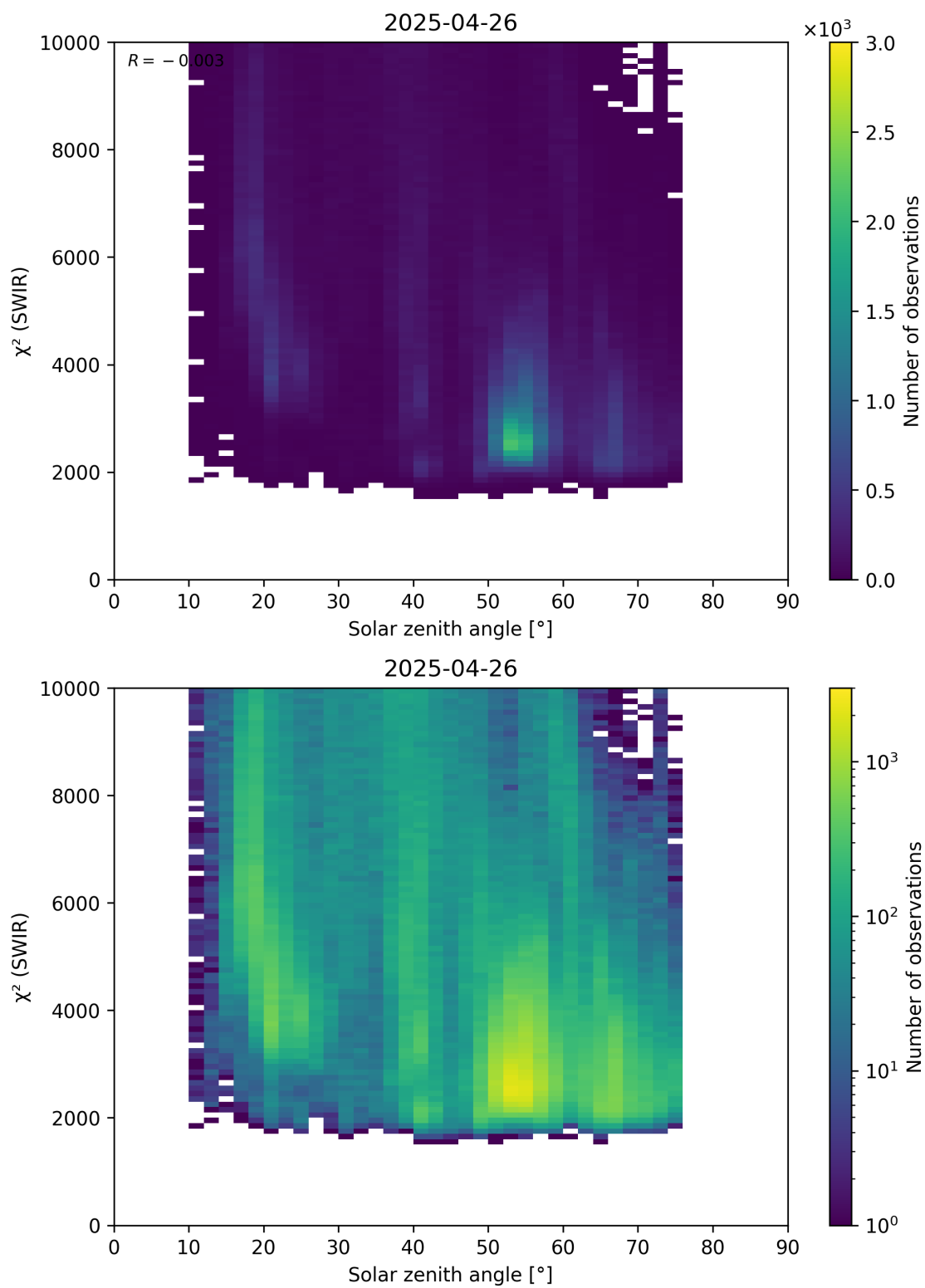
Figure 95: Scatter density plot of “Solar zenith angle” against “ \chi^2 (SWIR)” for 2025-04-25 to 2025-04-27.
