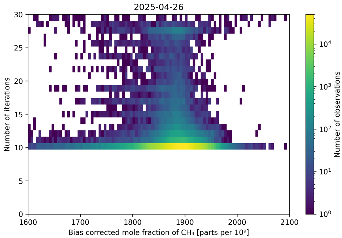
Figure 67: Scatter density plot of “Bias corrected mole fraction of CH 4 ” against “Number of iterations” for 2025-04-25 to 2025-04-27.
