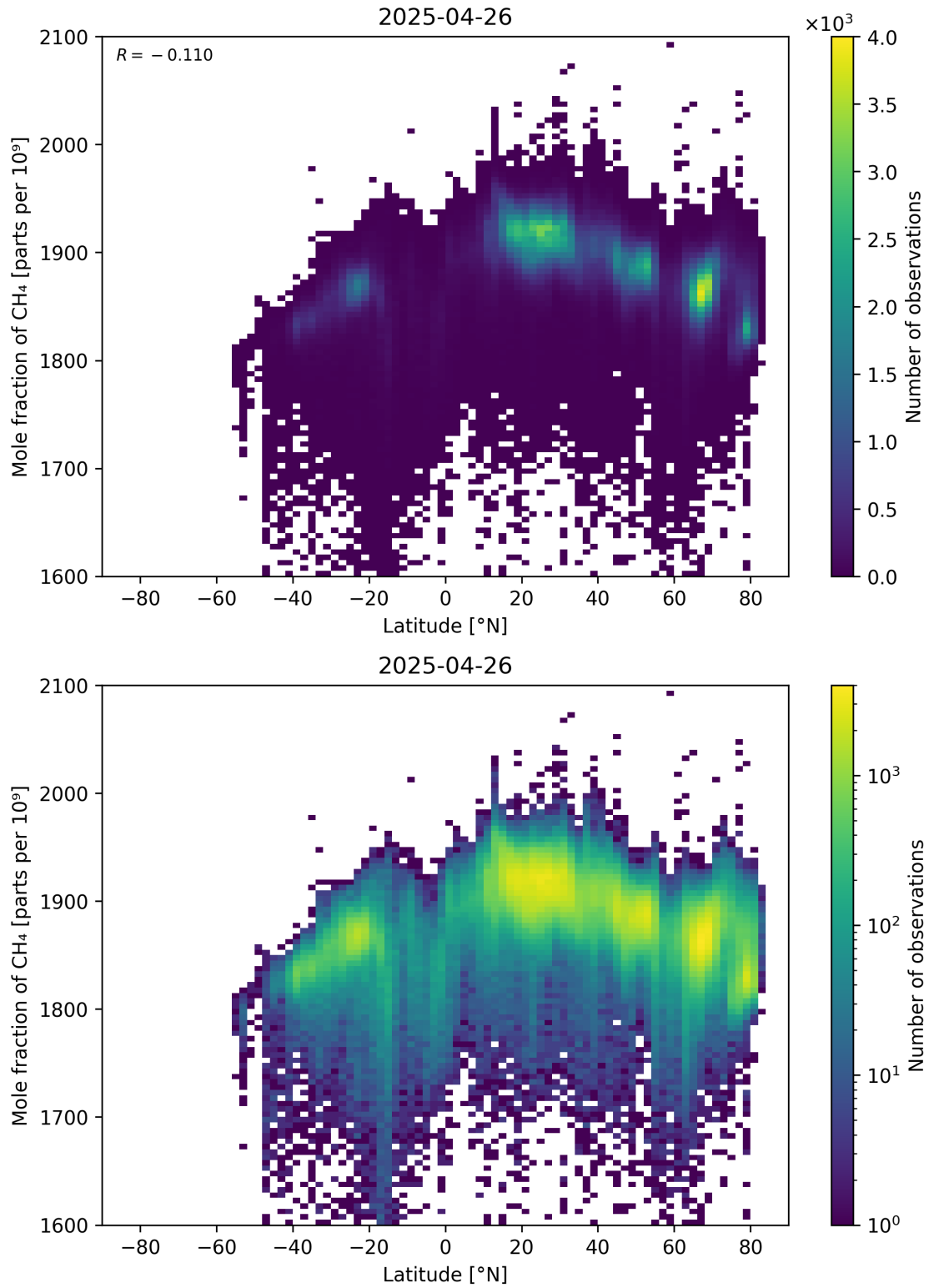
Figure 57: Scatter density plot of “Latitude” against “Mole fraction of CH 4 ” for 2025-04-25 to 2025-04-27.
