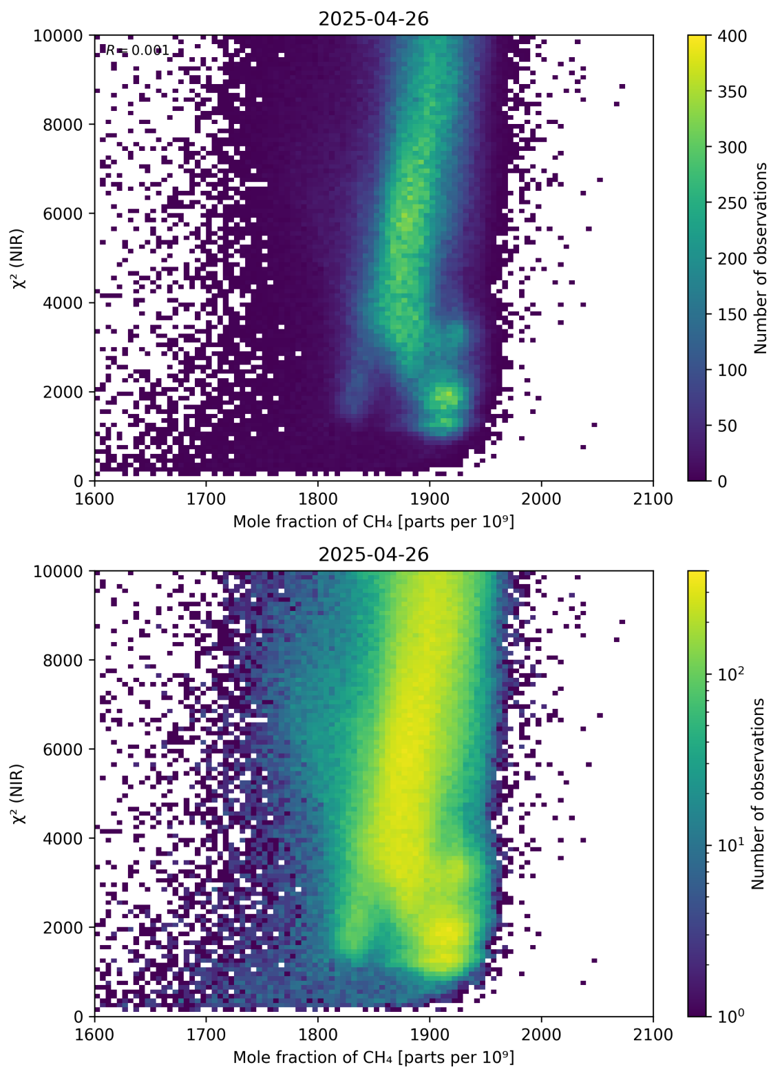
Figure 70: Scatter density plot of “Mole fraction of \text{CH}_4 ” against “ \chi^2 (NIR)” for 2025-04-25 to 2025-04-27.
