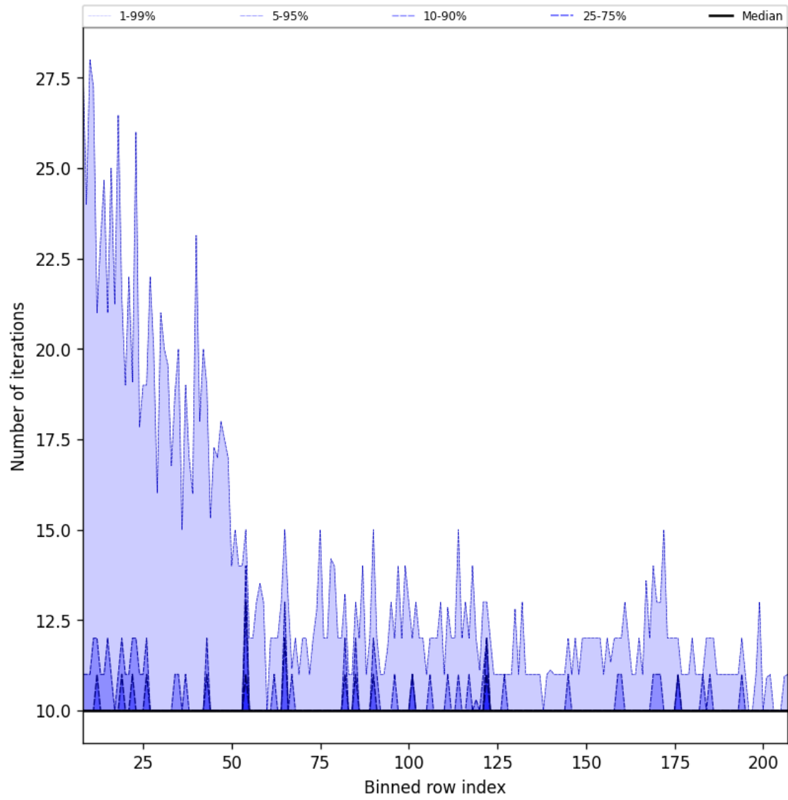
Figure 42: Along track statistics of “Number of iterations” for 2025-04-25 to 2025-04-27
