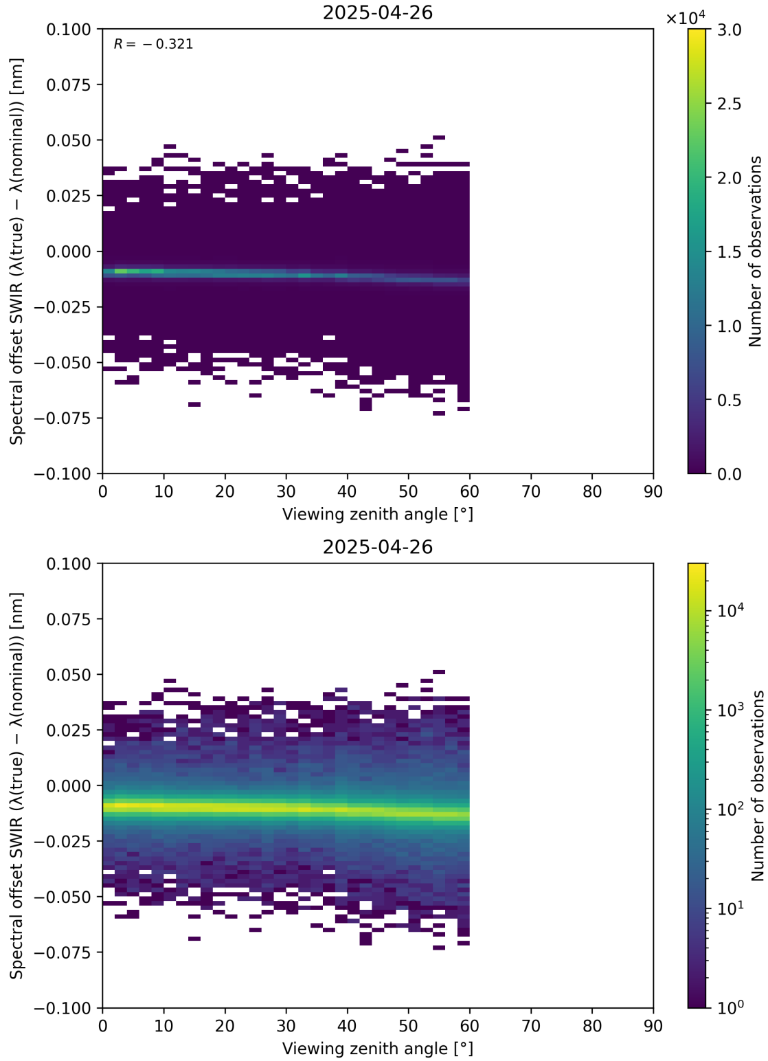
Figure 116: Scatter density plot of “Viewing zenith angle” against “Spectral offset SWIR ( \lambda_{\text{true}} - \lambda_{\text{nominal}} )” for 2025-04-25 to 2025-04-27.
