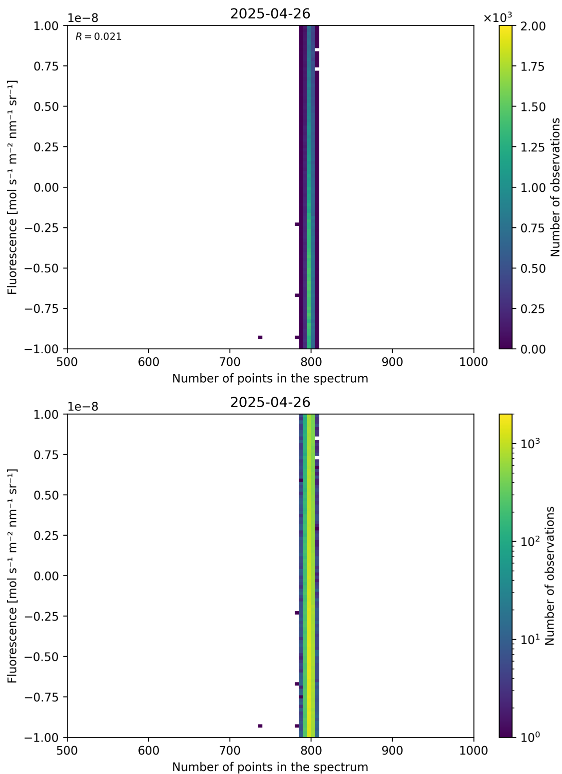
Figure 91: Scatter density plot of “Number of points in the spectrum” against “Fluorescence” for 2025-04-25 to 2025-04-27.
