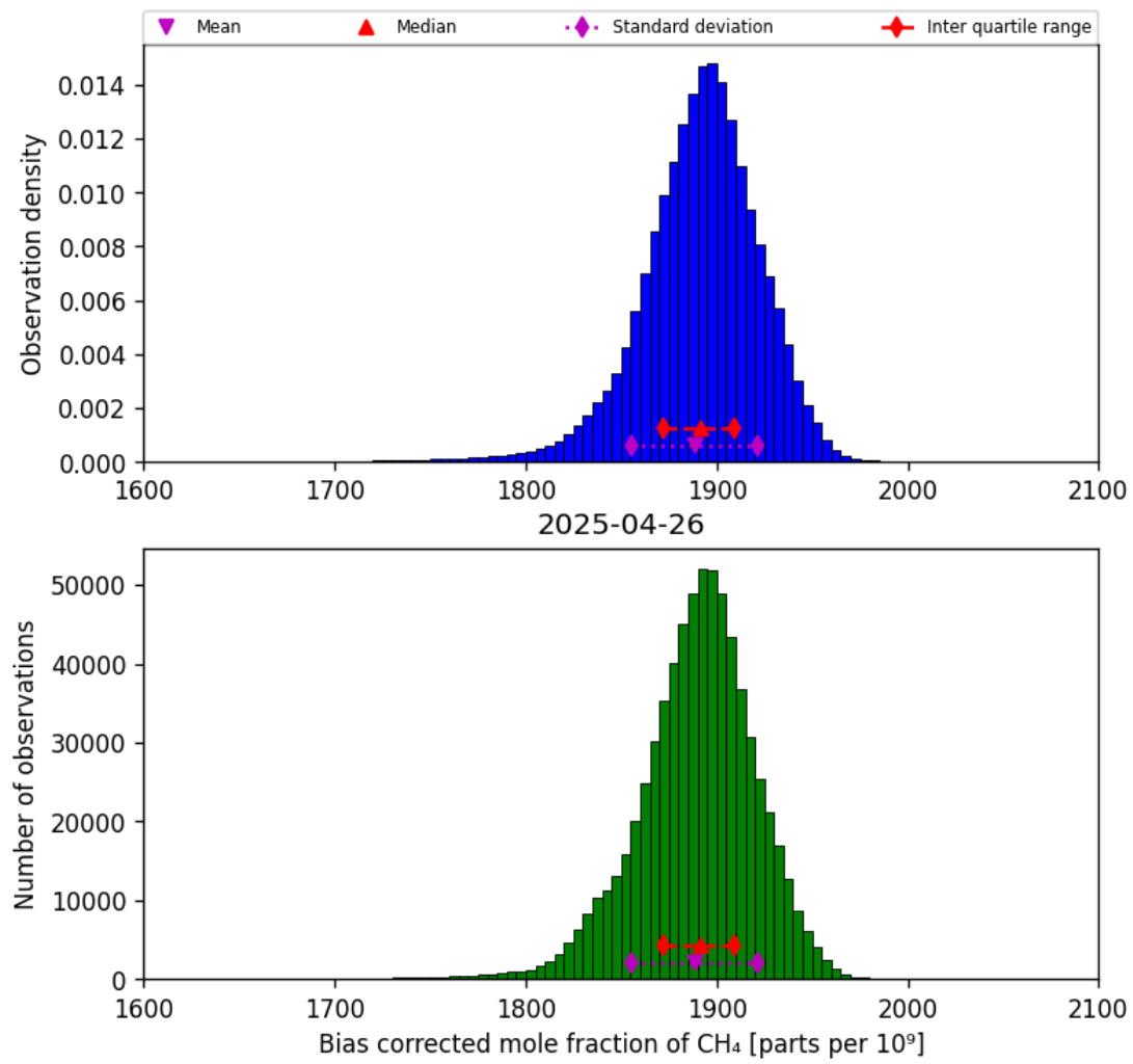
Figure 25: Histogram of “Bias corrected mole fraction of CH 4 ” for 2025-04-25 to 2025-04-27
