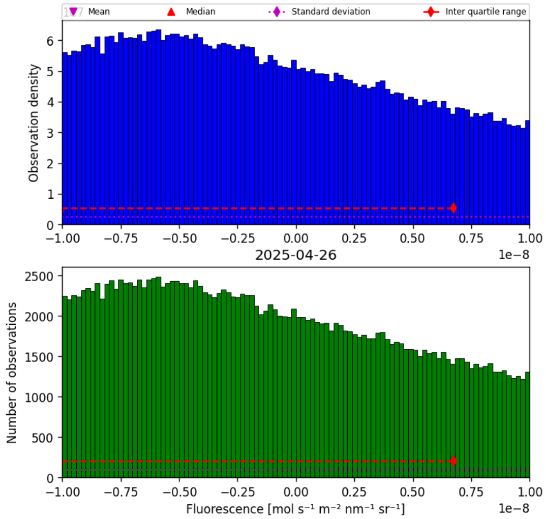
Figure 32: Histogram of “Fluorescence” for 2025-04-25 to 2025-04-27
