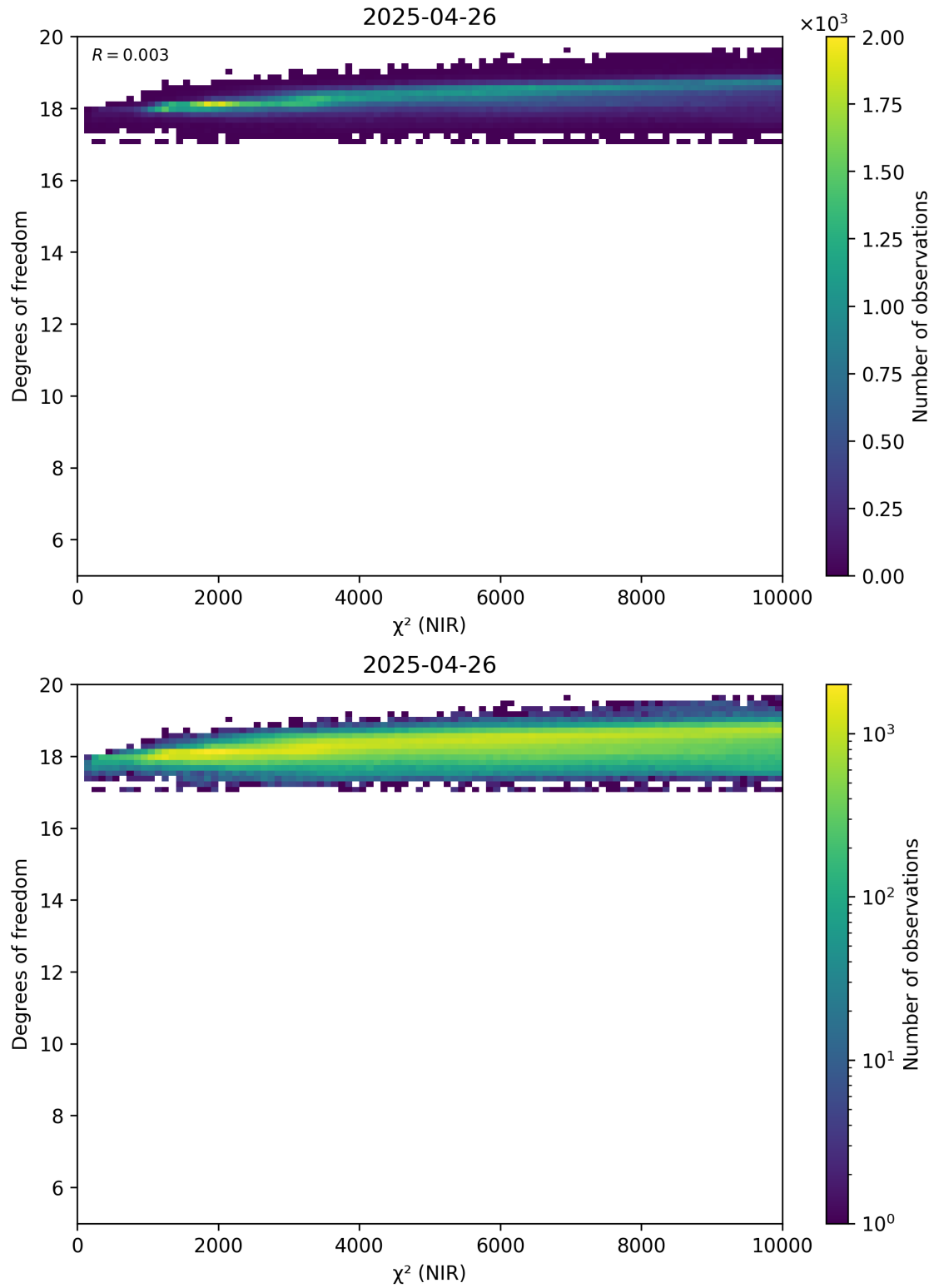
Figure 44: Scatter density plot of “ \chi^2 (NIR)” against “Degrees of freedom” for 2025-04-25 to 2025-04-27.
