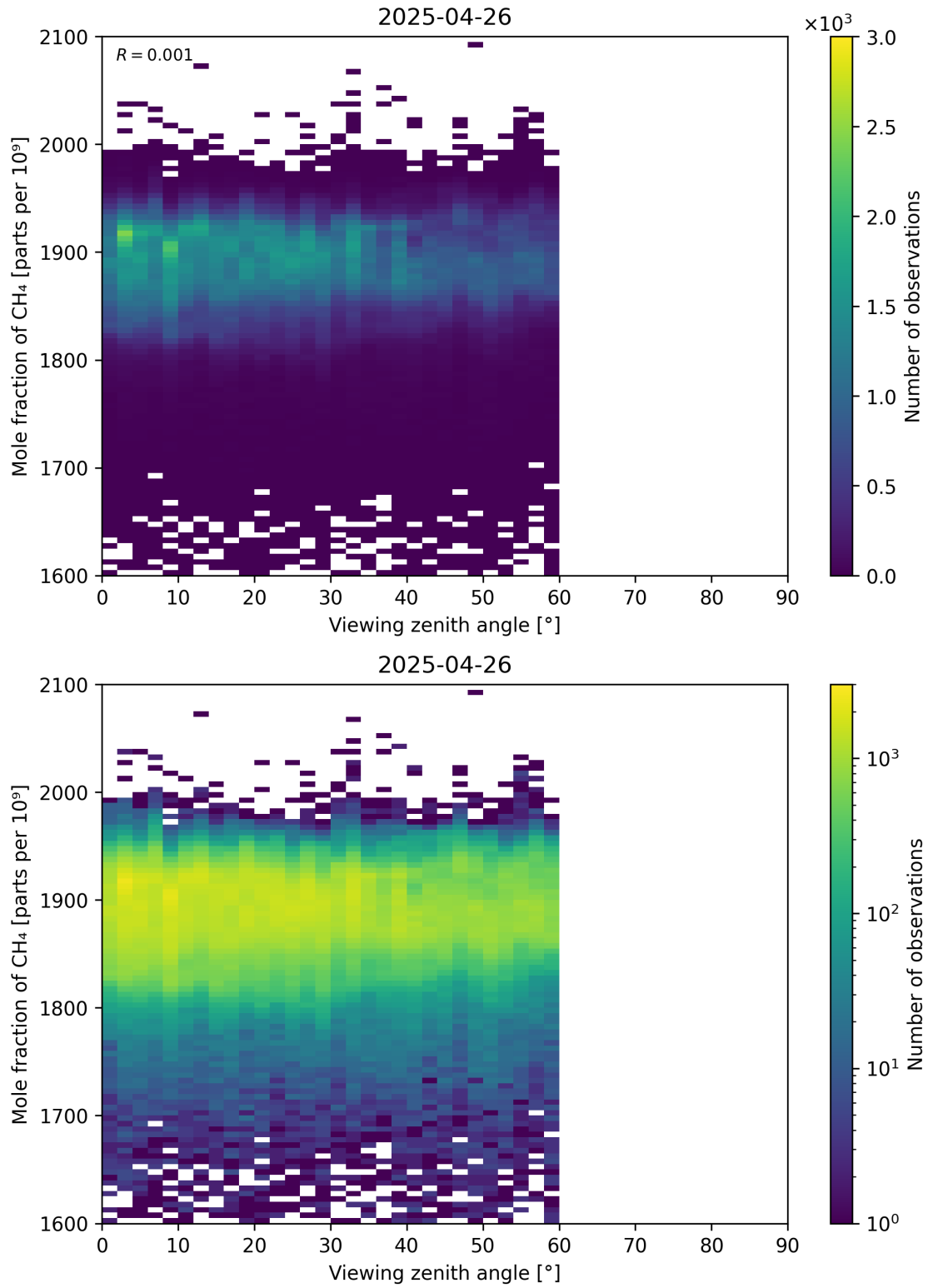
Figure 110: Scatter density plot of “Viewing zenith angle” against “Mole fraction of CH 4 ” for 2025-04-25 to 2025-04-27.
