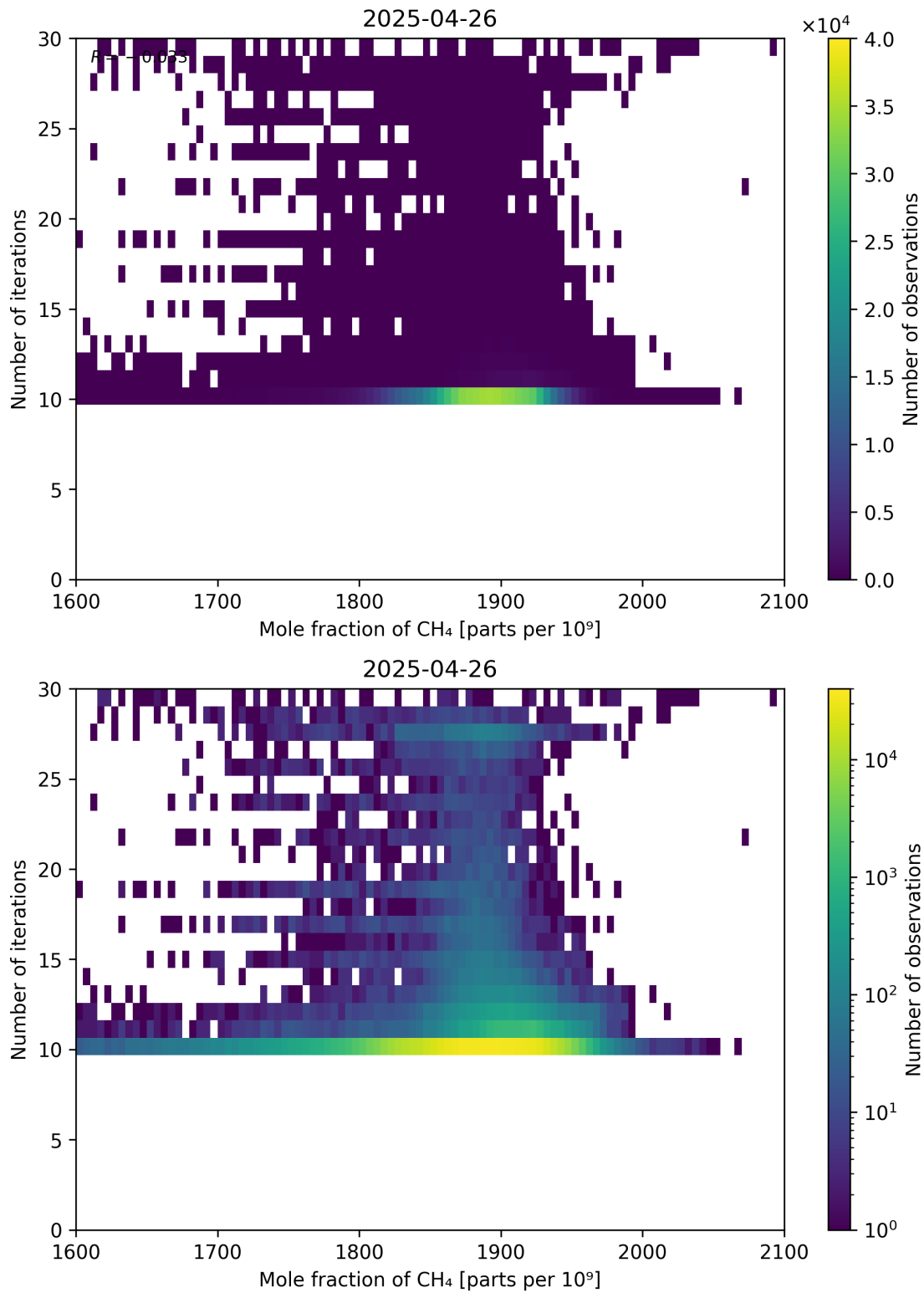
Figure 76: Scatter density plot of “Mole fraction of CH 4 ” against “Number of iterations” for 2025-04-25 to 2025-04-27.
