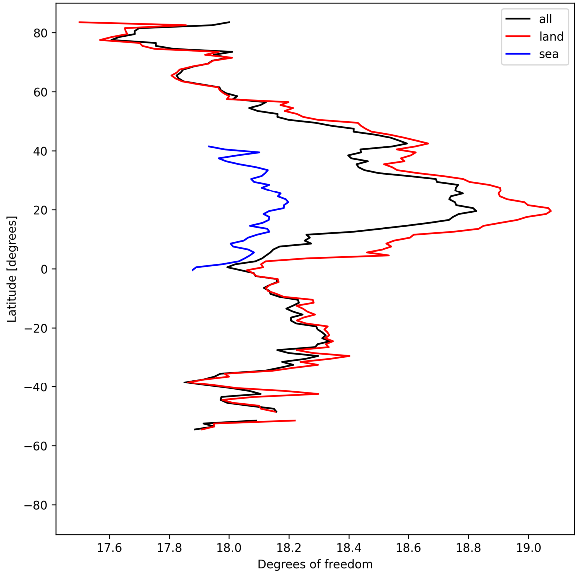
Figure 19: Zonal average of “Degrees of freedom” for 2025-04-25 to 2025-04-27.
