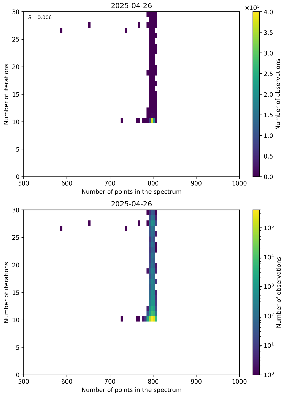
Figure 92: Scatter density plot of “Number of points in the spectrum” against “Number of iterations” for 2025-04-25 to 2025-04-27.
