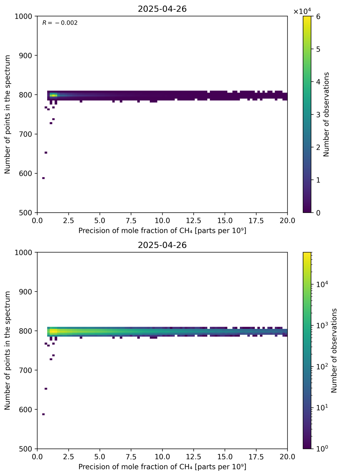
Figure 84: Scatter density plot of “Precision of mole fraction of CH 4 ” against “Number of points in the spectrum” for 2025-04-25 to 2025-04-27.
