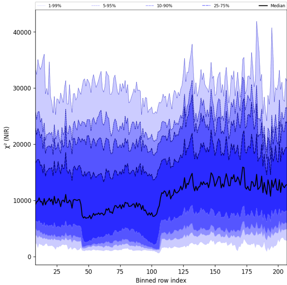
Figure 40: Along track statistics of “ \chi^2 (NIR)” for 2025-04-25 to 2025-04-27
