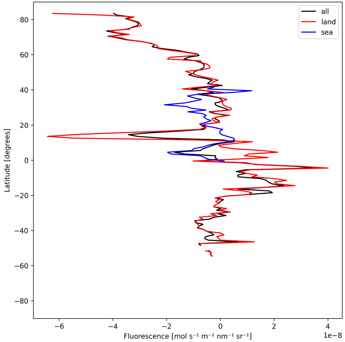
Figure 21: Zonal average of “Fluorescence” for 2025-04-25 to 2025-04-27.
