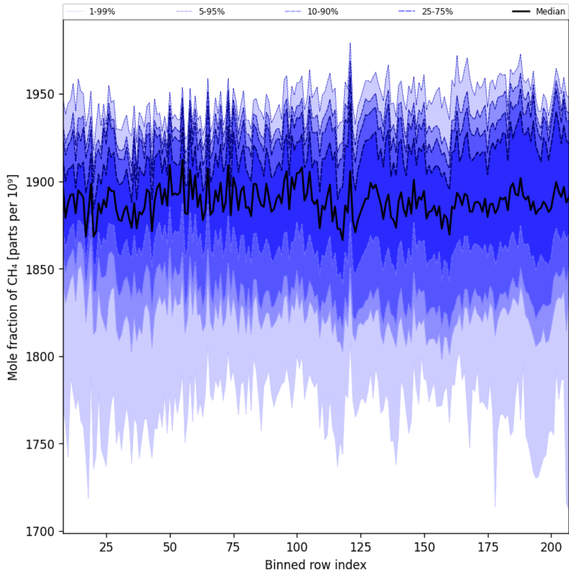
Figure 34: Along track statistics of “Mole fraction of CH 4 ” for 2025-04-25 to 2025-04-27
