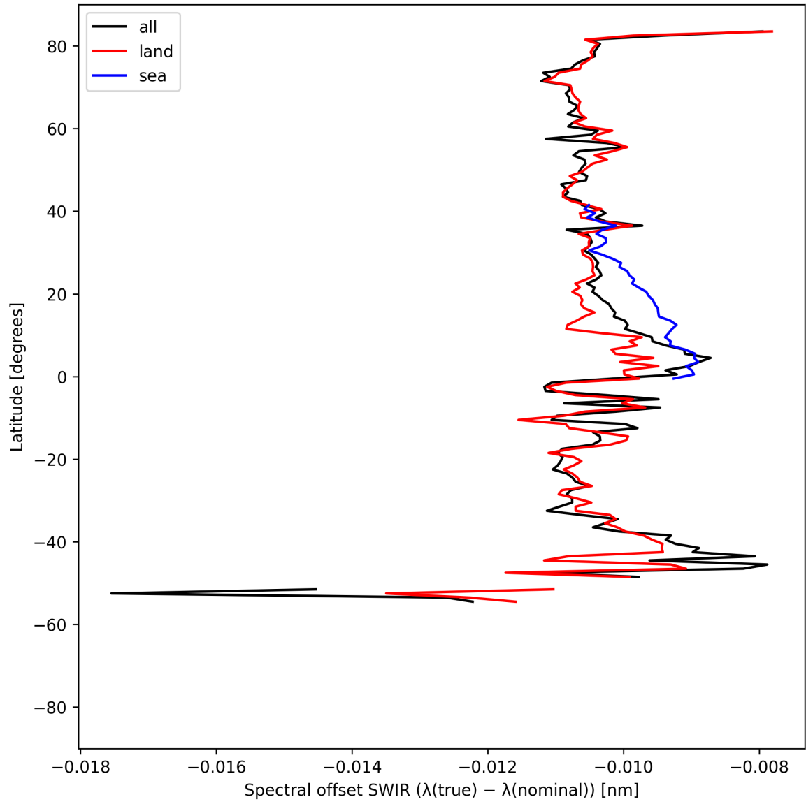
Figure 16: Zonal average of “Spectral offset SWIR ( \lambda_{\text{true}} - \lambda_{\text{nominal}} )” for 2025-04-25 to 2025-04-27.
