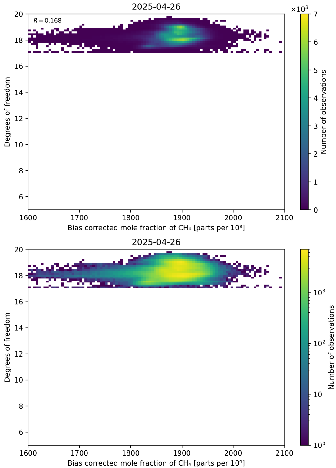
Figure 65: Scatter density plot of “Bias corrected mole fraction of CH 4 ” against “Degrees of freedom” for 2025-04-25 to 2025-04-27.
