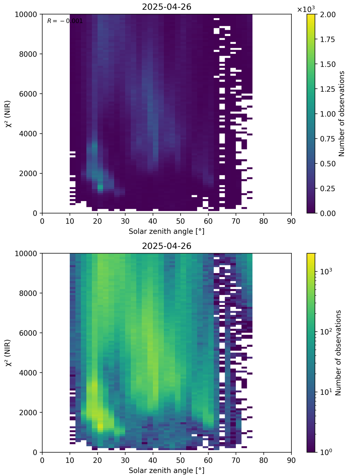
Figure 94: Scatter density plot of “Solar zenith angle” against “ \chi^2 (NIR)” for 2025-04-25 to 2025-04-27.
