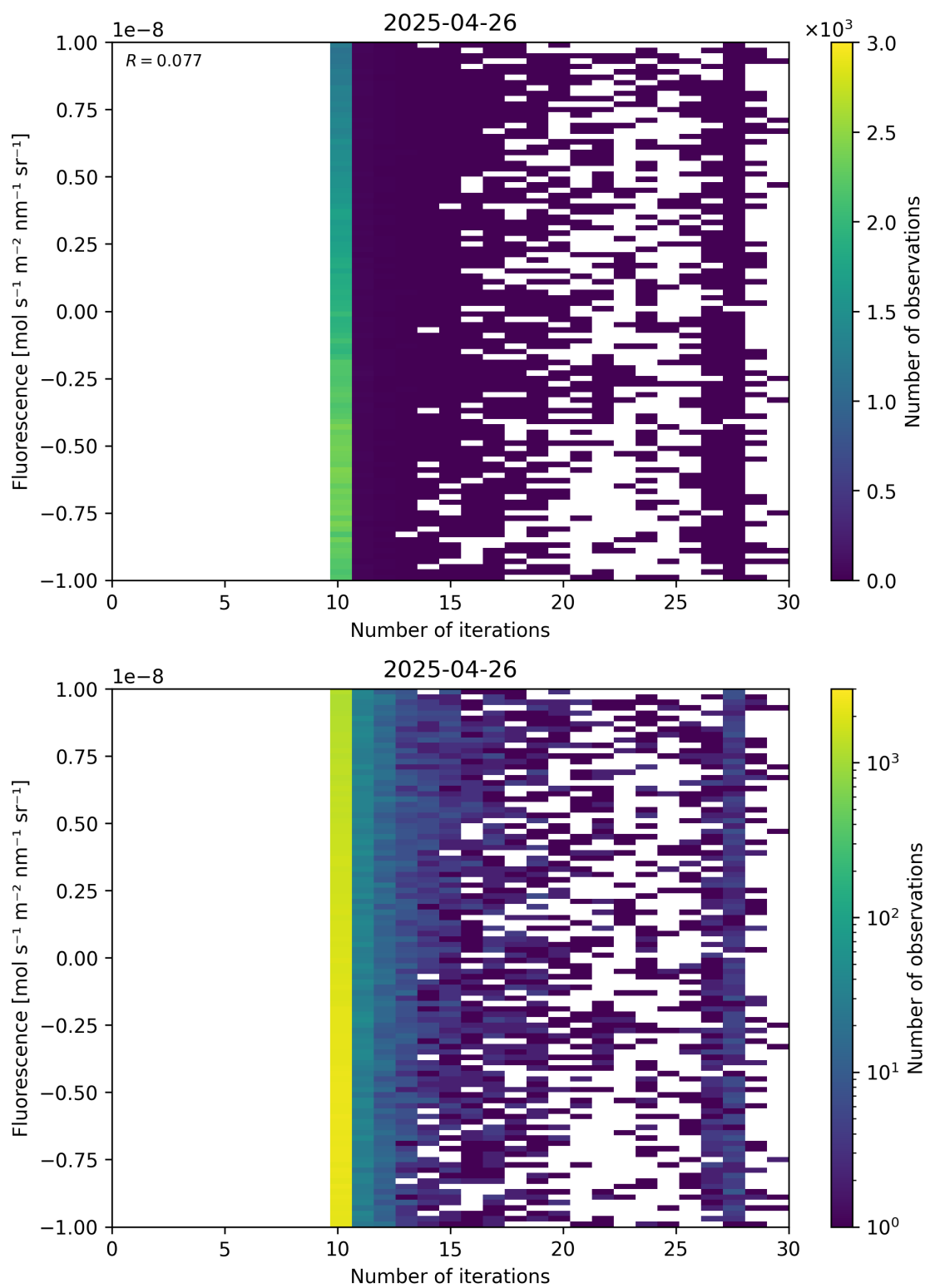
Figure 87: Scatter density plot of “Number of iterations” against “Fluorescence” for 2025-04-25 to 2025-04-27.
