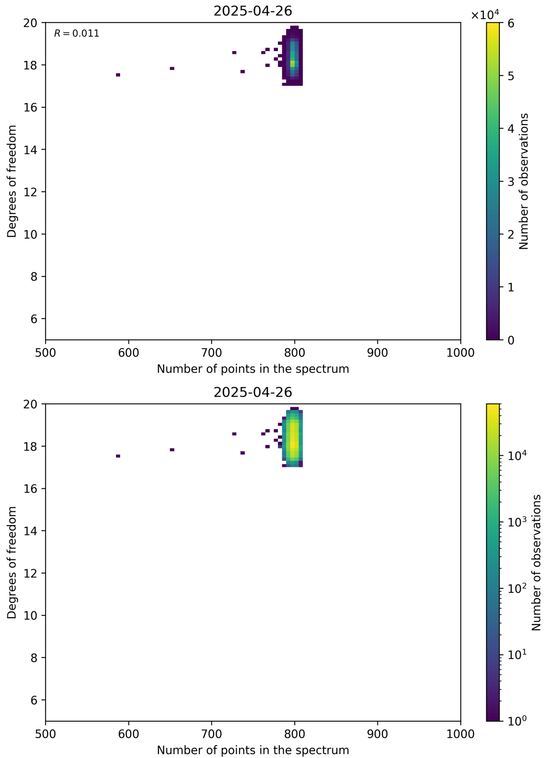
Figure 90: Scatter density plot of “Number of points in the spectrum” against “Degrees of freedom” for 2025-04-25 to 2025-04-27.
