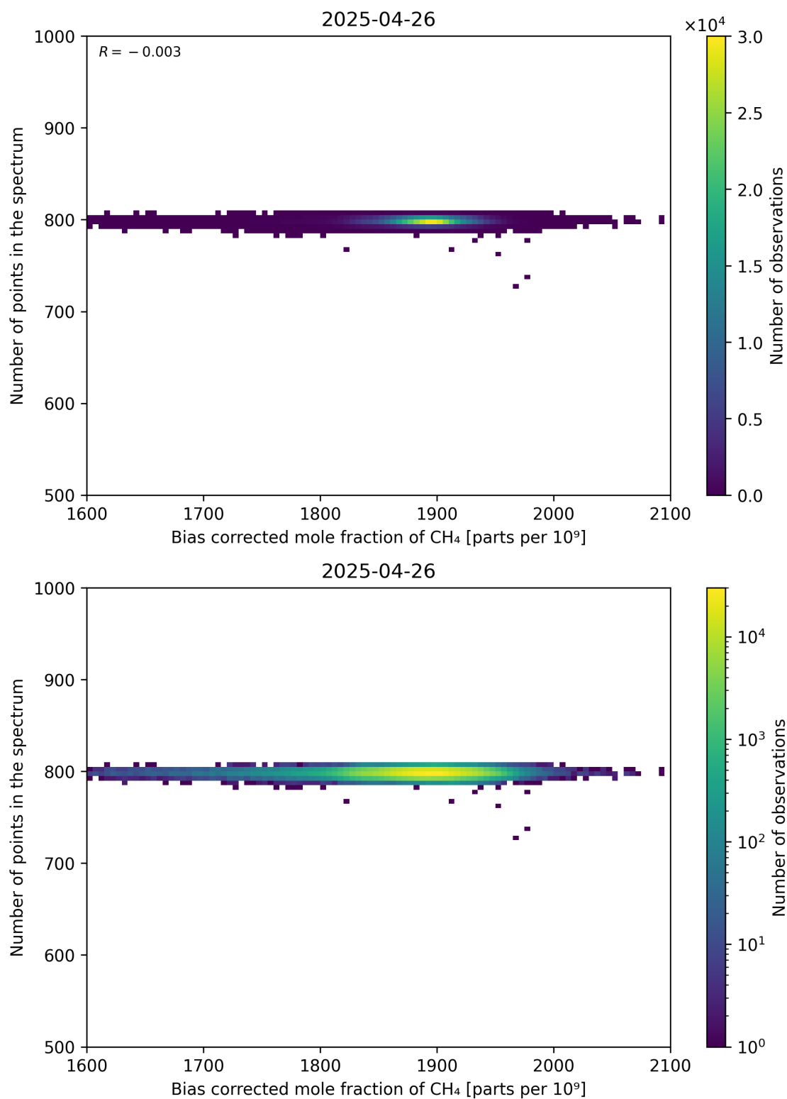
Figure 68: Scatter density plot of “Bias corrected mole fraction of CH 4 ” against “Number of points in the spectrum” for 2025-04-25 to 2025-04-27.
