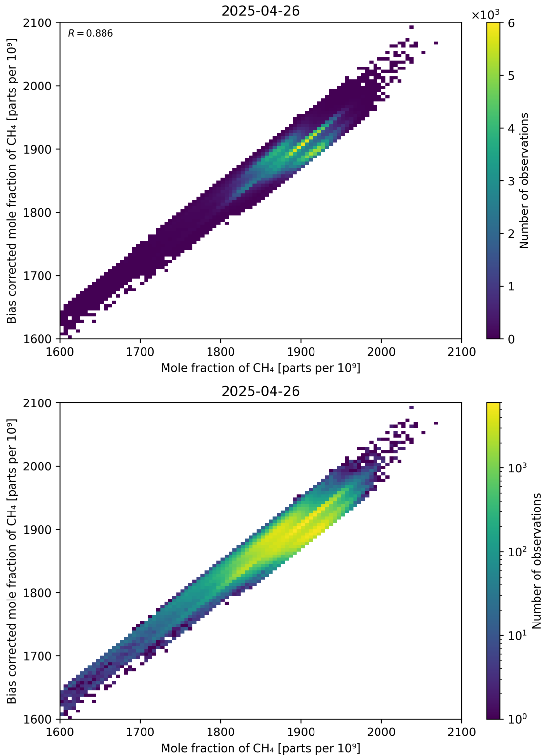
Figure 74: Scatter density plot of “Mole fraction of CH 4 ” against “Bias corrected mole fraction of CH 4 ” for 2025-04-25 to 2025-04-27.
