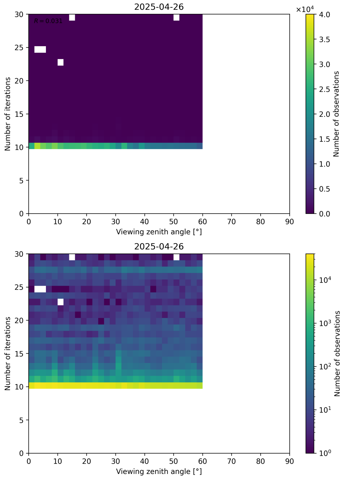
Figure 113: Scatter density plot of “Viewing zenith angle” against “Number of iterations” for 2025-04-25 to 2025-04-27.
