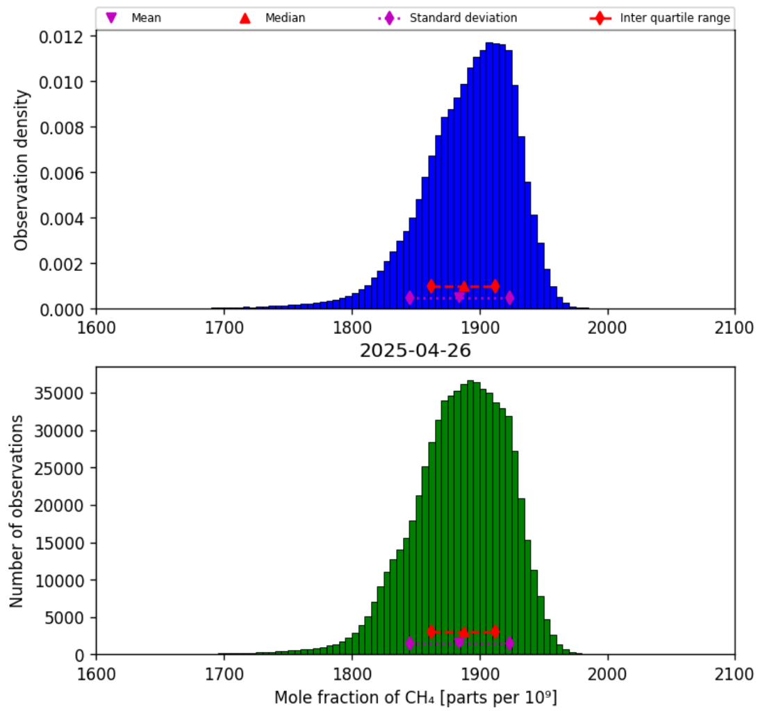
Figure 23: Histogram of “Mole fraction of CH 4 ” for 2025-04-25 to 2025-04-27
