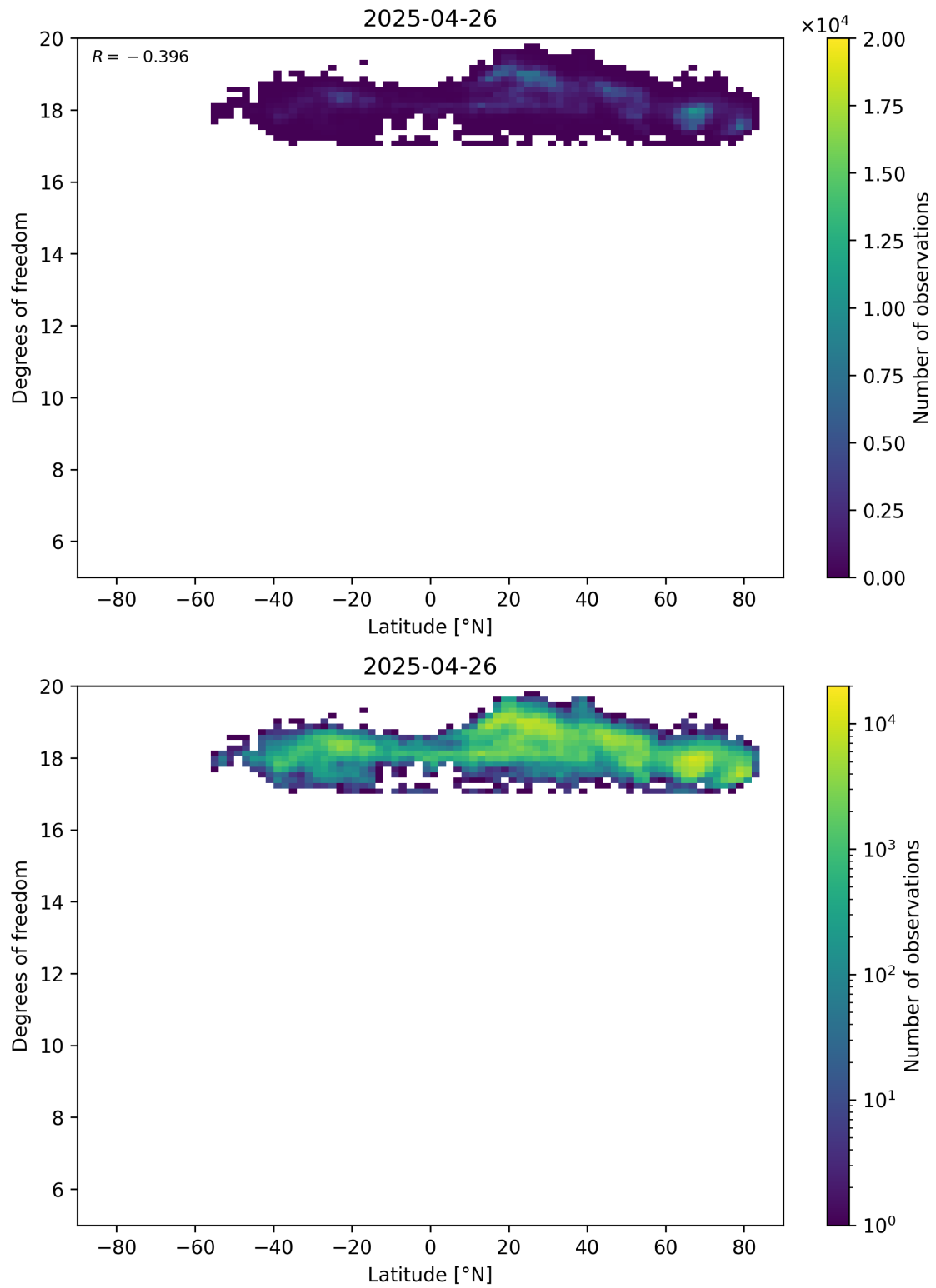
Figure 55: Scatter density plot of “Latitude” against “Degrees of freedom” for 2025-04-25 to 2025-04-27.
