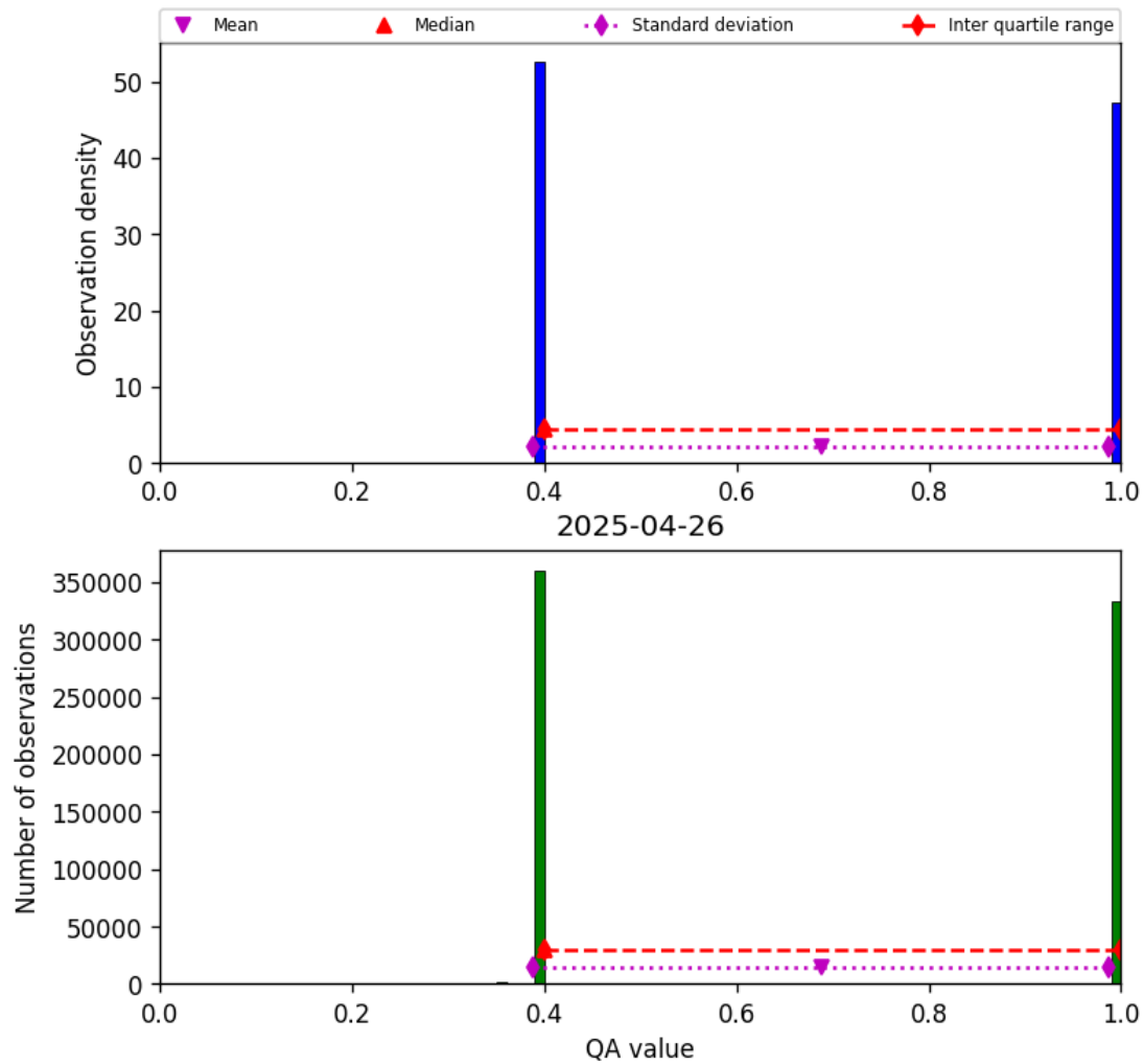
Figure 22: Histogram of “QA value” for 2025-04-25 to 2025-04-27
