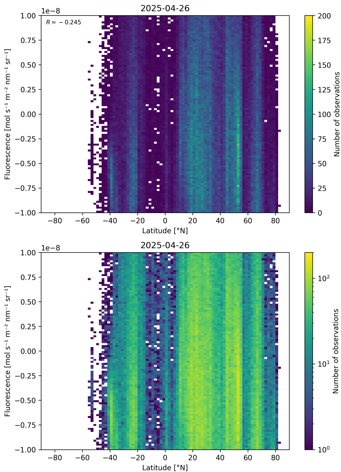
Figure 56: Scatter density plot of “Latitude” against “Fluorescence” for 2025-04-25 to 2025-04-27.
