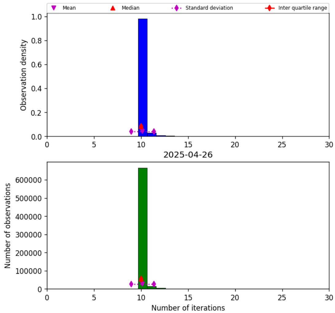
Figure 31: Histogram of “Number of iterations” for 2025-04-25 to 2025-04-27
