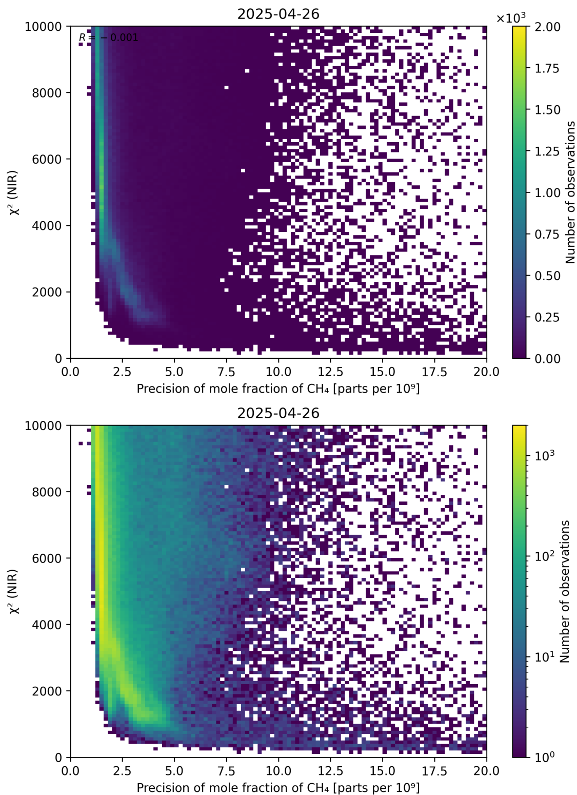
Figure 78: Scatter density plot of “Precision of mole fraction of \text{CH}_4 ” against “ \chi^2 (NIR)” for 2025-04-25 to 2025-04-27.
