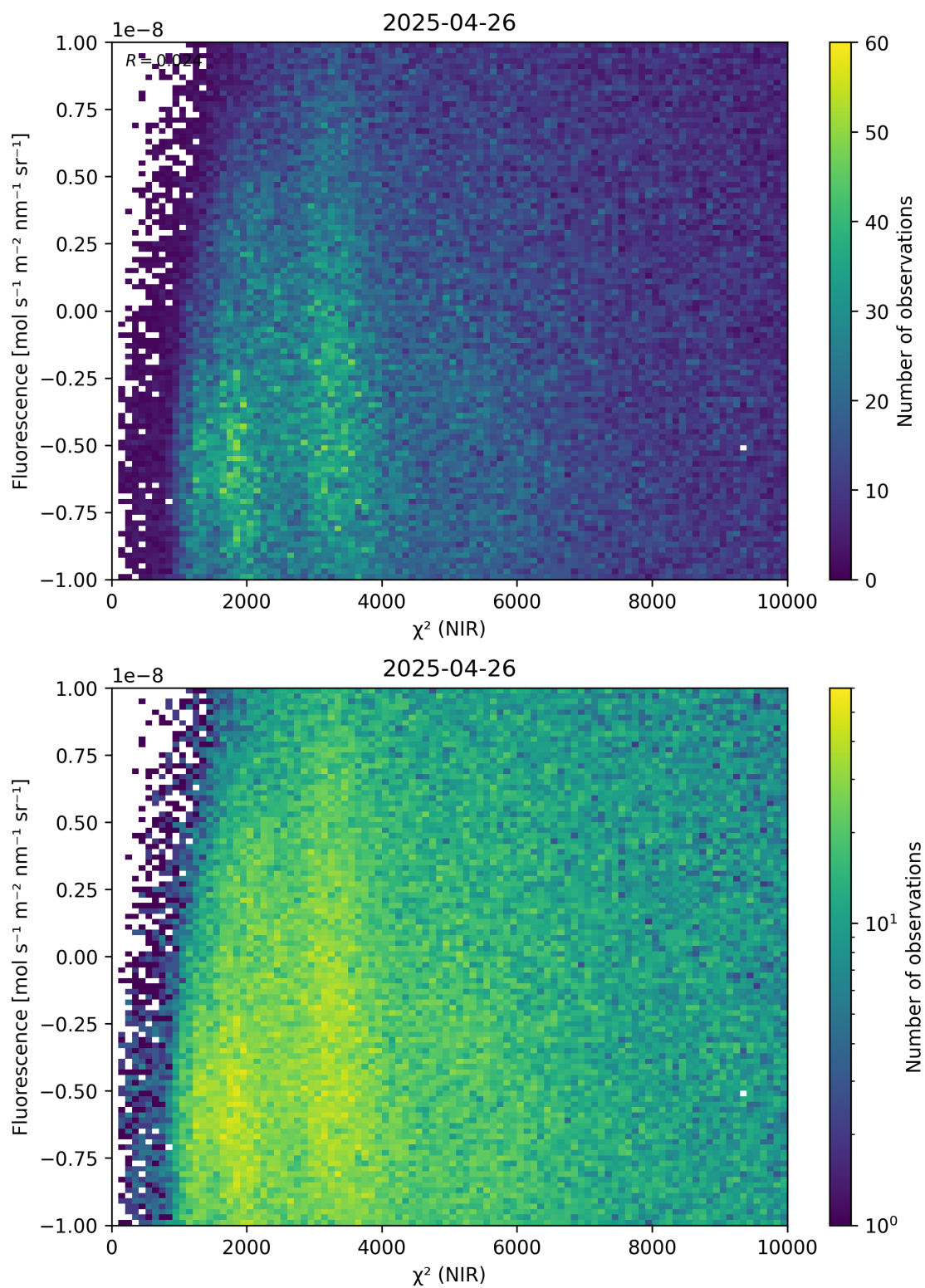
Figure 45: Scatter density plot of “ \chi^2 (NIR)” against “Fluorescence” for 2025-04-25 to 2025-04-27.
