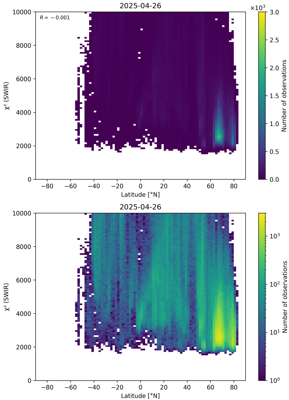
Figure 54: Scatter density plot of “Latitude” against “ \chi^2 (SWIR)” for 2025-04-25 to 2025-04-27.
