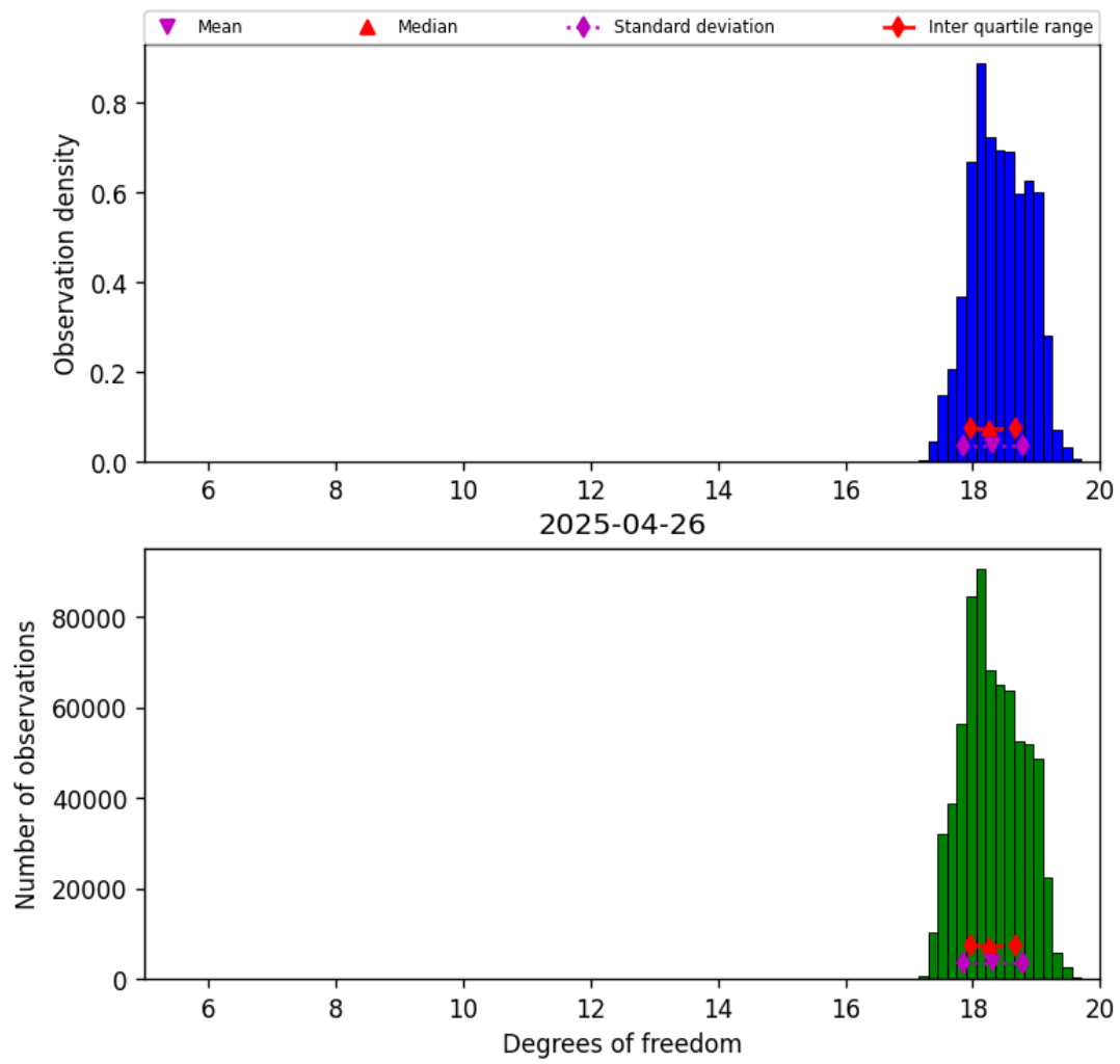
Figure 30: Histogram of "Degrees of freedom" for 2025-04-25 to 2025-04-27
