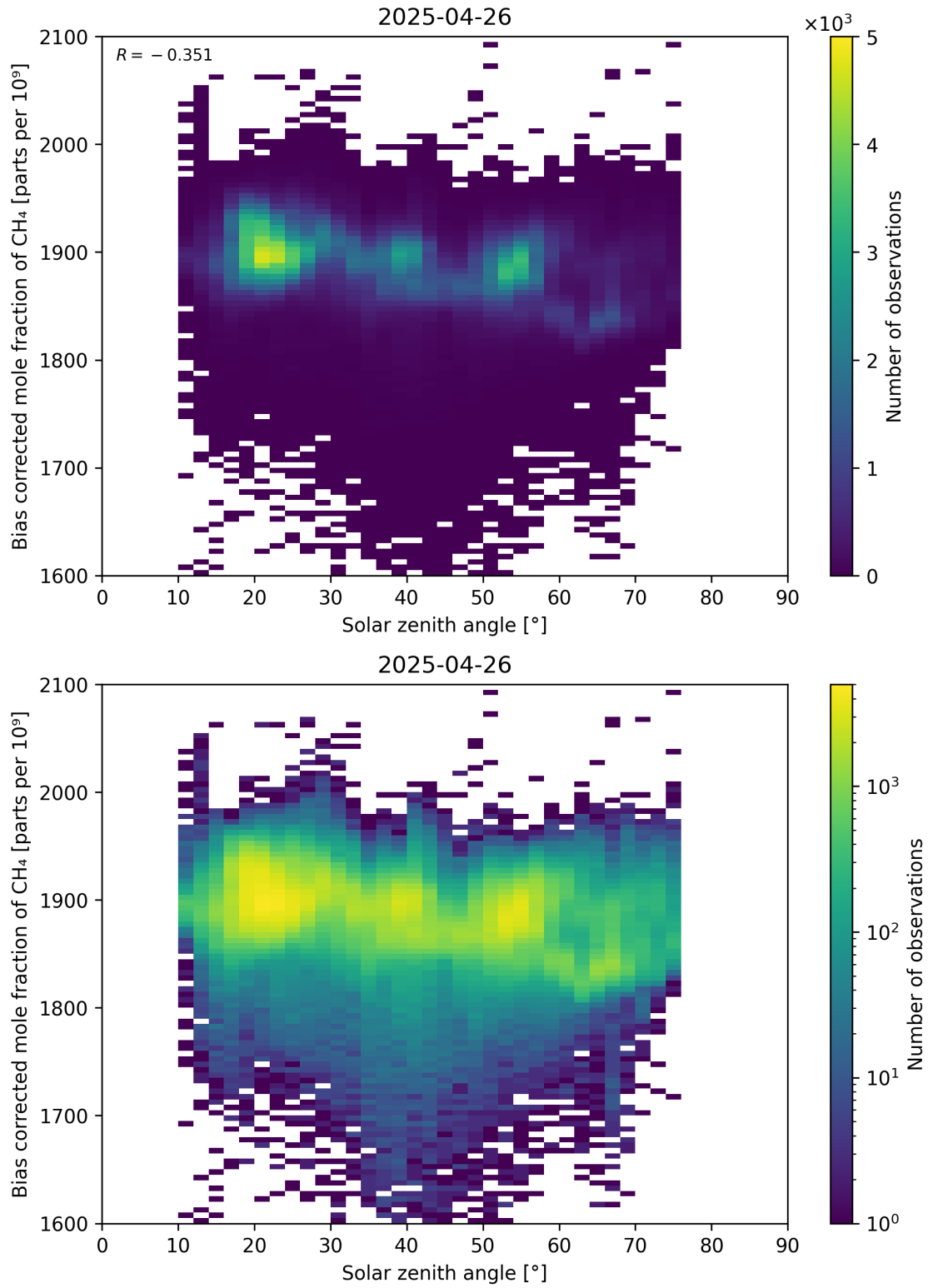
Figure 100: Scatter density plot of “Solar zenith angle” against “Bias corrected mole fraction of \text{CH}_4 ” for 2025-04-25 to 2025-04-27.
