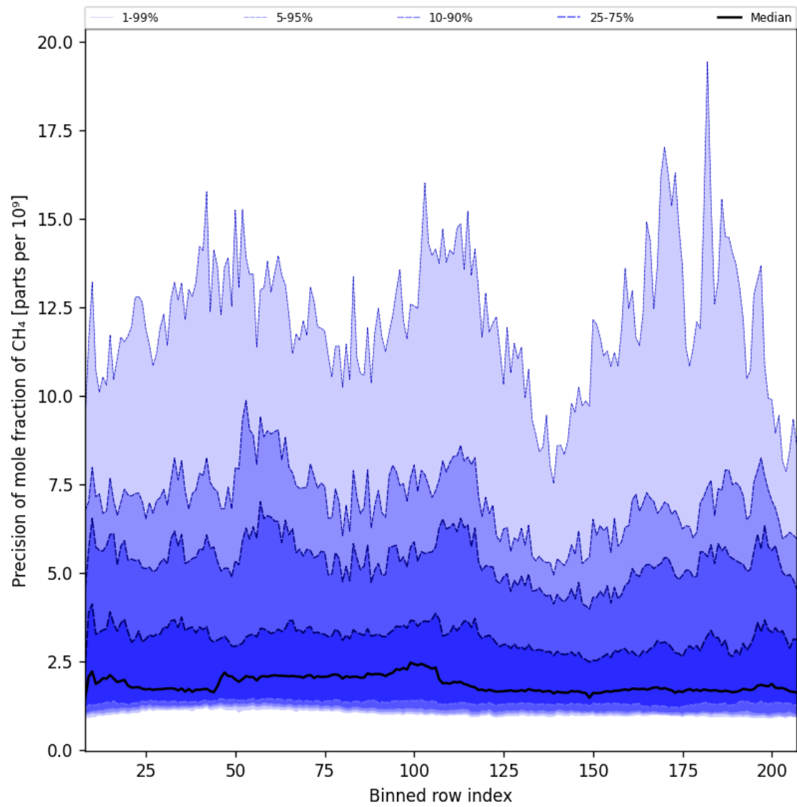
Figure 35: Along track statistics of “Precision of mole fraction of CH 4 ” for 2025-04-26 to 2025-04-28
