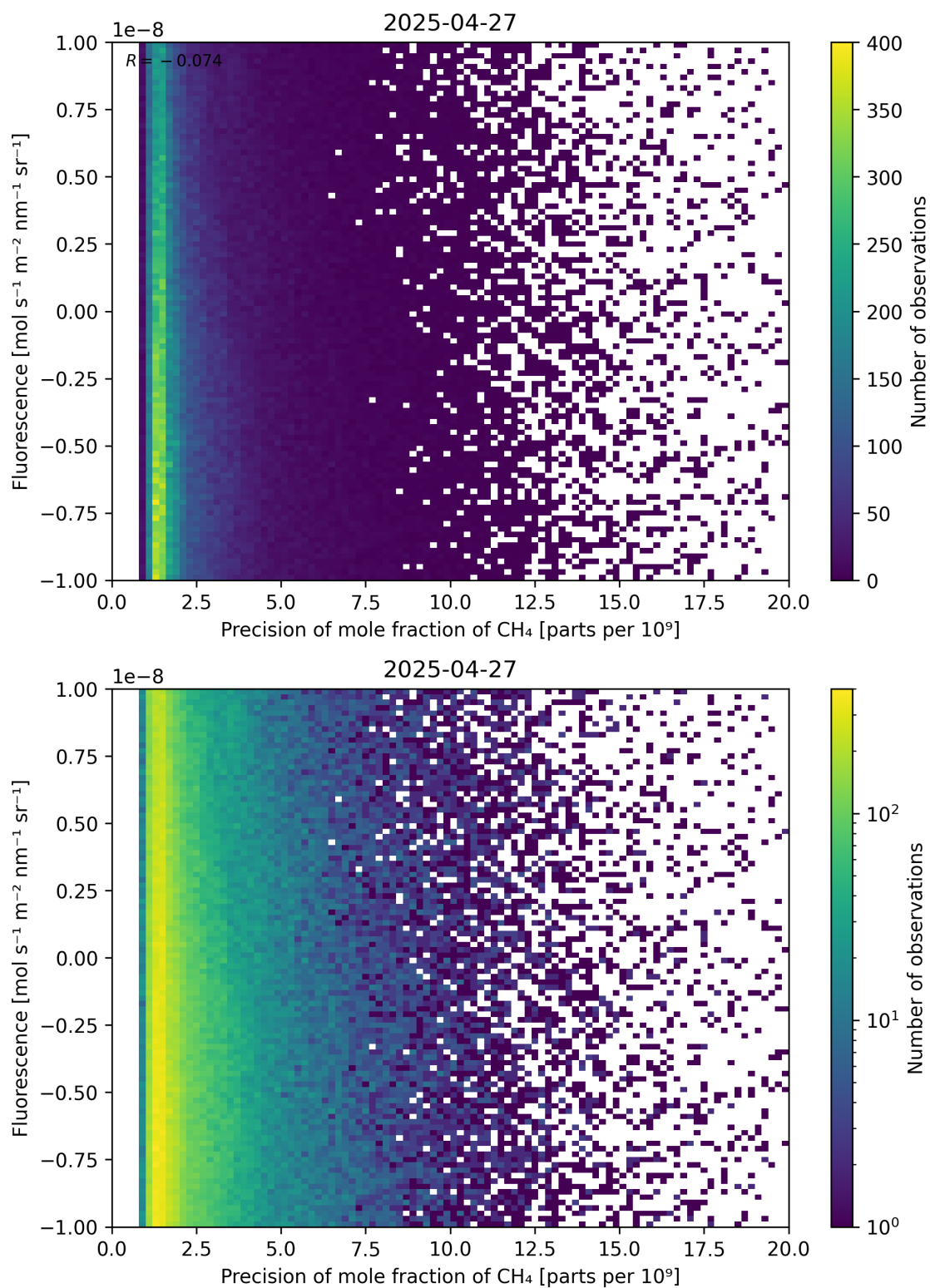
Figure 81: Scatter density plot of “Precision of mole fraction of CH 4 ” against “Fluorescence” for 2025-04-26 to 2025-04-28.
