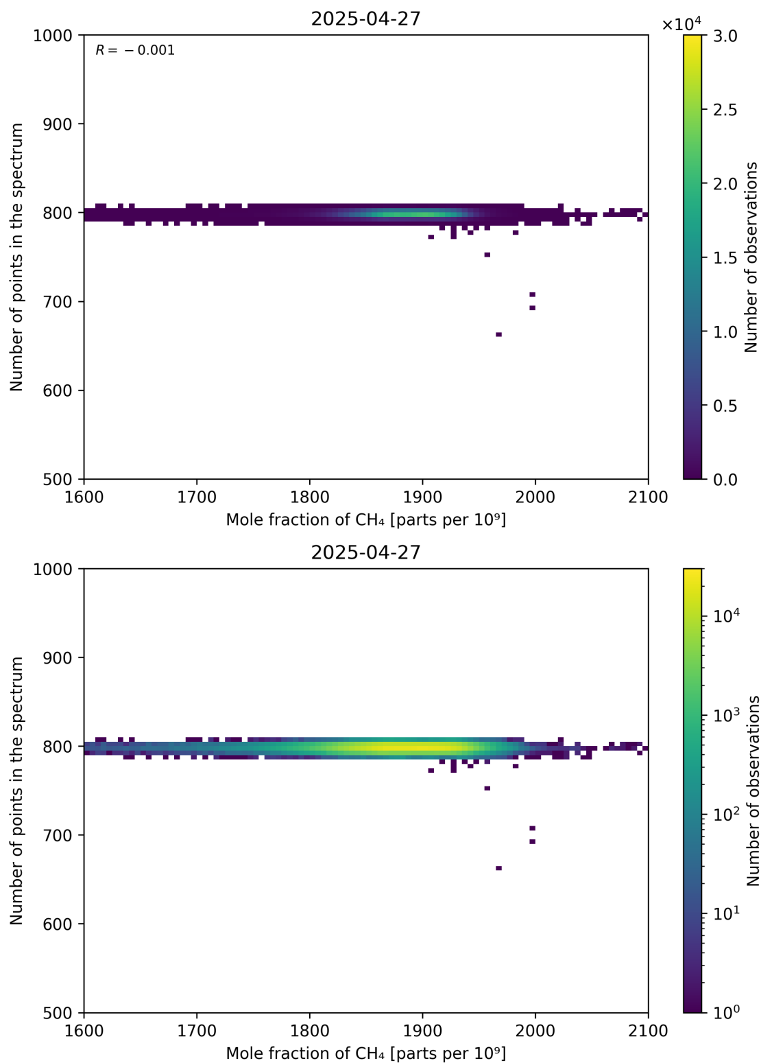
Figure 77: Scatter density plot of “Mole fraction of CH 4 ” against “Number of points in the spectrum” for 2025-04-26 to 2025-04-28.
