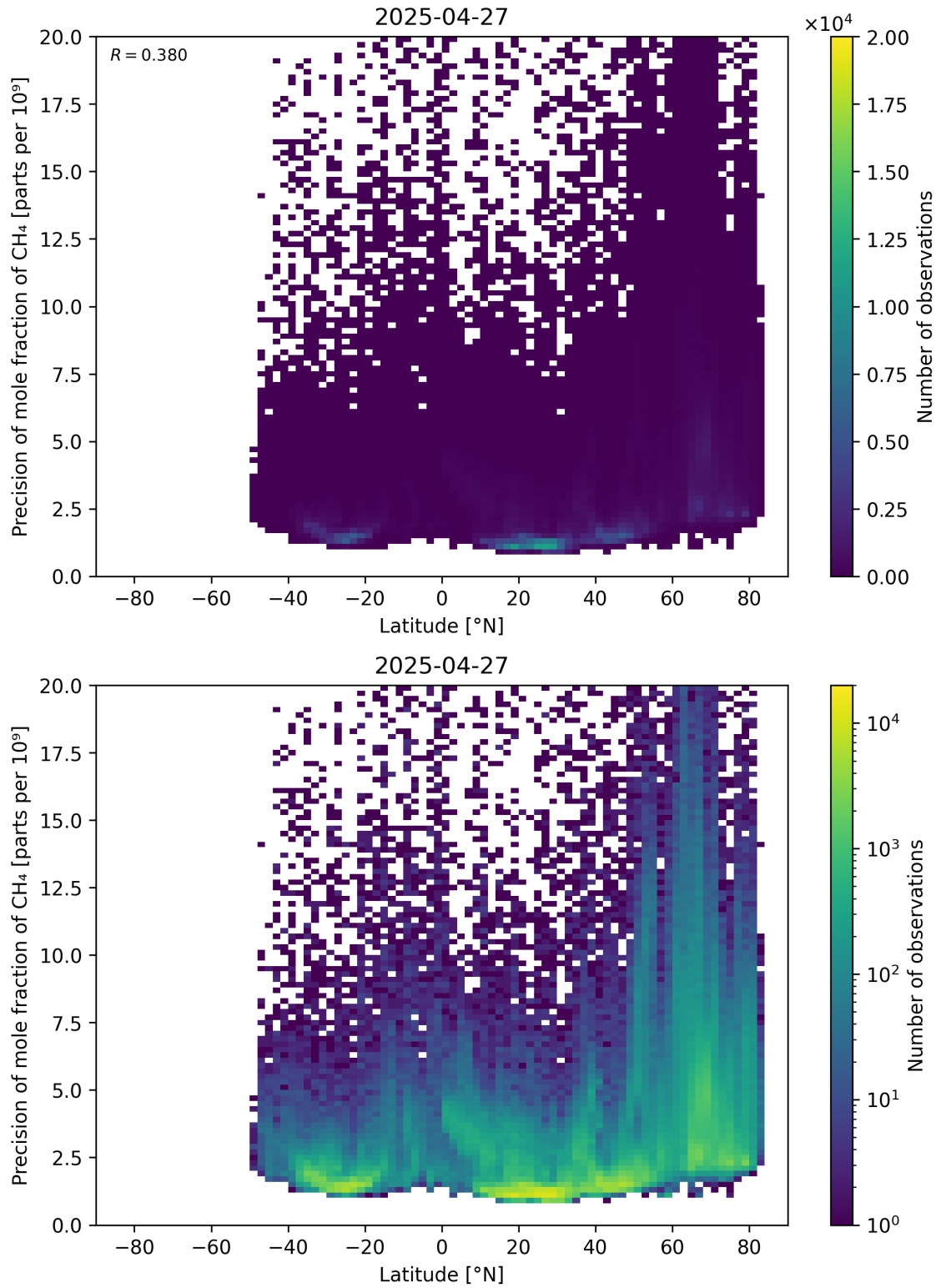
Figure 59: Scatter density plot of “Latitude” against “Precision of mole fraction of \text{CH}_4 ” for 2025-04-26 to 2025-04-28.
