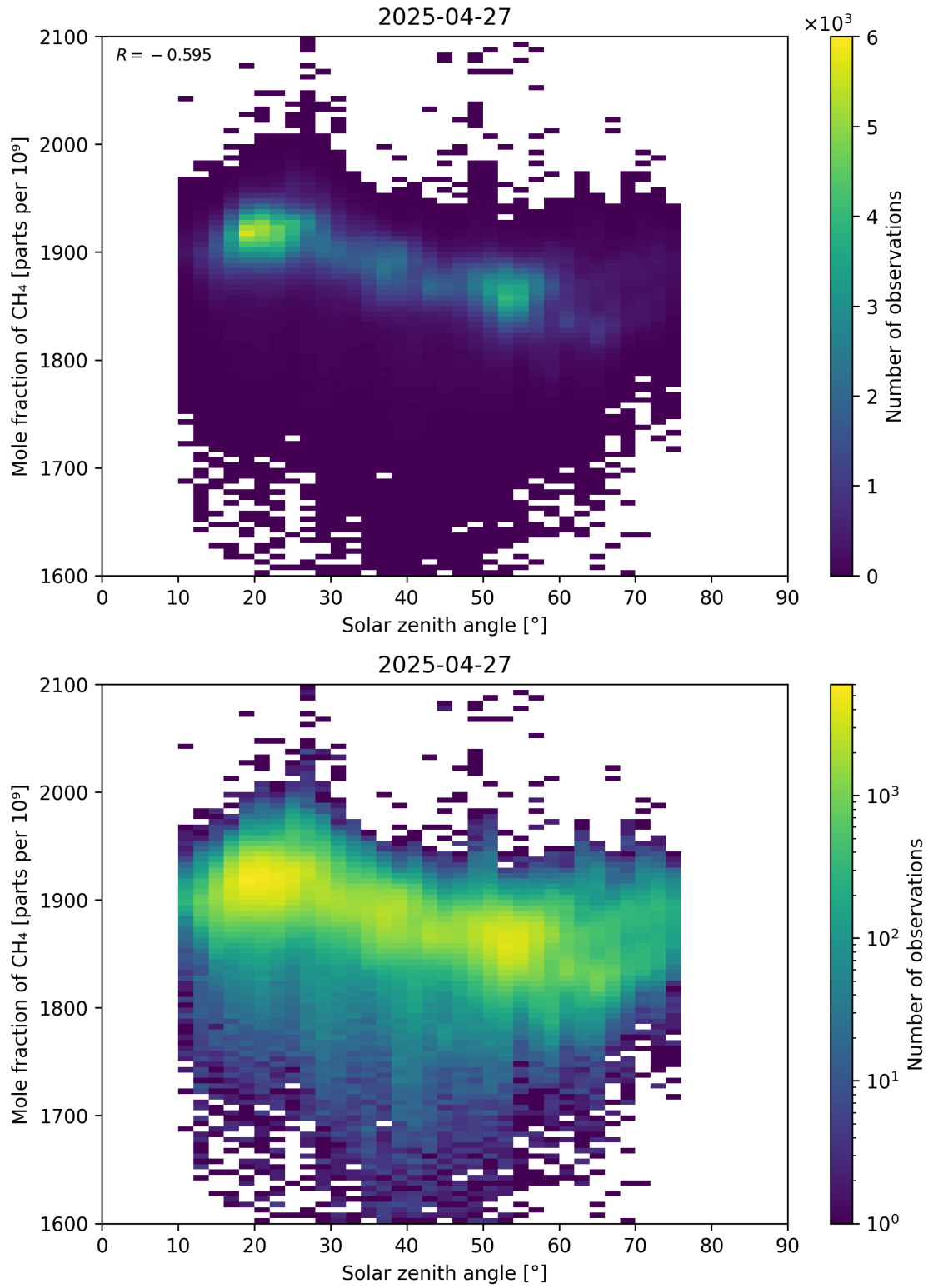
Figure 99: Scatter density plot of “Solar zenith angle” against “Mole fraction of CH 4 ” for 2025-04-26 to 2025-04-28.
