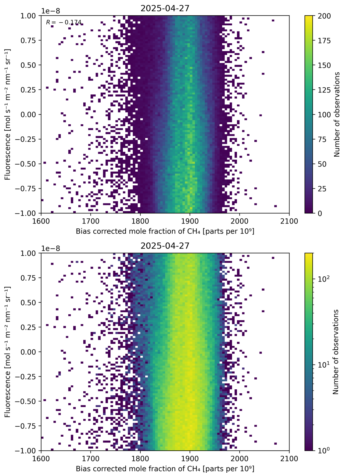
Figure 66: Scatter density plot of “Bias corrected mole fraction of \text{CH}_4 ” against “Fluorescence” for 2025-04-26 to 2025-04-28.
