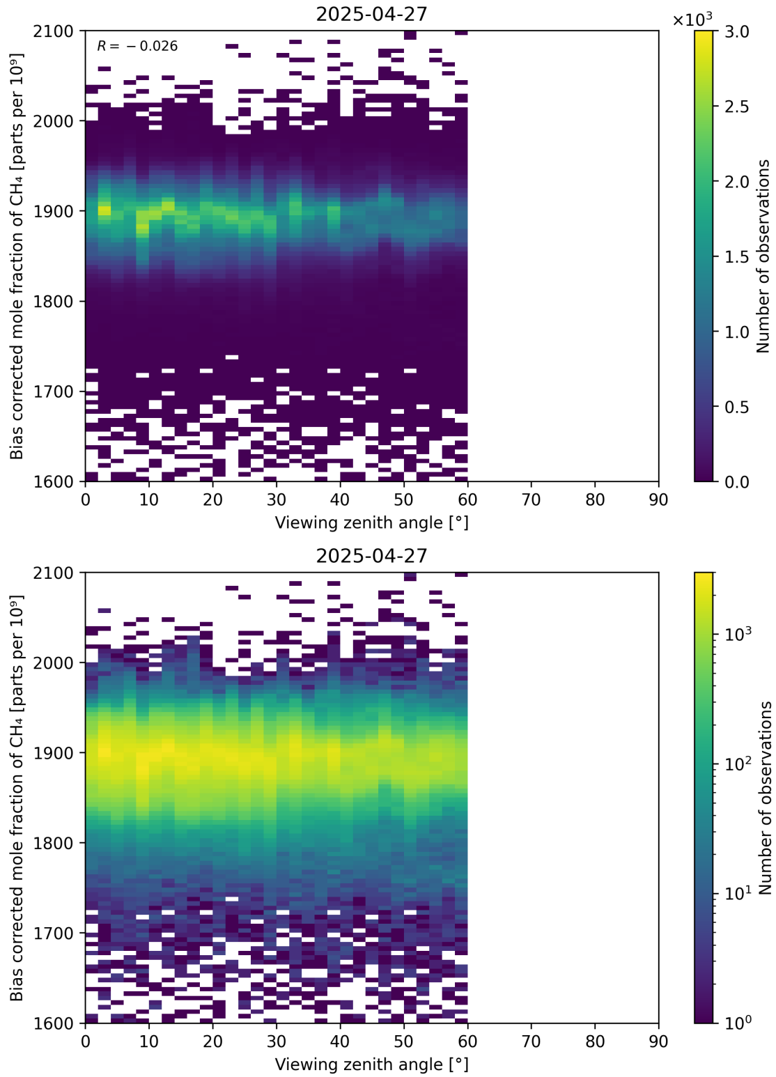
Figure 111: Scatter density plot of “Viewing zenith angle” against “Bias corrected mole fraction of CH 4 ” for 2025-04-26 to 2025-04-28.
