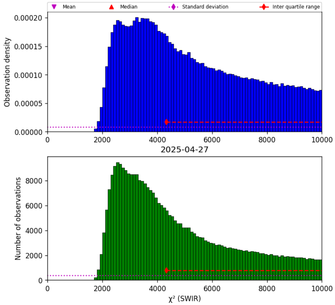
Figure 28: Histogram of “ \chi^2 (SWIR)” for 2025-04-26 to 2025-04-28
