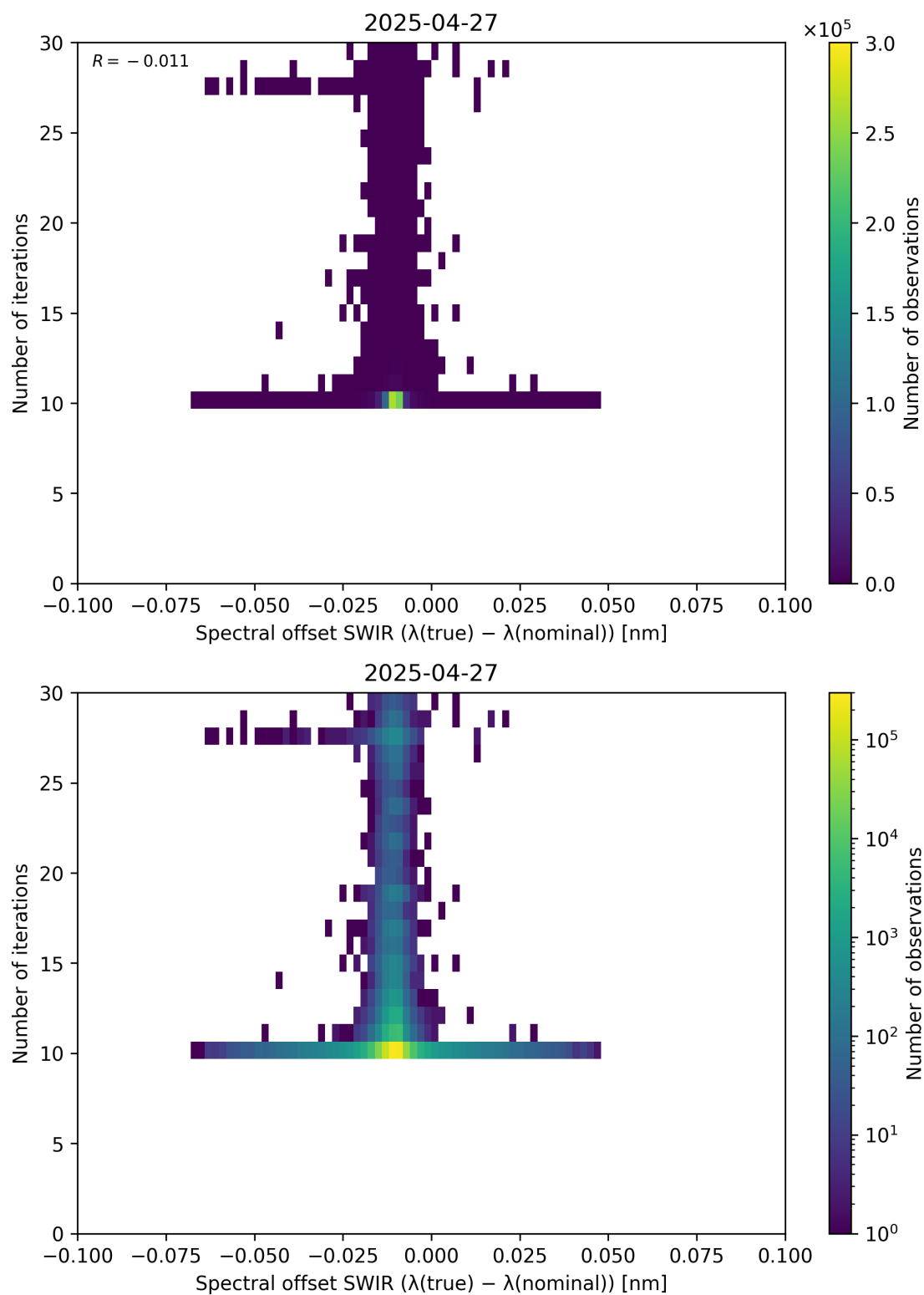
Figure 121: Scatter density plot of “Spectral offset SWIR ( \lambda_{\text{true}} - \lambda_{\text{nominal}} )” against “Number of iterations” for 2025-04-26 to 2025-04-28.
