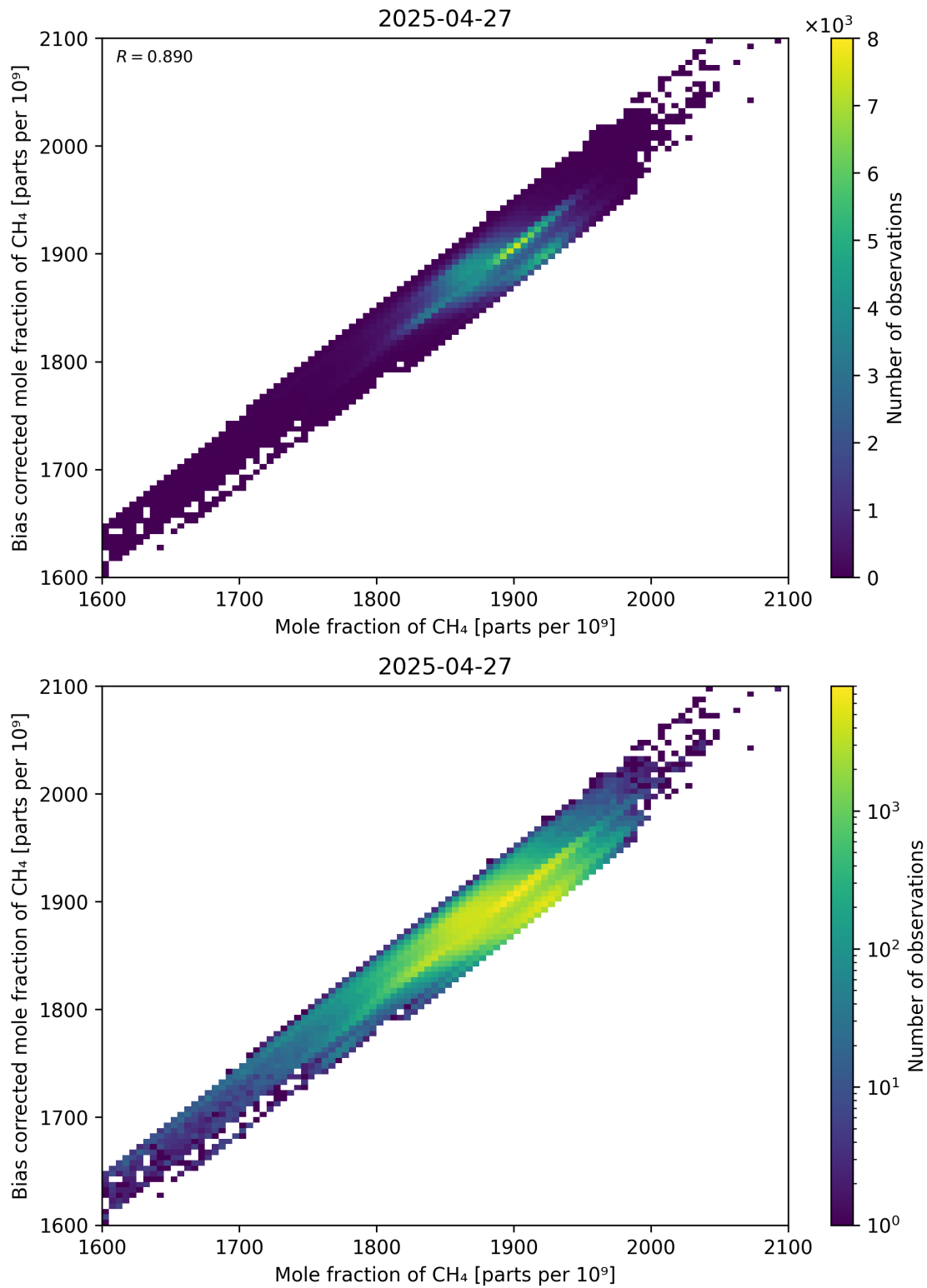
Figure 74: Scatter density plot of “Mole fraction of CH 4 ” against “Bias corrected mole fraction of CH 4 ” for 2025-04-26 to 2025-04-28.
