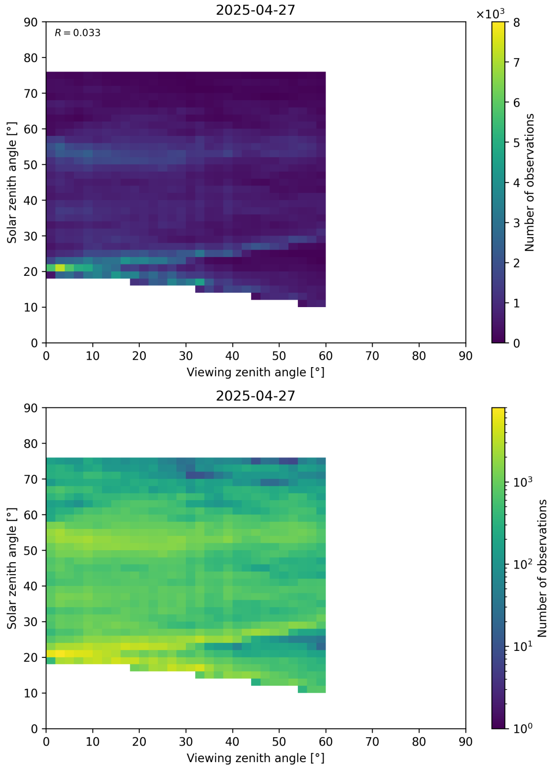
Figure 115: Scatter density plot of “Viewing zenith angle” against “Solar zenith angle” for 2025-04-26 to 2025-04-28.
