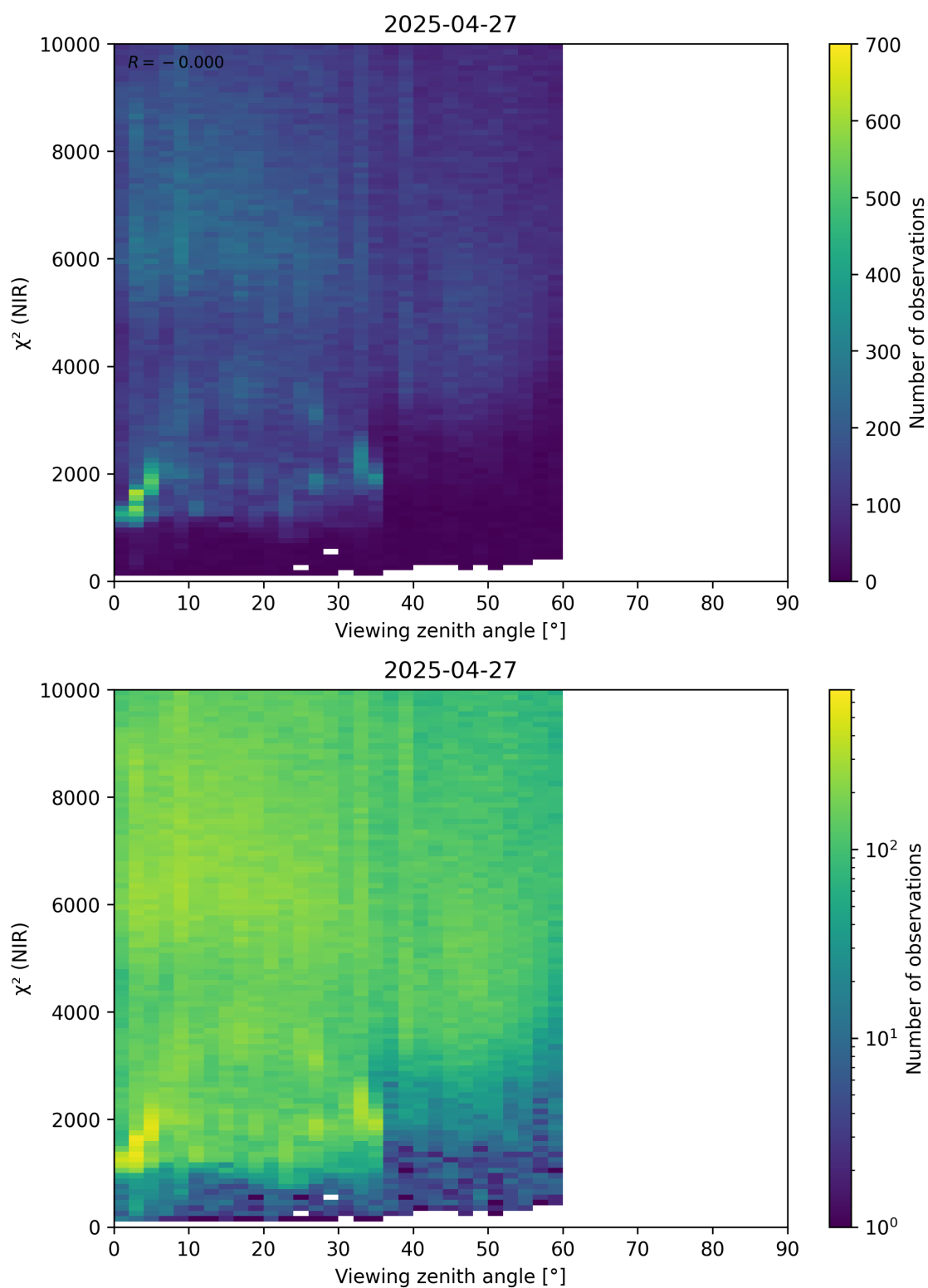
Figure 105: Scatter density plot of “Viewing zenith angle” against “ \chi^2 (NIR)” for 2025-04-26 to 2025-04-28.
