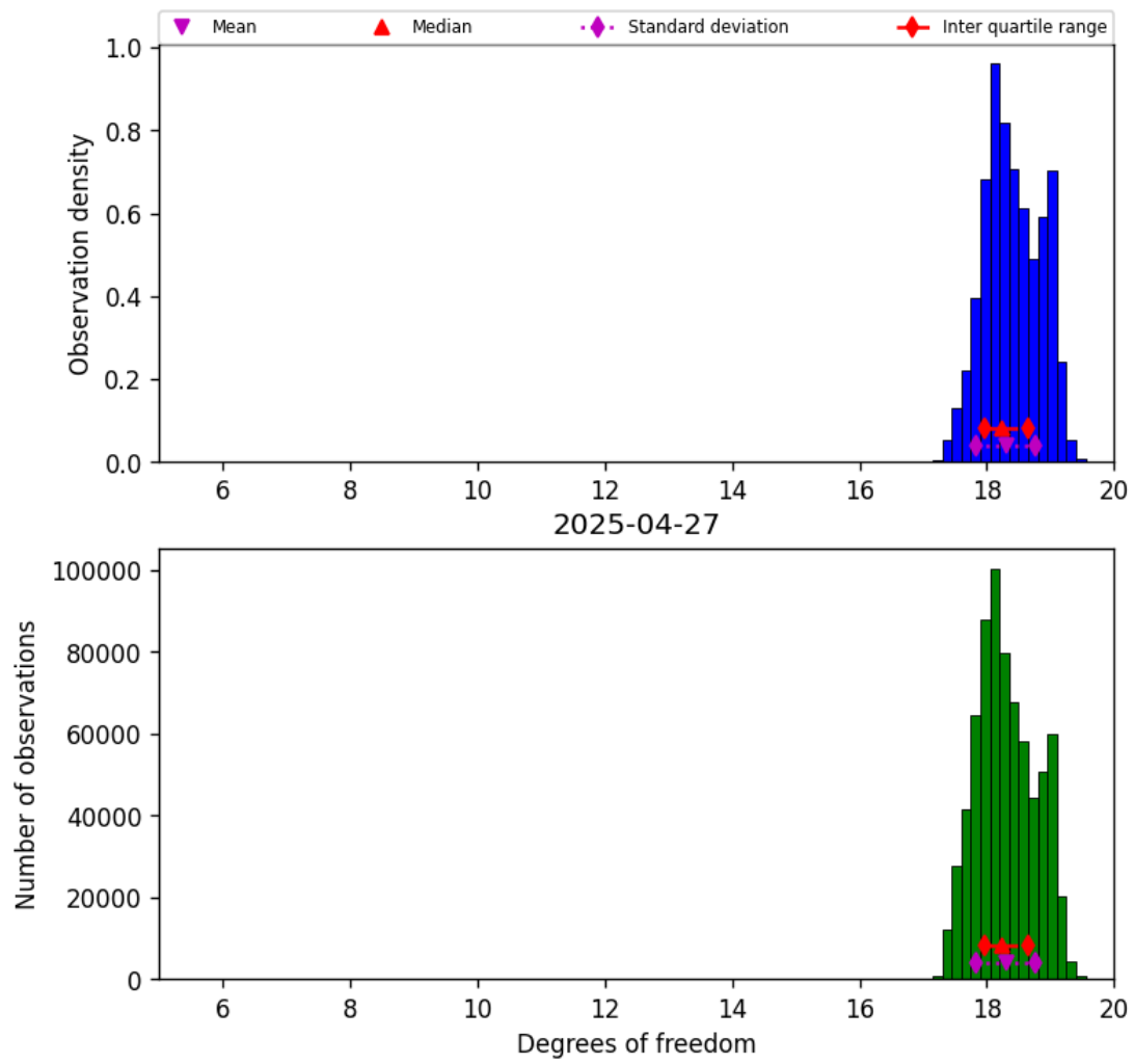
Figure 30: Histogram of “Degrees of freedom” for 2025-04-26 to 2025-04-28
