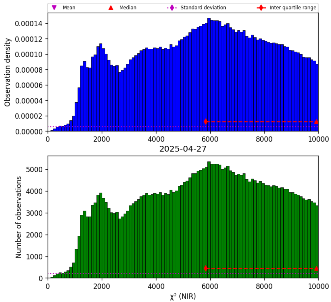
Figure 29: Histogram of “ \chi^2 (NIR)” for 2025-04-26 to 2025-04-28
