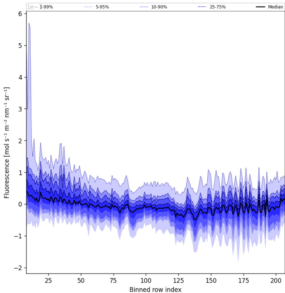
Figure 43: Along track statistics of “Fluorescence” for 2025-04-26 to 2025-04-28
