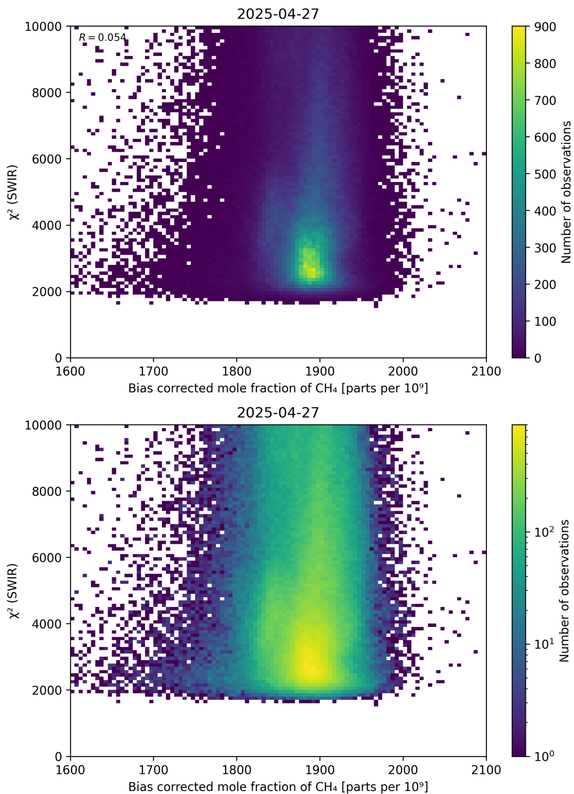
Figure 64: Scatter density plot of “Bias corrected mole fraction of \text{CH}_4 ” against “ \chi^2 (SWIR)” for 2025-04-26 to 2025-04-28.
