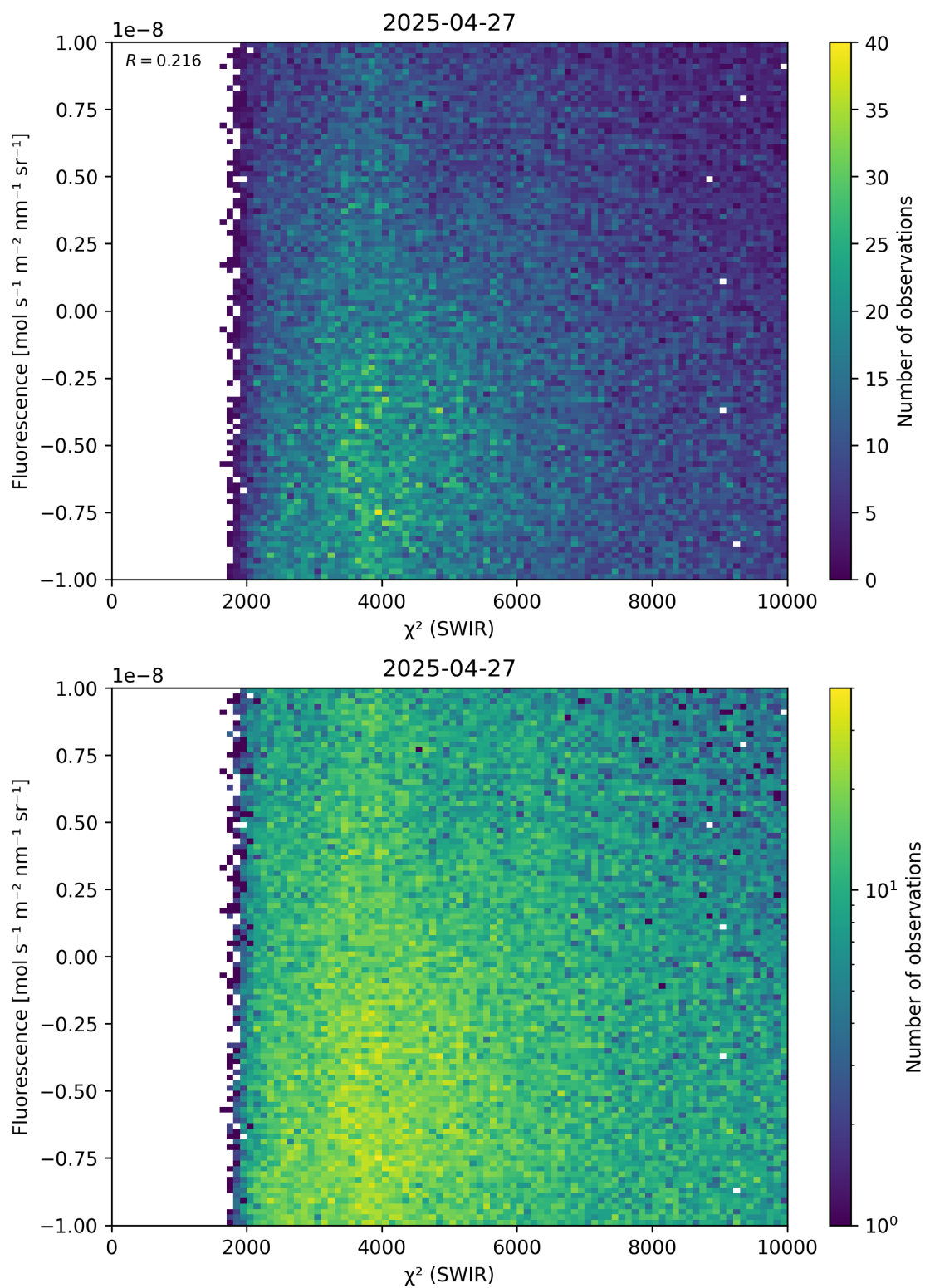
Figure 49: Scatter density plot of “ \chi^2 (SWIR)” against “Fluorescence” for 2025-04-26 to 2025-04-28.
