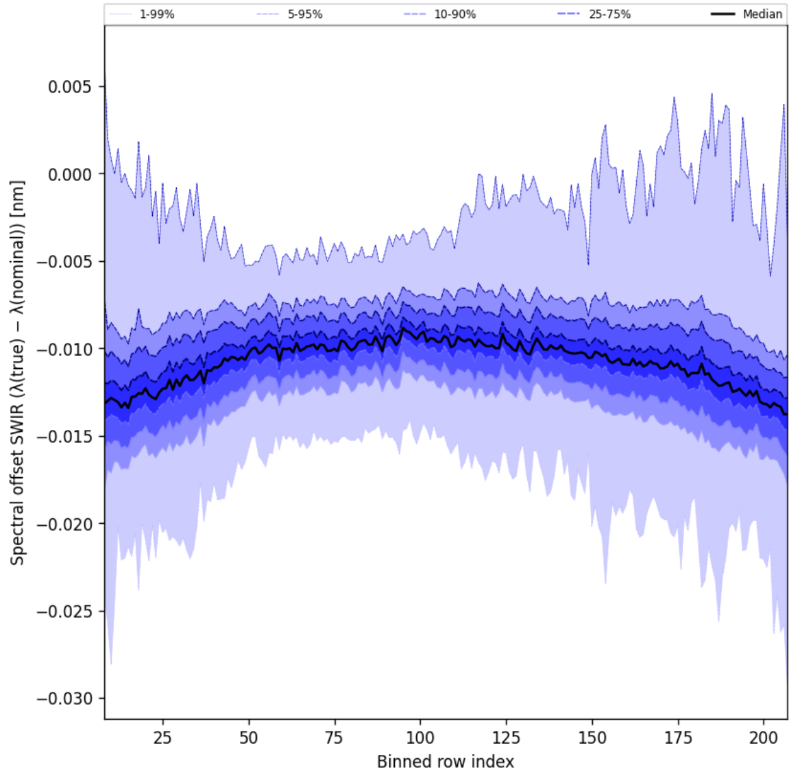
Figure 38: Along track statistics of “Spectral offset SWIR ( \lambda_{\text{true}} - \lambda_{\text{nominal}} )” for 2025-04-26 to 2025-04-28
