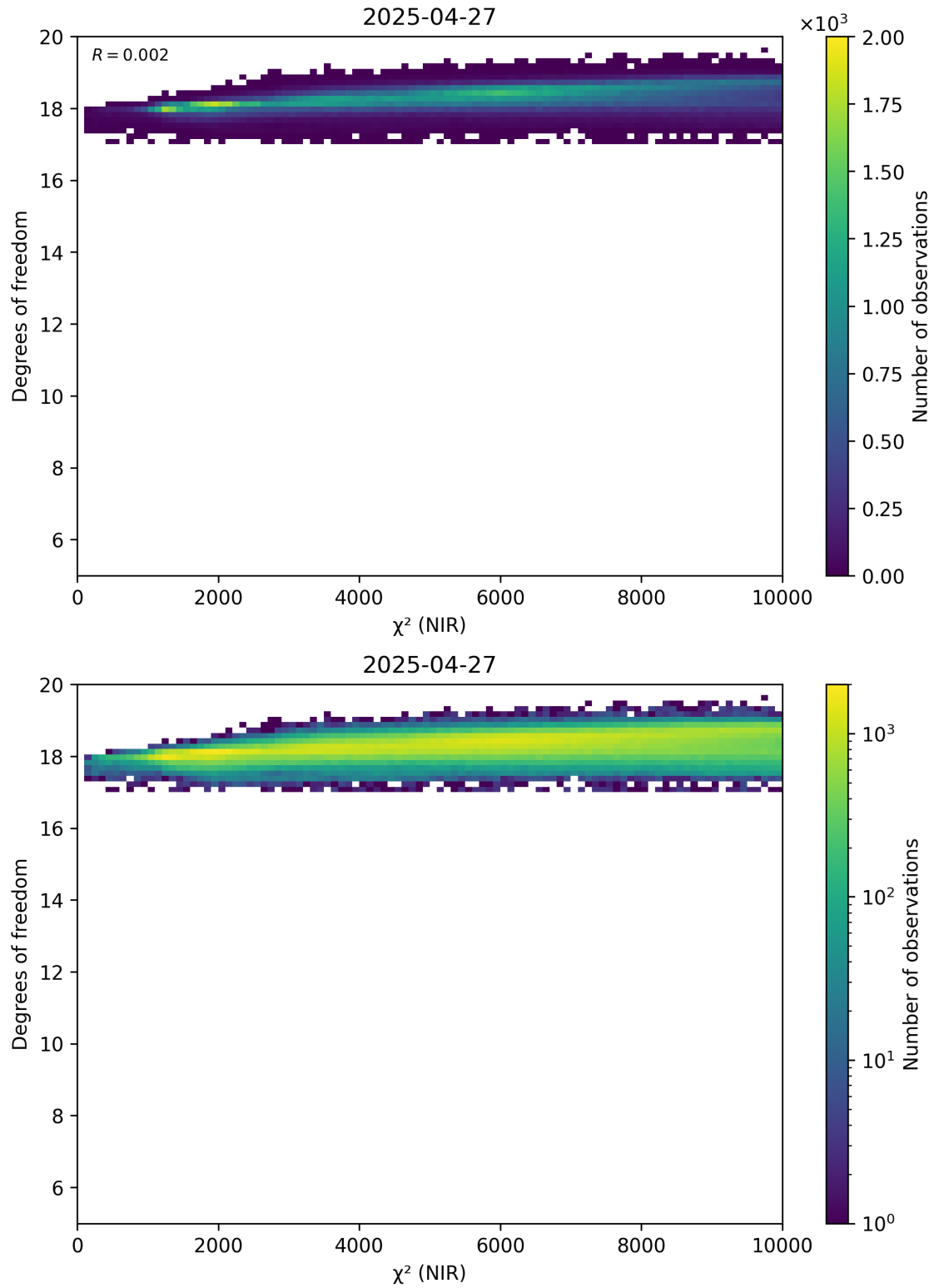
Figure 44: Scatter density plot of “ \chi^2 (NIR)” against “Degrees of freedom” for 2025-04-26 to 2025-04-28.
