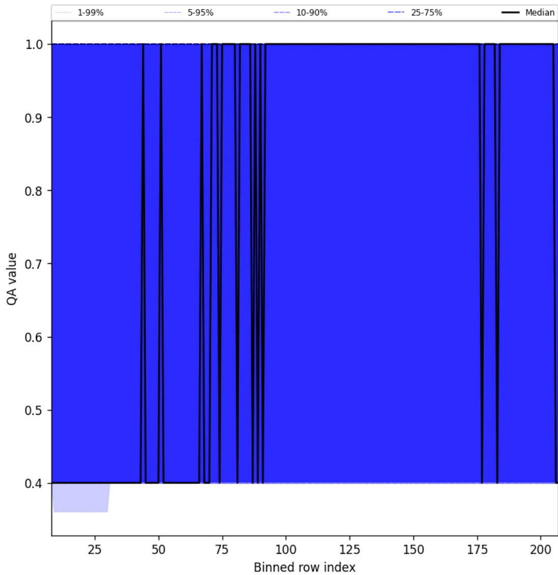
Figure 33: Along track statistics of “QA value” for 2025-04-26 to 2025-04-28
