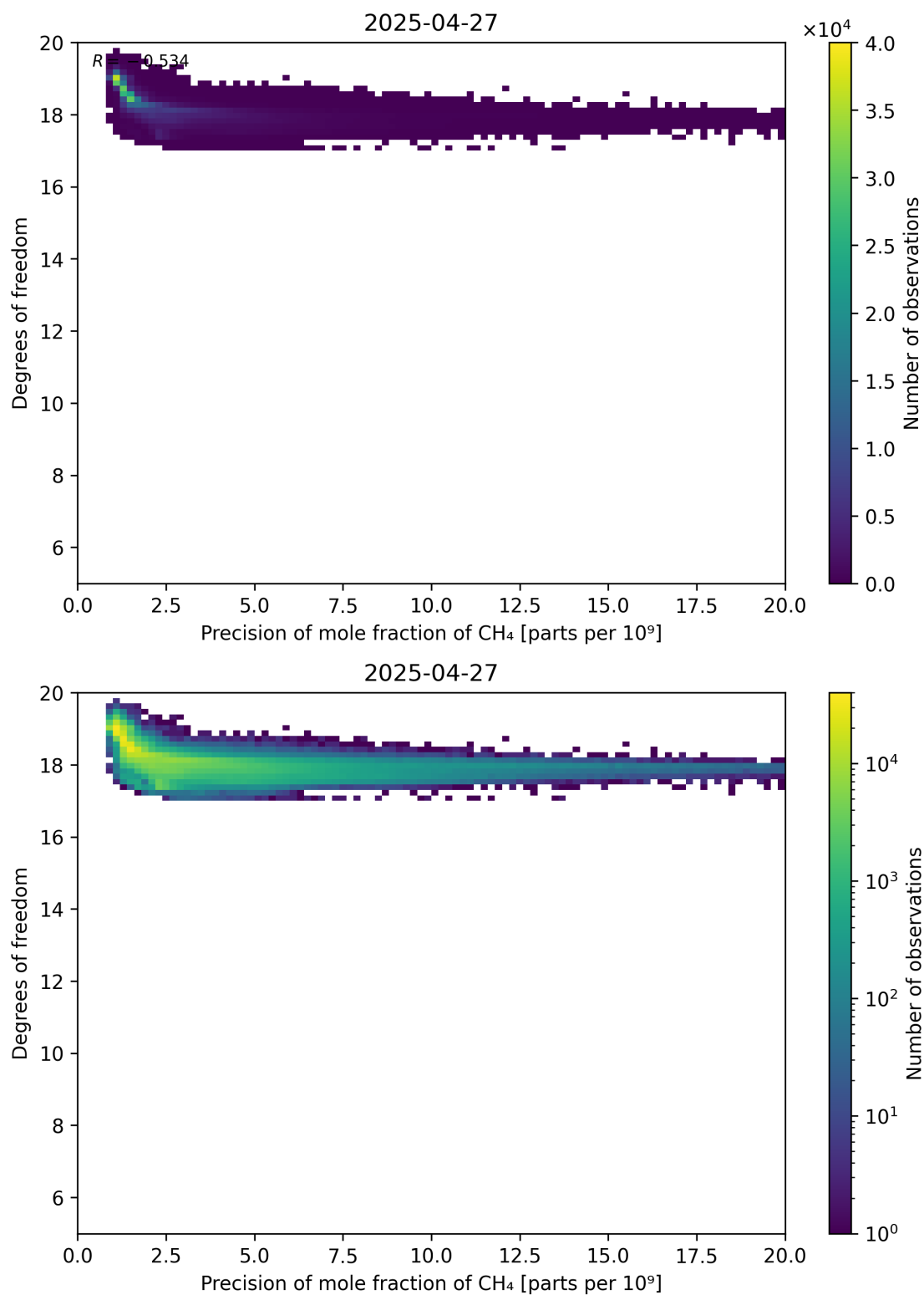
Figure 80: Scatter density plot of “Precision of mole fraction of CH 4 ” against “Degrees of freedom” for 2025-04-26 to 2025-04-28.
