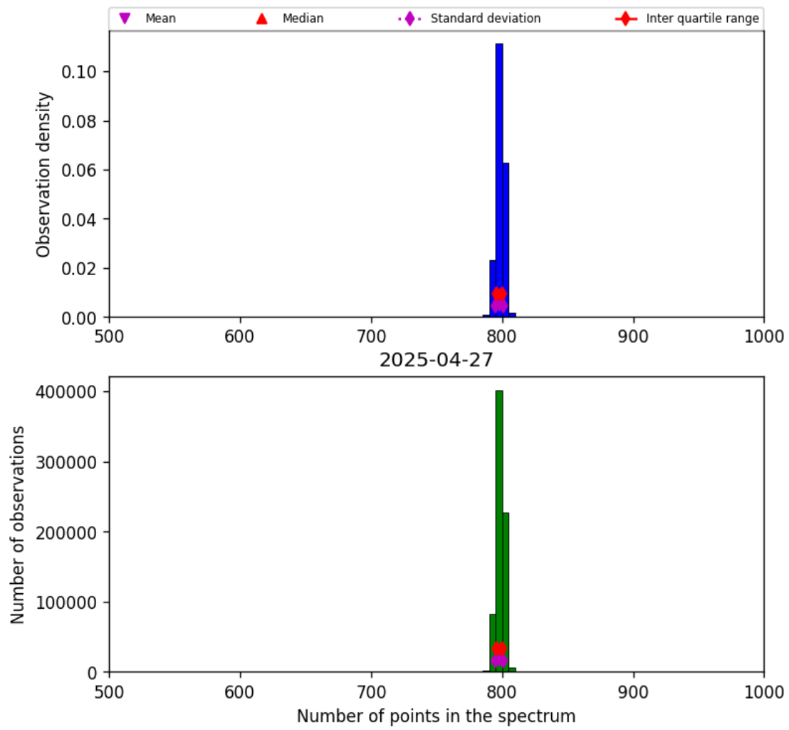
Figure 26: Histogram of “Number of points in the spectrum” for 2025-04-26 to 2025-04-28
