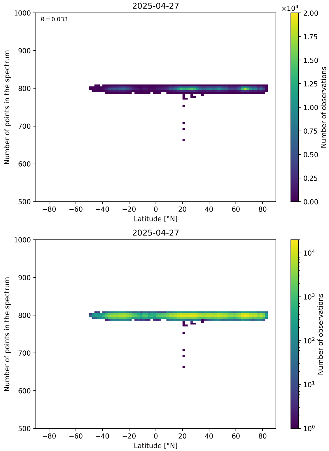
Figure 61: Scatter density plot of “Latitude” against “Number of points in the spectrum” for 2025-04-26 to 2025-04-28.
