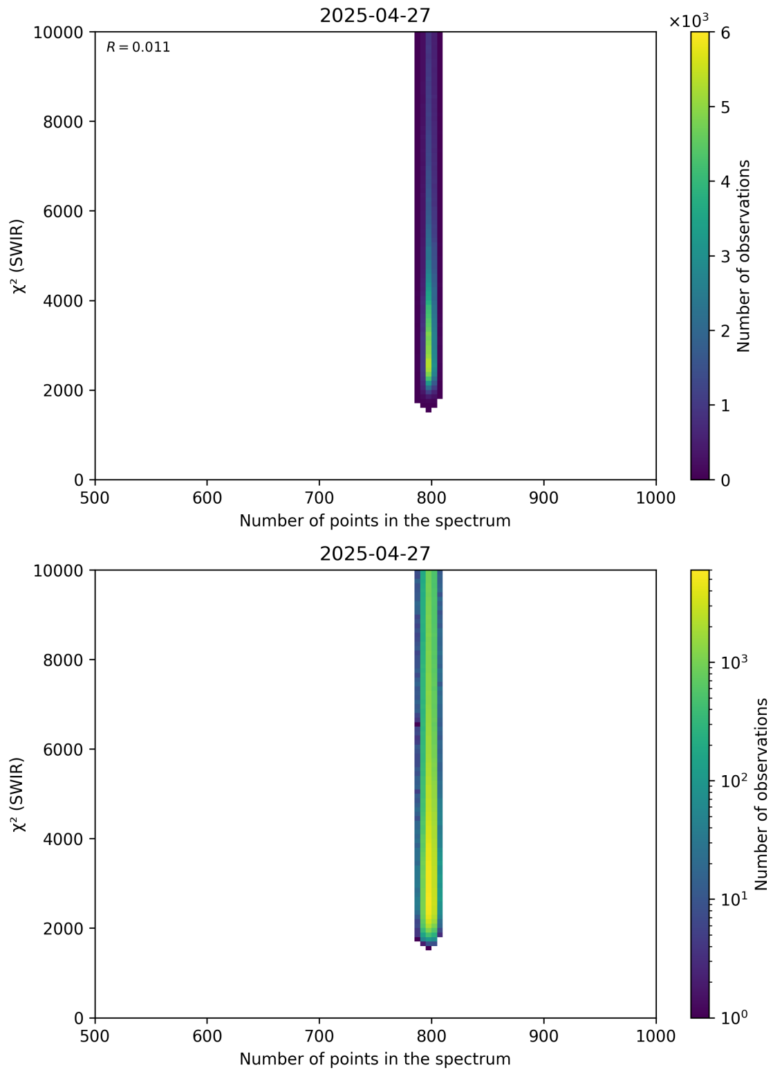
Figure 89: Scatter density plot of “Number of points in the spectrum” against “ \chi^2 (SWIR)” for 2025-04-26 to 2025-04-28.
