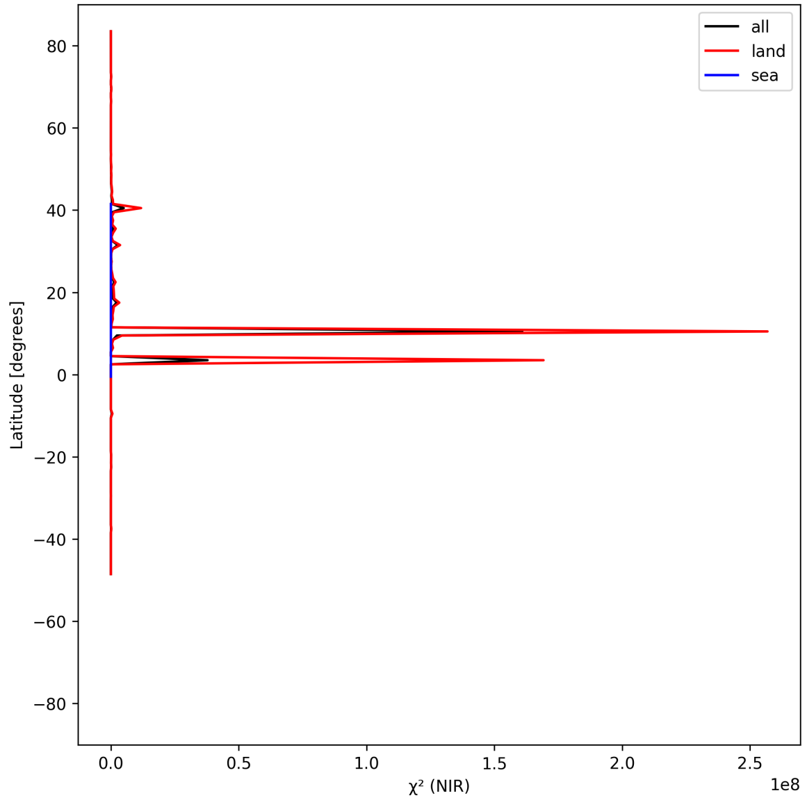
Figure 18: Zonal average of “ \chi^2 (NIR)” for 2025-04-26 to 2025-04-28.
