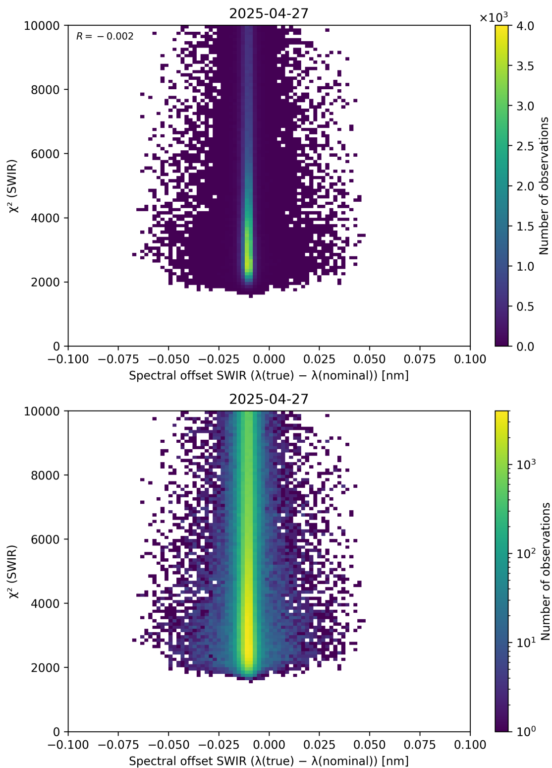
Figure 118: Scatter density plot of “Spectral offset SWIR ( \lambda_{\text{true}} - \lambda_{\text{nominal}} )” against “ \chi^2 (SWIR)” for 2025-04-26 to 2025-04-28.
