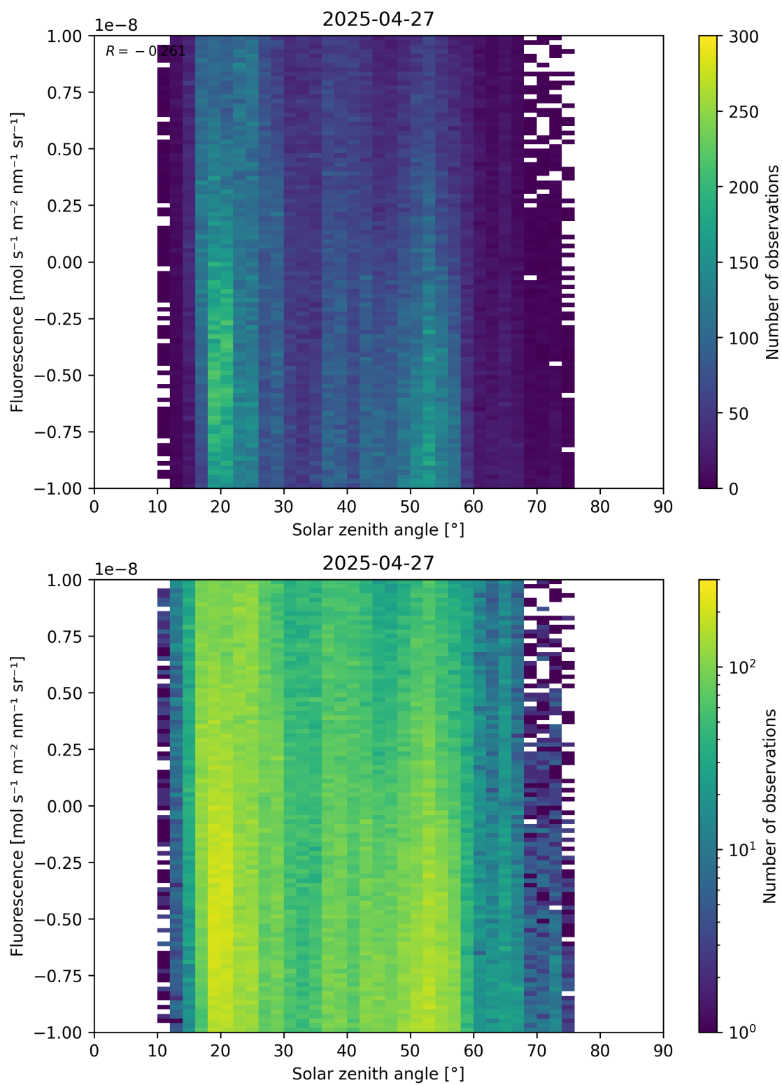
Figure 97: Scatter density plot of “Solar zenith angle” against “Fluorescence” for 2025-04-26 to 2025-04-28.
