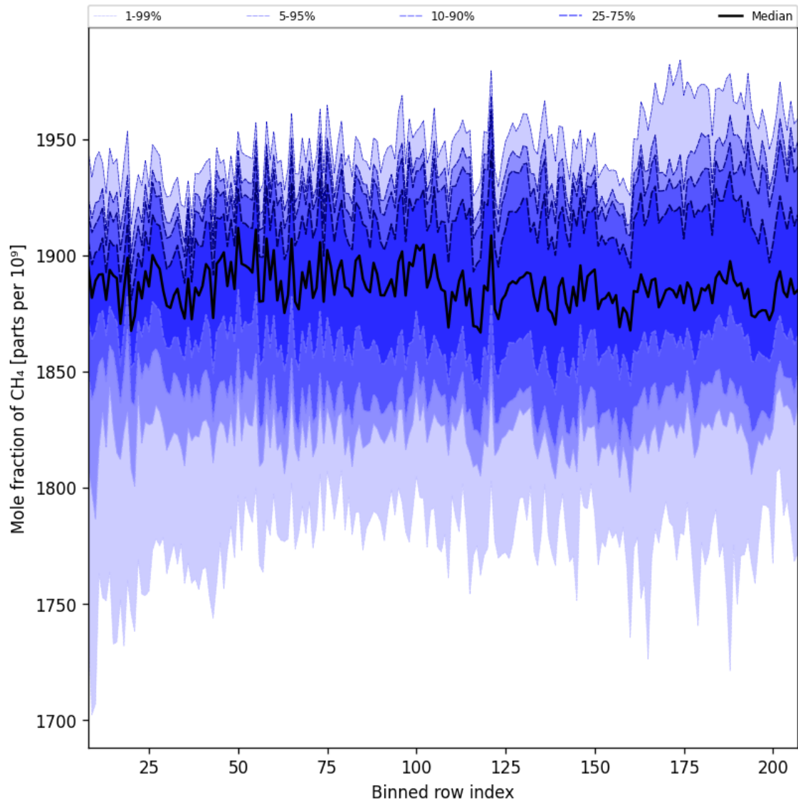
Figure 34: Along track statistics of “Mole fraction of CH 4 ” for 2025-04-26 to 2025-04-28
