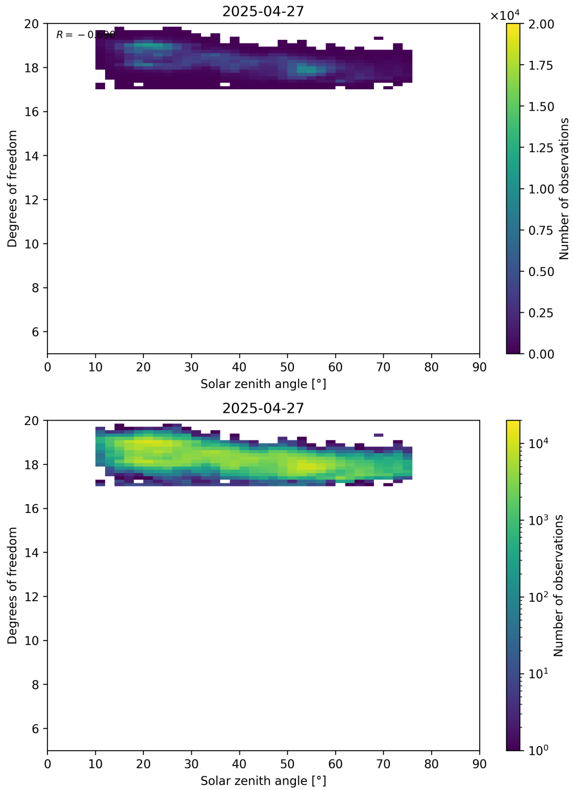
Figure 96: Scatter density plot of “Solar zenith angle” against “Degrees of freedom” for 2025-04-26 to 2025-04-28.
