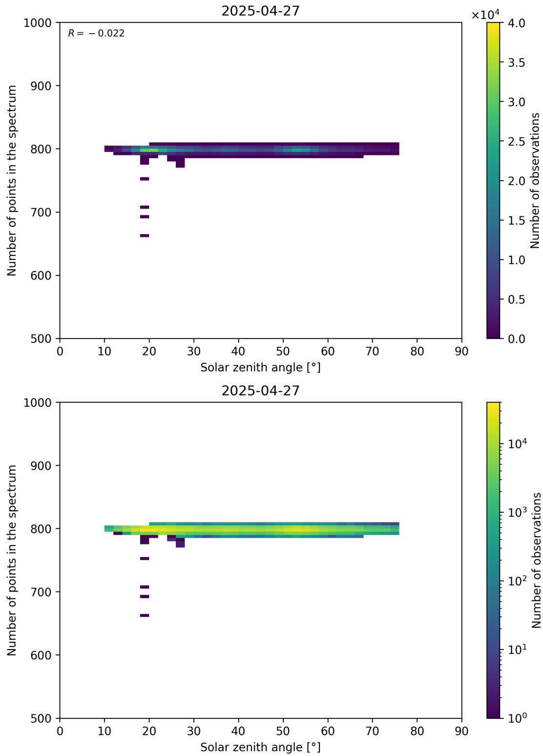
Figure 103: Scatter density plot of “Solar zenith angle” against “Number of points in the spectrum” for 2025-04-26 to 2025-04-28.
