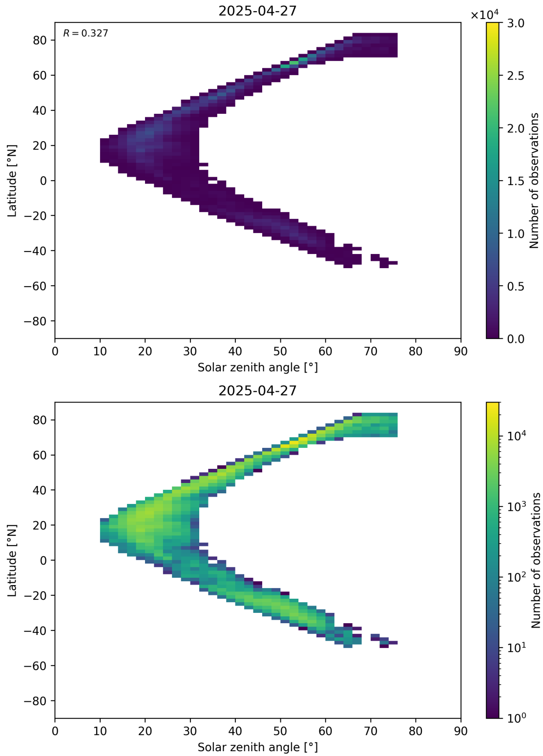
Figure 98: Scatter density plot of “Solar zenith angle” against “Latitude” for 2025-04-26 to 2025-04-28.
