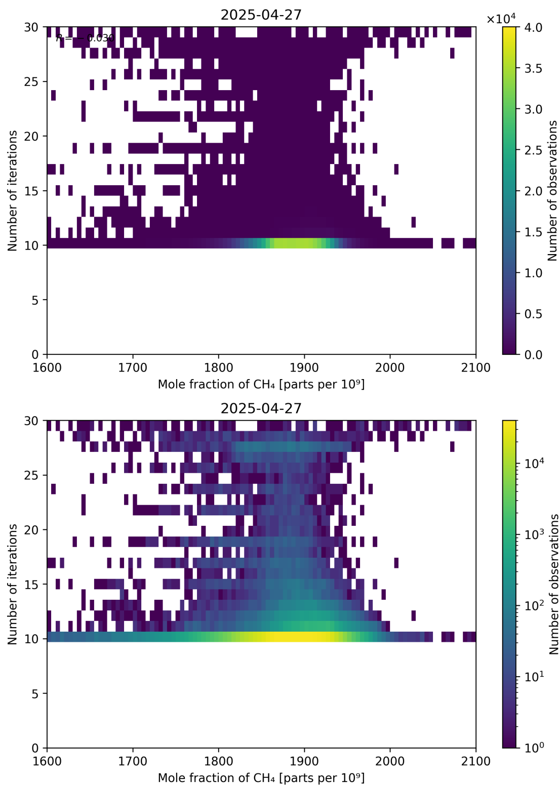
Figure 76: Scatter density plot of “Mole fraction of CH 4 ” against “Number of iterations” for 2025-04-26 to 2025-04-28.
