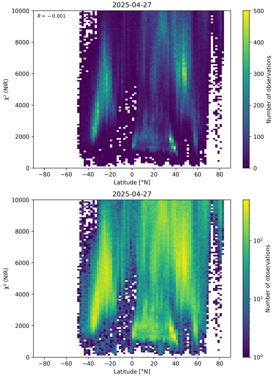
Figure 53: Scatter density plot of “Latitude” against “ \chi^2 (NIR)” for 2025-04-26 to 2025-04-28.
