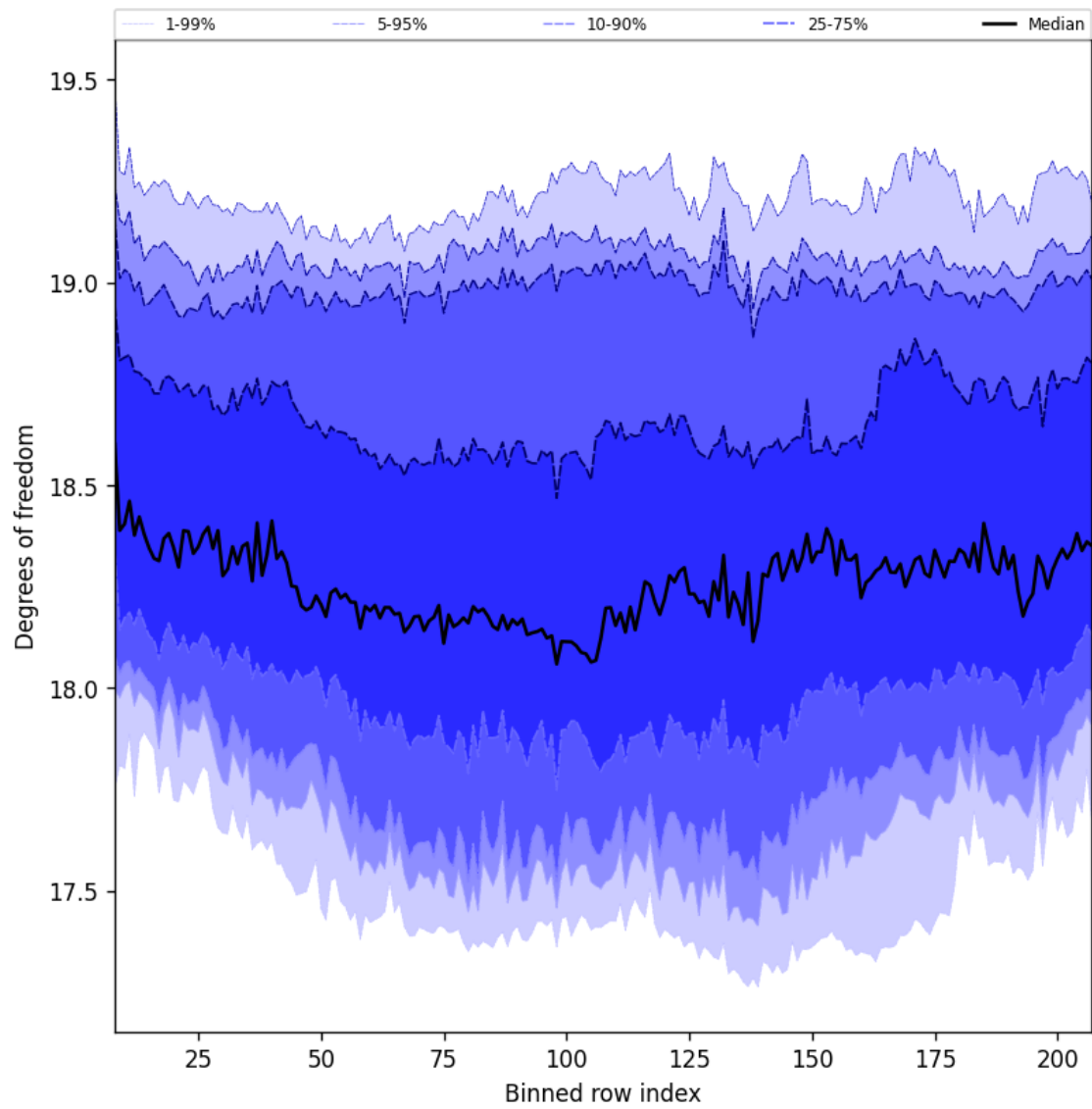
Figure 41: Along track statistics of “Degrees of freedom” for 2025-04-26 to 2025-04-28
