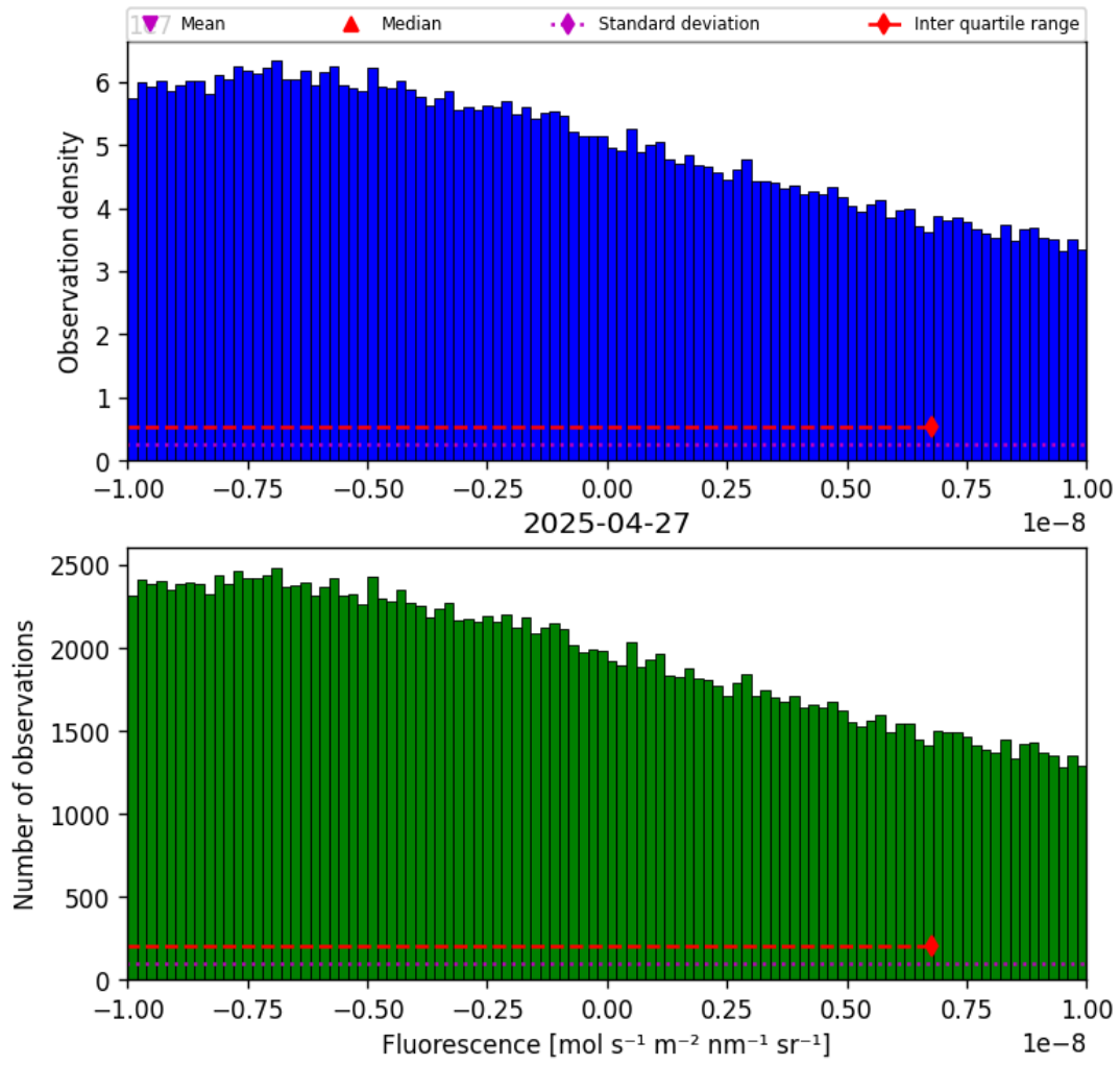
Figure 32: Histogram of “Fluorescence” for 2025-04-26 to 2025-04-28
