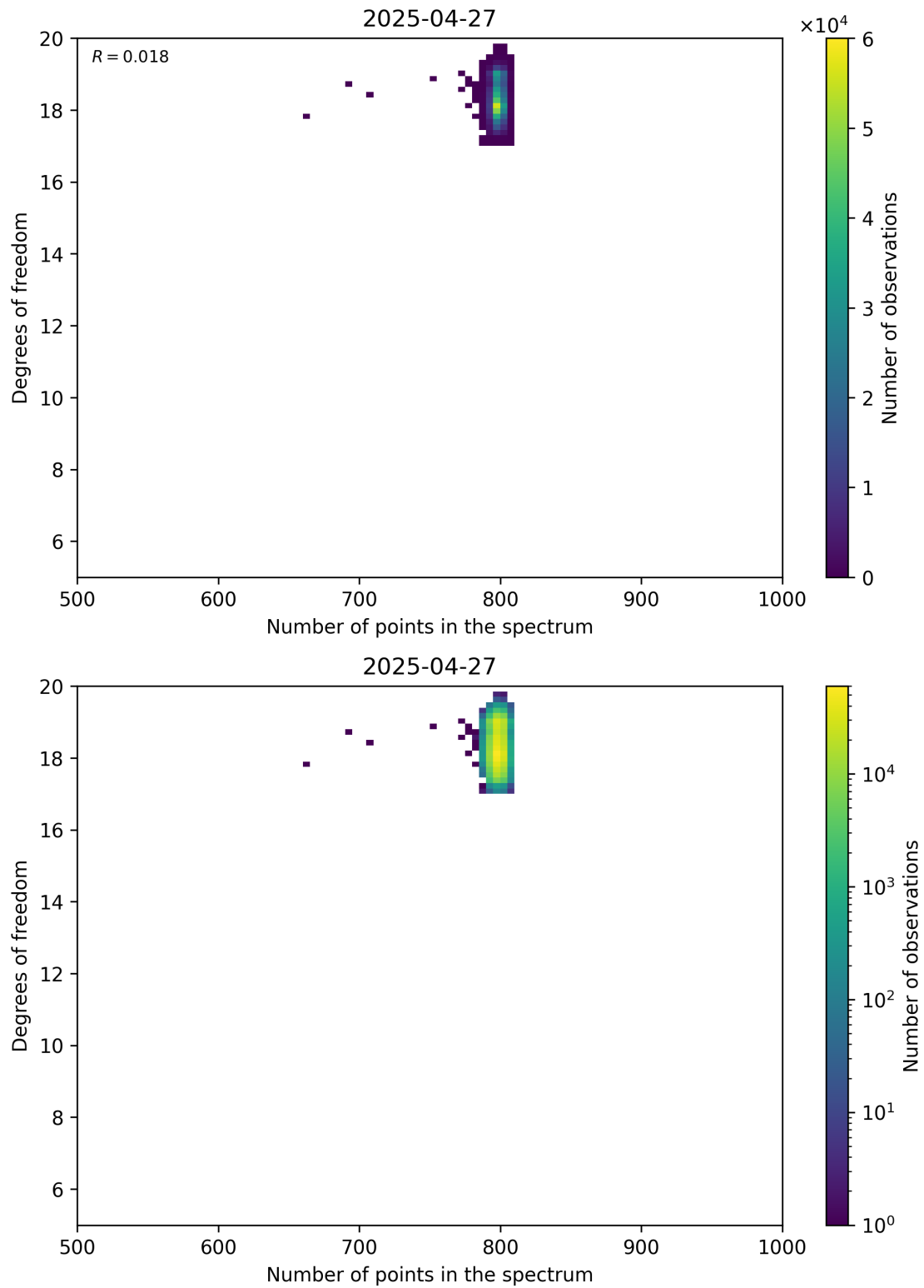
Figure 90: Scatter density plot of “Number of points in the spectrum” against “Degrees of freedom” for 2025-04-26 to 2025-04-28.
