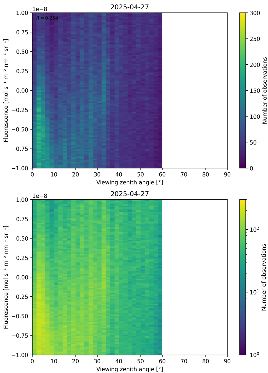
Figure 108: Scatter density plot of “Viewing zenith angle” against “Fluorescence” for 2025-04-26 to 2025-04-28.
