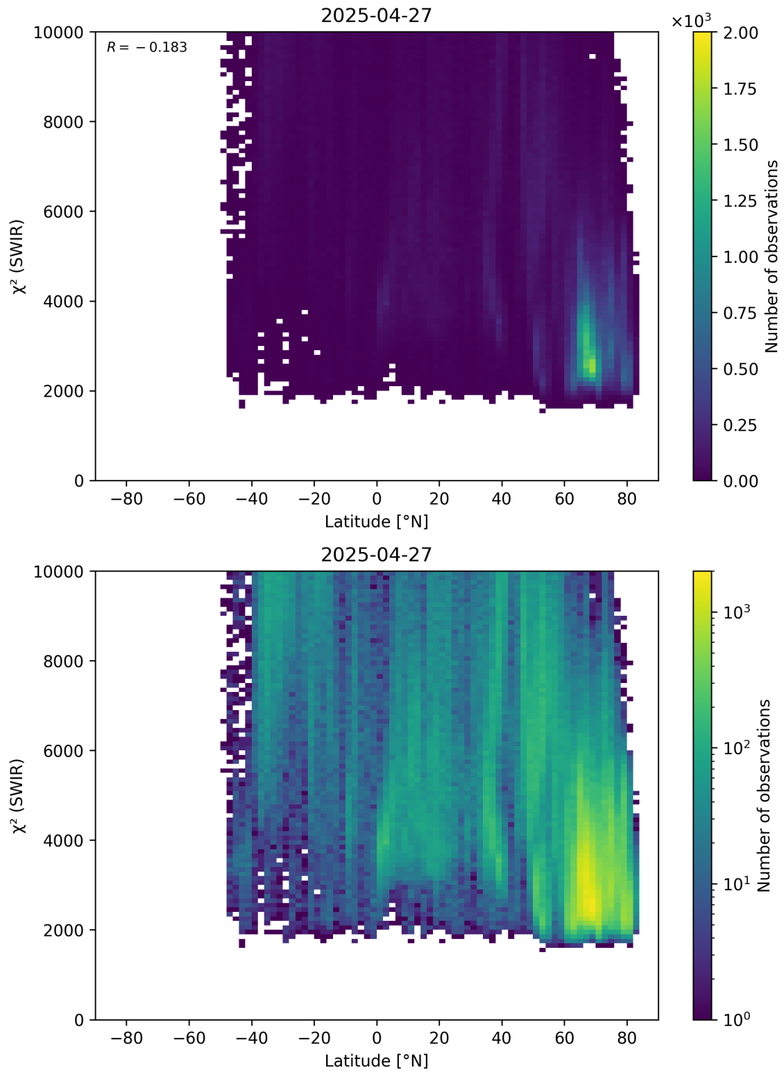
Figure 54: Scatter density plot of “Latitude” against “ \chi^2 (SWIR)” for 2025-04-26 to 2025-04-28.
