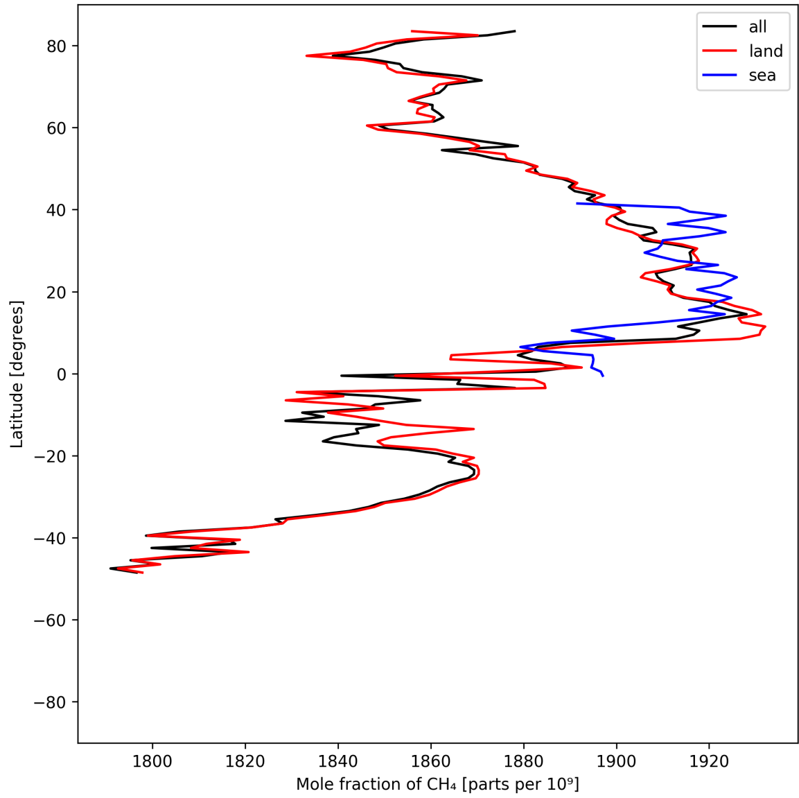
Figure 12: Zonal average of “Mole fraction of \text{CH}_4 ” for 2025-04-26 to 2025-04-28.
