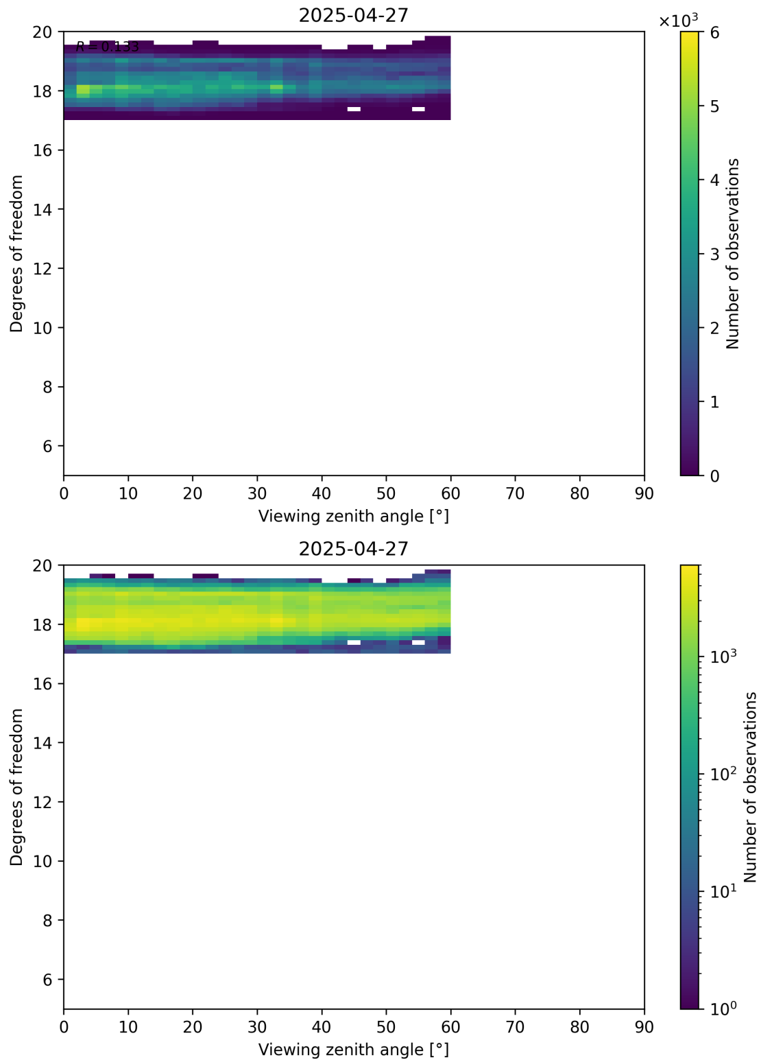
Figure 107: Scatter density plot of “Viewing zenith angle” against “Degrees of freedom” for 2025-04-26 to 2025-04-28.
