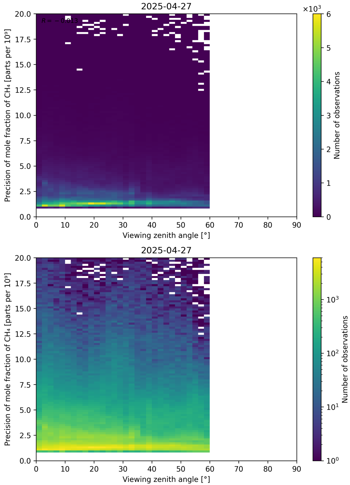
Figure 112: Scatter density plot of “Viewing zenith angle” against “Precision of mole fraction of CH 4 ” for 2025-04-26 to 2025-04-28.
