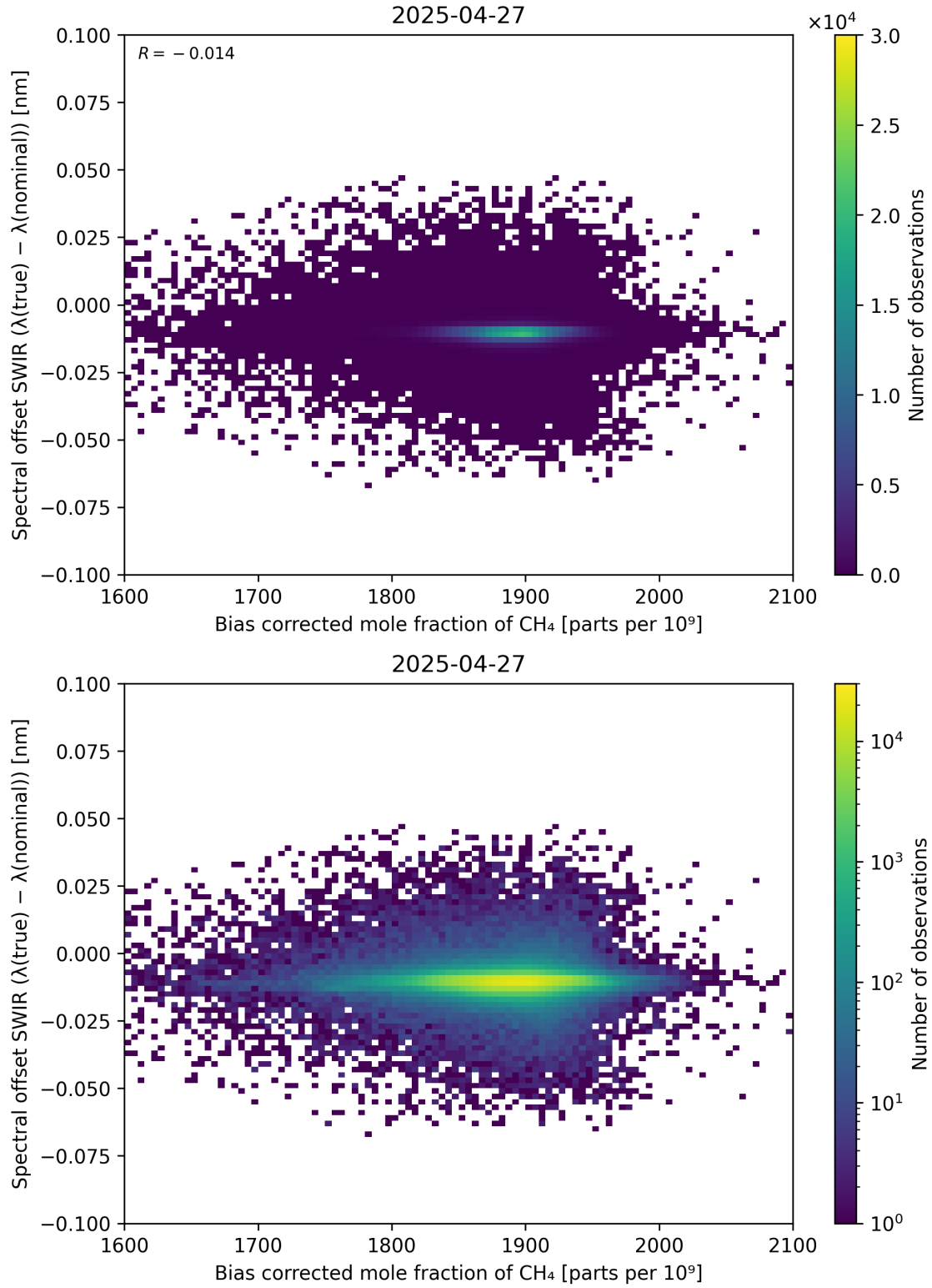
Figure 69: Scatter density plot of “Bias corrected mole fraction of CH 4 ” against “Spectral offset SWIR ( \lambda_{\text{true}} - \lambda_{\text{nominal}} )” for 2025-04-26 to 2025-04-28.
