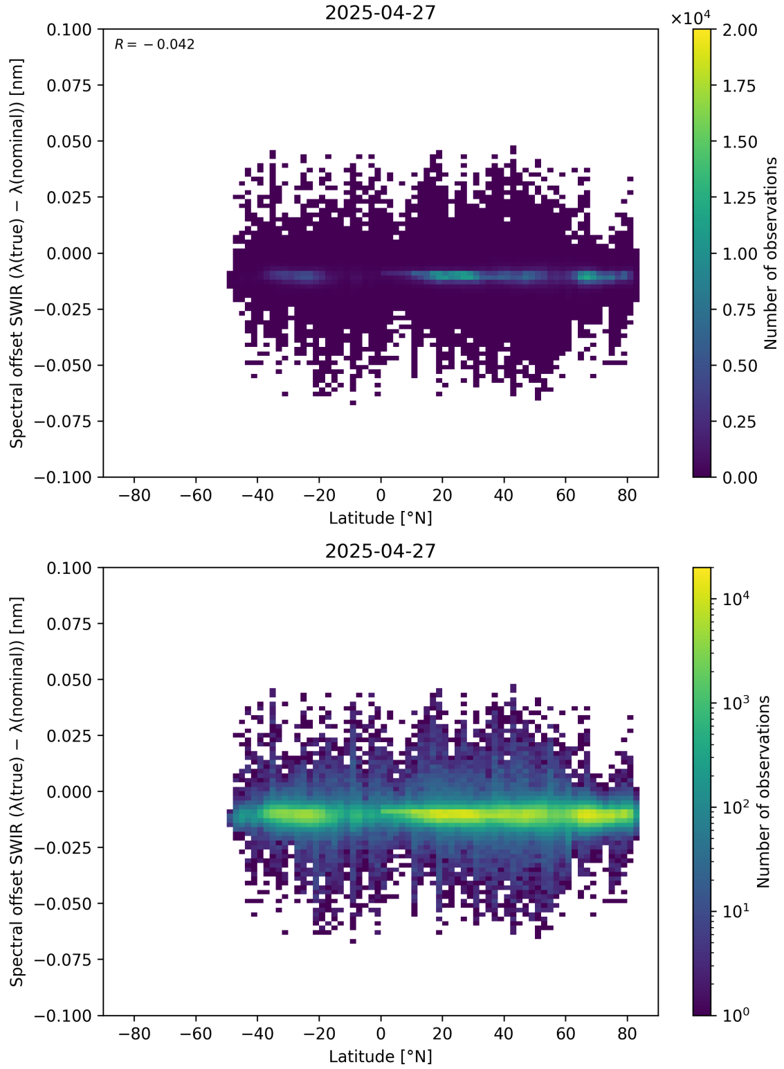
Figure 62: Scatter density plot of “Latitude” against “Spectral offset SWIR ( \lambda_{\text{true}} - \lambda_{\text{nominal}} )” for 2025-04-26 to 2025-04-28.
