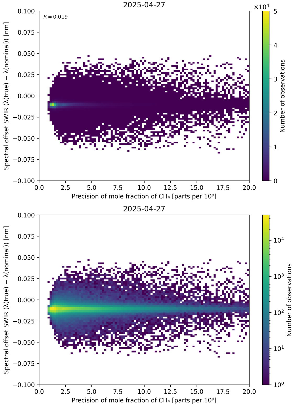
Figure 85: Scatter density plot of “Precision of mole fraction of CH 4 ” against “Spectral offset SWIR ( \lambda_{\text{true}} - \lambda_{\text{nominal}} )” for 2025-04-26 to 2025-04-28.
