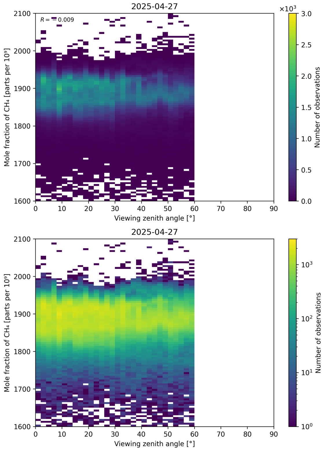
Figure 110: Scatter density plot of “Viewing zenith angle” against “Mole fraction of CH 4 ” for 2025-04-26 to 2025-04-28.
