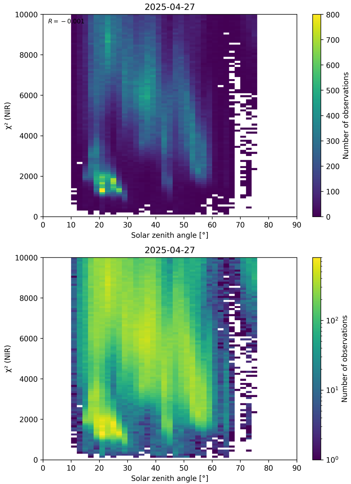
Figure 94: Scatter density plot of “Solar zenith angle” against “ \chi^2 (NIR)” for 2025-04-26 to 2025-04-28.
