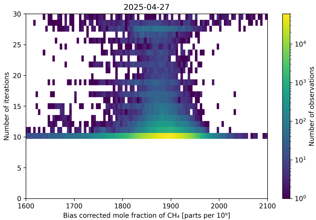
Figure 67: Scatter density plot of “Bias corrected mole fraction of CH 4 ” against “Number of iterations” for 2025-04-26 to 2025-04-28.
