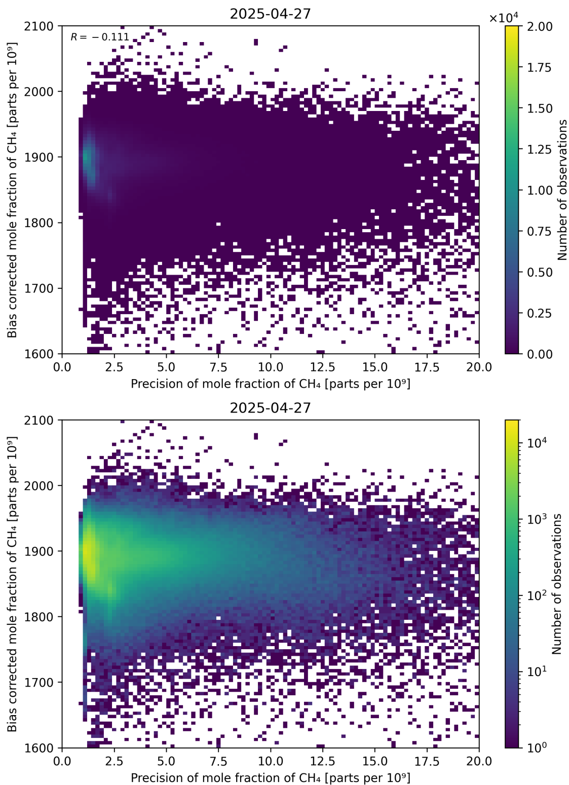
Figure 82: Scatter density plot of “Precision of mole fraction of CH 4 ” against “Bias corrected mole fraction of CH 4 ” for 2025-04-26 to 2025-04-28.
