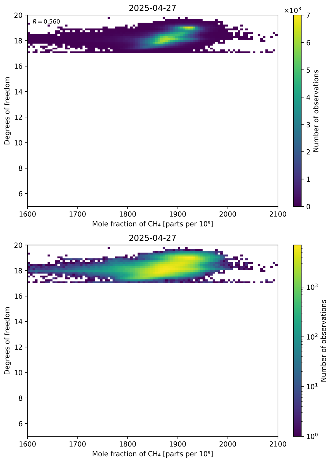
Figure 72: Scatter density plot of “Mole fraction of CH 4 ” against “Degrees of freedom” for 2025-04-26 to 2025-04-28.
