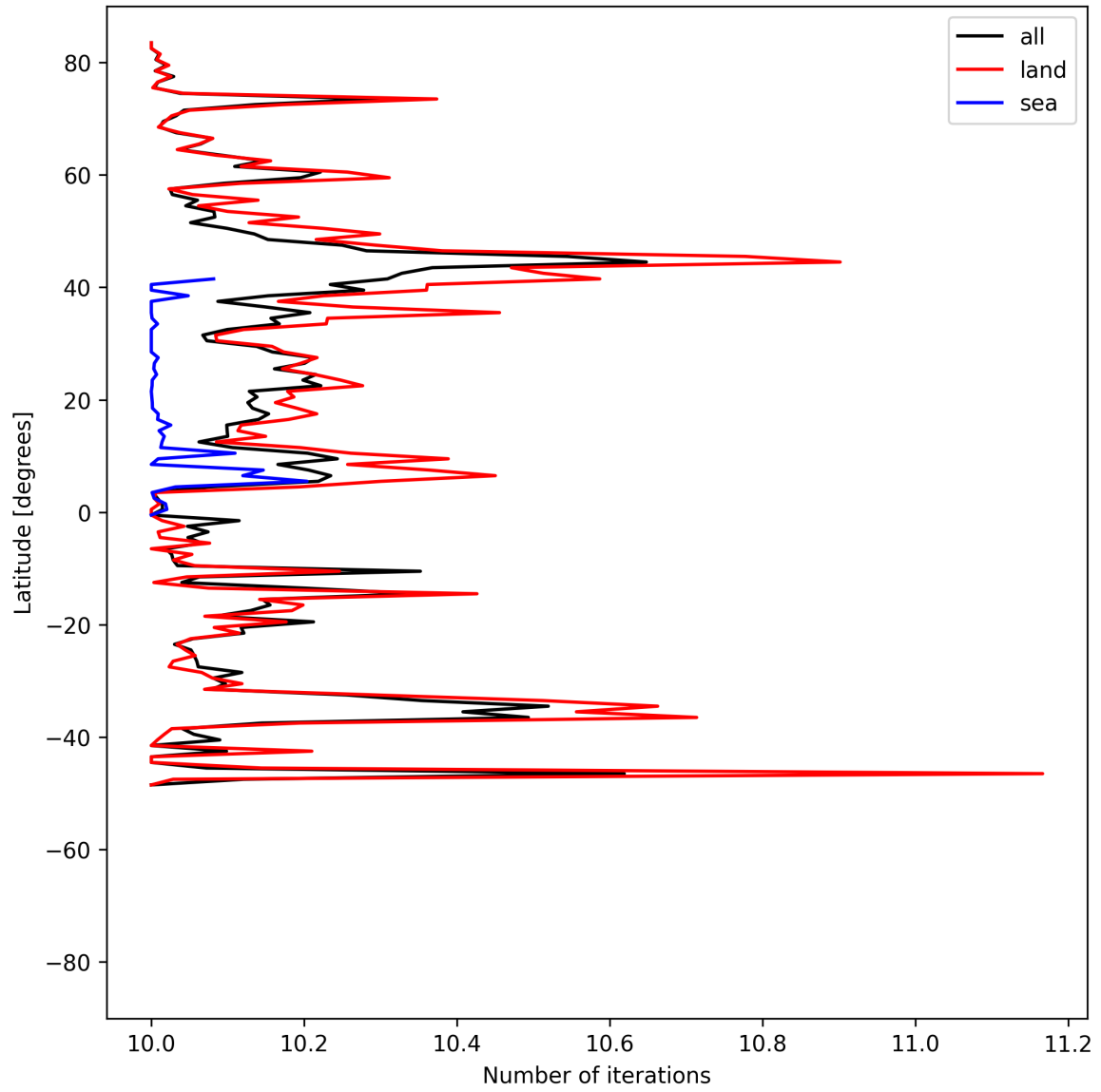
Figure 20: Zonal average of “Number of iterations” for 2025-04-26 to 2025-04-28.
