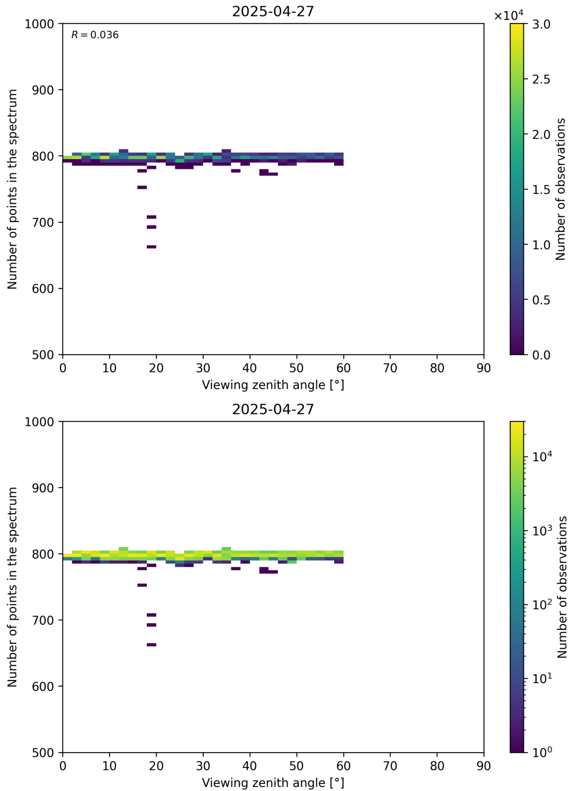
Figure 114: Scatter density plot of “Viewing zenith angle” against “Number of points in the spectrum” for 2025-04-26 to 2025-04-28.
