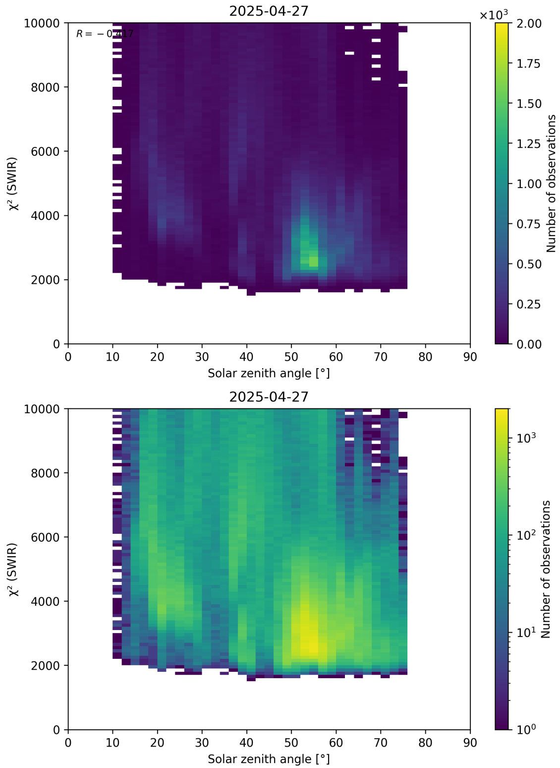
Figure 95: Scatter density plot of “Solar zenith angle” against “ \chi^2 (SWIR)” for 2025-04-26 to 2025-04-28.
