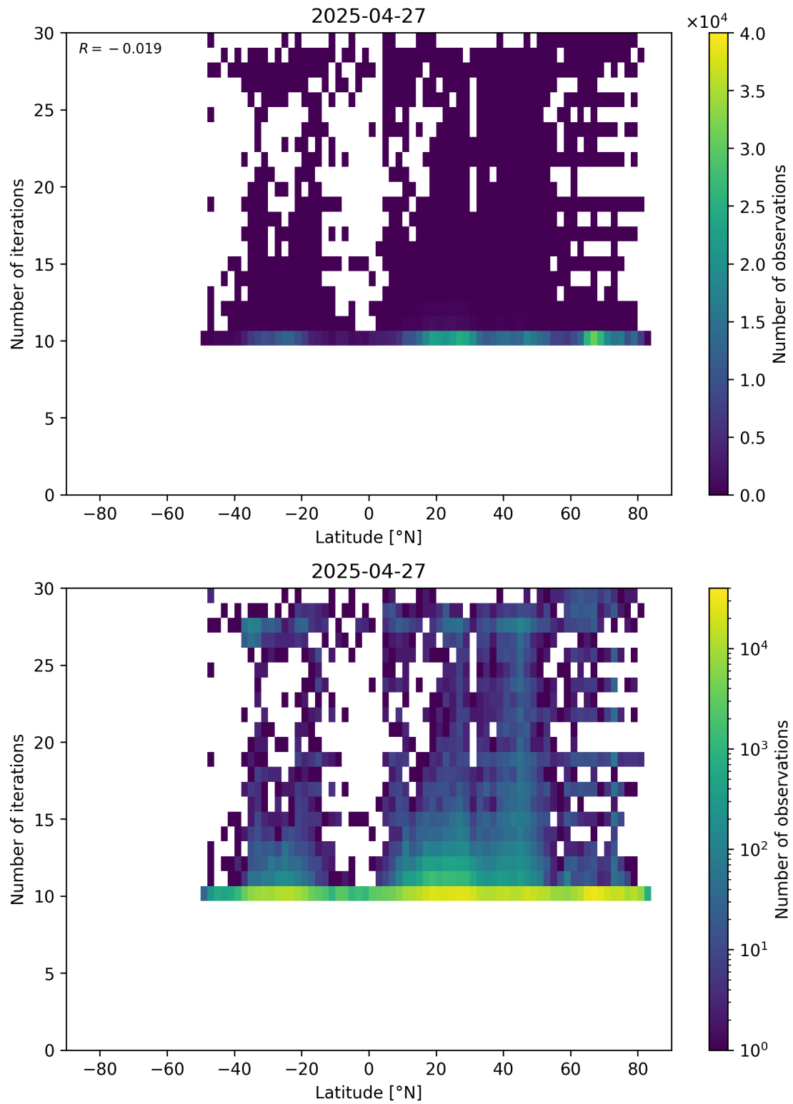
Figure 60: Scatter density plot of “Latitude” against “Number of iterations” for 2025-04-26 to 2025-04-28.
