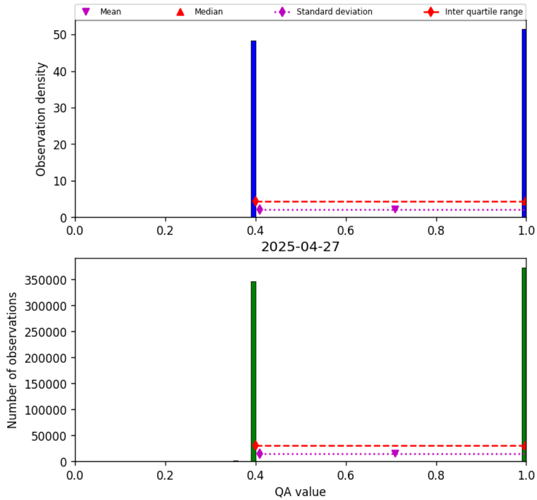
Figure 22: Histogram of “QA value” for 2025-04-26 to 2025-04-28
