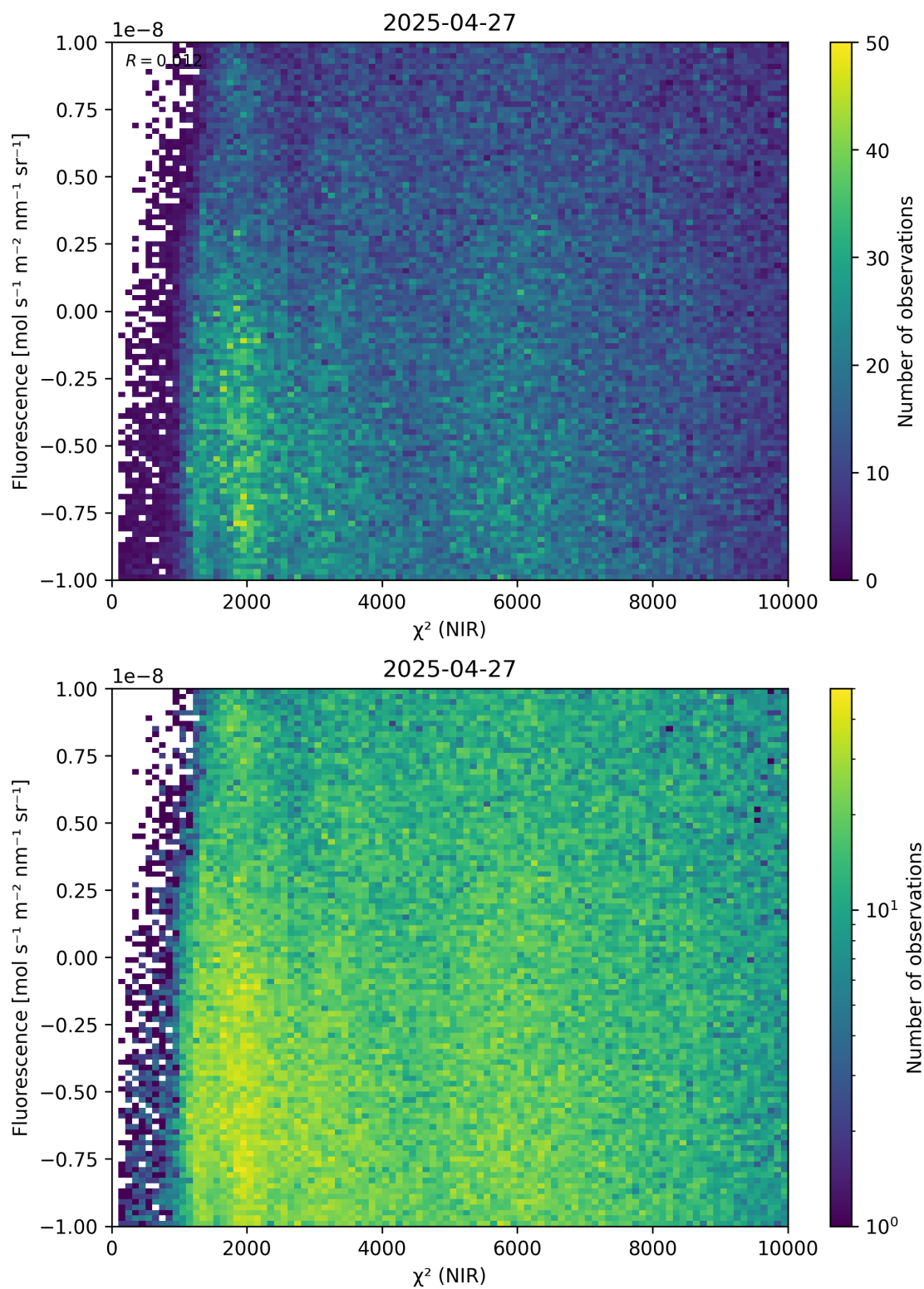
Figure 45: Scatter density plot of “ \chi^2 (NIR)” against “Fluorescence” for 2025-04-26 to 2025-04-28.
