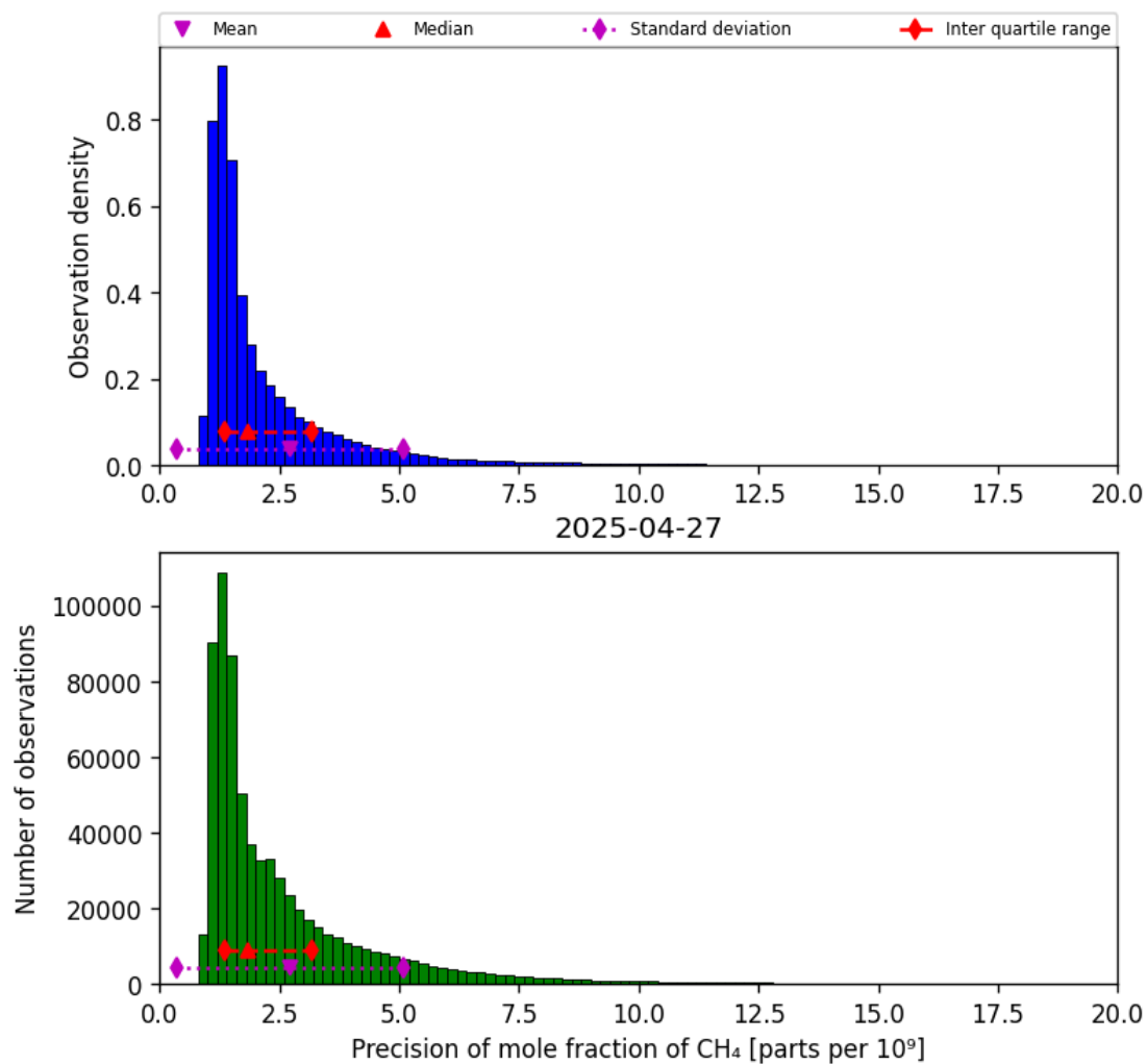
Figure 24: Histogram of “Precision of mole fraction of CH 4 ” for 2025-04-26 to 2025-04-28
