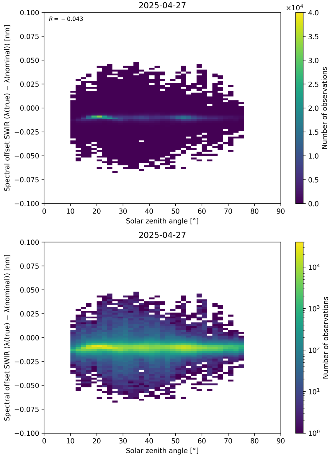
Figure 104: Scatter density plot of “Solar zenith angle” against “Spectral offset SWIR ( \lambda_{\text{true}} - \lambda_{\text{nominal}} )” for 2025-04-26 to 2025-04-28.
