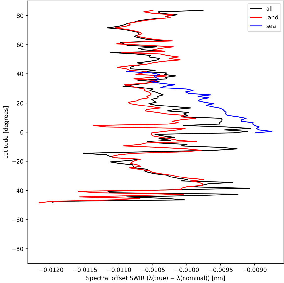
Figure 16: Zonal average of “Spectral offset SWIR ( \lambda_{\text{true}} - \lambda_{\text{nominal}} )” for 2025-04-26 to 2025-04-28.
