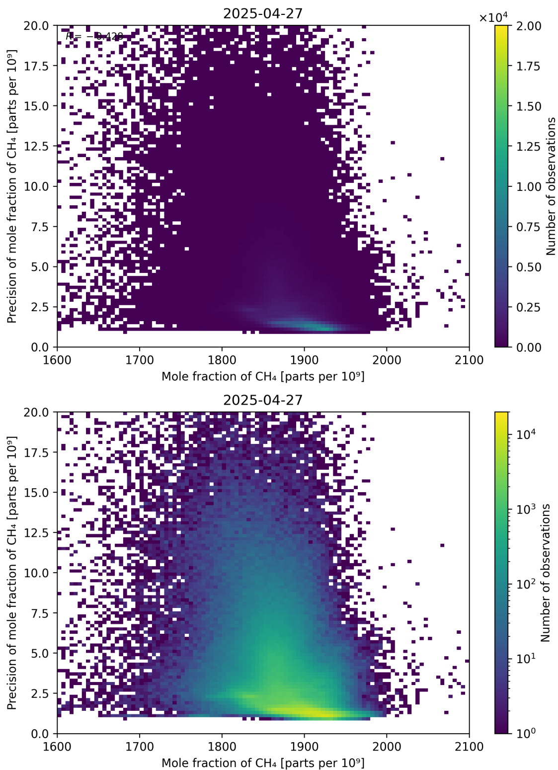
Figure 75: Scatter density plot of “Mole fraction of CH 4 ” against “Precision of mole fraction of CH 4 ” for 2025-04-26 to 2025-04-28.
