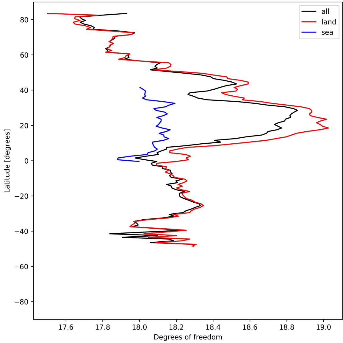
Figure 19: Zonal average of “Degrees of freedom” for 2025-04-26 to 2025-04-28.
