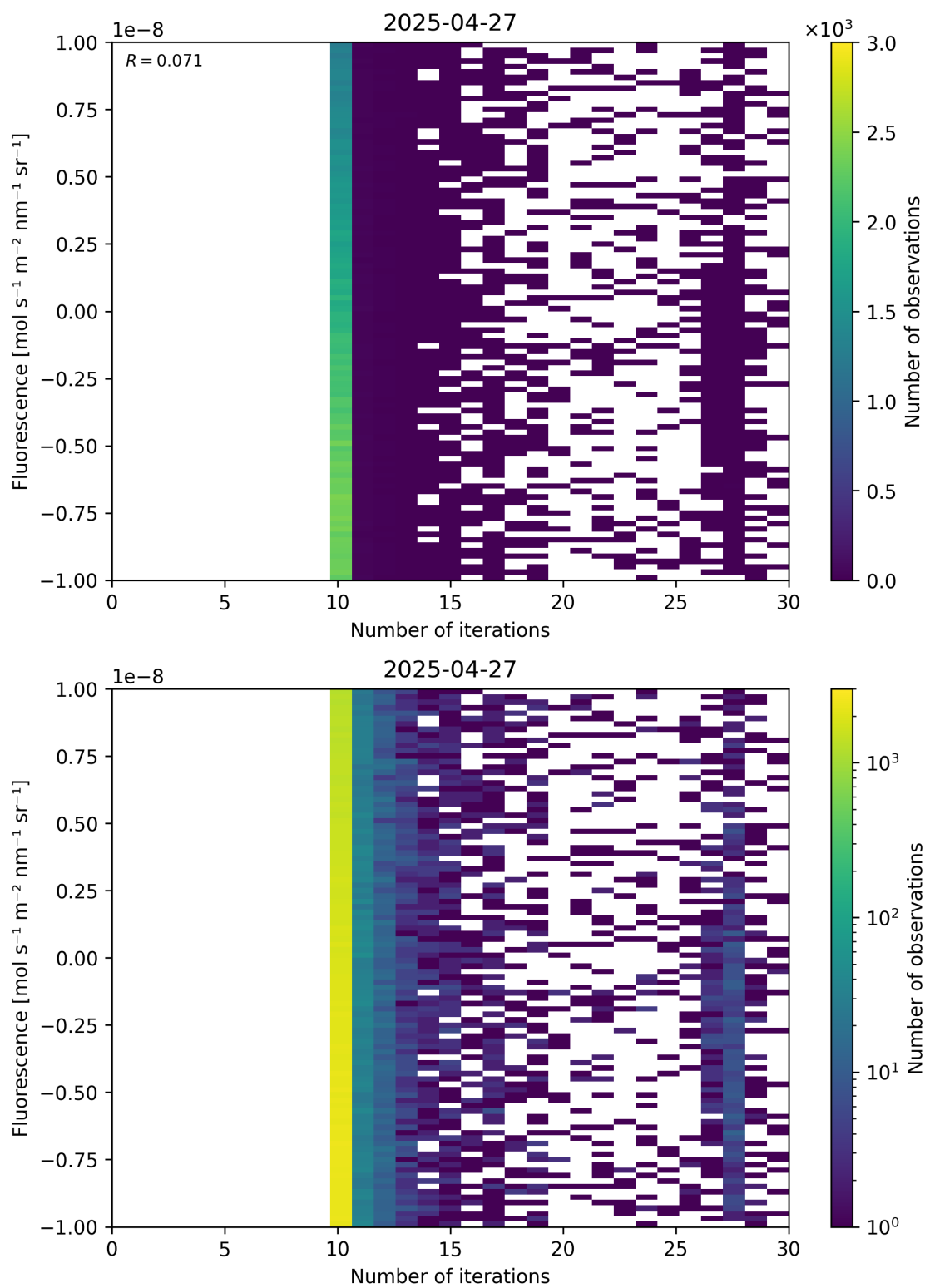
Figure 87: Scatter density plot of “Number of iterations” against “Fluorescence” for 2025-04-26 to 2025-04-28.
