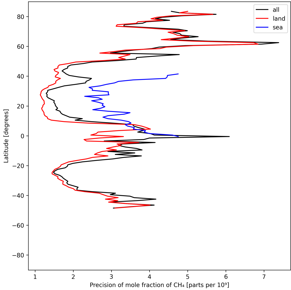
Figure 13: Zonal average of “Precision of mole fraction of CH 4 ” for 2025-04-26 to 2025-04-28.
