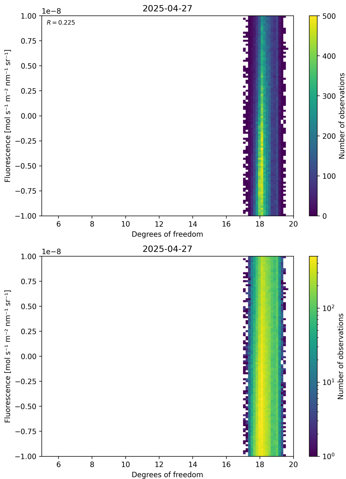
Figure 51: Scatter density plot of “Degrees of freedom” against “Fluorescence” for 2025-04-26 to 2025-04-28.
