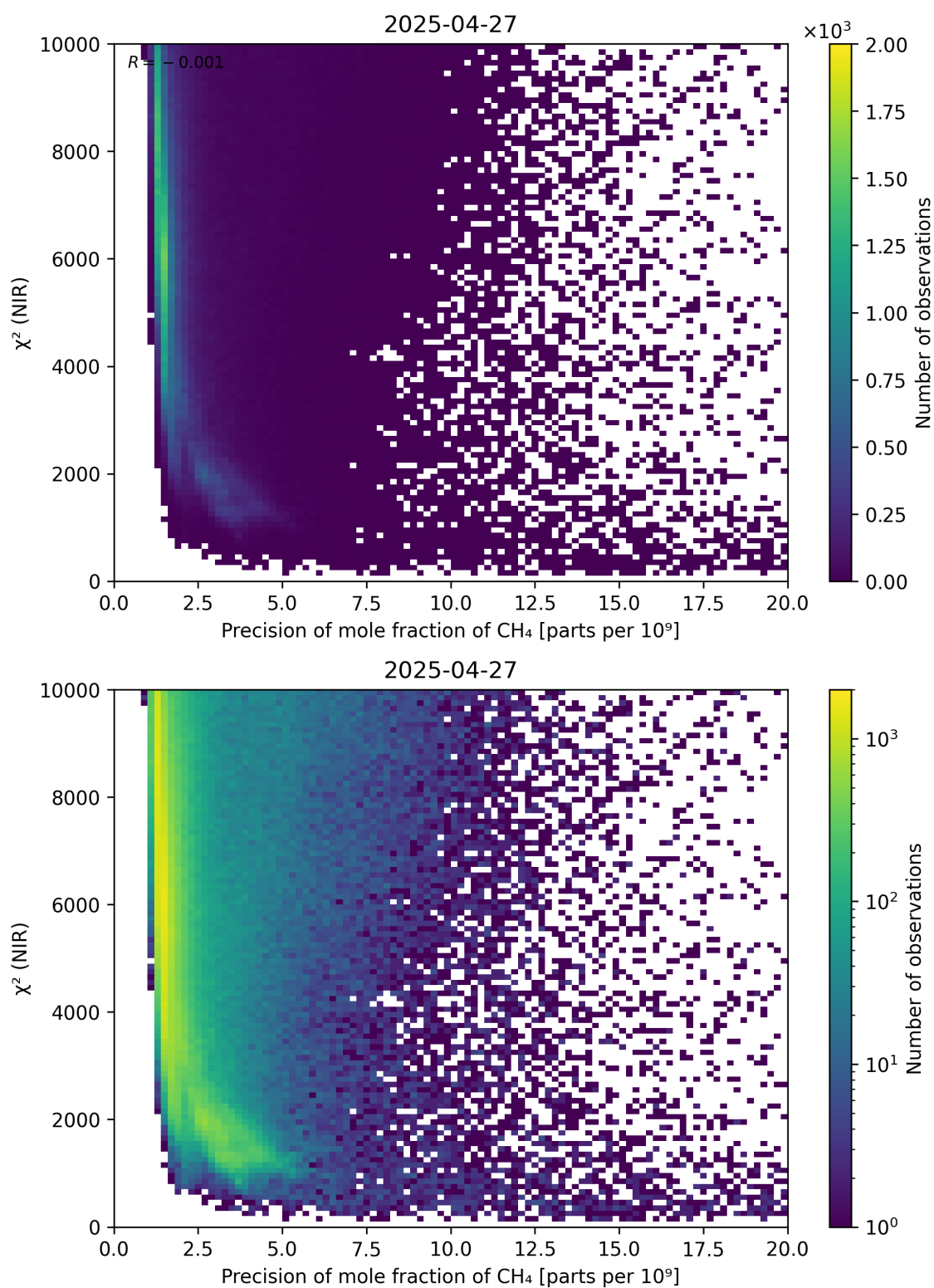
Figure 78: Scatter density plot of “Precision of mole fraction of CH 4 ” against “ \chi^2 (NIR)” for 2025-04-26 to 2025-04-28.
