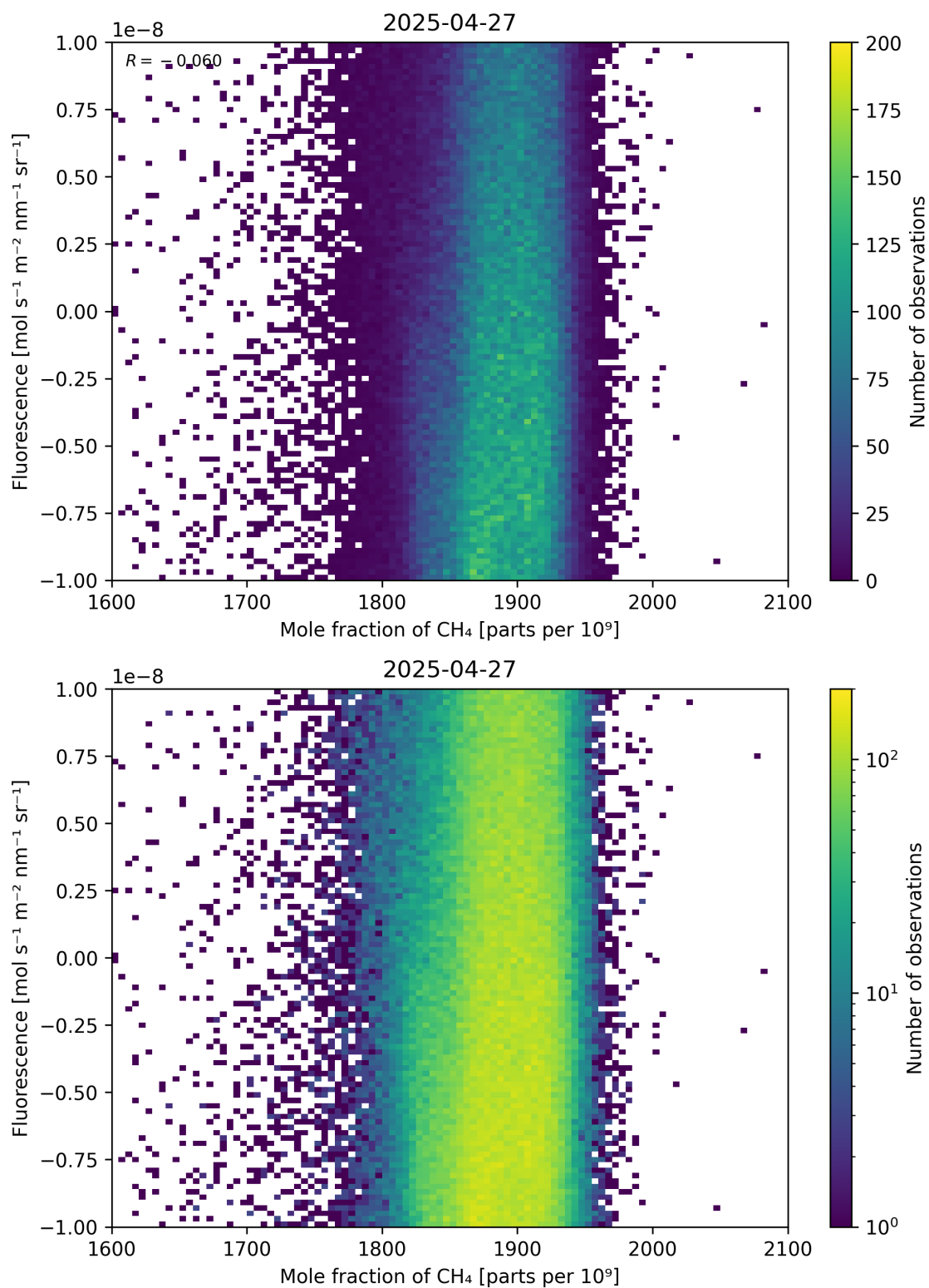
Figure 73: Scatter density plot of “Mole fraction of \text{CH}_4 ” against “Fluorescence” for 2025-04-26 to 2025-04-28.
