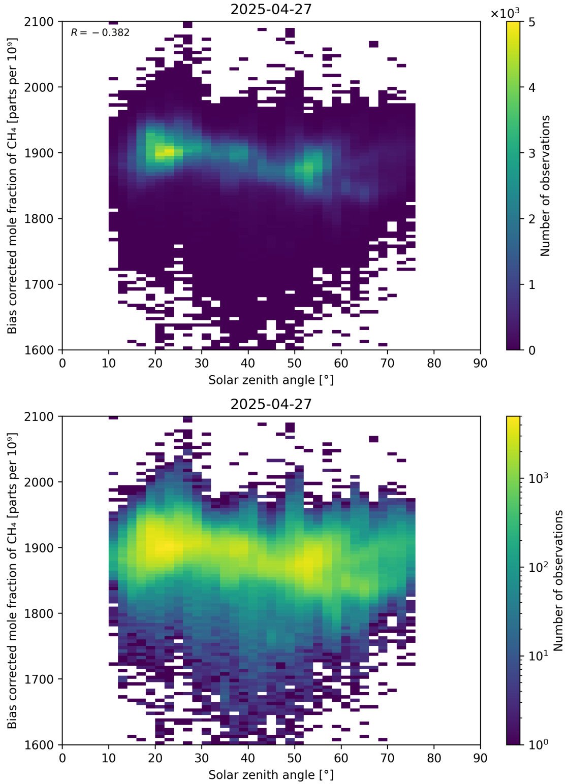
Figure 100: Scatter density plot of “Solar zenith angle” against “Bias corrected mole fraction of CH 4 ” for 2025-04-26 to 2025-04-28.
