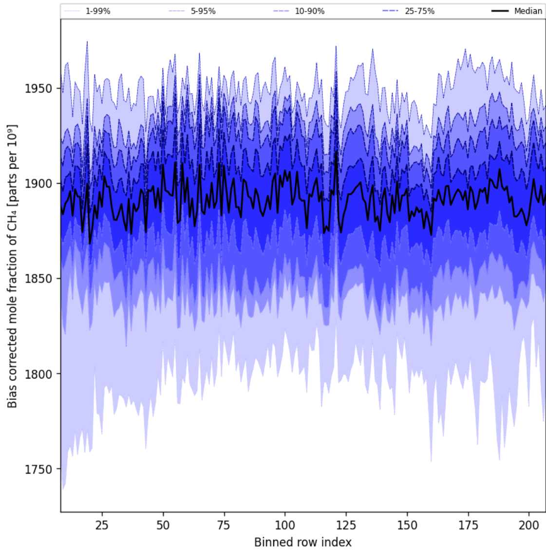
Figure 36: Along track statistics of “Bias corrected mole fraction of CH 4 ” for 2025-04-26 to 2025-04-28
