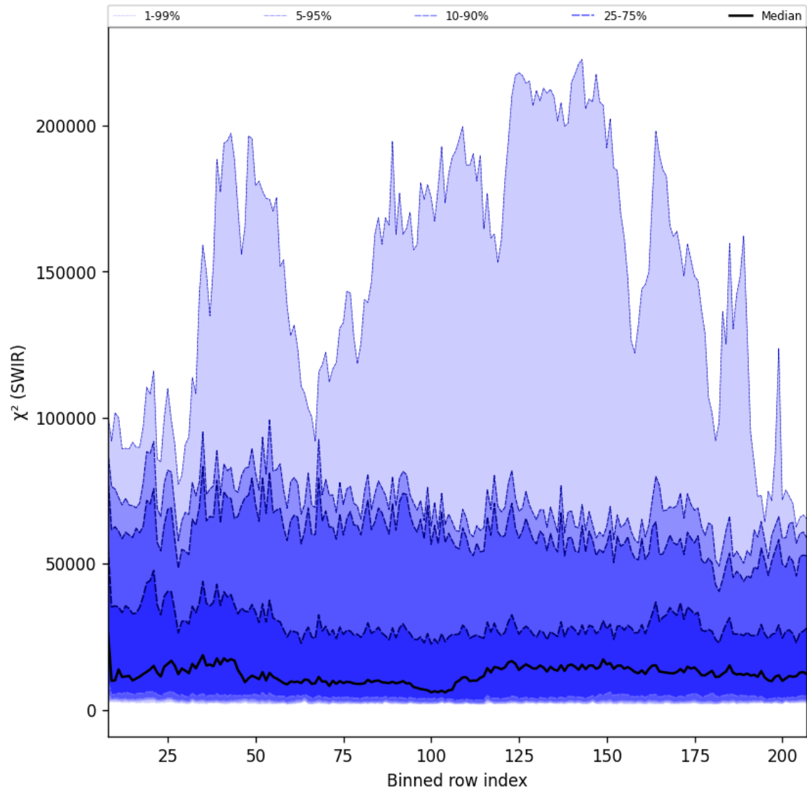
Figure 39: Along track statistics of “ \chi^2 (SWIR)” for 2025-04-26 to 2025-04-28
