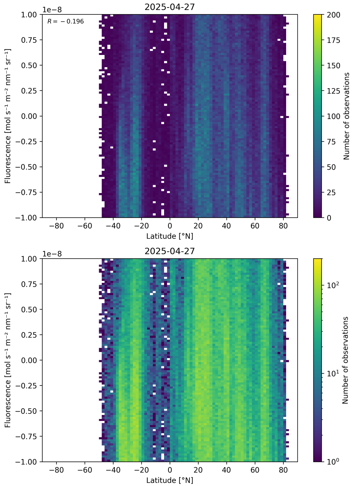
Figure 56: Scatter density plot of “Latitude” against “Fluorescence” for 2025-04-26 to 2025-04-28.
