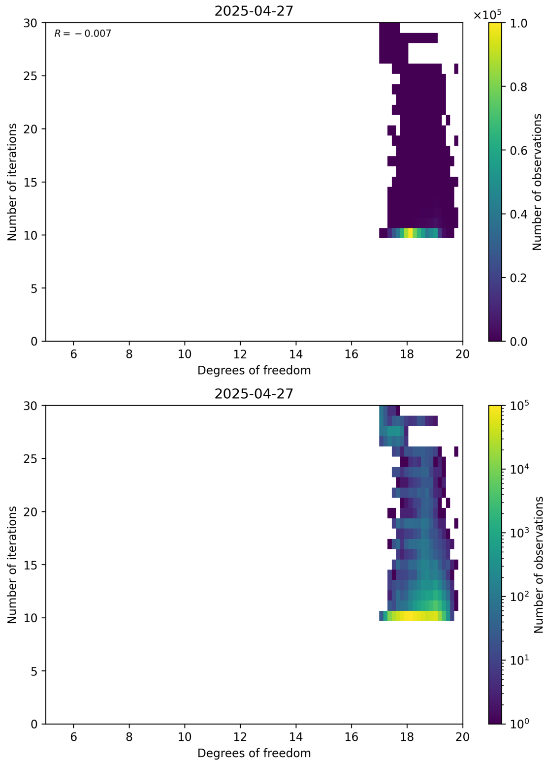
Figure 52: Scatter density plot of “Degrees of freedom” against “Number of iterations” for 2025-04-26 to 2025-04-28.
