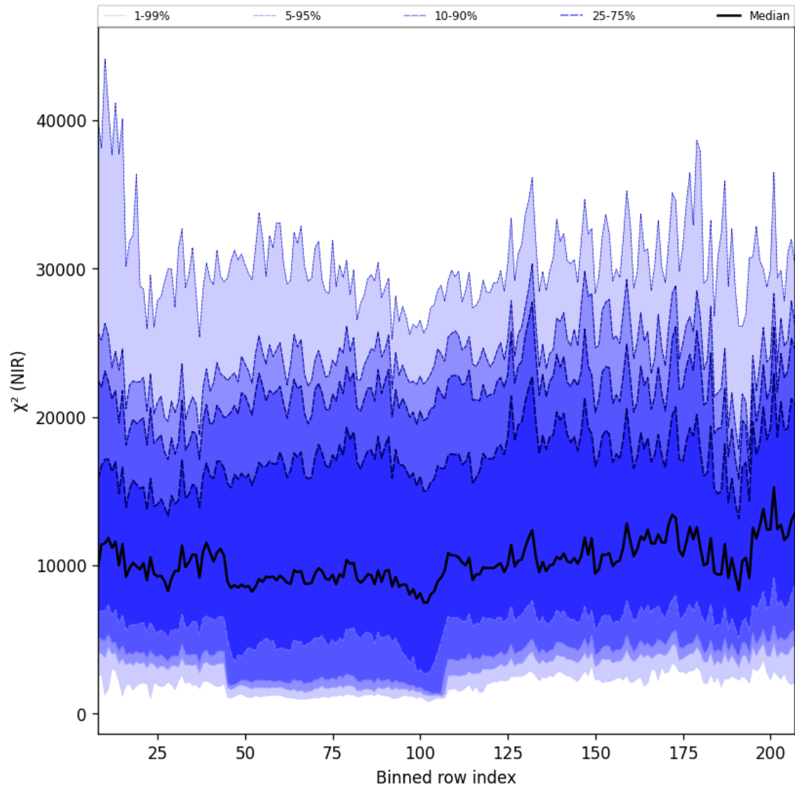
Figure 40: Along track statistics of “ \chi^2 (NIR)” for 2025-04-26 to 2025-04-28
