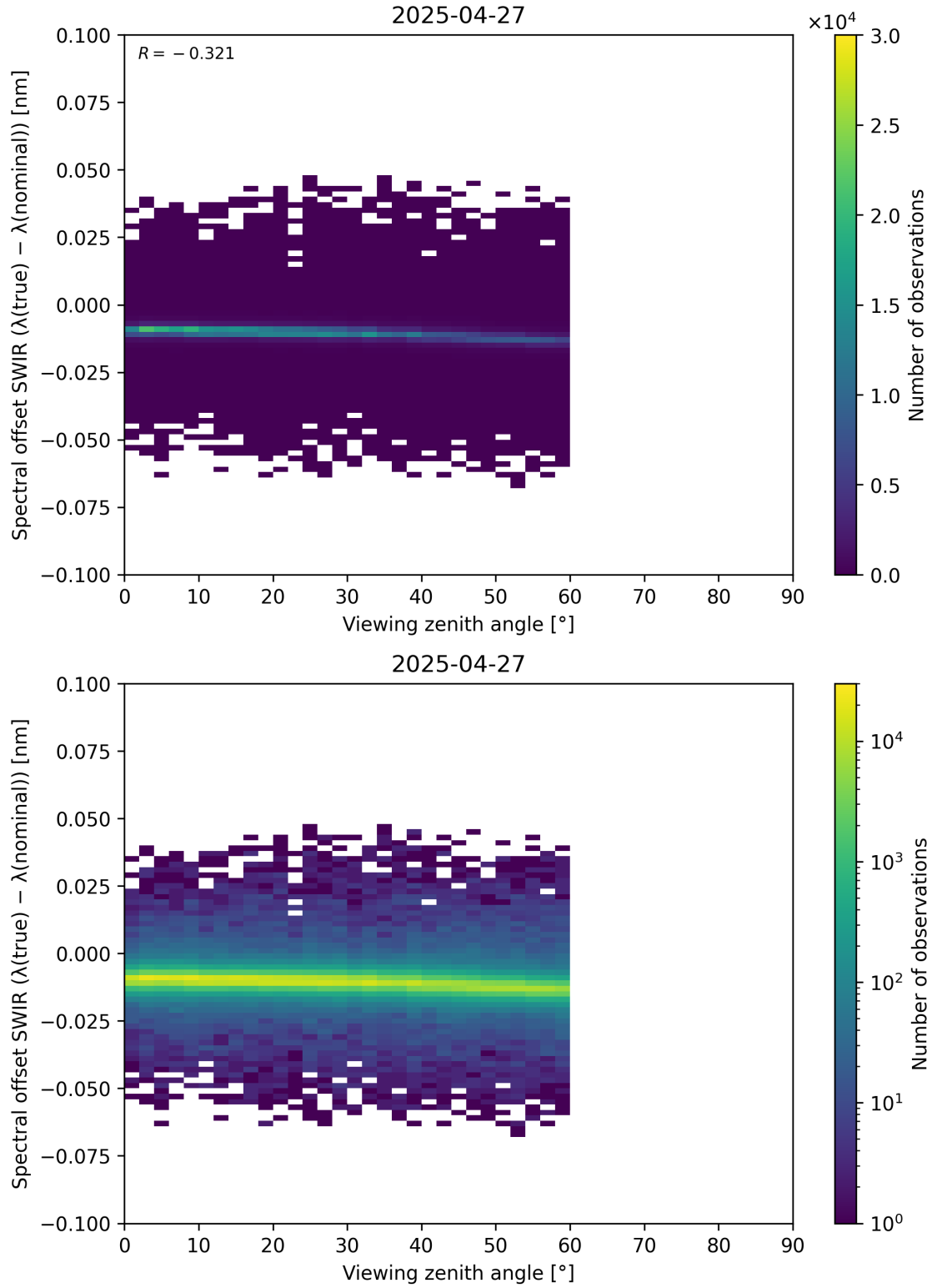
Figure 116: Scatter density plot of “Viewing zenith angle” against “Spectral offset SWIR ( \lambda_{\text{true}} - \lambda_{\text{nominal}} )” for 2025-04-26 to 2025-04-28.
