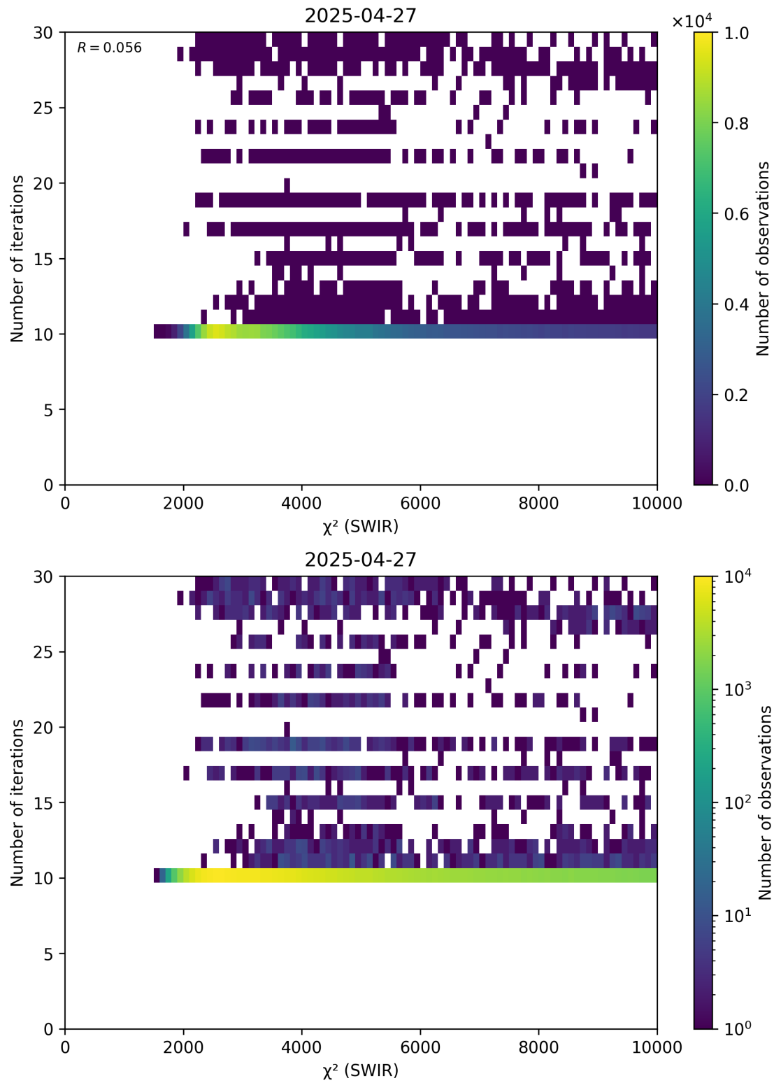
Figure 50: Scatter density plot of “ \chi^2 (SWIR)” against “Number of iterations” for 2025-04-26 to 2025-04-28.
