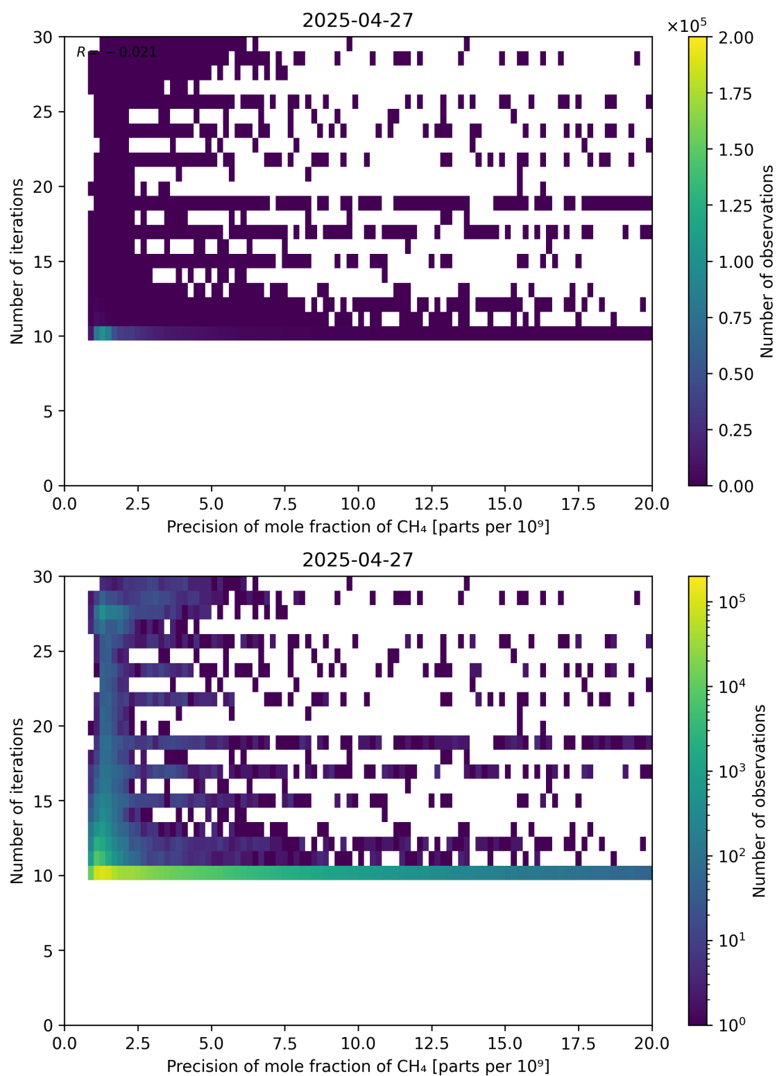
Figure 83: Scatter density plot of “Precision of mole fraction of \text{CH}_4 ” against “Number of iterations” for 2025-04-26 to 2025-04-28.
