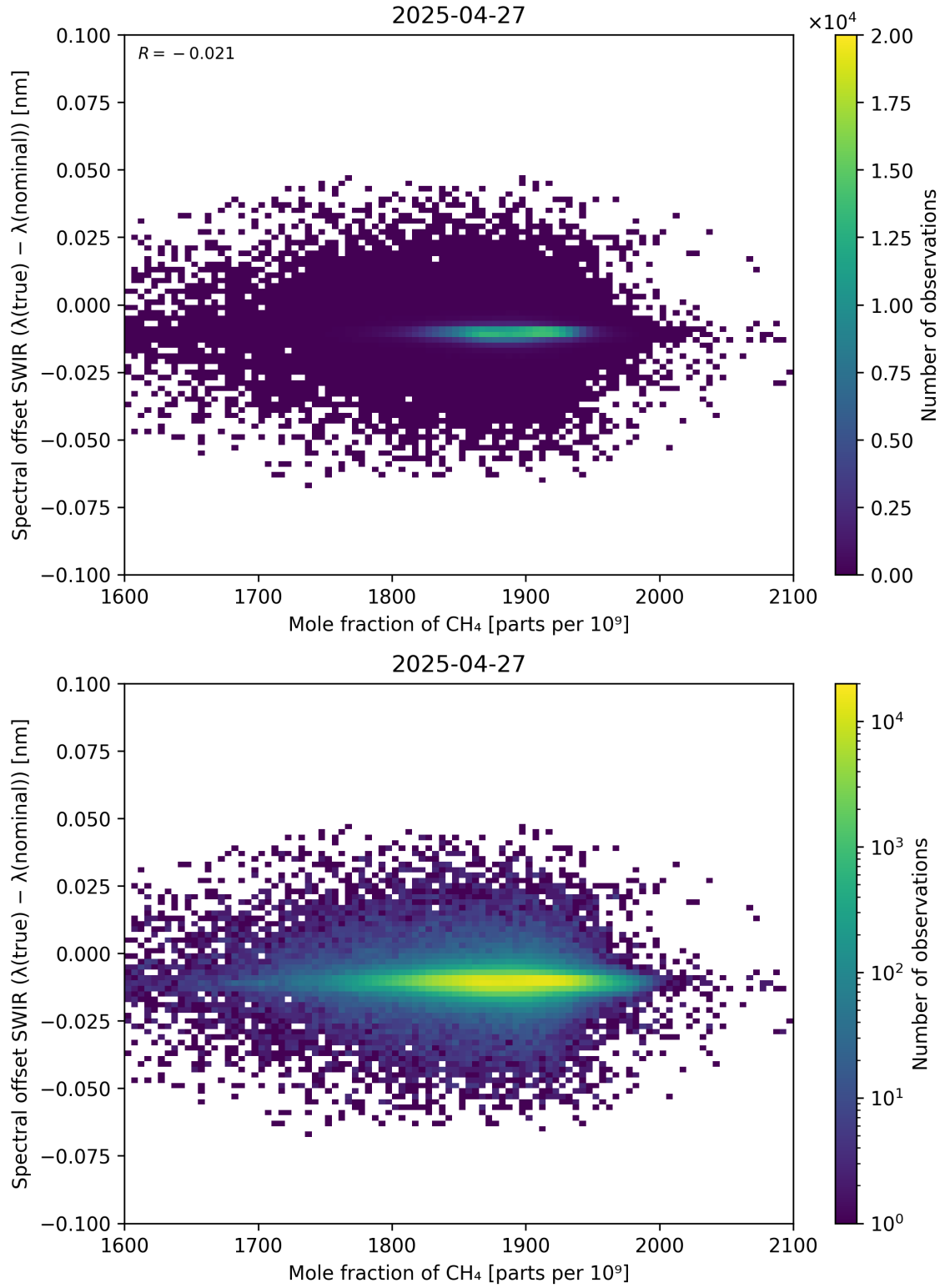
Figure 86: Scatter density plot of “Mole fraction of CH 4 ” against “Spectral offset SWIR ( \lambda_{\text{true}} - \lambda_{\text{nominal}} )” for 2025-04-26 to 2025-04-28.
