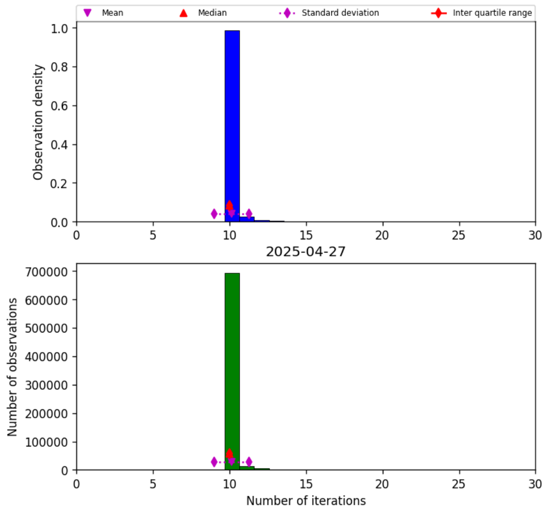
Figure 31: Histogram of “Number of iterations” for 2025-04-26 to 2025-04-28
