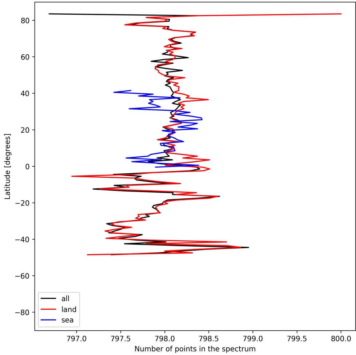
Figure 15: Zonal average of “Number of points in the spectrum” for 2025-04-26 to 2025-04-28.
