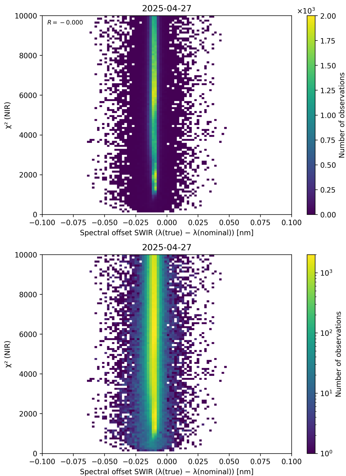
Figure 117: Scatter density plot of “Spectral offset SWIR ( \lambda_{\text{true}} - \lambda_{\text{nominal}} )” against “ \chi^2 (NIR)” for 2025-04-26 to 2025-04-28.
