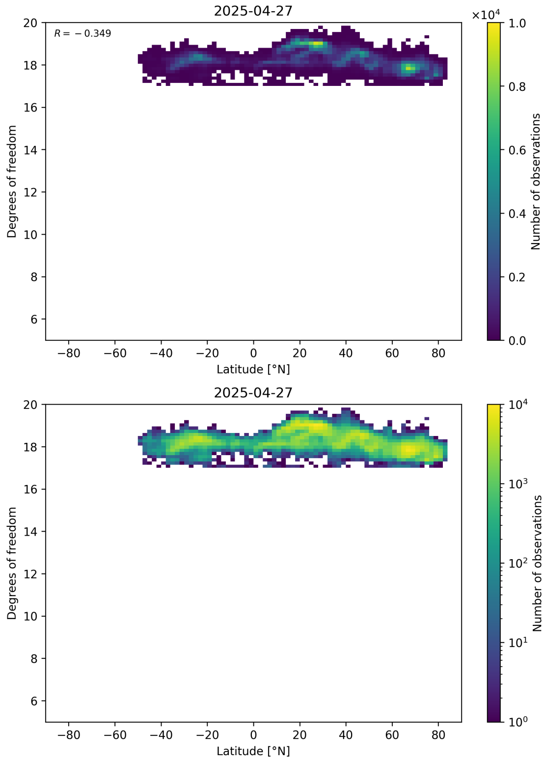
Figure 55: Scatter density plot of “Latitude” against “Degrees of freedom” for 2025-04-26 to 2025-04-28.
