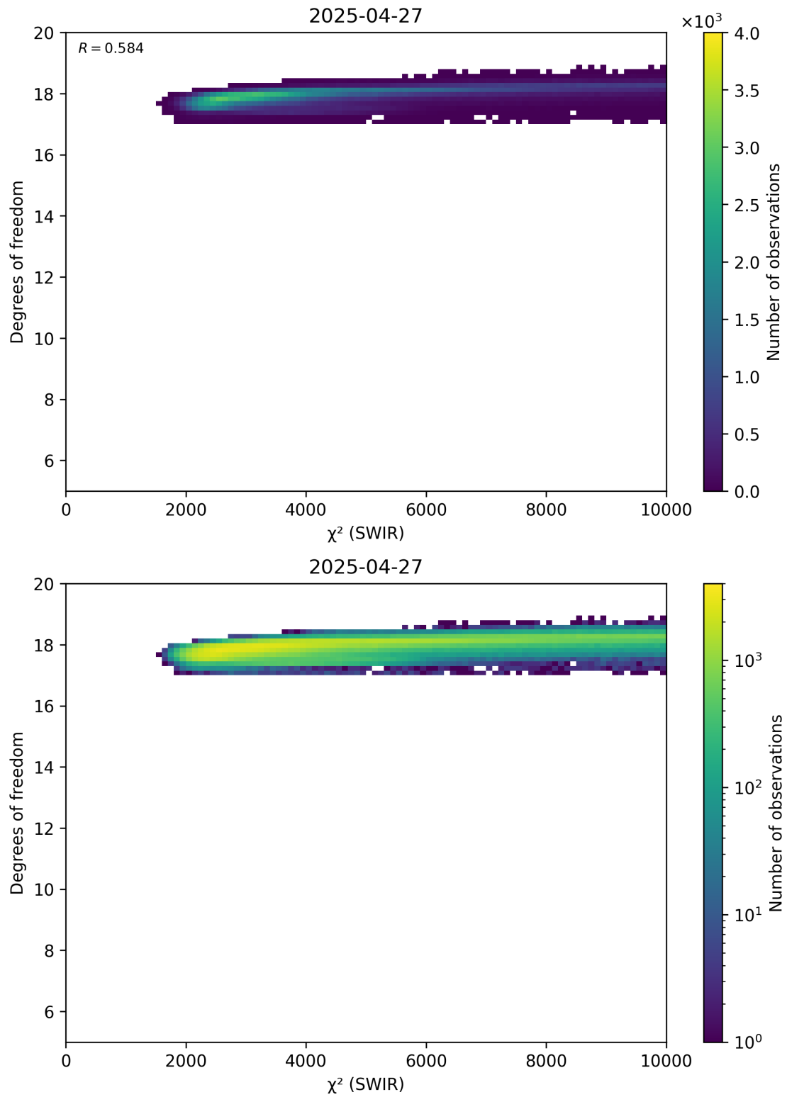
Figure 48: Scatter density plot of “ \chi^2 (SWIR)” against “Degrees of freedom” for 2025-04-26 to 2025-04-28.
