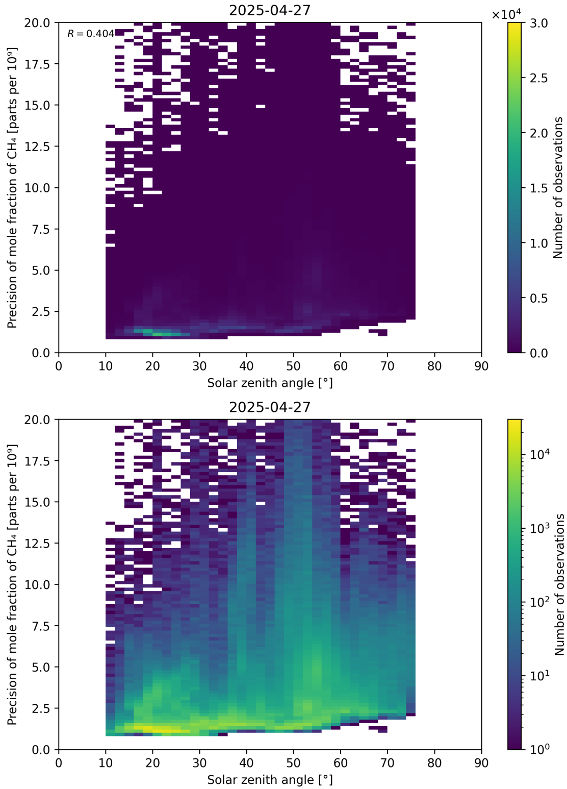
Figure 101: Scatter density plot of “Solar zenith angle” against “Precision of mole fraction of \text{CH}_4 ” for 2025-04-26 to 2025-04-28.
