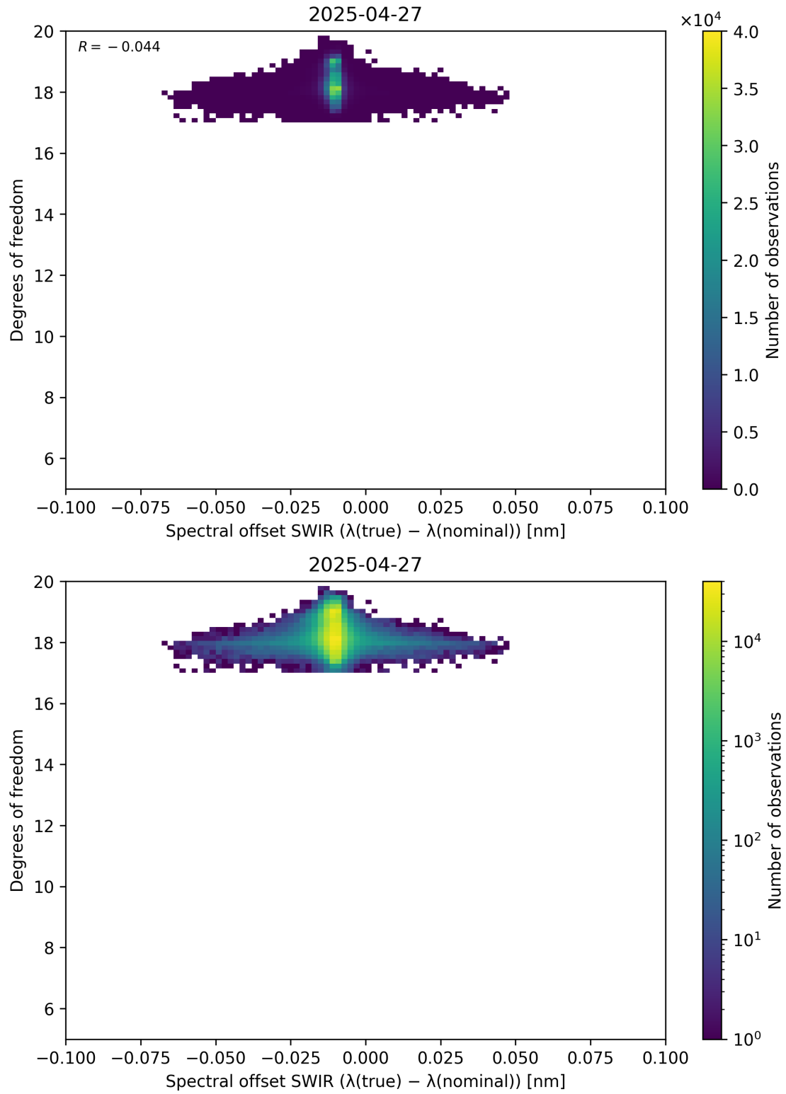
Figure 119: Scatter density plot of “Spectral offset SWIR ( \lambda_{\text{true}} - \lambda_{\text{nominal}} )” against “Degrees of freedom” for 2025-04-26 to 2025-04-28.
