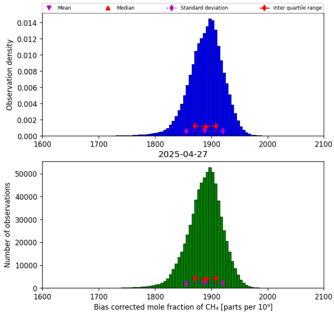
Figure 25: Histogram of “Bias corrected mole fraction of CH 4 ” for 2025-04-26 to 2025-04-28
