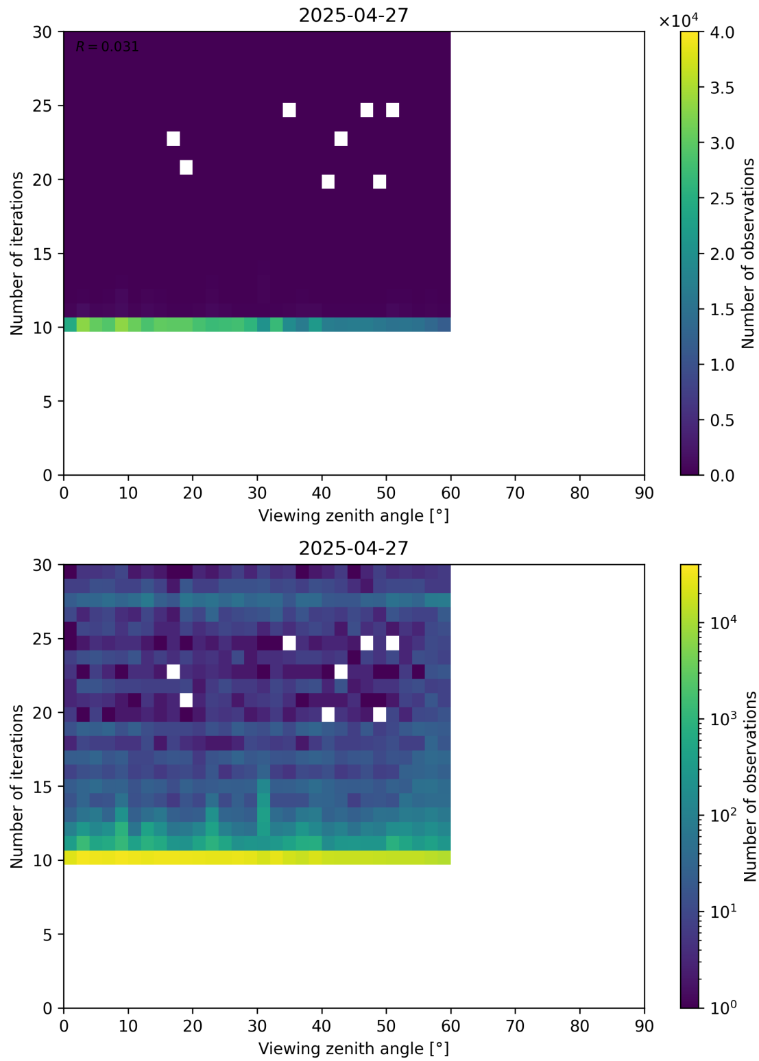
Figure 113: Scatter density plot of “Viewing zenith angle” against “Number of iterations” for 2025-04-26 to 2025-04-28.
