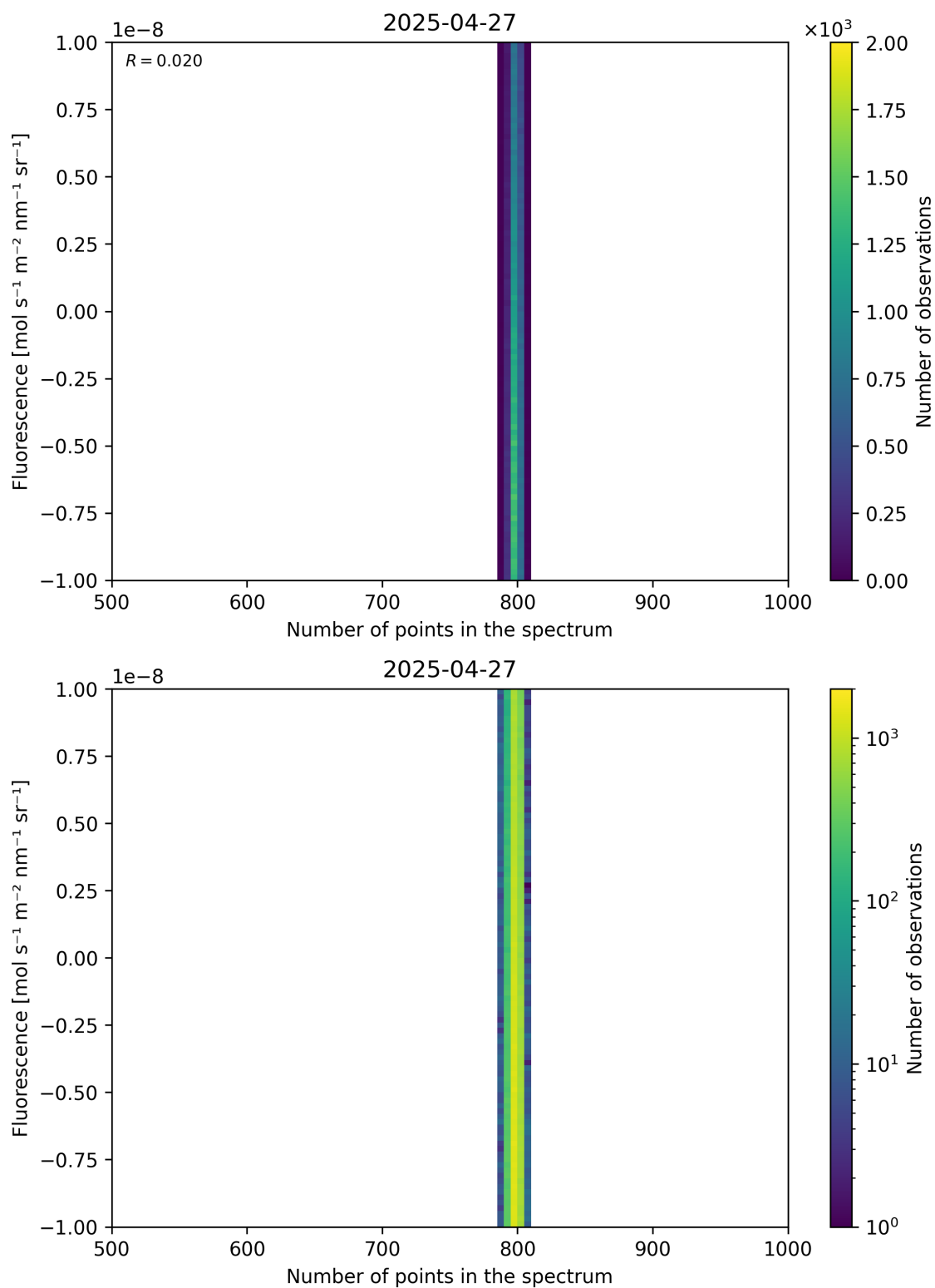
Figure 91: Scatter density plot of “Number of points in the spectrum” against “Fluorescence” for 2025-04-26 to 2025-04-28.
