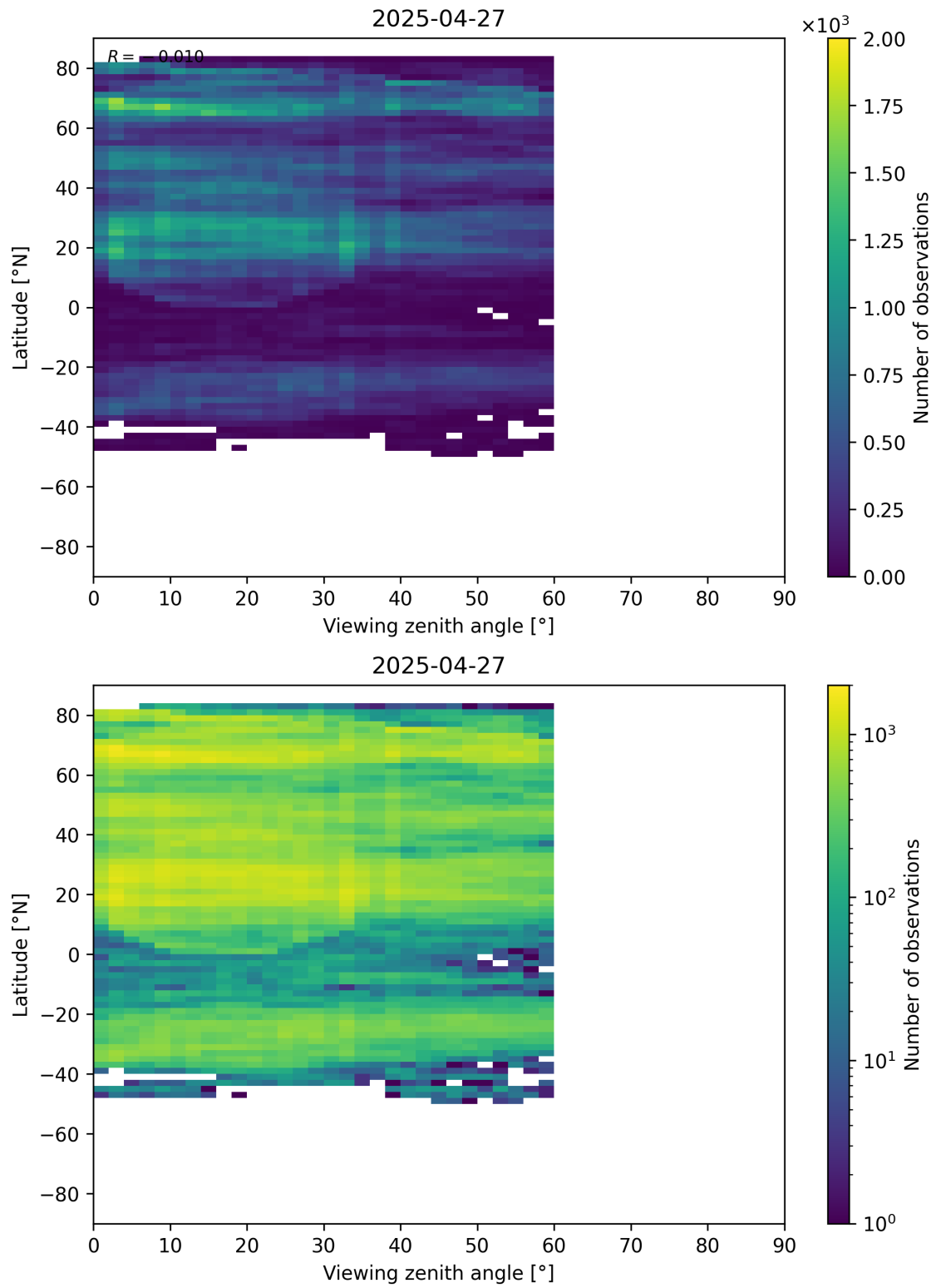
Figure 109: Scatter density plot of “Viewing zenith angle” against “Latitude” for 2025-04-26 to 2025-04-28.
