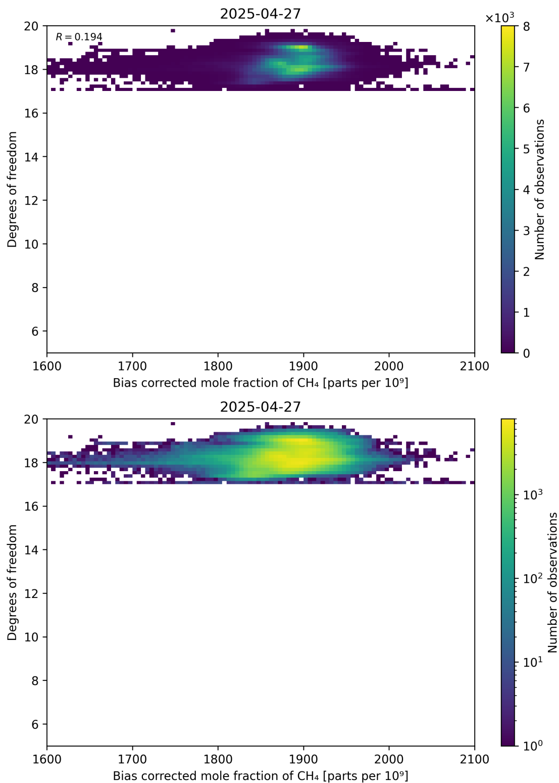
Figure 65: Scatter density plot of “Bias corrected mole fraction of CH 4 ” against “Degrees of freedom” for 2025-04-26 to 2025-04-28.
