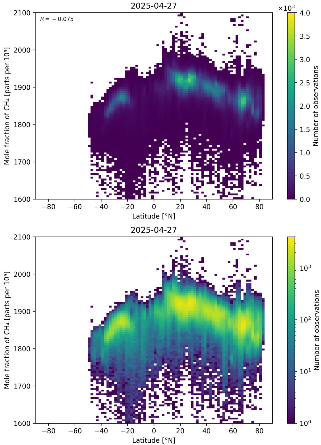
Figure 57: Scatter density plot of “Latitude” against “Mole fraction of CH 4 ” for 2025-04-26 to 2025-04-28.
