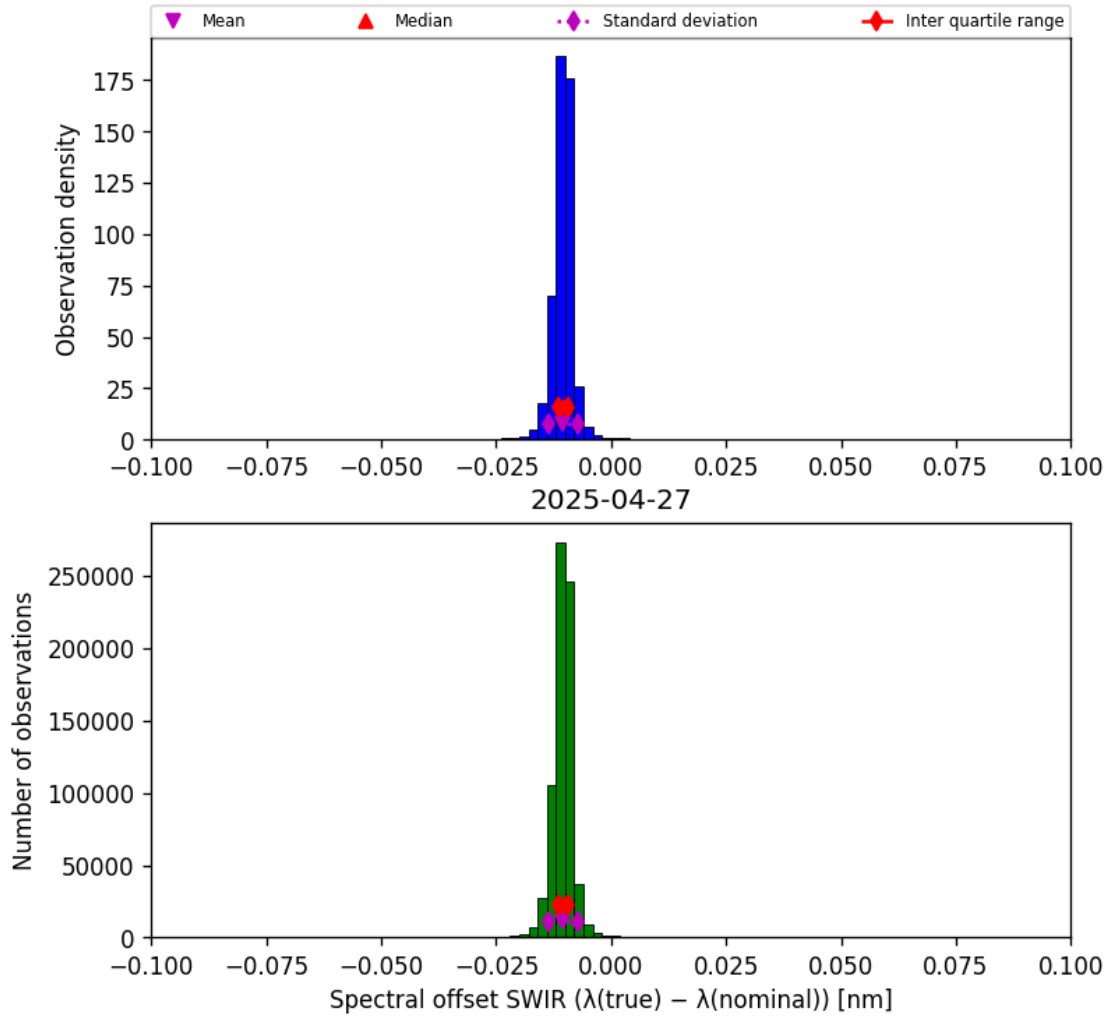
Figure 27: Histogram of “Spectral offset SWIR ( \lambda_{\text{true}} - \lambda_{\text{nominal}} )” for 2025-04-26 to 2025-04-28
