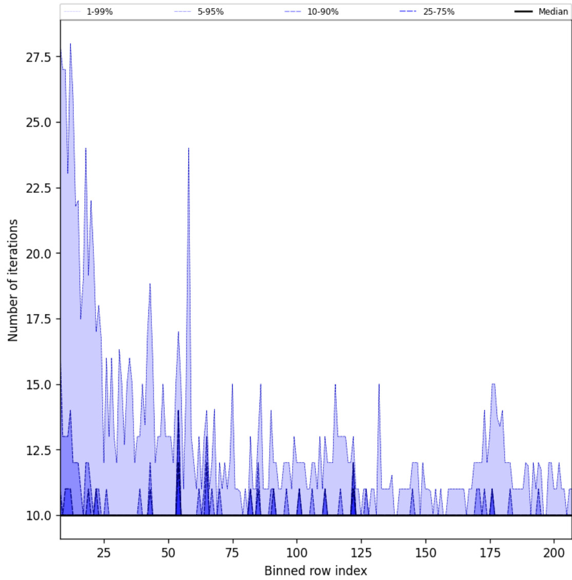
Figure 42: Along track statistics of “Number of iterations” for 2025-04-26 to 2025-04-28
