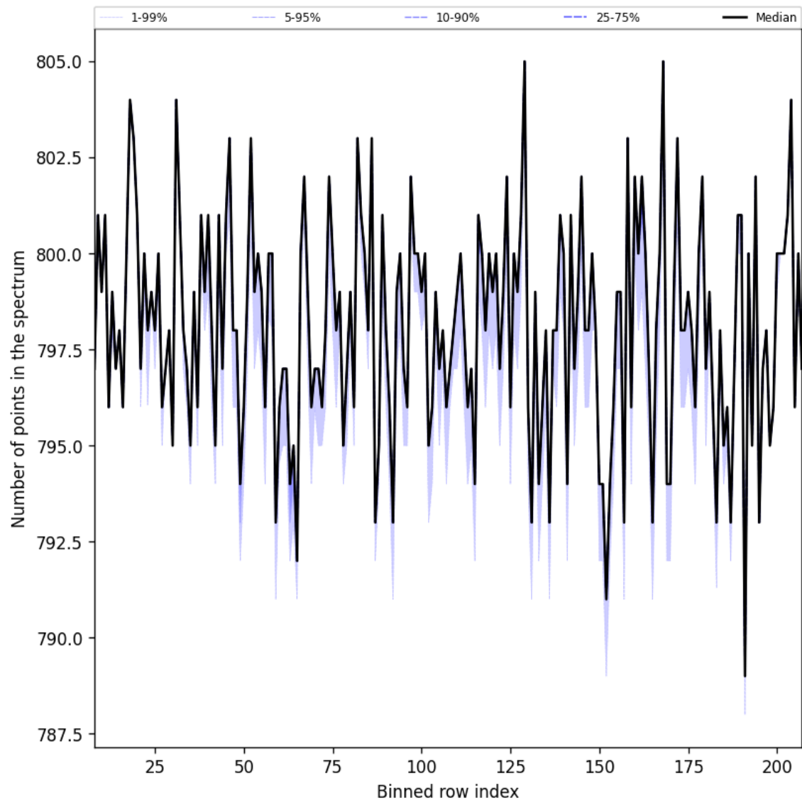
Figure 37: Along track statistics of “Number of points in the spectrum” for 2025-04-26 to 2025-04-28
