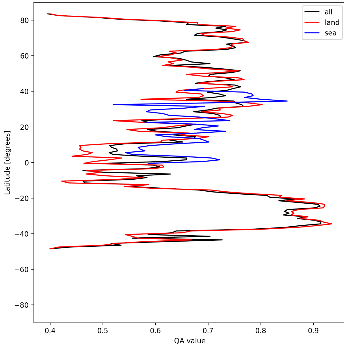
Figure 11: Zonal average of “QA value” for 2025-04-26 to 2025-04-28.
