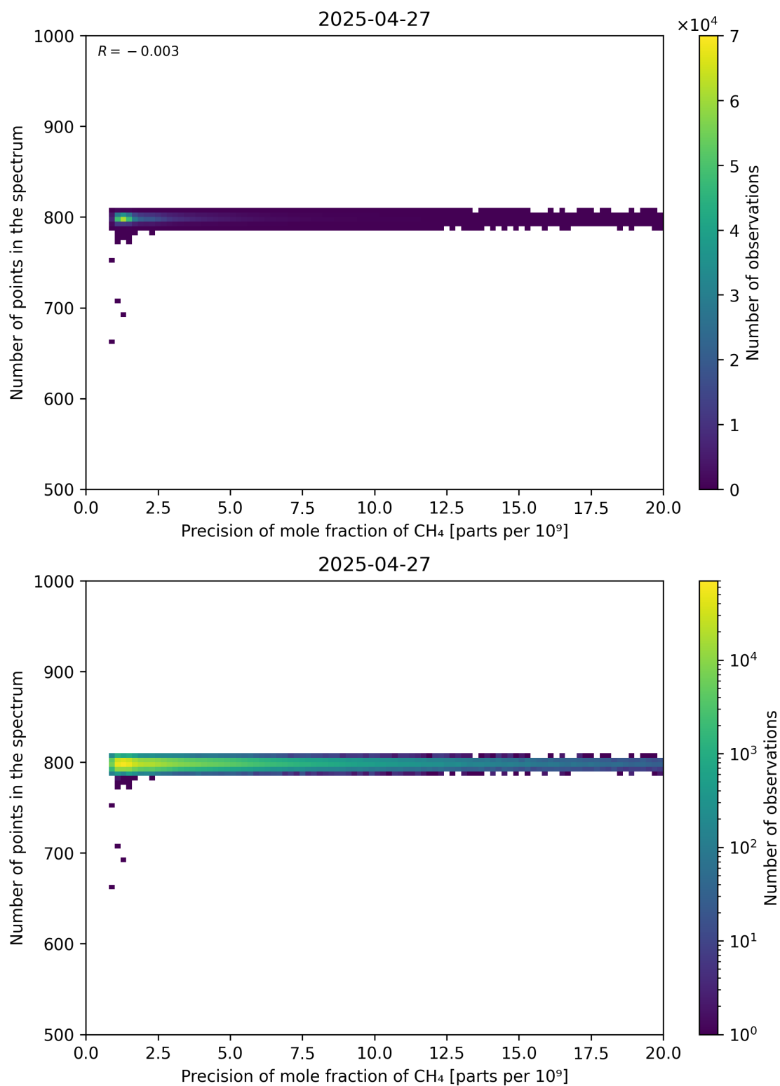
Figure 84: Scatter density plot of “Precision of mole fraction of CH 4 ” against “Number of points in the spectrum” for 2025-04-26 to 2025-04-28.
