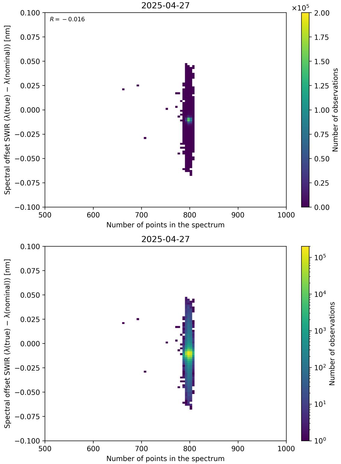
Figure 93: Scatter density plot of “Number of points in the spectrum” against “Spectral offset SWIR ( \lambda_{\text{true}} - \lambda_{\text{nominal}} )” for 2025-04-26 to 2025-04-28.
