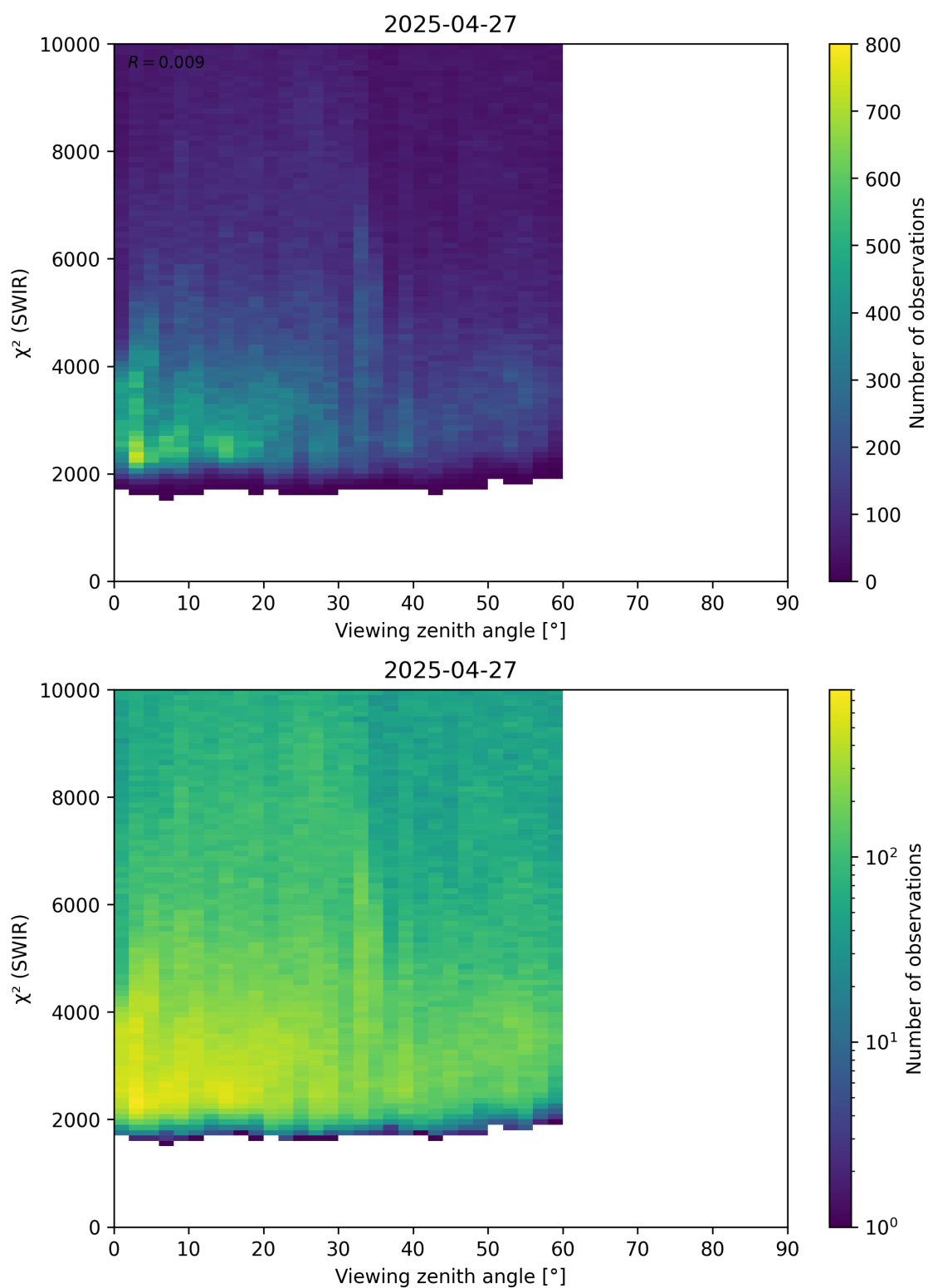
Figure 106: Scatter density plot of “Viewing zenith angle” against “ \chi^2 (SWIR)” for 2025-04-26 to 2025-04-28.
