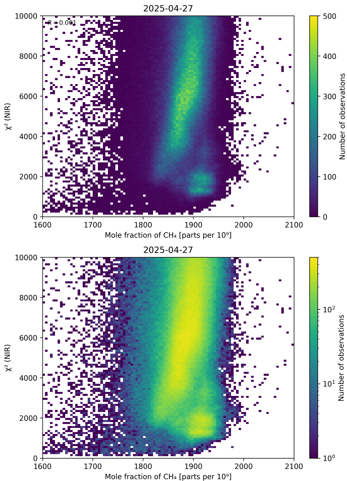
Figure 70: Scatter density plot of “Mole fraction of \text{CH}_4 ” against “ \chi^2 (NIR)” for 2025-04-26 to 2025-04-28.
