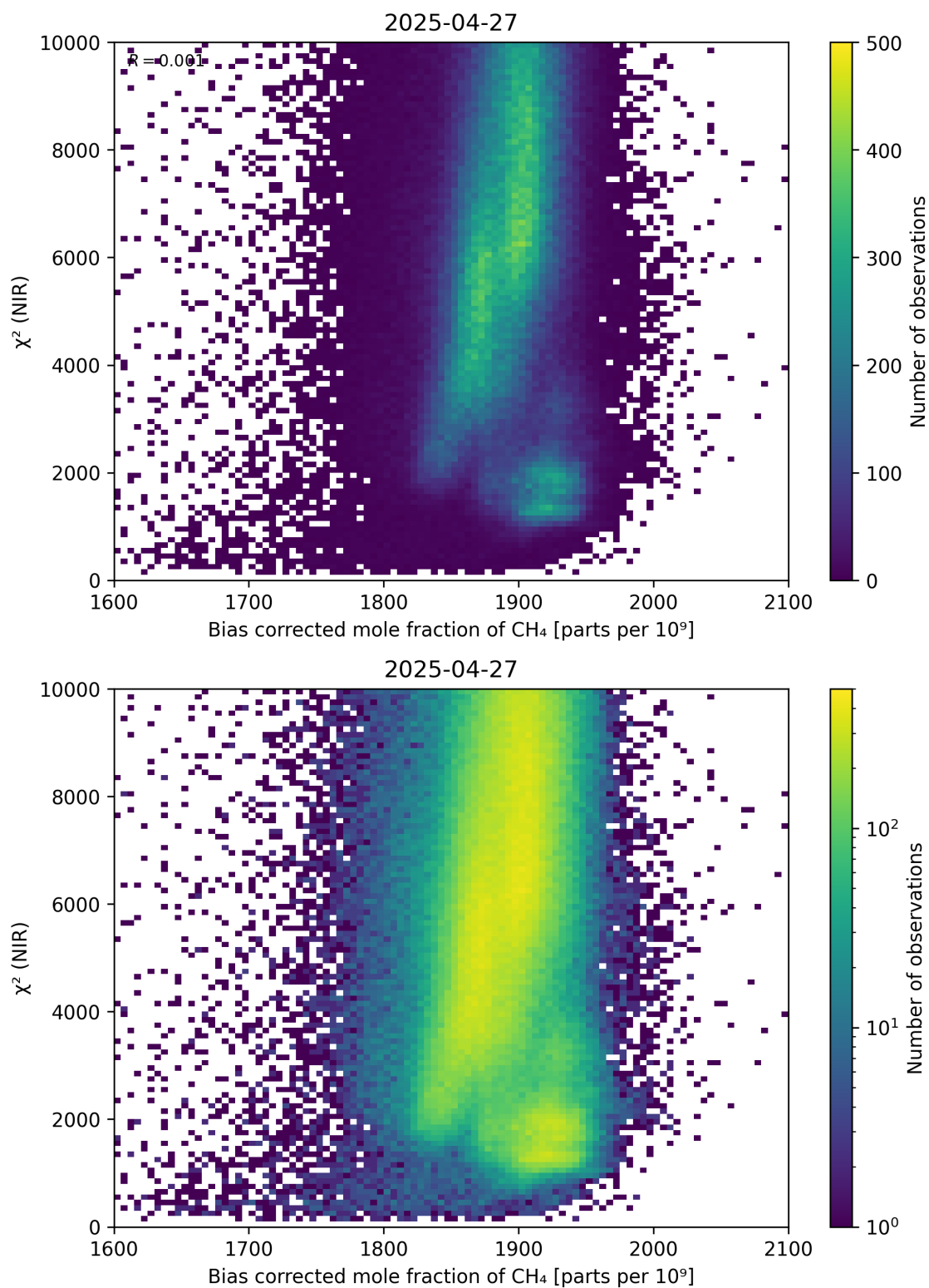
Figure 63: Scatter density plot of “Bias corrected mole fraction of \text{CH}_4 ” against “ \chi^2 (NIR)” for 2025-04-26 to 2025-04-28.
