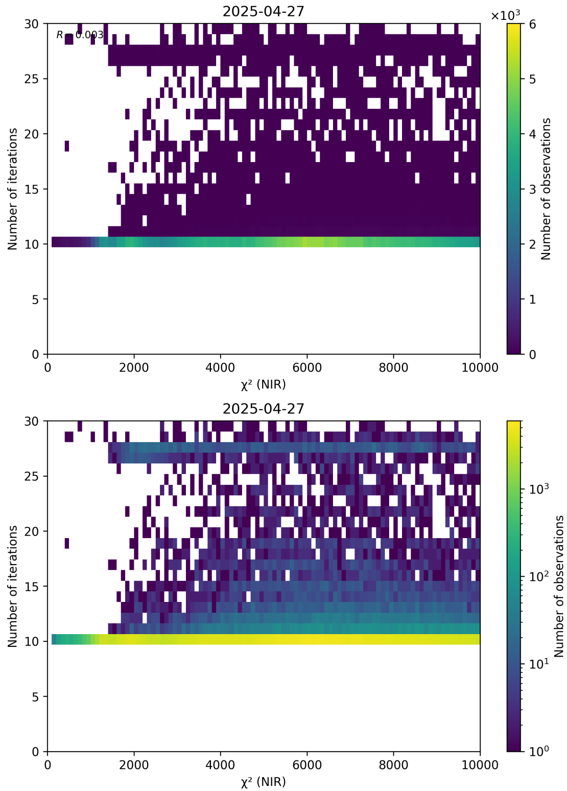
Figure 46: Scatter density plot of “ \chi^2 (NIR)” against “Number of iterations” for 2025-04-26 to 2025-04-28.
