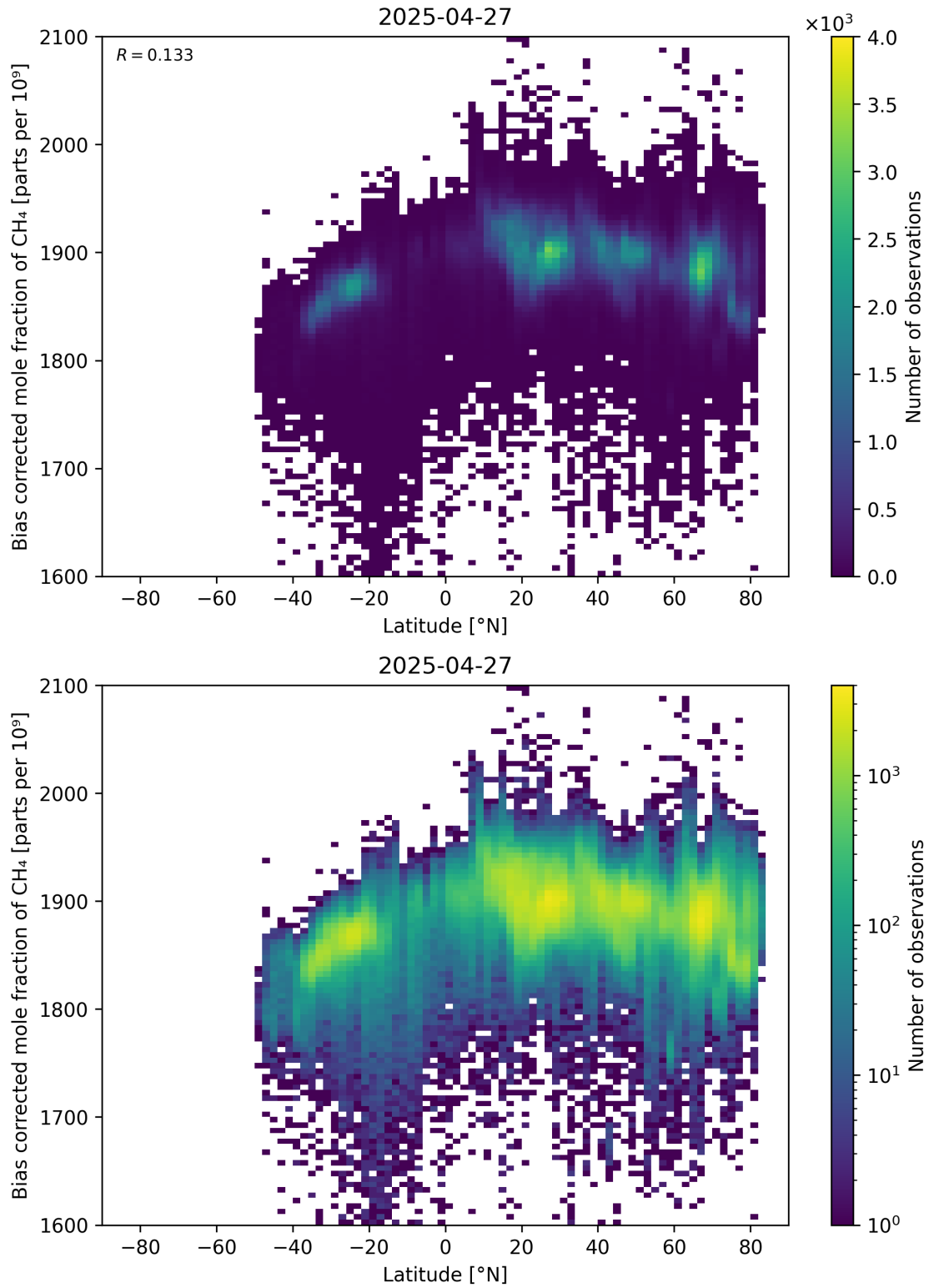
Figure 58: Scatter density plot of “Latitude” against “Bias corrected mole fraction of CH 4 ” for 2025-04-26 to 2025-04-28.
