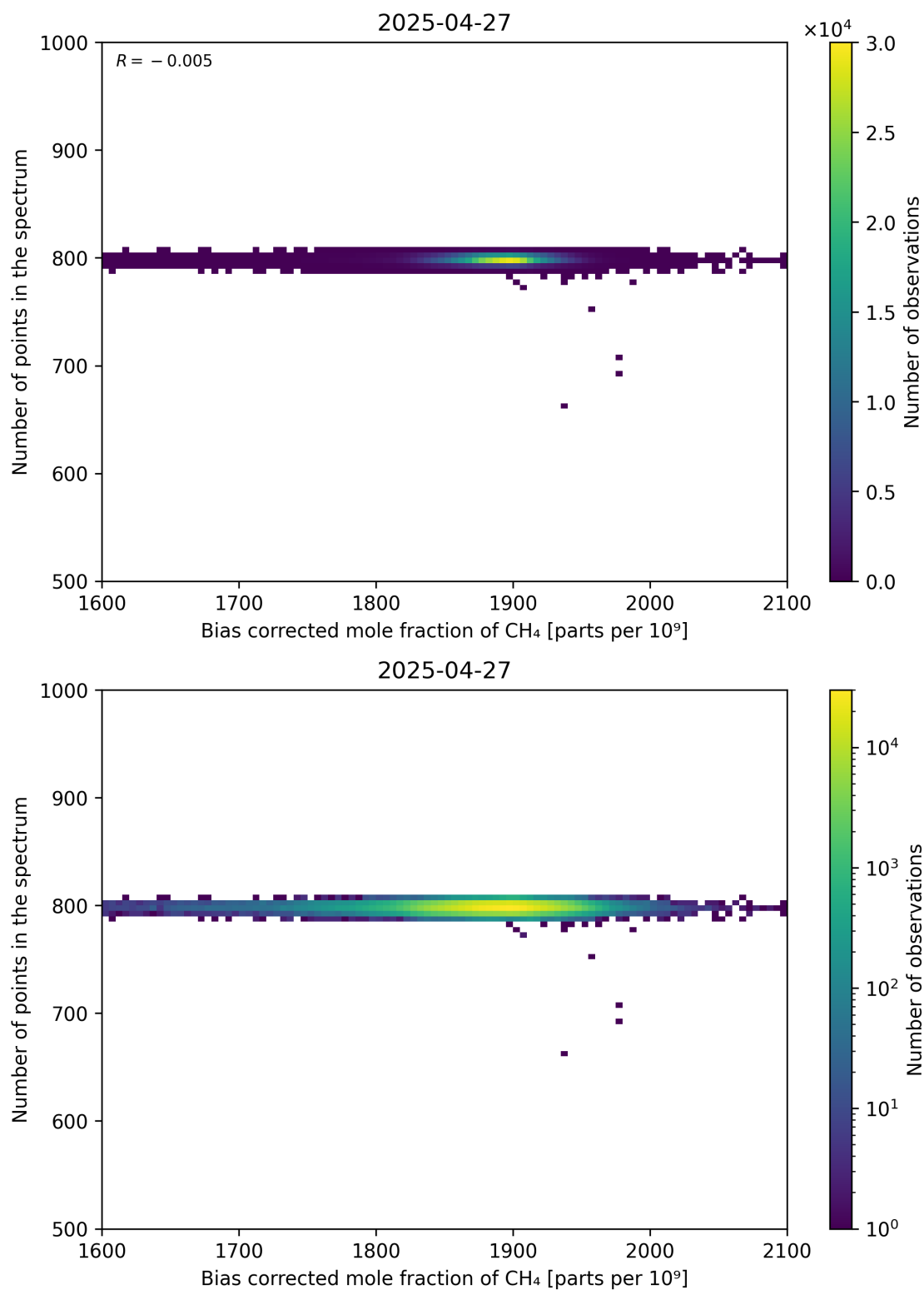
Figure 68: Scatter density plot of “Bias corrected mole fraction of CH 4 ” against “Number of points in the spectrum” for 2025-04-26 to 2025-04-28.
