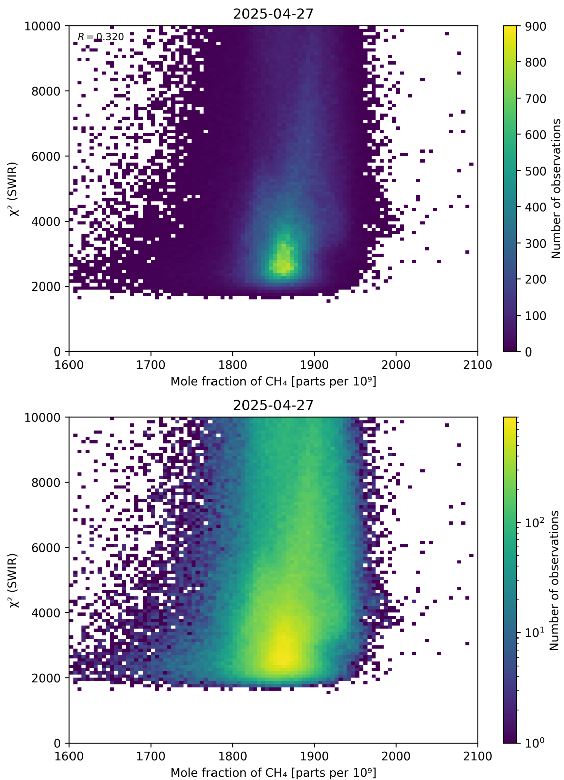
Figure 71: Scatter density plot of “Mole fraction of \text{CH}_4 ” against “ \chi^2 (SWIR)” for 2025-04-26 to 2025-04-28.
