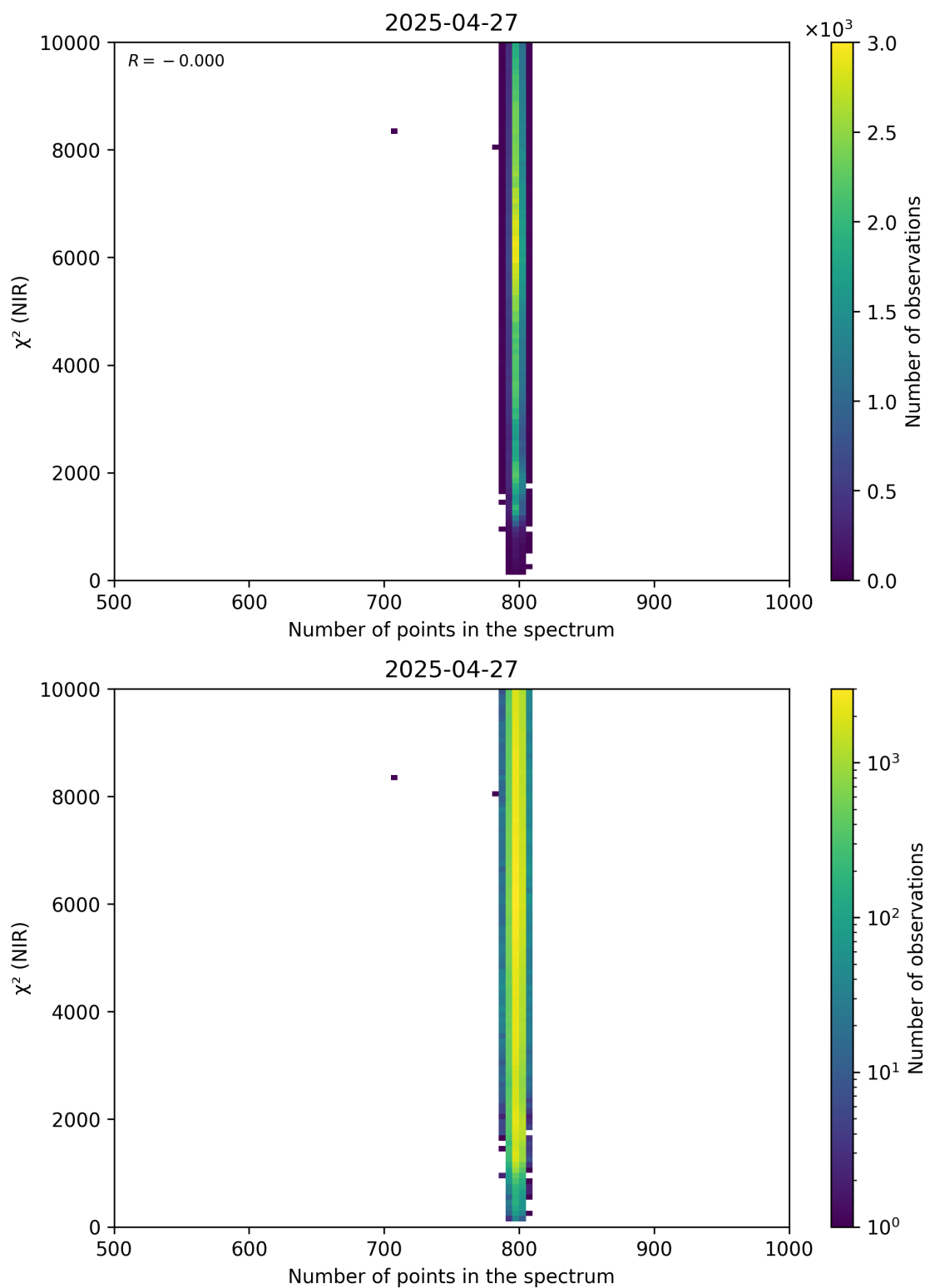
Figure 88: Scatter density plot of “Number of points in the spectrum” against “ \chi^2 (NIR)” for 2025-04-26 to 2025-04-28.
