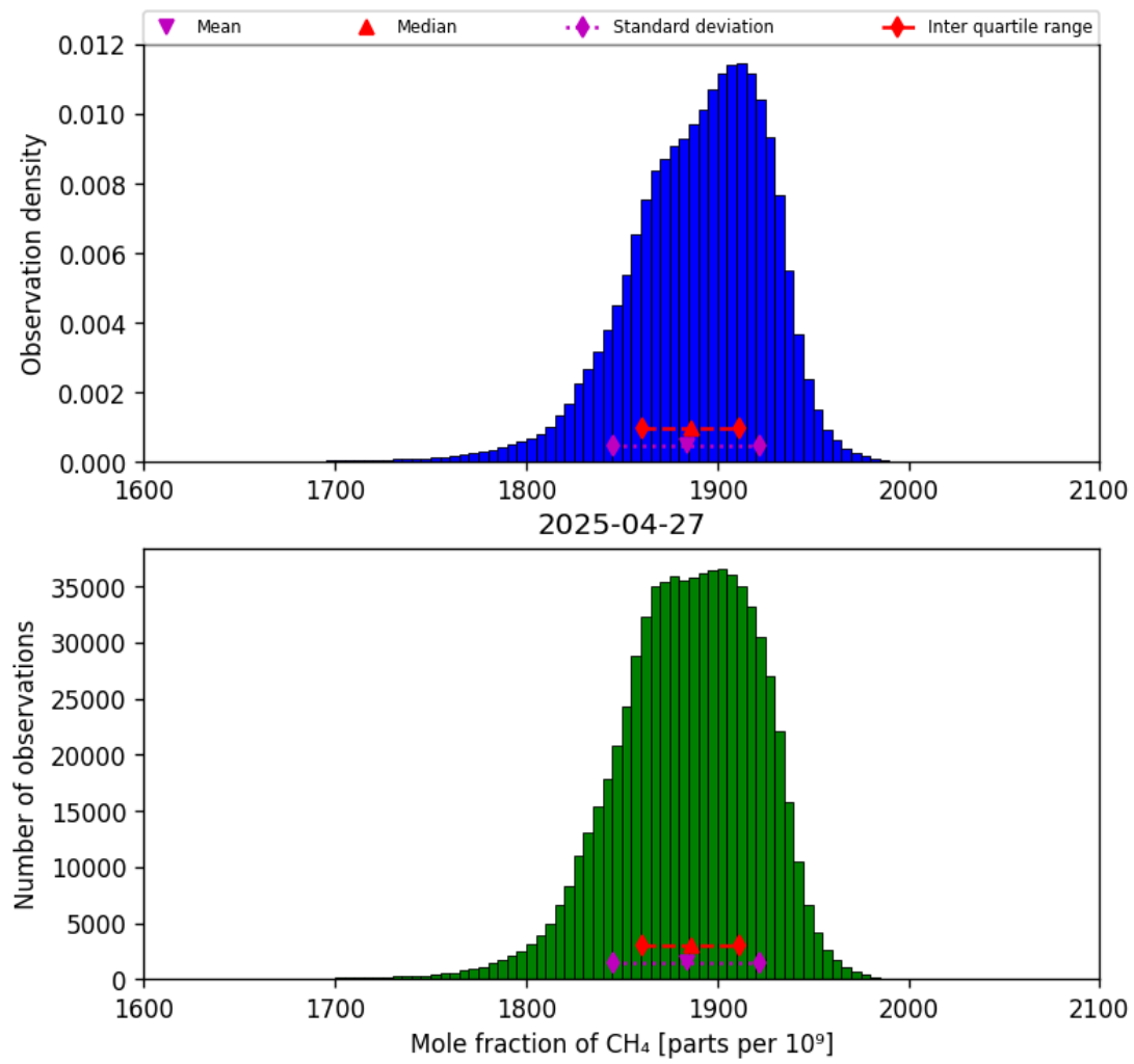
Figure 23: Histogram of “Mole fraction of CH 4 ” for 2025-04-26 to 2025-04-28
