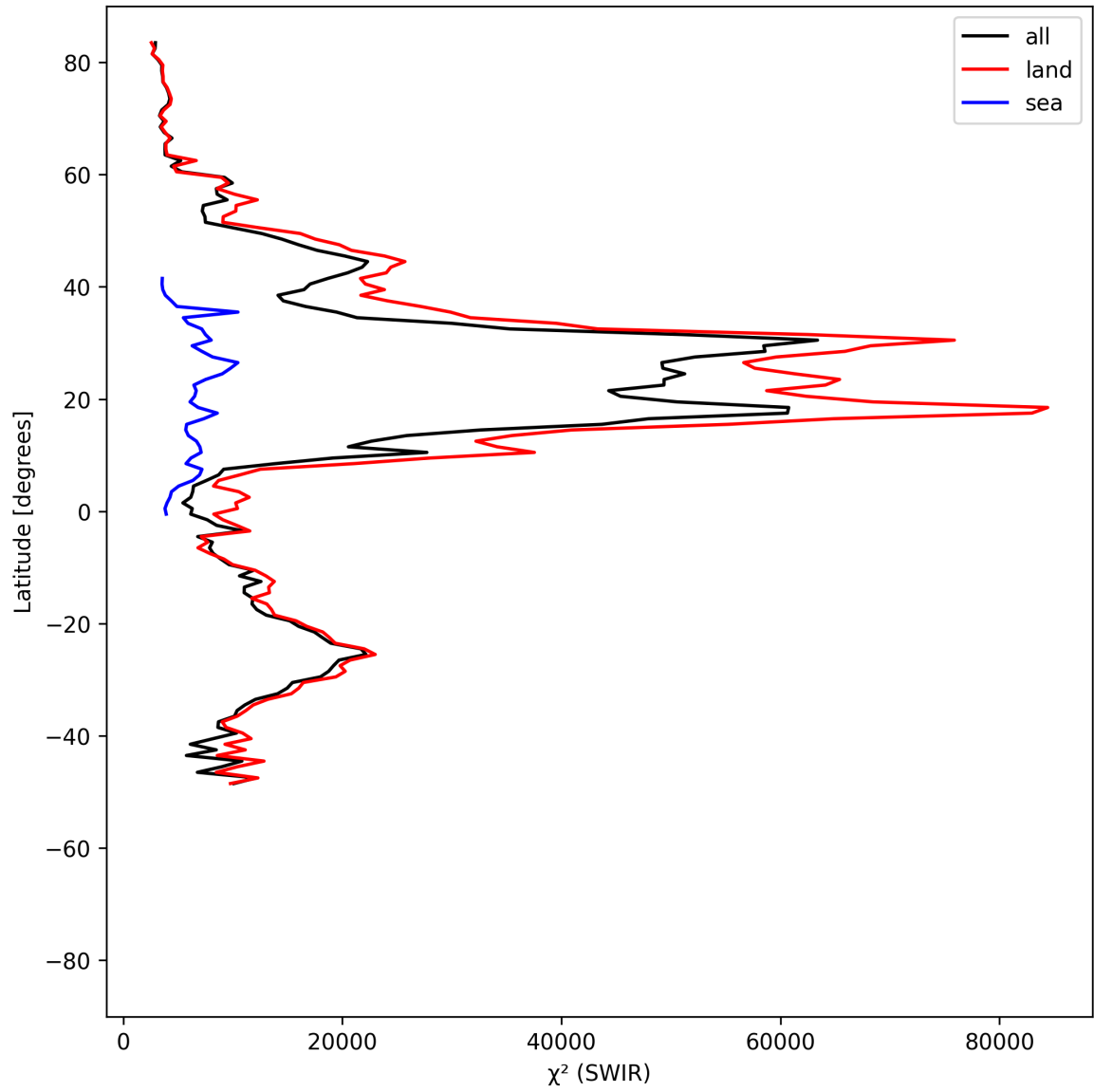
Figure 17: Zonal average of “ \chi^2 (SWIR)” for 2025-04-26 to 2025-04-28.
