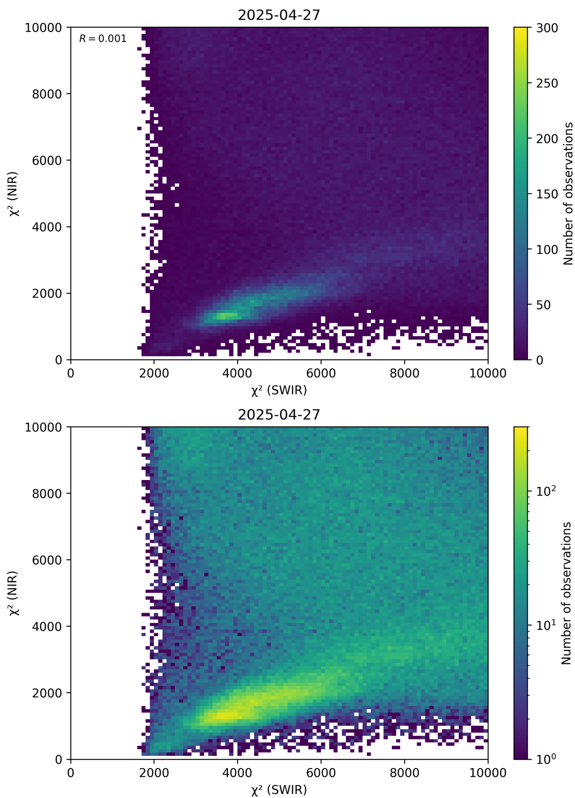
Figure 47: Scatter density plot of “ \chi^2 (SWIR)” against “ \chi^2 (NIR)” for 2025-04-26 to 2025-04-28.
