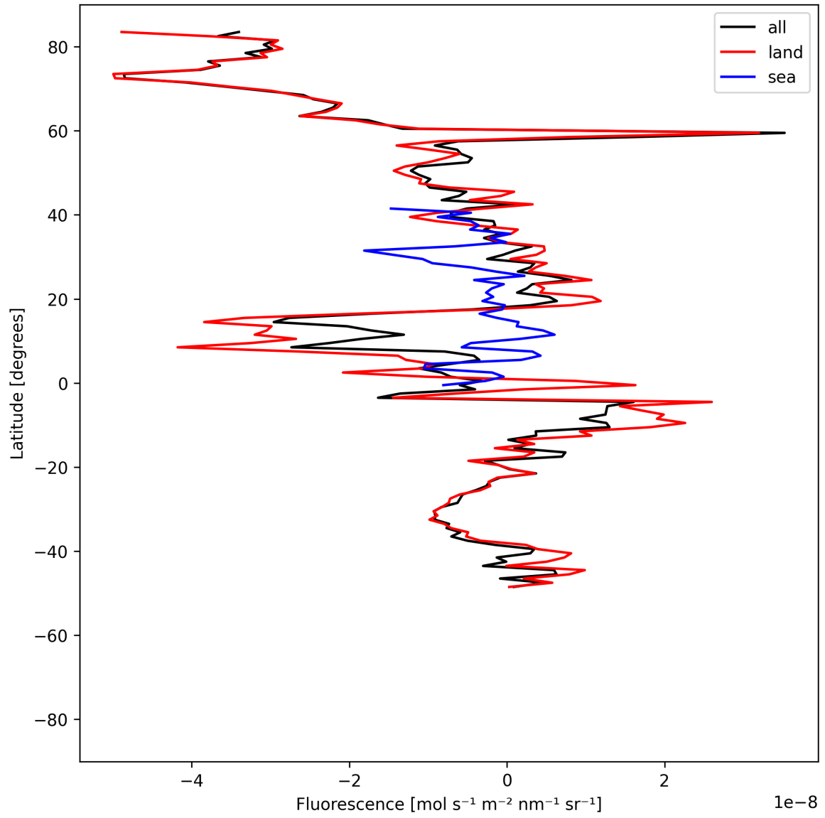
Figure 21: Zonal average of “Fluorescence” for 2025-04-26 to 2025-04-28.
