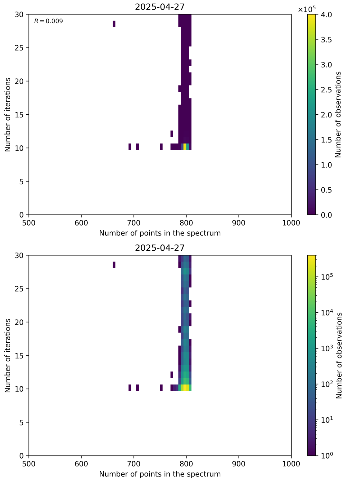
Figure 92: Scatter density plot of “Number of points in the spectrum” against “Number of iterations” for 2025-04-26 to 2025-04-28.
