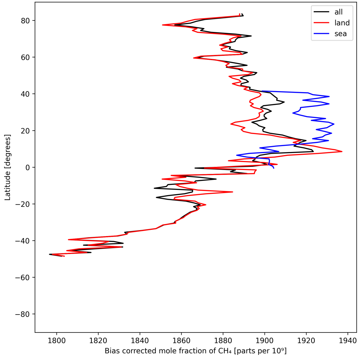
Figure 14: Zonal average of “Bias corrected mole fraction of CH 4 ” for 2025-04-26 to 2025-04-28.
