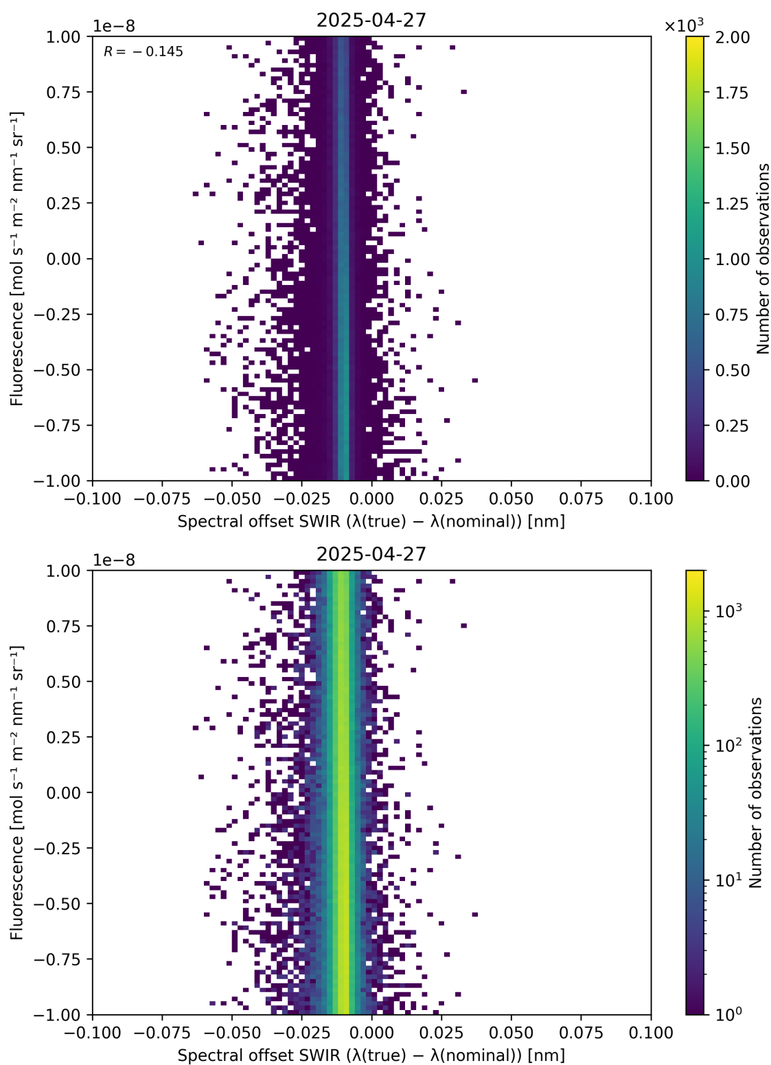
Figure 120: Scatter density plot of “Spectral offset SWIR ( \lambda_{\text{true}} - \lambda_{\text{nominal}} )” against “Fluorescence” for 2025-04-26 to 2025-04-28.
