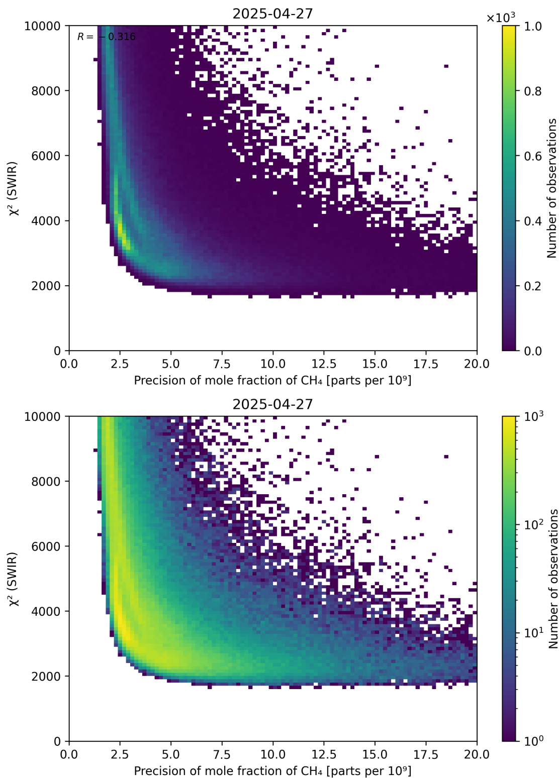
Figure 79: Scatter density plot of “Precision of mole fraction of CH 4 ” against “ \chi^2 (SWIR)” for 2025-04-26 to 2025-04-28.
