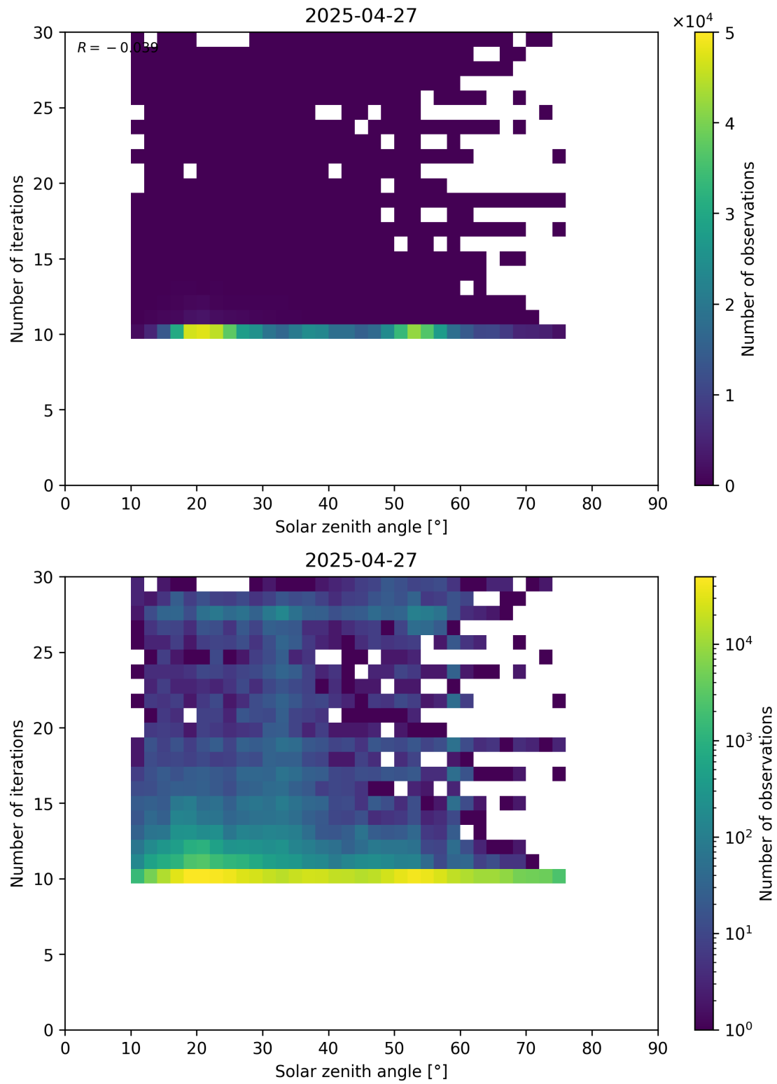
Figure 102: Scatter density plot of “Solar zenith angle” against “Number of iterations” for 2025-04-26 to 2025-04-28.
