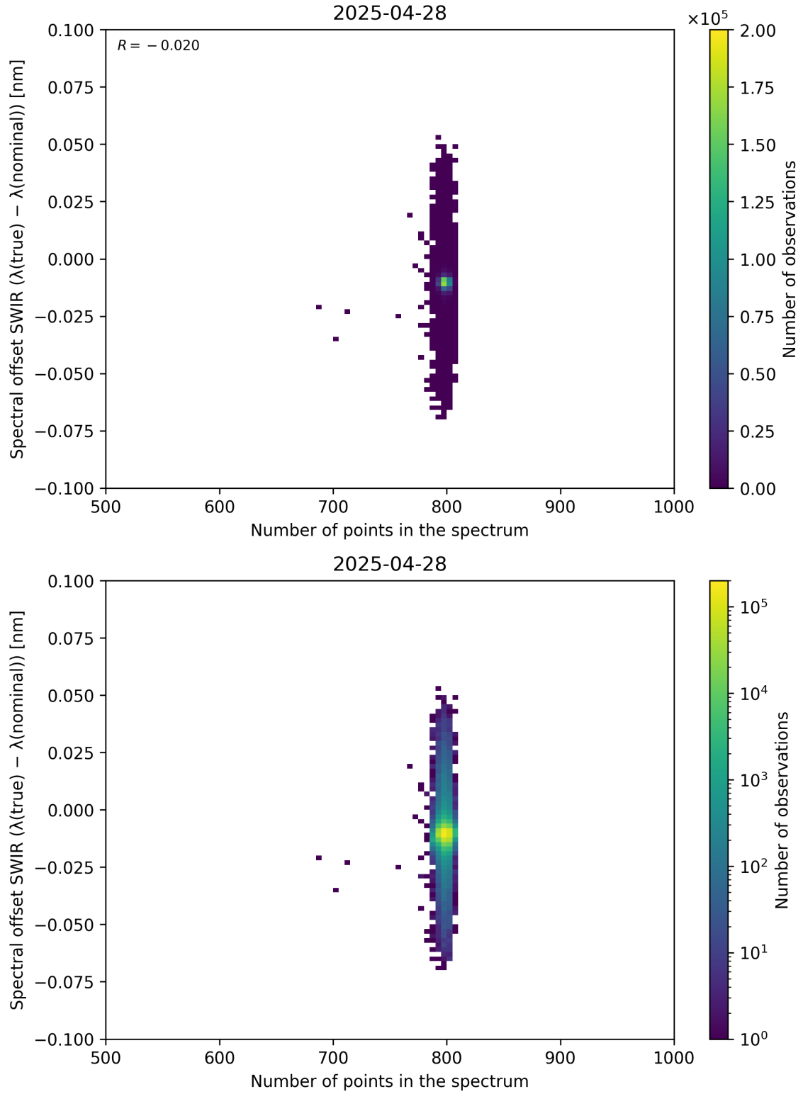
Figure 93: Scatter density plot of “Number of points in the spectrum” against “Spectral offset SWIR ( \lambda_{\text{true}} - \lambda_{\text{nominal}} )” for 2025-04-27 to 2025-04-29.
