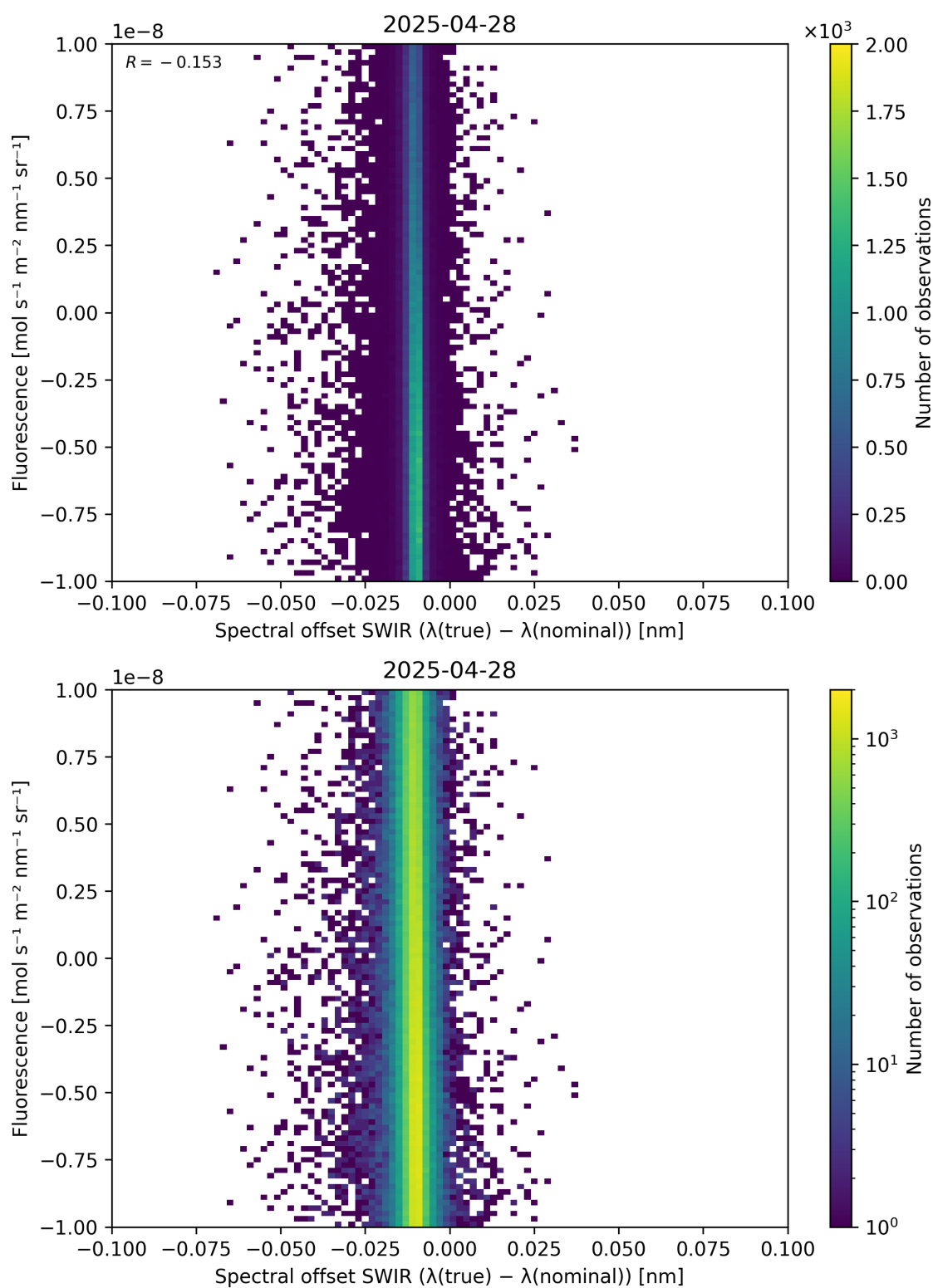
Figure 120: Scatter density plot of “Spectral offset SWIR ( \lambda_{\text{true}} - \lambda_{\text{nominal}} )” against “Fluorescence” for 2025-04-27 to 2025-04-29.
