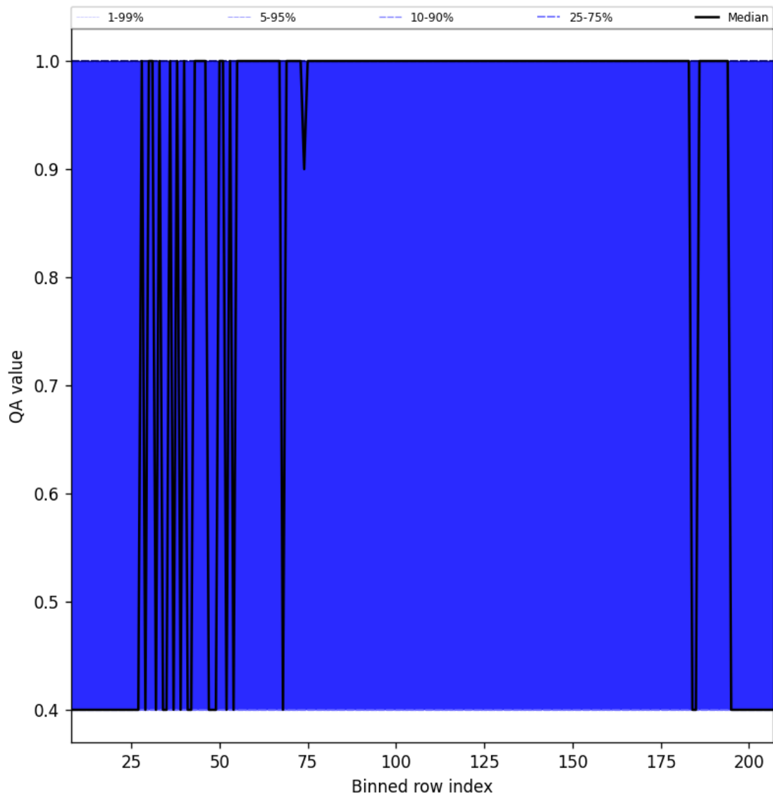
Figure 33: Along track statistics of “QA value” for 2025-04-27 to 2025-04-29
