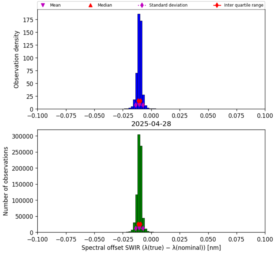
Figure 27: Histogram of “Spectral offset SWIR ( \lambda_{\text{true}} - \lambda_{\text{nominal}} )” for 2025-04-27 to 2025-04-29
