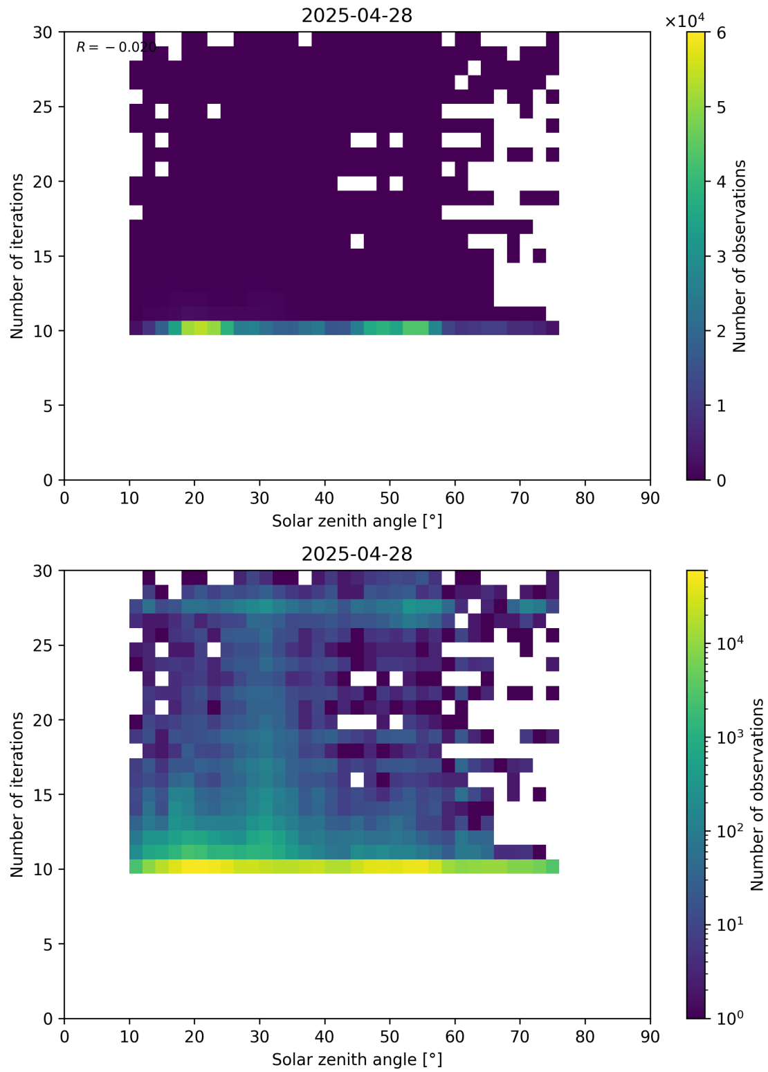
Figure 102: Scatter density plot of “Solar zenith angle” against “Number of iterations” for 2025-04-27 to 2025-04-29.
