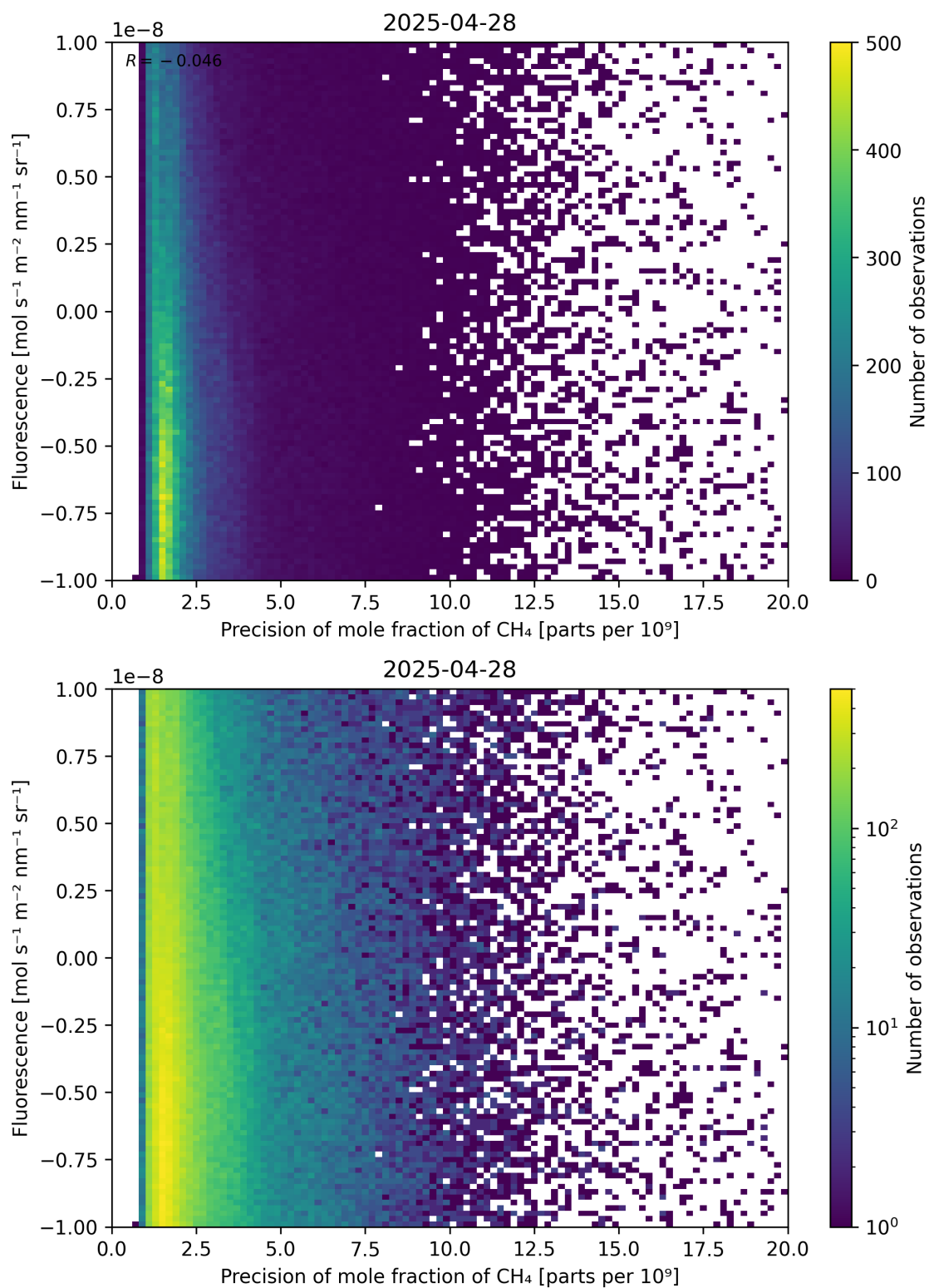
Figure 81: Scatter density plot of “Precision of mole fraction of CH 4 ” against “Fluorescence” for 2025-04-27 to 2025-04-29.
