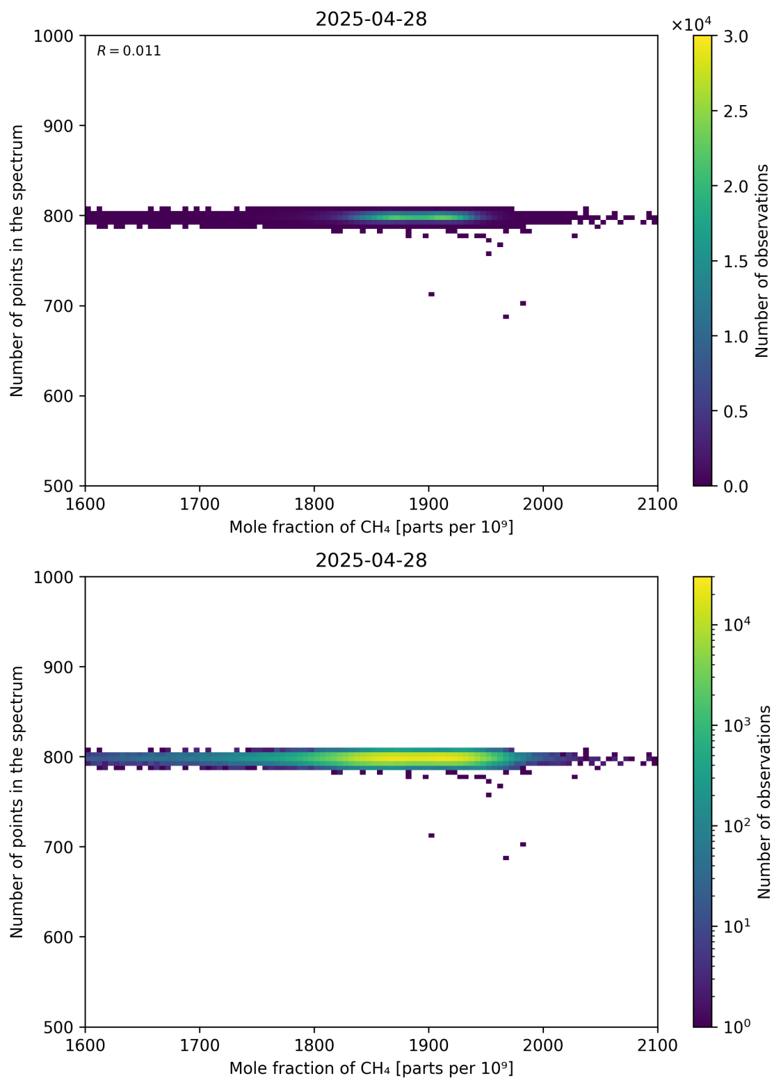
Figure 77: Scatter density plot of “Mole fraction of CH 4 ” against “Number of points in the spectrum” for 2025-04-27 to 2025-04-29.
