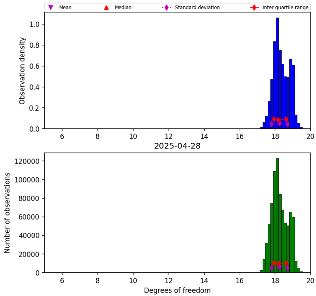
Figure 30: Histogram of “Degrees of freedom” for 2025-04-27 to 2025-04-29
