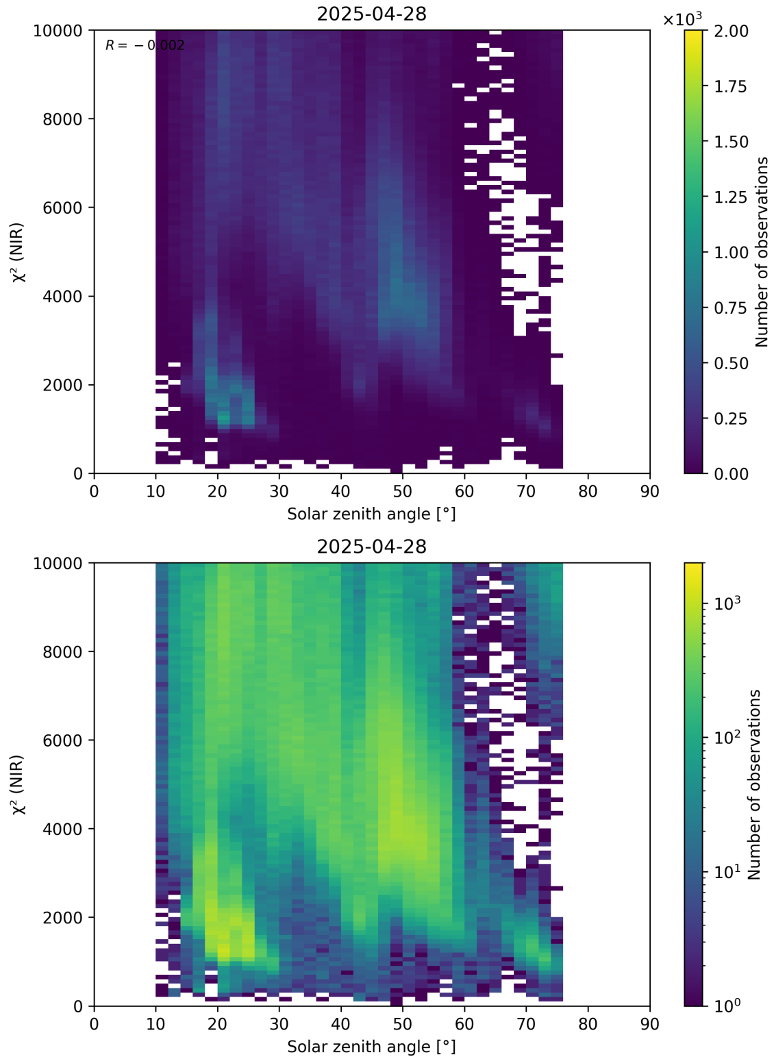
Figure 94: Scatter density plot of “Solar zenith angle” against “ \chi^2 (NIR)” for 2025-04-27 to 2025-04-29.
