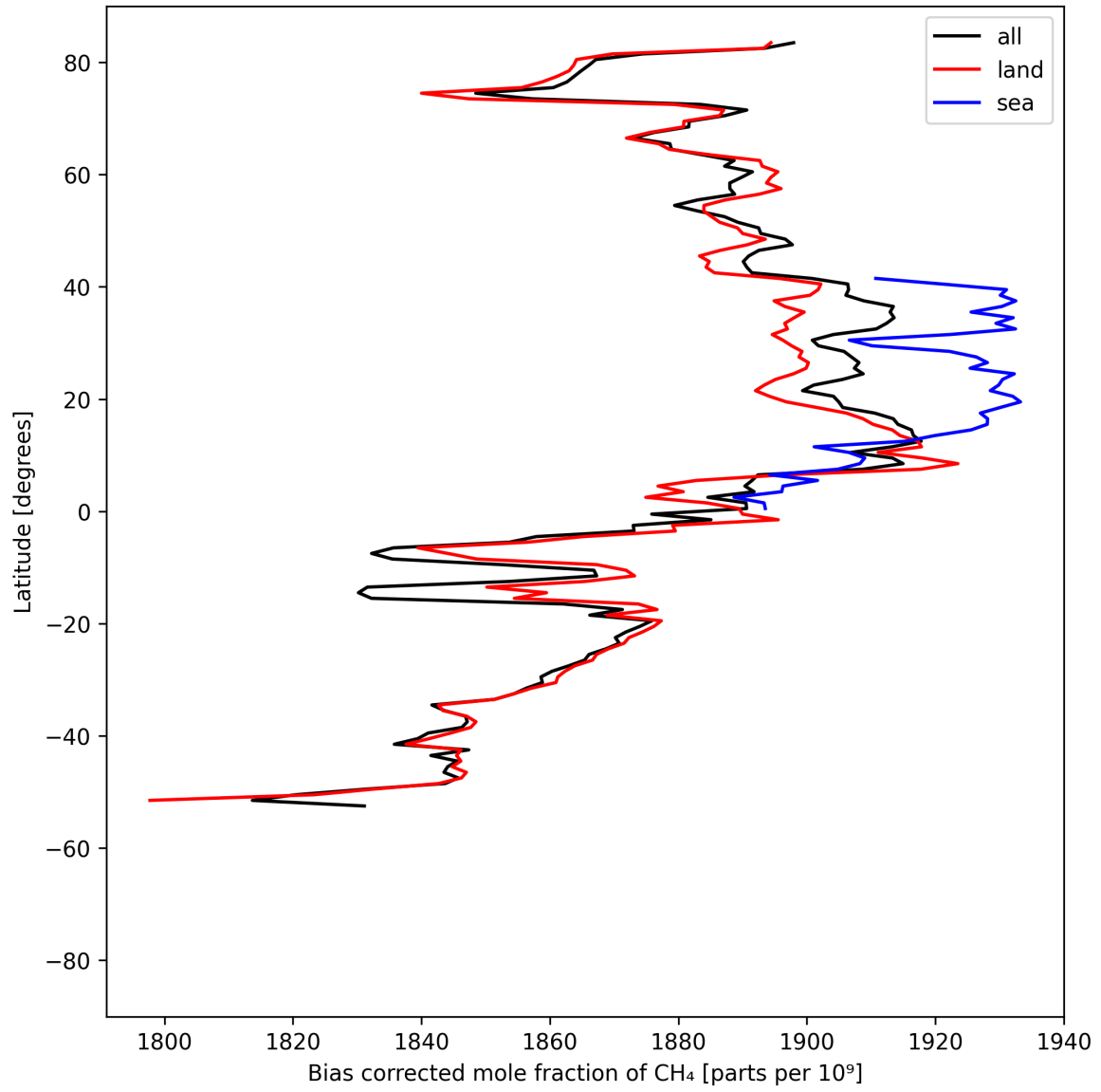
Figure 14: Zonal average of “Bias corrected mole fraction of CH 4 ” for 2025-04-27 to 2025-04-29.
