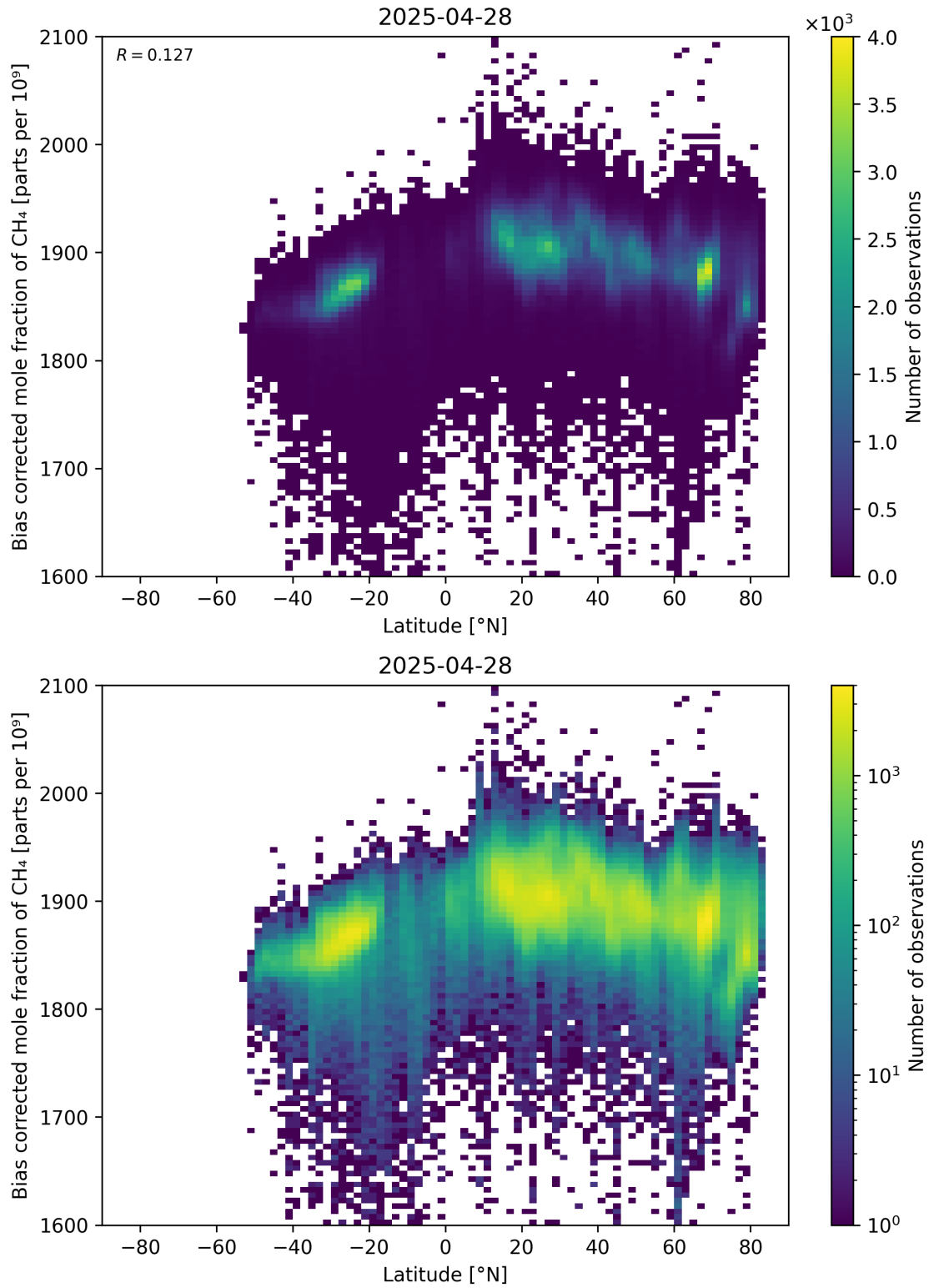
Figure 58: Scatter density plot of “Latitude” against “Bias corrected mole fraction of CH 4 ” for 2025-04-27 to 2025-04-29.
