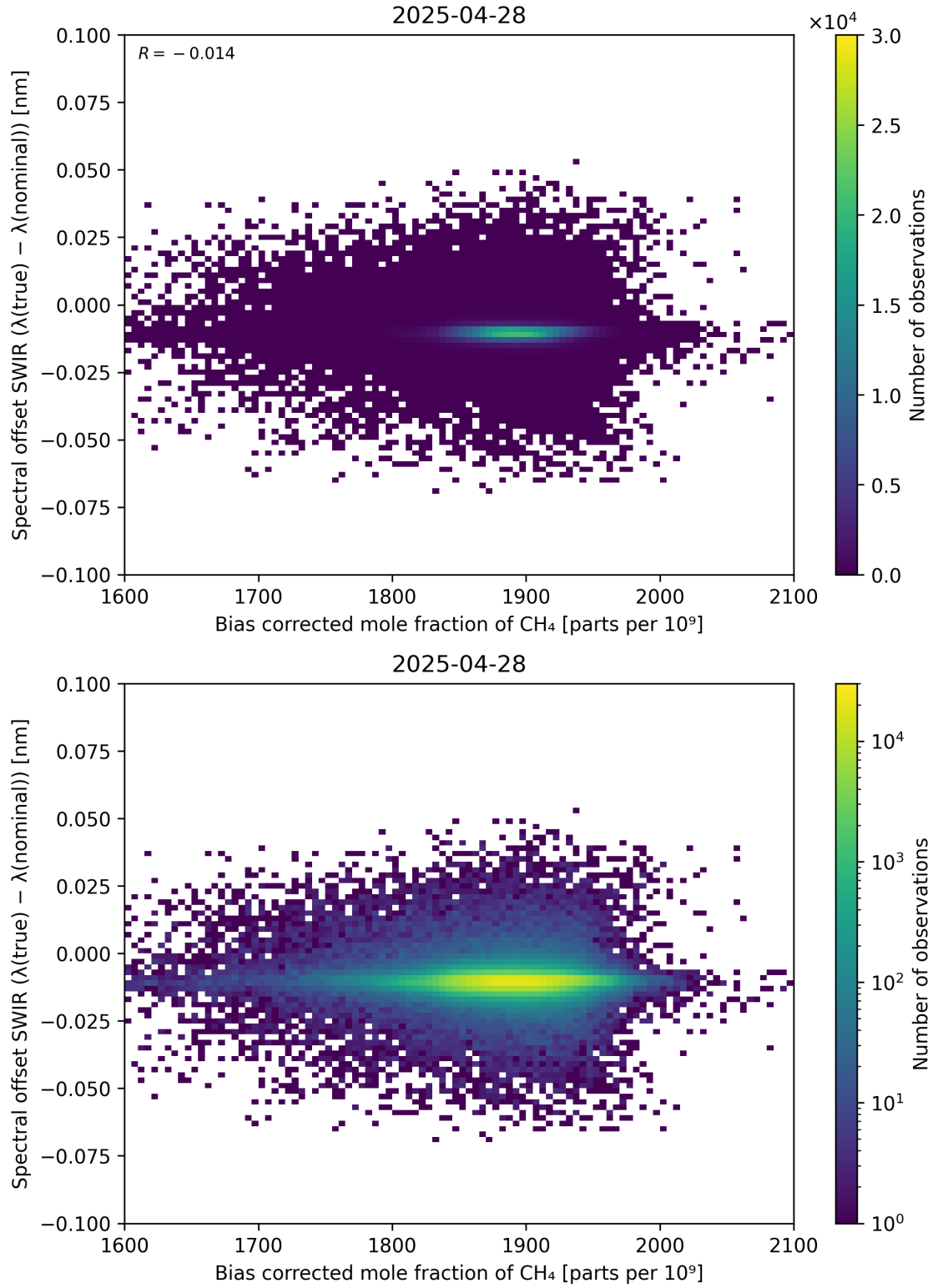
Figure 69: Scatter density plot of “Bias corrected mole fraction of \text{CH}_4 ” against “Spectral offset SWIR ( \lambda_{\text{true}} - \lambda_{\text{nominal}} )” for 2025-04-27 to 2025-04-29.
