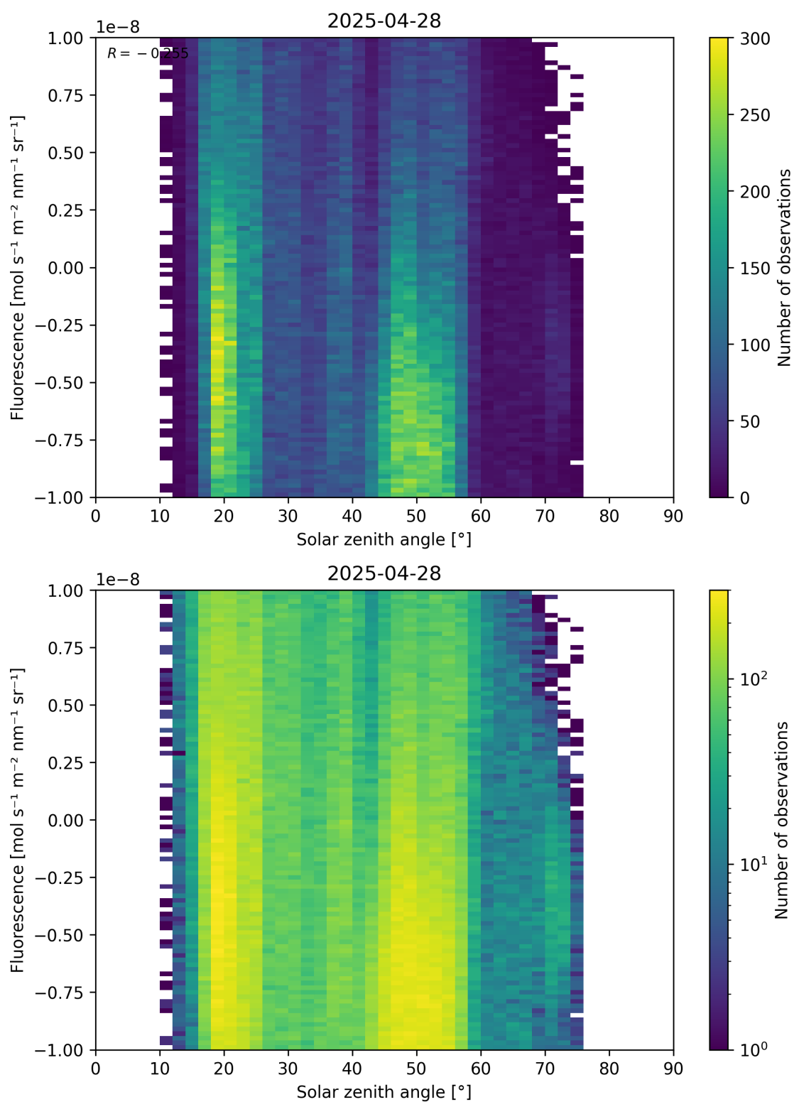
Figure 97: Scatter density plot of “Solar zenith angle” against “Fluorescence” for 2025-04-27 to 2025-04-29.
