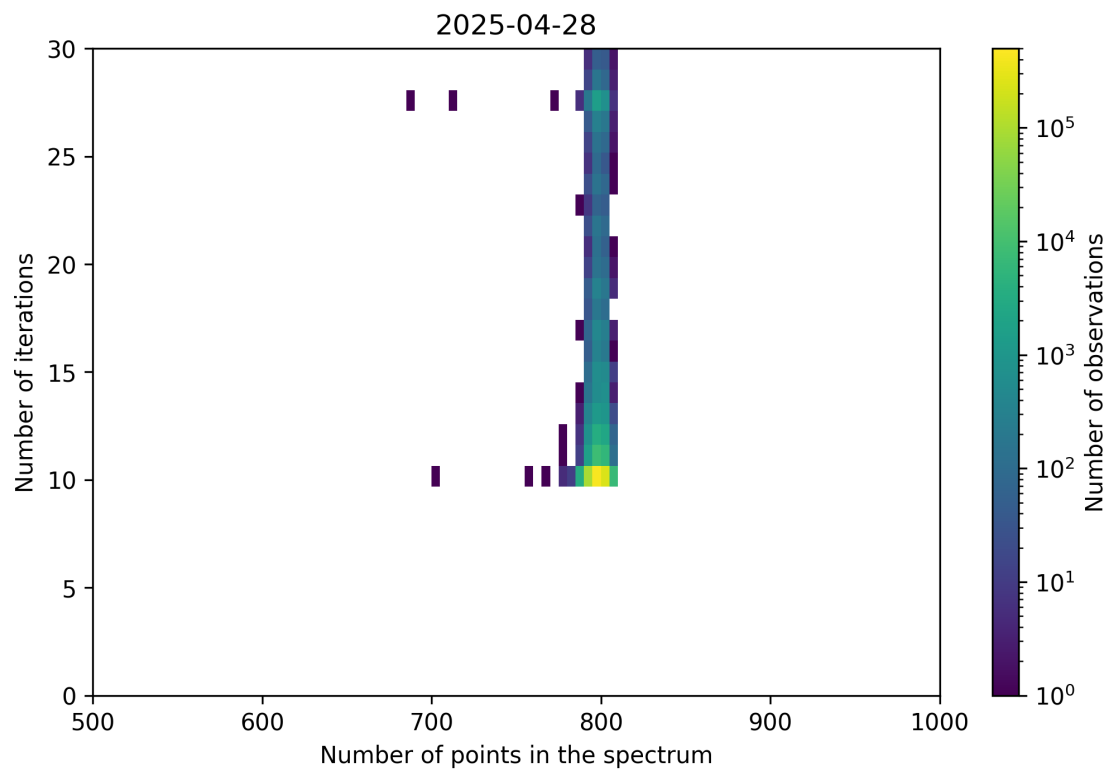
Figure 92: Scatter density plot of “Number of points in the spectrum” against “Number of iterations” for 2025-04-27 to 2025-04-29.
