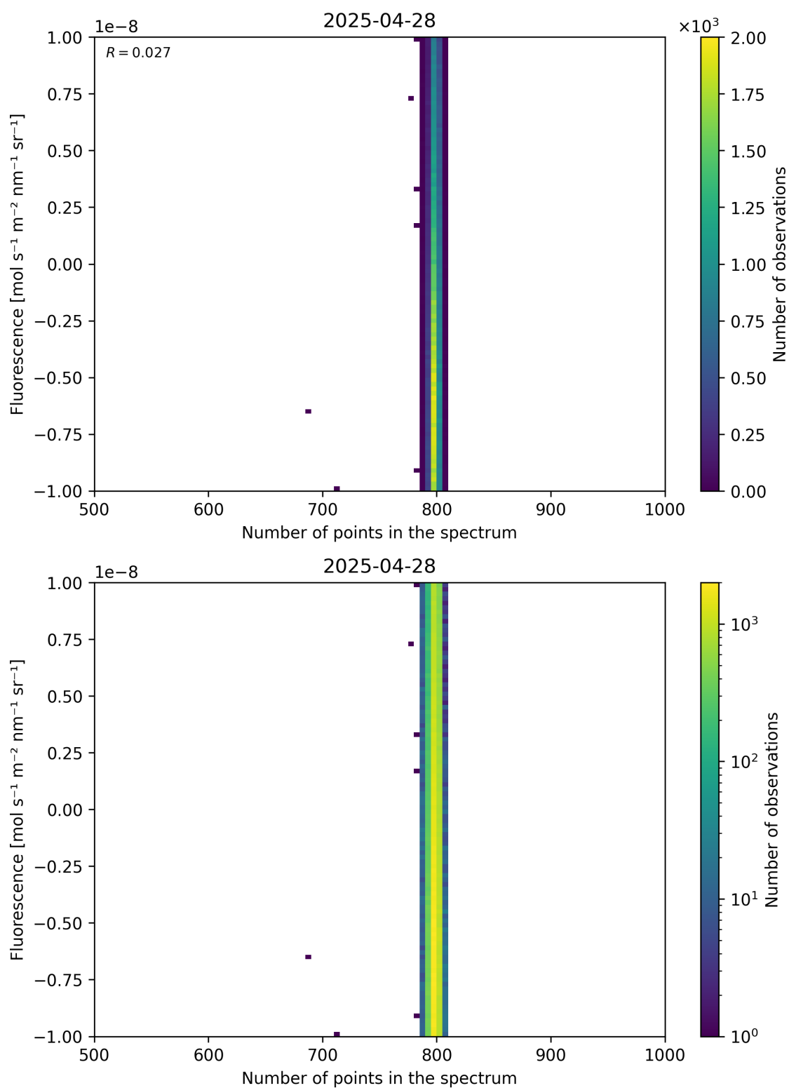
Figure 91: Scatter density plot of “Number of points in the spectrum” against “Fluorescence” for 2025-04-27 to 2025-04-29.
