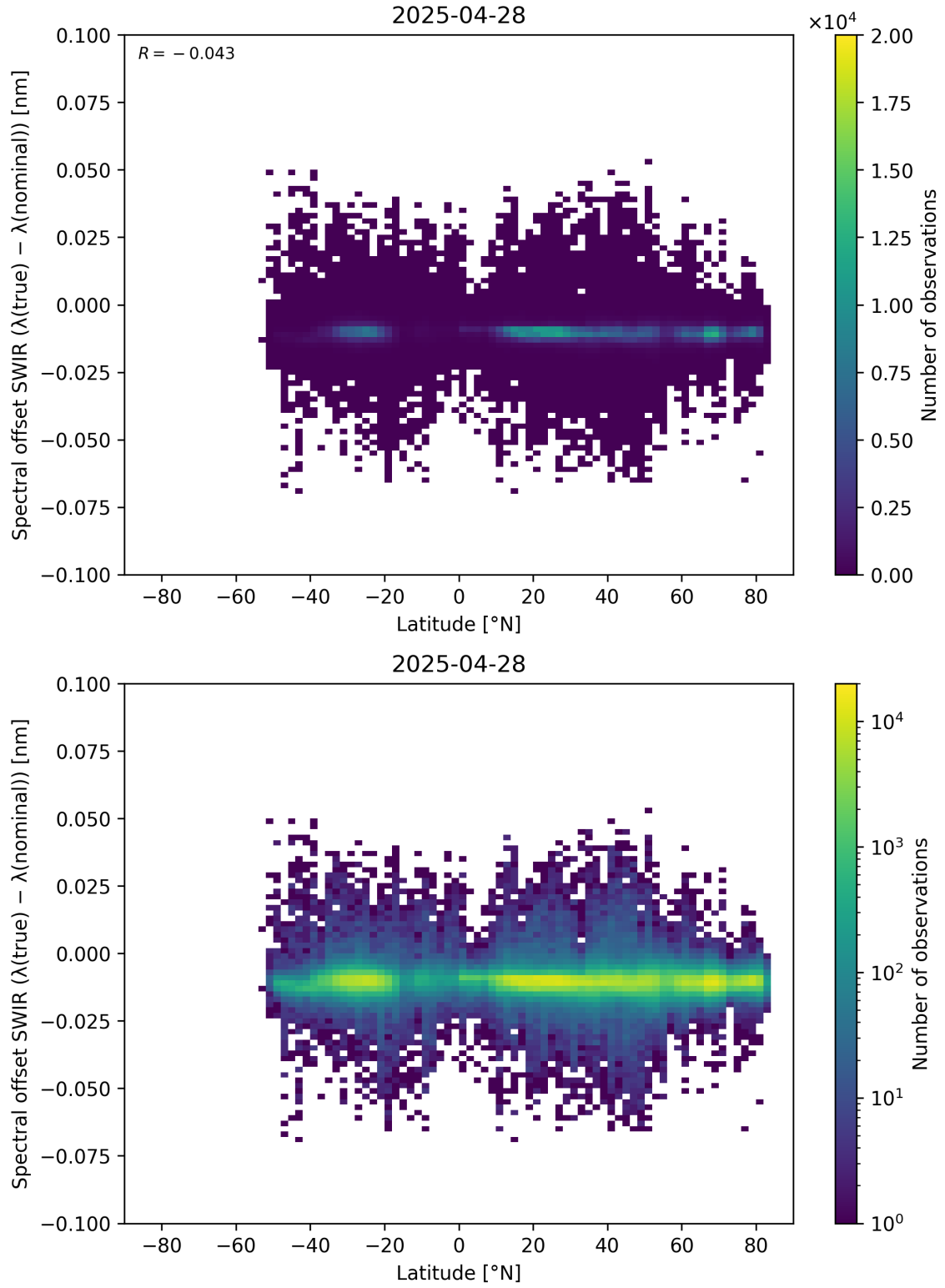
Figure 62: Scatter density plot of “Latitude” against “Spectral offset SWIR ( \lambda_{\text{true}} - \lambda_{\text{nominal}} )” for 2025-04-27 to 2025-04-29.
