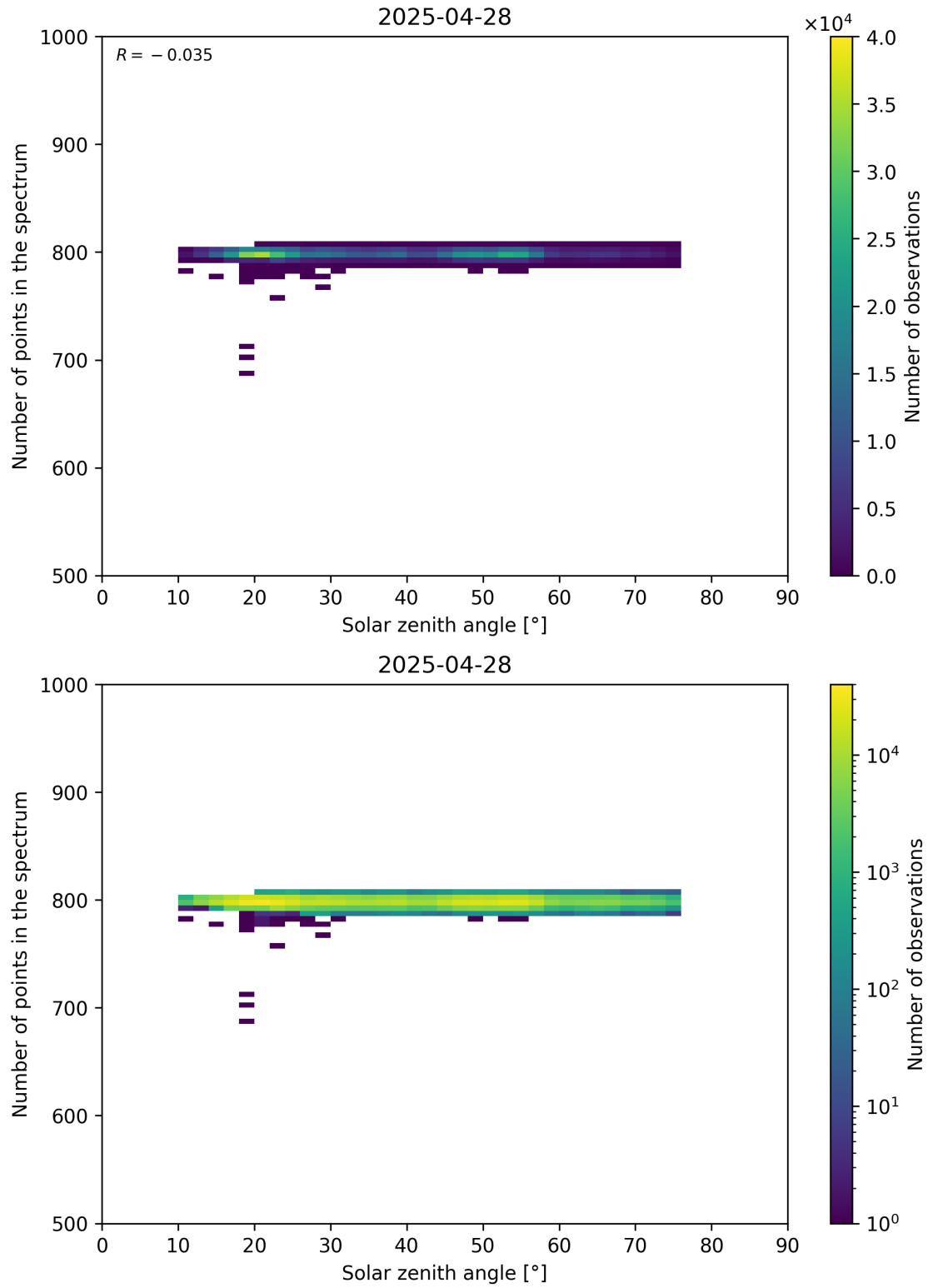
Figure 103: Scatter density plot of “Solar zenith angle” against “Number of points in the spectrum” for 2025-04-27 to 2025-04-29.
