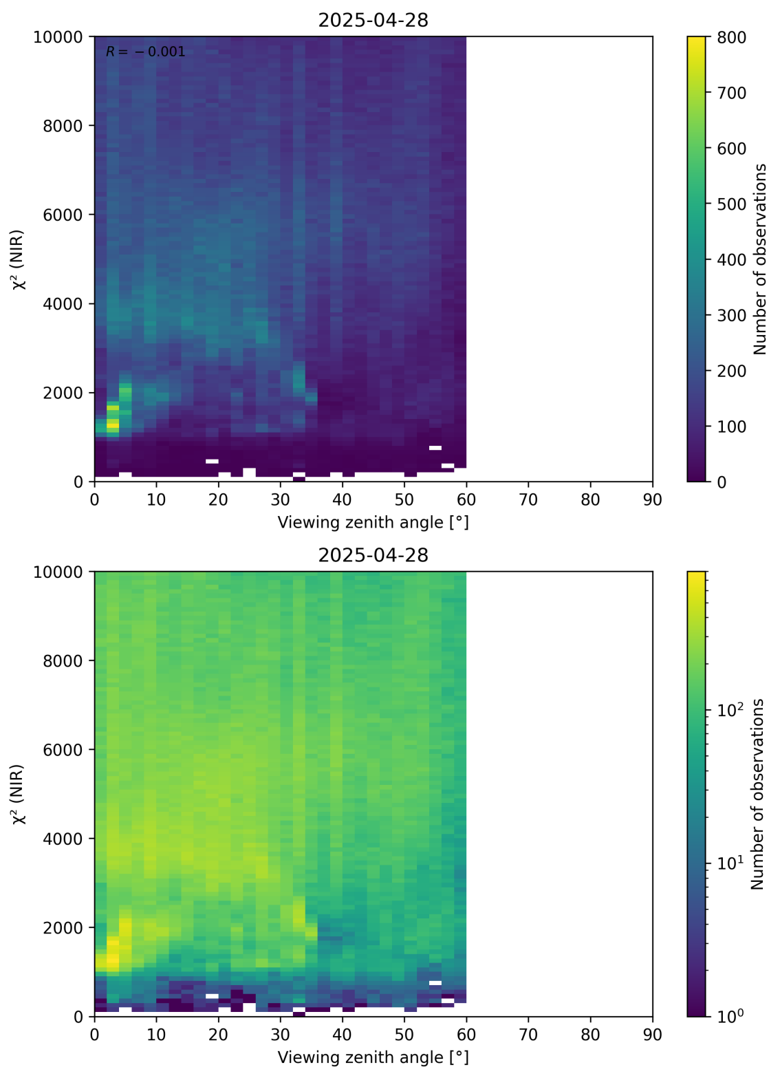
Figure 105: Scatter density plot of “Viewing zenith angle” against “ \chi^2 (NIR)” for 2025-04-27 to 2025-04-29.
