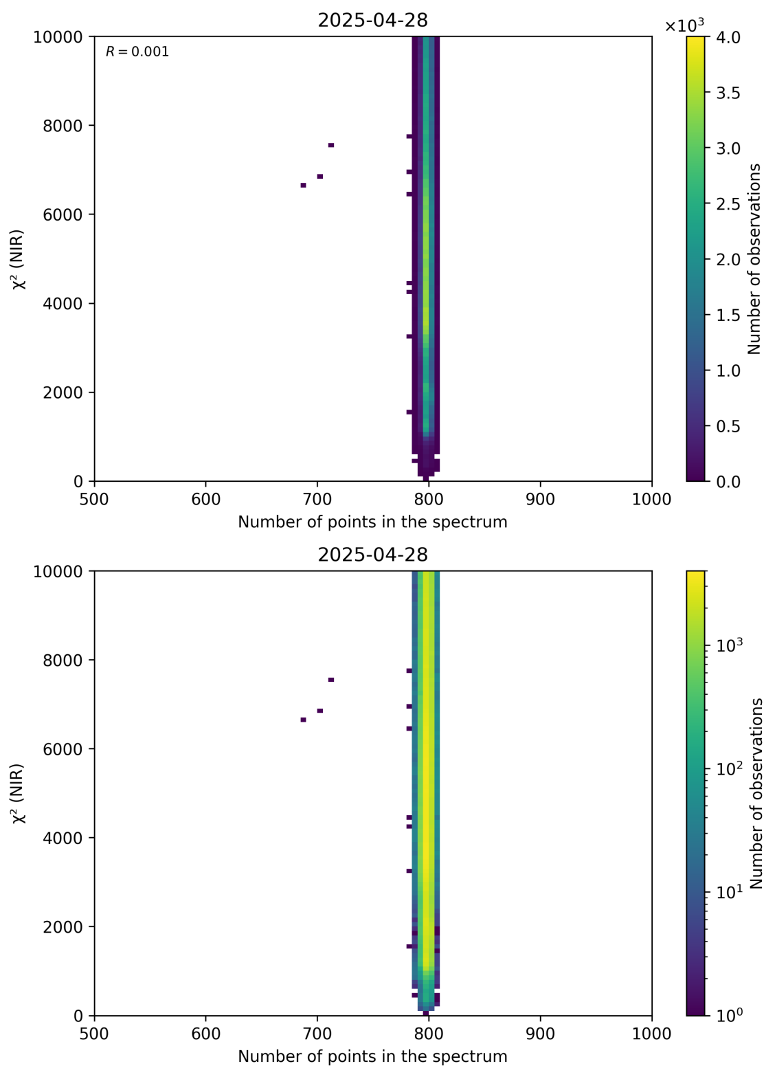
Figure 88: Scatter density plot of “Number of points in the spectrum” against “ \chi^2 (NIR)” for 2025-04-27 to 2025-04-29.
