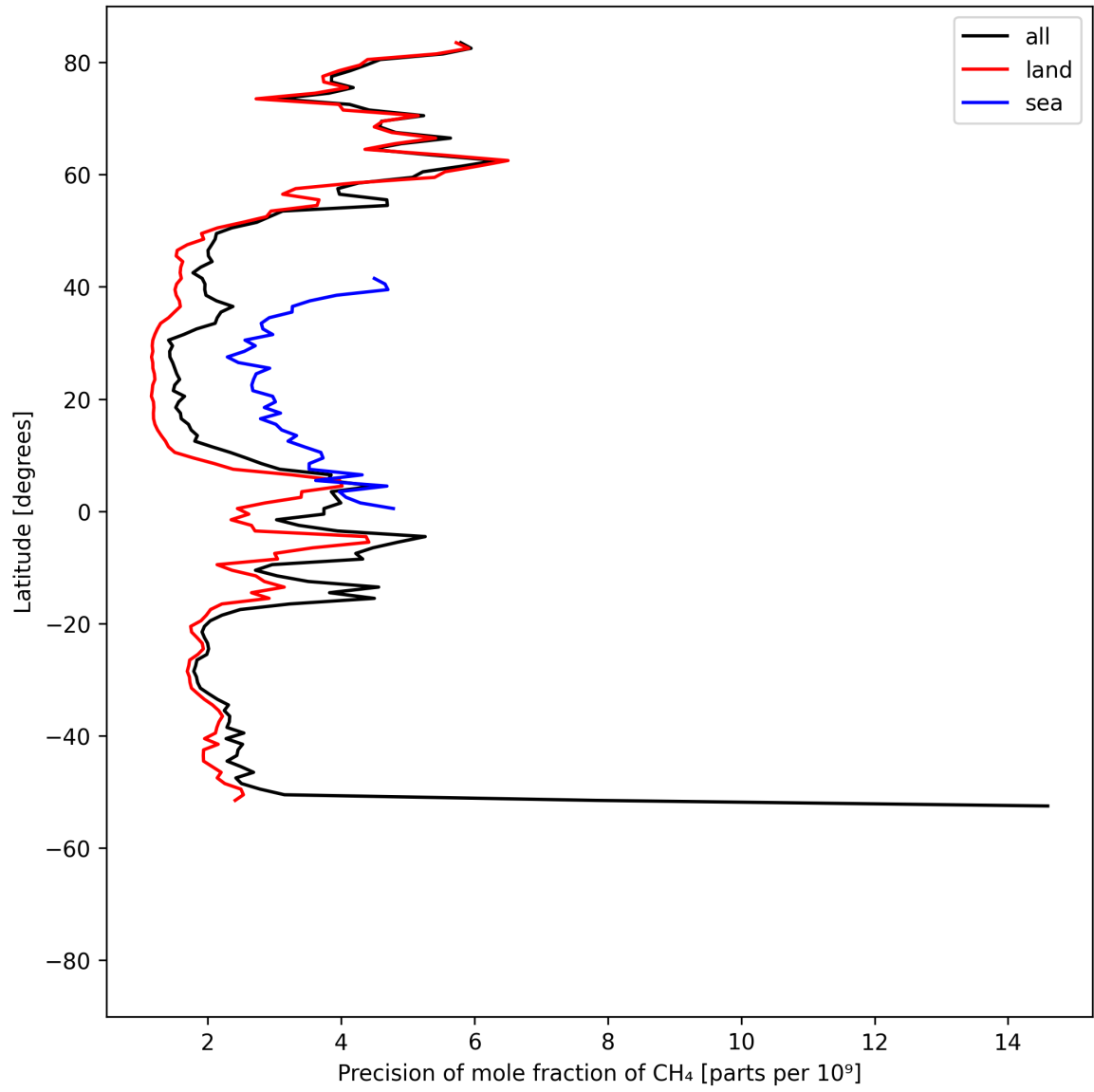
Figure 13: Zonal average of “Precision of mole fraction of CH 4 ” for 2025-04-27 to 2025-04-29.
