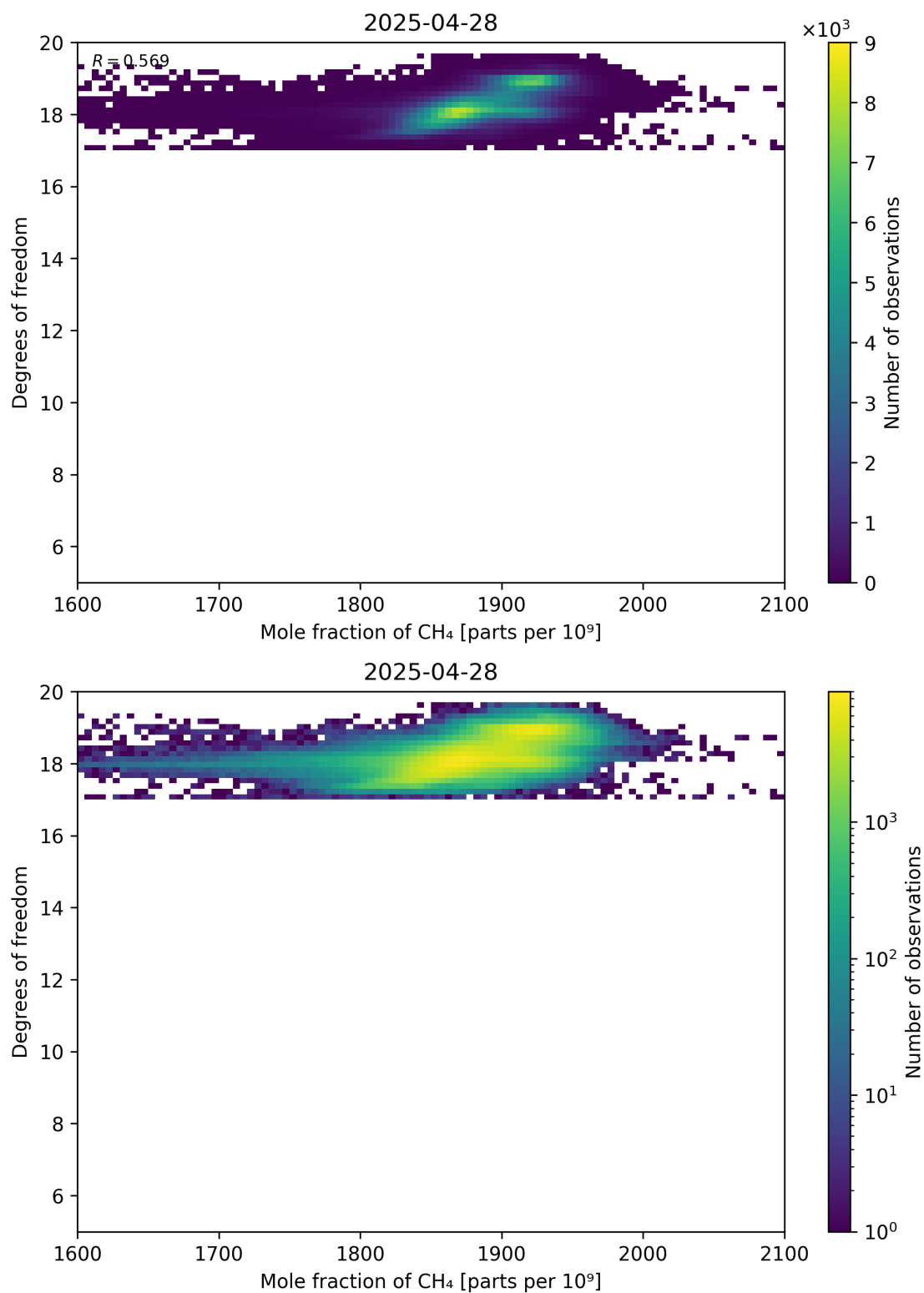
Figure 72: Scatter density plot of “Mole fraction of CH 4 ” against “Degrees of freedom” for 2025-04-27 to 2025-04-29.
