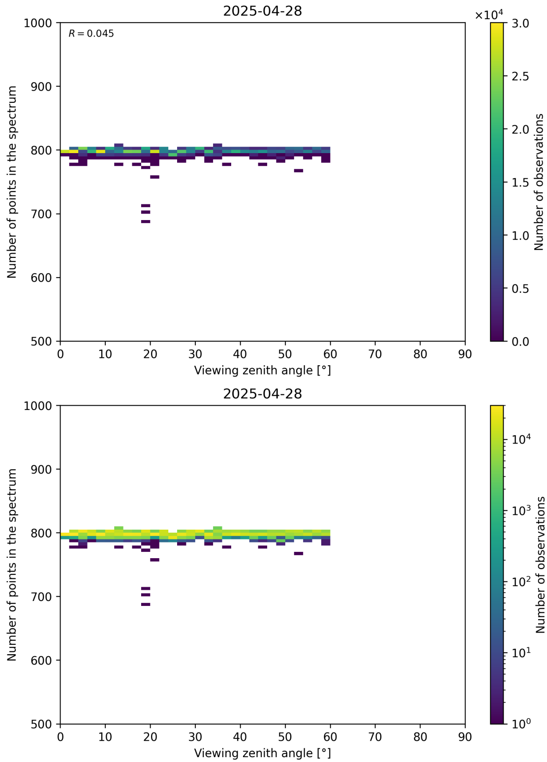
Figure 114: Scatter density plot of “Viewing zenith angle” against “Number of points in the spectrum” for 2025-04-27 to 2025-04-29.
