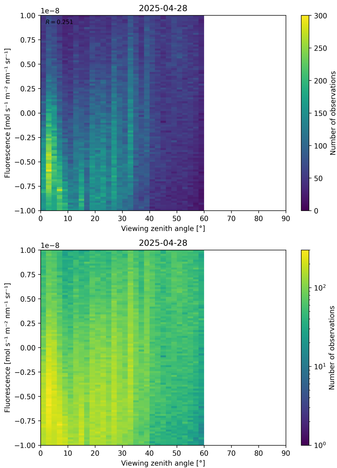
Figure 108: Scatter density plot of “Viewing zenith angle” against “Fluorescence” for 2025-04-27 to 2025-04-29.
