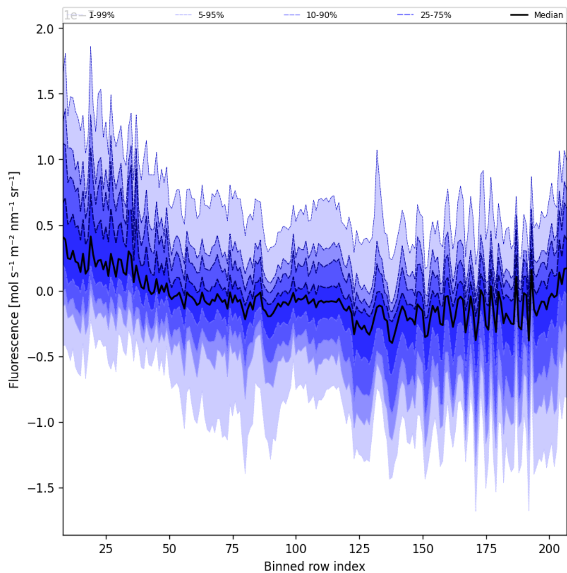
Figure 43: Along track statistics of “Fluorescence” for 2025-04-27 to 2025-04-29
