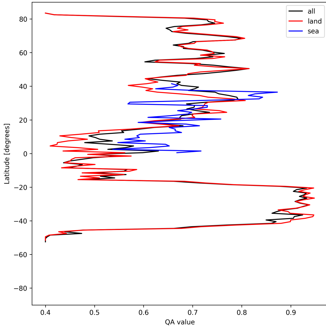
Figure 11: Zonal average of “QA value” for 2025-04-27 to 2025-04-29.
