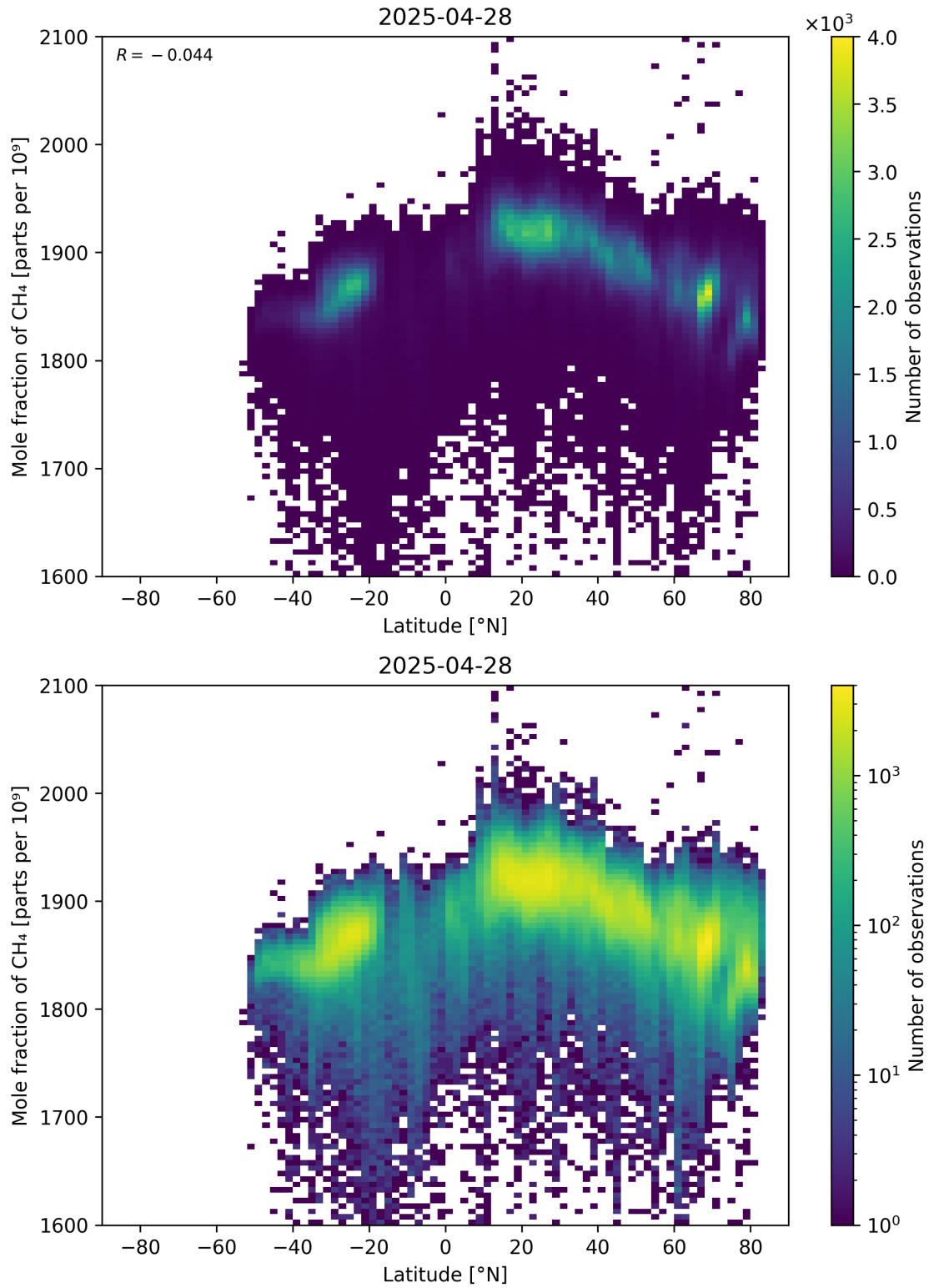
Figure 57: Scatter density plot of “Latitude” against “Mole fraction of CH 4 ” for 2025-04-27 to 2025-04-29.
