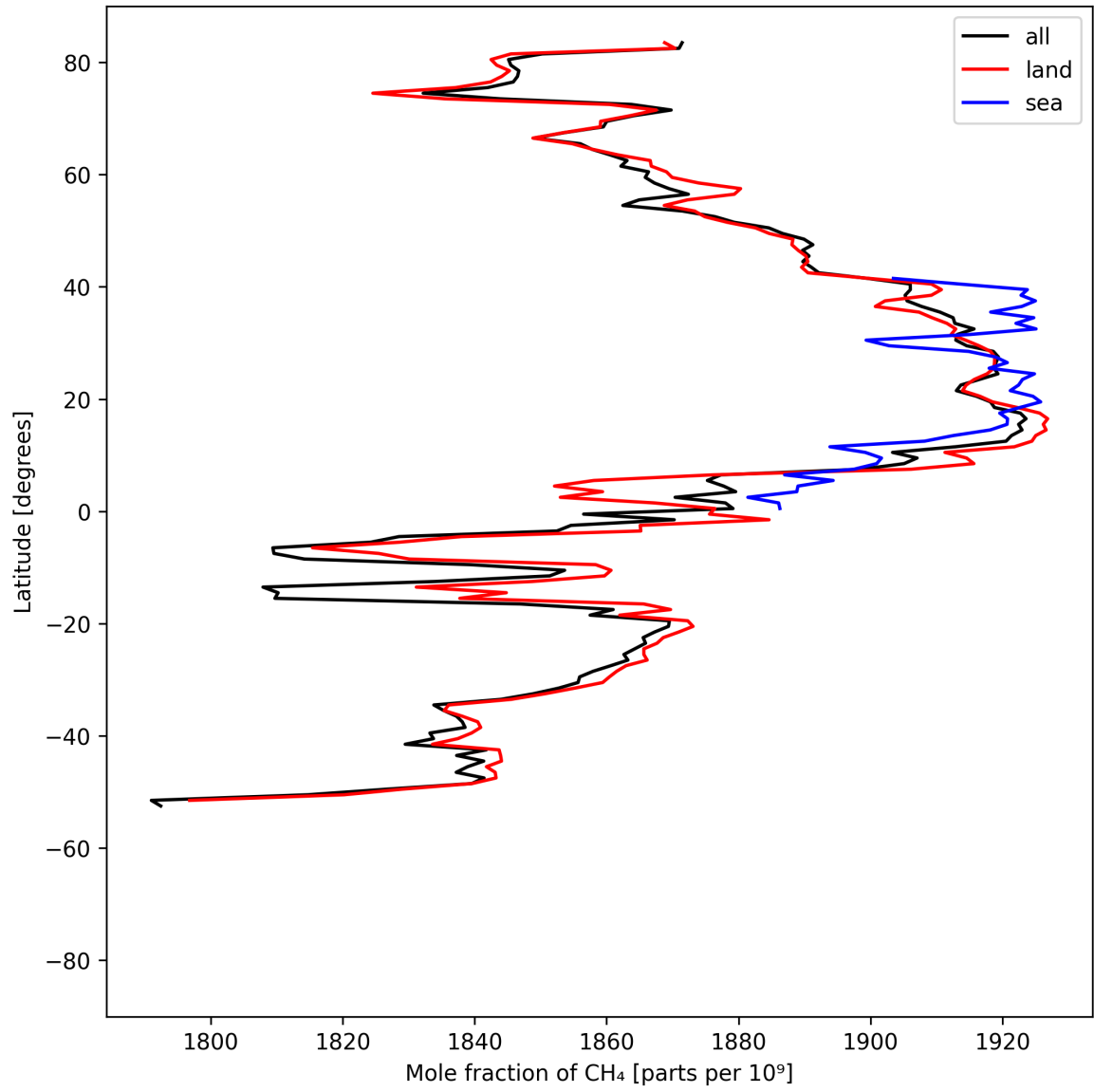
Figure 12: Zonal average of “Mole fraction of \text{CH}_4 ” for 2025-04-27 to 2025-04-29.
