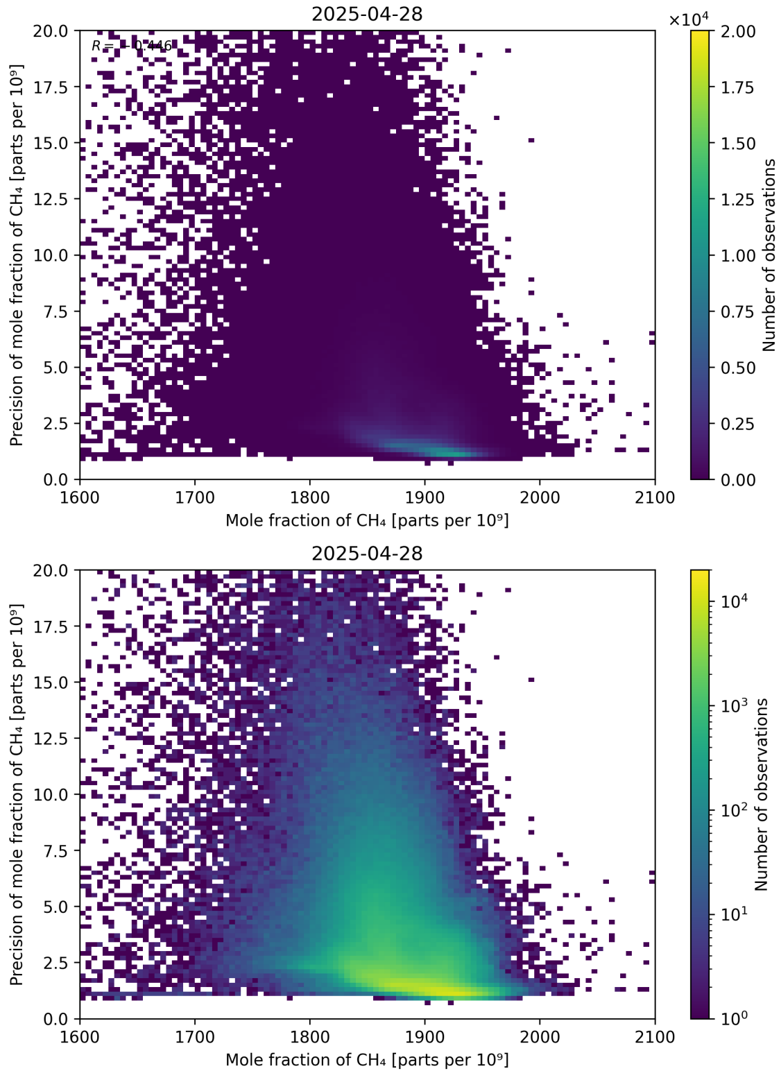
Figure 75: Scatter density plot of “Mole fraction of CH 4 ” against “Precision of mole fraction of CH 4 ” for 2025-04-27 to 2025-04-29.
