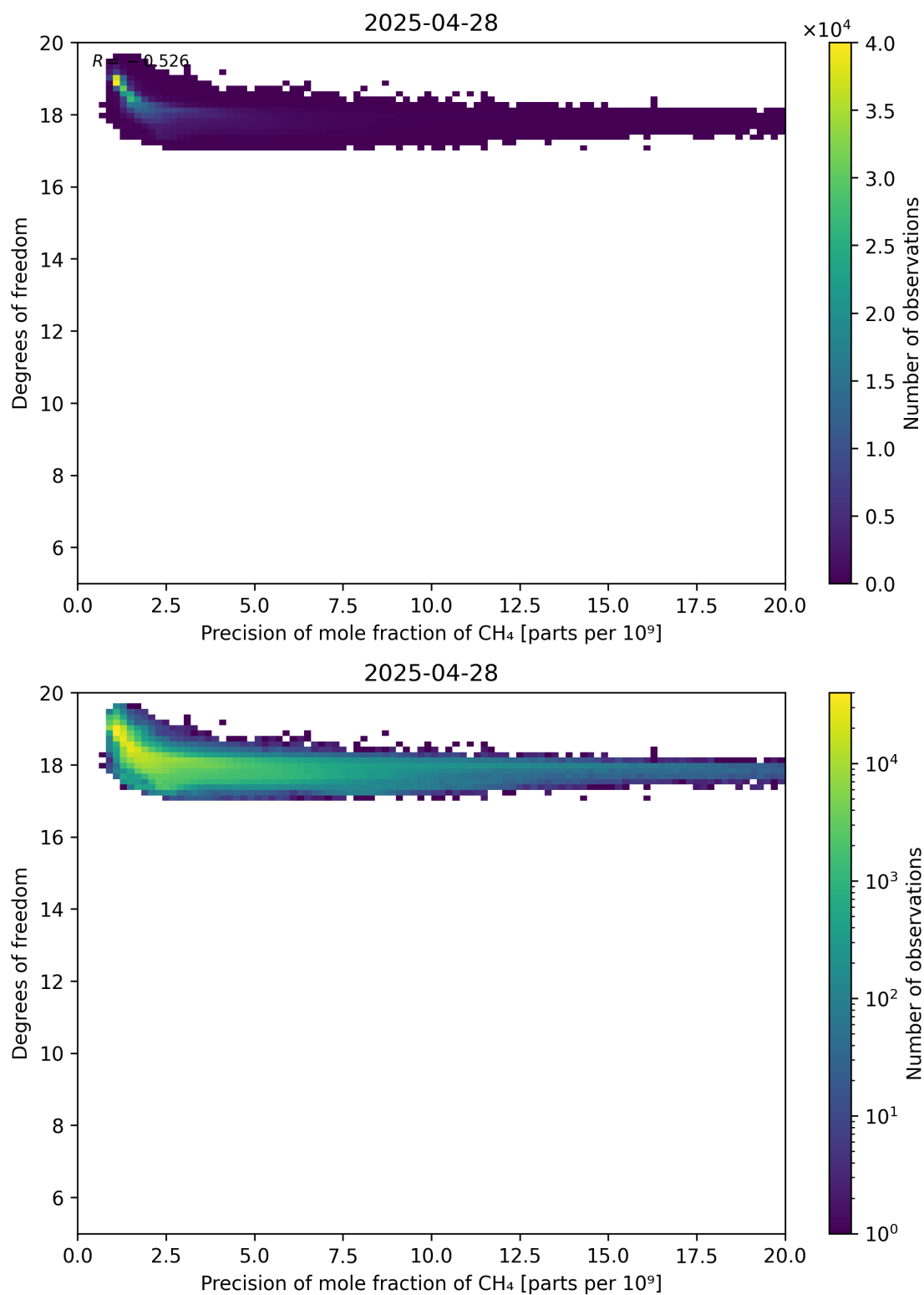
Figure 80: Scatter density plot of “Precision of mole fraction of CH 4 ” against “Degrees of freedom” for 2025-04-27 to 2025-04-29.
