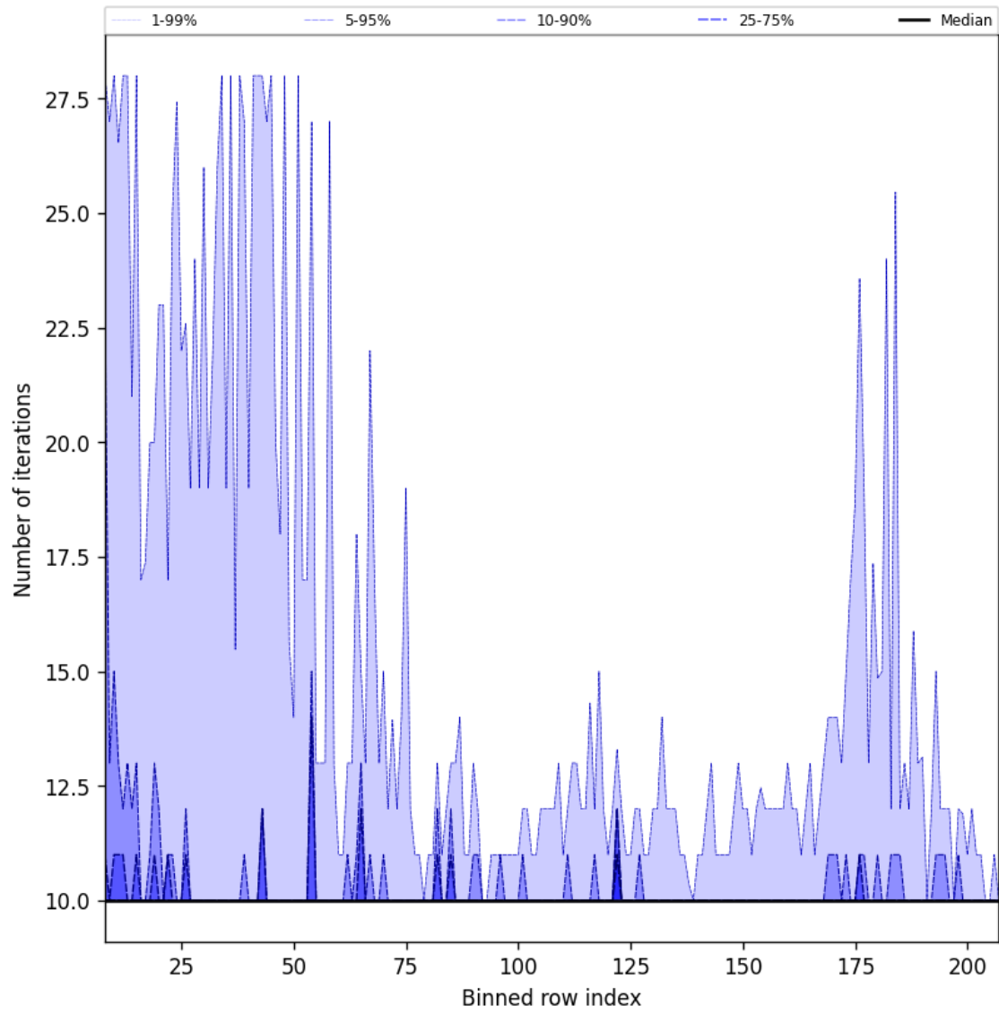
Figure 42: Along track statistics of “Number of iterations” for 2025-04-27 to 2025-04-29
