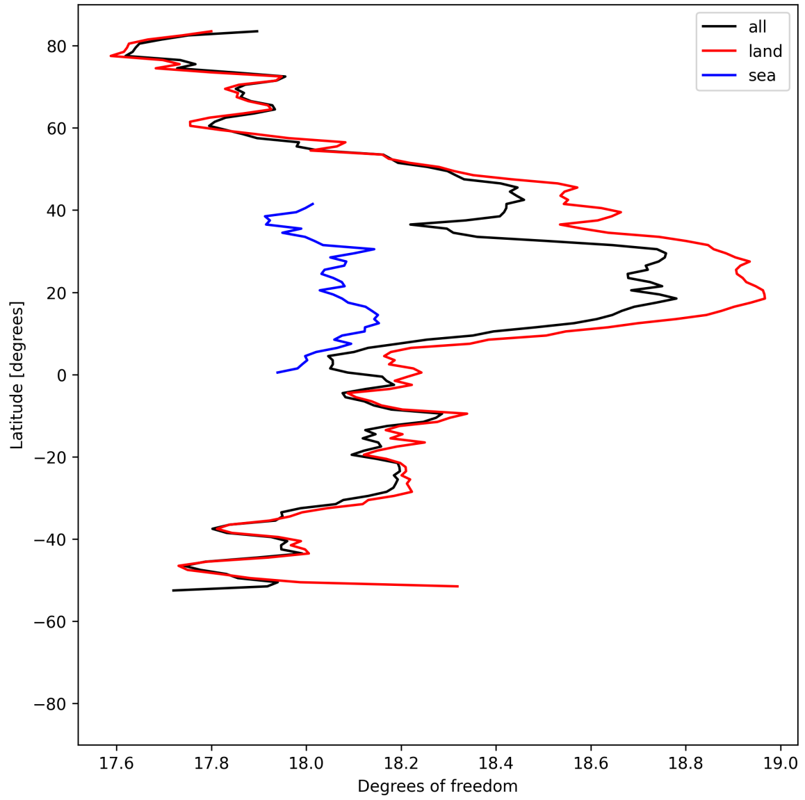
Figure 19: Zonal average of “Degrees of freedom” for 2025-04-27 to 2025-04-29.
