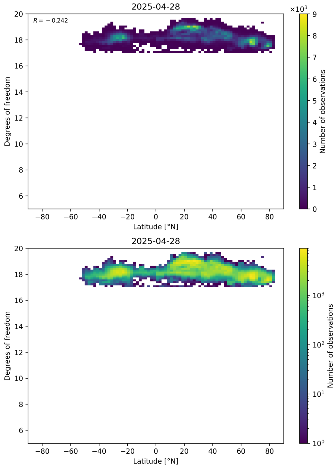
Figure 55: Scatter density plot of “Latitude” against “Degrees of freedom” for 2025-04-27 to 2025-04-29.
