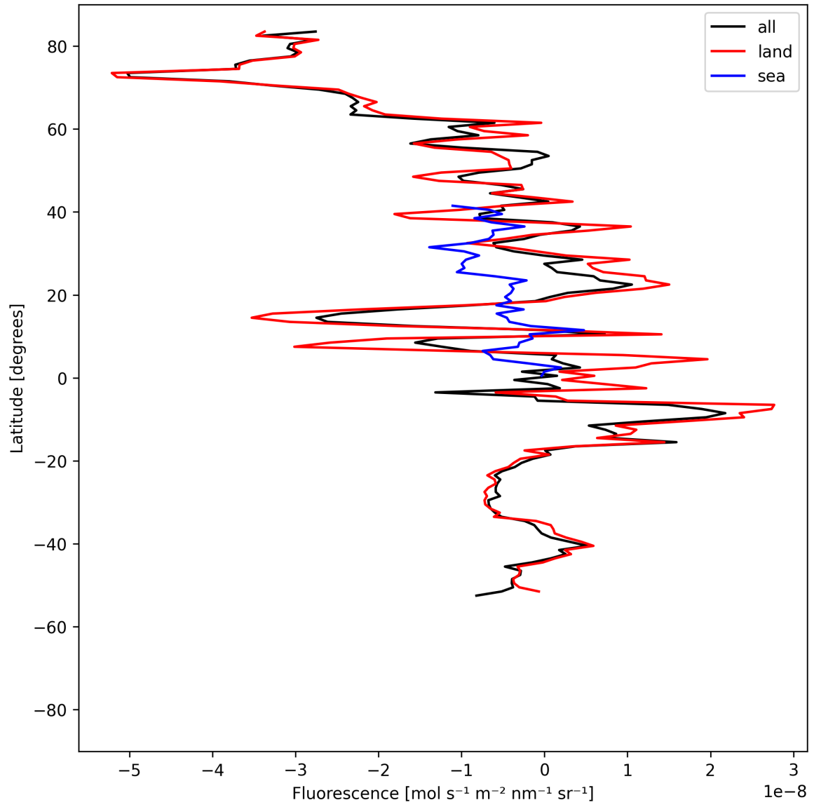
Figure 21: Zonal average of “Fluorescence” for 2025-04-27 to 2025-04-29.
