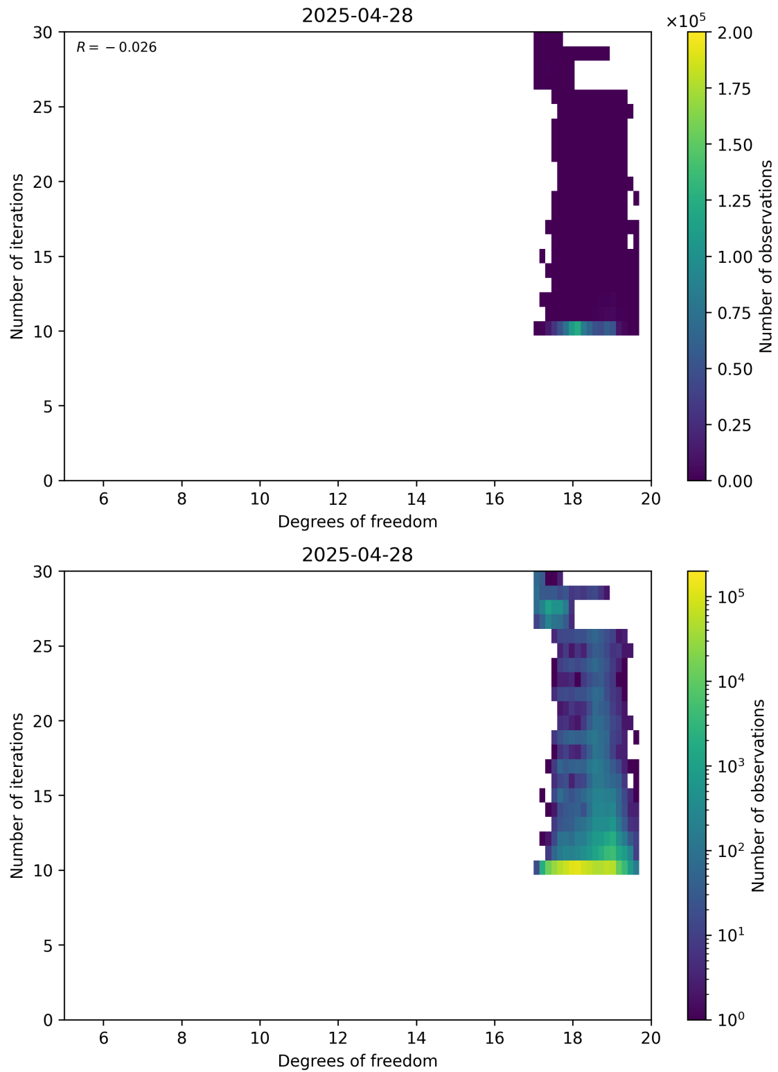
Figure 52: Scatter density plot of “Degrees of freedom” against “Number of iterations” for 2025-04-27 to 2025-04-29.
