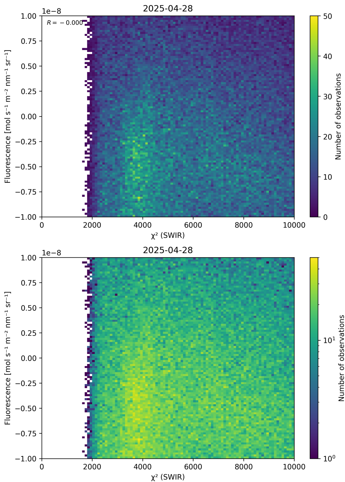
Figure 49: Scatter density plot of “ \chi^2 (SWIR)” against “Fluorescence” for 2025-04-27 to 2025-04-29.
