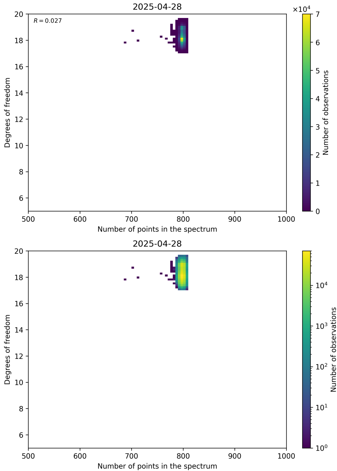
Figure 90: Scatter density plot of “Number of points in the spectrum” against “Degrees of freedom” for 2025-04-27 to 2025-04-29.
