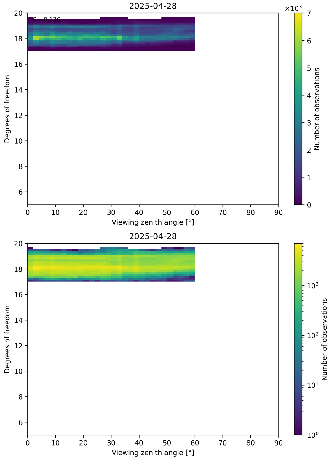
Figure 107: Scatter density plot of “Viewing zenith angle” against “Degrees of freedom” for 2025-04-27 to 2025-04-29.
