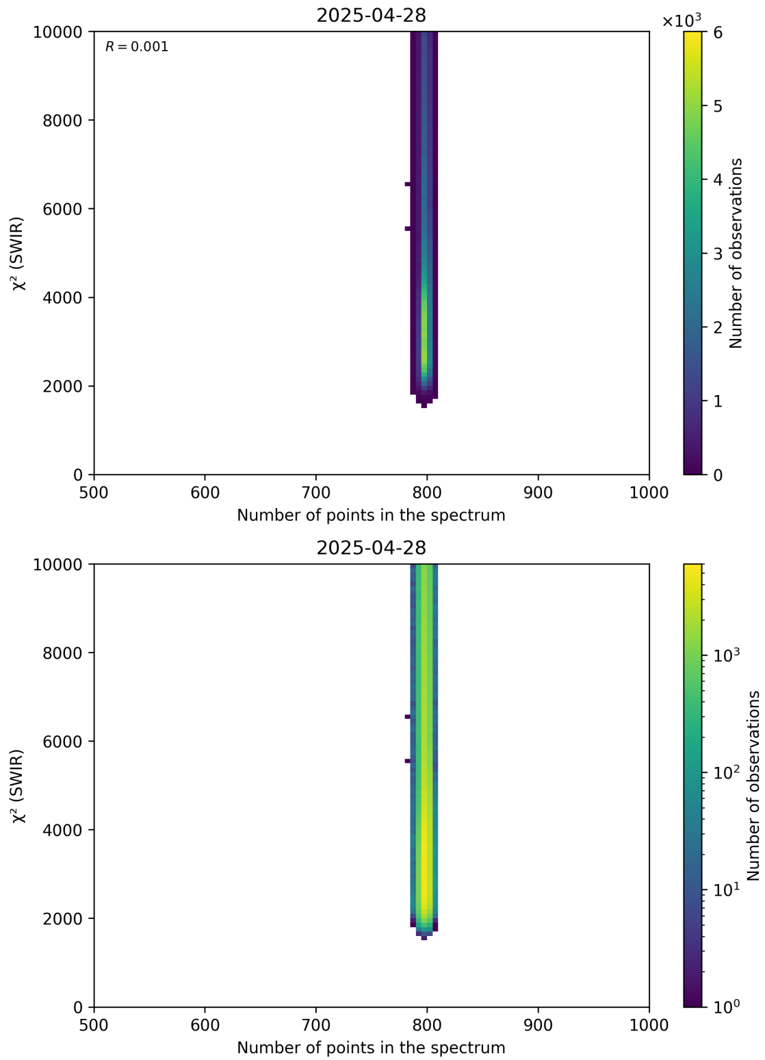
Figure 89: Scatter density plot of “Number of points in the spectrum” against “ \chi^2 (SWIR)” for 2025-04-27 to 2025-04-29.
