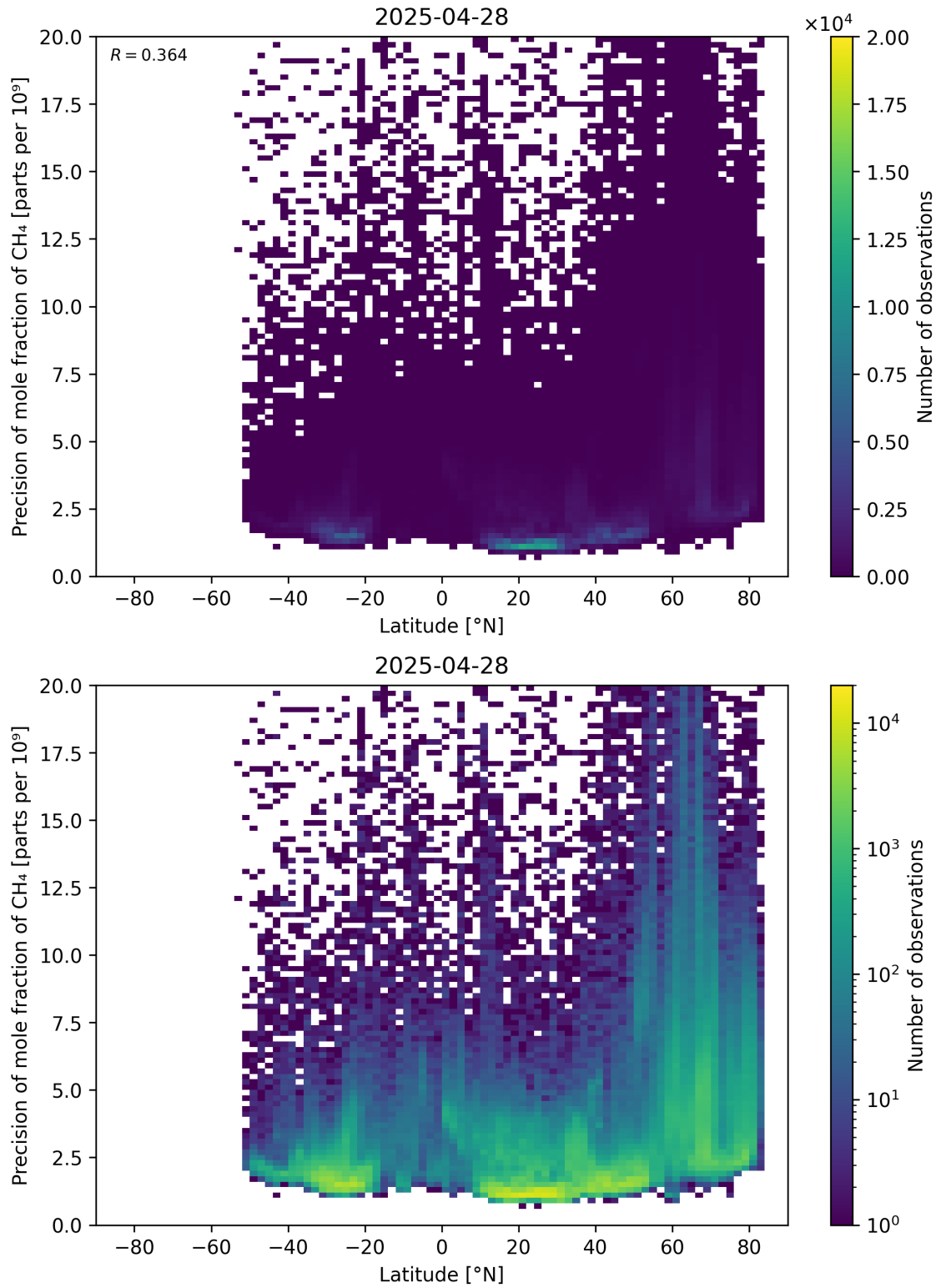
Figure 59: Scatter density plot of “Latitude” against “Precision of mole fraction of \text{CH}_4 ” for 2025-04-27 to 2025-04-29.
