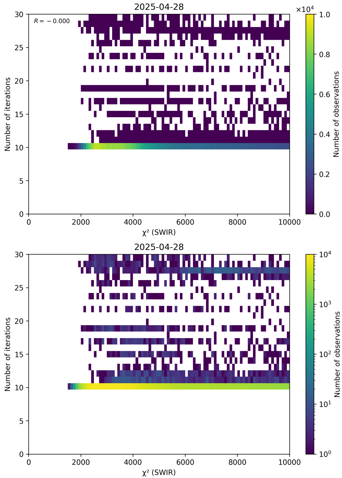
Figure 50: Scatter density plot of “ \chi^2 (SWIR)” against “Number of iterations” for 2025-04-27 to 2025-04-29.
