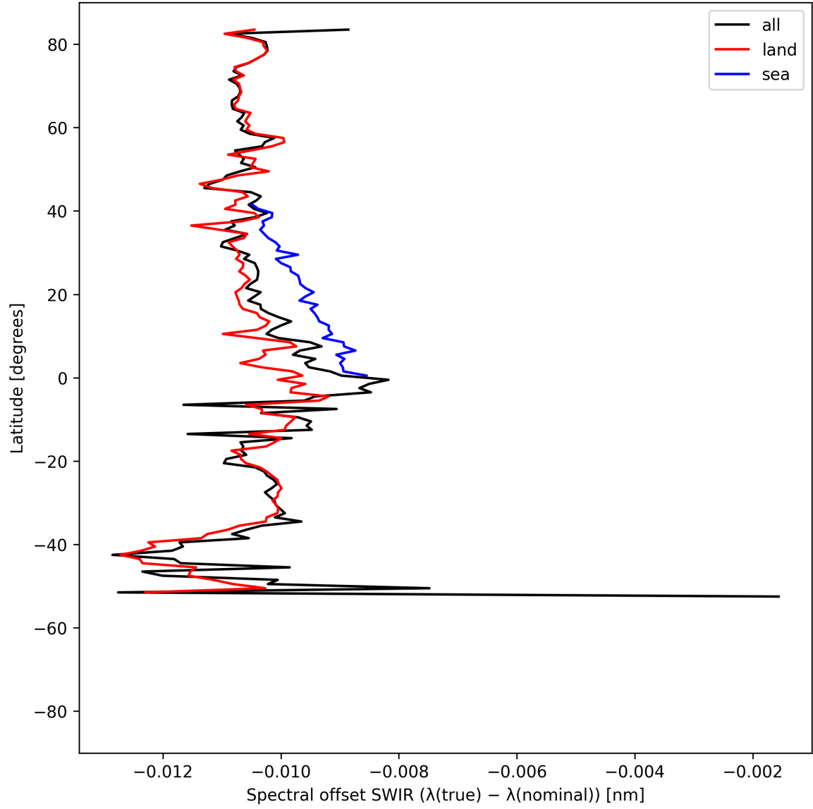
Figure 16: Zonal average of “Spectral offset SWIR ( \lambda_{\text{true}} - \lambda_{\text{nominal}} )” for 2025-04-27 to 2025-04-29.
