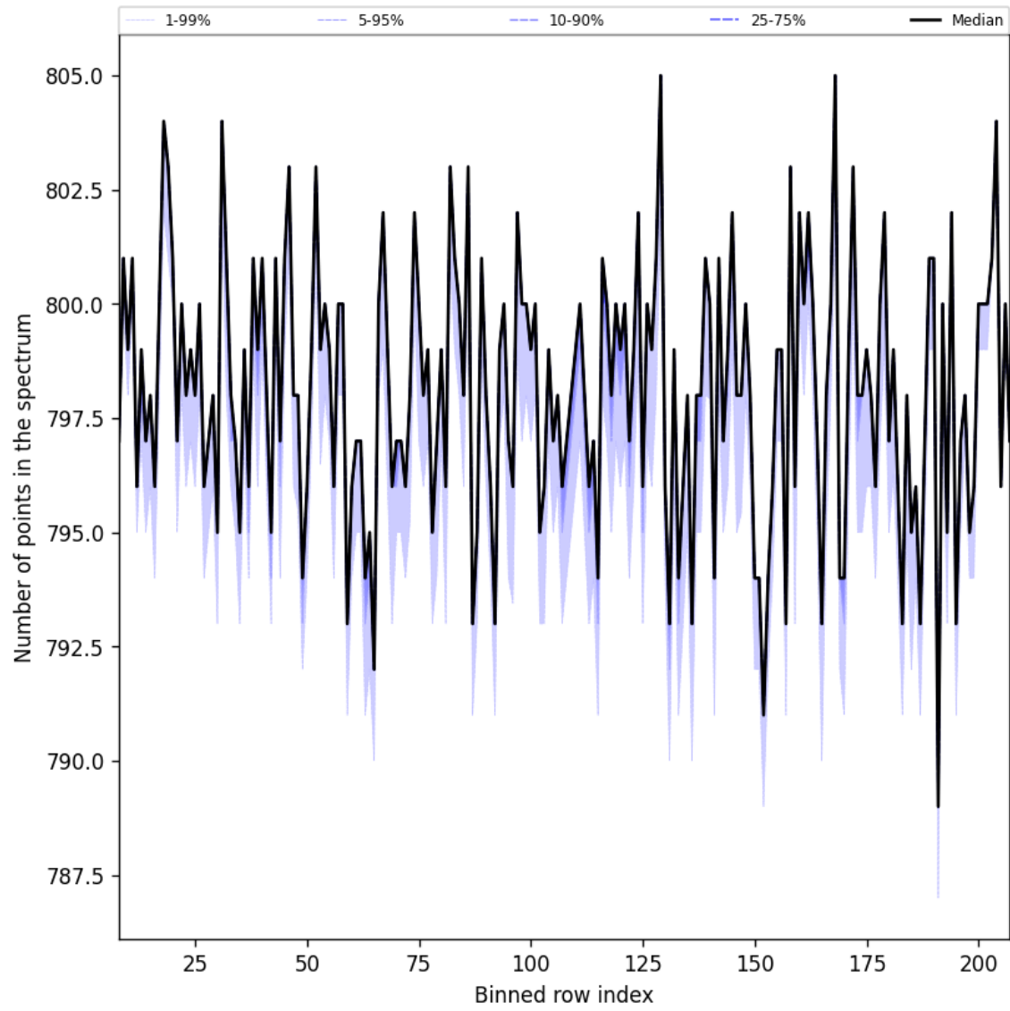
Figure 37: Along track statistics of “Number of points in the spectrum” for 2025-04-27 to 2025-04-29
