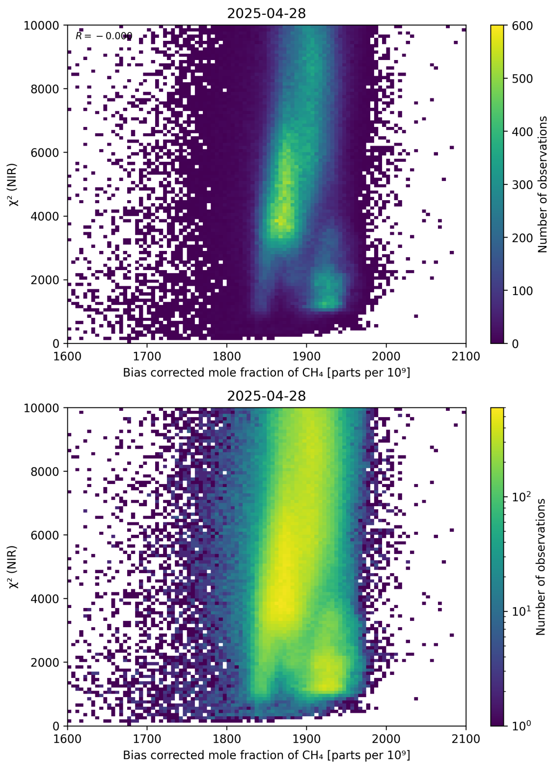
Figure 63: Scatter density plot of “Bias corrected mole fraction of CH 4 ” against “ \chi^2 (NIR)” for 2025-04-27 to 2025-04-29.
