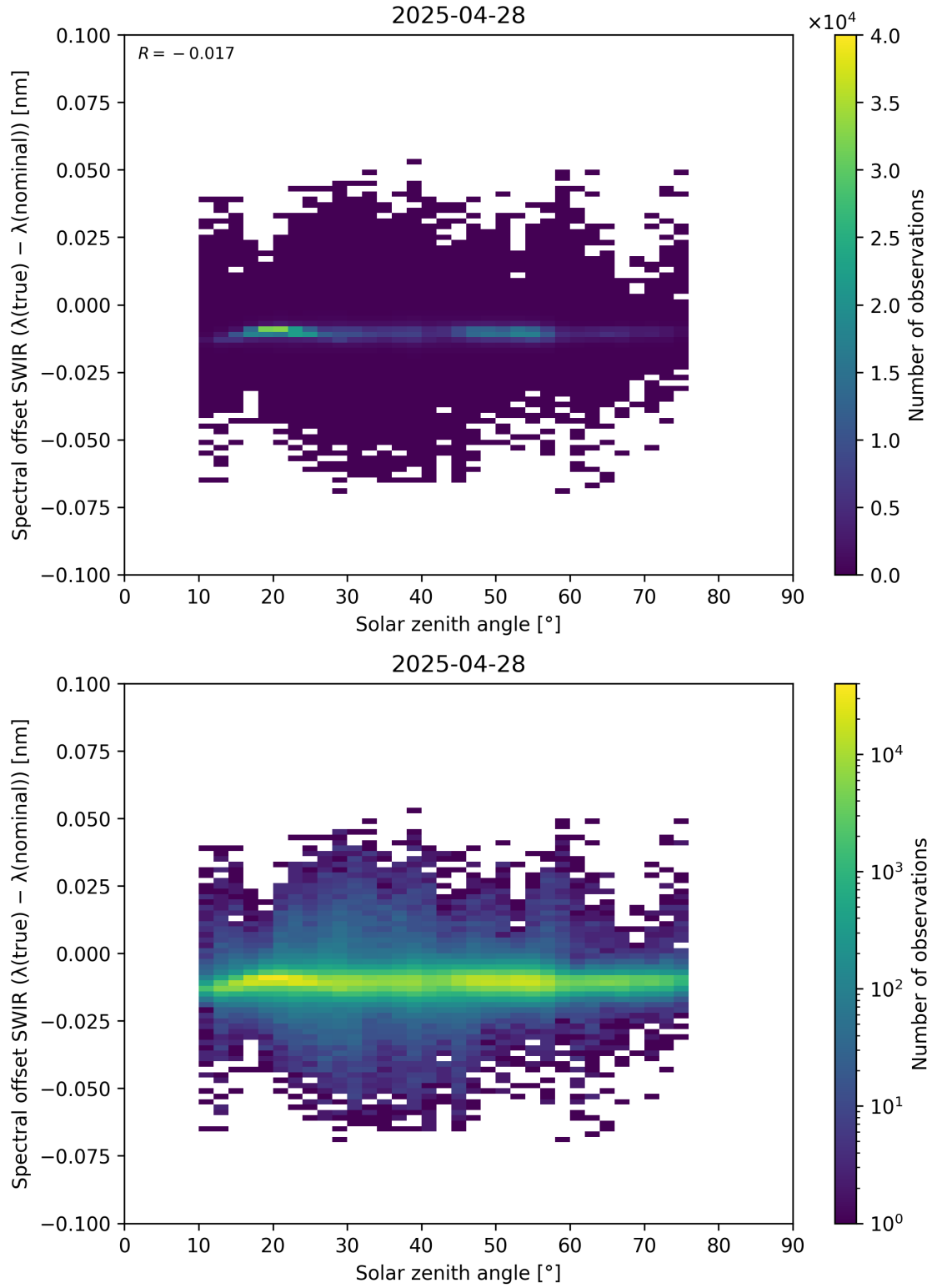
Figure 104: Scatter density plot of “Solar zenith angle” against “Spectral offset SWIR ( \lambda_{\text{true}} - \lambda_{\text{nominal}} )” for 2025-04-27 to 2025-04-29.
