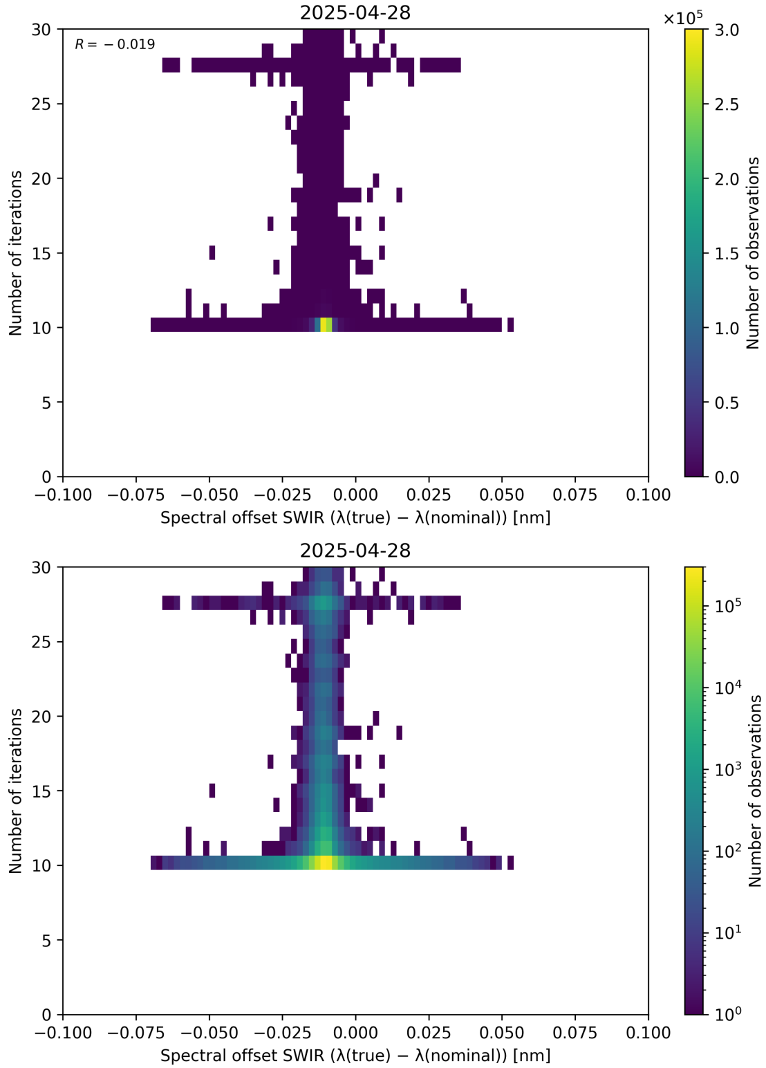
Figure 121: Scatter density plot of “Spectral offset SWIR ( \lambda_{\text{true}} - \lambda_{\text{nominal}} )” against “Number of iterations” for 2025-04-27 to 2025-04-29.
