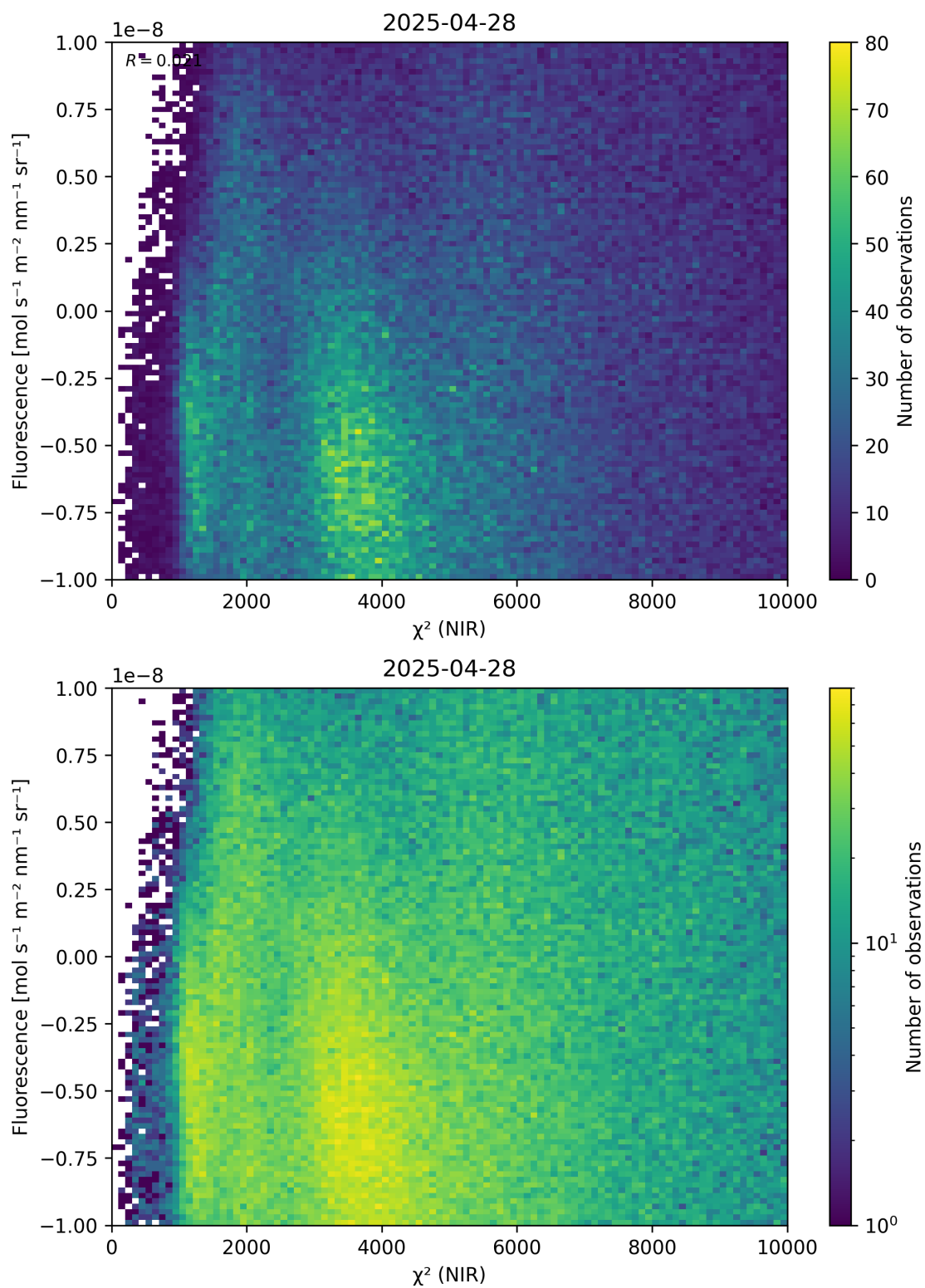
Figure 45: Scatter density plot of “ \chi^2 (NIR)” against “Fluorescence” for 2025-04-27 to 2025-04-29.
