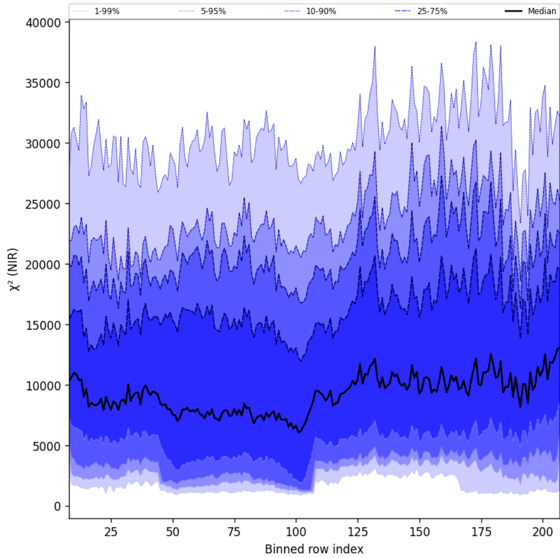
Figure 40: Along track statistics of “ \chi^2 (NIR)” for 2025-04-27 to 2025-04-29
