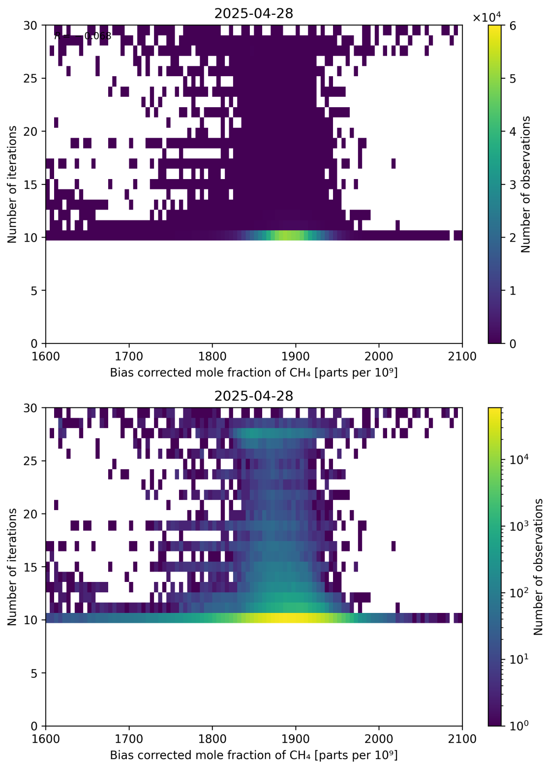
Figure 67: Scatter density plot of “Bias corrected mole fraction of CH 4 ” against “Number of iterations” for 2025-04-27 to 2025-04-29.
