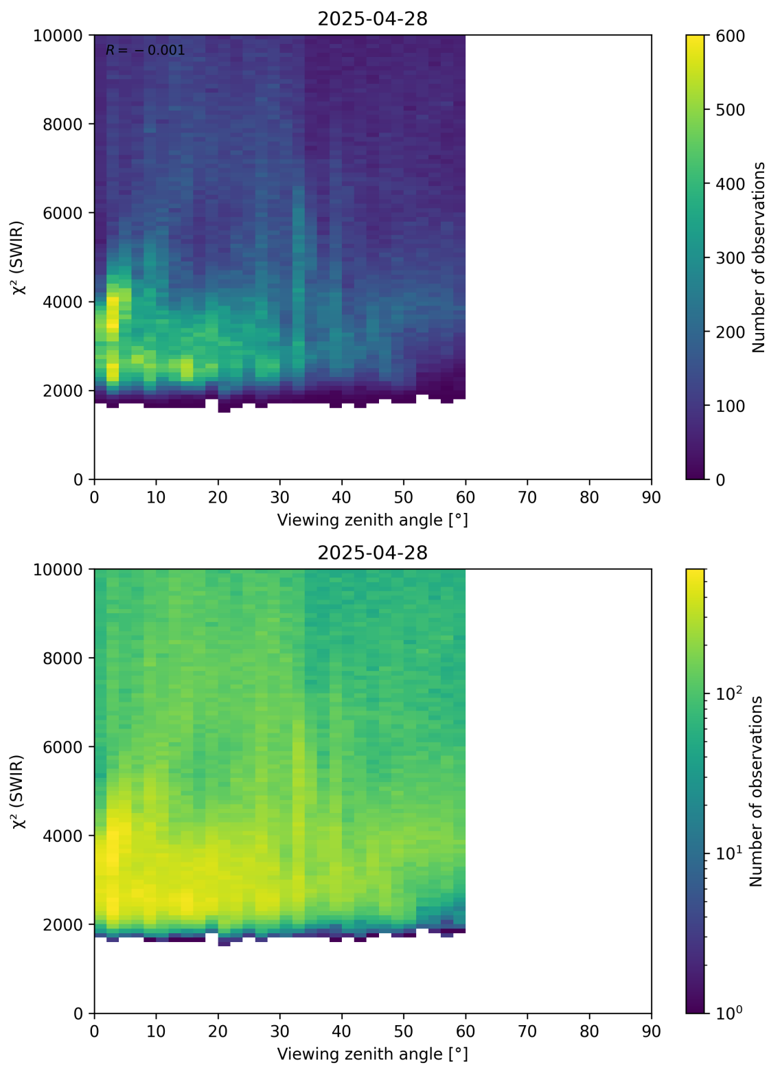
Figure 106: Scatter density plot of “Viewing zenith angle” against “ \chi^2 (SWIR)” for 2025-04-27 to 2025-04-29.
