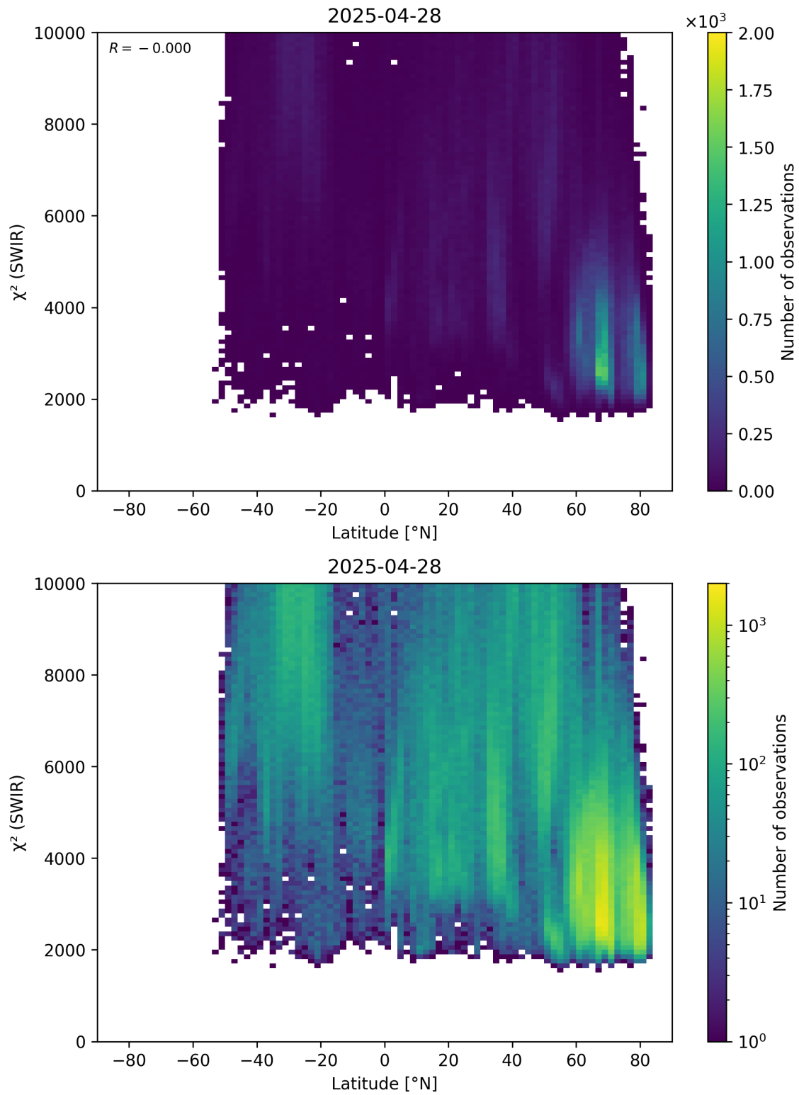
Figure 54: Scatter density plot of “Latitude” against “ \chi^2 (SWIR)” for 2025-04-27 to 2025-04-29.
