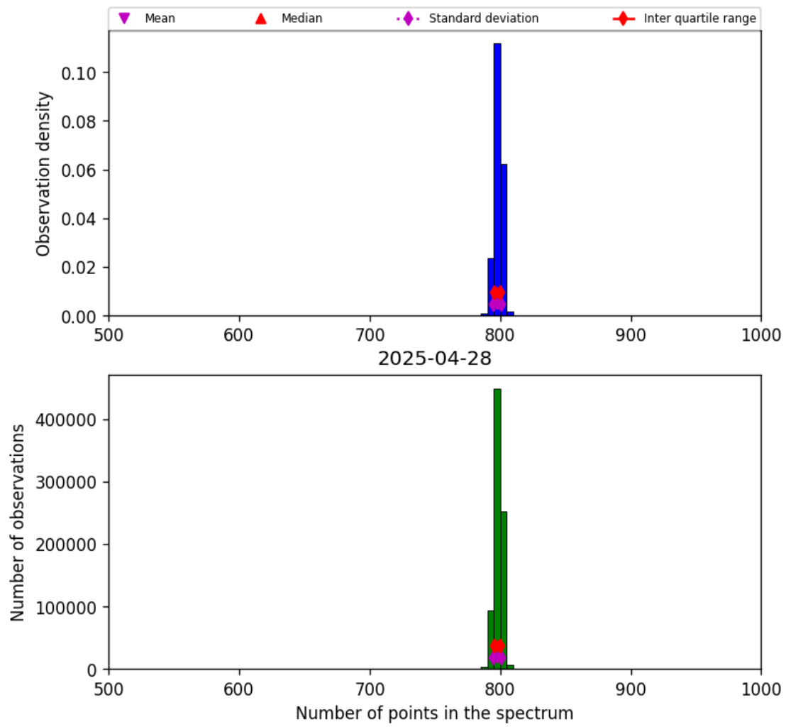
Figure 26: Histogram of “Number of points in the spectrum” for 2025-04-27 to 2025-04-29
