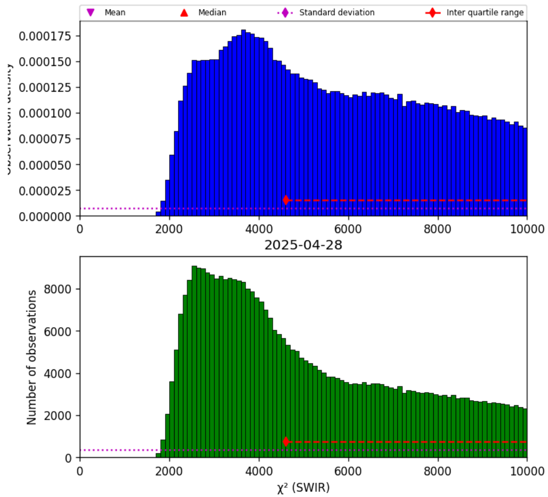
Figure 28: Histogram of “ \chi^2 (SWIR)” for 2025-04-27 to 2025-04-29
