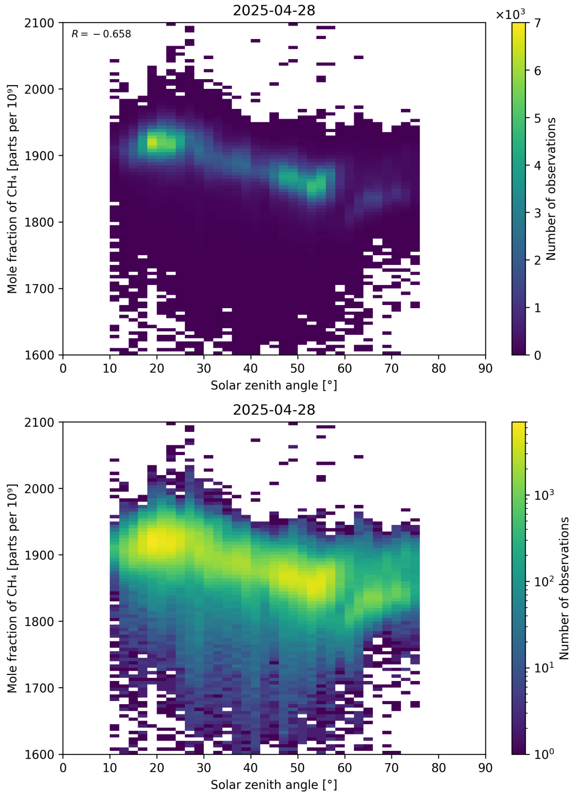
Figure 99: Scatter density plot of “Solar zenith angle” against “Mole fraction of \text{CH}_4 ” for 2025-04-27 to 2025-04-29.
