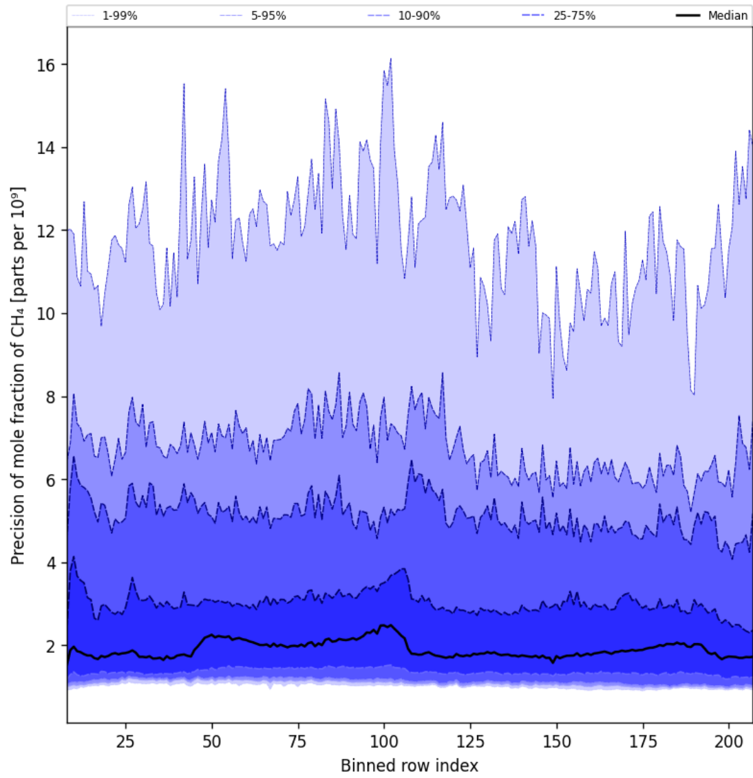
Figure 35: Along track statistics of “Precision of mole fraction of CH 4 ” for 2025-04-27 to 2025-04-29
