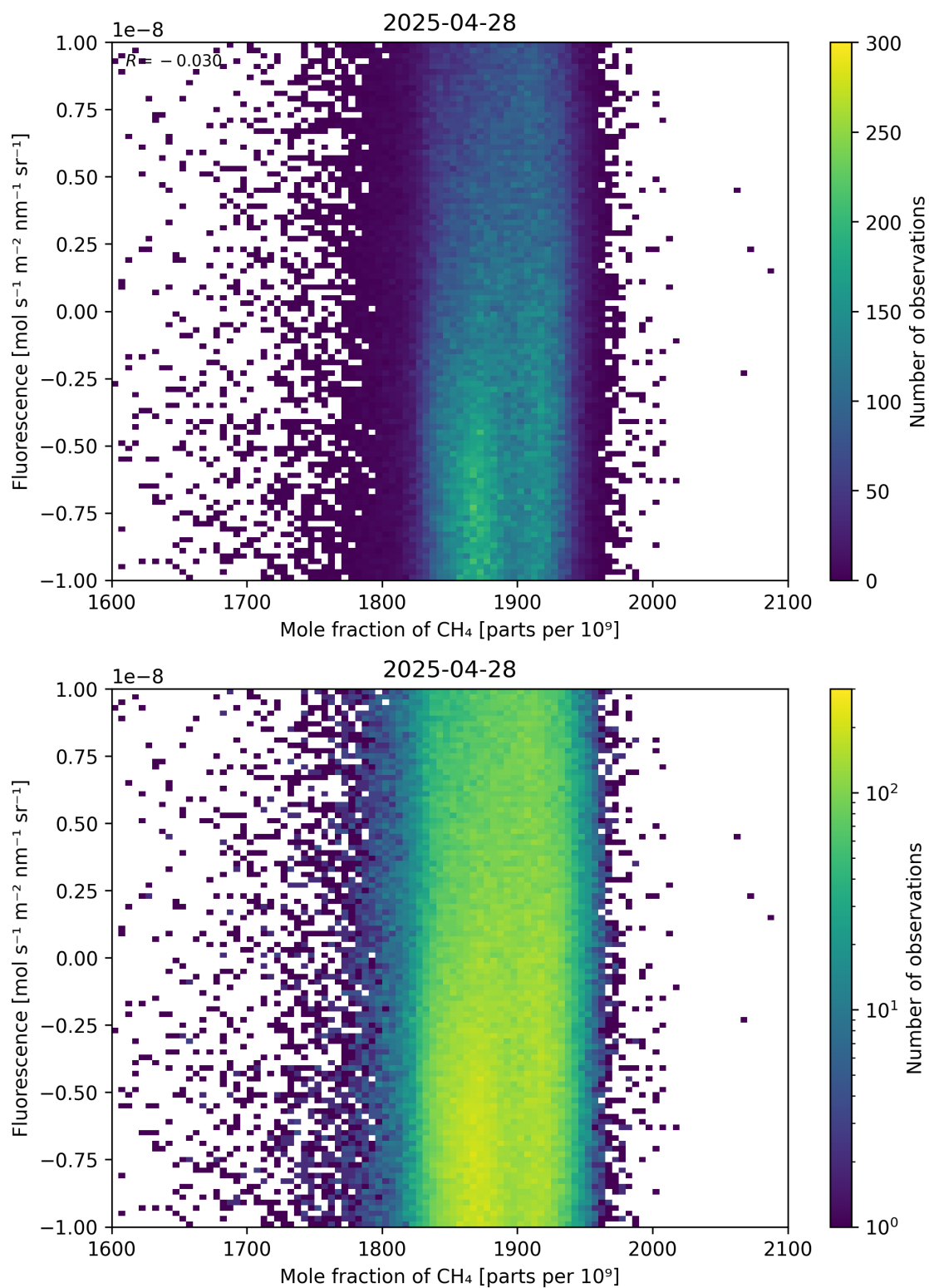
Figure 73: Scatter density plot of “Mole fraction of \text{CH}_4 ” against “Fluorescence” for 2025-04-27 to 2025-04-29.
