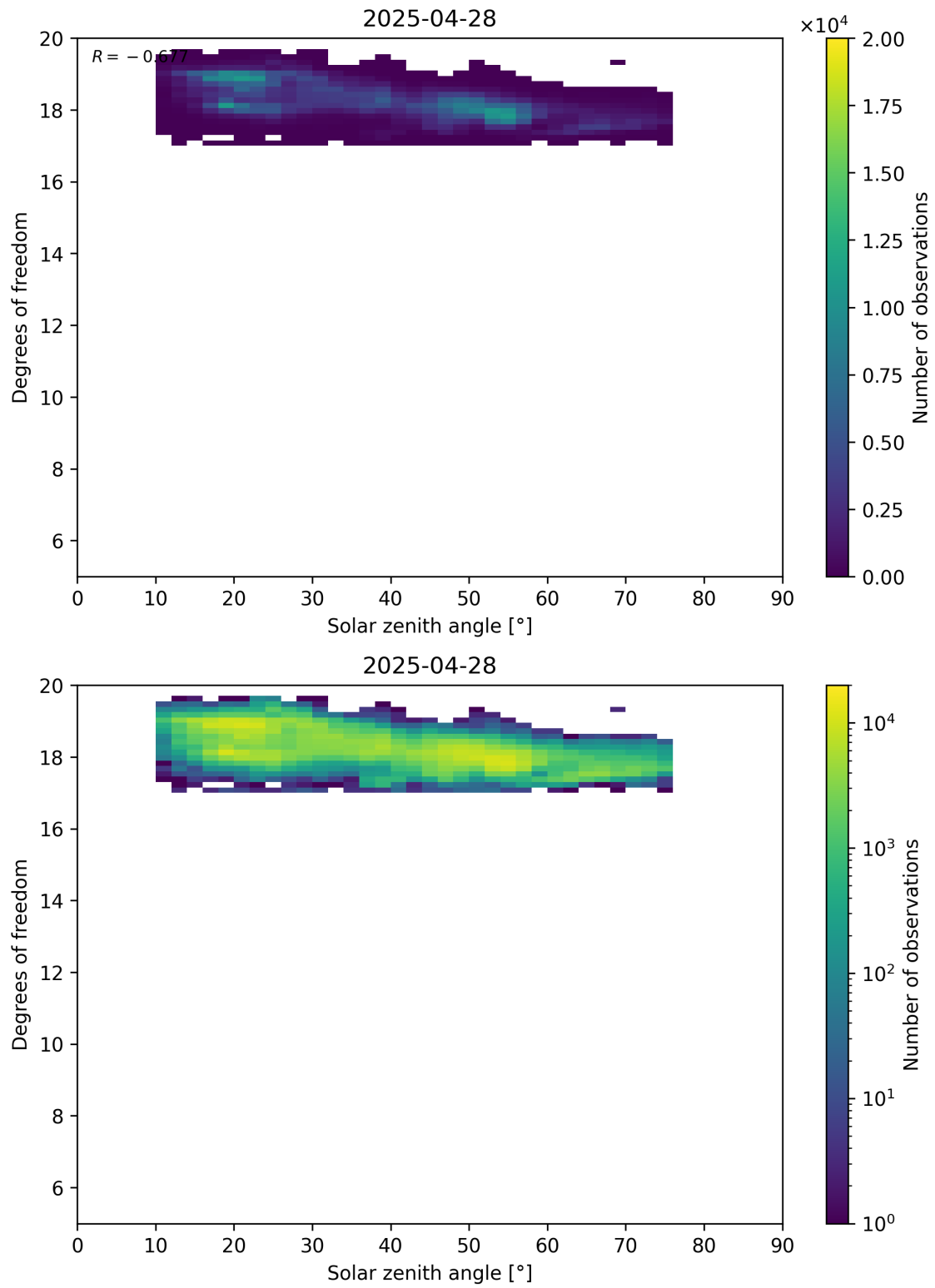
Figure 96: Scatter density plot of “Solar zenith angle” against “Degrees of freedom” for 2025-04-27 to 2025-04-29.
