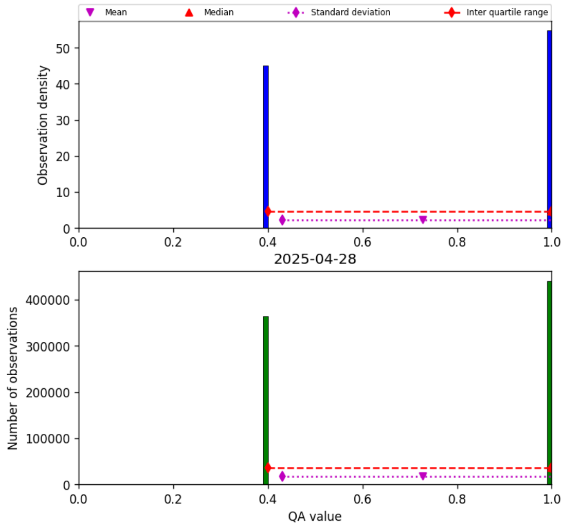
Figure 22: Histogram of “QA value” for 2025-04-27 to 2025-04-29
