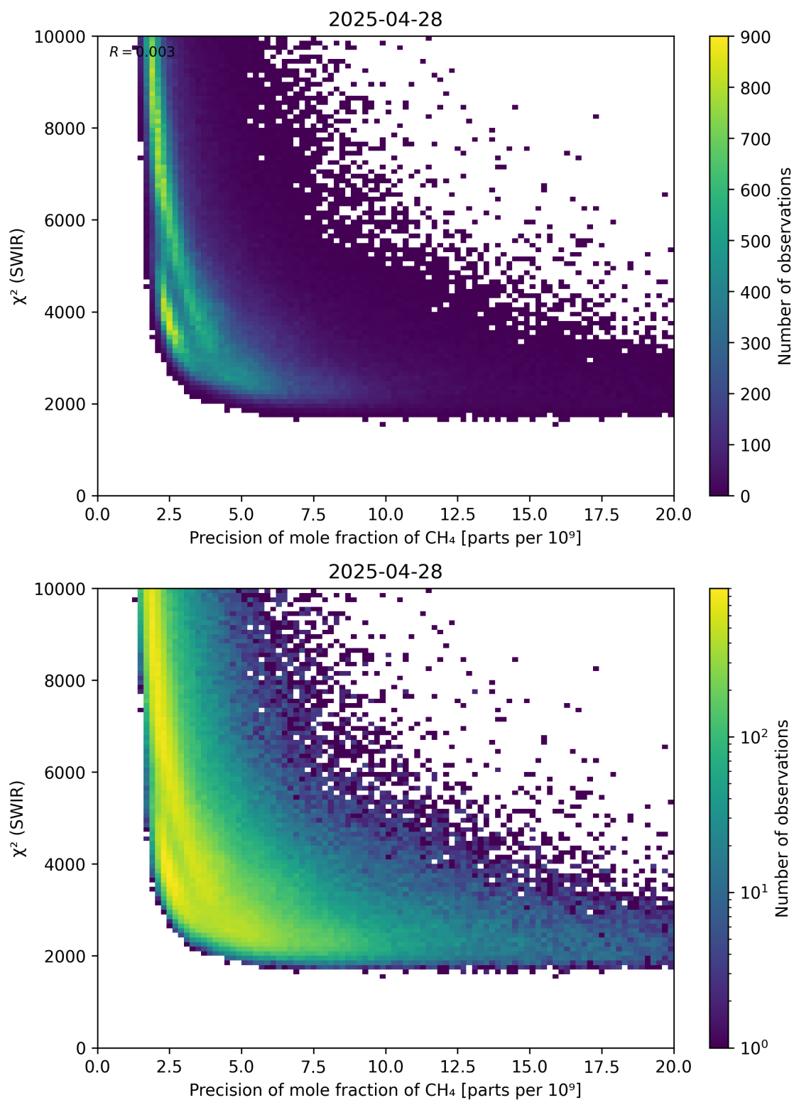
Figure 79: Scatter density plot of “Precision of mole fraction of \text{CH}_4 ” against “ \chi^2 (SWIR)” for 2025-04-27 to 2025-04-29.
