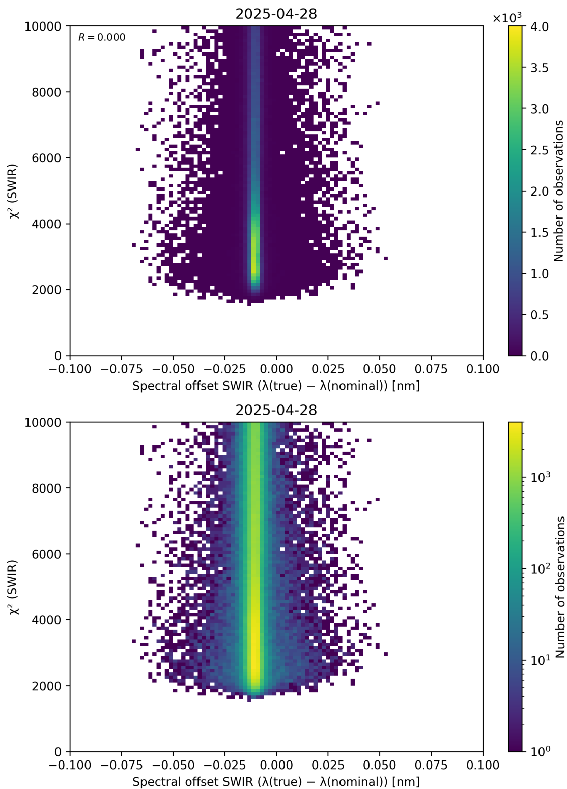
Figure 118: Scatter density plot of “Spectral offset SWIR ( \lambda_{\text{true}} - \lambda_{\text{nominal}} )” against “ \chi^2 (SWIR)” for 2025-04-27 to 2025-04-29.
