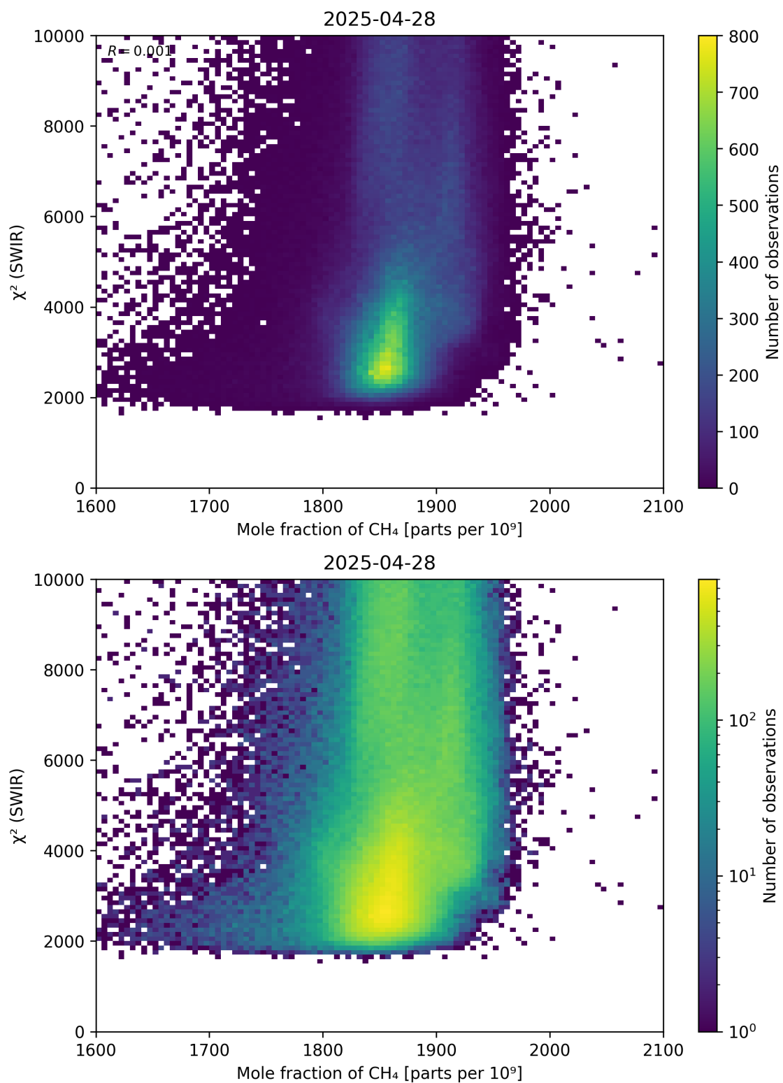
Figure 71: Scatter density plot of “Mole fraction of \text{CH}_4 ” against “ \chi^2 (SWIR)” for 2025-04-27 to 2025-04-29.
