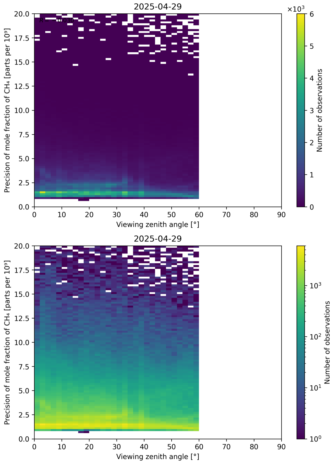
Figure 112: Scatter density plot of “Viewing zenith angle” against “Precision of mole fraction of CH 4 ” for 2025-04-29 to 2025-04-30.
