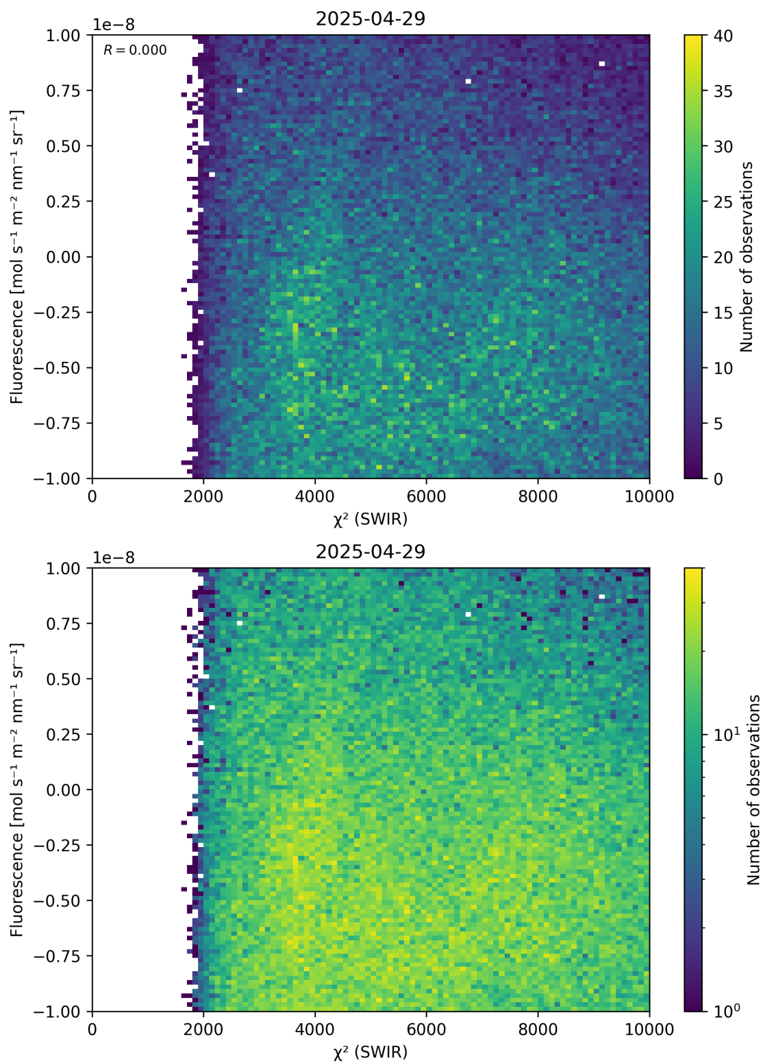
Figure 49: Scatter density plot of “ \chi^2 (SWIR)” against “Fluorescence” for 2025-04-29 to 2025-04-30.
