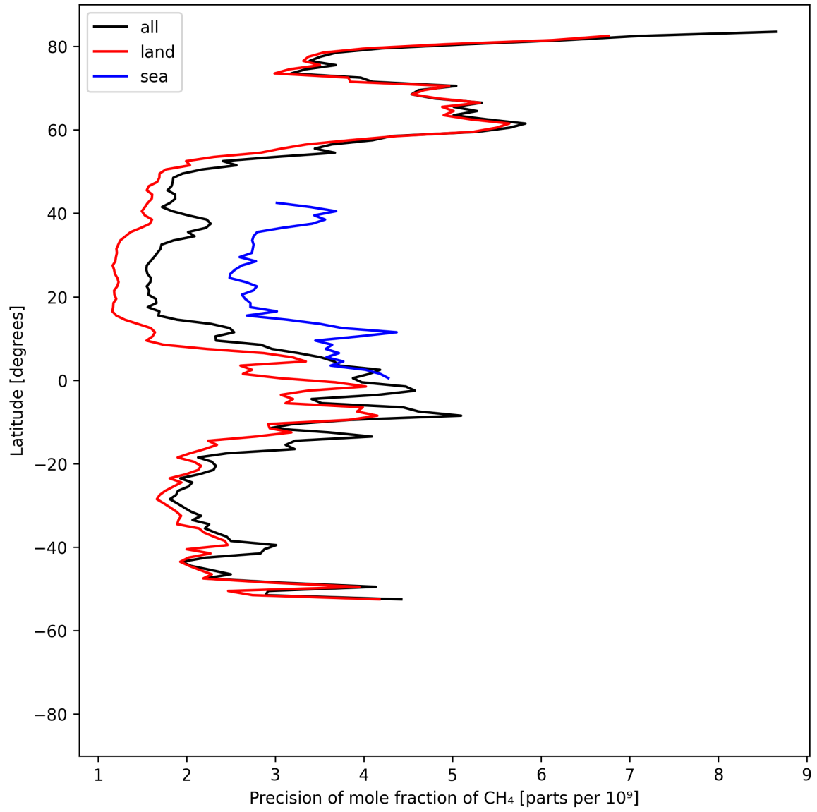
Figure 13: Zonal average of “Precision of mole fraction of CH 4 ” for 2025-04-29 to 2025-04-30.
