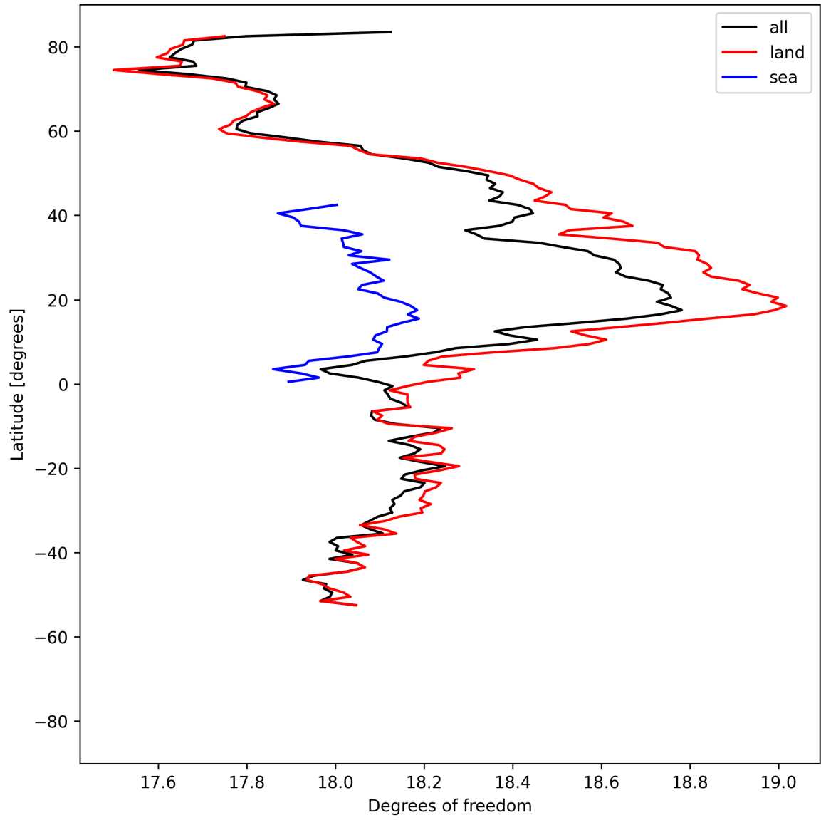
Figure 19: Zonal average of “Degrees of freedom” for 2025-04-29 to 2025-04-30.
