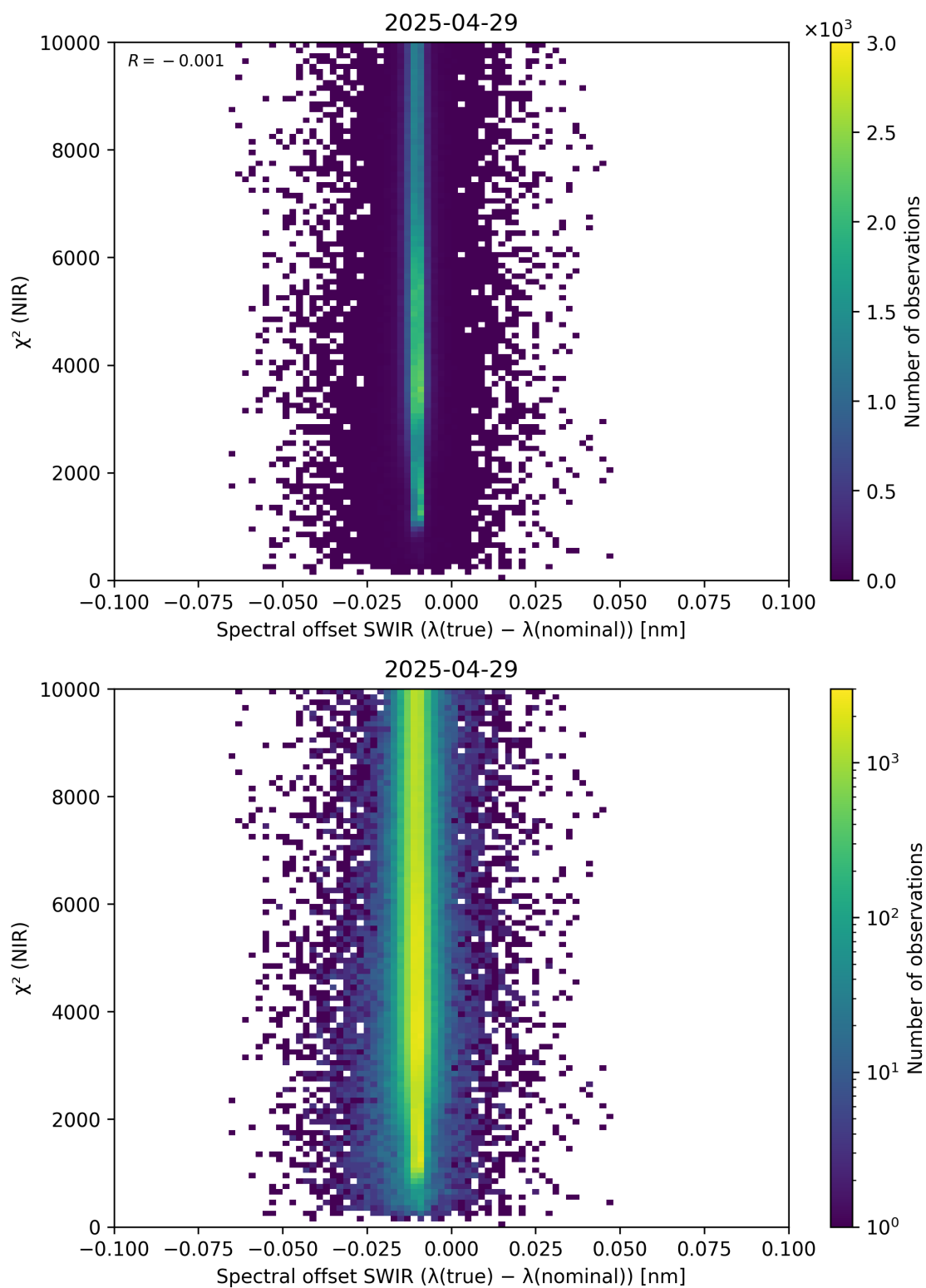
Figure 117: Scatter density plot of “Spectral offset SWIR ( \lambda_{\text{true}} - \lambda_{\text{nominal}} )” against “ \chi^2 (NIR)” for 2025-04-29 to 2025-04-30.
