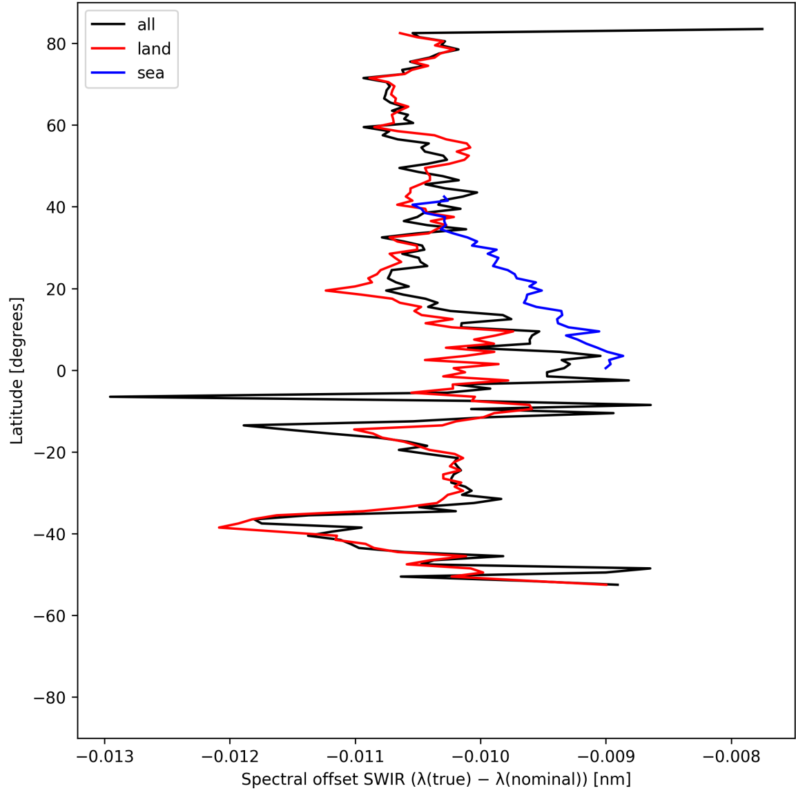
Figure 16: Zonal average of “Spectral offset SWIR ( \lambda_{\text{true}} - \lambda_{\text{nominal}} )” for 2025-04-29 to 2025-04-30.
