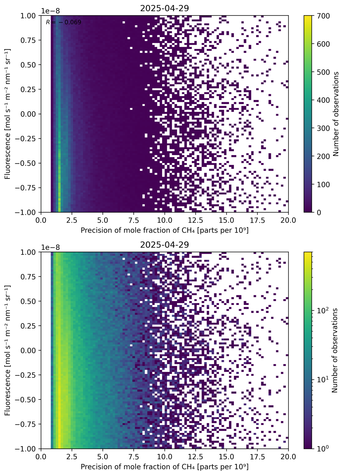
Figure 81: Scatter density plot of “Precision of mole fraction of CH 4 ” against “Fluorescence” for 2025-04-29 to 2025-04-30.
