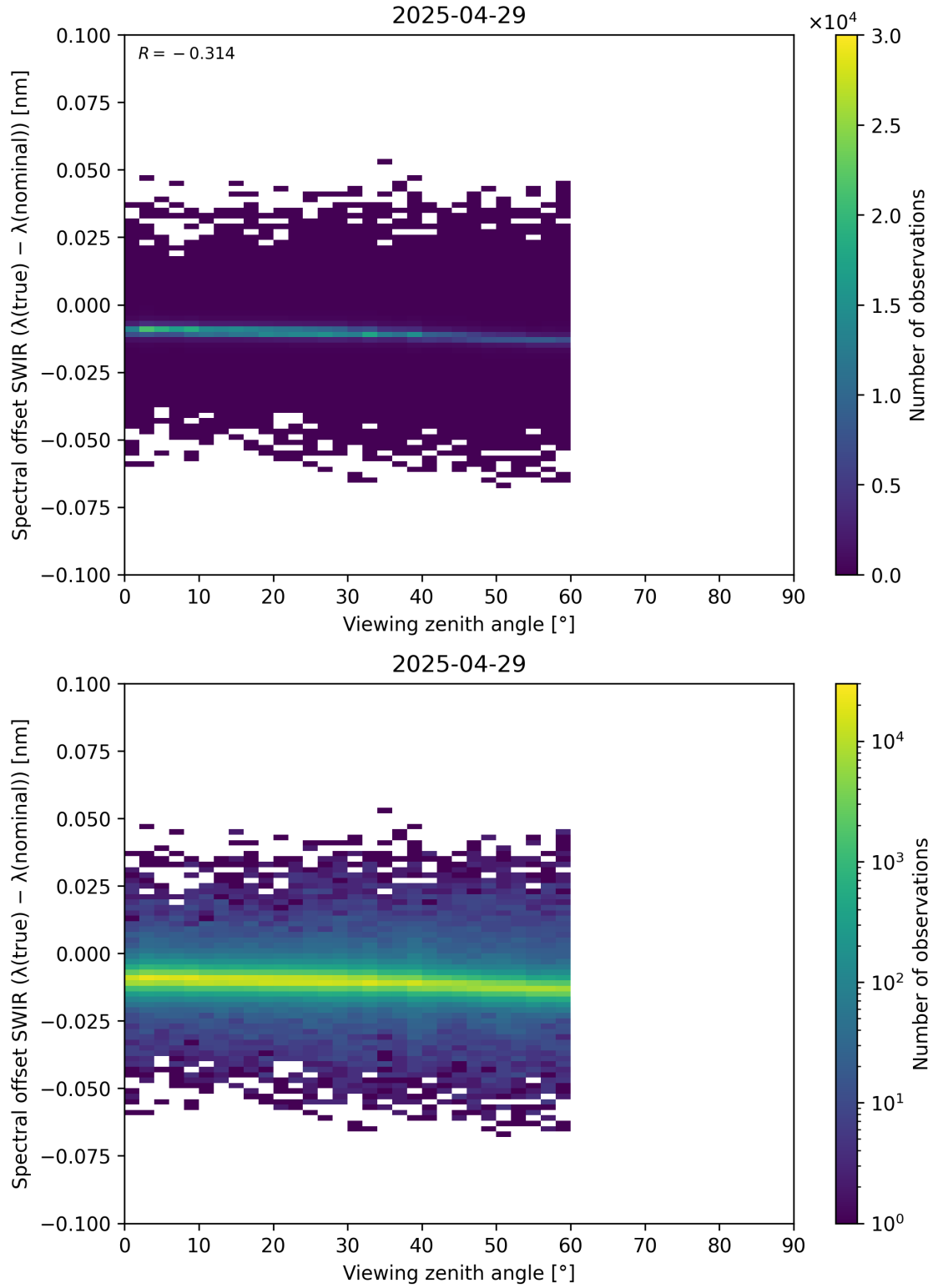
Figure 116: Scatter density plot of “Viewing zenith angle” against “Spectral offset SWIR ( \lambda_{\text{true}} - \lambda_{\text{nominal}} )” for 2025-04-29 to 2025-04-30.
