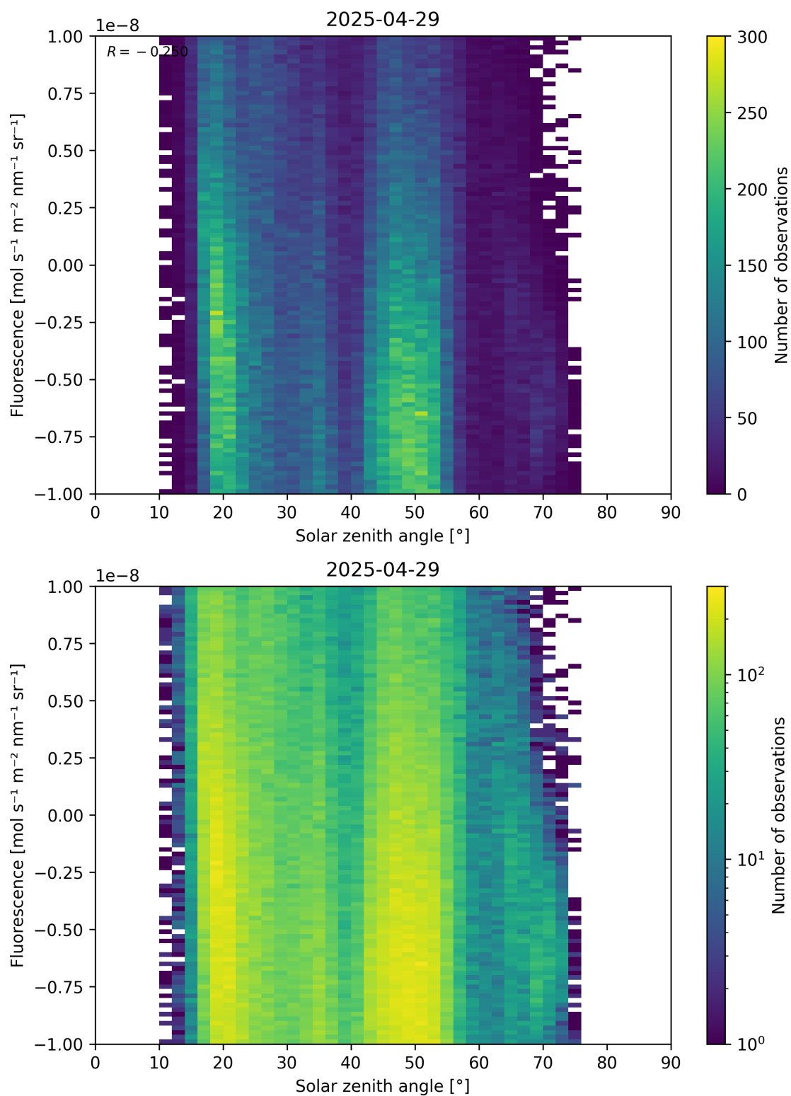
Figure 97: Scatter density plot of “Solar zenith angle” against “Fluorescence” for 2025-04-29 to 2025-04-30.
