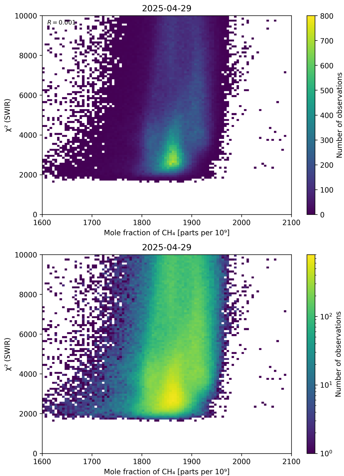
Figure 71: Scatter density plot of “Mole fraction of \text{CH}_4 ” against “ \chi^2 (SWIR)” for 2025-04-29 to 2025-04-30.
