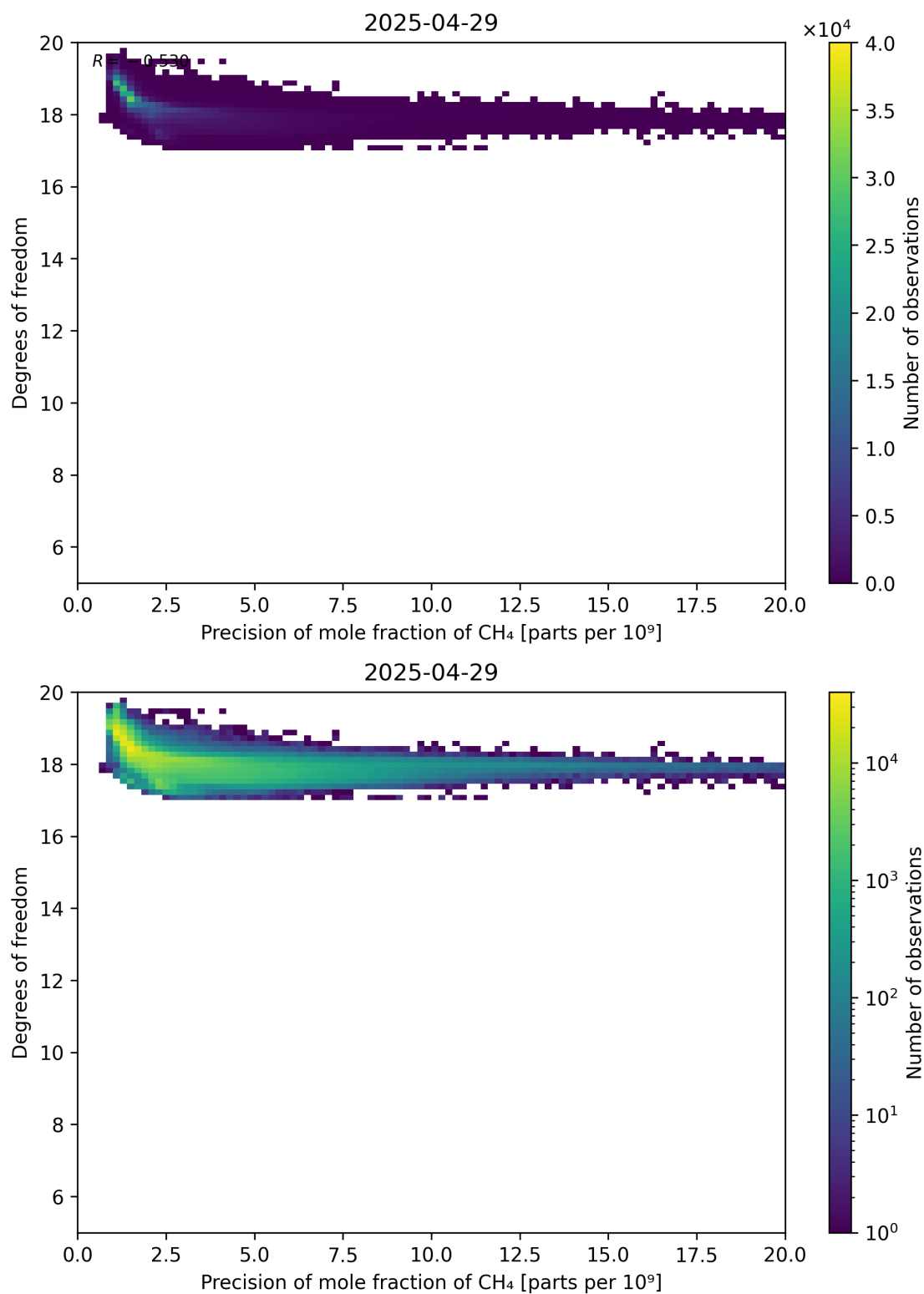
Figure 80: Scatter density plot of “Precision of mole fraction of CH 4 ” against “Degrees of freedom” for 2025-04-29 to 2025-04-30.
