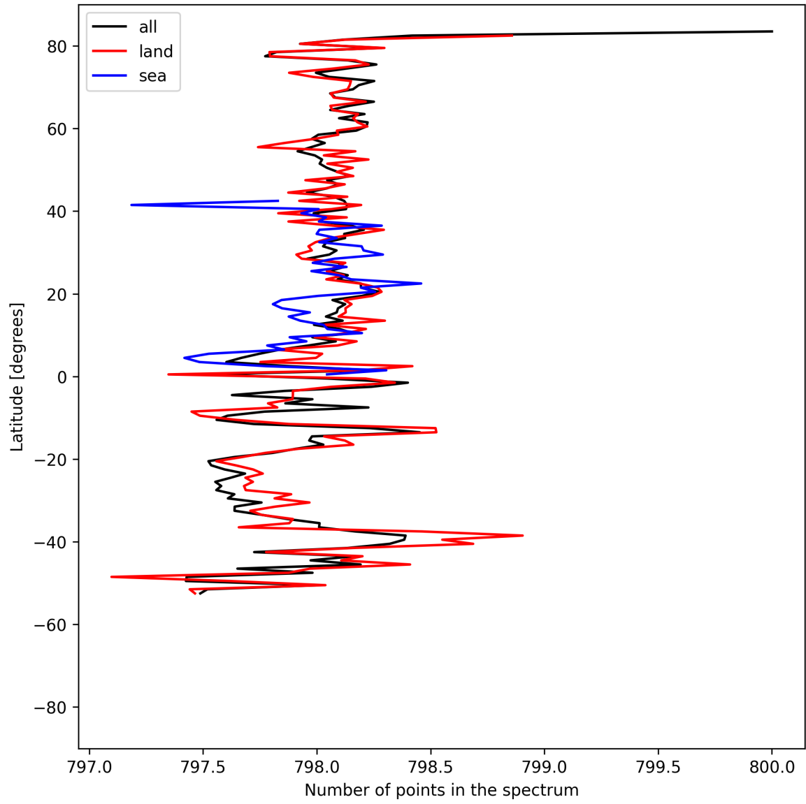
Figure 15: Zonal average of “Number of points in the spectrum” for 2025-04-29 to 2025-04-30.
