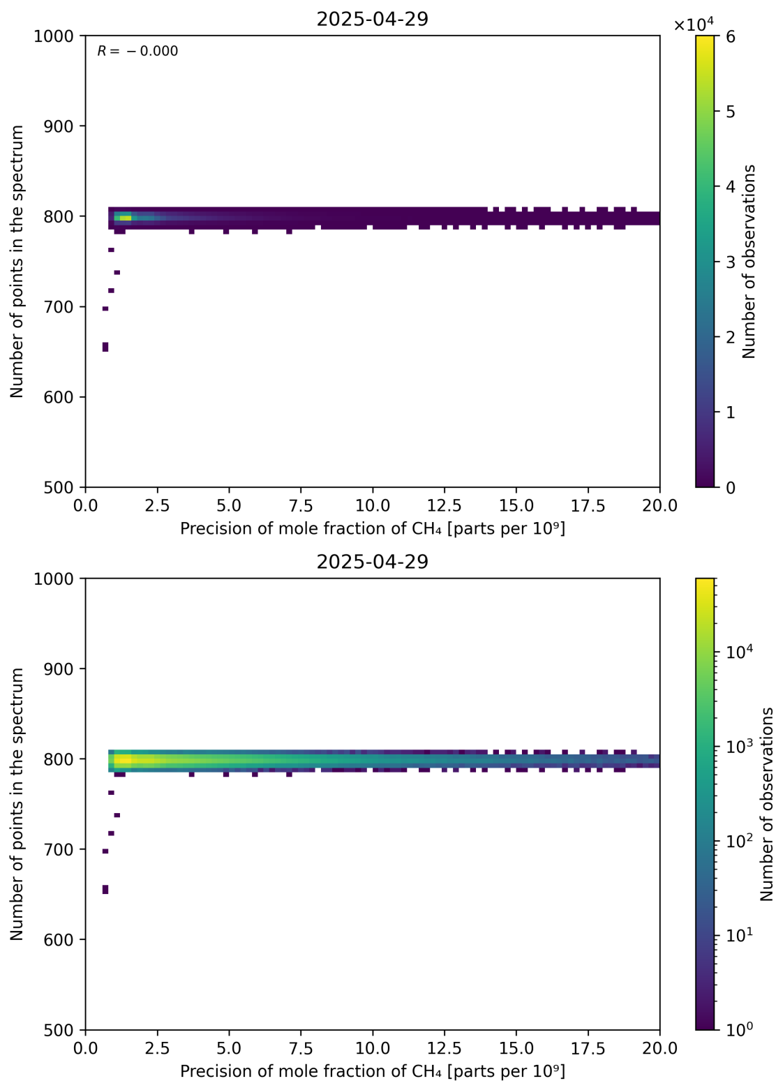
Figure 84: Scatter density plot of “Precision of mole fraction of CH 4 ” against “Number of points in the spectrum” for 2025-04-29 to 2025-04-30.
