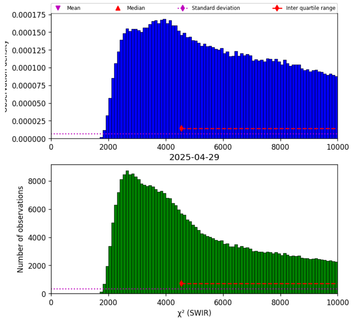
Figure 28: Histogram of “ \chi^2 (SWIR)” for 2025-04-29 to 2025-04-30
