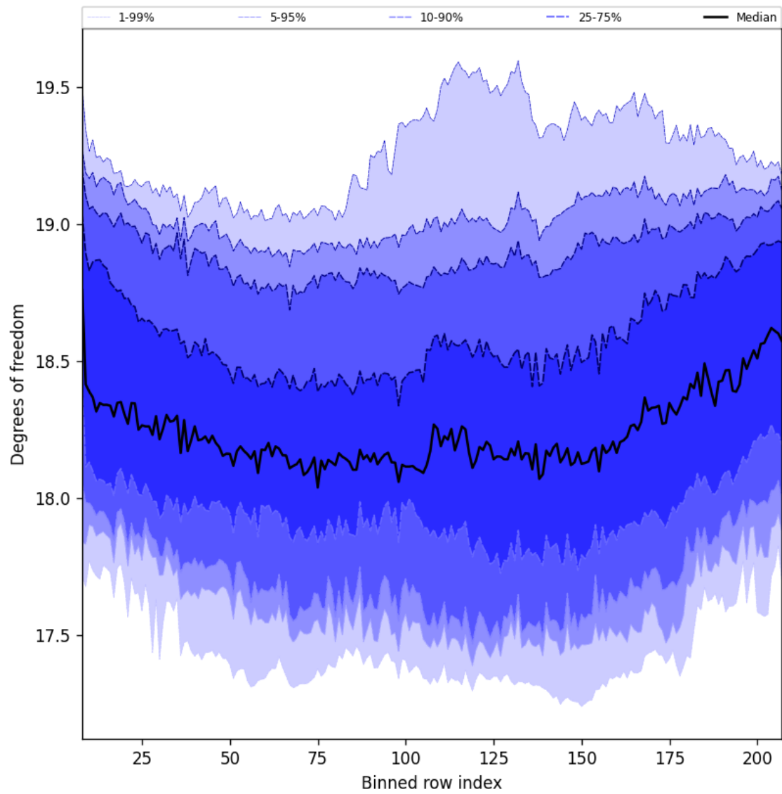
Figure 41: Along track statistics of “Degrees of freedom” for 2025-04-29 to 2025-04-30
