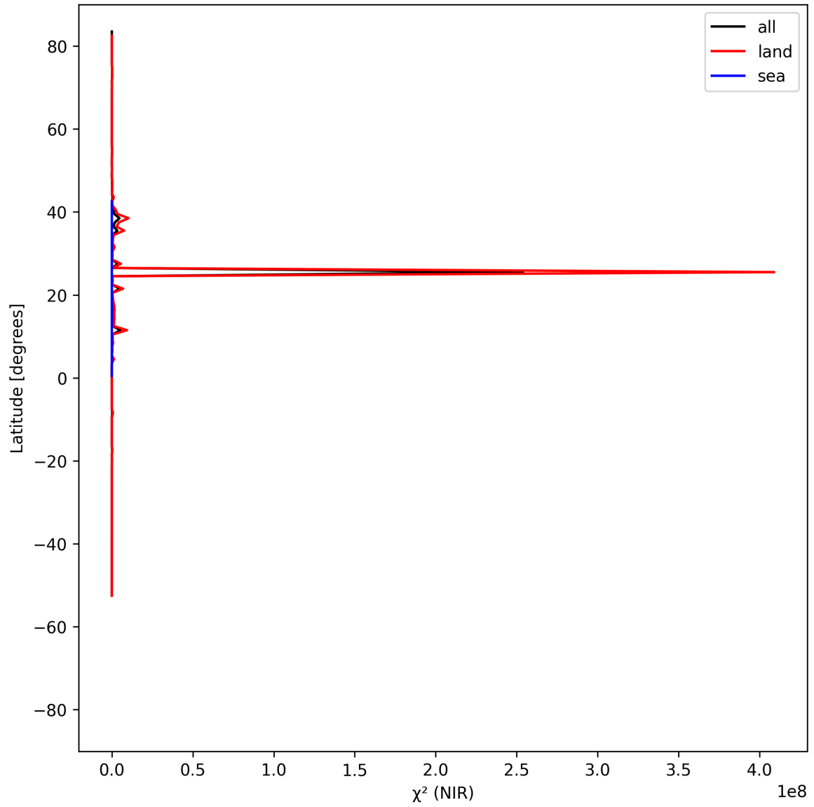
Figure 18: Zonal average of “ \chi^2 (NIR)” for 2025-04-29 to 2025-04-30.
