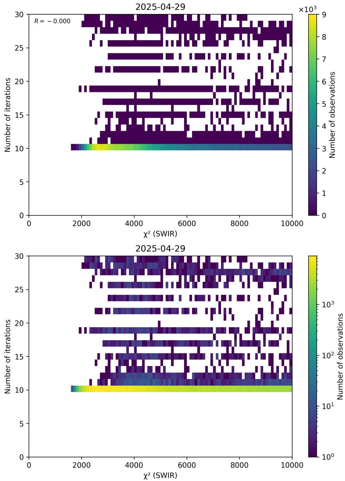
Figure 50: Scatter density plot of “ \chi^2 (SWIR)” against “Number of iterations” for 2025-04-29 to 2025-04-30.
