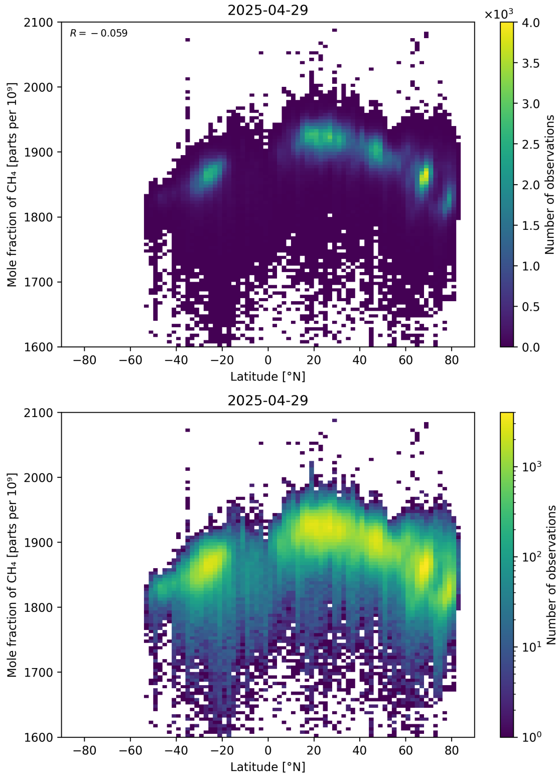
Figure 57: Scatter density plot of “Latitude” against “Mole fraction of CH 4 ” for 2025-04-29 to 2025-04-30.
