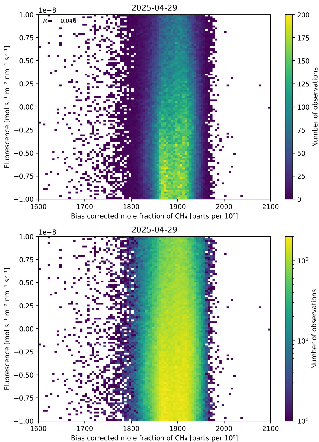
Figure 66: Scatter density plot of “Bias corrected mole fraction of \text{CH}_4 ” against “Fluorescence” for 2025-04-29 to 2025-04-30.
