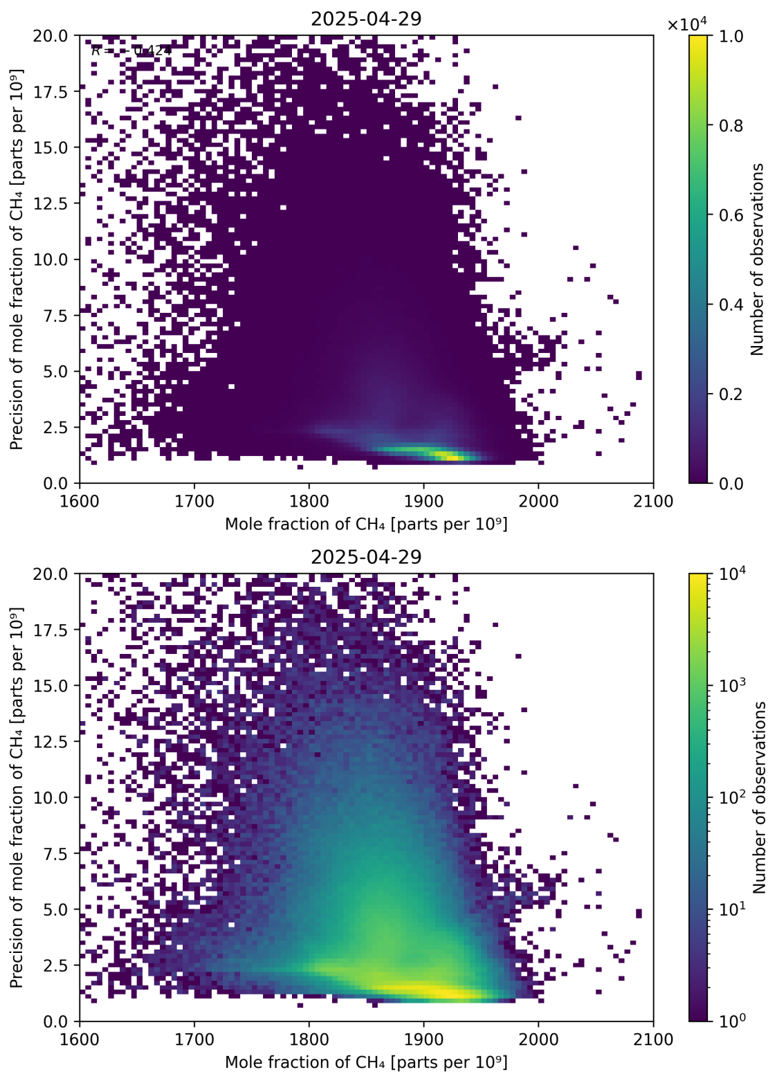
Figure 75: Scatter density plot of “Mole fraction of CH 4 ” against “Precision of mole fraction of CH 4 ” for 2025-04-29 to 2025-04-30.
