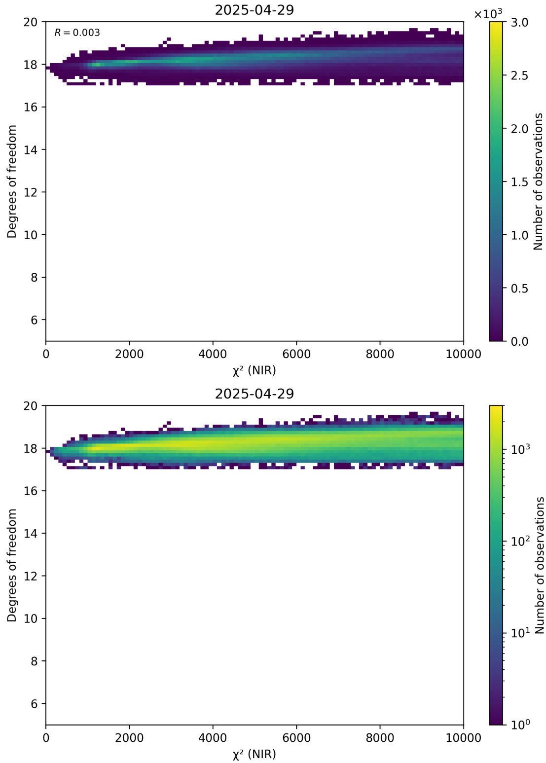
Figure 44: Scatter density plot of “ \chi^2 (NIR)” against “Degrees of freedom” for 2025-04-29 to 2025-04-30.
