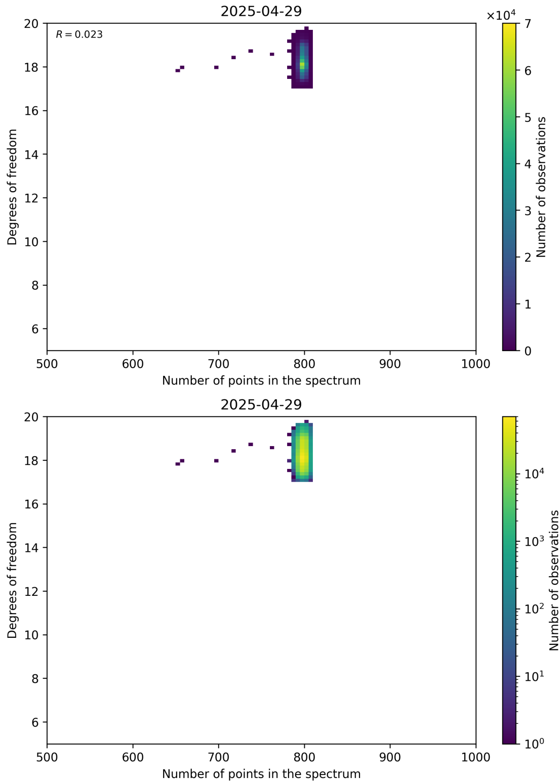
Figure 90: Scatter density plot of “Number of points in the spectrum” against “Degrees of freedom” for 2025-04-29 to 2025-04-30.
