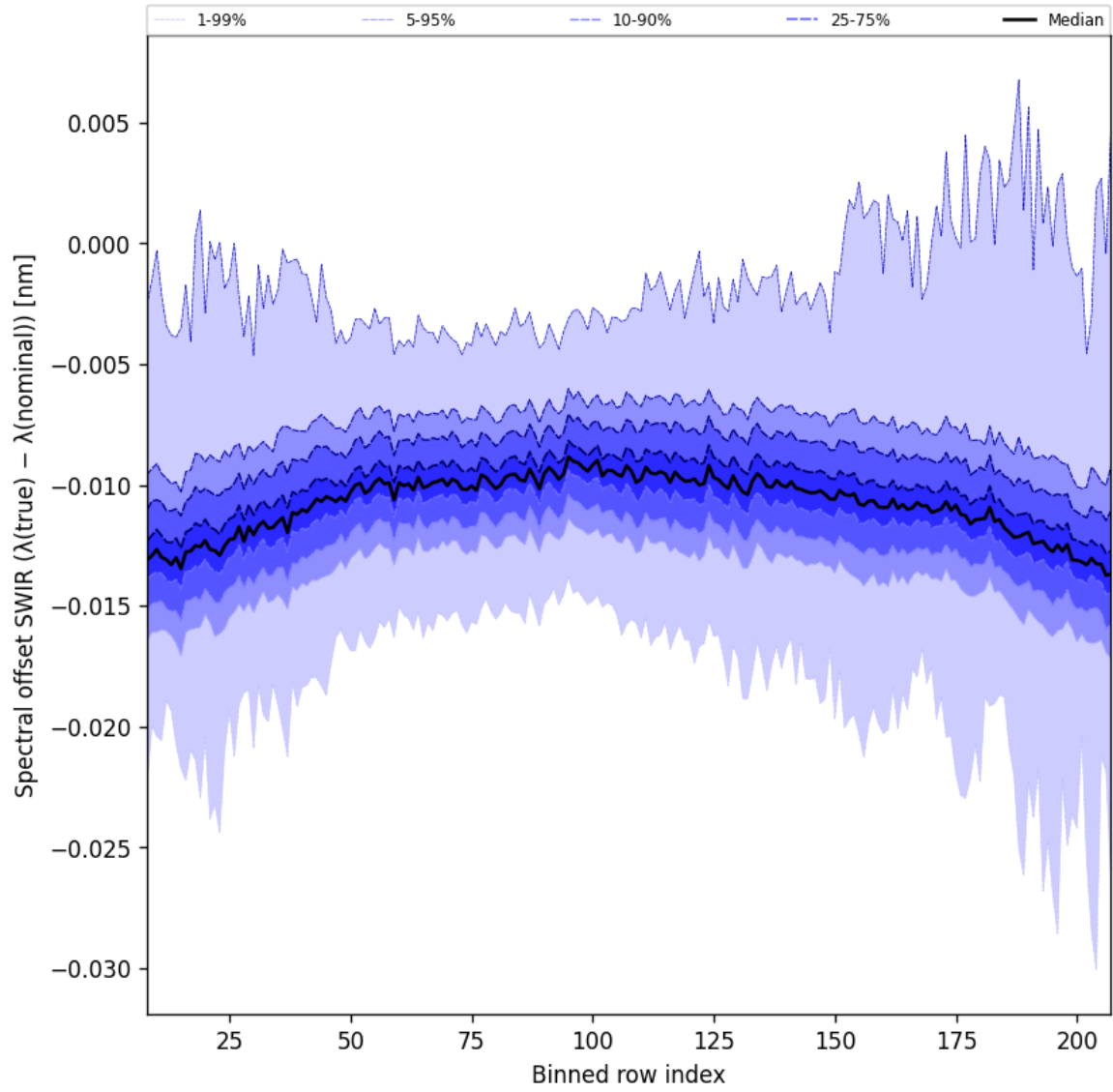
Figure 38: Along track statistics of “Spectral offset SWIR ( \lambda_{\text{true}} - \lambda_{\text{nominal}} )” for 2025-04-29 to 2025-04-30
