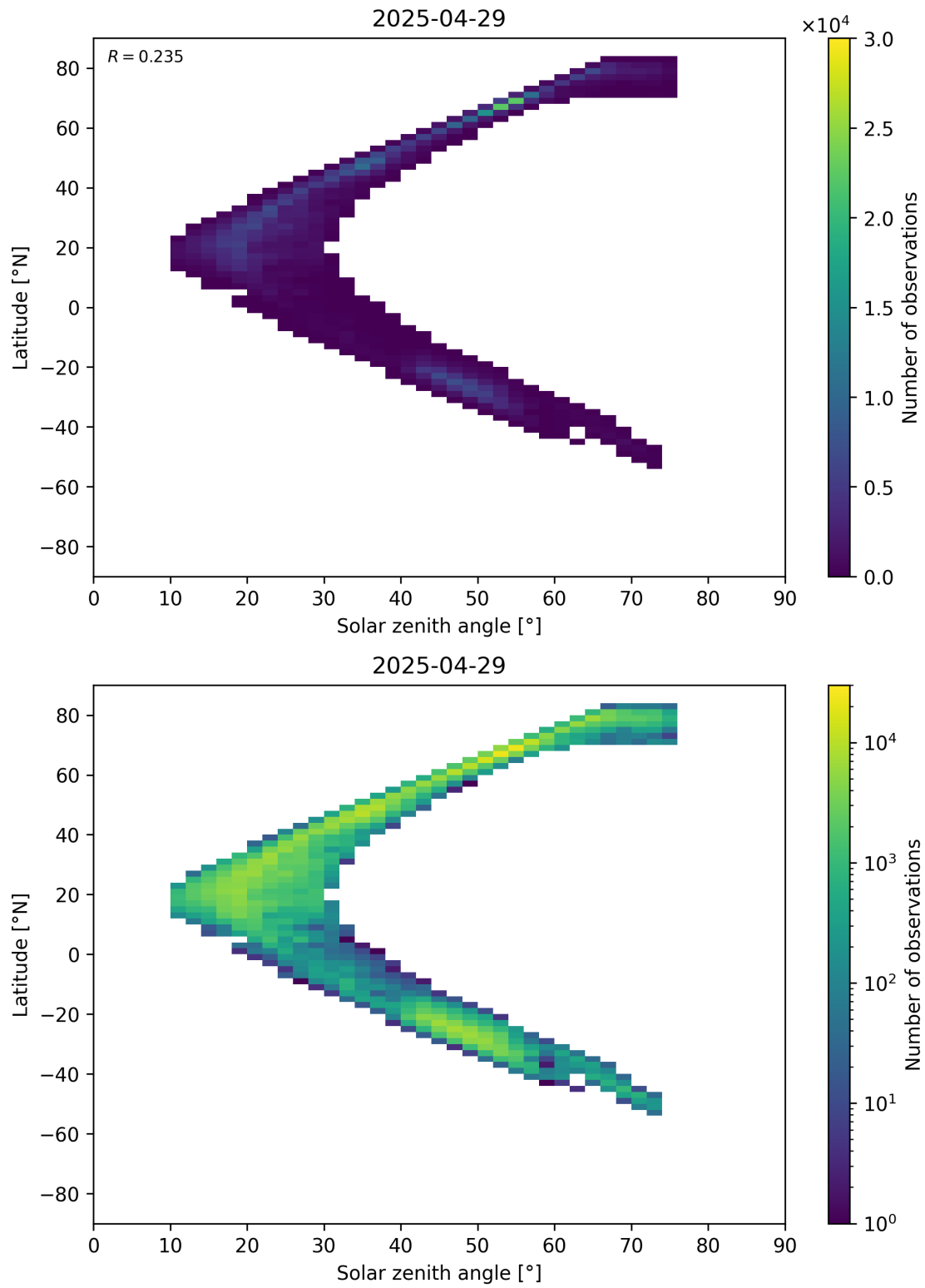
Figure 98: Scatter density plot of “Solar zenith angle” against “Latitude” for 2025-04-29 to 2025-04-30.
