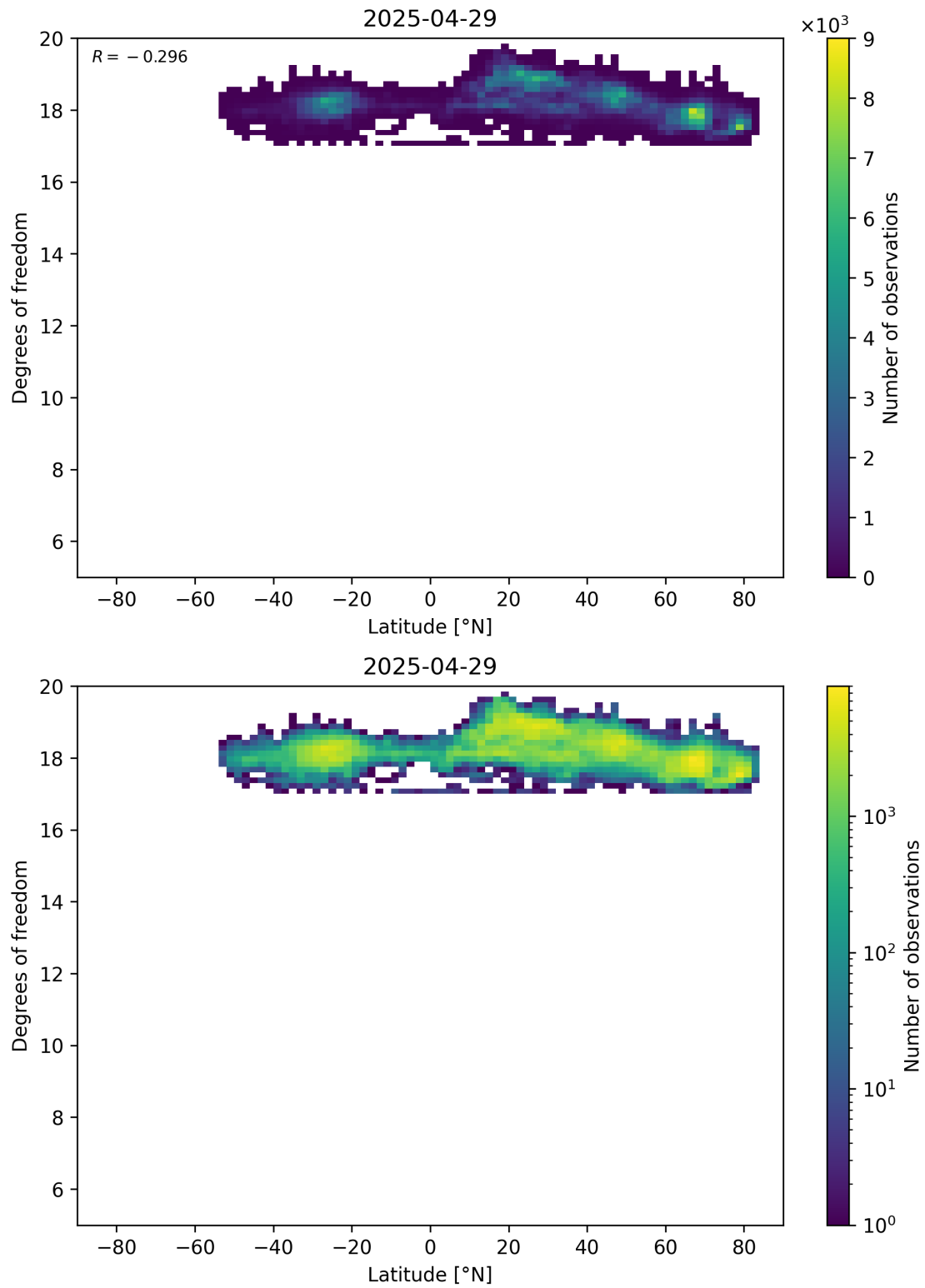
Figure 55: Scatter density plot of “Latitude” against “Degrees of freedom” for 2025-04-29 to 2025-04-30.
