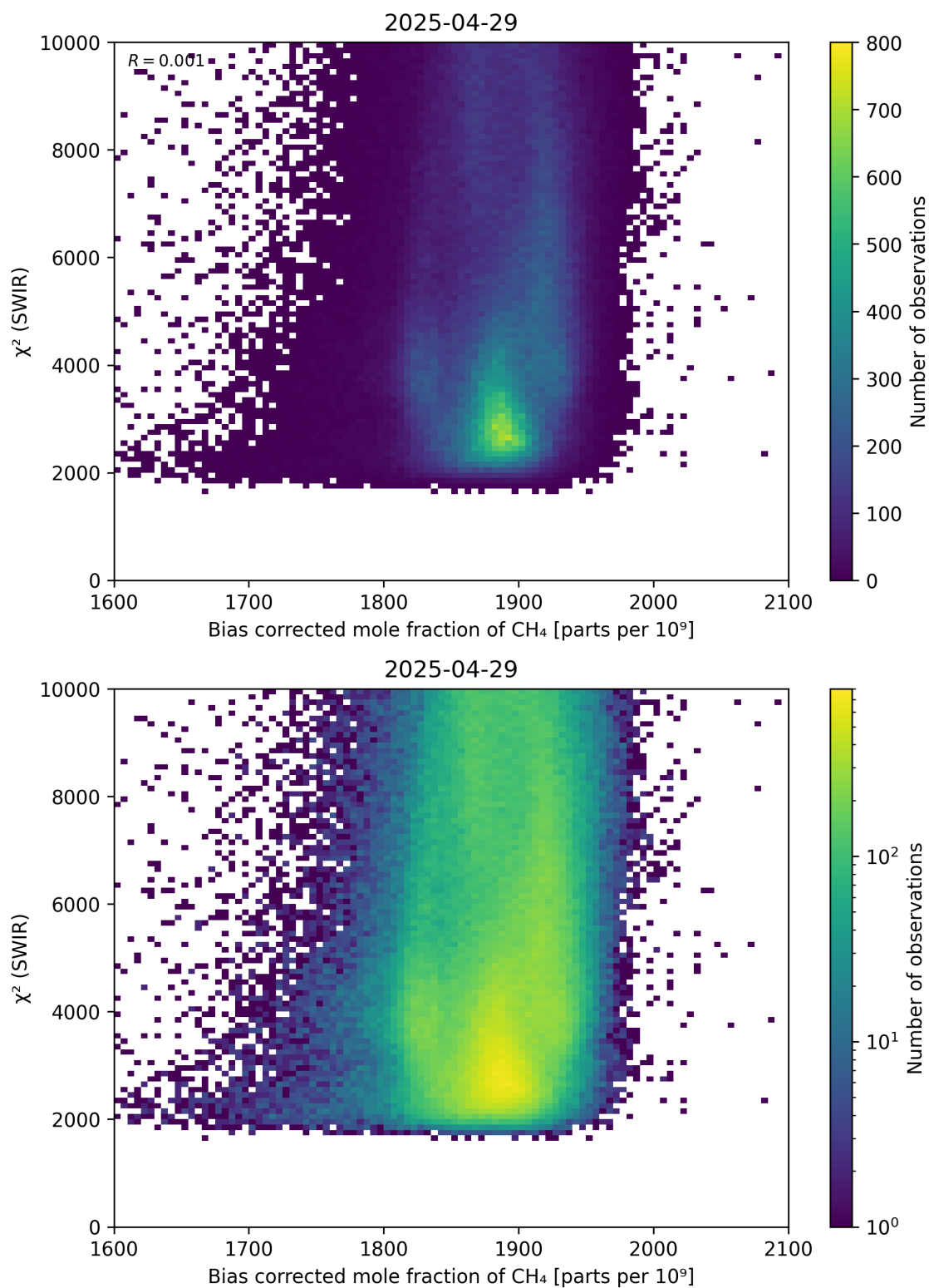
Figure 64: Scatter density plot of “Bias corrected mole fraction of \text{CH}_4 ” against “ \chi^2 (SWIR)” for 2025-04-29 to 2025-04-30.
