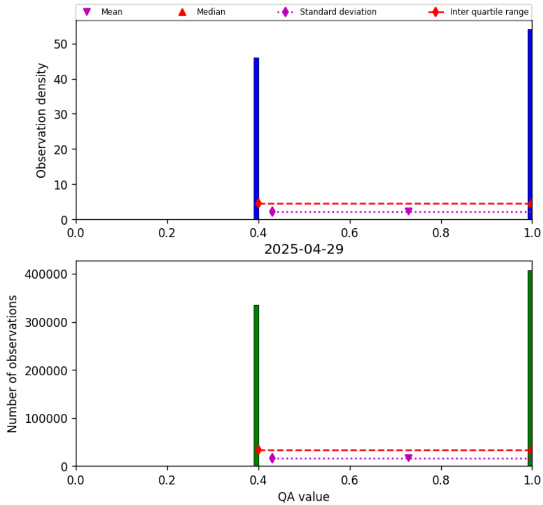
Figure 22: Histogram of “QA value” for 2025-04-29 to 2025-04-30
