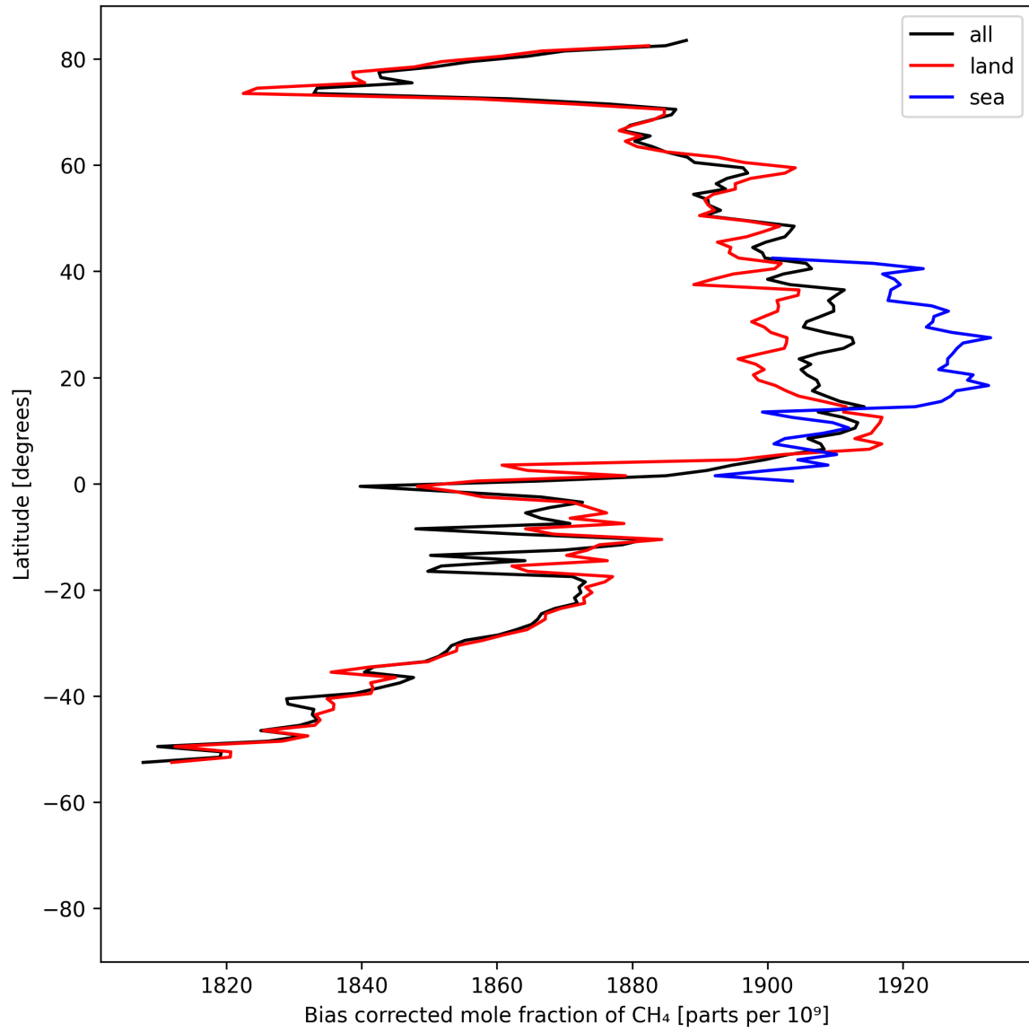
Figure 14: Zonal average of “Bias corrected mole fraction of CH 4 ” for 2025-04-29 to 2025-04-30.
