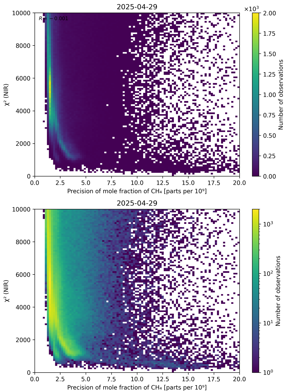
Figure 78: Scatter density plot of “Precision of mole fraction of CH 4 ” against “ \chi^2 (NIR)” for 2025-04-29 to 2025-04-30.
