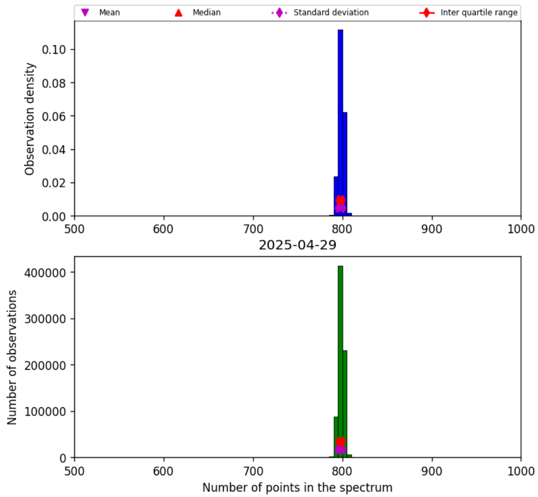
Figure 26: Histogram of “Number of points in the spectrum” for 2025-04-29 to 2025-04-30
