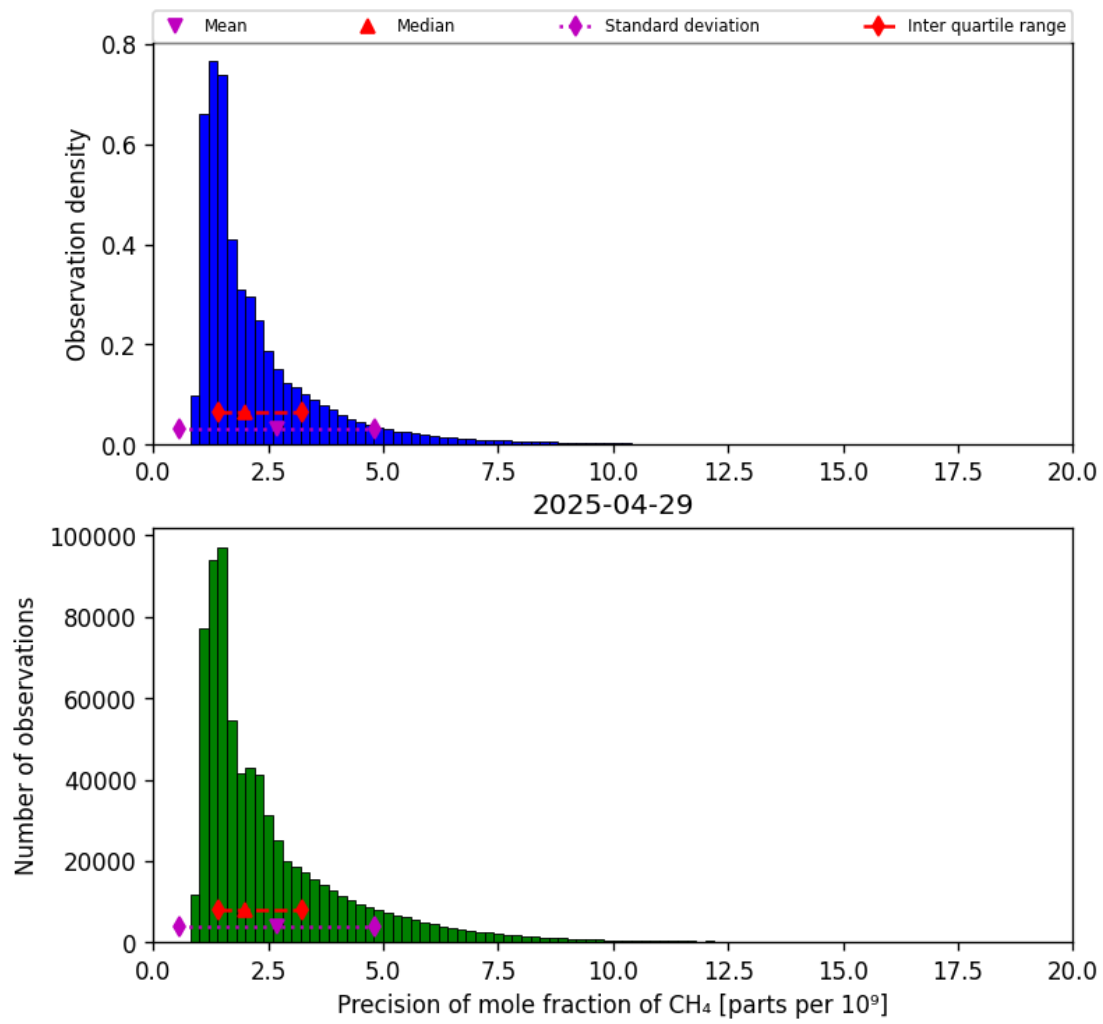
Figure 24: Histogram of “Precision of mole fraction of CH 4 ” for 2025-04-29 to 2025-04-30
