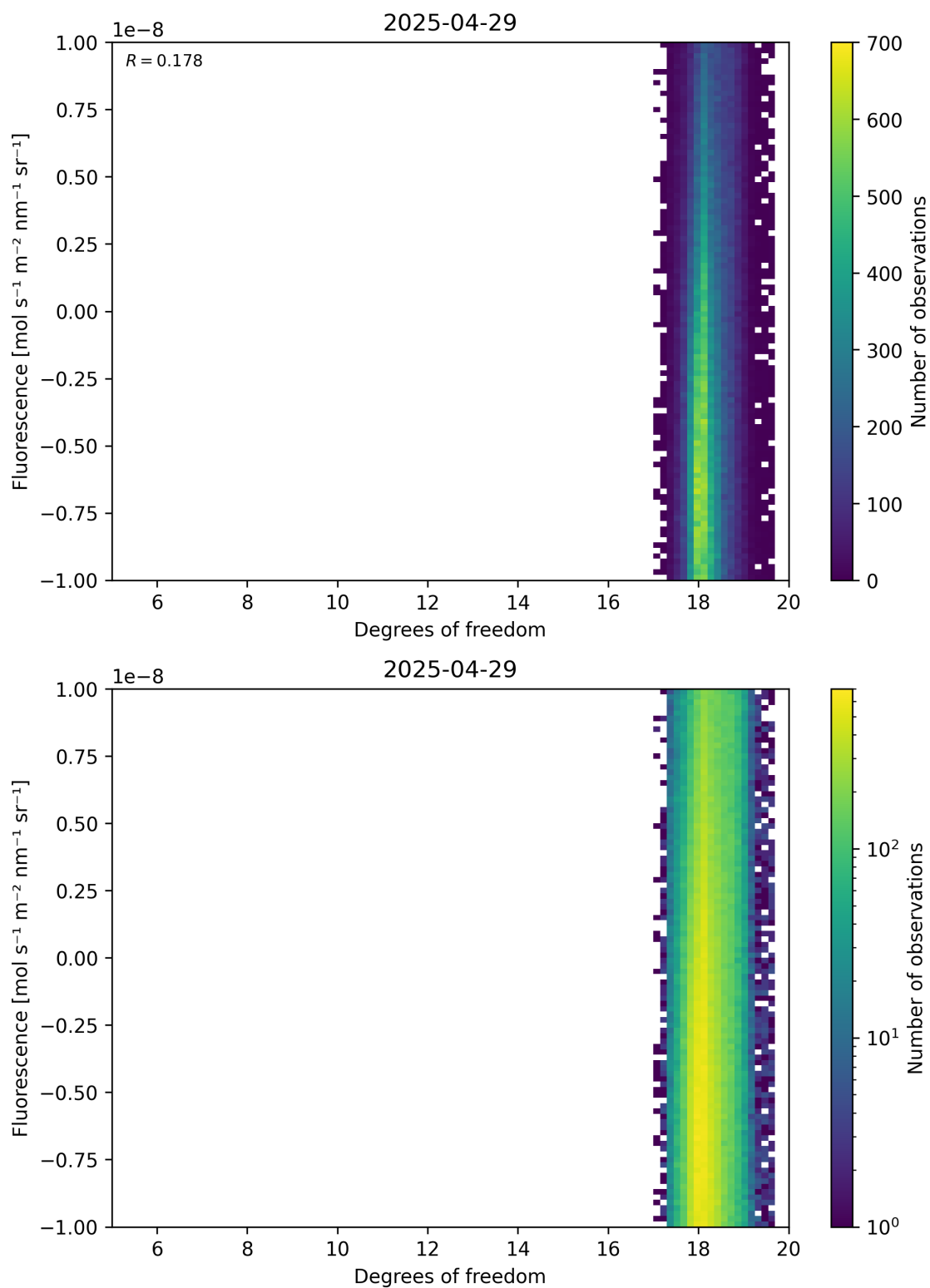
Figure 51: Scatter density plot of “Degrees of freedom” against “Fluorescence” for 2025-04-29 to 2025-04-30.
