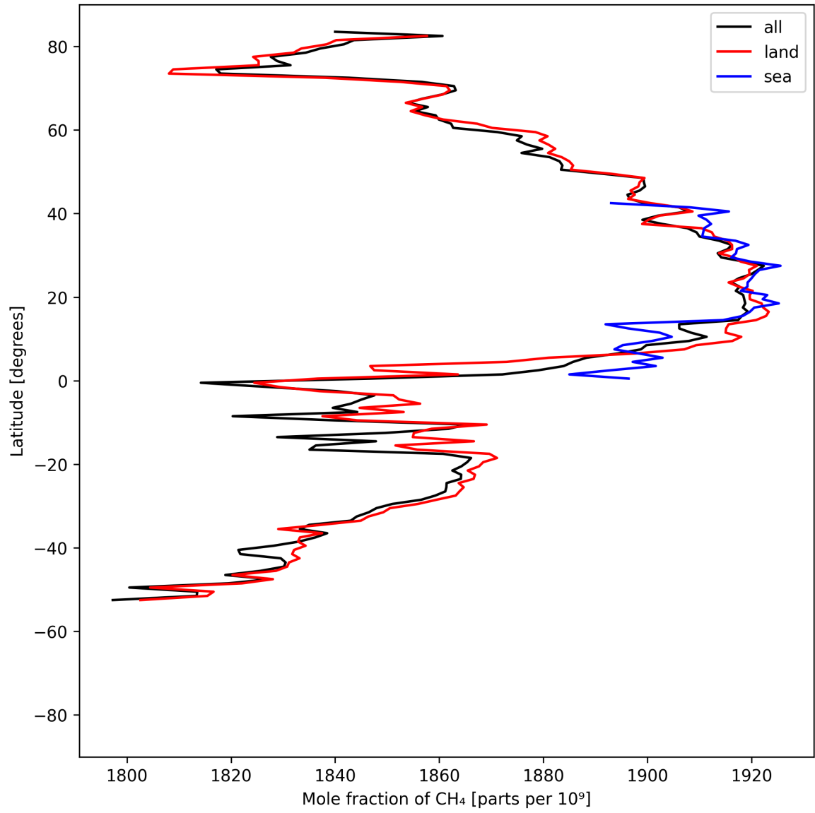
Figure 12: Zonal average of “Mole fraction of CH 4 ” for 2025-04-29 to 2025-04-30.
