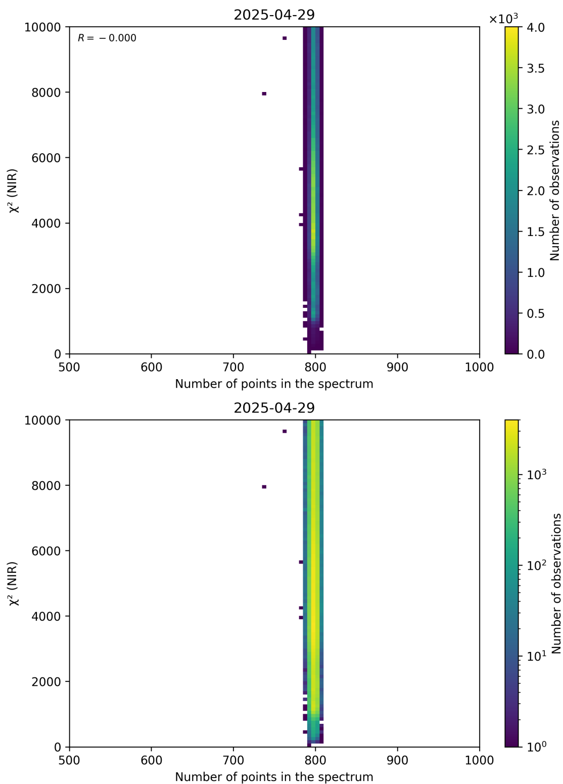
Figure 88: Scatter density plot of “Number of points in the spectrum” against “ \chi^2 (NIR)” for 2025-04-29 to 2025-04-30.
