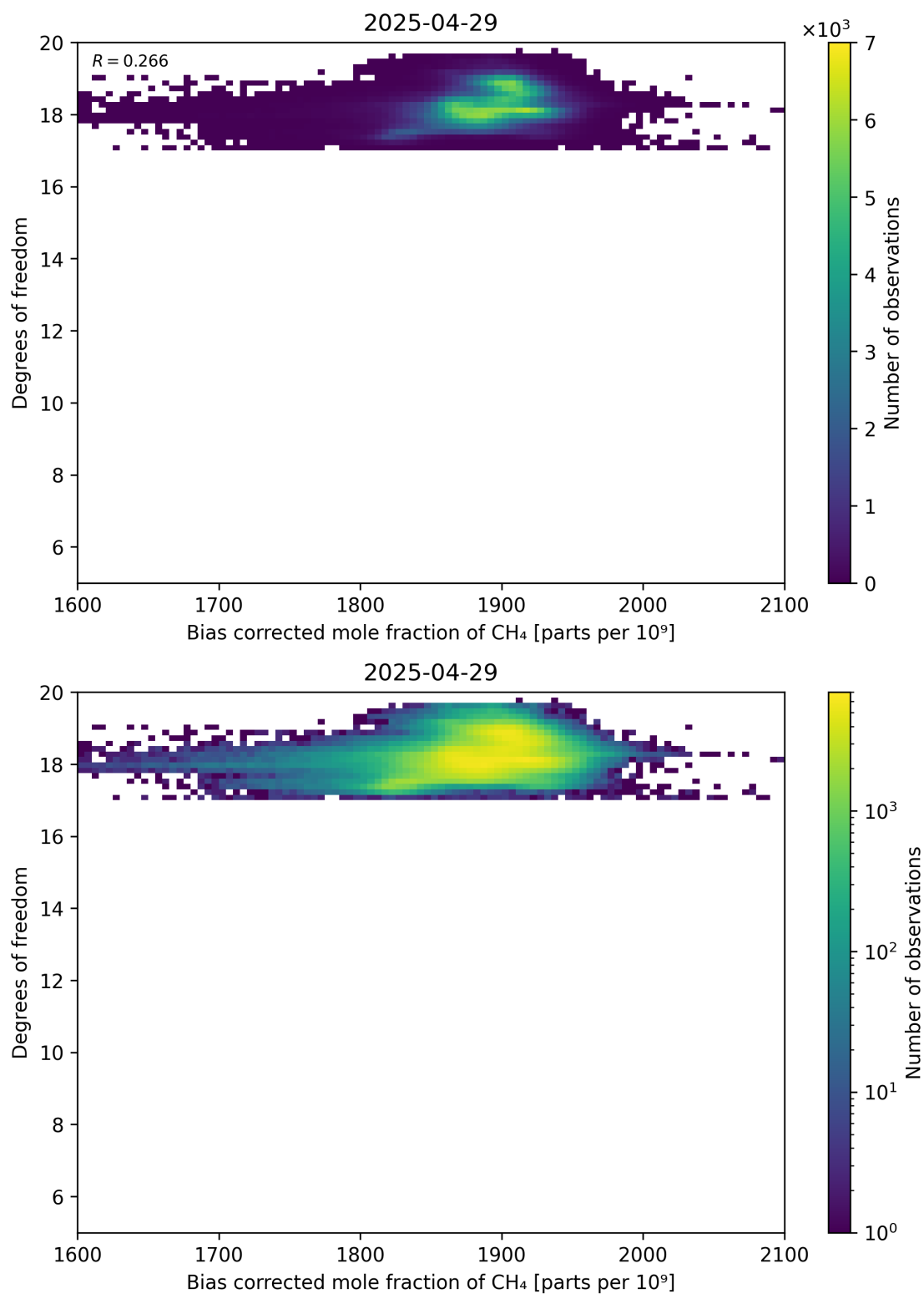
Figure 65: Scatter density plot of “Bias corrected mole fraction of CH 4 ” against “Degrees of freedom” for 2025-04-29 to 2025-04-30.
