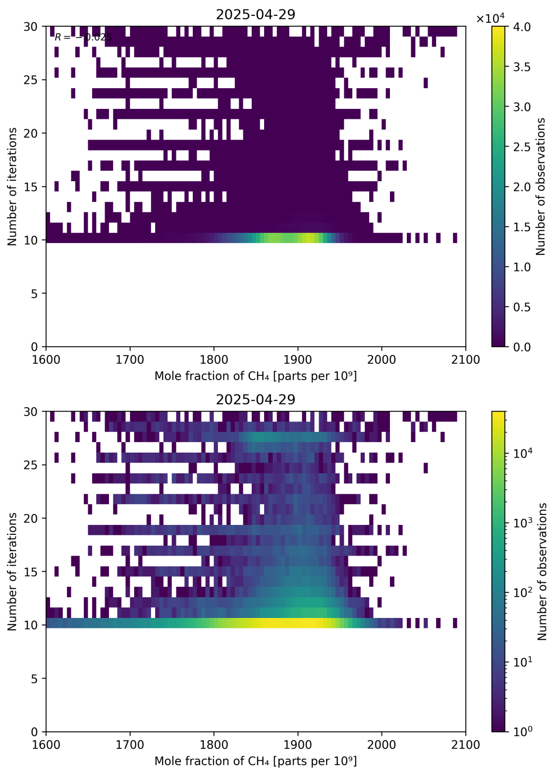
Figure 76: Scatter density plot of “Mole fraction of CH 4 ” against “Number of iterations” for 2025-04-29 to 2025-04-30.
