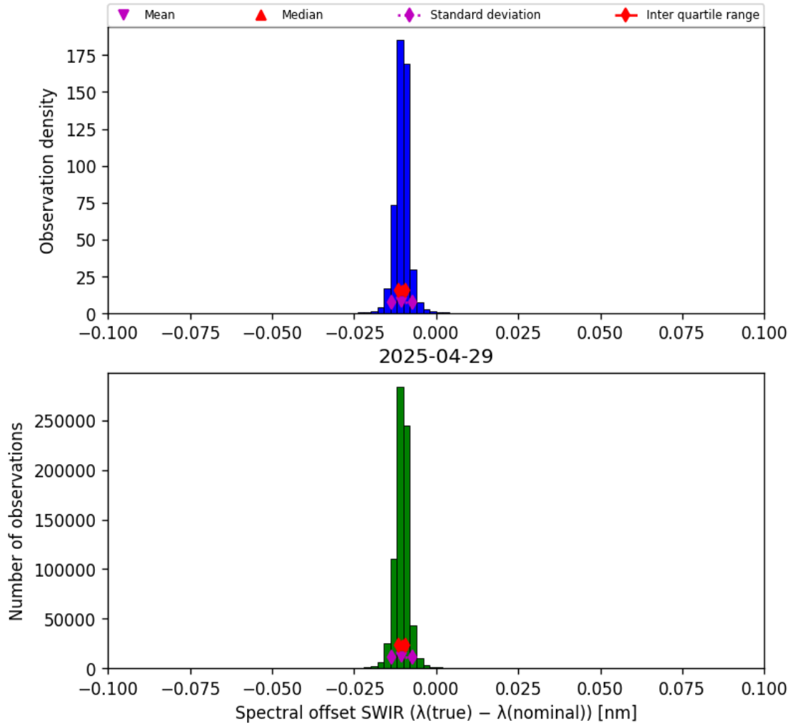
Figure 27: Histogram of “Spectral offset SWIR ( \lambda_{\text{true}} - \lambda_{\text{nominal}} )” for 2025-04-29 to 2025-04-30
