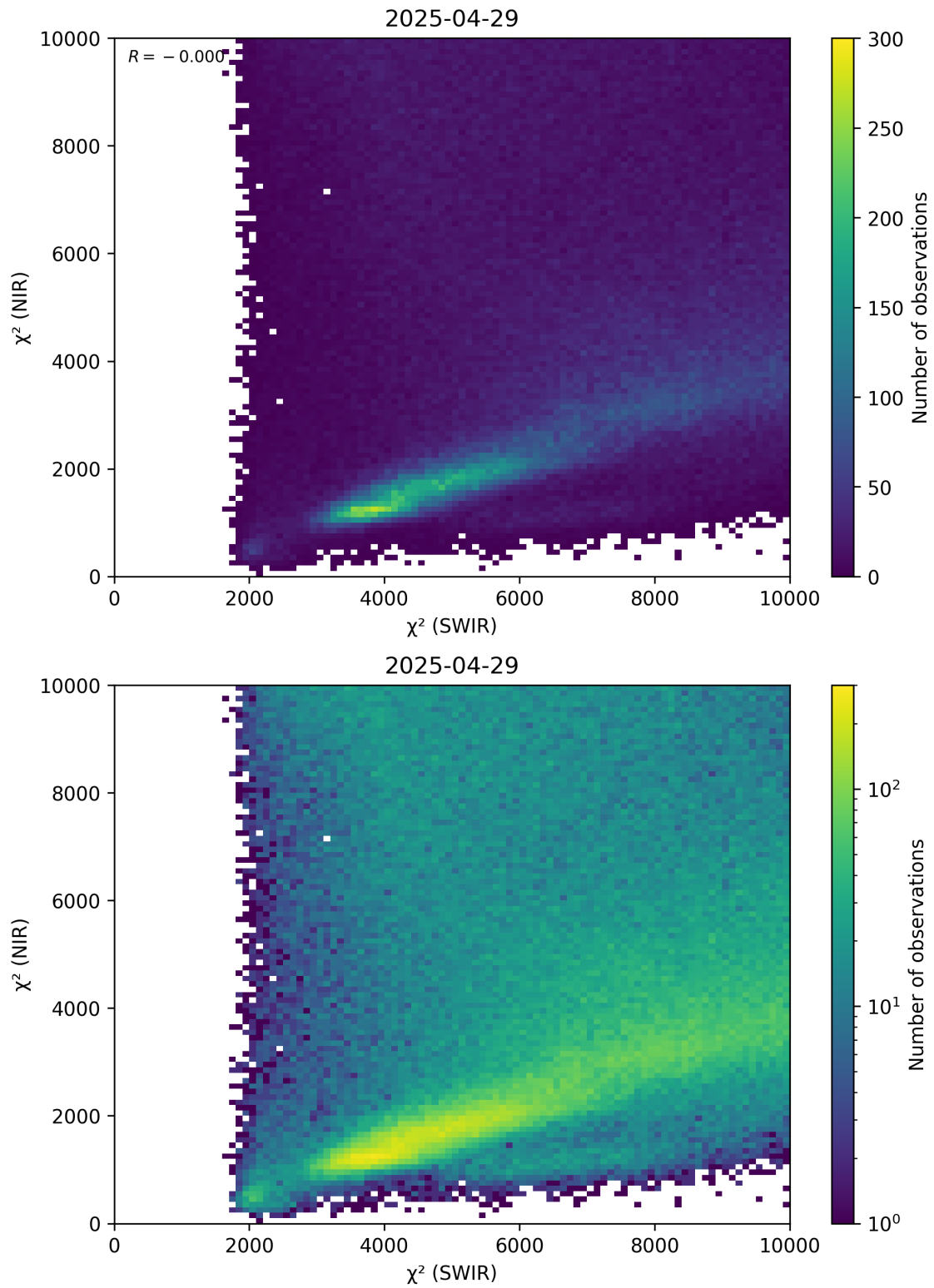
Figure 47: Scatter density plot of “ \chi^2 (SWIR)” against “ \chi^2 (NIR)” for 2025-04-29 to 2025-04-30.
