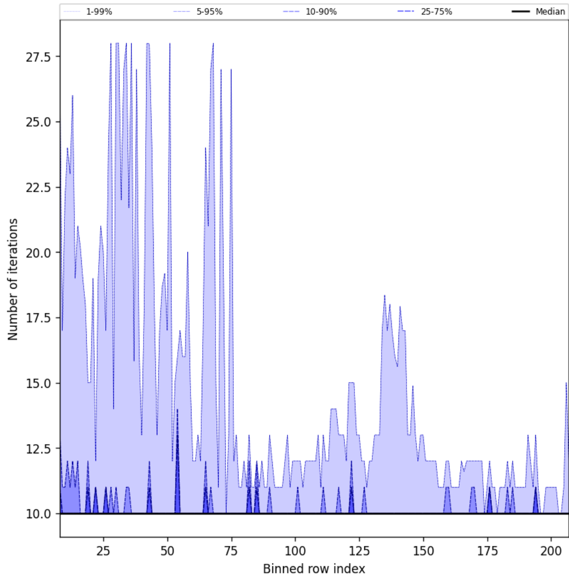
Figure 42: Along track statistics of “Number of iterations” for 2025-04-29 to 2025-04-30
