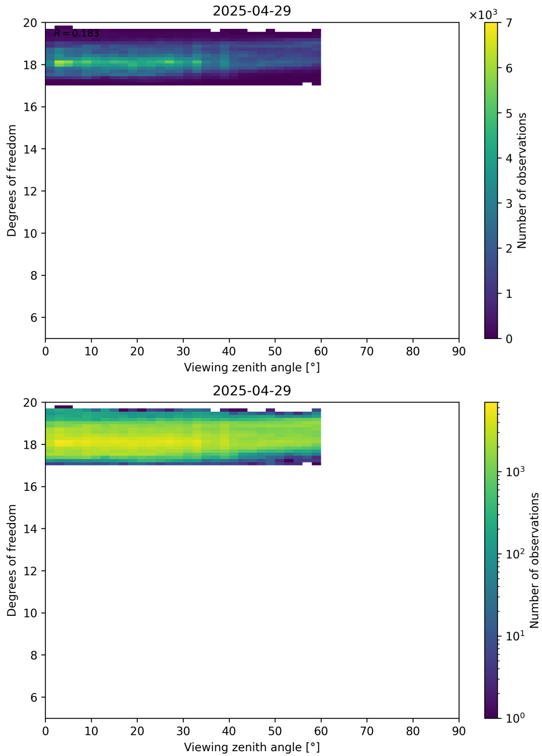
Figure 107: Scatter density plot of “Viewing zenith angle” against “Degrees of freedom” for 2025-04-29 to 2025-04-30.
