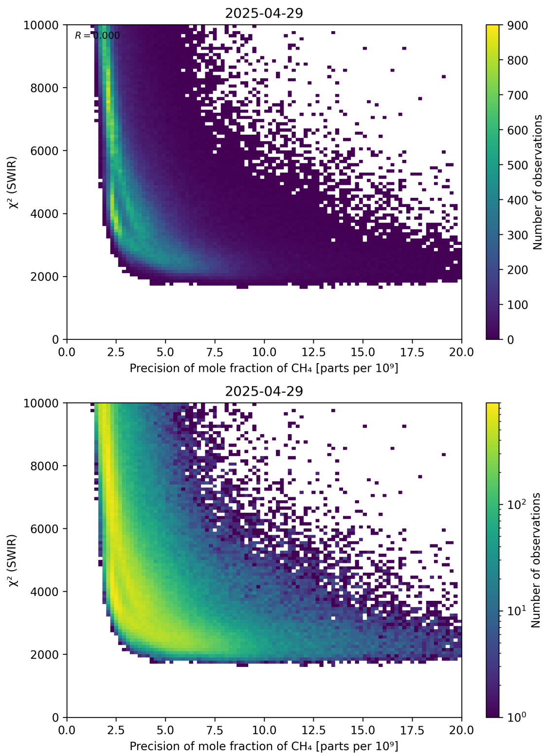
Figure 79: Scatter density plot of “Precision of mole fraction of \text{CH}_4 ” against “ \chi^2 (SWIR)” for 2025-04-29 to 2025-04-30.
