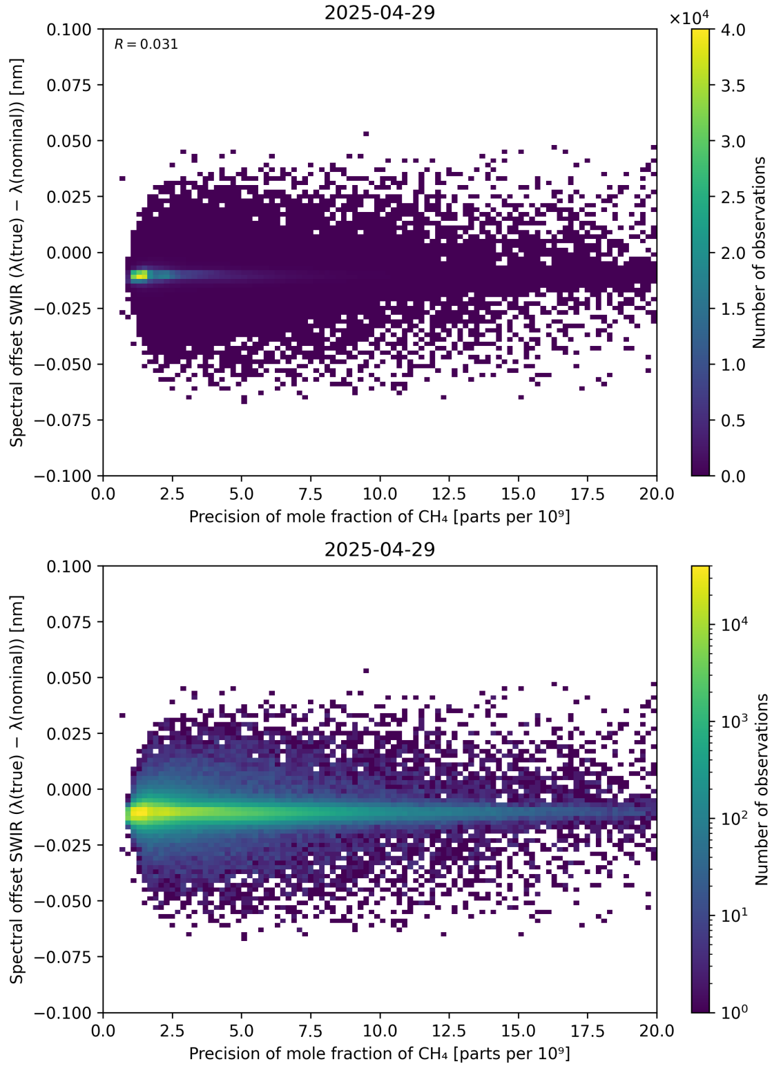
Figure 85: Scatter density plot of “Precision of mole fraction of \text{CH}_4 ” against “Spectral offset SWIR ( \lambda_{\text{true}} - \lambda_{\text{nominal}} )” for 2025-04-29 to 2025-04-30.
