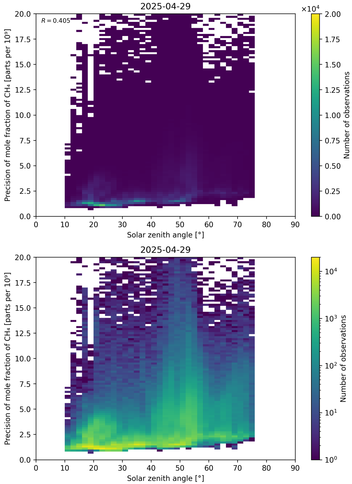
Figure 101: Scatter density plot of “Solar zenith angle” against “Precision of mole fraction of CH 4 ” for 2025-04-29 to 2025-04-30.
