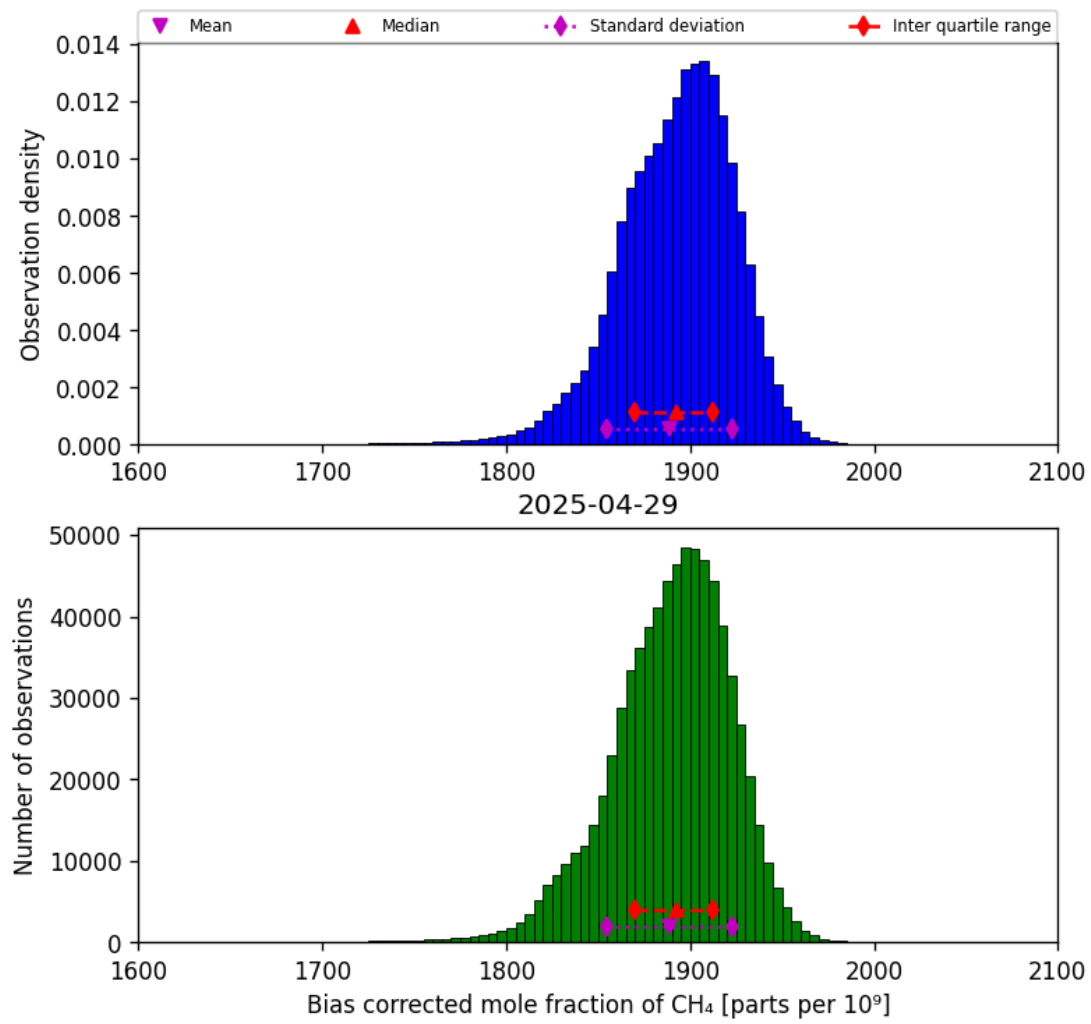
Figure 25: Histogram of “Bias corrected mole fraction of CH 4 ” for 2025-04-29 to 2025-04-30
