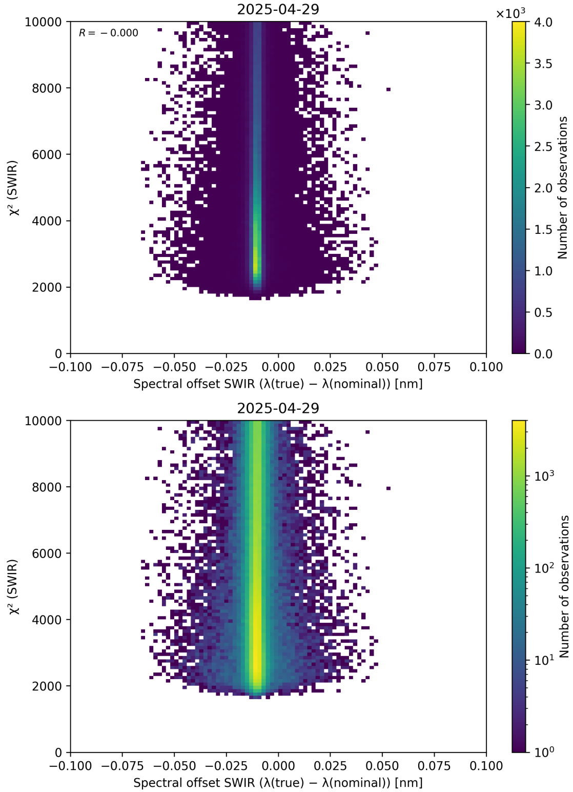
Figure 118: Scatter density plot of “Spectral offset SWIR ( \lambda_{\text{true}} - \lambda_{\text{nominal}} )” against “ \chi^2 (SWIR)” for 2025-04-29 to 2025-04-30.
