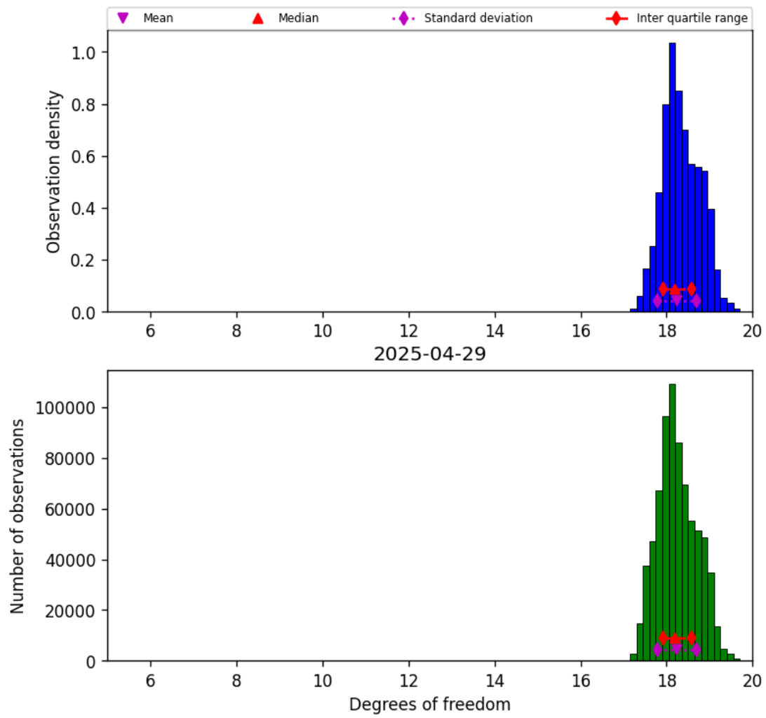
Figure 30: Histogram of “Degrees of freedom” for 2025-04-29 to 2025-04-30
