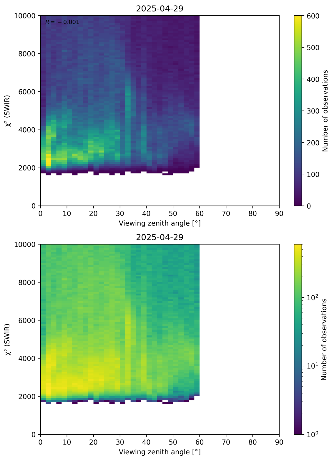
Figure 106: Scatter density plot of “Viewing zenith angle” against “ \chi^2 (SWIR)” for 2025-04-29 to 2025-04-30.
