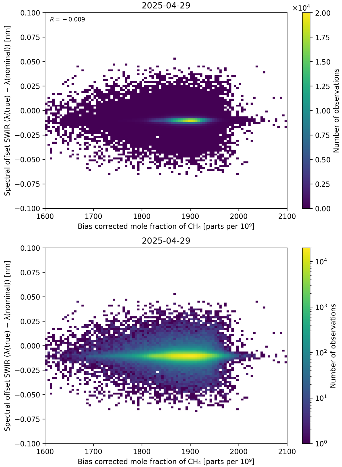
Figure 69: Scatter density plot of “Bias corrected mole fraction of \text{CH}_4 ” against “Spectral offset SWIR ( \lambda_{\text{true}} - \lambda_{\text{nominal}} )” for 2025-04-29 to 2025-04-30.
