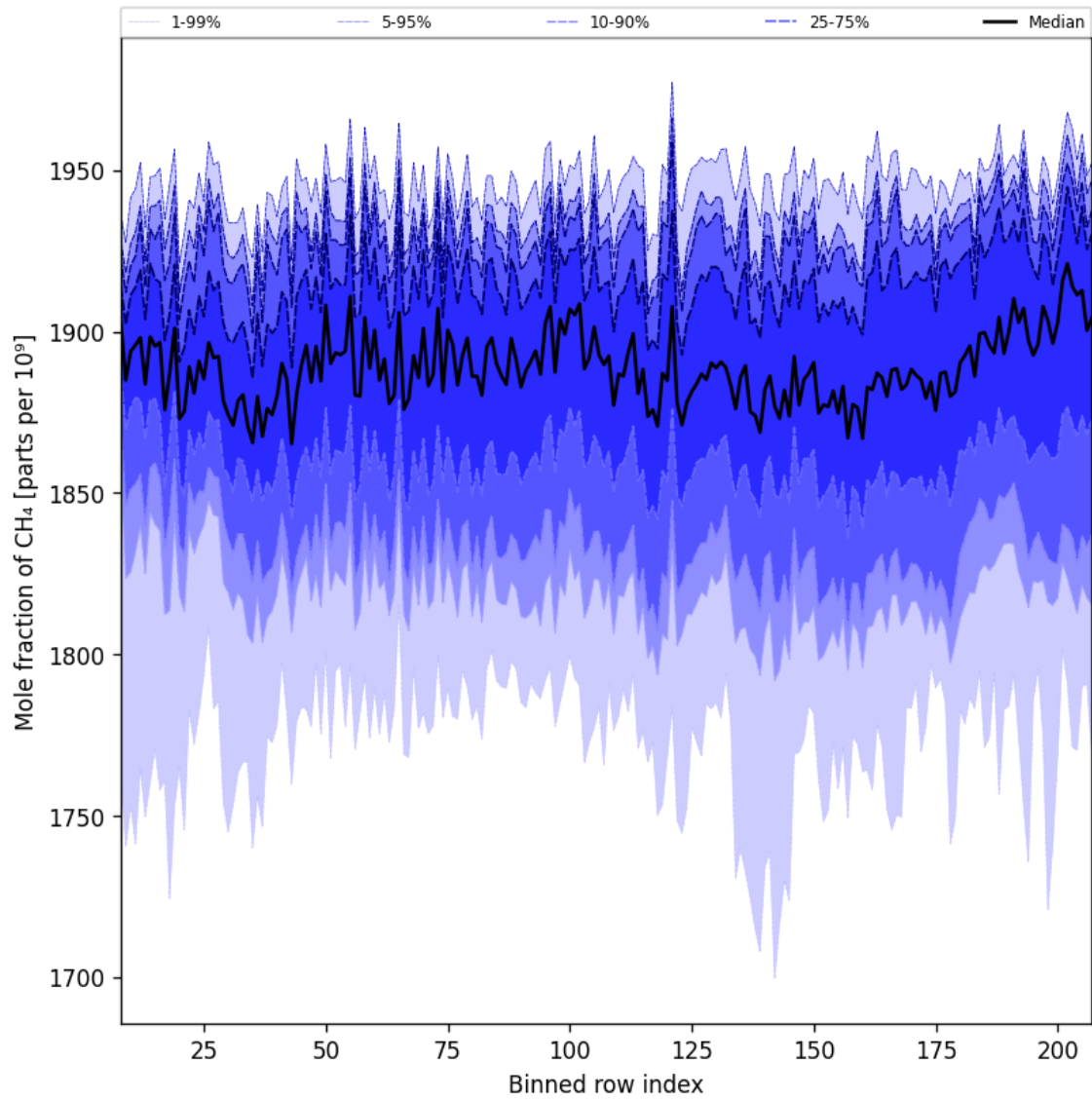
Figure 34: Along track statistics of “Mole fraction of CH 4 ” for 2025-04-29 to 2025-04-30
