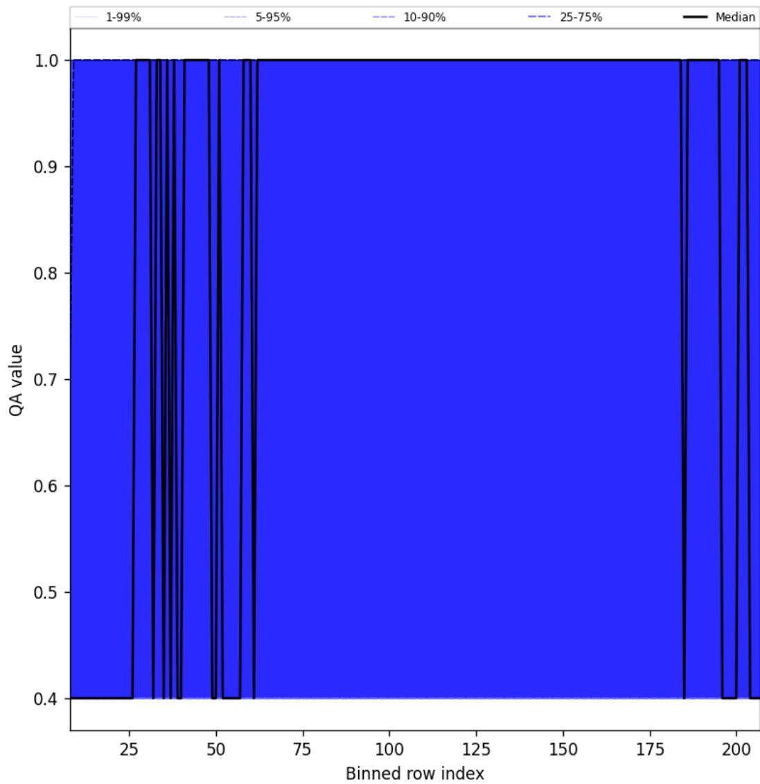
Figure 33: Along track statistics of “QA value” for 2025-04-29 to 2025-04-30
