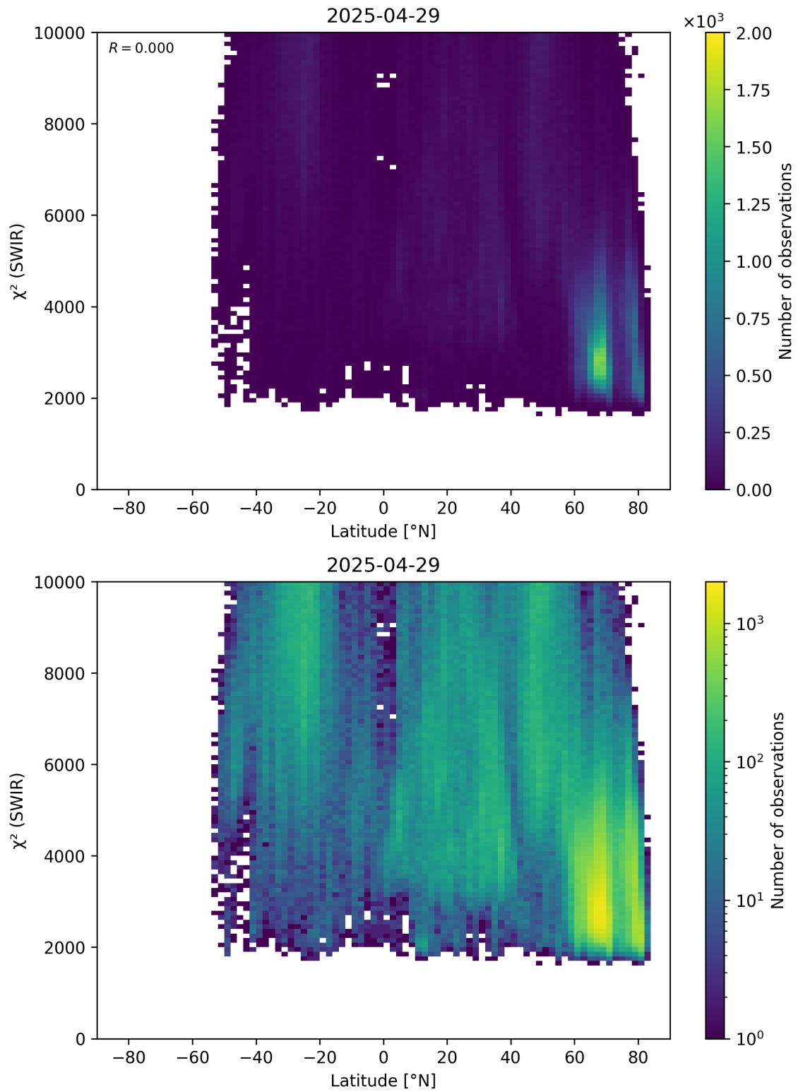
Figure 54: Scatter density plot of “Latitude” against “ \chi^2 (SWIR)” for 2025-04-29 to 2025-04-30.
