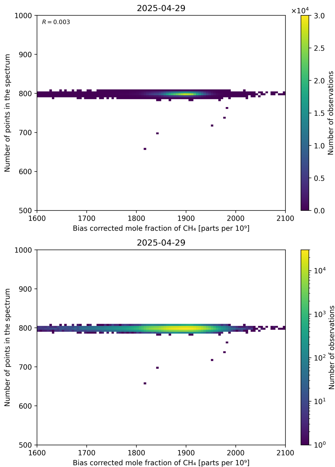
Figure 68: Scatter density plot of “Bias corrected mole fraction of CH 4 ” against “Number of points in the spectrum” for 2025-04-29 to 2025-04-30.
