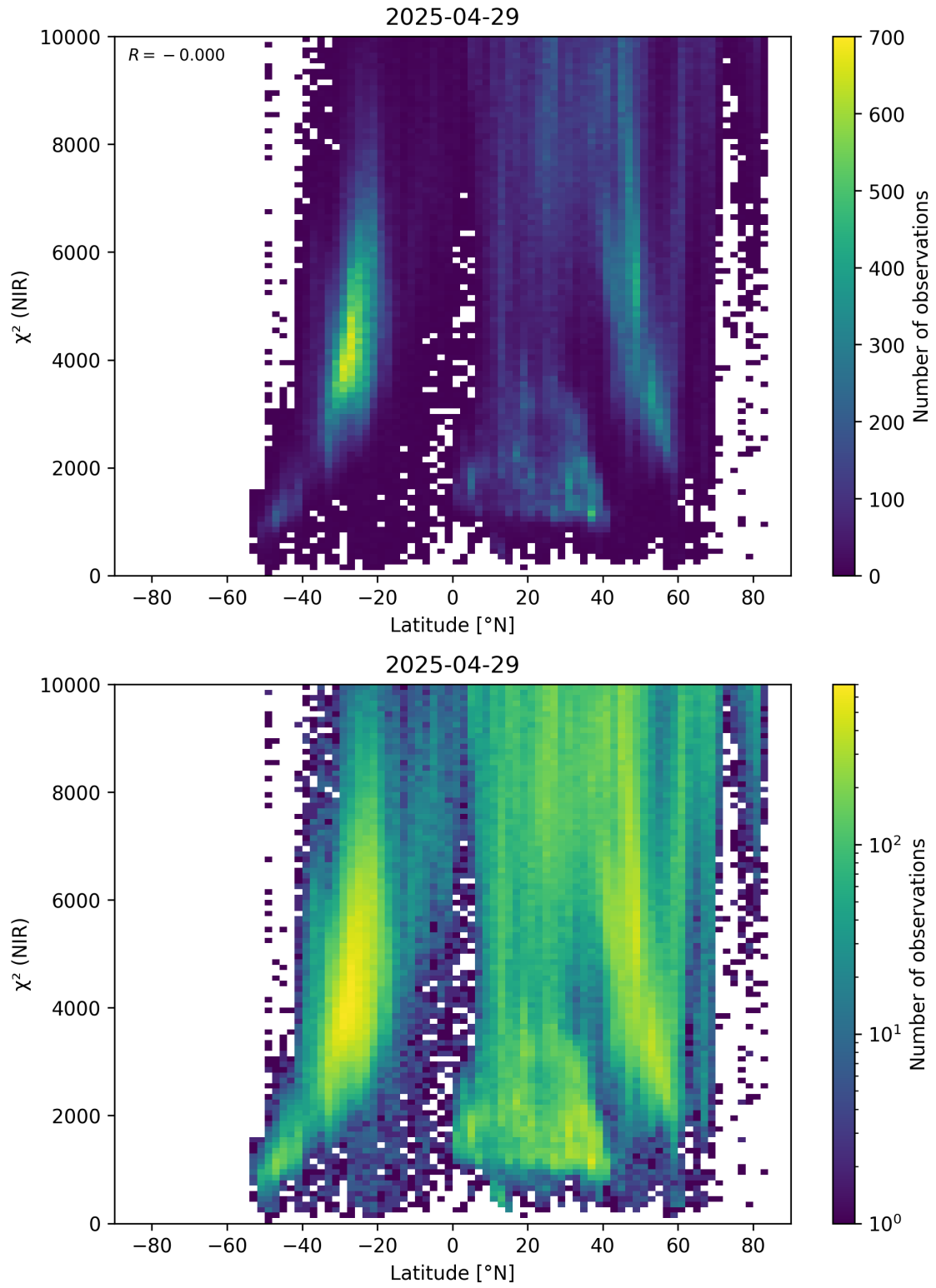
Figure 53: Scatter density plot of “Latitude” against “ \chi^2 (NIR)” for 2025-04-29 to 2025-04-30.
