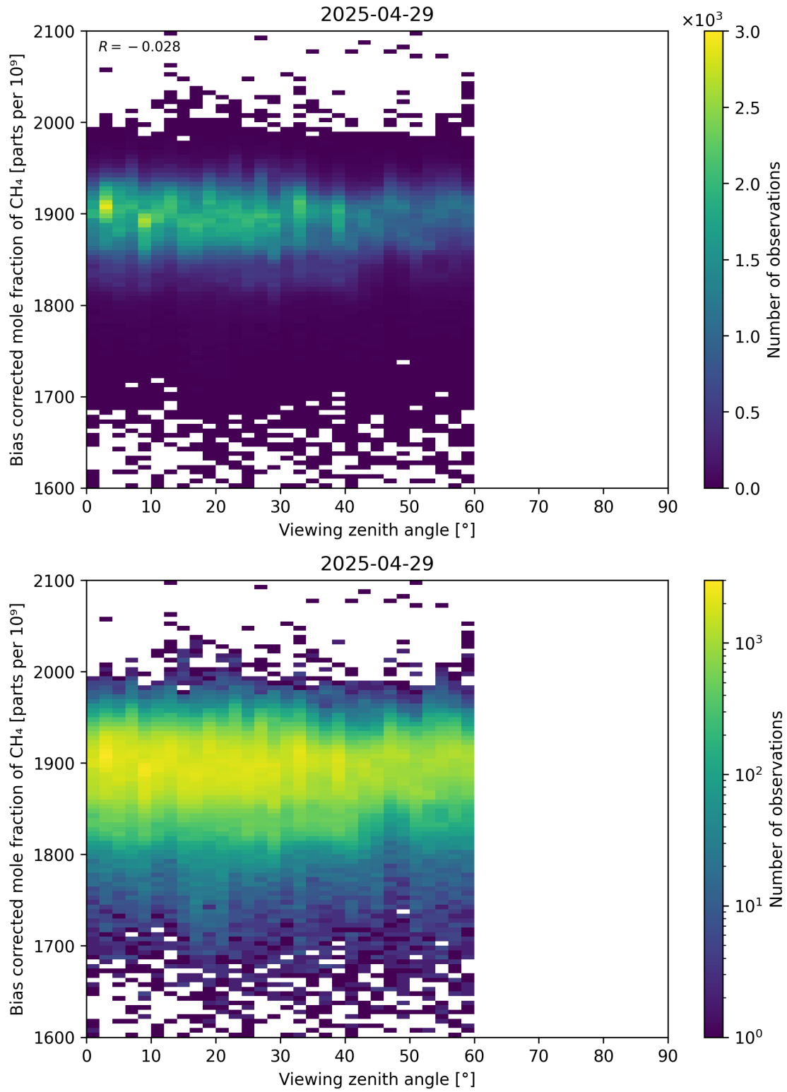
Figure 111: Scatter density plot of “Viewing zenith angle” against “Bias corrected mole fraction of CH 4 ” for 2025-04-29 to 2025-04-30.
