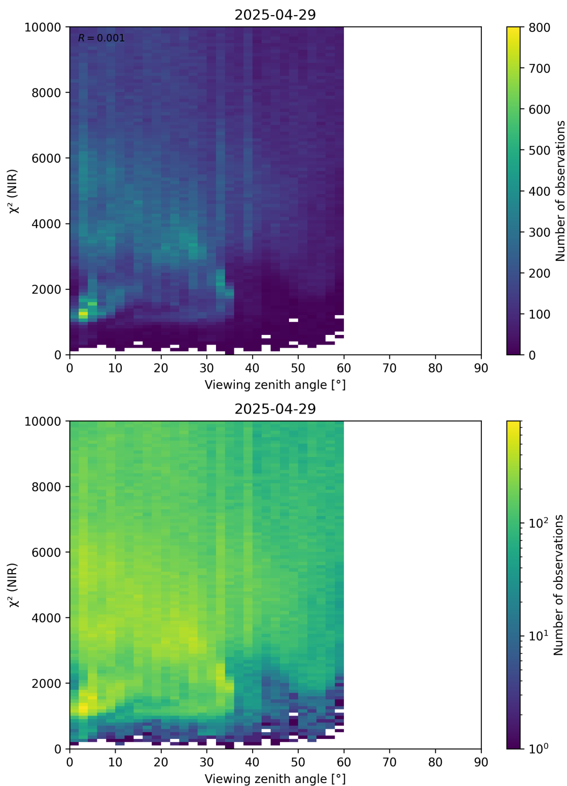
Figure 105: Scatter density plot of “Viewing zenith angle” against “ \chi^2 (NIR)” for 2025-04-29 to 2025-04-30.
