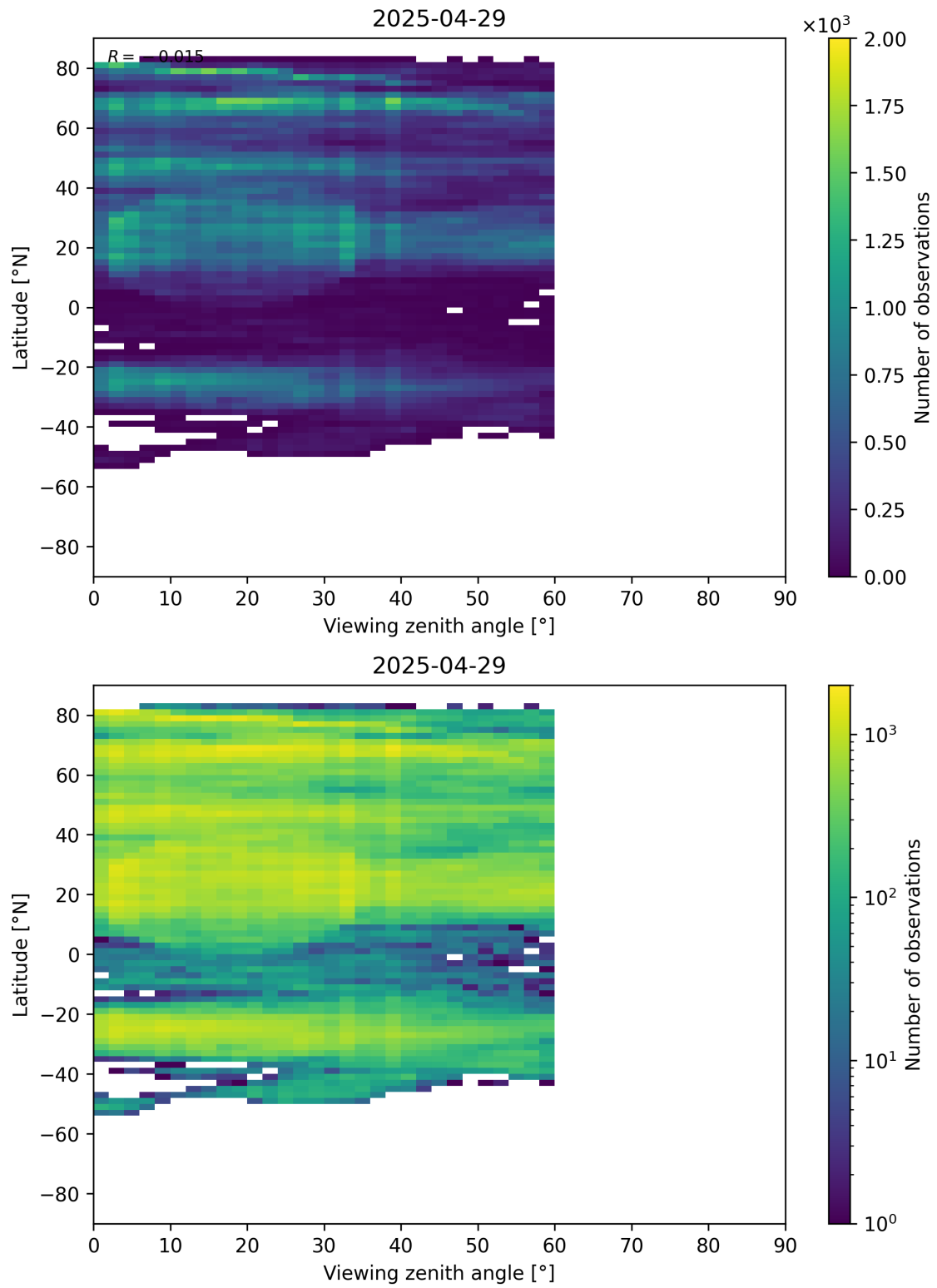
Figure 109: Scatter density plot of “Viewing zenith angle” against “Latitude” for 2025-04-29 to 2025-04-30.
