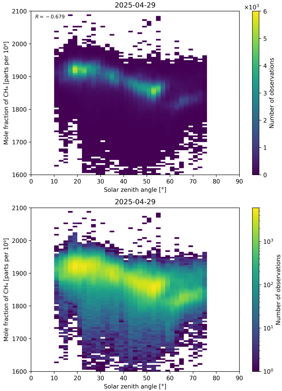
Figure 99: Scatter density plot of “Solar zenith angle” against “Mole fraction of CH 4 ” for 2025-04-29 to 2025-04-30.
