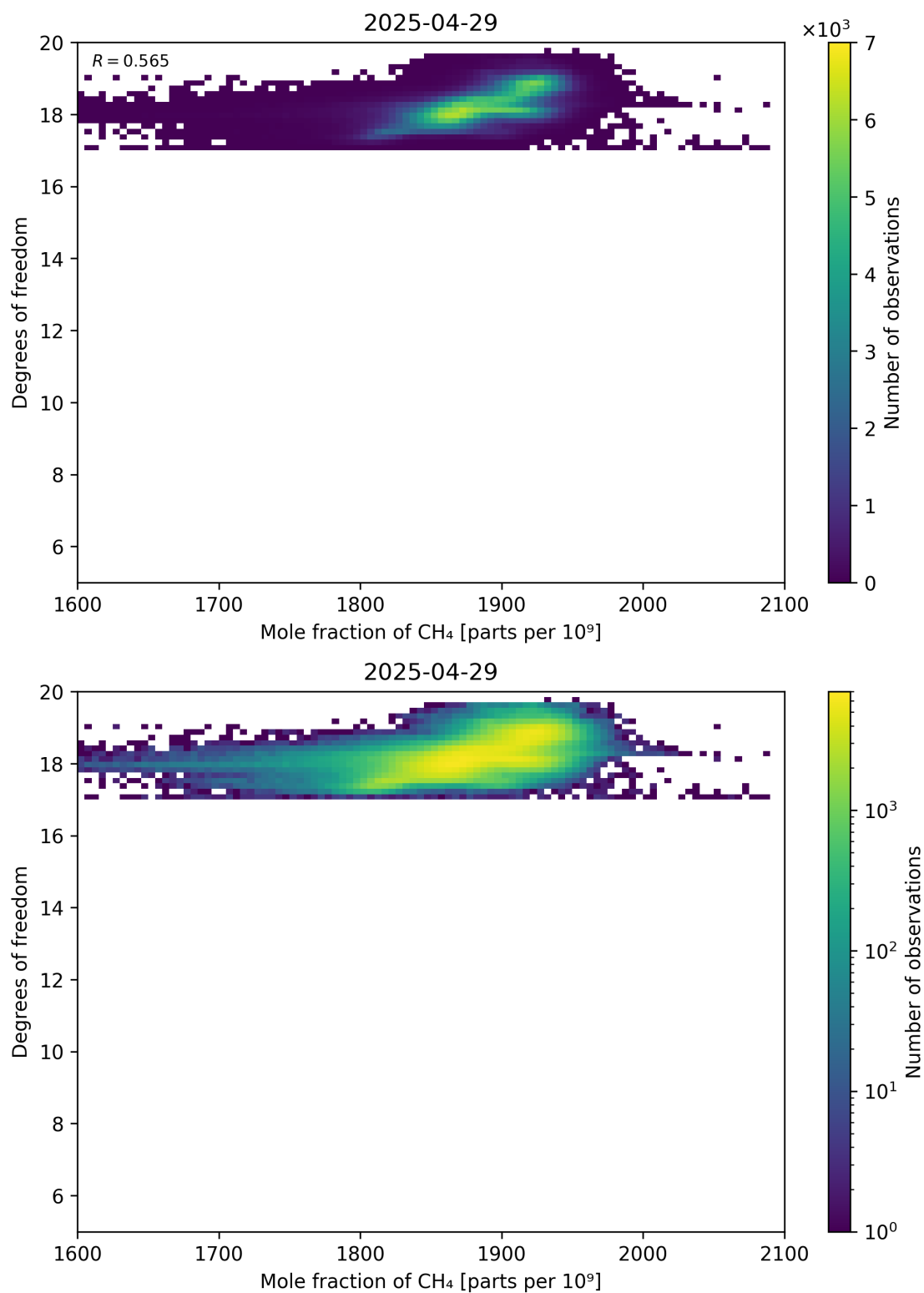
Figure 72: Scatter density plot of “Mole fraction of CH 4 ” against “Degrees of freedom” for 2025-04-29 to 2025-04-30.
