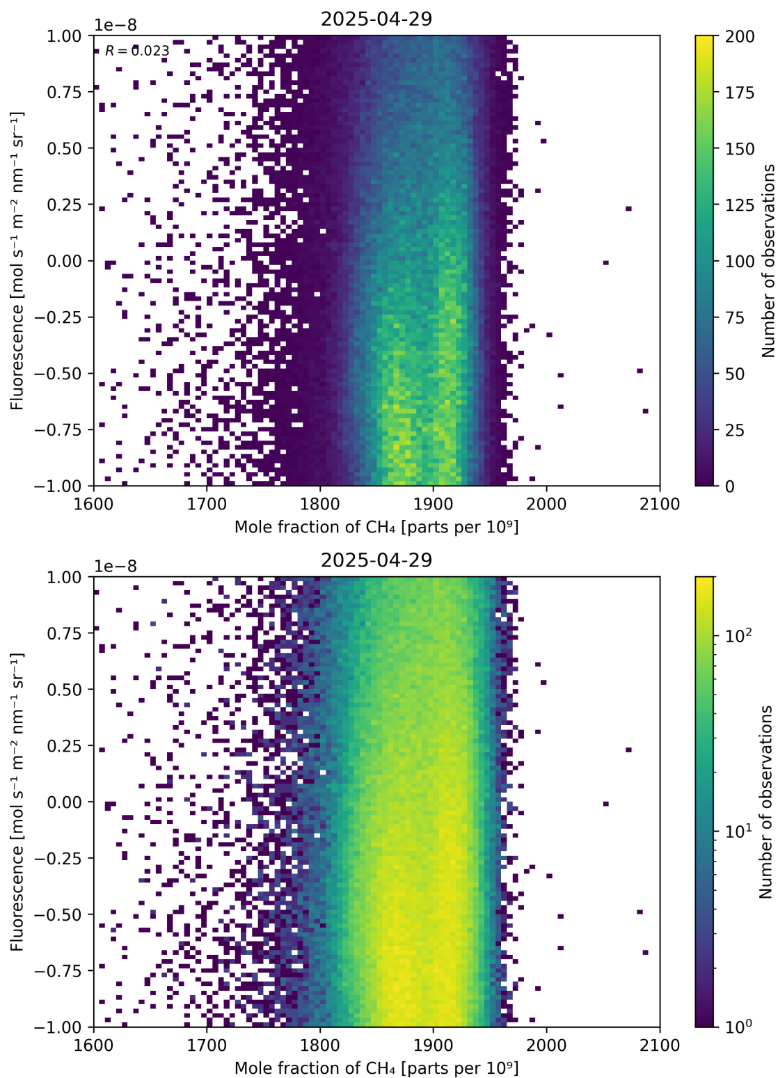
Figure 73: Scatter density plot of “Mole fraction of \text{CH}_4 ” against “Fluorescence” for 2025-04-29 to 2025-04-30.
