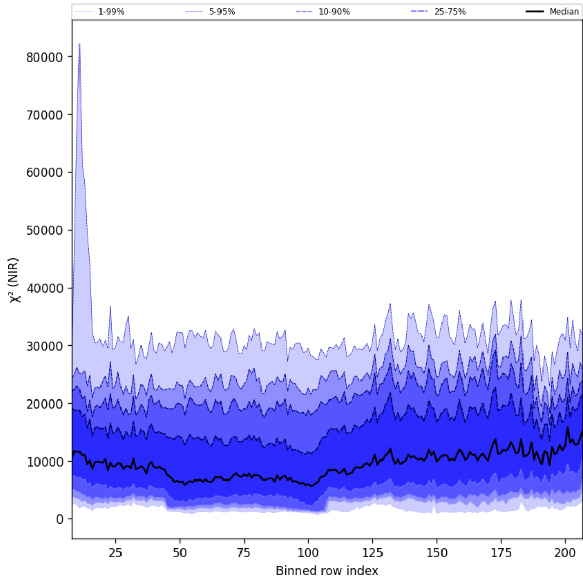
Figure 40: Along track statistics of “ \chi^2 (NIR)” for 2025-04-29 to 2025-04-30
