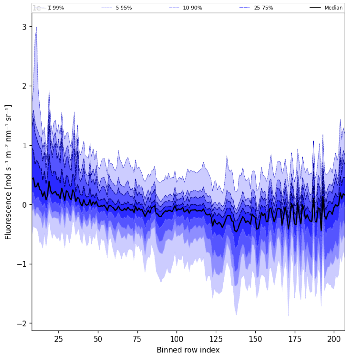
Figure 43: Along track statistics of “Fluorescence” for 2025-04-29 to 2025-04-30
