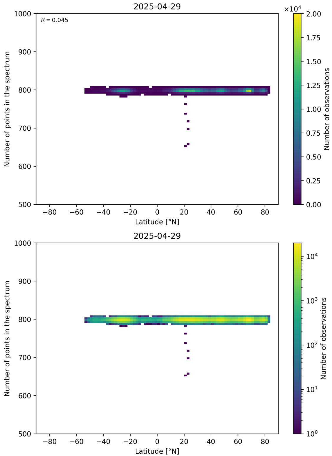
Figure 61: Scatter density plot of “Latitude” against “Number of points in the spectrum” for 2025-04-29 to 2025-04-30.
