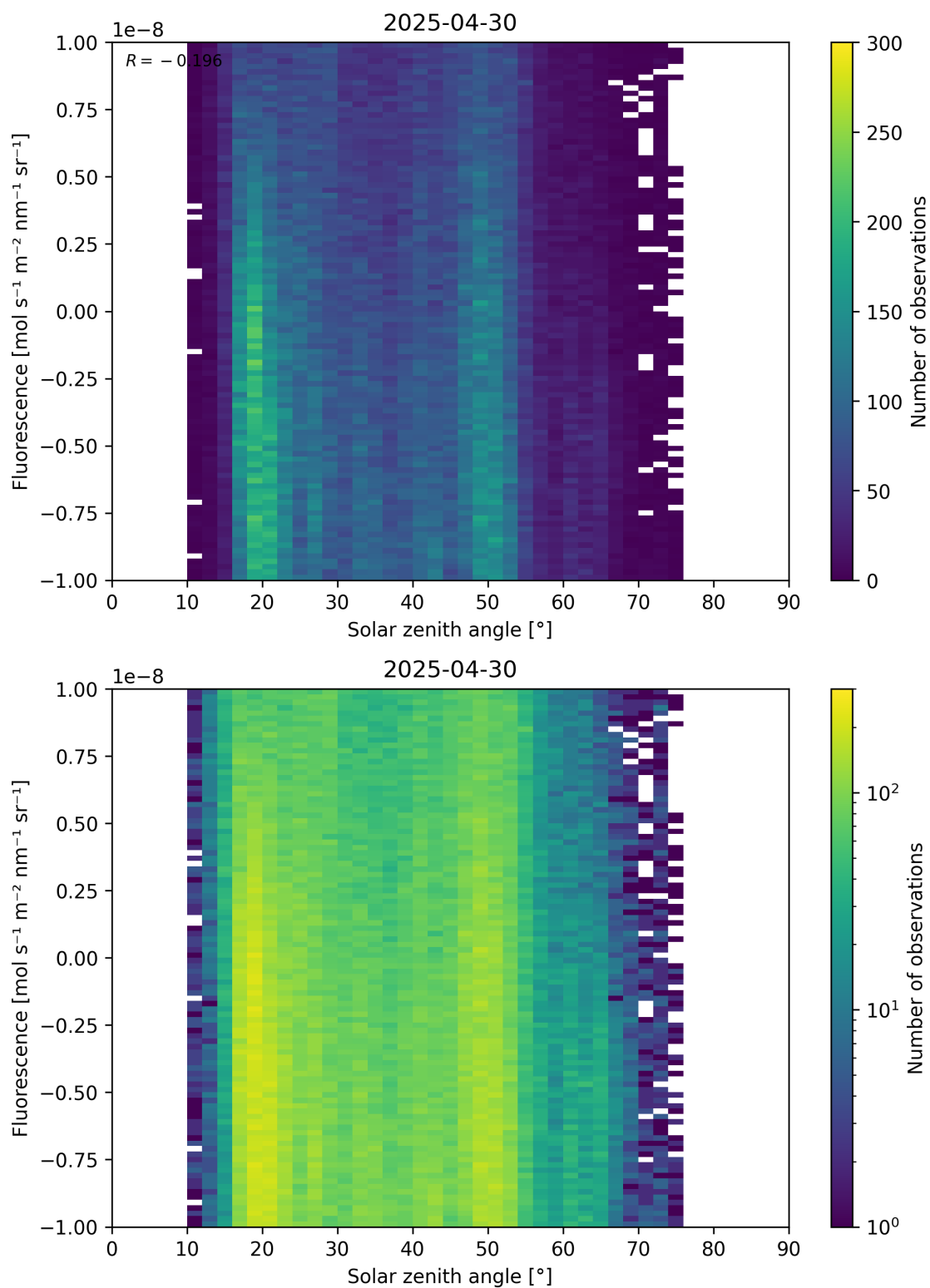
Figure 97: Scatter density plot of “Solar zenith angle” against “Fluorescence” for 2025-04-29 to 2025-05-01.
