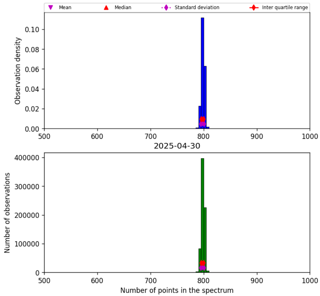
Figure 26: Histogram of “Number of points in the spectrum” for 2025-04-29 to 2025-05-01
