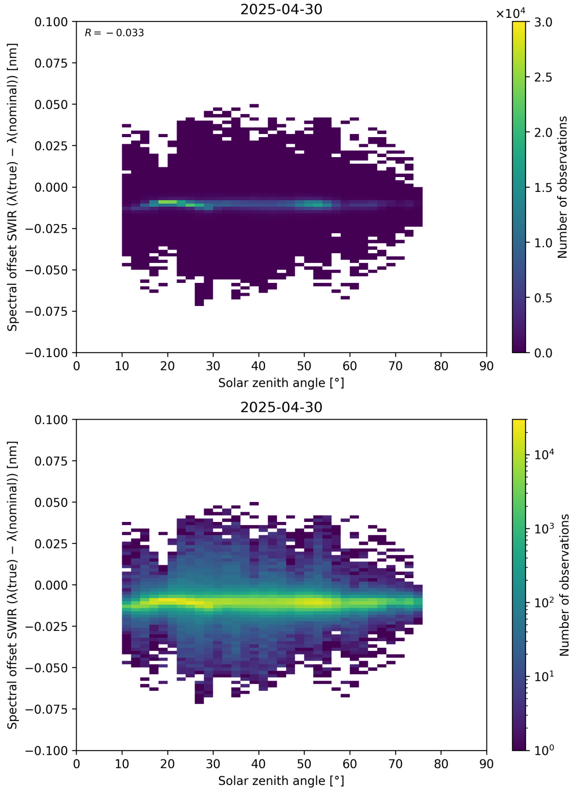
Figure 104: Scatter density plot of “Solar zenith angle” against “Spectral offset SWIR ( \lambda_{\text{true}} - \lambda_{\text{nominal}} )” for 2025-04-29 to 2025-05-01.
