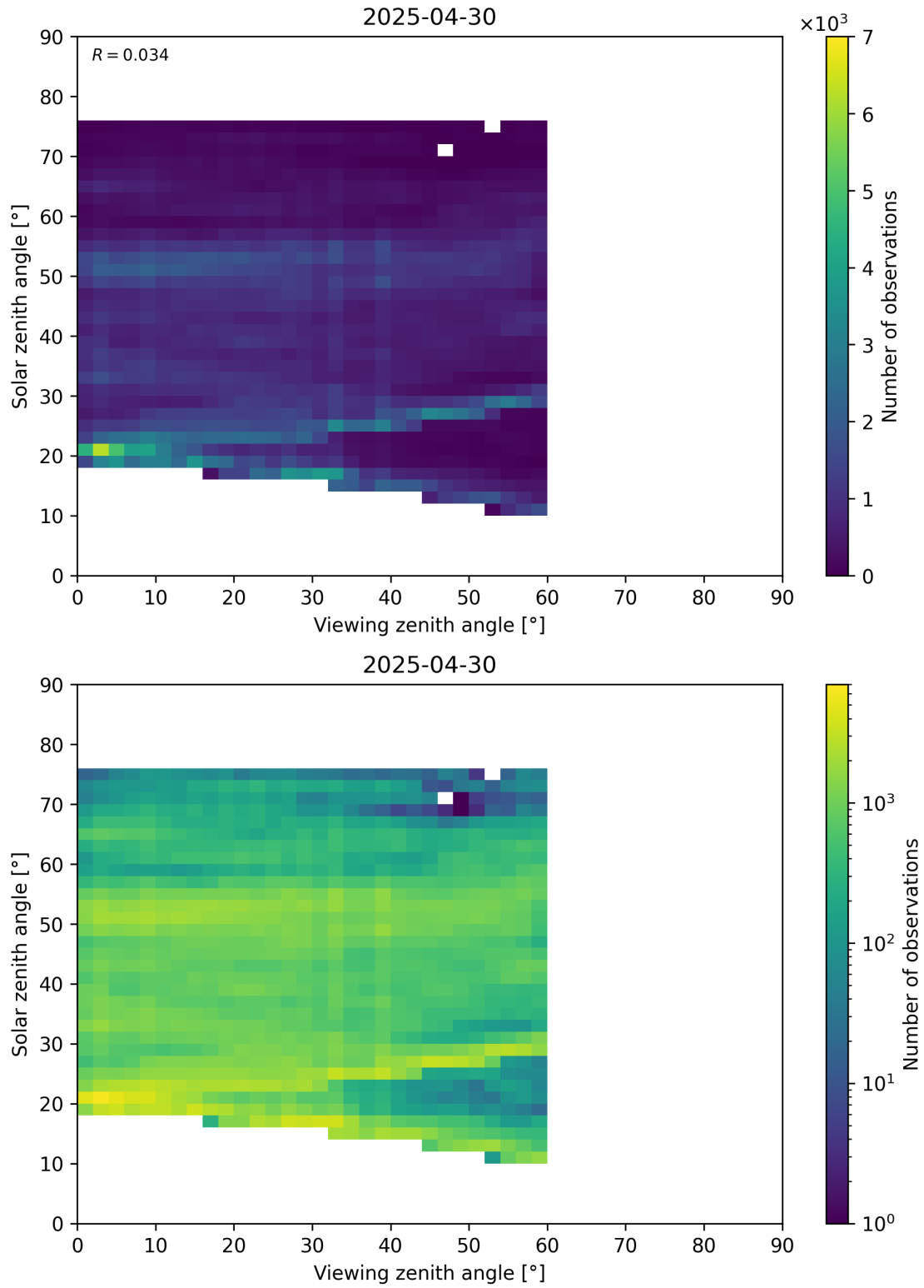
Figure 115: Scatter density plot of “Viewing zenith angle” against “Solar zenith angle” for 2025-04-29 to 2025-05-01.
