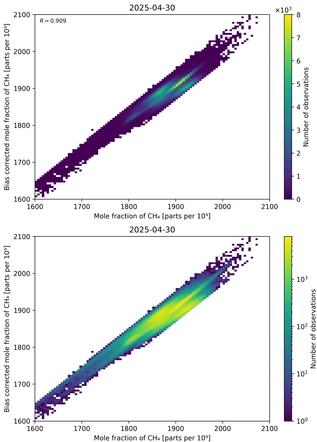
Figure 74: Scatter density plot of “Mole fraction of CH 4 ” against “Bias corrected mole fraction of CH 4 ” for 2025-04-29 to 2025-05-01.
