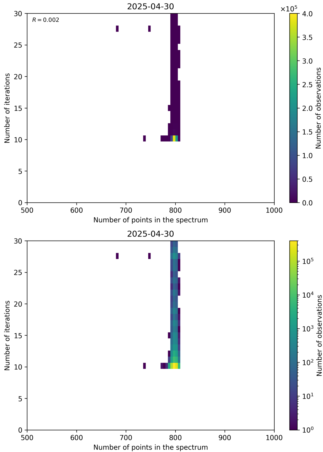
Figure 92: Scatter density plot of “Number of points in the spectrum” against “Number of iterations” for 2025-04-29 to 2025-05-01.
