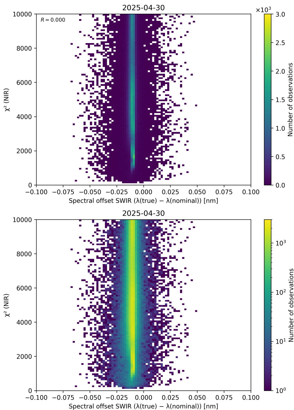
Figure 117: Scatter density plot of “Spectral offset SWIR ( \lambda_{\text{true}} - \lambda_{\text{nominal}} )” against “ \chi^2 (NIR)” for 2025-04-29 to 2025-05-01.
