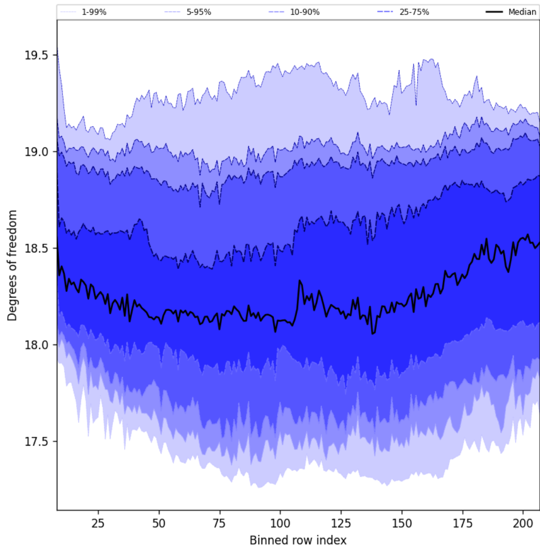
Figure 41: Along track statistics of “Degrees of freedom” for 2025-04-29 to 2025-05-01
