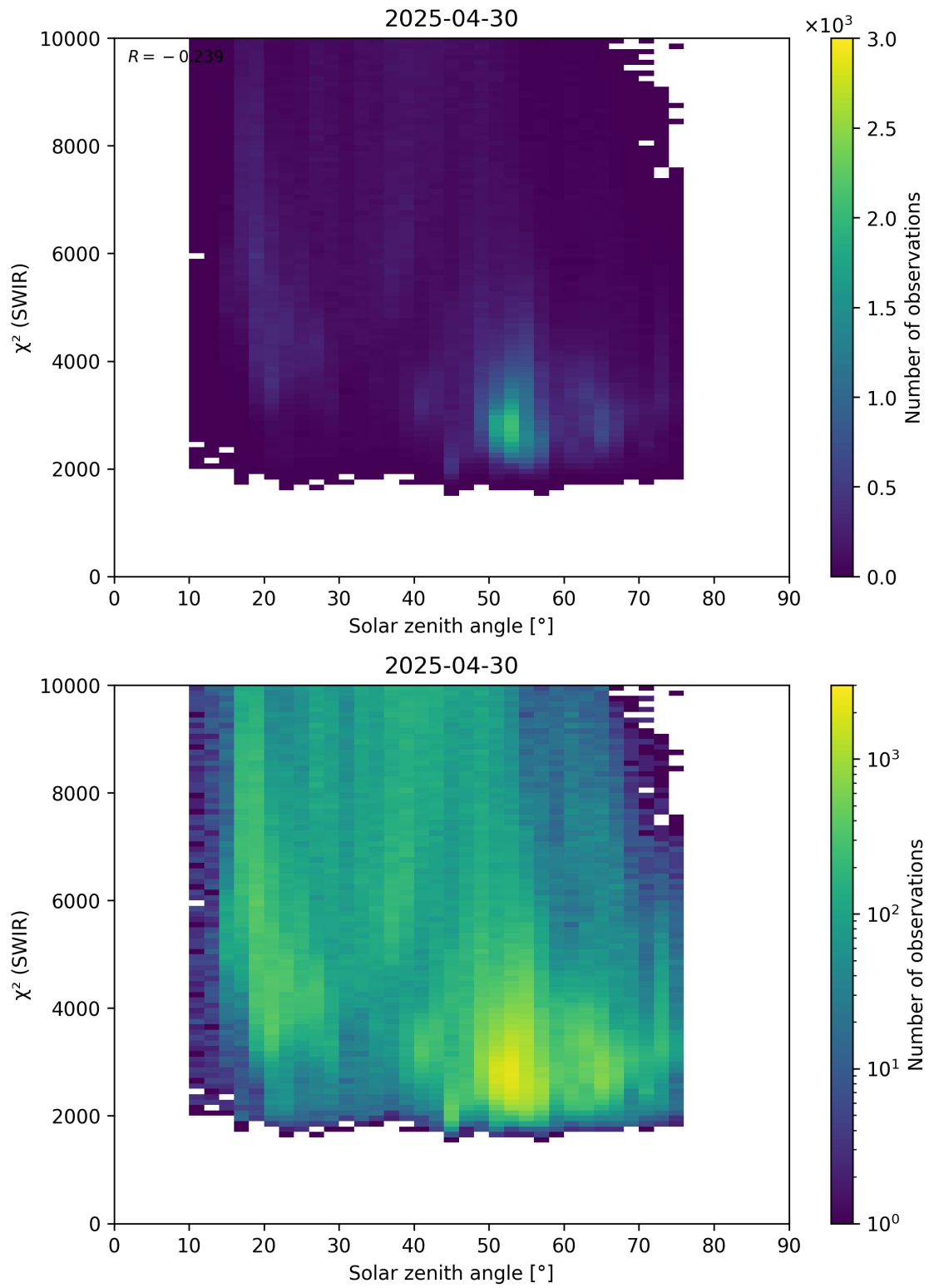
Figure 95: Scatter density plot of “Solar zenith angle” against “ \chi^2 (SWIR)” for 2025-04-29 to 2025-05-01.
