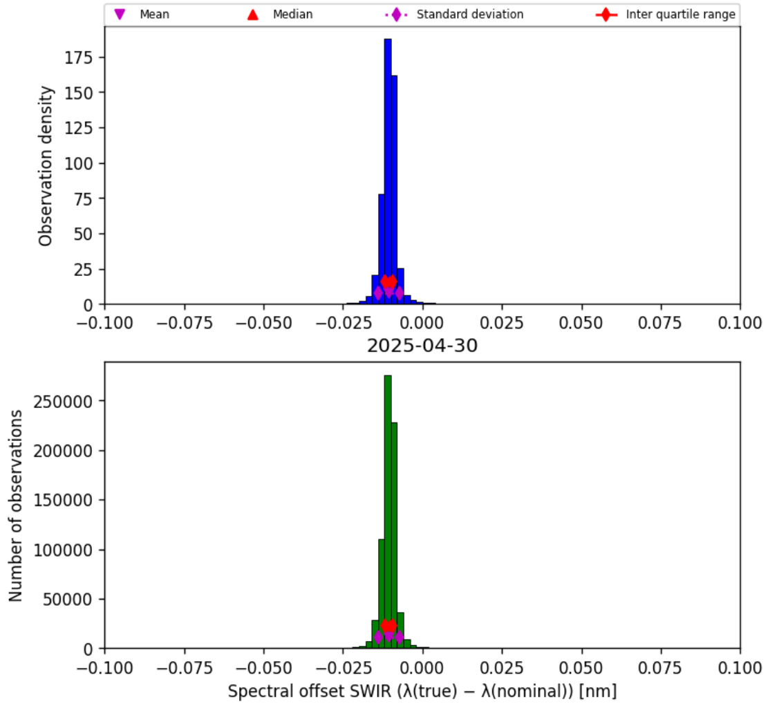
Figure 27: Histogram of “Spectral offset SWIR ( \lambda_{\text{true}} - \lambda_{\text{nominal}} )” for 2025-04-29 to 2025-05-01
