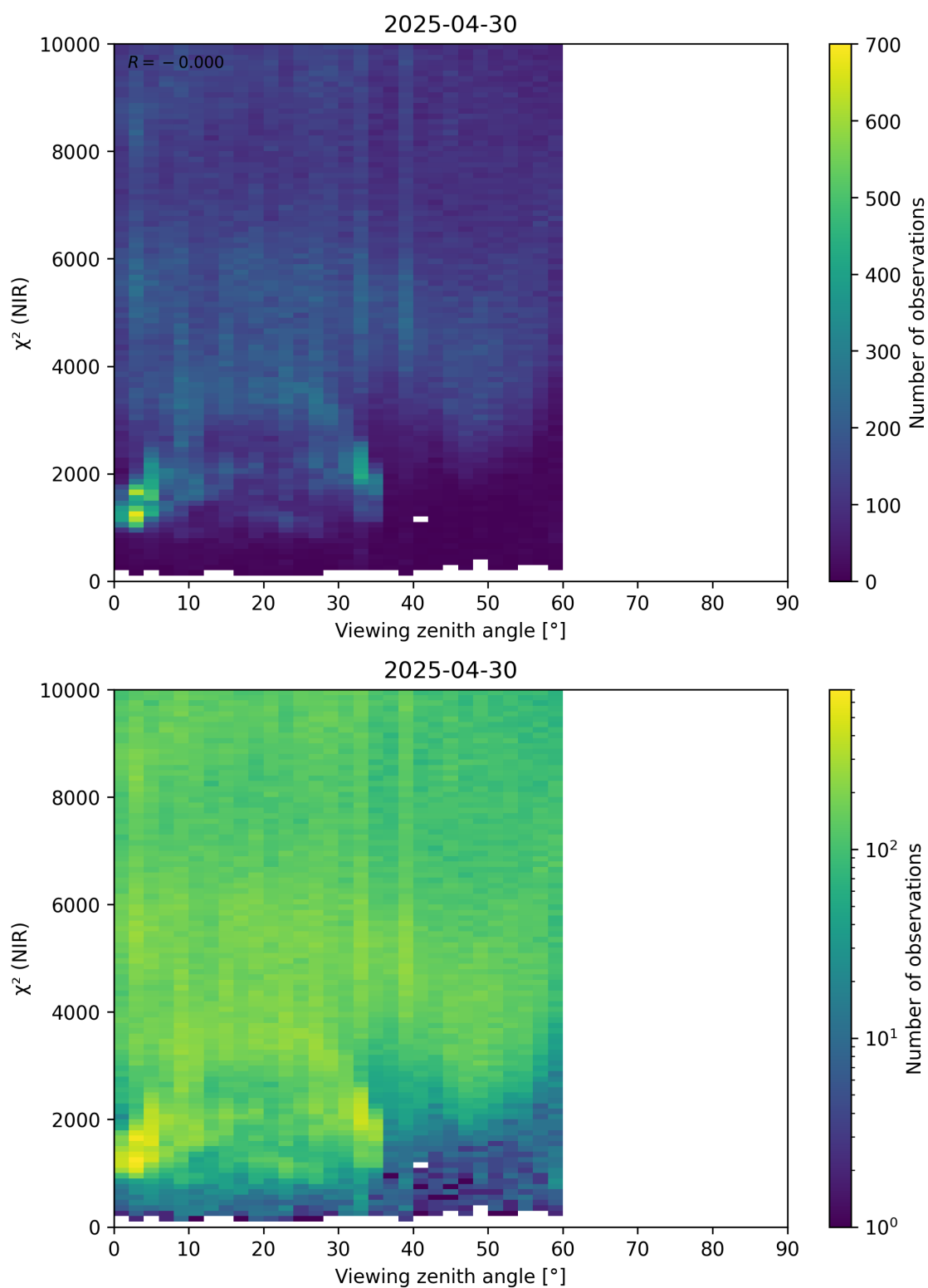
Figure 105: Scatter density plot of “Viewing zenith angle” against “ \chi^2 (NIR)” for 2025-04-29 to 2025-05-01.
