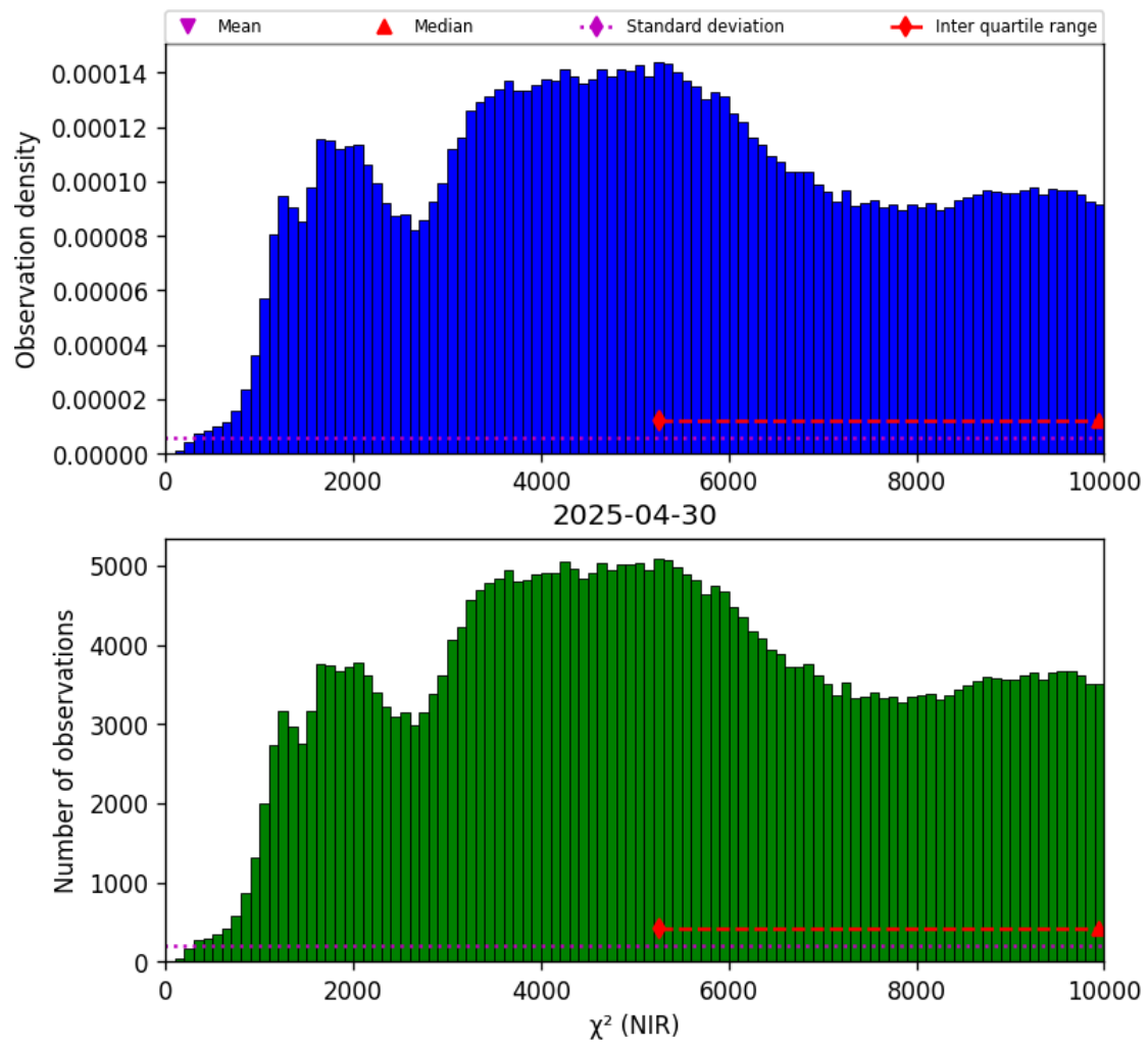
Figure 29: Histogram of “ \chi^2 (NIR)” for 2025-04-29 to 2025-05-01
