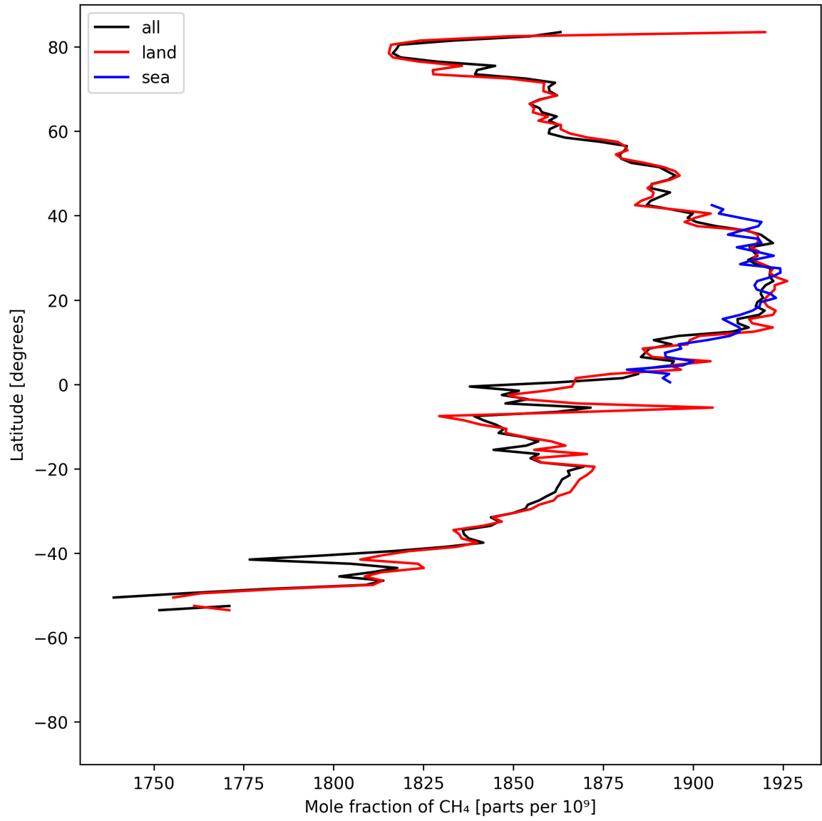
Figure 12: Zonal average of “Mole fraction of \text{CH}_4 ” for 2025-04-29 to 2025-05-01.
