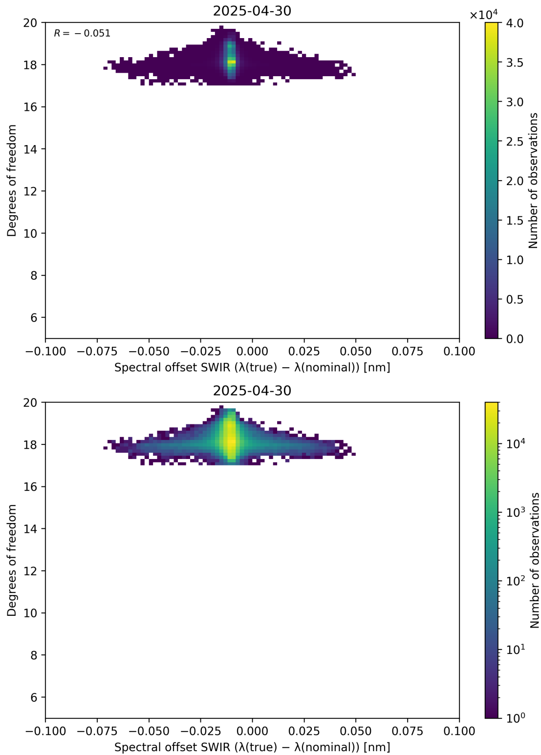
Figure 119: Scatter density plot of “Spectral offset SWIR ( \lambda_{\text{true}} - \lambda_{\text{nominal}} )” against “Degrees of freedom” for 2025-04-29 to 2025-05-01.
