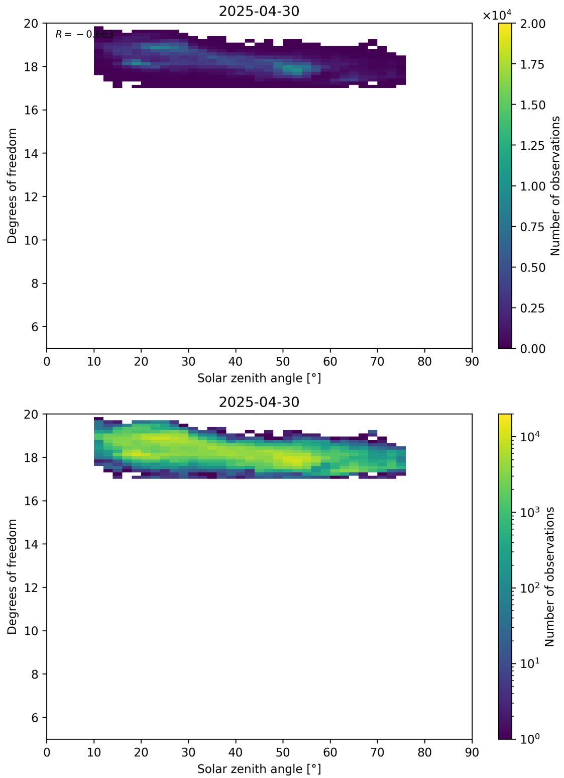
Figure 96: Scatter density plot of “Solar zenith angle” against “Degrees of freedom” for 2025-04-29 to 2025-05-01.
