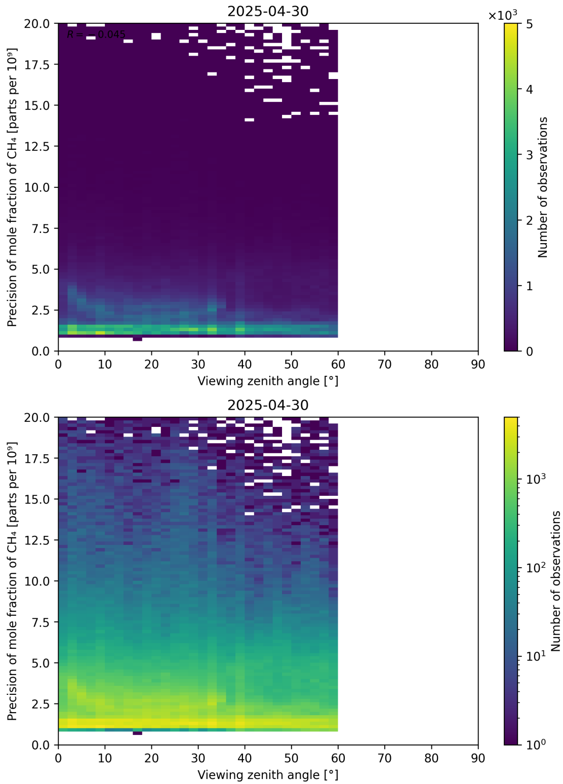
Figure 112: Scatter density plot of “Viewing zenith angle” against “Precision of mole fraction of CH 4 ” for 2025-04-29 to 2025-05-01.
