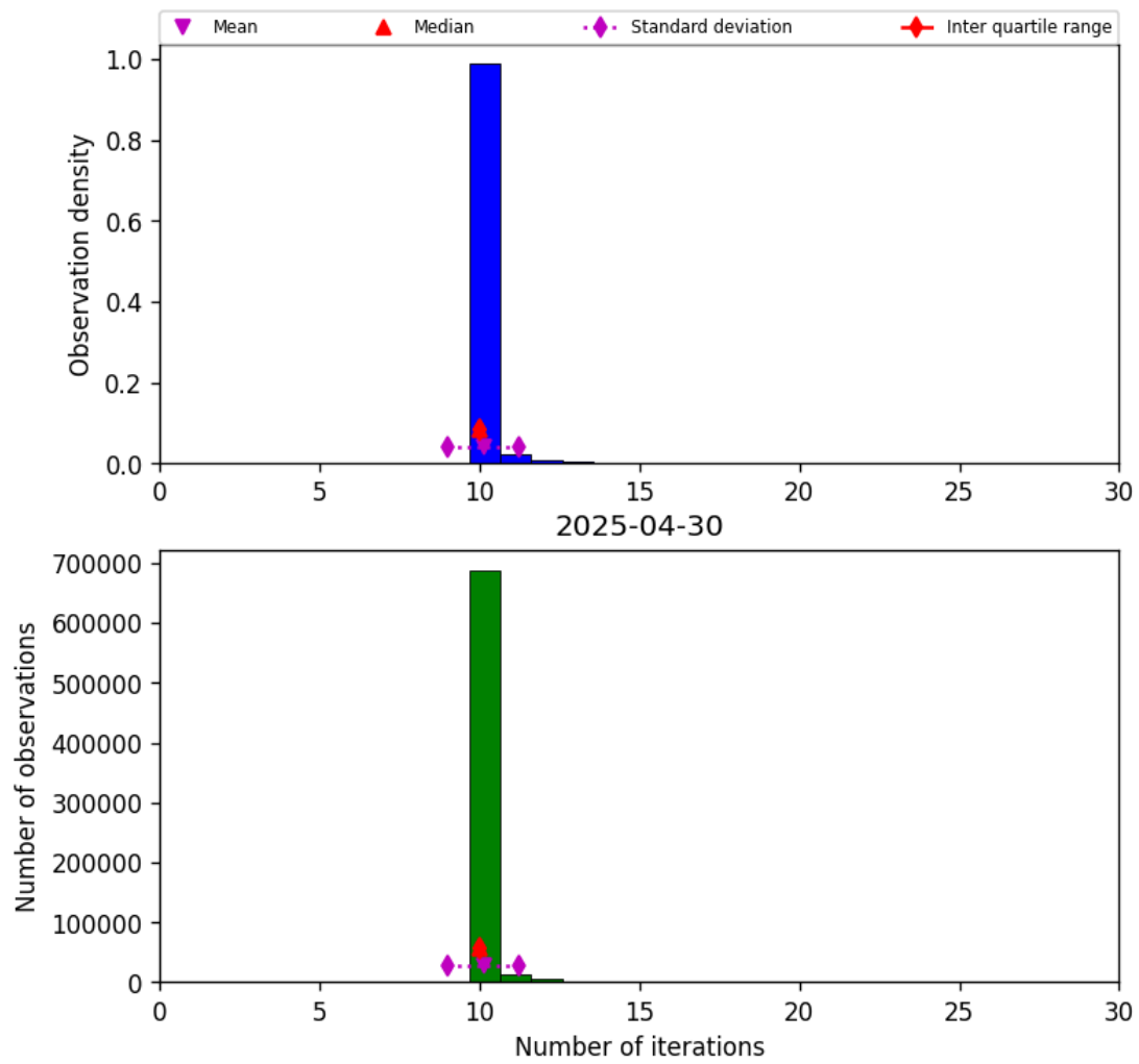
Figure 31: Histogram of “Number of iterations” for 2025-04-29 to 2025-05-01
