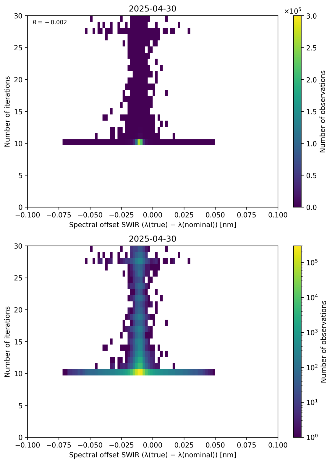
Figure 121: Scatter density plot of “Spectral offset SWIR ( \lambda_{\text{true}} - \lambda_{\text{nominal}} )” against “Number of iterations” for 2025-04-29 to 2025-05-01.
