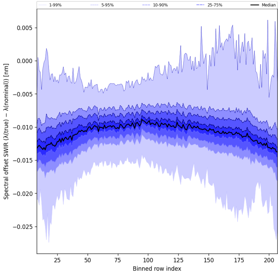
Figure 38: Along track statistics of “Spectral offset SWIR ( \lambda_{\text{true}} - \lambda_{\text{nominal}} )” for 2025-04-29 to 2025-05-01
