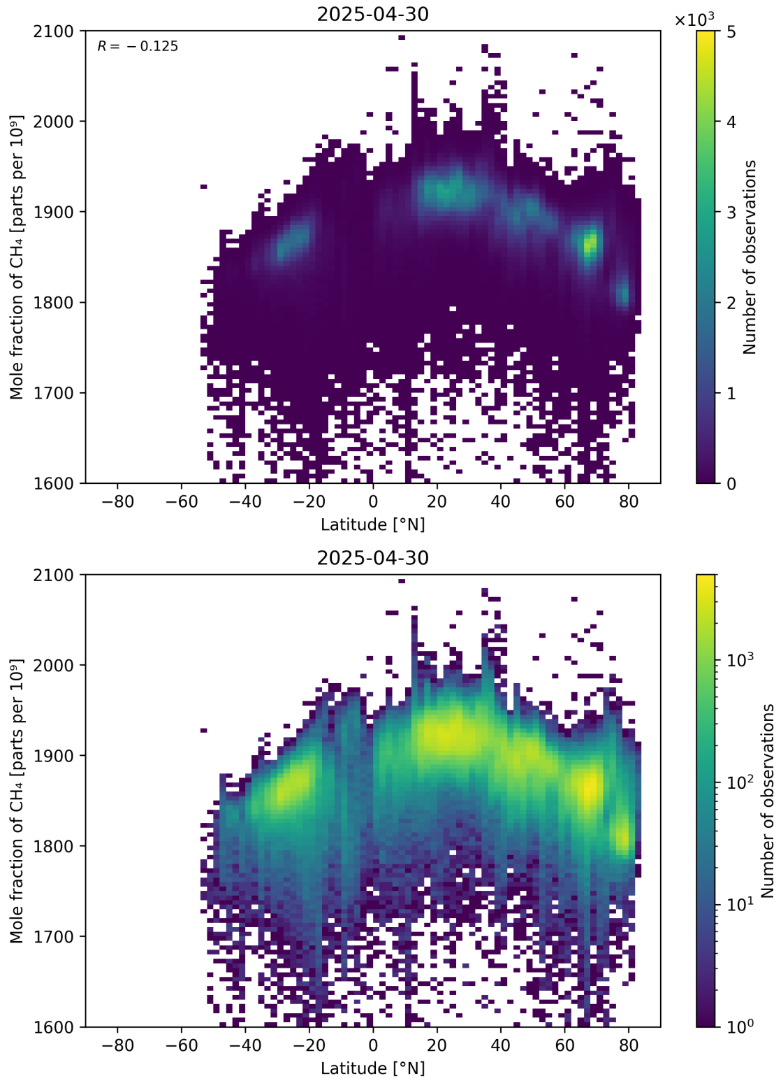
Figure 57: Scatter density plot of “Latitude” against “Mole fraction of CH 4 ” for 2025-04-29 to 2025-05-01.
