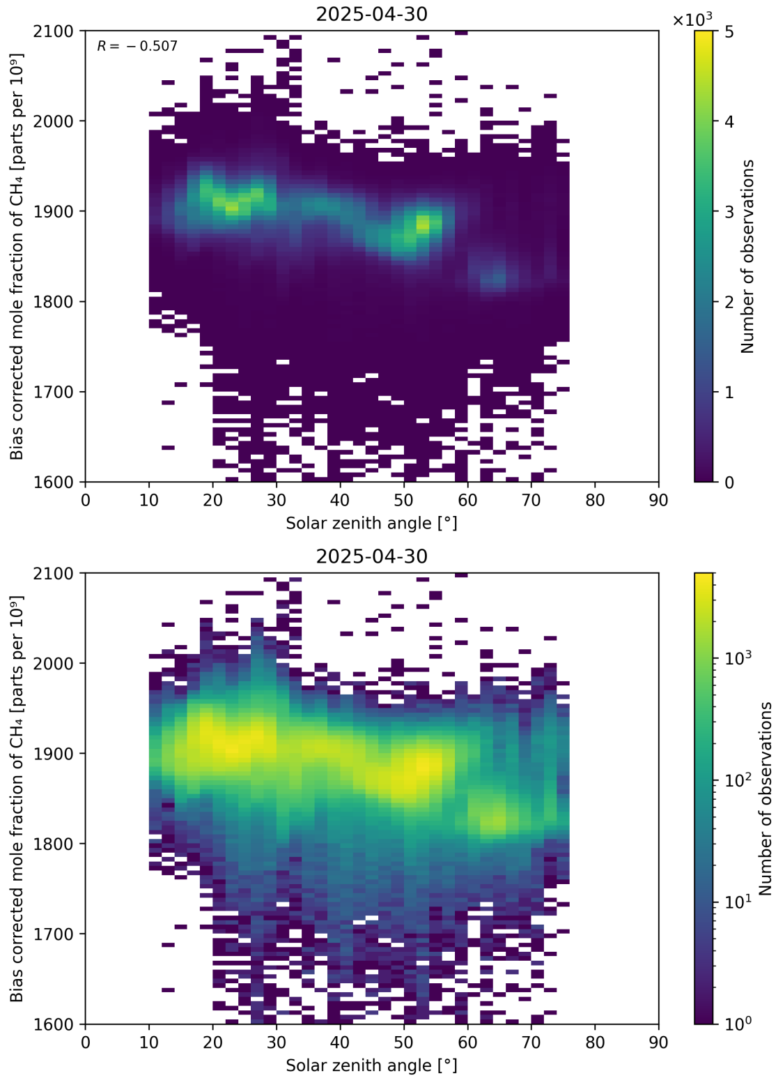
Figure 100: Scatter density plot of “Solar zenith angle” against “Bias corrected mole fraction of \text{CH}_4 ” for 2025-04-29 to 2025-05-01.
