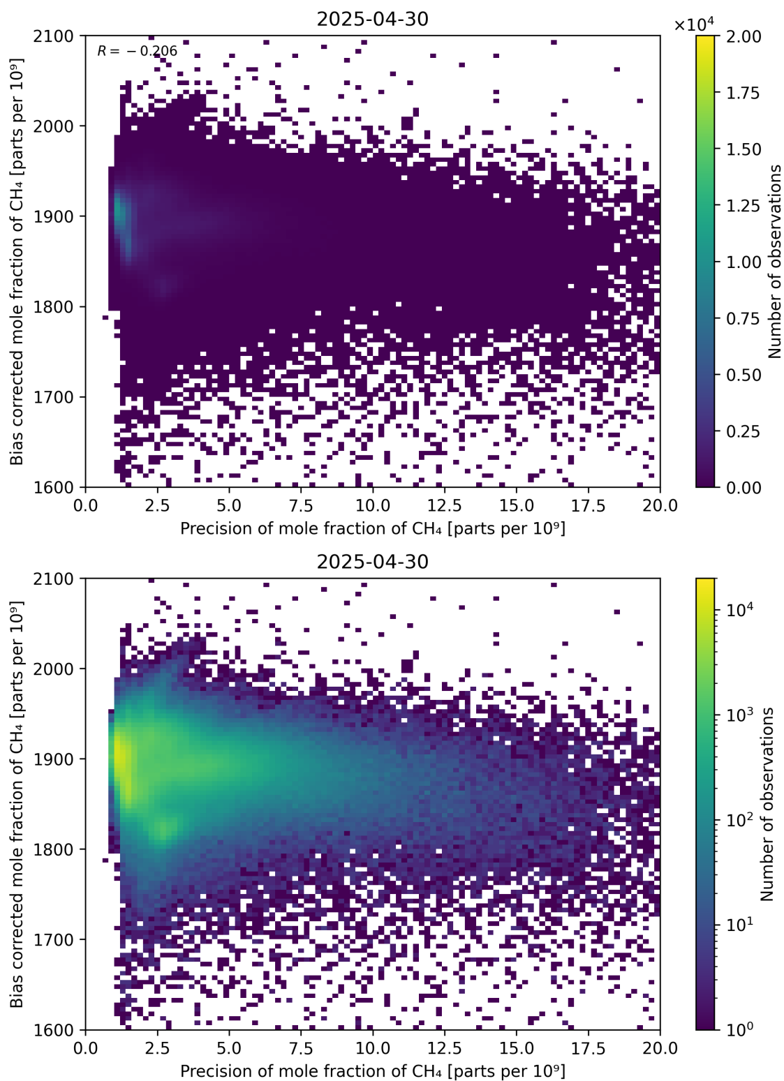
Figure 82: Scatter density plot of “Precision of mole fraction of CH 4 ” against “Bias corrected mole fraction of CH 4 ” for 2025-04-29 to 2025-05-01.
