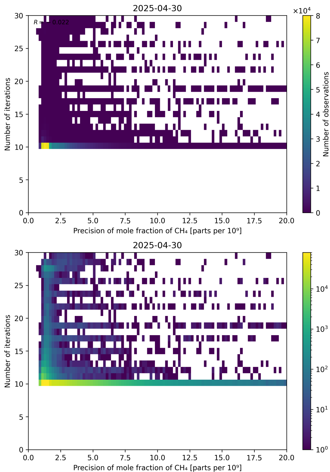
Figure 83: Scatter density plot of “Precision of mole fraction of CH 4 ” against “Number of iterations” for 2025-04-29 to 2025-05-01.
