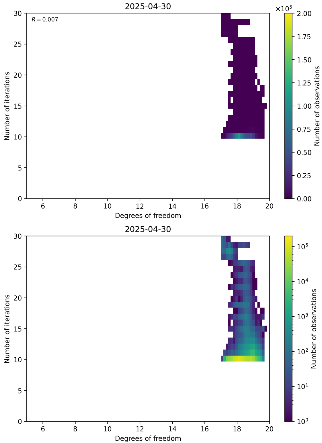
Figure 52: Scatter density plot of “Degrees of freedom” against “Number of iterations” for 2025-04-29 to 2025-05-01.
