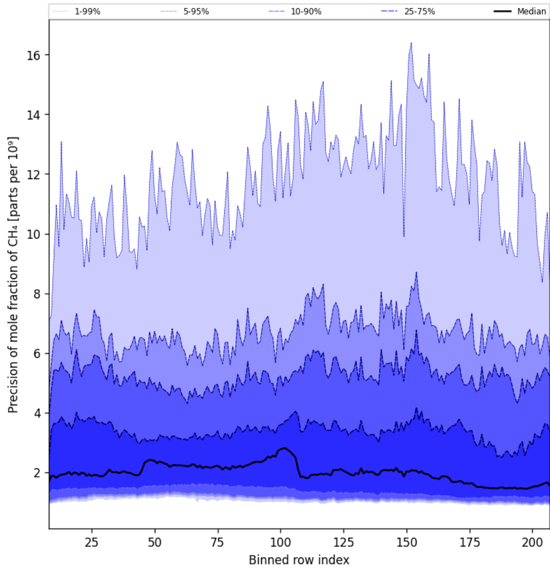
Figure 35: Along track statistics of "Precision of mole fraction of CH 4 " for 2025-04-29 to 2025-05-01
