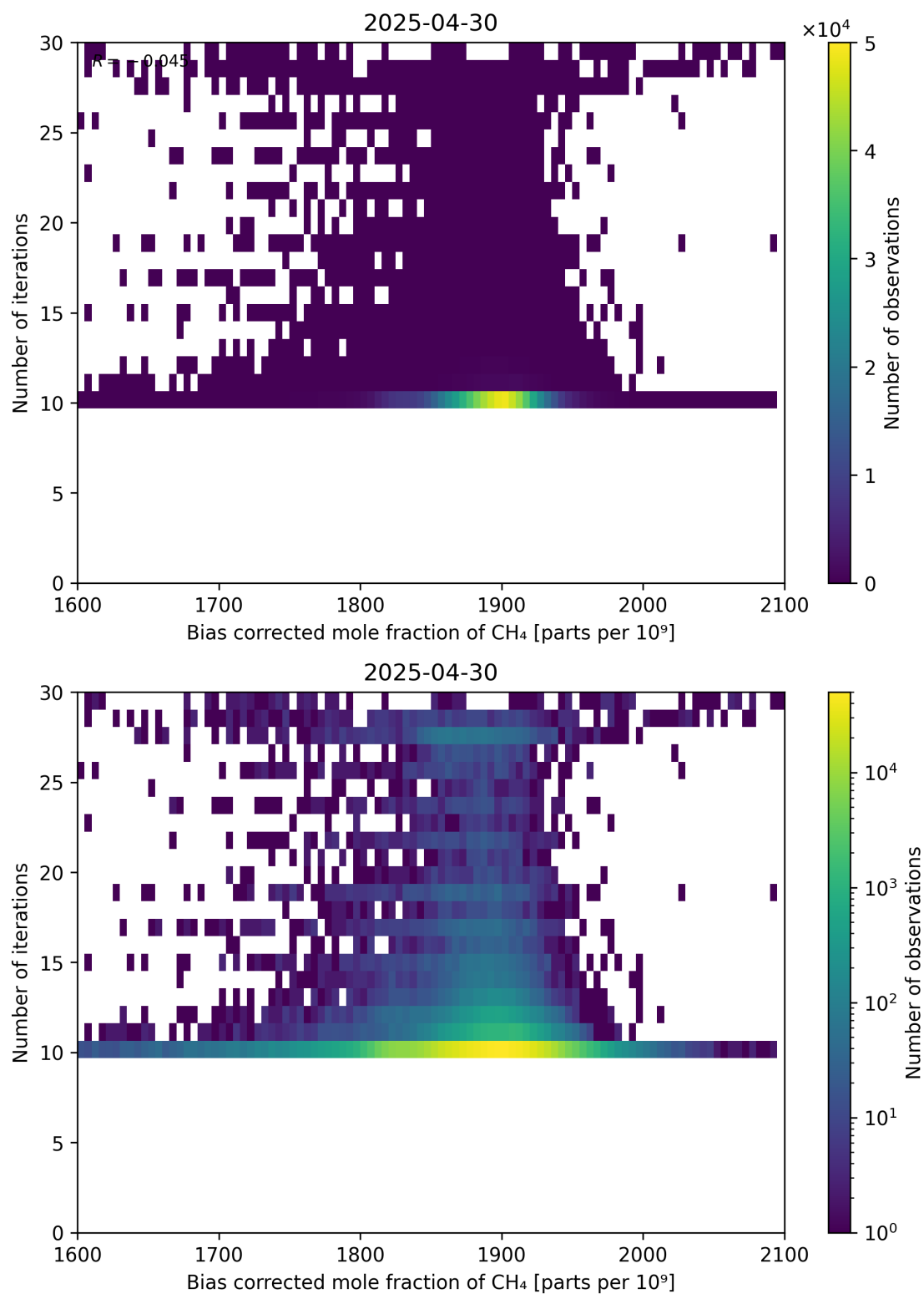
Figure 67: Scatter density plot of “Bias corrected mole fraction of CH 4 ” against “Number of iterations” for 2025-04-29 to 2025-05-01.
