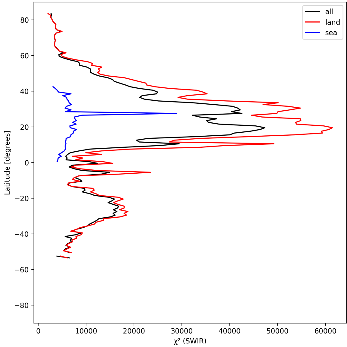
Figure 17: Zonal average of “ \chi^2 (SWIR)” for 2025-04-29 to 2025-05-01.
