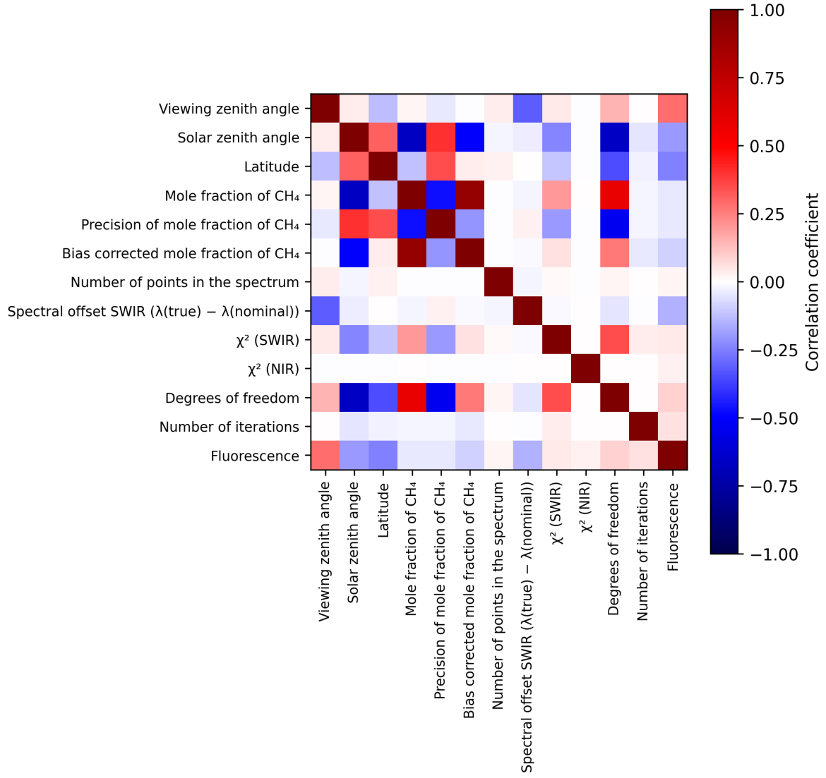
Figure 2: Map of correlation matrix for 2025-04-29 to 2025-05-01.
