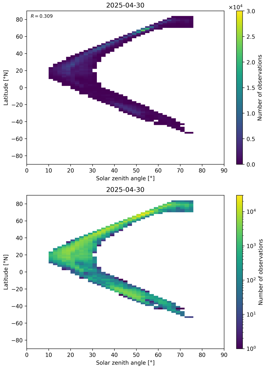
Figure 98: Scatter density plot of “Solar zenith angle” against “Latitude” for 2025-04-29 to 2025-05-01.
