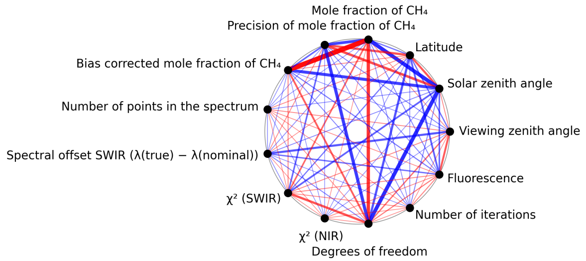
Figure 1: Map of correlation graph for 2025-04-29 to 2025-05-01.
