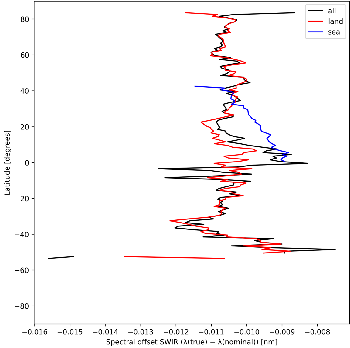
Figure 16: Zonal average of “Spectral offset SWIR ( \lambda_{\text{true}} - \lambda_{\text{nominal}} )” for 2025-04-29 to 2025-05-01.
