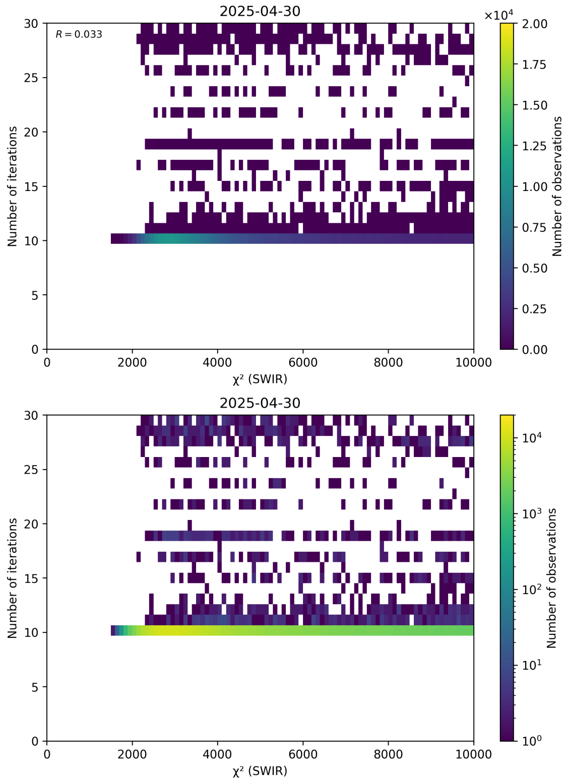
Figure 50: Scatter density plot of “ \chi^2 (SWIR)” against “Number of iterations” for 2025-04-29 to 2025-05-01.
