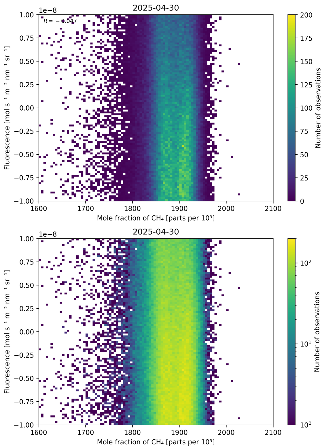
Figure 73: Scatter density plot of “Mole fraction of \text{CH}_4 ” against “Fluorescence” for 2025-04-29 to 2025-05-01.
