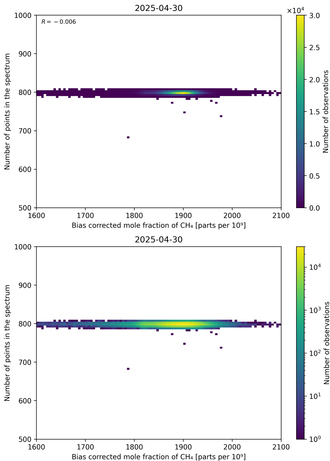
Figure 68: Scatter density plot of “Bias corrected mole fraction of CH 4 ” against “Number of points in the spectrum” for 2025-04-29 to 2025-05-01.
