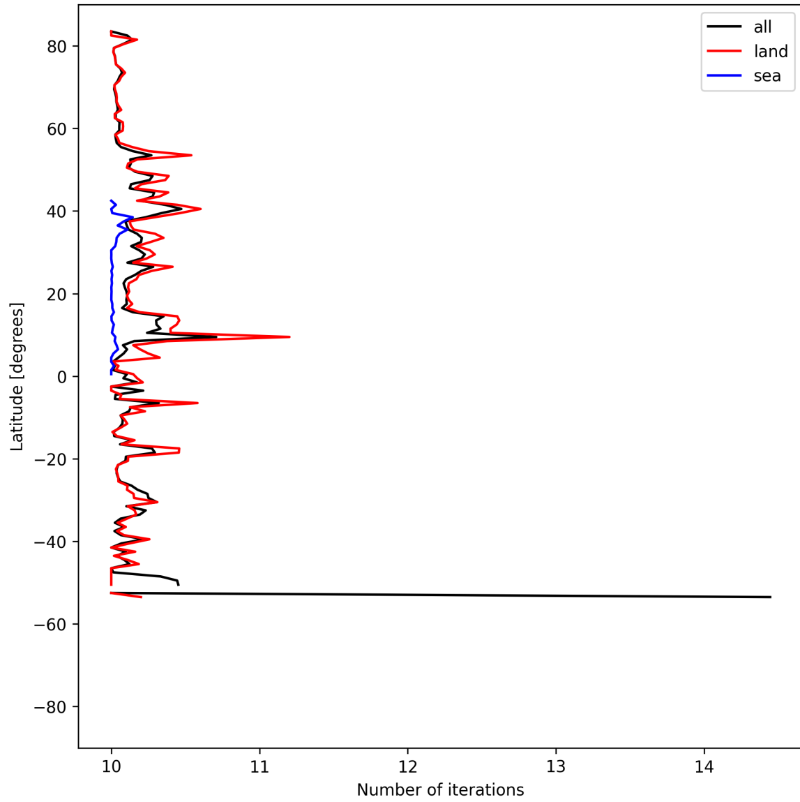
Figure 20: Zonal average of “Number of iterations” for 2025-04-29 to 2025-05-01.
