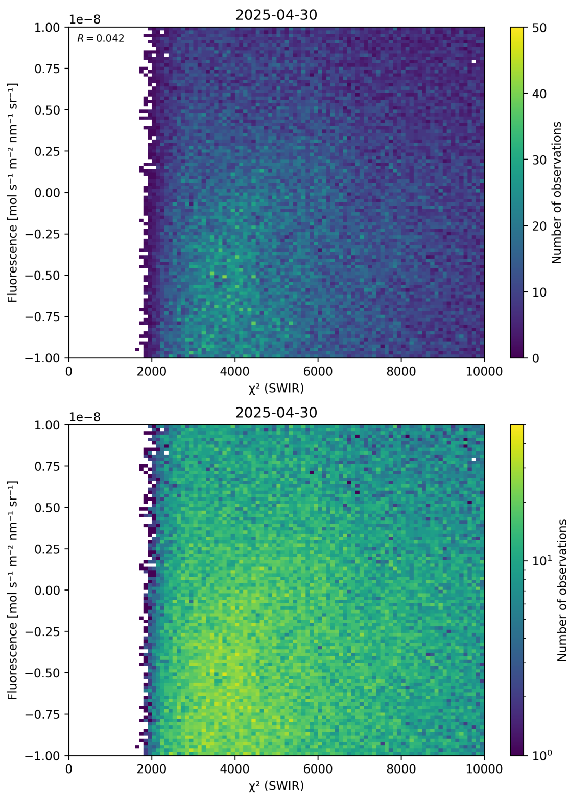
Figure 49: Scatter density plot of “ \chi^2 (SWIR)” against “Fluorescence” for 2025-04-29 to 2025-05-01.
