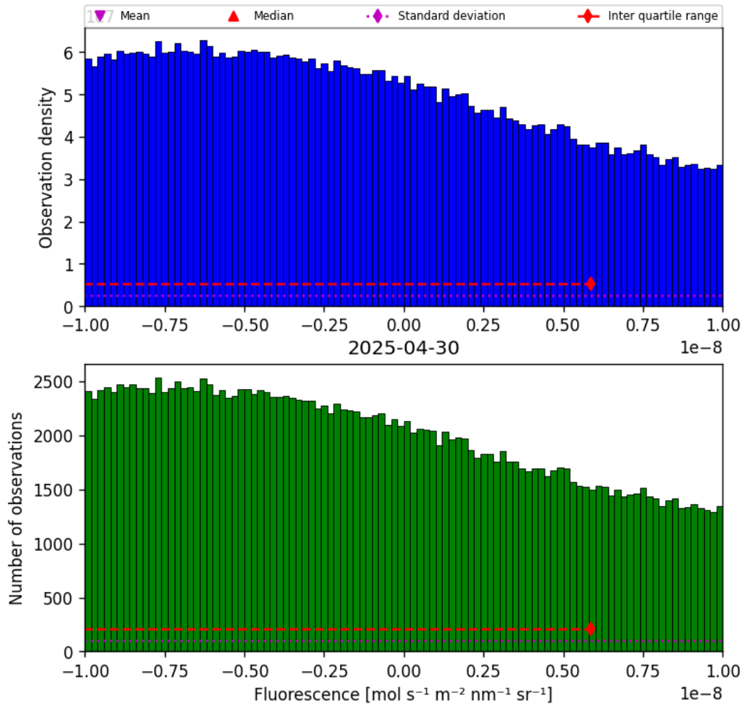
Figure 32: Histogram of “Fluorescence” for 2025-04-29 to 2025-05-01
