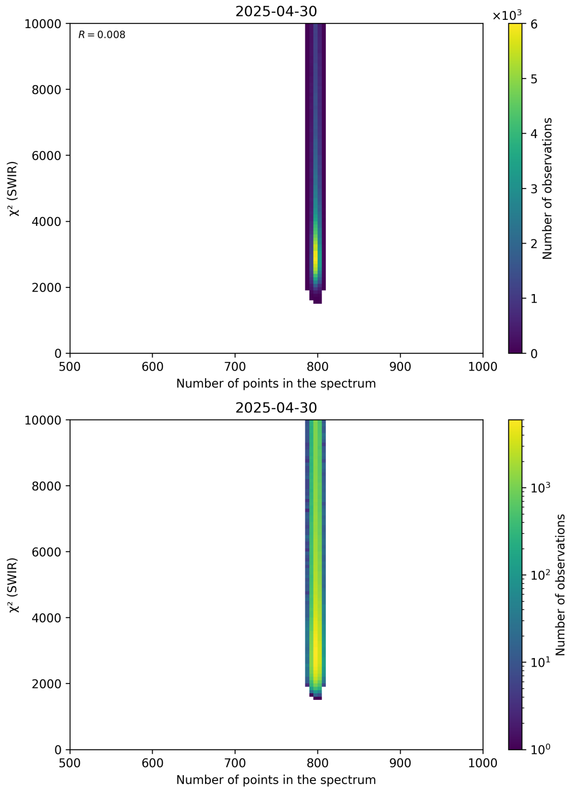
Figure 89: Scatter density plot of “Number of points in the spectrum” against “ \chi^2 (SWIR)” for 2025-04-29 to 2025-05-01.
