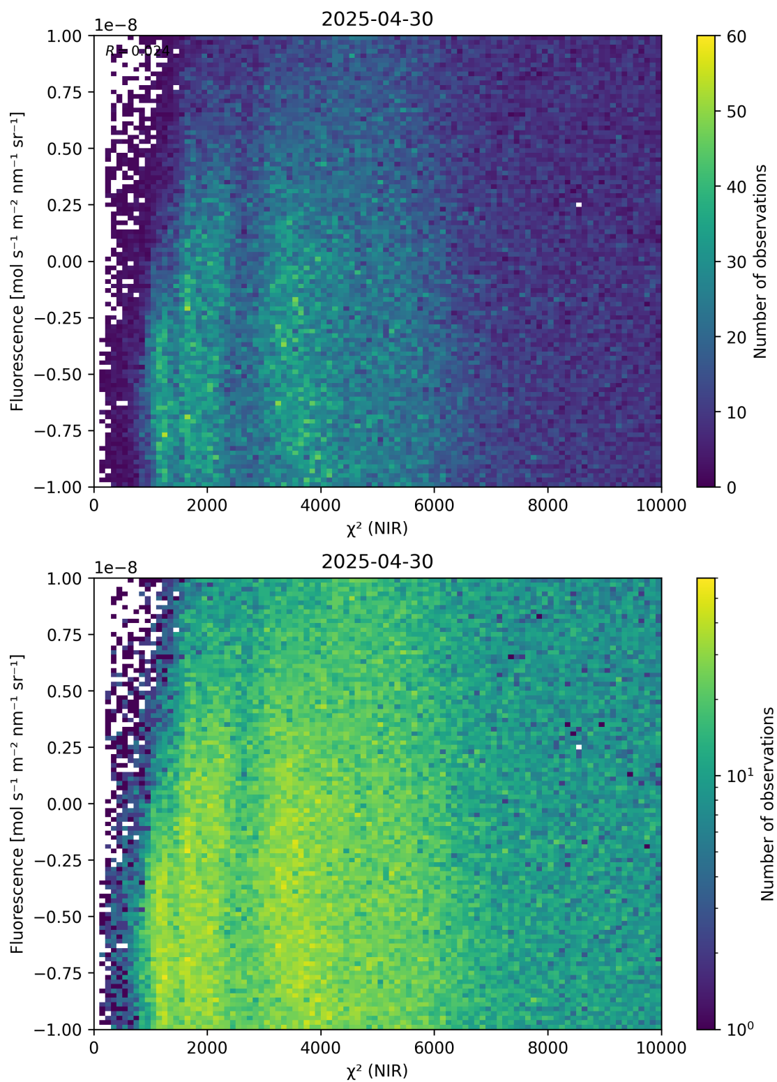
Figure 45: Scatter density plot of “ \chi^2 (NIR)” against “Fluorescence” for 2025-04-29 to 2025-05-01.
