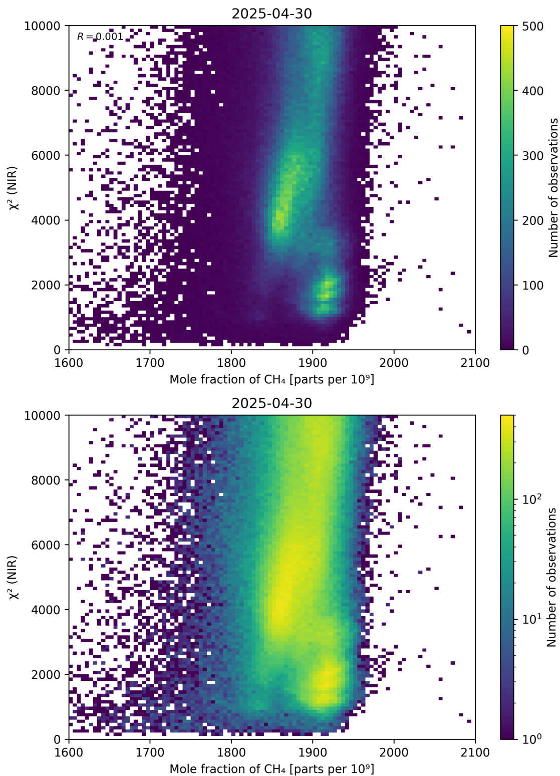
Figure 70: Scatter density plot of “Mole fraction of CH 4 ” against “ \chi^2 (NIR)” for 2025-04-29 to 2025-05-01.
