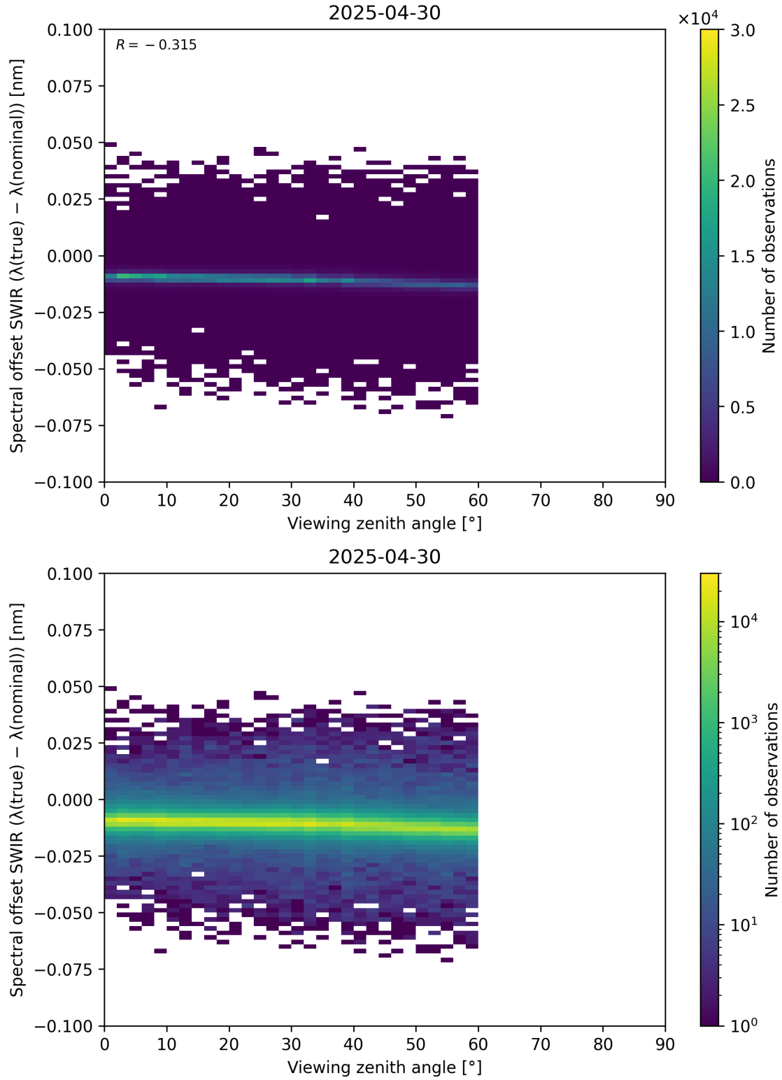
Figure 116: Scatter density plot of “Viewing zenith angle” against “Spectral offset SWIR ( \lambda_{\text{true}} - \lambda_{\text{nominal}} )” for 2025-04-29 to 2025-05-01.
