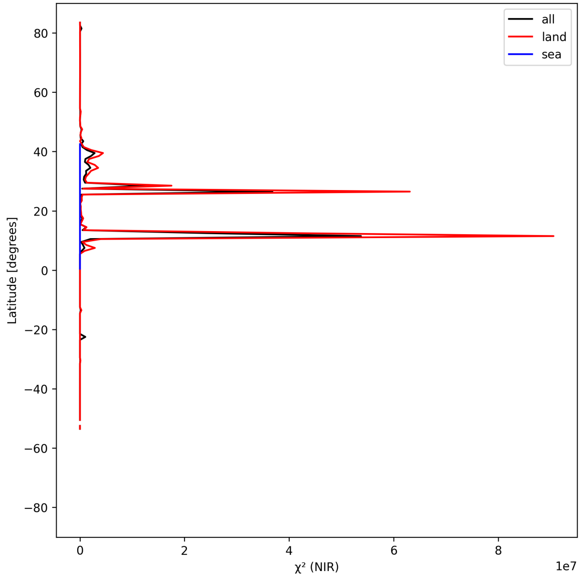
Figure 18: Zonal average of “ \chi^2 (NIR)” for 2025-04-29 to 2025-05-01.
