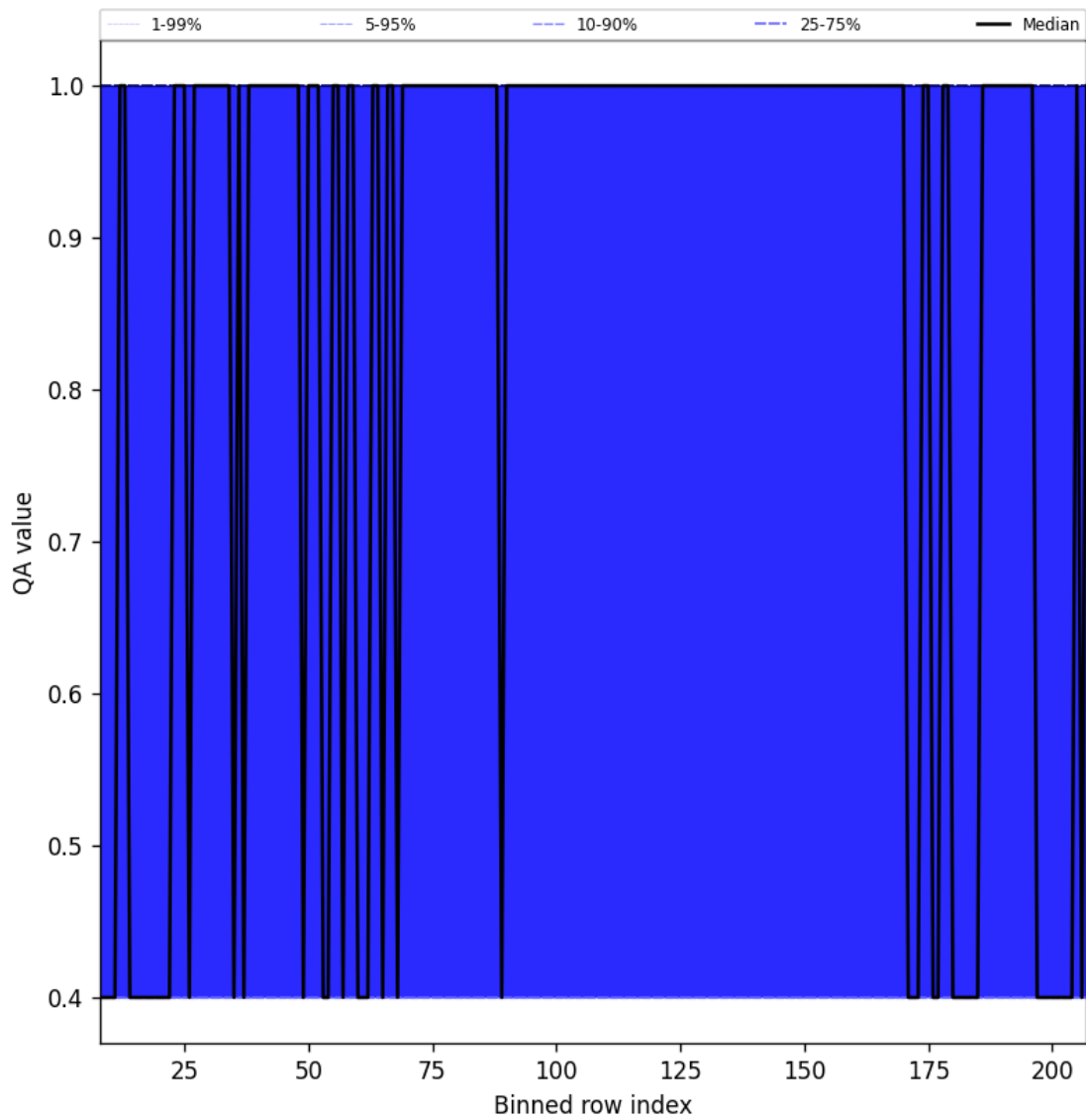
Figure 33: Along track statistics of “QA value” for 2025-04-29 to 2025-05-01
