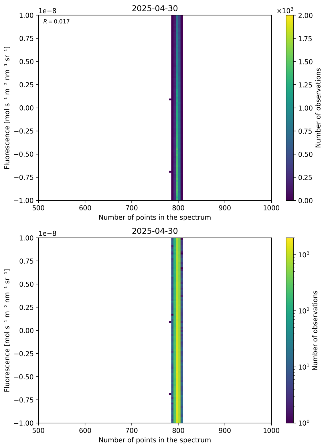
Figure 91: Scatter density plot of “Number of points in the spectrum” against “Fluorescence” for 2025-04-29 to 2025-05-01.
