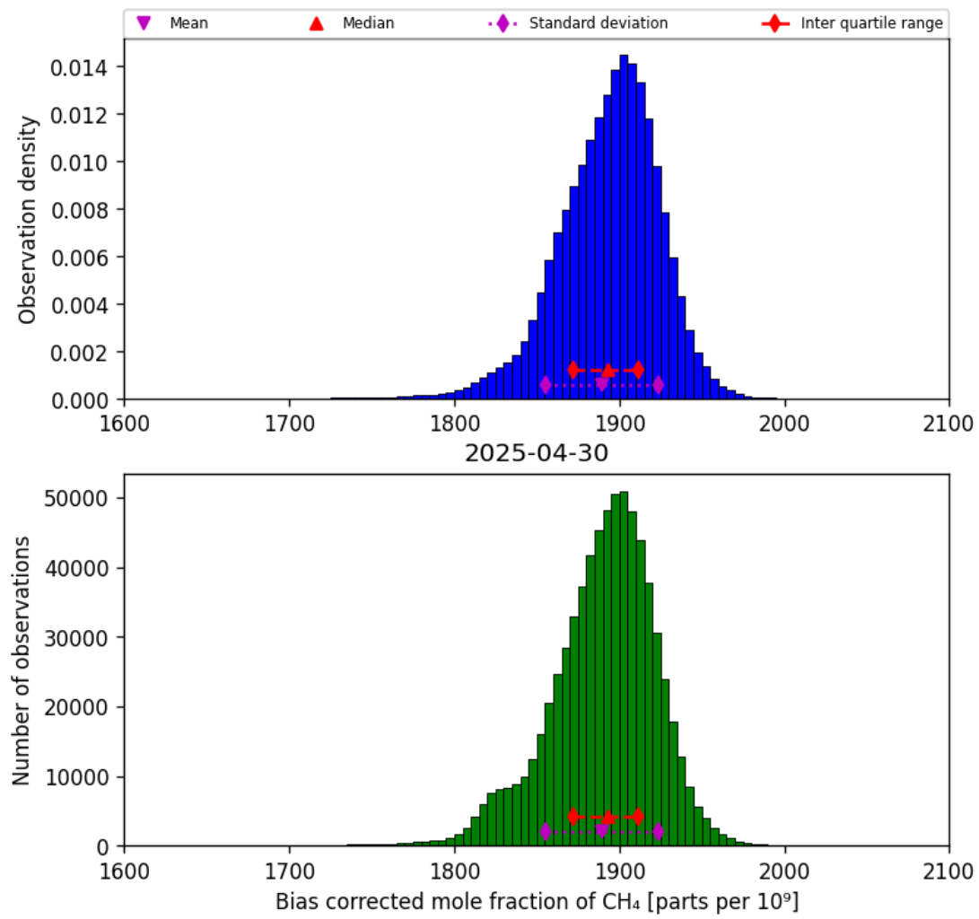
Figure 25: Histogram of “Bias corrected mole fraction of CH 4 ” for 2025-04-29 to 2025-05-01
