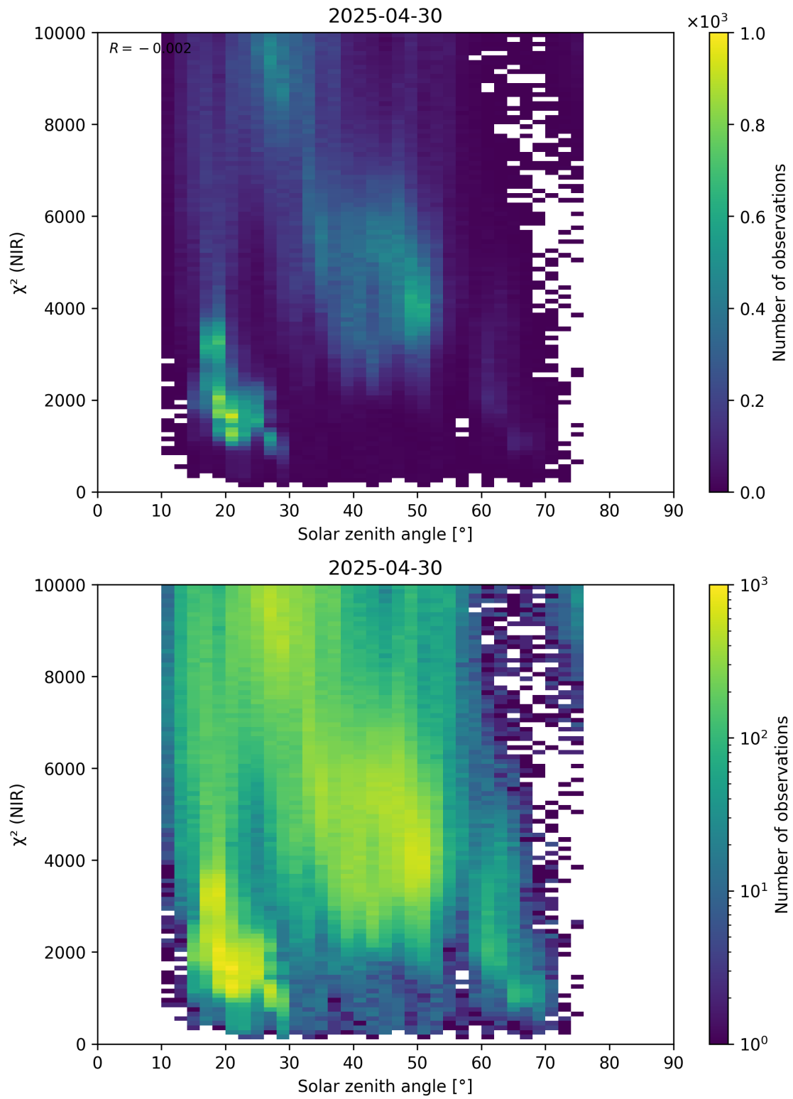
Figure 94: Scatter density plot of “Solar zenith angle” against “ \chi^2 (NIR)” for 2025-04-29 to 2025-05-01.
