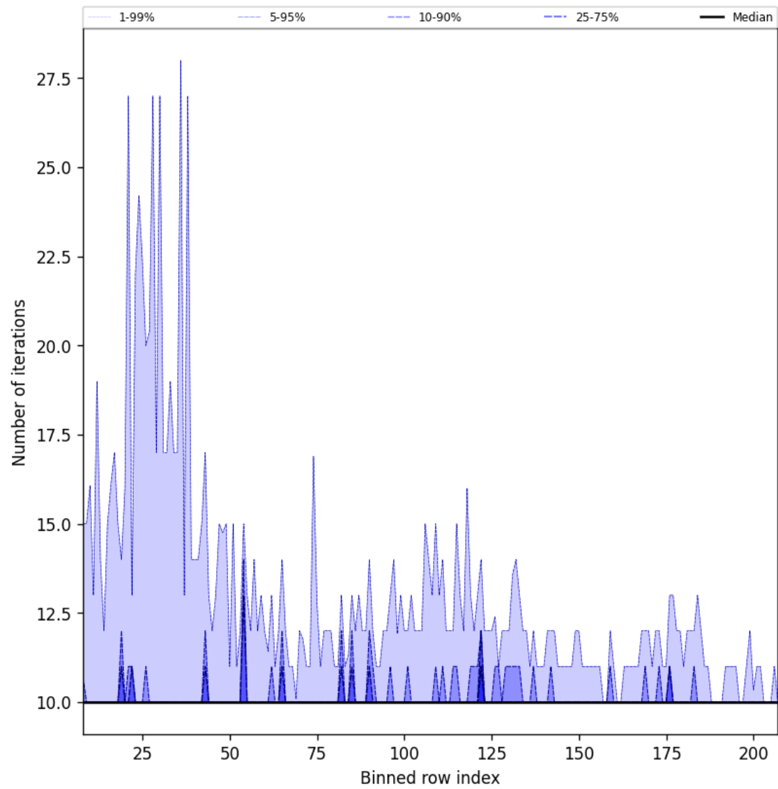
Figure 42: Along track statistics of “Number of iterations” for 2025-04-29 to 2025-05-01
