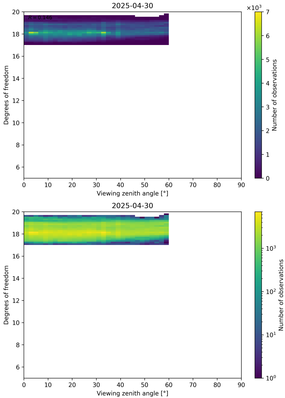
Figure 107: Scatter density plot of “Viewing zenith angle” against “Degrees of freedom” for 2025-04-29 to 2025-05-01.
