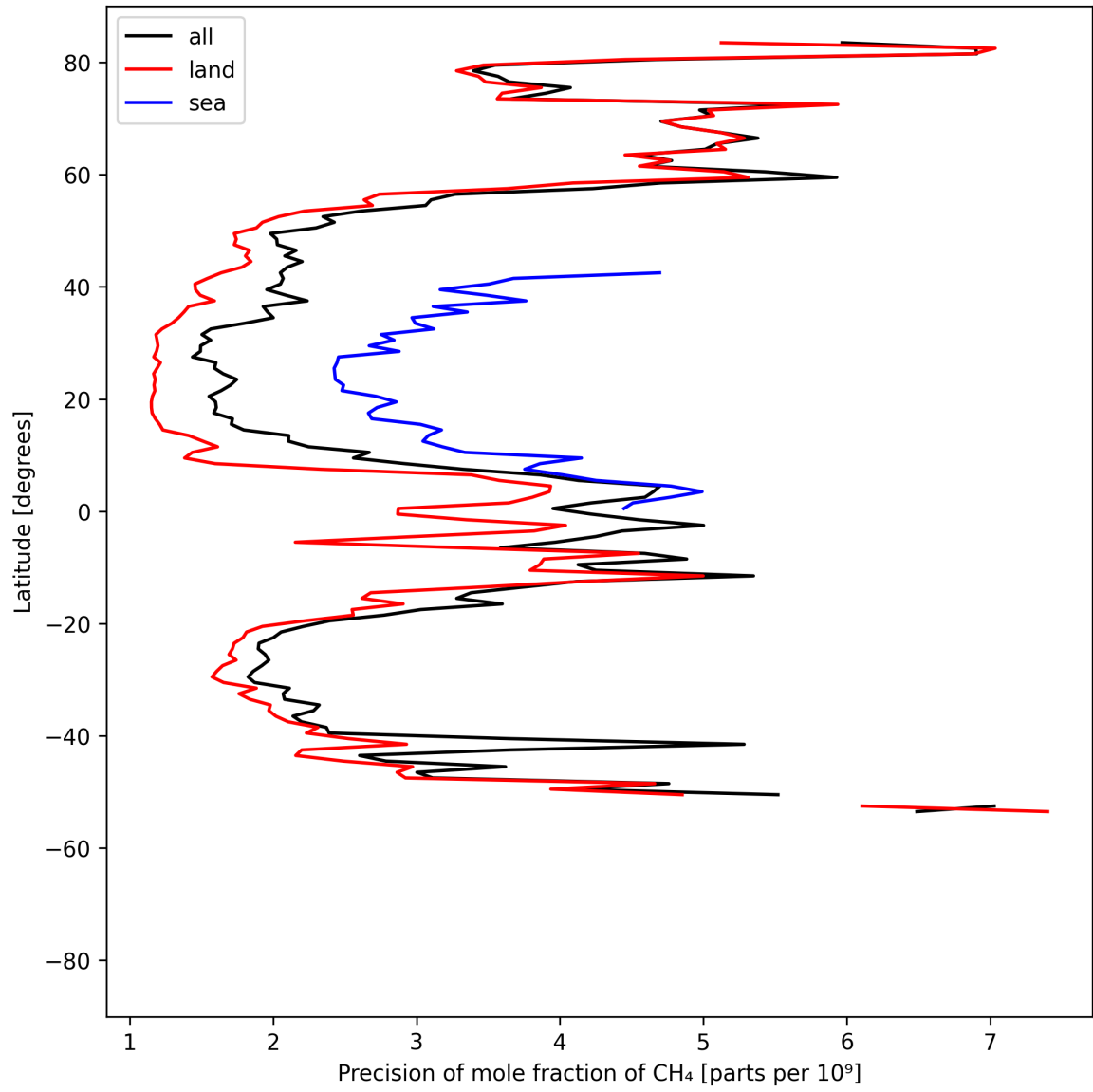
Figure 13: Zonal average of “Precision of mole fraction of CH 4 ” for 2025-04-29 to 2025-05-01.
