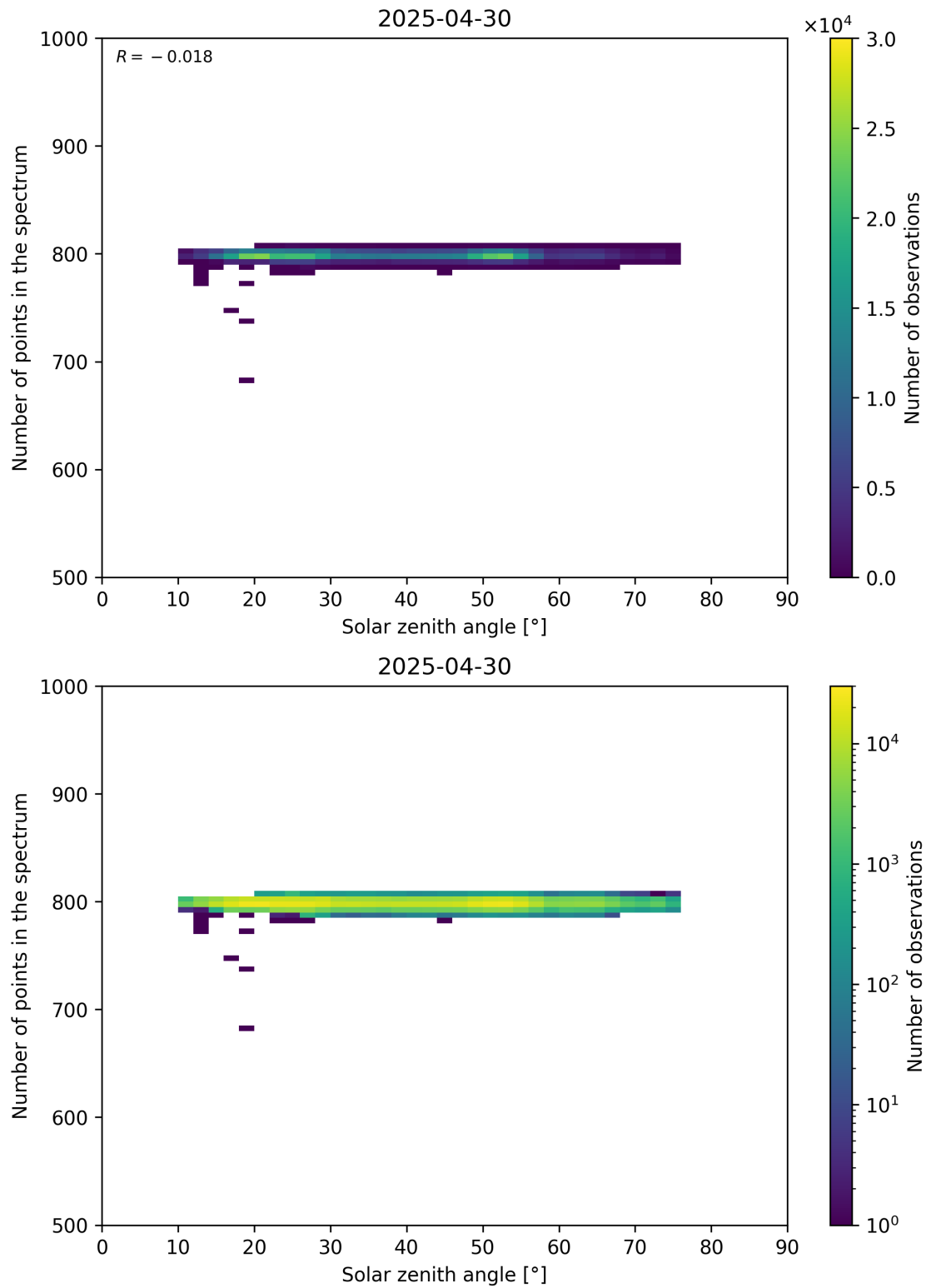
Figure 103: Scatter density plot of “Solar zenith angle” against “Number of points in the spectrum” for 2025-04-29 to 2025-05-01.
