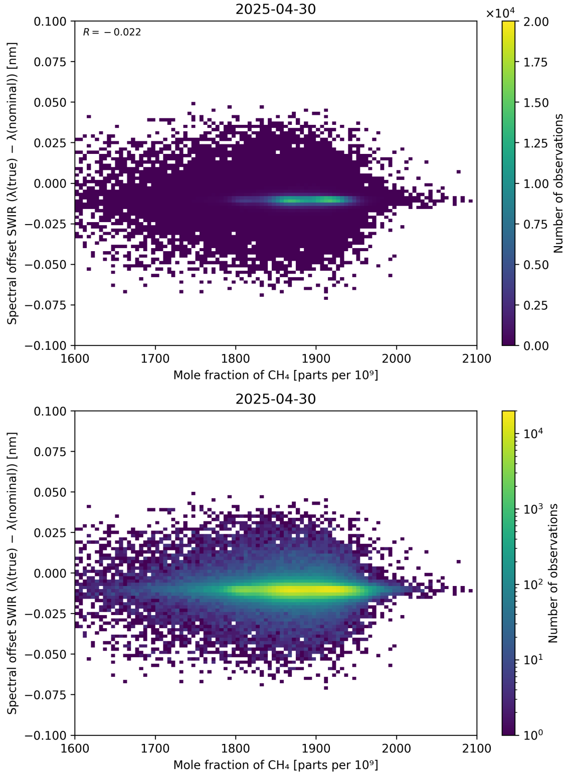
Figure 86: Scatter density plot of “Mole fraction of CH 4 ” against “Spectral offset SWIR ( \lambda_{\text{true}} - \lambda_{\text{nominal}} )” for 2025-04-29 to 2025-05-01.
