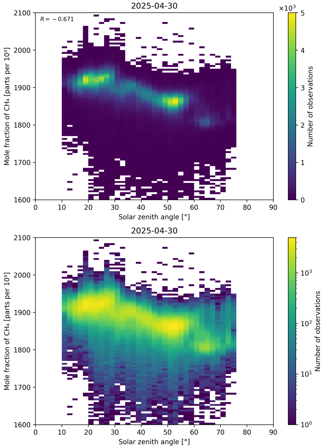
Figure 99: Scatter density plot of “Solar zenith angle” against “Mole fraction of \text{CH}_4 ” for 2025-04-29 to 2025-05-01.
