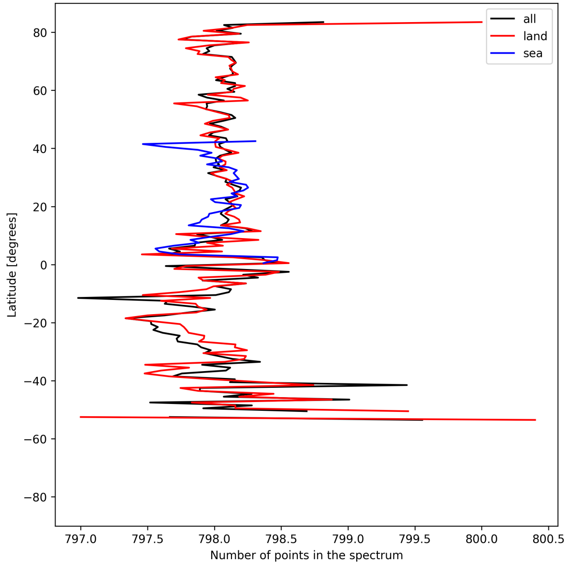
Figure 15: Zonal average of “Number of points in the spectrum” for 2025-04-29 to 2025-05-01.
