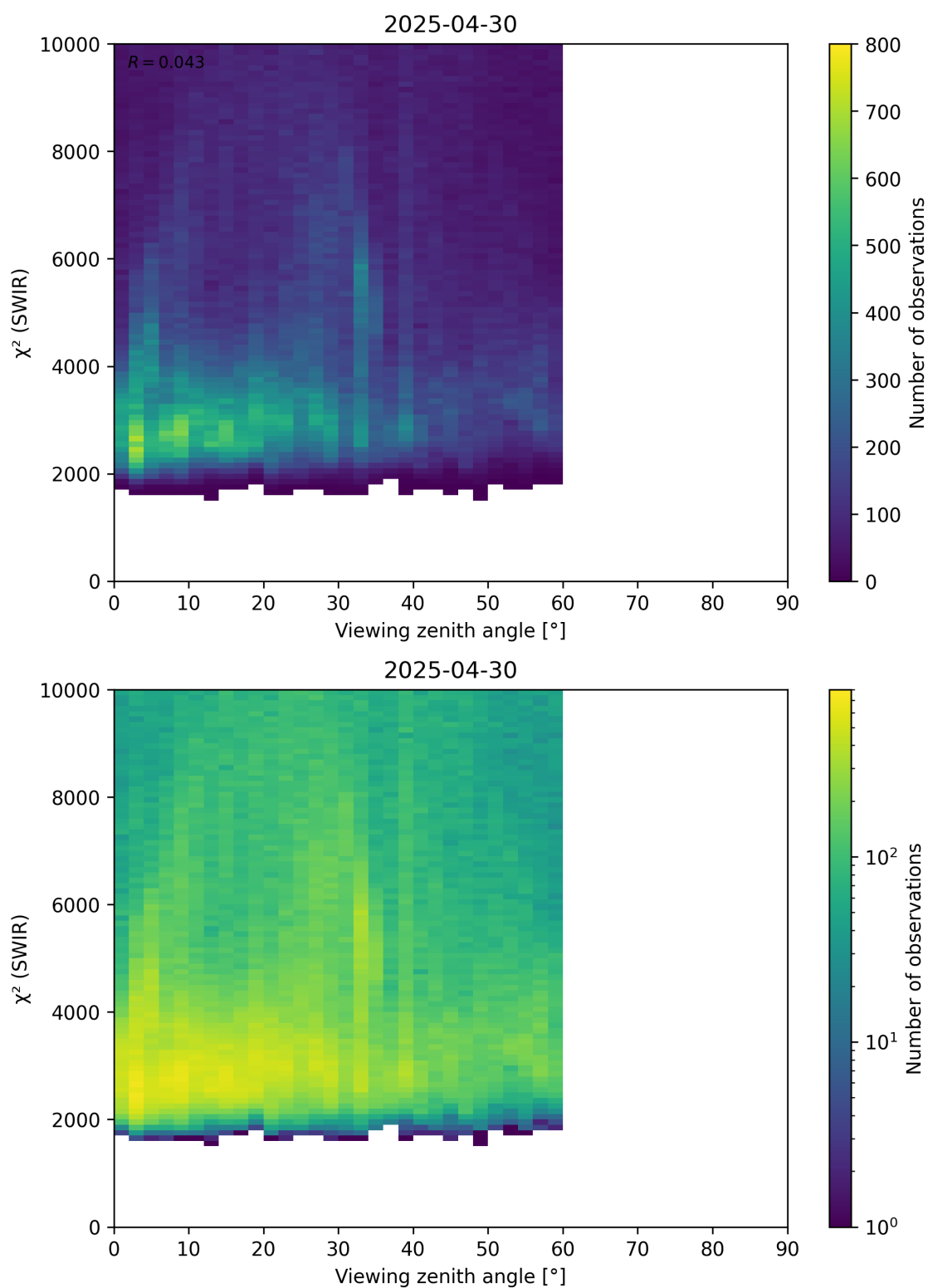
Figure 106: Scatter density plot of “Viewing zenith angle” against “ \chi^2 (SWIR)” for 2025-04-29 to 2025-05-01.
