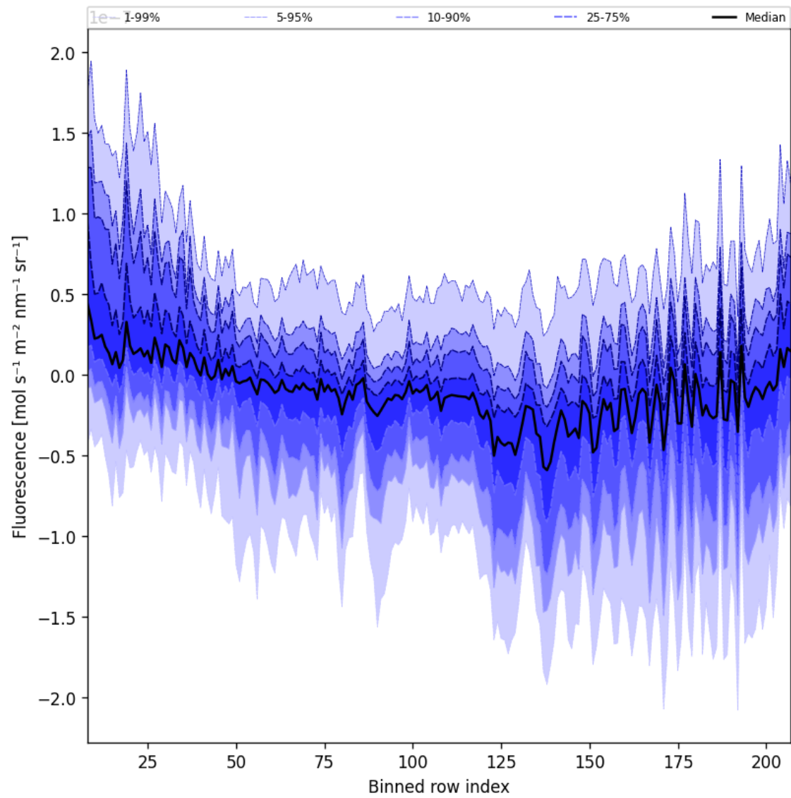
Figure 43: Along track statistics of “Fluorescence” for 2025-04-29 to 2025-05-01
