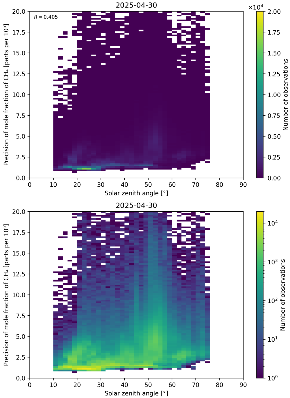
Figure 101: Scatter density plot of “Solar zenith angle” against “Precision of mole fraction of \text{CH}_4 ” for 2025-04-29 to 2025-05-01.
