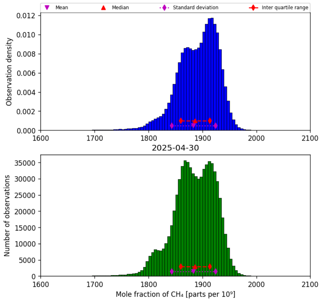
Figure 23: Histogram of “Mole fraction of CH 4 ” for 2025-04-29 to 2025-05-01
