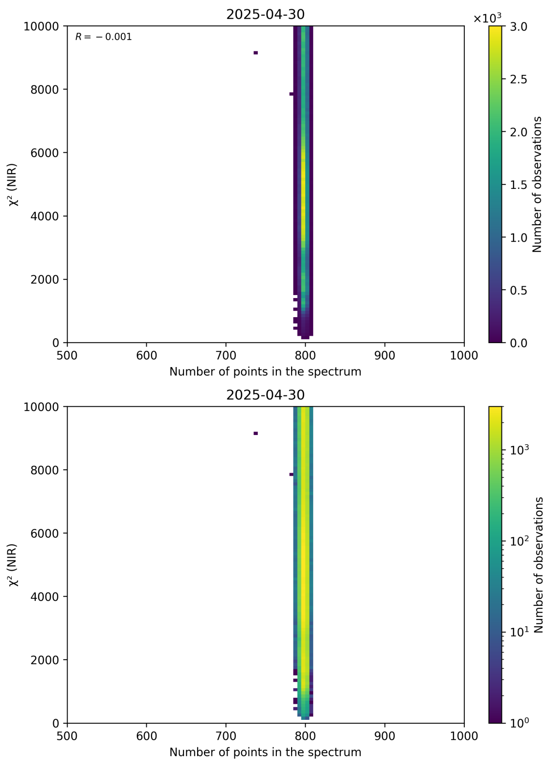
Figure 88: Scatter density plot of “Number of points in the spectrum” against “ \chi^2 (NIR)” for 2025-04-29 to 2025-05-01.
