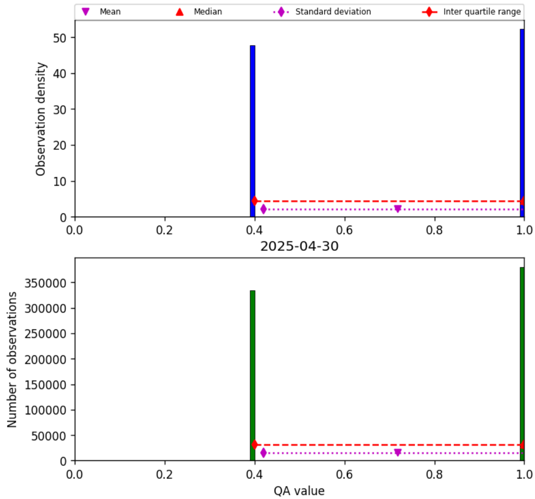
Figure 22: Histogram of “QA value” for 2025-04-29 to 2025-05-01
