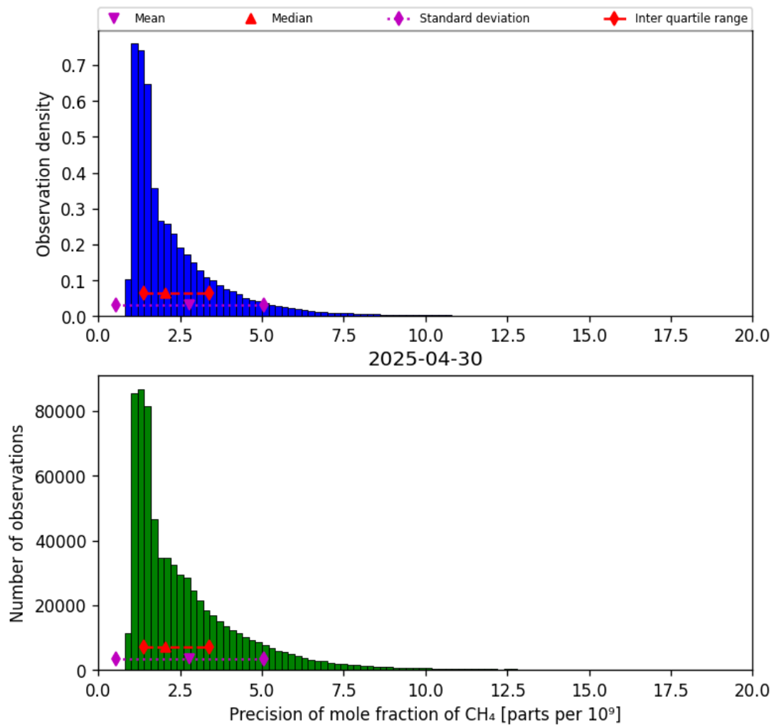
Figure 24: Histogram of “Precision of mole fraction of CH 4 ” for 2025-04-29 to 2025-05-01
