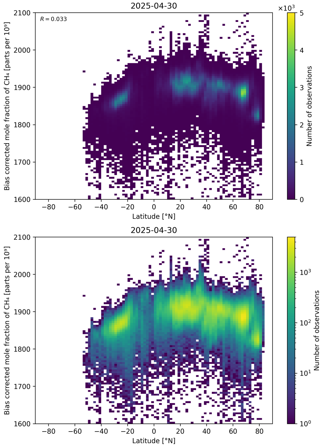
Figure 58: Scatter density plot of “Latitude” against “Bias corrected mole fraction of CH 4 ” for 2025-04-29 to 2025-05-01.
