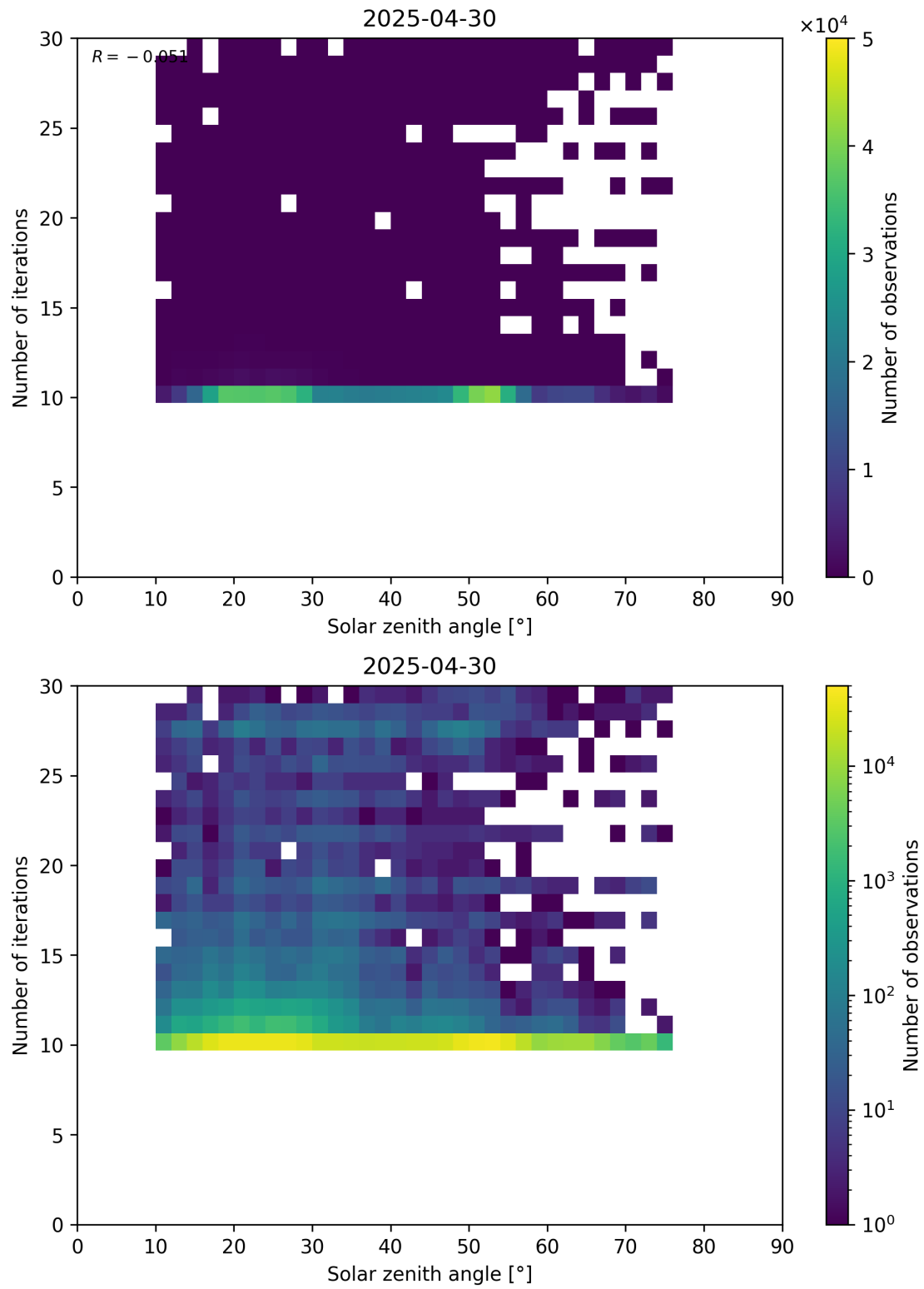
Figure 102: Scatter density plot of “Solar zenith angle” against “Number of iterations” for 2025-04-29 to 2025-05-01.
