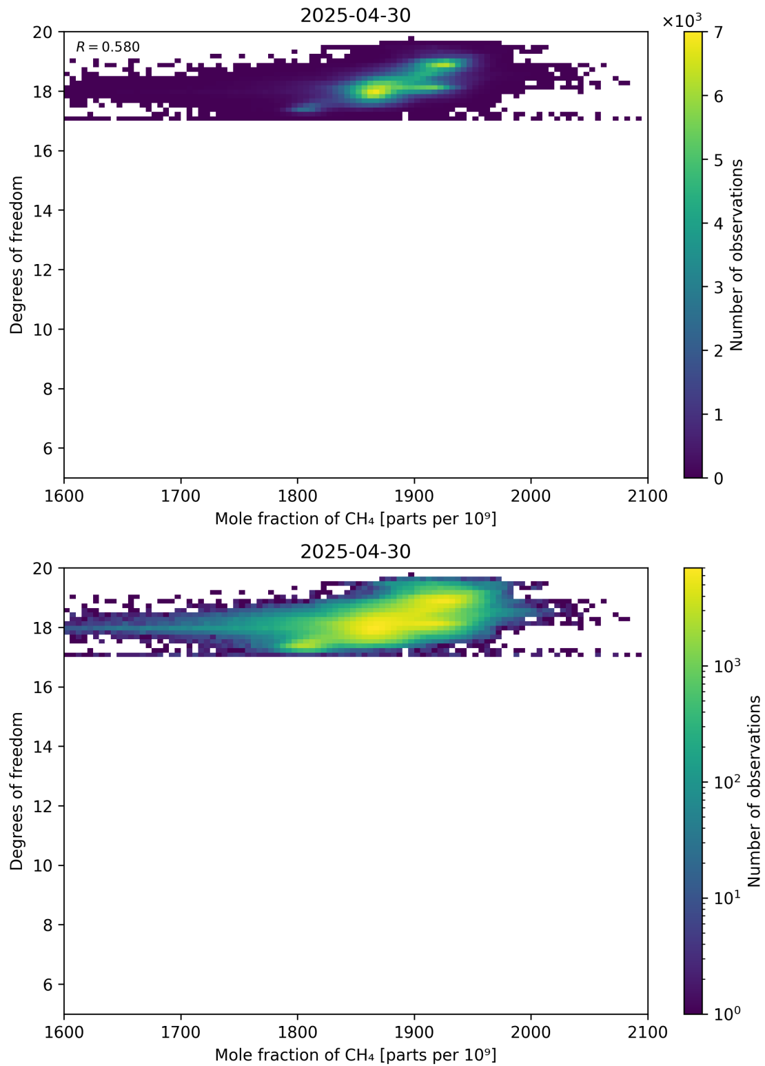
Figure 72: Scatter density plot of “Mole fraction of CH 4 ” against “Degrees of freedom” for 2025-04-29 to 2025-05-01.
