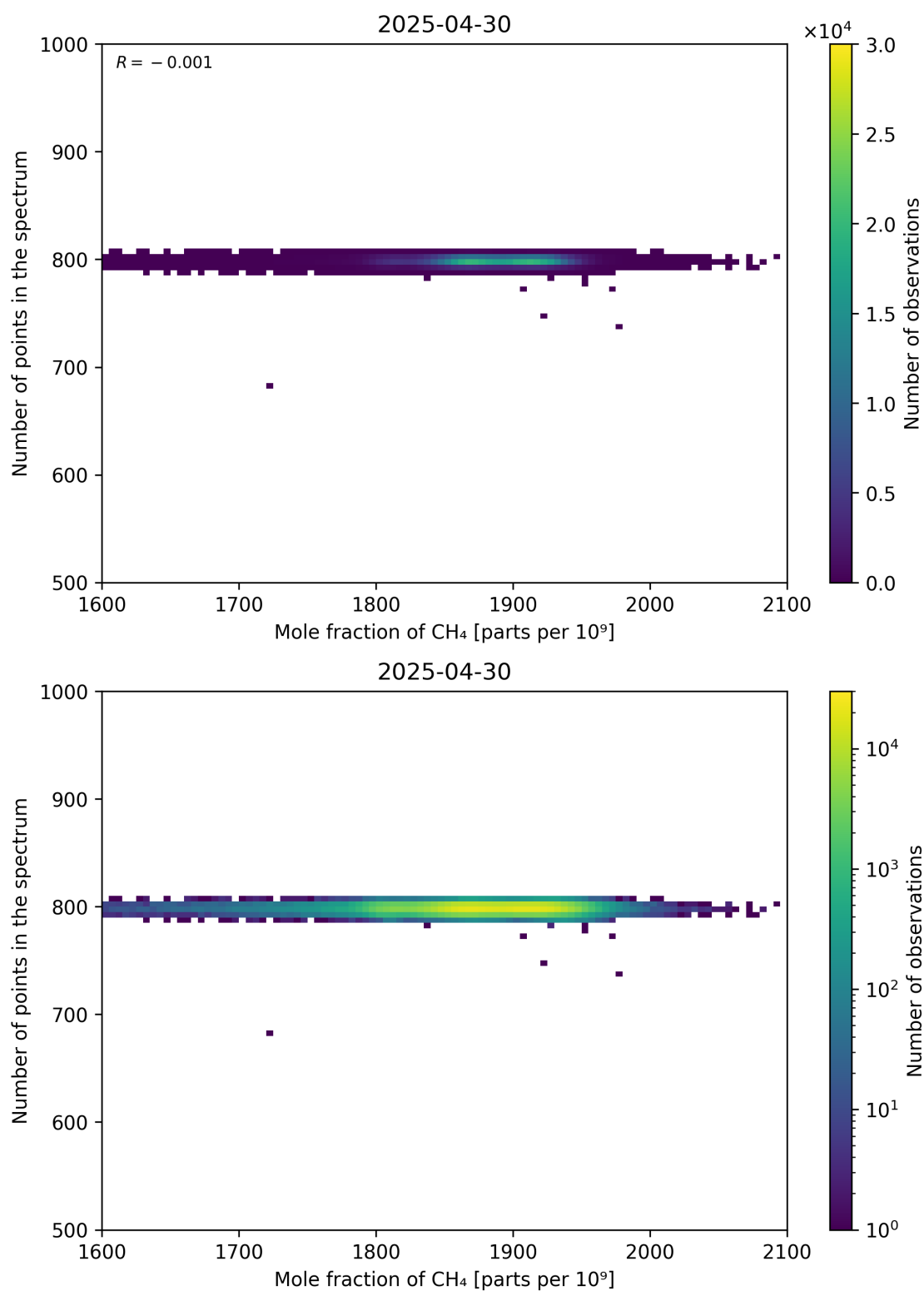
Figure 77: Scatter density plot of “Mole fraction of CH 4 ” against “Number of points in the spectrum” for 2025-04-29 to 2025-05-01.
