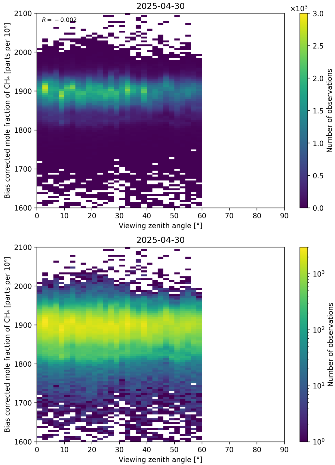
Figure 111: Scatter density plot of “Viewing zenith angle” against “Bias corrected mole fraction of CH 4 ” for 2025-04-29 to 2025-05-01.
