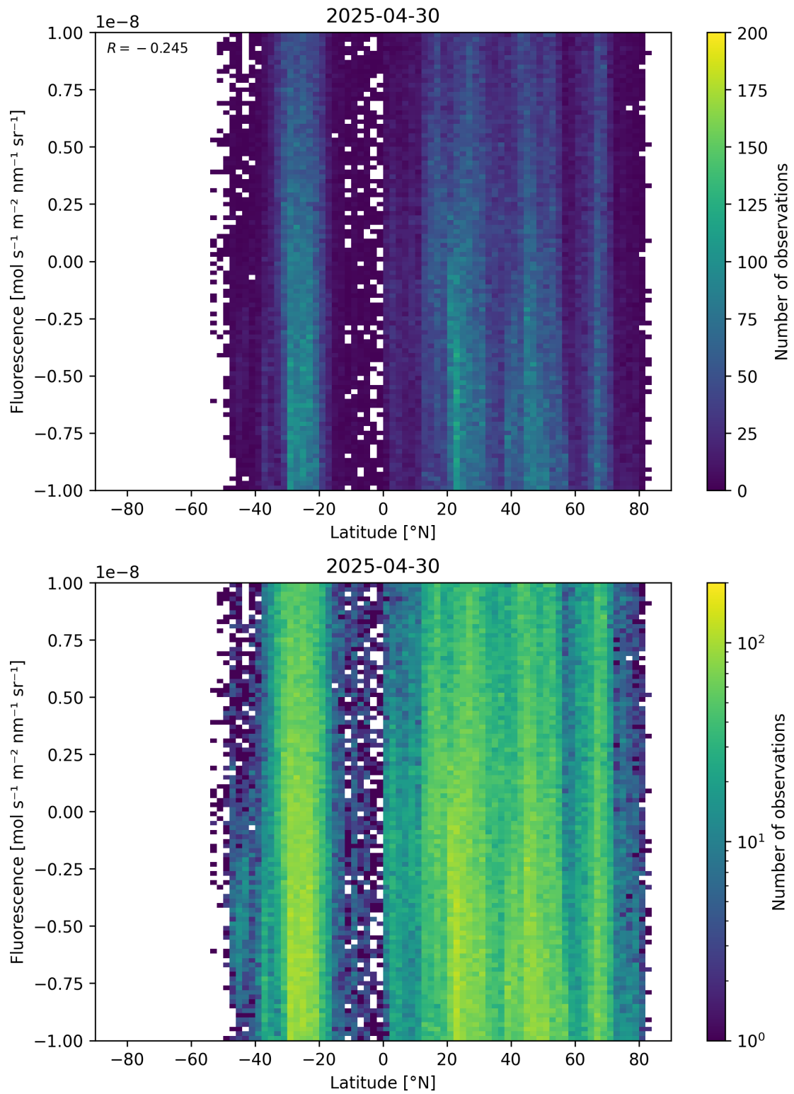
Figure 56: Scatter density plot of “Latitude” against “Fluorescence” for 2025-04-29 to 2025-05-01.
