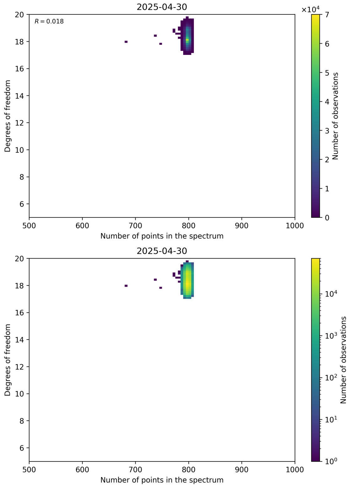
Figure 90: Scatter density plot of “Number of points in the spectrum” against “Degrees of freedom” for 2025-04-29 to 2025-05-01.
