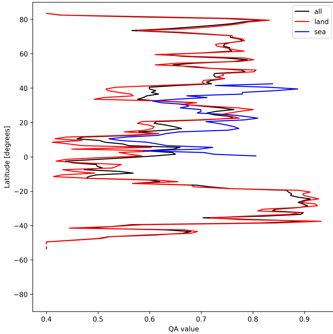
Figure 11: Zonal average of “QA value” for 2025-04-29 to 2025-05-01.
