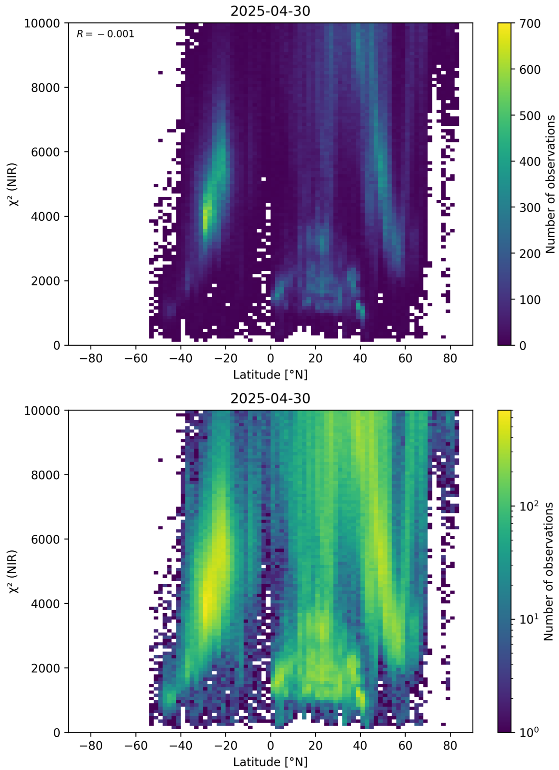
Figure 53: Scatter density plot of “Latitude” against “ \chi^2 (NIR)” for 2025-04-29 to 2025-05-01.
