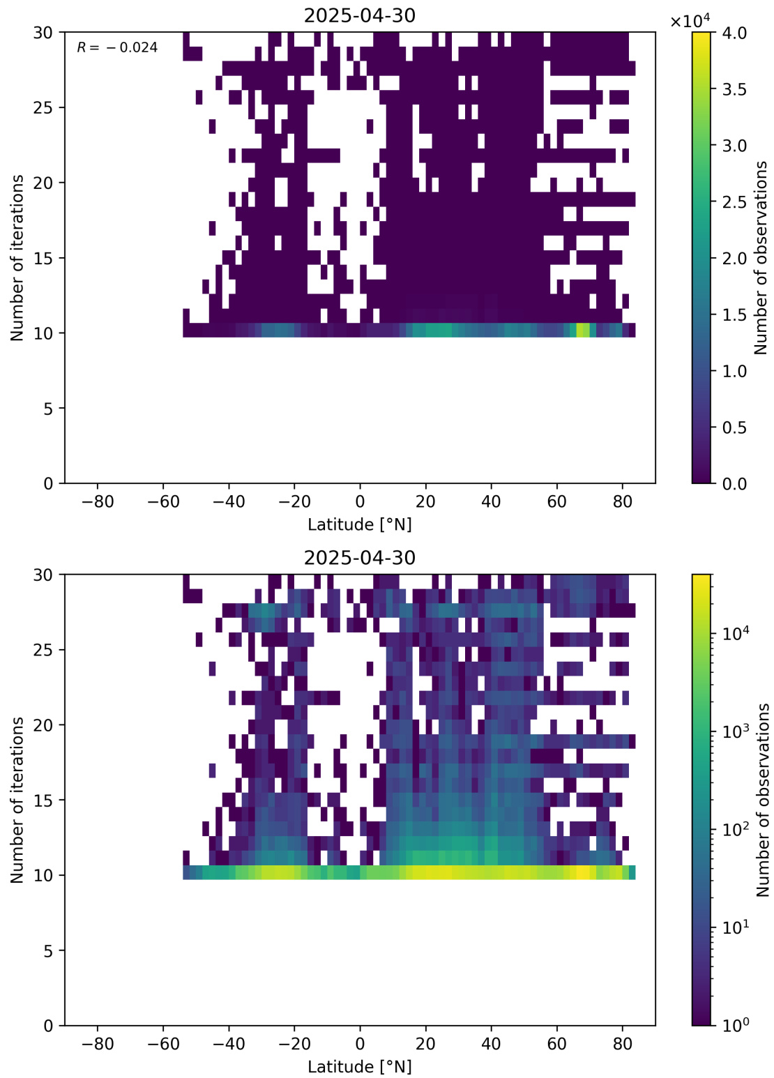
Figure 60: Scatter density plot of “Latitude” against “Number of iterations” for 2025-04-29 to 2025-05-01.
