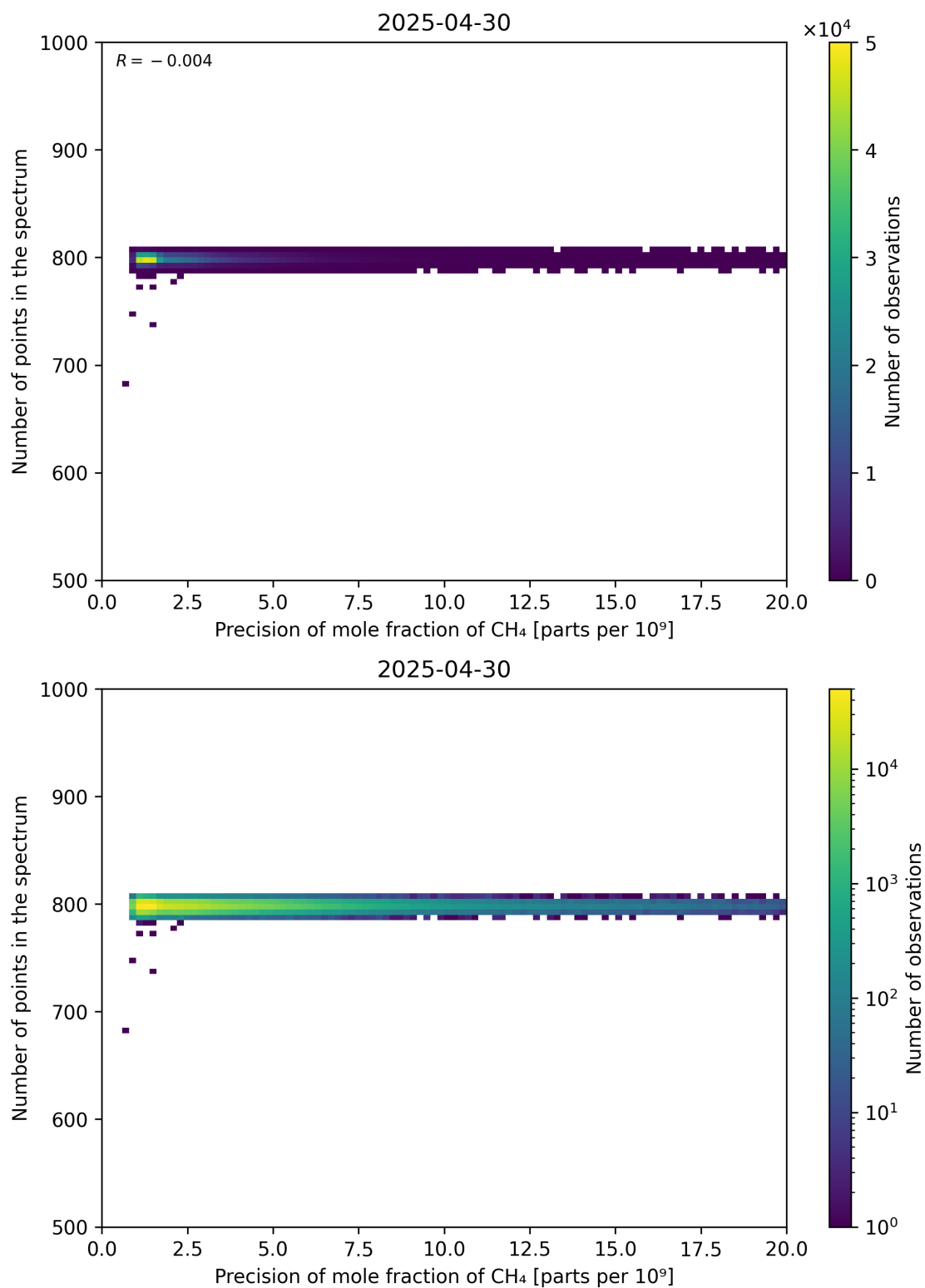
Figure 84: Scatter density plot of “Precision of mole fraction of CH 4 ” against “Number of points in the spectrum” for 2025-04-29 to 2025-05-01.
