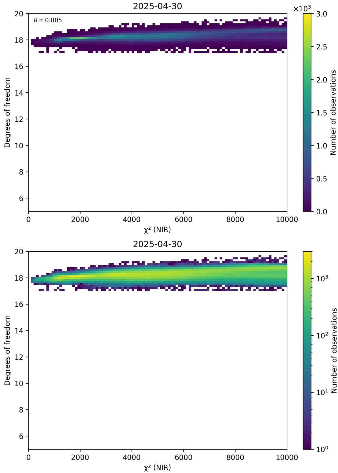
Figure 44: Scatter density plot of “ \chi^2 (NIR)” against “Degrees of freedom” for 2025-04-29 to 2025-05-01.
