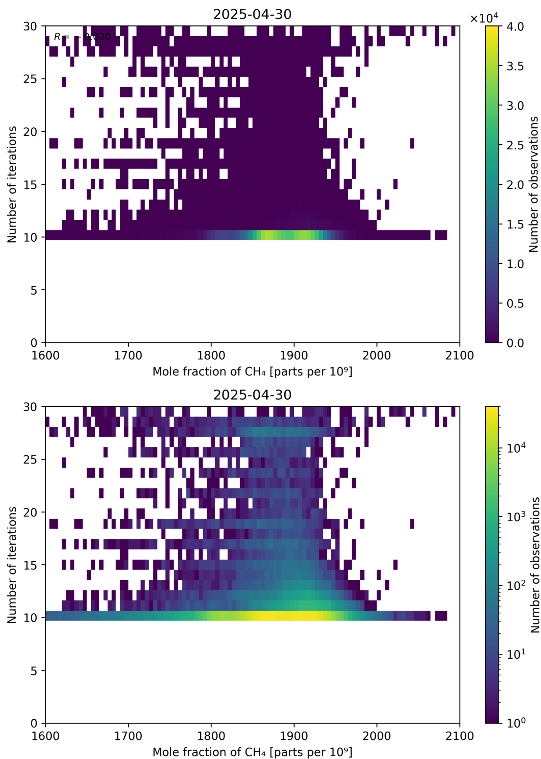
Figure 76: Scatter density plot of “Mole fraction of CH 4 ” against “Number of iterations” for 2025-04-29 to 2025-05-01.
