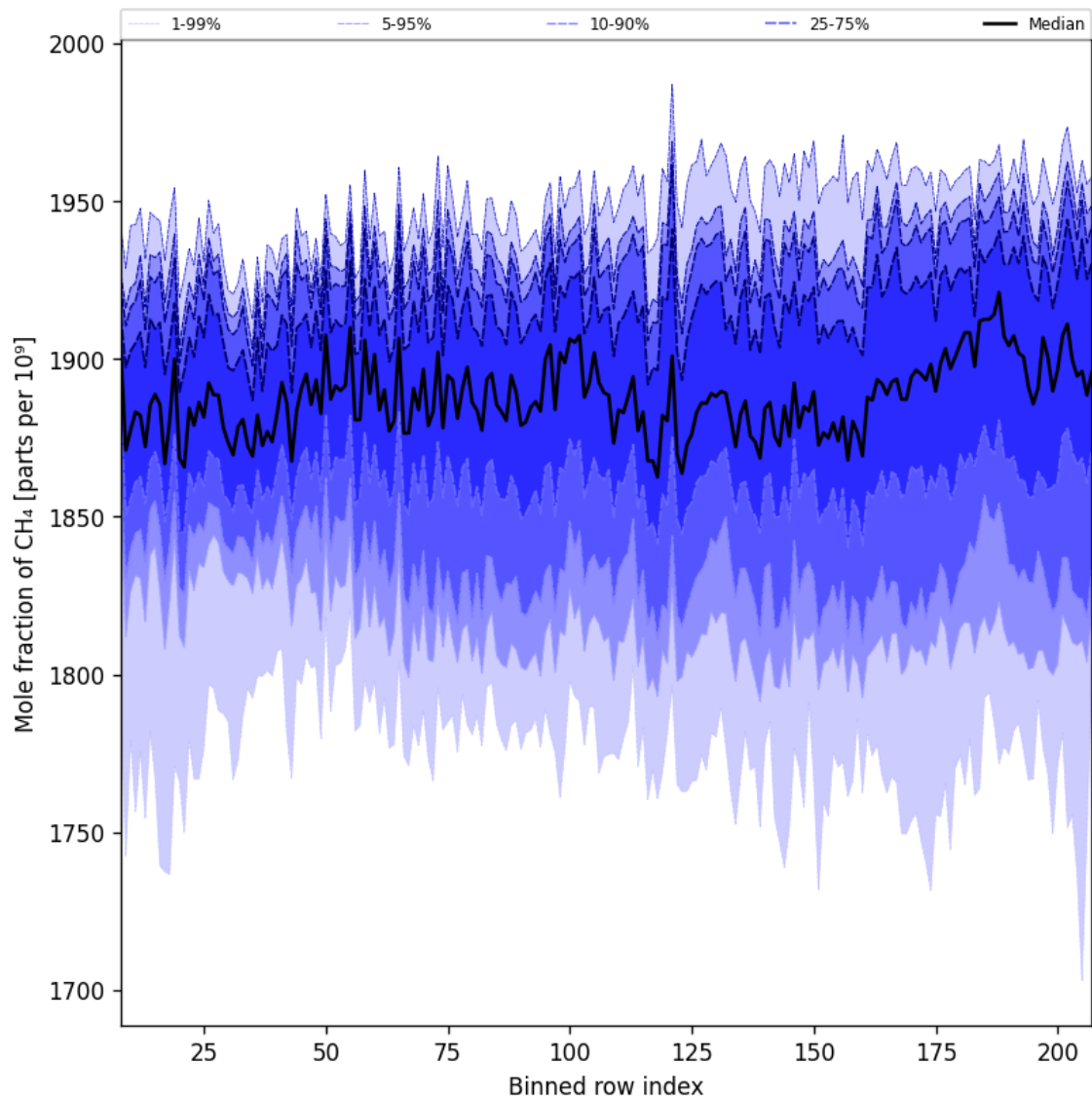
Figure 34: Along track statistics of “Mole fraction of CH 4 ” for 2025-04-29 to 2025-05-01
