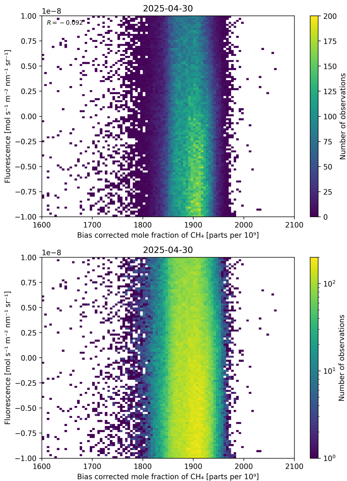
Figure 66: Scatter density plot of “Bias corrected mole fraction of \text{CH}_4 ” against “Fluorescence” for 2025-04-29 to 2025-05-01.
