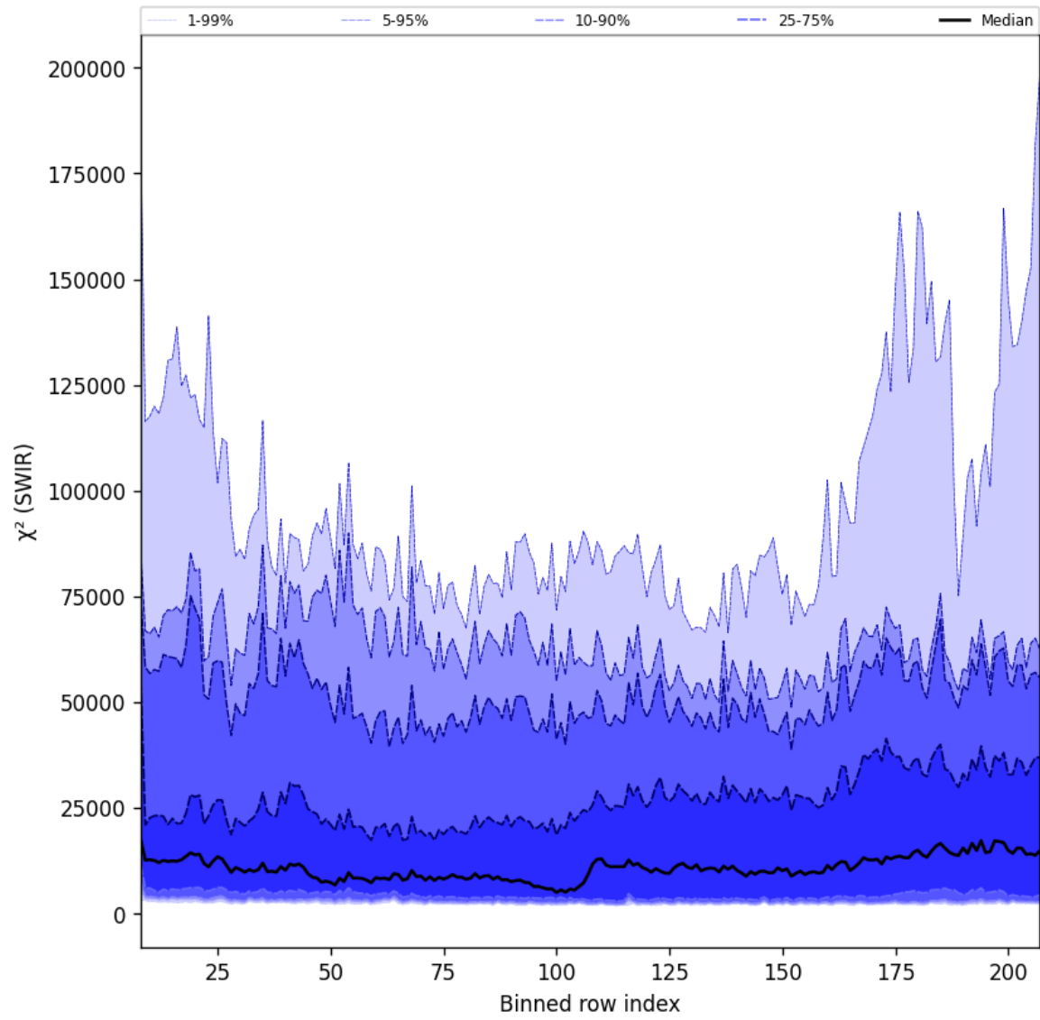
Figure 39: Along track statistics of “ \chi^2 (SWIR)” for 2025-04-29 to 2025-05-01
