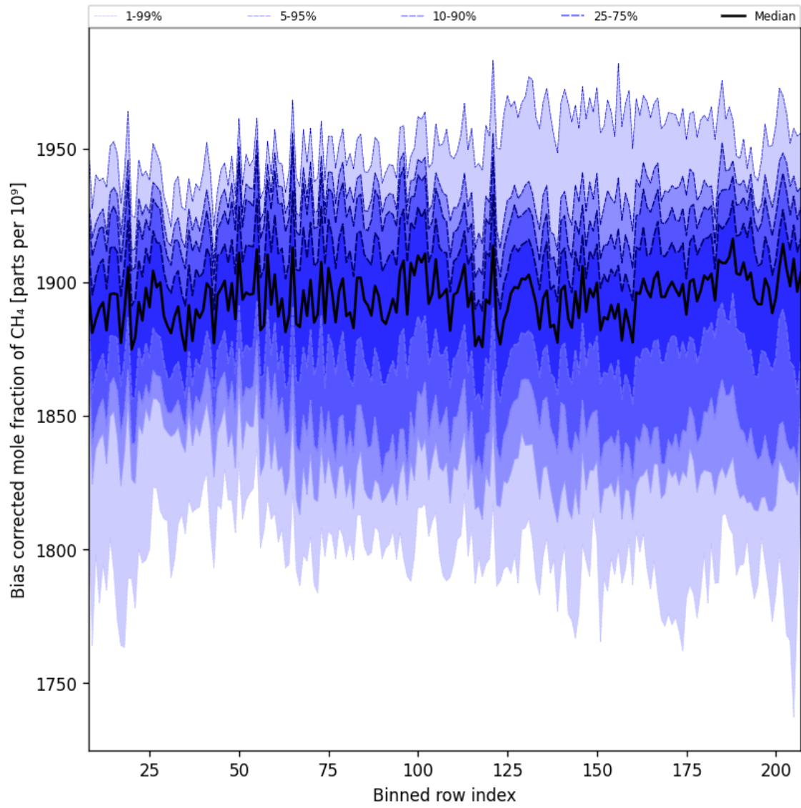
Figure 36: Along track statistics of “Bias corrected mole fraction of CH 4 ” for 2025-04-29 to 2025-05-01
