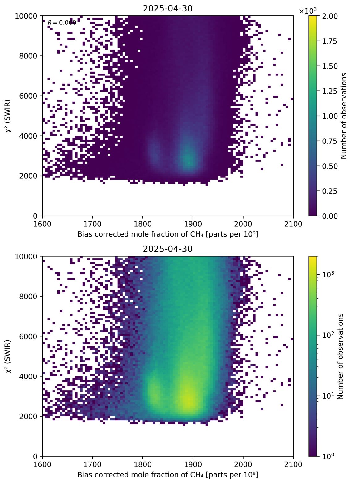
Figure 64: Scatter density plot of “Bias corrected mole fraction of \text{CH}_4 ” against “ \chi^2 (SWIR)” for 2025-04-29 to 2025-05-01.
