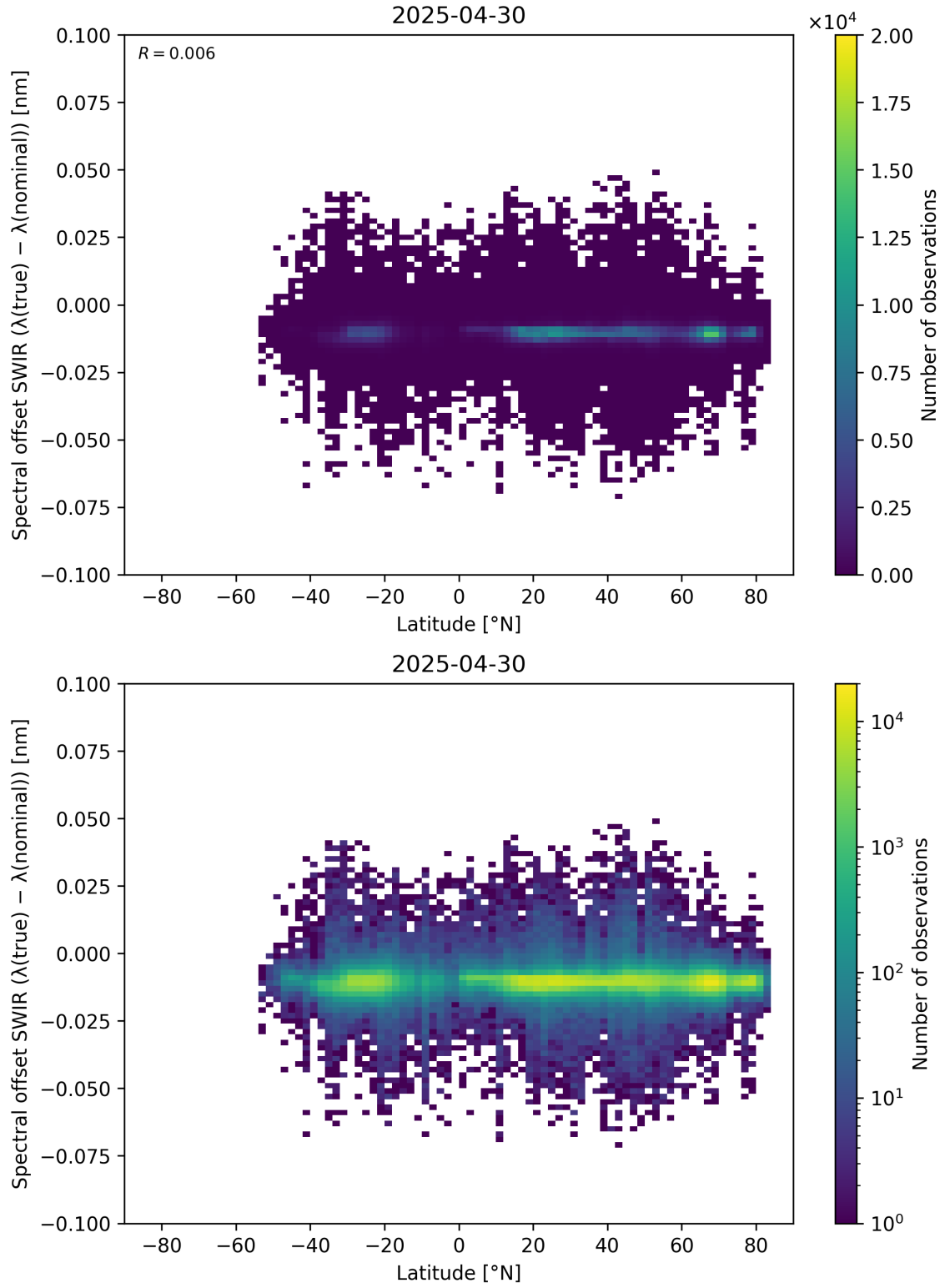
Figure 62: Scatter density plot of “Latitude” against “Spectral offset SWIR ( \lambda_{\text{true}} - \lambda_{\text{nominal}} )” for 2025-04-29 to 2025-05-01.
