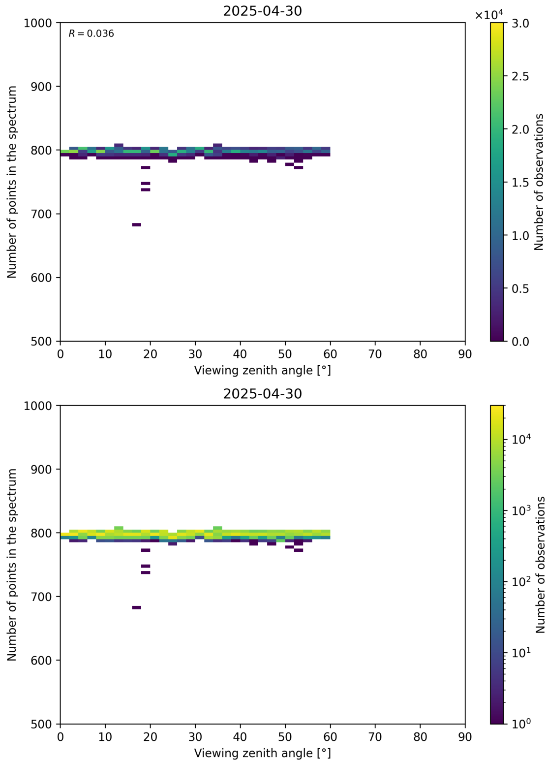
Figure 114: Scatter density plot of “Viewing zenith angle” against “Number of points in the spectrum” for 2025-04-29 to 2025-05-01.
