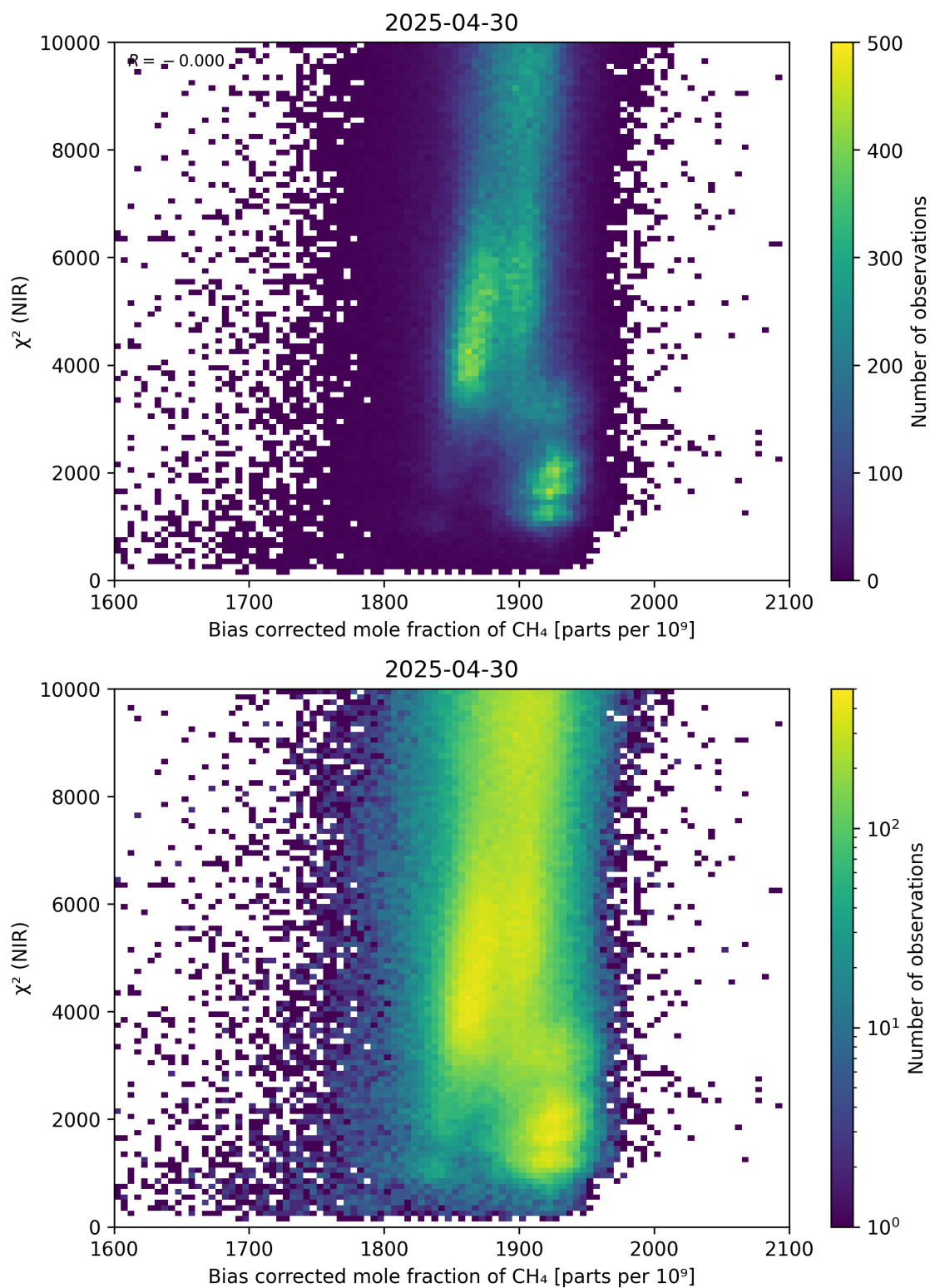
Figure 63: Scatter density plot of “Bias corrected mole fraction of CH 4 ” against “ \chi^2 (NIR)” for 2025-04-29 to 2025-05-01.
