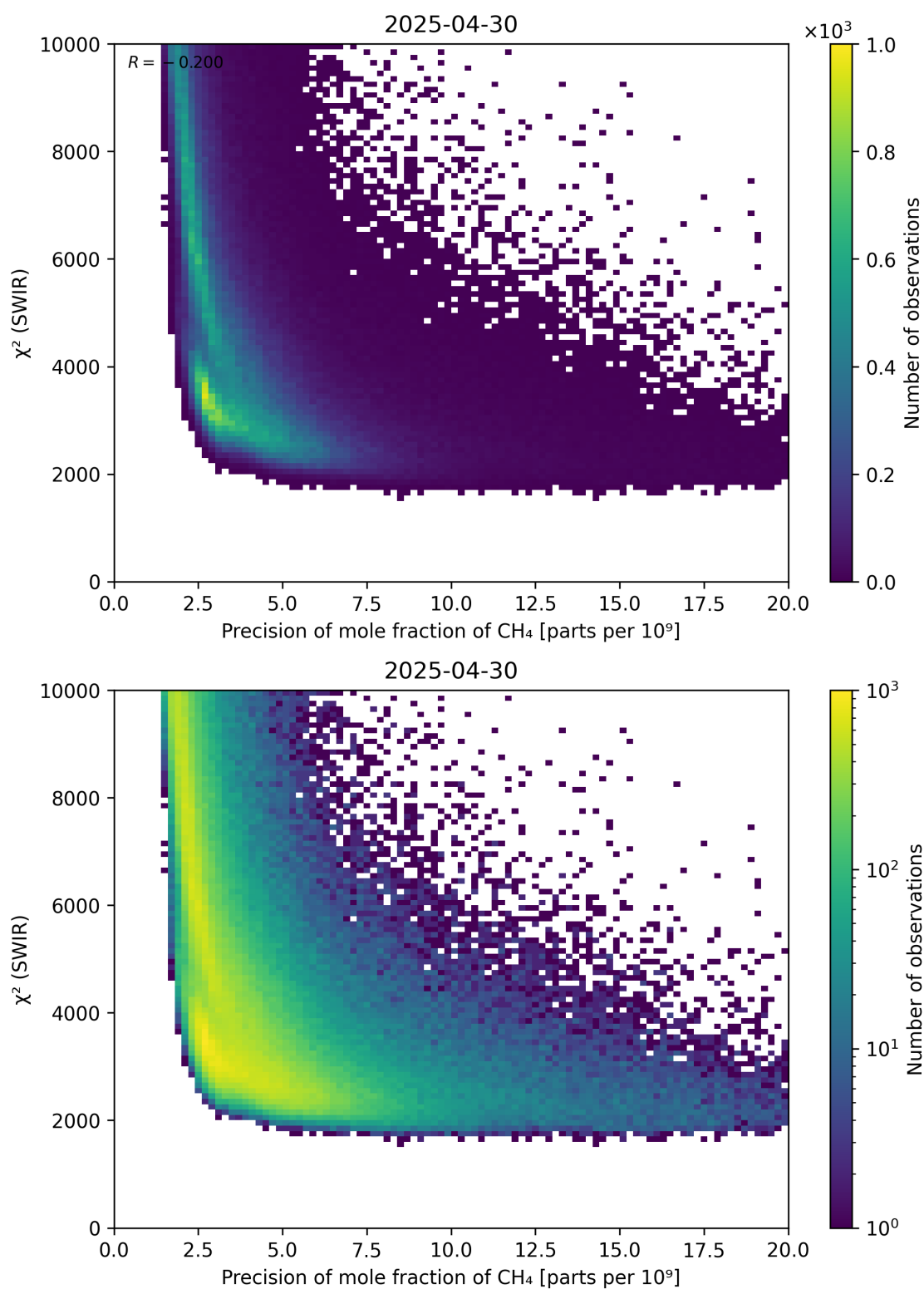
Figure 79: Scatter density plot of “Precision of mole fraction of CH 4 ” against “ \chi^2 (SWIR)” for 2025-04-29 to 2025-05-01.
