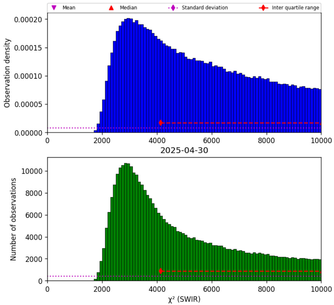
Figure 28: Histogram of “ \chi^2 (SWIR)” for 2025-04-29 to 2025-05-01
