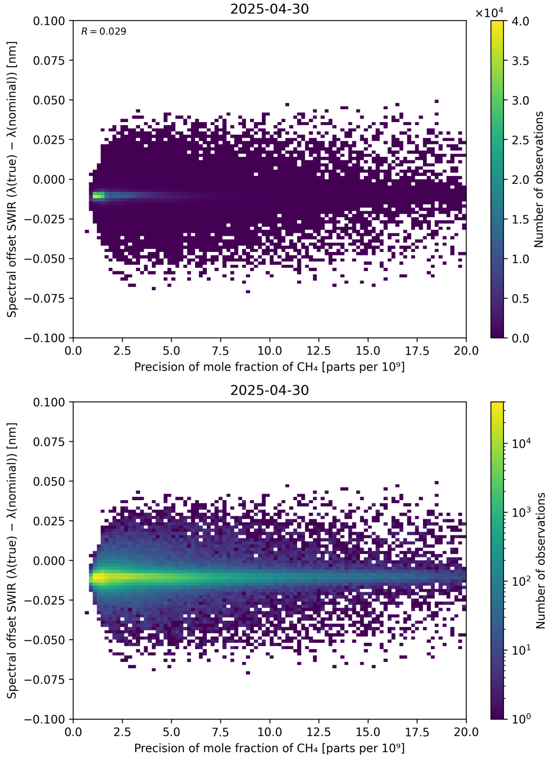
Figure 85: Scatter density plot of “Precision of mole fraction of CH 4 ” against “Spectral offset SWIR ( \lambda_{\text{true}} - \lambda_{\text{nominal}} )” for 2025-04-29 to 2025-05-01.
