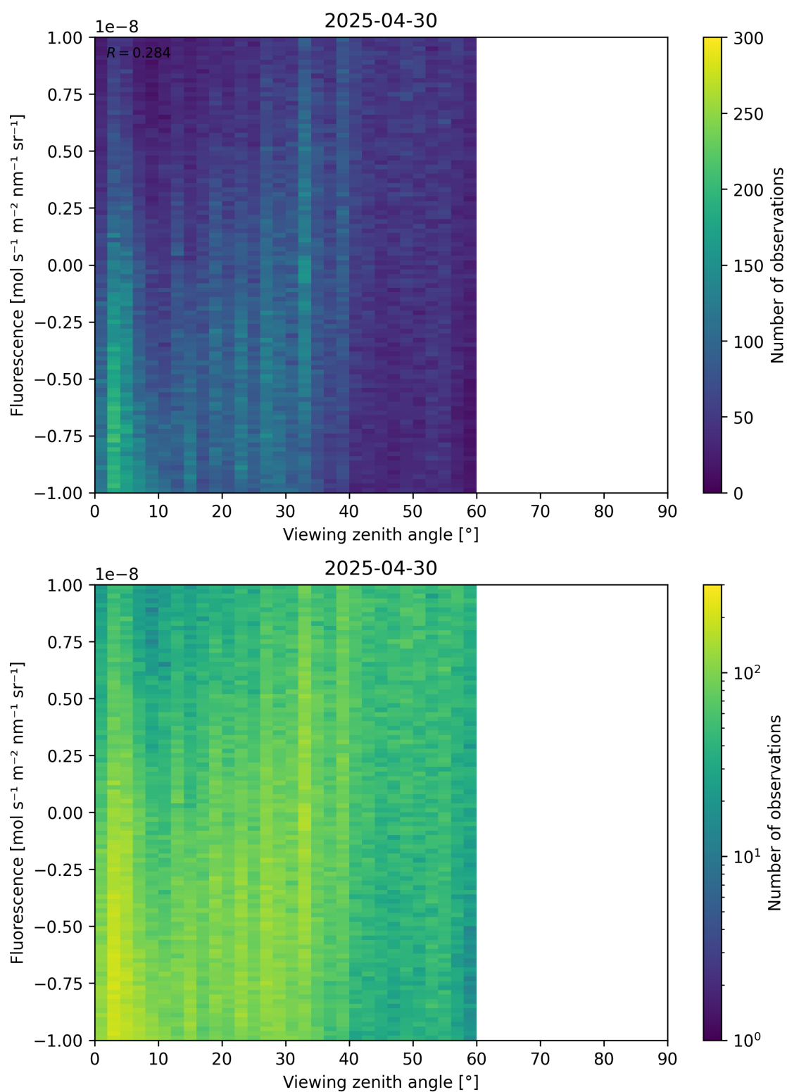
Figure 108: Scatter density plot of “Viewing zenith angle” against “Fluorescence” for 2025-04-29 to 2025-05-01.
