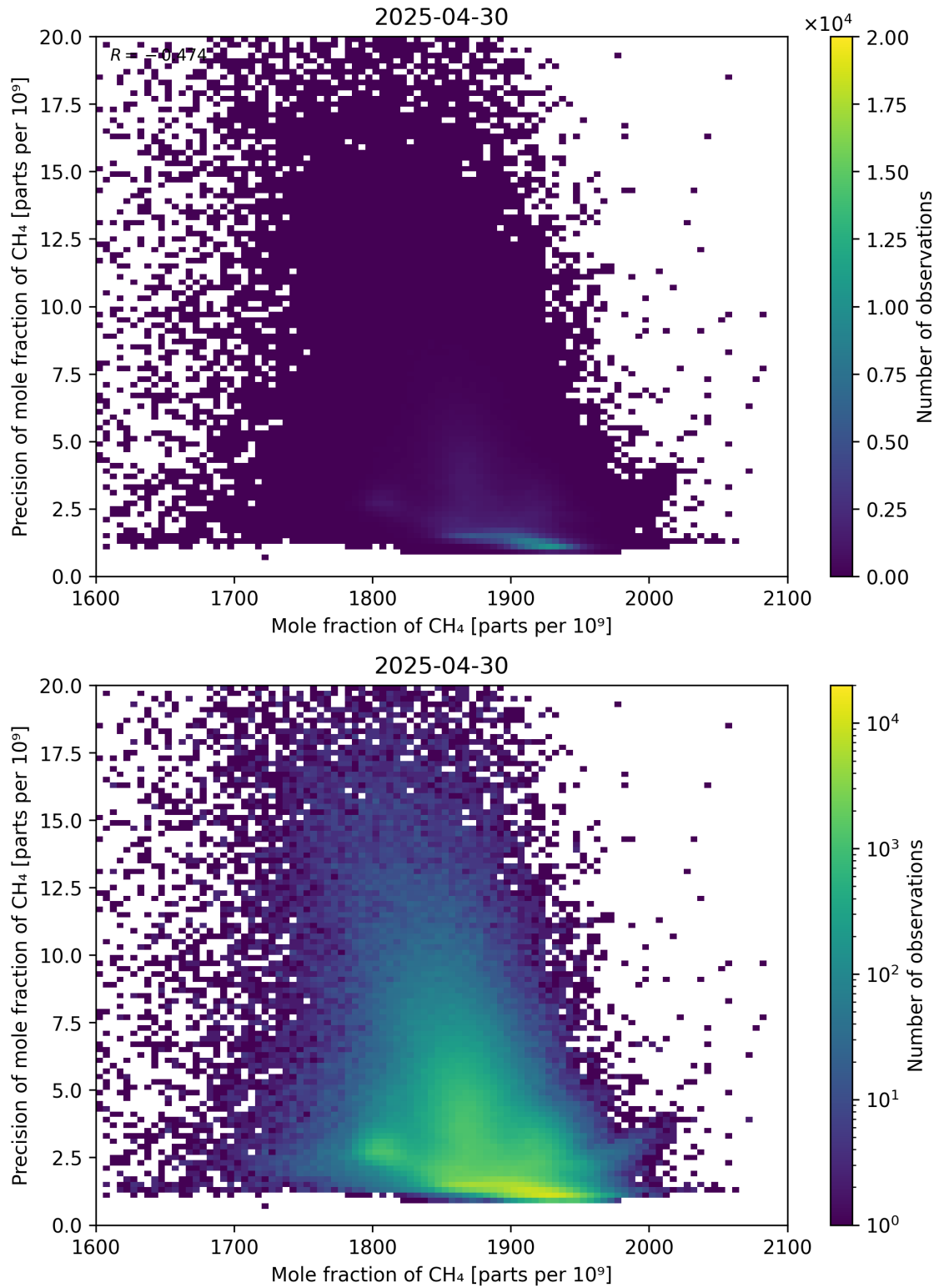
Figure 75: Scatter density plot of “Mole fraction of CH 4 ” against “Precision of mole fraction of CH 4 ” for 2025-04-29 to 2025-05-01.
