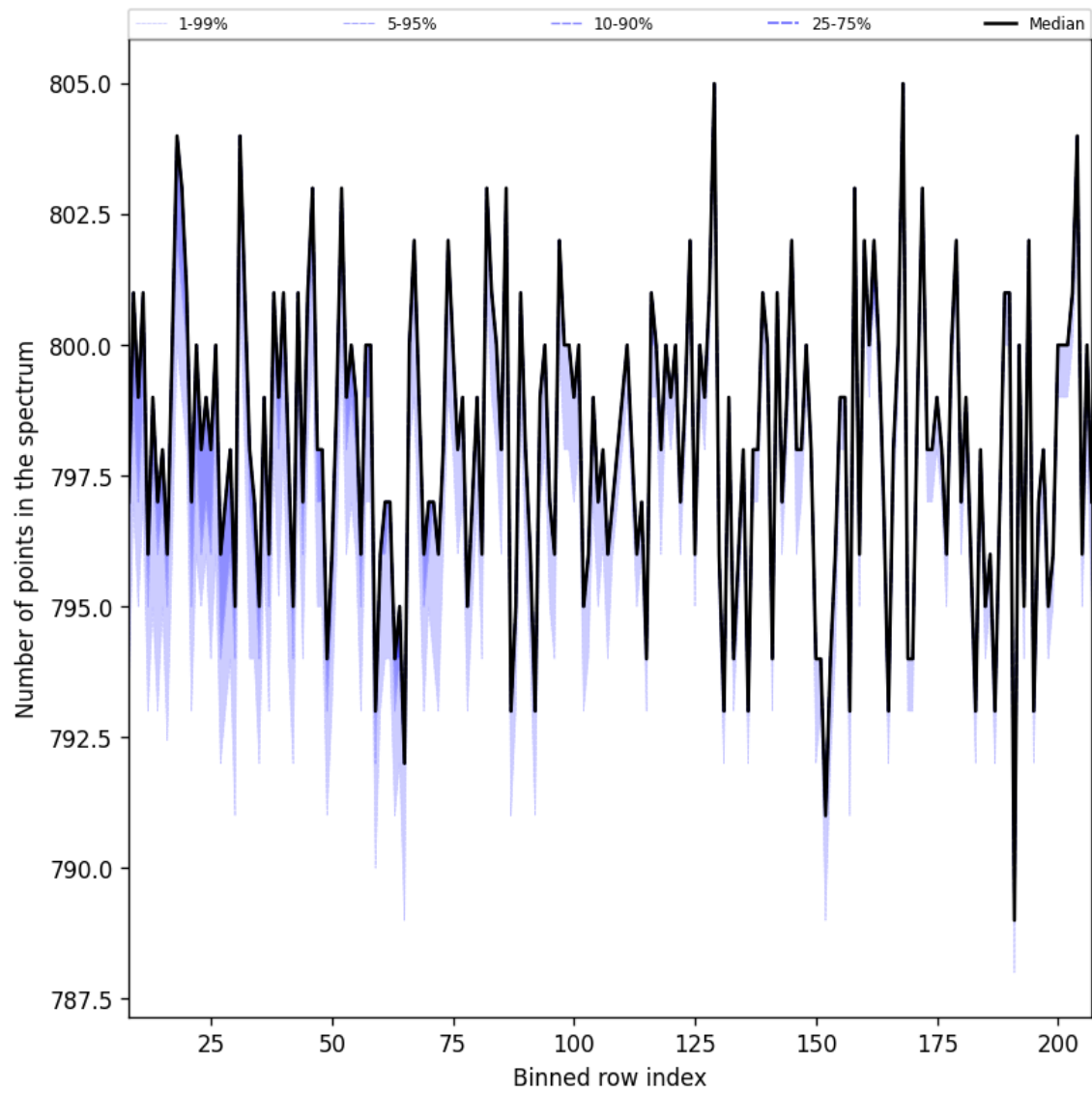
Figure 37: Along track statistics of “Number of points in the spectrum” for 2025-04-29 to 2025-05-01
