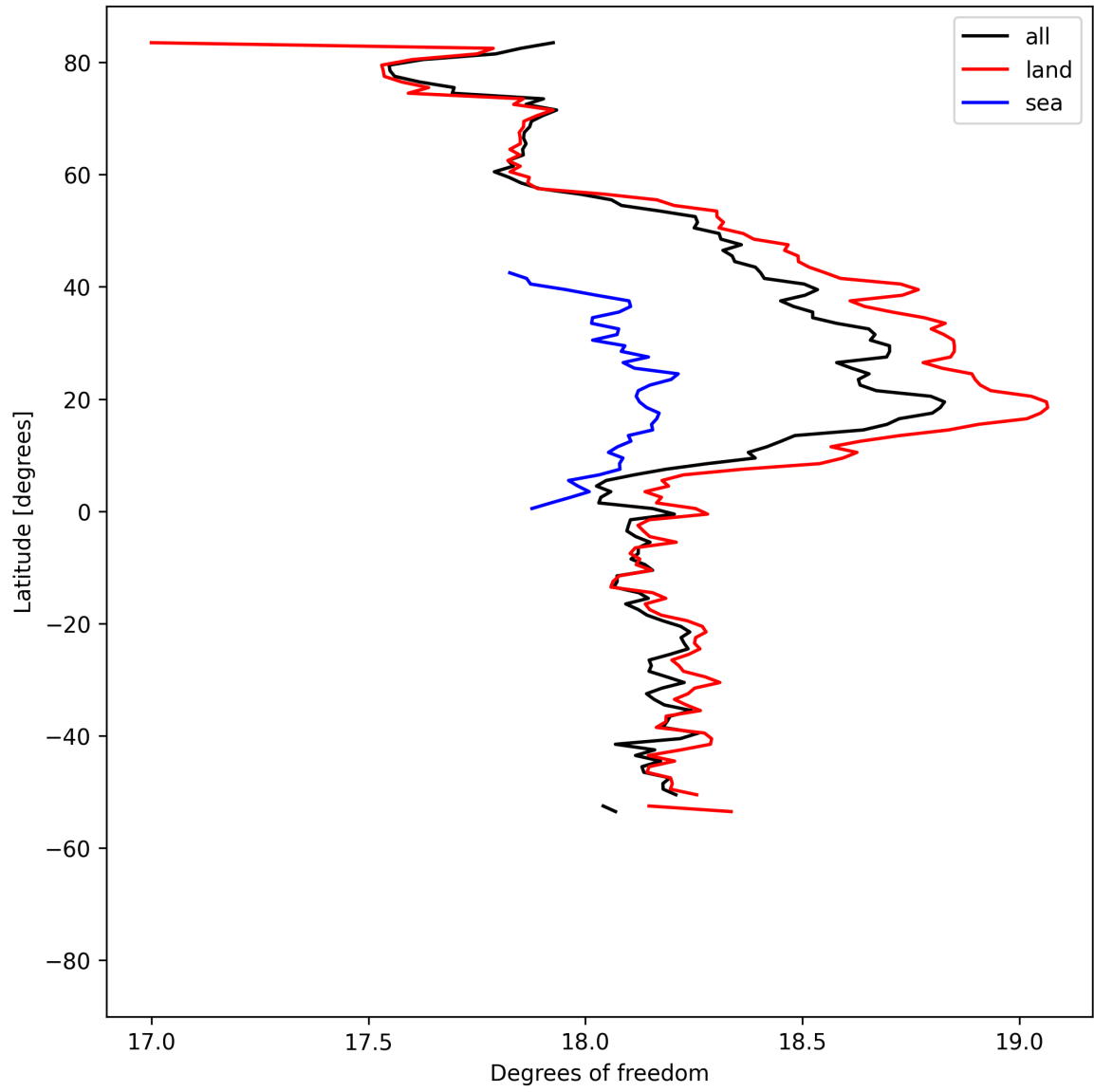
Figure 19: Zonal average of “Degrees of freedom” for 2025-04-29 to 2025-05-01.
