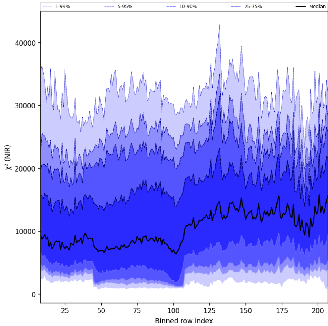
Figure 40: Along track statistics of “ \chi^2 (NIR)” for 2025-04-29 to 2025-05-01
