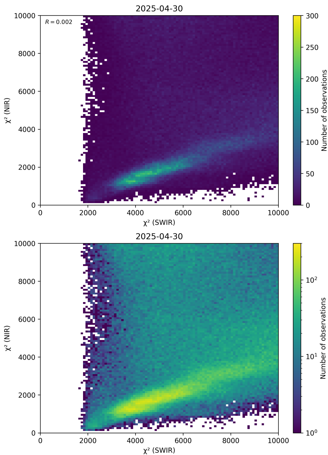
Figure 47: Scatter density plot of “ \chi^2 (SWIR)” against “ \chi^2 (NIR)” for 2025-04-29 to 2025-05-01.
