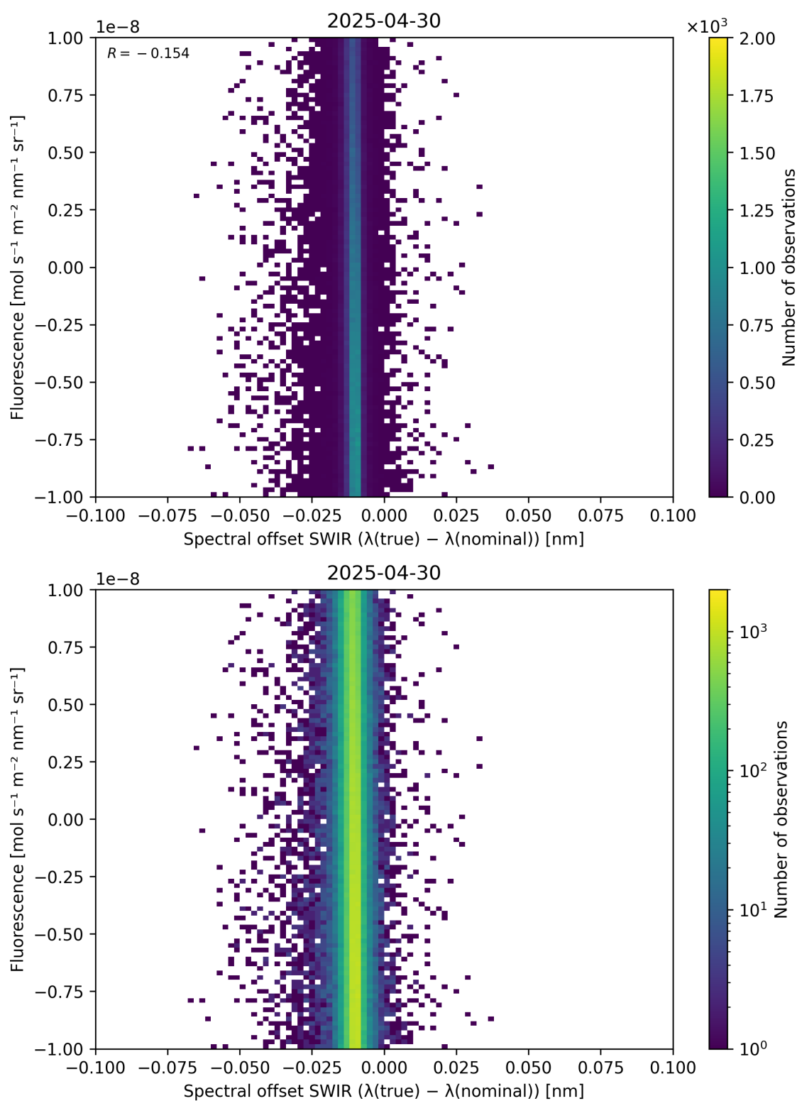
Figure 120: Scatter density plot of “Spectral offset SWIR ( \lambda_{\text{true}} - \lambda_{\text{nominal}} )” against “Fluorescence” for 2025-04-29 to 2025-05-01.
