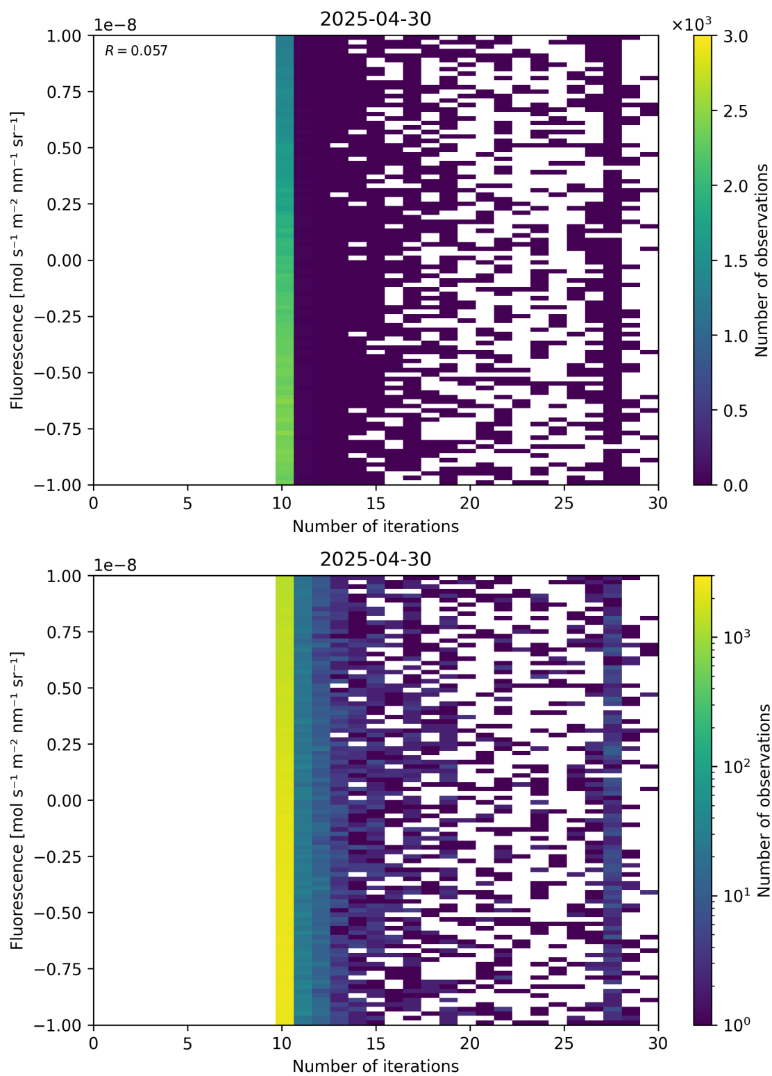
Figure 87: Scatter density plot of “Number of iterations” against “Fluorescence” for 2025-04-29 to 2025-05-01.
