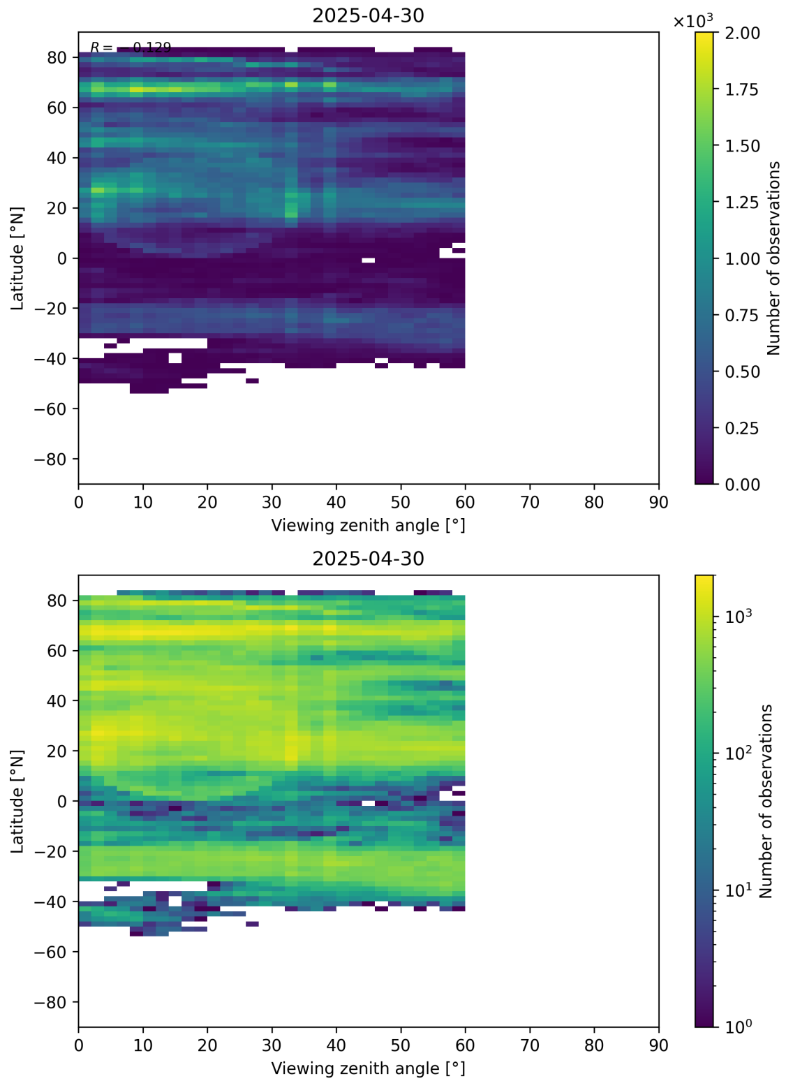
Figure 109: Scatter density plot of “Viewing zenith angle” against “Latitude” for 2025-04-29 to 2025-05-01.
