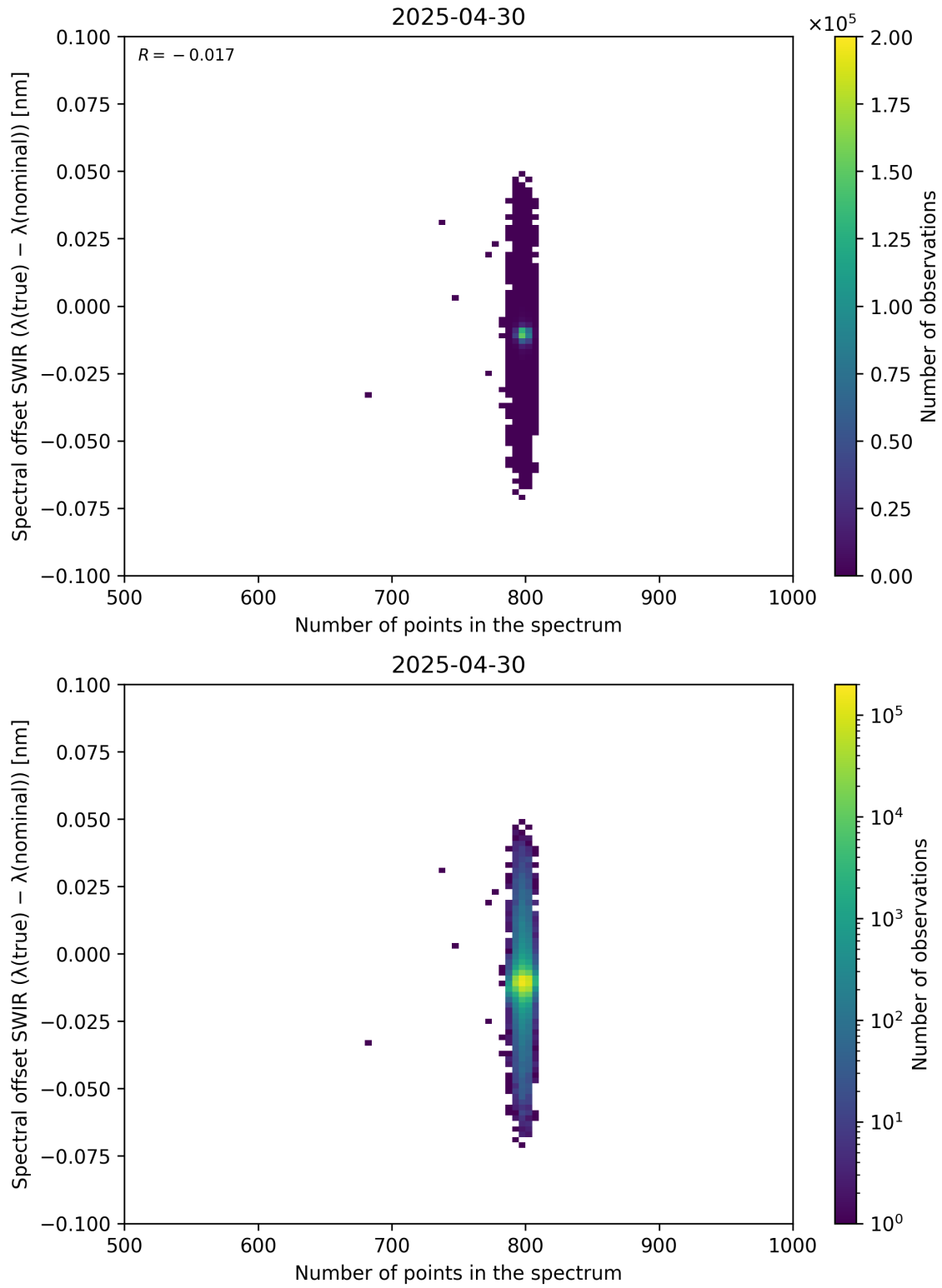
Figure 93: Scatter density plot of “Number of points in the spectrum” against “Spectral offset SWIR ( \lambda_{\text{true}} - \lambda_{\text{nominal}} )” for 2025-04-29 to 2025-05-01.
