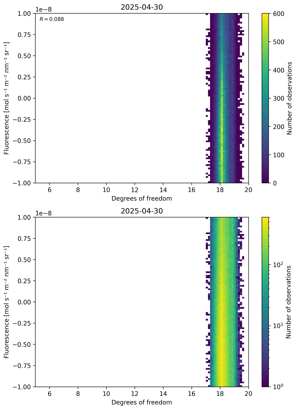
Figure 51: Scatter density plot of “Degrees of freedom” against “Fluorescence” for 2025-04-29 to 2025-05-01.
