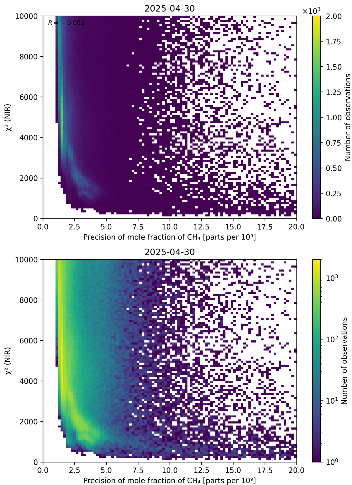
Figure 78: Scatter density plot of “Precision of mole fraction of CH 4 ” against “ \chi^2 (NIR)” for 2025-04-29 to 2025-05-01.
