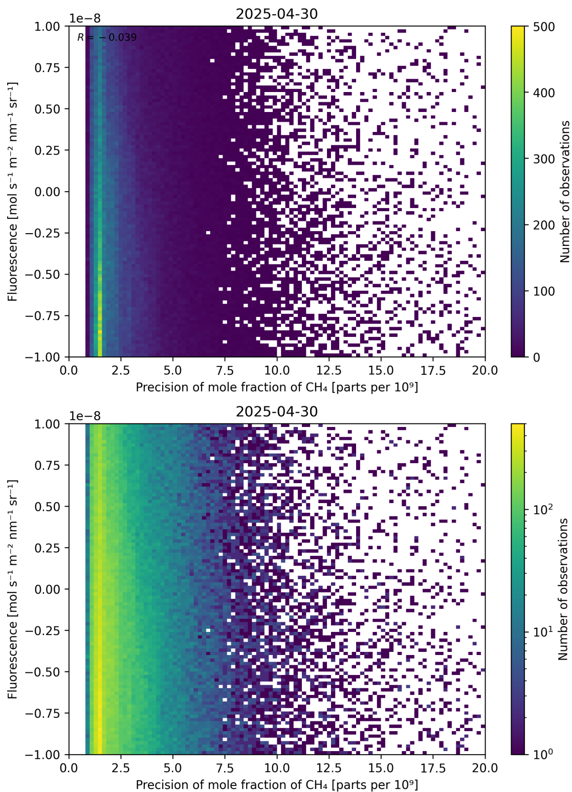
Figure 81: Scatter density plot of “Precision of mole fraction of CH 4 ” against “Fluorescence” for 2025-04-29 to 2025-05-01.
