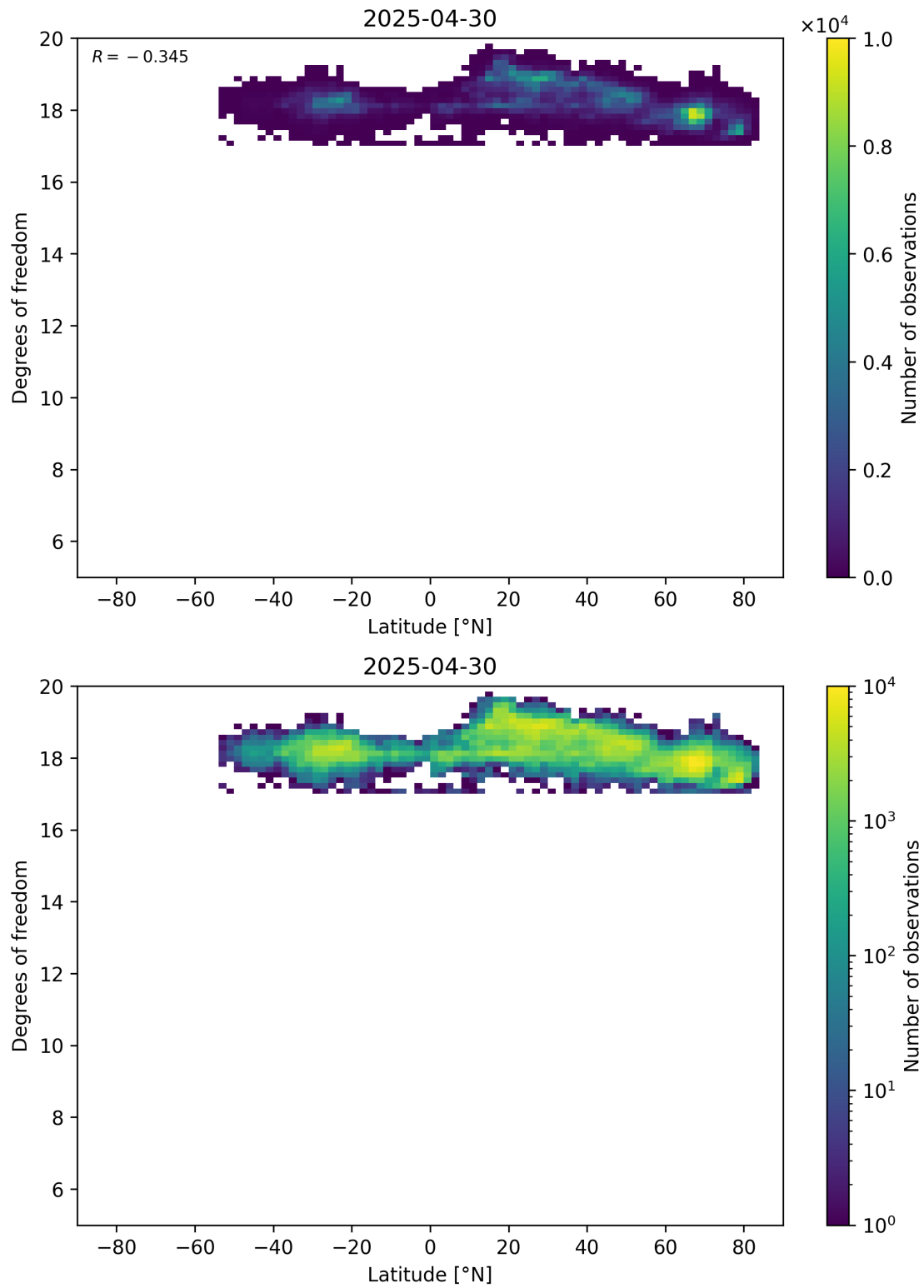
Figure 55: Scatter density plot of “Latitude” against “Degrees of freedom” for 2025-04-29 to 2025-05-01.
