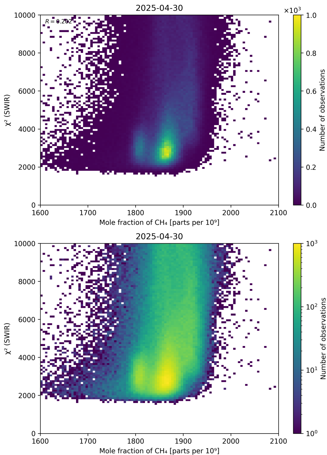
Figure 71: Scatter density plot of “Mole fraction of \text{CH}_4 ” against “ \chi^2 (SWIR)” for 2025-04-29 to 2025-05-01.
