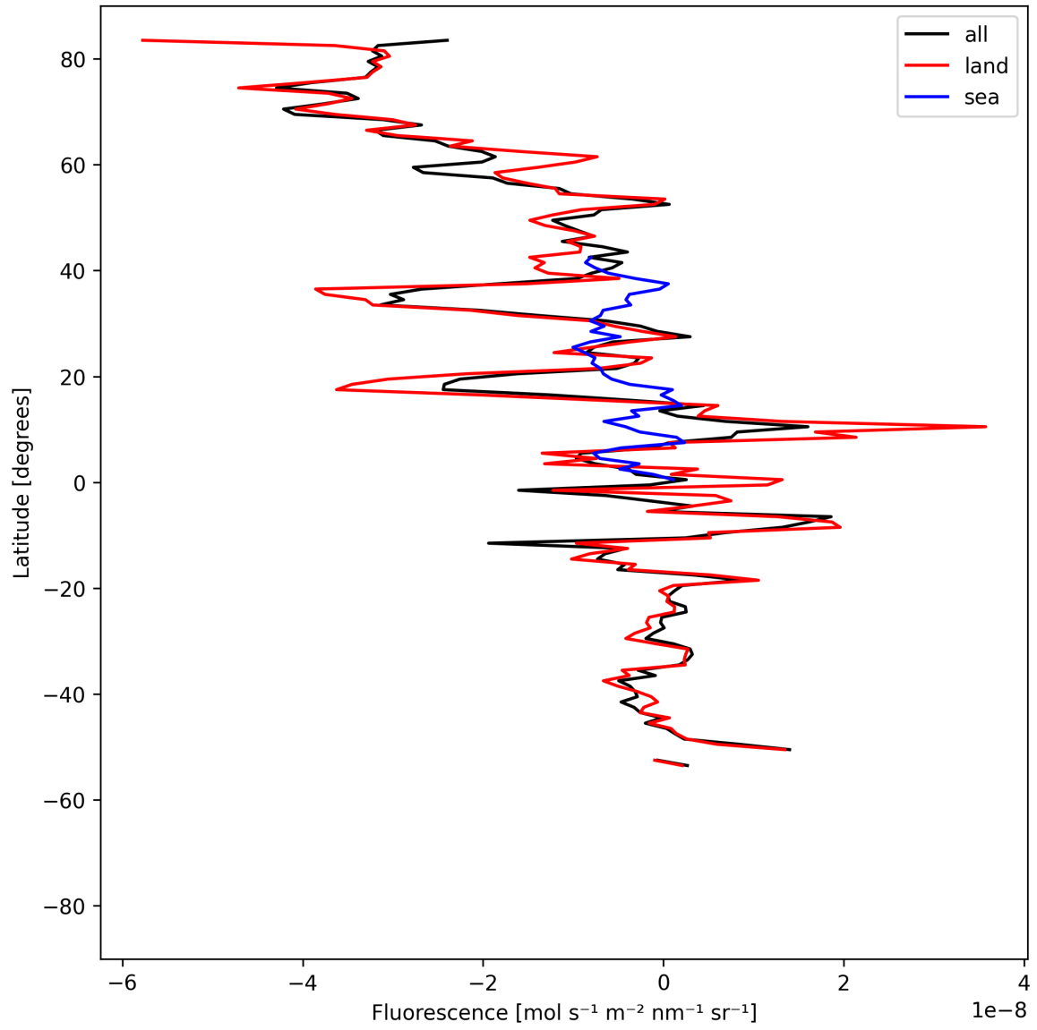
Figure 21: Zonal average of “Fluorescence” for 2025-04-29 to 2025-05-01.
