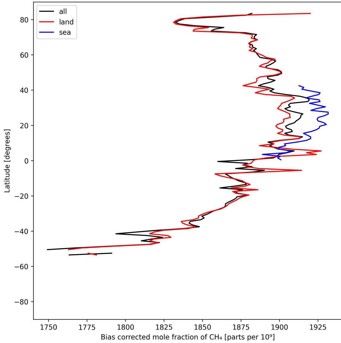
Figure 14: Zonal average of “Bias corrected mole fraction of \text{CH}_4 ” for 2025-04-29 to 2025-05-01.
