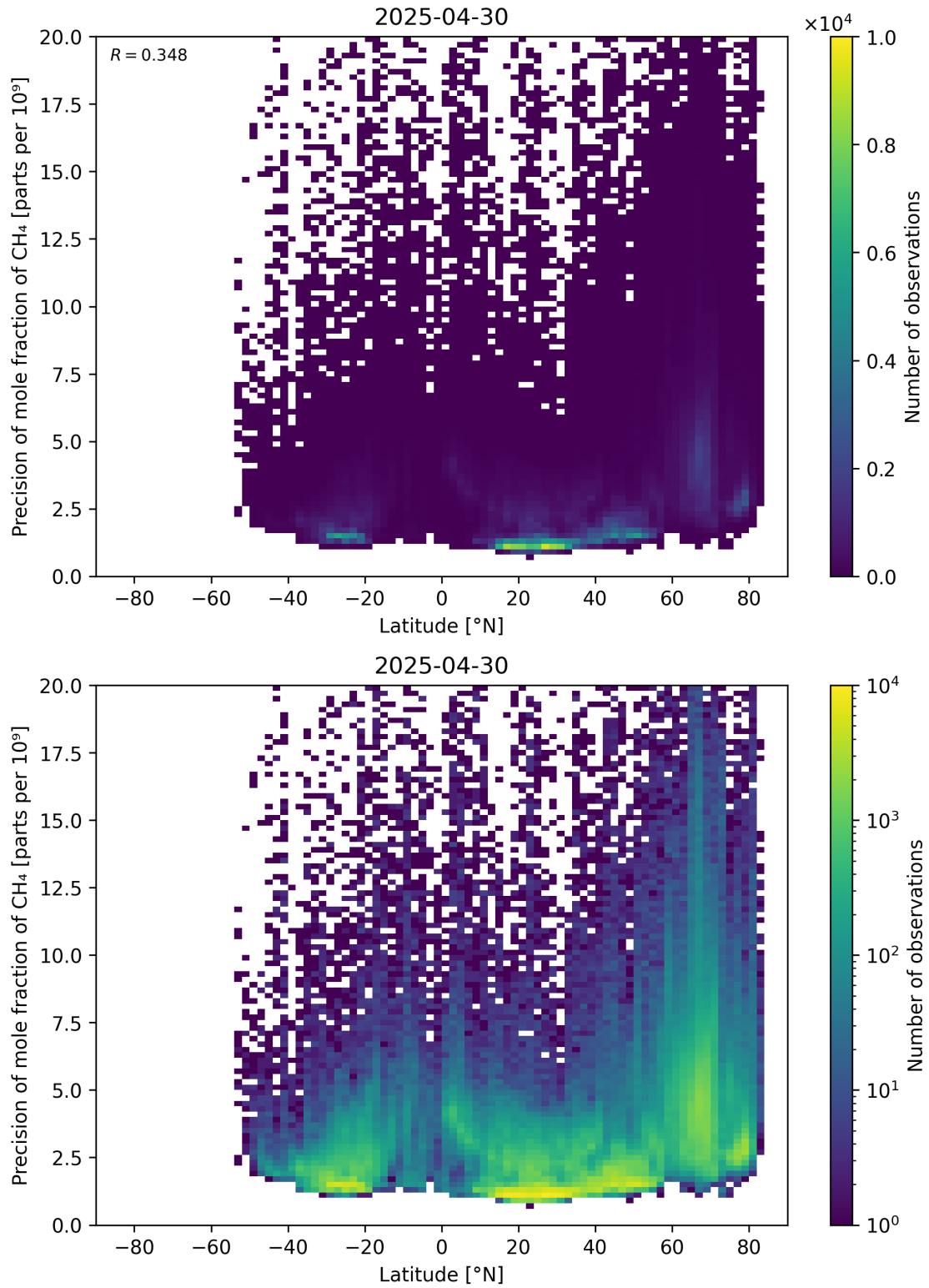
Figure 59: Scatter density plot of “Latitude” against “Precision of mole fraction of \text{CH}_4 ” for 2025-04-29 to 2025-05-01.
