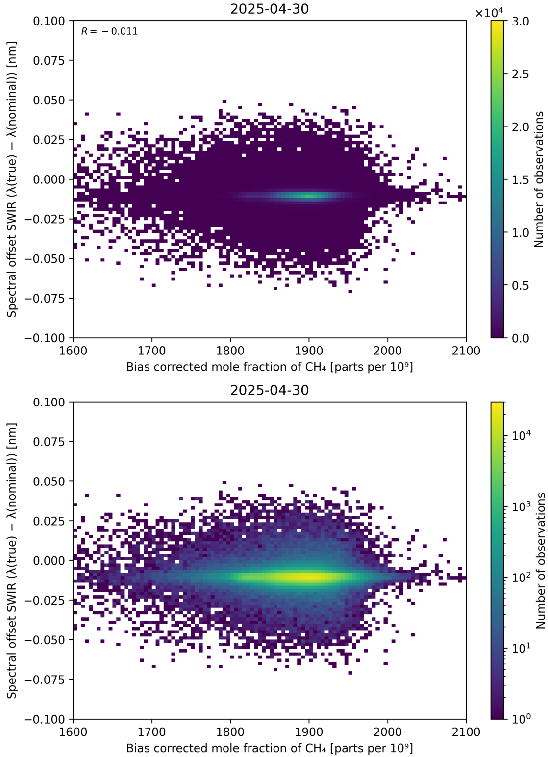
Figure 69: Scatter density plot of “Bias corrected mole fraction of \text{CH}_4 ” against “Spectral offset SWIR ( \lambda_{\text{true}} - \lambda_{\text{nominal}} )” for 2025-04-29 to 2025-05-01.
