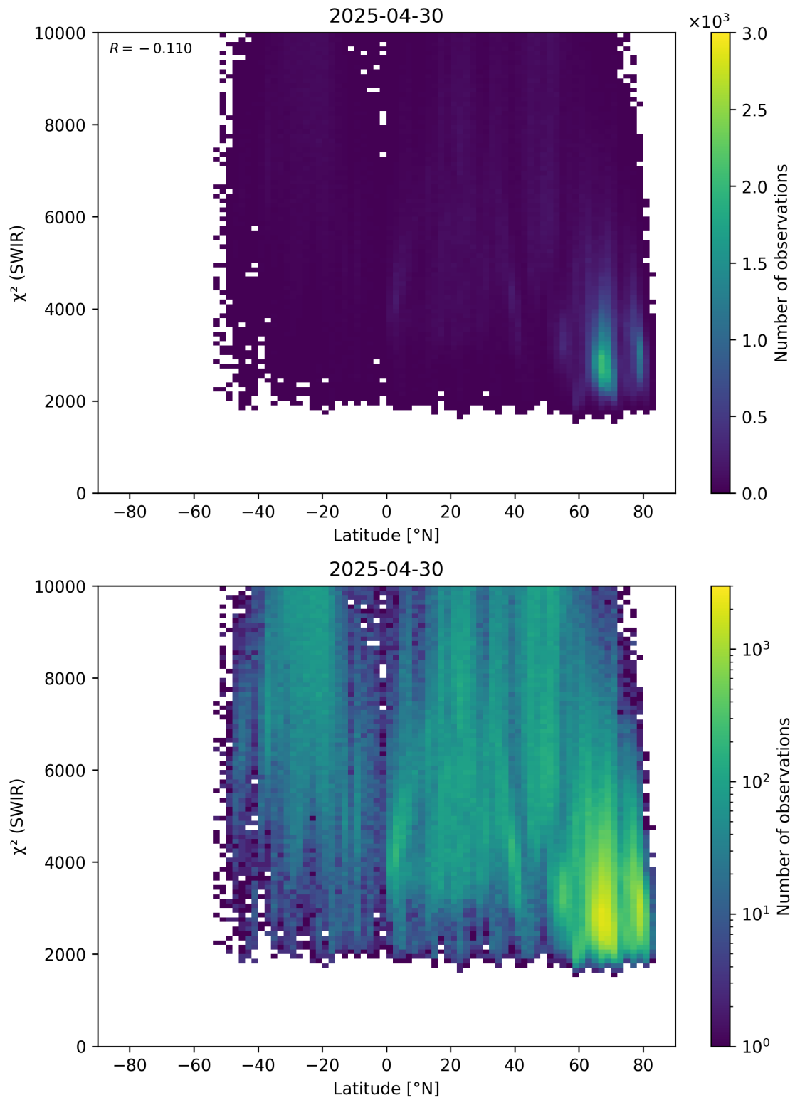
Figure 54: Scatter density plot of “Latitude” against “ \chi^2 (SWIR)” for 2025-04-29 to 2025-05-01.
