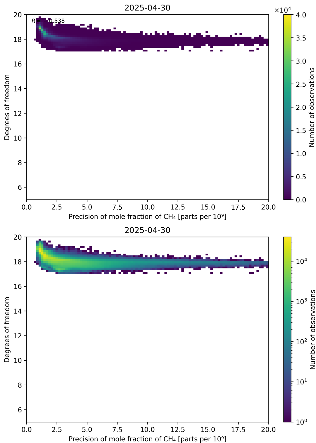
Figure 80: Scatter density plot of “Precision of mole fraction of CH 4 ” against “Degrees of freedom” for 2025-04-29 to 2025-05-01.
