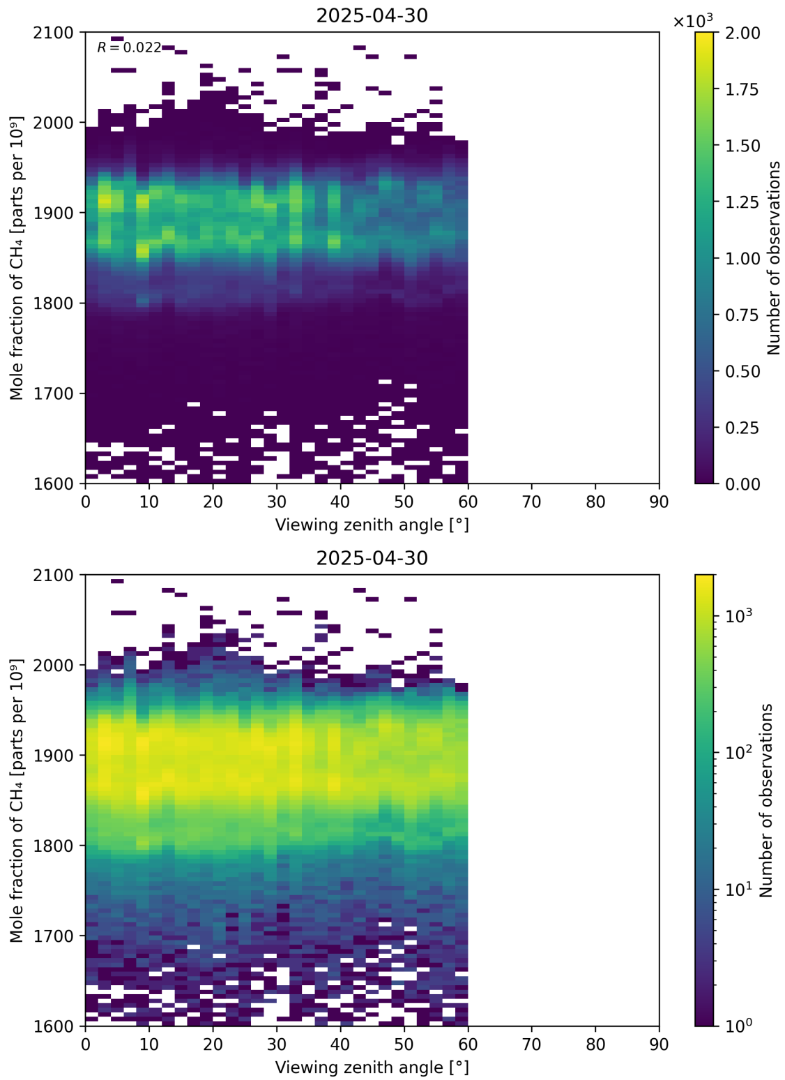
Figure 110: Scatter density plot of “Viewing zenith angle” against “Mole fraction of CH 4 ” for 2025-04-29 to 2025-05-01.
