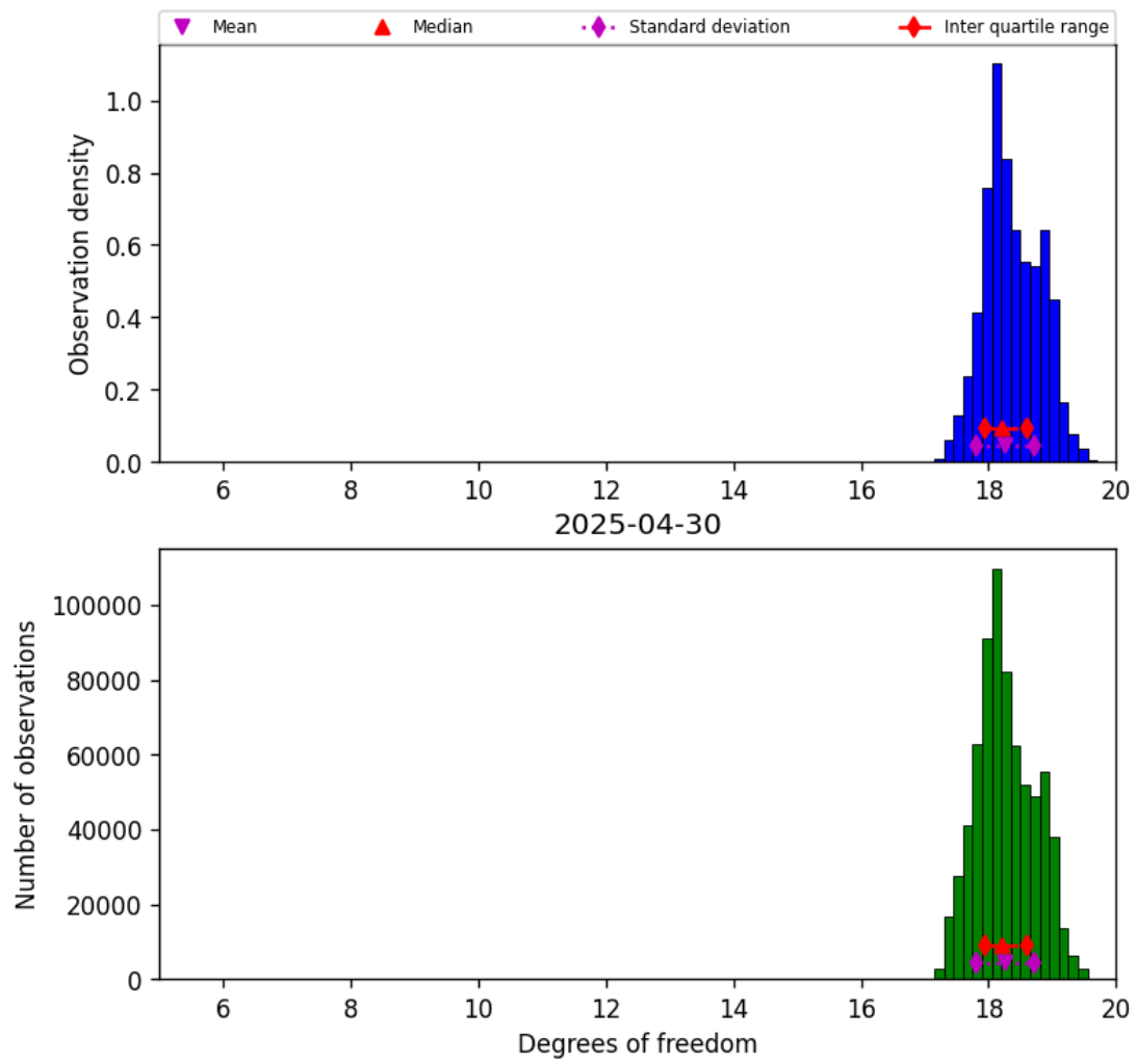
Figure 30: Histogram of “Degrees of freedom” for 2025-04-29 to 2025-05-01
