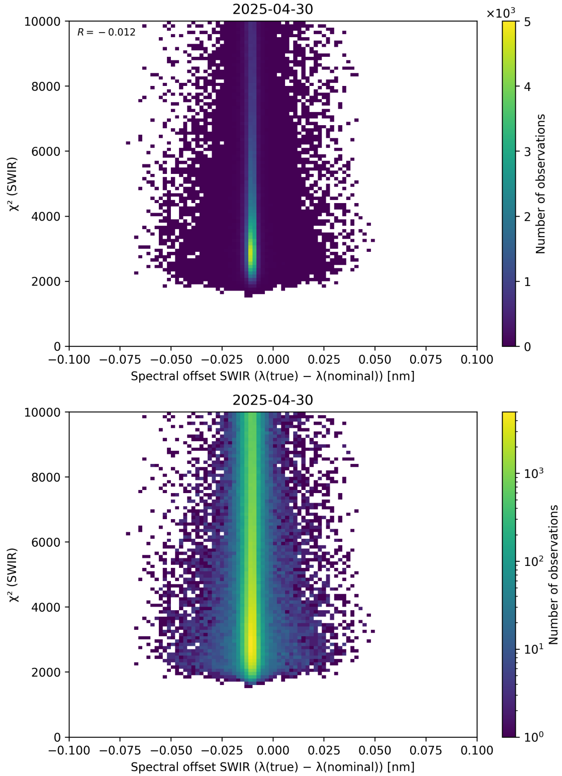
Figure 118: Scatter density plot of “Spectral offset SWIR ( \lambda_{\text{true}} - \lambda_{\text{nominal}} )” against “ \chi^2 (SWIR)” for 2025-04-29 to 2025-05-01.
