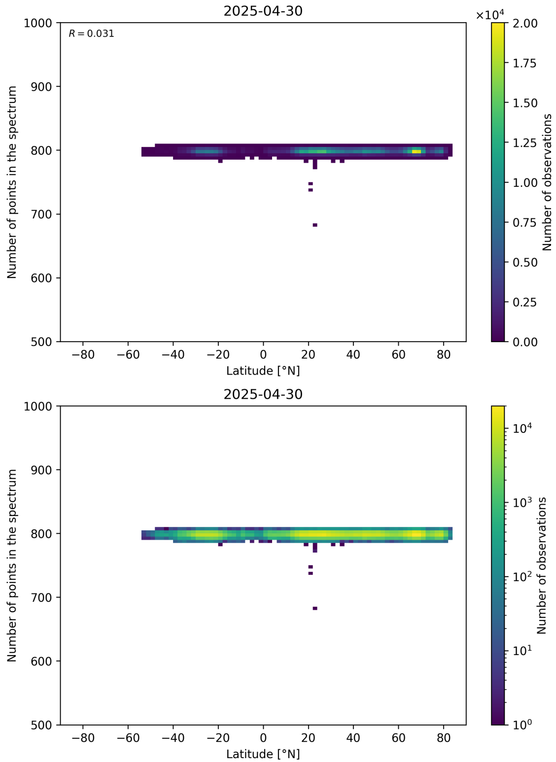
Figure 61: Scatter density plot of “Latitude” against “Number of points in the spectrum” for 2025-04-29 to 2025-05-01.
