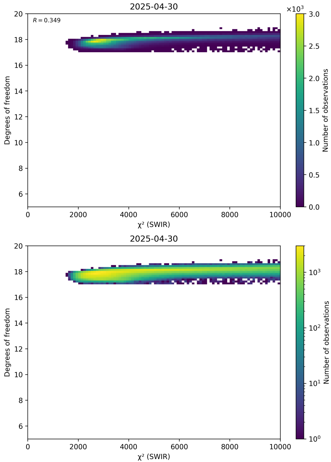
Figure 48: Scatter density plot of “ \chi^2 (SWIR)” against “Degrees of freedom” for 2025-04-29 to 2025-05-01.
