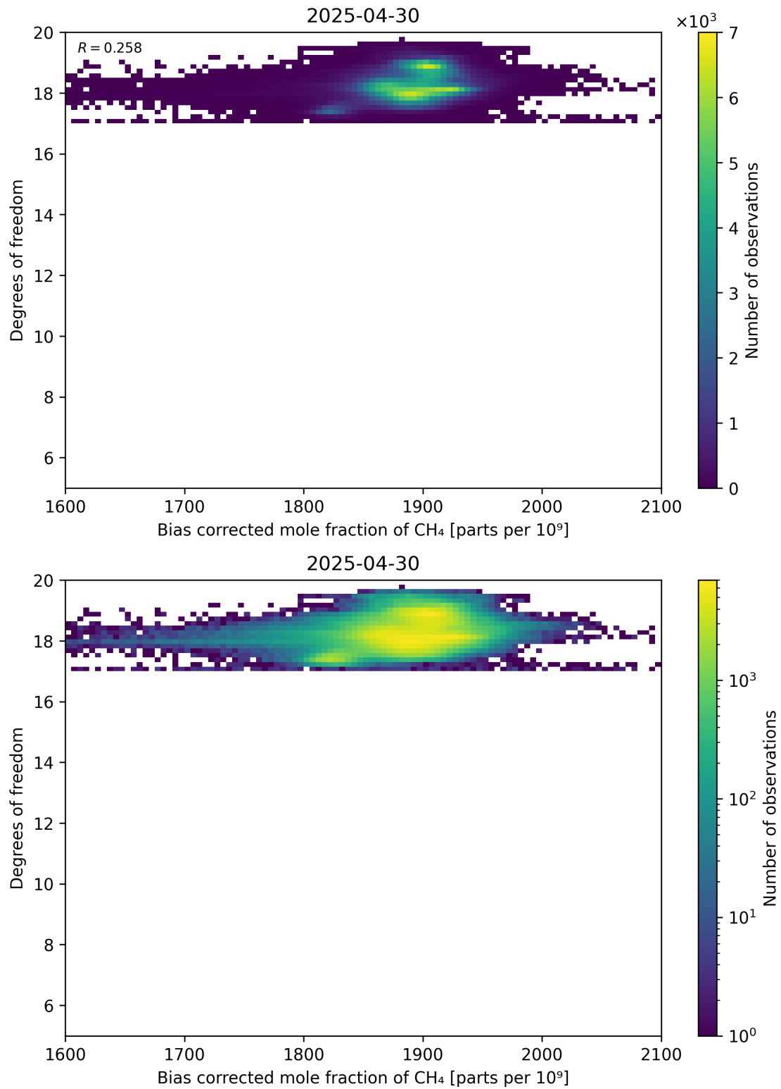
Figure 65: Scatter density plot of “Bias corrected mole fraction of CH 4 ” against “Degrees of freedom” for 2025-04-29 to 2025-05-01.
