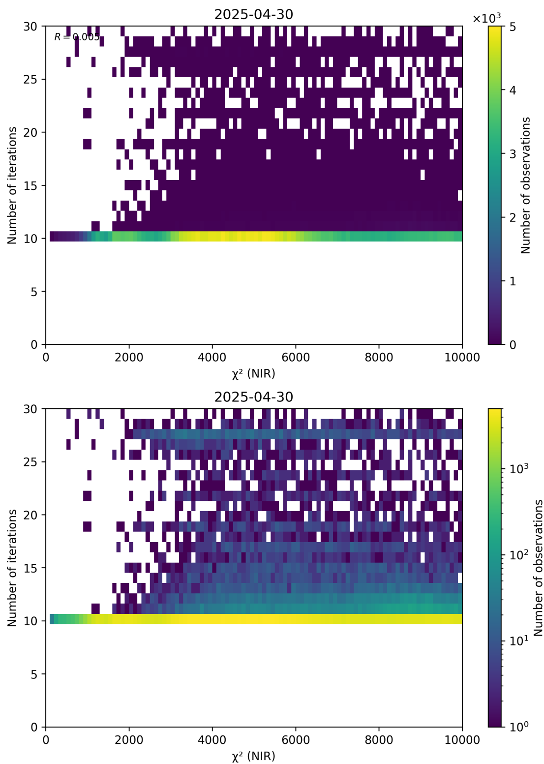
Figure 46: Scatter density plot of “ \chi^2 (NIR)” against “Number of iterations” for 2025-04-29 to 2025-05-01.
