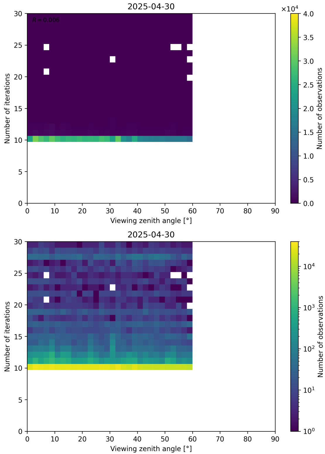
Figure 113: Scatter density plot of “Viewing zenith angle” against “Number of iterations” for 2025-04-29 to 2025-05-01.
