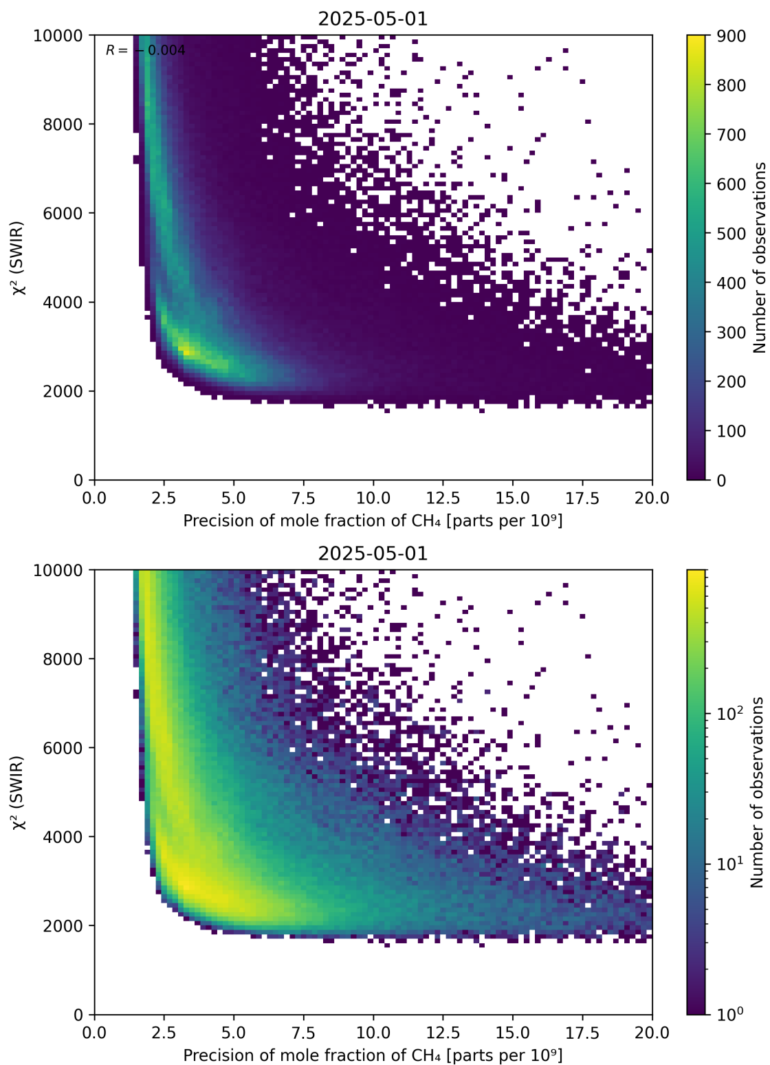
Figure 79: Scatter density plot of “Precision of mole fraction of \text{CH}_4 ” against “ \chi^2 (SWIR)” for 2025-04-30 to 2025-05-02.
