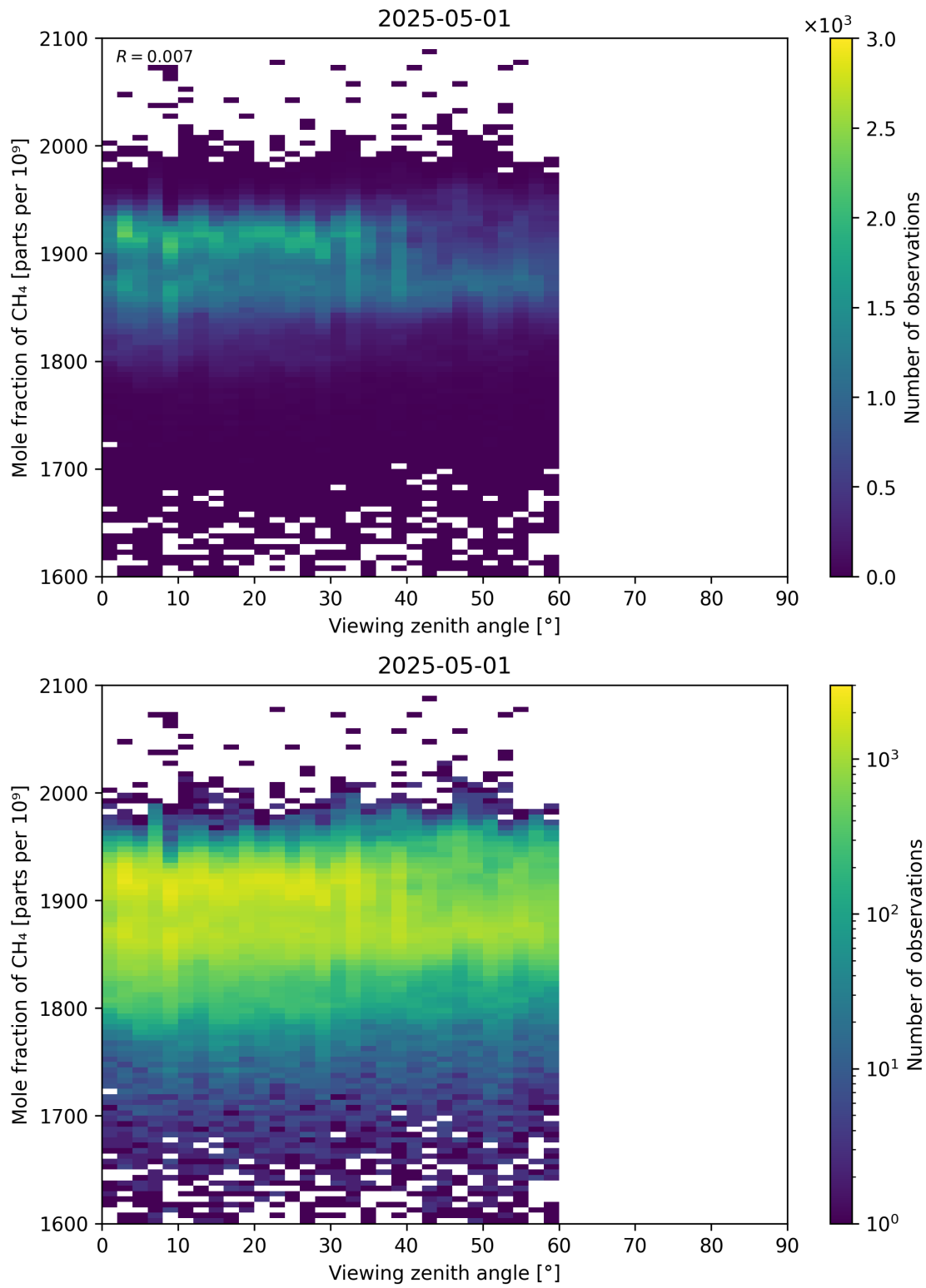
Figure 110: Scatter density plot of “Viewing zenith angle” against “Mole fraction of CH 4 ” for 2025-04-30 to 2025-05-02.
