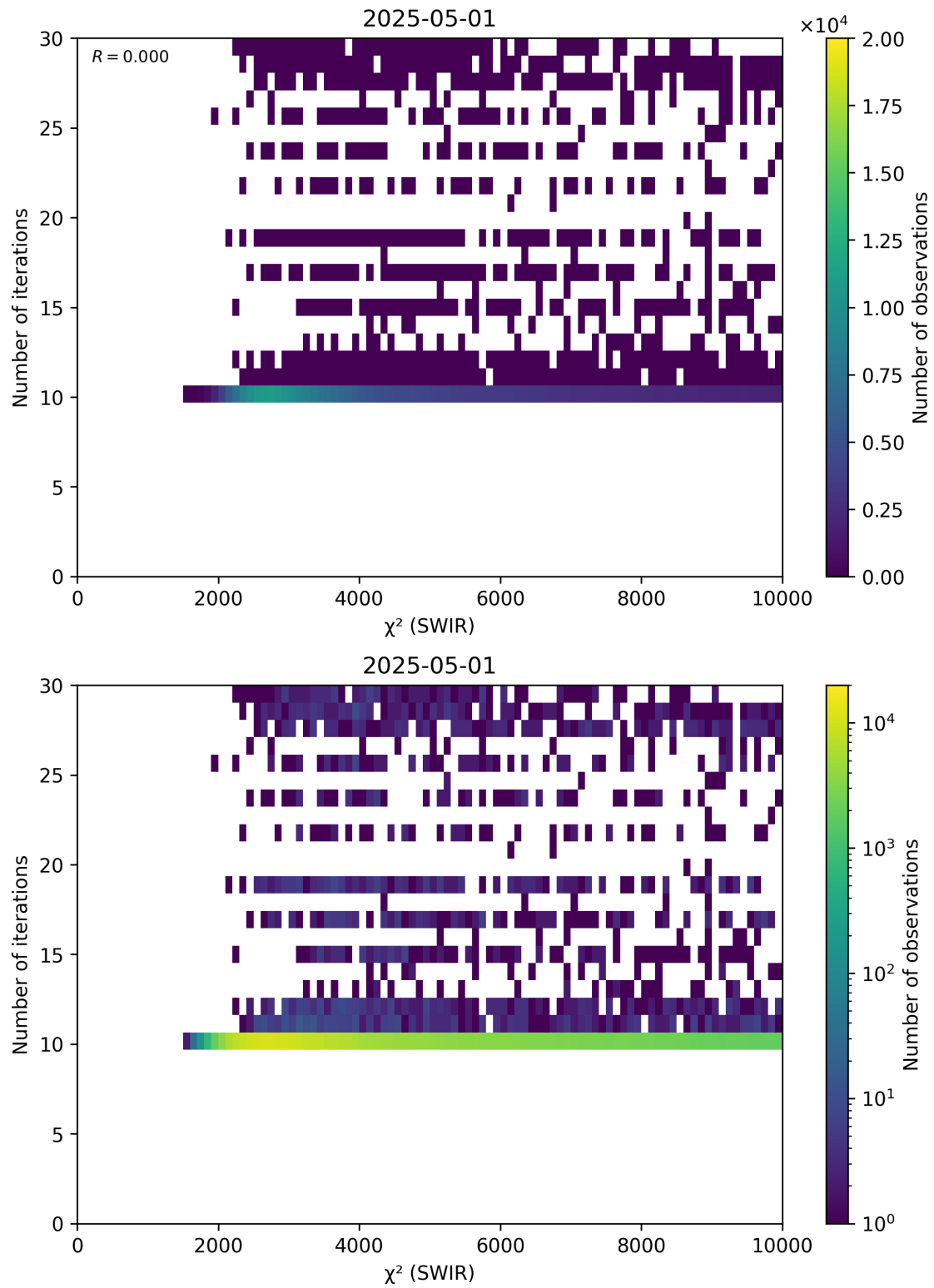
Figure 50: Scatter density plot of “ \chi^2 (SWIR)” against “Number of iterations” for 2025-04-30 to 2025-05-02.
