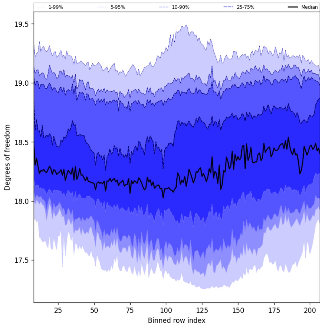
Figure 41: Along track statistics of “Degrees of freedom” for 2025-04-30 to 2025-05-02
