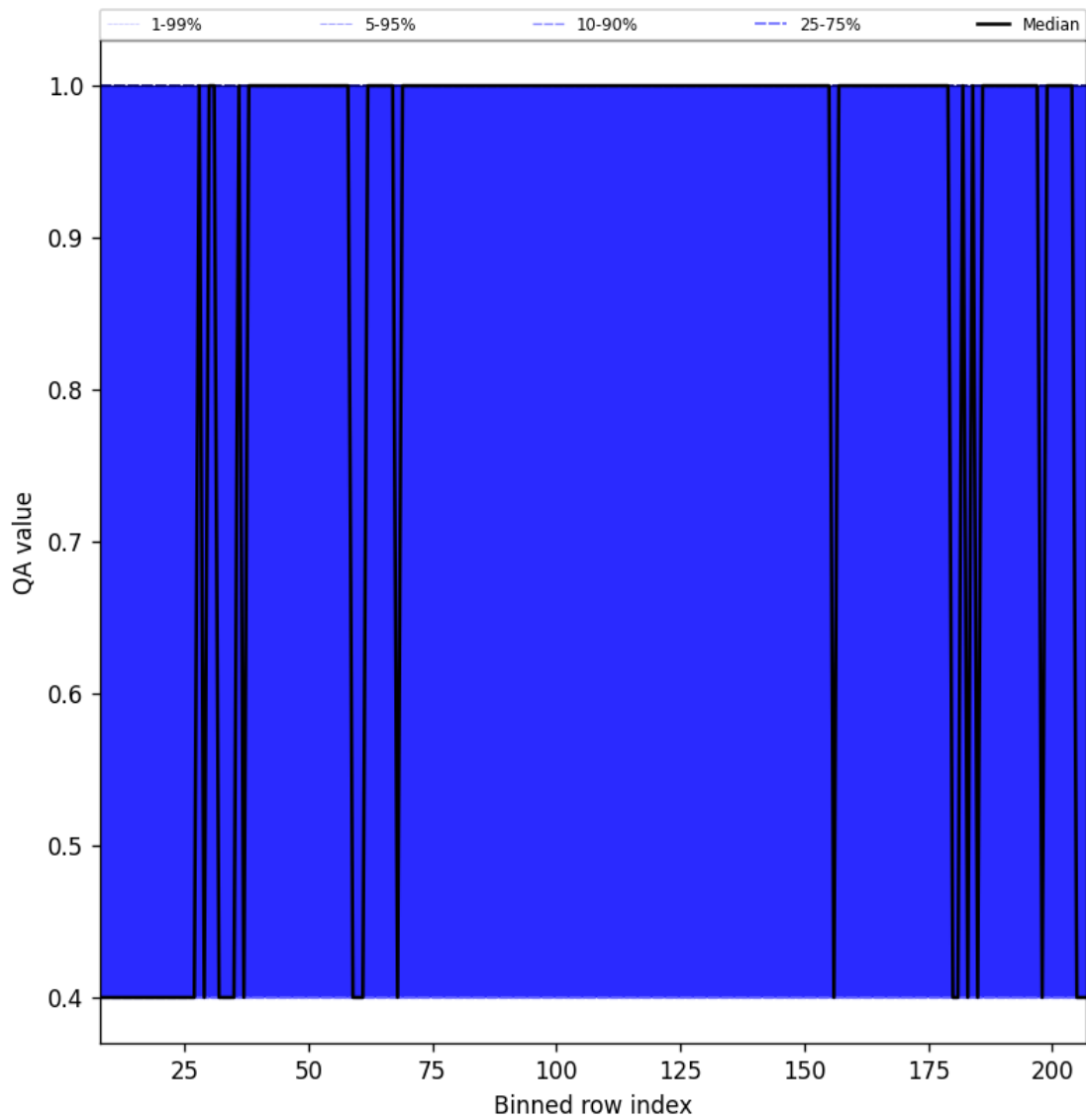
Figure 33: Along track statistics of “QA value” for 2025-04-30 to 2025-05-02
