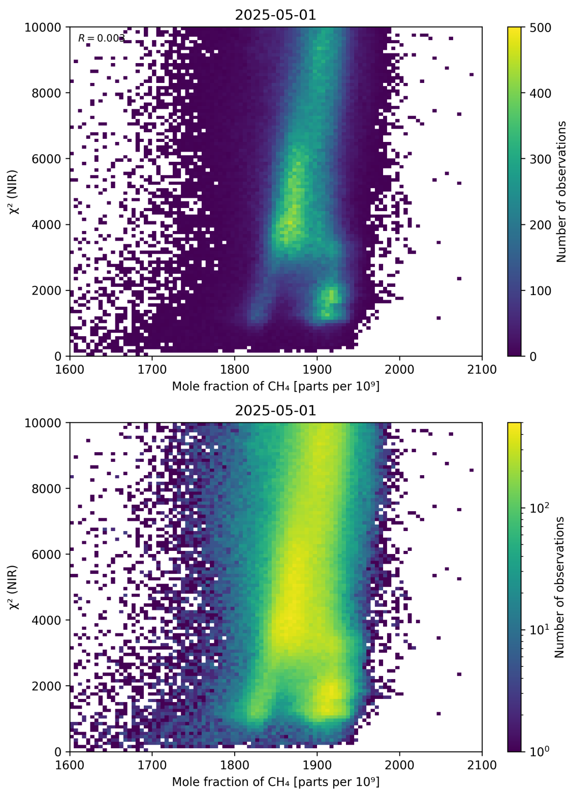
Figure 70: Scatter density plot of “Mole fraction of CH 4 ” against “ \chi^2 (NIR)” for 2025-04-30 to 2025-05-02.
