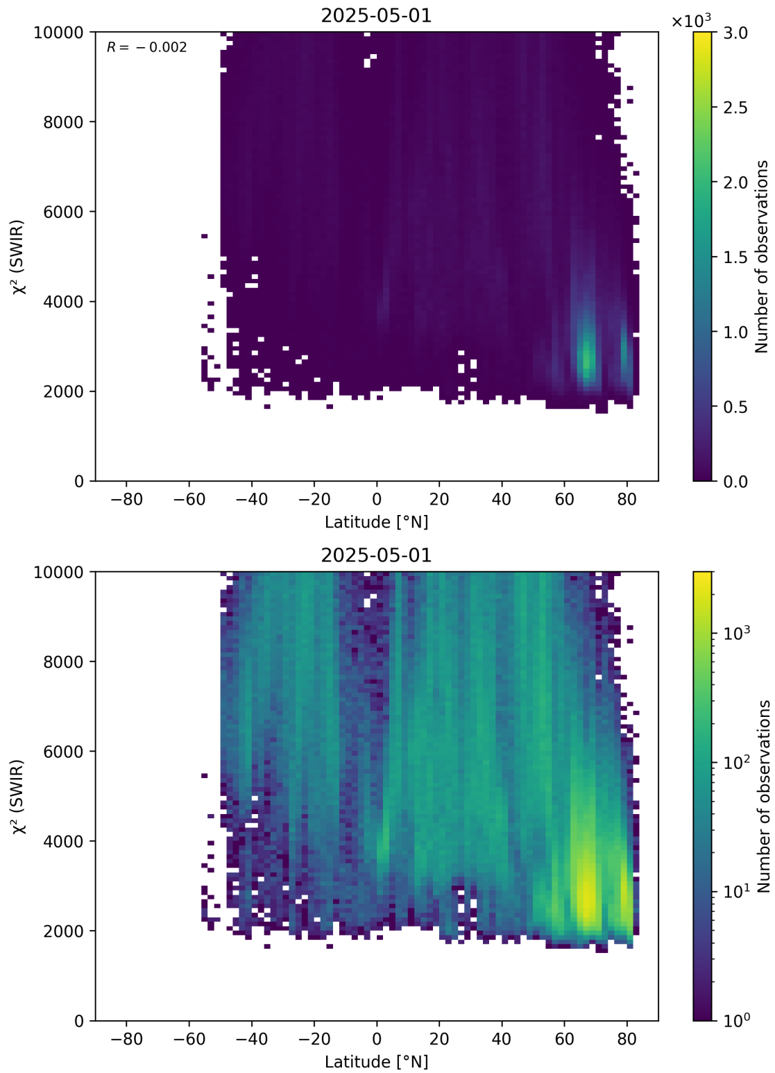
Figure 54: Scatter density plot of “Latitude” against “ \chi^2 (SWIR)” for 2025-04-30 to 2025-05-02.
