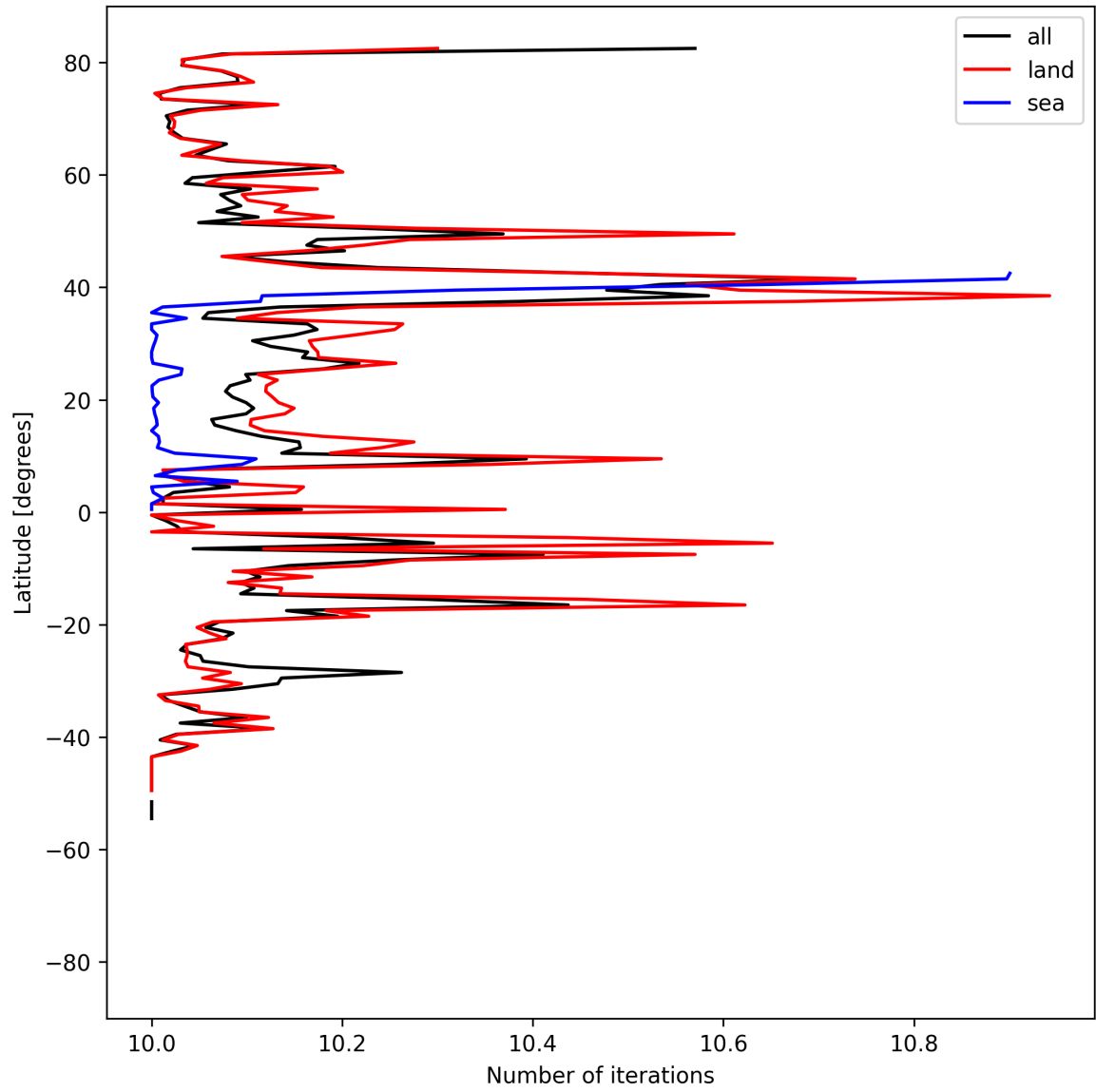
Figure 20: Zonal average of “Number of iterations” for 2025-04-30 to 2025-05-02.
