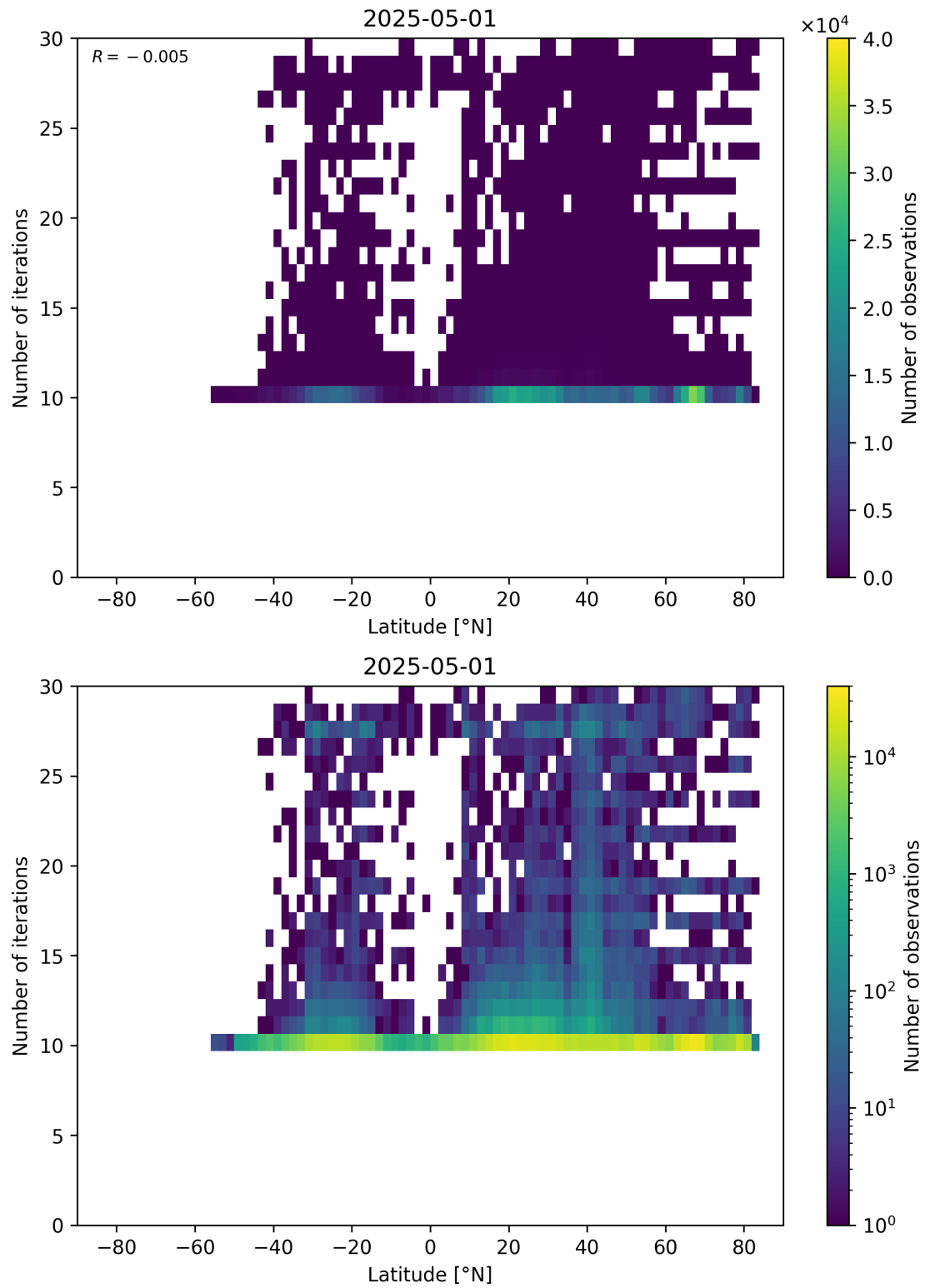
Figure 60: Scatter density plot of “Latitude” against “Number of iterations” for 2025-04-30 to 2025-05-02.
