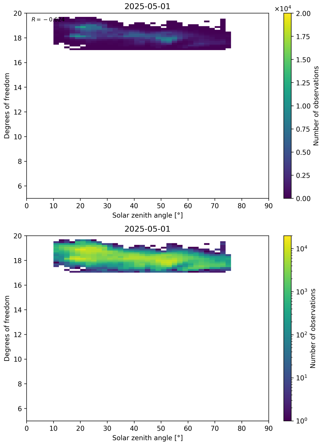
Figure 96: Scatter density plot of “Solar zenith angle” against “Degrees of freedom” for 2025-04-30 to 2025-05-02.
