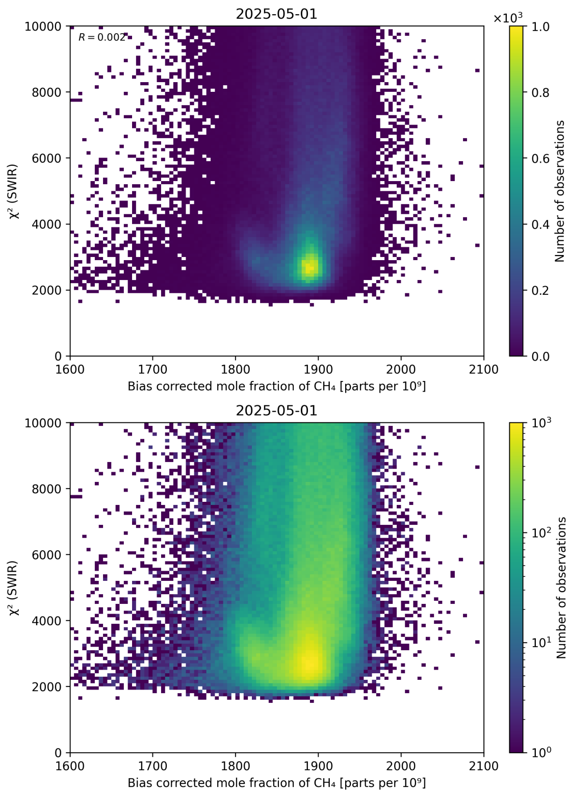
Figure 64: Scatter density plot of “Bias corrected mole fraction of \text{CH}_4 ” against “ \chi^2 (SWIR)” for 2025-04-30 to 2025-05-02.
