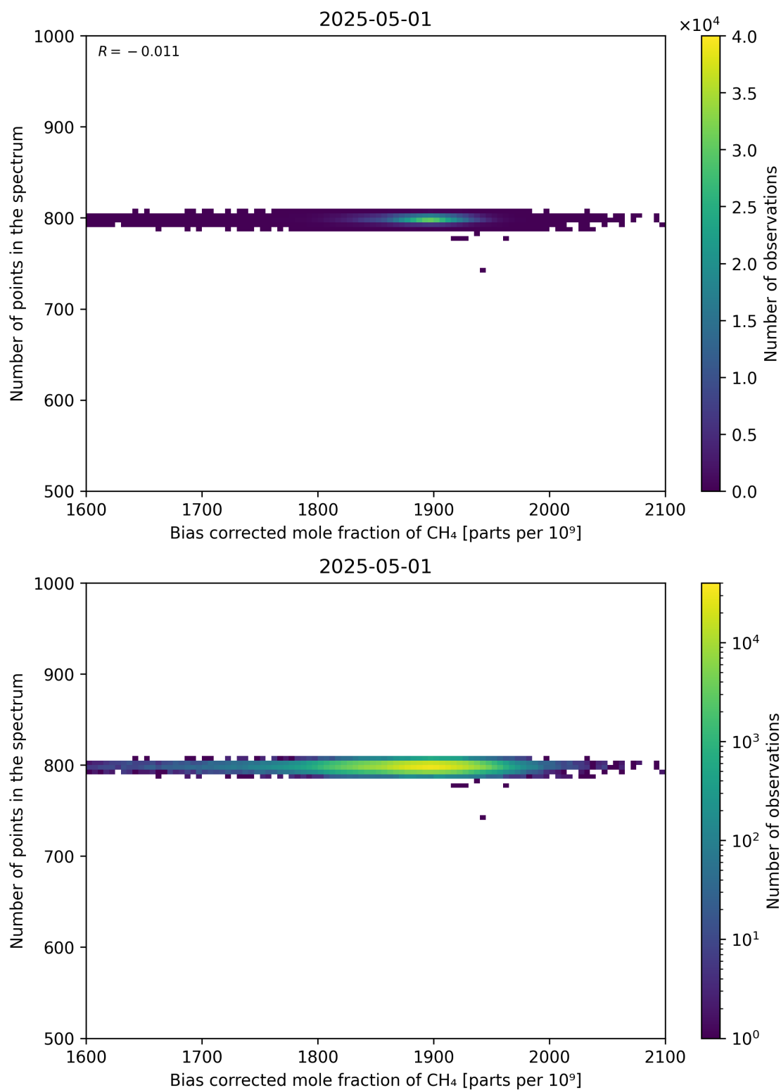
Figure 68: Scatter density plot of “Bias corrected mole fraction of CH 4 ” against “Number of points in the spectrum” for 2025-04-30 to 2025-05-02.
