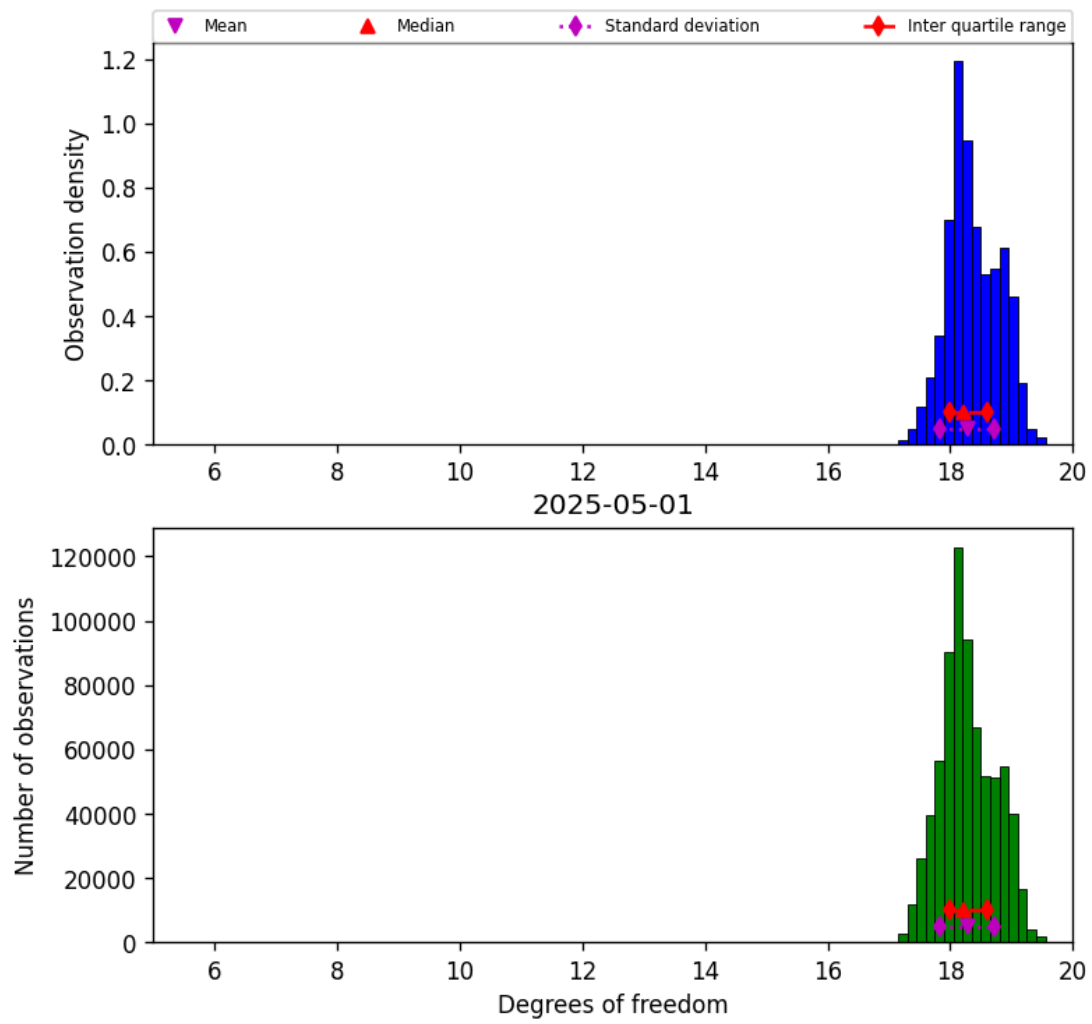
Figure 30: Histogram of “Degrees of freedom” for 2025-04-30 to 2025-05-02
