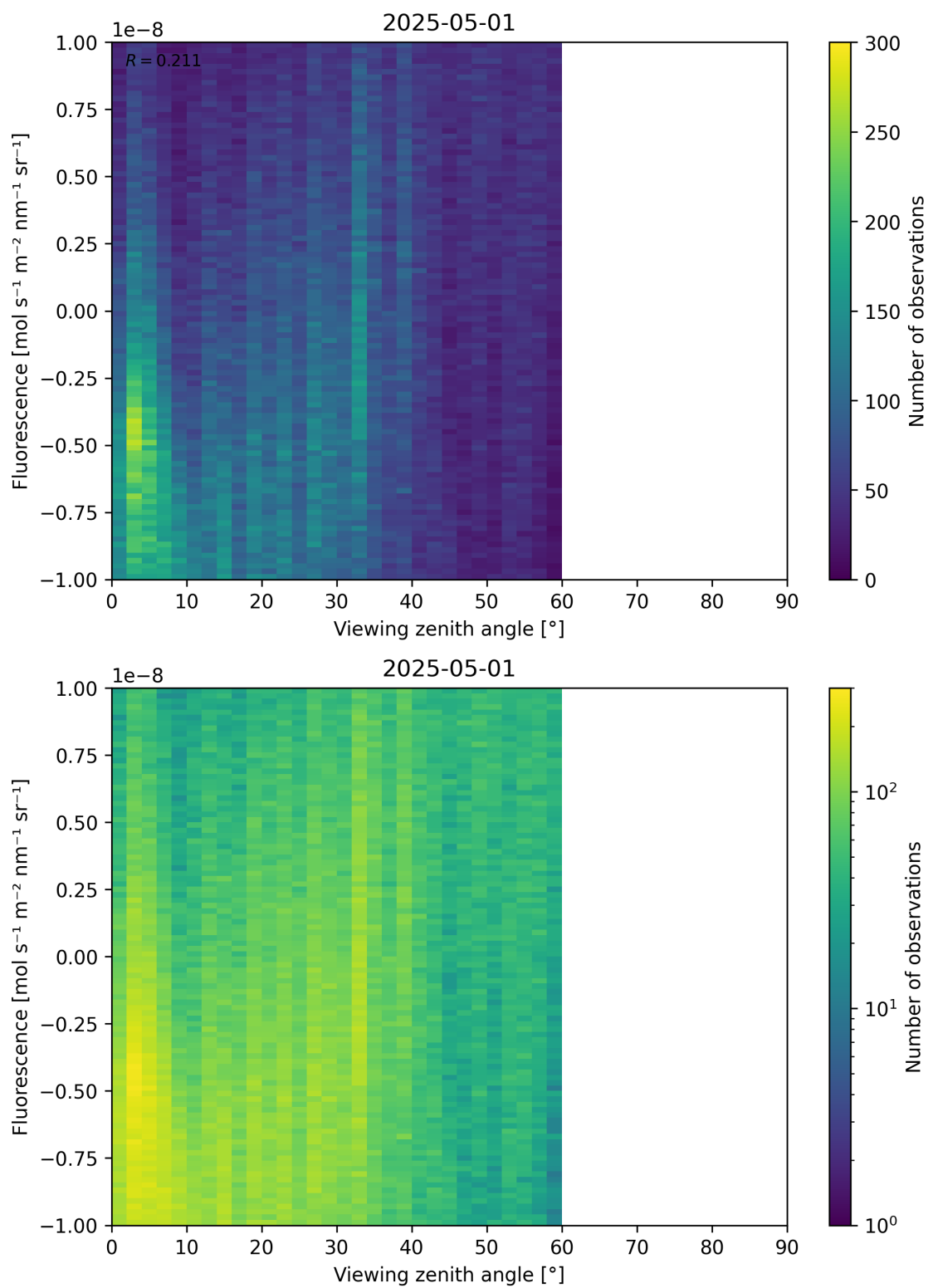
Figure 108: Scatter density plot of “Viewing zenith angle” against “Fluorescence” for 2025-04-30 to 2025-05-02.
