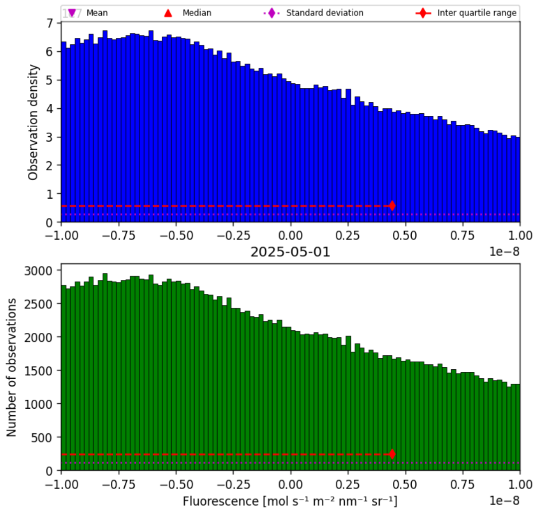
Figure 32: Histogram of “Fluorescence” for 2025-04-30 to 2025-05-02
