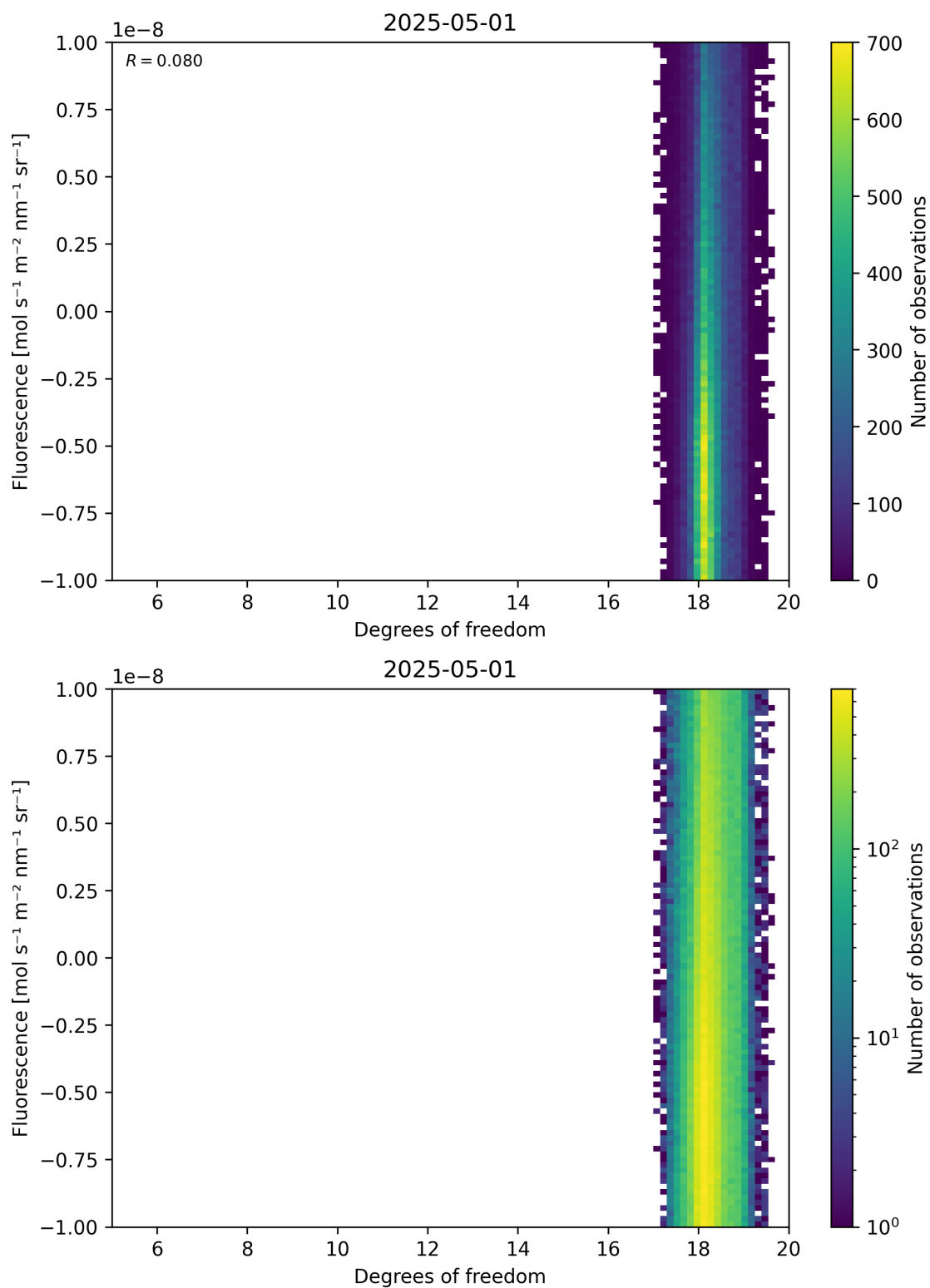
Figure 51: Scatter density plot of “Degrees of freedom” against “Fluorescence” for 2025-04-30 to 2025-05-02.
