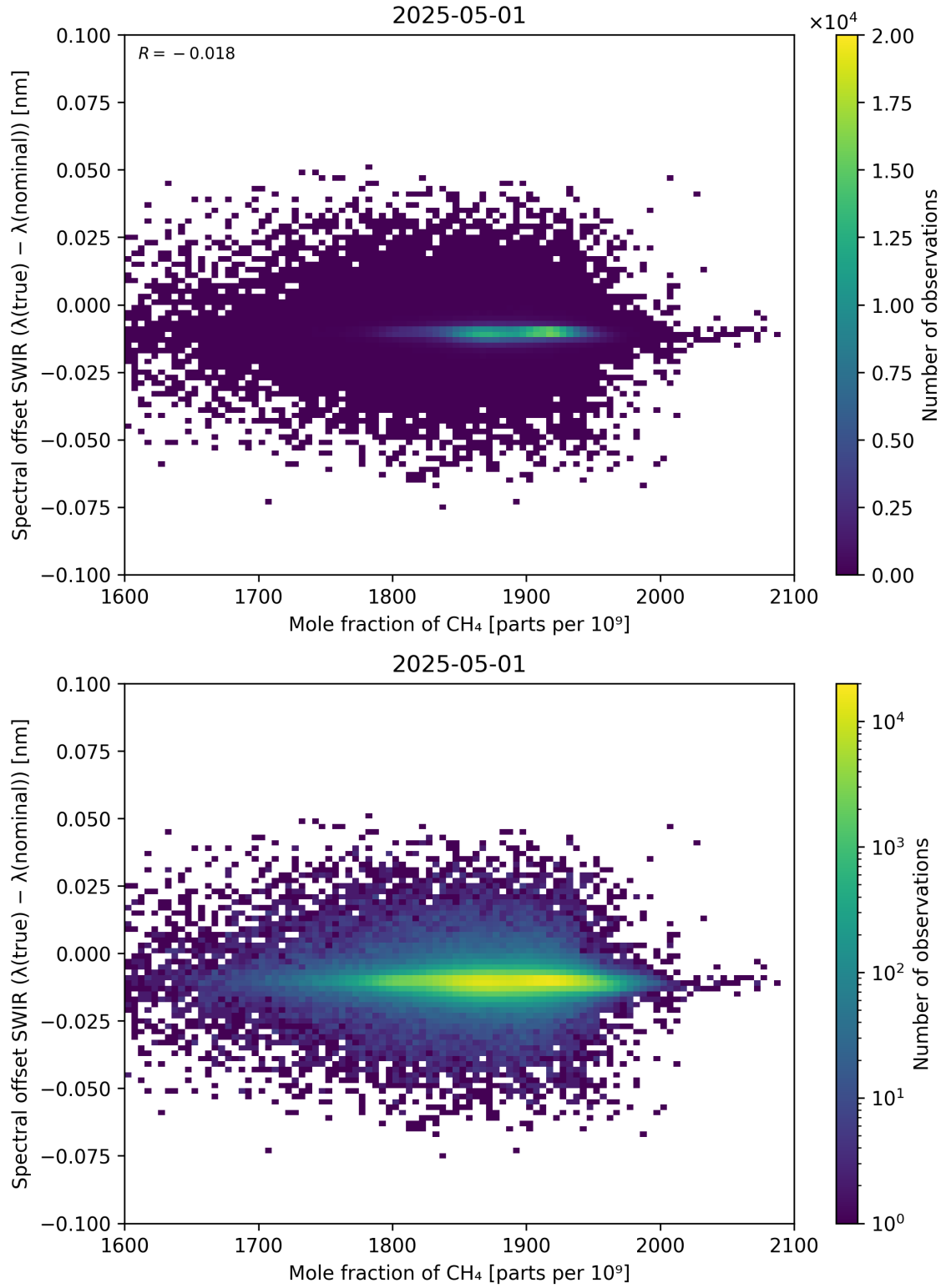
Figure 86: Scatter density plot of “Mole fraction of CH 4 ” against “Spectral offset SWIR ( \lambda_{\text{true}} - \lambda_{\text{nominal}} )” for 2025-04-30 to 2025-05-02.
