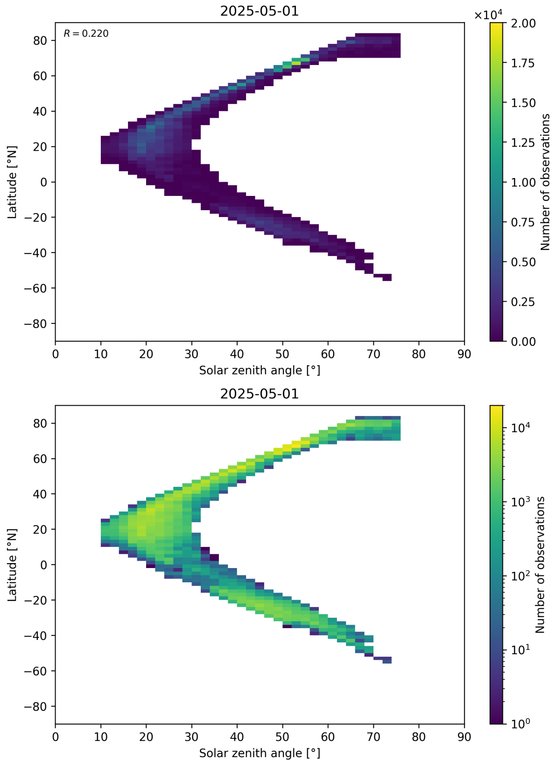
Figure 98: Scatter density plot of “Solar zenith angle” against “Latitude” for 2025-04-30 to 2025-05-02.
