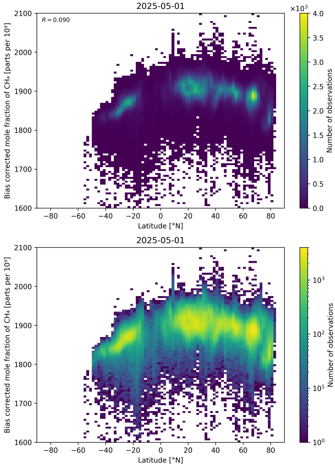
Figure 58: Scatter density plot of “Latitude” against “Bias corrected mole fraction of CH 4 ” for 2025-04-30 to 2025-05-02.
