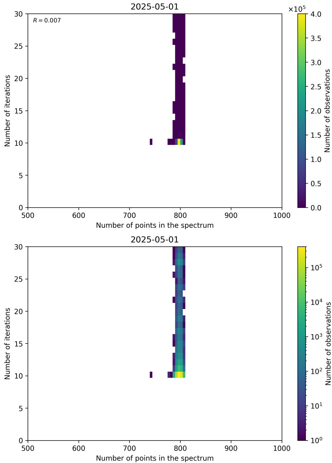
Figure 92: Scatter density plot of “Number of points in the spectrum” against “Number of iterations” for 2025-04-30 to 2025-05-02.
