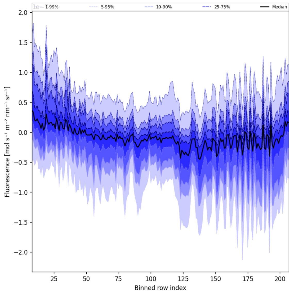
Figure 43: Along track statistics of “Fluorescence” for 2025-04-30 to 2025-05-02
