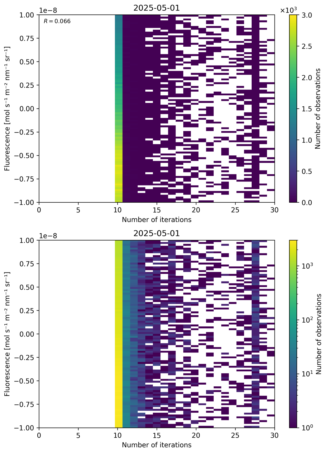
Figure 87: Scatter density plot of "Number of iterations" against "Fluorescence" for 2025-04-30 to 2025-05-02.
