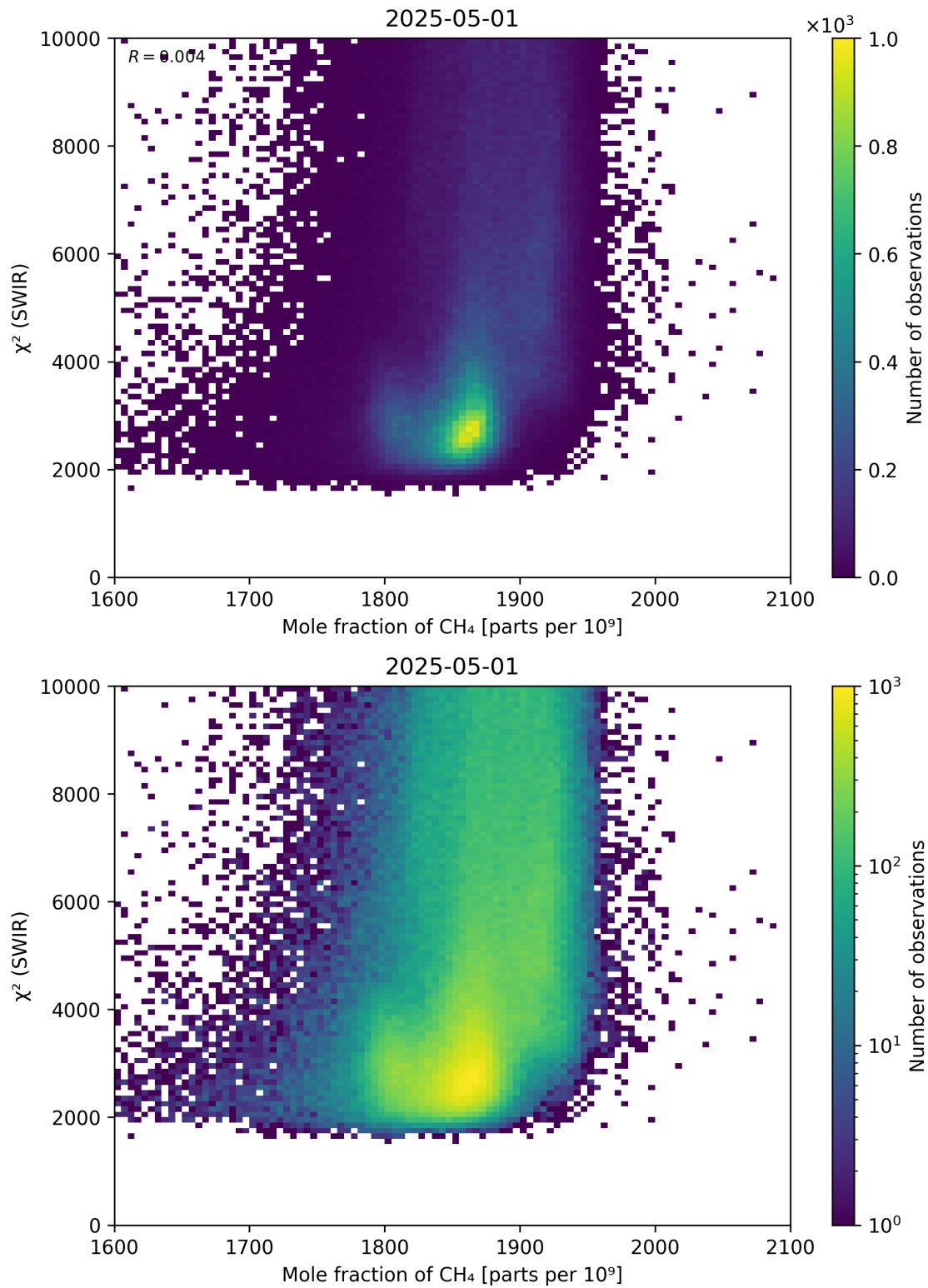
Figure 71: Scatter density plot of “Mole fraction of \text{CH}_4 ” against “ \chi^2 (SWIR)” for 2025-04-30 to 2025-05-02.
