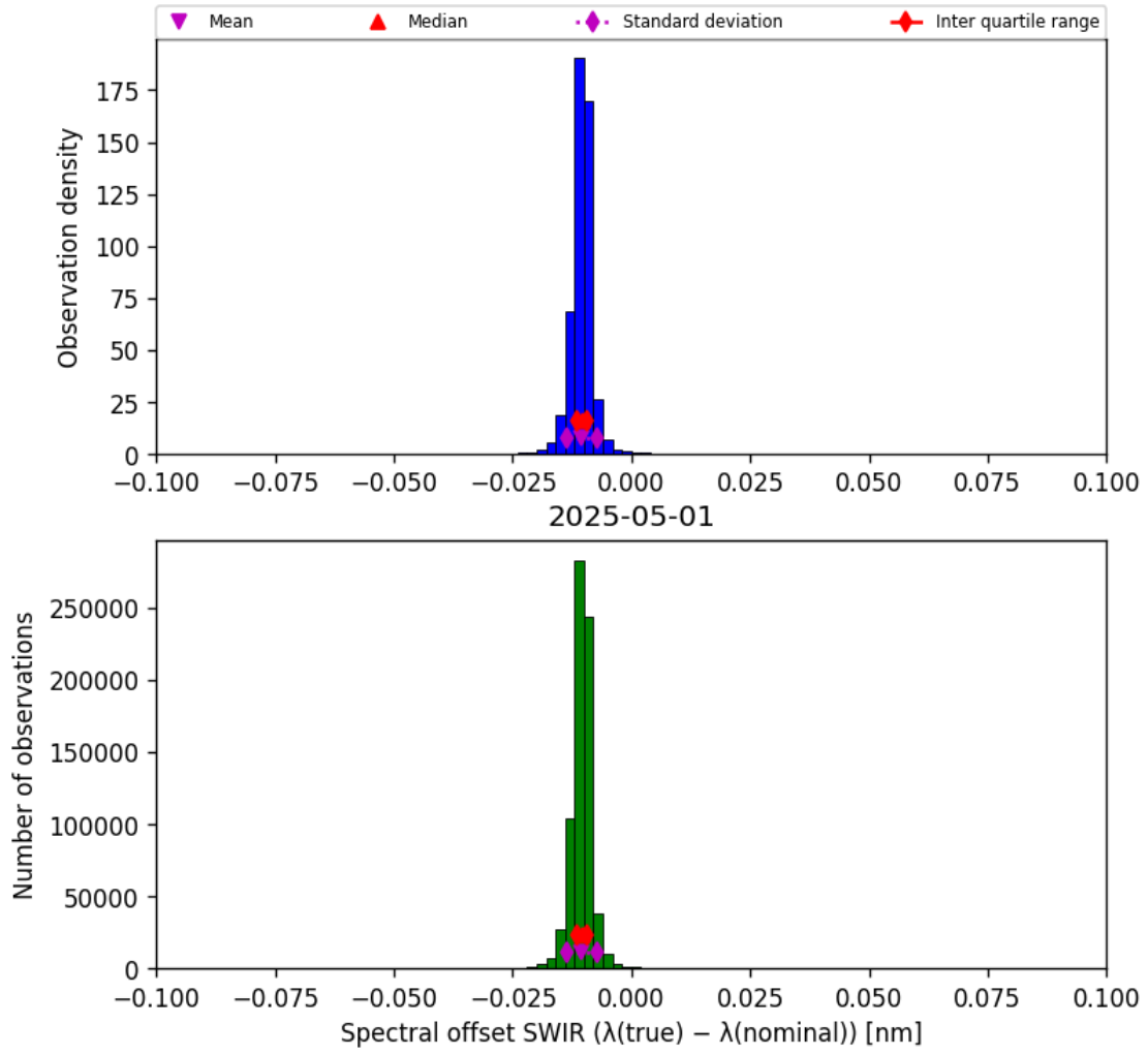
Figure 27: Histogram of “Spectral offset SWIR ( \lambda_{\text{true}} - \lambda_{\text{nominal}} )” for 2025-04-30 to 2025-05-02
