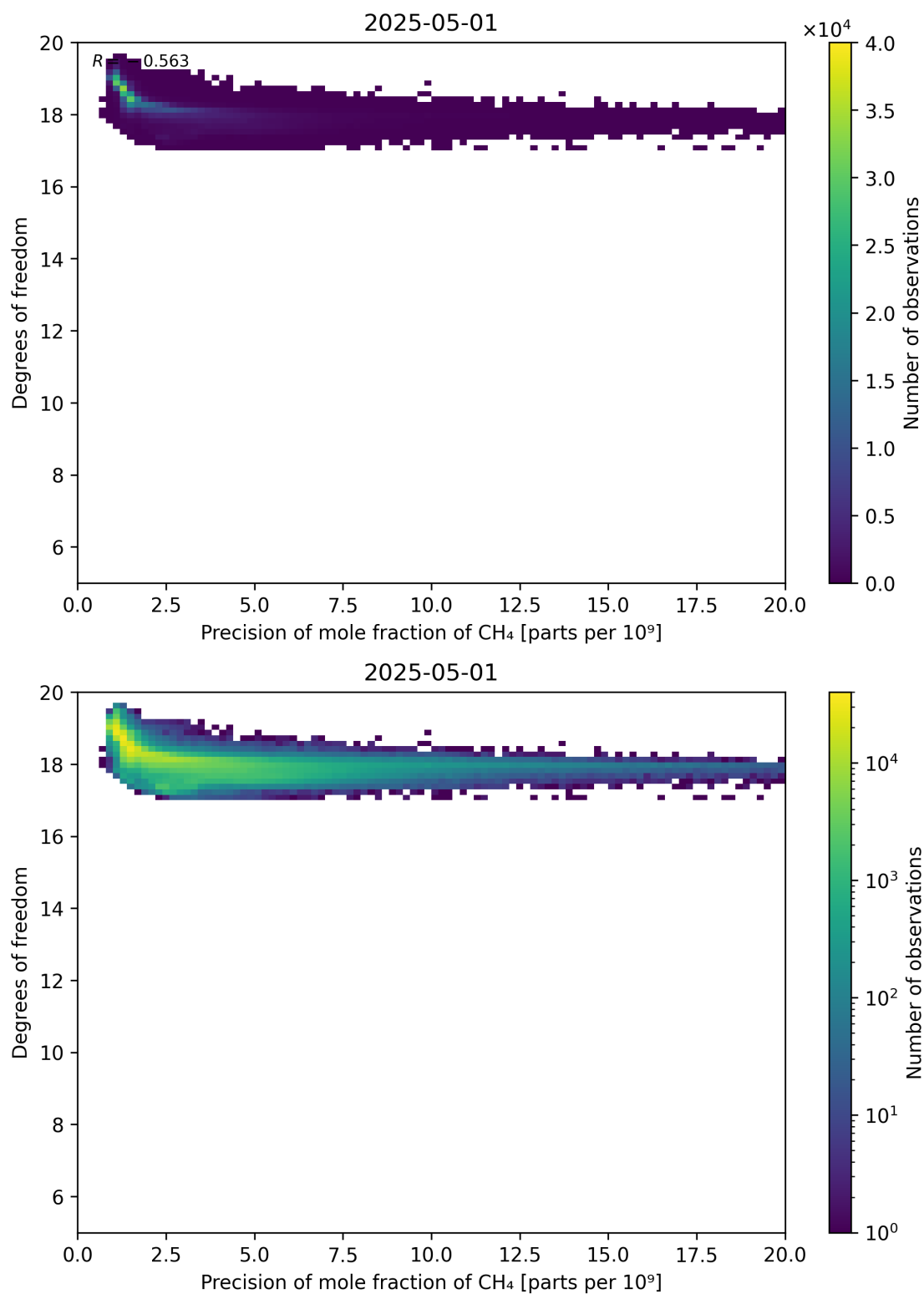
Figure 80: Scatter density plot of “Precision of mole fraction of CH 4 ” against “Degrees of freedom” for 2025-04-30 to 2025-05-02.
