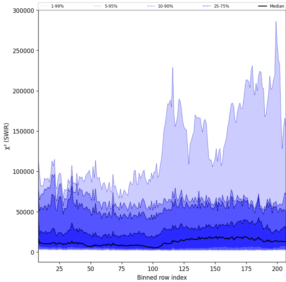
Figure 39: Along track statistics of “ \chi^2 (SWIR)” for 2025-04-30 to 2025-05-02
