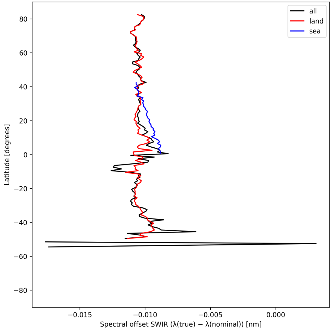
Figure 16: Zonal average of “Spectral offset SWIR ( \lambda_{\text{true}} - \lambda_{\text{nominal}} )” for 2025-04-30 to 2025-05-02.
