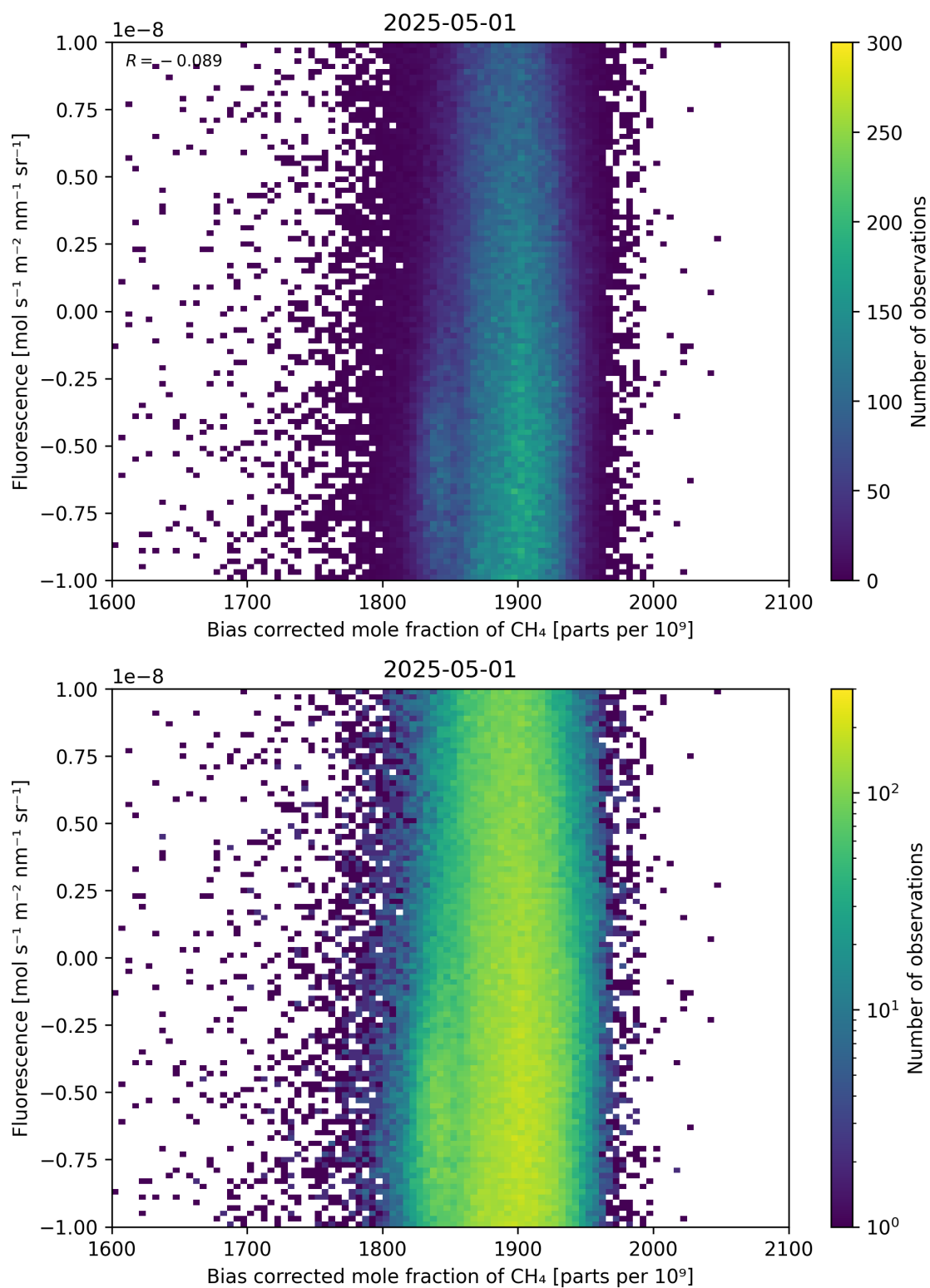
Figure 66: Scatter density plot of “Bias corrected mole fraction of \text{CH}_4 ” against “Fluorescence” for 2025-04-30 to 2025-05-02.
