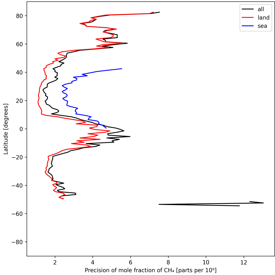
Figure 13: Zonal average of “Precision of mole fraction of CH 4 ” for 2025-04-30 to 2025-05-02.
