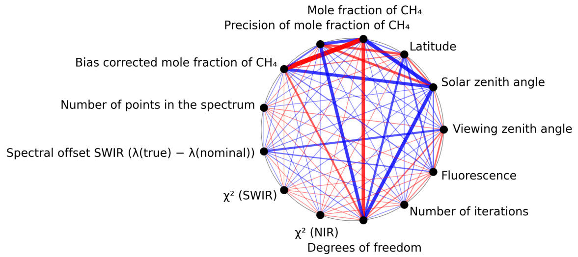
Figure 1: Map of correlation graph for 2025-04-30 to 2025-05-02.
