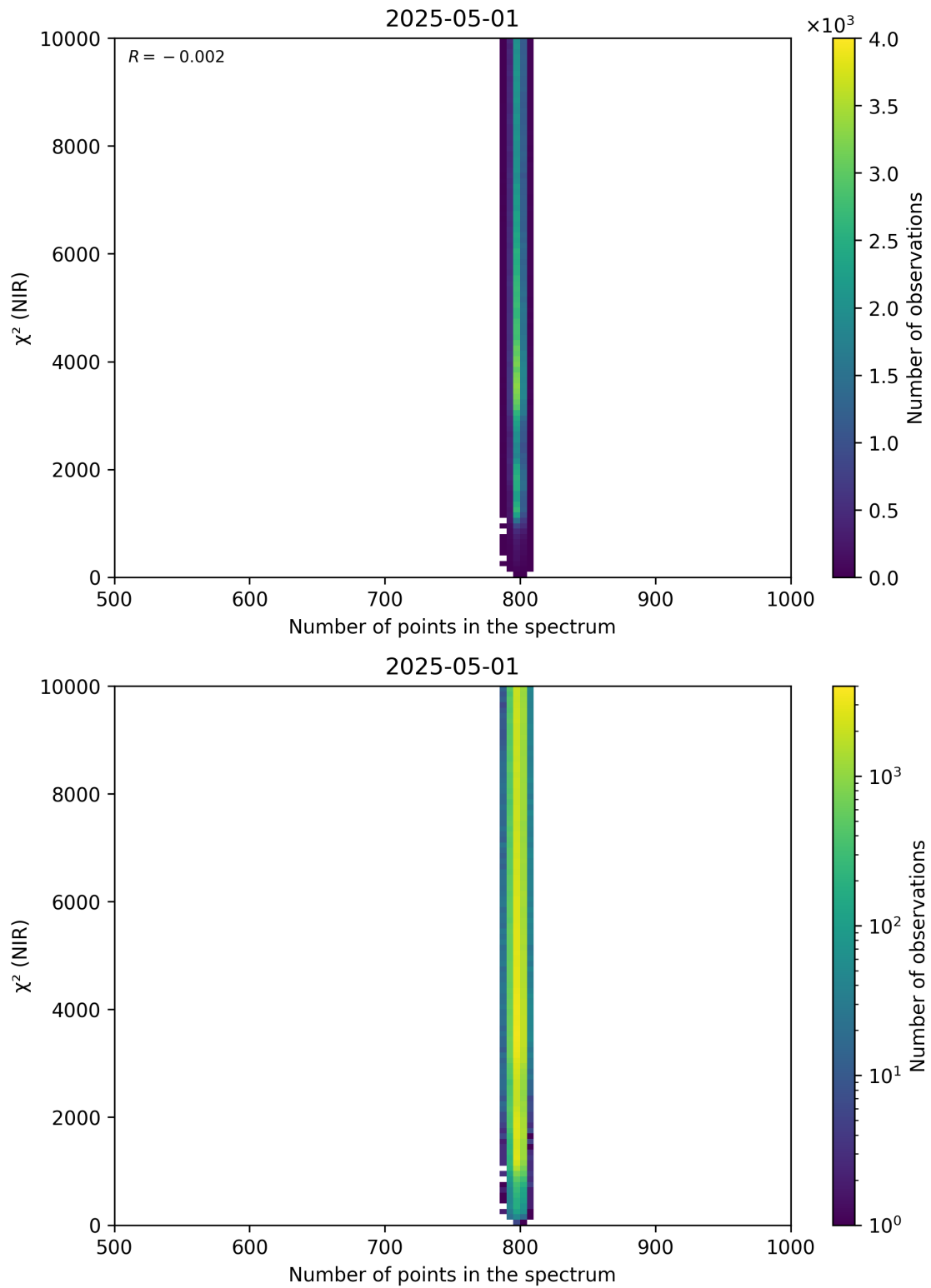
Figure 88: Scatter density plot of “Number of points in the spectrum” against “ \chi^2 (NIR)” for 2025-04-30 to 2025-05-02.
