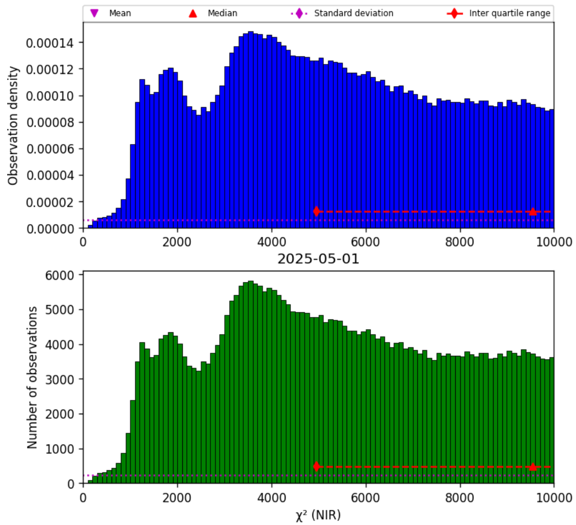
Figure 29: Histogram of " \chi^2 (NIR)" for 2025-04-30 to 2025-05-02
