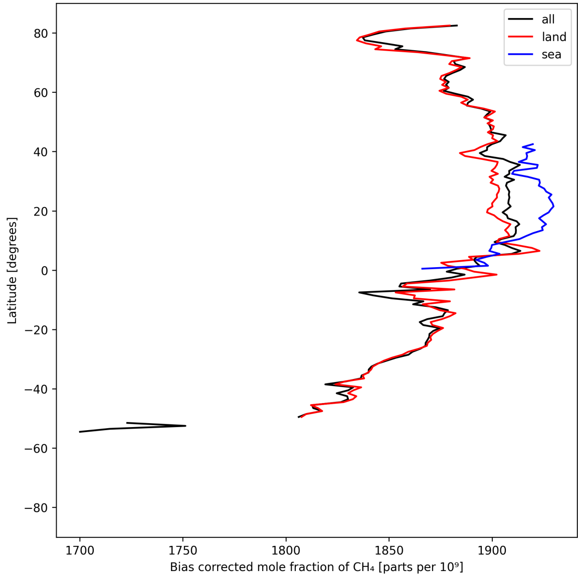
Figure 14: Zonal average of “Bias corrected mole fraction of CH 4 ” for 2025-04-30 to 2025-05-02.
