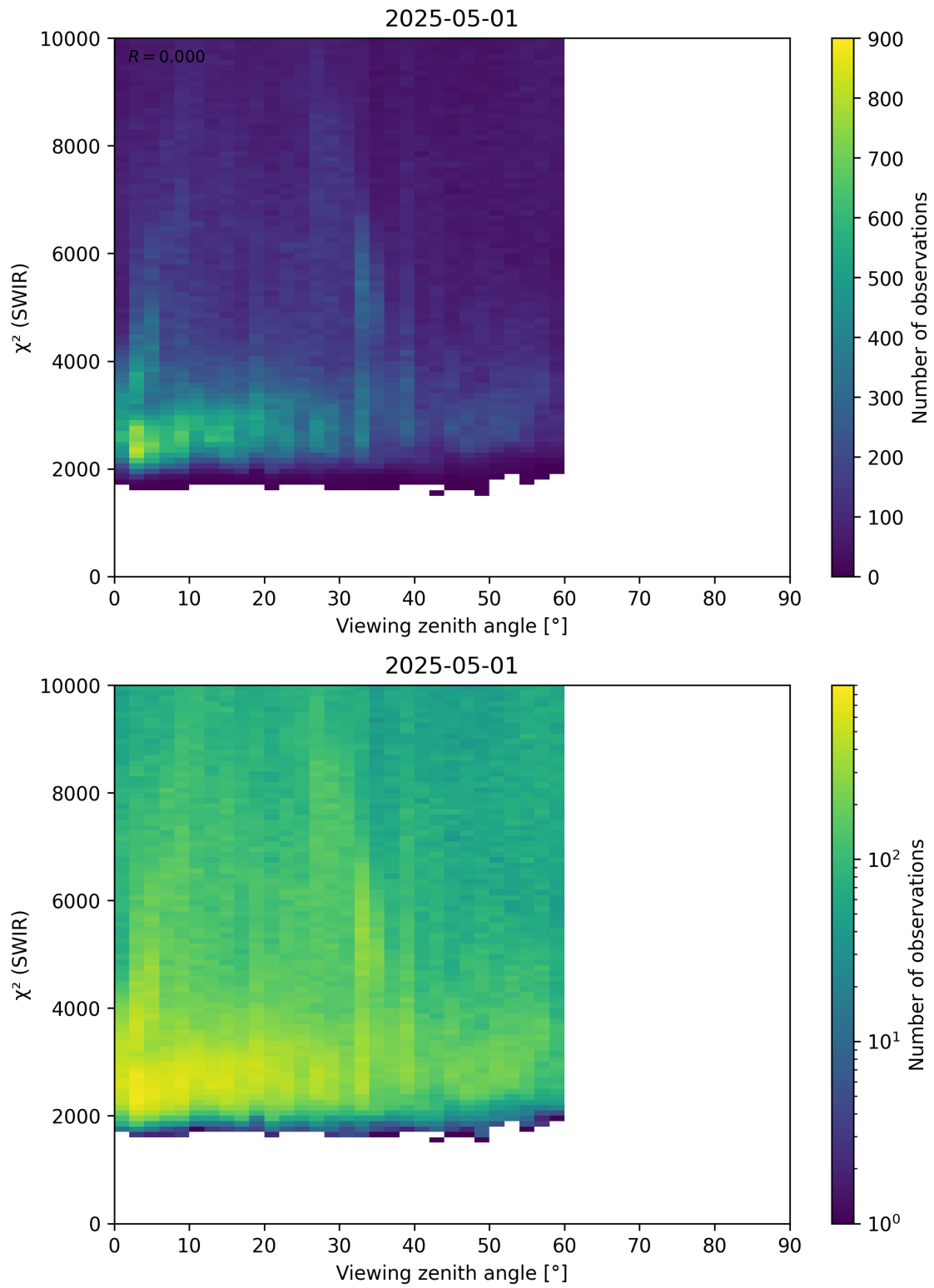
Figure 106: Scatter density plot of “Viewing zenith angle” against “ \chi^2 (SWIR)” for 2025-04-30 to 2025-05-02.
