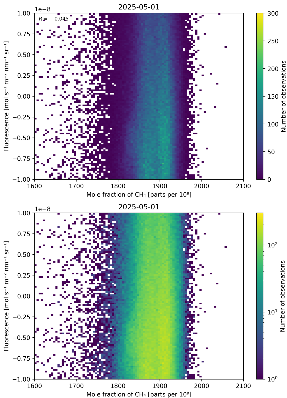
Figure 73: Scatter density plot of “Mole fraction of \text{CH}_4 ” against “Fluorescence” for 2025-04-30 to 2025-05-02.
