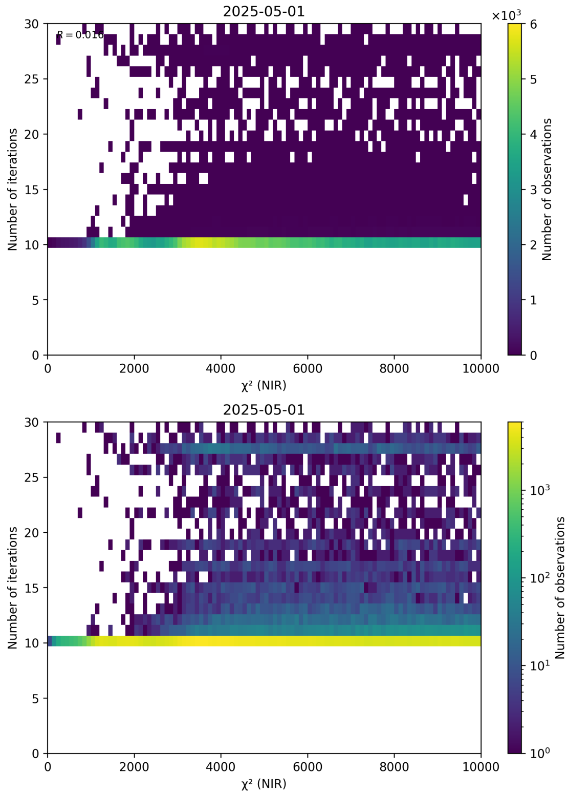
Figure 46: Scatter density plot of “ \chi^2 (NIR)” against “Number of iterations” for 2025-04-30 to 2025-05-02.
