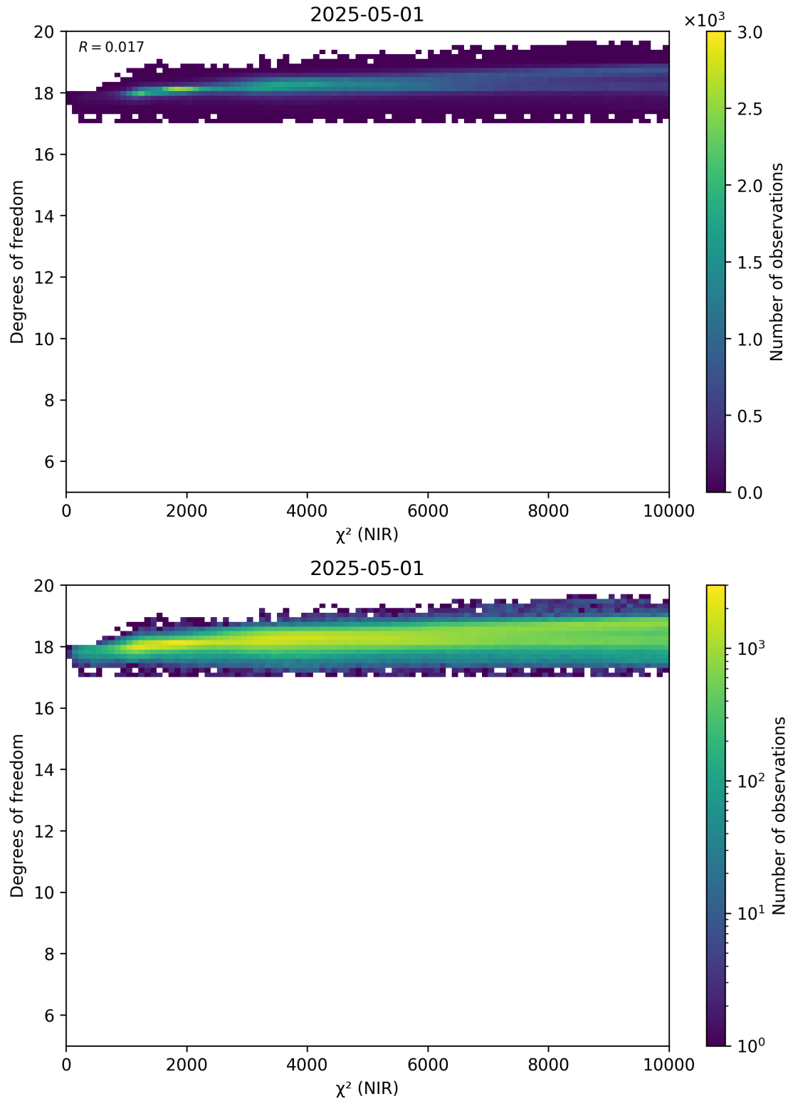
Figure 44: Scatter density plot of “ \chi^2 (NIR)” against “Degrees of freedom” for 2025-04-30 to 2025-05-02.
