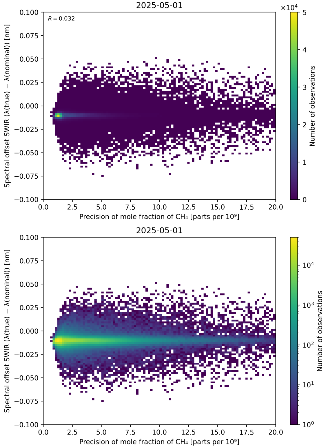
Figure 85: Scatter density plot of “Precision of mole fraction of CH 4 ” against “Spectral offset SWIR ( \lambda_{\text{true}} - \lambda_{\text{nominal}} )” for 2025-04-30 to 2025-05-02.
