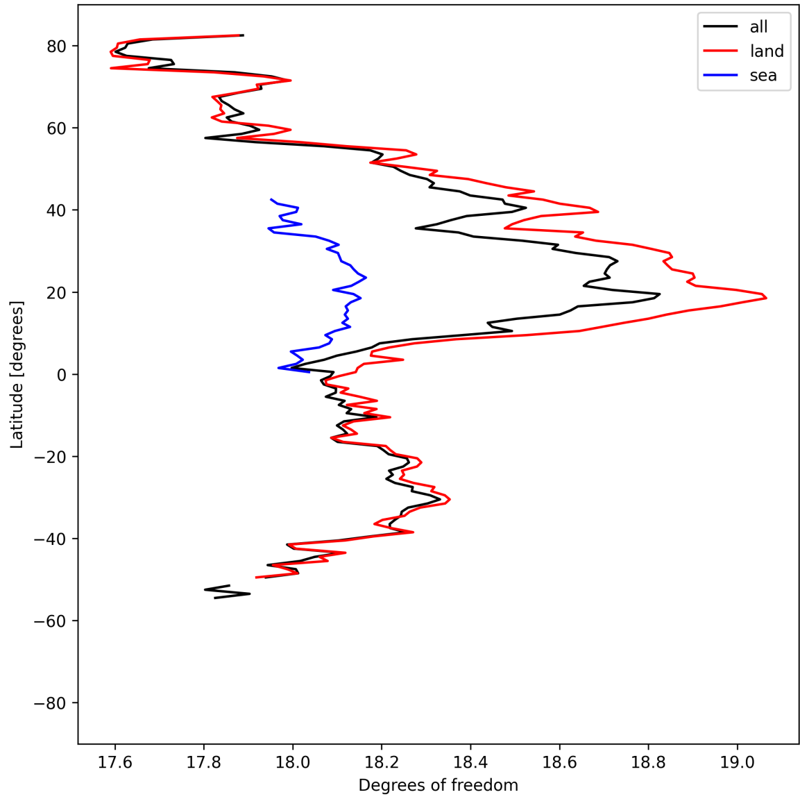
Figure 19: Zonal average of “Degrees of freedom” for 2025-04-30 to 2025-05-02.
