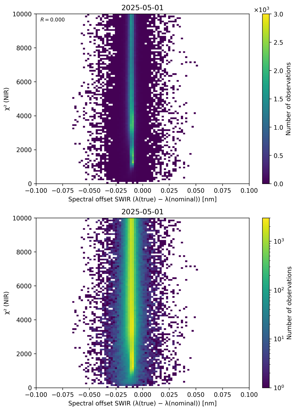
Figure 117: Scatter density plot of “Spectral offset SWIR ( \lambda_{\text{true}} - \lambda_{\text{nominal}} )” against “ \chi^2 (NIR)” for 2025-04-30 to 2025-05-02.
