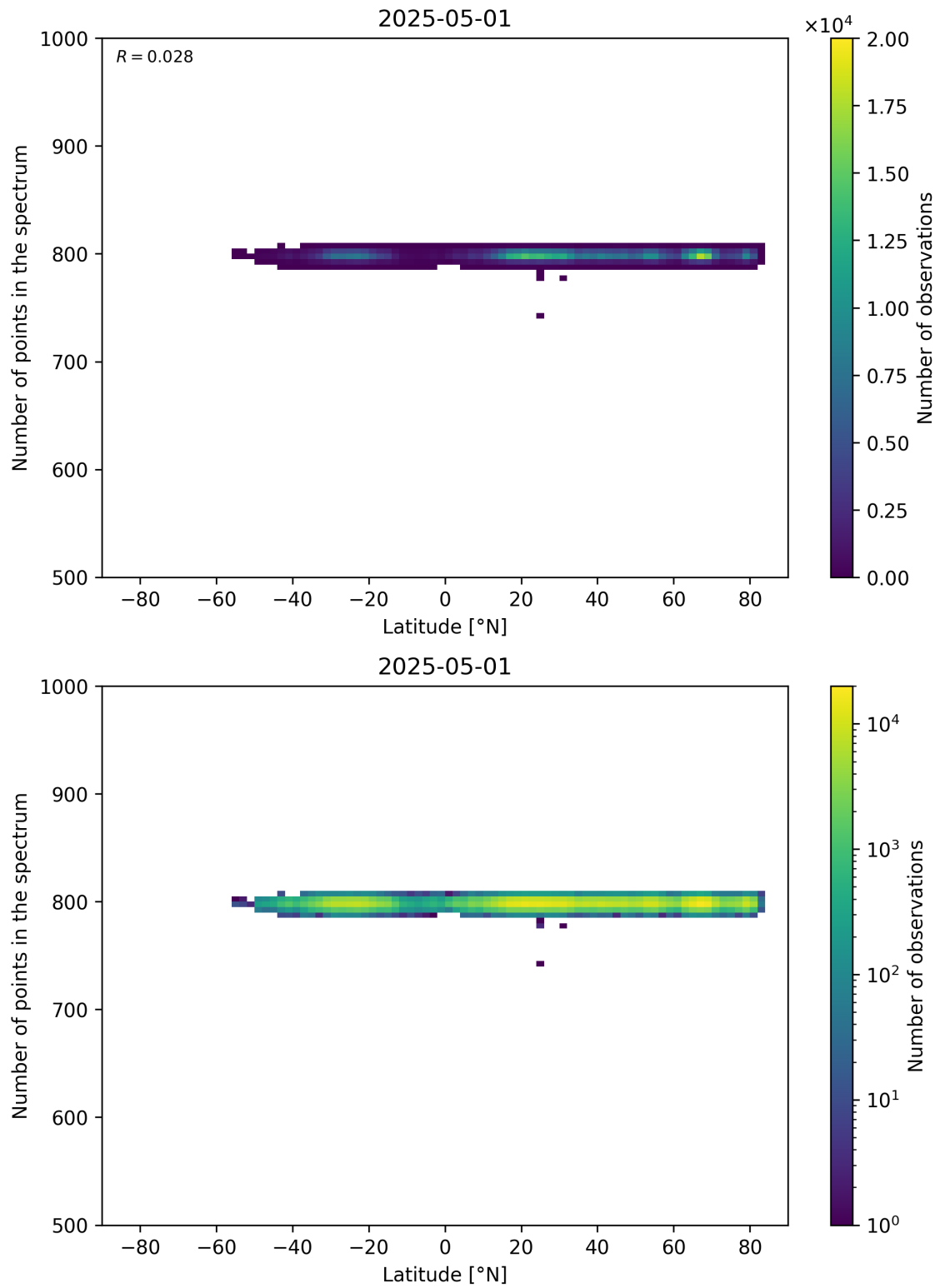
Figure 61: Scatter density plot of “Latitude” against “Number of points in the spectrum” for 2025-04-30 to 2025-05-02.
