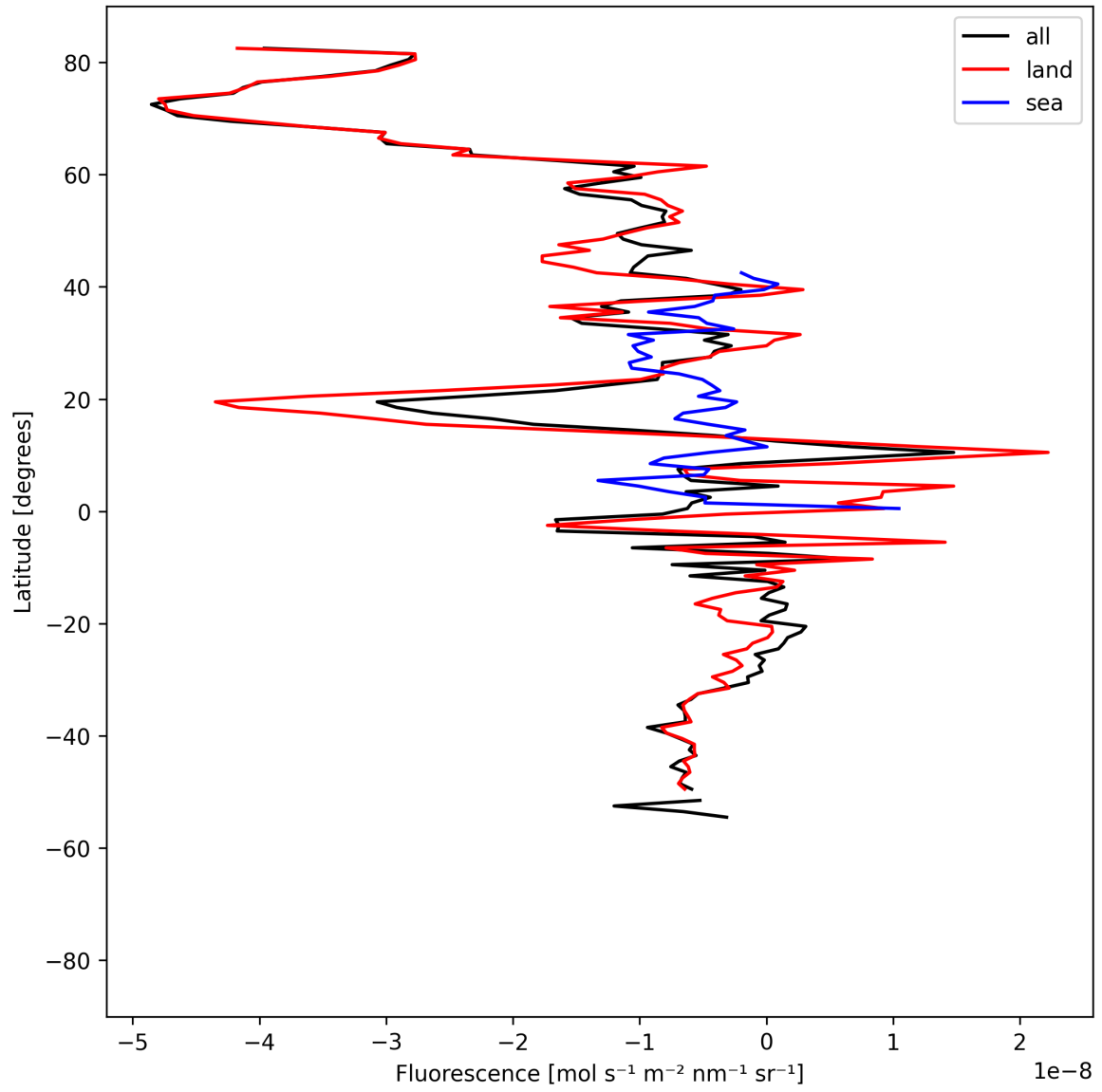
Figure 21: Zonal average of “Fluorescence” for 2025-04-30 to 2025-05-02.
