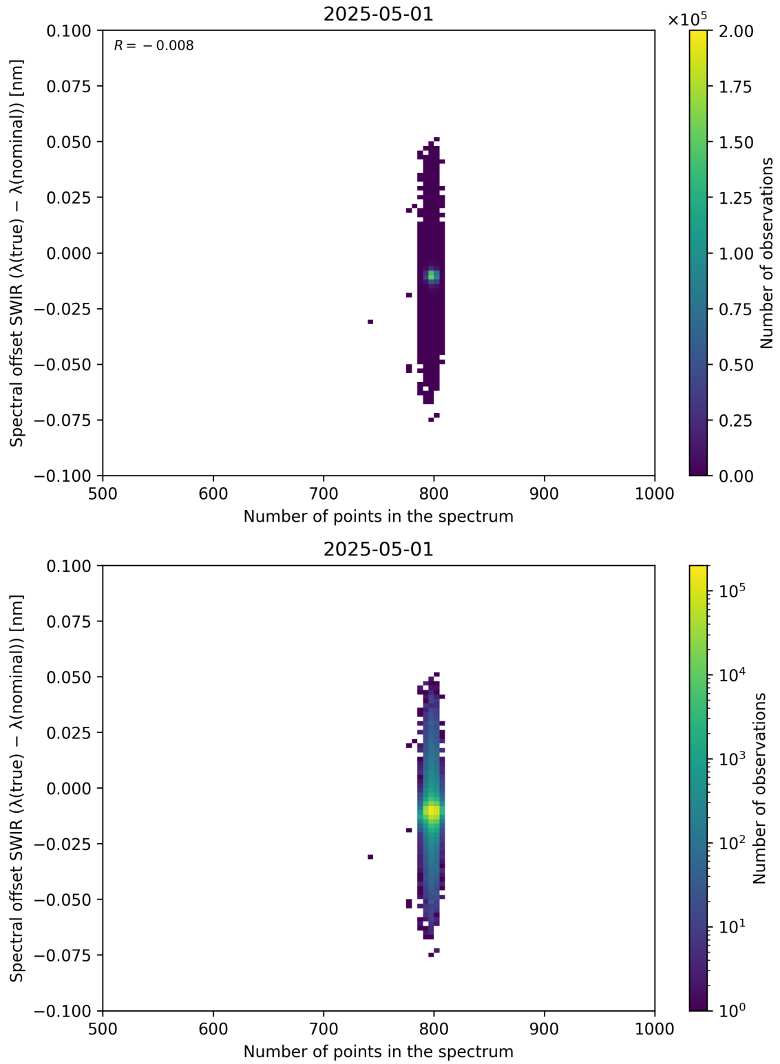
Figure 93: Scatter density plot of “Number of points in the spectrum” against “Spectral offset SWIR ( \lambda_{\text{true}} - \lambda_{\text{nominal}} )” for 2025-04-30 to 2025-05-02.
