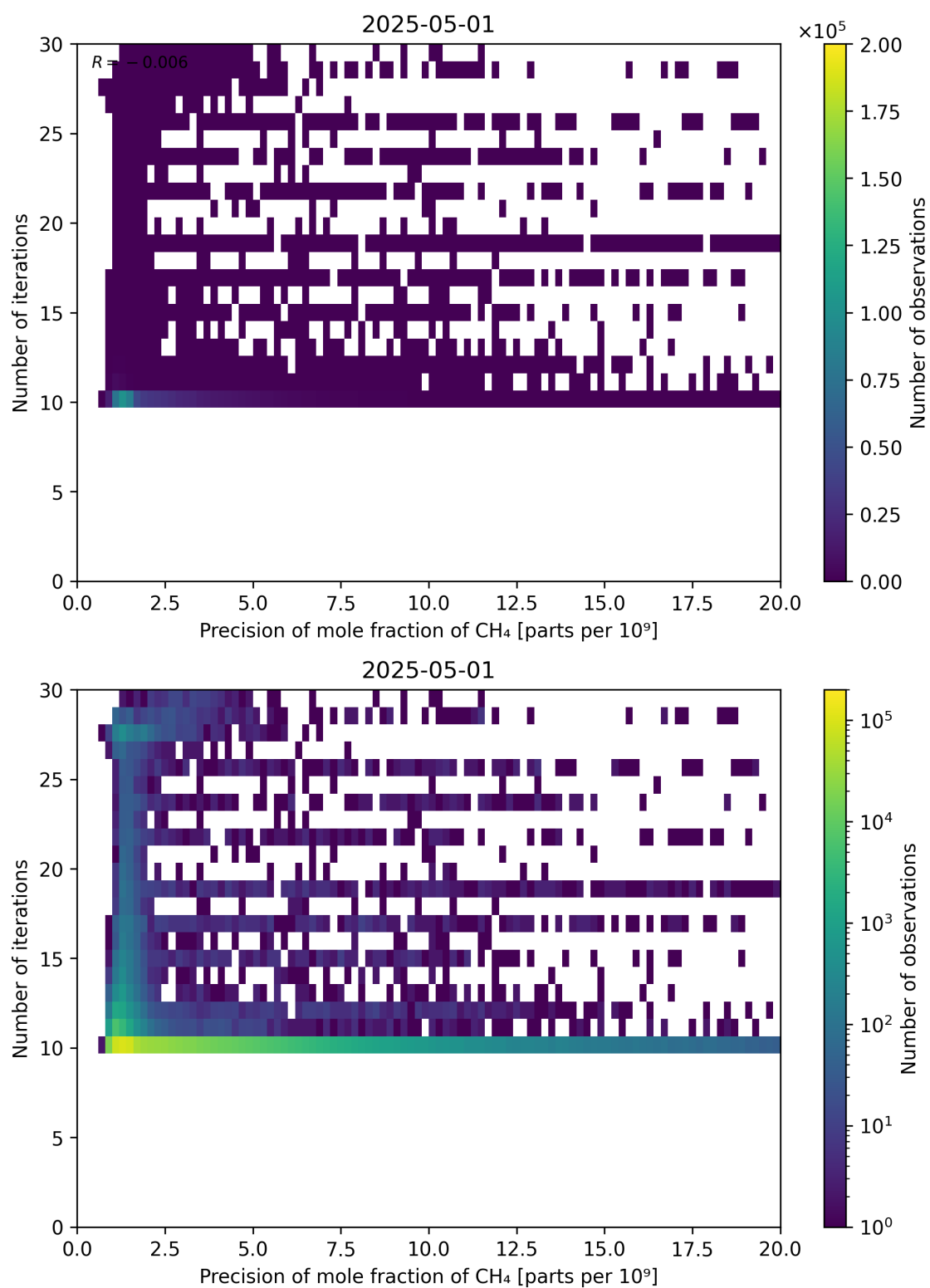
Figure 83: Scatter density plot of “Precision of mole fraction of CH 4 ” against “Number of iterations” for 2025-04-30 to 2025-05-02.
