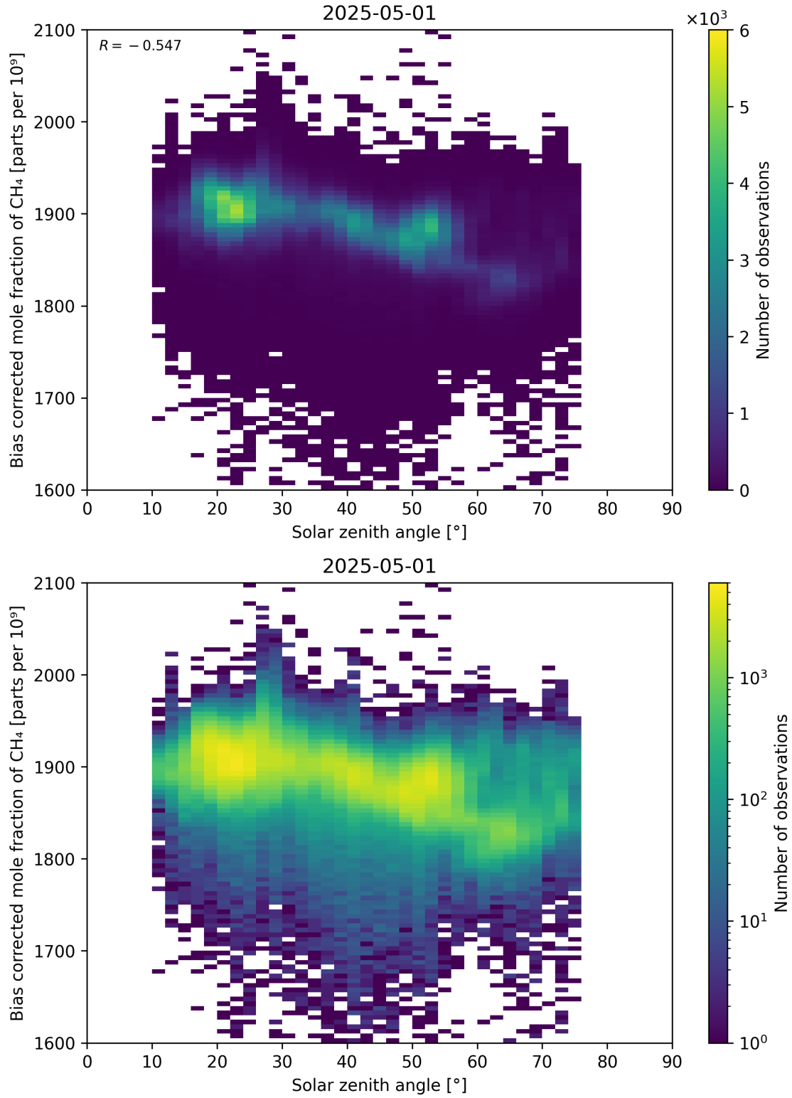
Figure 100: Scatter density plot of “Solar zenith angle” against “Bias corrected mole fraction of CH 4 ” for 2025-04-30 to 2025-05-02.
