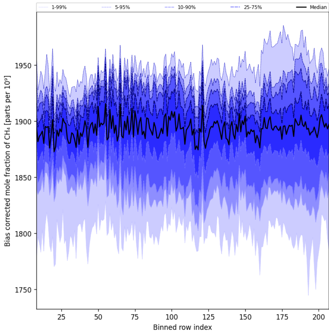
Figure 36: Along track statistics of “Bias corrected mole fraction of CH 4 ” for 2025-04-30 to 2025-05-02
