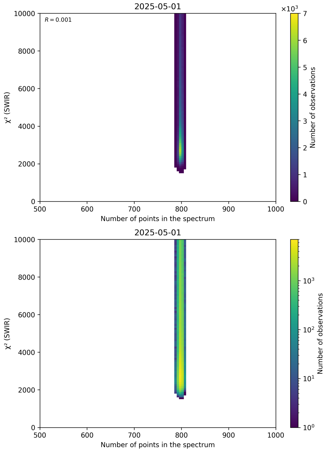
Figure 89: Scatter density plot of “Number of points in the spectrum” against “ \chi^2 (SWIR)” for 2025-04-30 to 2025-05-02.
