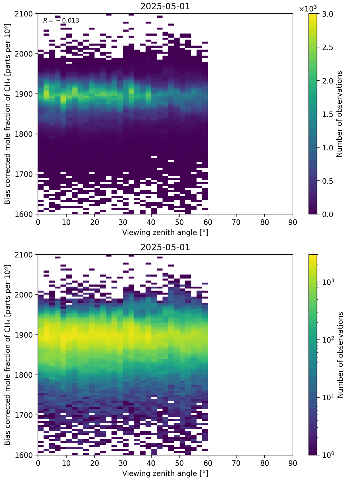
Figure 111: Scatter density plot of “Viewing zenith angle” against “Bias corrected mole fraction of CH 4 ” for 2025-04-30 to 2025-05-02.
