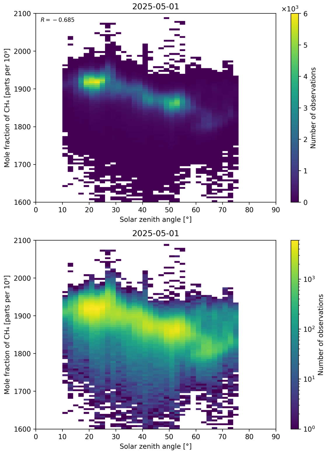
Figure 99: Scatter density plot of “Solar zenith angle” against “Mole fraction of CH 4 ” for 2025-04-30 to 2025-05-02.
