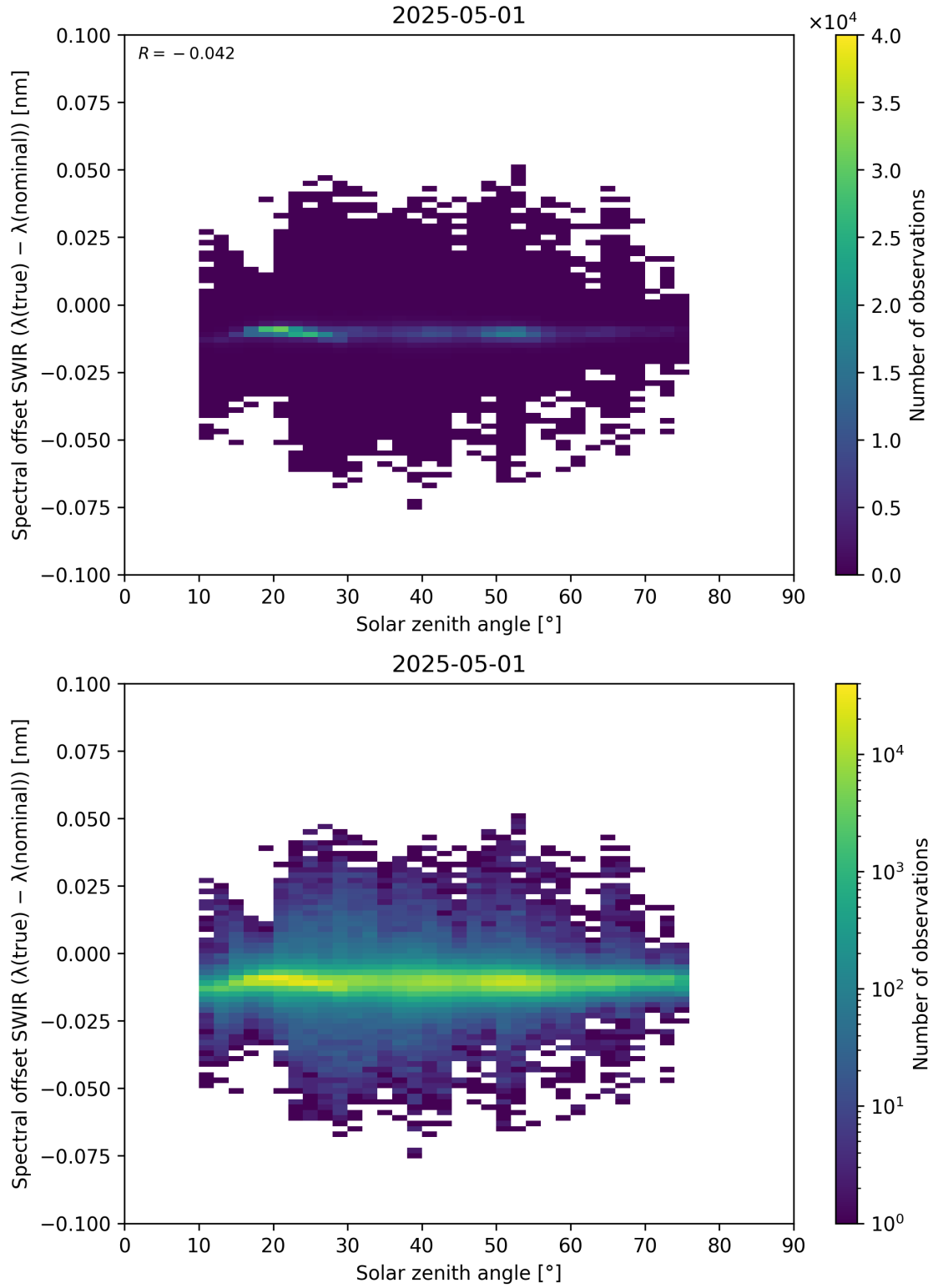
Figure 104: Scatter density plot of “Solar zenith angle” against “Spectral offset SWIR ( \lambda_{\text{true}} - \lambda_{\text{nominal}} )” for 2025-04-30 to 2025-05-02.
