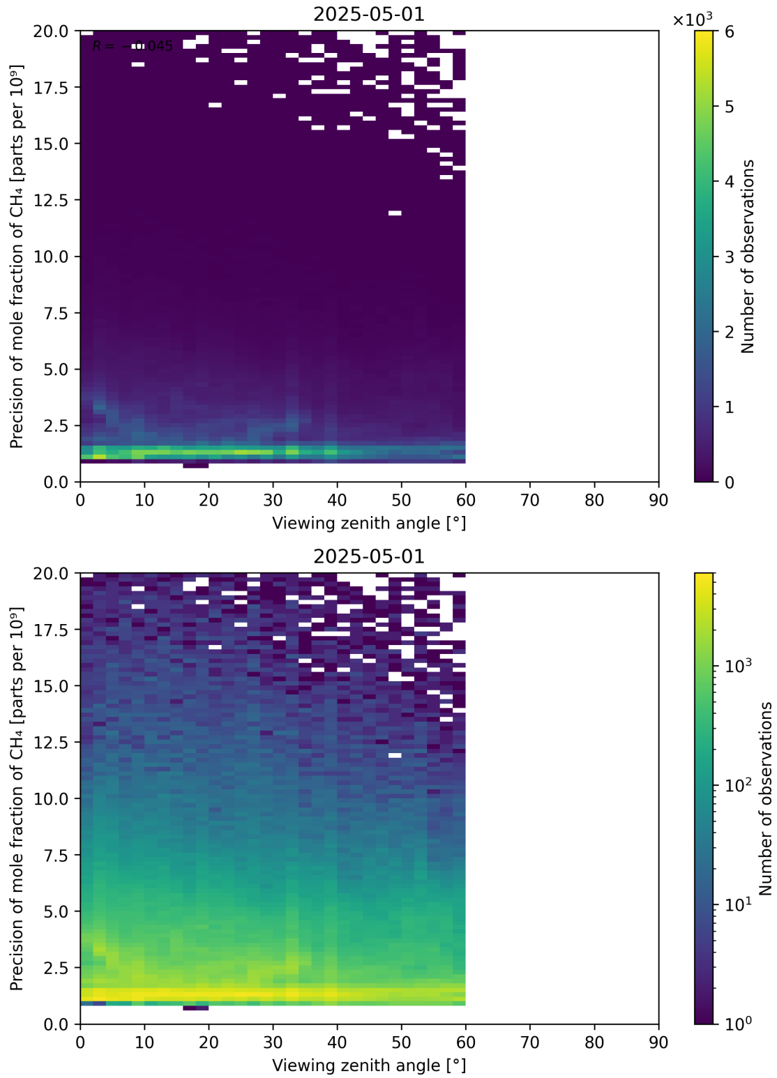
Figure 112: Scatter density plot of “Viewing zenith angle” against “Precision of mole fraction of CH 4 ” for 2025-04-30 to 2025-05-02.
