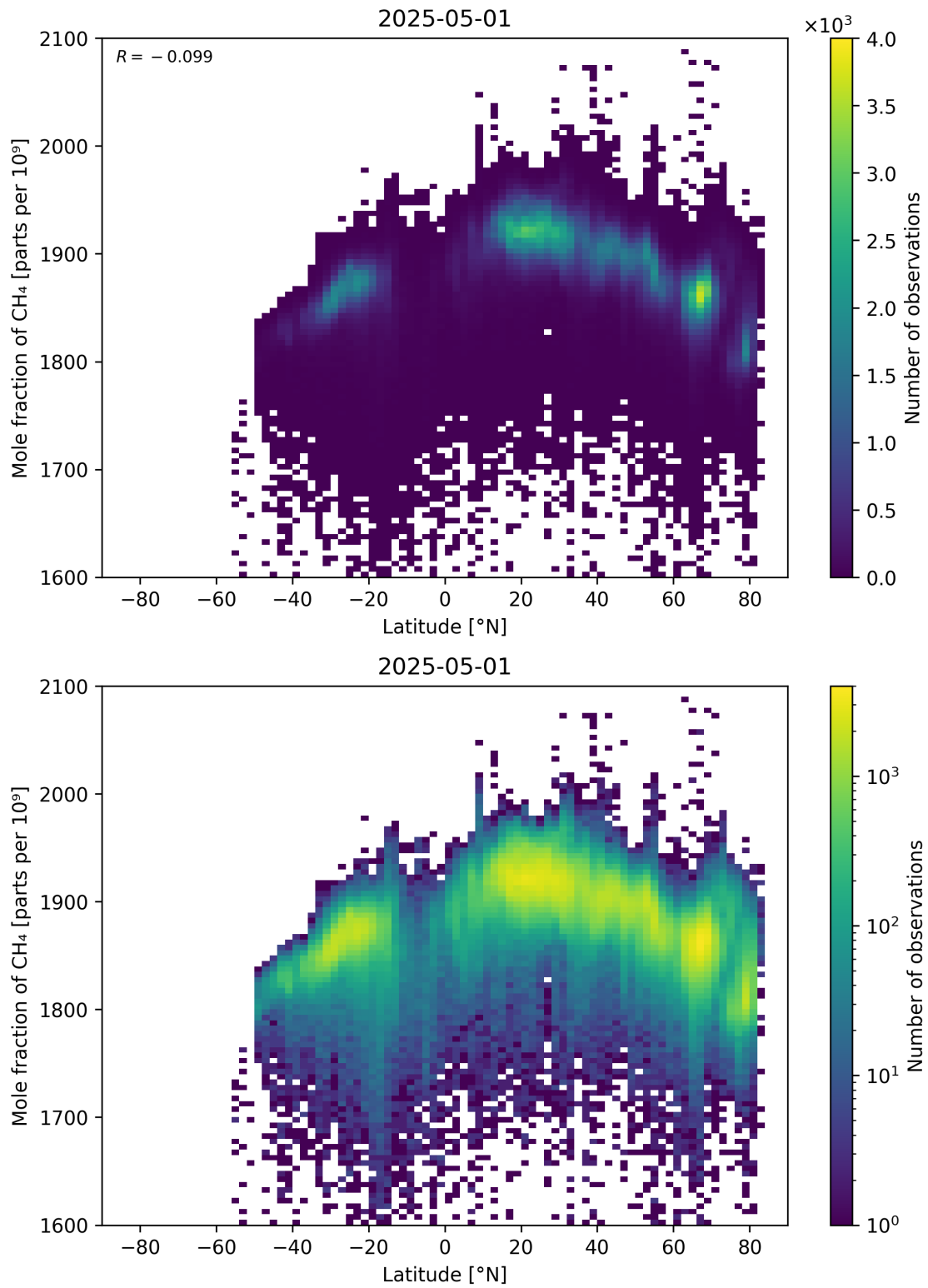
Figure 57: Scatter density plot of “Latitude” against “Mole fraction of CH 4 ” for 2025-04-30 to 2025-05-02.
