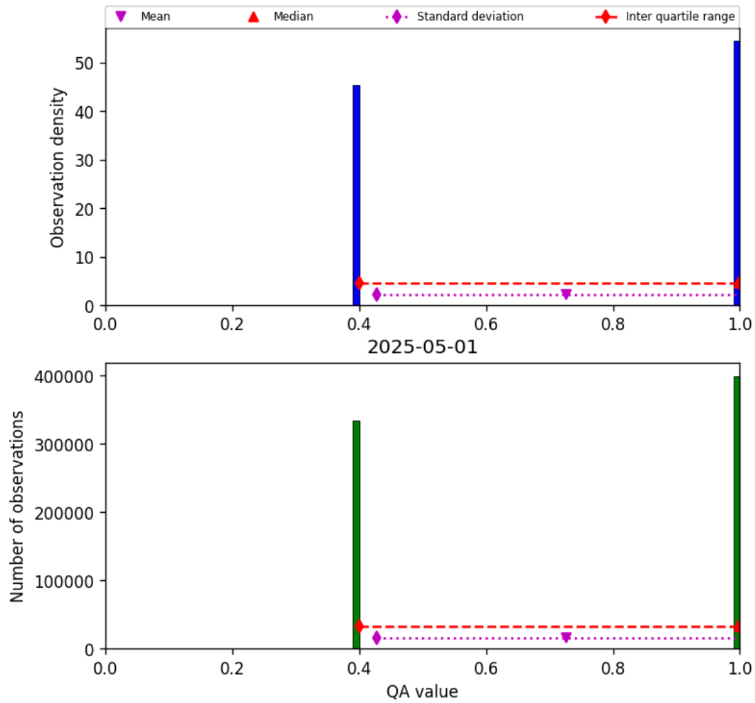
Figure 22: Histogram of “QA value” for 2025-04-30 to 2025-05-02
