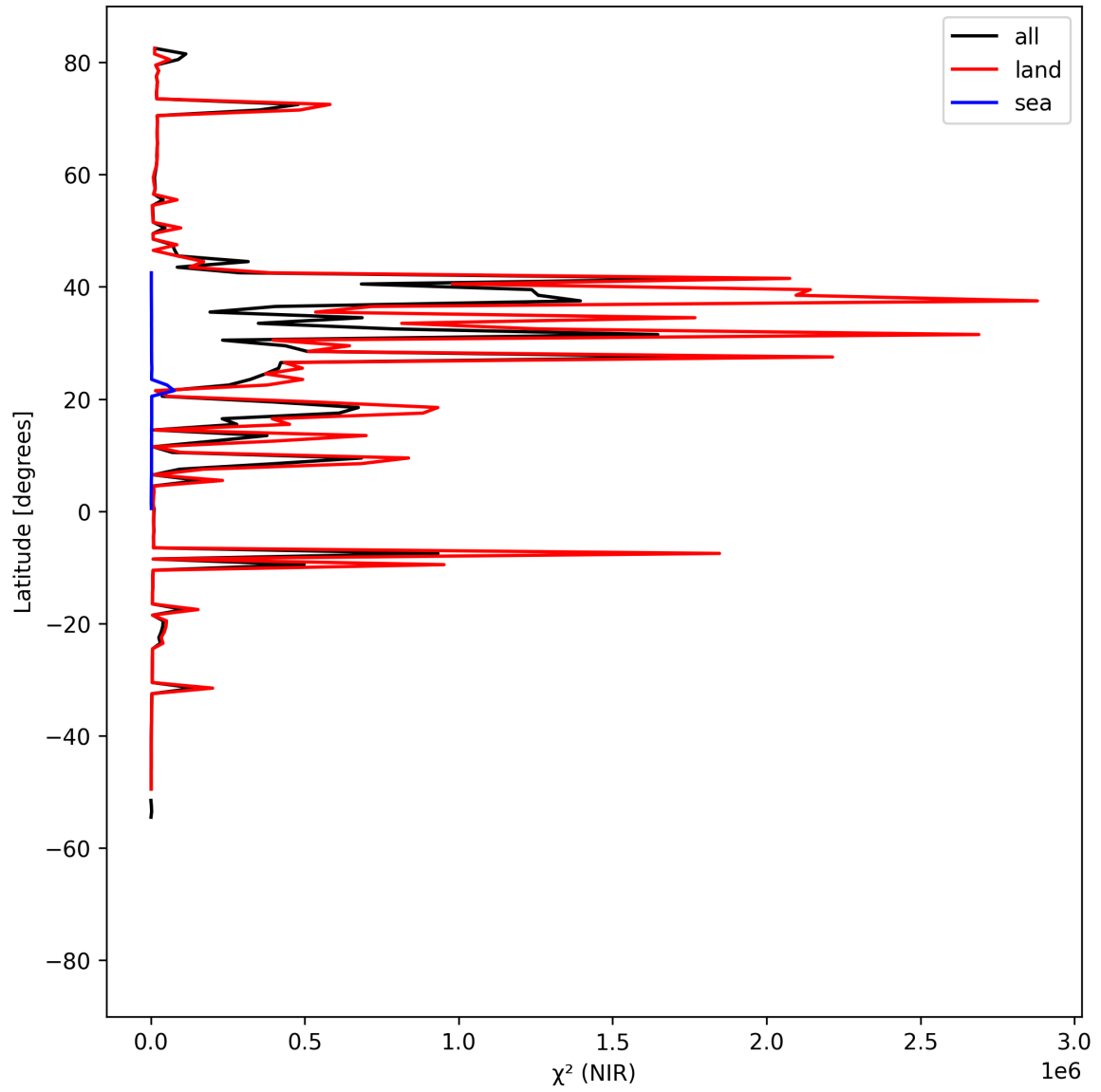
Figure 18: Zonal average of “ \chi^2 (NIR)” for 2025-04-30 to 2025-05-02.
