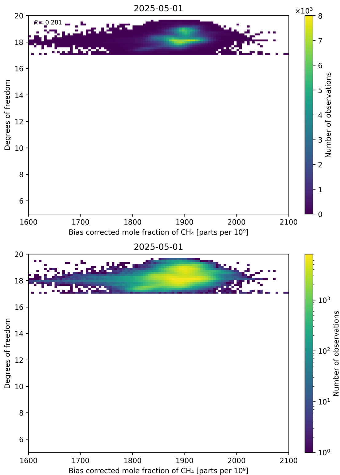
Figure 65: Scatter density plot of “Bias corrected mole fraction of CH 4 ” against “Degrees of freedom” for 2025-04-30 to 2025-05-02.
