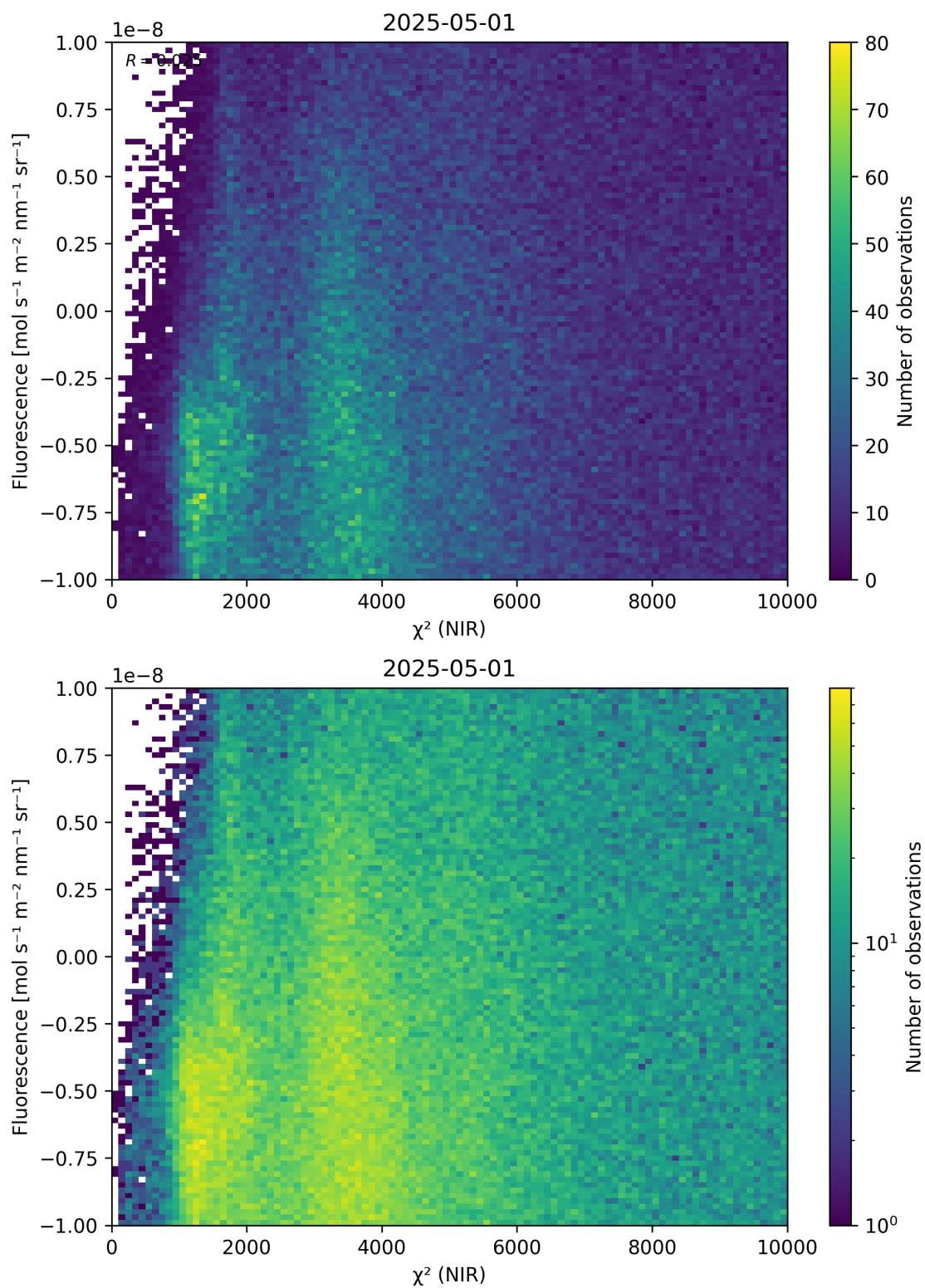
Figure 45: Scatter density plot of “ \chi^2 (NIR)” against “Fluorescence” for 2025-04-30 to 2025-05-02.
