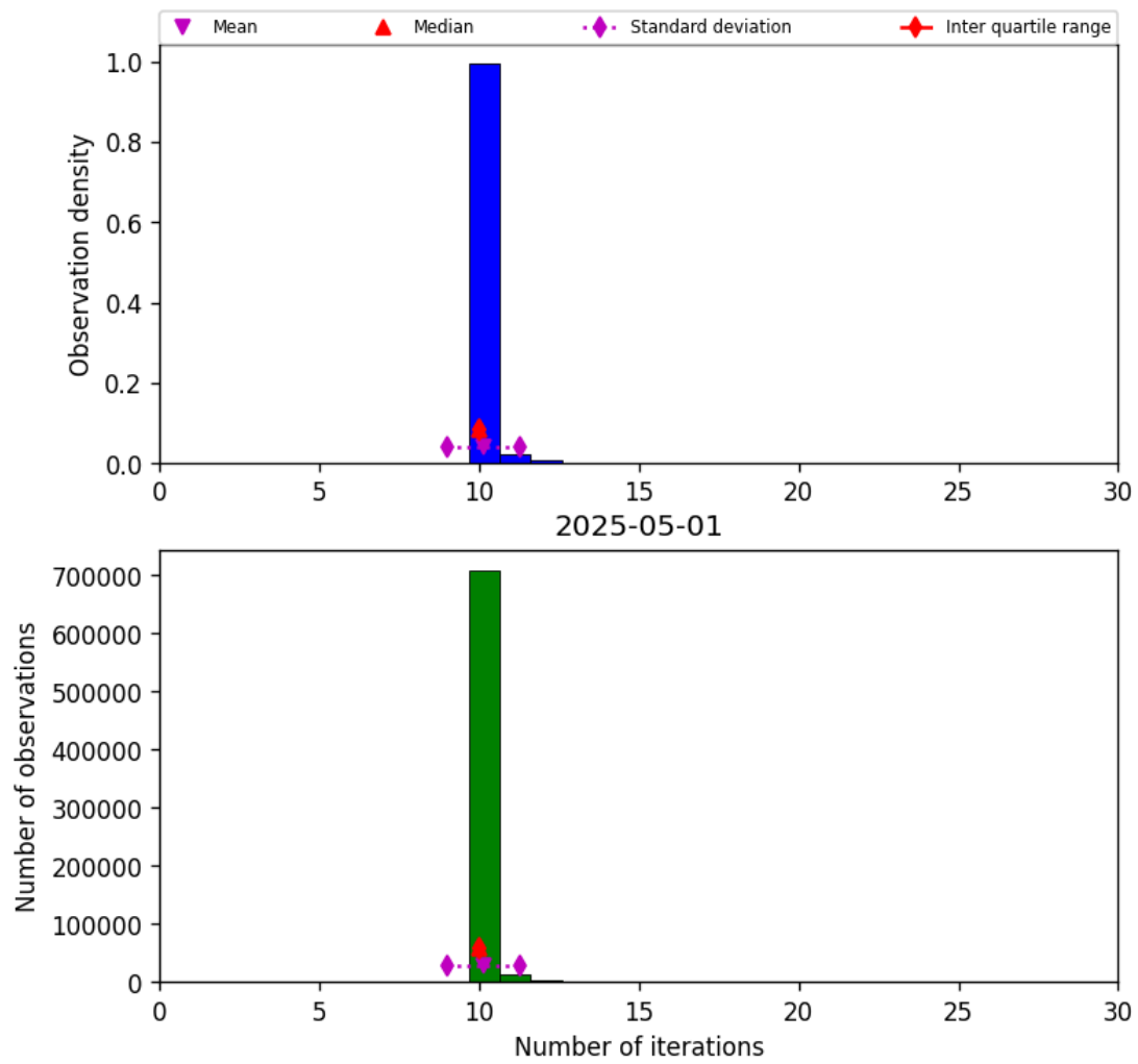
Figure 31: Histogram of “Number of iterations” for 2025-04-30 to 2025-05-02
