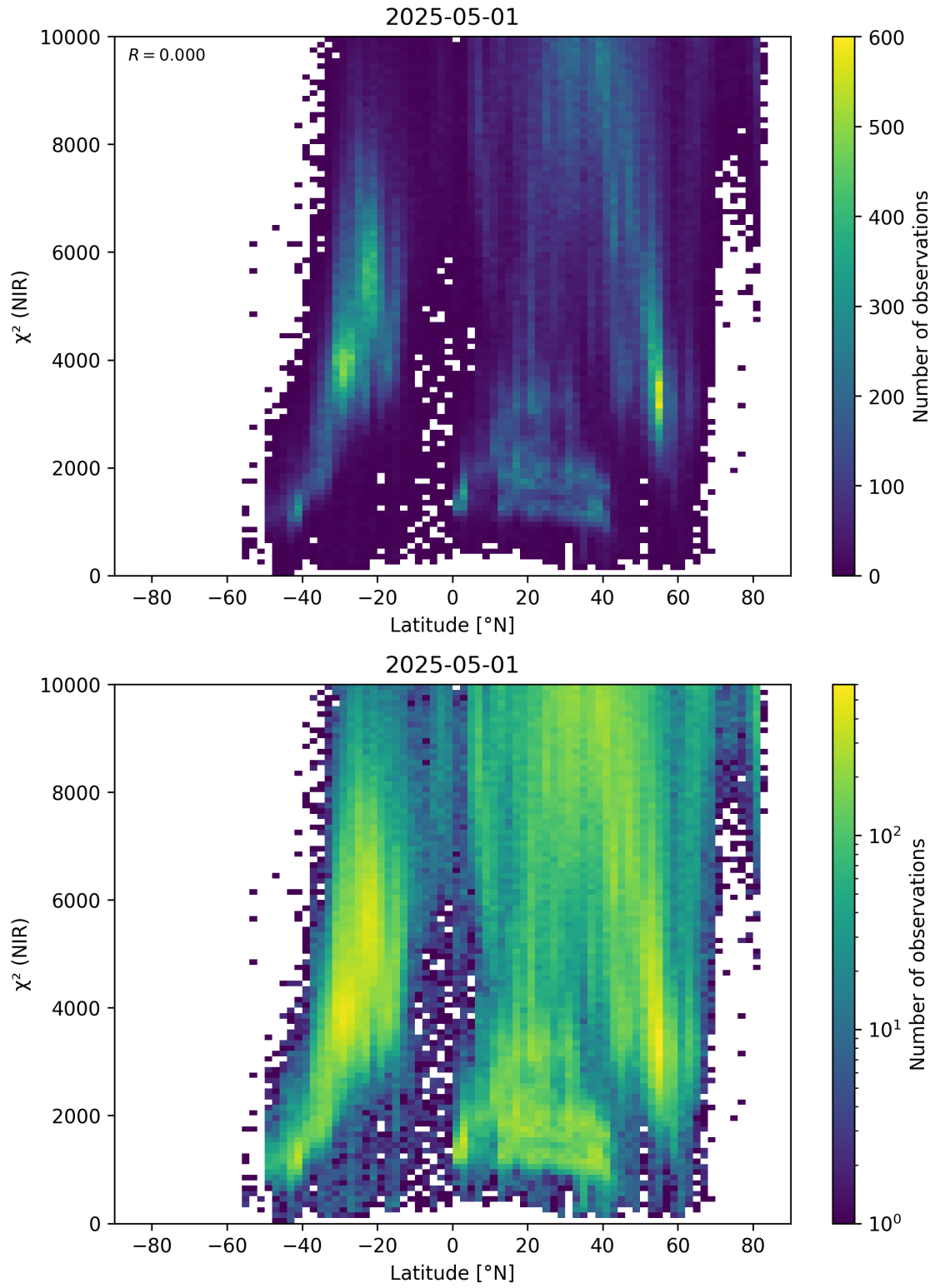
Figure 53: Scatter density plot of “Latitude” against “ \chi^2 (NIR)” for 2025-04-30 to 2025-05-02.
