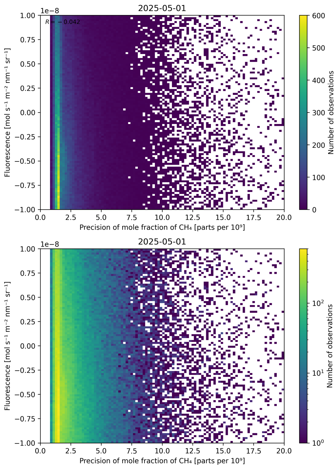
Figure 81: Scatter density plot of “Precision of mole fraction of \text{CH}_4 ” against “Fluorescence” for 2025-04-30 to 2025-05-02.
