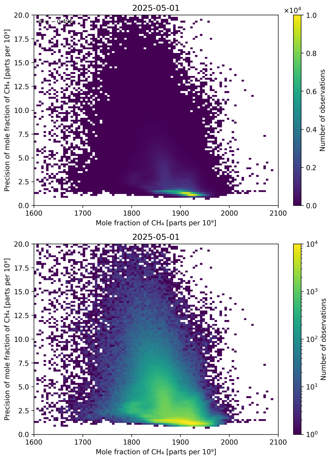
Figure 75: Scatter density plot of “Mole fraction of CH 4 ” against “Precision of mole fraction of CH 4 ” for 2025-04-30 to 2025-05-02.
