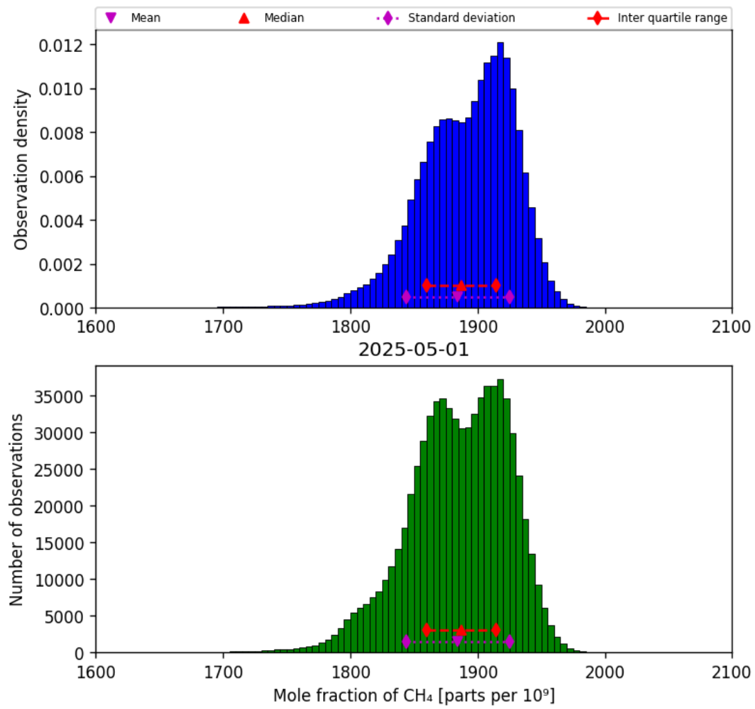
Figure 23: Histogram of “Mole fraction of CH 4 ” for 2025-04-30 to 2025-05-02
