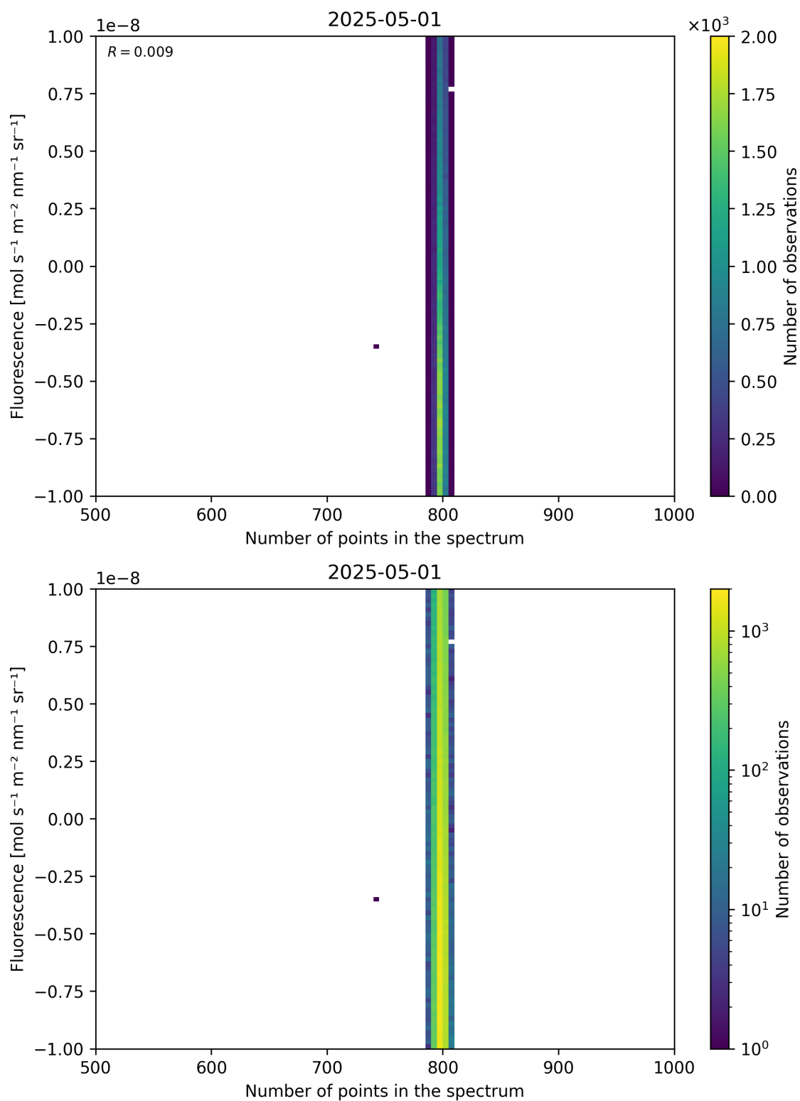
Figure 91: Scatter density plot of “Number of points in the spectrum” against “Fluorescence” for 2025-04-30 to 2025-05-02.
