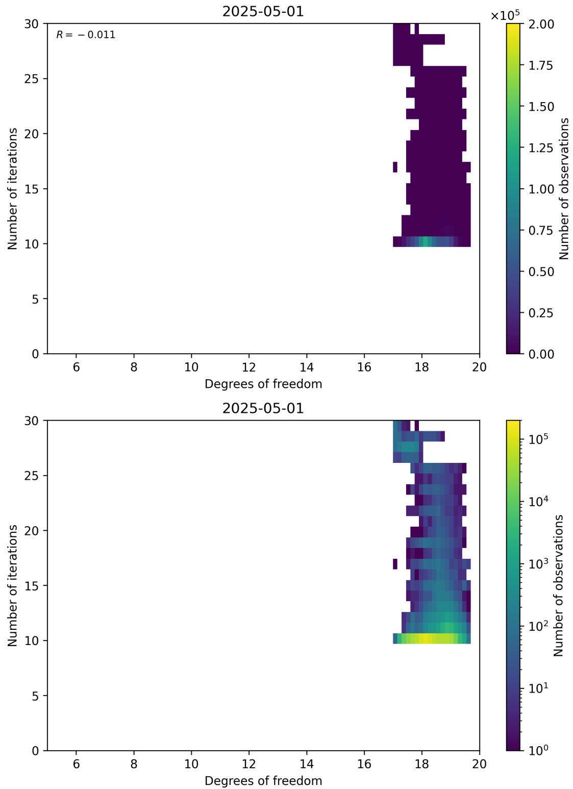
Figure 52: Scatter density plot of “Degrees of freedom” against “Number of iterations” for 2025-04-30 to 2025-05-02.
