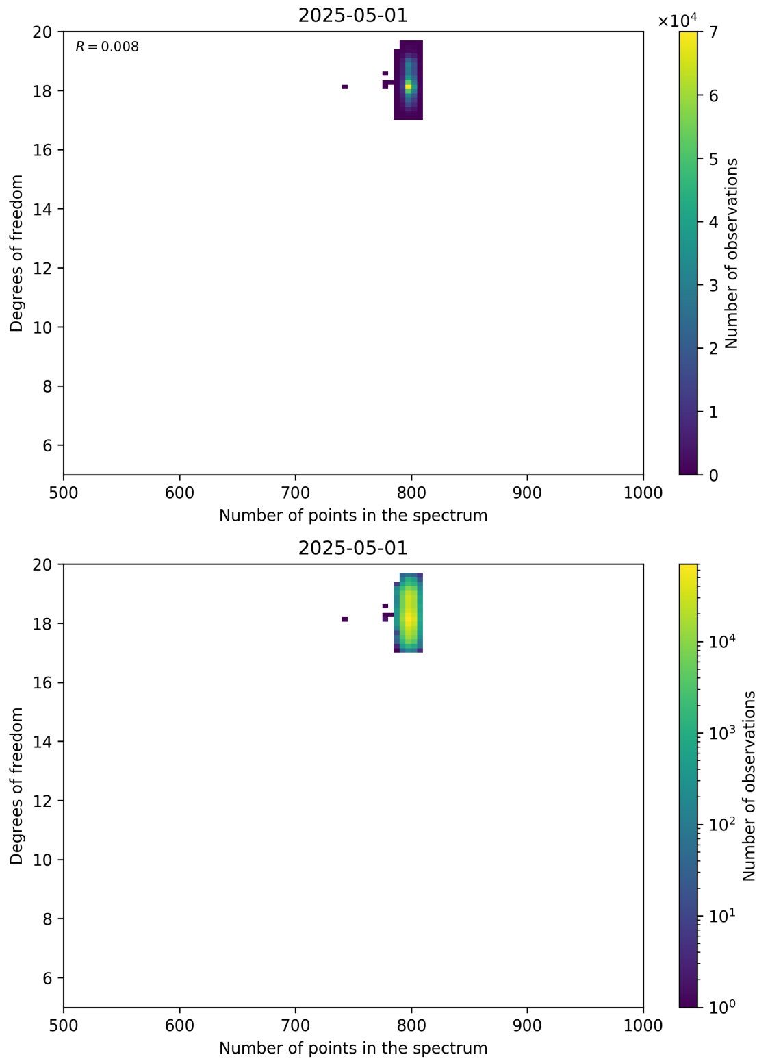
Figure 90: Scatter density plot of “Number of points in the spectrum” against “Degrees of freedom” for 2025-04-30 to 2025-05-02.
