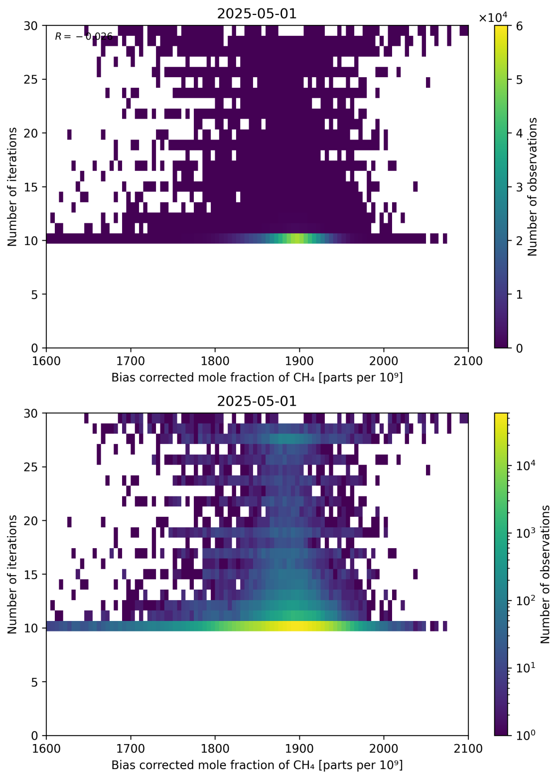
Figure 67: Scatter density plot of “Bias corrected mole fraction of CH 4 ” against “Number of iterations” for 2025-04-30 to 2025-05-02.
