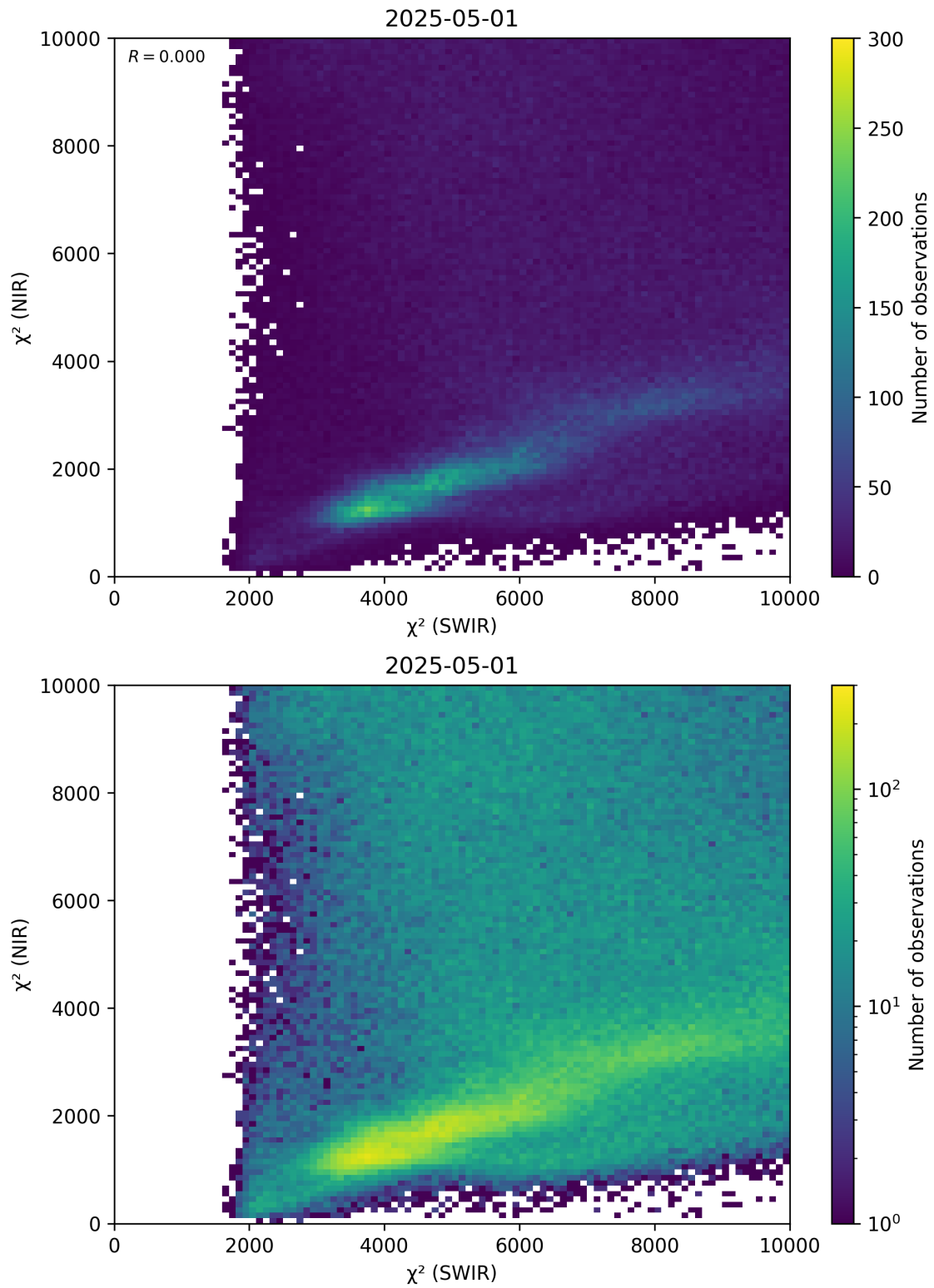
Figure 47: Scatter density plot of “ \chi^2 (SWIR)” against “ \chi^2 (NIR)” for 2025-04-30 to 2025-05-02.
