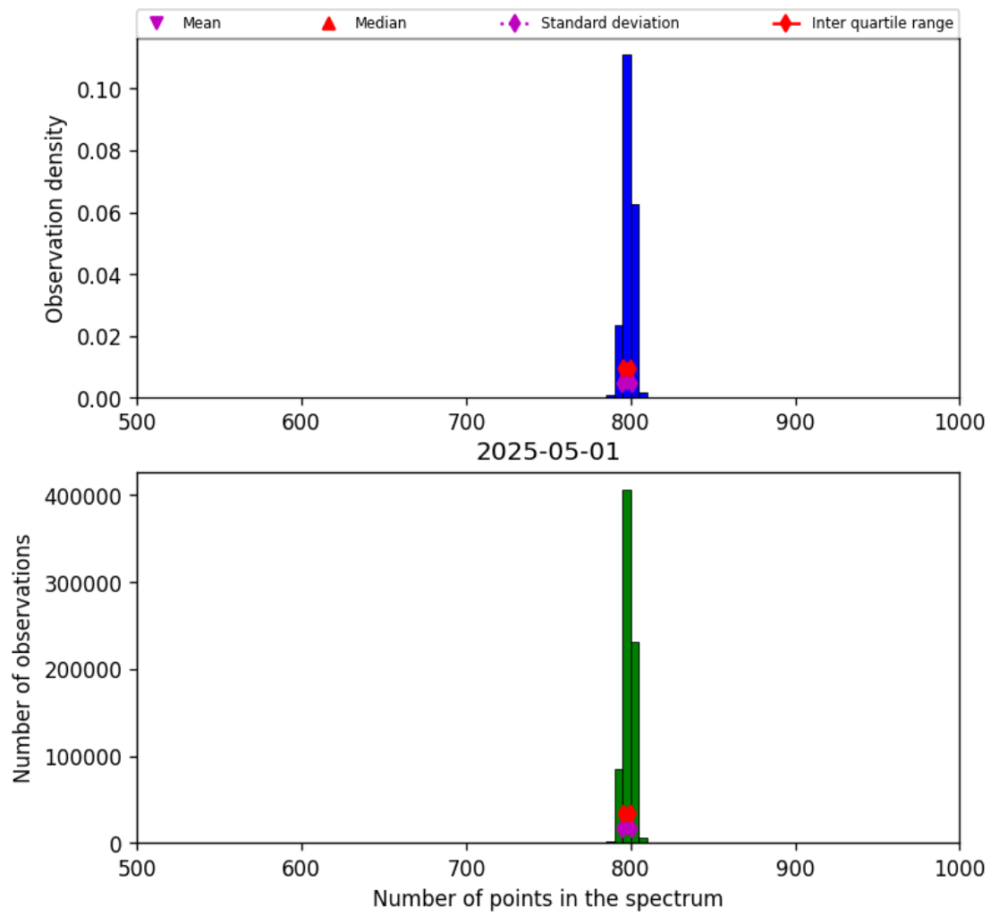
Figure 26: Histogram of “Number of points in the spectrum” for 2025-04-30 to 2025-05-02
