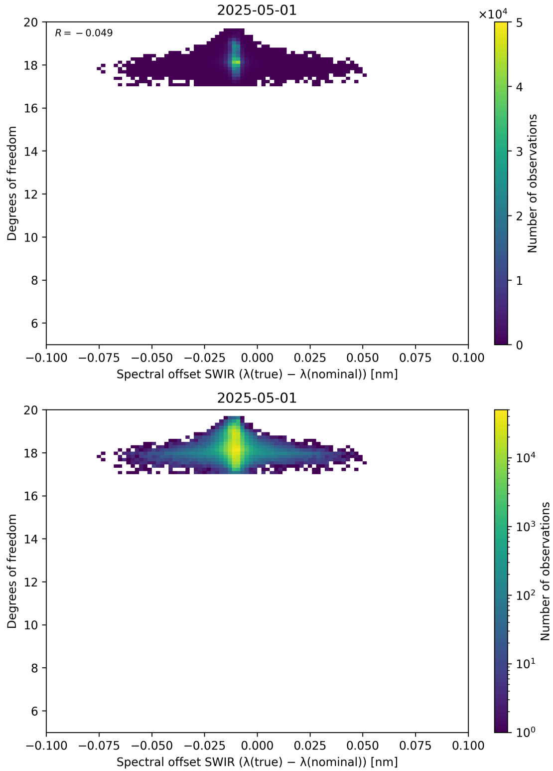
Figure 119: Scatter density plot of “Spectral offset SWIR ( \lambda_{\text{true}} - \lambda_{\text{nominal}} )” against “Degrees of freedom” for 2025-04-30 to 2025-05-02.
