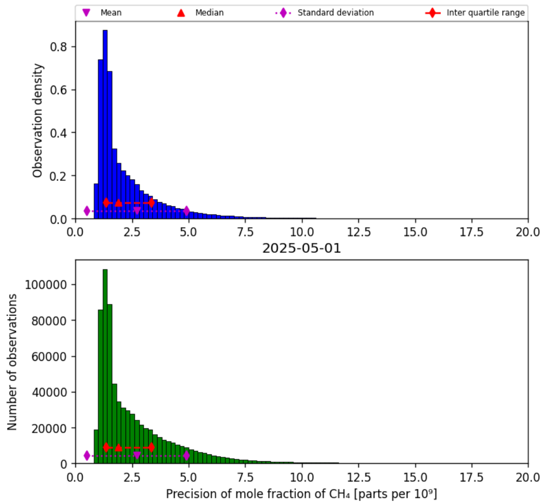
Figure 24: Histogram of “Precision of mole fraction of CH 4 ” for 2025-04-30 to 2025-05-02
