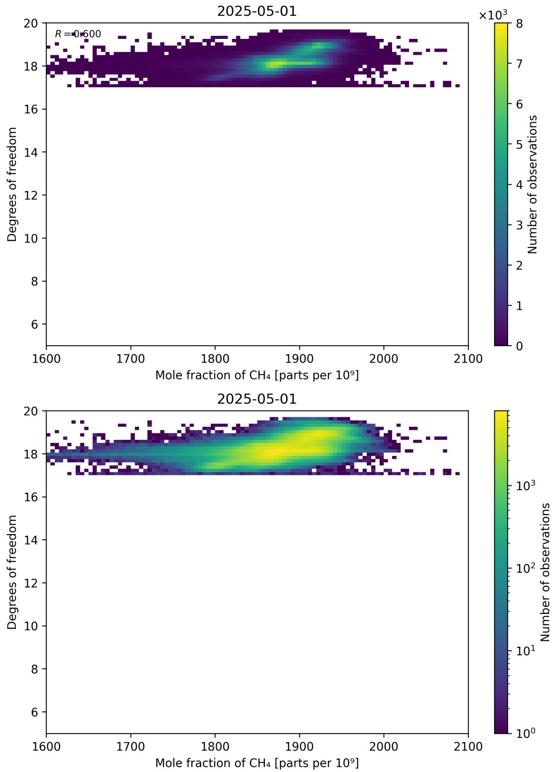
Figure 72: Scatter density plot of “Mole fraction of CH 4 ” against “Degrees of freedom” for 2025-04-30 to 2025-05-02.
