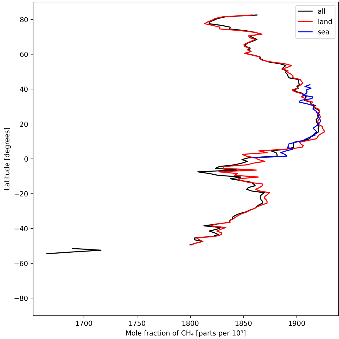
Figure 12: Zonal average of “Mole fraction of \text{CH}_4 ” for 2025-04-30 to 2025-05-02.
