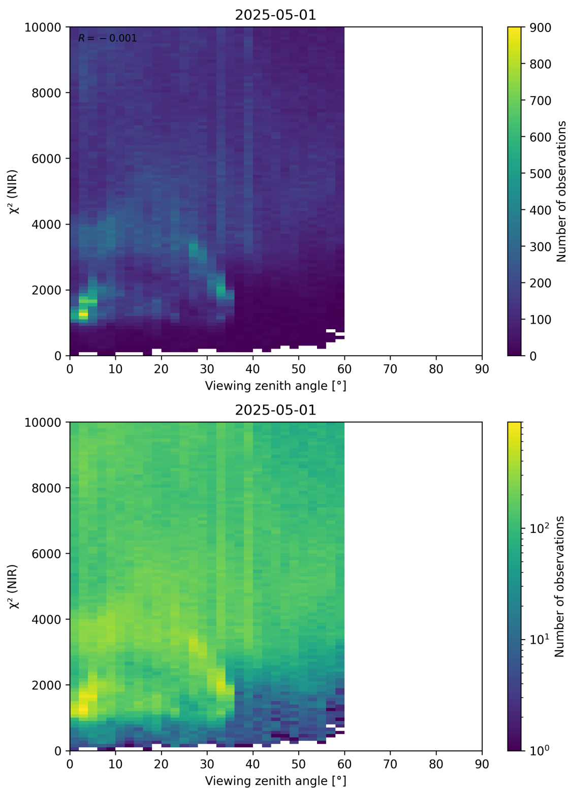
Figure 105: Scatter density plot of “Viewing zenith angle” against “ \chi^2 (NIR)” for 2025-04-30 to 2025-05-02.
