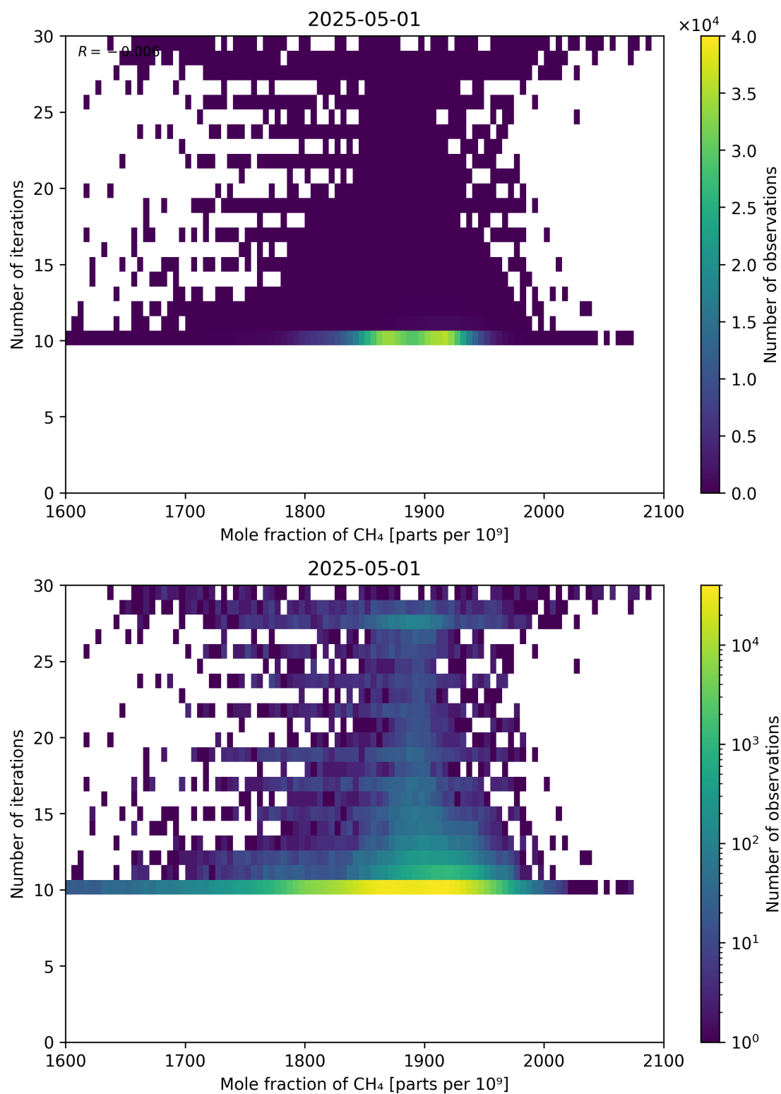
Figure 76: Scatter density plot of “Mole fraction of CH 4 ” against “Number of iterations” for 2025-04-30 to 2025-05-02.
