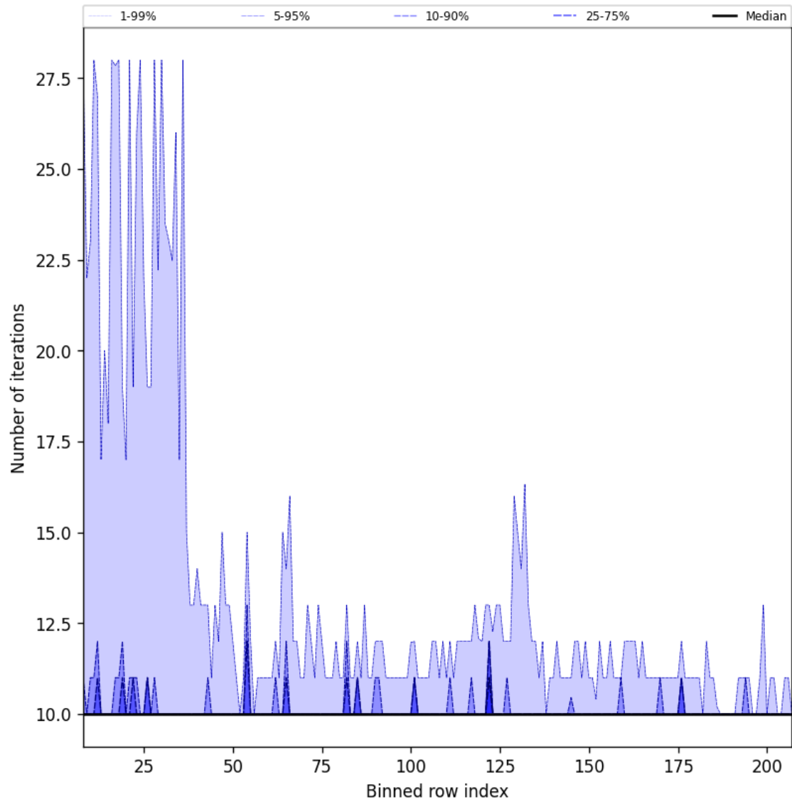
Figure 42: Along track statistics of “Number of iterations” for 2025-04-30 to 2025-05-02
