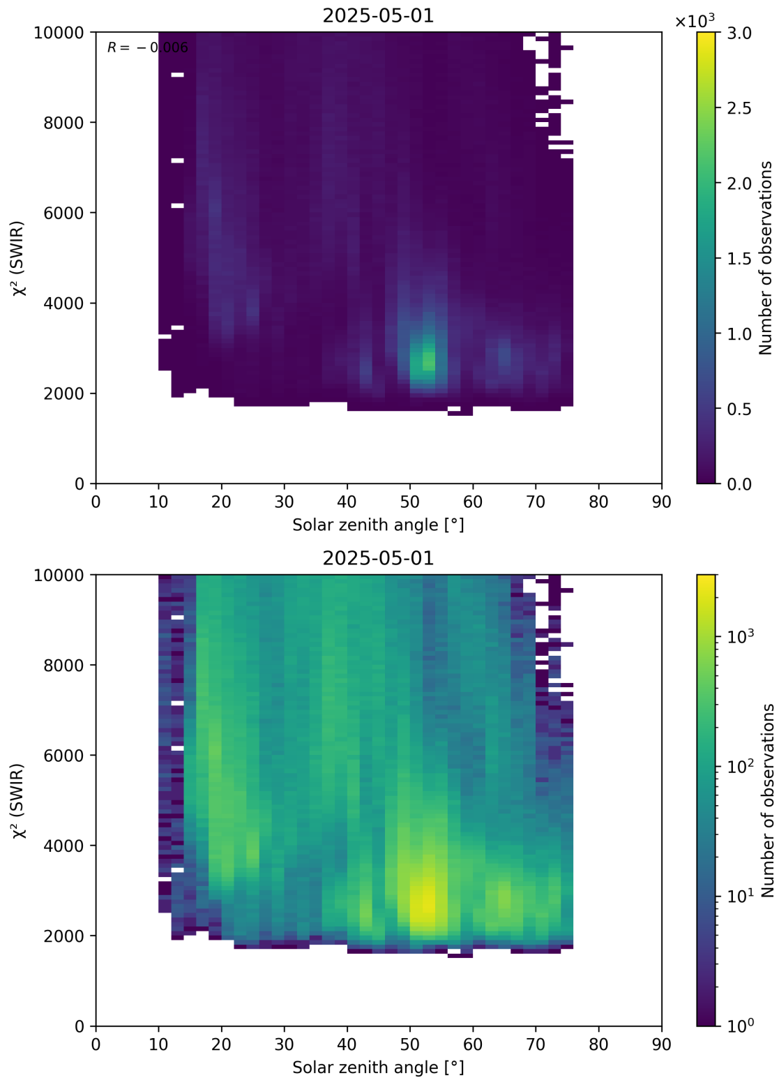
Figure 95: Scatter density plot of “Solar zenith angle” against “ \chi^2 (SWIR)” for 2025-04-30 to 2025-05-02.
