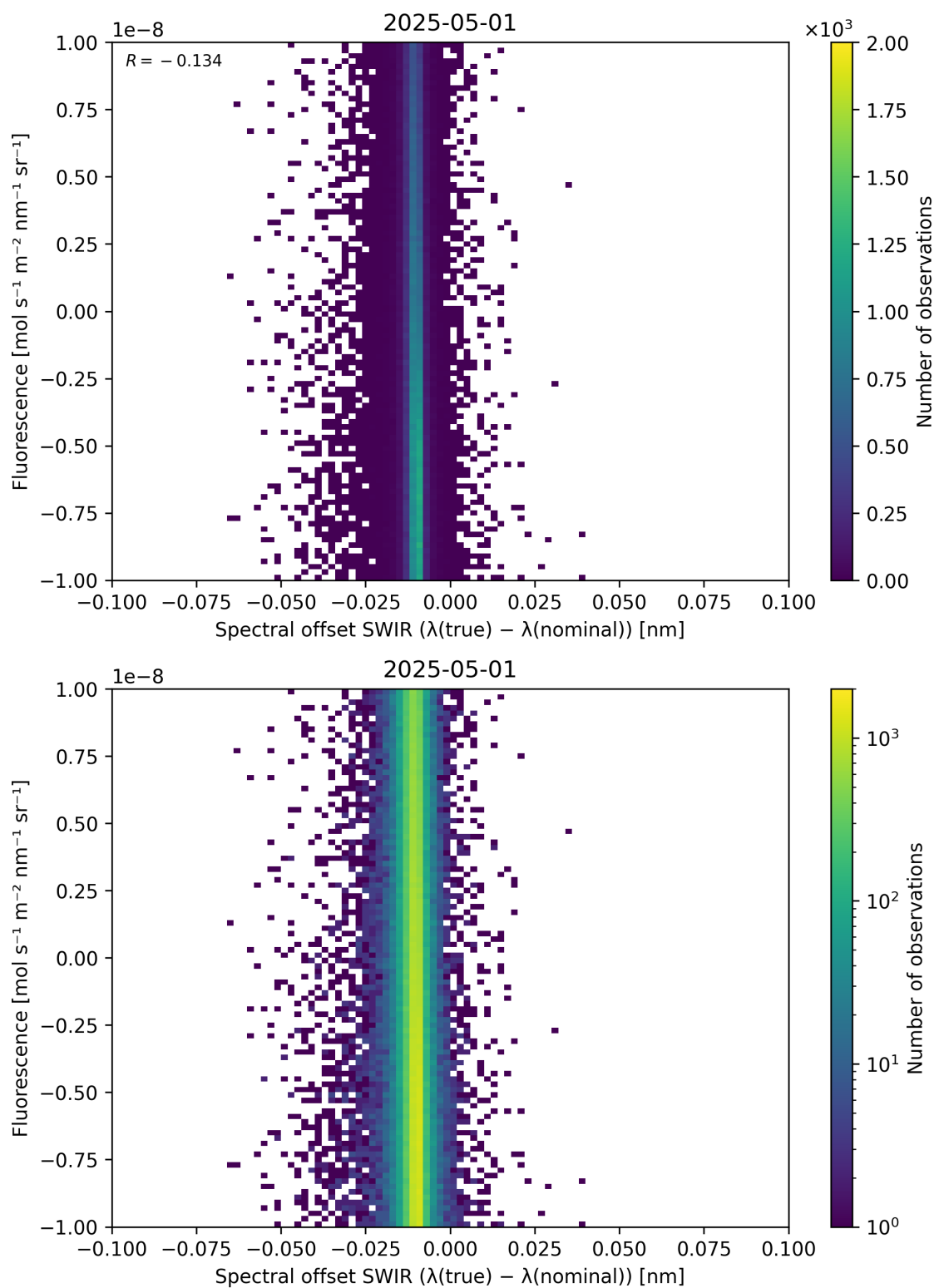
Figure 120: Scatter density plot of “Spectral offset SWIR ( \lambda_{\text{true}} - \lambda_{\text{nominal}} )” against “Fluorescence” for 2025-04-30 to 2025-05-02.
