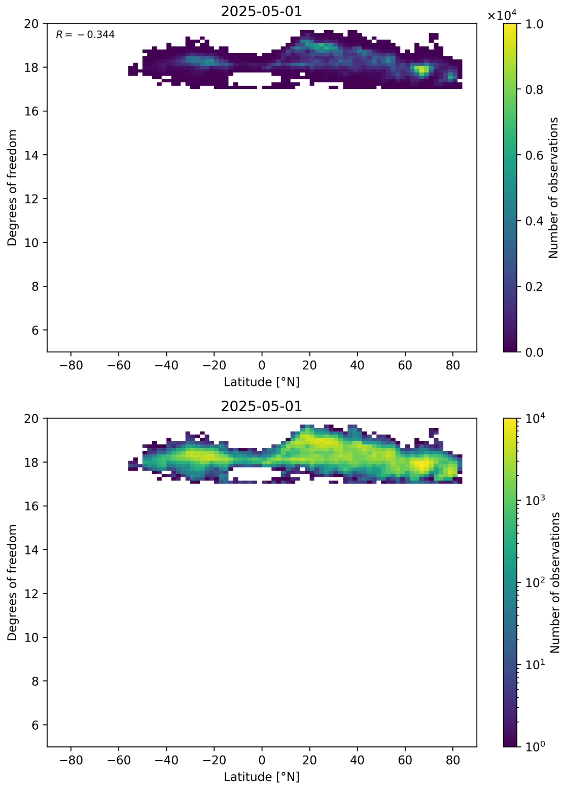
Figure 55: Scatter density plot of “Latitude” against “Degrees of freedom” for 2025-04-30 to 2025-05-02.
