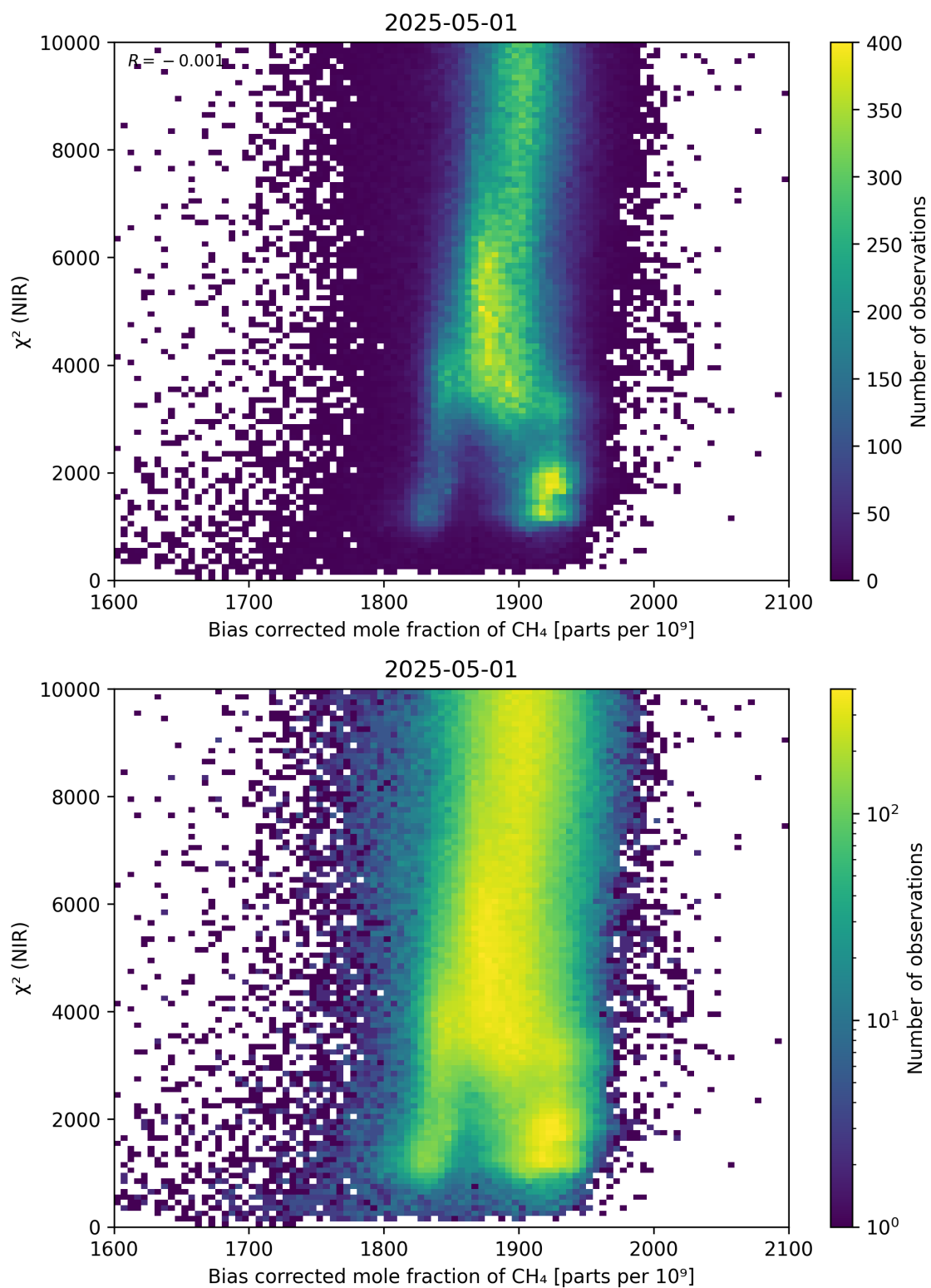
Figure 63: Scatter density plot of “Bias corrected mole fraction of \text{CH}_4 ” against “ \chi^2 (NIR)” for 2025-04-30 to 2025-05-02.
