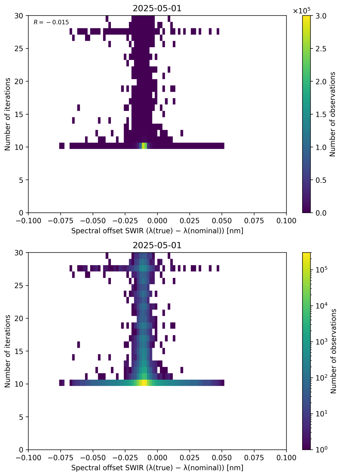
Figure 121: Scatter density plot of “Spectral offset SWIR ( \lambda_{\text{true}} - \lambda_{\text{nominal}} )” against “Number of iterations” for 2025-04-30 to 2025-05-02.
