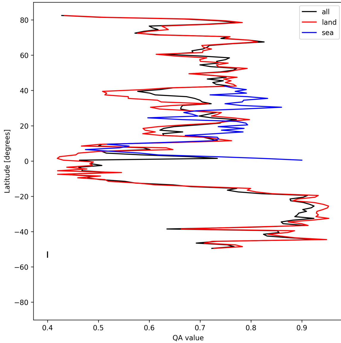
Figure 11: Zonal average of “QA value” for 2025-04-30 to 2025-05-02.
