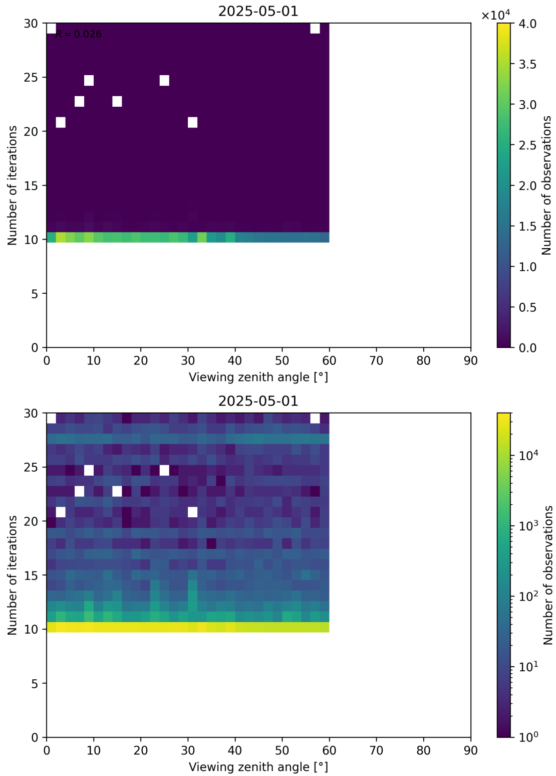
Figure 113: Scatter density plot of “Viewing zenith angle” against “Number of iterations” for 2025-04-30 to 2025-05-02.
