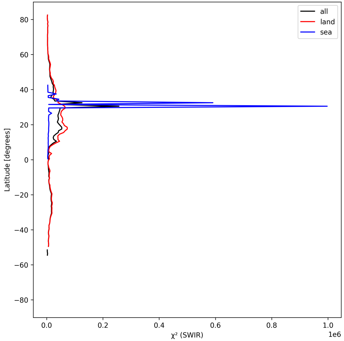
Figure 17: Zonal average of “ \chi^2 (SWIR)” for 2025-04-30 to 2025-05-02.
