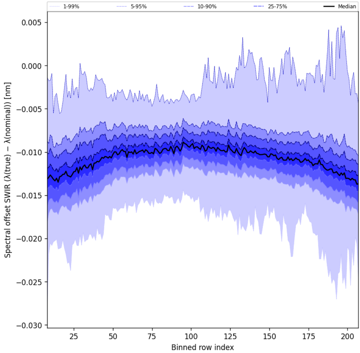
Figure 38: Along track statistics of “Spectral offset SWIR ( \lambda_{\text{true}} - \lambda_{\text{nominal}} )” for 2025-04-30 to 2025-05-02
