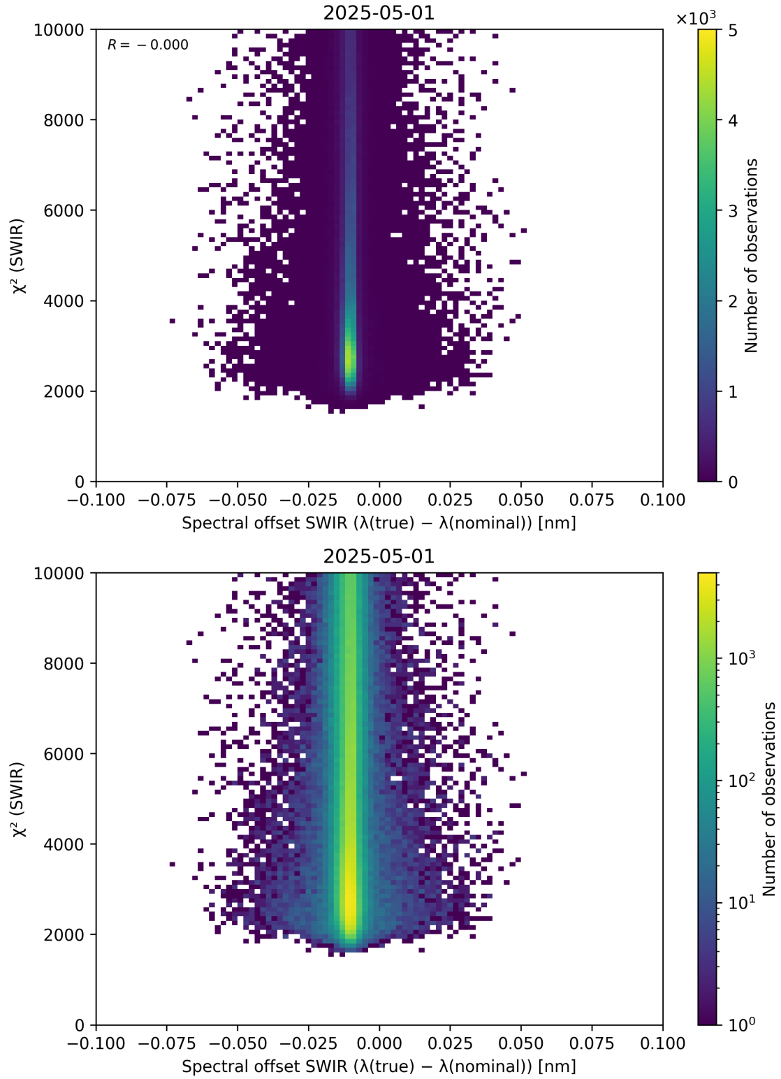
Figure 118: Scatter density plot of “Spectral offset SWIR ( \lambda_{\text{true}} - \lambda_{\text{nominal}} )” against “ \chi^2 (SWIR)” for 2025-04-30 to 2025-05-02.
