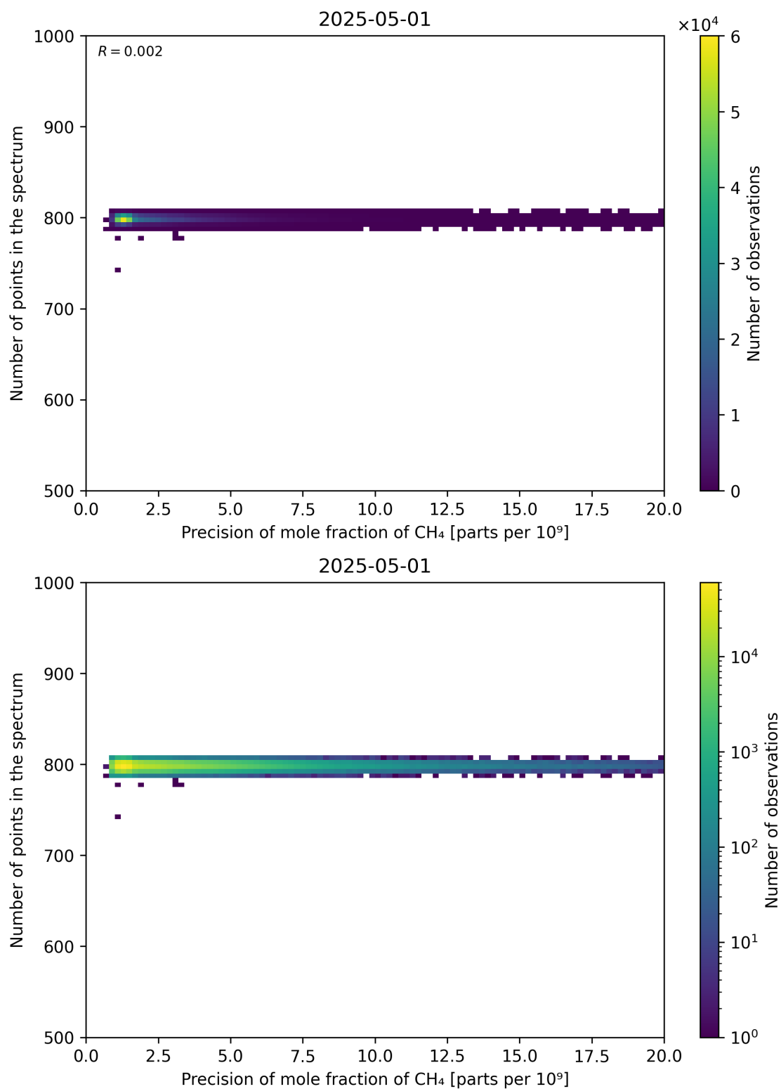
Figure 84: Scatter density plot of “Precision of mole fraction of CH 4 ” against “Number of points in the spectrum” for 2025-04-30 to 2025-05-02.
