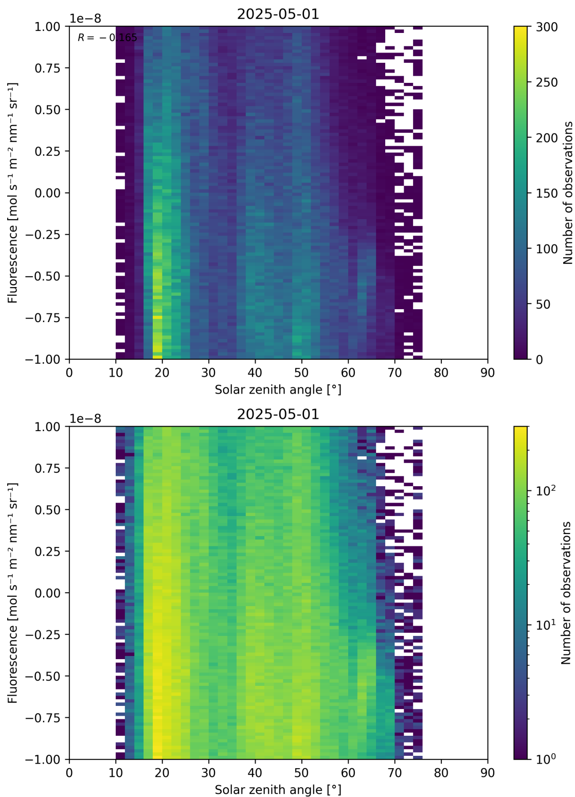
Figure 97: Scatter density plot of “Solar zenith angle” against “Fluorescence” for 2025-04-30 to 2025-05-02.
