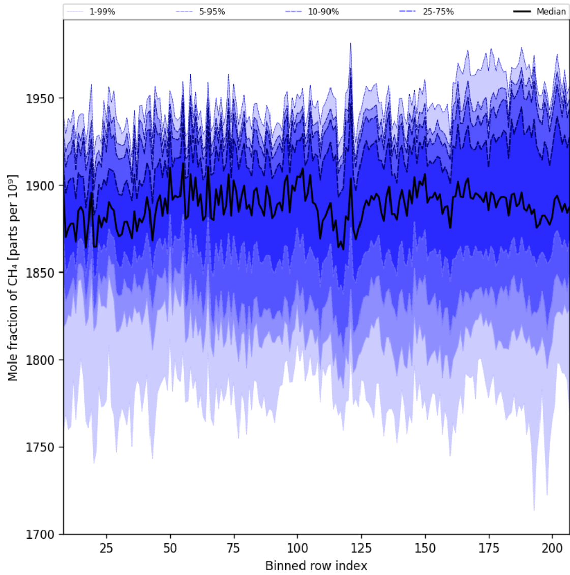
Figure 34: Along track statistics of “Mole fraction of CH 4 ” for 2025-04-30 to 2025-05-02
