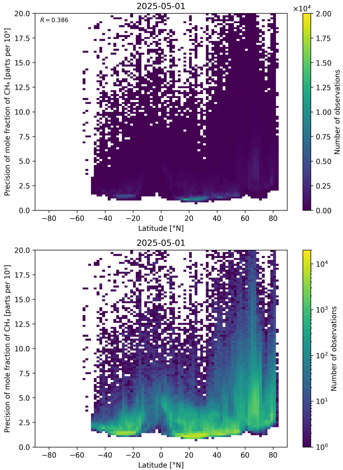
Figure 59: Scatter density plot of “Latitude” against “Precision of mole fraction of \text{CH}_4 ” for 2025-04-30 to 2025-05-02.
