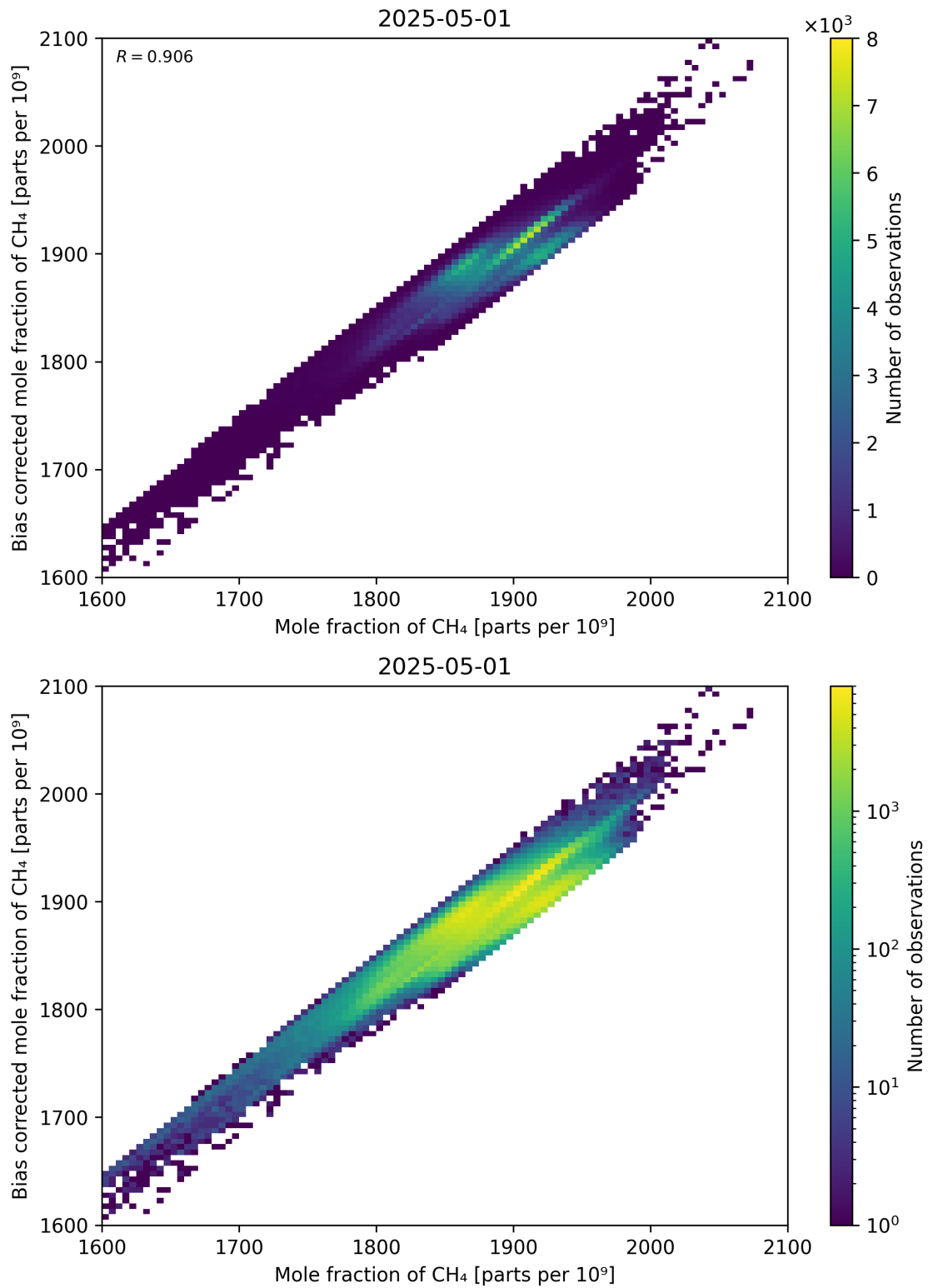
Figure 74: Scatter density plot of “Mole fraction of CH 4 ” against “Bias corrected mole fraction of CH 4 ” for 2025-04-30 to 2025-05-02.
