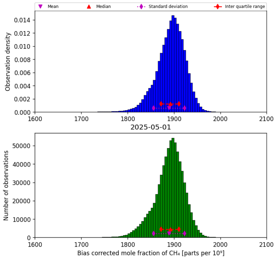
Figure 25: Histogram of “Bias corrected mole fraction of CH 4 ” for 2025-04-30 to 2025-05-02
