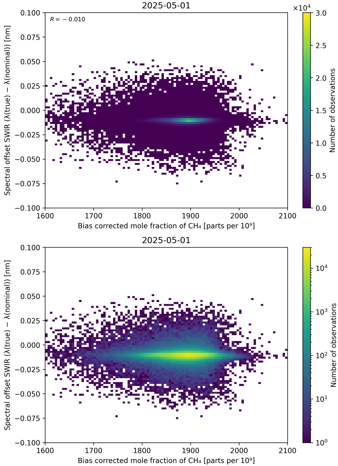
Figure 69: Scatter density plot of “Bias corrected mole fraction of \text{CH}_4 ” against “Spectral offset SWIR ( \lambda_{\text{true}} - \lambda_{\text{nominal}} )” for 2025-04-30 to 2025-05-02.
