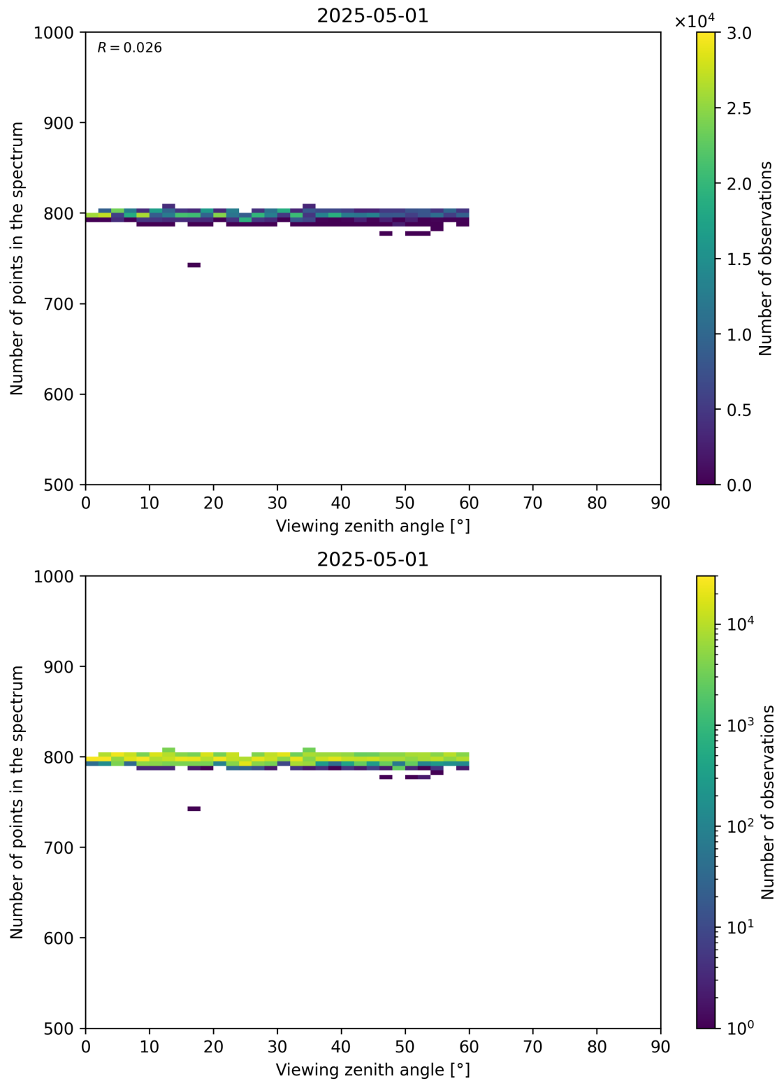
Figure 114: Scatter density plot of “Viewing zenith angle” against “Number of points in the spectrum” for 2025-04-30 to 2025-05-02.
