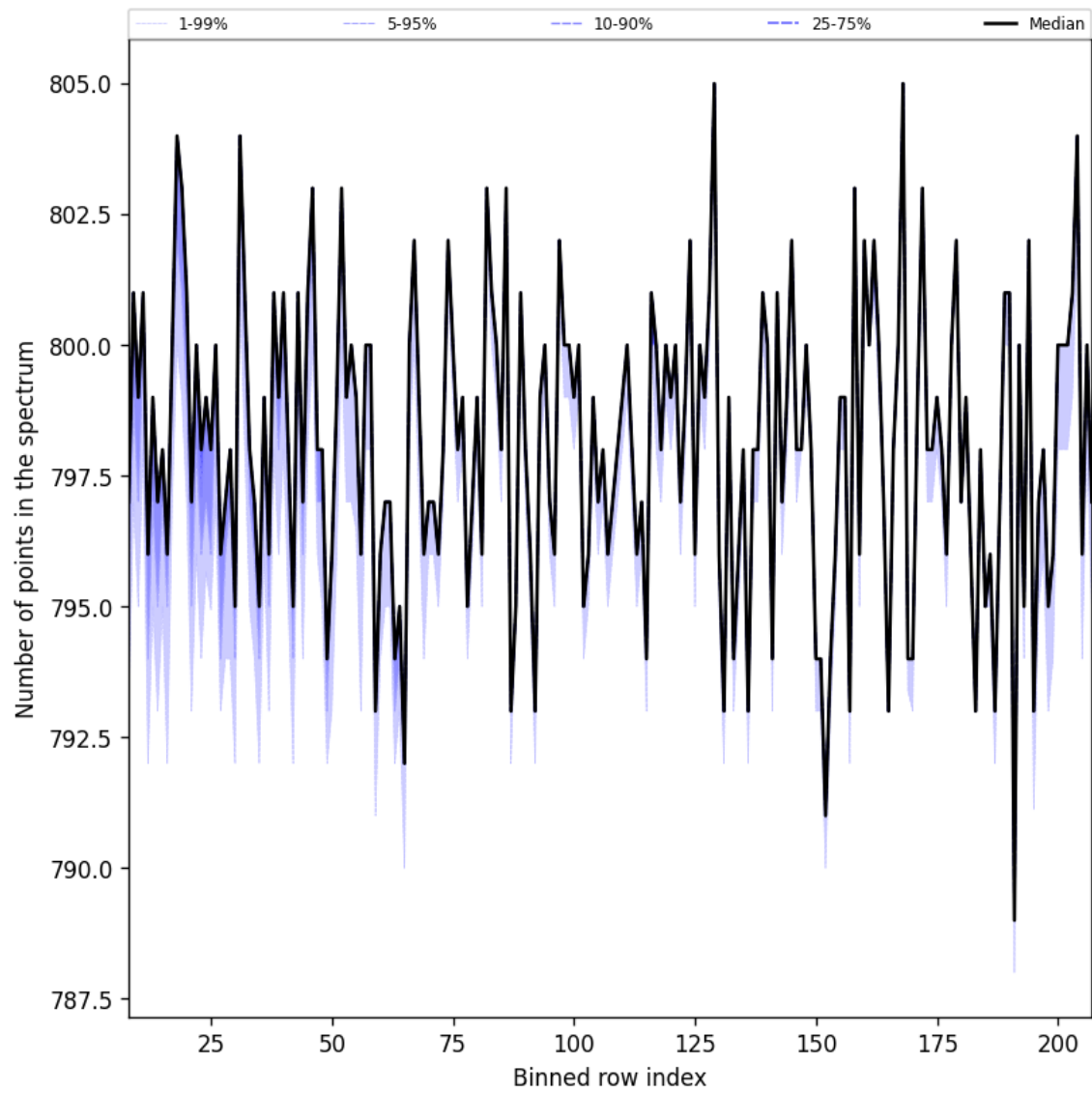
Figure 37: Along track statistics of “Number of points in the spectrum” for 2025-04-30 to 2025-05-02
