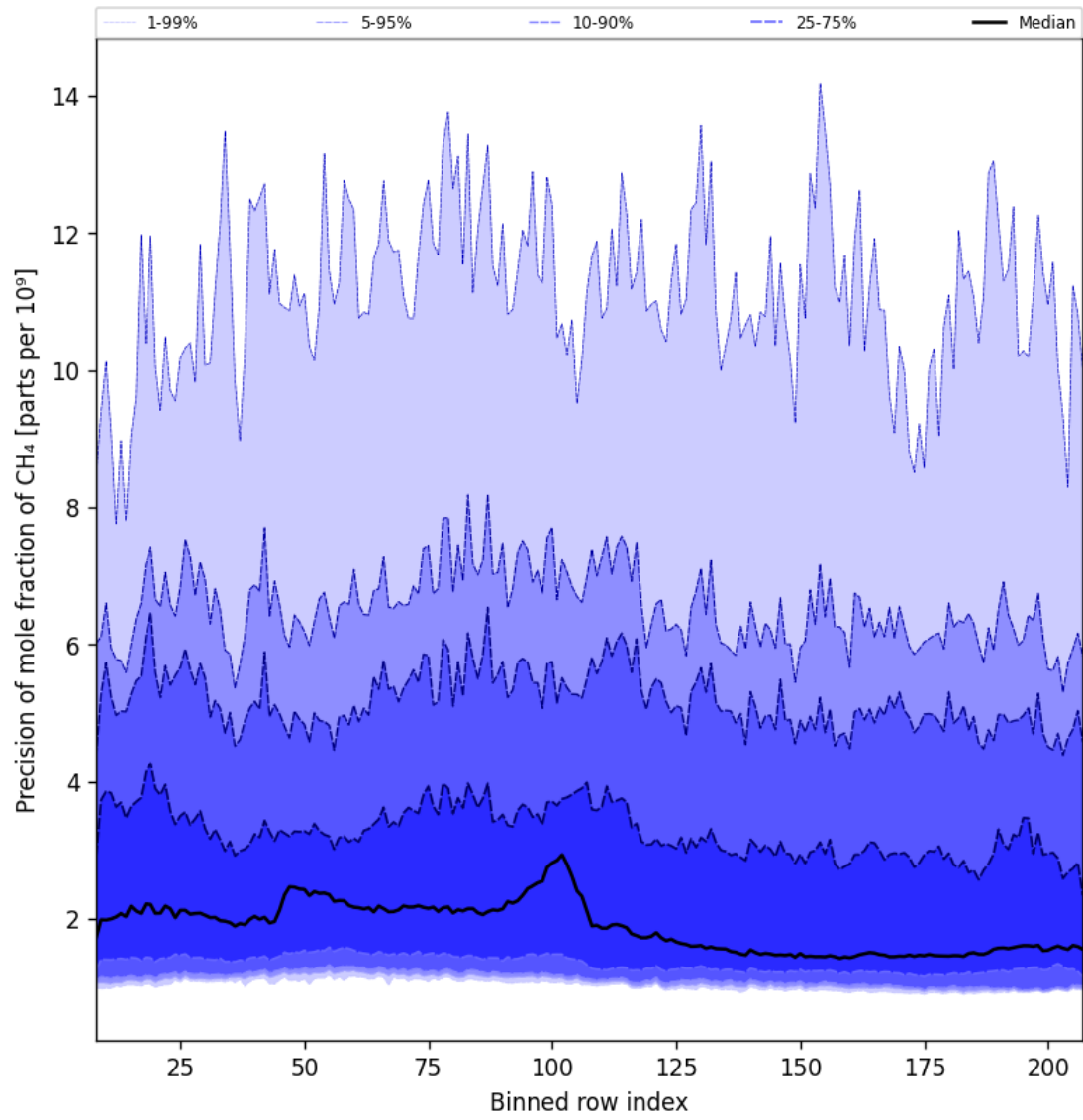
Figure 35: Along track statistics of “Precision of mole fraction of CH 4 ” for 2025-04-30 to 2025-05-02
