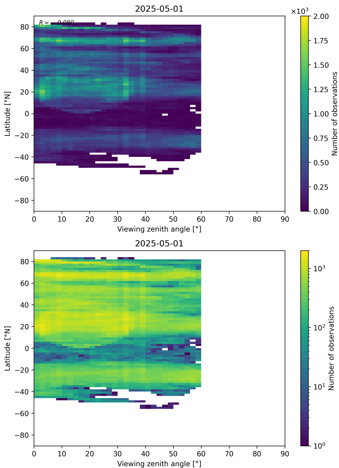
Figure 109: Scatter density plot of “Viewing zenith angle” against “Latitude” for 2025-04-30 to 2025-05-02.
