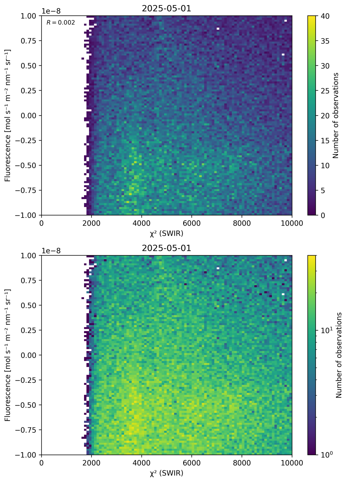
Figure 49: Scatter density plot of “ \chi^2 (SWIR)” against “Fluorescence” for 2025-04-30 to 2025-05-02.
