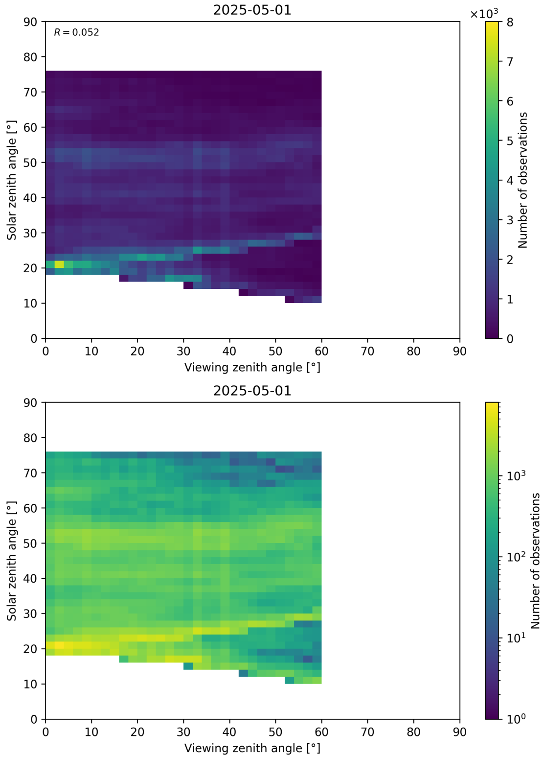
Figure 115: Scatter density plot of “Viewing zenith angle” against “Solar zenith angle” for 2025-04-30 to 2025-05-02.
