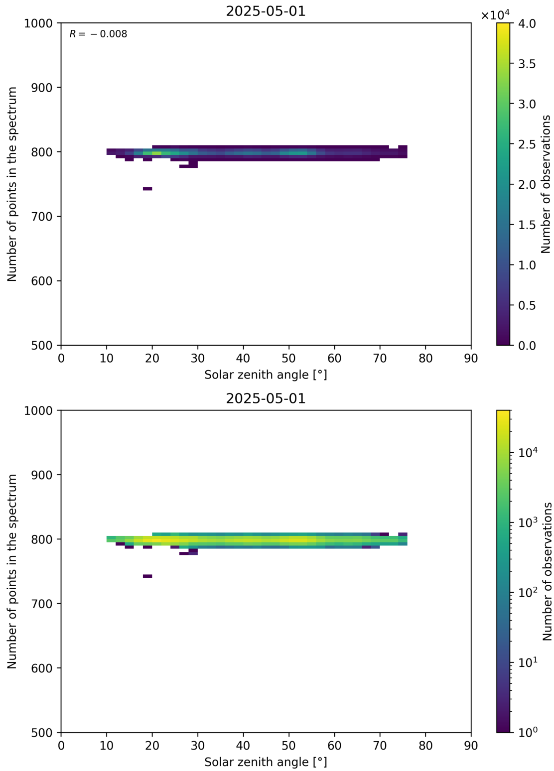
Figure 103: Scatter density plot of “Solar zenith angle” against “Number of points in the spectrum” for 2025-04-30 to 2025-05-02.
