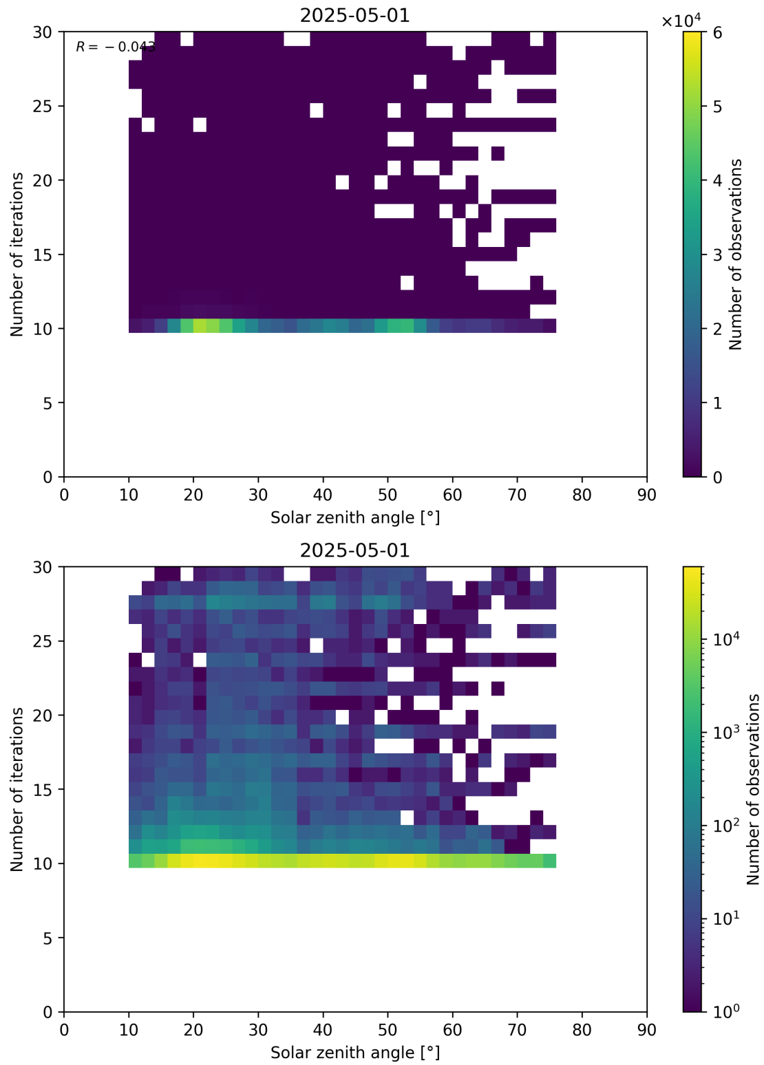
Figure 102: Scatter density plot of “Solar zenith angle” against “Number of iterations” for 2025-04-30 to 2025-05-02.
