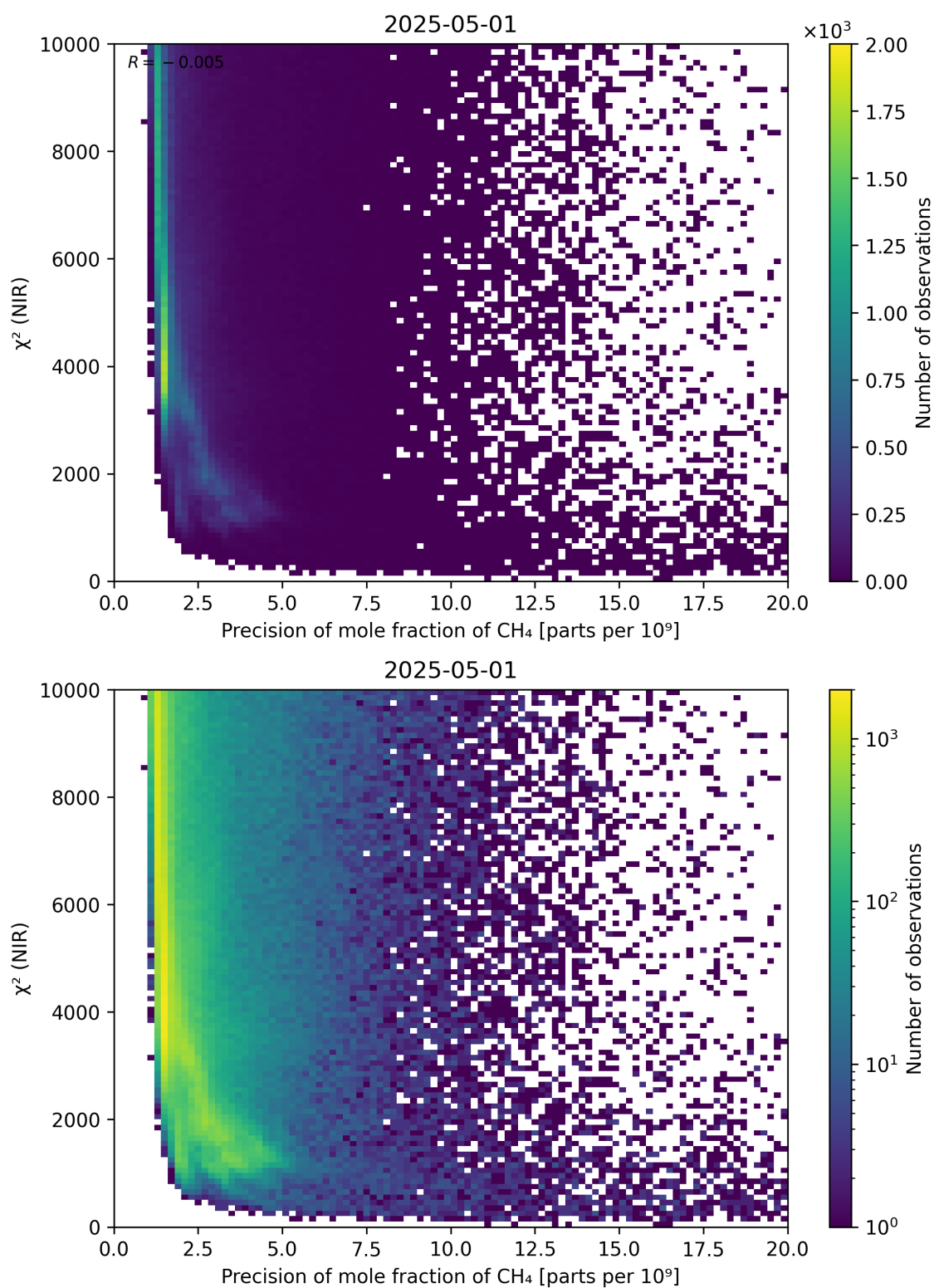
Figure 78: Scatter density plot of “Precision of mole fraction of \text{CH}_4 ” against “ \chi^2 (NIR)” for 2025-04-30 to 2025-05-02.
