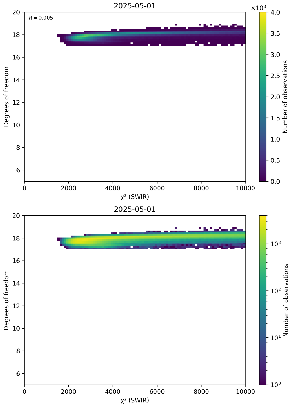
Figure 48: Scatter density plot of " \chi^2 (SWIR)" against "Degrees of freedom" for 2025-04-30 to 2025-05-02.
