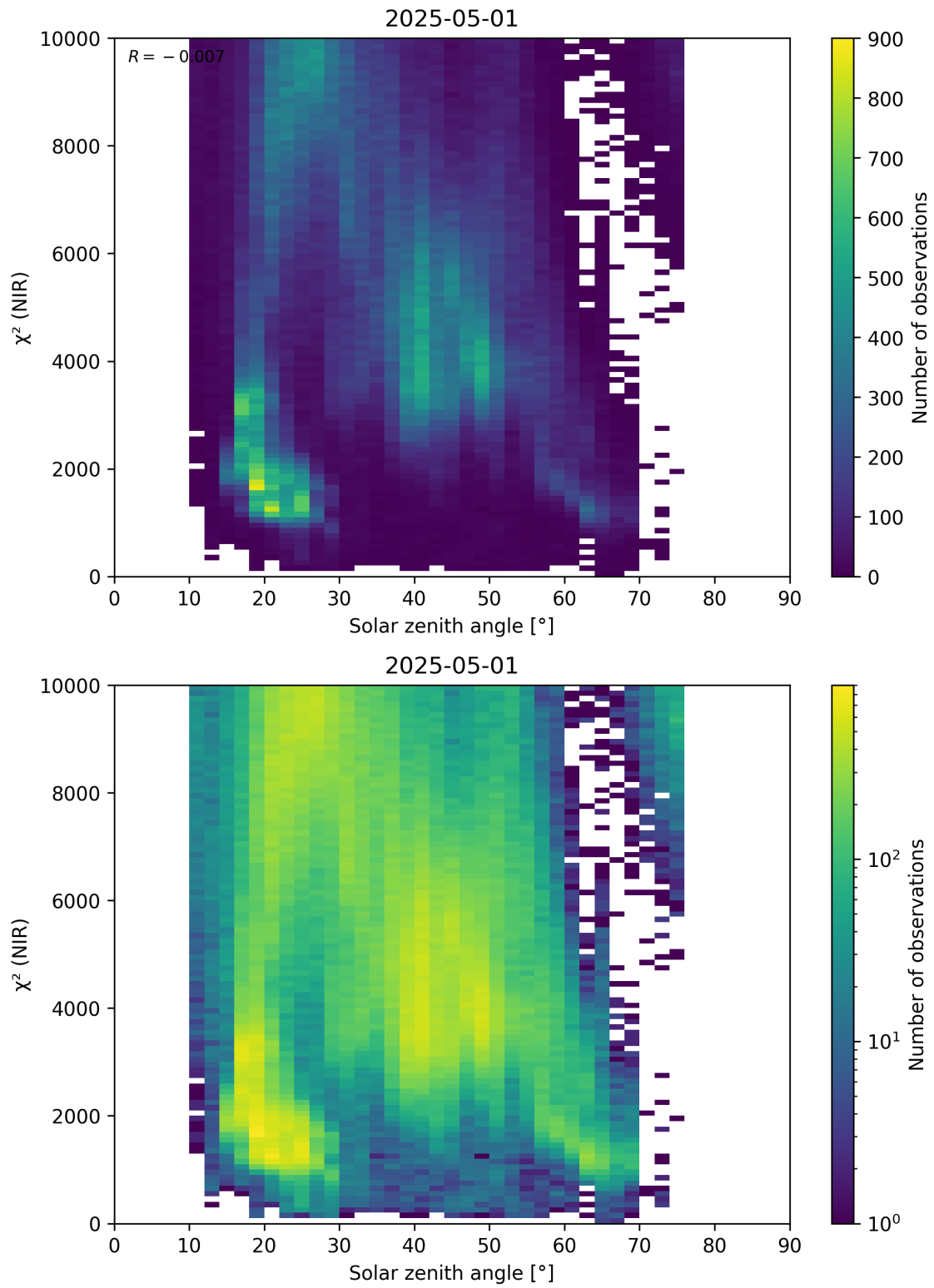
Figure 94: Scatter density plot of “Solar zenith angle” against “ \chi^2 (NIR)” for 2025-04-30 to 2025-05-02.
