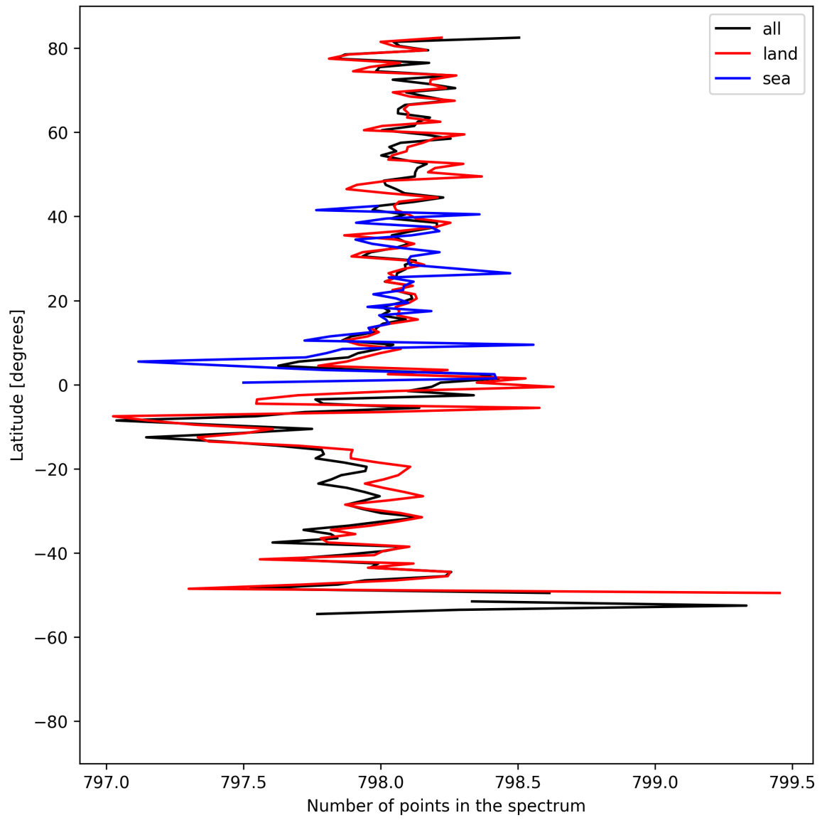
Figure 15: Zonal average of “Number of points in the spectrum” for 2025-04-30 to 2025-05-02.
