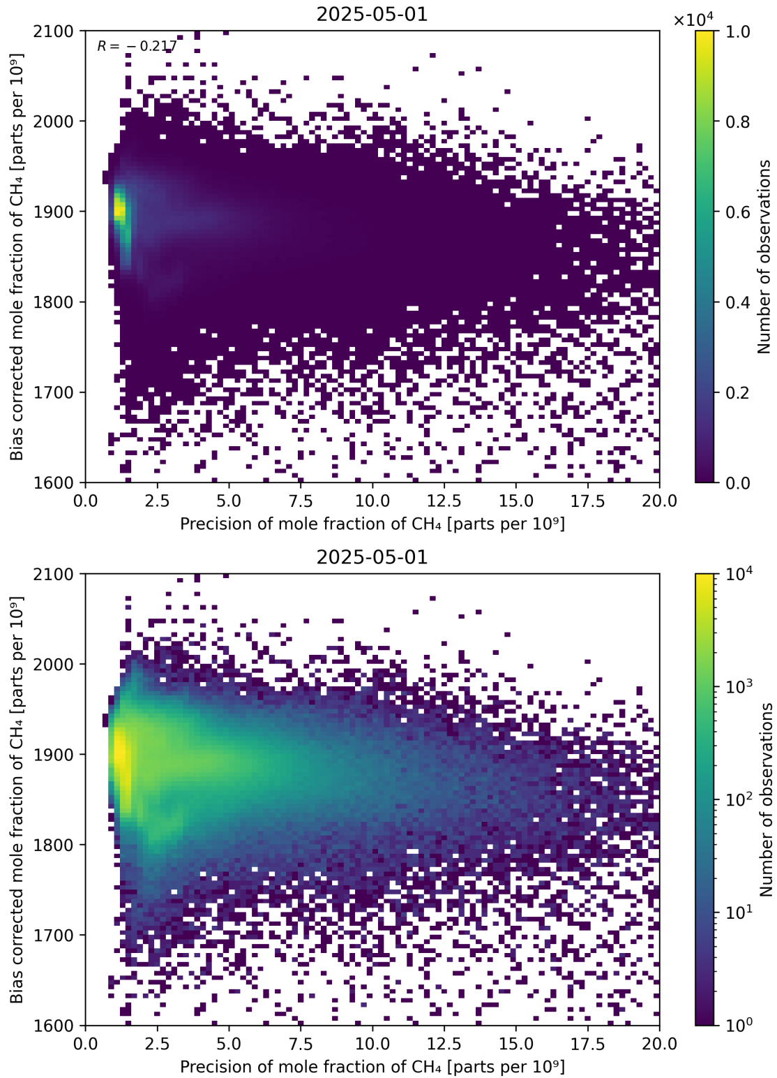
Figure 82: Scatter density plot of “Precision of mole fraction of CH 4 ” against “Bias corrected mole fraction of CH 4 ” for 2025-04-30 to 2025-05-02.
