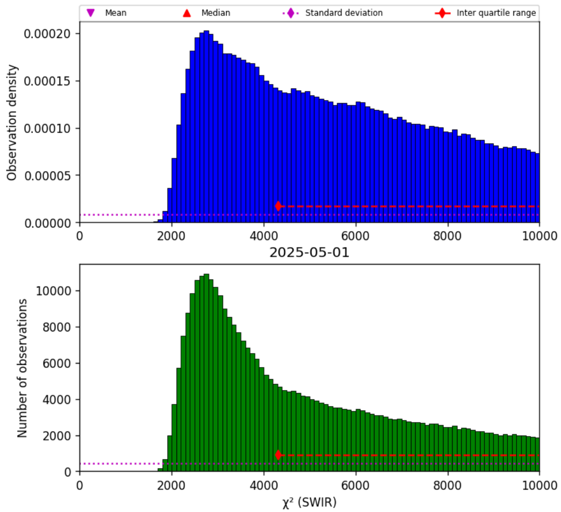
Figure 28: Histogram of " \chi^2 (SWIR)" for 2025-04-30 to 2025-05-02
