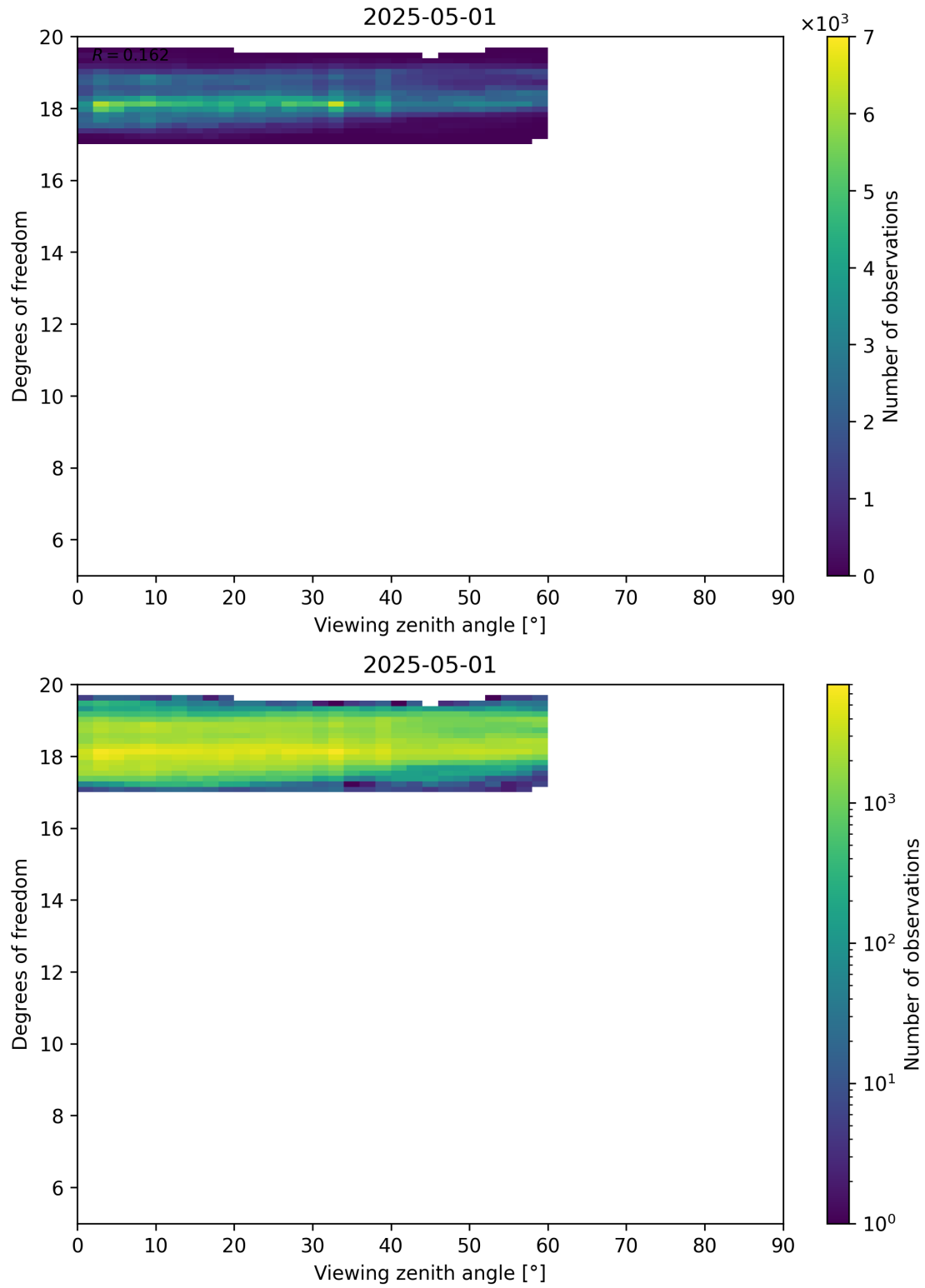
Figure 107: Scatter density plot of “Viewing zenith angle” against “Degrees of freedom” for 2025-04-30 to 2025-05-02.
