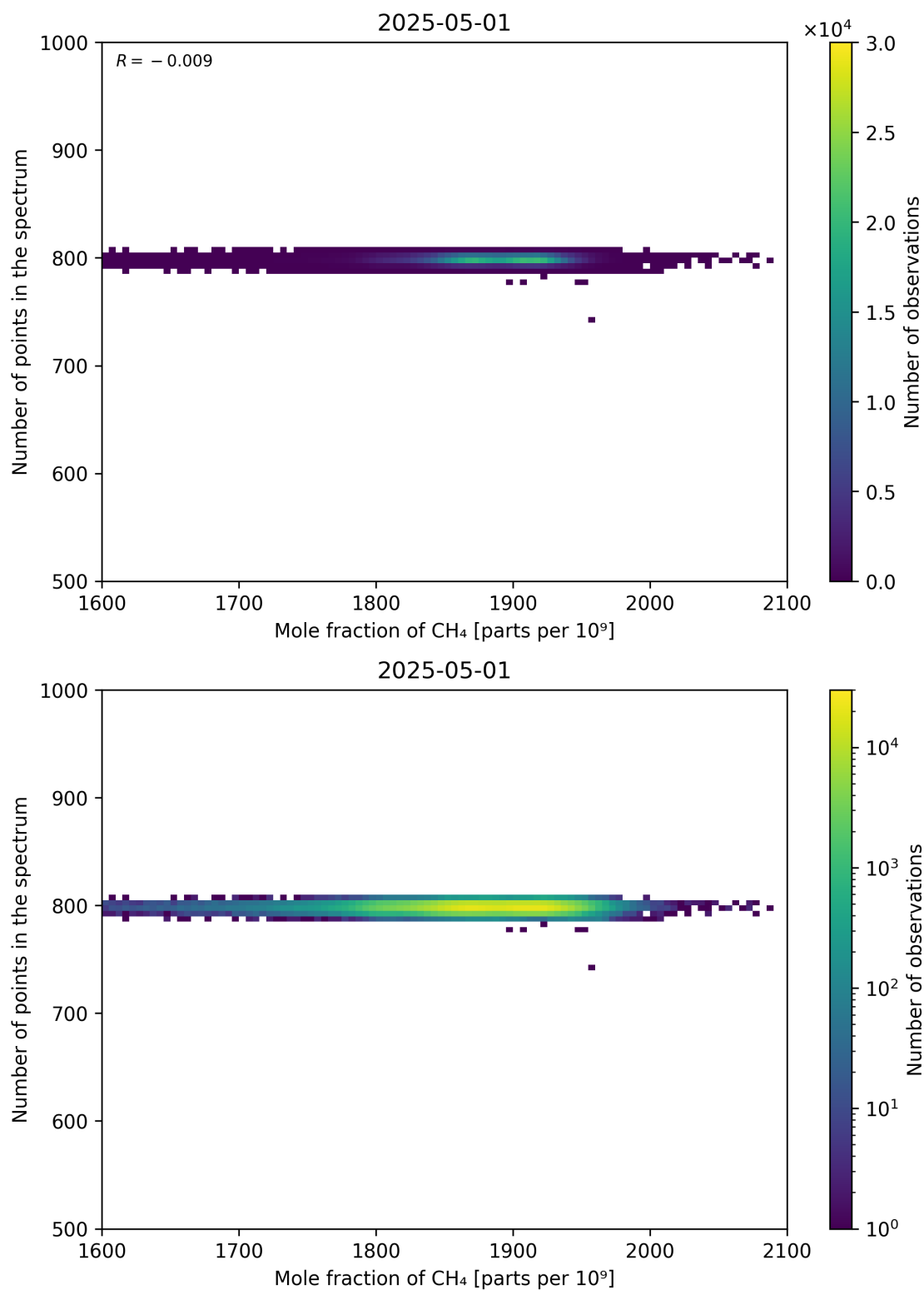
Figure 77: Scatter density plot of “Mole fraction of CH 4 ” against “Number of points in the spectrum” for 2025-04-30 to 2025-05-02.
