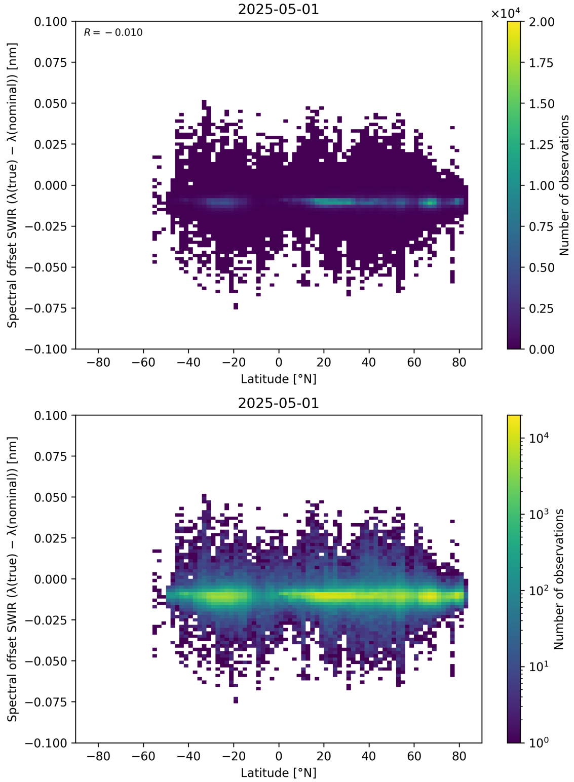
Figure 62: Scatter density plot of “Latitude” against “Spectral offset SWIR ( \lambda_{\text{true}} - \lambda_{\text{nominal}} )” for 2025-04-30 to 2025-05-02.
