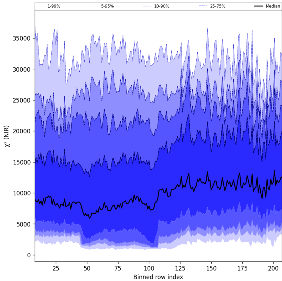
Figure 40: Along track statistics of “ \chi^2 (NIR)” for 2025-04-30 to 2025-05-02
