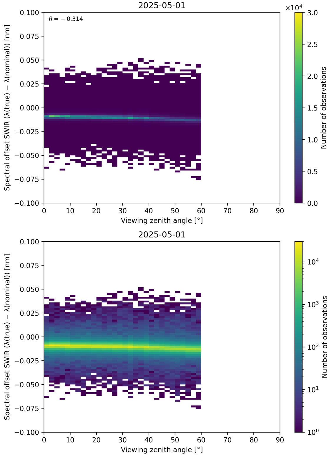
Figure 116: Scatter density plot of “Viewing zenith angle” against “Spectral offset SWIR ( \lambda_{\text{true}} - \lambda_{\text{nominal}} )” for 2025-04-30 to 2025-05-02.
