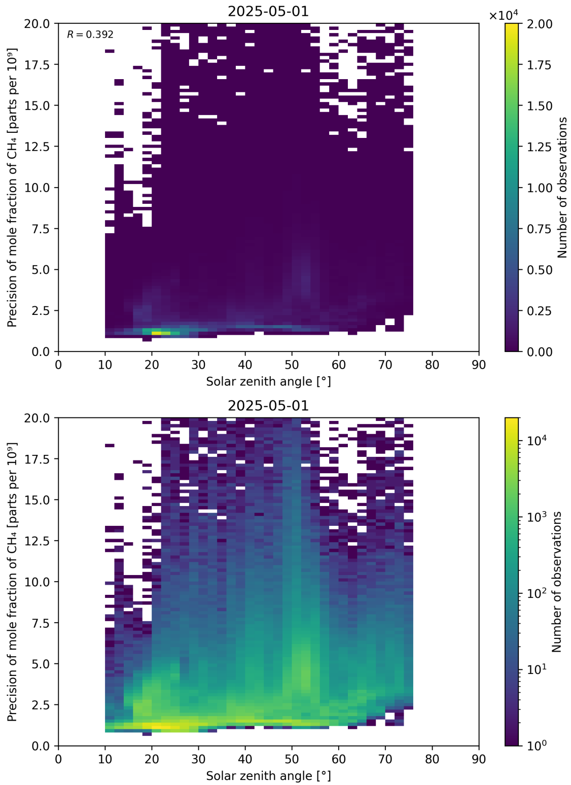
Figure 101: Scatter density plot of “Solar zenith angle” against “Precision of mole fraction of CH 4 ” for 2025-04-30 to 2025-05-02.
