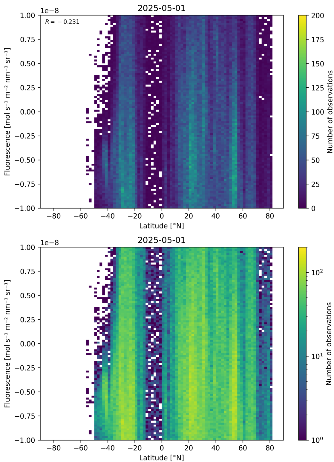
Figure 56: Scatter density plot of “Latitude” against “Fluorescence” for 2025-04-30 to 2025-05-02.
