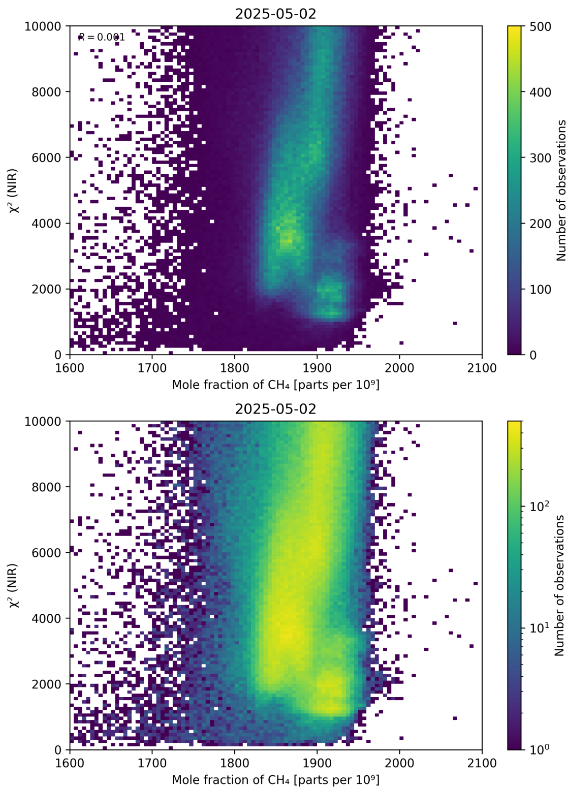
Figure 70: Scatter density plot of “Mole fraction of \text{CH}_4 ” against “ \chi^2 (NIR)” for 2025-05-01 to 2025-05-03.
