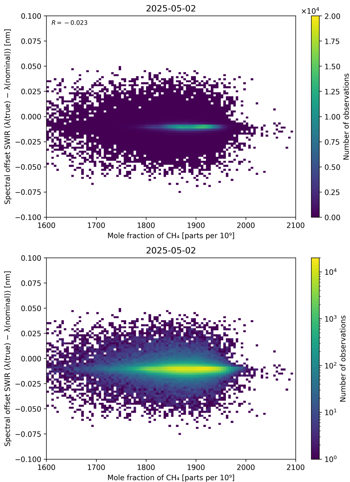
Figure 86: Scatter density plot of “Mole fraction of \text{CH}_4 ” against “Spectral offset SWIR ( \lambda_{\text{true}} - \lambda_{\text{nominal}} )” for 2025-05-01 to 2025-05-03.
