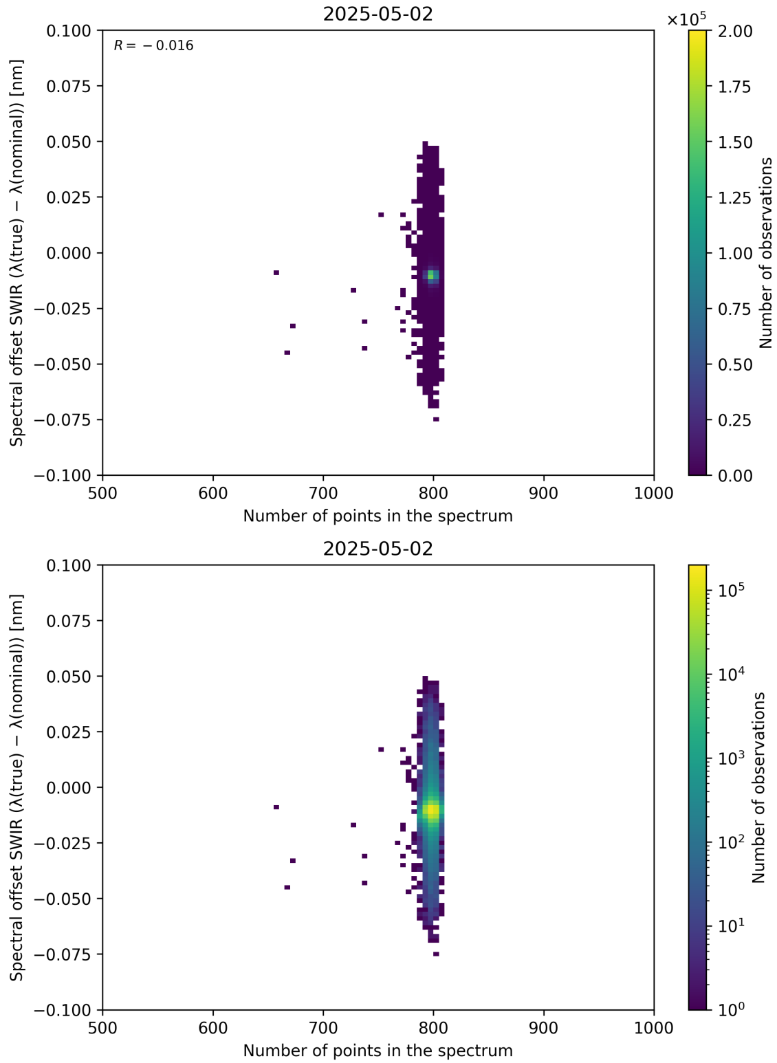
Figure 93: Scatter density plot of “Number of points in the spectrum” against “Spectral offset SWIR ( \lambda_{\text{true}} - \lambda_{\text{nominal}} )” for 2025-05-01 to 2025-05-03.
