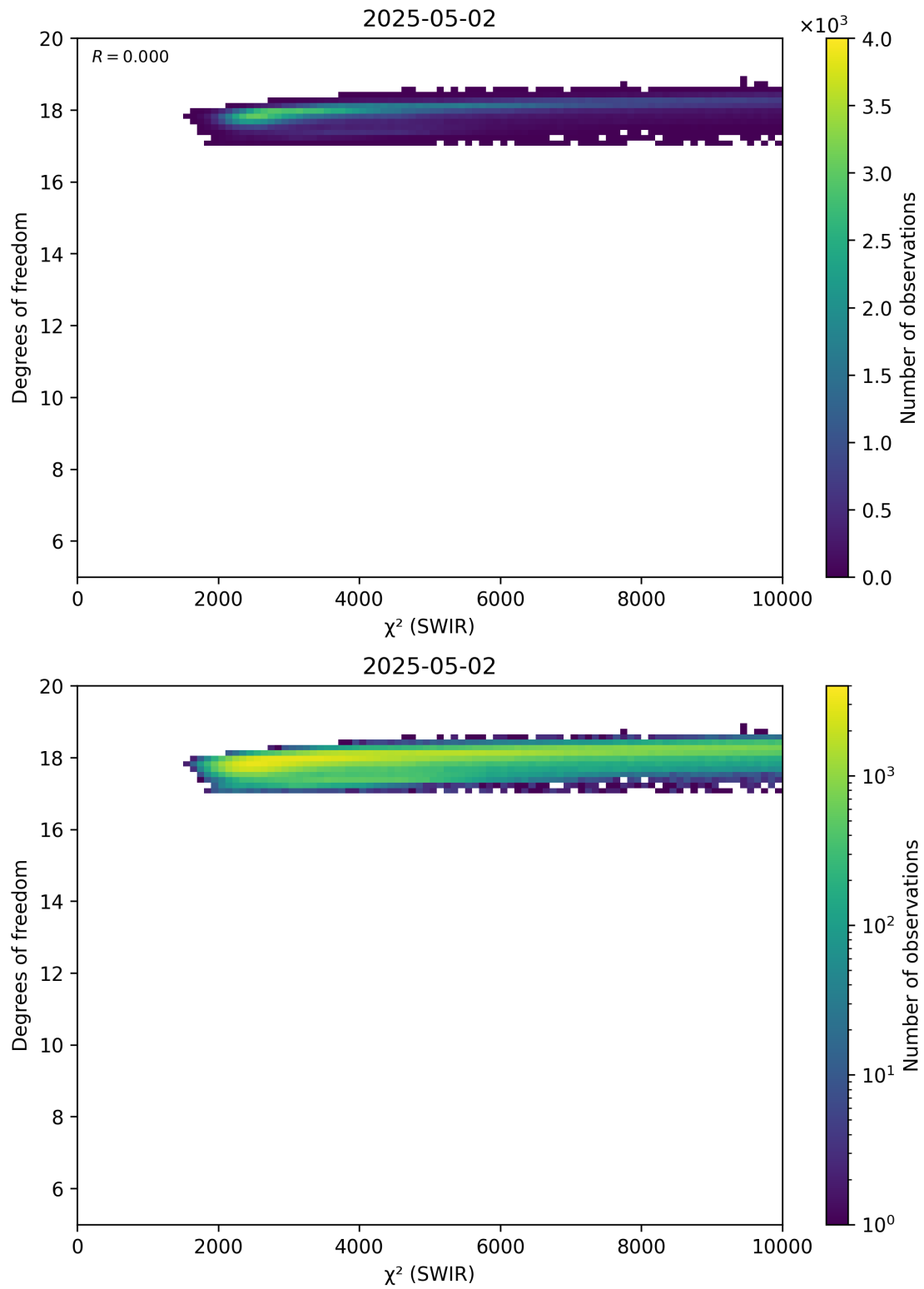
Figure 48: Scatter density plot of “ \chi^2 (SWIR)” against “Degrees of freedom” for 2025-05-01 to 2025-05-03.
