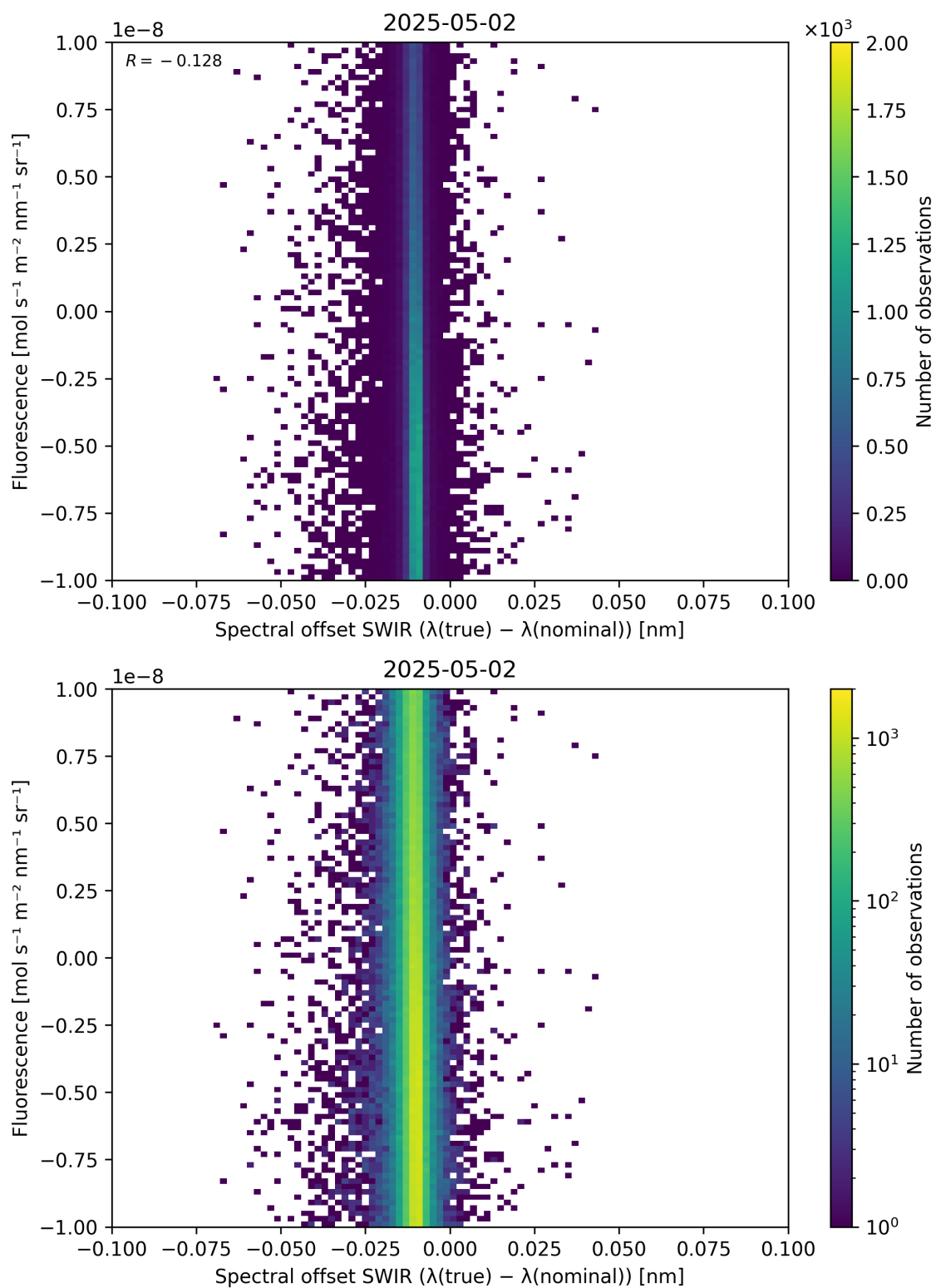
Figure 120: Scatter density plot of “Spectral offset SWIR ( \lambda_{\text{true}} - \lambda_{\text{nominal}} )” against “Fluorescence” for 2025-05-01 to 2025-05-03.
