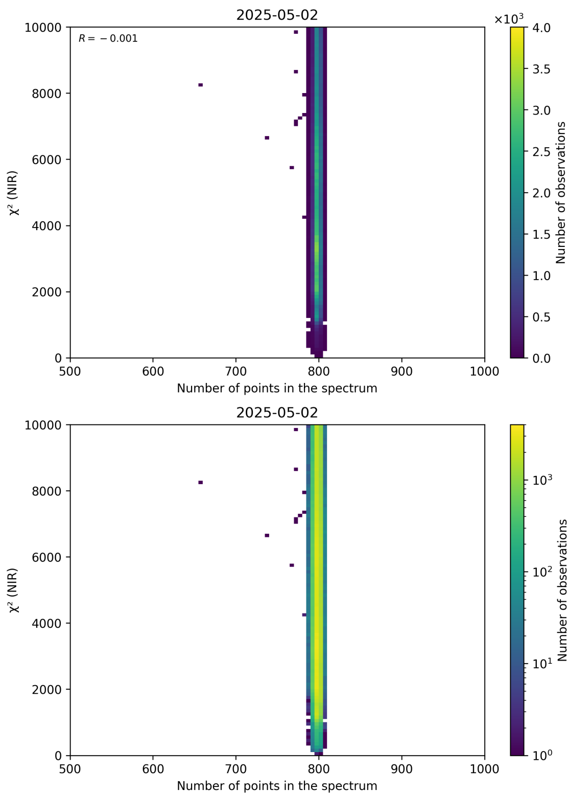
Figure 88: Scatter density plot of “Number of points in the spectrum” against “ \chi^2 (NIR)” for 2025-05-01 to 2025-05-03.
