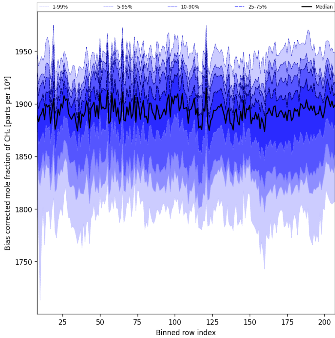
Figure 36: Along track statistics of “Bias corrected mole fraction of CH 4 ” for 2025-05-01 to 2025-05-03
