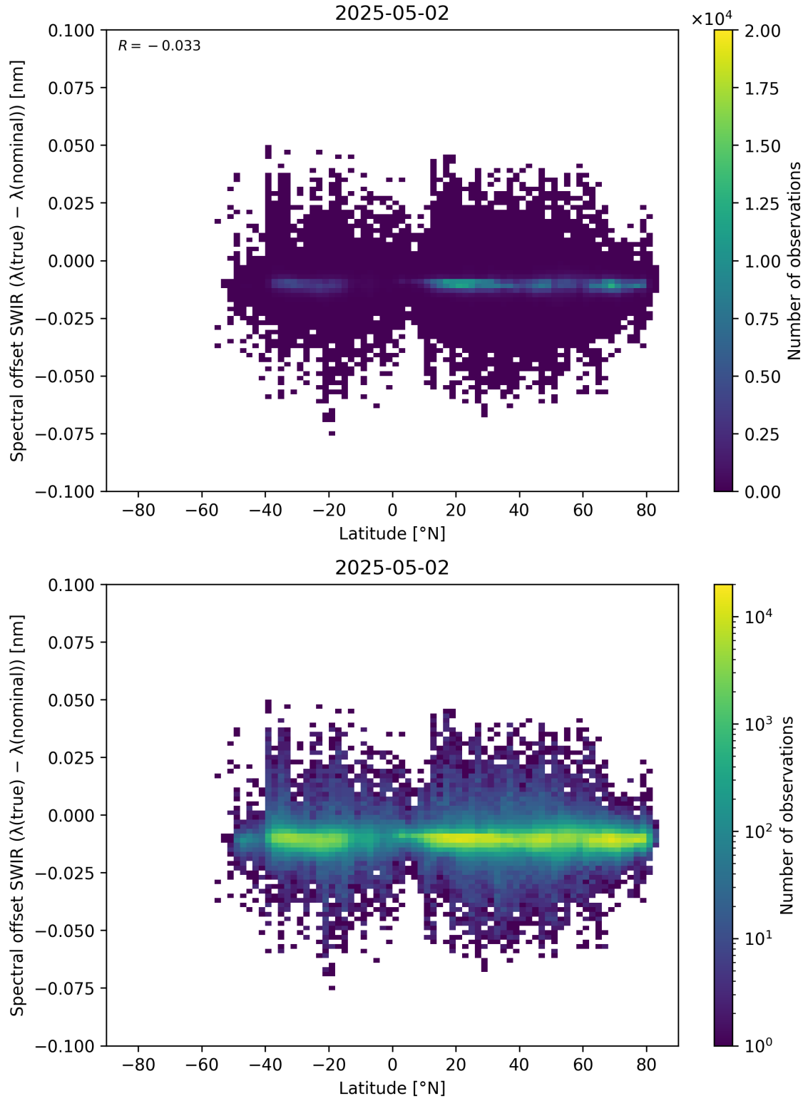
Figure 62: Scatter density plot of “Latitude” against “Spectral offset SWIR ( \lambda_{\text{true}} - \lambda_{\text{nominal}} )” for 2025-05-01 to 2025-05-03.
