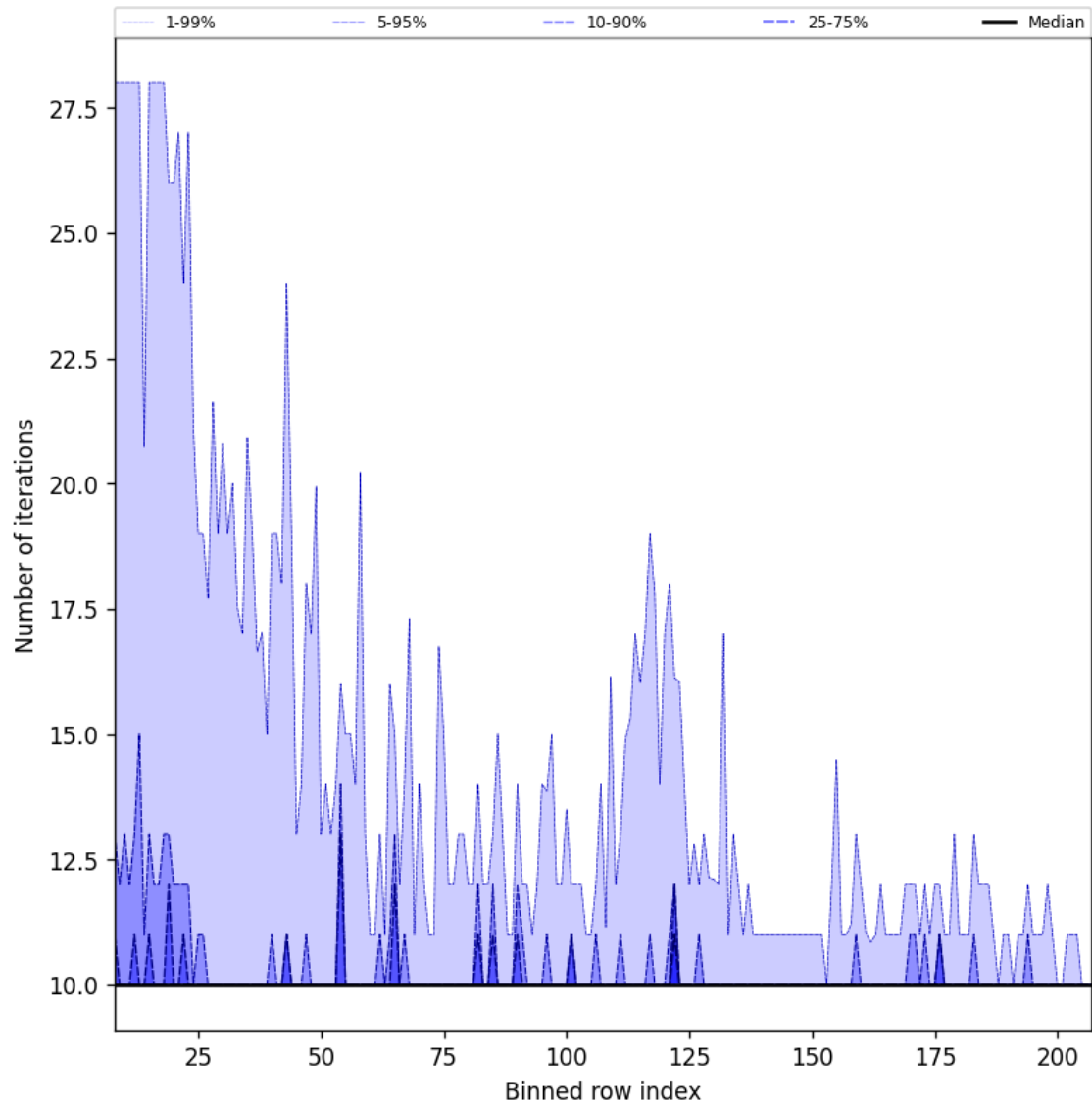
Figure 42: Along track statistics of “Number of iterations” for 2025-05-01 to 2025-05-03
