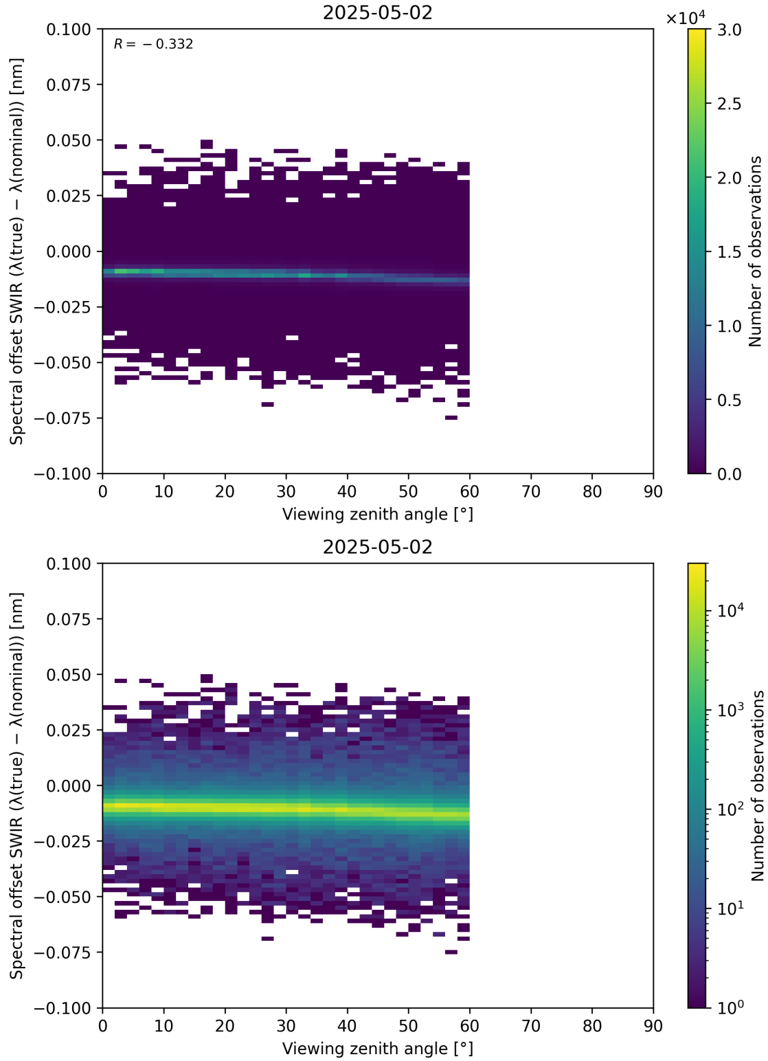
Figure 116: Scatter density plot of “Viewing zenith angle” against “Spectral offset SWIR ( \lambda_{\text{true}} - \lambda_{\text{nominal}} )” for 2025-05-01 to 2025-05-03.
