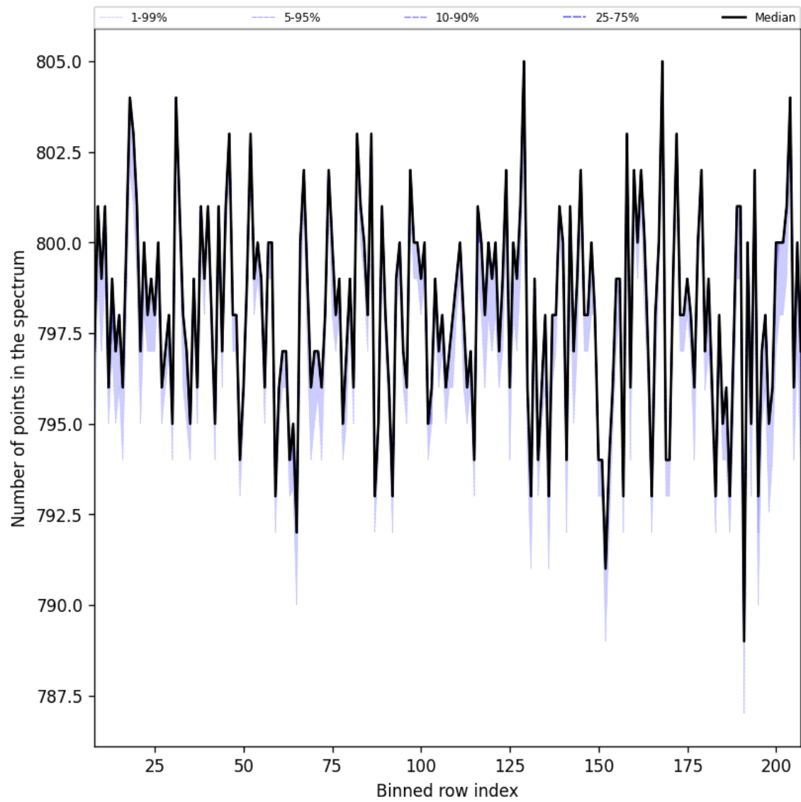
Figure 37: Along track statistics of “Number of points in the spectrum” for 2025-05-01 to 2025-05-03
