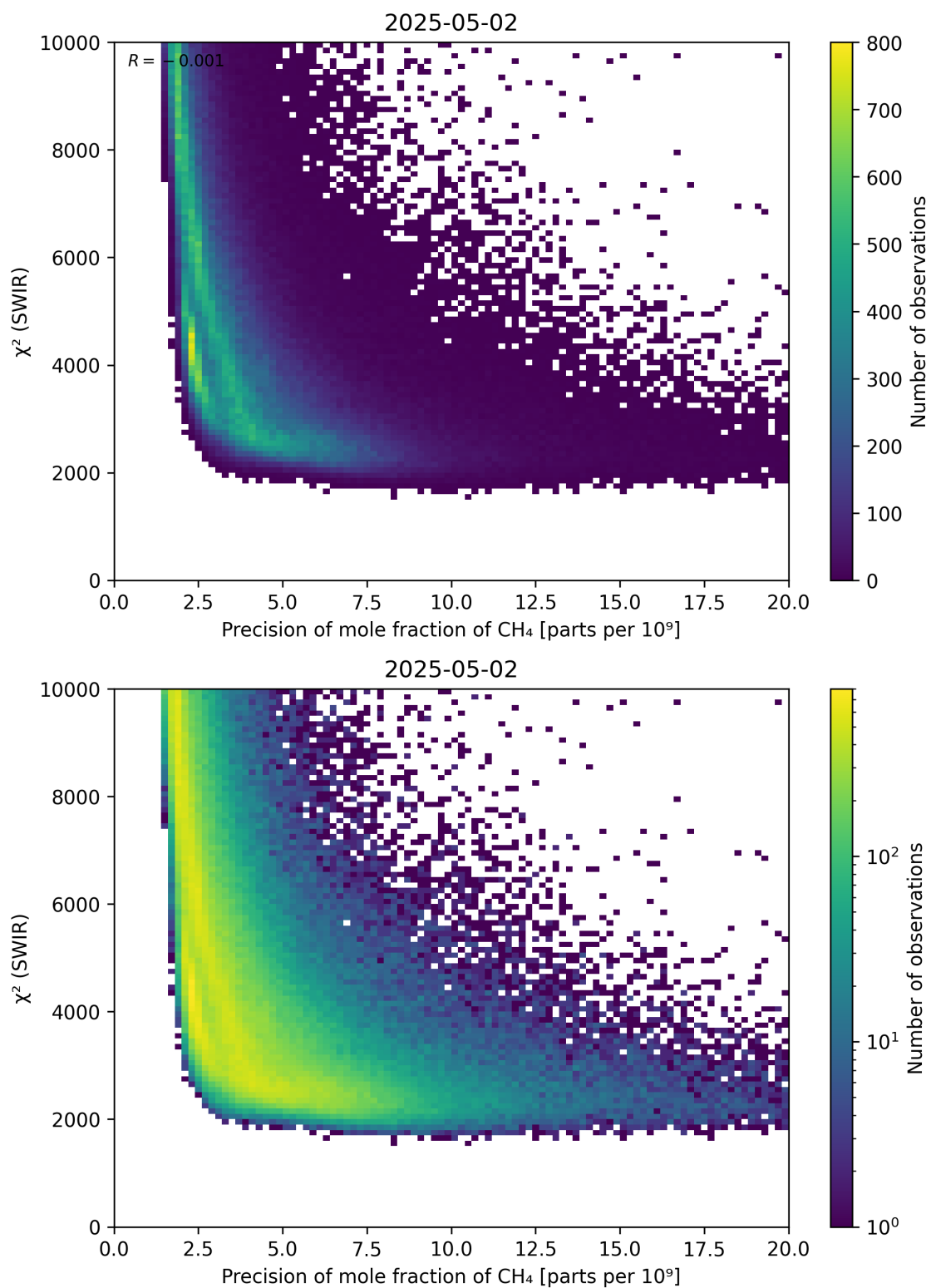
Figure 79: Scatter density plot of “Precision of mole fraction of CH 4 ” against “ \chi^2 (SWIR)” for 2025-05-01 to 2025-05-03.
