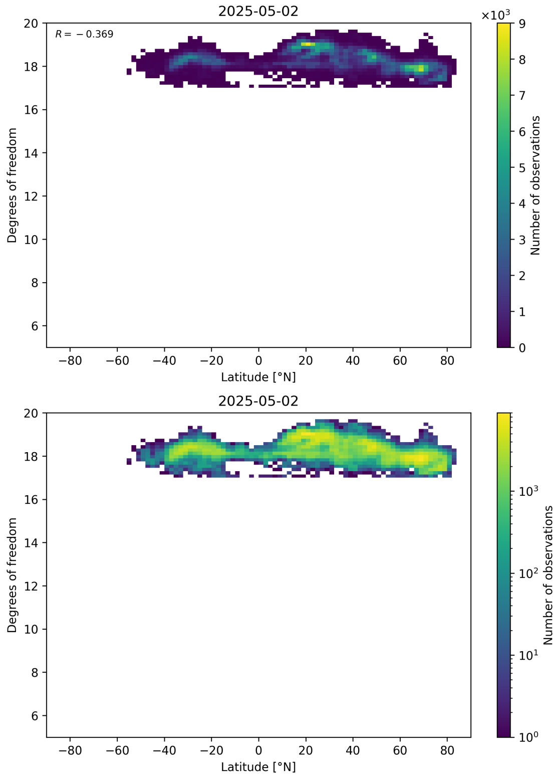
Figure 55: Scatter density plot of “Latitude” against “Degrees of freedom” for 2025-05-01 to 2025-05-03.
