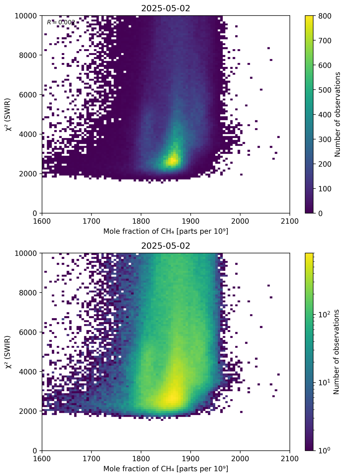
Figure 71: Scatter density plot of “Mole fraction of CH 4 ” against “ \chi^2 (SWIR)” for 2025-05-01 to 2025-05-03.
