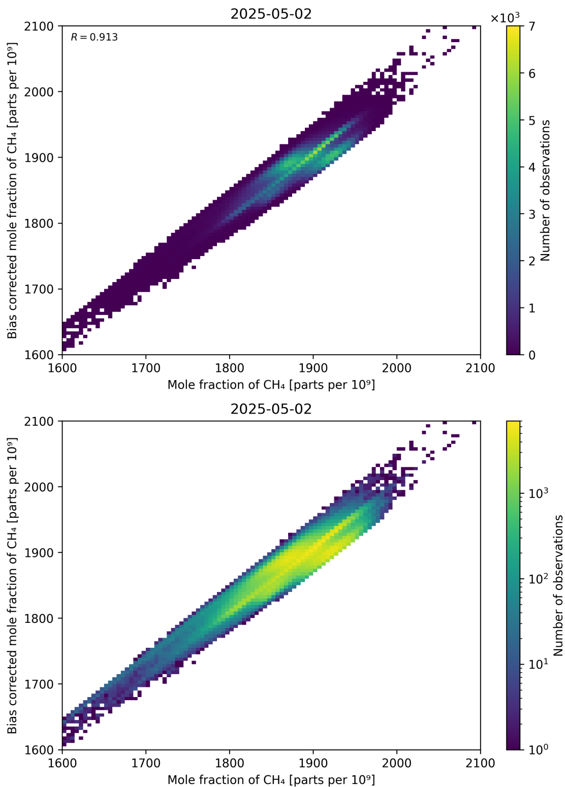
Figure 74: Scatter density plot of “Mole fraction of CH 4 ” against “Bias corrected mole fraction of CH 4 ” for 2025-05-01 to 2025-05-03.
