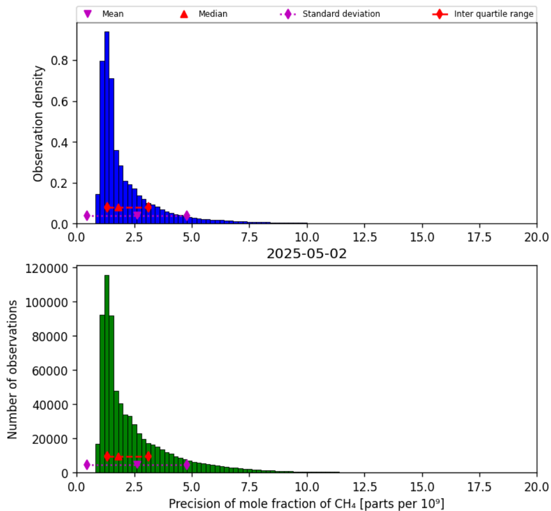
Figure 24: Histogram of “Precision of mole fraction of CH 4 ” for 2025-05-01 to 2025-05-03
