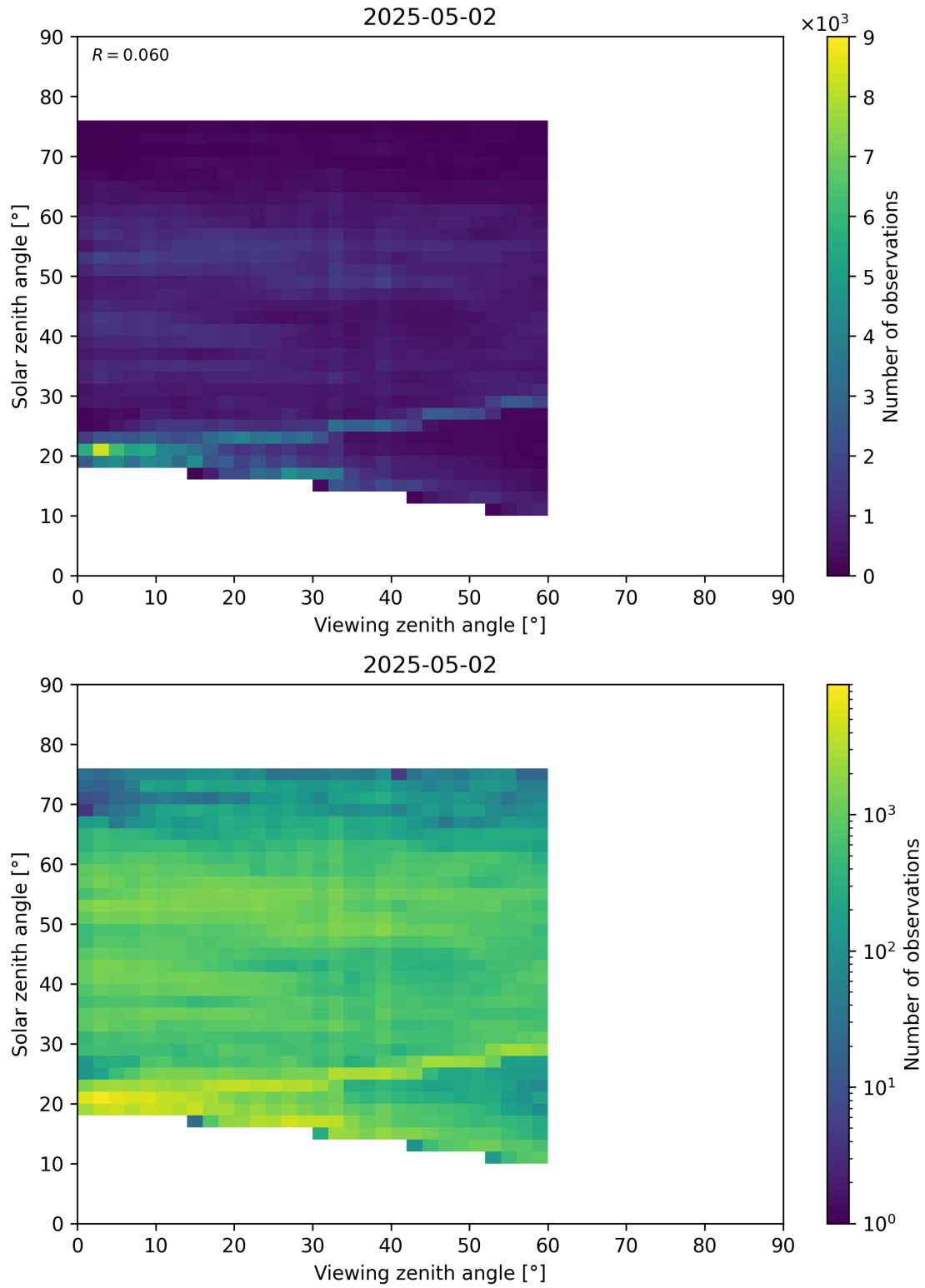
Figure 115: Scatter density plot of “Viewing zenith angle” against “Solar zenith angle” for 2025-05-01 to 2025-05-03.
