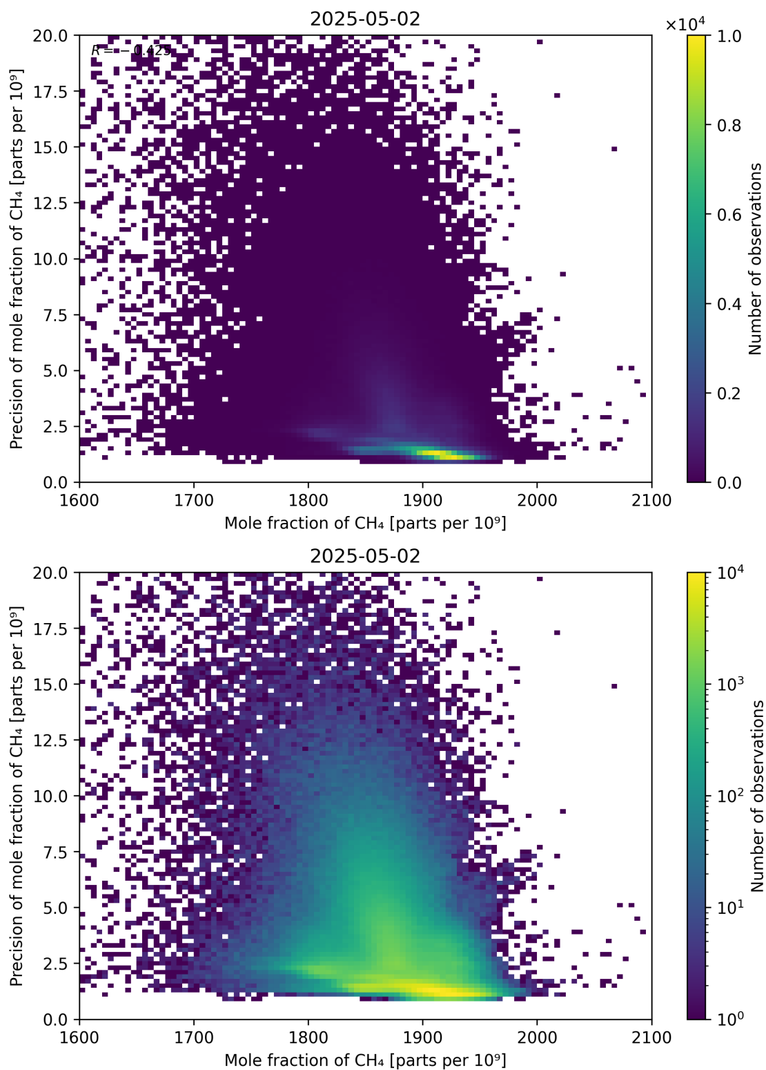
Figure 75: Scatter density plot of “Mole fraction of CH 4 ” against “Precision of mole fraction of CH 4 ” for 2025-05-01 to 2025-05-03.
