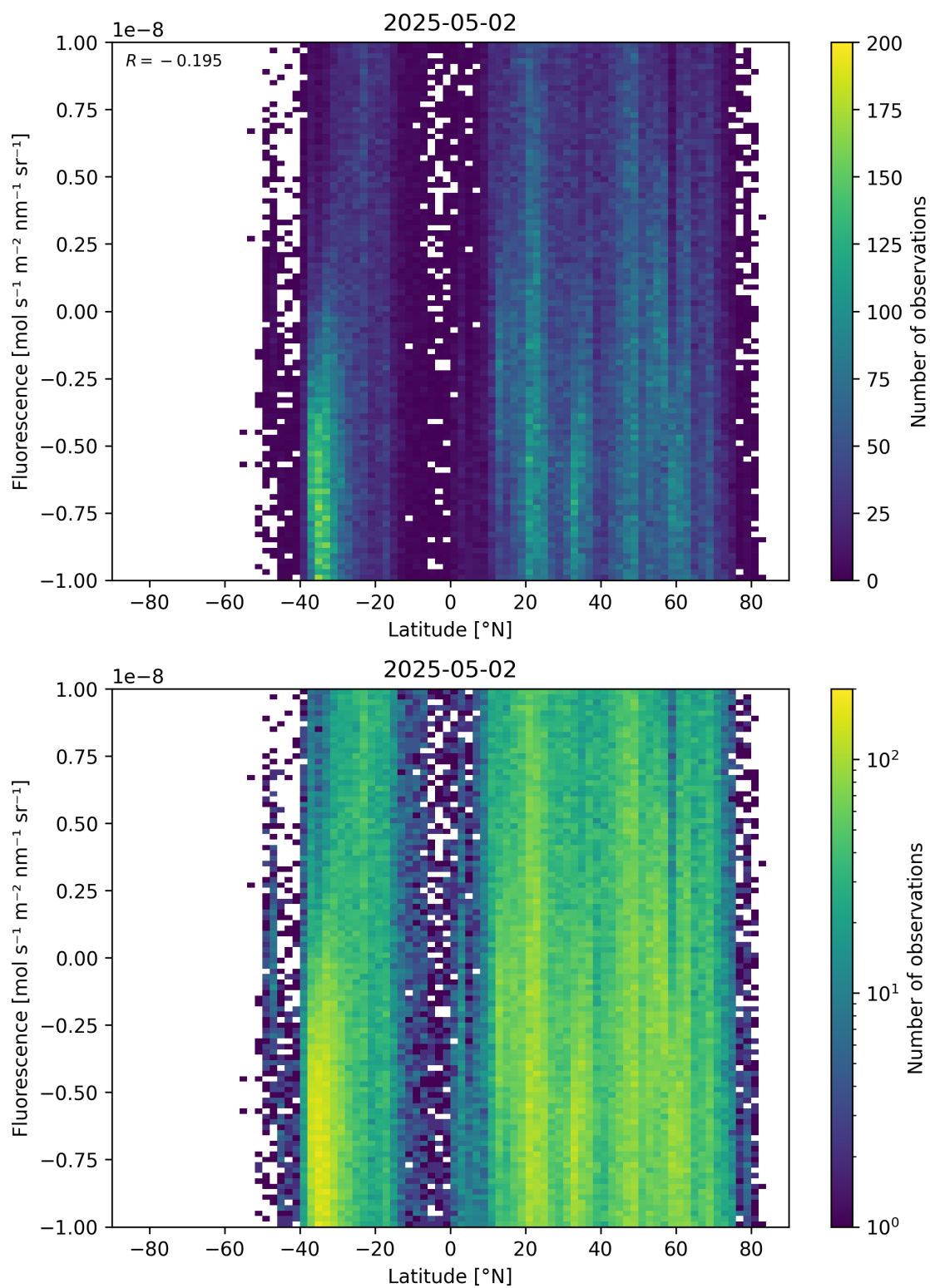
Figure 56: Scatter density plot of “Latitude” against “Fluorescence” for 2025-05-01 to 2025-05-03.
