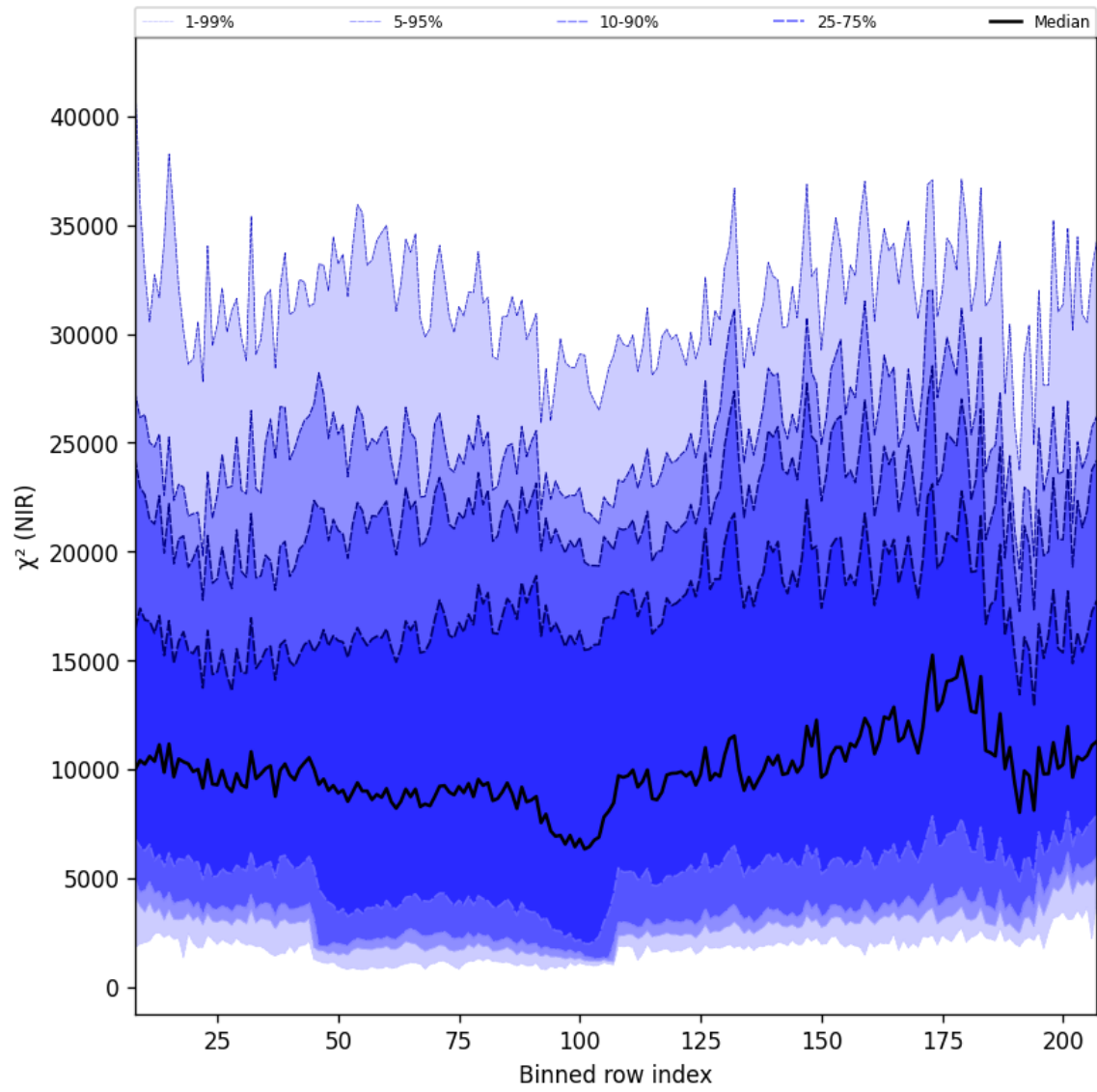
Figure 40: Along track statistics of “ \chi^2 (NIR)” for 2025-05-01 to 2025-05-03
