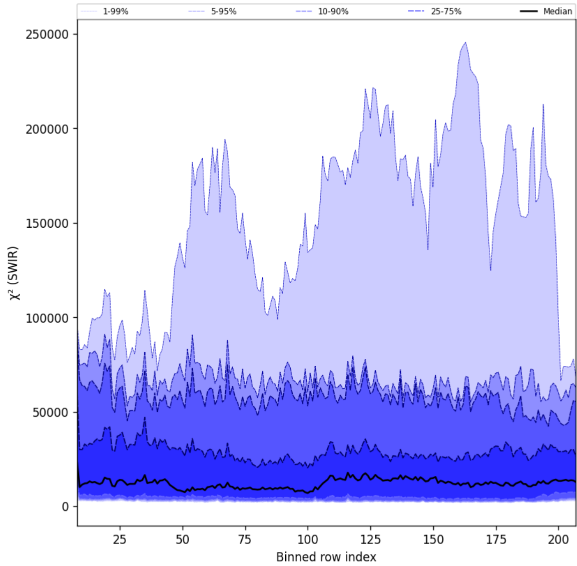
Figure 39: Along track statistics of " \chi^2 (SWIR)" for 2025-05-01 to 2025-05-03
