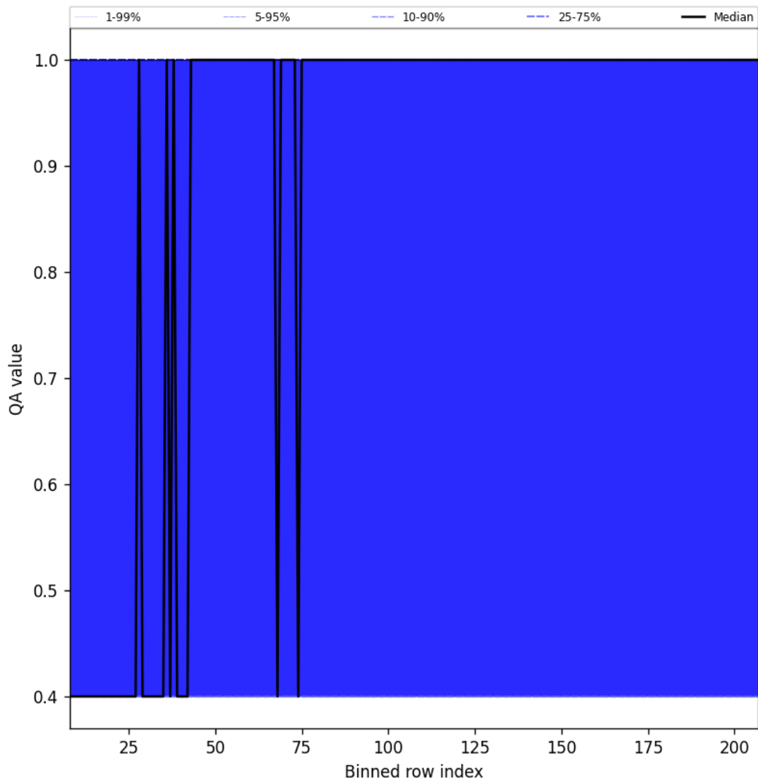
Figure 33: Along track statistics of “QA value” for 2025-05-01 to 2025-05-03
