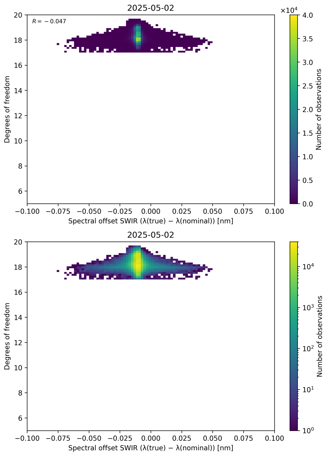
Figure 119: Scatter density plot of “Spectral offset SWIR ( \lambda_{\text{true}} - \lambda_{\text{nominal}} )” against “Degrees of freedom” for 2025-05-01 to 2025-05-03.
