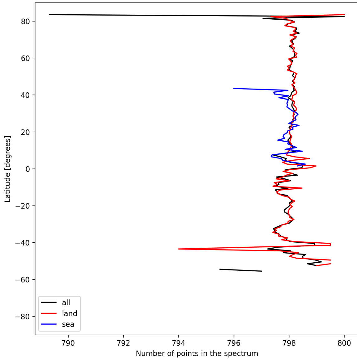
Figure 15: Zonal average of “Number of points in the spectrum” for 2025-05-01 to 2025-05-03.
