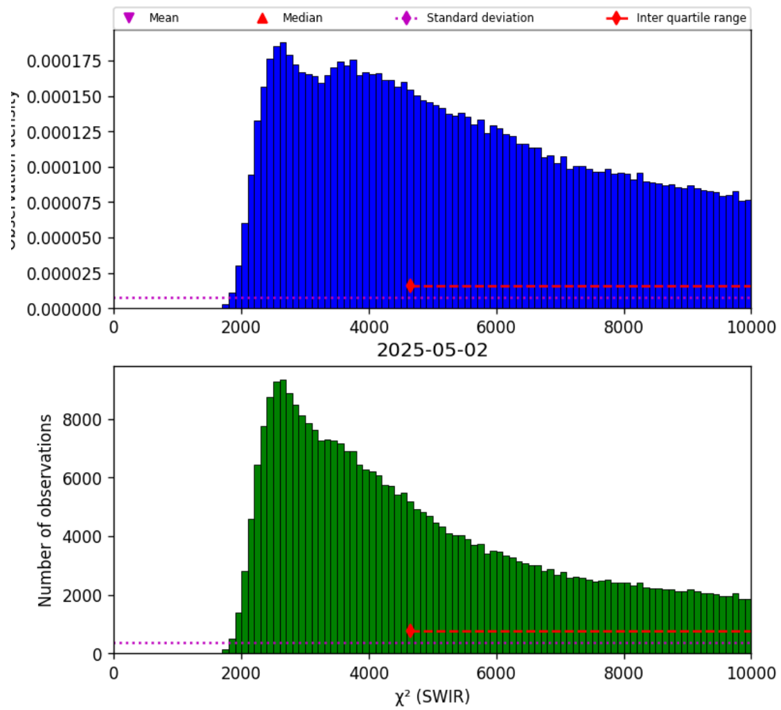
Figure 28: Histogram of “ \chi^2 (SWIR)” for 2025-05-01 to 2025-05-03
