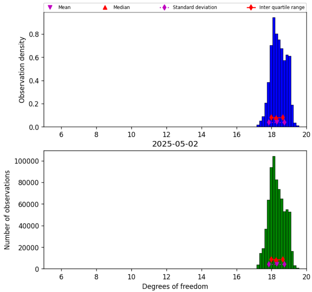
Figure 30: Histogram of “Degrees of freedom” for 2025-05-01 to 2025-05-03
