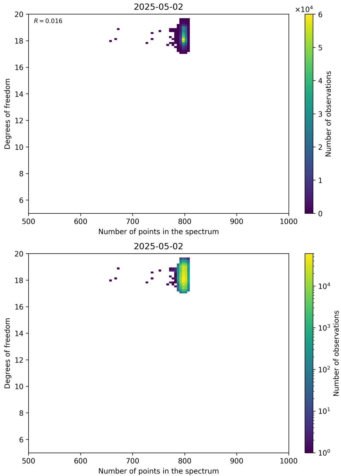
Figure 90: Scatter density plot of “Number of points in the spectrum” against “Degrees of freedom” for 2025-05-01 to 2025-05-03.
