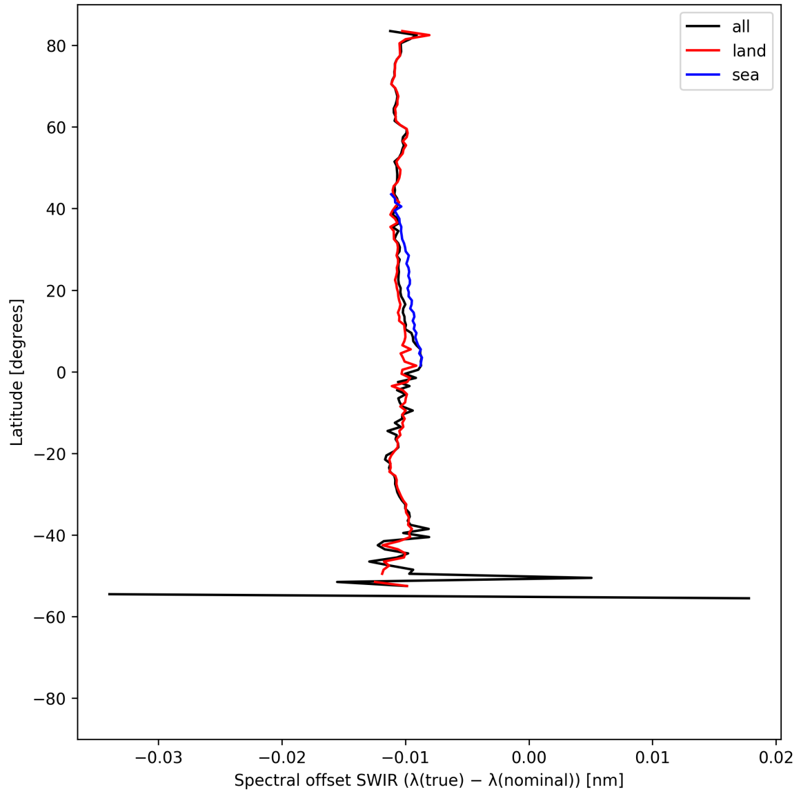
Figure 16: Zonal average of “Spectral offset SWIR ( \lambda_{\text{true}} - \lambda_{\text{nominal}} )” for 2025-05-01 to 2025-05-03.
