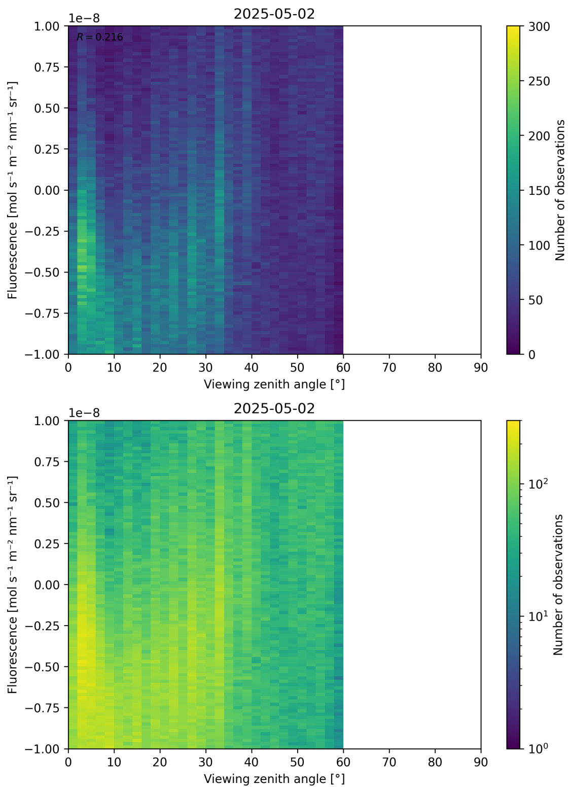
Figure 108: Scatter density plot of “Viewing zenith angle” against “Fluorescence” for 2025-05-01 to 2025-05-03.
