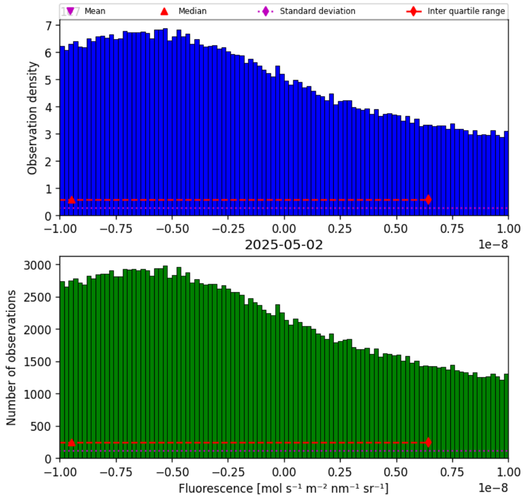
Figure 32: Histogram of “Fluorescence” for 2025-05-01 to 2025-05-03
