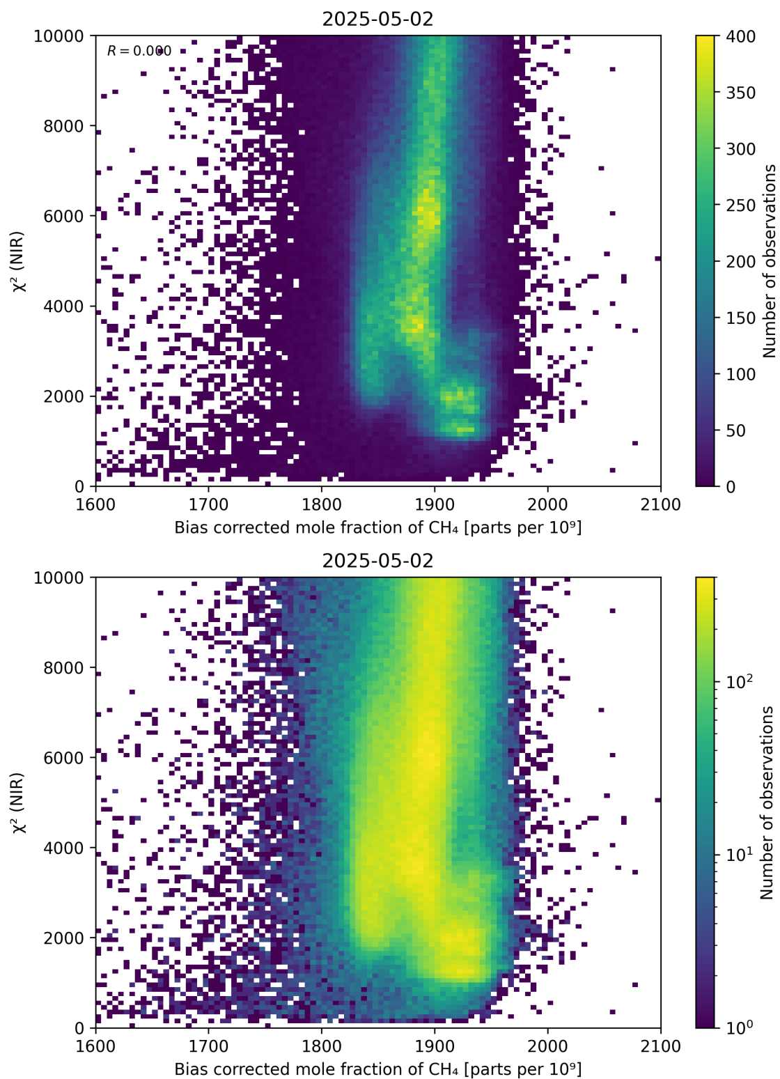
Figure 63: Scatter density plot of “Bias corrected mole fraction of CH 4 ” against “ \chi^2 (NIR)” for 2025-05-01 to 2025-05-03.
