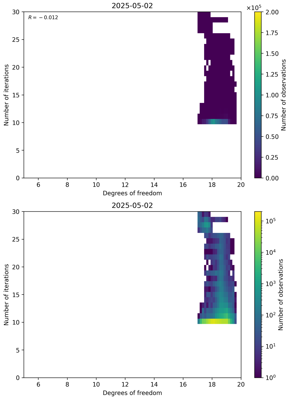
Figure 52: Scatter density plot of “Degrees of freedom” against “Number of iterations” for 2025-05-01 to 2025-05-03.
