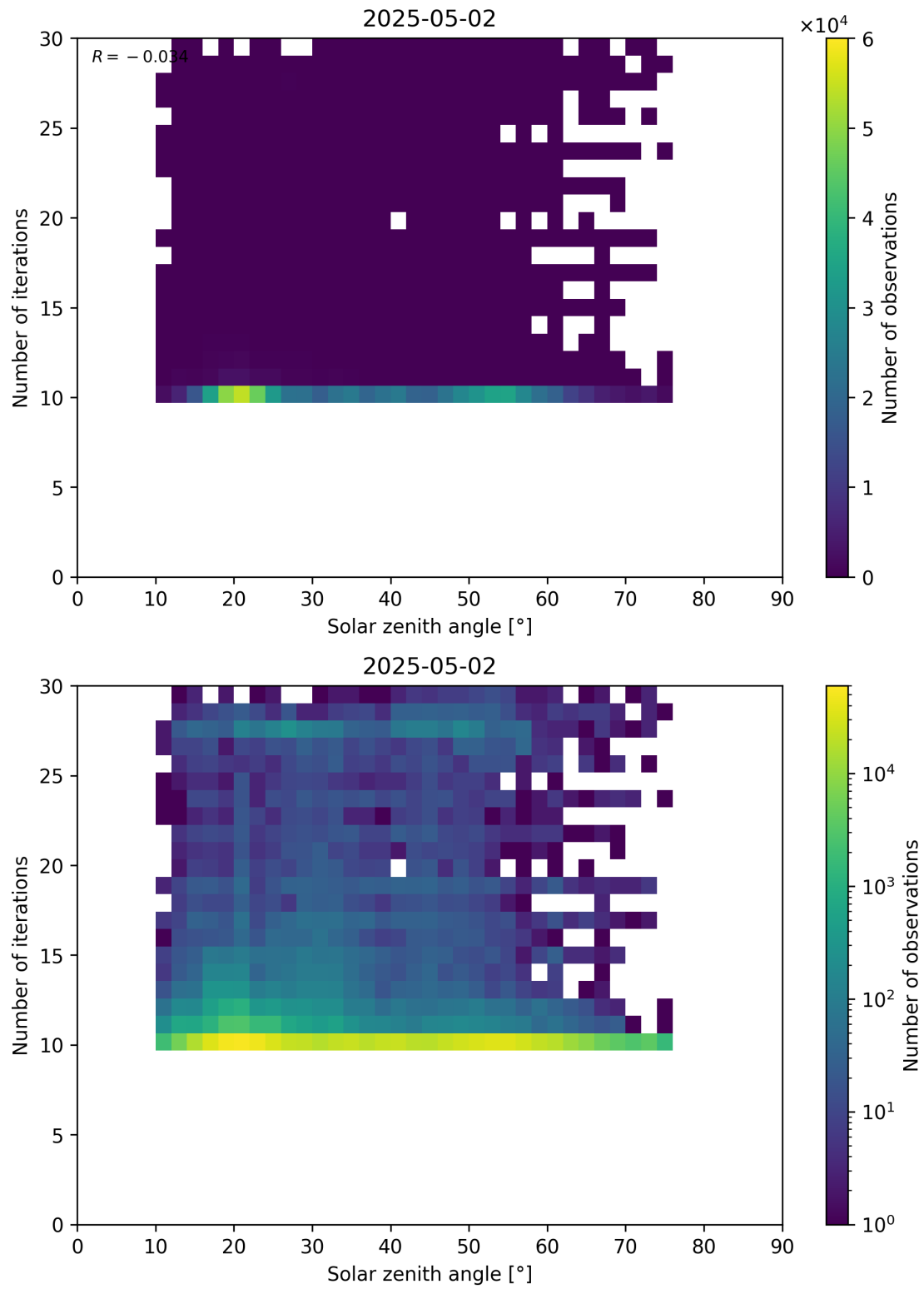
Figure 102: Scatter density plot of “Solar zenith angle” against “Number of iterations” for 2025-05-01 to 2025-05-03.
