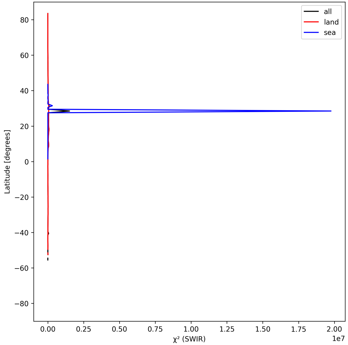
Figure 17: Zonal average of “ \chi^2 (SWIR)” for 2025-05-01 to 2025-05-03.
