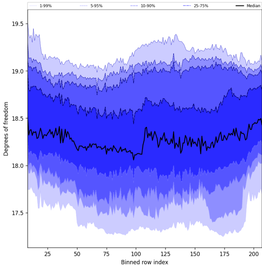
Figure 41: Along track statistics of “Degrees of freedom” for 2025-05-01 to 2025-05-03
