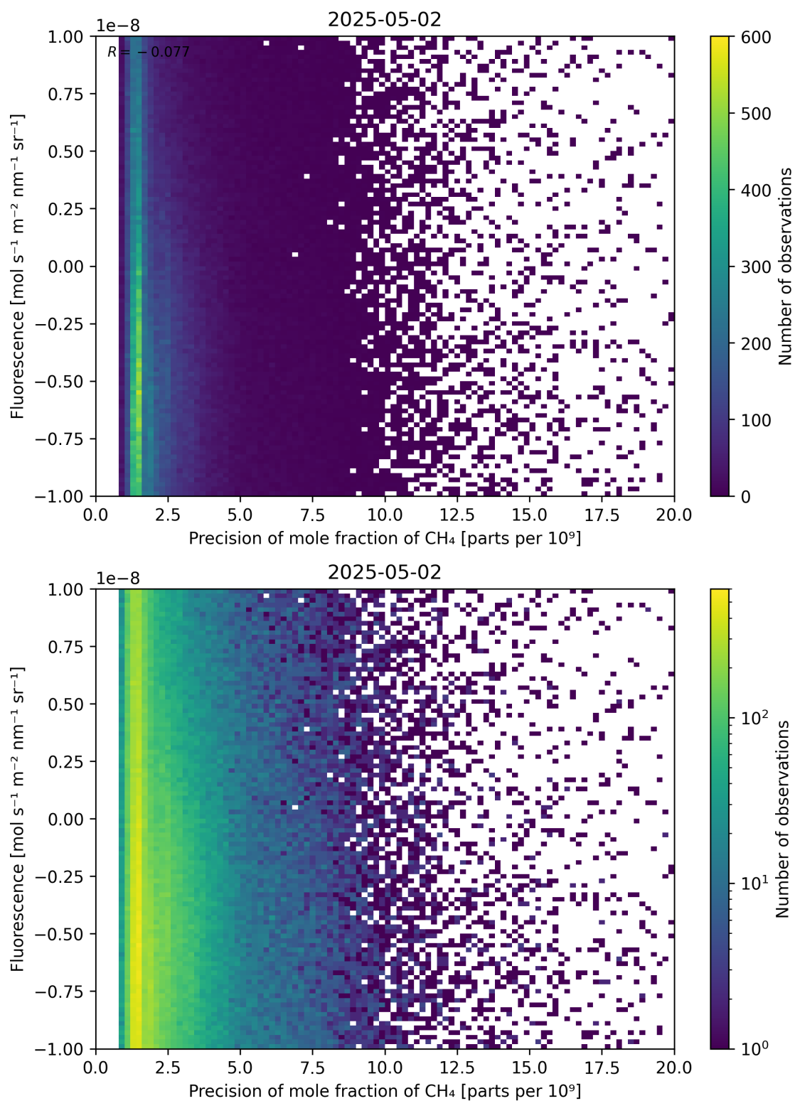
Figure 81: Scatter density plot of “Precision of mole fraction of \text{CH}_4 ” against “Fluorescence” for 2025-05-01 to 2025-05-03.
