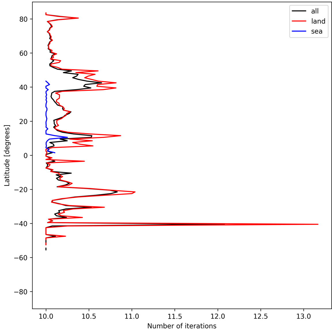
Figure 20: Zonal average of “Number of iterations” for 2025-05-01 to 2025-05-03.
