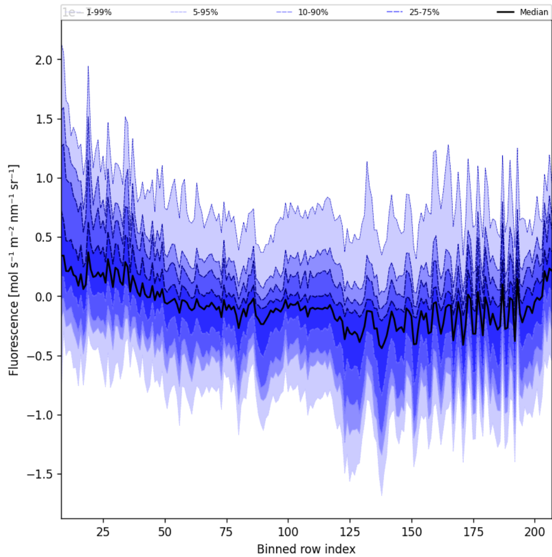
Figure 43: Along track statistics of “Fluorescence” for 2025-05-01 to 2025-05-03
