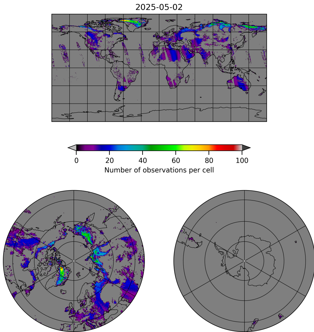
Figure 10: Map of the number of observations for 2025-05-01 to 2025-05-03
