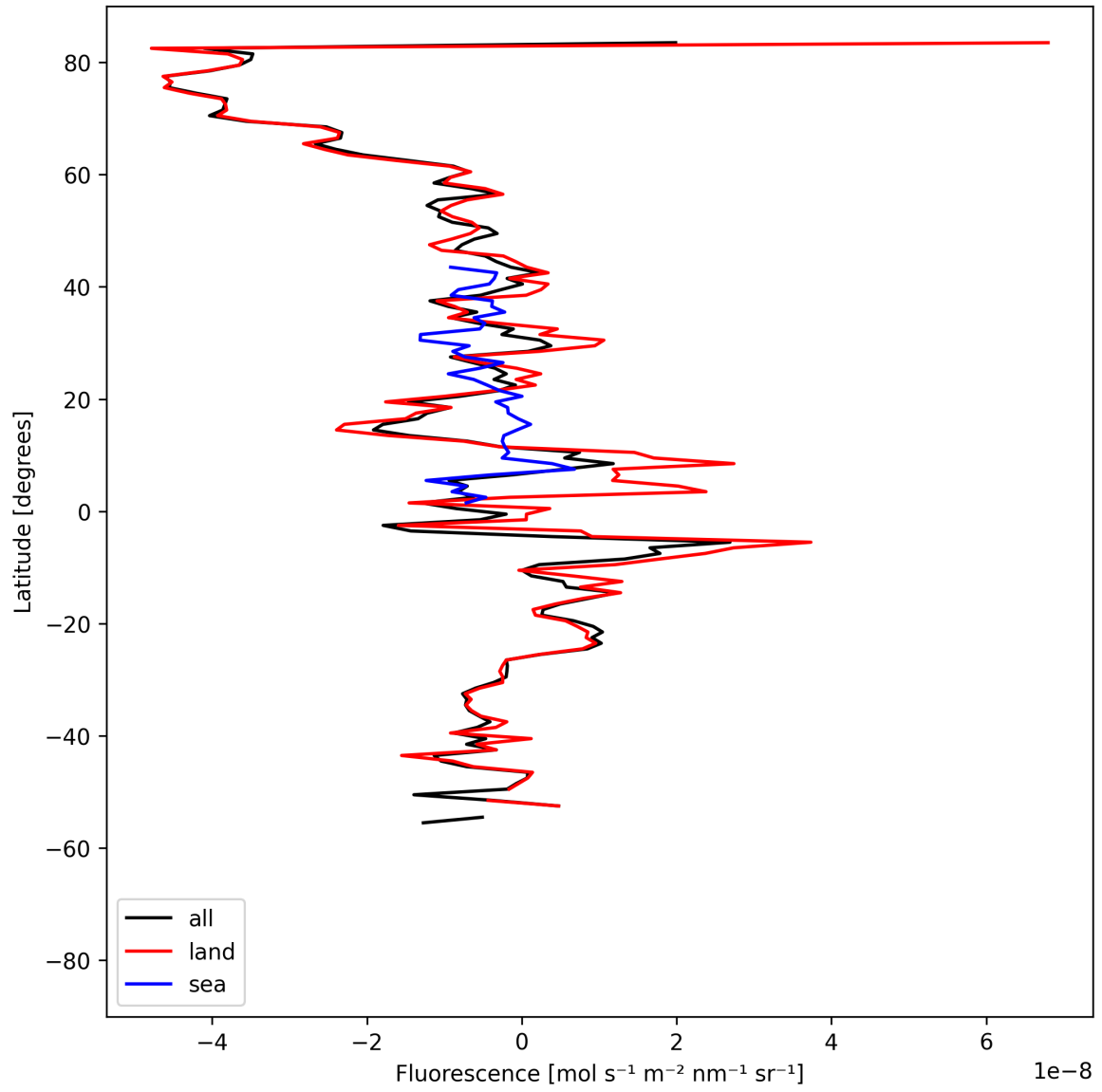
Figure 21: Zonal average of “Fluorescence” for 2025-05-01 to 2025-05-03.
