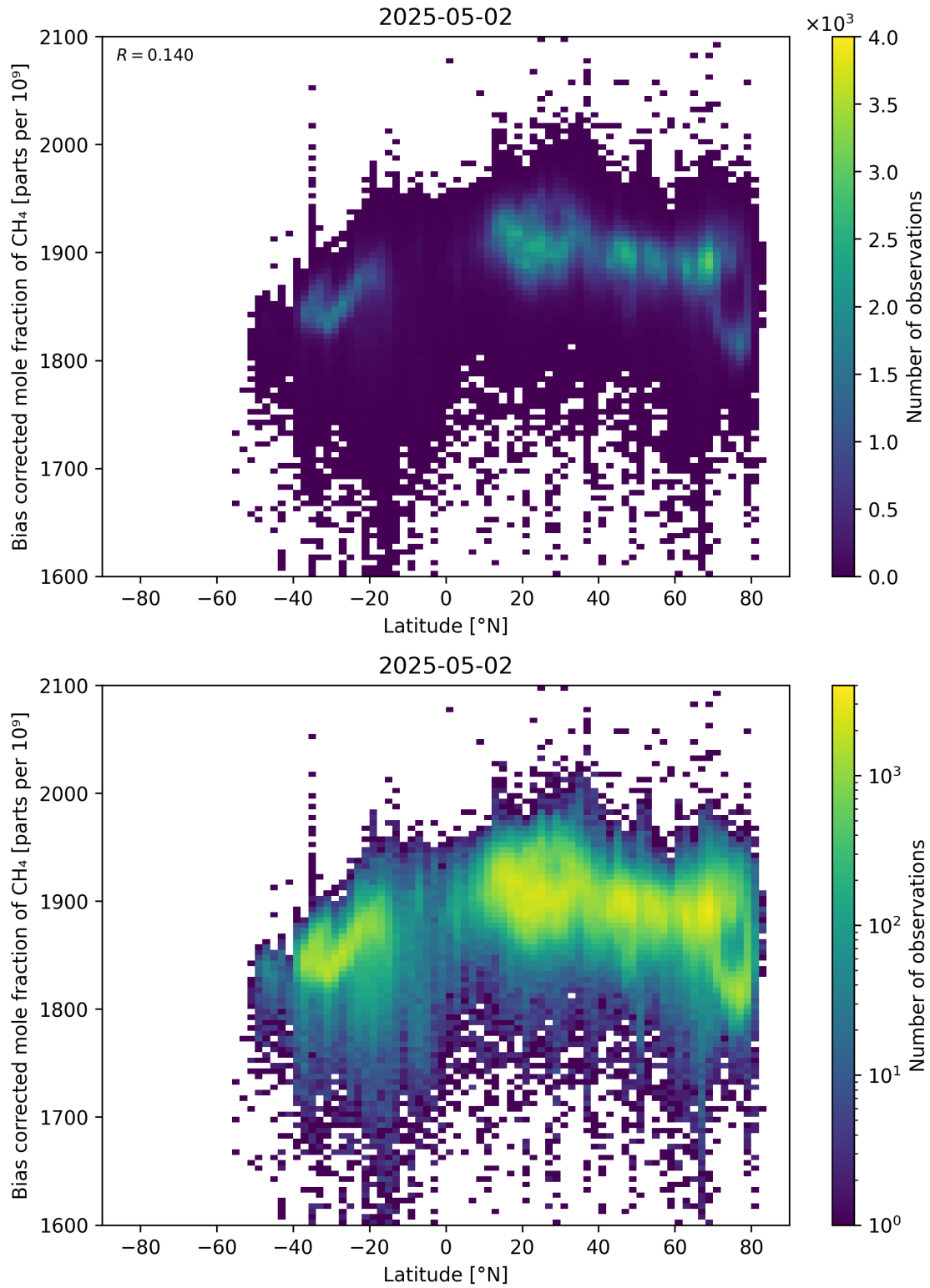
Figure 58: Scatter density plot of “Latitude” against “Bias corrected mole fraction of CH 4 ” for 2025-05-01 to 2025-05-03.
