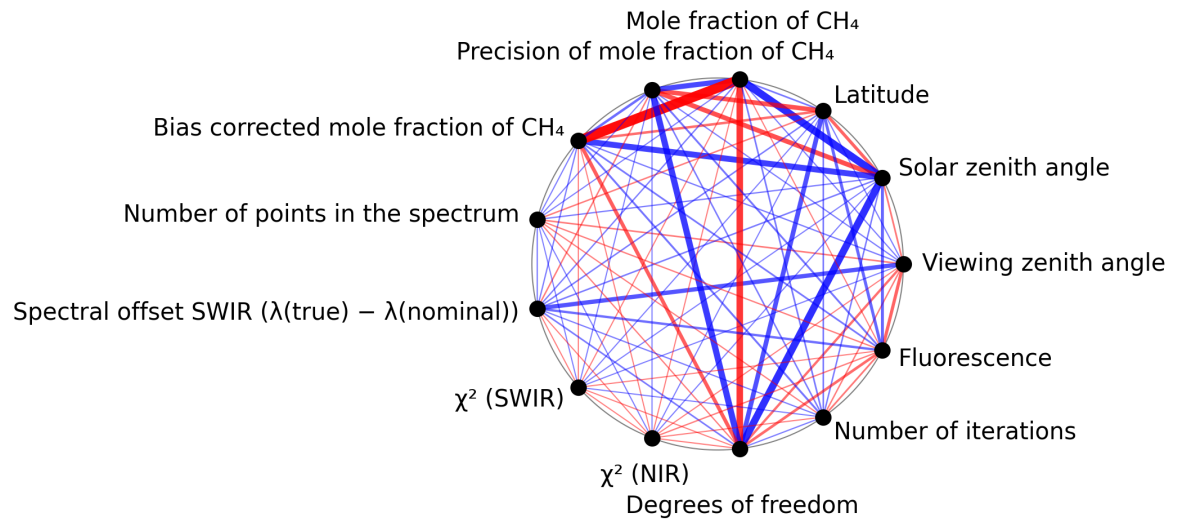
Figure 1: Map of correlation graph for 2025-05-01 to 2025-05-03.
