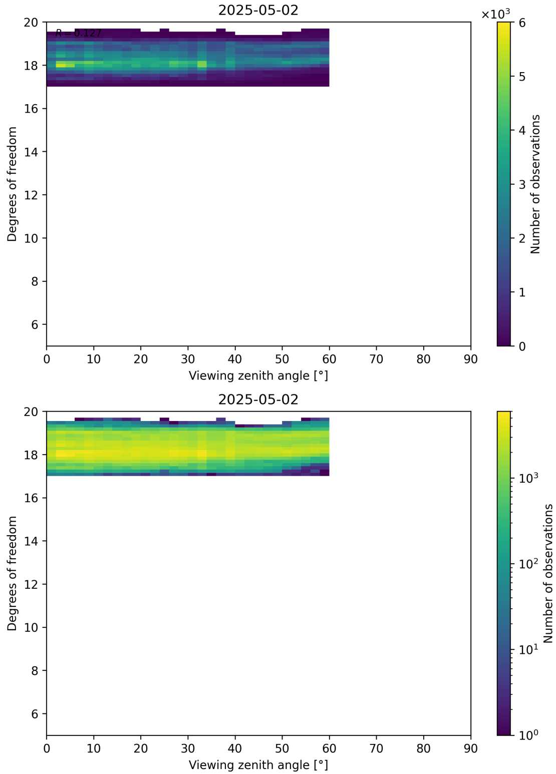
Figure 107: Scatter density plot of “Viewing zenith angle” against “Degrees of freedom” for 2025-05-01 to 2025-05-03.
