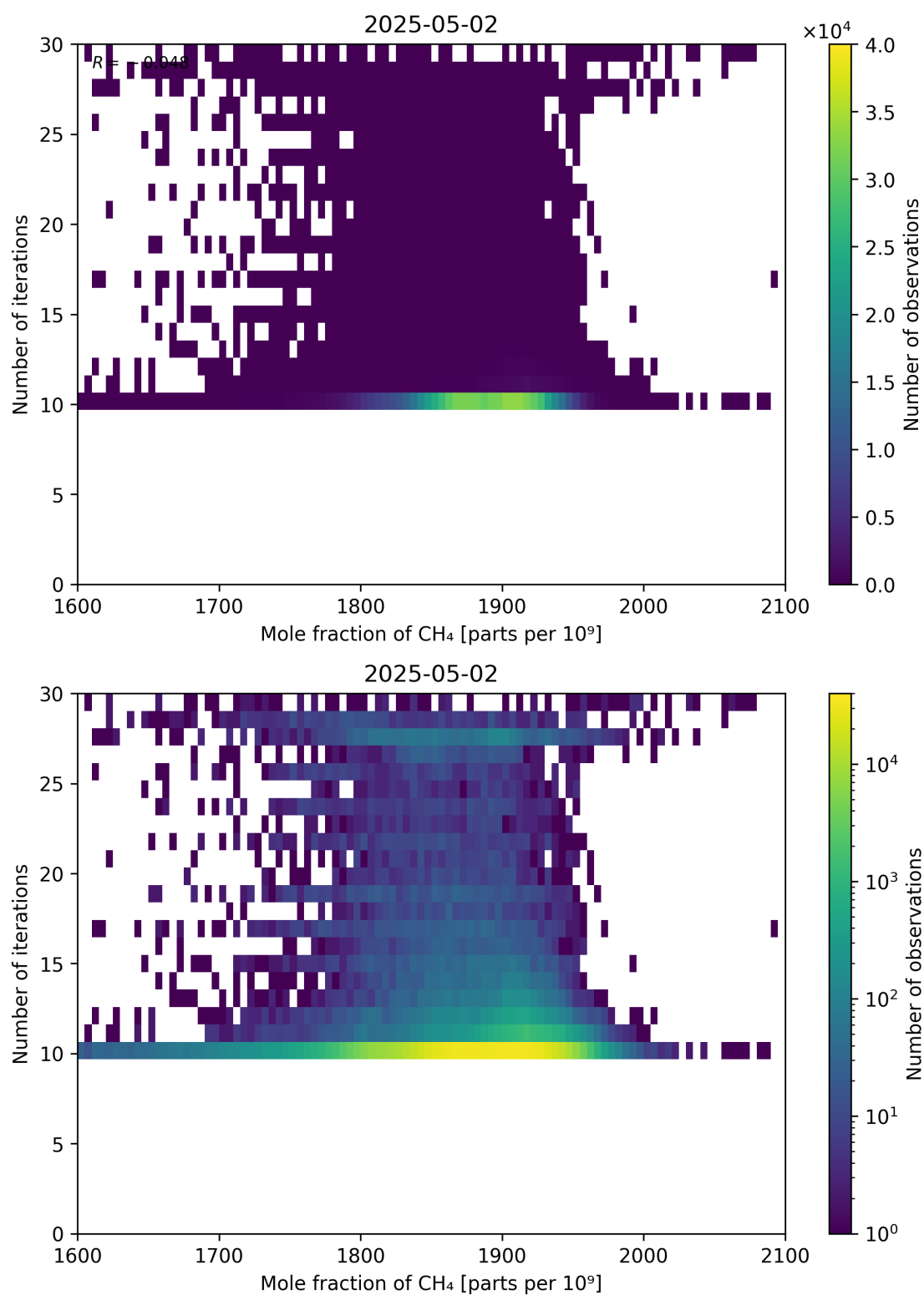
Figure 76: Scatter density plot of “Mole fraction of CH 4 ” against “Number of iterations” for 2025-05-01 to 2025-05-03.
