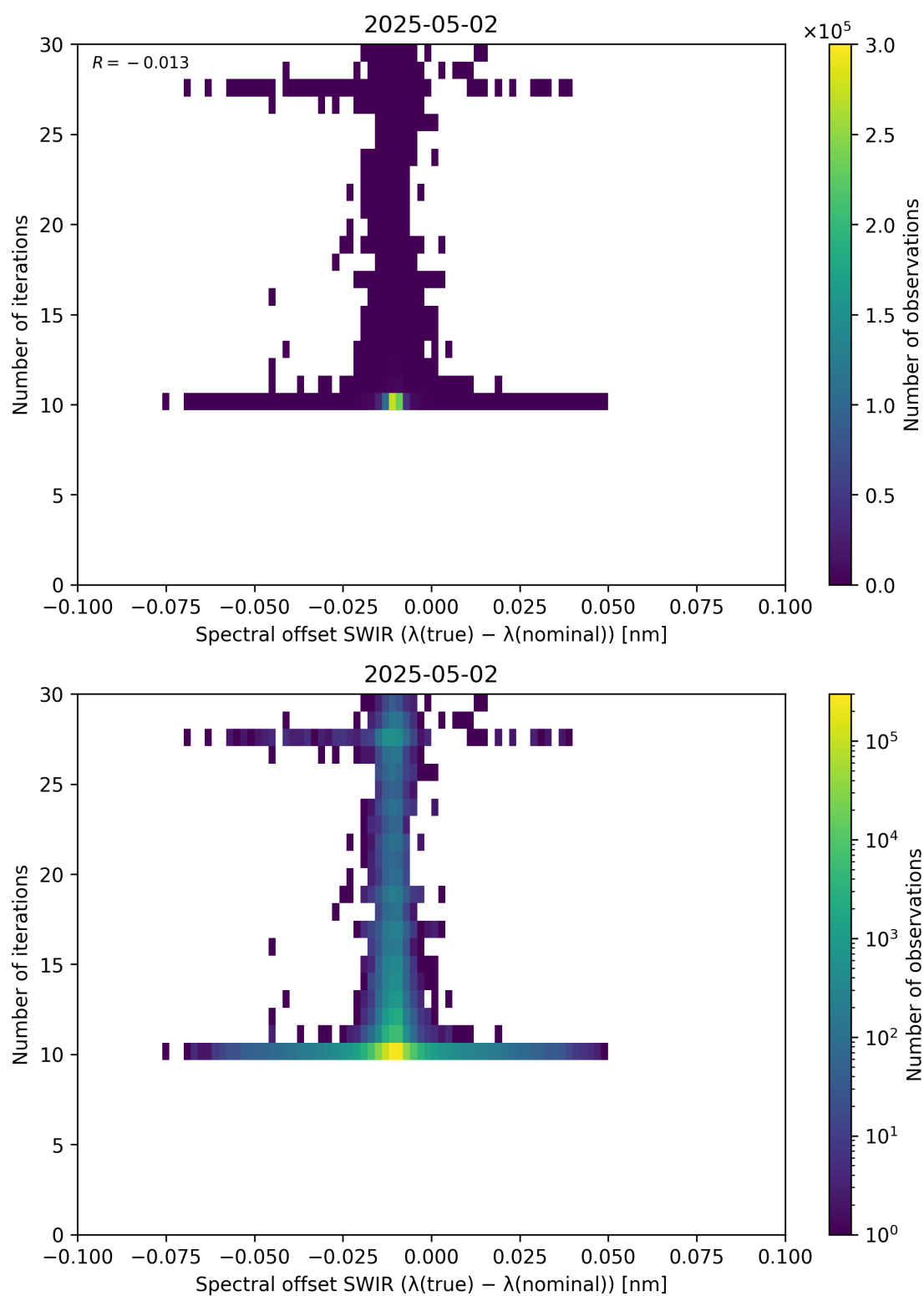
Figure 121: Scatter density plot of “Spectral offset SWIR ( \lambda_{\text{true}} - \lambda_{\text{nominal}} )” against “Number of iterations” for 2025-05-01 to 2025-05-03.
