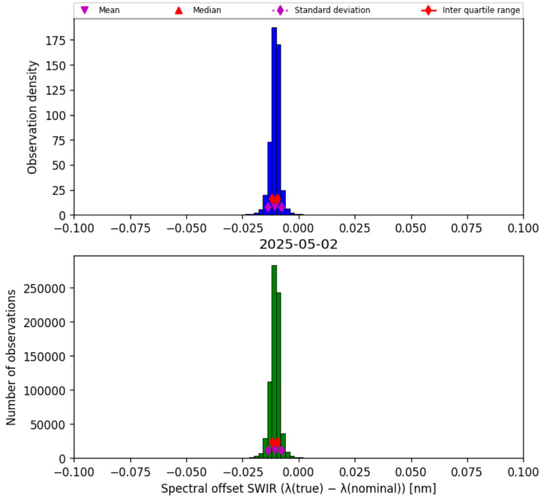
Figure 27: Histogram of “Spectral offset SWIR ( \lambda_{\text{true}} - \lambda_{\text{nominal}} )” for 2025-05-01 to 2025-05-03
