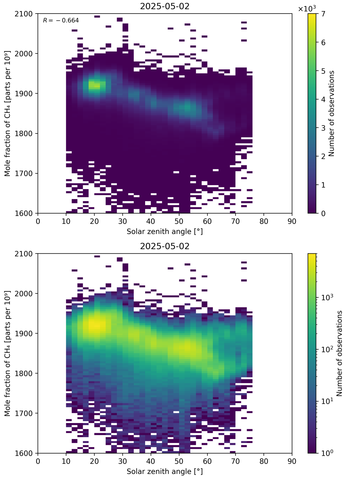
Figure 99: Scatter density plot of “Solar zenith angle” against “Mole fraction of \text{CH}_4 ” for 2025-05-01 to 2025-05-03.
