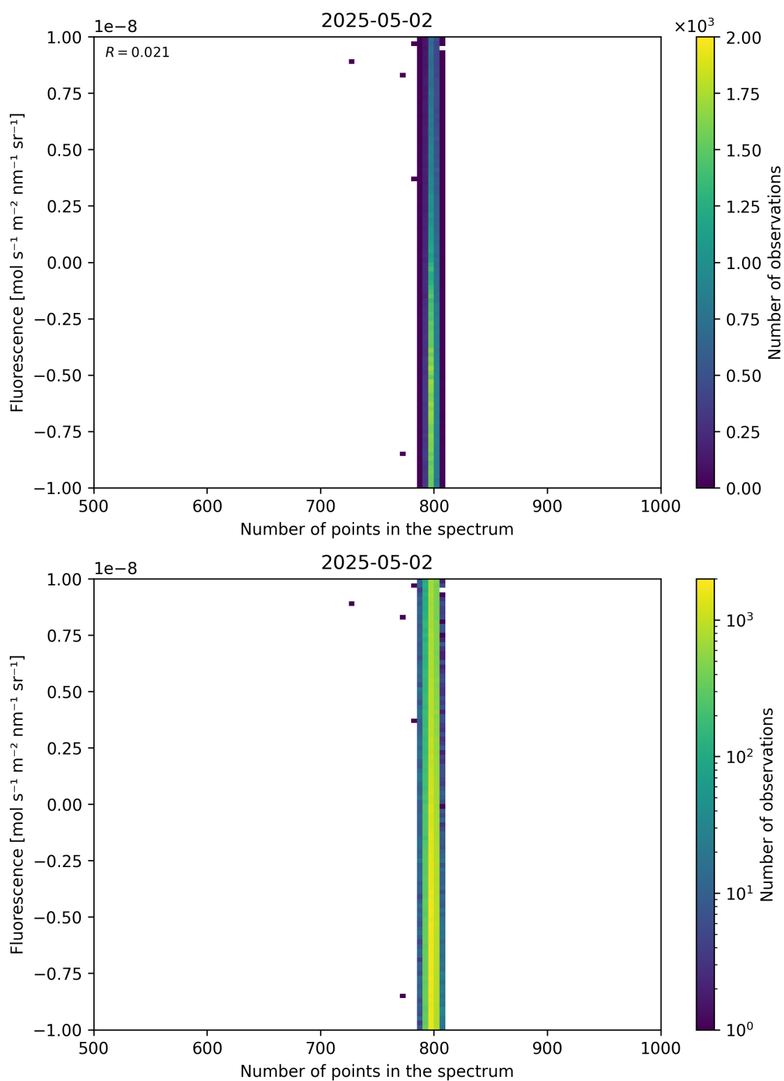
Figure 91: Scatter density plot of “Number of points in the spectrum” against “Fluorescence” for 2025-05-01 to 2025-05-03.
