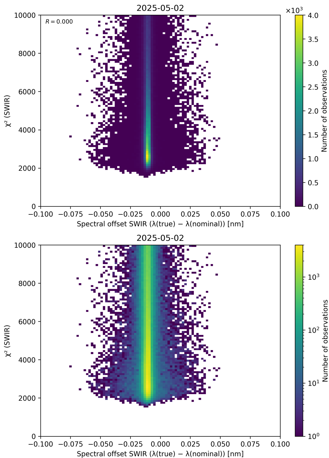
Figure 118: Scatter density plot of “Spectral offset SWIR ( \lambda_{\text{true}} - \lambda_{\text{nominal}} )” against “ \chi^2 (SWIR)” for 2025-05-01 to 2025-05-03.
