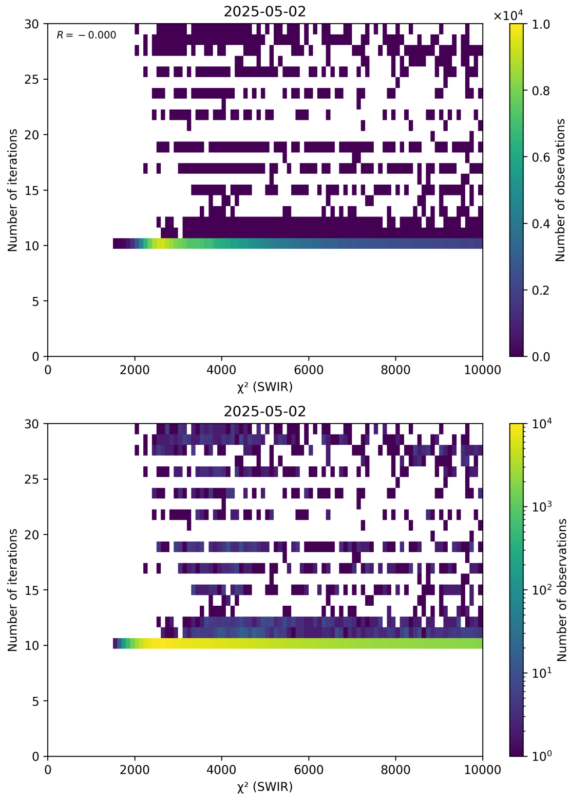
Figure 50: Scatter density plot of “ \chi^2 (SWIR)” against “Number of iterations” for 2025-05-01 to 2025-05-03.
