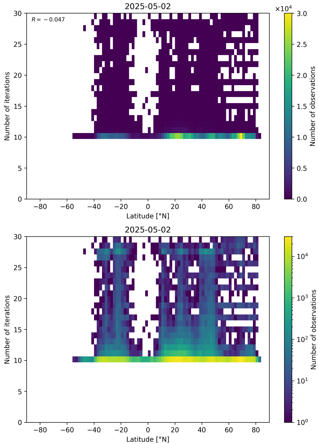
Figure 60: Scatter density plot of “Latitude” against “Number of iterations” for 2025-05-01 to 2025-05-03.
