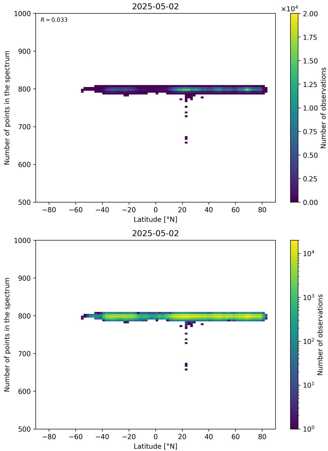
Figure 61: Scatter density plot of “Latitude” against “Number of points in the spectrum” for 2025-05-01 to 2025-05-03.
