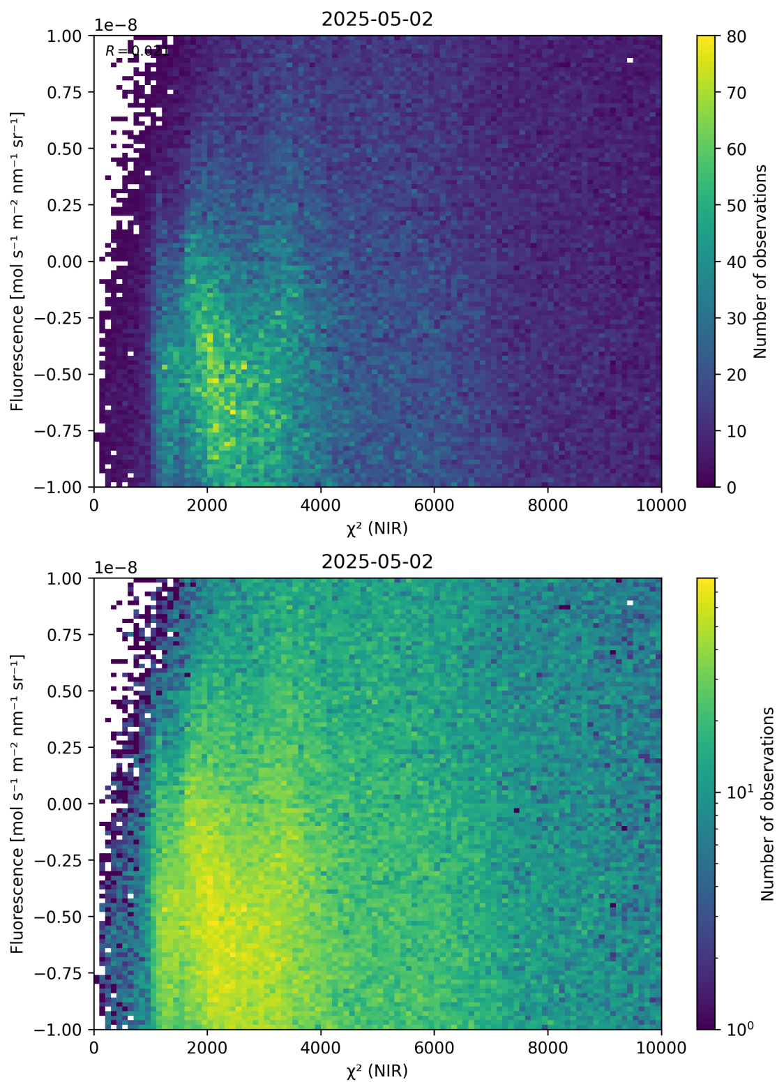
Figure 45: Scatter density plot of “ \chi^2 (NIR)” against “Fluorescence” for 2025-05-01 to 2025-05-03.
