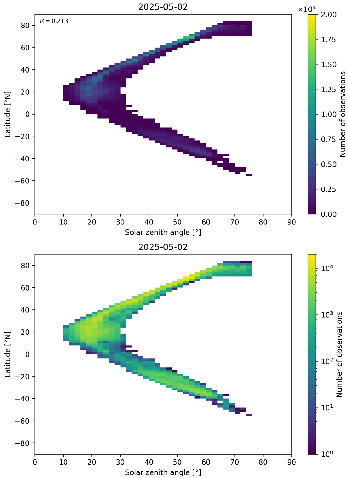
Figure 98: Scatter density plot of “Solar zenith angle” against “Latitude” for 2025-05-01 to 2025-05-03.
