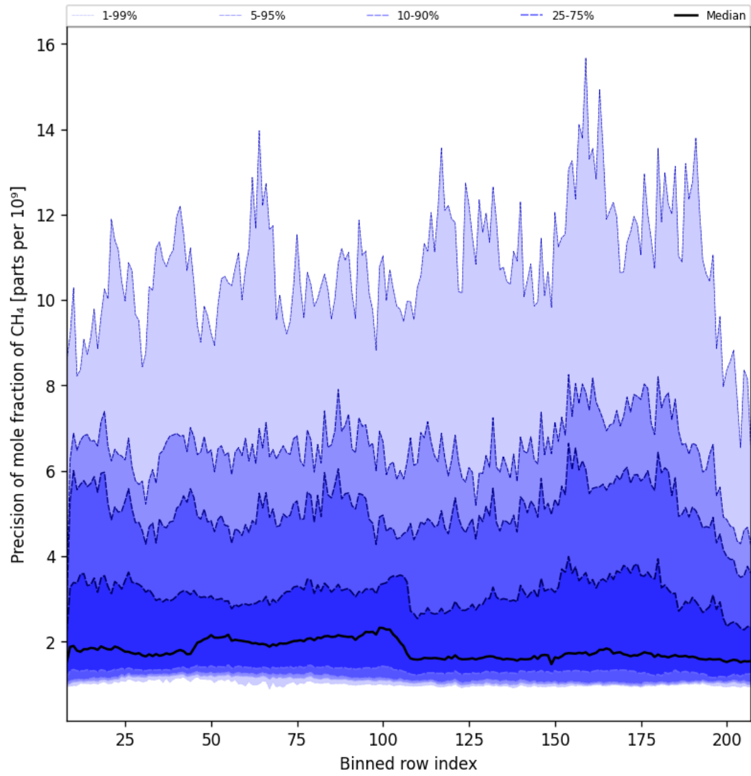
Figure 35: Along track statistics of “Precision of mole fraction of CH 4 ” for 2025-05-01 to 2025-05-03
