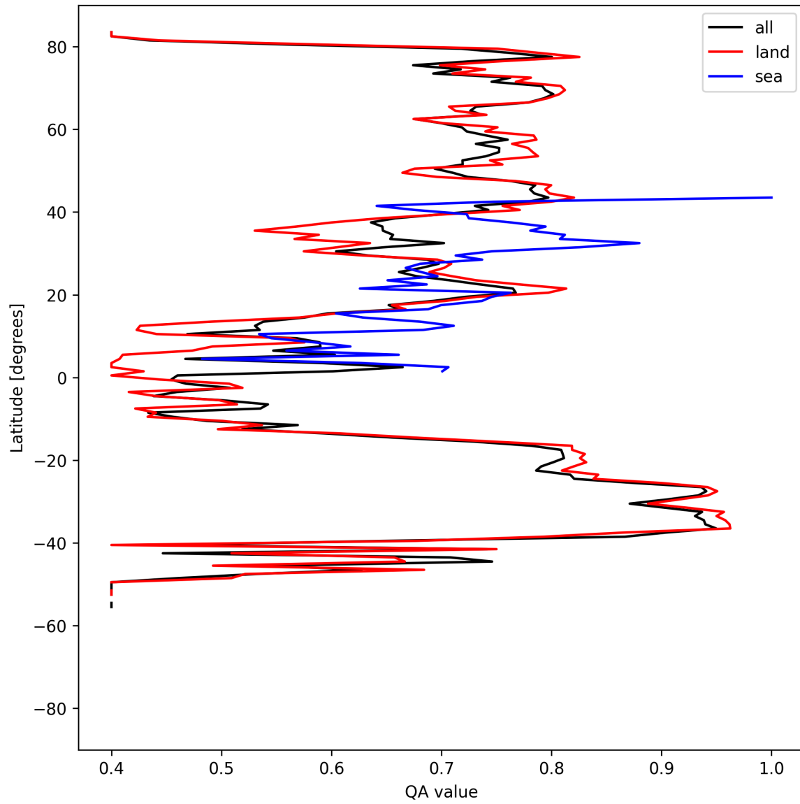
Figure 11: Zonal average of “QA value” for 2025-05-01 to 2025-05-03.
