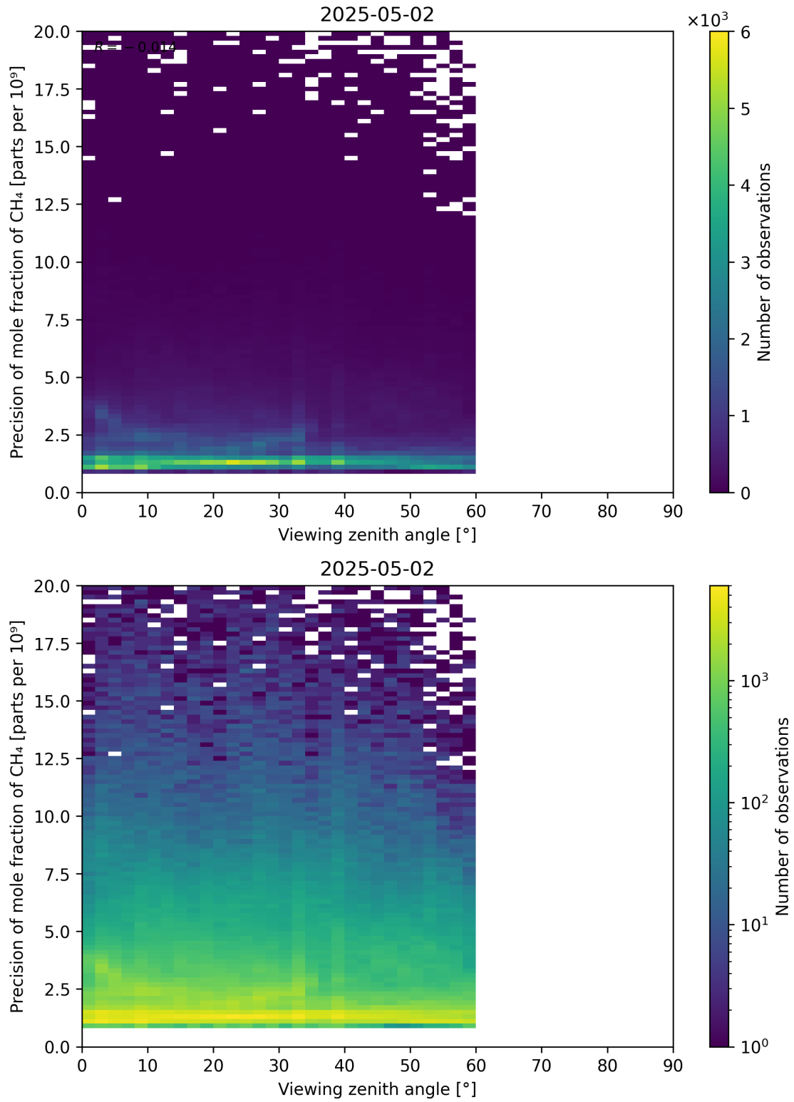
Figure 112: Scatter density plot of “Viewing zenith angle” against “Precision of mole fraction of CH 4 ” for 2025-05-01 to 2025-05-03.
