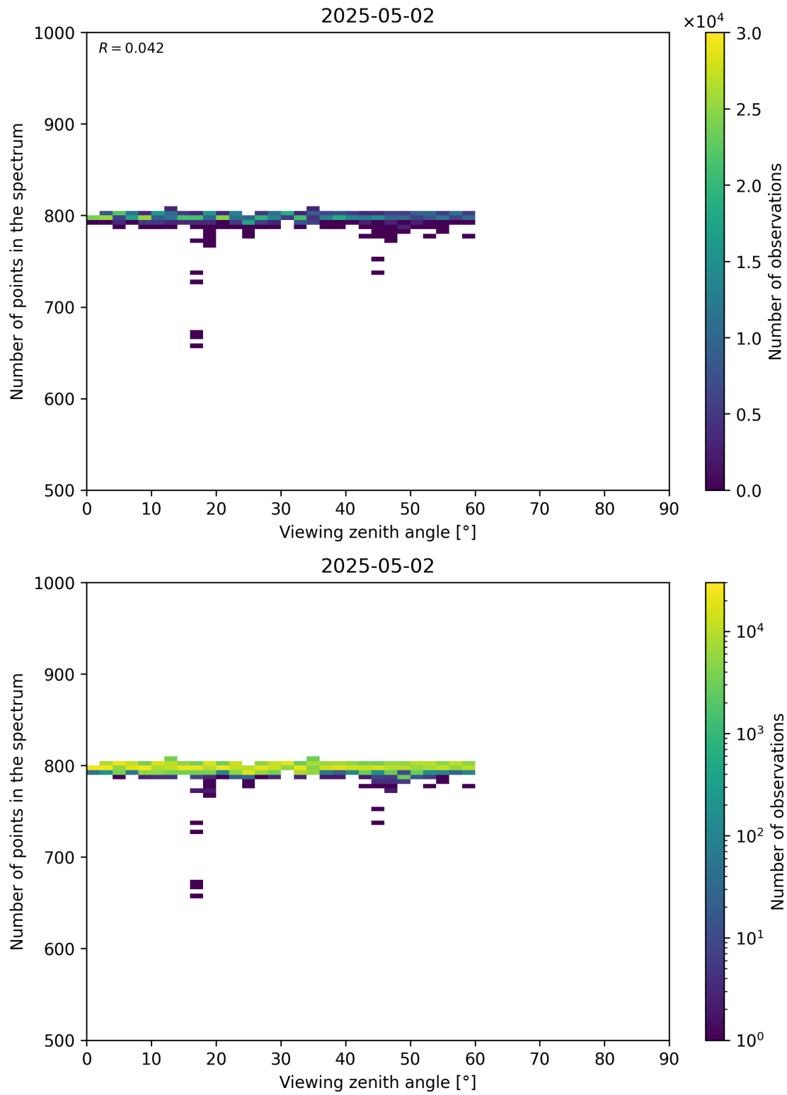
Figure 114: Scatter density plot of “Viewing zenith angle” against “Number of points in the spectrum” for 2025-05-01 to 2025-05-03.
