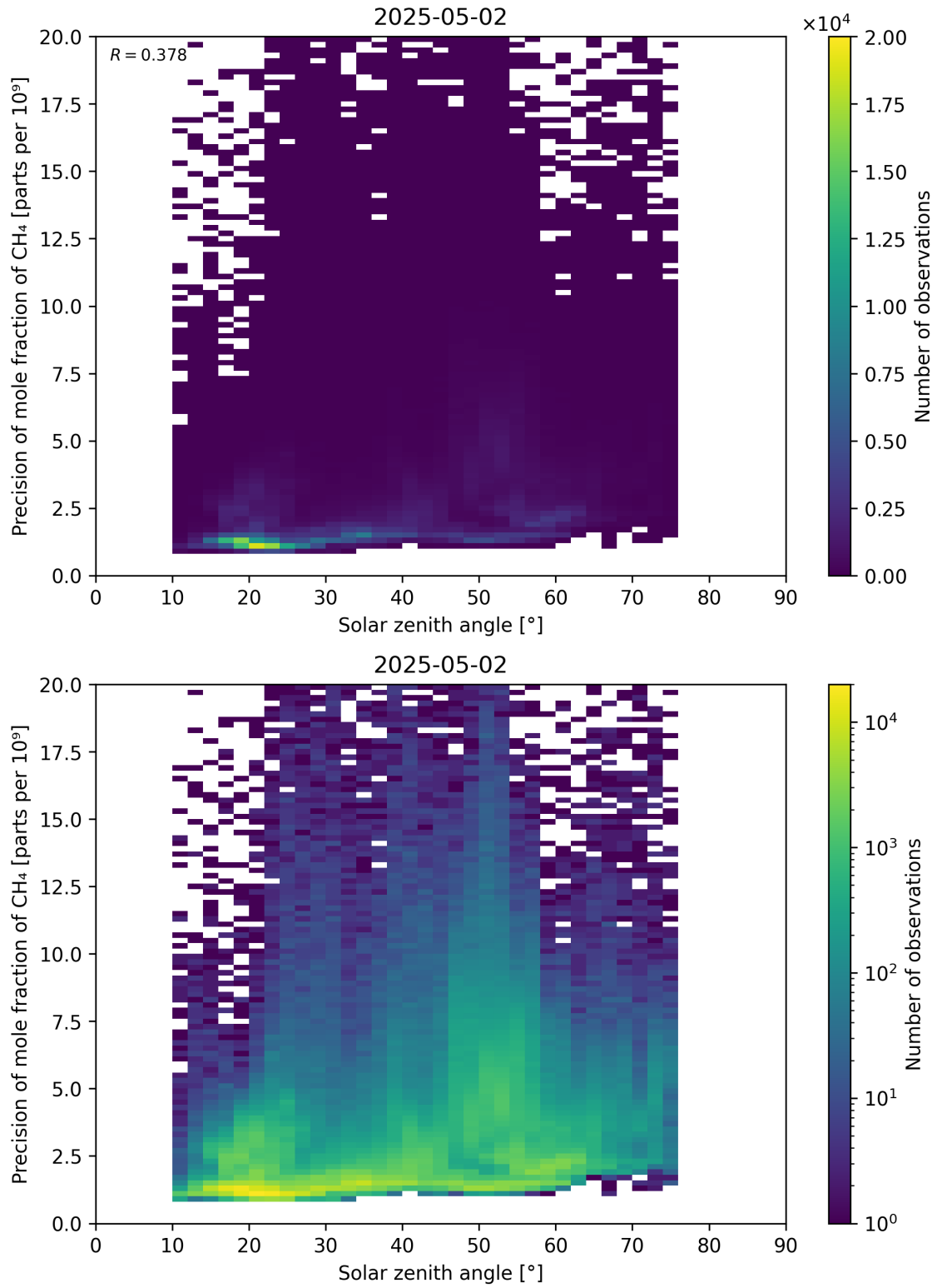
Figure 101: Scatter density plot of “Solar zenith angle” against “Precision of mole fraction of \text{CH}_4 ” for 2025-05-01 to 2025-05-03.
