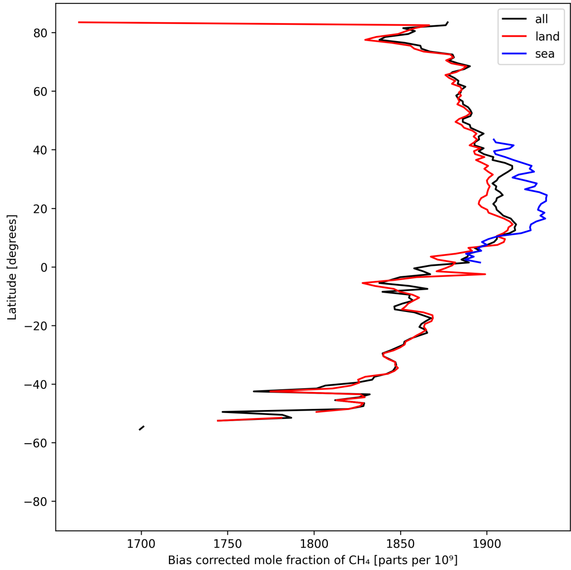
Figure 14: Zonal average of “Bias corrected mole fraction of \text{CH}_4 ” for 2025-05-01 to 2025-05-03.
