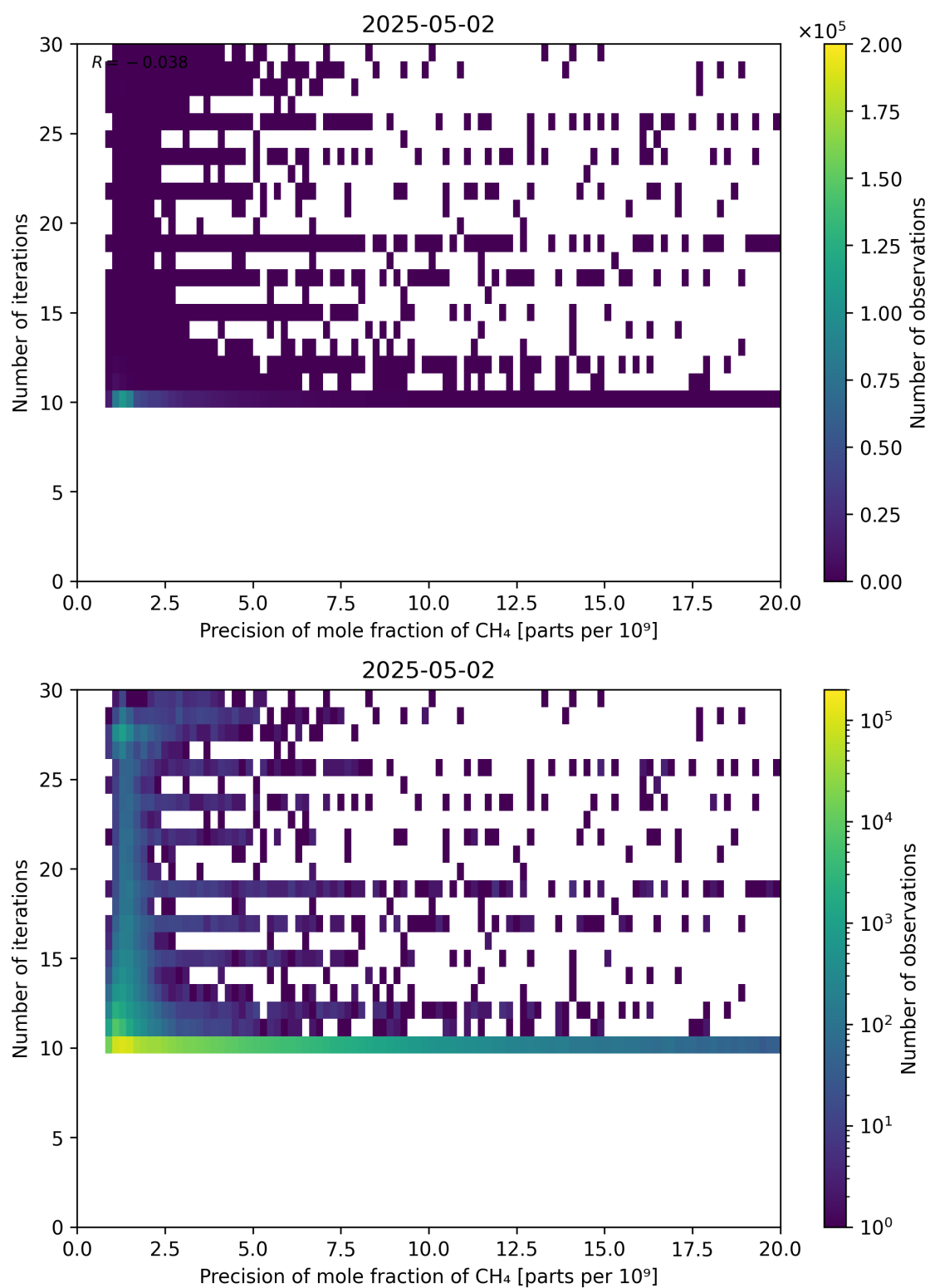
Figure 83: Scatter density plot of “Precision of mole fraction of CH 4 ” against “Number of iterations” for 2025-05-01 to 2025-05-03.
