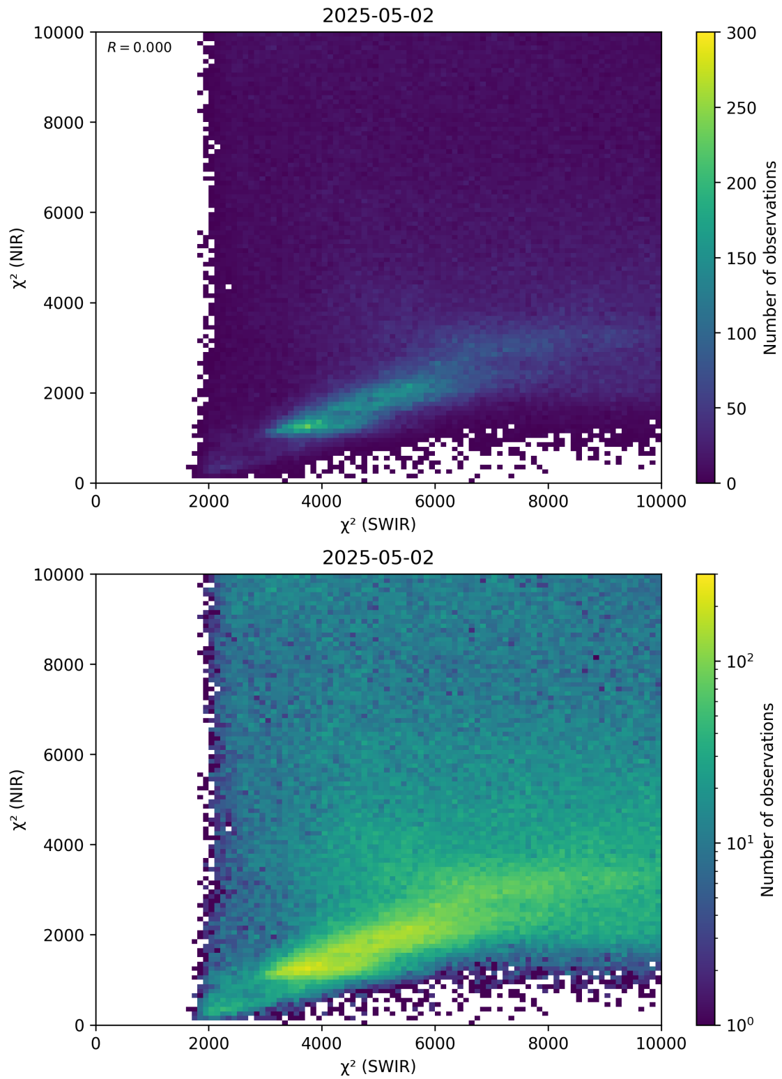
Figure 47: Scatter density plot of “ \chi^2 (SWIR)” against “ \chi^2 (NIR)” for 2025-05-01 to 2025-05-03.
