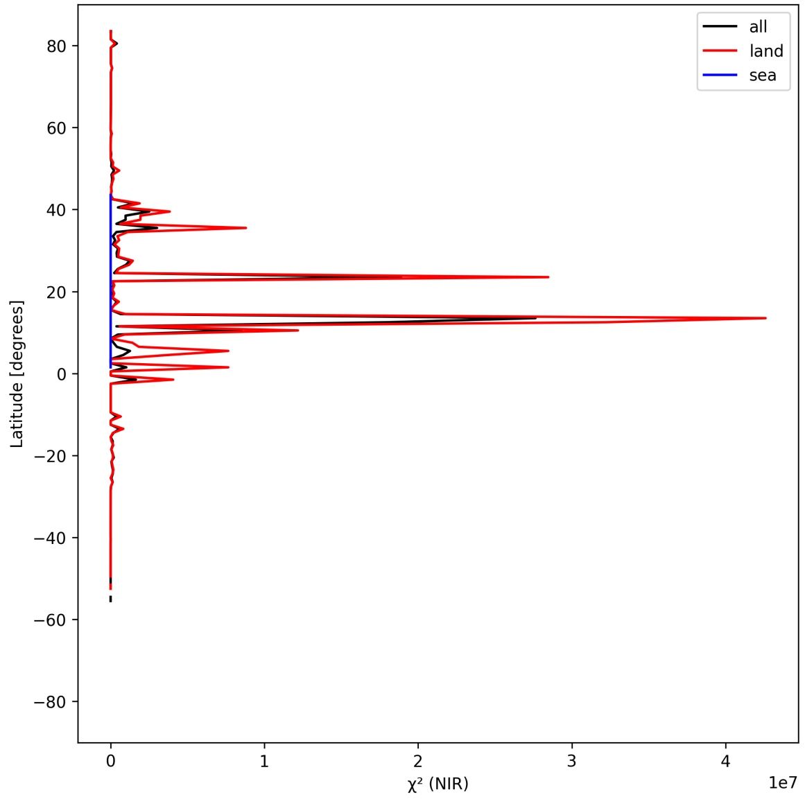
Figure 18: Zonal average of “ \chi^2 (NIR)” for 2025-05-01 to 2025-05-03.
