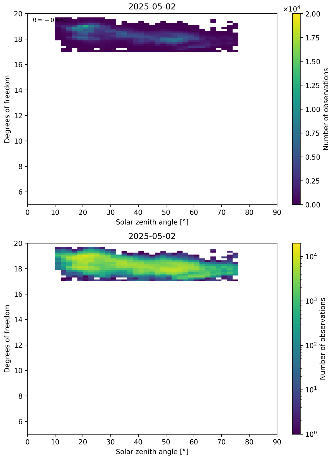
Figure 96: Scatter density plot of “Solar zenith angle” against “Degrees of freedom” for 2025-05-01 to 2025-05-03.
