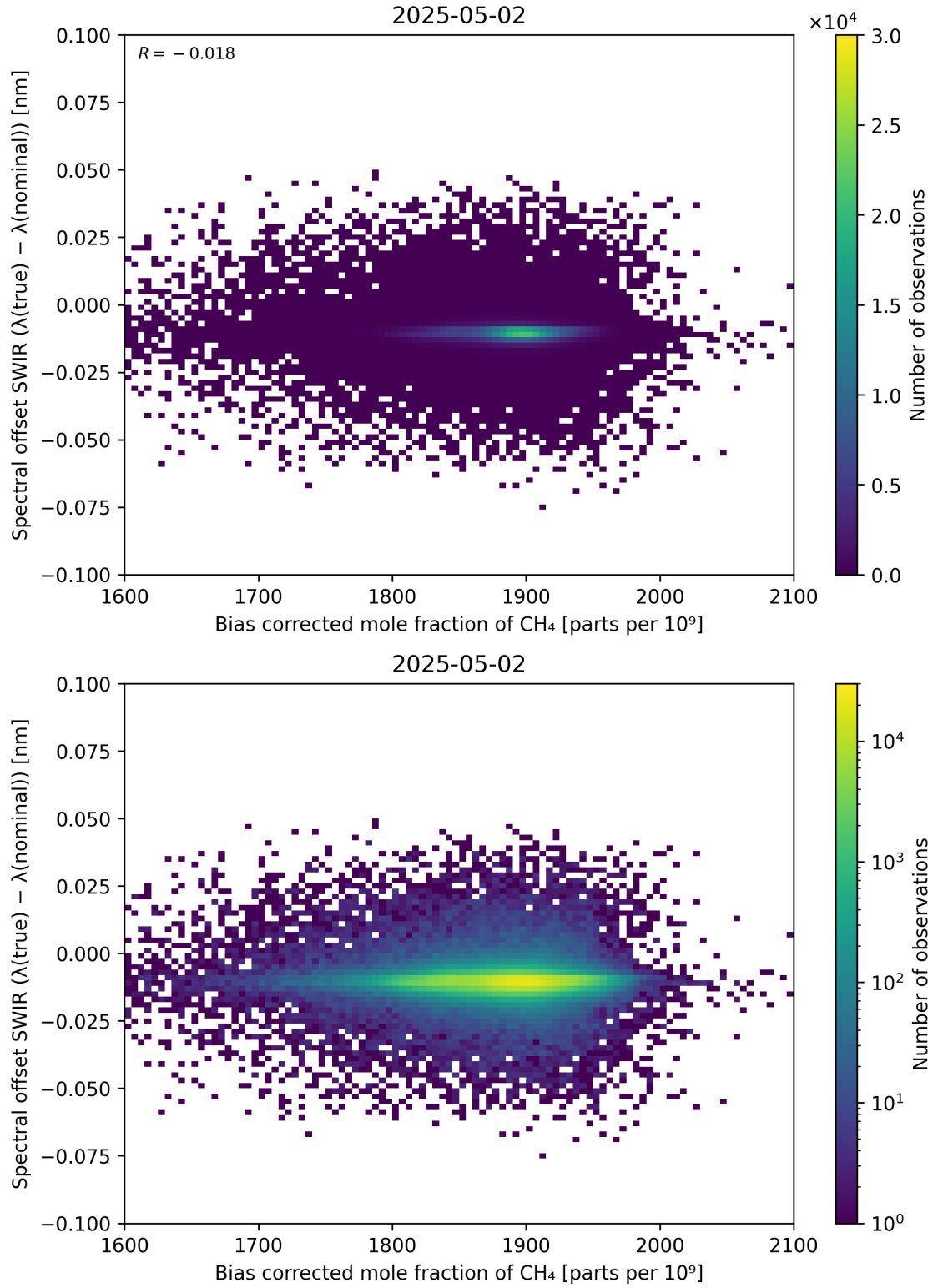
Figure 69: Scatter density plot of “Bias corrected mole fraction of \text{CH}_4 ” against “Spectral offset SWIR ( \lambda_{\text{true}} - \lambda_{\text{nominal}} )” for 2025-05-01 to 2025-05-03.
