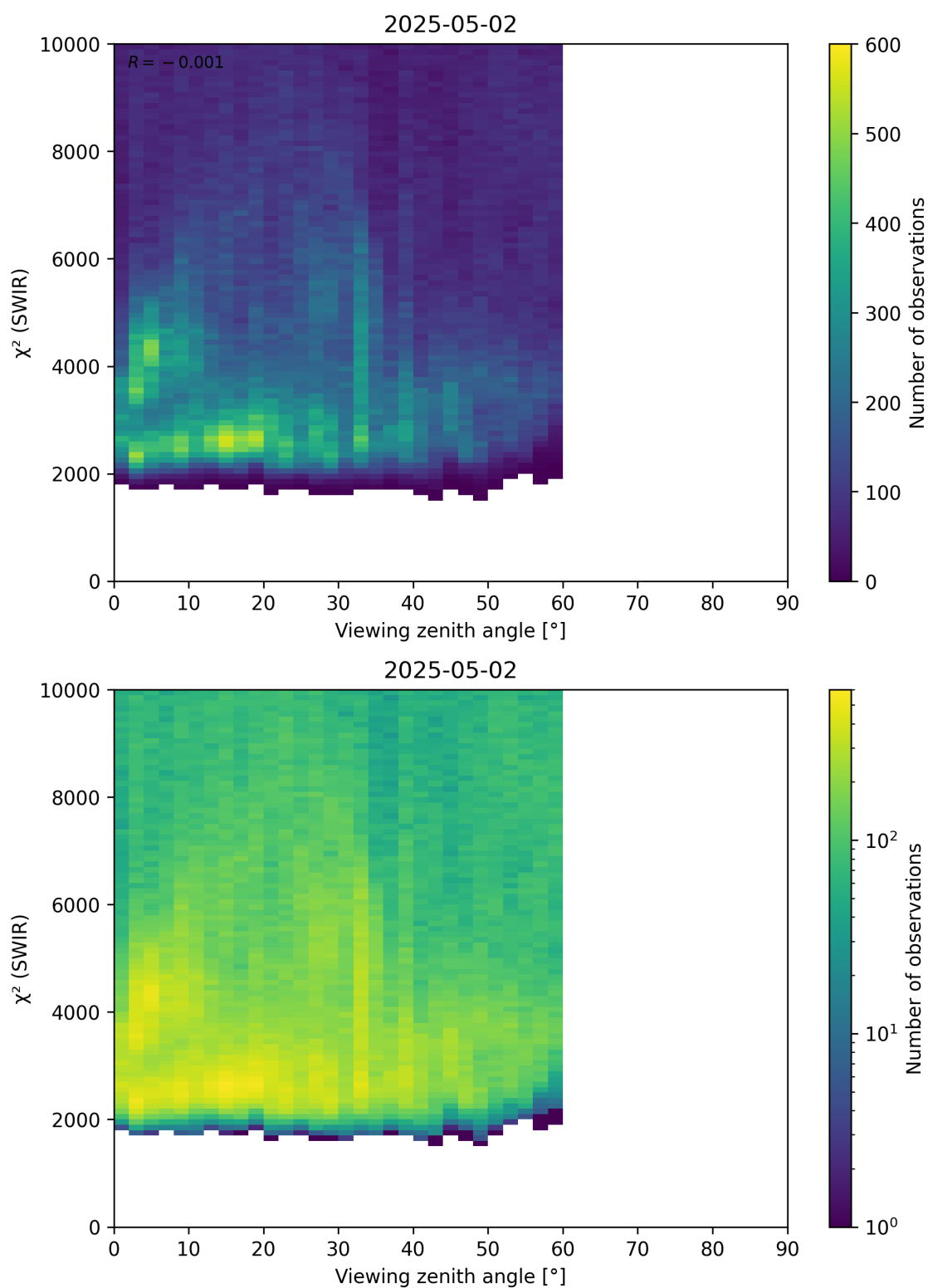
Figure 106: Scatter density plot of “Viewing zenith angle” against “ \chi^2 (SWIR)” for 2025-05-01 to 2025-05-03.
