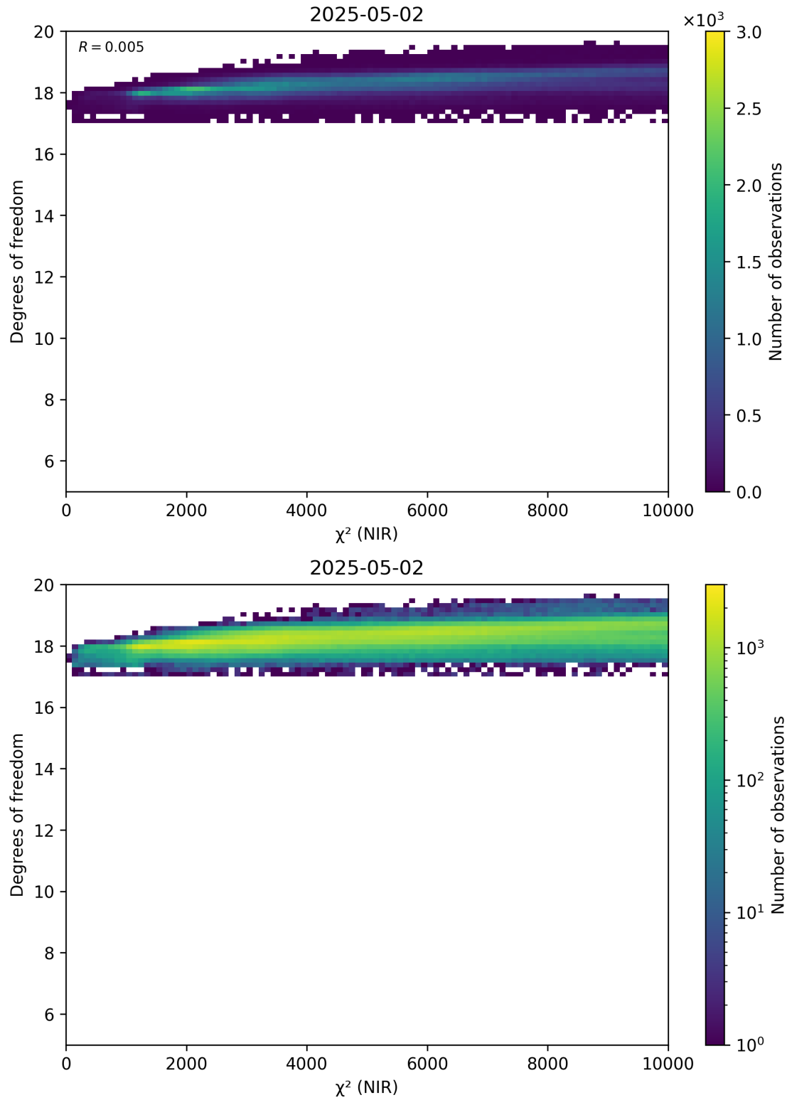
Figure 44: Scatter density plot of “ \chi^2 (NIR)” against “Degrees of freedom” for 2025-05-01 to 2025-05-03.
