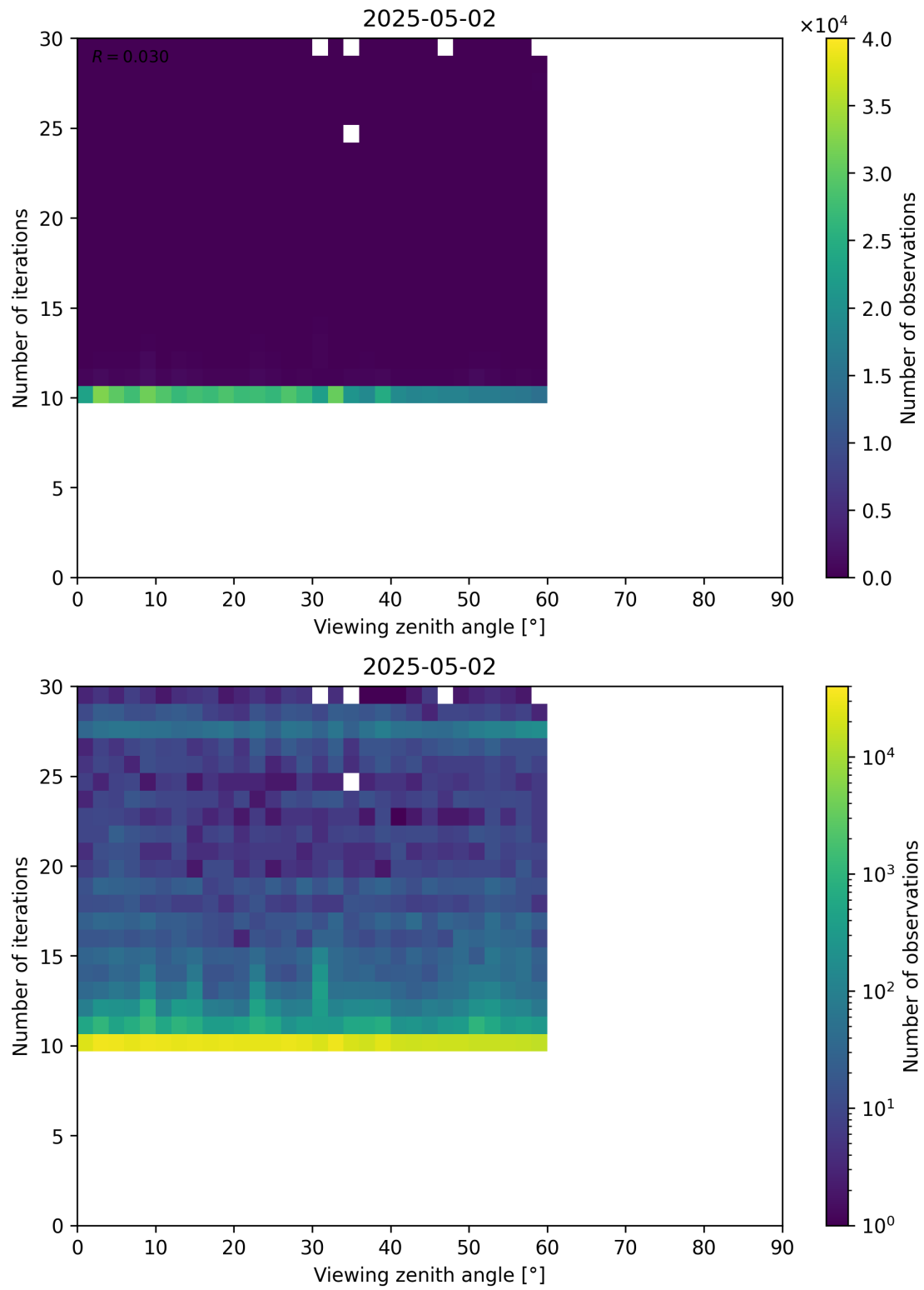
Figure 113: Scatter density plot of “Viewing zenith angle” against “Number of iterations” for 2025-05-01 to 2025-05-03.
