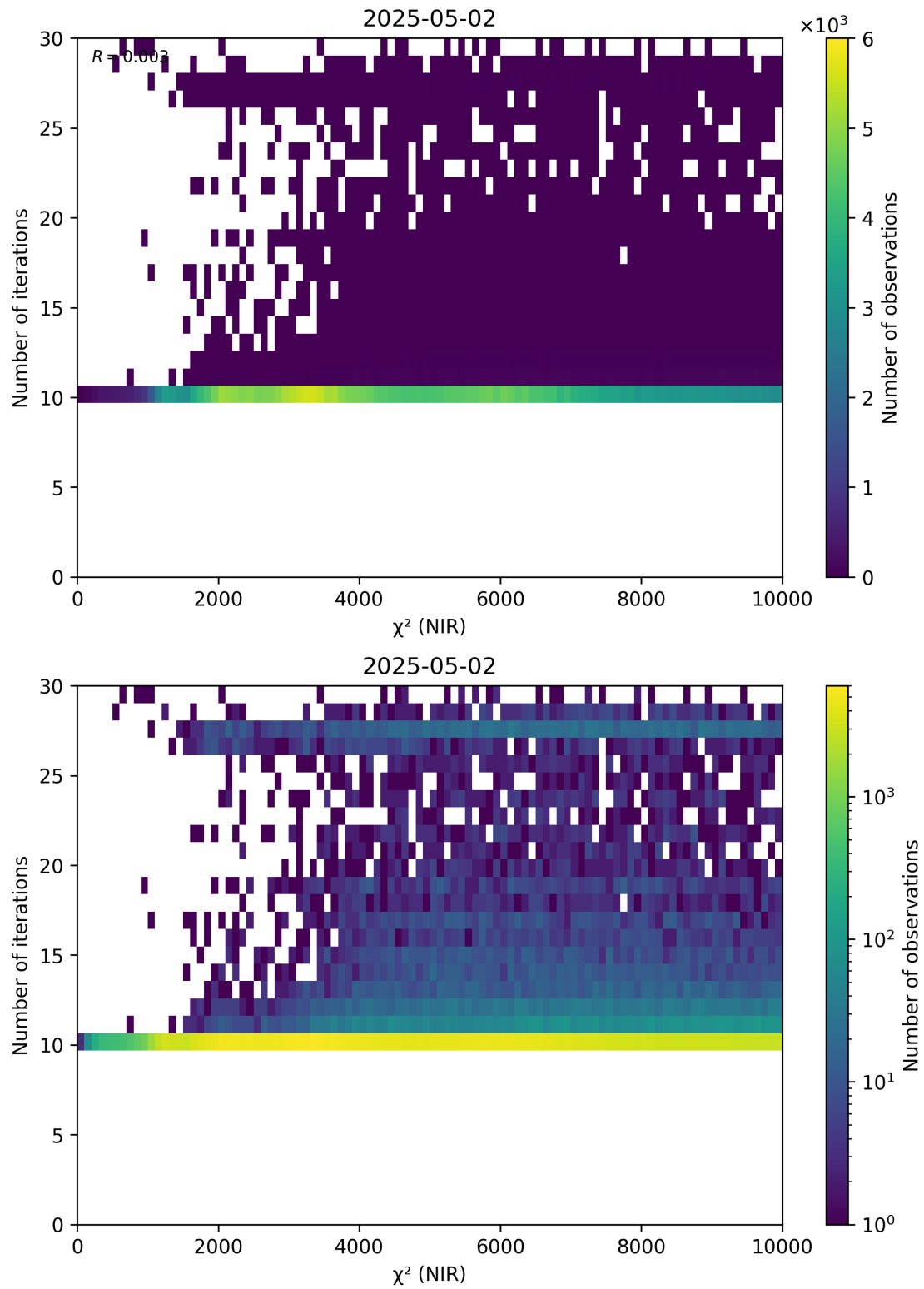
Figure 46: Scatter density plot of “ \chi^2 (NIR)” against “Number of iterations” for 2025-05-01 to 2025-05-03.
