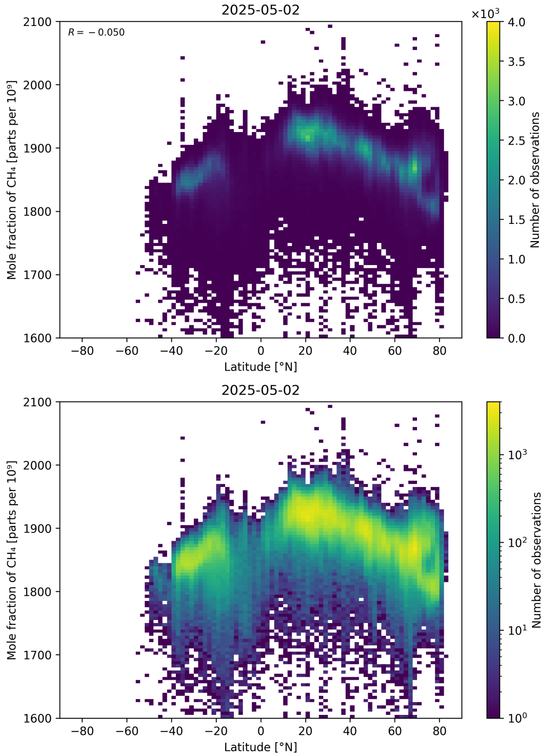
Figure 57: Scatter density plot of “Latitude” against “Mole fraction of CH 4 ” for 2025-05-01 to 2025-05-03.
