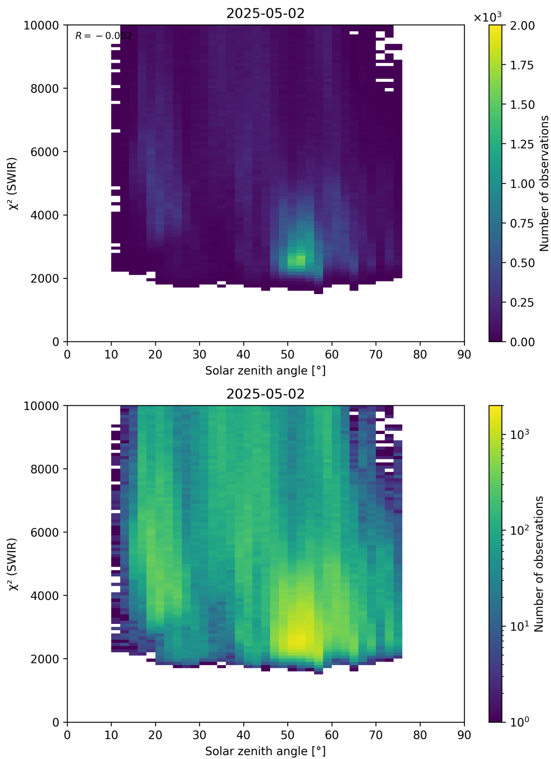
Figure 95: Scatter density plot of “Solar zenith angle” against “ \chi^2 (SWIR)” for 2025-05-01 to 2025-05-03.
