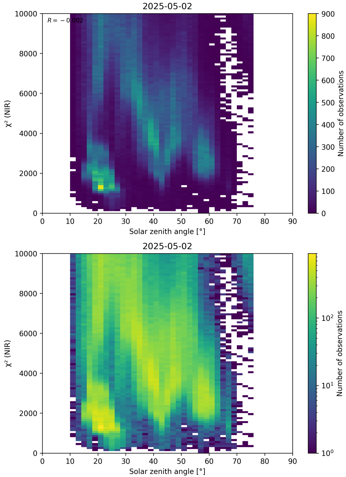
Figure 94: Scatter density plot of “Solar zenith angle” against “ \chi^2 (NIR)” for 2025-05-01 to 2025-05-03.
