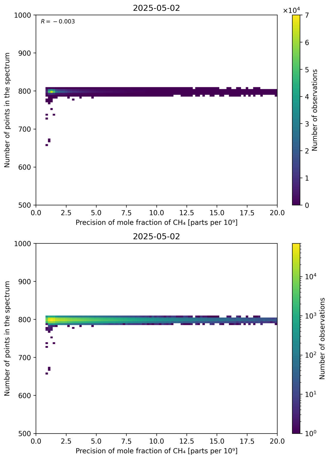
Figure 84: Scatter density plot of “Precision of mole fraction of CH 4 ” against “Number of points in the spectrum” for 2025-05-01 to 2025-05-03.
