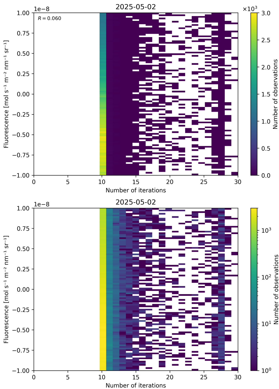
Figure 87: Scatter density plot of “Number of iterations” against “Fluorescence” for 2025-05-01 to 2025-05-03.
