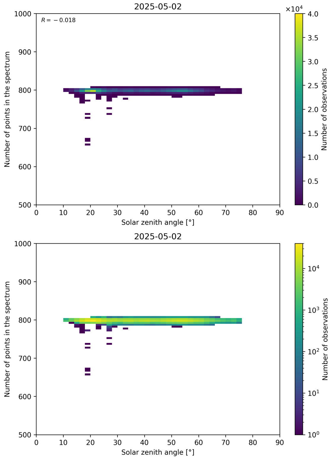
Figure 103: Scatter density plot of “Solar zenith angle” against “Number of points in the spectrum” for 2025-05-01 to 2025-05-03.
