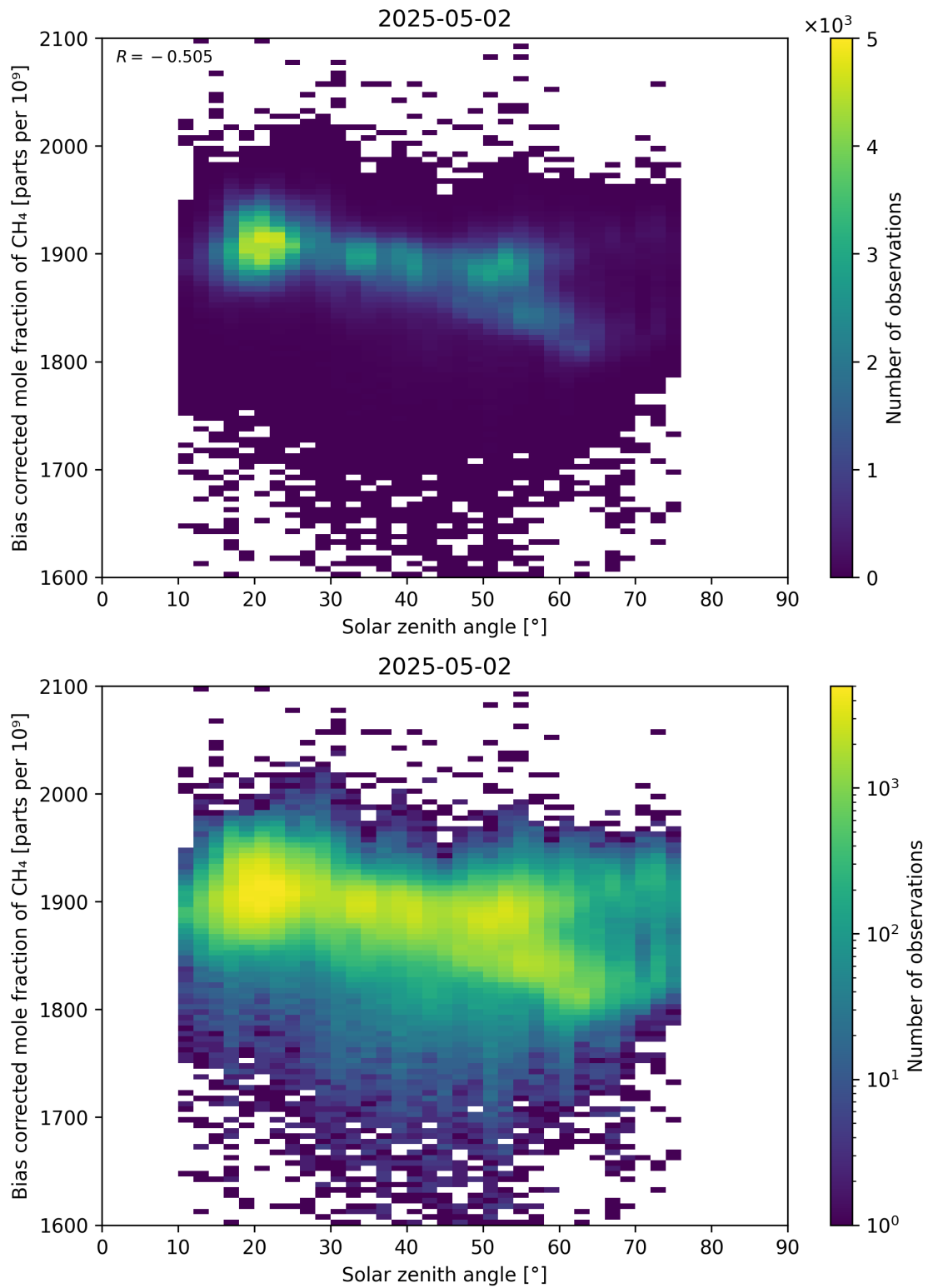
Figure 100: Scatter density plot of “Solar zenith angle” against “Bias corrected mole fraction of CH 4 ” for 2025-05-01 to 2025-05-03.
