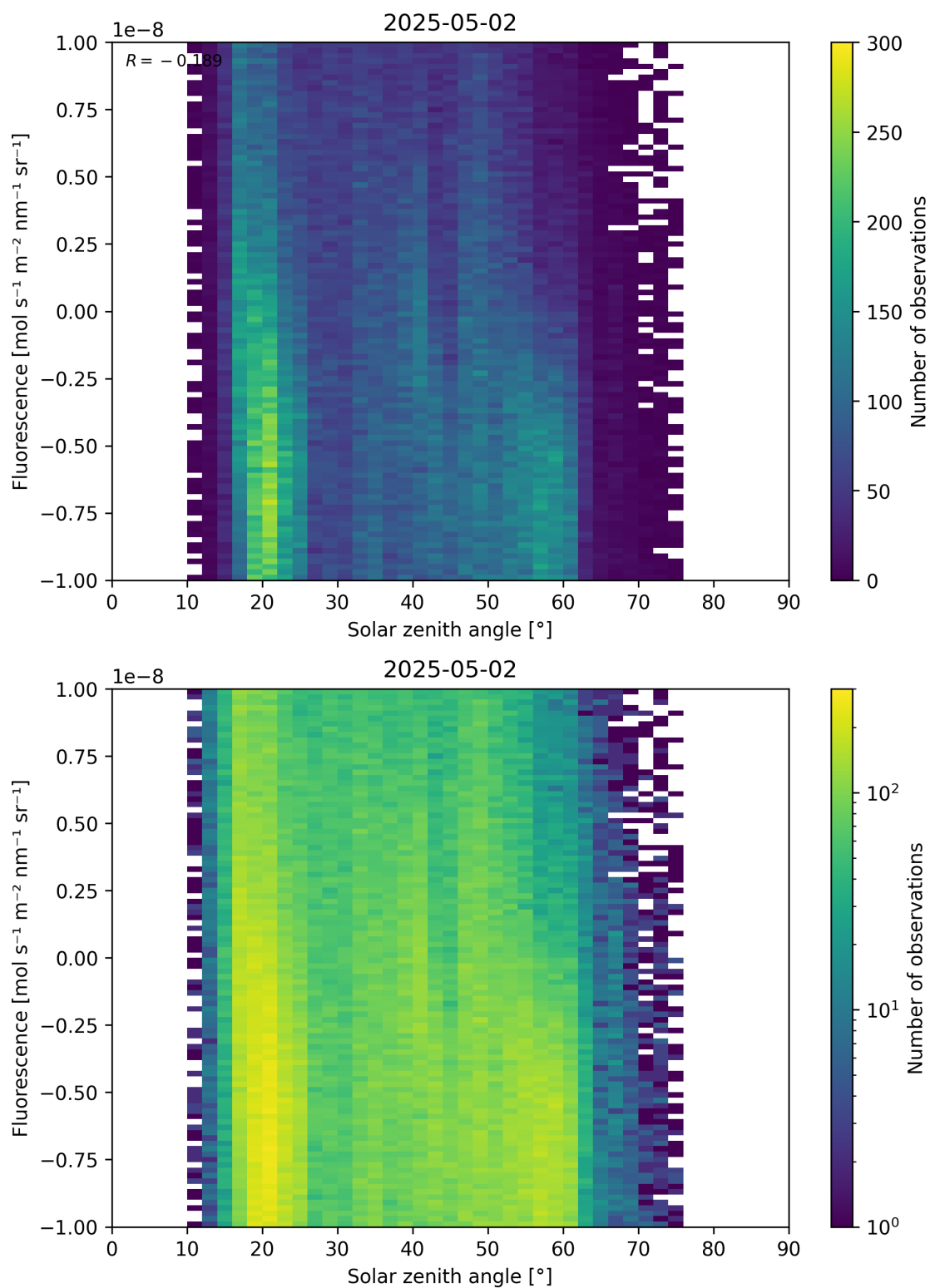
Figure 97: Scatter density plot of “Solar zenith angle” against “Fluorescence” for 2025-05-01 to 2025-05-03.
