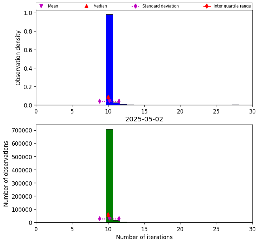
Figure 31: Histogram of “Number of iterations” for 2025-05-01 to 2025-05-03
