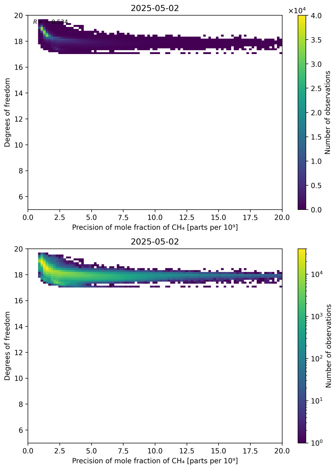
Figure 80: Scatter density plot of “Precision of mole fraction of CH 4 ” against “Degrees of freedom” for 2025-05-01 to 2025-05-03.
