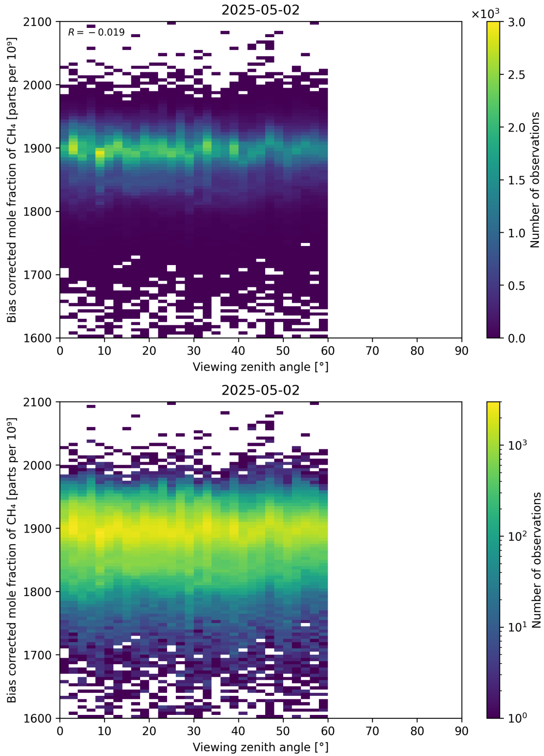
Figure 111: Scatter density plot of “Viewing zenith angle” against “Bias corrected mole fraction of CH 4 ” for 2025-05-01 to 2025-05-03.
