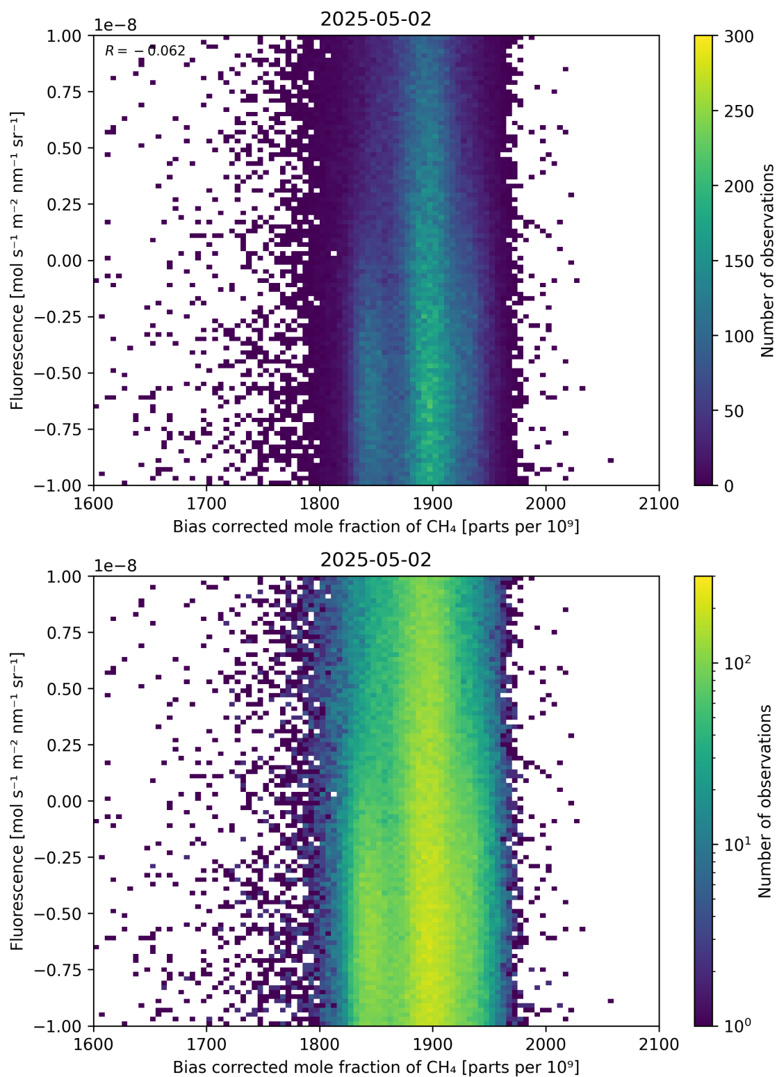
Figure 66: Scatter density plot of “Bias corrected mole fraction of \text{CH}_4 ” against “Fluorescence” for 2025-05-01 to 2025-05-03.
