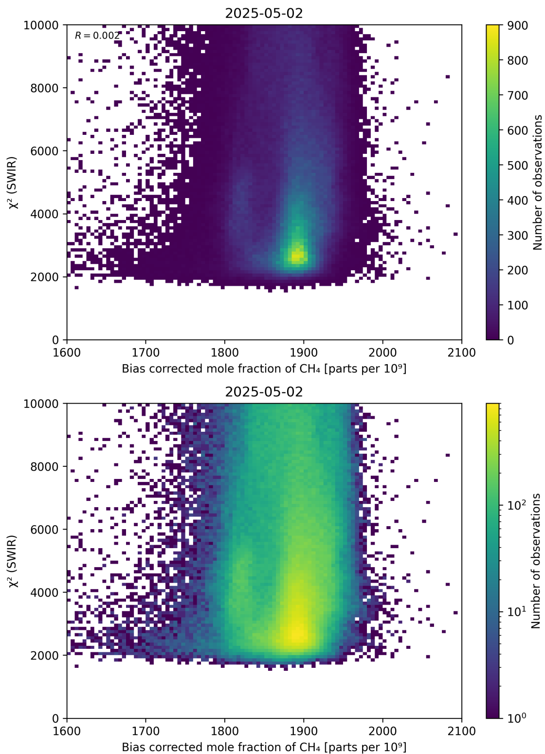
Figure 64: Scatter density plot of “Bias corrected mole fraction of \text{CH}_4 ” against “ \chi^2 (SWIR)” for 2025-05-01 to 2025-05-03.
