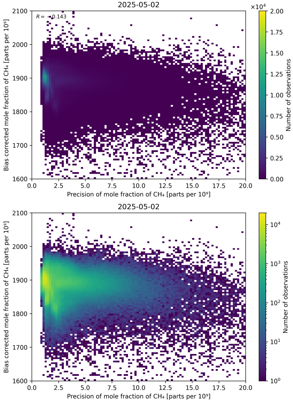
Figure 82: Scatter density plot of “Precision of mole fraction of CH 4 ” against “Bias corrected mole fraction of CH 4 ” for 2025-05-01 to 2025-05-03.
