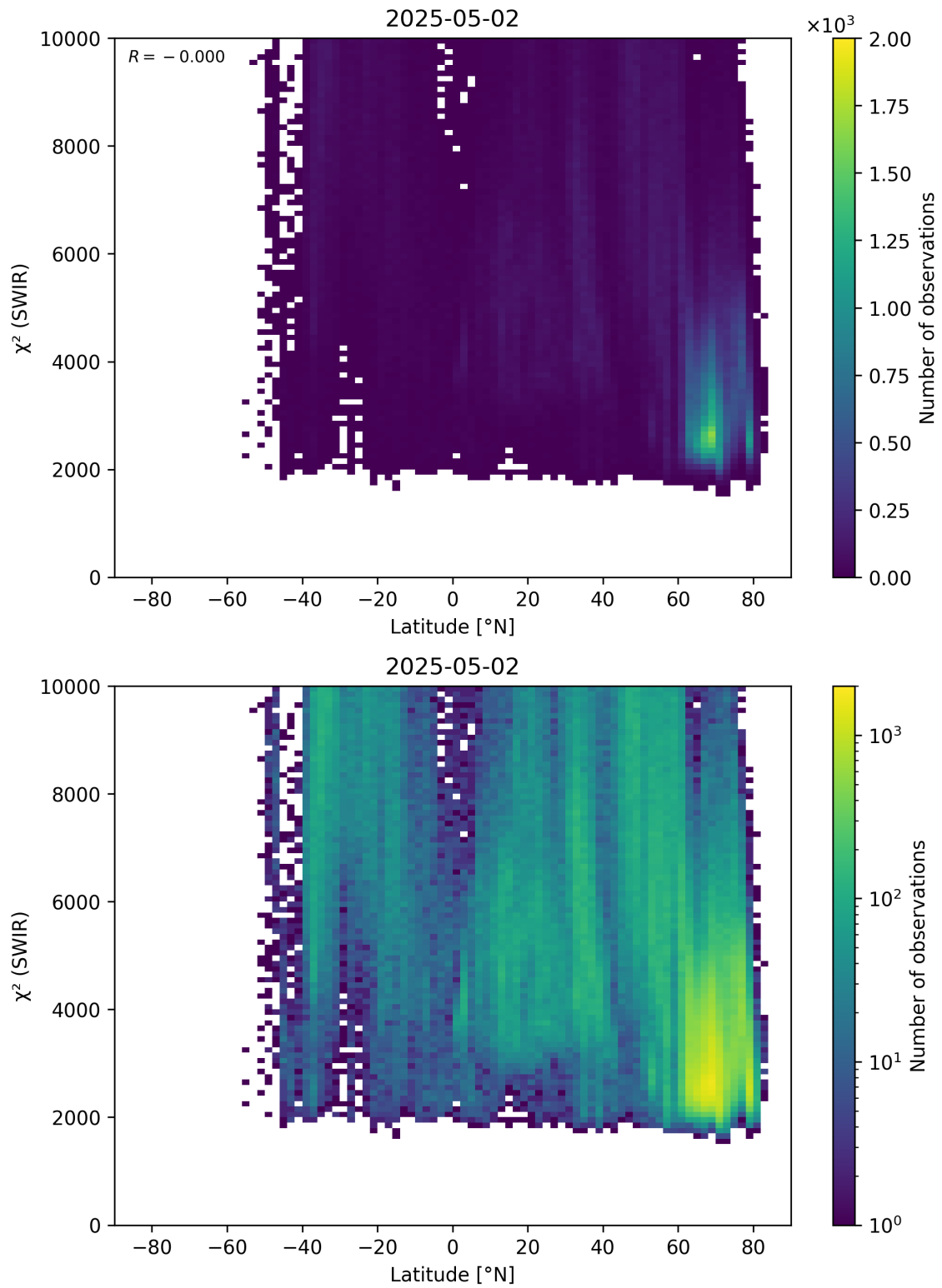
Figure 54: Scatter density plot of “Latitude” against “ \chi^2 (SWIR)” for 2025-05-01 to 2025-05-03.
