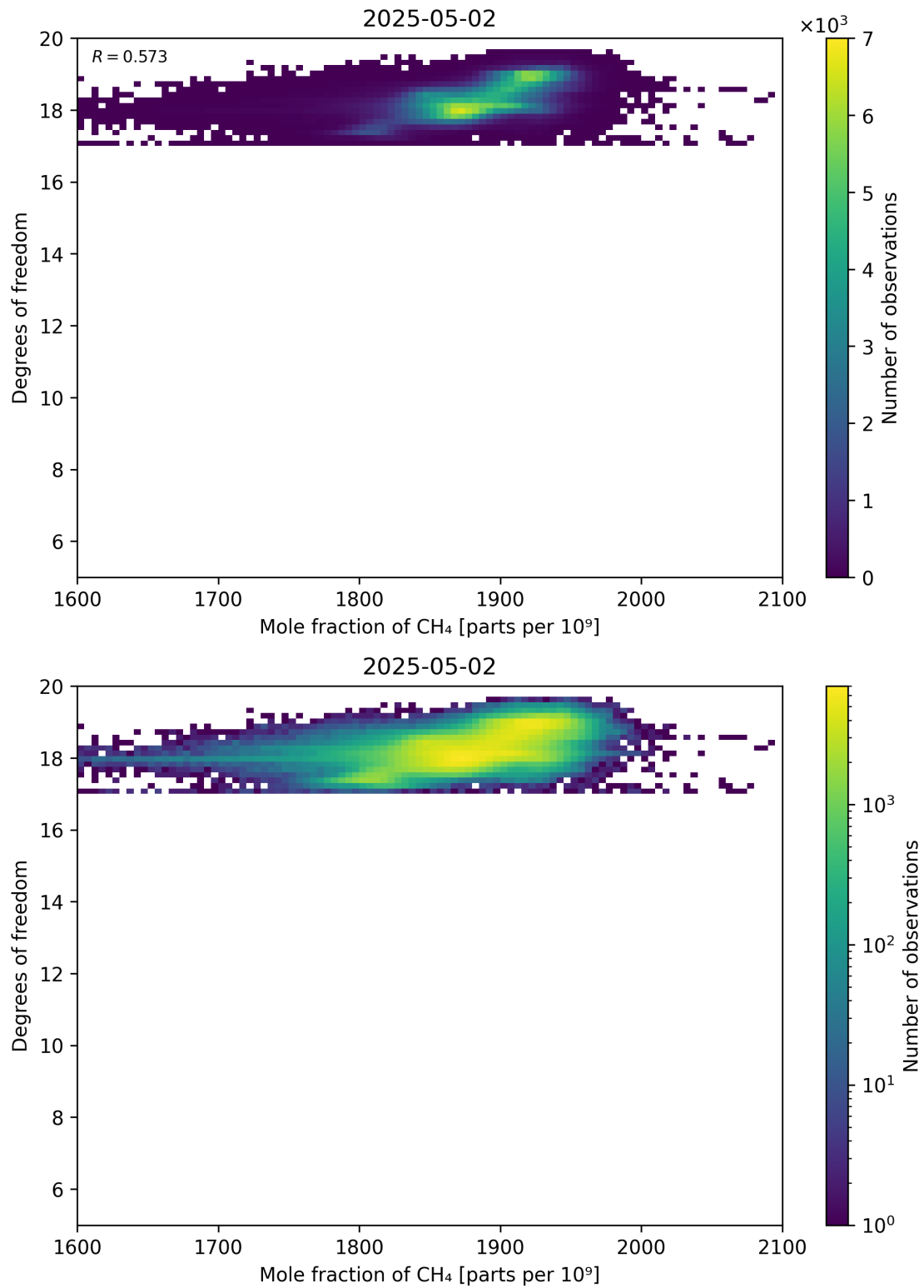
Figure 72: Scatter density plot of “Mole fraction of CH 4 ” against “Degrees of freedom” for 2025-05-01 to 2025-05-03.
