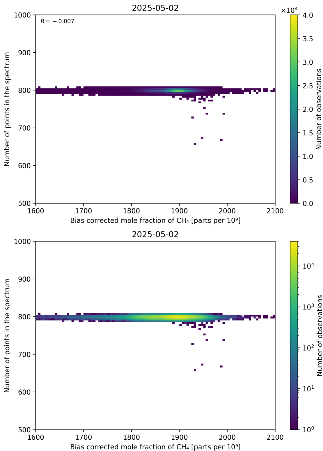
Figure 68: Scatter density plot of “Bias corrected mole fraction of CH 4 ” against “Number of points in the spectrum” for 2025-05-01 to 2025-05-03.
