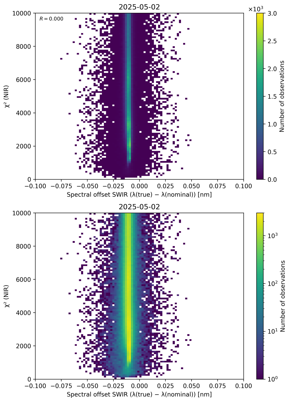
Figure 117: Scatter density plot of “Spectral offset SWIR ( \lambda_{\text{true}} - \lambda_{\text{nominal}} )” against “ \chi^2 (NIR)” for 2025-05-01 to 2025-05-03.
