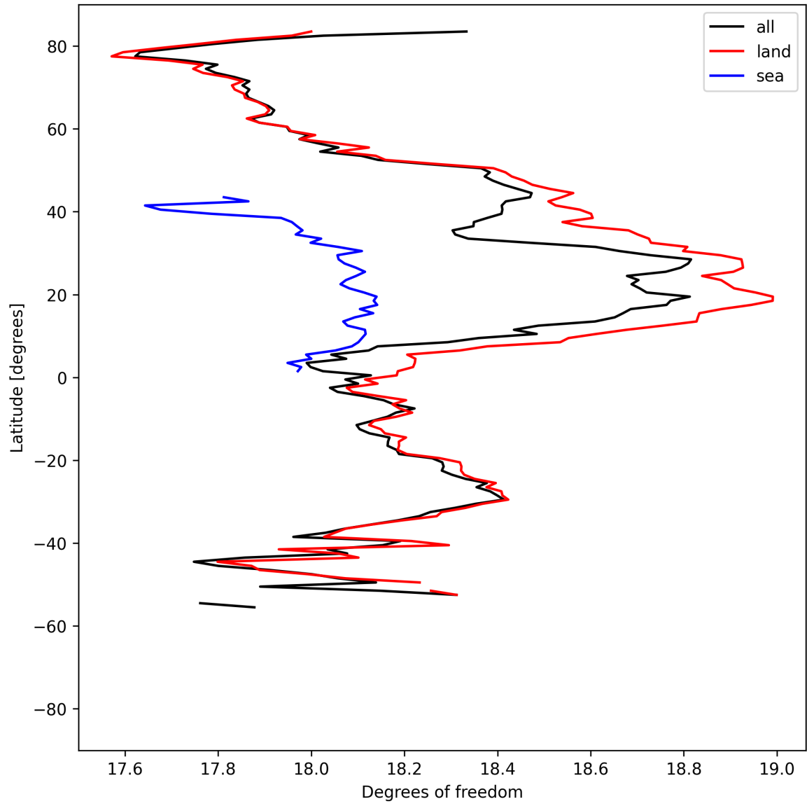
Figure 19: Zonal average of “Degrees of freedom” for 2025-05-01 to 2025-05-03.
