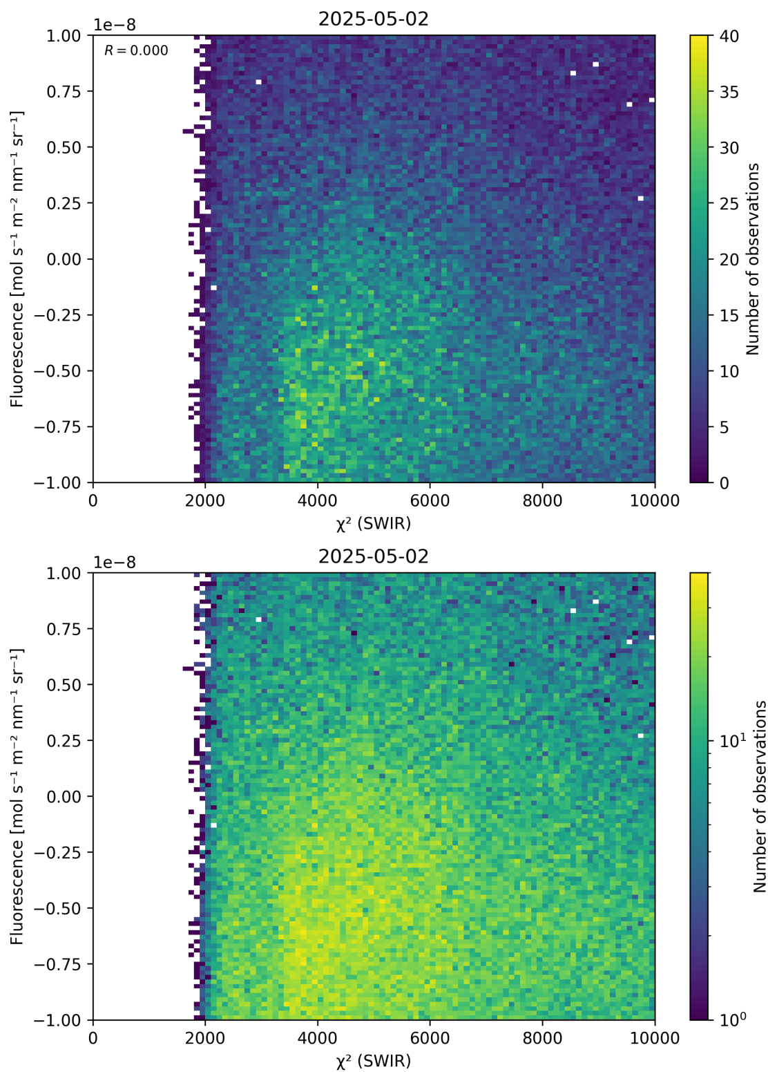
Figure 49: Scatter density plot of “ \chi^2 (SWIR)” against “Fluorescence” for 2025-05-01 to 2025-05-03.
