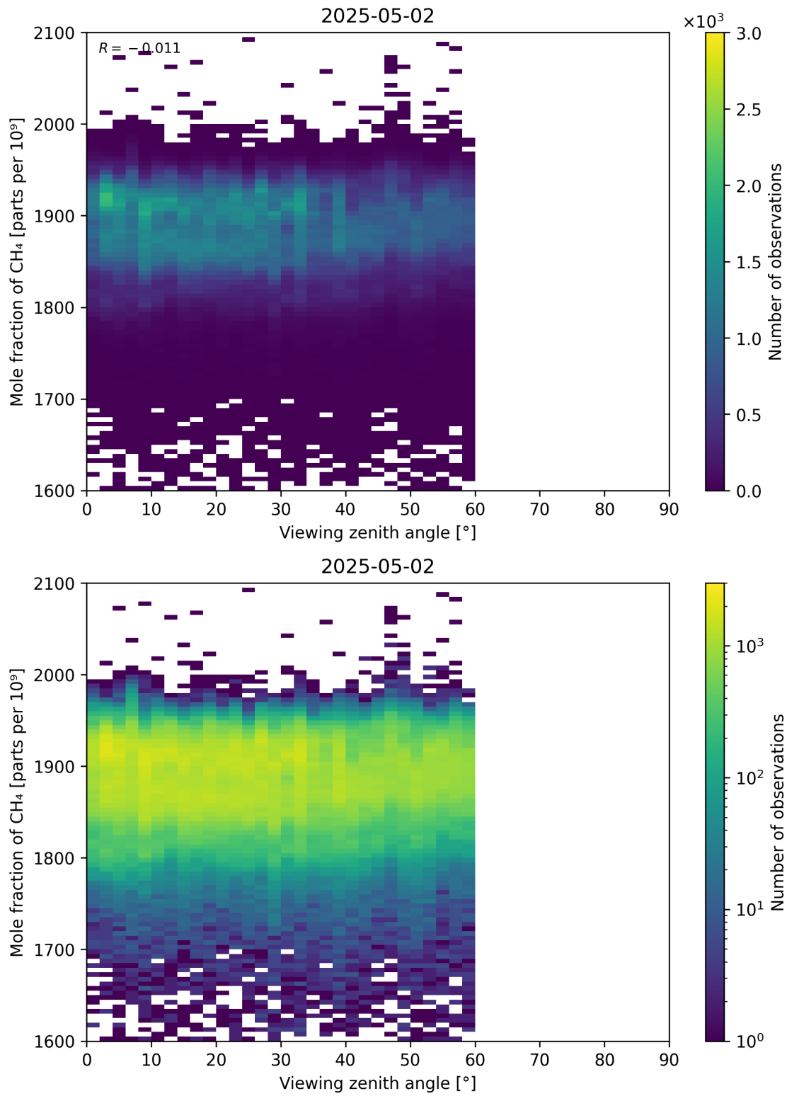
Figure 110: Scatter density plot of “Viewing zenith angle” against “Mole fraction of CH 4 ” for 2025-05-01 to 2025-05-03.
