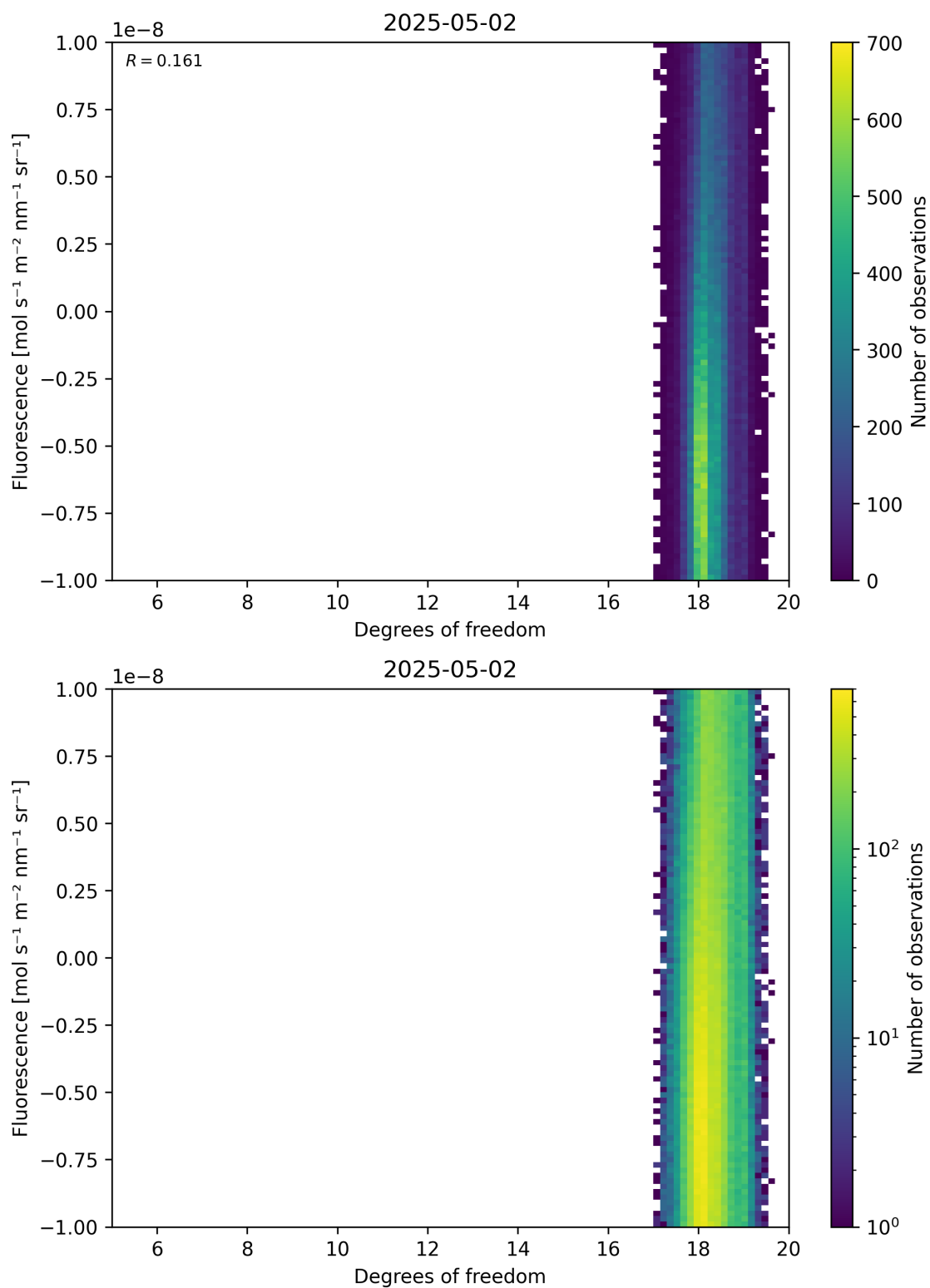
Figure 51: Scatter density plot of “Degrees of freedom” against “Fluorescence” for 2025-05-01 to 2025-05-03.
