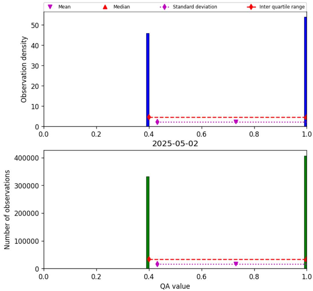
Figure 22: Histogram of “QA value” for 2025-05-01 to 2025-05-03
