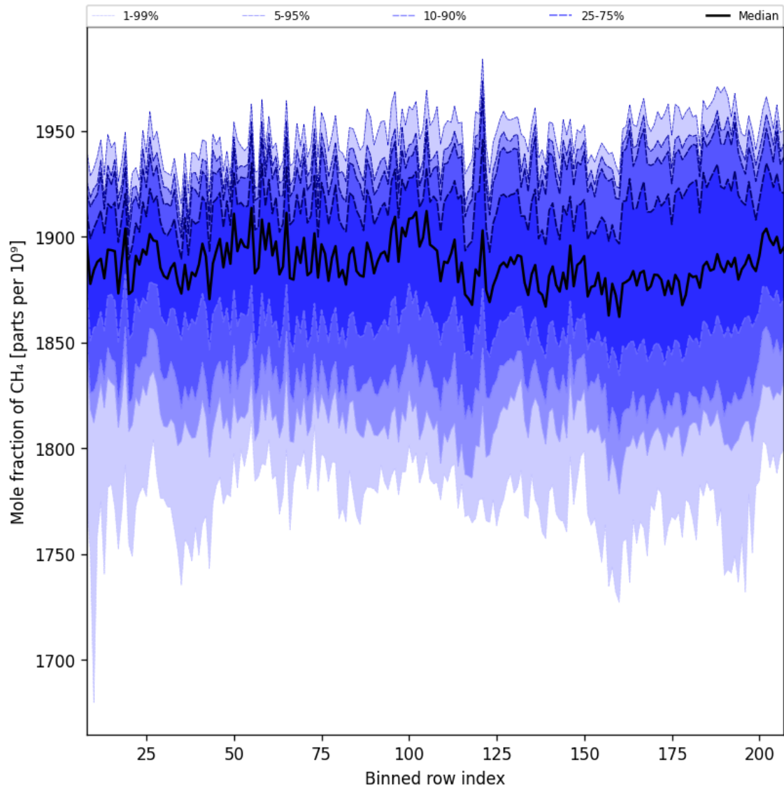
Figure 34: Along track statistics of “Mole fraction of CH 4 ” for 2025-05-01 to 2025-05-03
