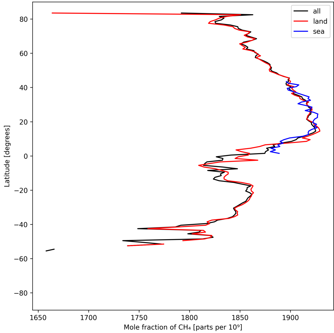
Figure 12: Zonal average of “Mole fraction of \text{CH}_4 ” for 2025-05-01 to 2025-05-03.
