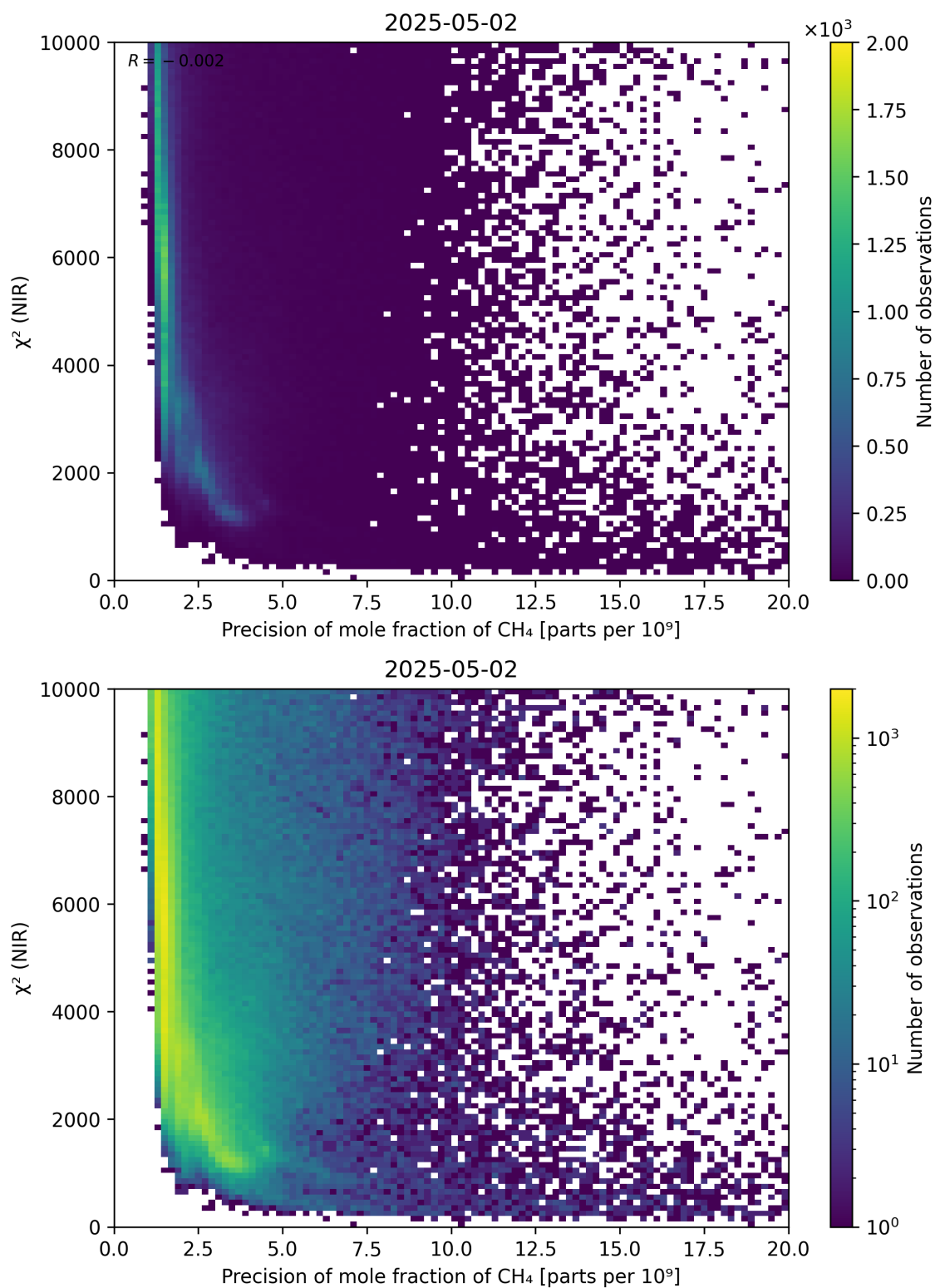
Figure 78: Scatter density plot of “Precision of mole fraction of CH 4 ” against “ \chi^2 (NIR)” for 2025-05-01 to 2025-05-03.
