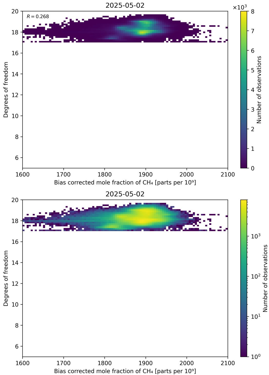
Figure 65: Scatter density plot of “Bias corrected mole fraction of CH 4 ” against “Degrees of freedom” for 2025-05-01 to 2025-05-03.
