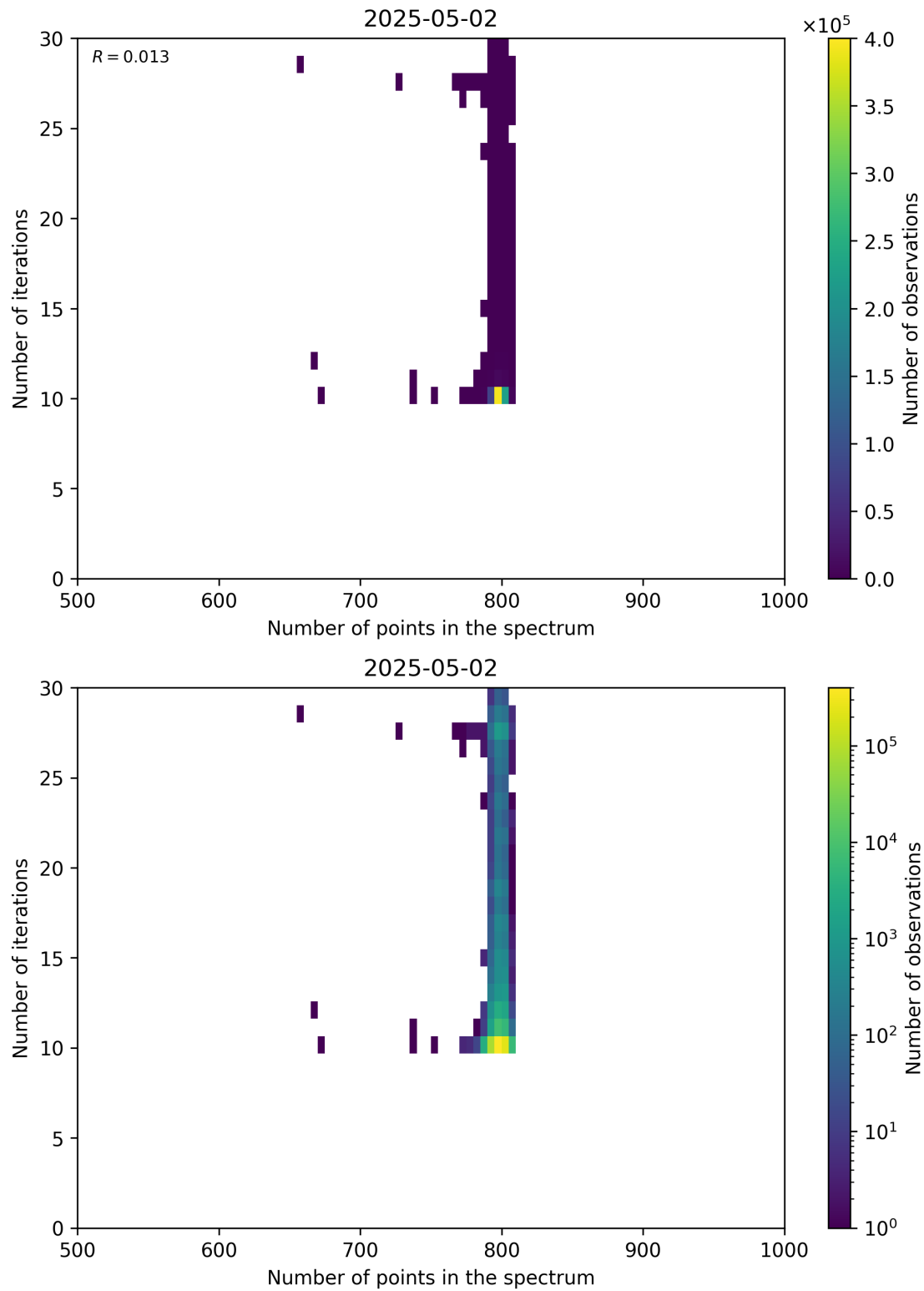
Figure 92: Scatter density plot of “Number of points in the spectrum” against “Number of iterations” for 2025-05-01 to 2025-05-03.
