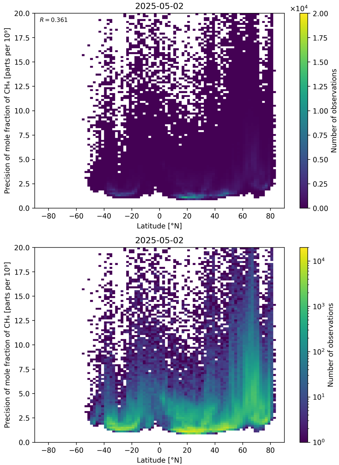
Figure 59: Scatter density plot of “Latitude” against “Precision of mole fraction of \text{CH}_4 ” for 2025-05-01 to 2025-05-03.
