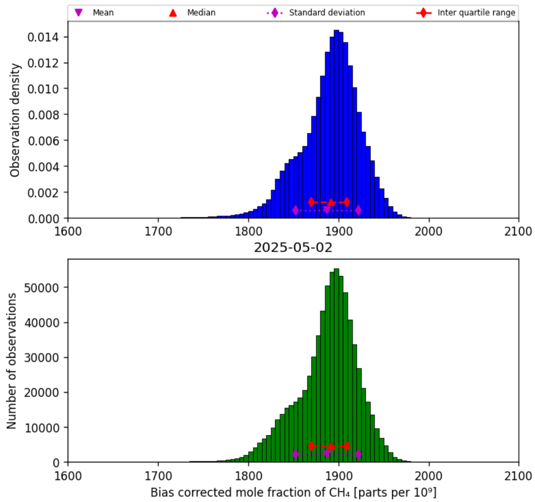
Figure 25: Histogram of “Bias corrected mole fraction of CH 4 ” for 2025-05-01 to 2025-05-03
