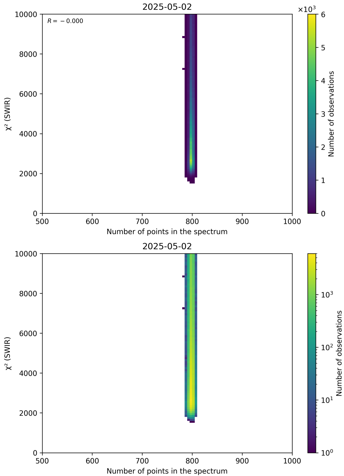
Figure 89: Scatter density plot of “Number of points in the spectrum” against “ \chi^2 (SWIR)” for 2025-05-01 to 2025-05-03.
