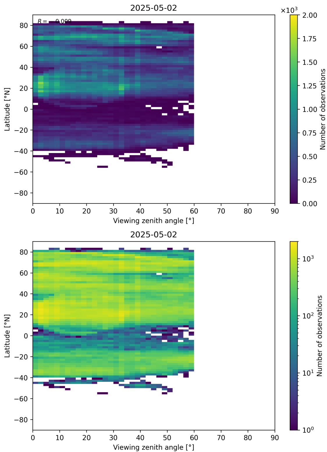
Figure 109: Scatter density plot of “Viewing zenith angle” against “Latitude” for 2025-05-01 to 2025-05-03.
