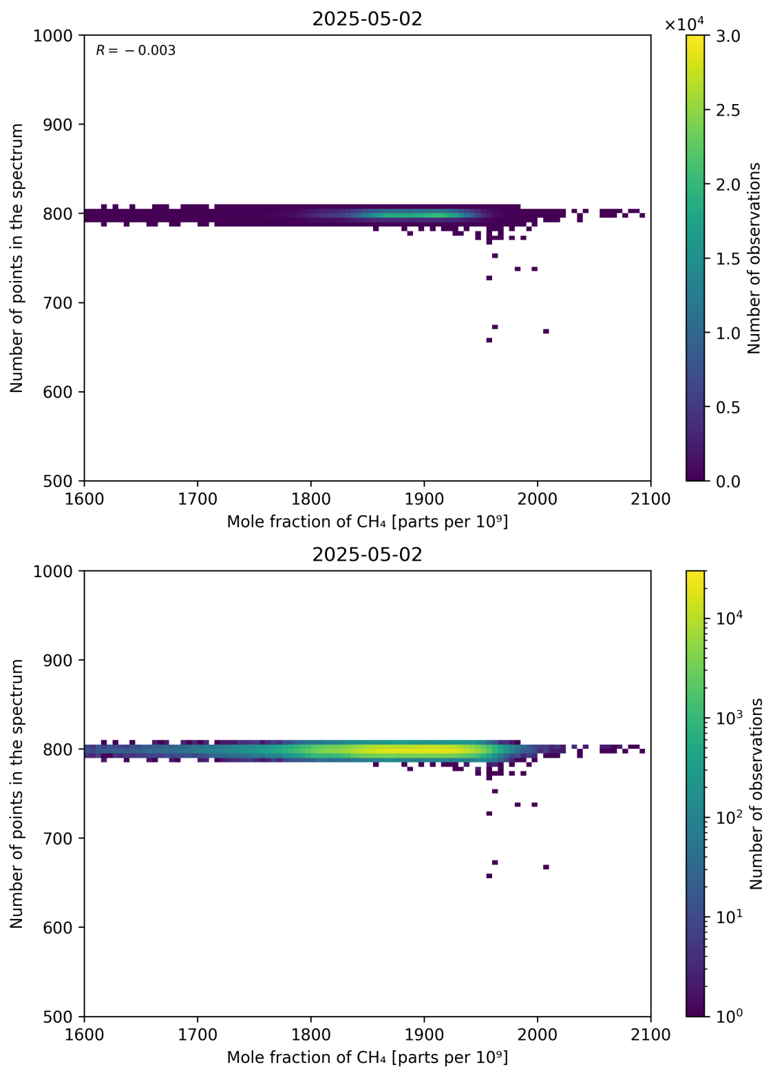
Figure 77: Scatter density plot of “Mole fraction of CH 4 ” against “Number of points in the spectrum” for 2025-05-01 to 2025-05-03.
