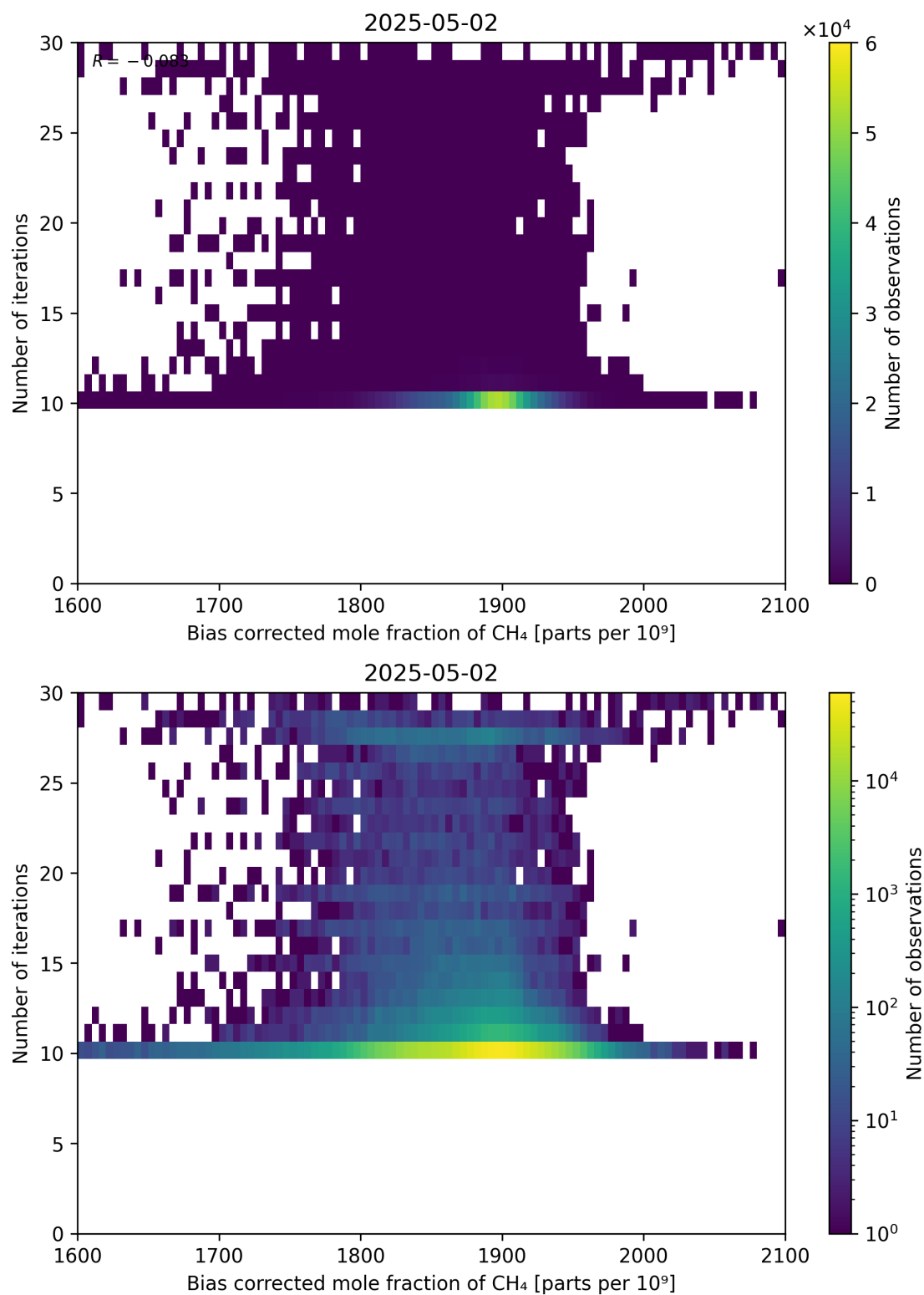
Figure 67: Scatter density plot of “Bias corrected mole fraction of CH 4 ” against “Number of iterations” for 2025-05-01 to 2025-05-03.
