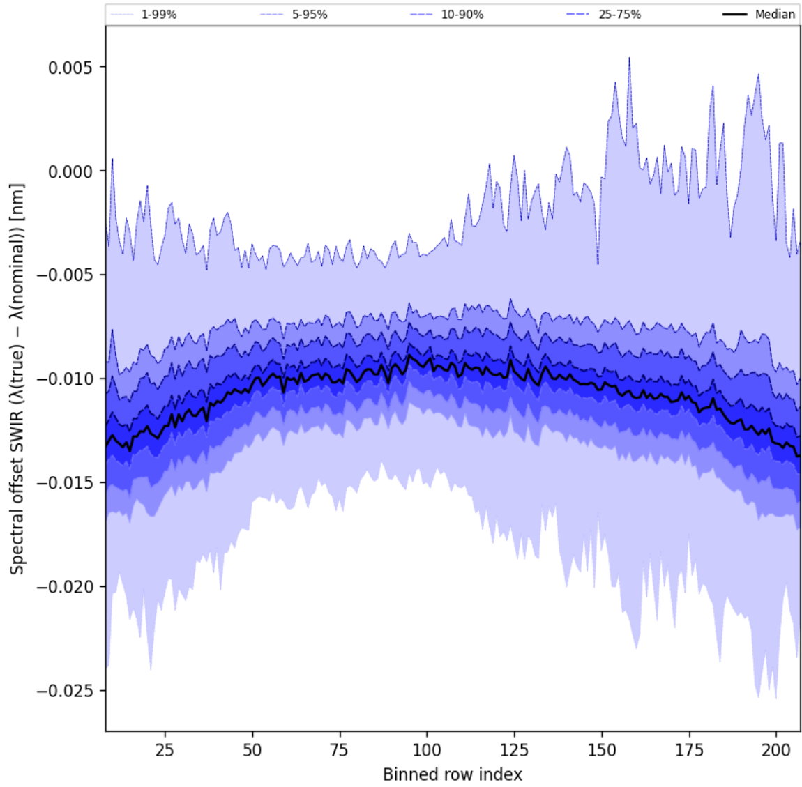
Figure 38: Along track statistics of “Spectral offset SWIR ( \lambda_{\text{true}} - \lambda_{\text{nominal}} )” for 2025-05-01 to 2025-05-03
