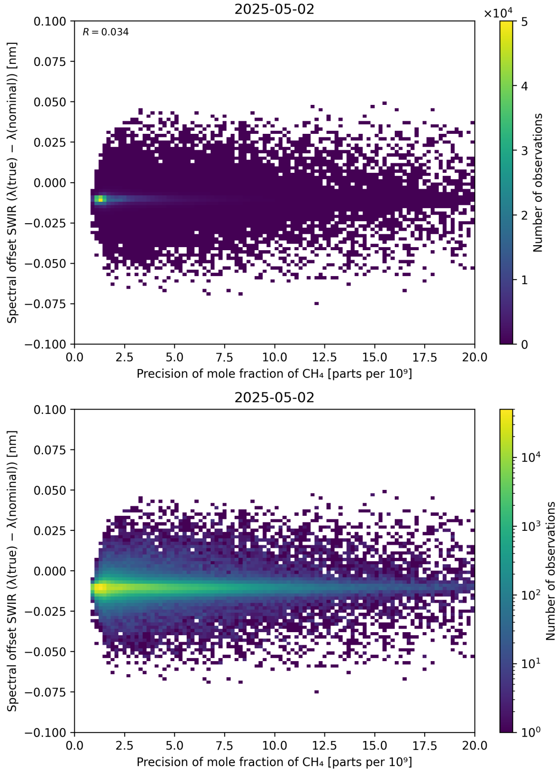
Figure 85: Scatter density plot of “Precision of mole fraction of \text{CH}_4 ” against “Spectral offset SWIR ( \lambda_{\text{true}} - \lambda_{\text{nominal}} )” for 2025-05-01 to 2025-05-03.
