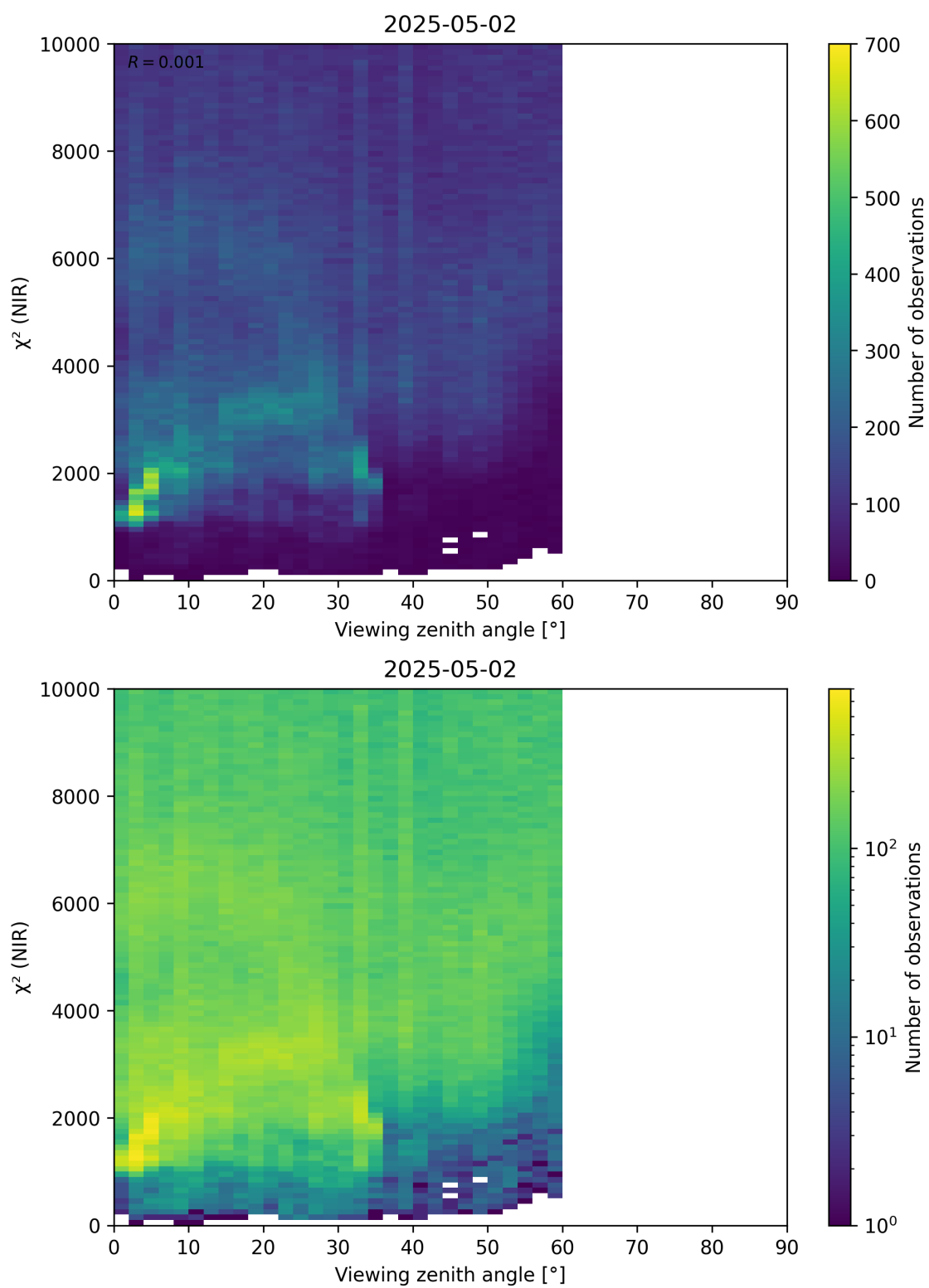
Figure 105: Scatter density plot of “Viewing zenith angle” against “ \chi^2 (NIR)” for 2025-05-01 to 2025-05-03.
