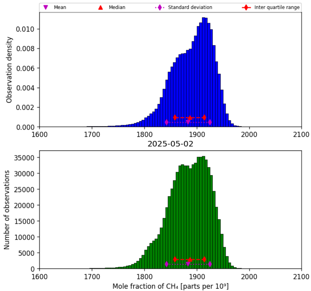
Figure 23: Histogram of "Mole fraction of CH 4 " for 2025-05-01 to 2025-05-03
