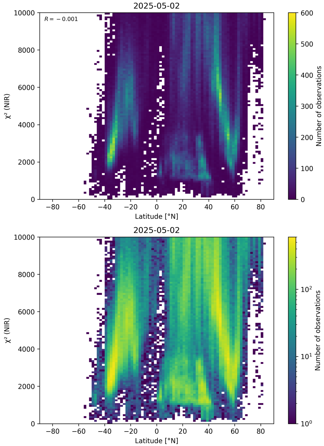
Figure 53: Scatter density plot of “Latitude” against “ \chi^2 (NIR)” for 2025-05-01 to 2025-05-03.
