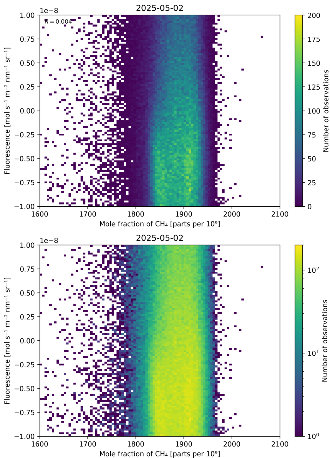
Figure 73: Scatter density plot of “Mole fraction of \text{CH}_4 ” against “Fluorescence” for 2025-05-01 to 2025-05-03.
