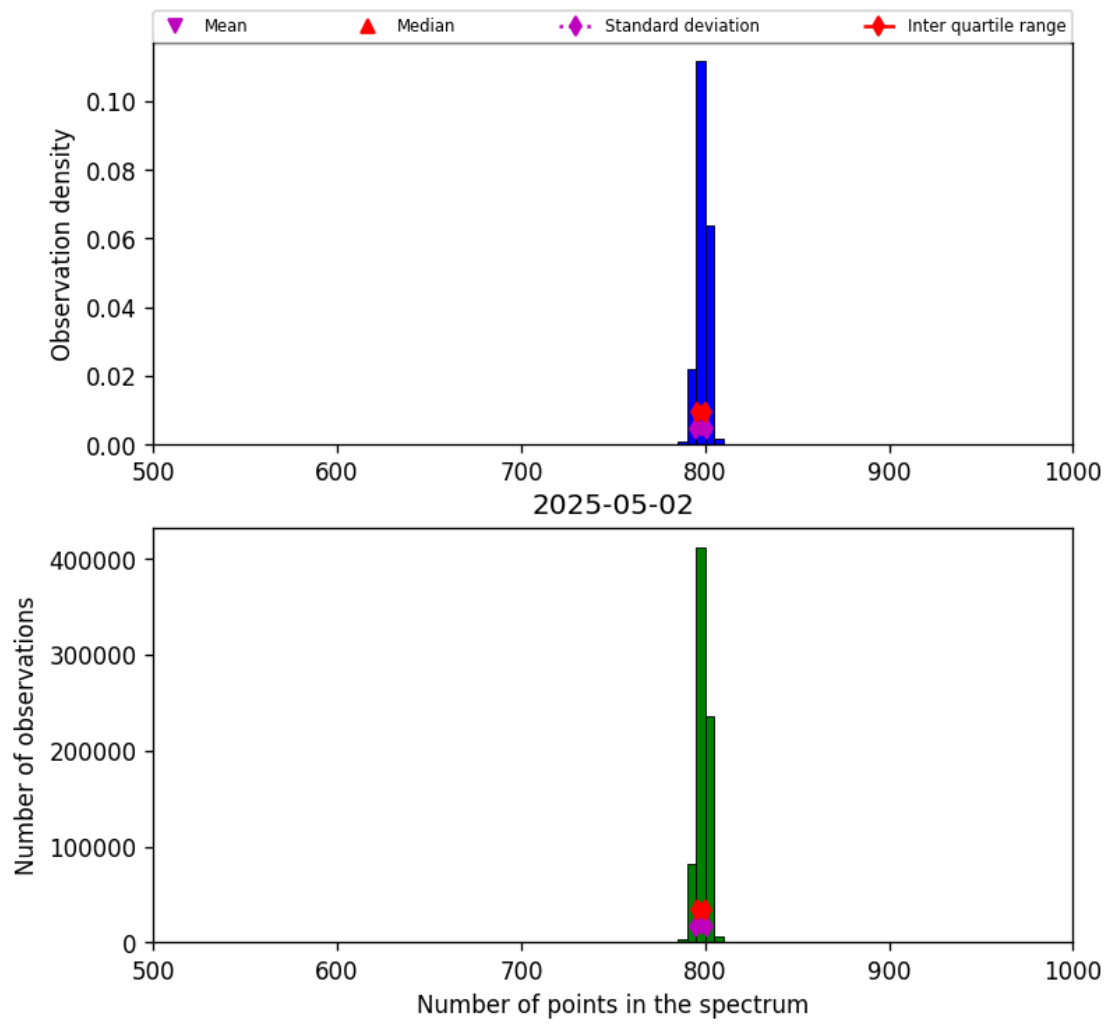
Figure 26: Histogram of “Number of points in the spectrum” for 2025-05-01 to 2025-05-03
