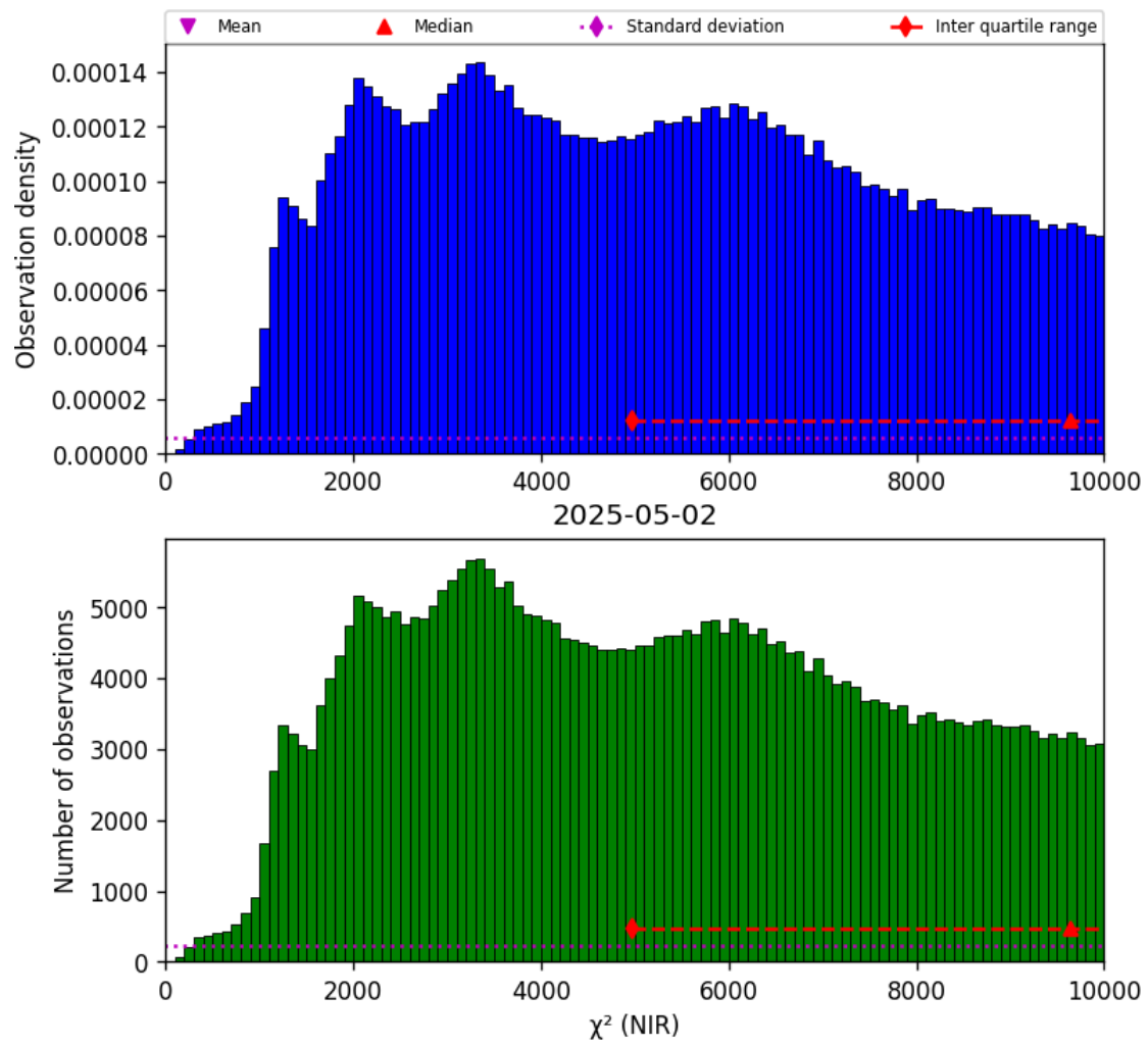
Figure 29: Histogram of “ \chi^2 (NIR)” for 2025-05-01 to 2025-05-03
