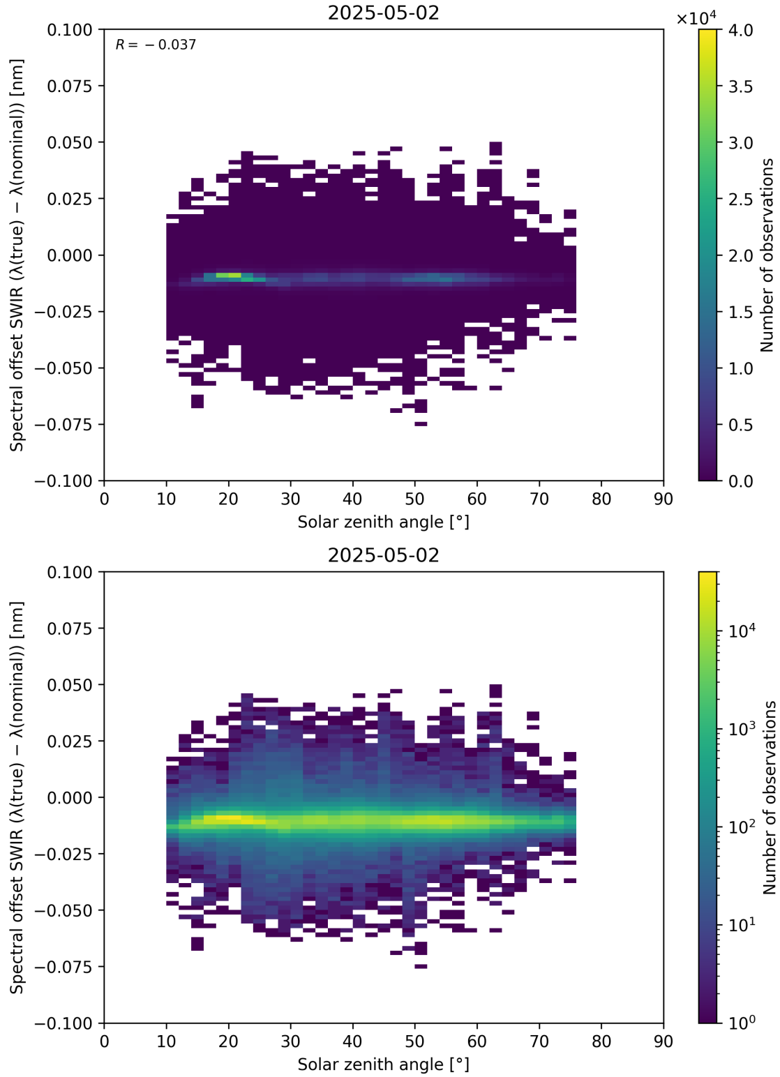
Figure 104: Scatter density plot of “Solar zenith angle” against “Spectral offset SWIR ( \lambda_{\text{true}} - \lambda_{\text{nominal}} )” for 2025-05-01 to 2025-05-03.
