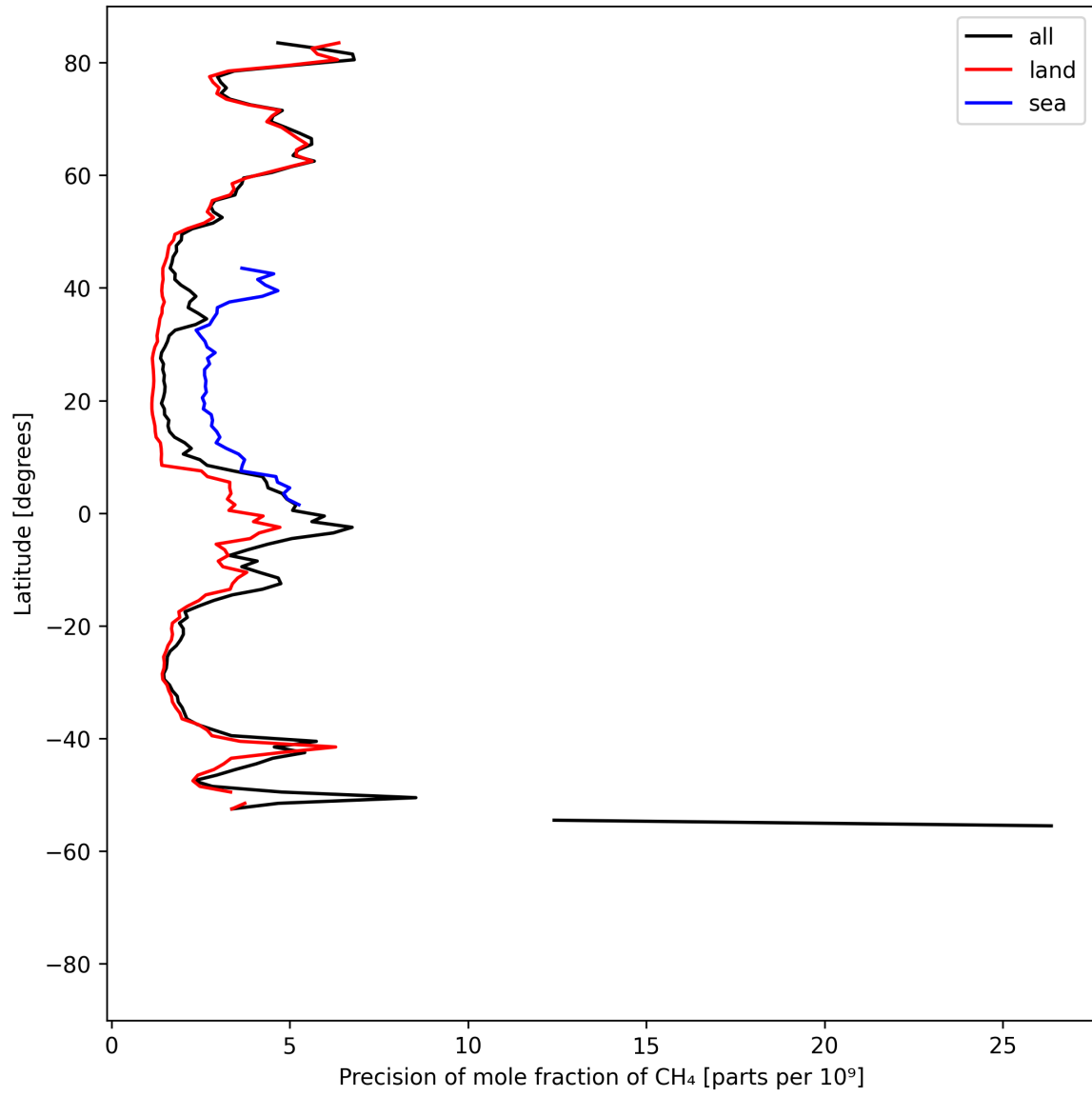
Figure 13: Zonal average of “Precision of mole fraction of CH 4 ” for 2025-05-01 to 2025-05-03.
