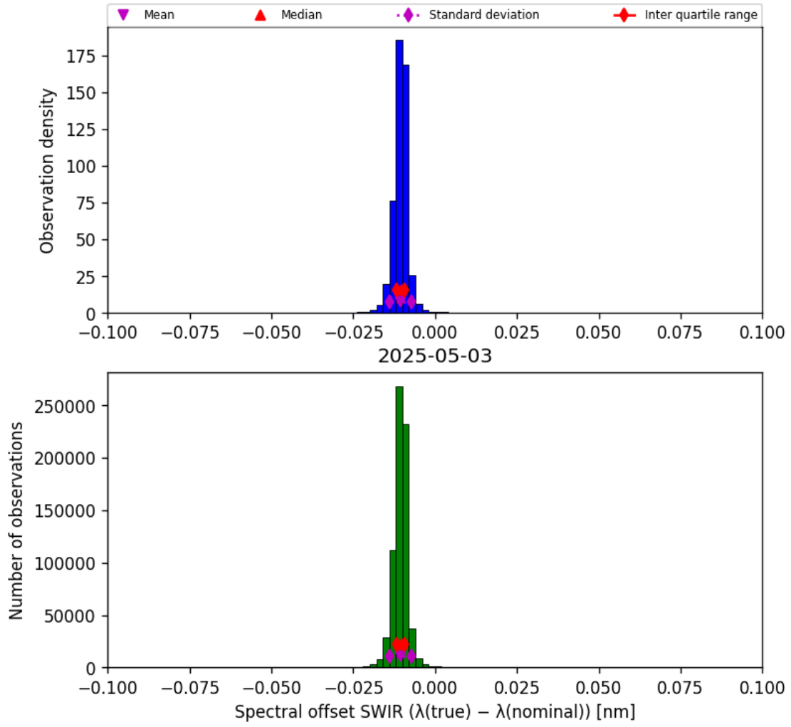
Figure 27: Histogram of “Spectral offset SWIR ( \lambda_{\text{true}} - \lambda_{\text{nominal}} )” for 2025-05-02 to 2025-05-04
