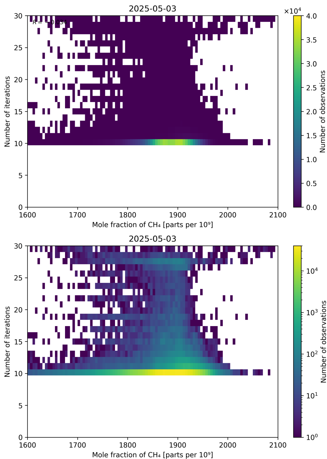
Figure 76: Scatter density plot of “Mole fraction of CH 4 ” against “Number of iterations” for 2025-05-02 to 2025-05-04.
