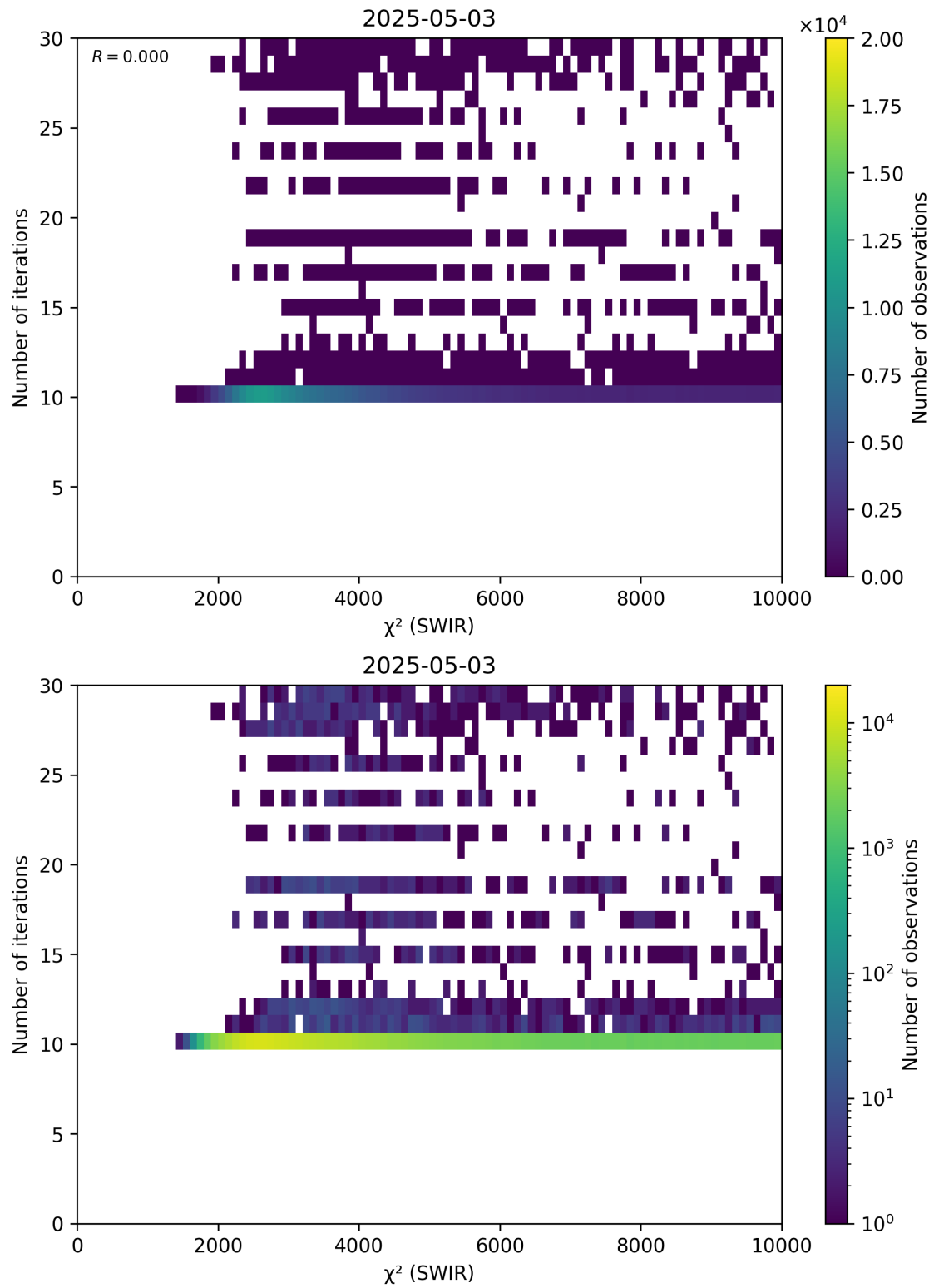
Figure 50: Scatter density plot of “ \chi^2 (SWIR)” against “Number of iterations” for 2025-05-02 to 2025-05-04.
