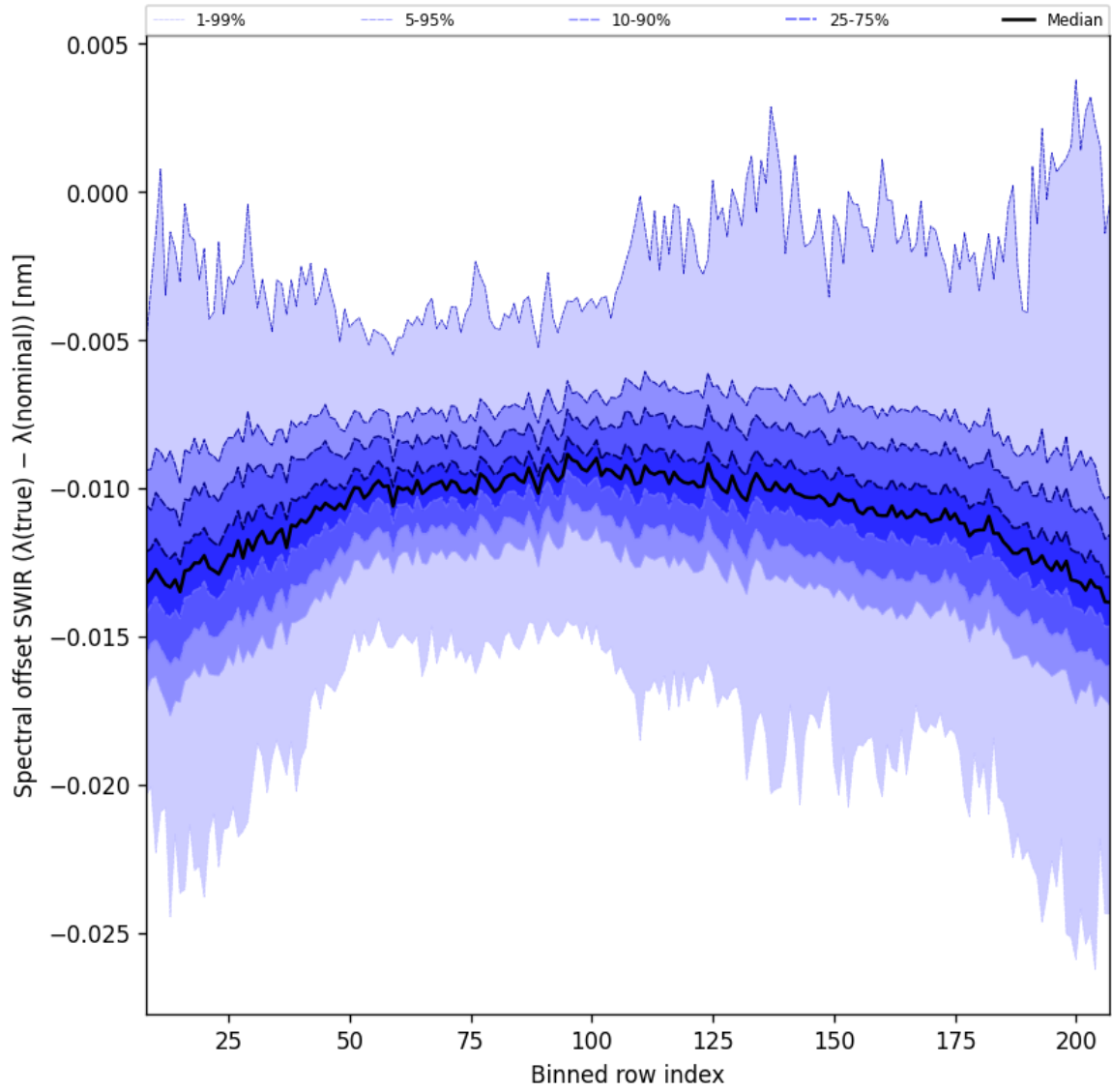
Figure 38: Along track statistics of “Spectral offset SWIR ( \lambda_{\text{true}} - \lambda_{\text{nominal}} )” for 2025-05-02 to 2025-05-04
