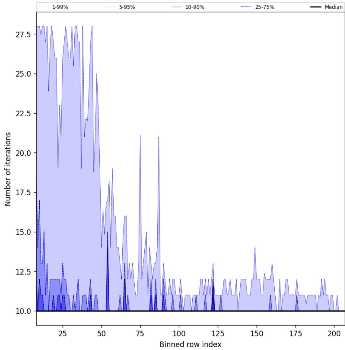
Figure 42: Along track statistics of “Number of iterations” for 2025-05-02 to 2025-05-04
