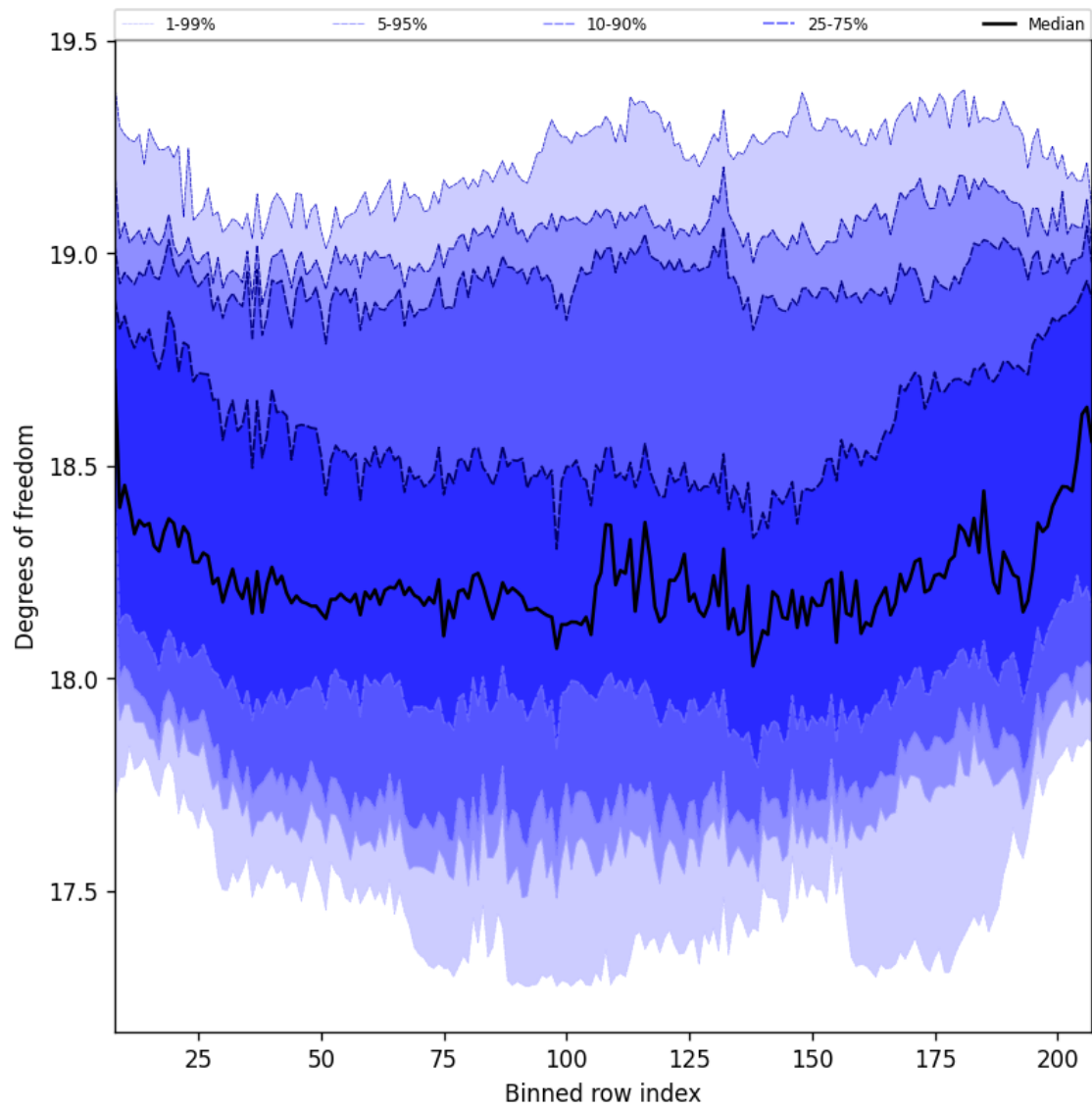
Figure 41: Along track statistics of “Degrees of freedom” for 2025-05-02 to 2025-05-04
