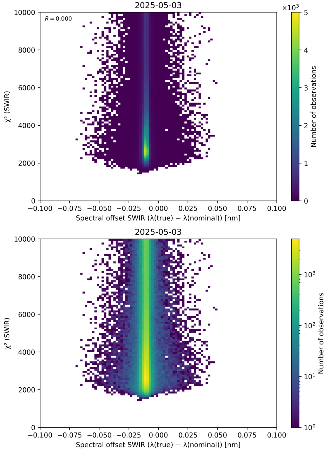
Figure 118: Scatter density plot of “Spectral offset SWIR ( \lambda_{\text{true}} - \lambda_{\text{nominal}} )” against “ \chi^2 (SWIR)” for 2025-05-02 to 2025-05-04.
