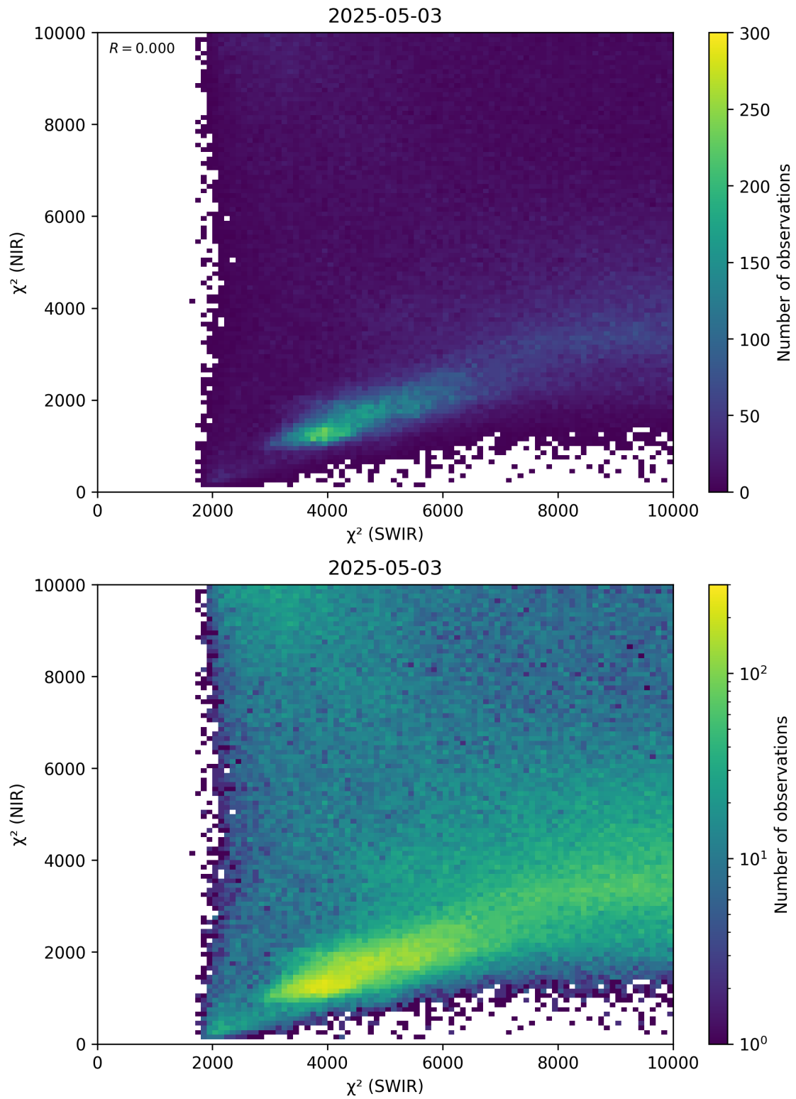
Figure 47: Scatter density plot of “ \chi^2 (SWIR)” against “ \chi^2 (NIR)” for 2025-05-02 to 2025-05-04.
