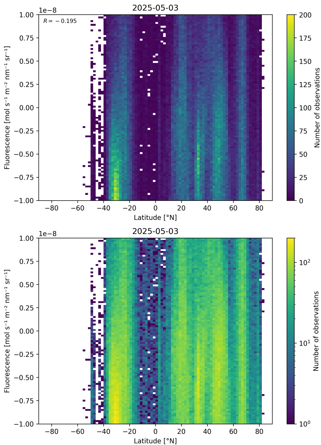
Figure 56: Scatter density plot of “Latitude” against “Fluorescence” for 2025-05-02 to 2025-05-04.
