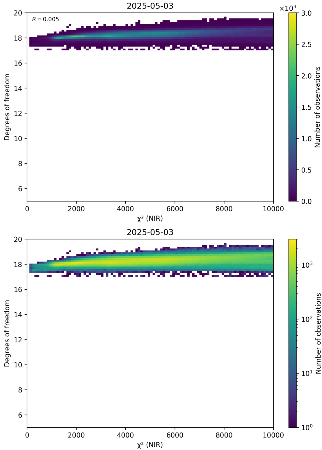
Figure 44: Scatter density plot of “ \chi^2 (NIR)” against “Degrees of freedom” for 2025-05-02 to 2025-05-04.
