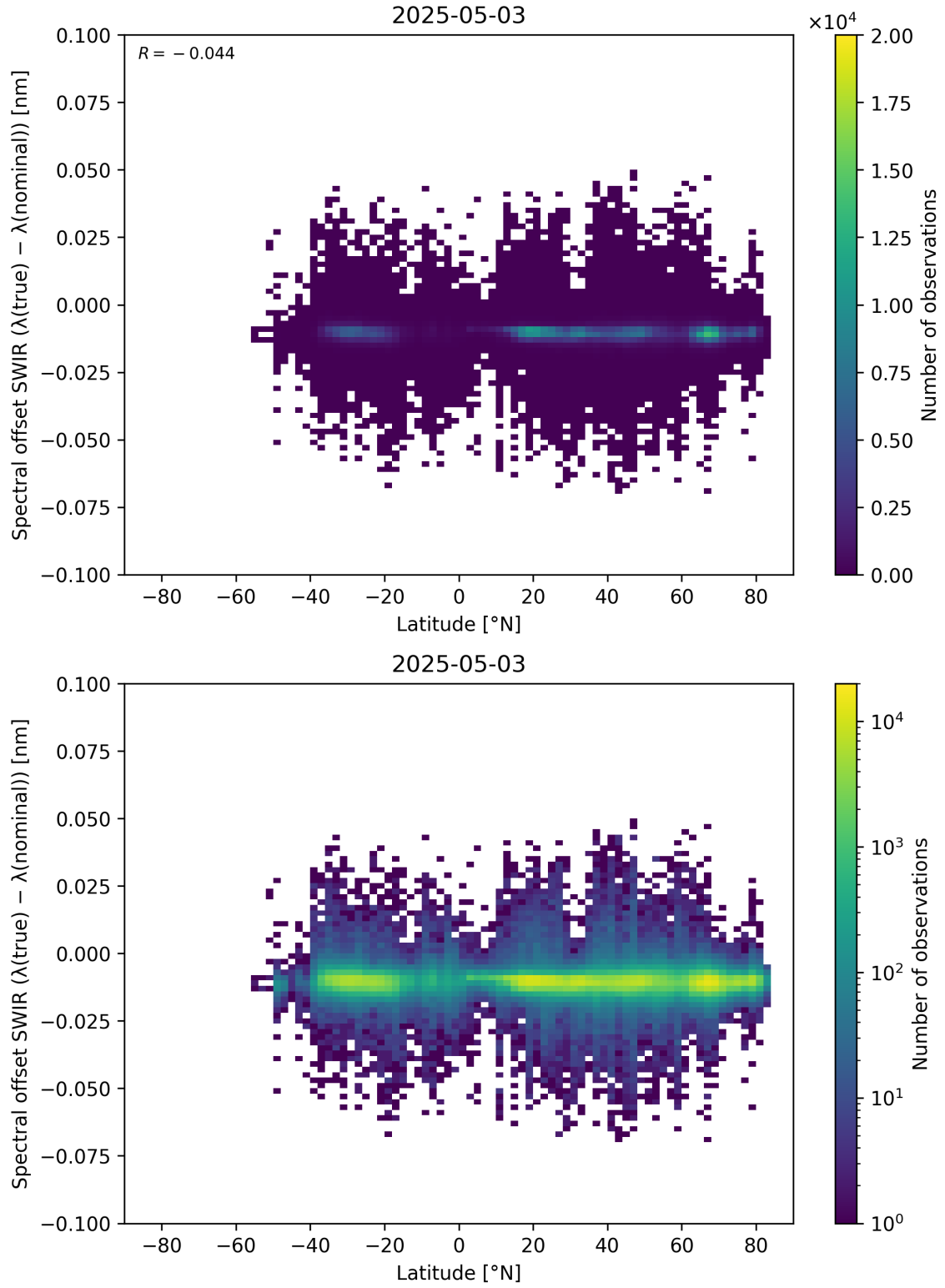
Figure 62: Scatter density plot of “Latitude” against “Spectral offset SWIR ( \lambda_{\text{true}} - \lambda_{\text{nominal}} )” for 2025-05-02 to 2025-05-04.
