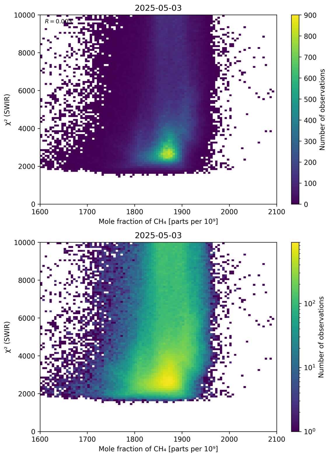
Figure 71: Scatter density plot of “Mole fraction of \text{CH}_4 ” against “ \chi^2 (SWIR)” for 2025-05-02 to 2025-05-04.
