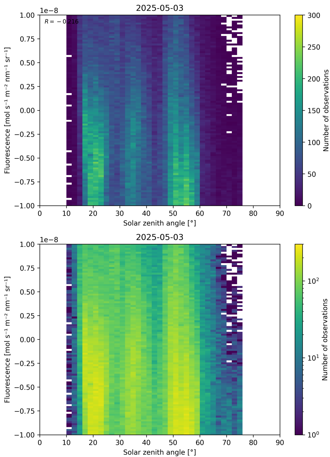
Figure 97: Scatter density plot of “Solar zenith angle” against “Fluorescence” for 2025-05-02 to 2025-05-04.
