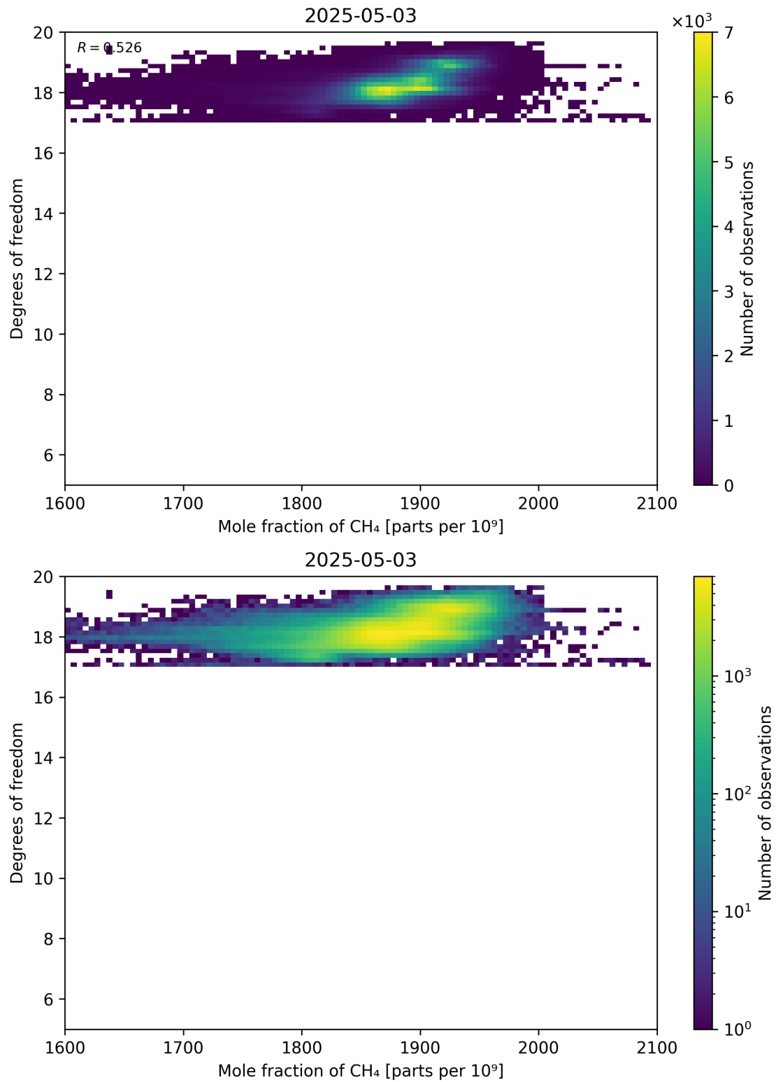
Figure 72: Scatter density plot of “Mole fraction of CH 4 ” against “Degrees of freedom” for 2025-05-02 to 2025-05-04.
