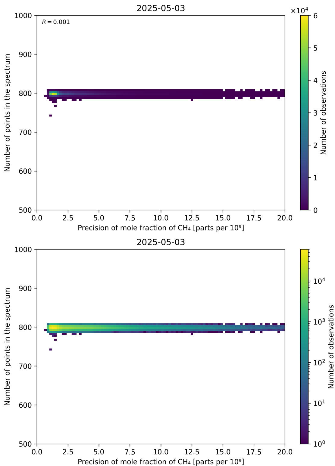
Figure 84: Scatter density plot of “Precision of mole fraction of CH 4 ” against “Number of points in the spectrum” for 2025-05-02 to 2025-05-04.
