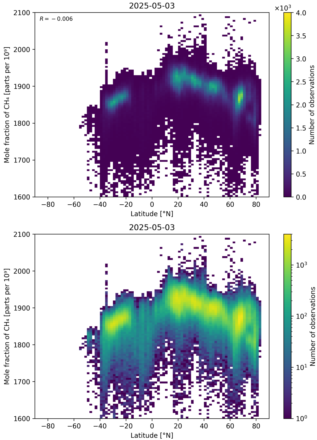
Figure 57: Scatter density plot of “Latitude” against “Mole fraction of \text{CH}_4 ” for 2025-05-02 to 2025-05-04.
