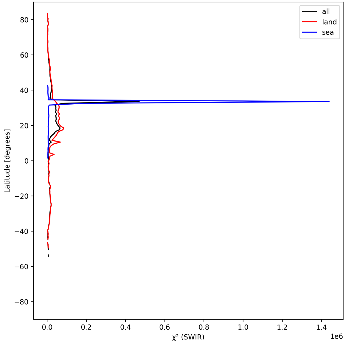
Figure 17: Zonal average of “ \chi^2 (SWIR)” for 2025-05-02 to 2025-05-04.
