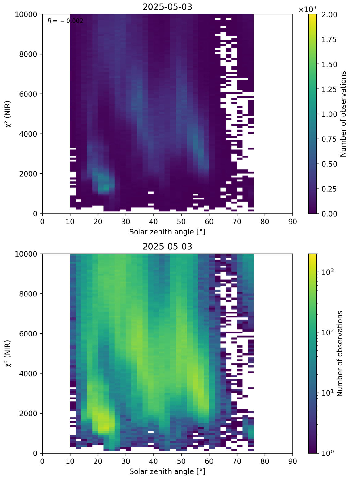
Figure 94: Scatter density plot of “Solar zenith angle” against “ \chi^2 (NIR)” for 2025-05-02 to 2025-05-04.
