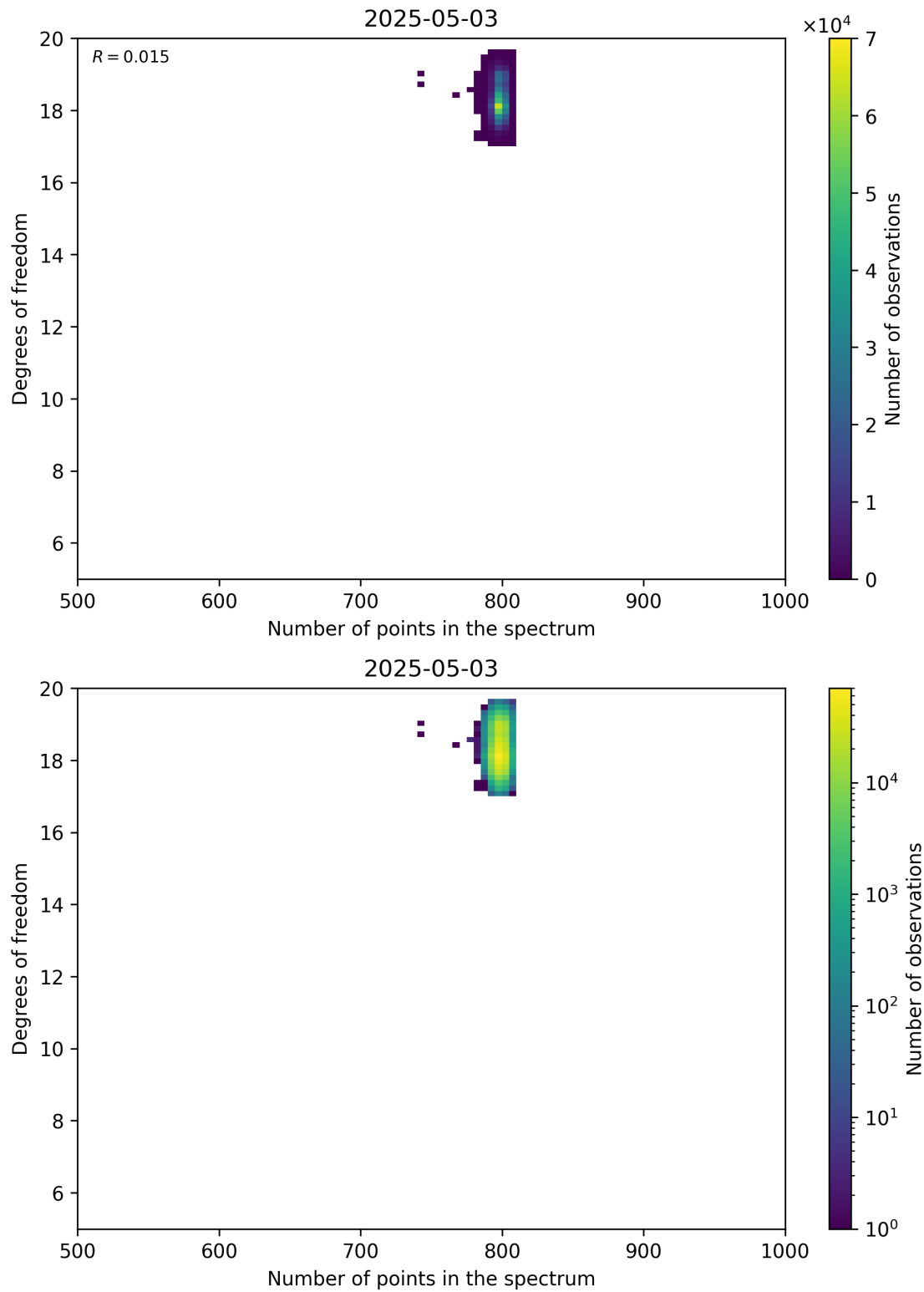
Figure 90: Scatter density plot of “Number of points in the spectrum” against “Degrees of freedom” for 2025-05-02 to 2025-05-04.
