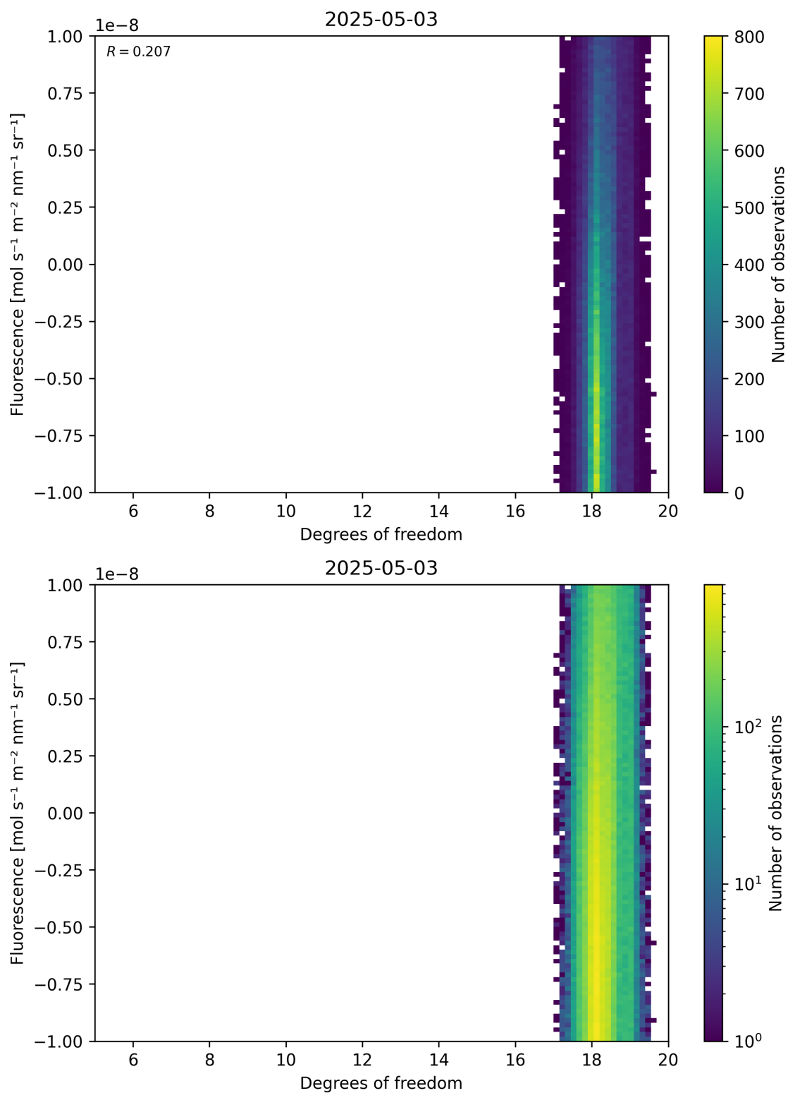
Figure 51: Scatter density plot of “Degrees of freedom” against “Fluorescence” for 2025-05-02 to 2025-05-04.
