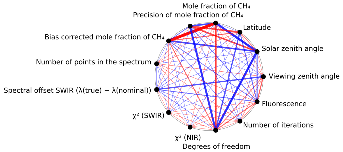
Figure 1: Map of correlation graph for 2025-05-02 to 2025-05-04.
