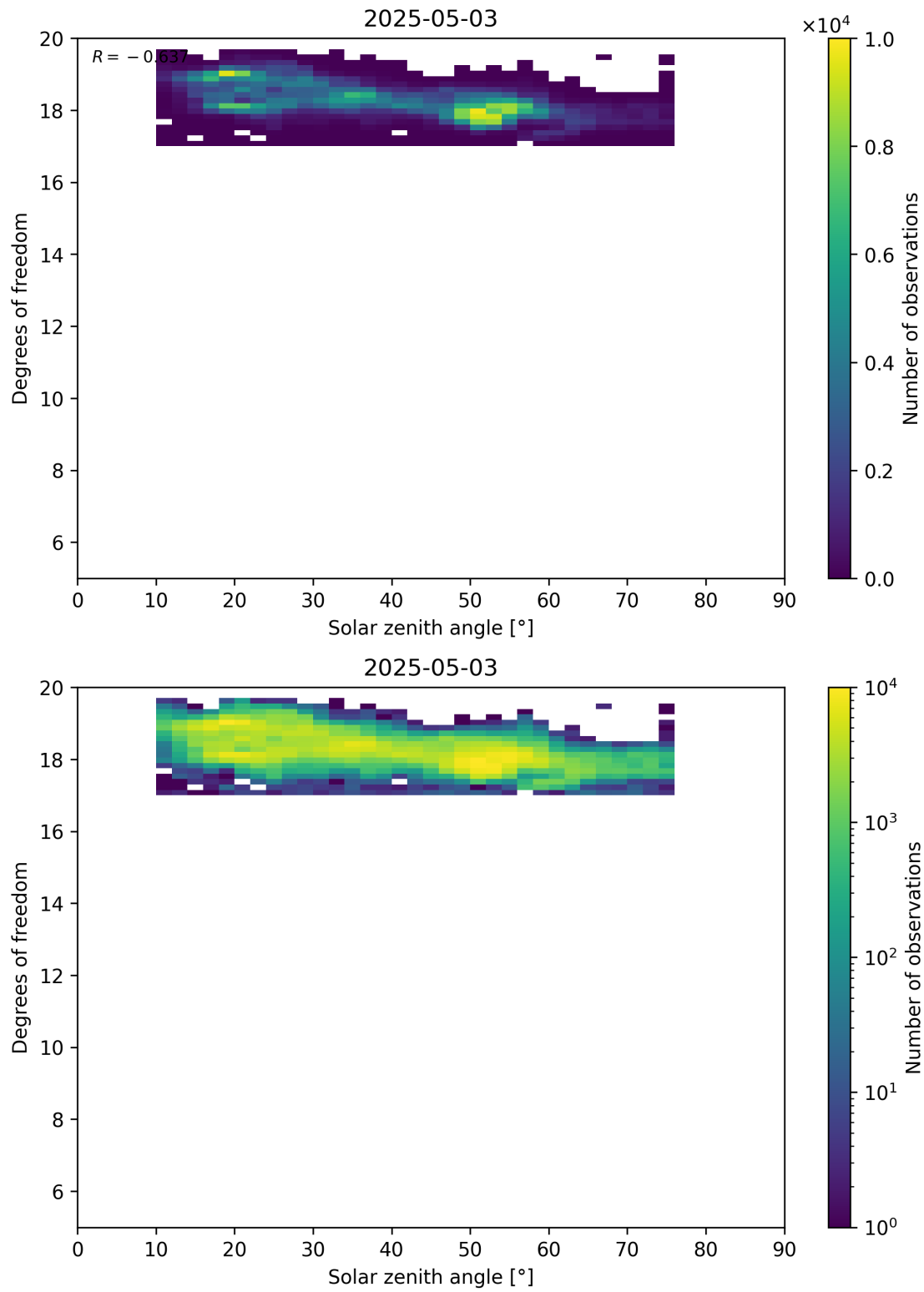
Figure 96: Scatter density plot of “Solar zenith angle” against “Degrees of freedom” for 2025-05-02 to 2025-05-04.
