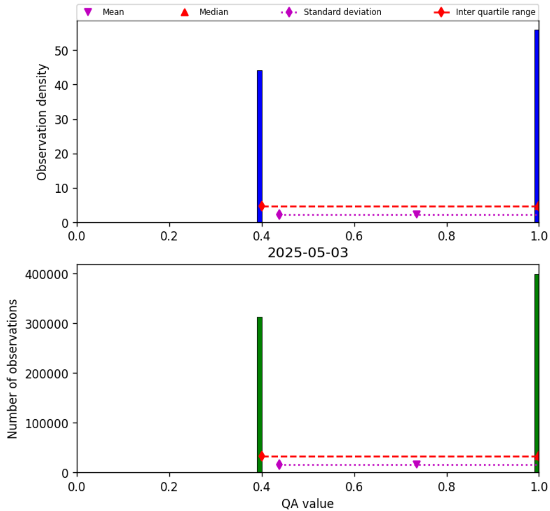
Figure 22: Histogram of “QA value” for 2025-05-02 to 2025-05-04
