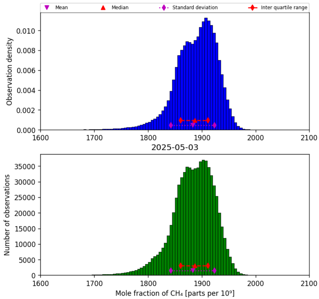
Figure 23: Histogram of “Mole fraction of CH 4 ” for 2025-05-02 to 2025-05-04
