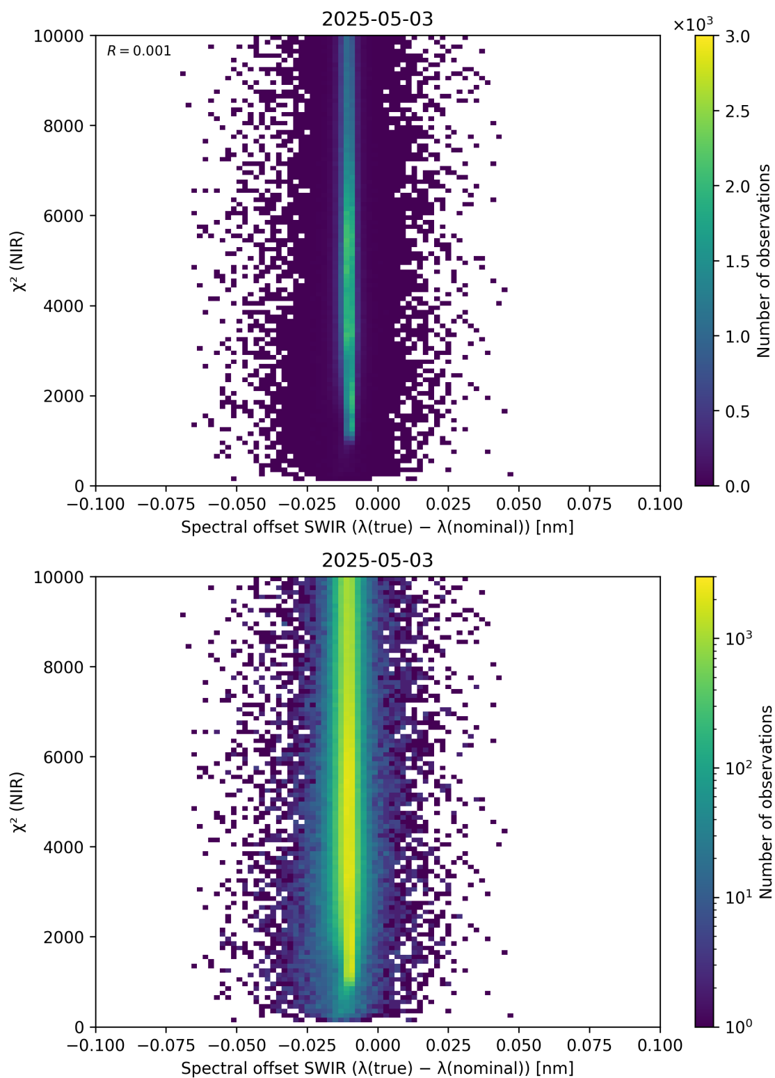
Figure 117: Scatter density plot of “Spectral offset SWIR ( \lambda_{\text{true}} - \lambda_{\text{nominal}} )” against “ \chi^2 (NIR)” for 2025-05-02 to 2025-05-04.
