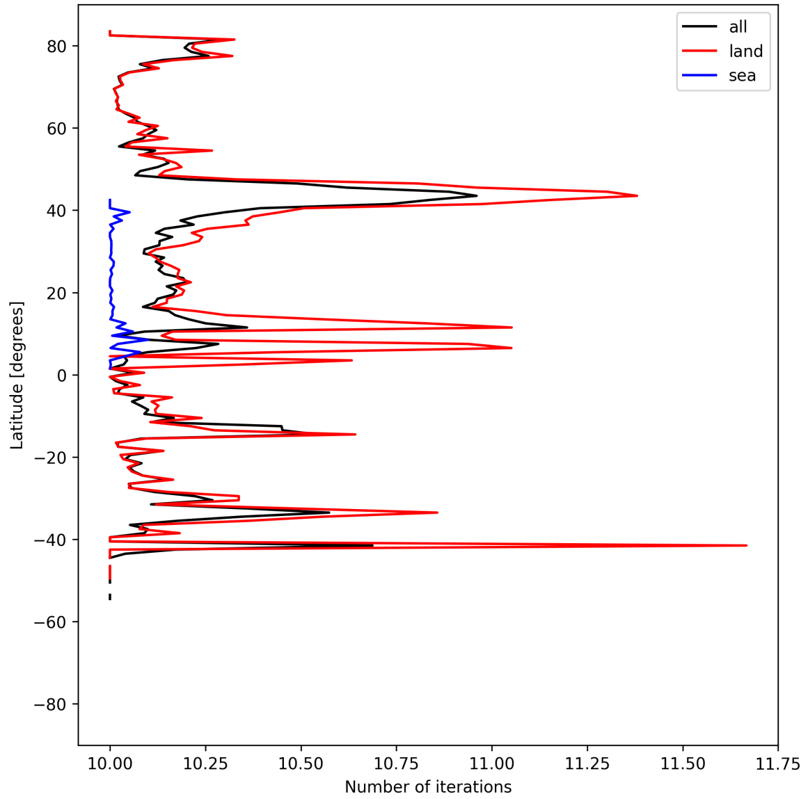
Figure 20: Zonal average of “Number of iterations” for 2025-05-02 to 2025-05-04.
