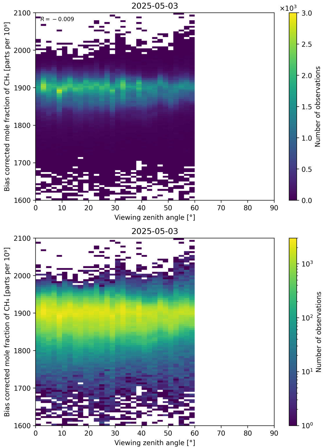
Figure 111: Scatter density plot of “Viewing zenith angle” against “Bias corrected mole fraction of CH 4 ” for 2025-05-02 to 2025-05-04.
