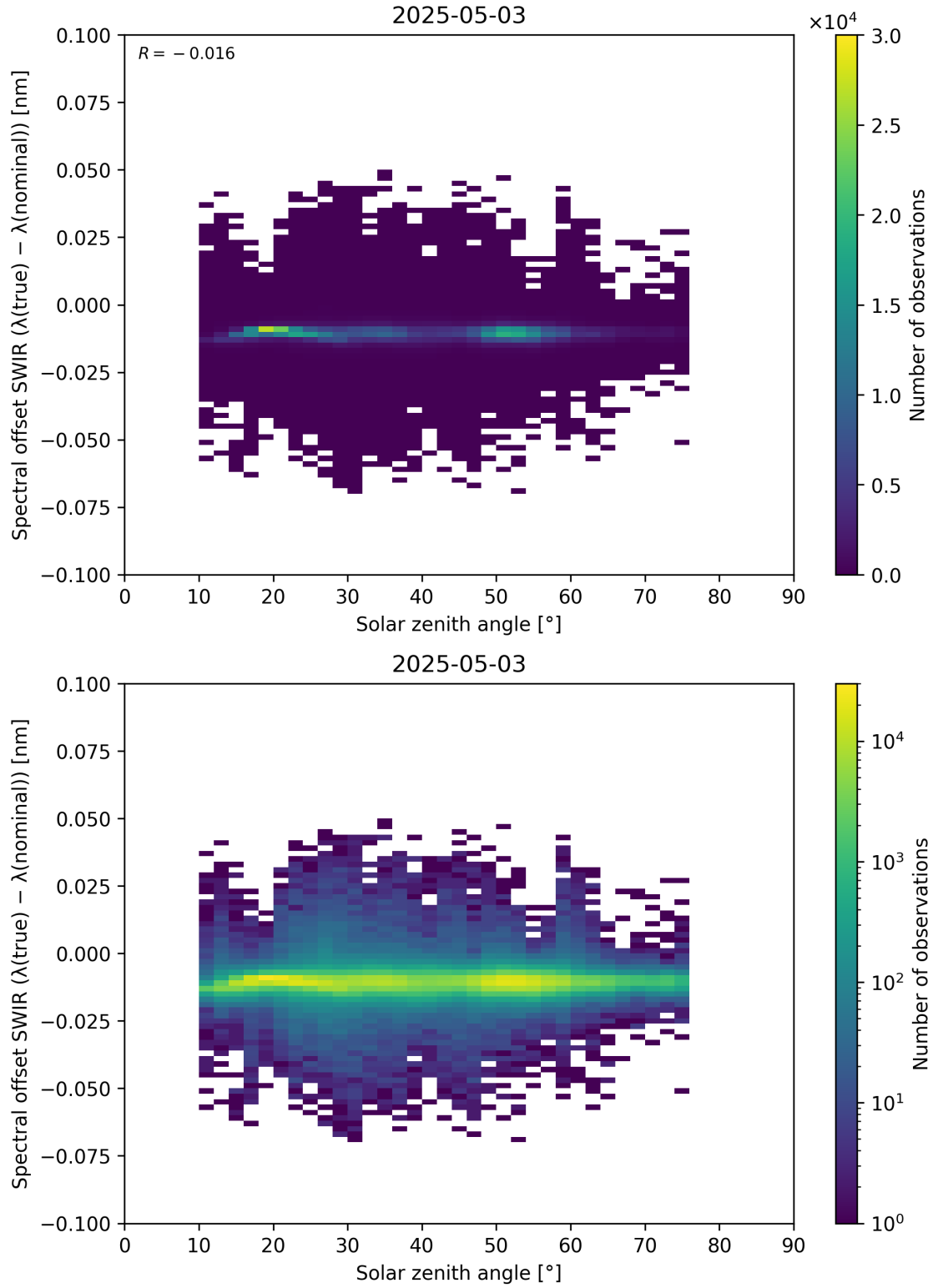
Figure 104: Scatter density plot of “Solar zenith angle” against “Spectral offset SWIR ( \lambda_{\text{true}} - \lambda_{\text{nominal}} )” for 2025-05-02 to 2025-05-04.
