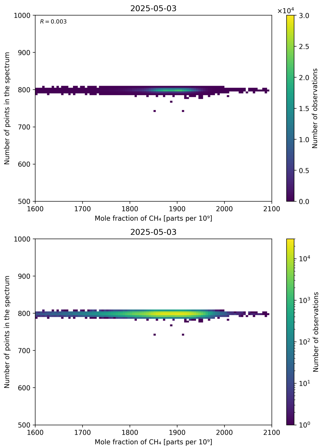
Figure 77: Scatter density plot of “Mole fraction of CH 4 ” against “Number of points in the spectrum” for 2025-05-02 to 2025-05-04.
