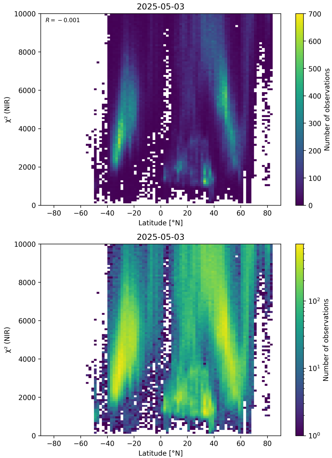
Figure 53: Scatter density plot of “Latitude” against “ \chi^2 (NIR)” for 2025-05-02 to 2025-05-04.
