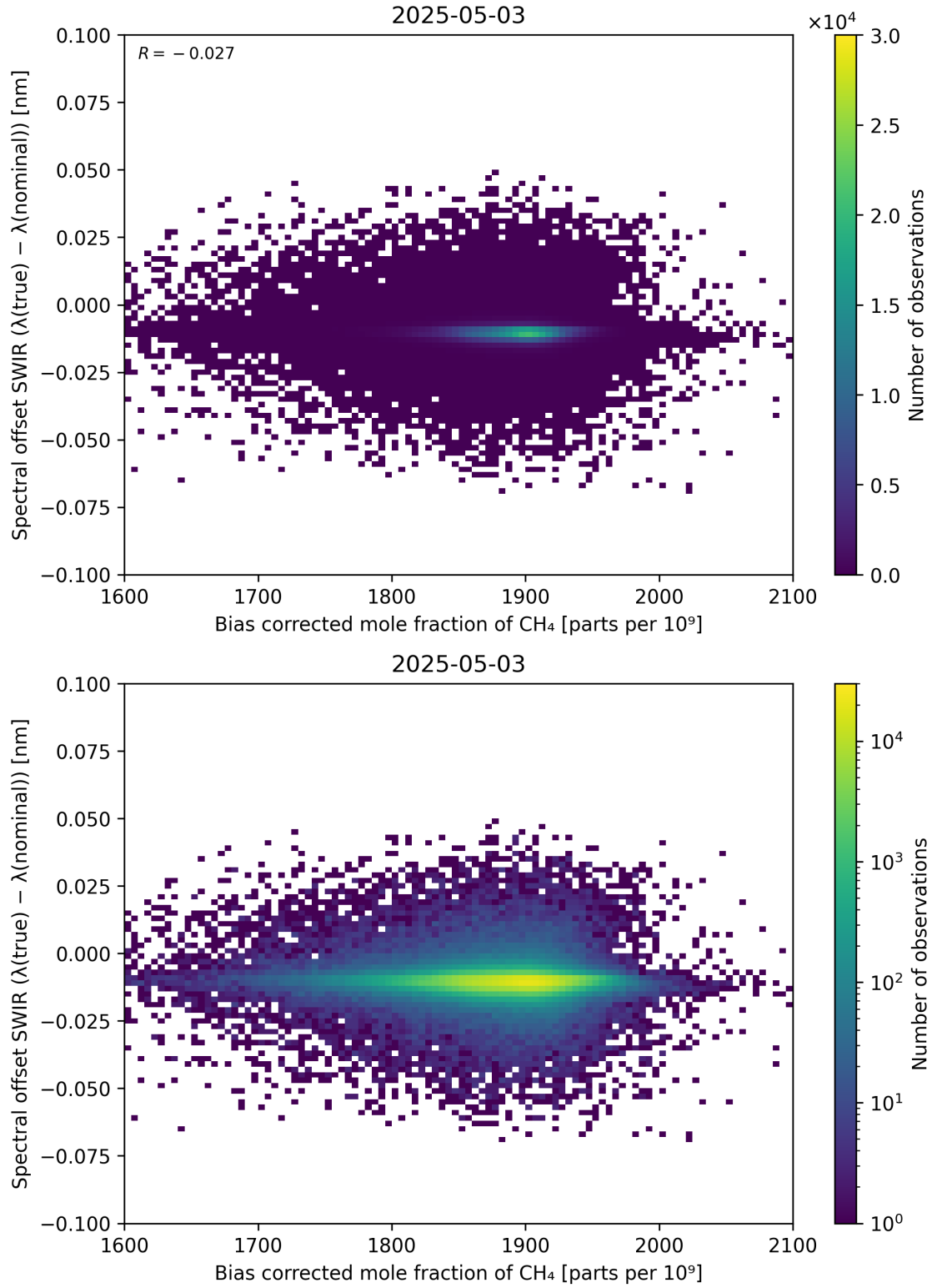
Figure 69: Scatter density plot of “Bias corrected mole fraction of CH 4 ” against “Spectral offset SWIR ( \lambda_{\text{true}} - \lambda_{\text{nominal}} )” for 2025-05-02 to 2025-05-04.
