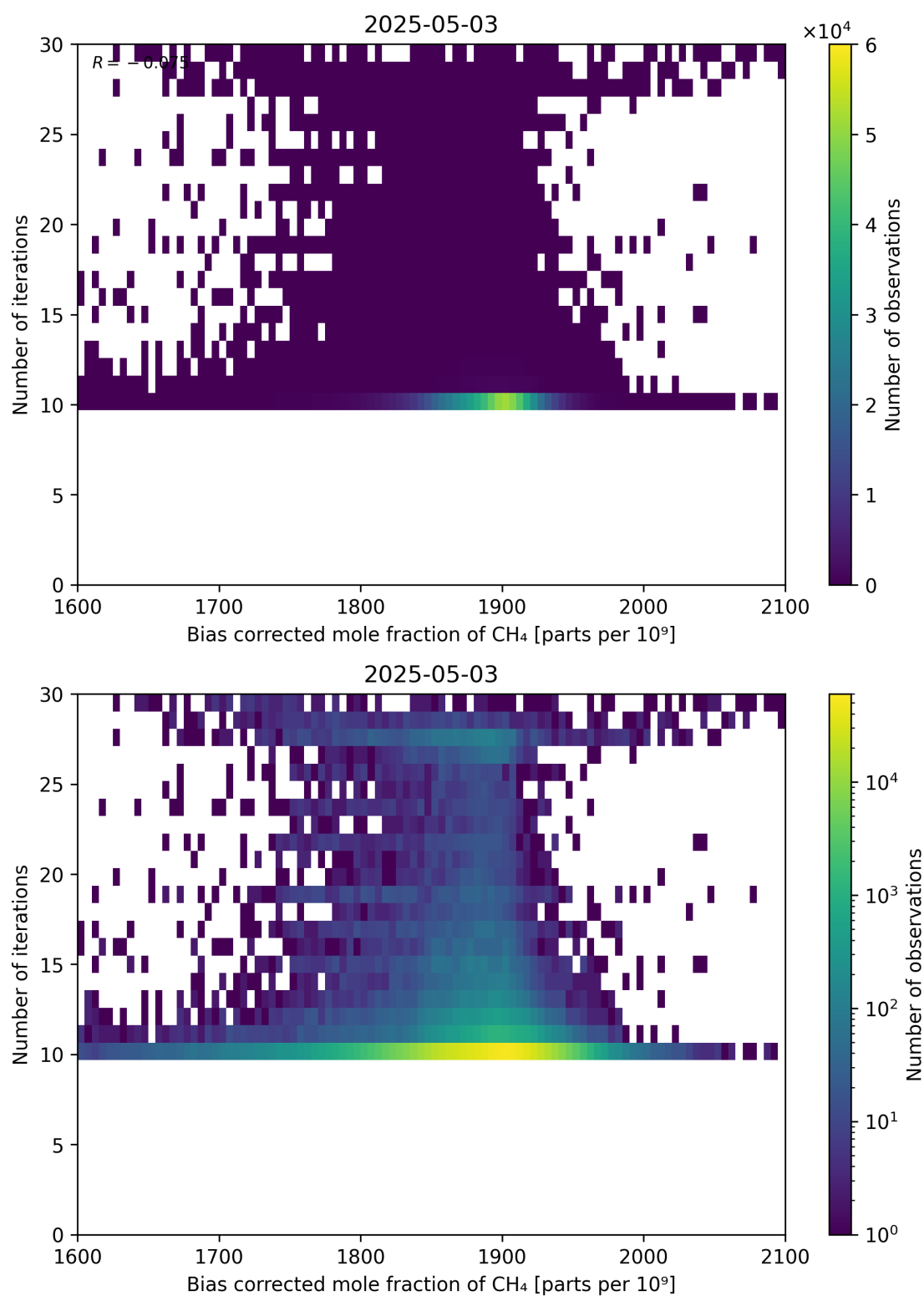
Figure 67: Scatter density plot of “Bias corrected mole fraction of CH 4 ” against “Number of iterations” for 2025-05-02 to 2025-05-04.
