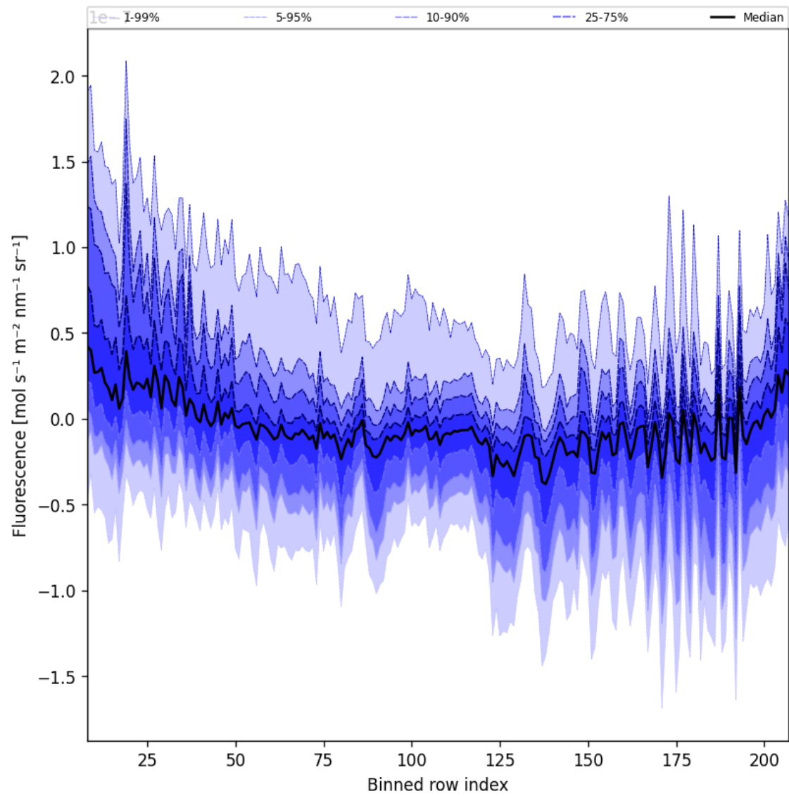
Figure 43: Along track statistics of “Fluorescence” for 2025-05-02 to 2025-05-04
