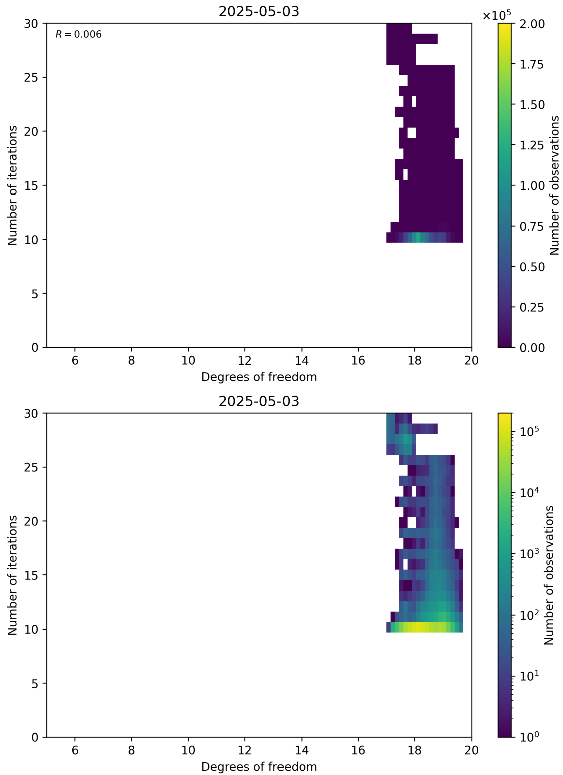
Figure 52: Scatter density plot of “Degrees of freedom” against “Number of iterations” for 2025-05-02 to 2025-05-04.
