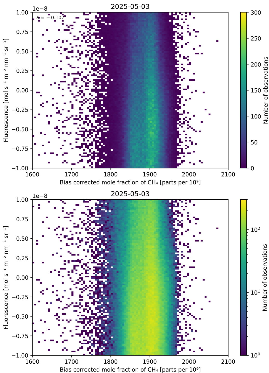
Figure 66: Scatter density plot of “Bias corrected mole fraction of \text{CH}_4 ” against “Fluorescence” for 2025-05-02 to 2025-05-04.
