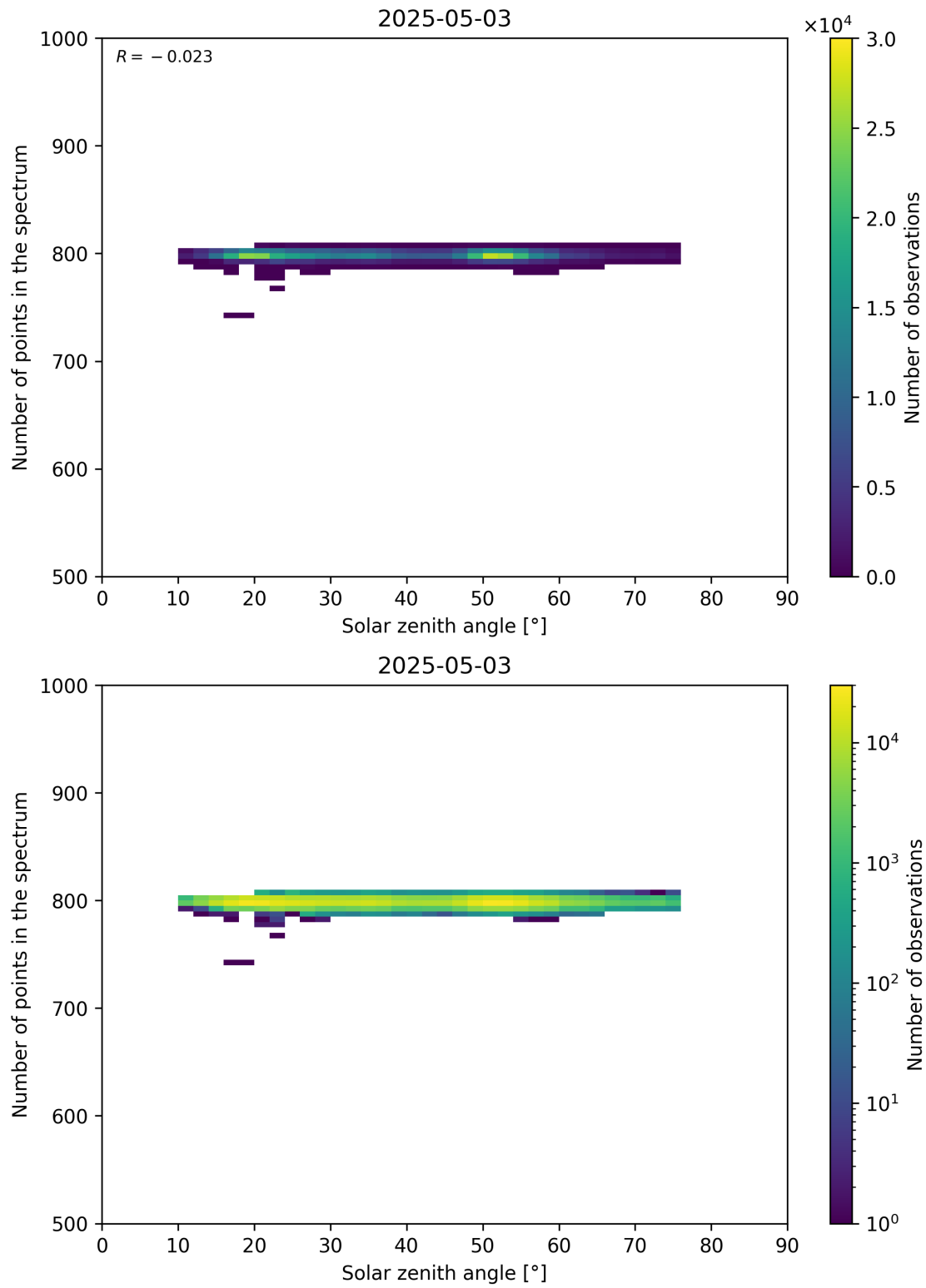
Figure 103: Scatter density plot of “Solar zenith angle” against “Number of points in the spectrum” for 2025-05-02 to 2025-05-04.
