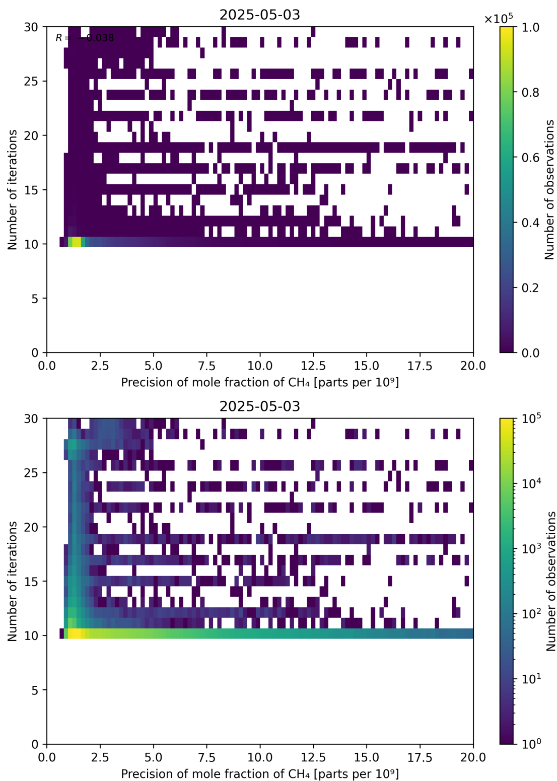
Figure 83: Scatter density plot of “Precision of mole fraction of CH 4 ” against “Number of iterations” for 2025-05-02 to 2025-05-04.
