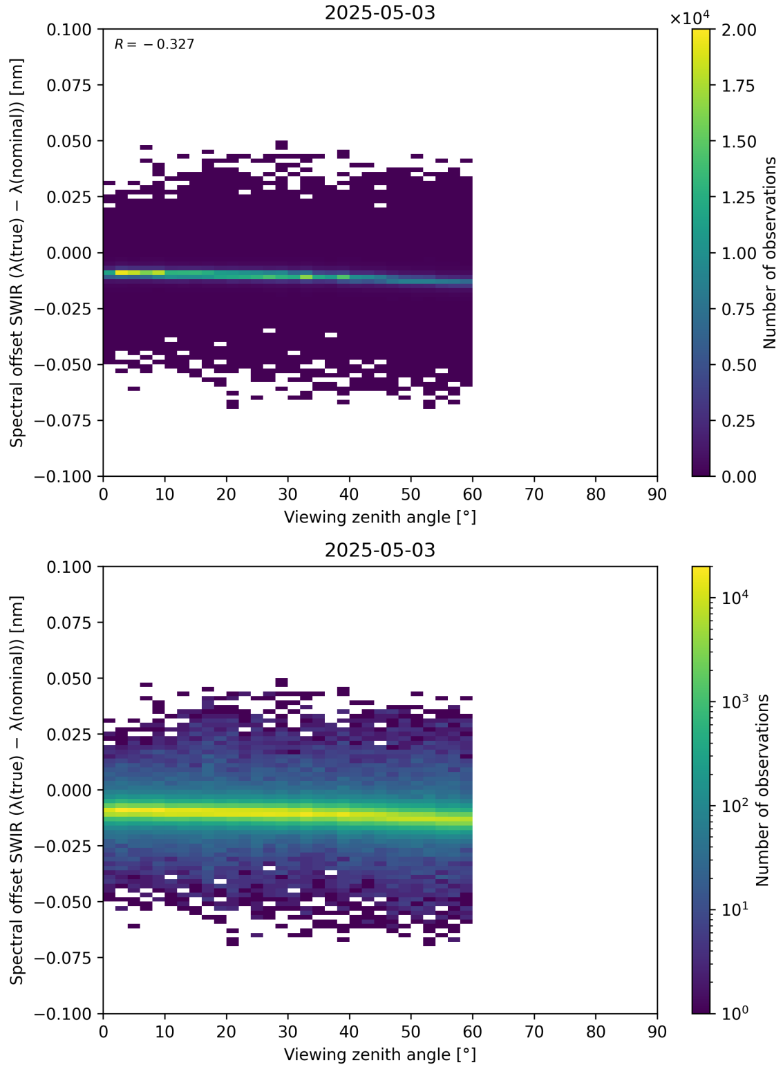
Figure 116: Scatter density plot of “Viewing zenith angle” against “Spectral offset SWIR ( \lambda_{\text{true}} - \lambda_{\text{nominal}} )” for 2025-05-02 to 2025-05-04.
