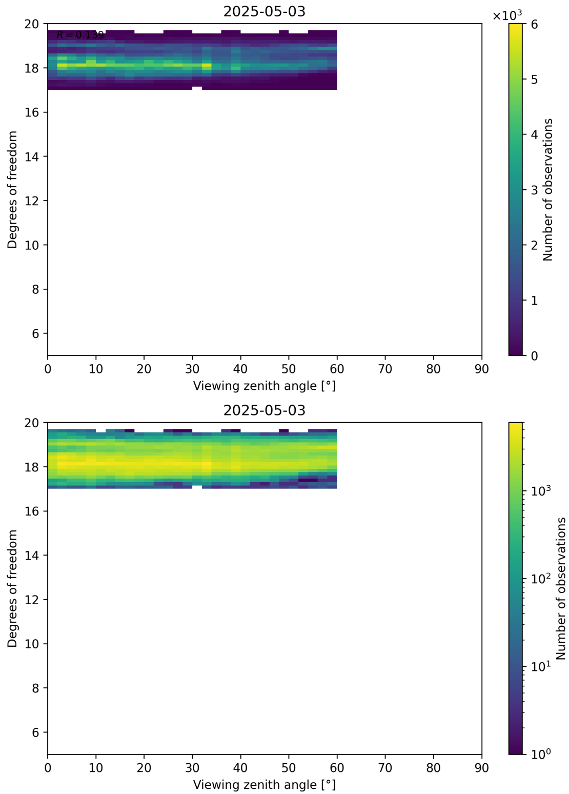
Figure 107: Scatter density plot of “Viewing zenith angle” against “Degrees of freedom” for 2025-05-02 to 2025-05-04.
