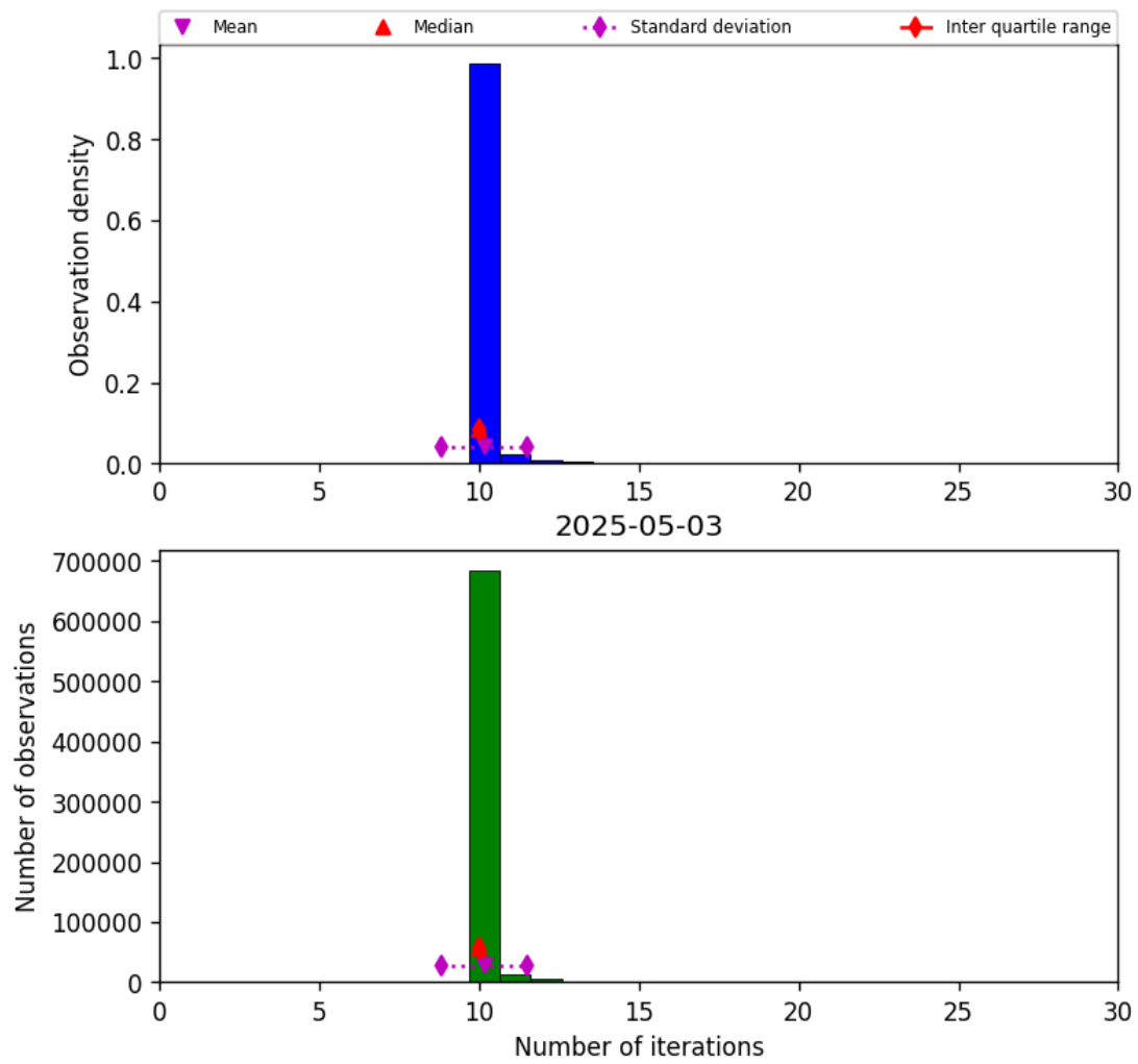
Figure 31: Histogram of “Number of iterations” for 2025-05-02 to 2025-05-04
