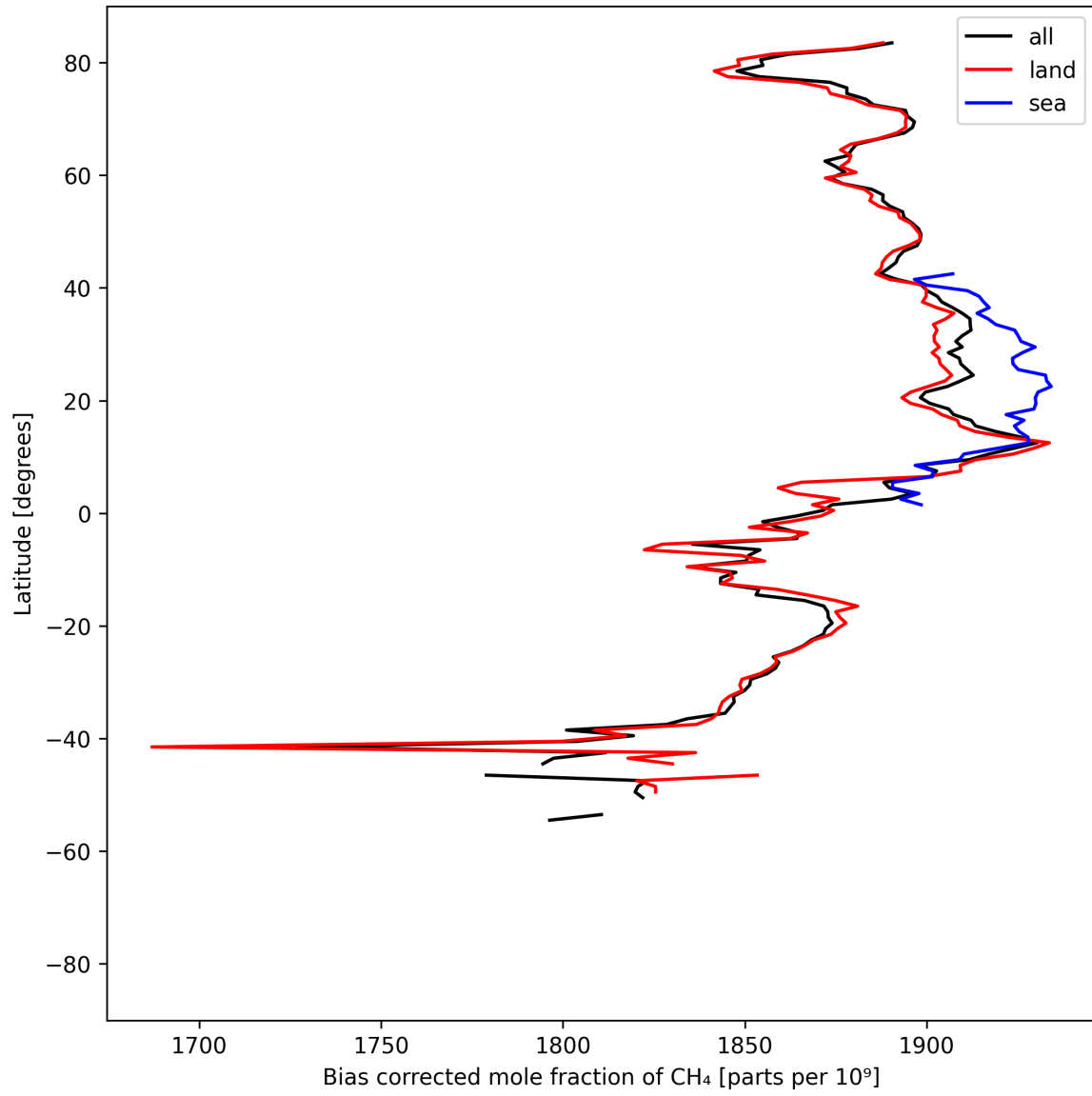
Figure 14: Zonal average of “Bias corrected mole fraction of CH 4 ” for 2025-05-02 to 2025-05-04.
