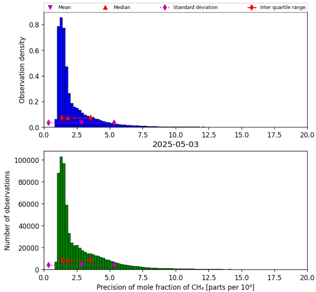
Figure 24: Histogram of “Precision of mole fraction of CH 4 ” for 2025-05-02 to 2025-05-04
