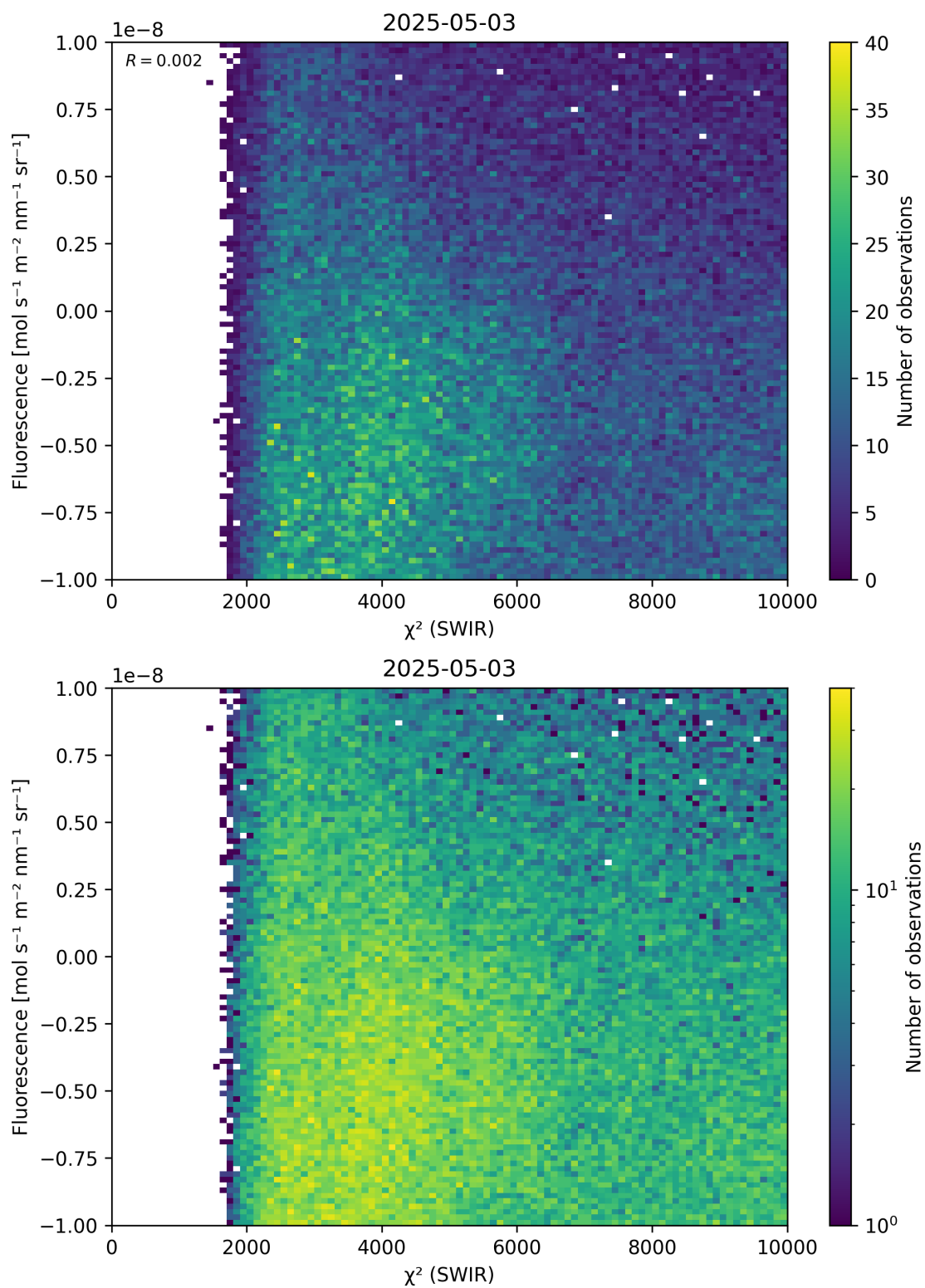
Figure 49: Scatter density plot of “ \chi^2 (SWIR)” against “Fluorescence” for 2025-05-02 to 2025-05-04.
