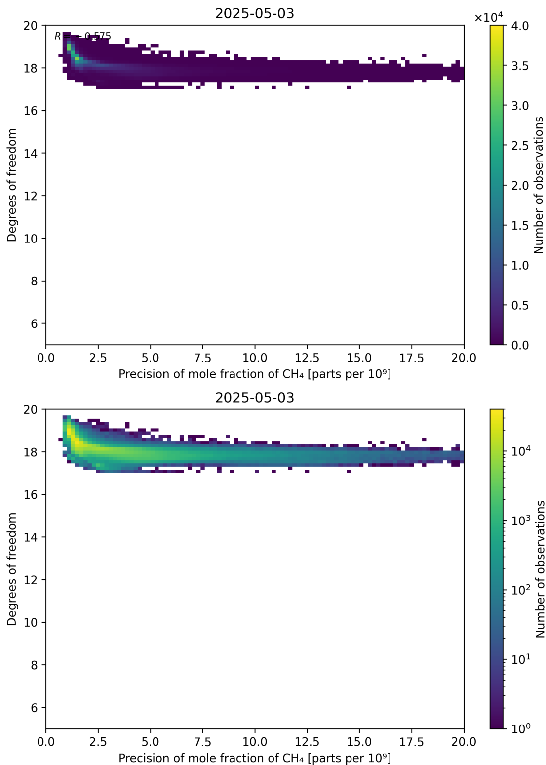
Figure 80: Scatter density plot of “Precision of mole fraction of CH 4 ” against “Degrees of freedom” for 2025-05-02 to 2025-05-04.
