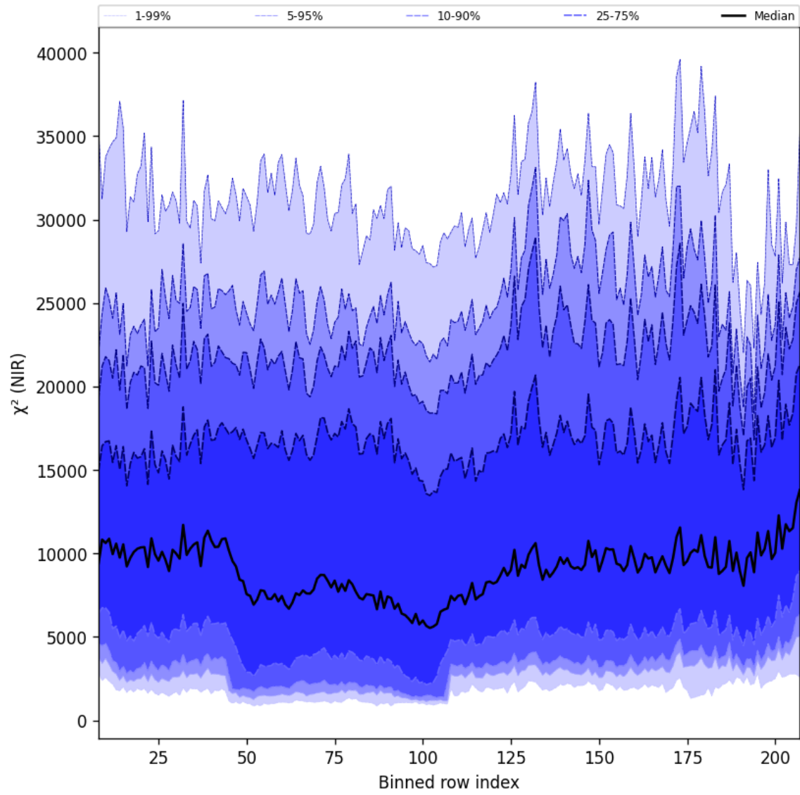
Figure 40: Along track statistics of " \chi^2 (NIR)" for 2025-05-02 to 2025-05-04
