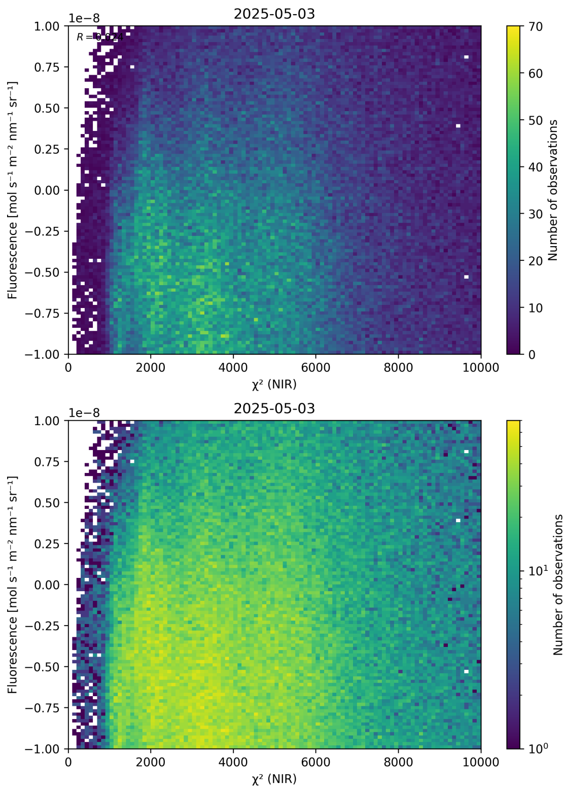
Figure 45: Scatter density plot of “ \chi^2 (NIR)” against “Fluorescence” for 2025-05-02 to 2025-05-04.
