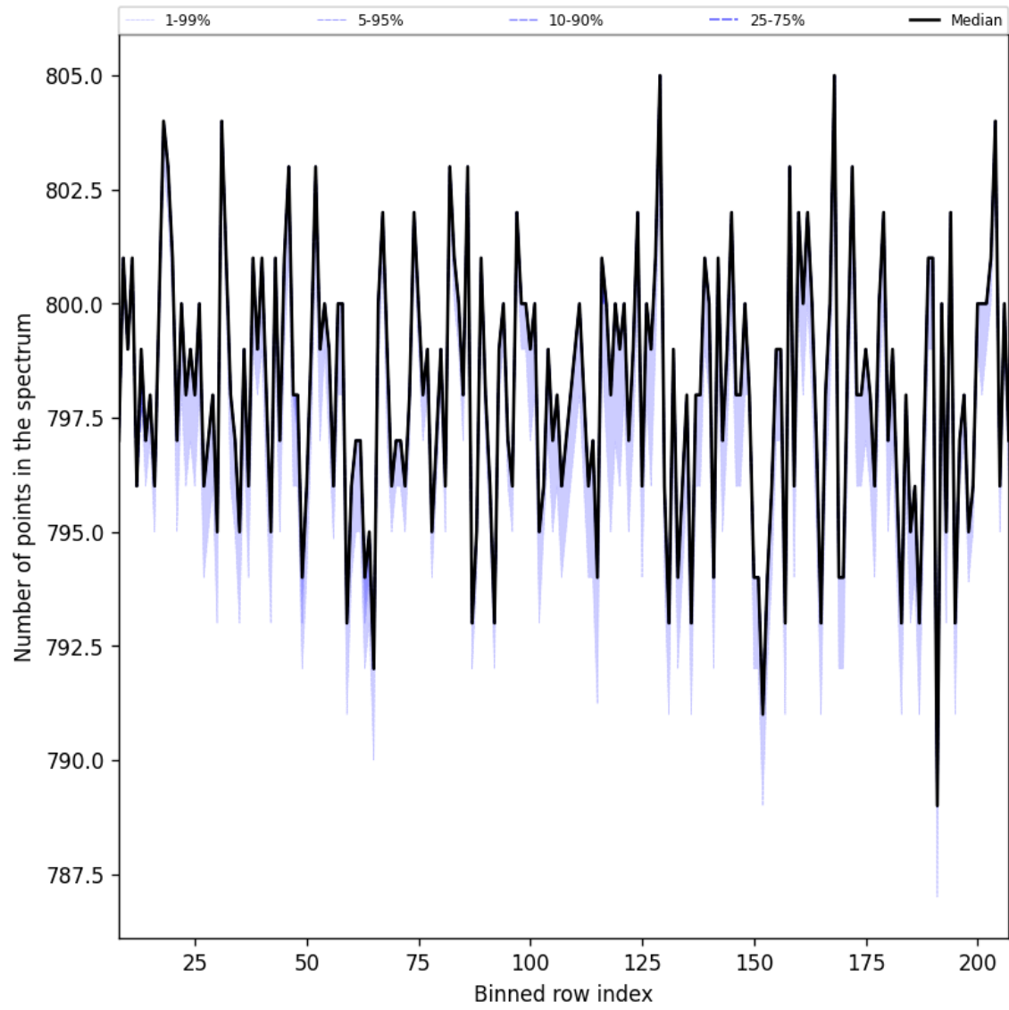
Figure 37: Along track statistics of “Number of points in the spectrum” for 2025-05-02 to 2025-05-04
