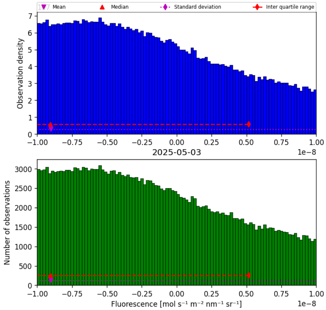
Figure 32: Histogram of “Fluorescence” for 2025-05-02 to 2025-05-04
