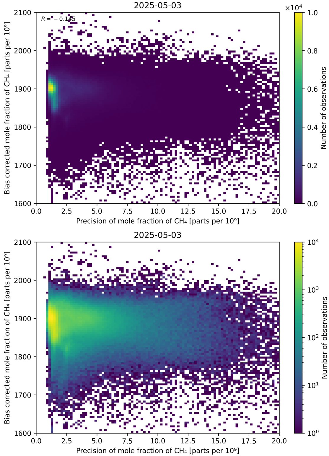
Figure 82: Scatter density plot of “Precision of mole fraction of \text{CH}_4 ” against “Bias corrected mole fraction of \text{CH}_4 ” for 2025-05-02 to 2025-05-04.
