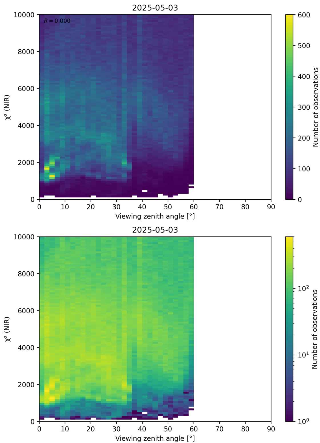
Figure 105: Scatter density plot of “Viewing zenith angle” against “ \chi^2 (NIR)” for 2025-05-02 to 2025-05-04.
