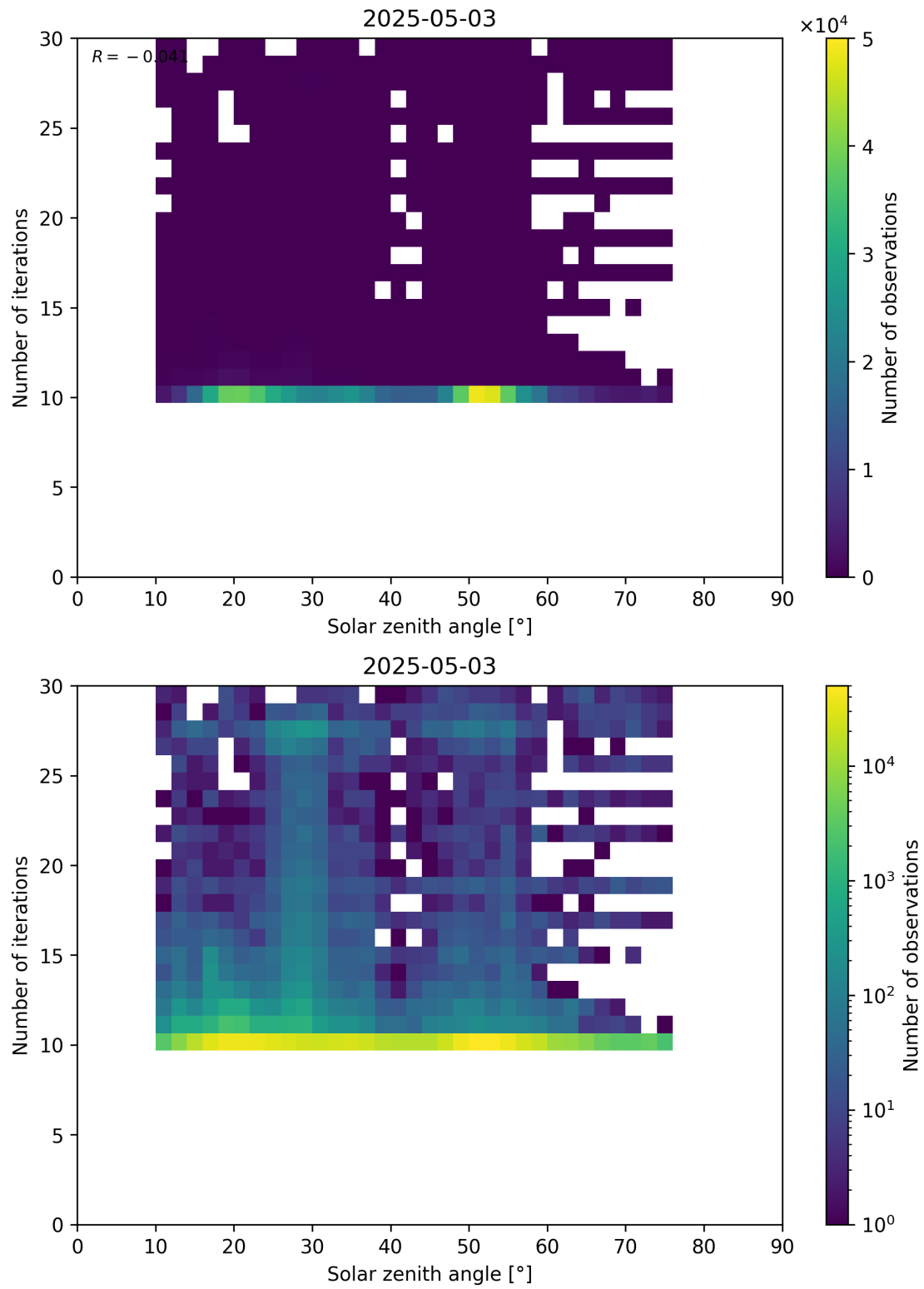
Figure 102: Scatter density plot of “Solar zenith angle” against “Number of iterations” for 2025-05-02 to 2025-05-04.
