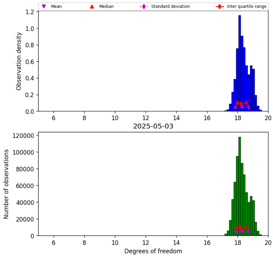
Figure 30: Histogram of “Degrees of freedom” for 2025-05-02 to 2025-05-04
