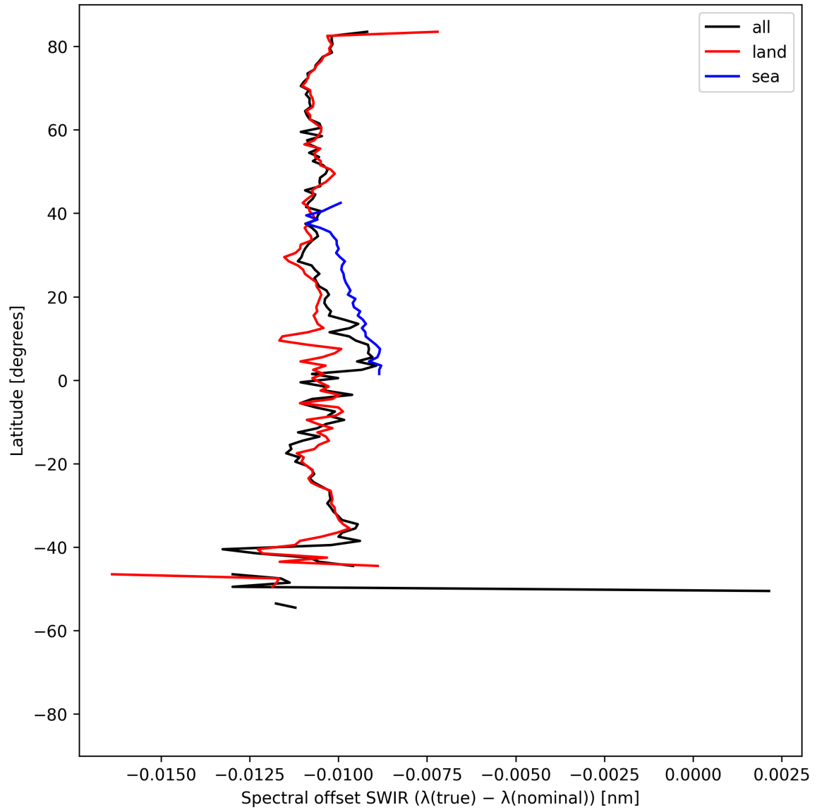
Figure 16: Zonal average of “Spectral offset SWIR ( \lambda_{\text{true}} - \lambda_{\text{nominal}} )” for 2025-05-02 to 2025-05-04.
