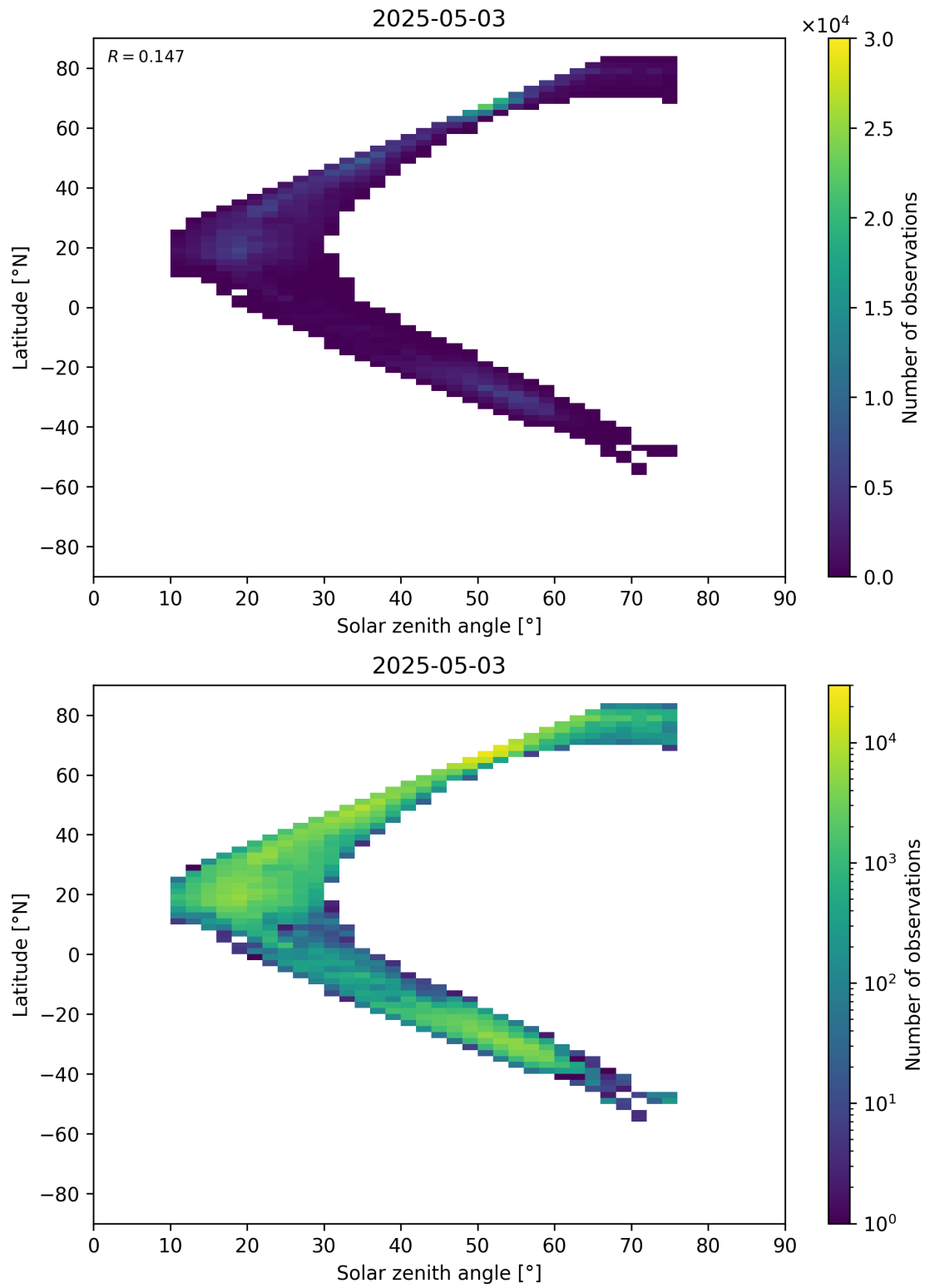
Figure 98: Scatter density plot of “Solar zenith angle” against “Latitude” for 2025-05-02 to 2025-05-04.
