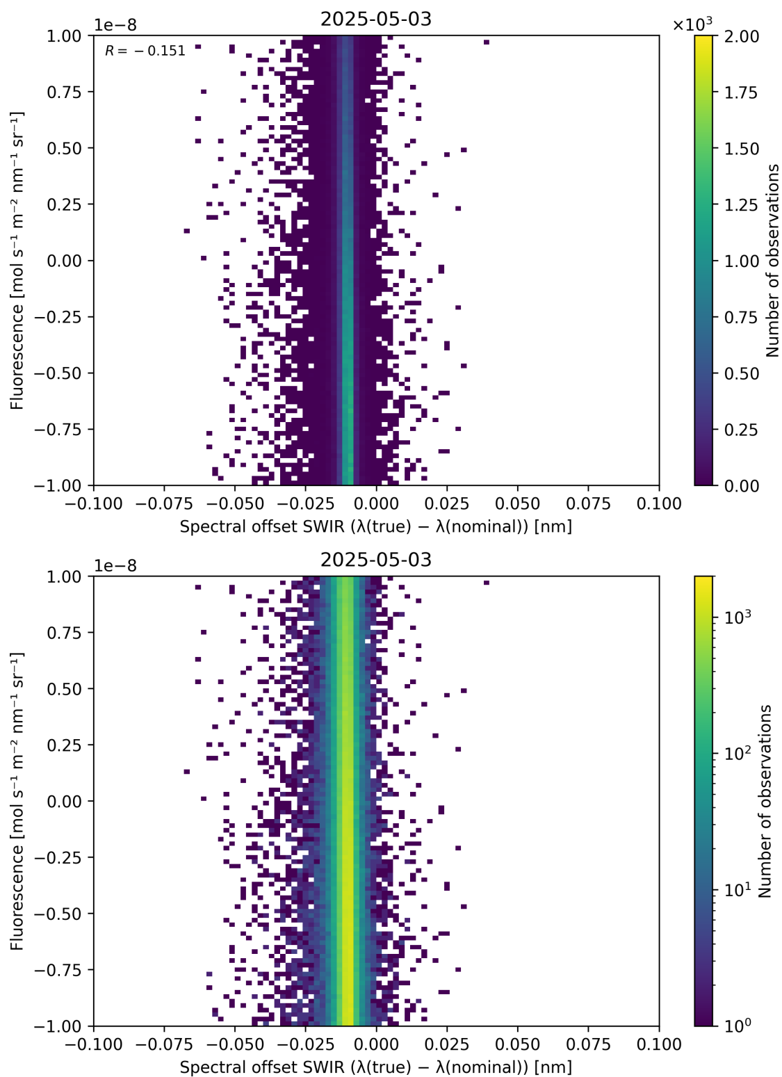
Figure 120: Scatter density plot of “Spectral offset SWIR ( \lambda_{\text{true}} - \lambda_{\text{nominal}} )” against “Fluorescence” for 2025-05-02 to 2025-05-04.
