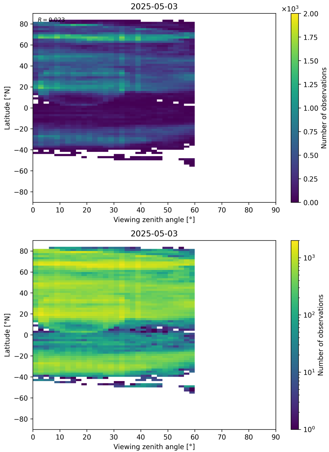
Figure 109: Scatter density plot of “Viewing zenith angle” against “Latitude” for 2025-05-02 to 2025-05-04.
