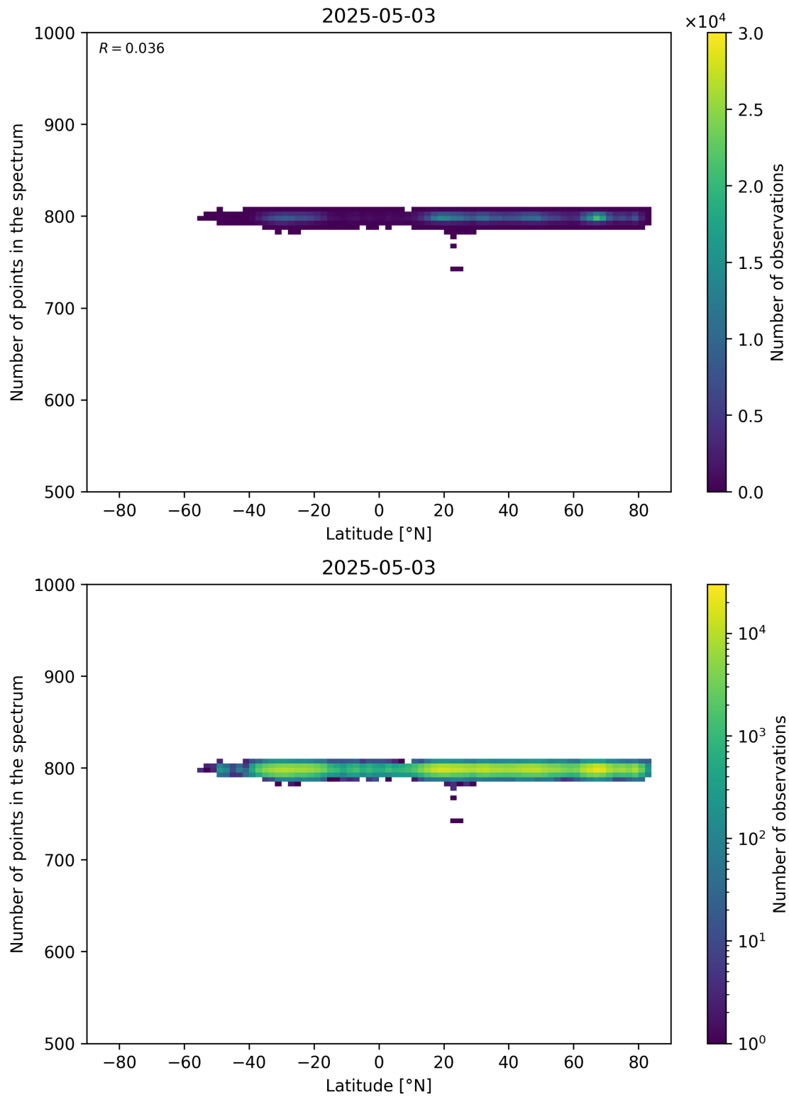
Figure 61: Scatter density plot of “Latitude” against “Number of points in the spectrum” for 2025-05-02 to 2025-05-04.
