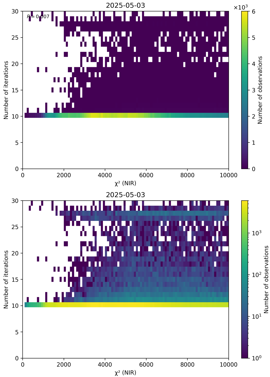
Figure 46: Scatter density plot of “ \chi^2 (NIR)” against “Number of iterations” for 2025-05-02 to 2025-05-04.
