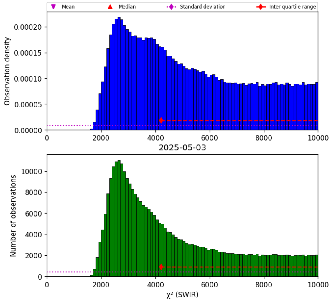
Figure 28: Histogram of " \chi^2 (SWIR)" for 2025-05-02 to 2025-05-04
