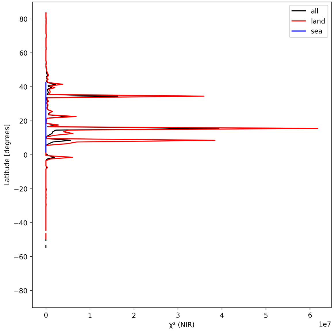
Figure 18: Zonal average of “ \chi^2 (NIR)” for 2025-05-02 to 2025-05-04.
