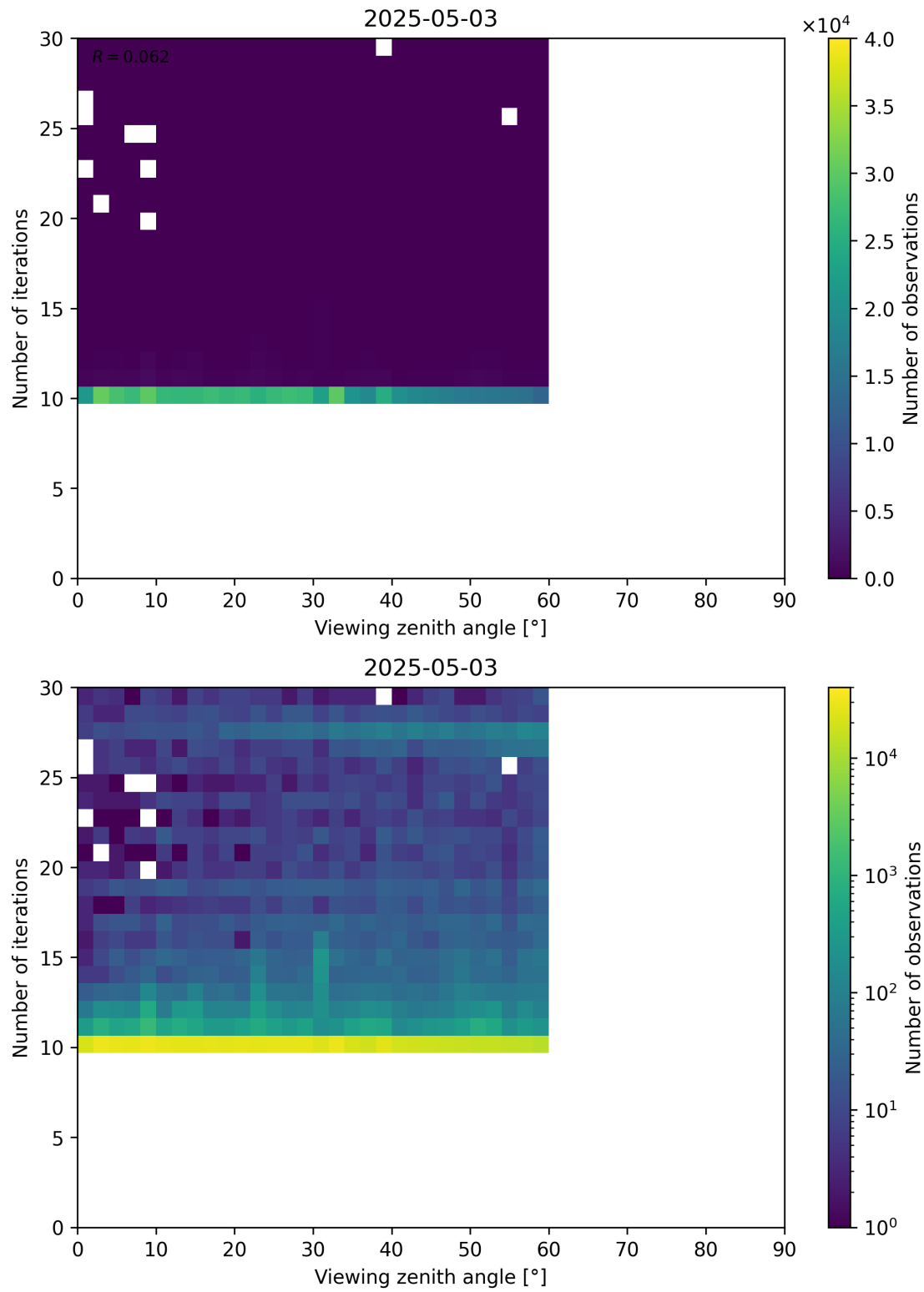
Figure 113: Scatter density plot of “Viewing zenith angle” against “Number of iterations” for 2025-05-02 to 2025-05-04.
