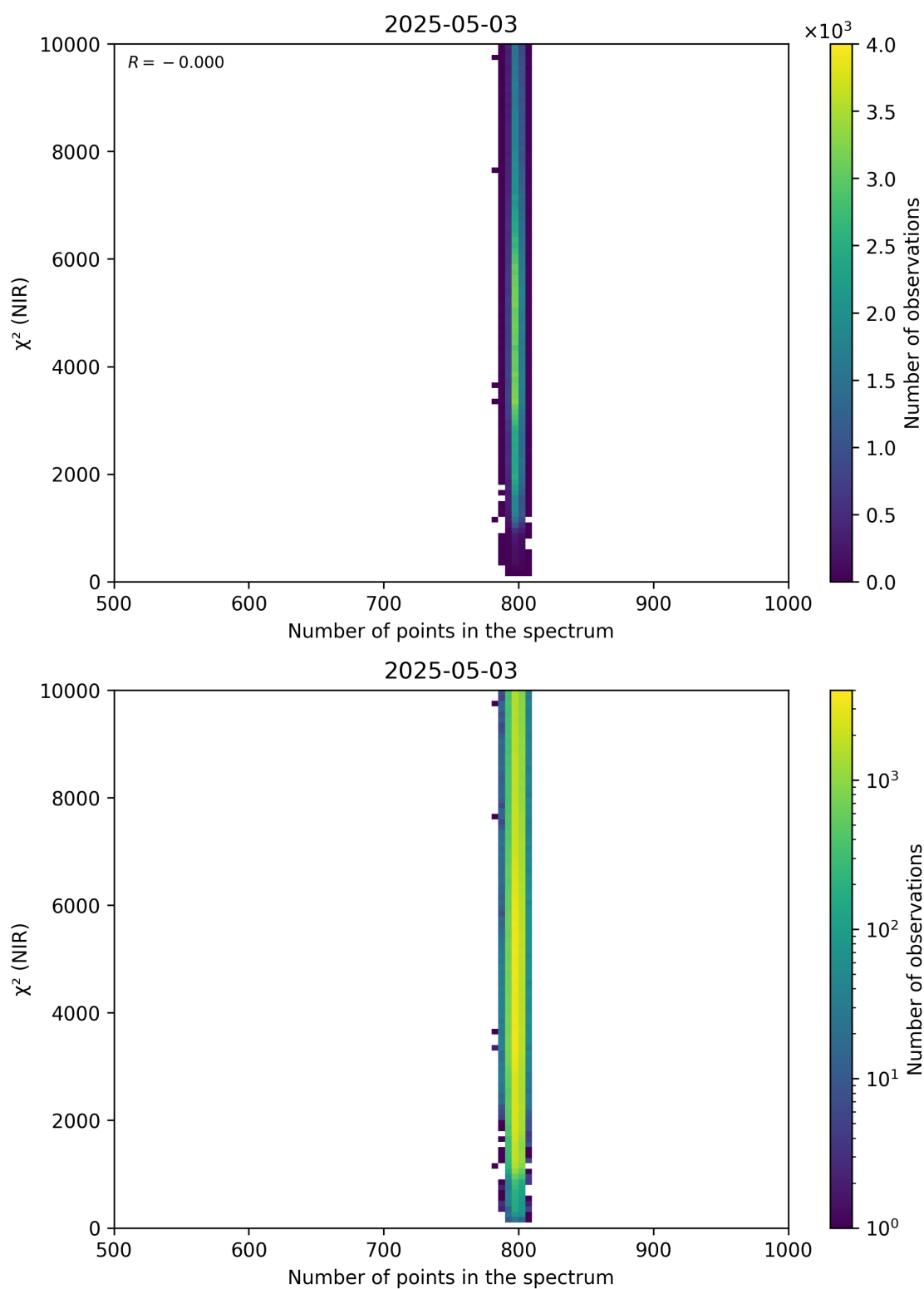
Figure 88: Scatter density plot of “Number of points in the spectrum” against “ \chi^2 (NIR)” for 2025-05-02 to 2025-05-04.
