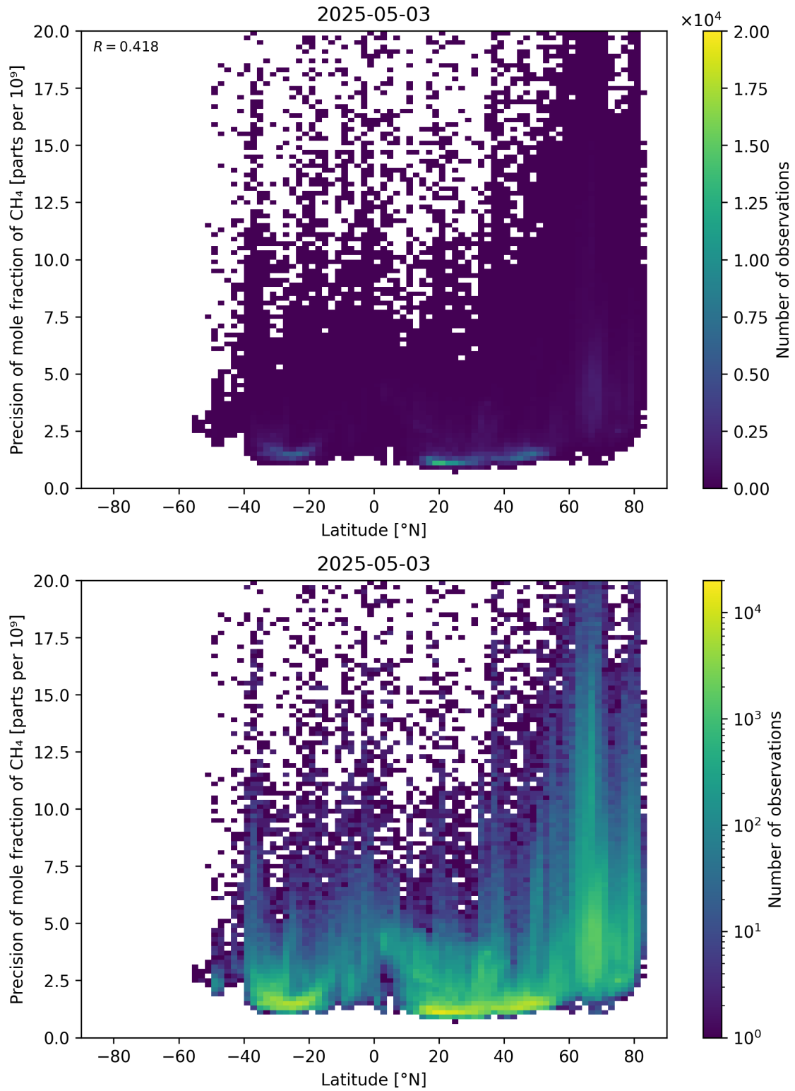
Figure 59: Scatter density plot of “Latitude” against “Precision of mole fraction of \text{CH}_4 ” for 2025-05-02 to 2025-05-04.
