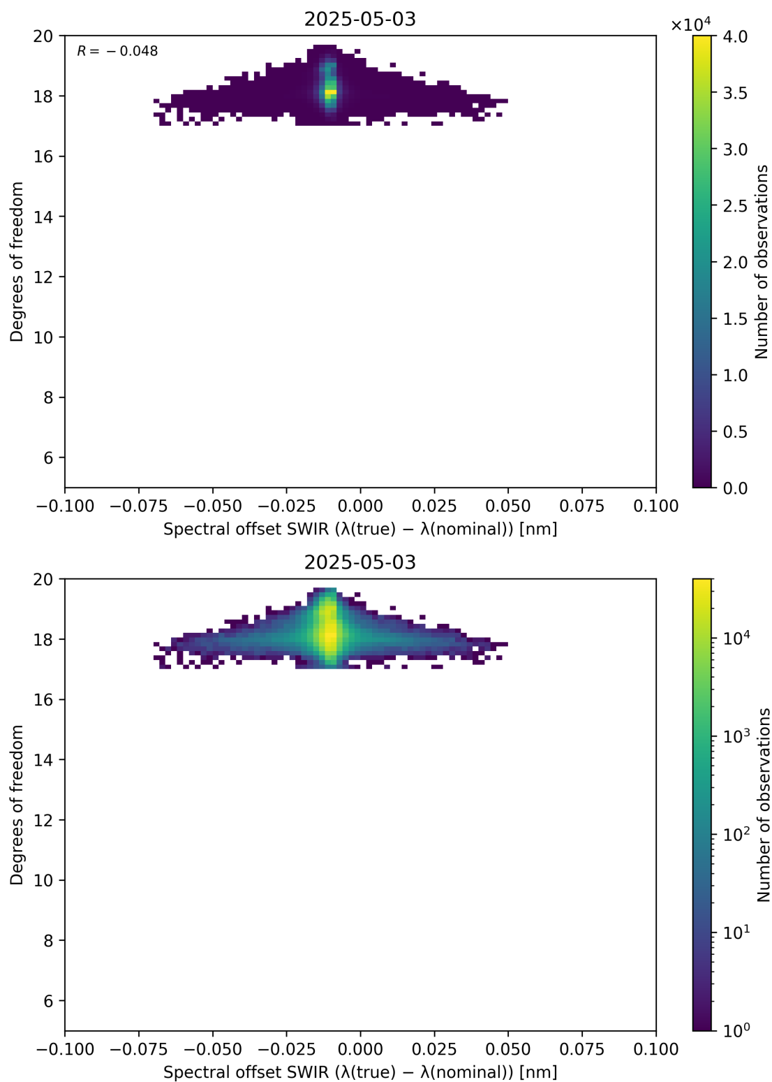
Figure 119: Scatter density plot of “Spectral offset SWIR ( \lambda_{\text{true}} - \lambda_{\text{nominal}} )” against “Degrees of freedom” for 2025-05-02 to 2025-05-04.
