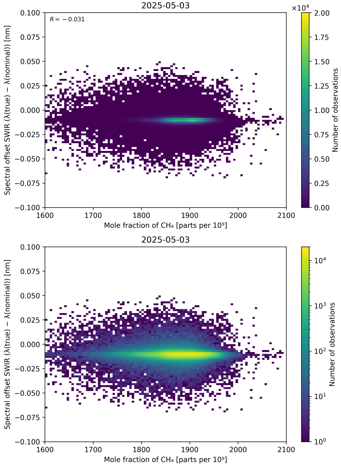
Figure 86: Scatter density plot of “Mole fraction of CH 4 ” against “Spectral offset SWIR ( \lambda_{\text{true}} - \lambda_{\text{nominal}} )” for 2025-05-02 to 2025-05-04.
