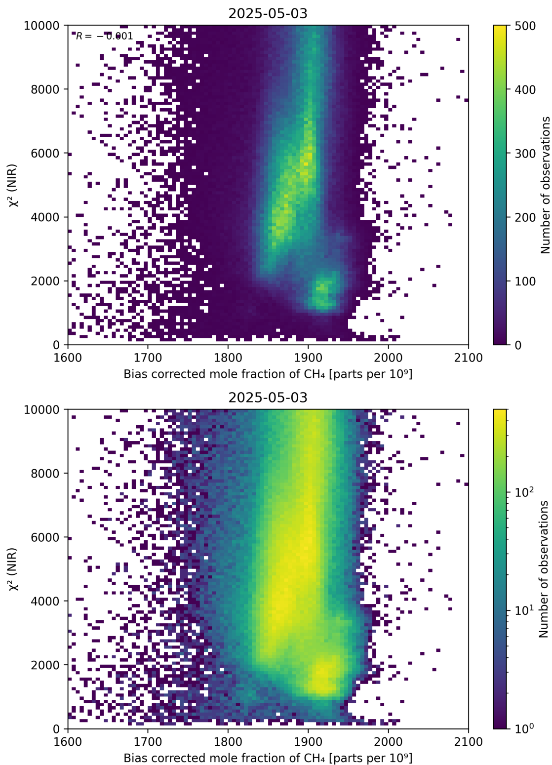
Figure 63: Scatter density plot of “Bias corrected mole fraction of CH 4 ” against “ \chi^2 (NIR)” for 2025-05-02 to 2025-05-04.
