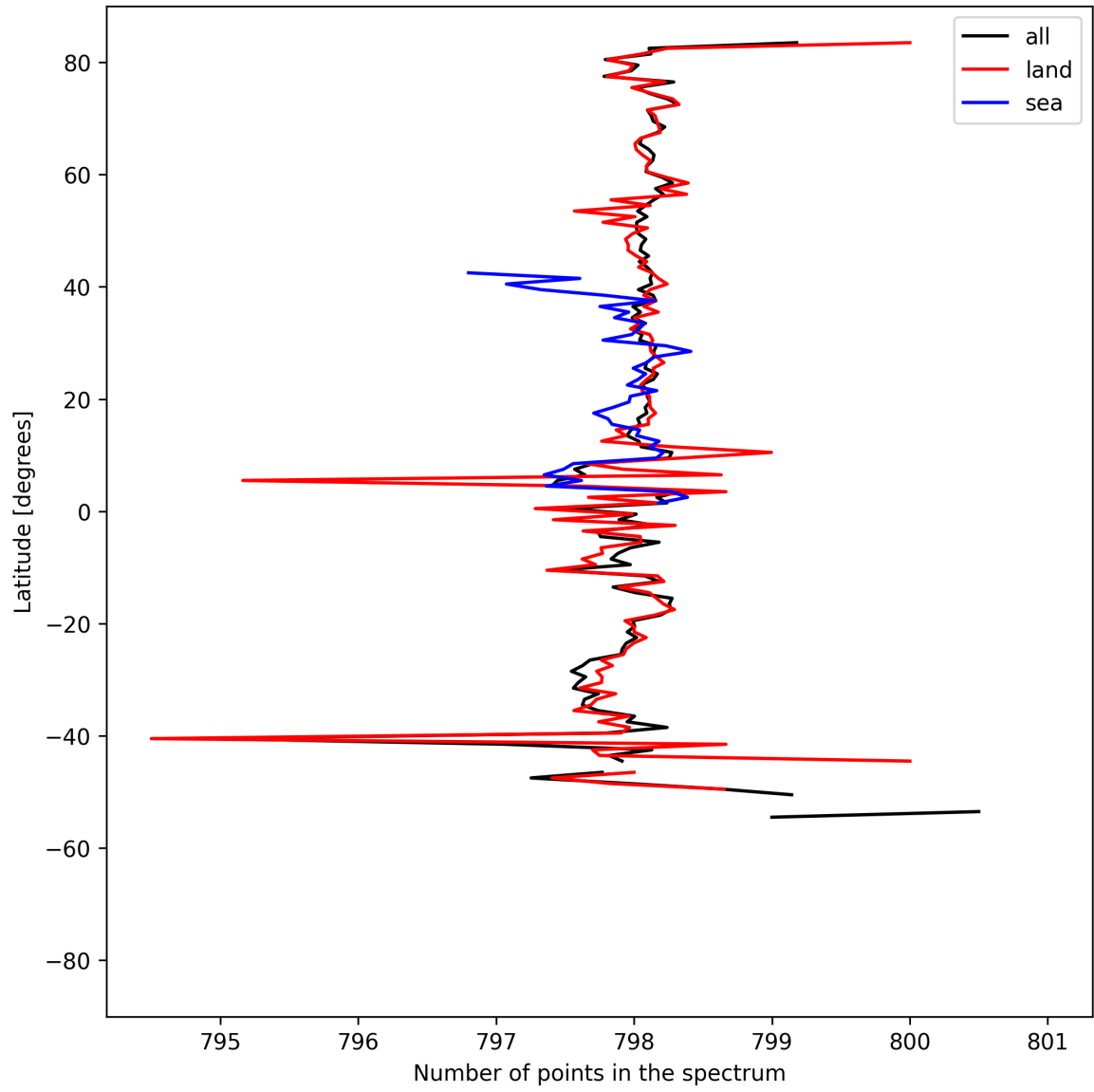
Figure 15: Zonal average of “Number of points in the spectrum” for 2025-05-02 to 2025-05-04.
