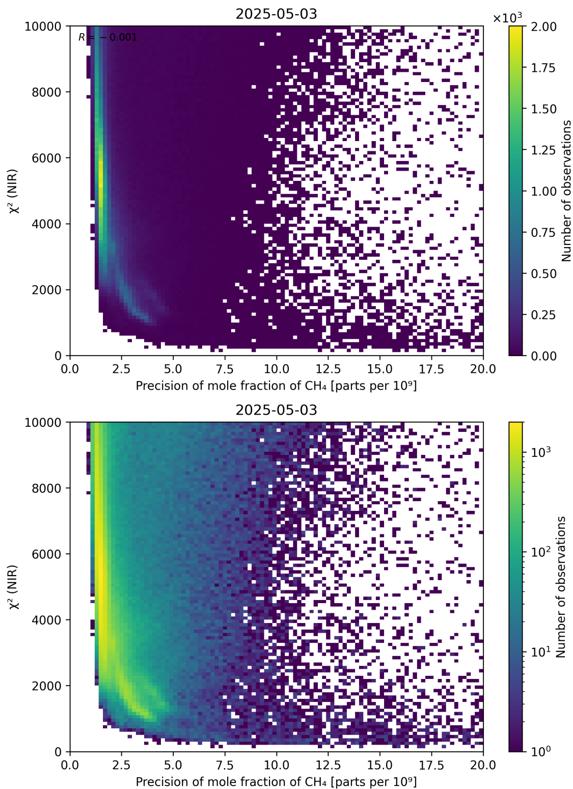
Figure 78: Scatter density plot of “Precision of mole fraction of CH 4 ” against “ \chi^2 (NIR)” for 2025-05-02 to 2025-05-04.
