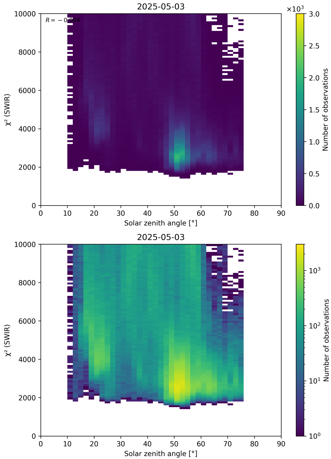
Figure 95: Scatter density plot of “Solar zenith angle” against “ \chi^2 (SWIR)” for 2025-05-02 to 2025-05-04.
