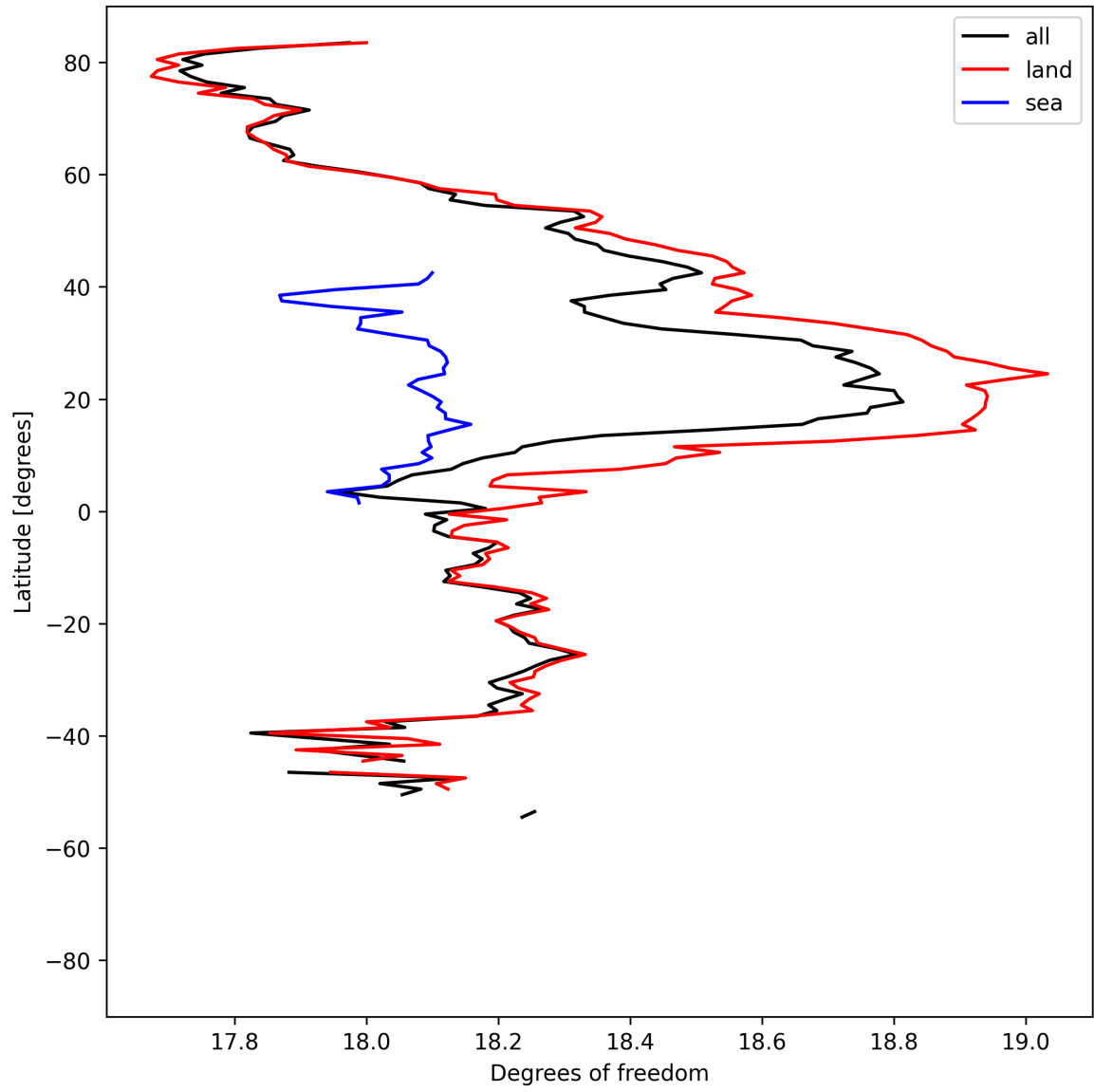
Figure 19: Zonal average of “Degrees of freedom” for 2025-05-02 to 2025-05-04.
