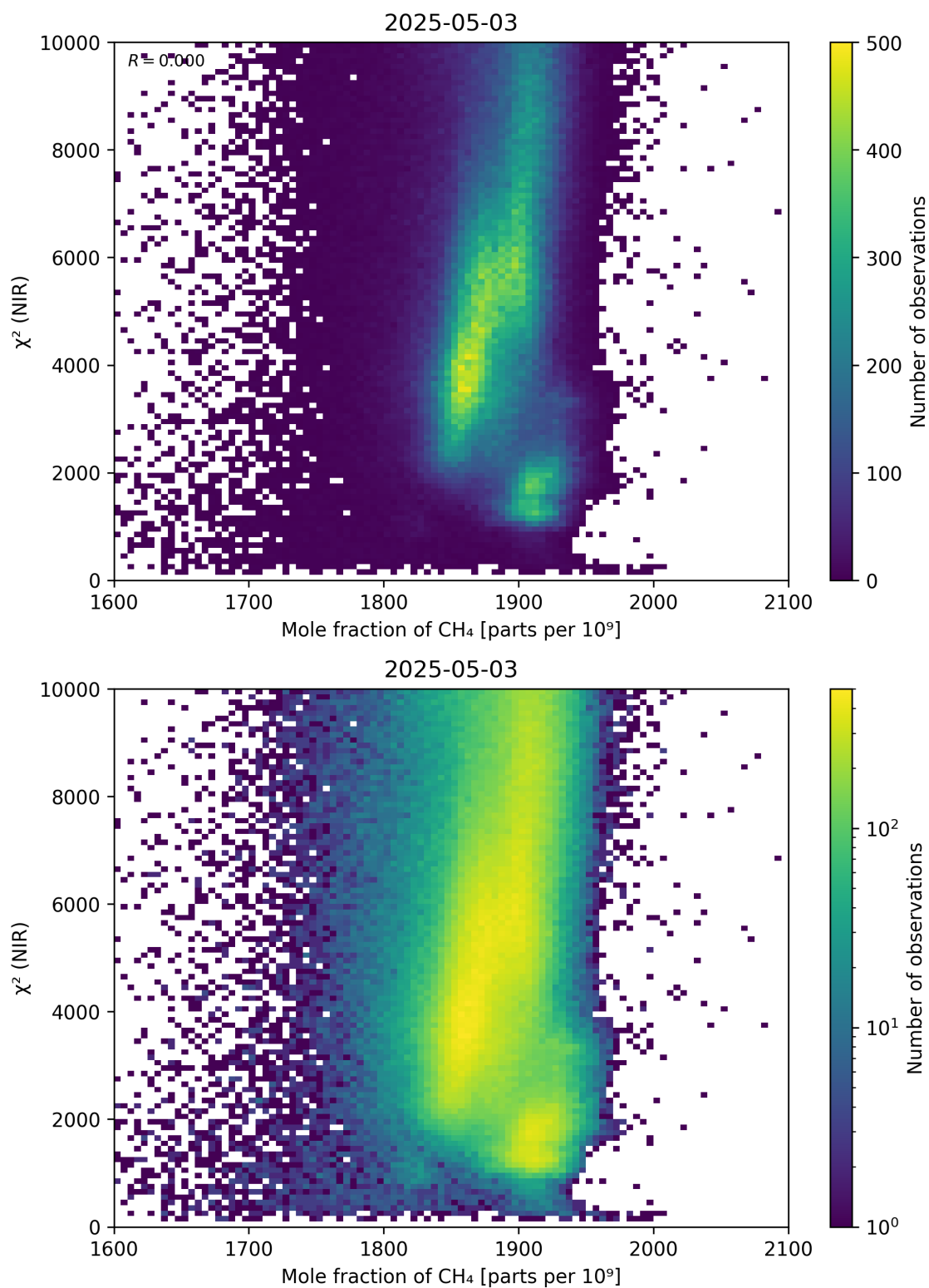
Figure 70: Scatter density plot of “Mole fraction of \text{CH}_4 ” against “ \chi^2 (NIR)” for 2025-05-02 to 2025-05-04.
