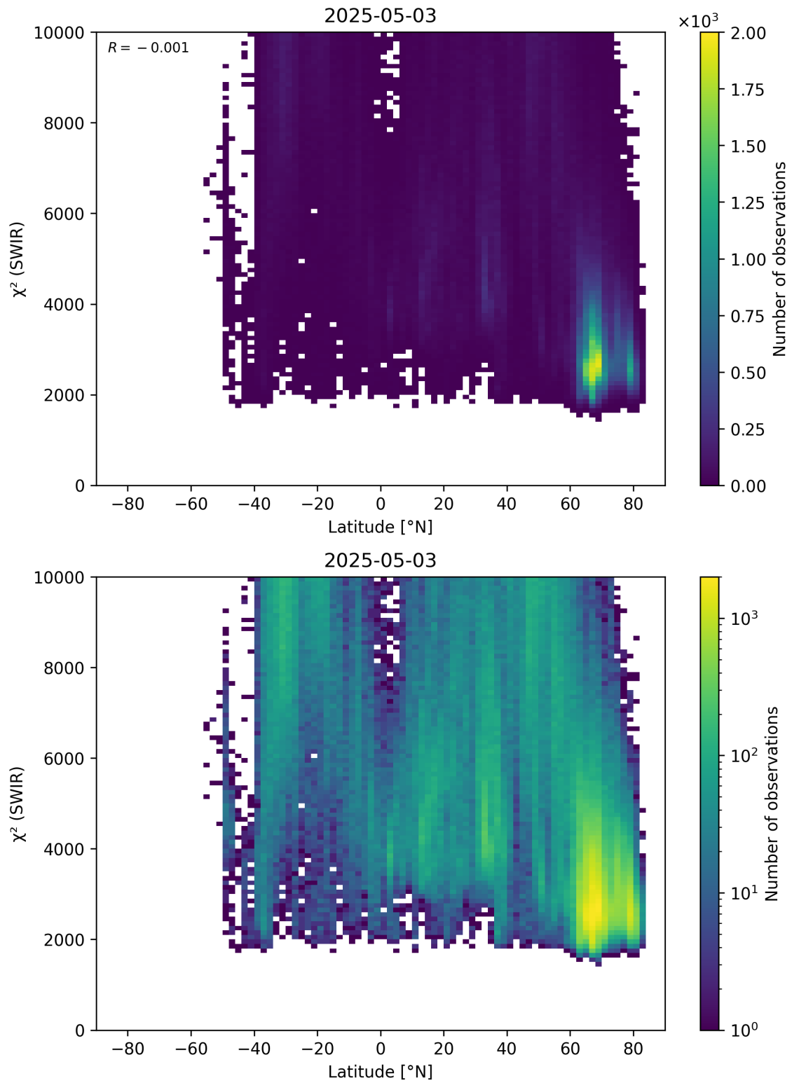
Figure 54: Scatter density plot of “Latitude” against “ \chi^2 (SWIR)” for 2025-05-02 to 2025-05-04.
