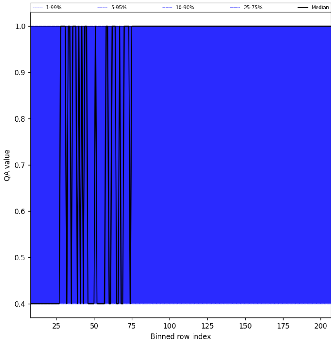
Figure 33: Along track statistics of “QA value” for 2025-05-02 to 2025-05-04
