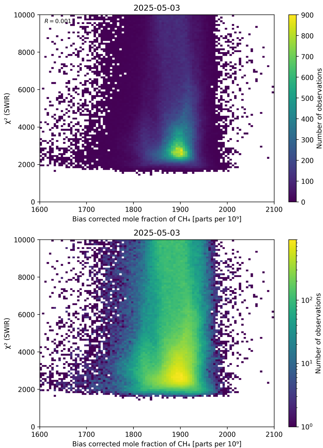
Figure 64: Scatter density plot of “Bias corrected mole fraction of \text{CH}_4 ” against “ \chi^2 (SWIR)” for 2025-05-02 to 2025-05-04.
