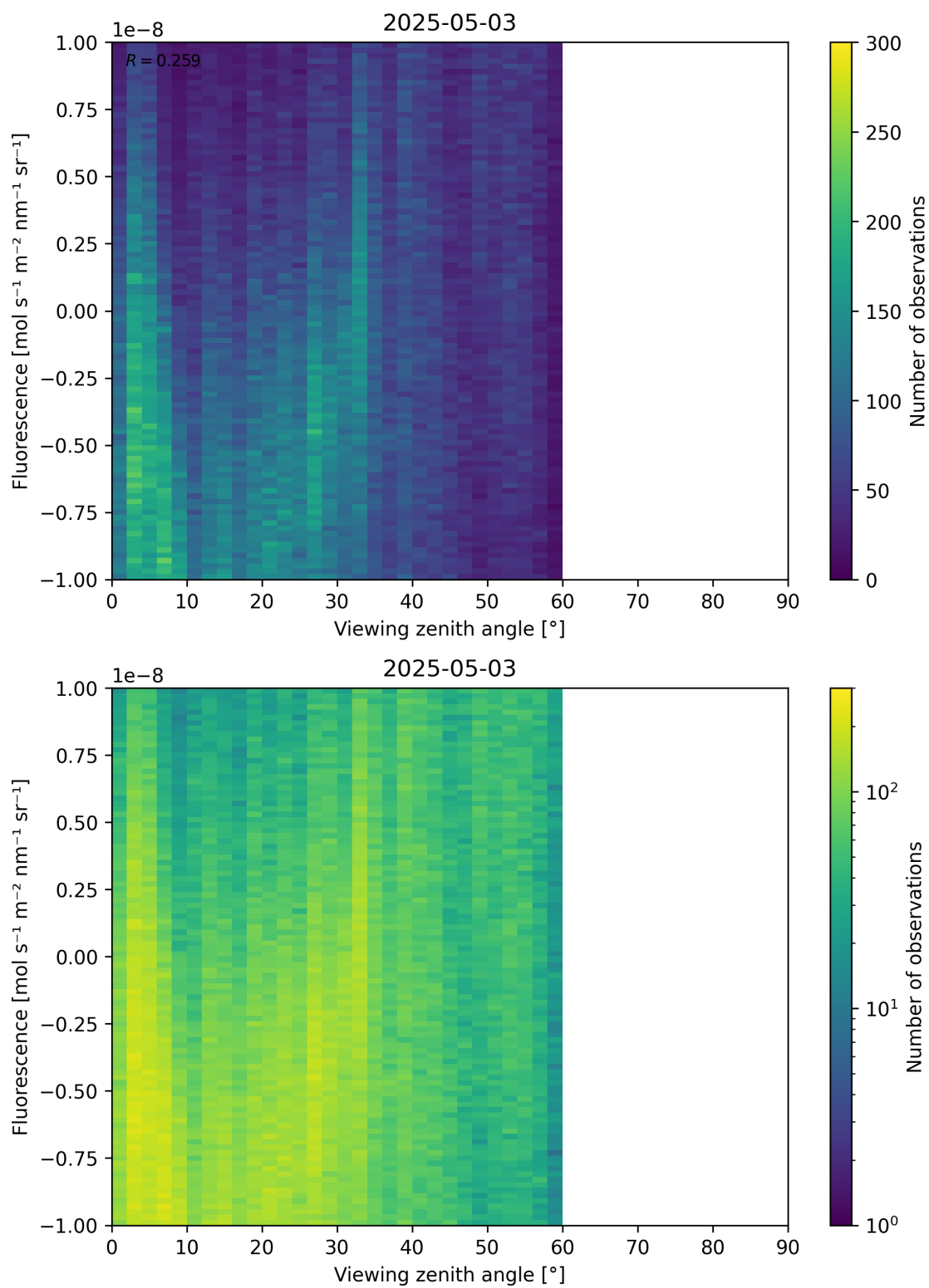
Figure 108: Scatter density plot of “Viewing zenith angle” against “Fluorescence” for 2025-05-02 to 2025-05-04.
