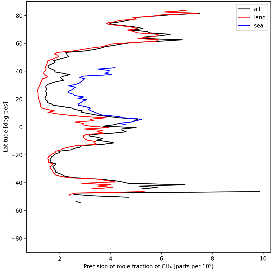
Figure 13: Zonal average of “Precision of mole fraction of CH 4 ” for 2025-05-02 to 2025-05-04.
