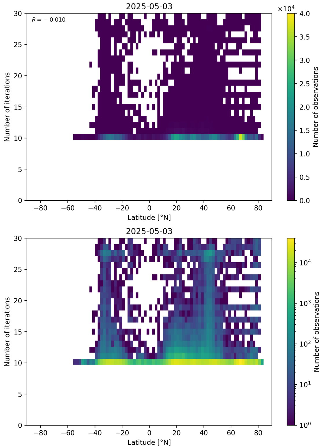
Figure 60: Scatter density plot of “Latitude” against “Number of iterations” for 2025-05-02 to 2025-05-04.
