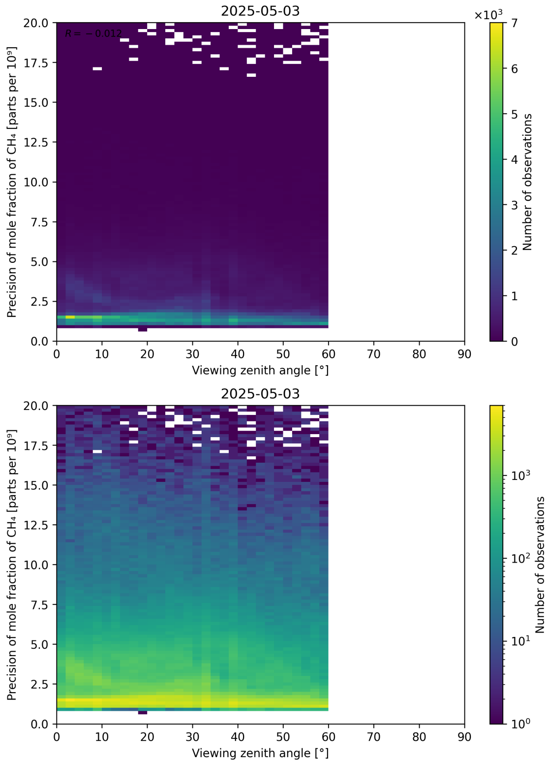
Figure 112: Scatter density plot of “Viewing zenith angle” against “Precision of mole fraction of CH 4 ” for 2025-05-02 to 2025-05-04.
