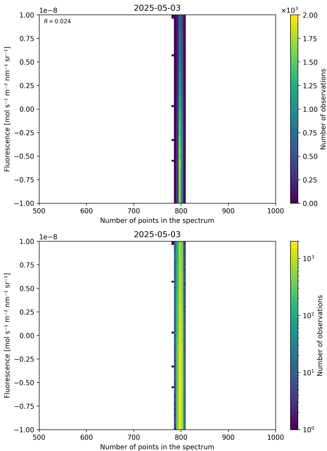
Figure 91: Scatter density plot of “Number of points in the spectrum” against “Fluorescence” for 2025-05-02 to 2025-05-04.
