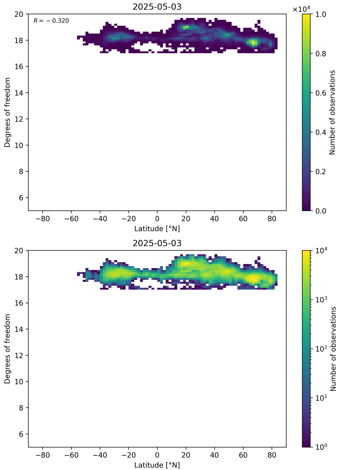
Figure 55: Scatter density plot of “Latitude” against “Degrees of freedom” for 2025-05-02 to 2025-05-04.
