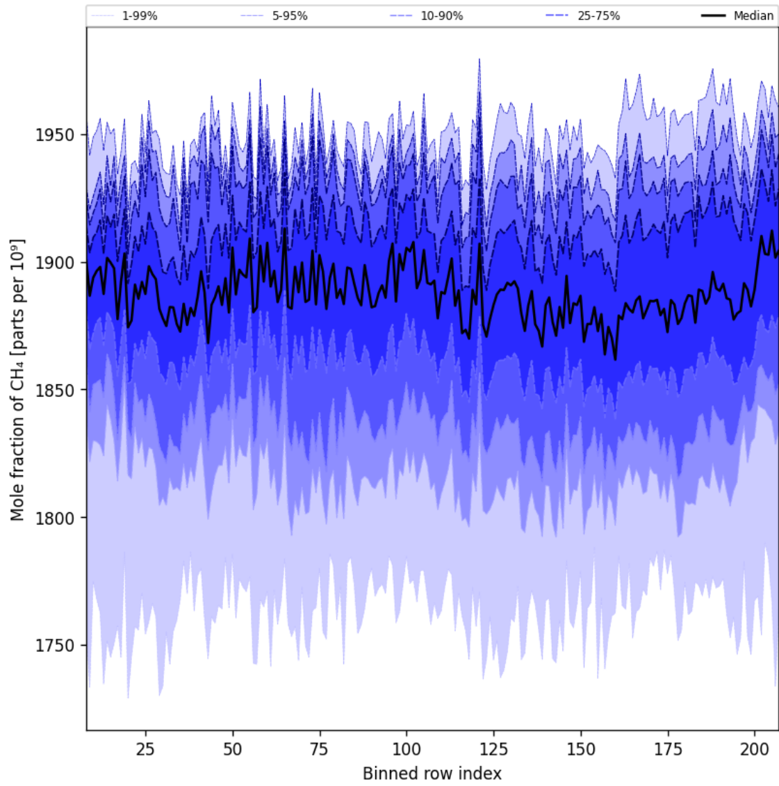
Figure 34: Along track statistics of “Mole fraction of CH 4 ” for 2025-05-02 to 2025-05-04
