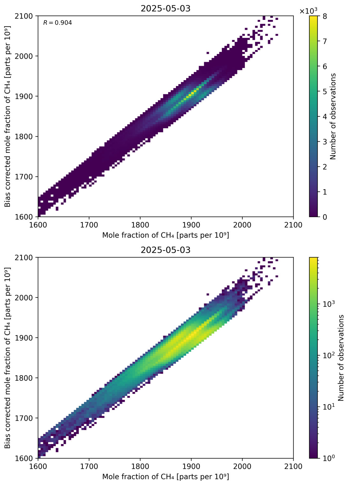
Figure 74: Scatter density plot of “Mole fraction of CH 4 ” against “Bias corrected mole fraction of CH 4 ” for 2025-05-02 to 2025-05-04.
