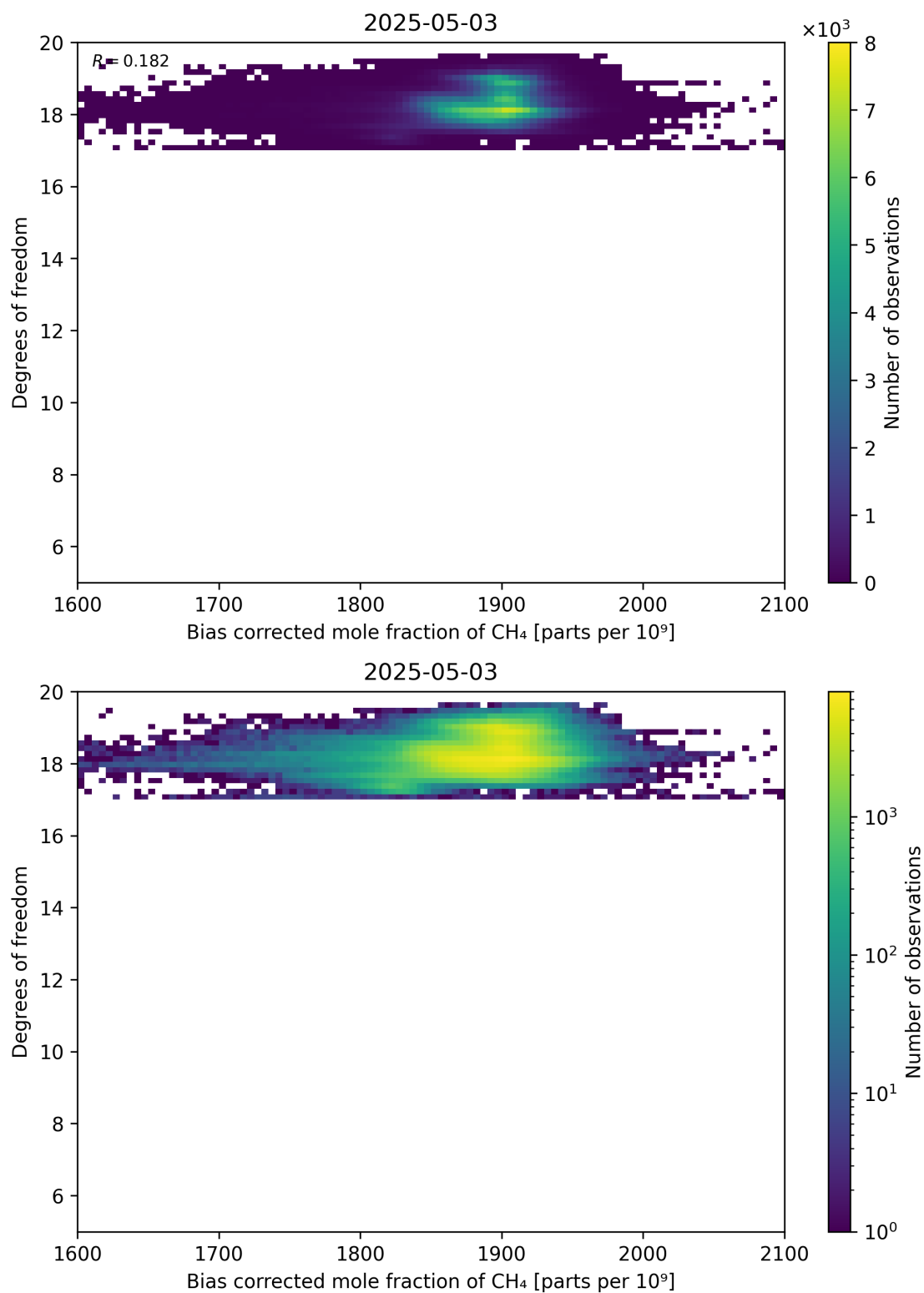
Figure 65: Scatter density plot of “Bias corrected mole fraction of CH 4 ” against “Degrees of freedom” for 2025-05-02 to 2025-05-04.
