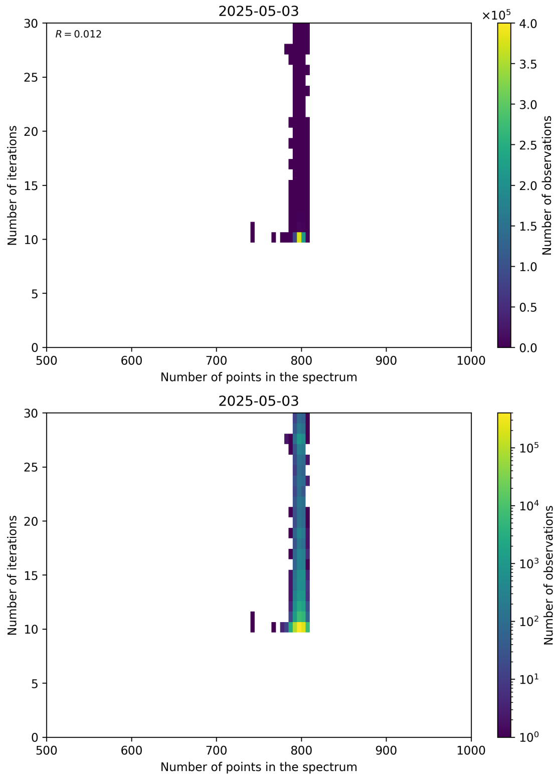
Figure 92: Scatter density plot of “Number of points in the spectrum” against “Number of iterations” for 2025-05-02 to 2025-05-04.
