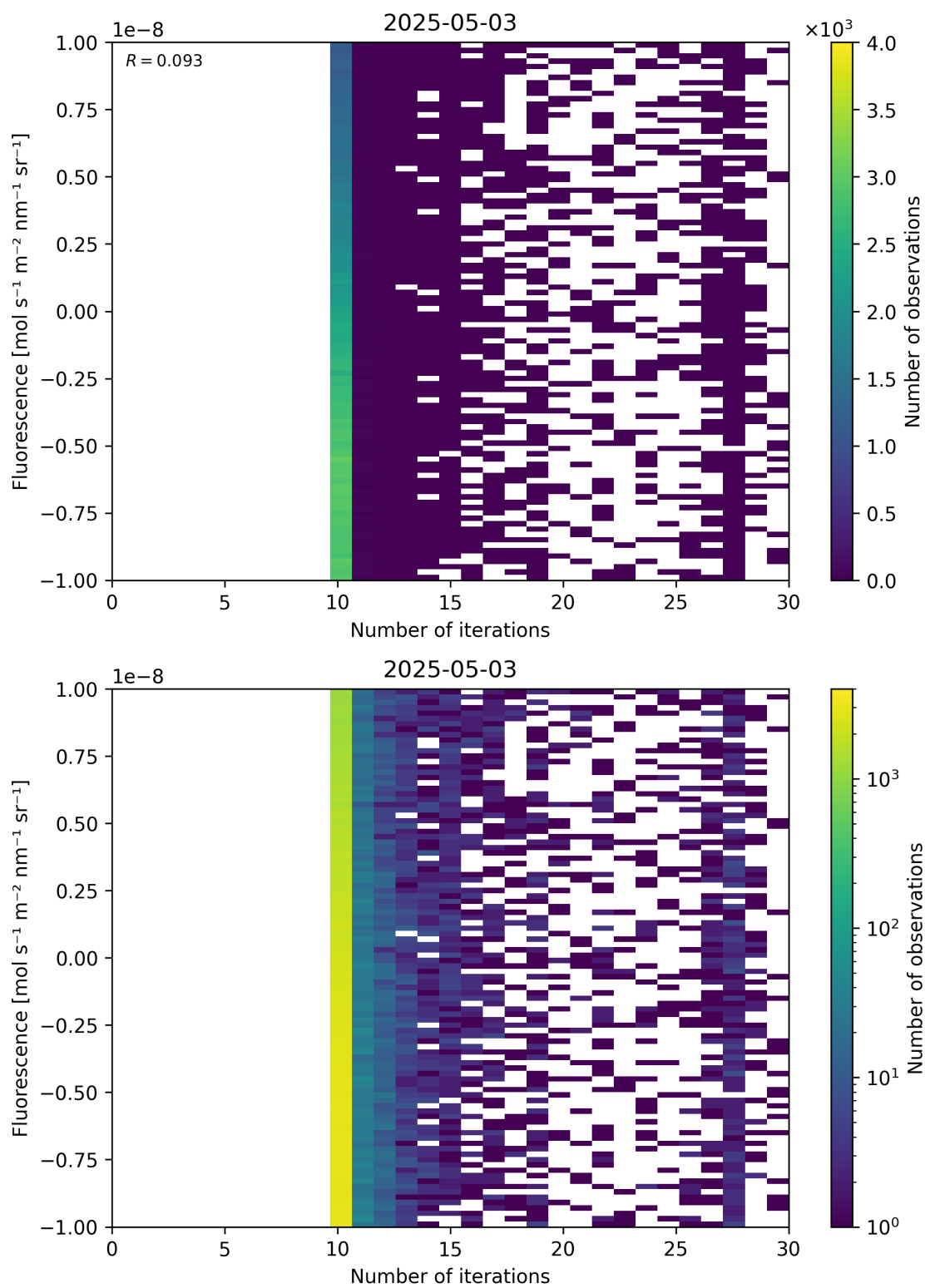
Figure 87: Scatter density plot of “Number of iterations” against “Fluorescence” for 2025-05-02 to 2025-05-04.
