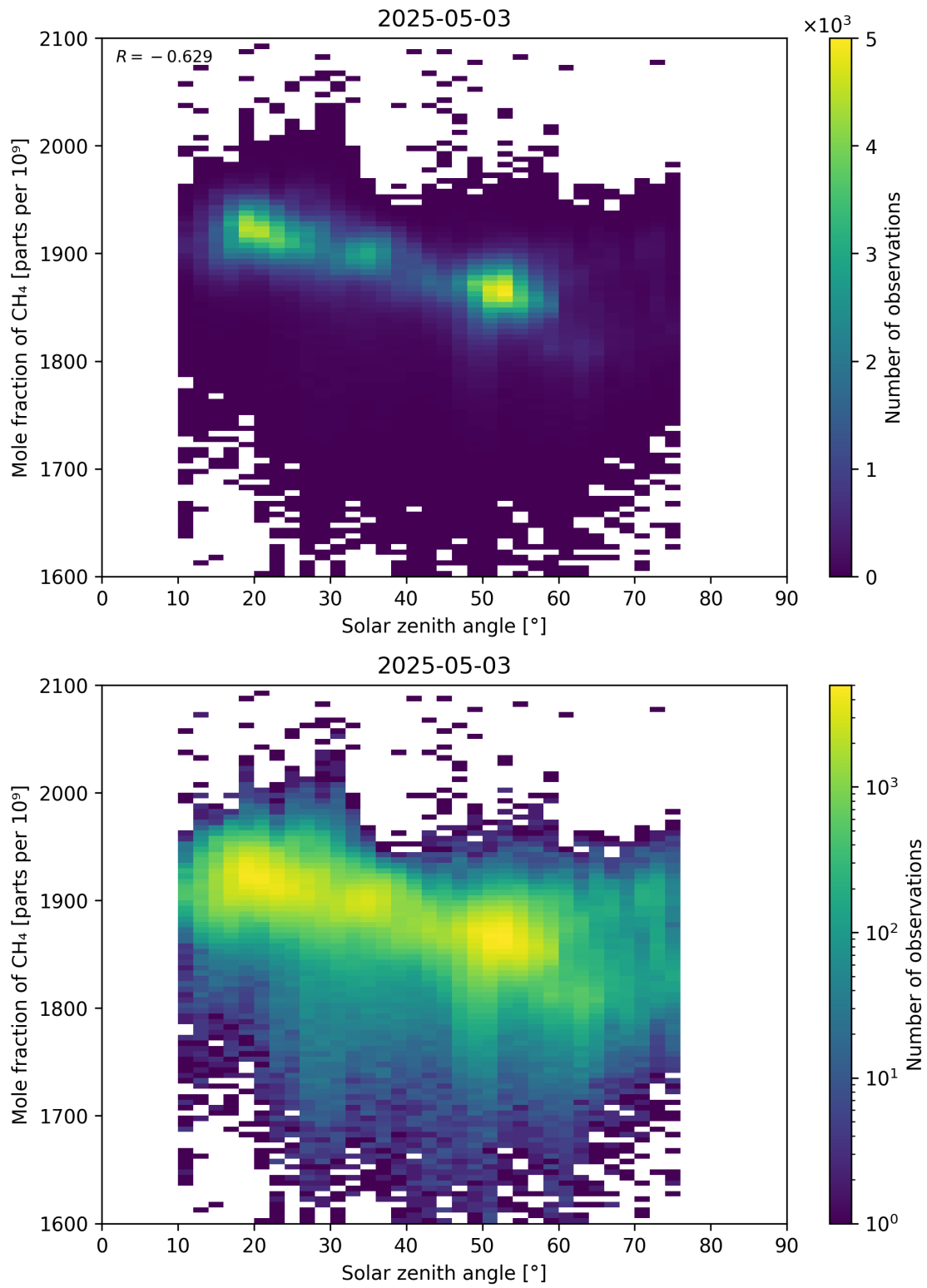
Figure 99: Scatter density plot of “Solar zenith angle” against “Mole fraction of CH 4 ” for 2025-05-02 to 2025-05-04.
