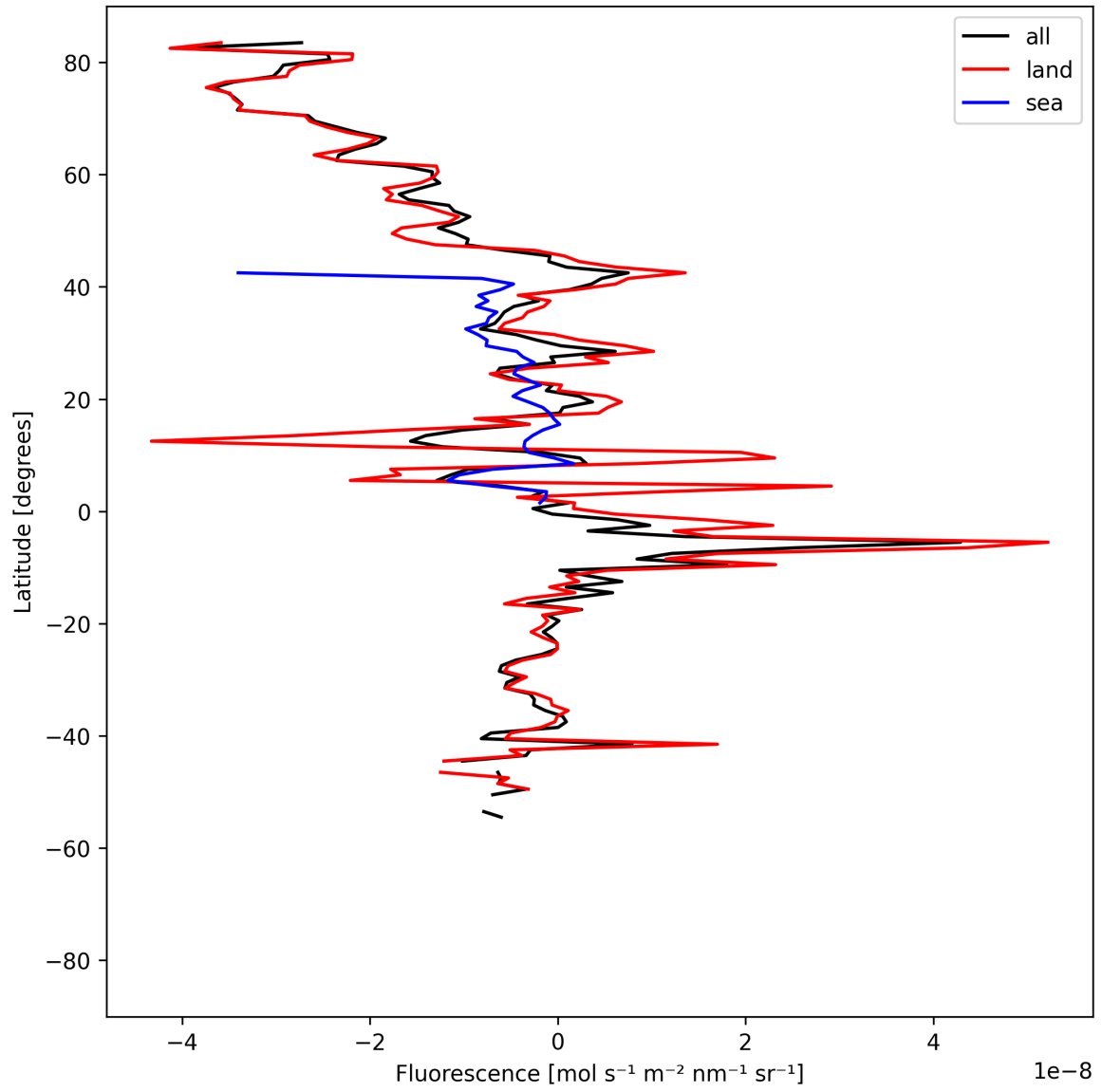
Figure 21: Zonal average of “Fluorescence” for 2025-05-02 to 2025-05-04.
