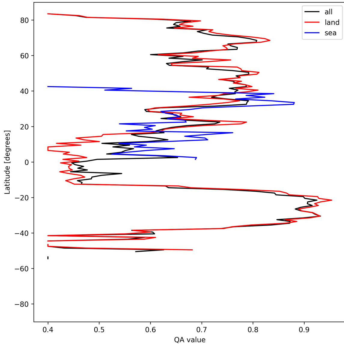
Figure 11: Zonal average of “QA value” for 2025-05-02 to 2025-05-04.
