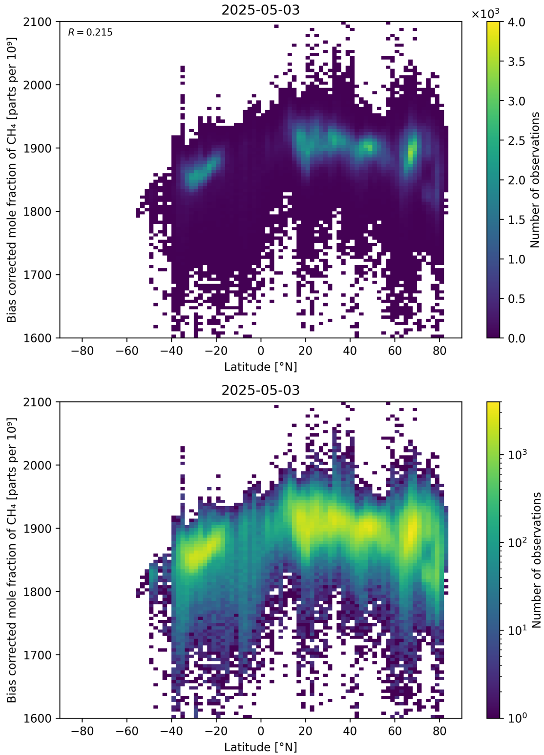
Figure 58: Scatter density plot of “Latitude” against “Bias corrected mole fraction of CH 4 ” for 2025-05-02 to 2025-05-04.
