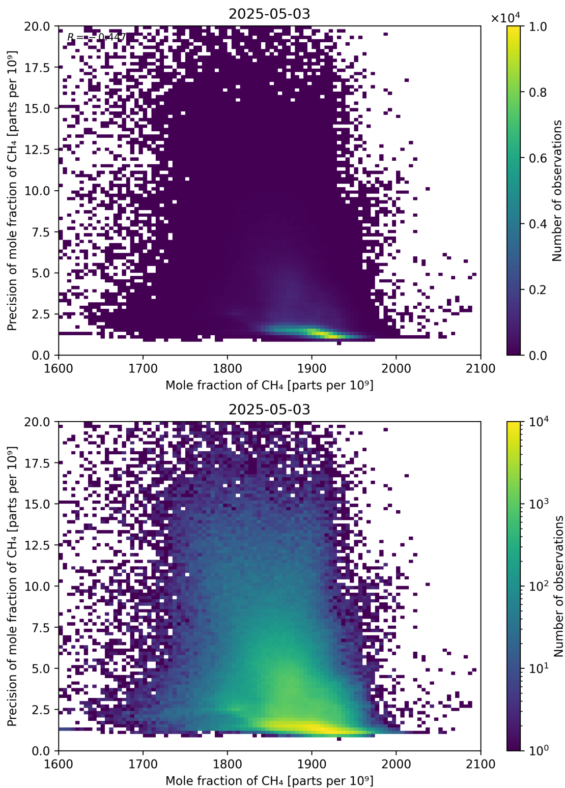
Figure 75: Scatter density plot of “Mole fraction of CH 4 ” against “Precision of mole fraction of CH 4 ” for 2025-05-02 to 2025-05-04.
