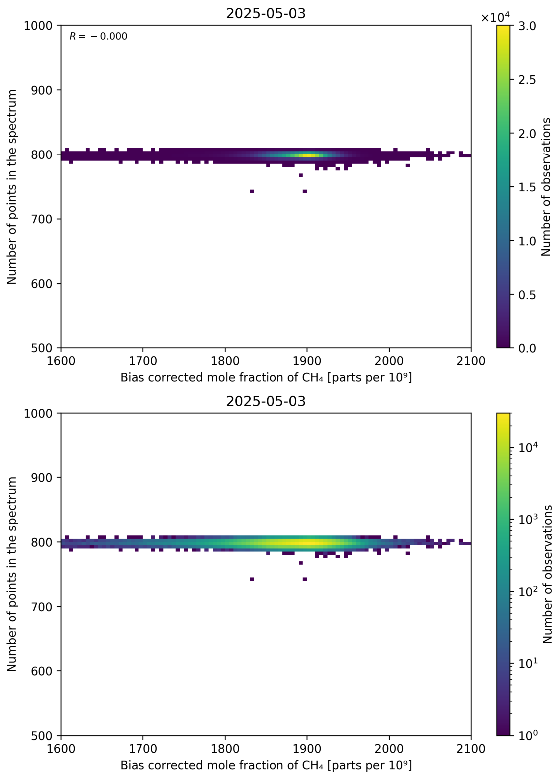
Figure 68: Scatter density plot of “Bias corrected mole fraction of CH 4 ” against “Number of points in the spectrum” for 2025-05-02 to 2025-05-04.
