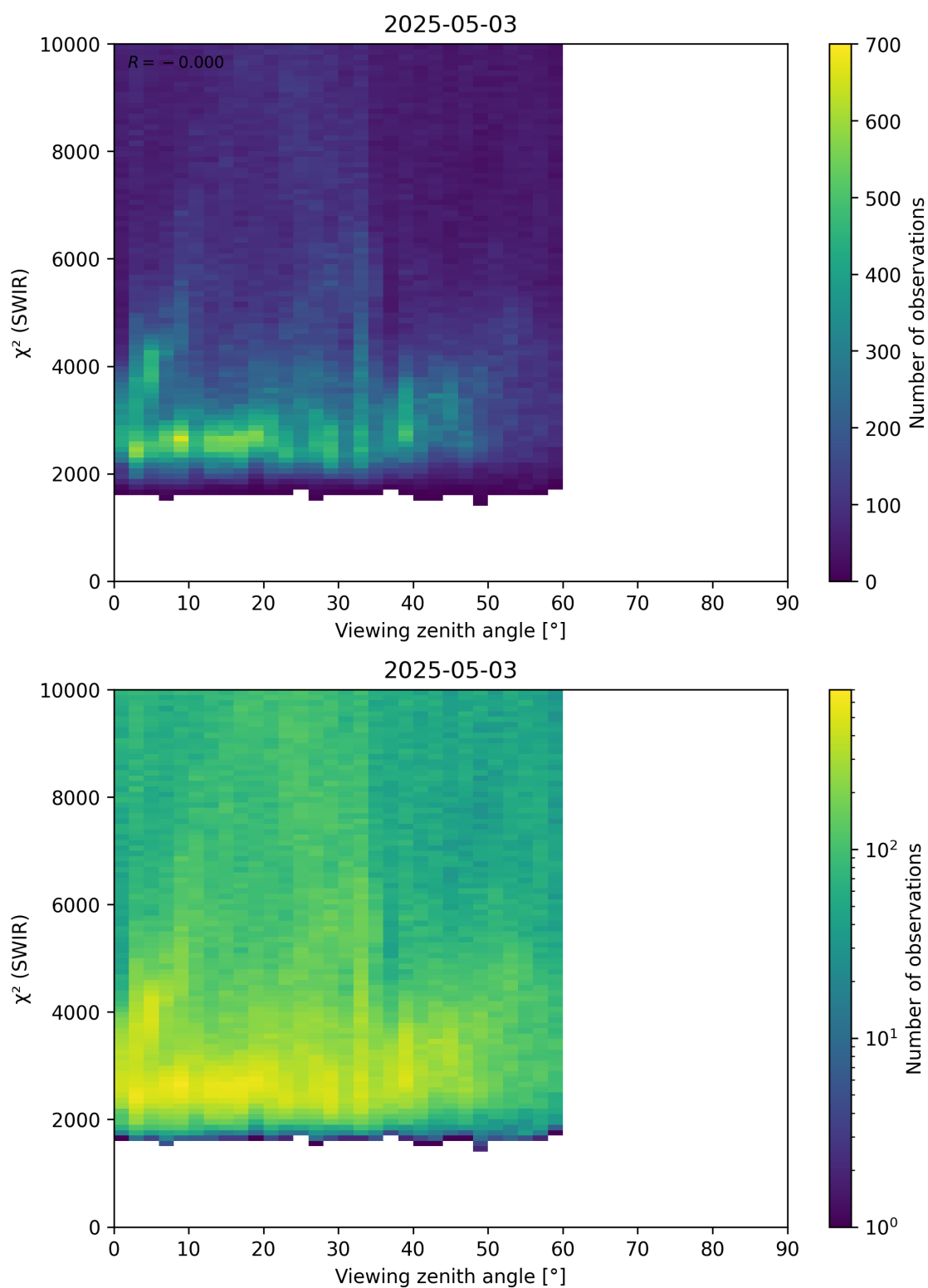
Figure 106: Scatter density plot of “Viewing zenith angle” against “ \chi^2 (SWIR)” for 2025-05-02 to 2025-05-04.
