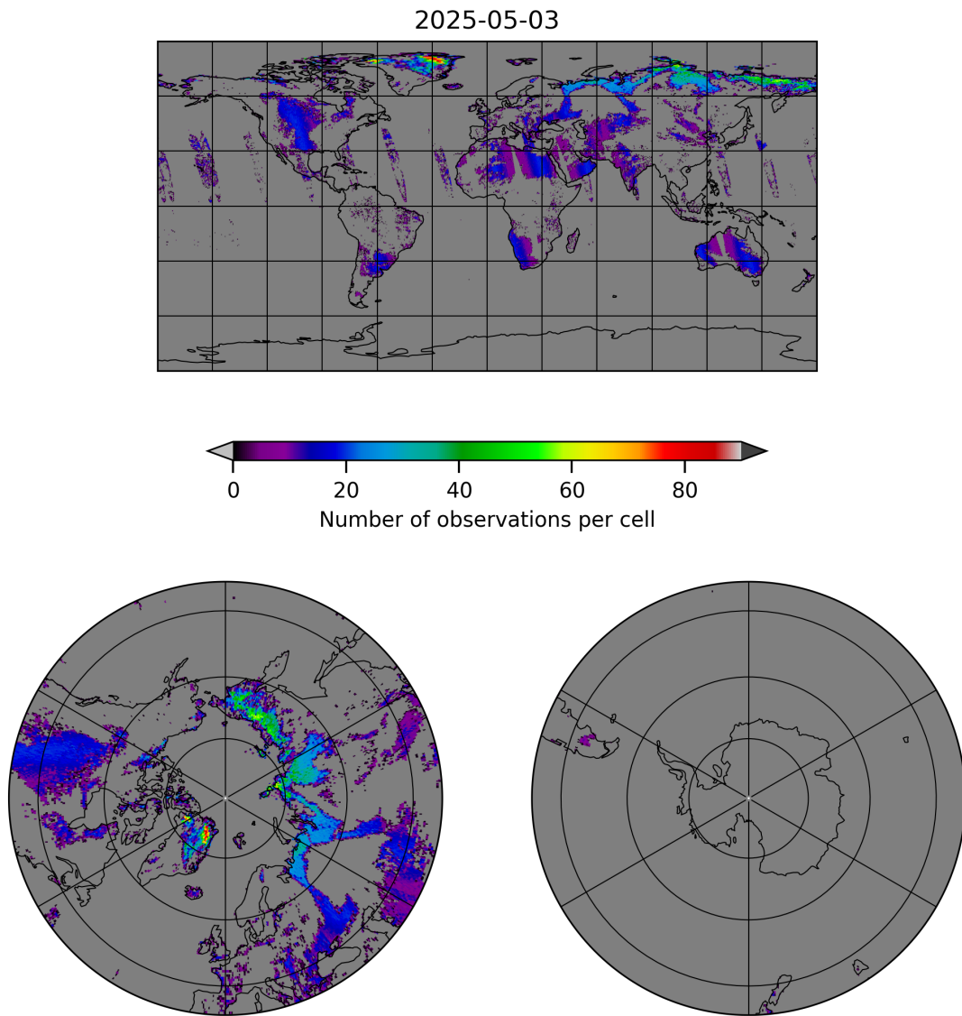
Figure 10: Map of the number of observations for 2025-05-02 to 2025-05-04
