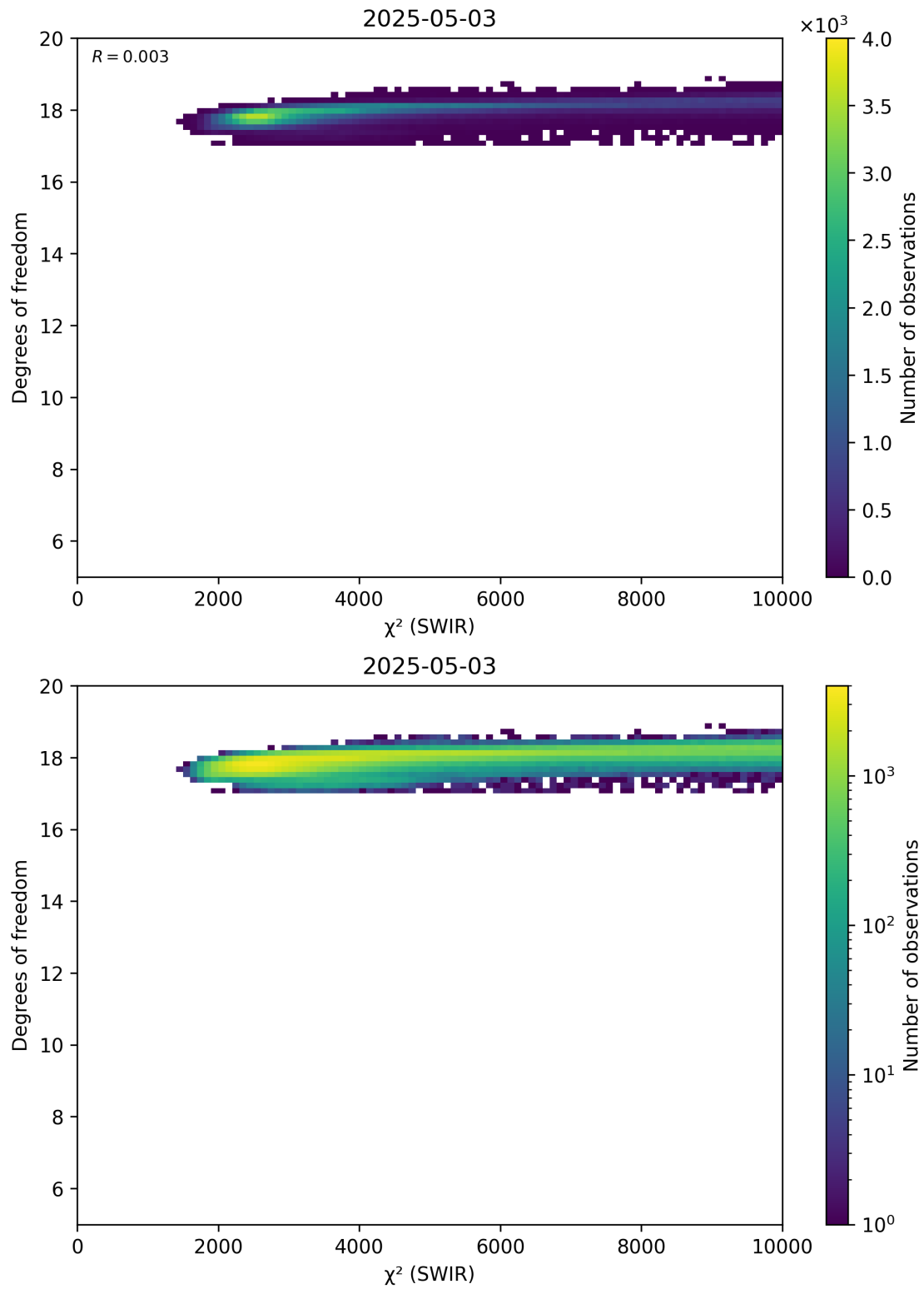
Figure 48: Scatter density plot of “ \chi^2 (SWIR)” against “Degrees of freedom” for 2025-05-02 to 2025-05-04.
