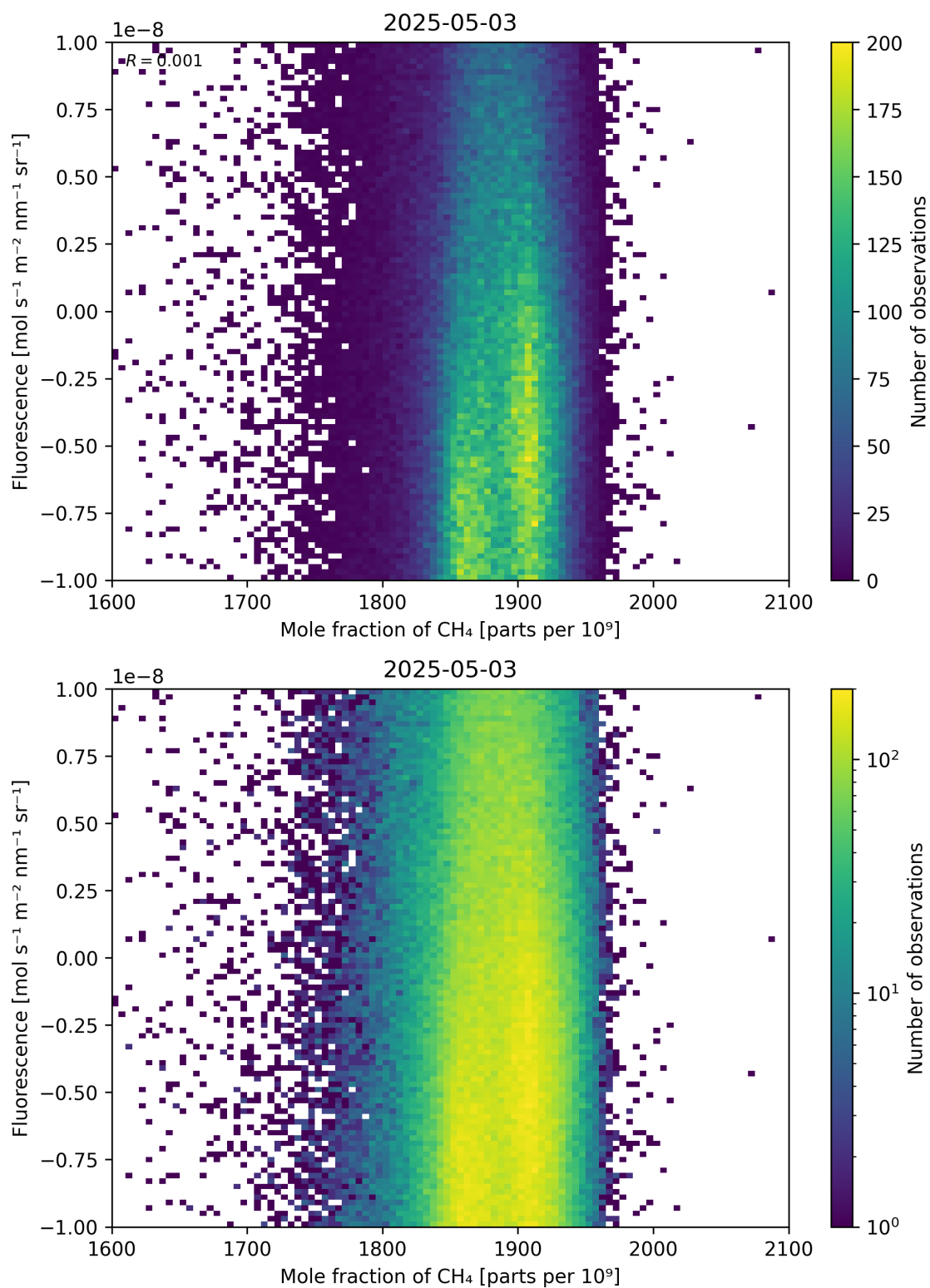
Figure 73: Scatter density plot of “Mole fraction of \text{CH}_4 ” against “Fluorescence” for 2025-05-02 to 2025-05-04.
