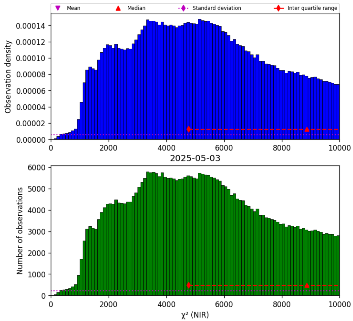
Figure 29: Histogram of “ \chi^2 (NIR)” for 2025-05-02 to 2025-05-04
