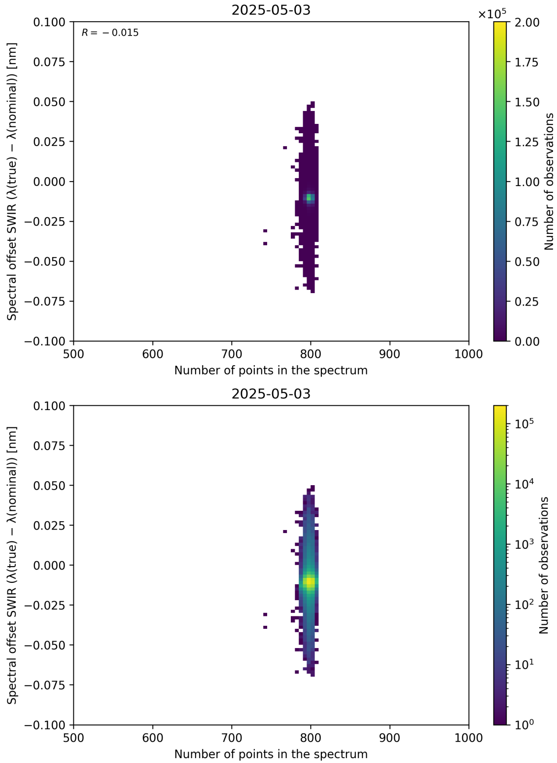
Figure 93: Scatter density plot of “Number of points in the spectrum” against “Spectral offset SWIR ( \lambda_{\text{true}} - \lambda_{\text{nominal}} )” for 2025-05-02 to 2025-05-04.
