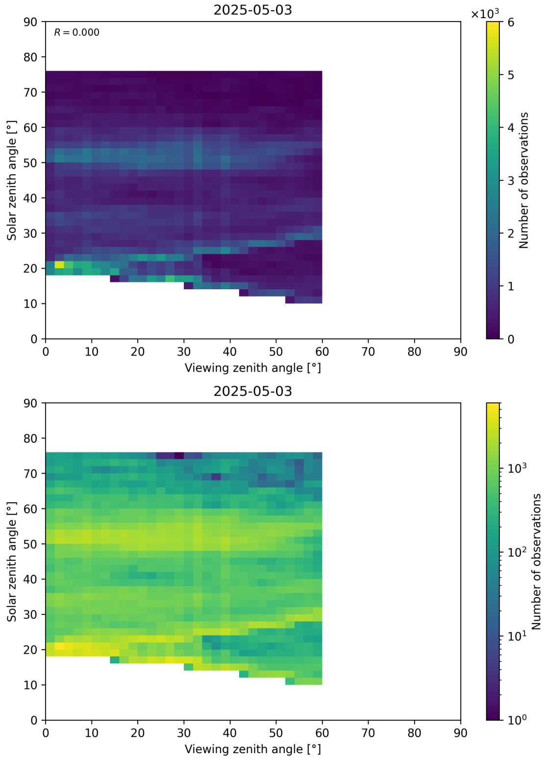
Figure 115: Scatter density plot of “Viewing zenith angle” against “Solar zenith angle” for 2025-05-02 to 2025-05-04.
