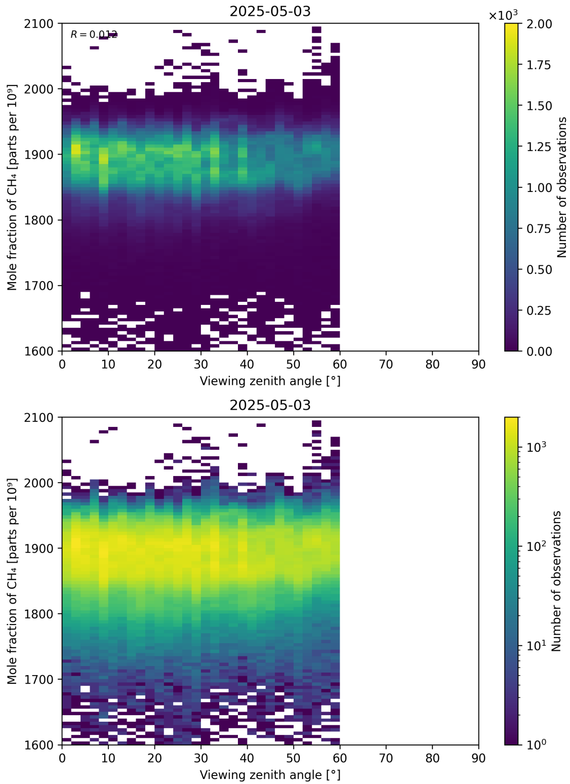
Figure 110: Scatter density plot of “Viewing zenith angle” against “Mole fraction of CH 4 ” for 2025-05-02 to 2025-05-04.
