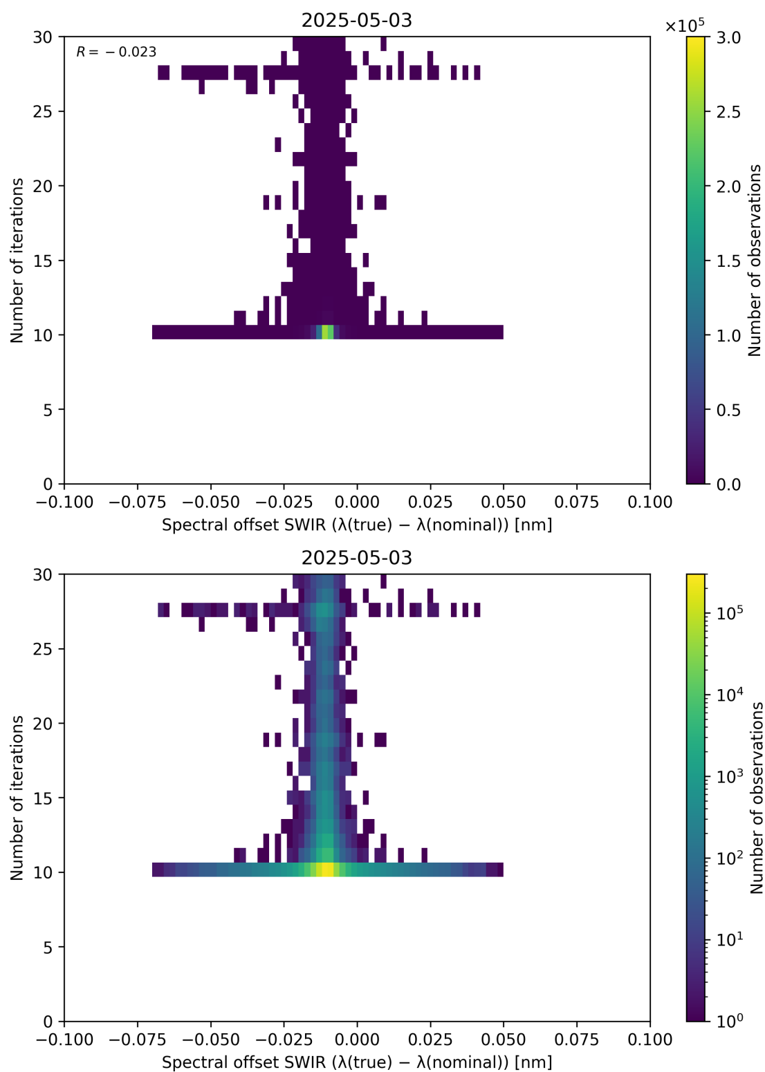
Figure 121: Scatter density plot of “Spectral offset SWIR ( \lambda_{\text{true}} - \lambda_{\text{nominal}} )” against “Number of iterations” for 2025-05-02 to 2025-05-04.
