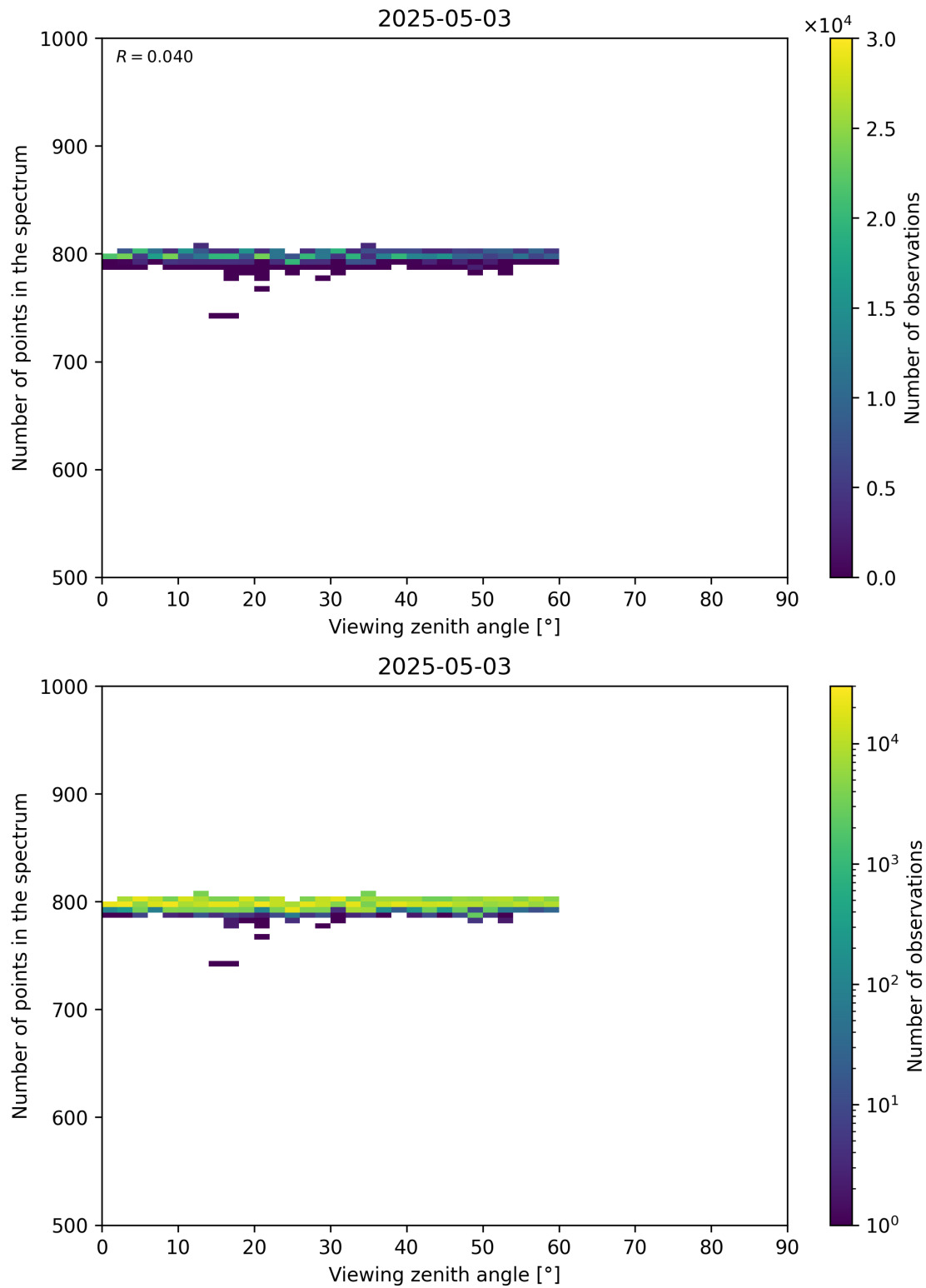
Figure 114: Scatter density plot of “Viewing zenith angle” against “Number of points in the spectrum” for 2025-05-02 to 2025-05-04.
