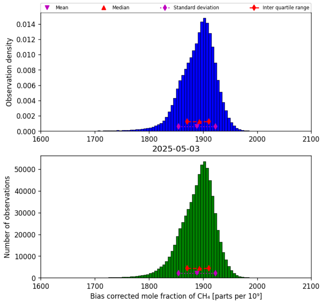
Figure 25: Histogram of “Bias corrected mole fraction of CH 4 ” for 2025-05-02 to 2025-05-04
