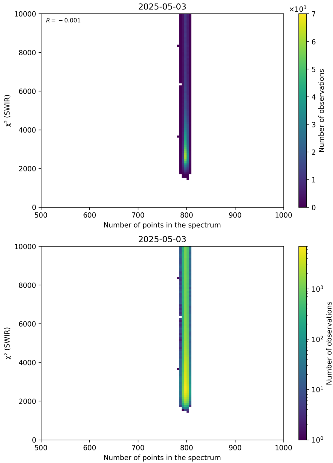
Figure 89: Scatter density plot of “Number of points in the spectrum” against “ \chi^2 (SWIR)” for 2025-05-02 to 2025-05-04.
