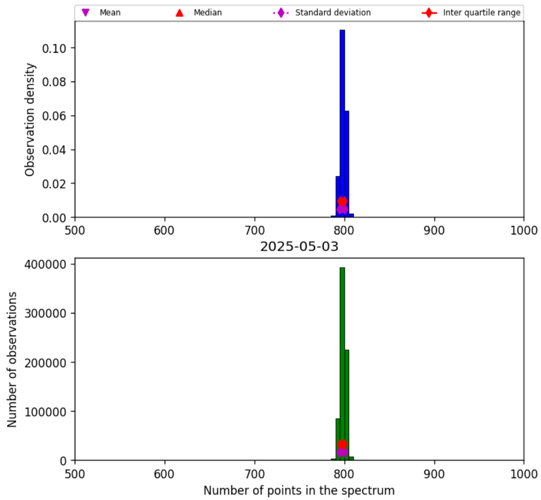
Figure 26: Histogram of “Number of points in the spectrum” for 2025-05-02 to 2025-05-04
