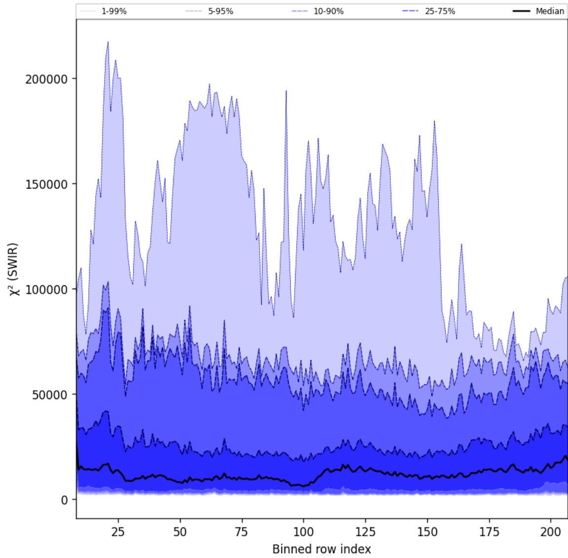
Figure 39: Along track statistics of “ \chi^2 (SWIR)” for 2025-05-02 to 2025-05-04
