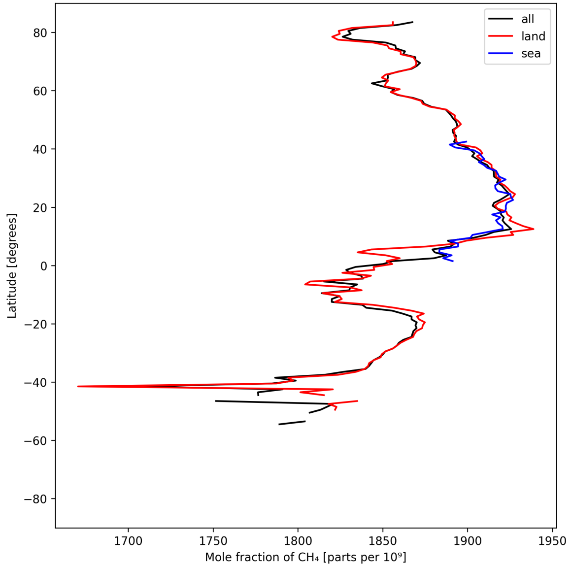
Figure 12: Zonal average of “Mole fraction of \text{CH}_4 ” for 2025-05-02 to 2025-05-04.
