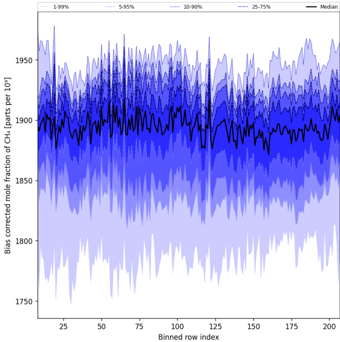
Figure 36: Along track statistics of “Bias corrected mole fraction of CH 4 ” for 2025-05-02 to 2025-05-04
