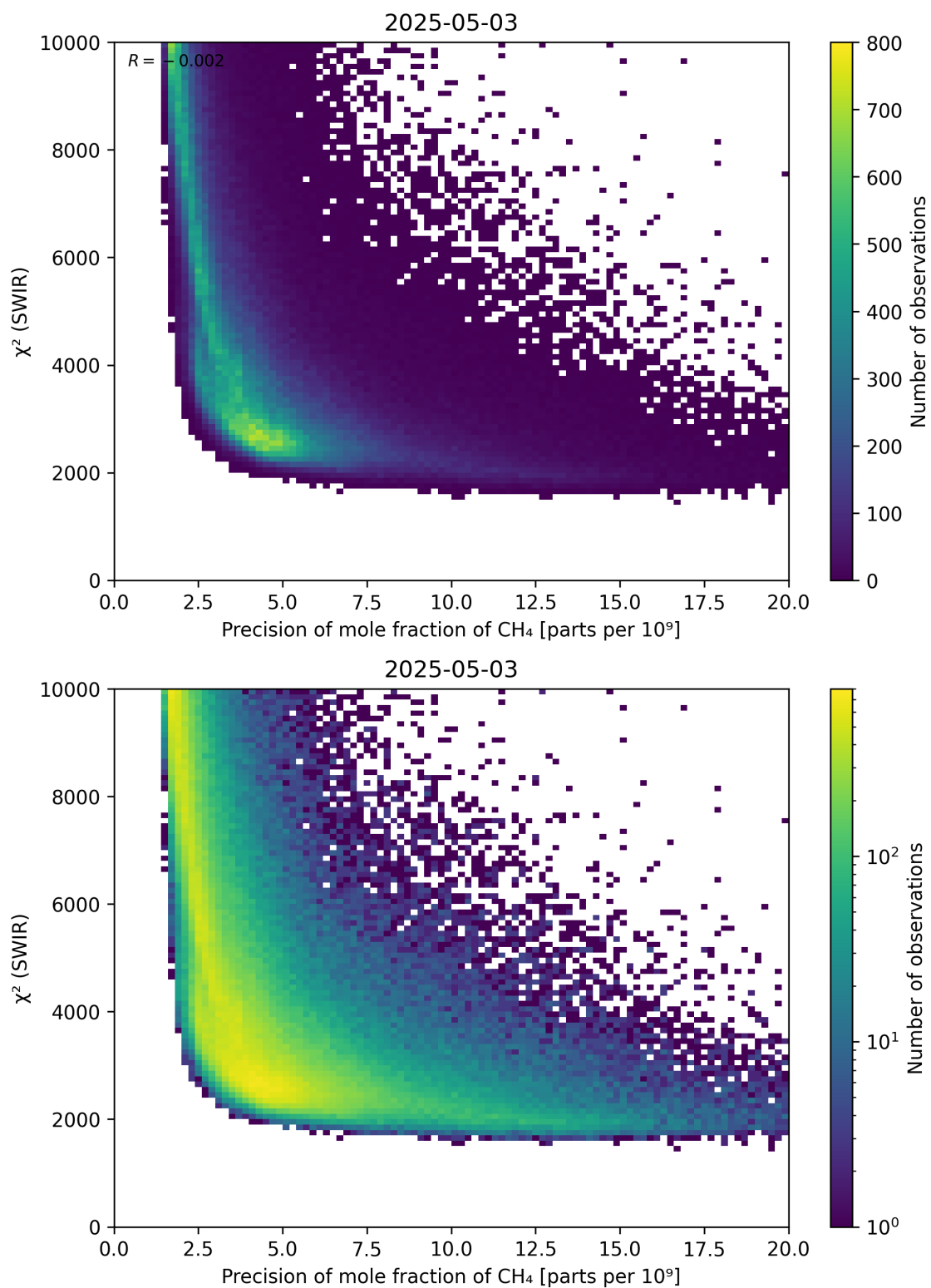
Figure 79: Scatter density plot of “Precision of mole fraction of CH 4 ” against “ \chi^2 (SWIR)” for 2025-05-02 to 2025-05-04.
