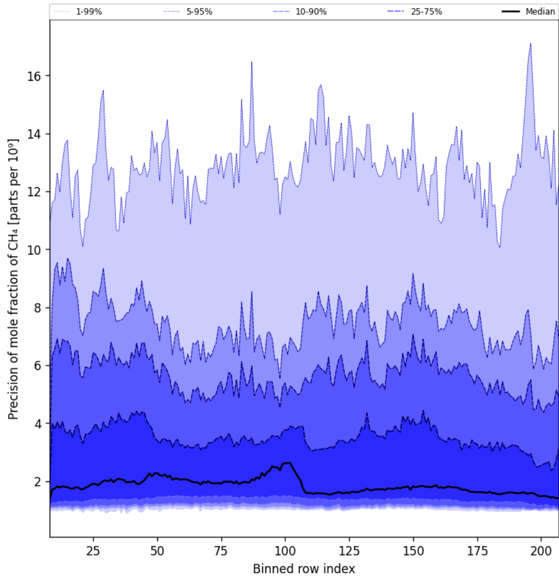
Figure 35: Along track statistics of “Precision of mole fraction of CH 4 ” for 2025-05-02 to 2025-05-04
