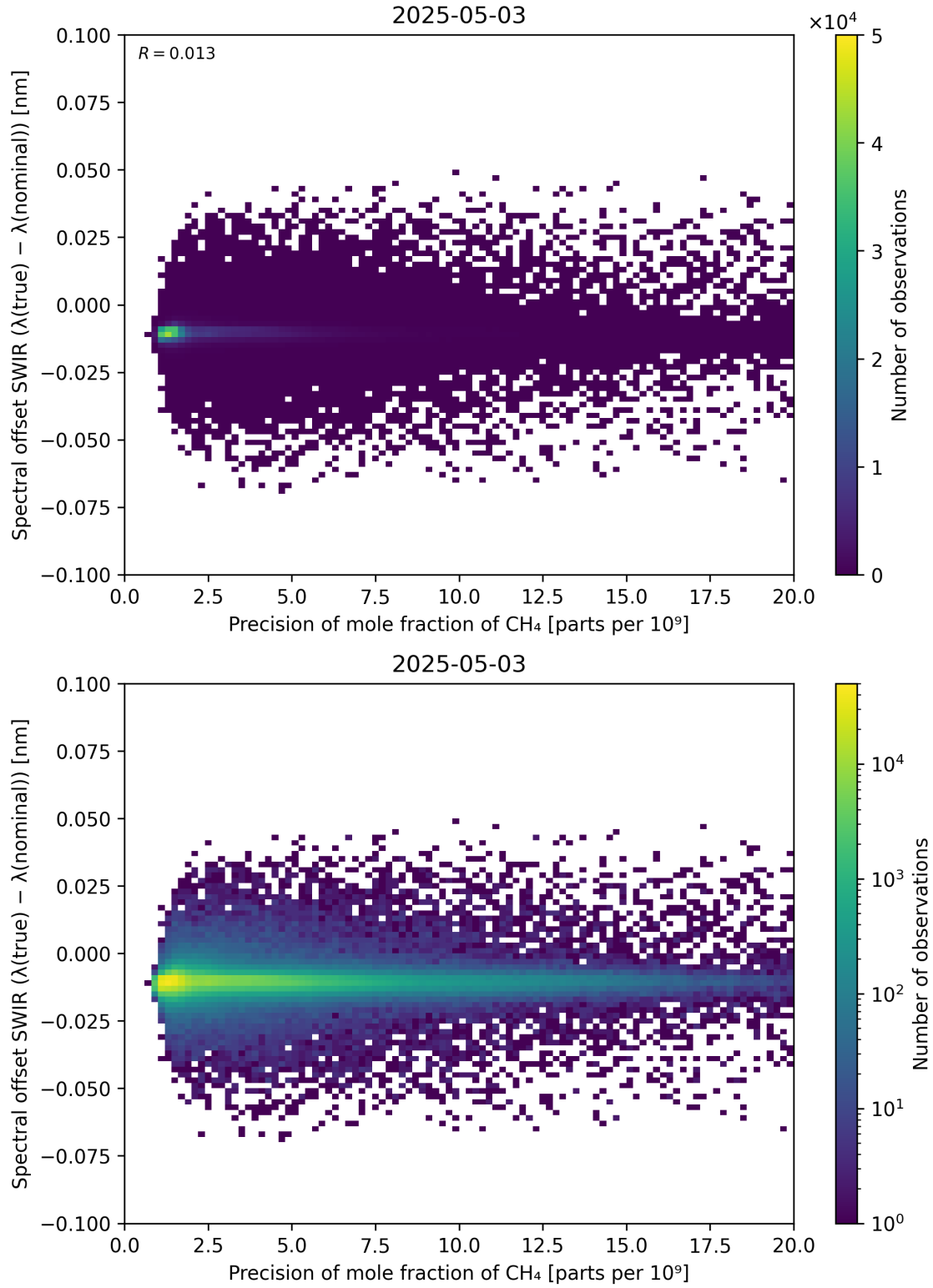
Figure 85: Scatter density plot of “Precision of mole fraction of \text{CH}_4 ” against “Spectral offset SWIR ( \lambda_{\text{true}} - \lambda_{\text{nominal}} )” for 2025-05-02 to 2025-05-04.
