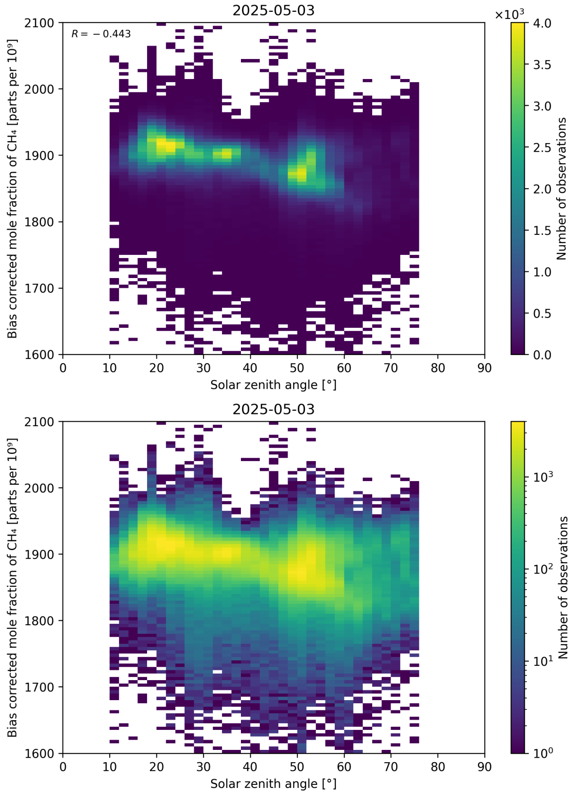
Figure 100: Scatter density plot of “Solar zenith angle” against “Bias corrected mole fraction of CH 4 ” for 2025-05-02 to 2025-05-04.
