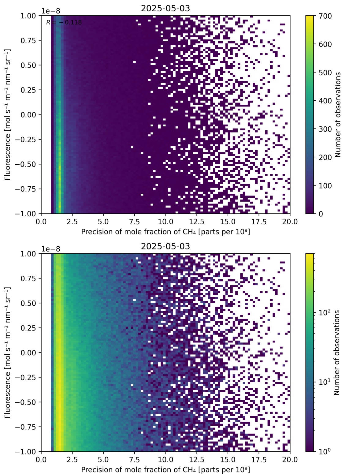
Figure 81: Scatter density plot of “Precision of mole fraction of \text{CH}_4 ” against “Fluorescence” for 2025-05-02 to 2025-05-04.
