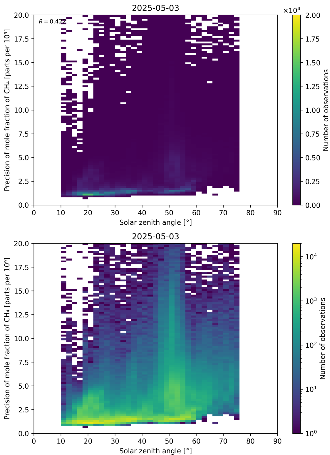
Figure 101: Scatter density plot of “Solar zenith angle” against “Precision of mole fraction of CH 4 ” for 2025-05-02 to 2025-05-04.
