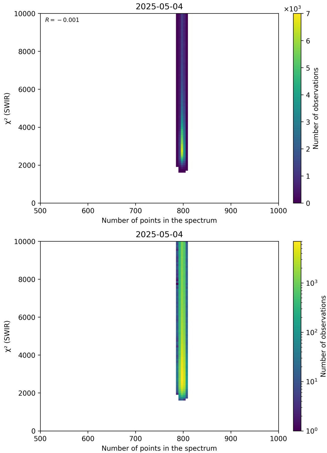
Figure 89: Scatter density plot of “Number of points in the spectrum” against “ \chi^2 (SWIR)” for 2025-05-03 to 2025-05-05.
