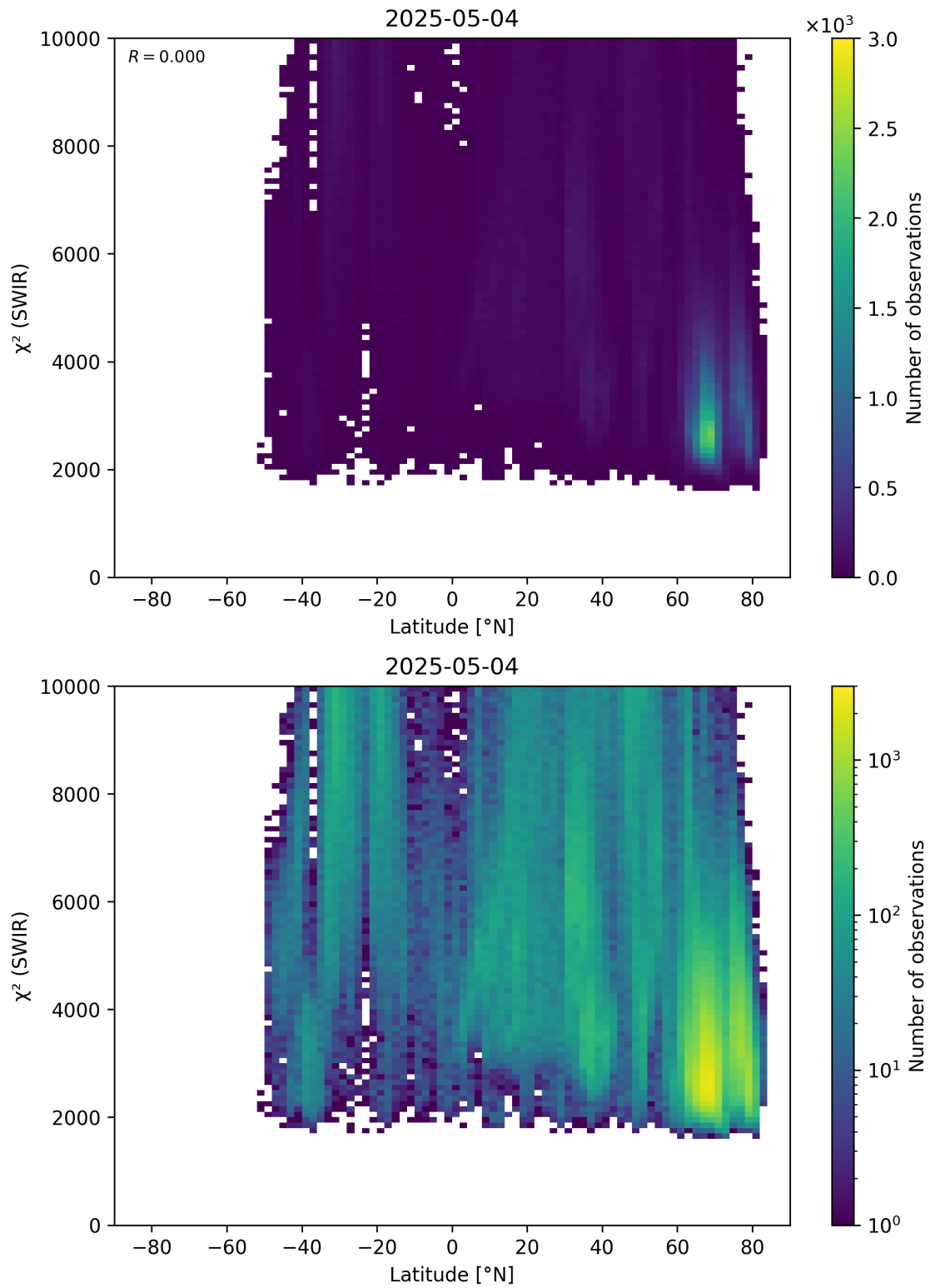
Figure 54: Scatter density plot of “Latitude” against “ \chi^2 (SWIR)” for 2025-05-03 to 2025-05-05.
