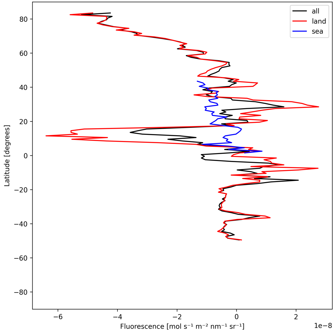
Figure 21: Zonal average of “Fluorescence” for 2025-05-03 to 2025-05-05.
