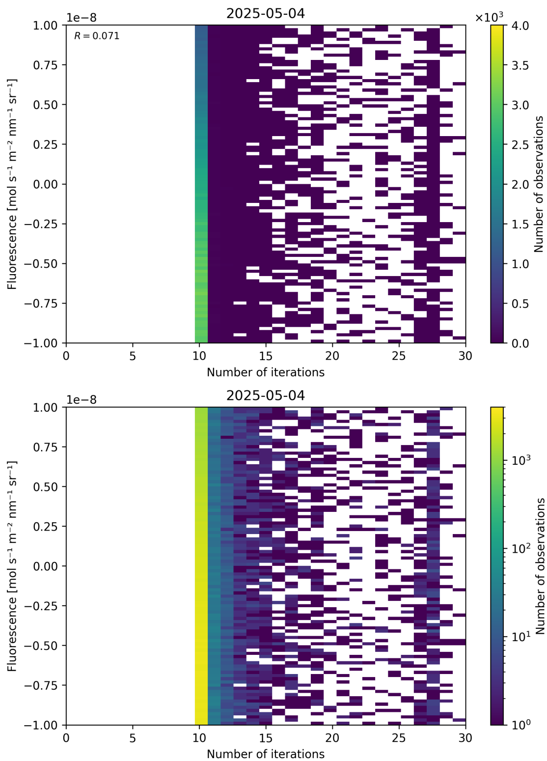
Figure 87: Scatter density plot of “Number of iterations” against “Fluorescence” for 2025-05-03 to 2025-05-05.
