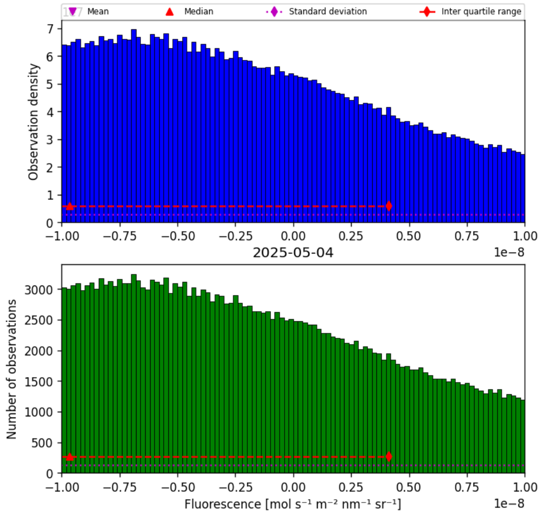
Figure 32: Histogram of “Fluorescence” for 2025-05-03 to 2025-05-05
