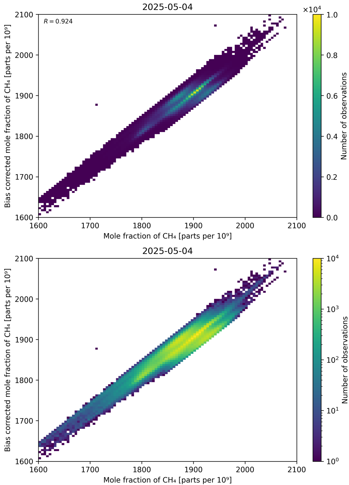
Figure 74: Scatter density plot of “Mole fraction of CH 4 ” against “Bias corrected mole fraction of CH 4 ” for 2025-05-03 to 2025-05-05.
