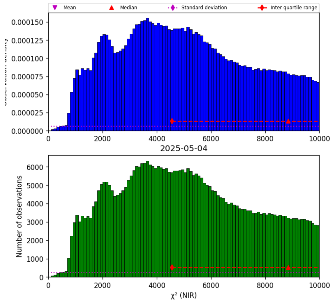
Figure 29: Histogram of “ \chi^2 (NIR)” for 2025-05-03 to 2025-05-05
