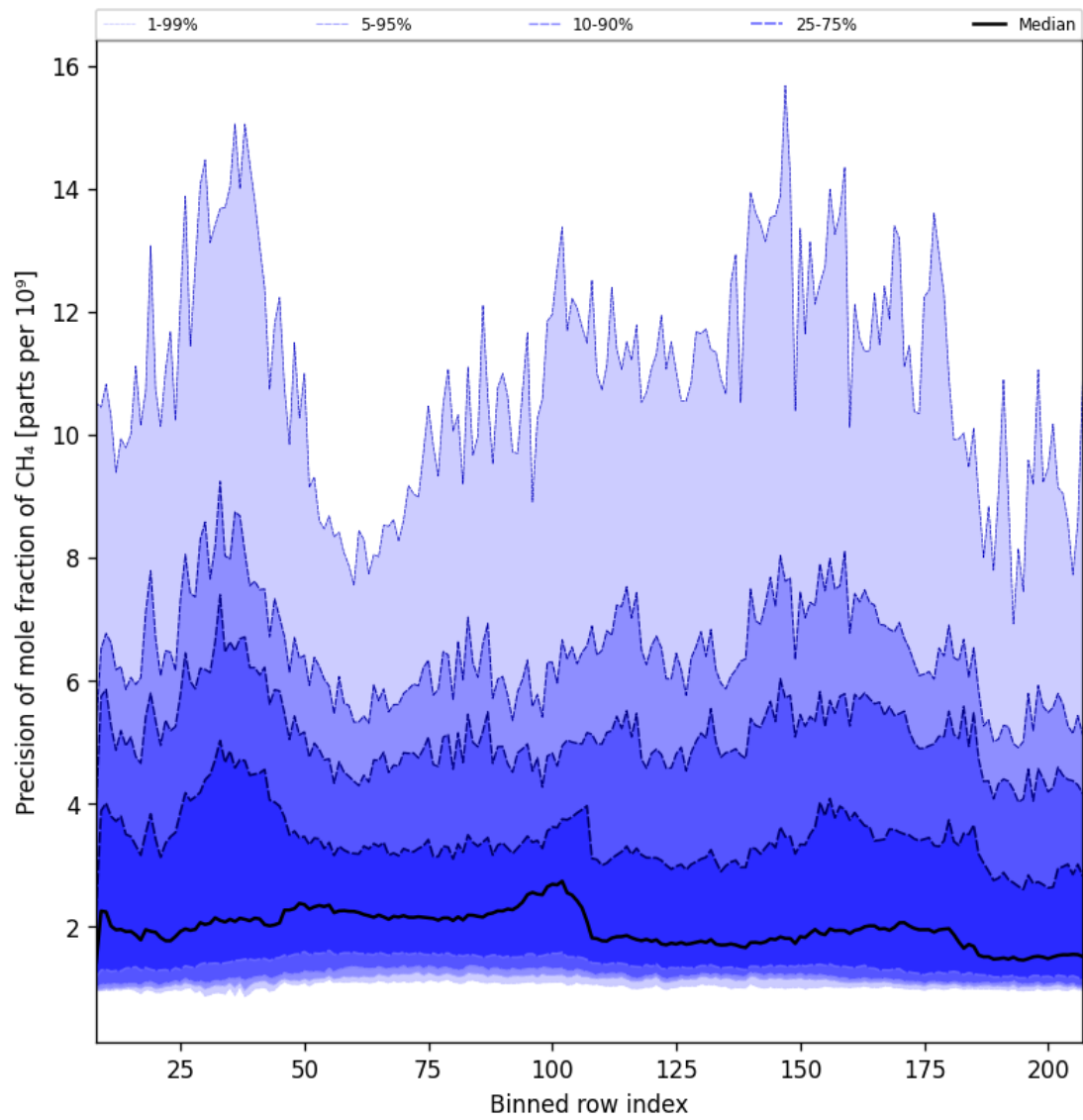
Figure 35: Along track statistics of “Precision of mole fraction of CH 4 ” for 2025-05-03 to 2025-05-05
