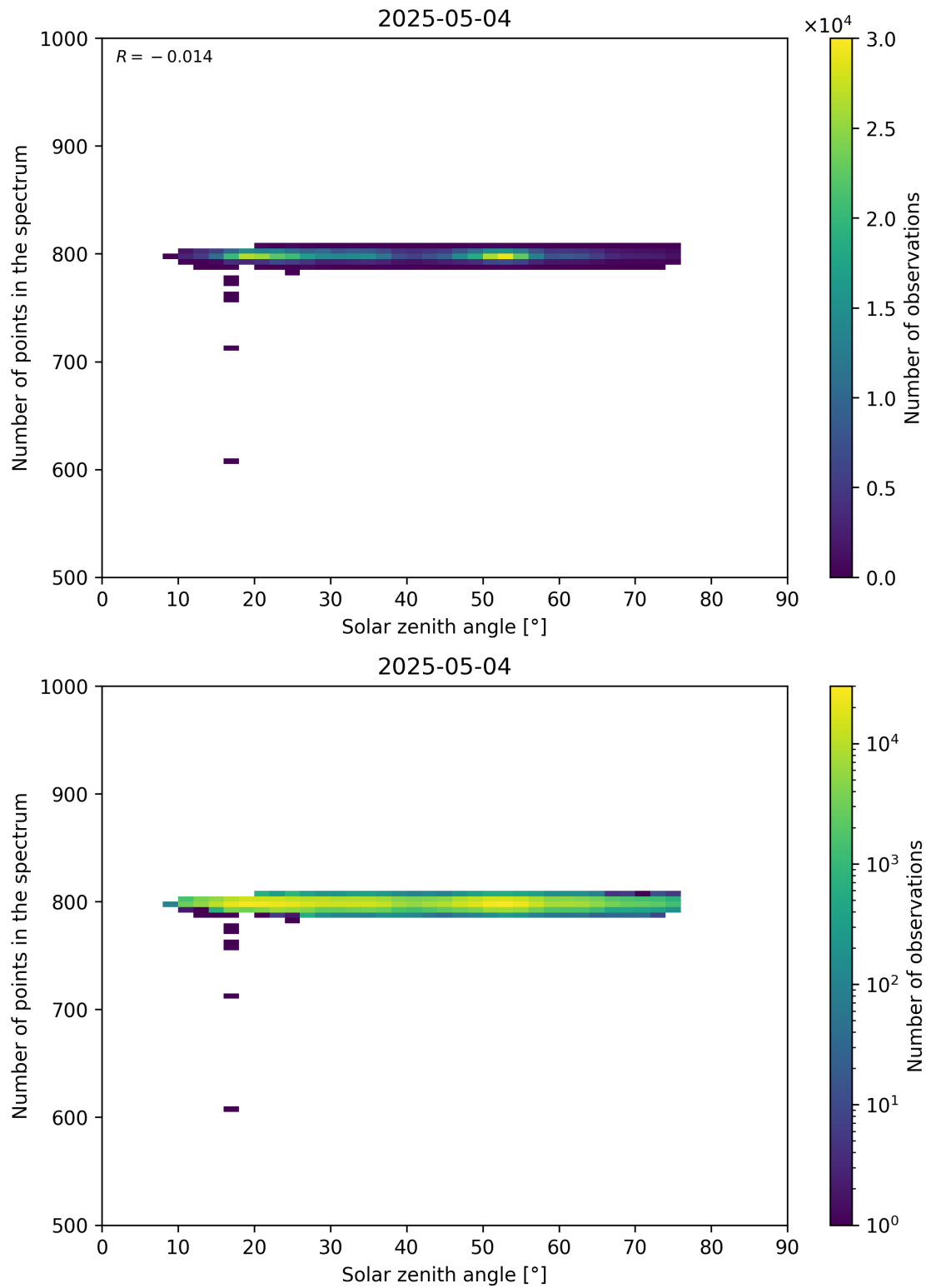
Figure 103: Scatter density plot of “Solar zenith angle” against “Number of points in the spectrum” for 2025-05-03 to 2025-05-05.
