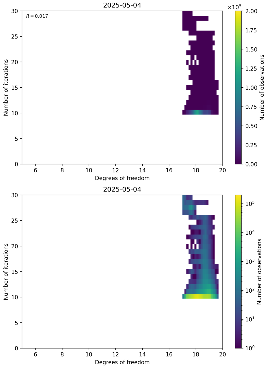
Figure 52: Scatter density plot of “Degrees of freedom” against “Number of iterations” for 2025-05-03 to 2025-05-05.
