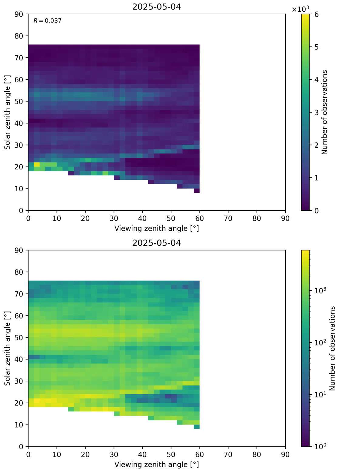
Figure 115: Scatter density plot of “Viewing zenith angle” against “Solar zenith angle” for 2025-05-03 to 2025-05-05.
