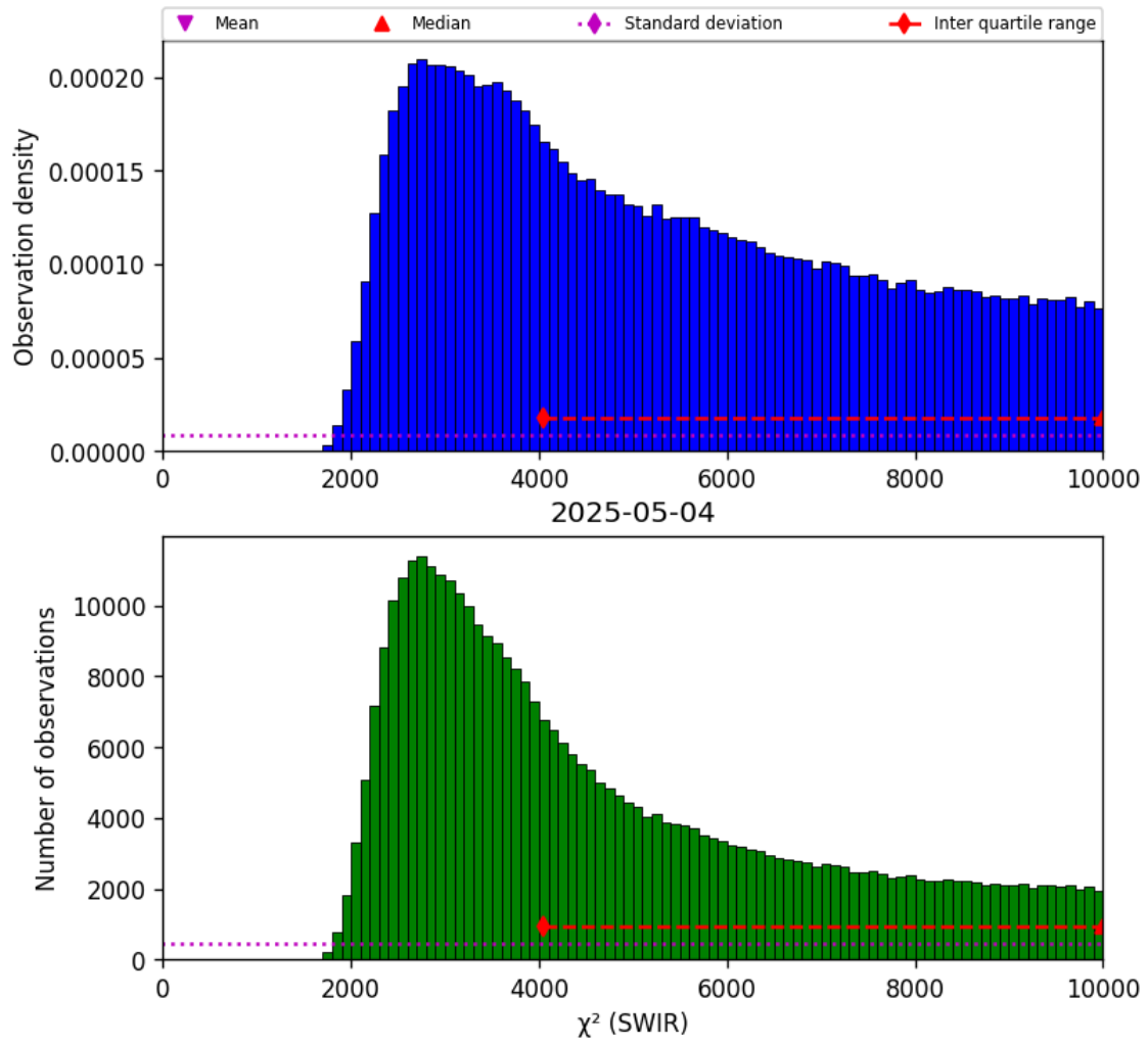
Figure 28: Histogram of “ \chi^2 (SWIR)” for 2025-05-03 to 2025-05-05
