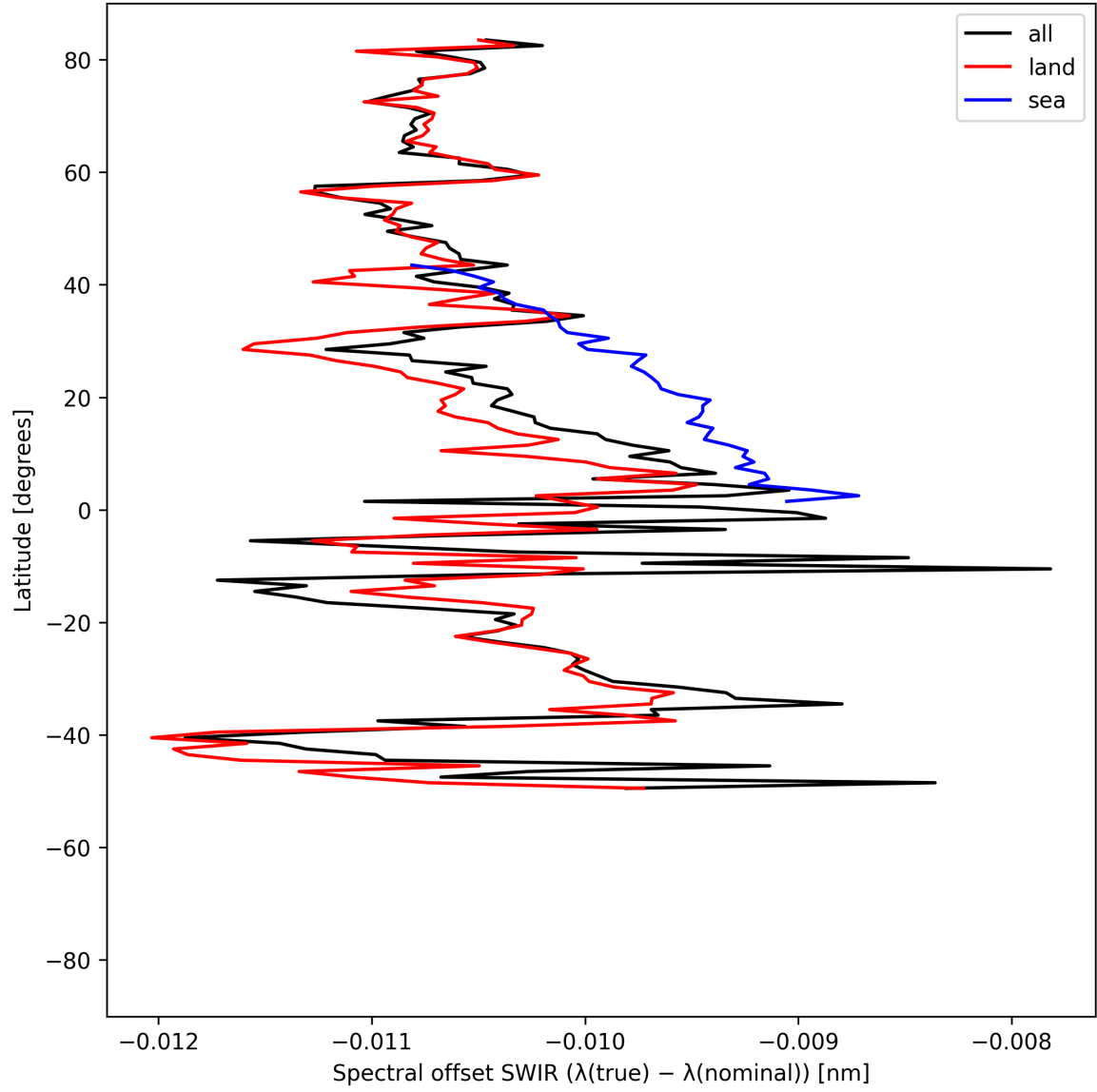
Figure 16: Zonal average of “Spectral offset SWIR ( \lambda_{\text{true}} - \lambda_{\text{nominal}} )” for 2025-05-03 to 2025-05-05.
