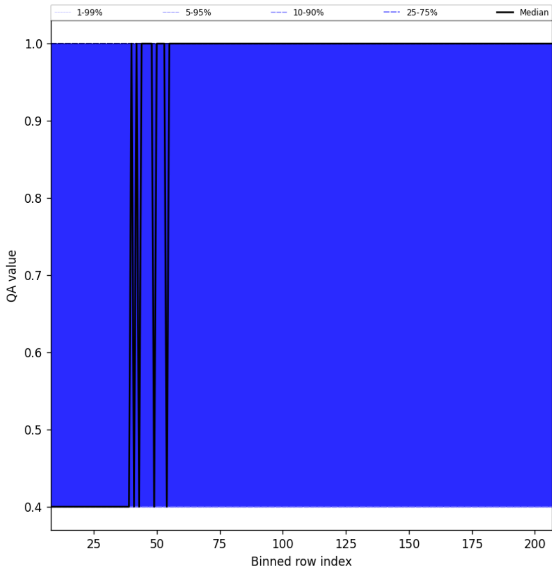
Figure 33: Along track statistics of “QA value” for 2025-05-03 to 2025-05-05
