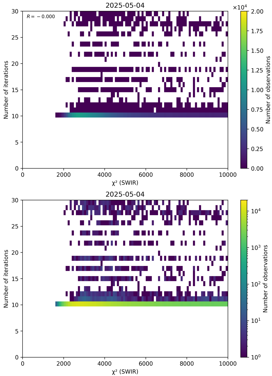
Figure 50: Scatter density plot of “ \chi^2 (SWIR)” against “Number of iterations” for 2025-05-03 to 2025-05-05.
