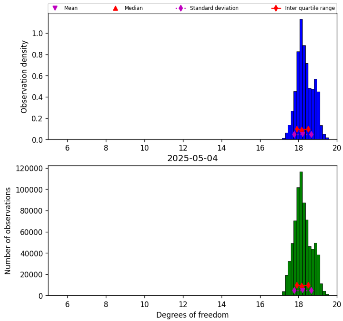
Figure 30: Histogram of “Degrees of freedom” for 2025-05-03 to 2025-05-05
