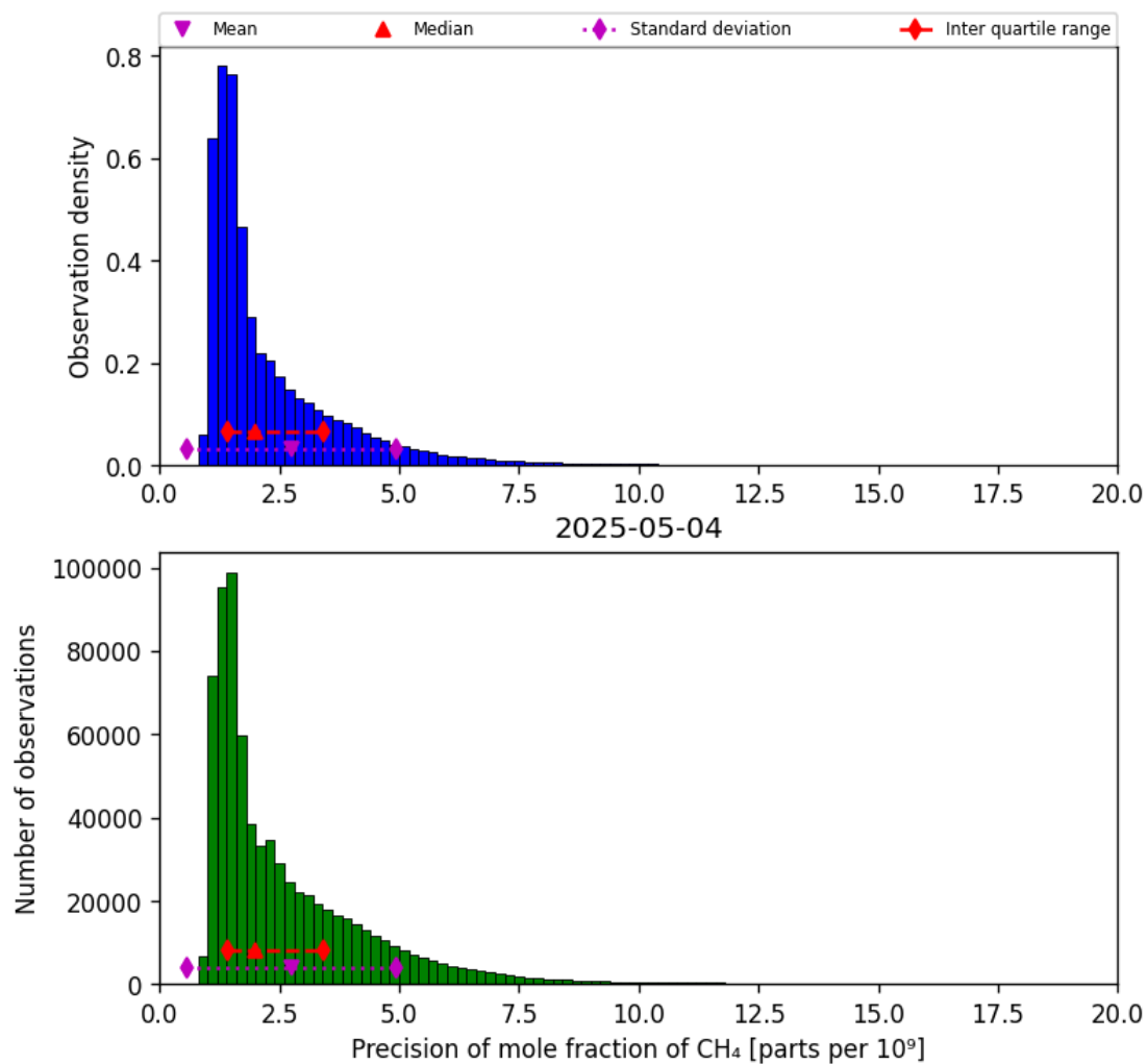
Figure 24: Histogram of “Precision of mole fraction of CH 4 ” for 2025-05-03 to 2025-05-05
