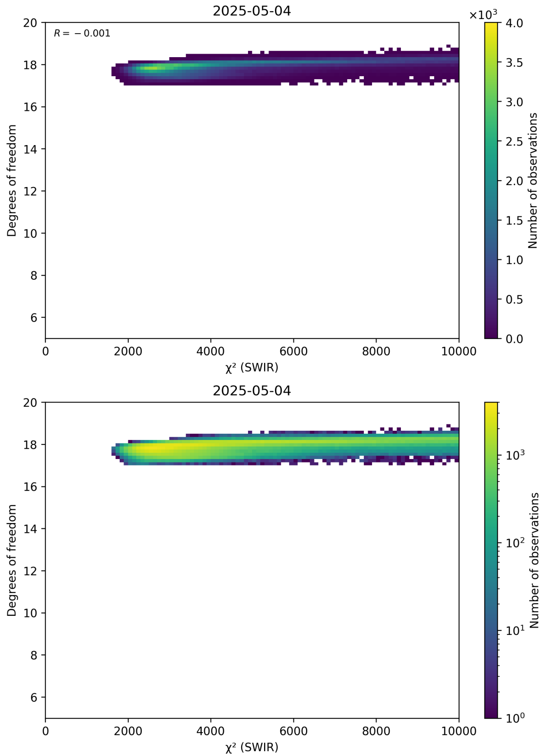
Figure 48: Scatter density plot of “ \chi^2 (SWIR)” against “Degrees of freedom” for 2025-05-03 to 2025-05-05.
