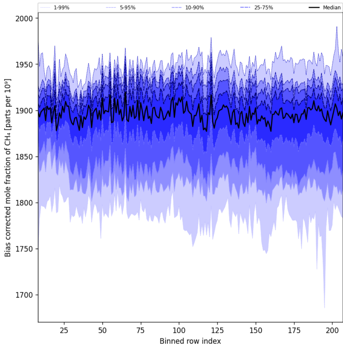
Figure 36: Along track statistics of “Bias corrected mole fraction of CH 4 ” for 2025-05-03 to 2025-05-05
