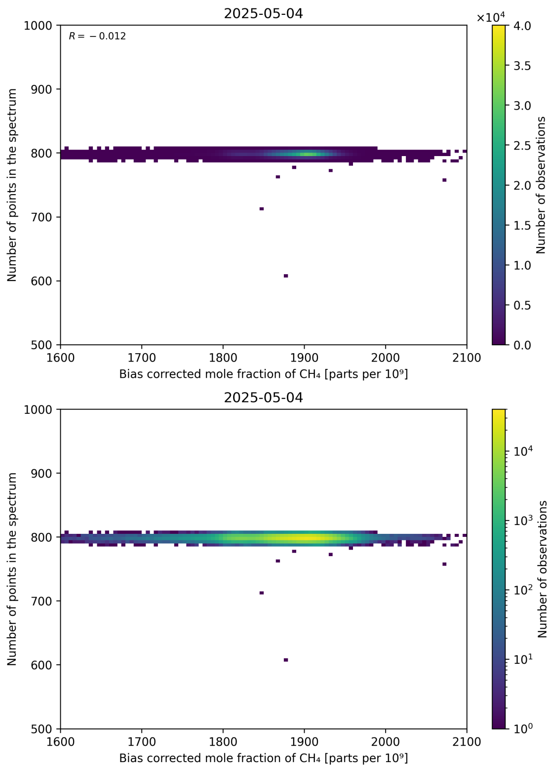
Figure 68: Scatter density plot of “Bias corrected mole fraction of CH 4 ” against “Number of points in the spectrum” for 2025-05-03 to 2025-05-05.
