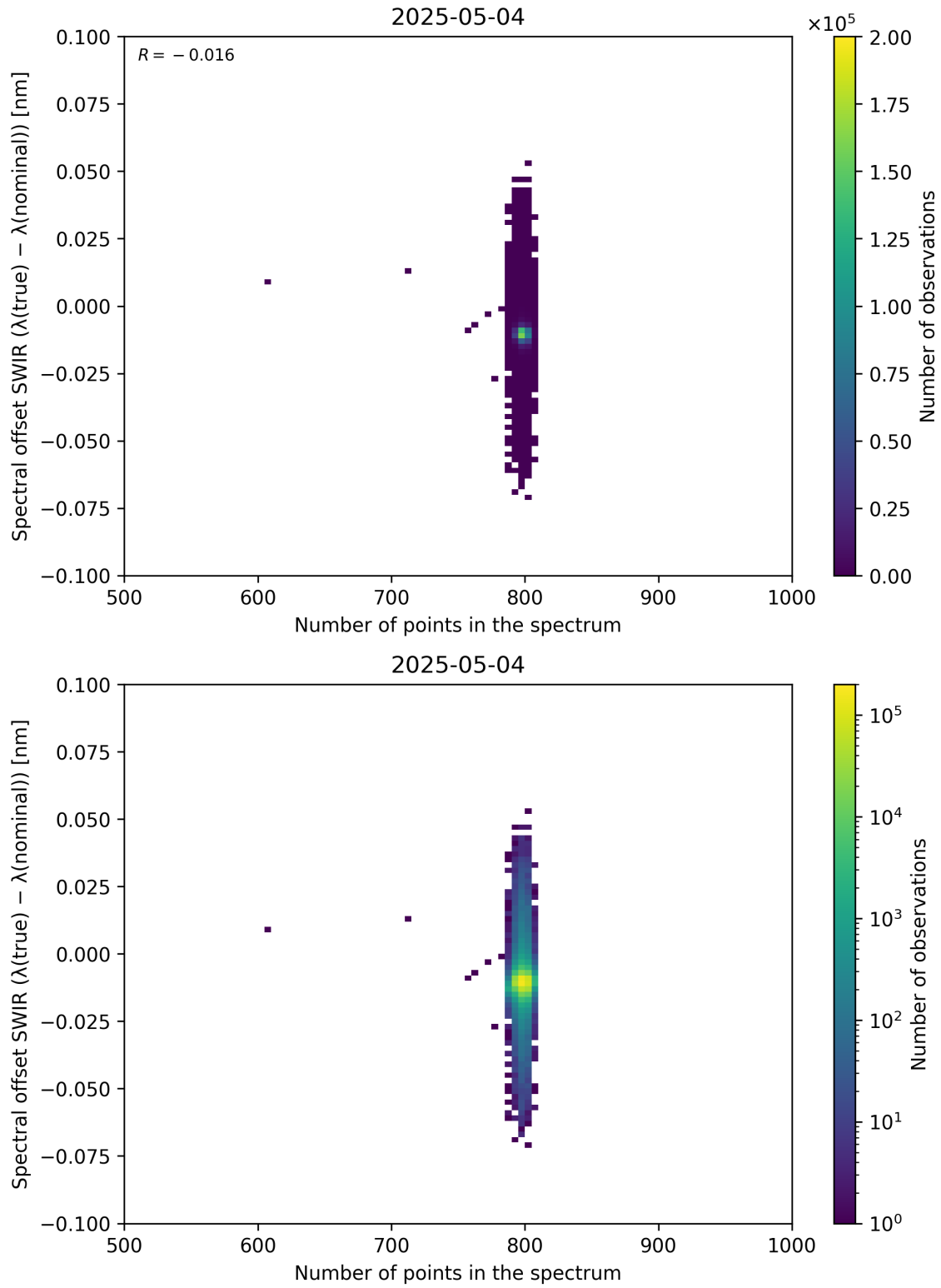
Figure 93: Scatter density plot of “Number of points in the spectrum” against “Spectral offset SWIR ( \lambda_{\text{true}} - \lambda_{\text{nominal}} )” for 2025-05-03 to 2025-05-05.
