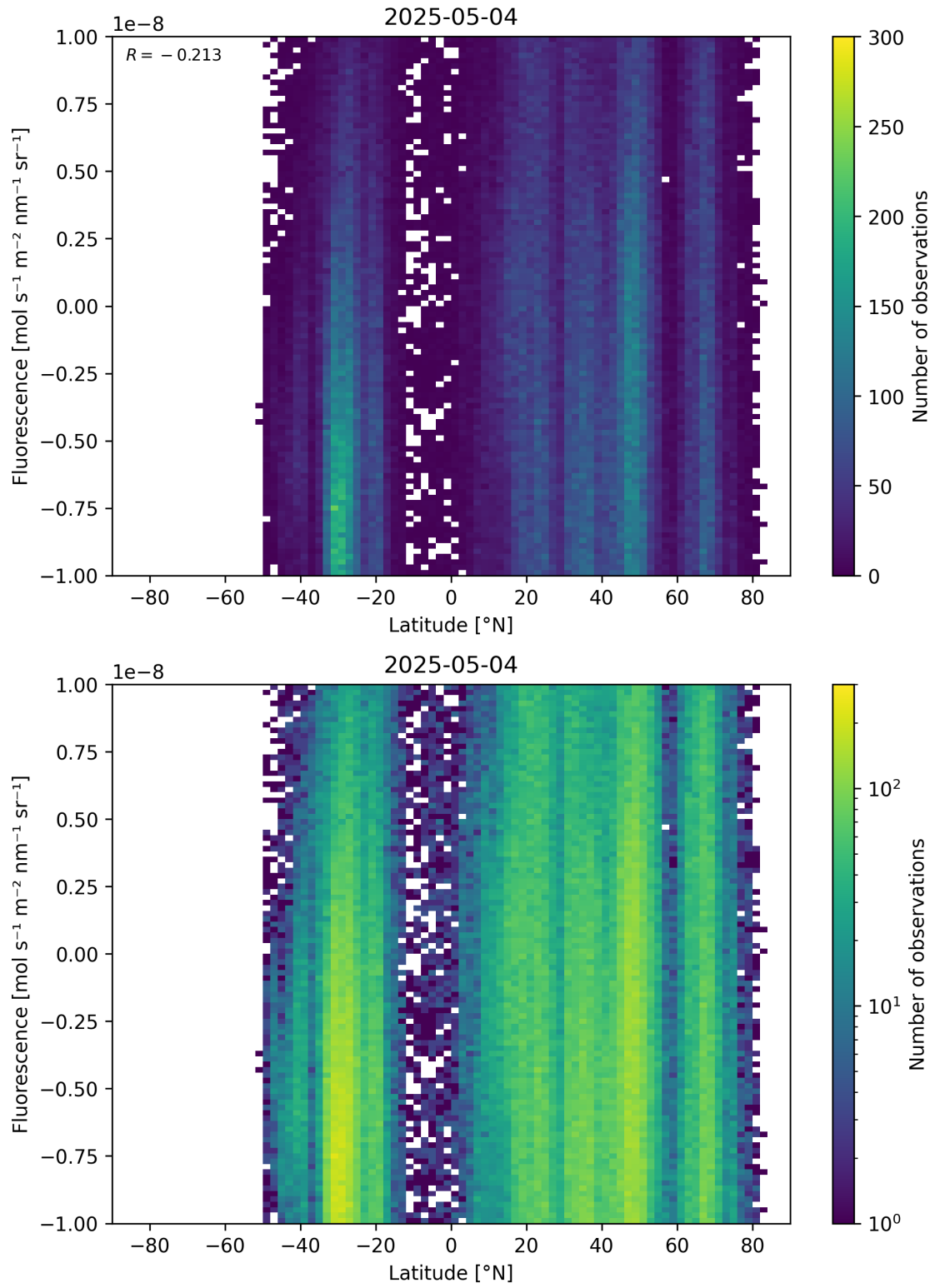
Figure 56: Scatter density plot of “Latitude” against “Fluorescence” for 2025-05-03 to 2025-05-05.
