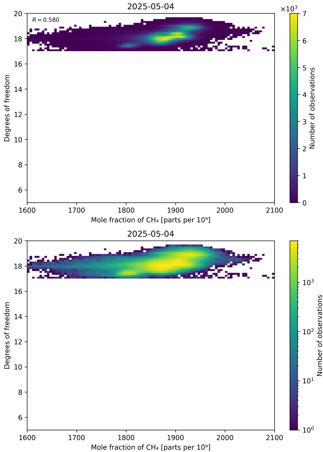
Figure 72: Scatter density plot of “Mole fraction of CH 4 ” against “Degrees of freedom” for 2025-05-03 to 2025-05-05.
