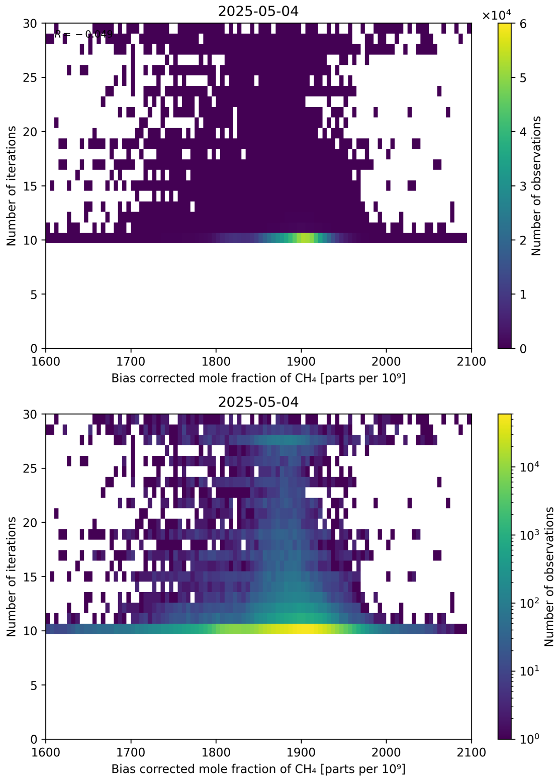
Figure 67: Scatter density plot of “Bias corrected mole fraction of \text{CH}_4 ” against “Number of iterations” for 2025-05-03 to 2025-05-05.
