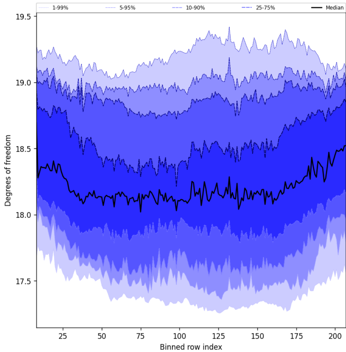
Figure 41: Along track statistics of “Degrees of freedom” for 2025-05-03 to 2025-05-05
