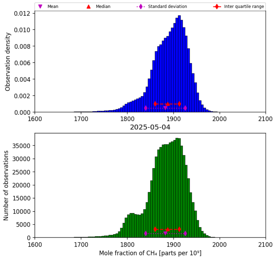
Figure 23: Histogram of “Mole fraction of CH 4 ” for 2025-05-03 to 2025-05-05
