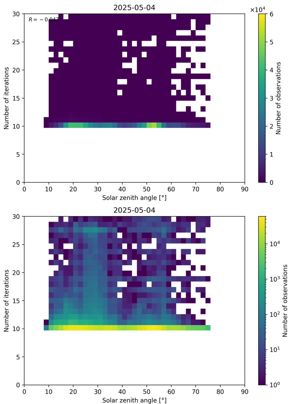
Figure 102: Scatter density plot of “Solar zenith angle” against “Number of iterations” for 2025-05-03 to 2025-05-05.
