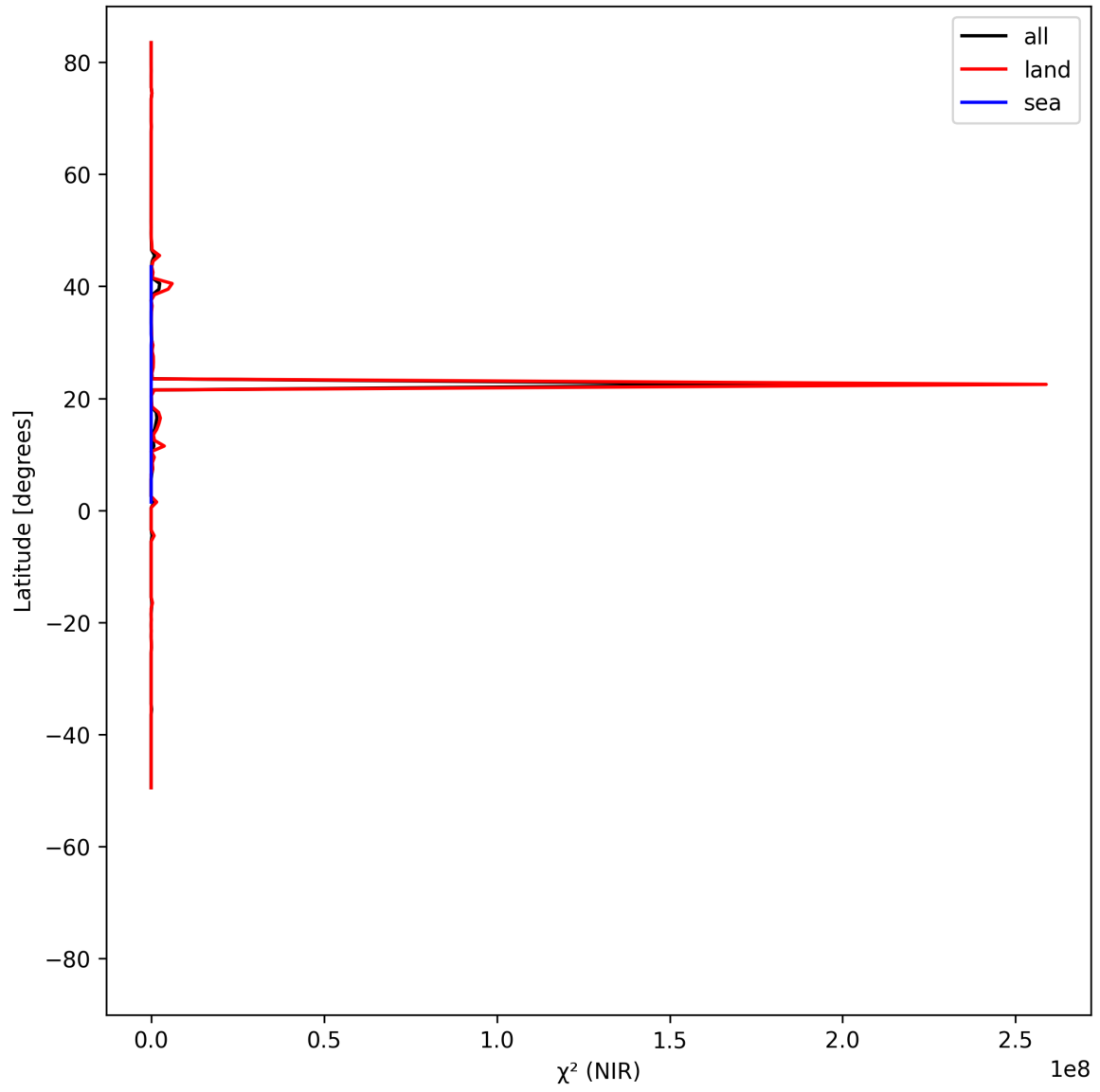
Figure 18: Zonal average of “ \chi^2 (NIR)” for 2025-05-03 to 2025-05-05.
