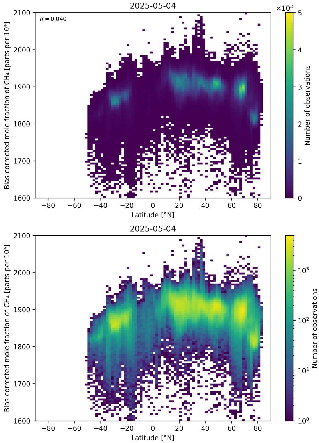
Figure 58: Scatter density plot of “Latitude” against “Bias corrected mole fraction of CH 4 ” for 2025-05-03 to 2025-05-05.
