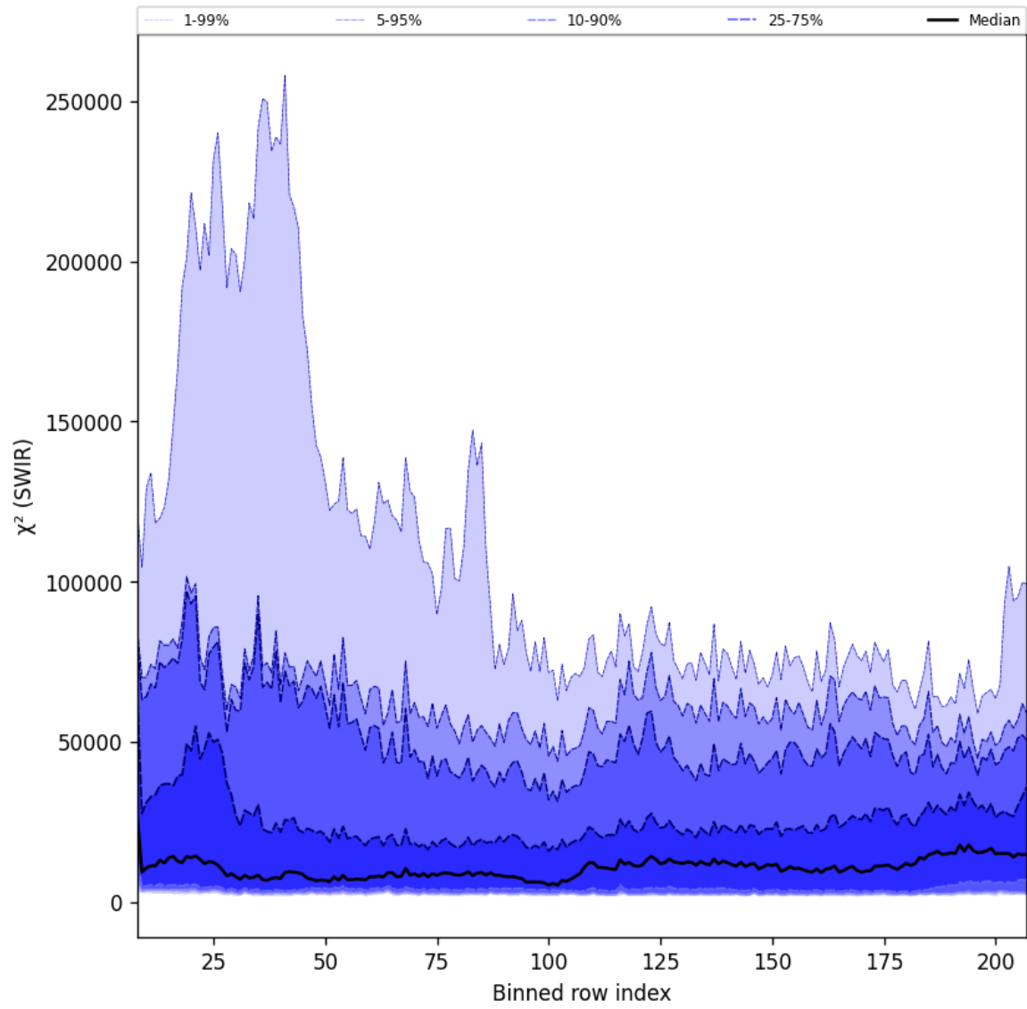
Figure 39: Along track statistics of " \chi^2 (SWIR)" for 2025-05-03 to 2025-05-05
