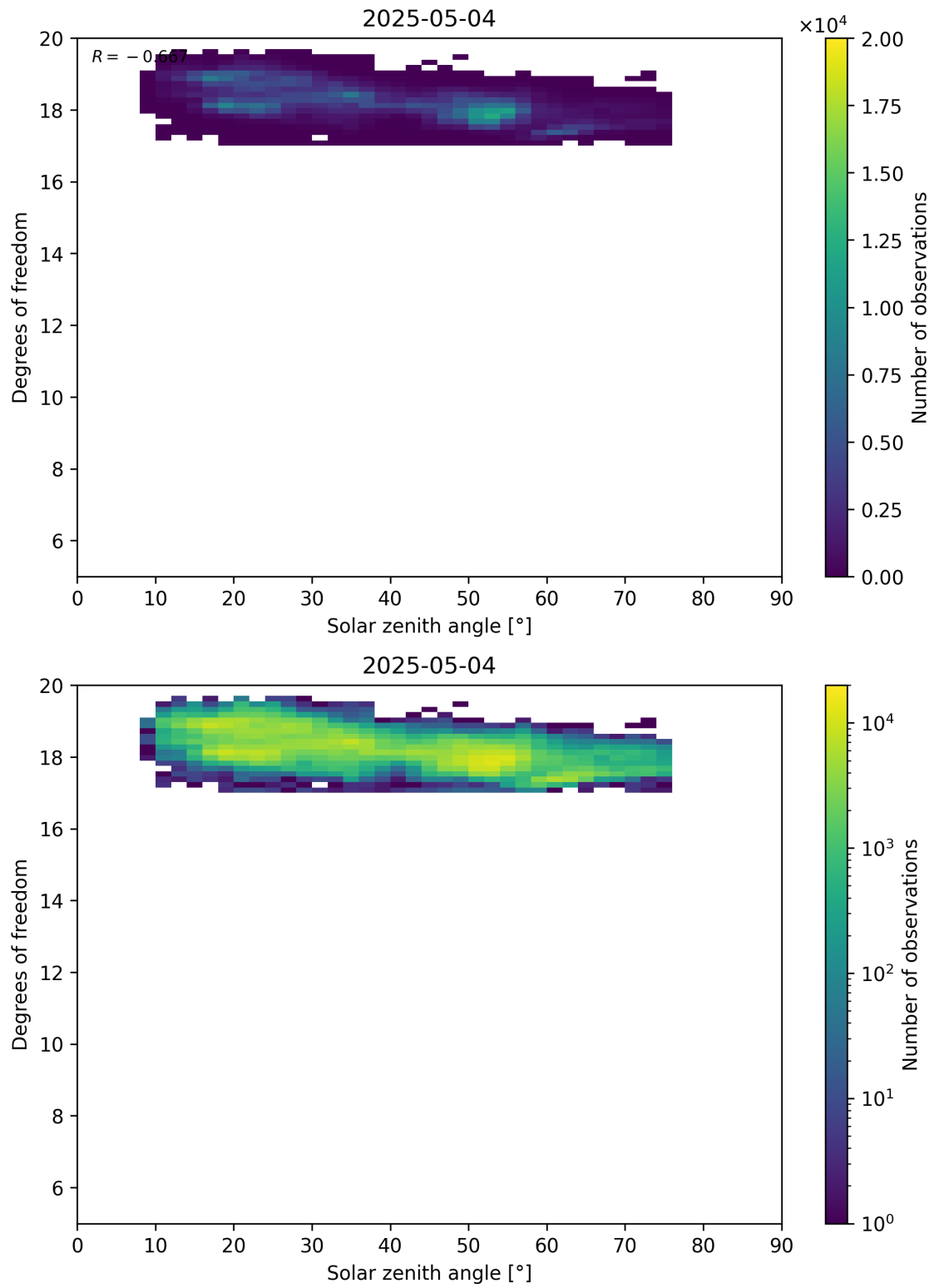
Figure 96: Scatter density plot of “Solar zenith angle” against “Degrees of freedom” for 2025-05-03 to 2025-05-05.
