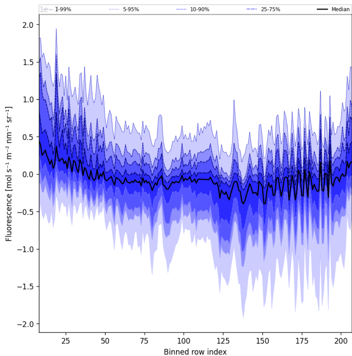
Figure 43: Along track statistics of “Fluorescence” for 2025-05-03 to 2025-05-05
