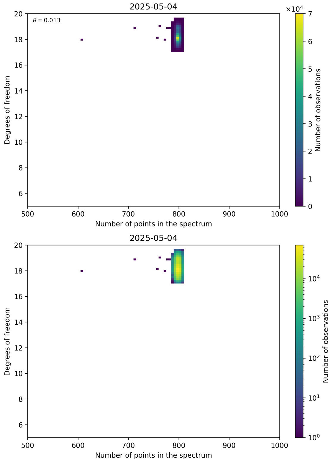
Figure 90: Scatter density plot of “Number of points in the spectrum” against “Degrees of freedom” for 2025-05-03 to 2025-05-05.
