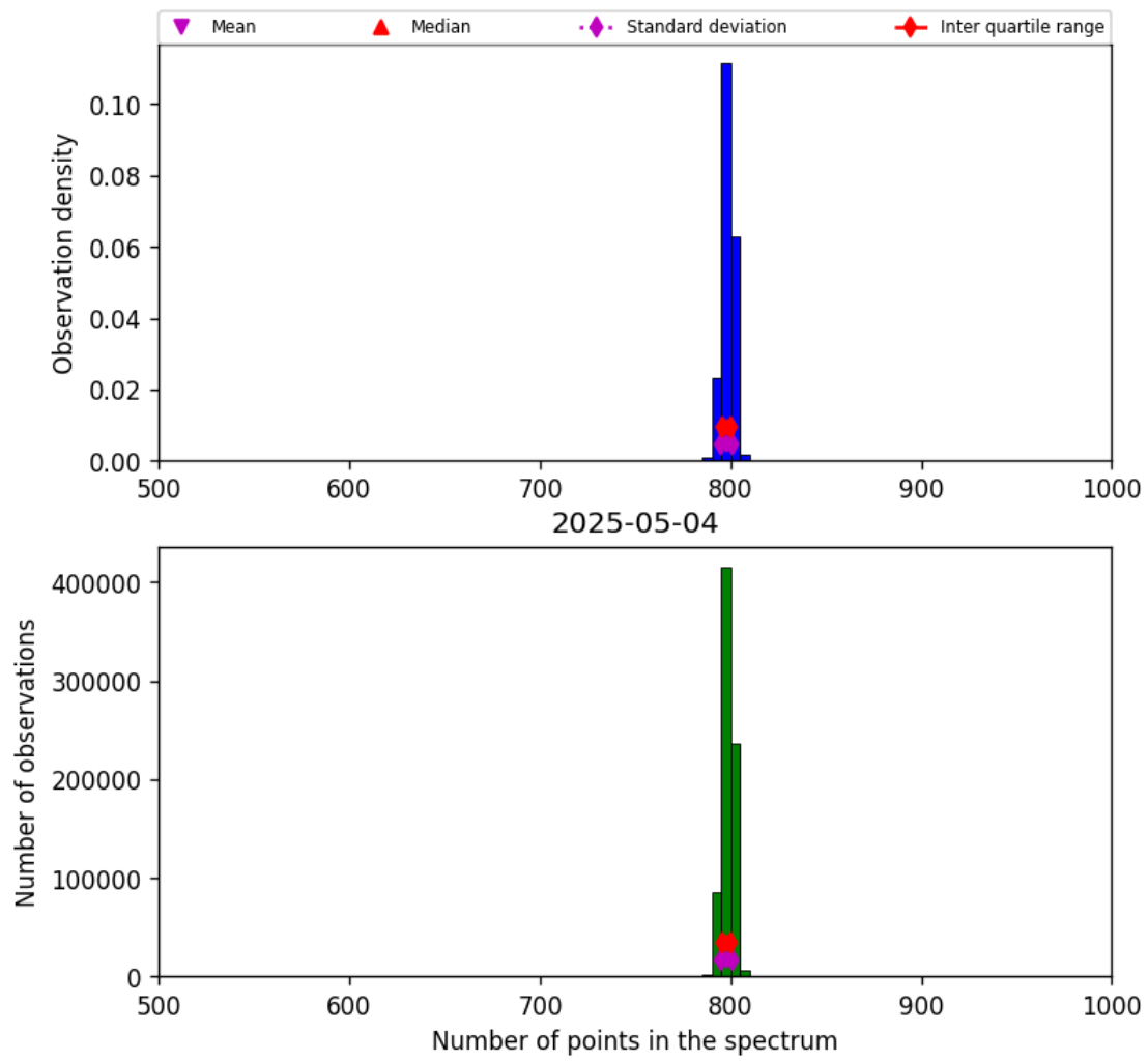
Figure 26: Histogram of “Number of points in the spectrum” for 2025-05-03 to 2025-05-05
