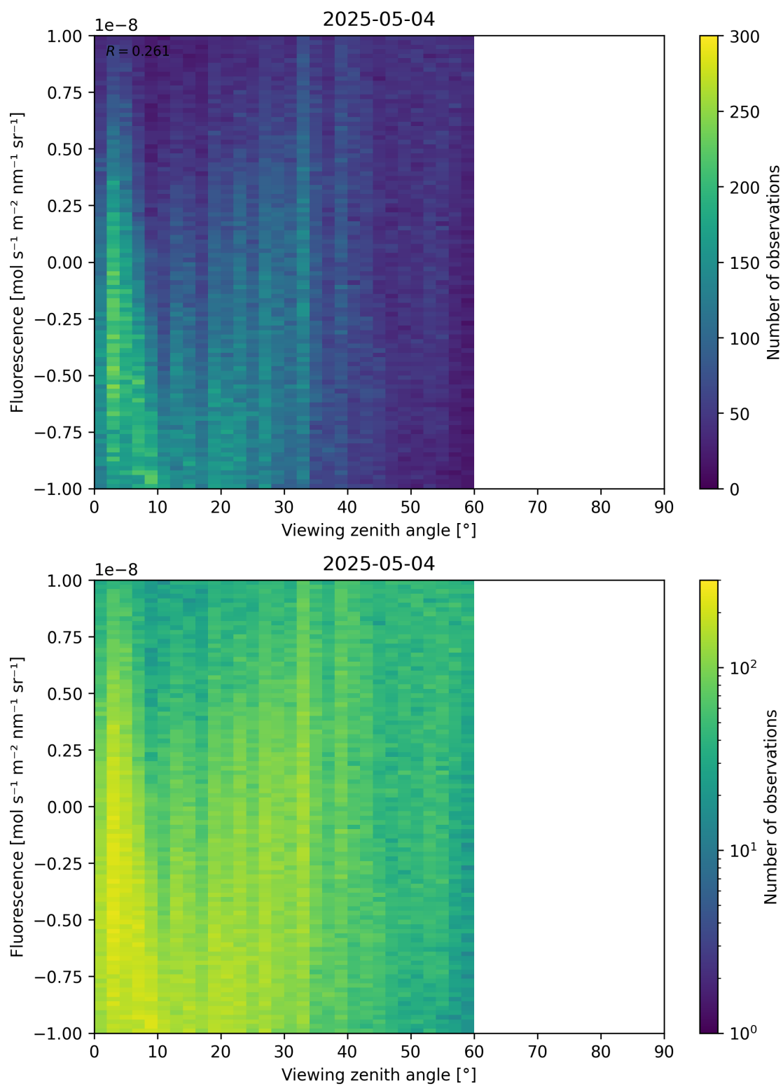
Figure 108: Scatter density plot of “Viewing zenith angle” against “Fluorescence” for 2025-05-03 to 2025-05-05.
