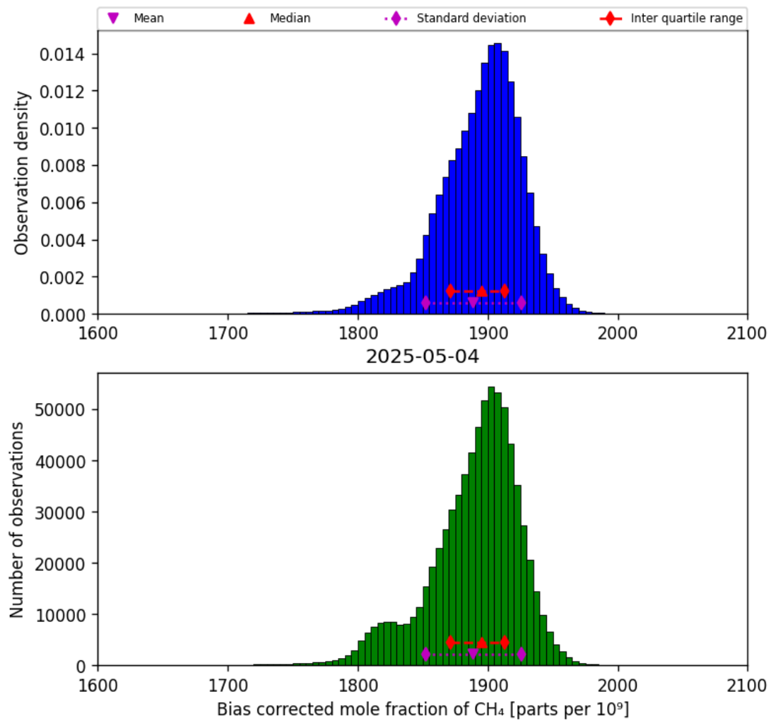
Figure 25: Histogram of “Bias corrected mole fraction of CH 4 ” for 2025-05-03 to 2025-05-05
