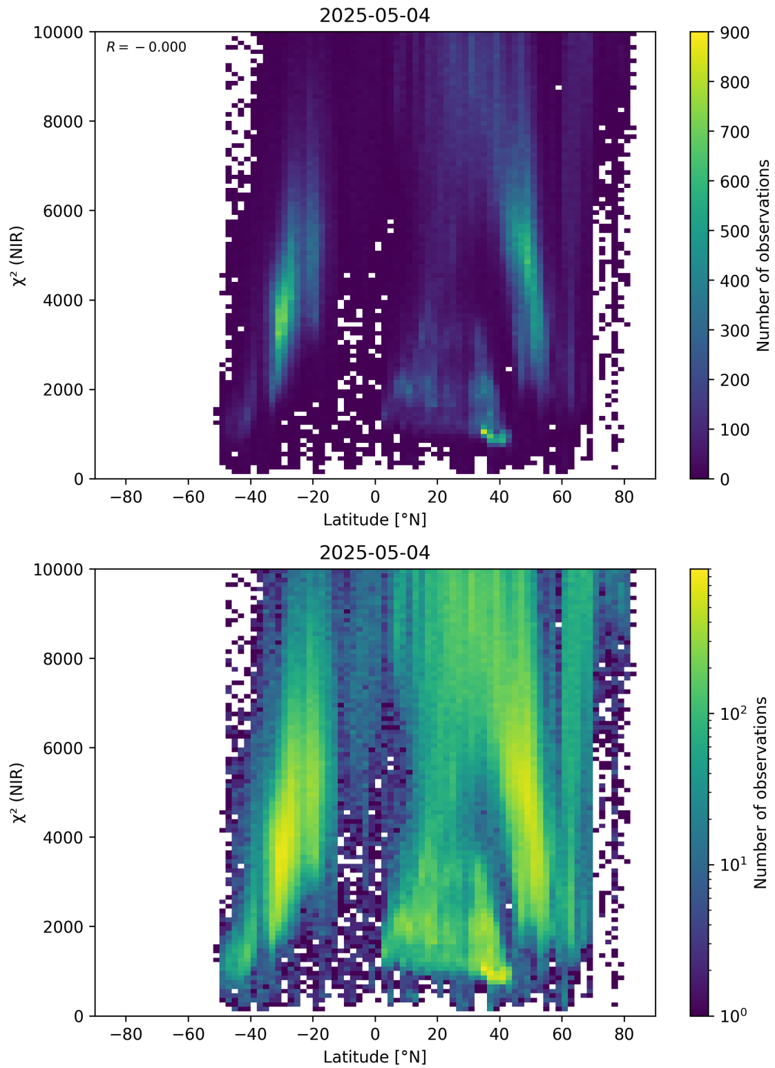
Figure 53: Scatter density plot of “Latitude” against “ \chi^2 (NIR)” for 2025-05-03 to 2025-05-05.
