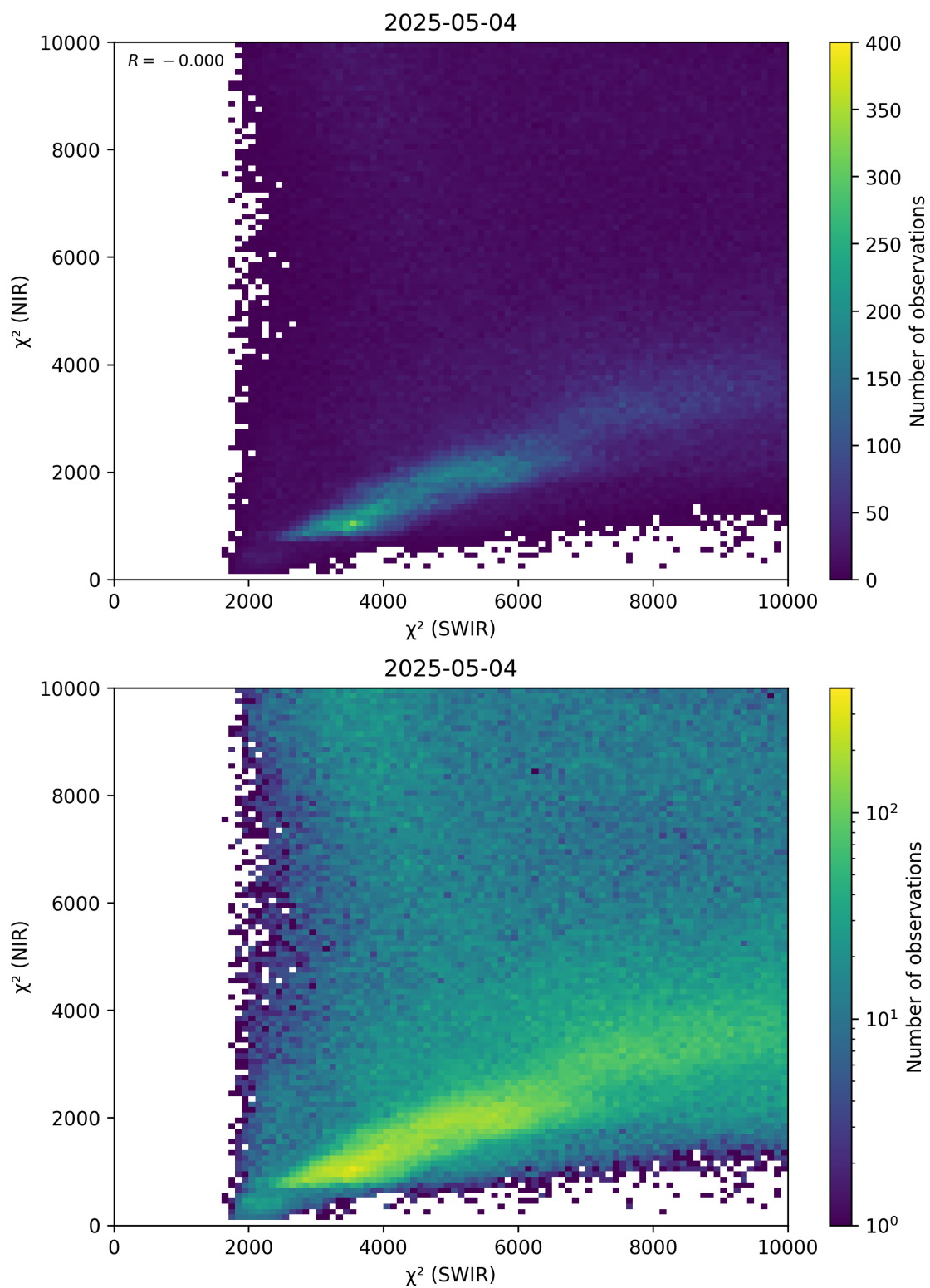
Figure 47: Scatter density plot of “ \chi^2 (SWIR)” against “ \chi^2 (NIR)” for 2025-05-03 to 2025-05-05.
