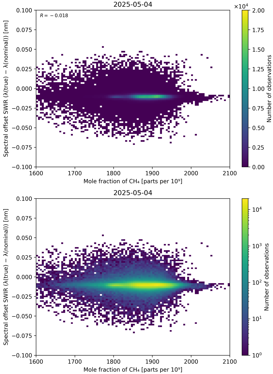
Figure 86: Scatter density plot of “Mole fraction of \text{CH}_4 ” against “Spectral offset SWIR ( \lambda_{\text{true}} - \lambda_{\text{nominal}} )” for 2025-05-03 to 2025-05-05.
