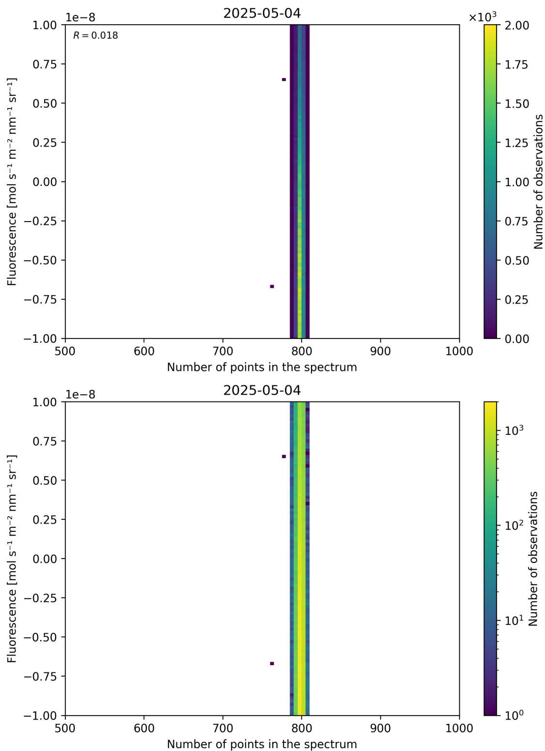
Figure 91: Scatter density plot of “Number of points in the spectrum” against “Fluorescence” for 2025-05-03 to 2025-05-05.
