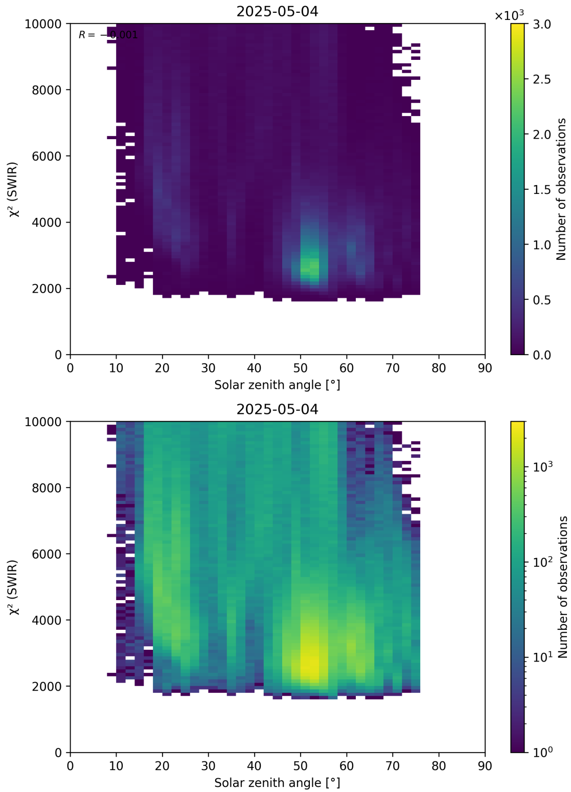
Figure 95: Scatter density plot of “Solar zenith angle” against “ \chi^2 (SWIR)” for 2025-05-03 to 2025-05-05.
