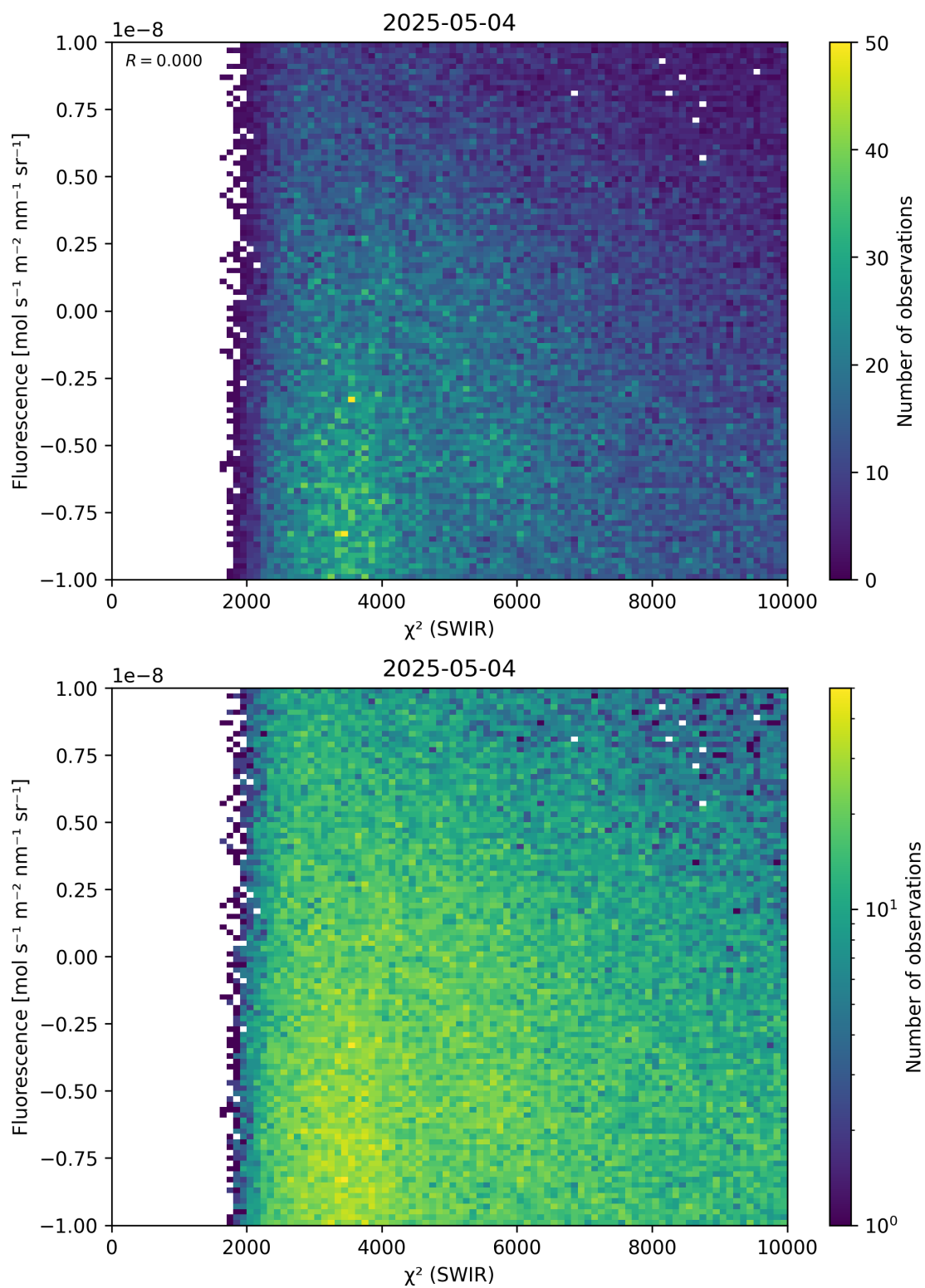
Figure 49: Scatter density plot of “ \chi^2 (SWIR)” against “Fluorescence” for 2025-05-03 to 2025-05-05.
