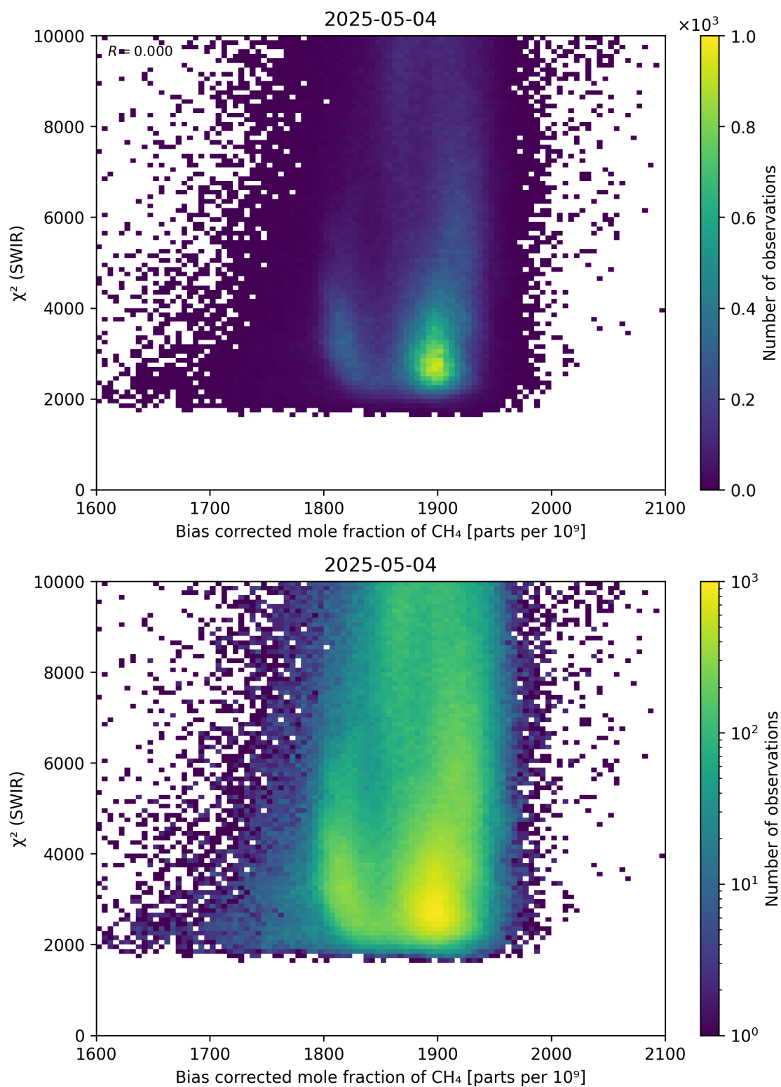
Figure 64: Scatter density plot of “Bias corrected mole fraction of \text{CH}_4 ” against “ \chi^2 (SWIR)” for 2025-05-03 to 2025-05-05.
