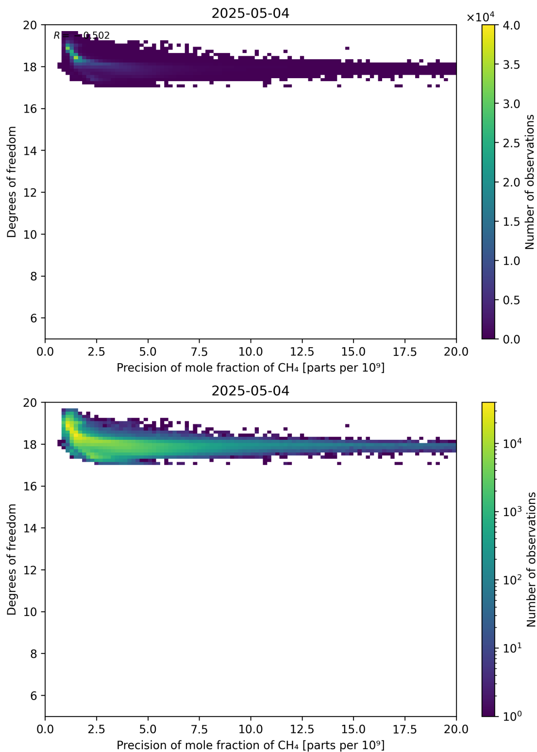
Figure 80: Scatter density plot of “Precision of mole fraction of CH 4 ” against “Degrees of freedom” for 2025-05-03 to 2025-05-05.
