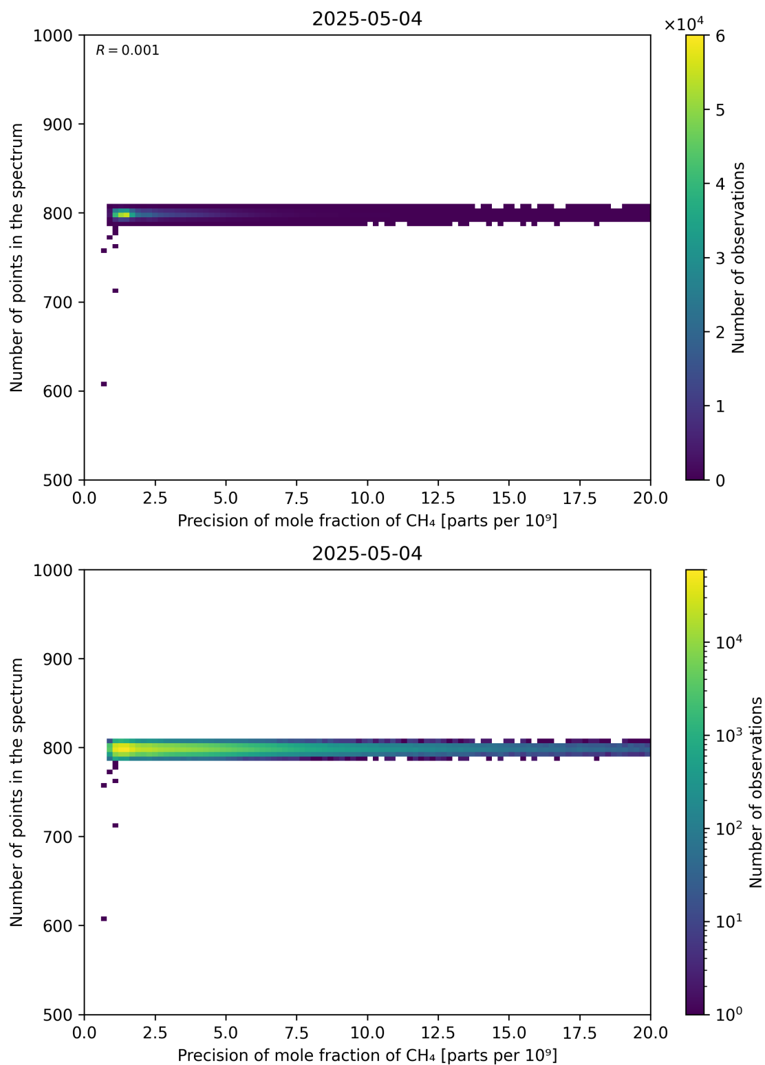
Figure 84: Scatter density plot of “Precision of mole fraction of CH 4 ” against “Number of points in the spectrum” for 2025-05-03 to 2025-05-05.
