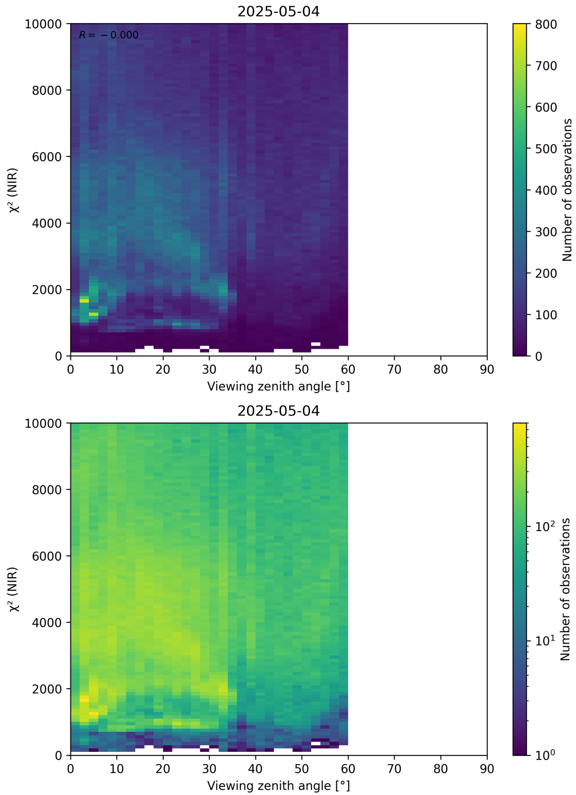
Figure 105: Scatter density plot of “Viewing zenith angle” against “ \chi^2 (NIR)” for 2025-05-03 to 2025-05-05.
