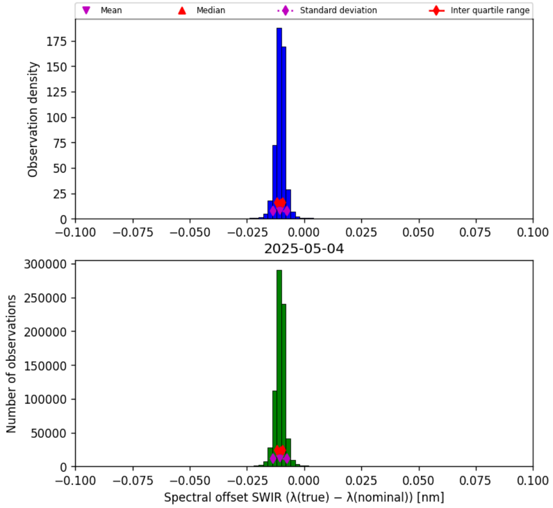
Figure 27: Histogram of “Spectral offset SWIR ( \lambda_{\text{true}} - \lambda_{\text{nominal}} )” for 2025-05-03 to 2025-05-05
