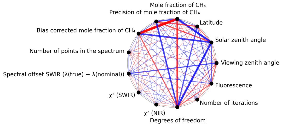
Figure 1: Map of correlation graph for 2025-05-03 to 2025-05-05.
