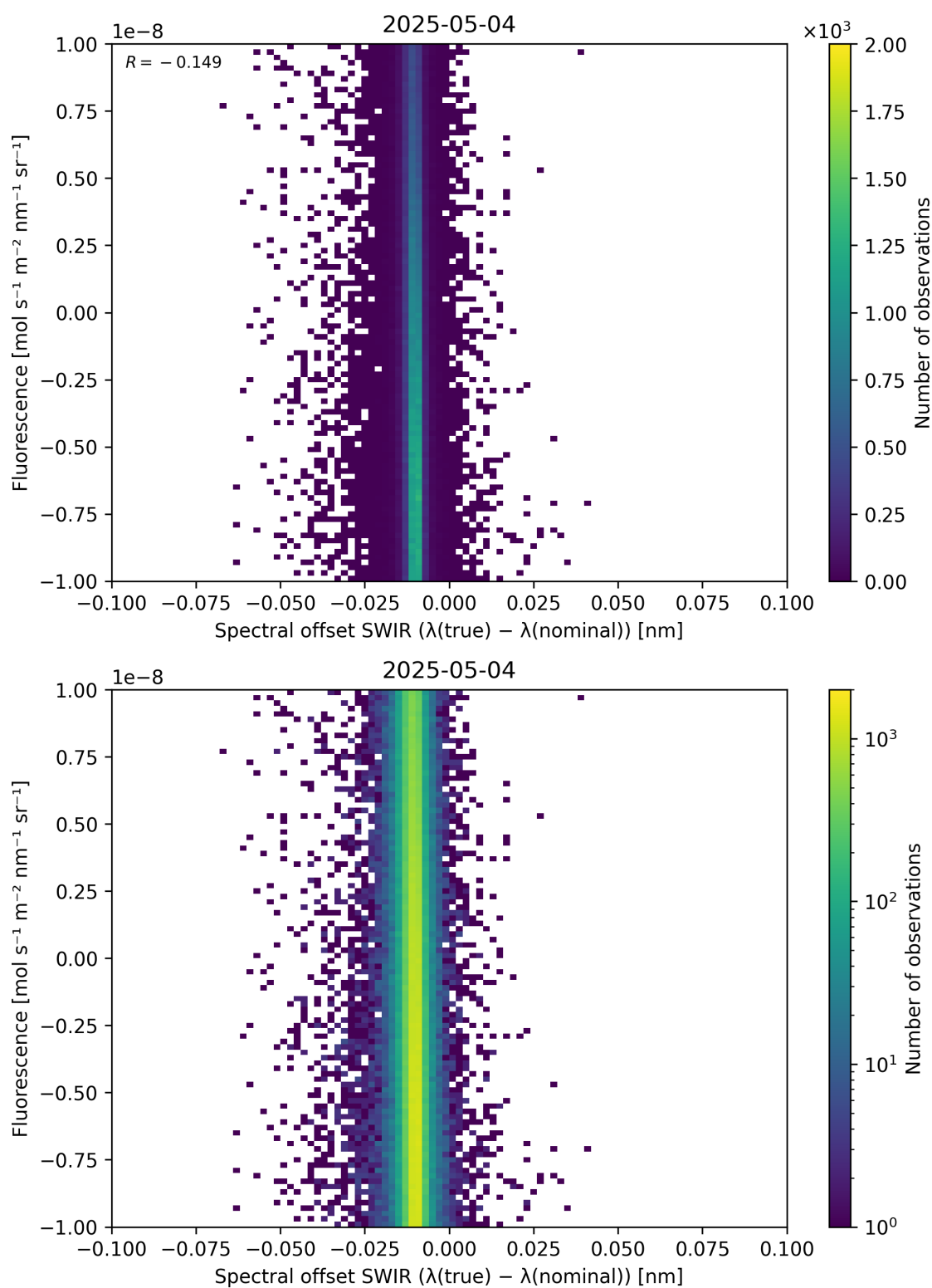
Figure 120: Scatter density plot of “Spectral offset SWIR ( \lambda_{\text{true}} - \lambda_{\text{nominal}} )” against “Fluorescence” for 2025-05-03 to 2025-05-05.
