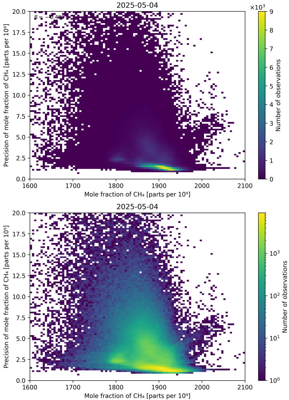
Figure 75: Scatter density plot of “Mole fraction of CH 4 ” against “Precision of mole fraction of CH 4 ” for 2025-05-03 to 2025-05-05.
