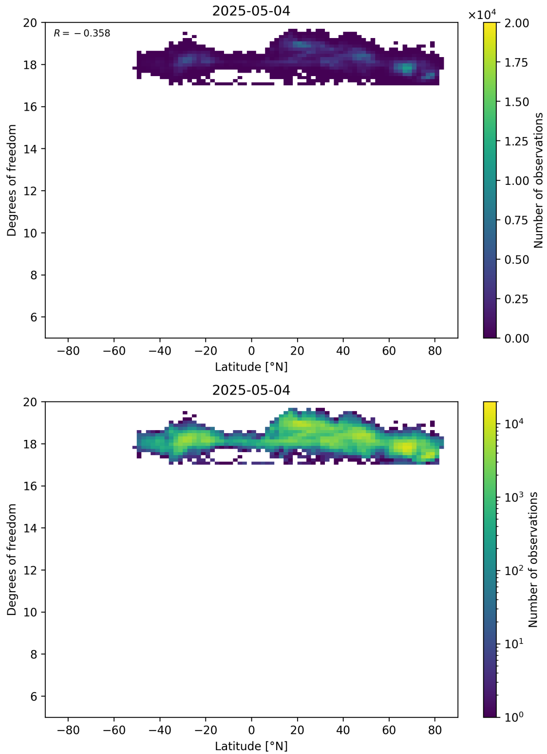
Figure 55: Scatter density plot of “Latitude” against “Degrees of freedom” for 2025-05-03 to 2025-05-05.
