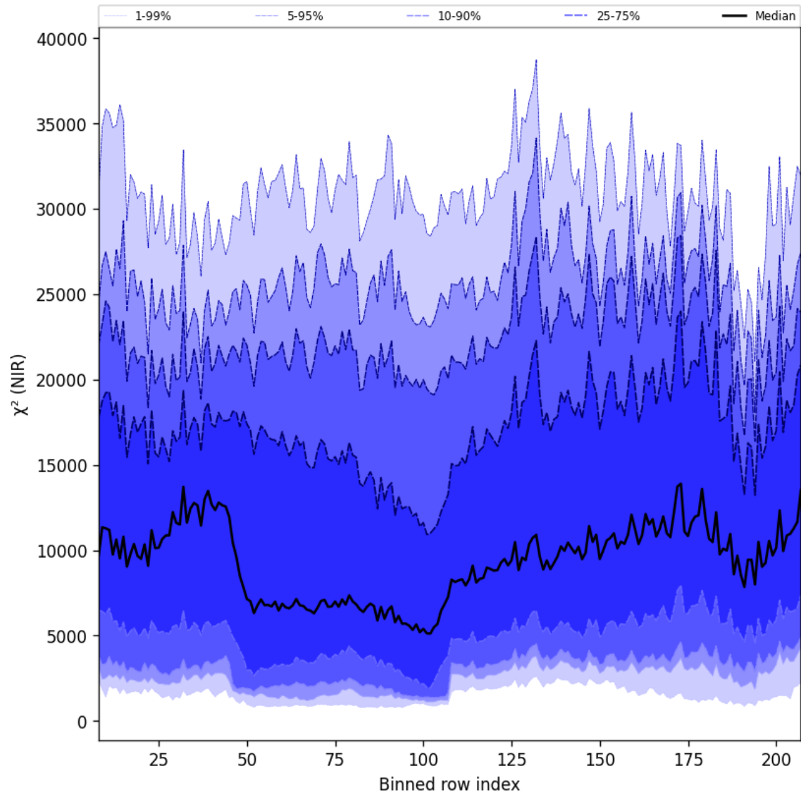
Figure 40: Along track statistics of “ \chi^2 (NIR)” for 2025-05-03 to 2025-05-05
