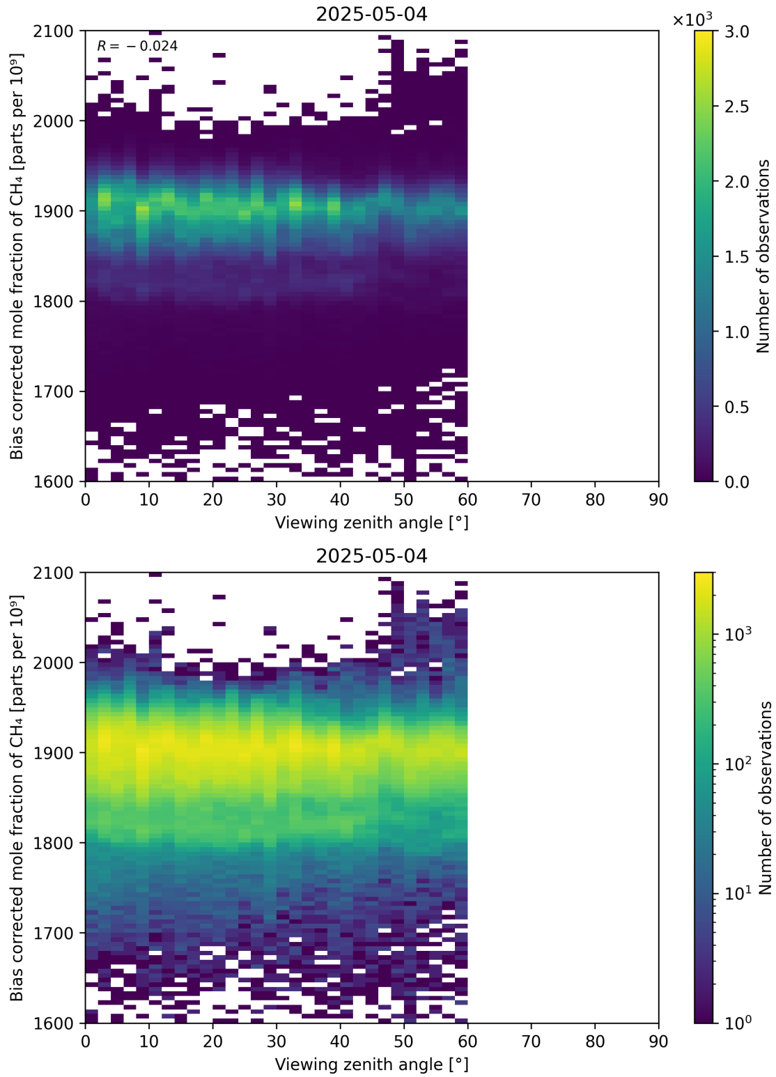
Figure 111: Scatter density plot of “Viewing zenith angle” against “Bias corrected mole fraction of CH 4 ” for 2025-05-03 to 2025-05-05.
