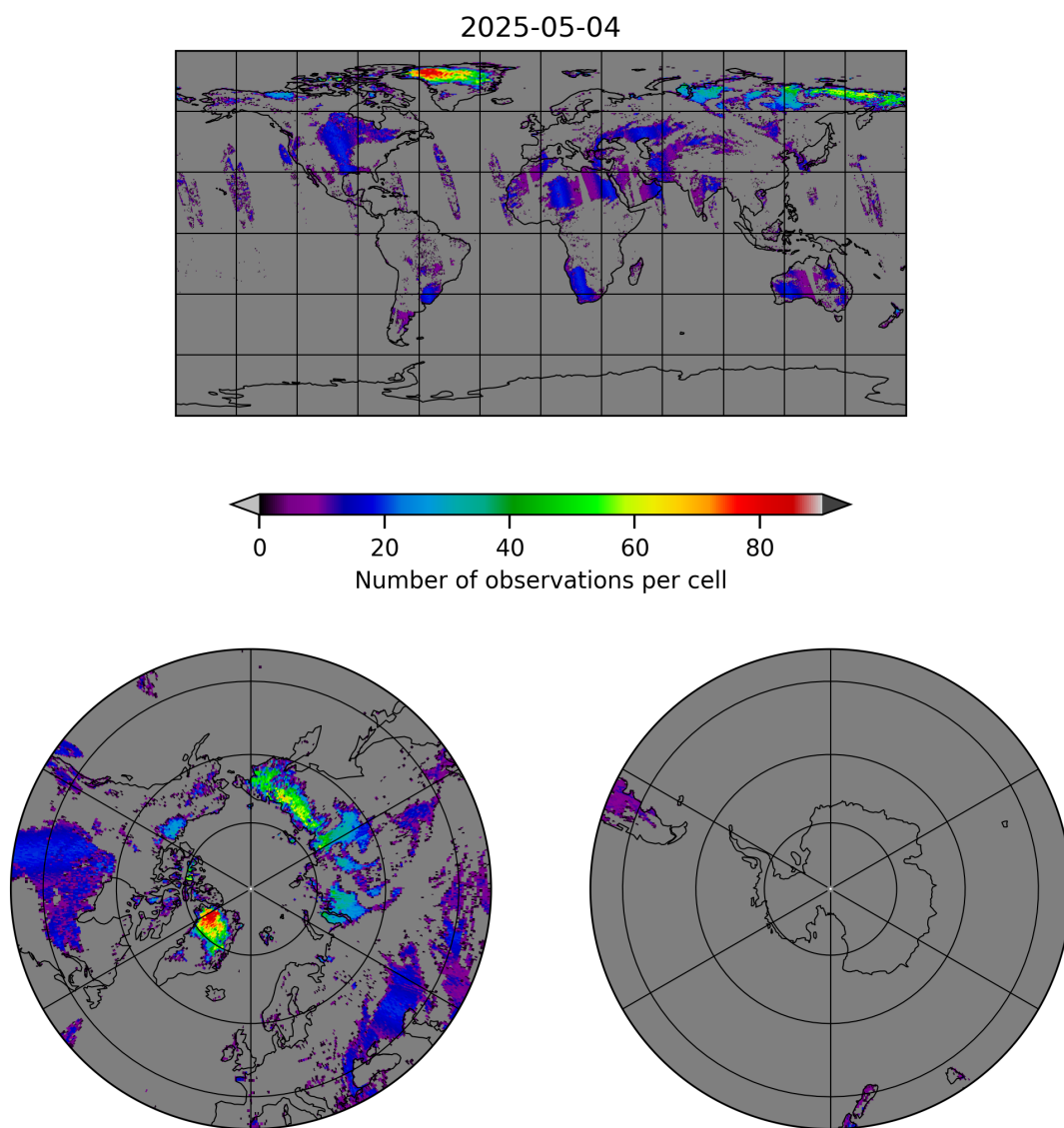
Figure 10: Map of the number of observations for 2025-05-03 to 2025-05-05
