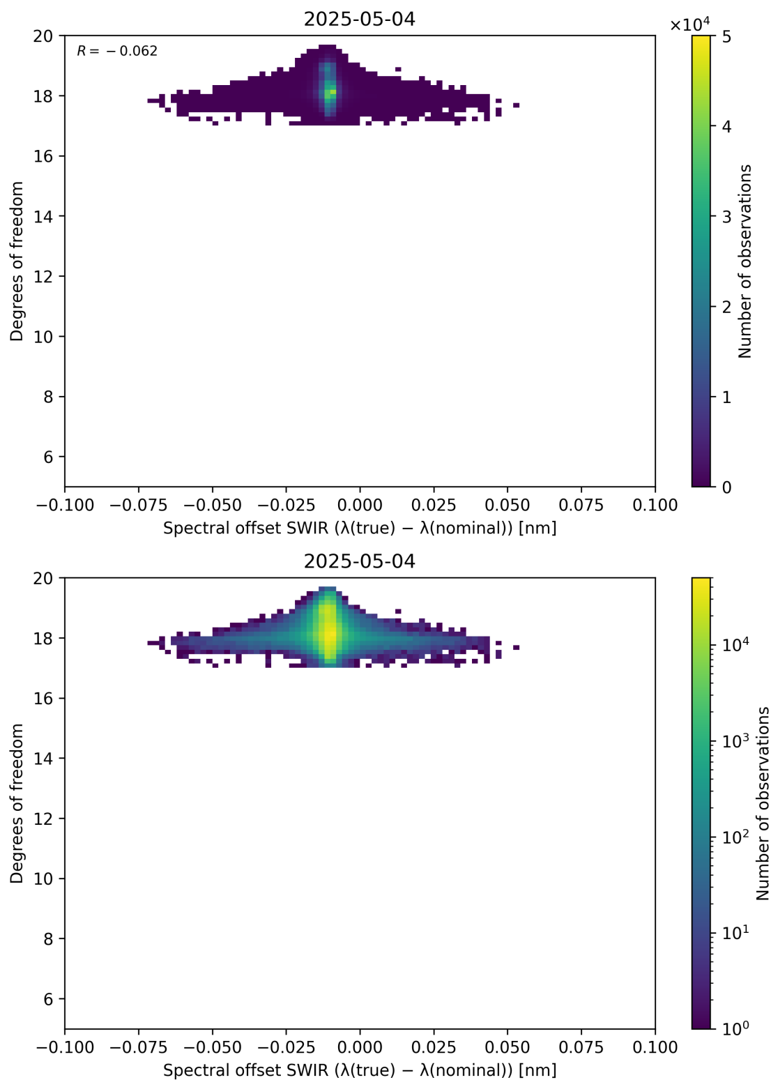
Figure 119: Scatter density plot of “Spectral offset SWIR ( \lambda_{\text{true}} - \lambda_{\text{nominal}} )” against “Degrees of freedom” for 2025-05-03 to 2025-05-05.
