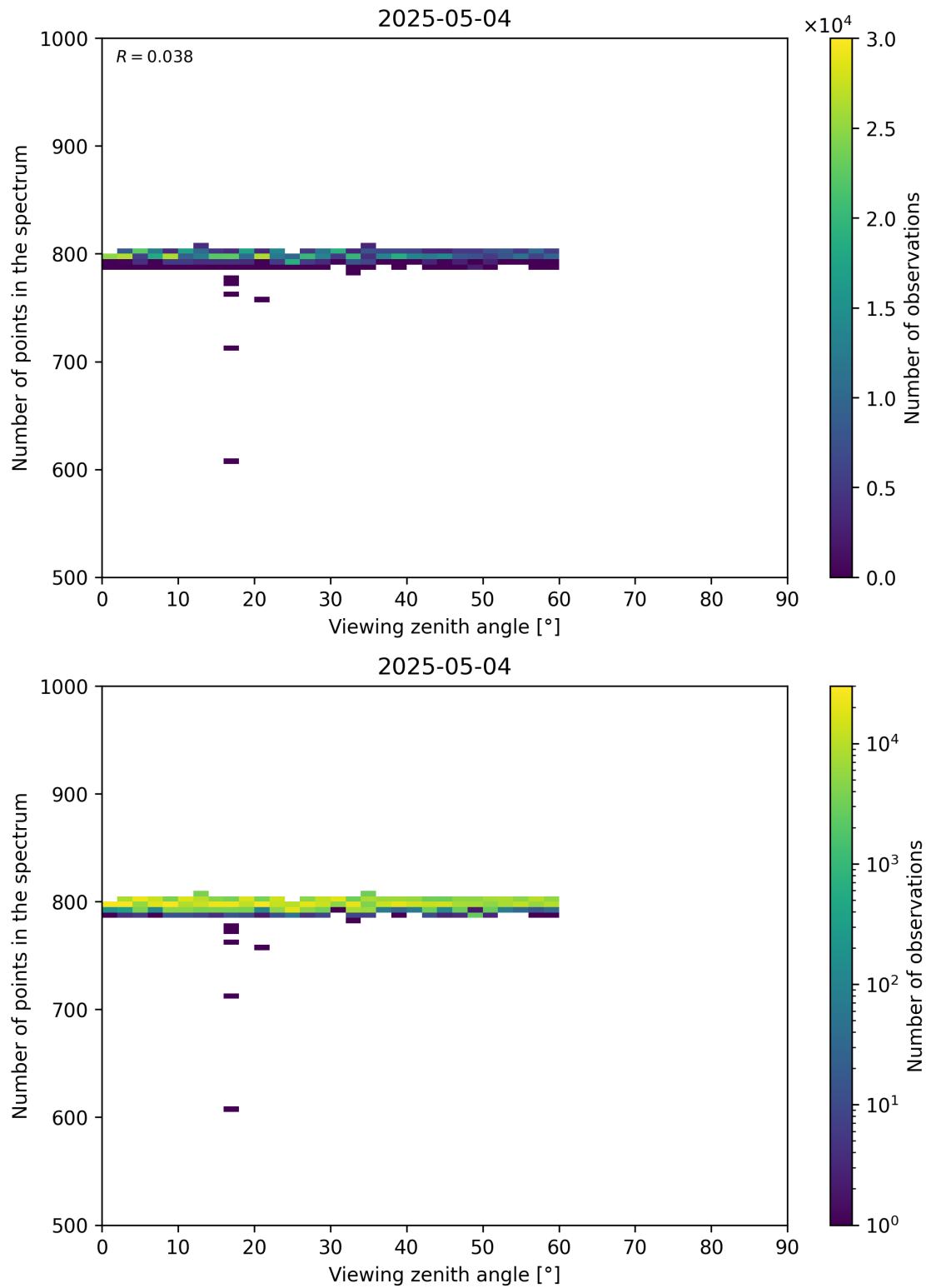
Figure 114: Scatter density plot of “Viewing zenith angle” against “Number of points in the spectrum” for 2025-05-03 to 2025-05-05.
