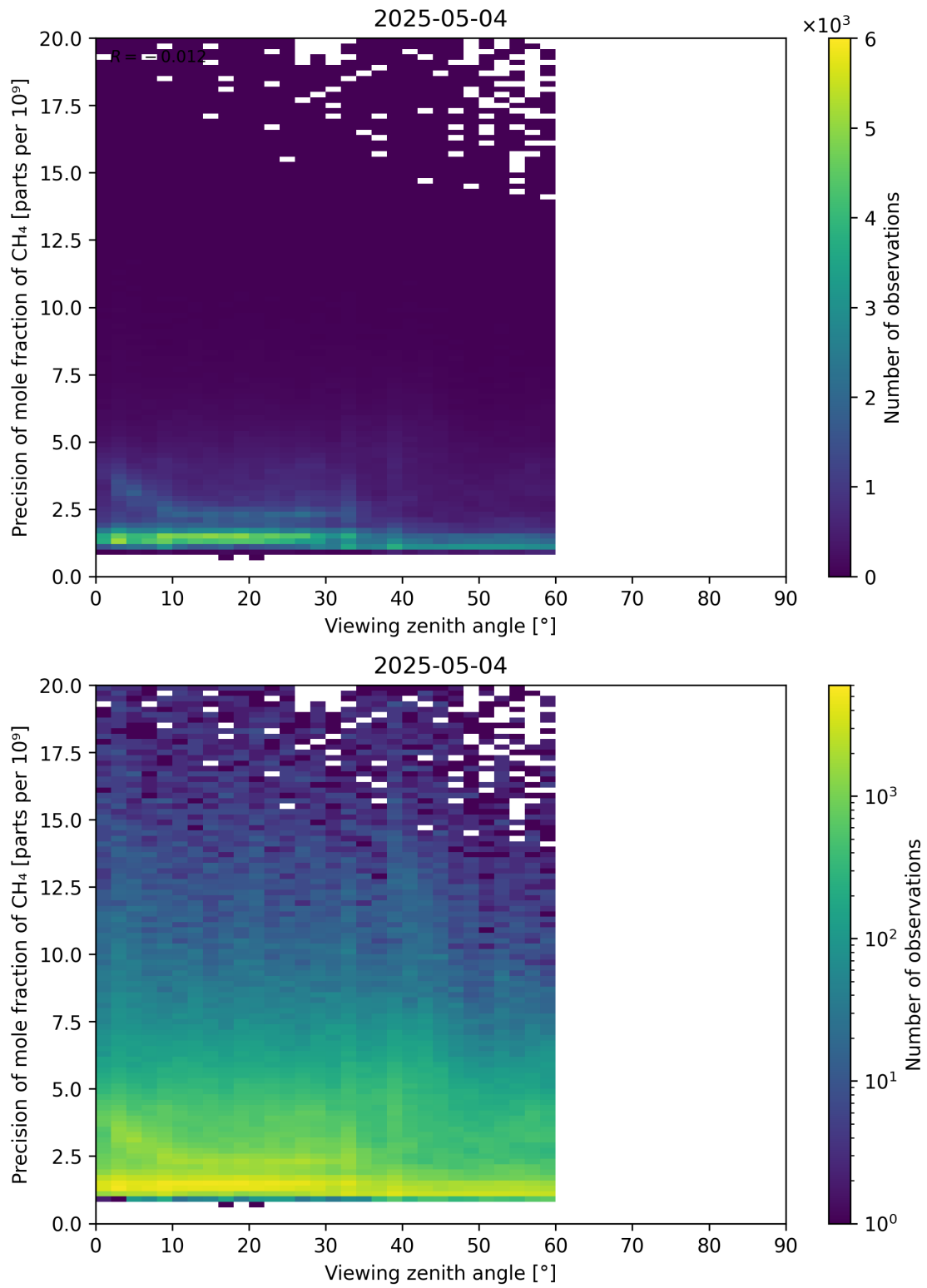
Figure 112: Scatter density plot of “Viewing zenith angle” against “Precision of mole fraction of CH 4 ” for 2025-05-03 to 2025-05-05.
