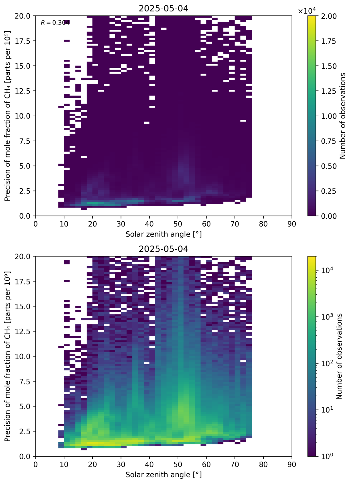
Figure 101: Scatter density plot of “Solar zenith angle” against “Precision of mole fraction of CH 4 ” for 2025-05-03 to 2025-05-05.
