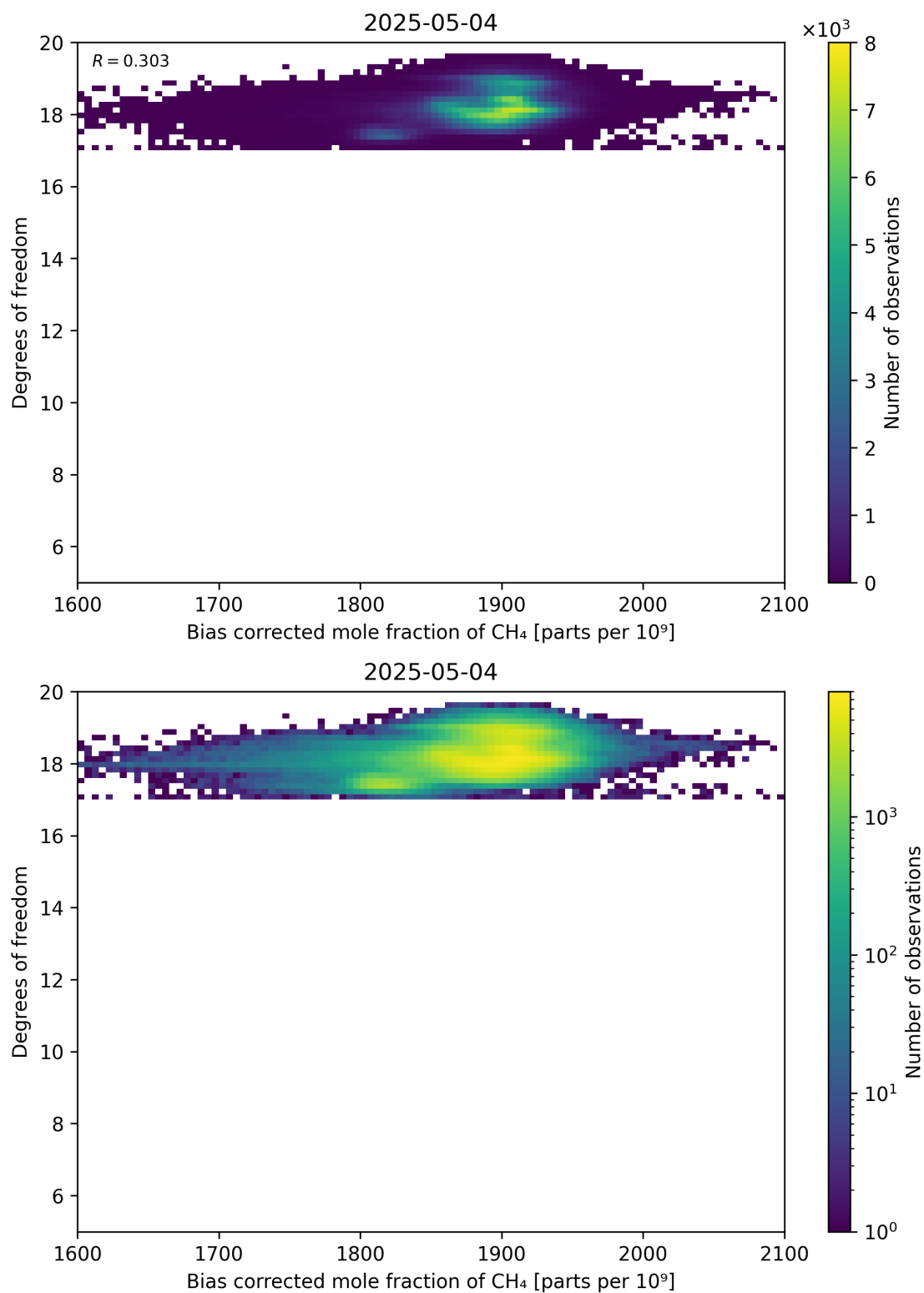
Figure 65: Scatter density plot of “Bias corrected mole fraction of CH 4 ” against “Degrees of freedom” for 2025-05-03 to 2025-05-05.
