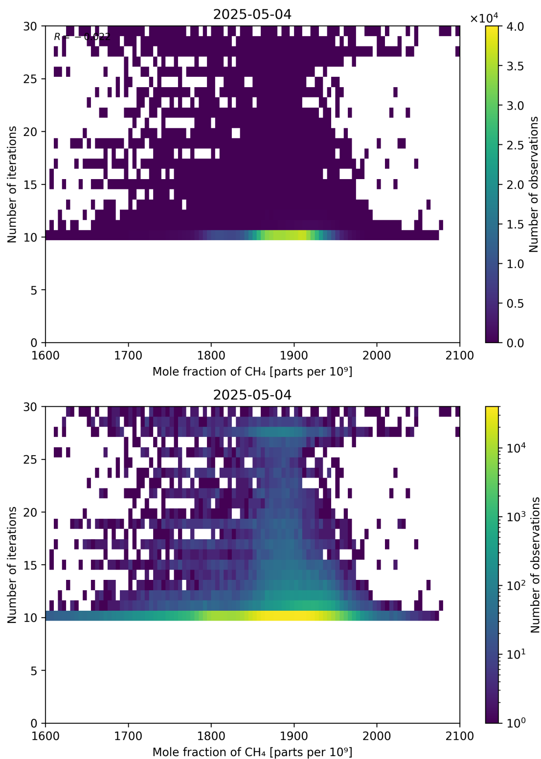
Figure 76: Scatter density plot of “Mole fraction of CH 4 ” against “Number of iterations” for 2025-05-03 to 2025-05-05.
