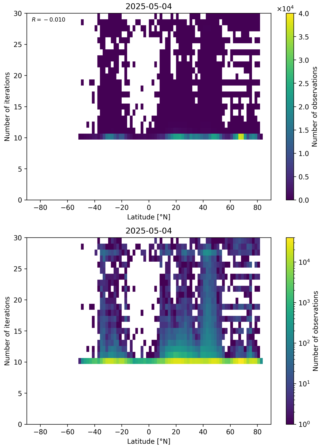
Figure 60: Scatter density plot of “Latitude” against “Number of iterations” for 2025-05-03 to 2025-05-05.
