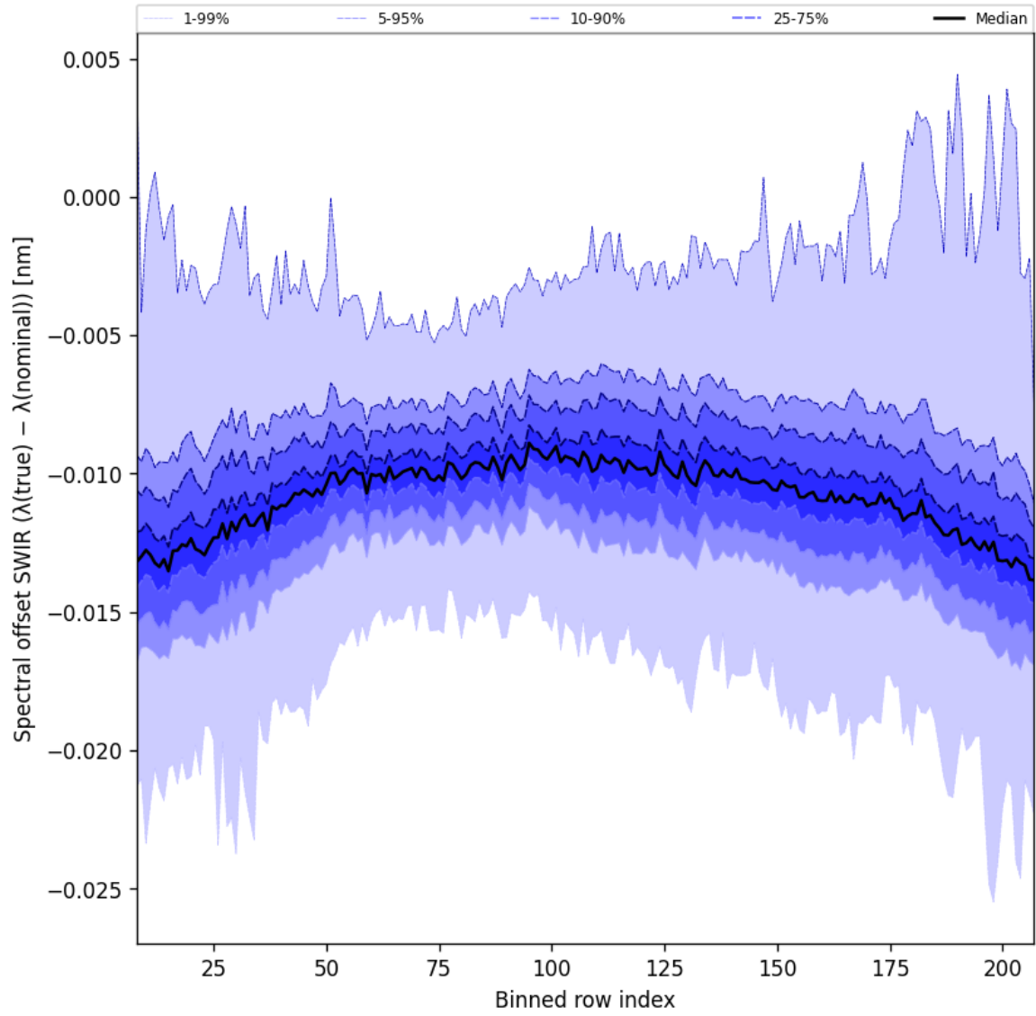
Figure 38: Along track statistics of “Spectral offset SWIR ( \lambda_{\text{true}} - \lambda_{\text{nominal}} )” for 2025-05-03 to 2025-05-05
