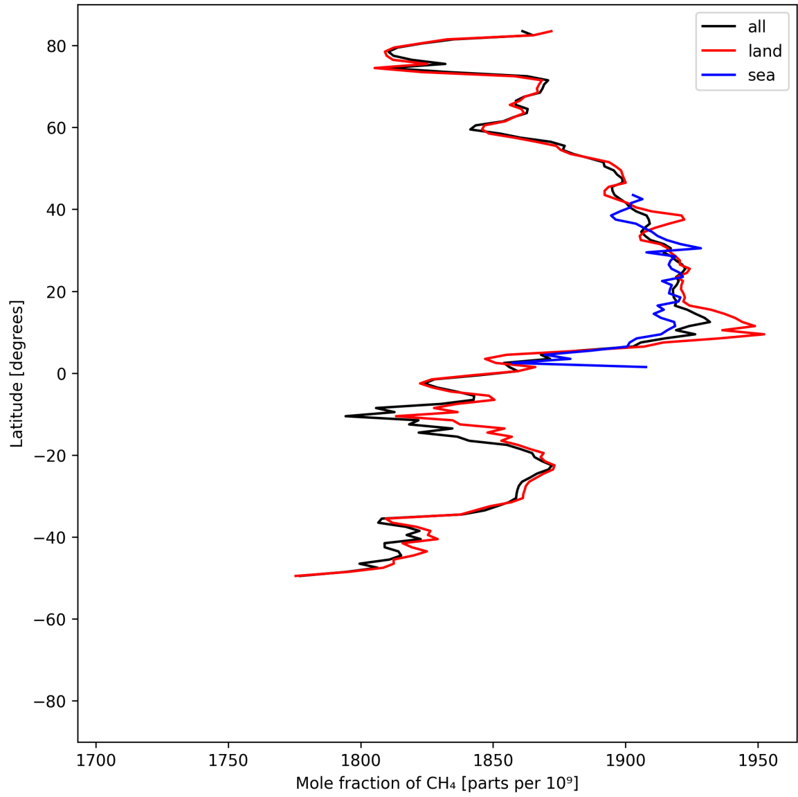
Figure 12: Zonal average of “Mole fraction of \text{CH}_4 ” for 2025-05-03 to 2025-05-05.
