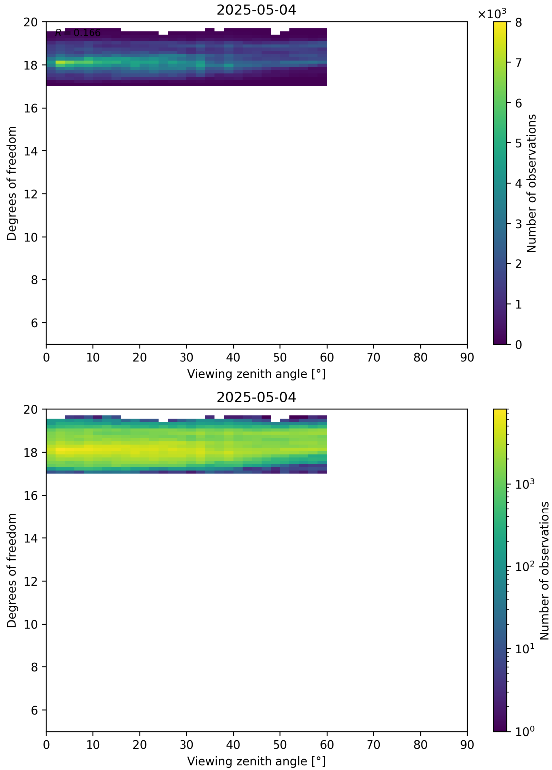
Figure 107: Scatter density plot of “Viewing zenith angle” against “Degrees of freedom” for 2025-05-03 to 2025-05-05.
