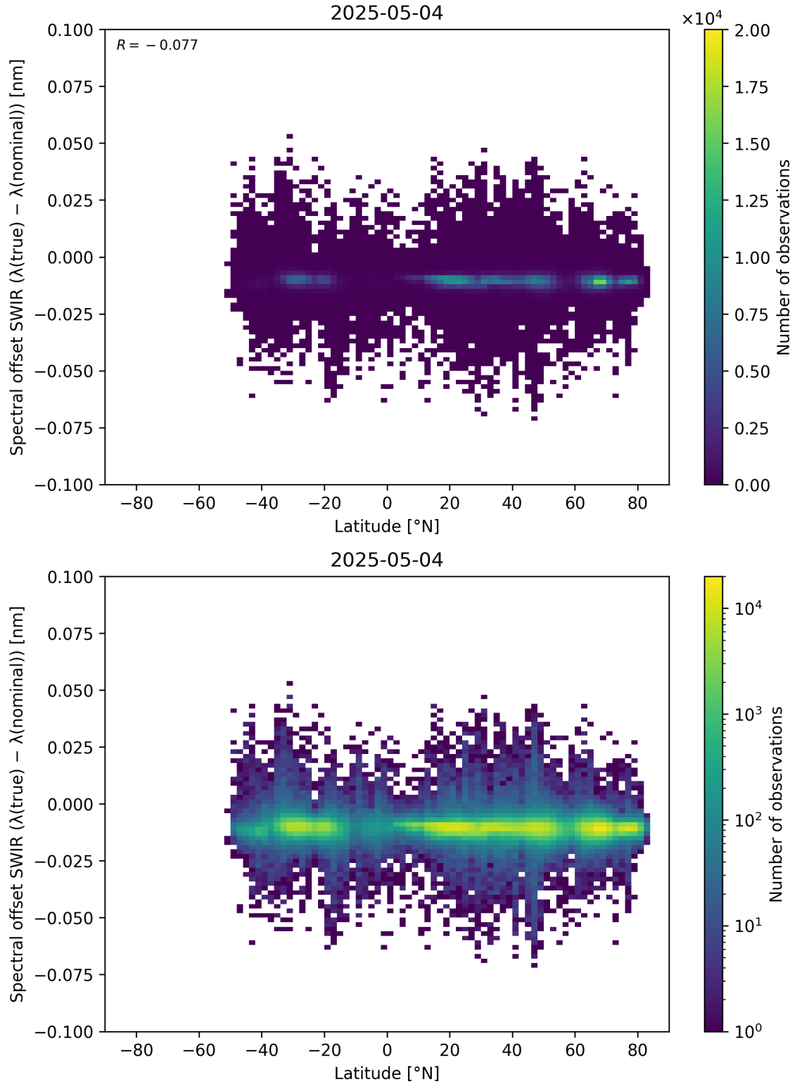
Figure 62: Scatter density plot of “Latitude” against “Spectral offset SWIR ( \lambda_{\text{true}} - \lambda_{\text{nominal}} )” for 2025-05-03 to 2025-05-05.
