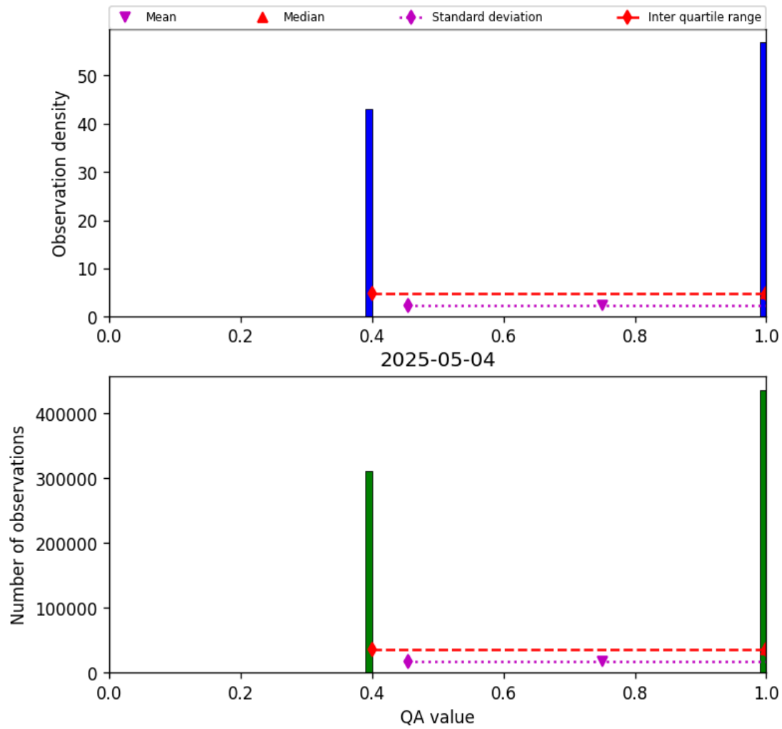
Figure 22: Histogram of “QA value” for 2025-05-03 to 2025-05-05
