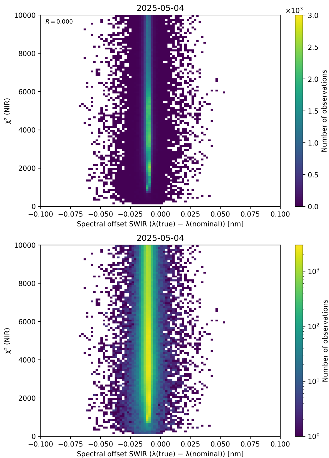
Figure 117: Scatter density plot of “Spectral offset SWIR ( \lambda_{\text{true}} - \lambda_{\text{nominal}} )” against “ \chi^2 (NIR)” for 2025-05-03 to 2025-05-05.
