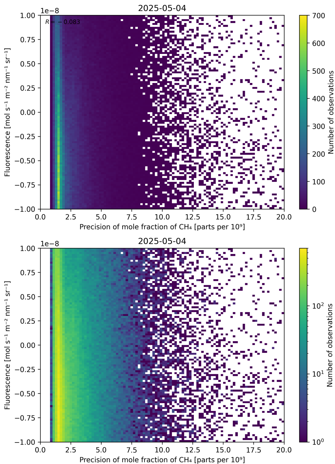
Figure 81: Scatter density plot of “Precision of mole fraction of \text{CH}_4 ” against “Fluorescence” for 2025-05-03 to 2025-05-05.
