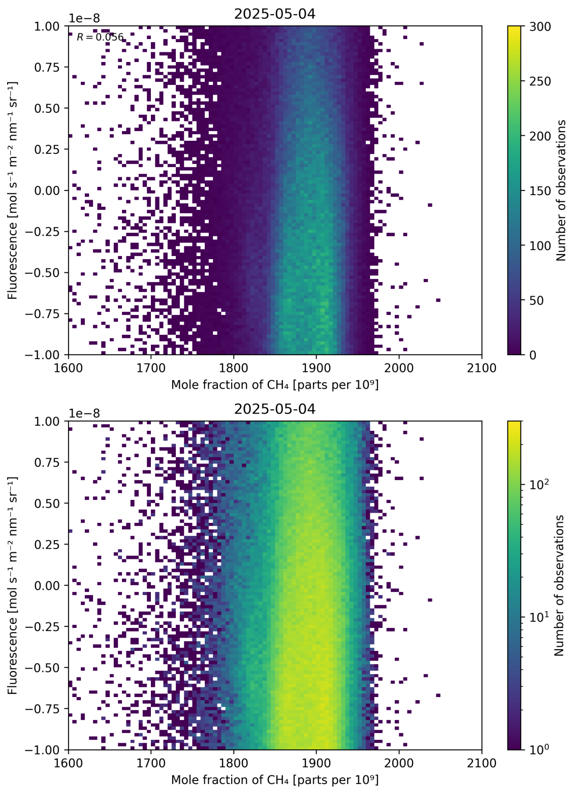
Figure 73: Scatter density plot of “Mole fraction of \text{CH}_4 ” against “Fluorescence” for 2025-05-03 to 2025-05-05.
