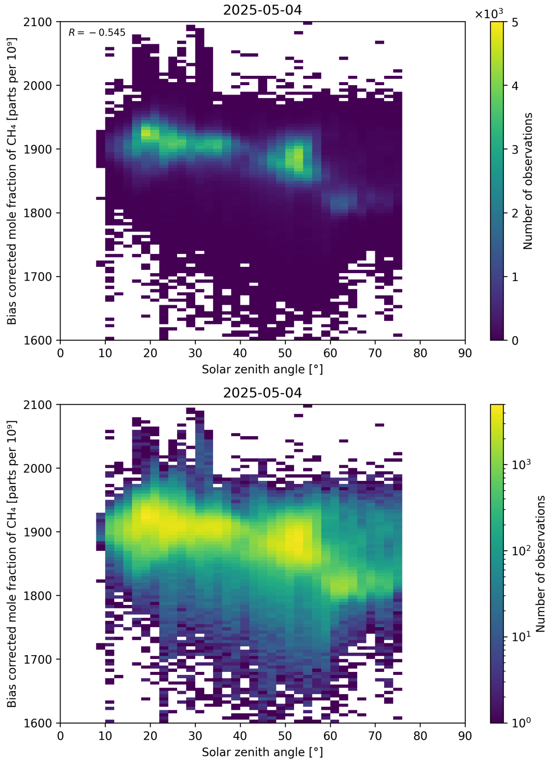
Figure 100: Scatter density plot of “Solar zenith angle” against “Bias corrected mole fraction of CH 4 ” for 2025-05-03 to 2025-05-05.
