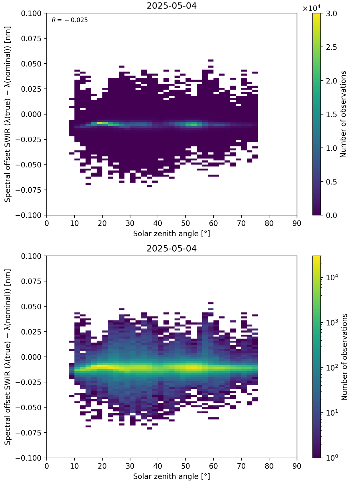
Figure 104: Scatter density plot of “Solar zenith angle” against “Spectral offset SWIR ( \lambda_{\text{true}} - \lambda_{\text{nominal}} )” for 2025-05-03 to 2025-05-05.
