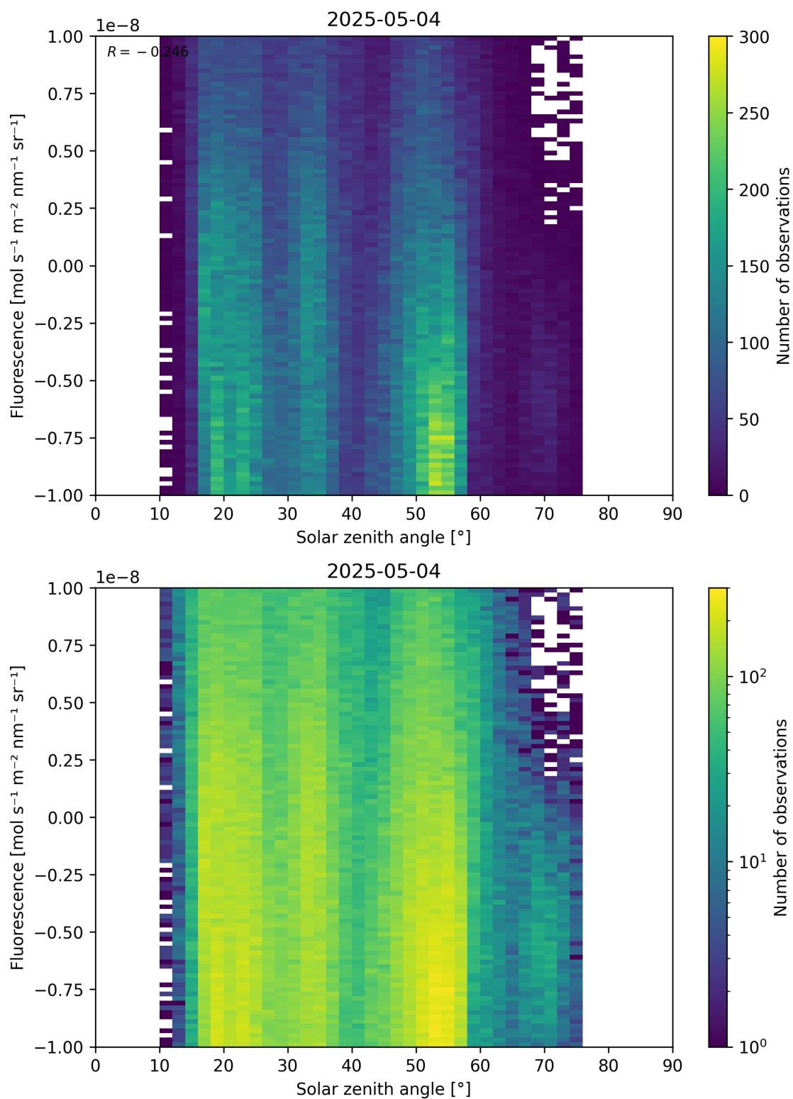
Figure 97: Scatter density plot of “Solar zenith angle” against “Fluorescence” for 2025-05-03 to 2025-05-05.
