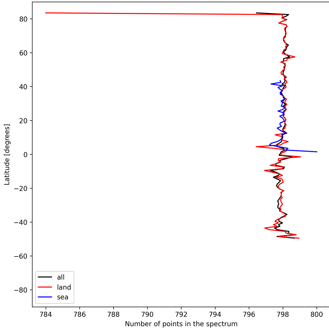
Figure 15: Zonal average of “Number of points in the spectrum” for 2025-05-03 to 2025-05-05.
