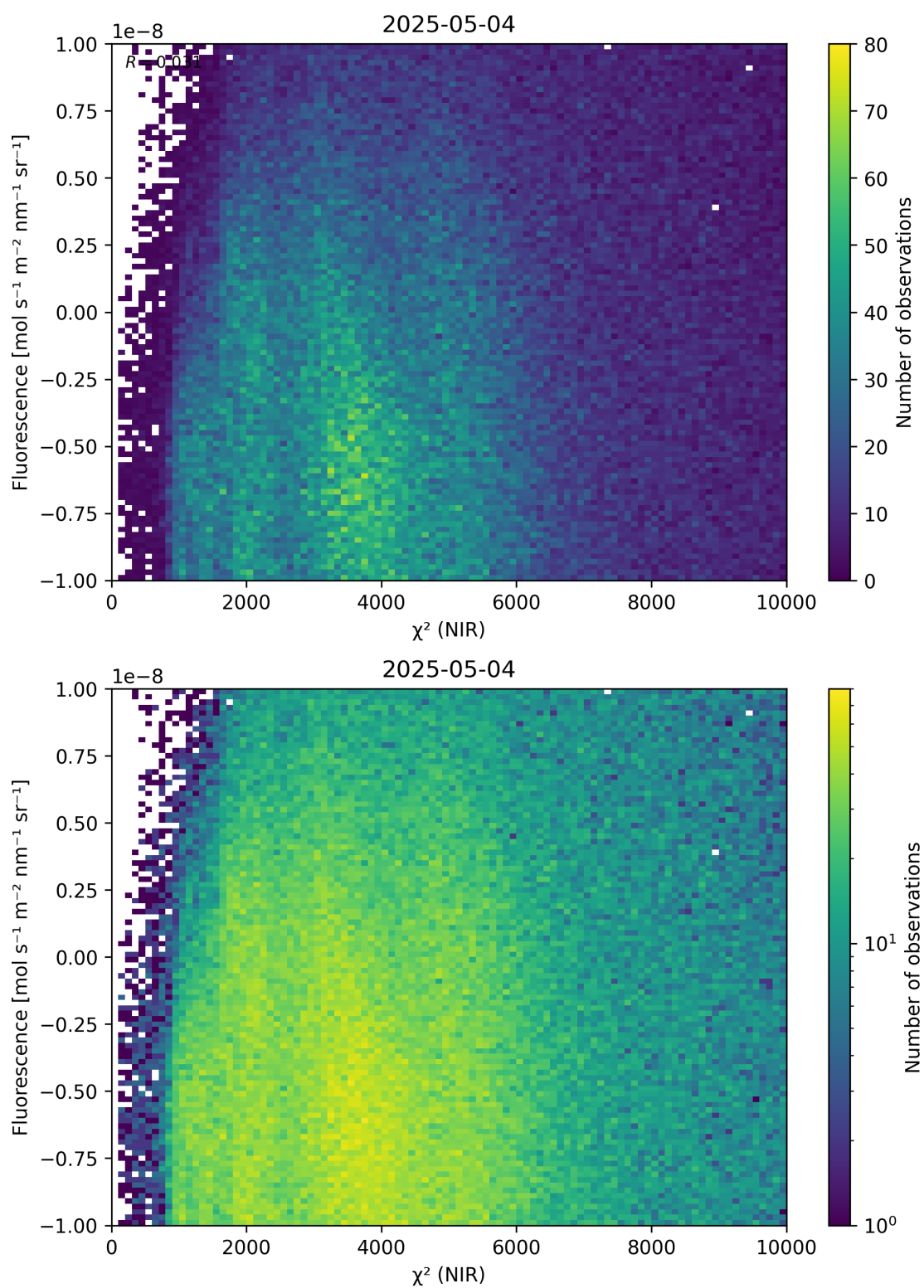
Figure 45: Scatter density plot of “ \chi^2 (NIR)” against “Fluorescence” for 2025-05-03 to 2025-05-05.
