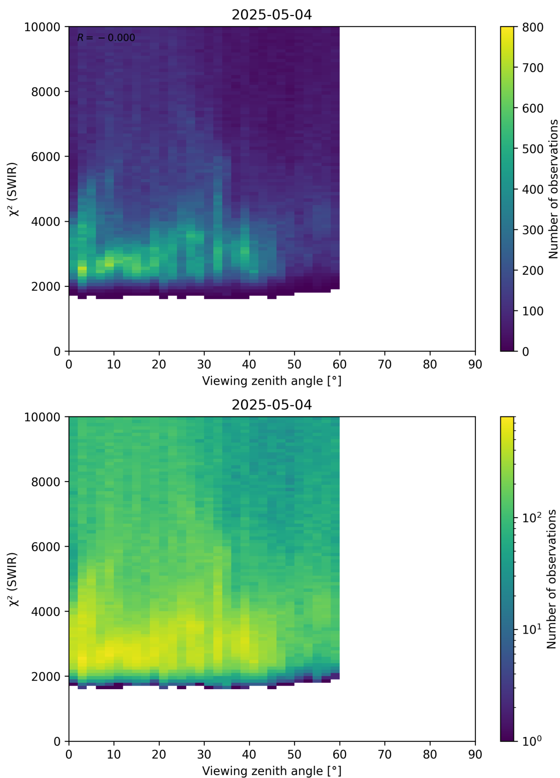
Figure 106: Scatter density plot of “Viewing zenith angle” against “ \chi^2 (SWIR)” for 2025-05-03 to 2025-05-05.
