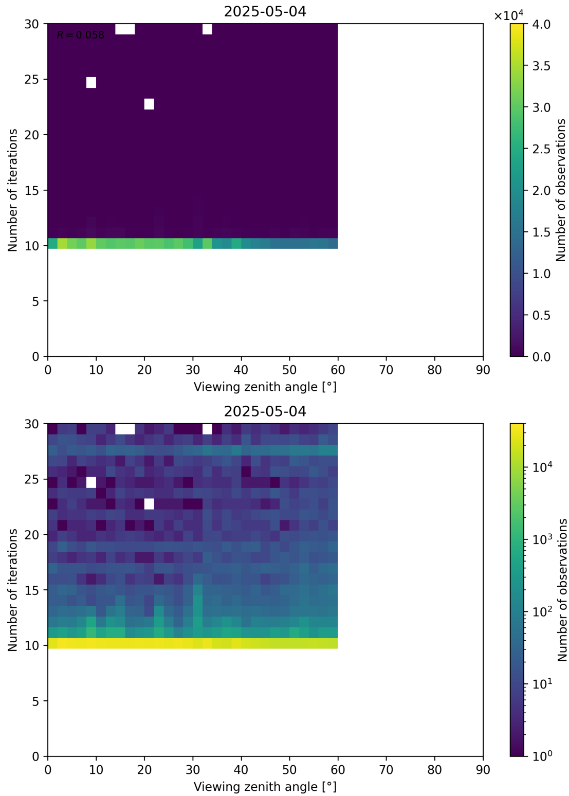
Figure 113: Scatter density plot of “Viewing zenith angle” against “Number of iterations” for 2025-05-03 to 2025-05-05.
