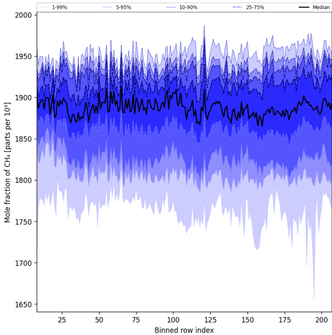
Figure 34: Along track statistics of “Mole fraction of CH 4 ” for 2025-05-03 to 2025-05-05
