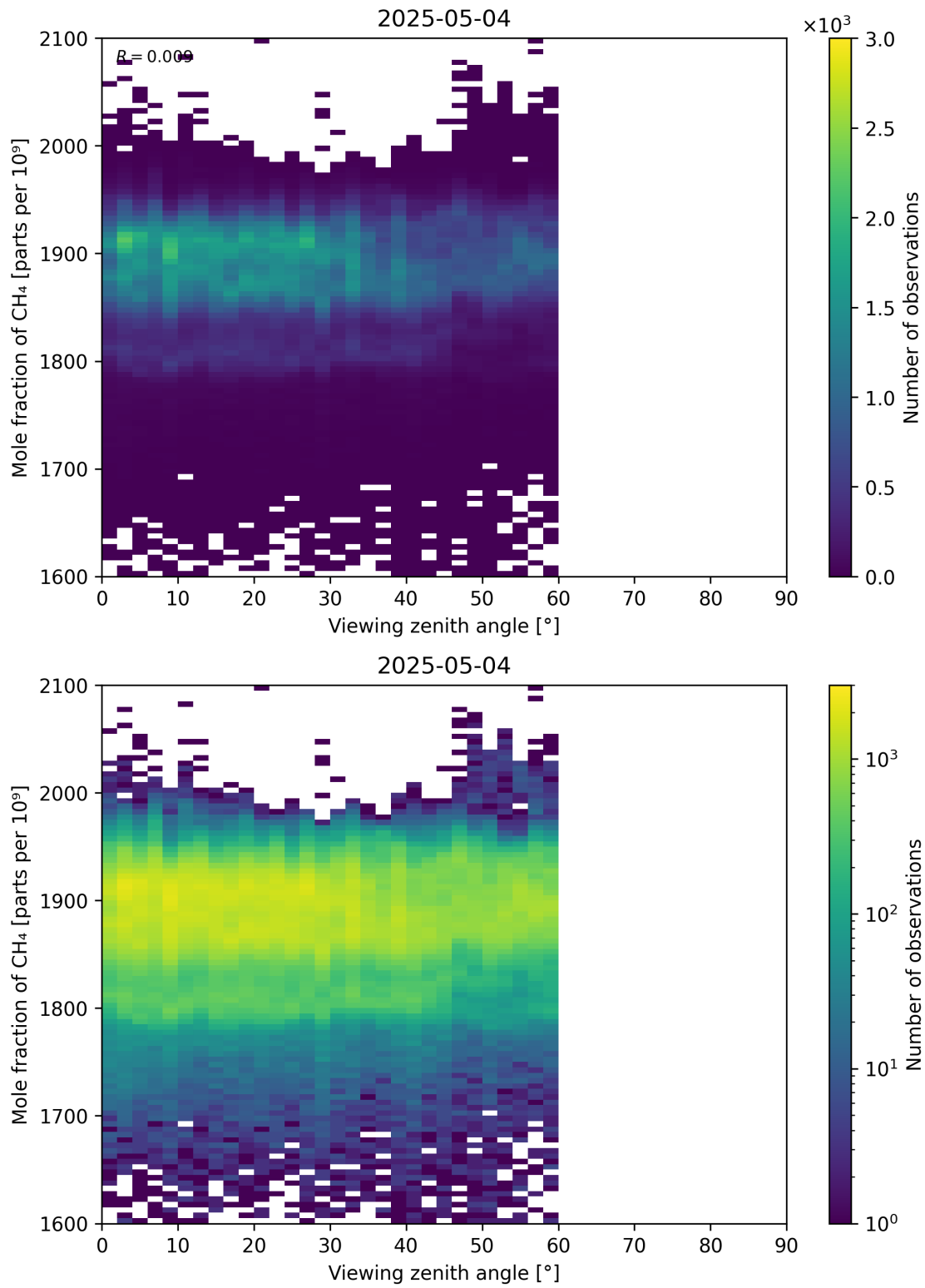
Figure 110: Scatter density plot of “Viewing zenith angle” against “Mole fraction of CH 4 ” for 2025-05-03 to 2025-05-05.
