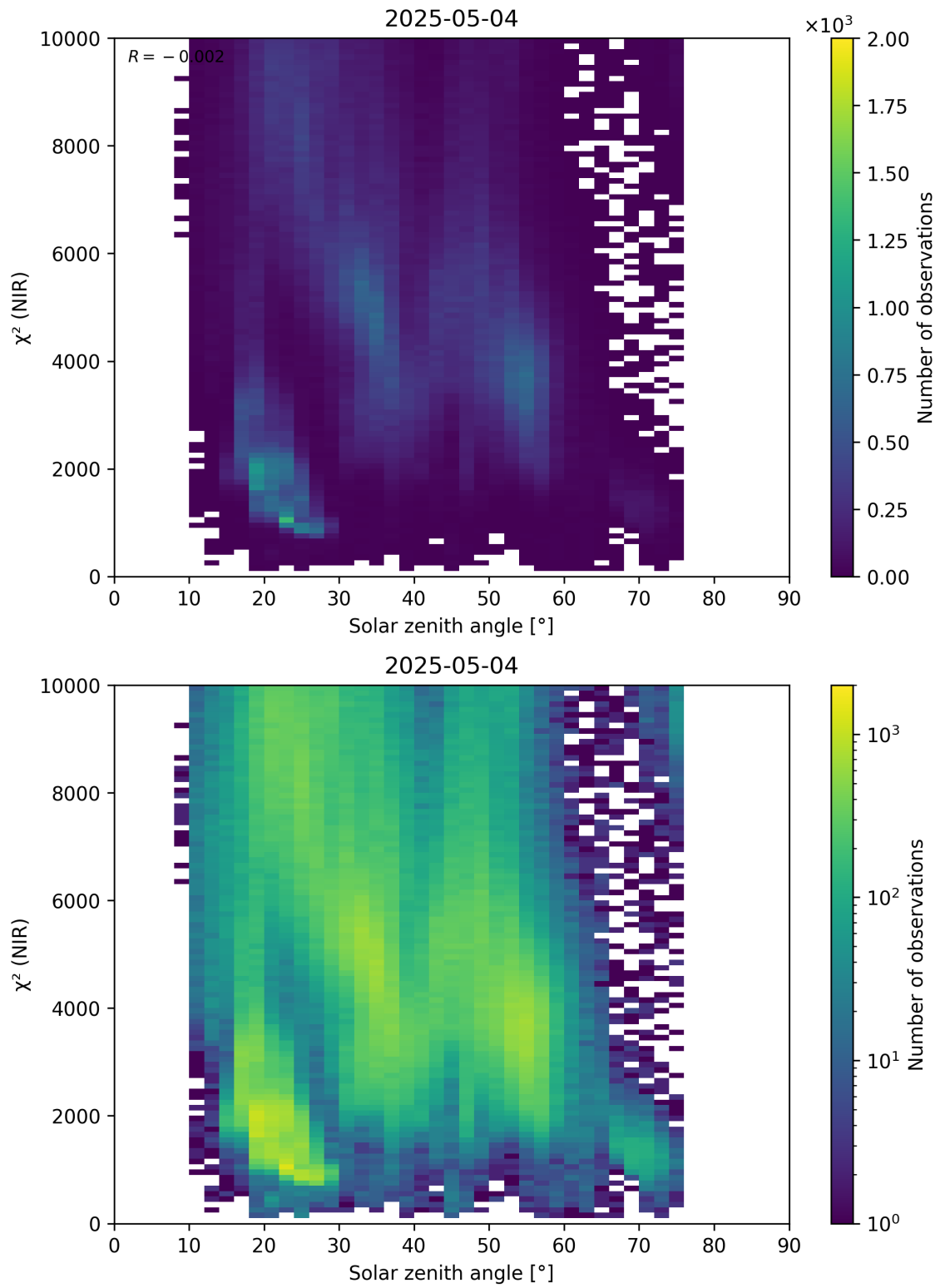
Figure 94: Scatter density plot of “Solar zenith angle” against “ \chi^2 (NIR)” for 2025-05-03 to 2025-05-05.
