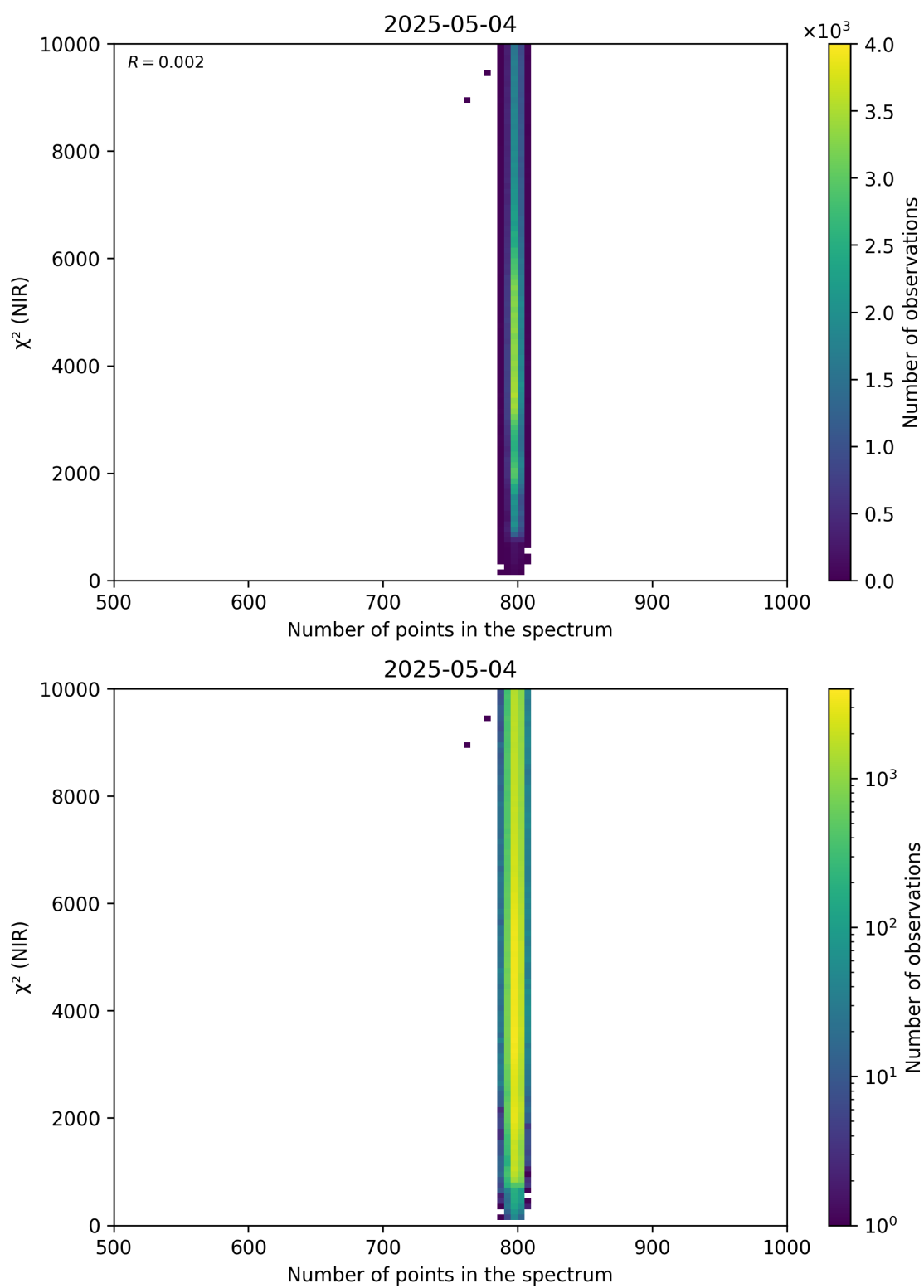
Figure 88: Scatter density plot of “Number of points in the spectrum” against “ \chi^2 (NIR)” for 2025-05-03 to 2025-05-05.
