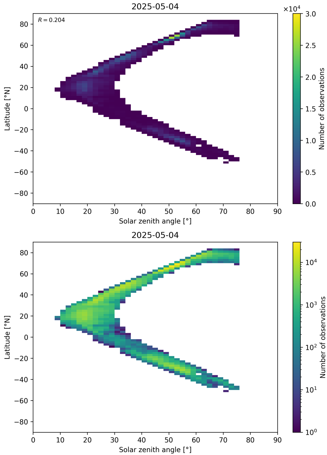
Figure 98: Scatter density plot of “Solar zenith angle” against “Latitude” for 2025-05-03 to 2025-05-05.
