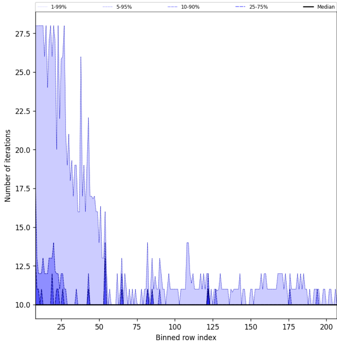
Figure 42: Along track statistics of “Number of iterations” for 2025-05-03 to 2025-05-05
