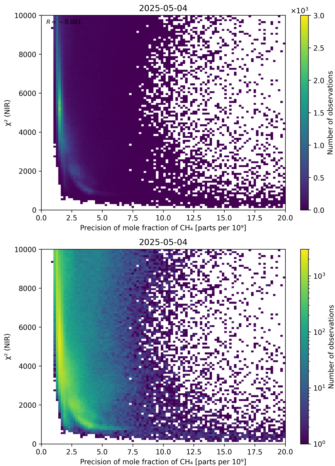
Figure 78: Scatter density plot of “Precision of mole fraction of CH 4 ” against “ \chi^2 (NIR)” for 2025-05-03 to 2025-05-05.
