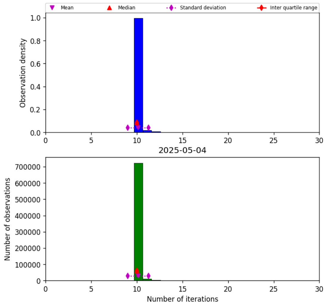
Figure 31: Histogram of “Number of iterations” for 2025-05-03 to 2025-05-05
