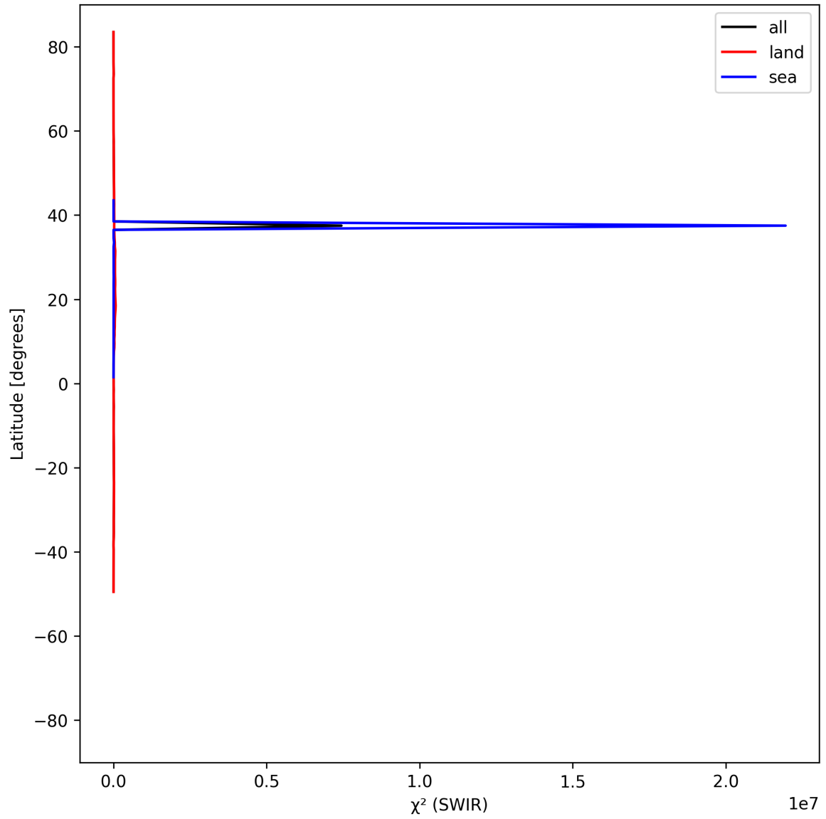
Figure 17: Zonal average of “ \chi^2 (SWIR)” for 2025-05-03 to 2025-05-05.
