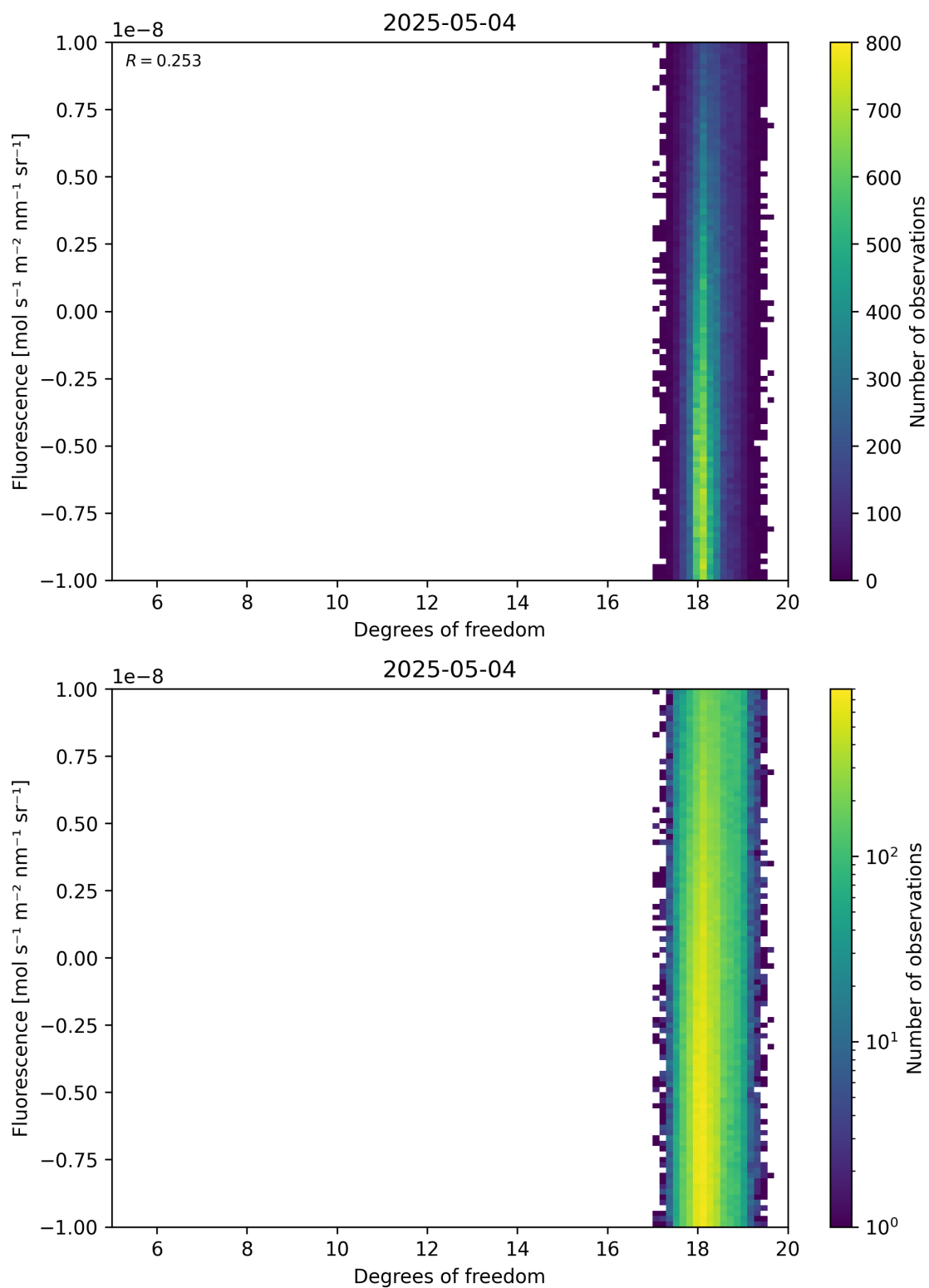
Figure 51: Scatter density plot of “Degrees of freedom” against “Fluorescence” for 2025-05-03 to 2025-05-05.
