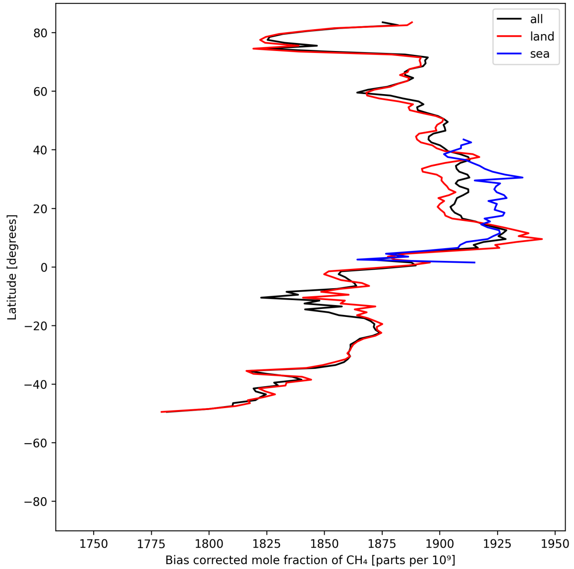
Figure 14: Zonal average of “Bias corrected mole fraction of \text{CH}_4 ” for 2025-05-03 to 2025-05-05.
