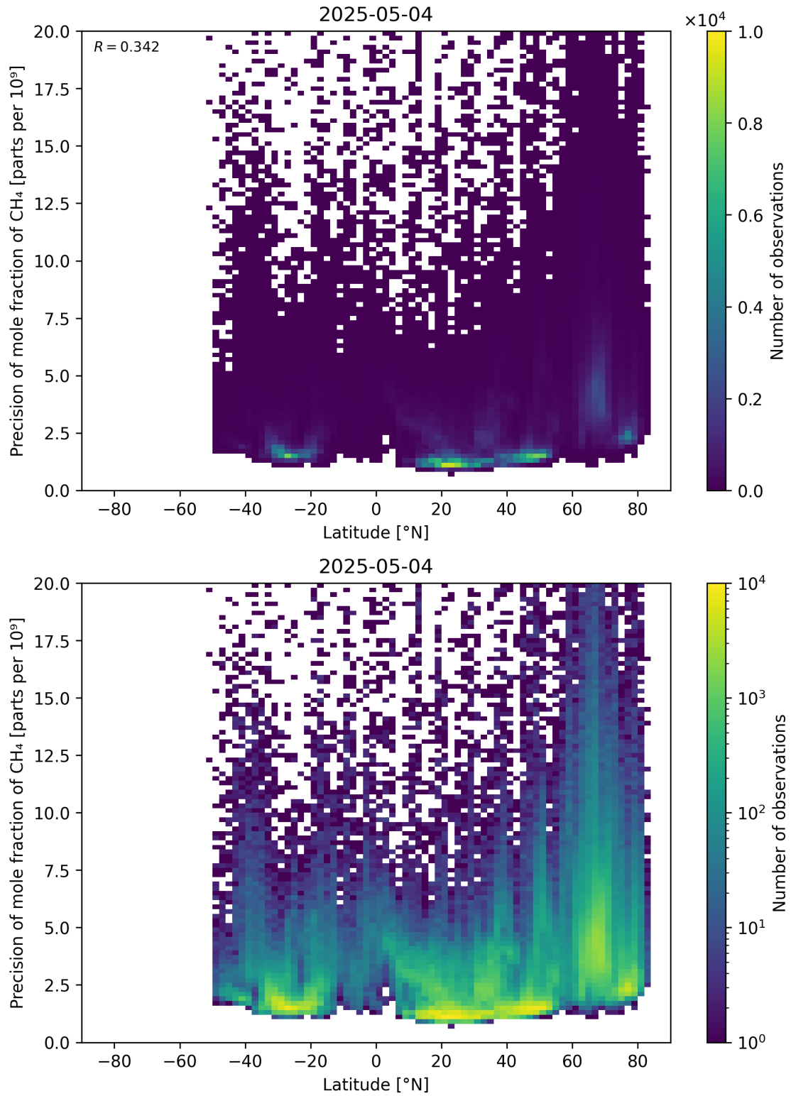
Figure 59: Scatter density plot of “Latitude” against “Precision of mole fraction of \text{CH}_4 ” for 2025-05-03 to 2025-05-05.
