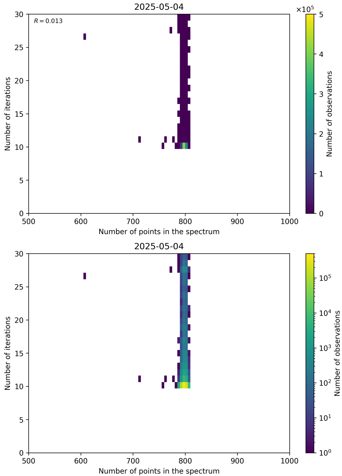
Figure 92: Scatter density plot of “Number of points in the spectrum” against “Number of iterations” for 2025-05-03 to 2025-05-05.
