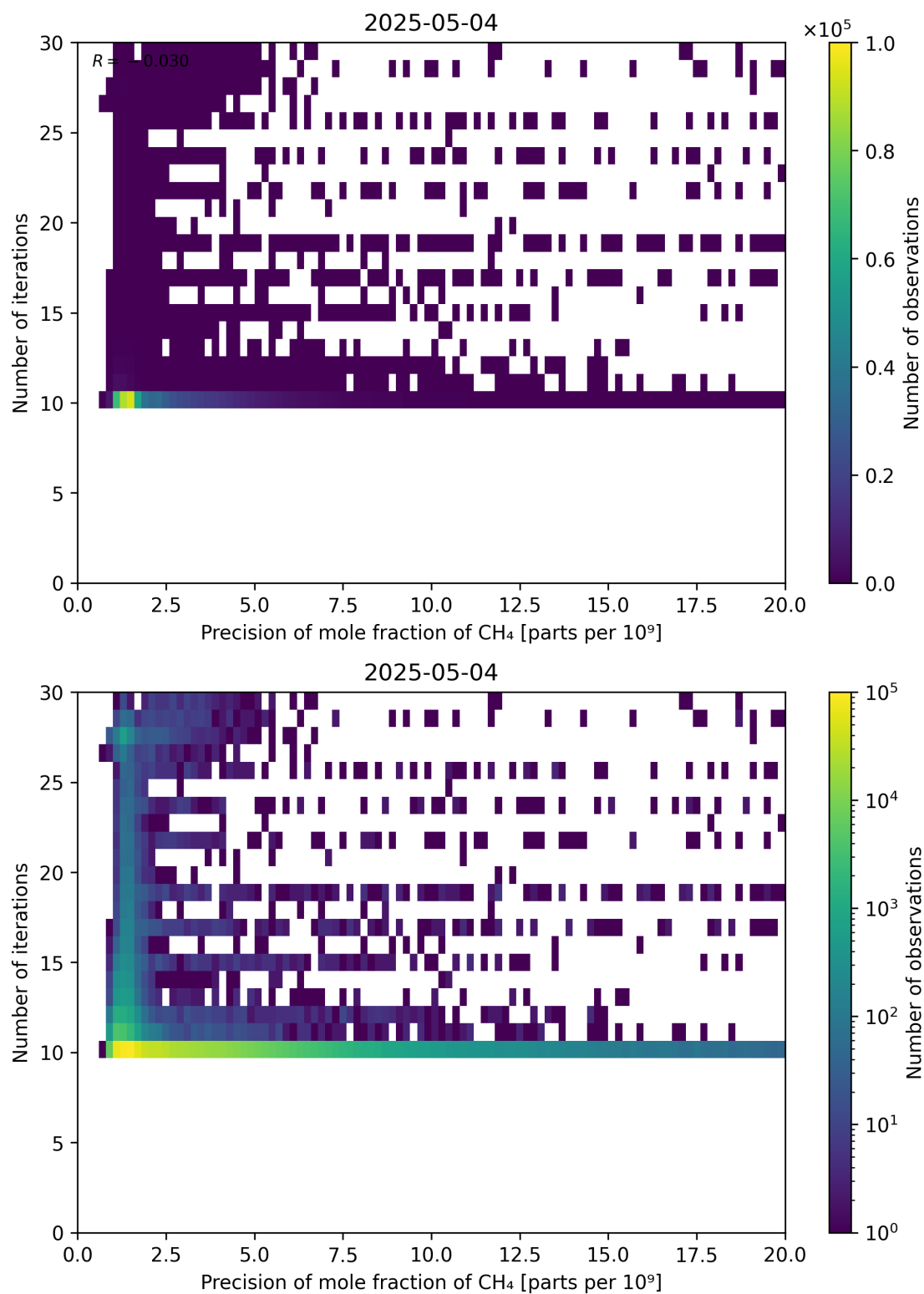
Figure 83: Scatter density plot of “Precision of mole fraction of CH 4 ” against “Number of iterations” for 2025-05-03 to 2025-05-05.
