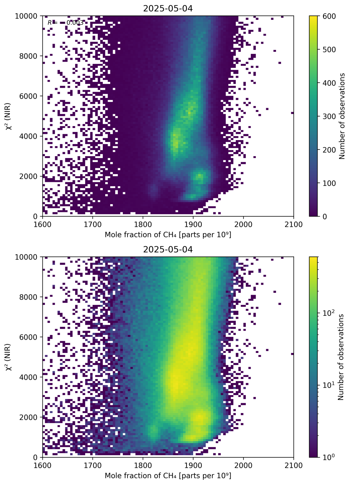
Figure 70: Scatter density plot of “Mole fraction of \text{CH}_4 ” against “ \chi^2 (NIR)” for 2025-05-03 to 2025-05-05.
