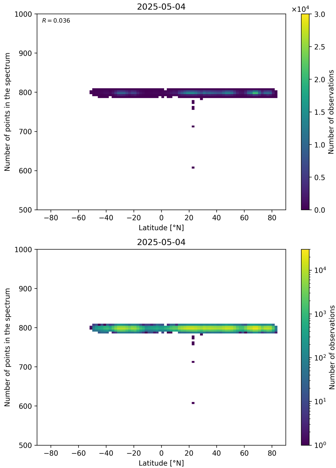
Figure 61: Scatter density plot of “Latitude” against “Number of points in the spectrum” for 2025-05-03 to 2025-05-05.
