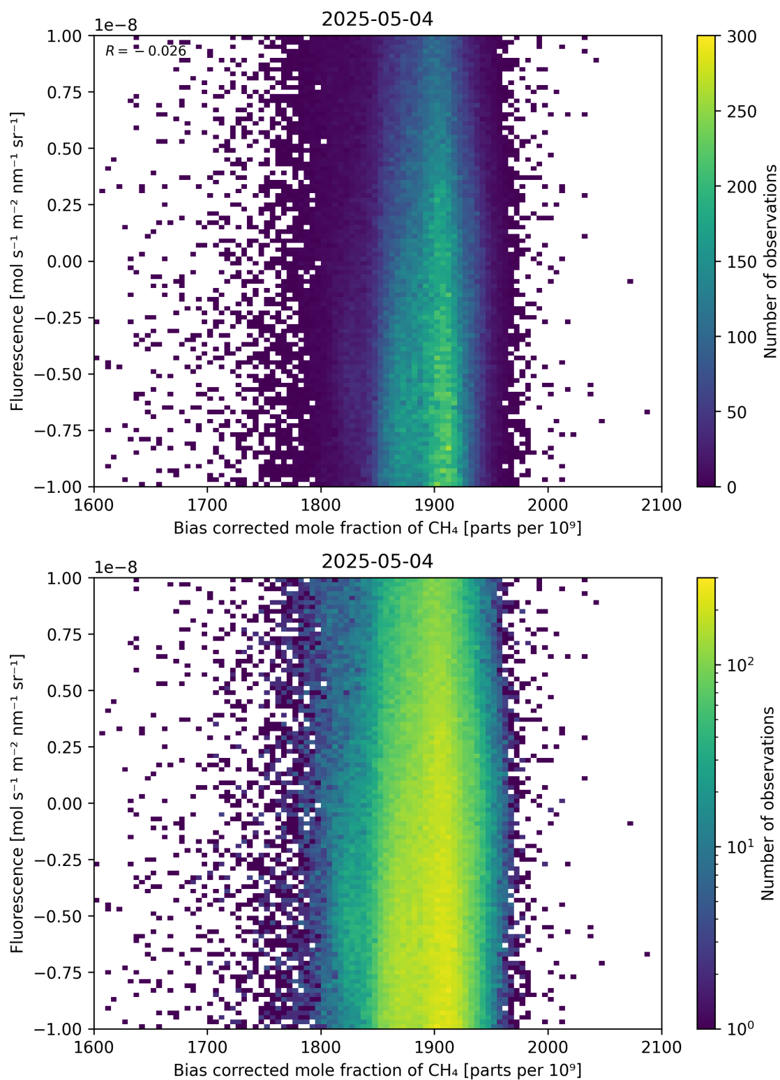
Figure 66: Scatter density plot of “Bias corrected mole fraction of \text{CH}_4 ” against “Fluorescence” for 2025-05-03 to 2025-05-05.
