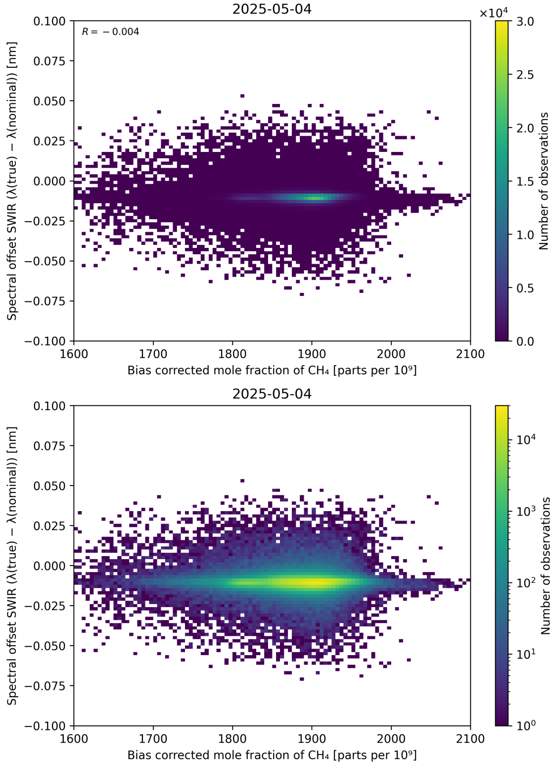
Figure 69: Scatter density plot of “Bias corrected mole fraction of \text{CH}_4 ” against “Spectral offset SWIR ( \lambda_{\text{true}} - \lambda_{\text{nominal}} )” for 2025-05-03 to 2025-05-05.
