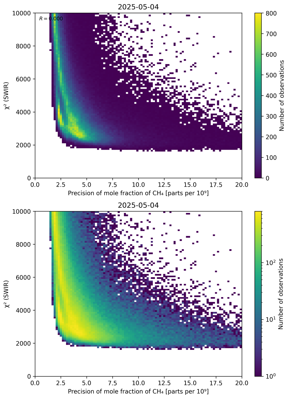
Figure 79: Scatter density plot of “Precision of mole fraction of \text{CH}_4 ” against “ \chi^2 (SWIR)” for 2025-05-03 to 2025-05-05.
