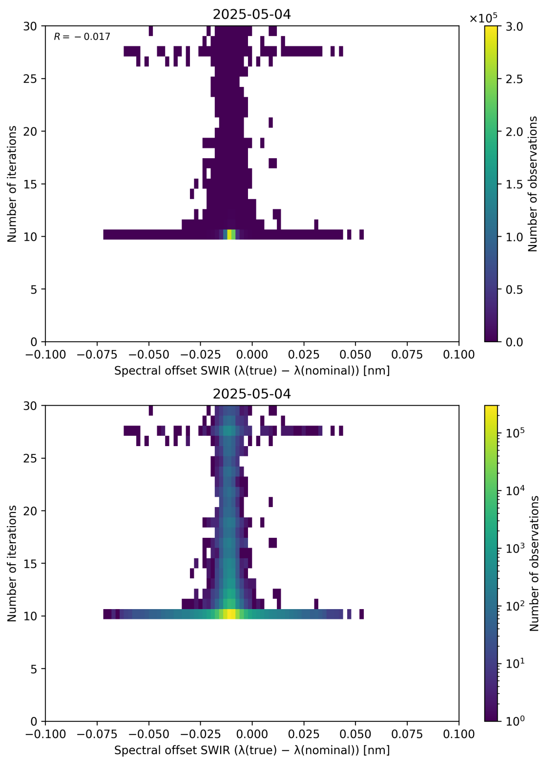
Figure 121: Scatter density plot of “Spectral offset SWIR ( \lambda_{\text{true}} - \lambda_{\text{nominal}} )” against “Number of iterations” for 2025-05-03 to 2025-05-05.
