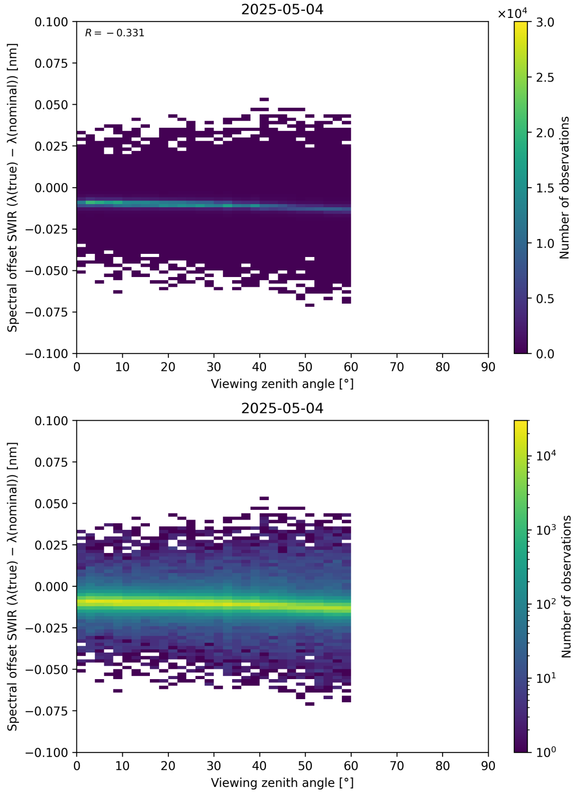
Figure 116: Scatter density plot of “Viewing zenith angle” against “Spectral offset SWIR ( \lambda_{\text{true}} - \lambda_{\text{nominal}} )” for 2025-05-03 to 2025-05-05.
