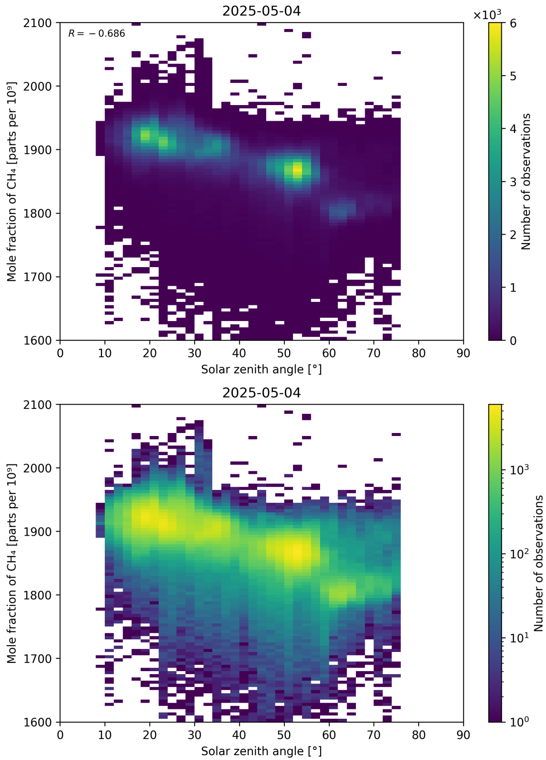
Figure 99: Scatter density plot of “Solar zenith angle” against “Mole fraction of \text{CH}_4 ” for 2025-05-03 to 2025-05-05.
