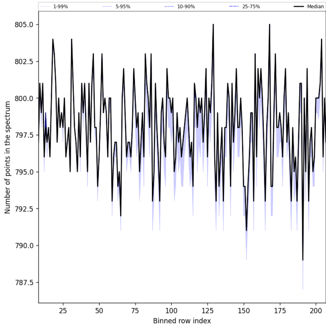
Figure 37: Along track statistics of “Number of points in the spectrum” for 2025-05-03 to 2025-05-05
