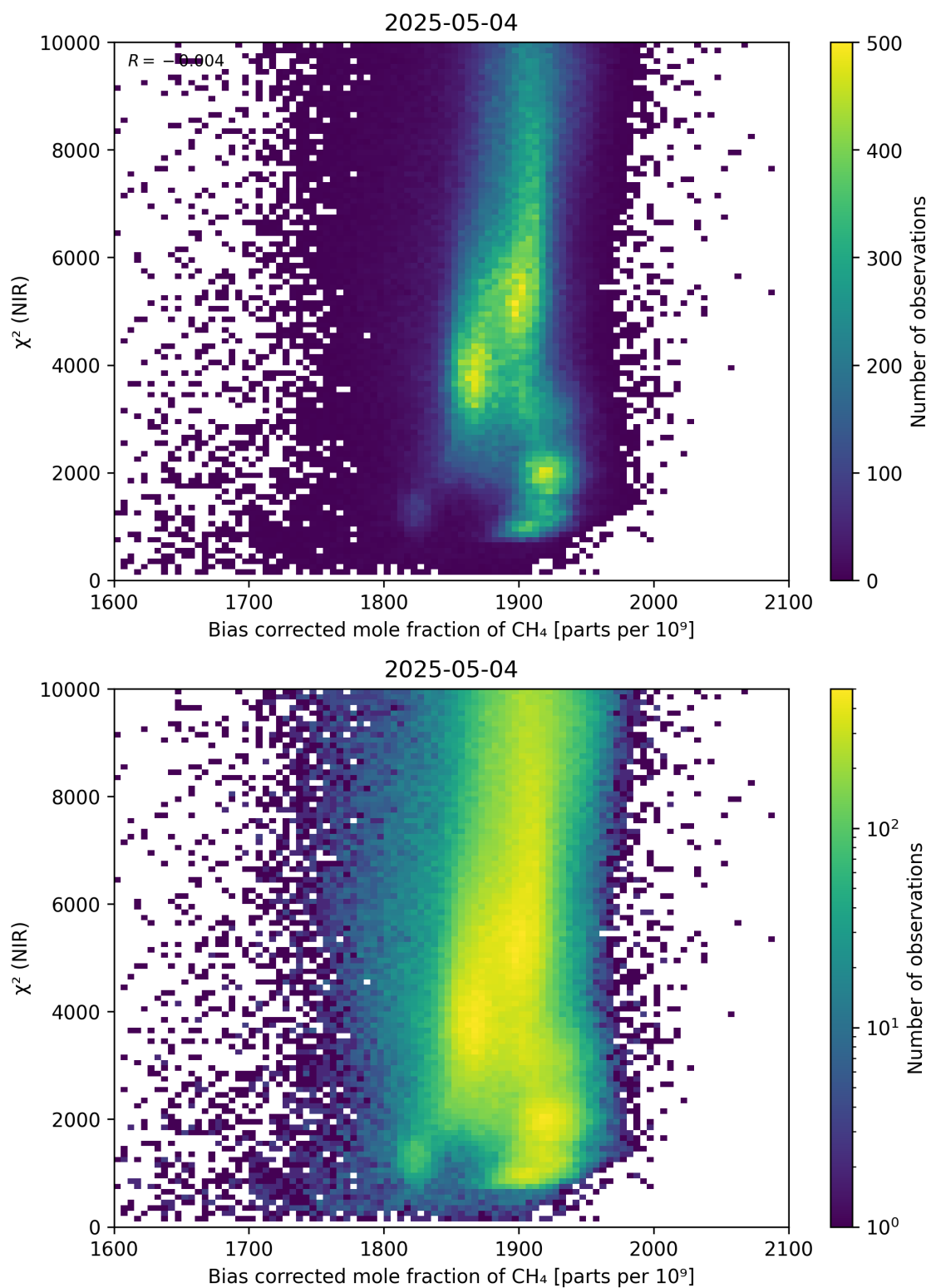
Figure 63: Scatter density plot of “Bias corrected mole fraction of CH 4 ” against “ \chi^2 (NIR)” for 2025-05-03 to 2025-05-05.
