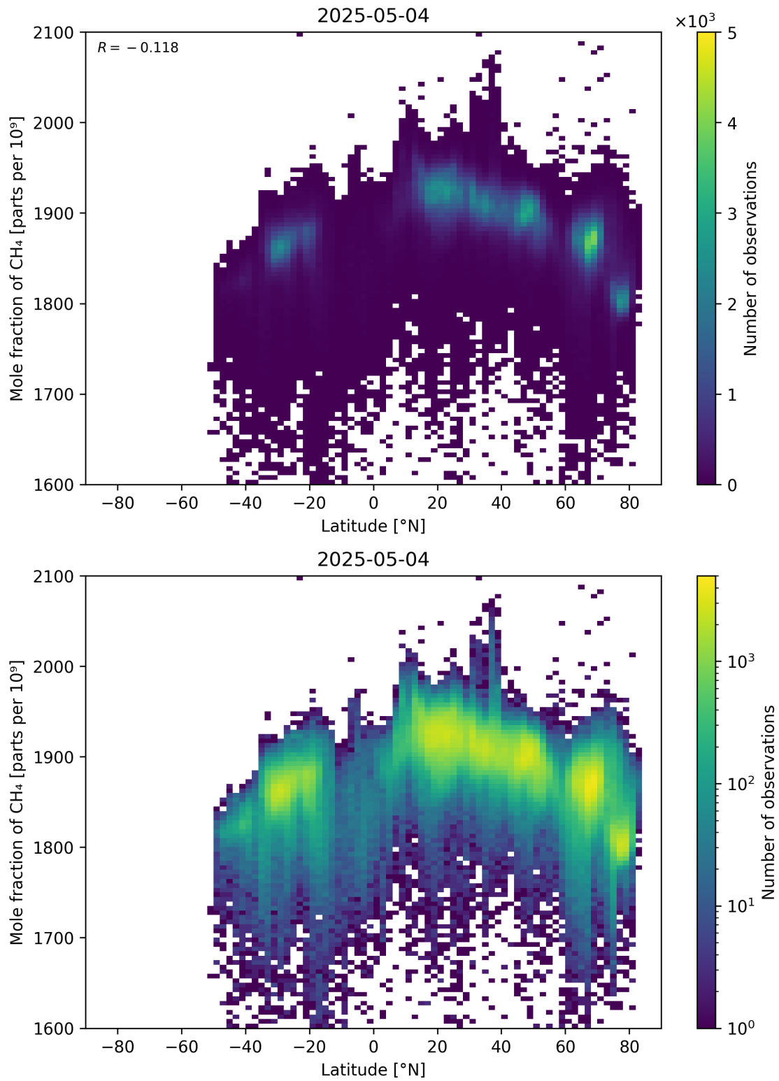
Figure 57: Scatter density plot of “Latitude” against “Mole fraction of CH 4 ” for 2025-05-03 to 2025-05-05.
