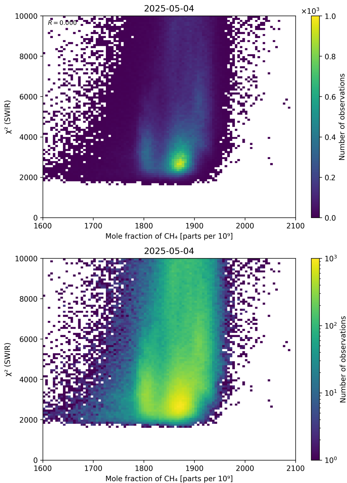
Figure 71: Scatter density plot of “Mole fraction of \text{CH}_4 ” against “ \chi^2 (SWIR)” for 2025-05-03 to 2025-05-05.
