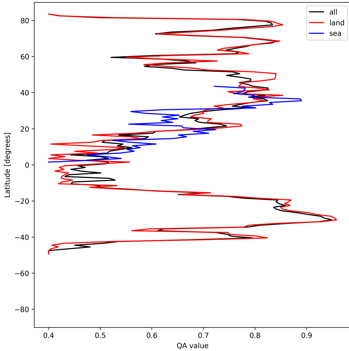
Figure 11: Zonal average of “QA value” for 2025-05-03 to 2025-05-05.
