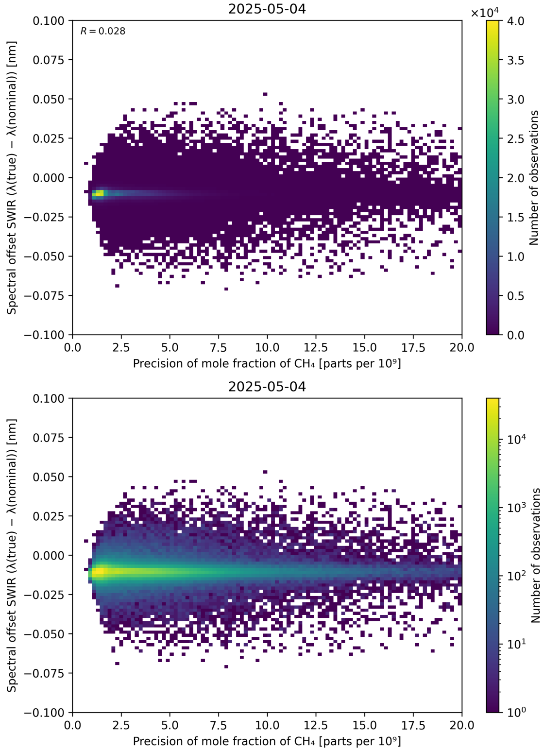
Figure 85: Scatter density plot of “Precision of mole fraction of CH 4 ” against “Spectral offset SWIR ( \lambda_{\text{true}} - \lambda_{\text{nominal}} )” for 2025-05-03 to 2025-05-05.
