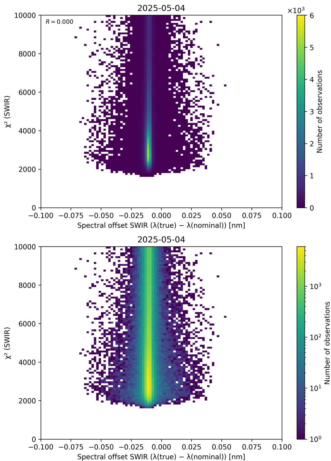
Figure 118: Scatter density plot of “Spectral offset SWIR ( \lambda_{\text{true}} - \lambda_{\text{nominal}} )” against “ \chi^2 (SWIR)” for 2025-05-03 to 2025-05-05.
