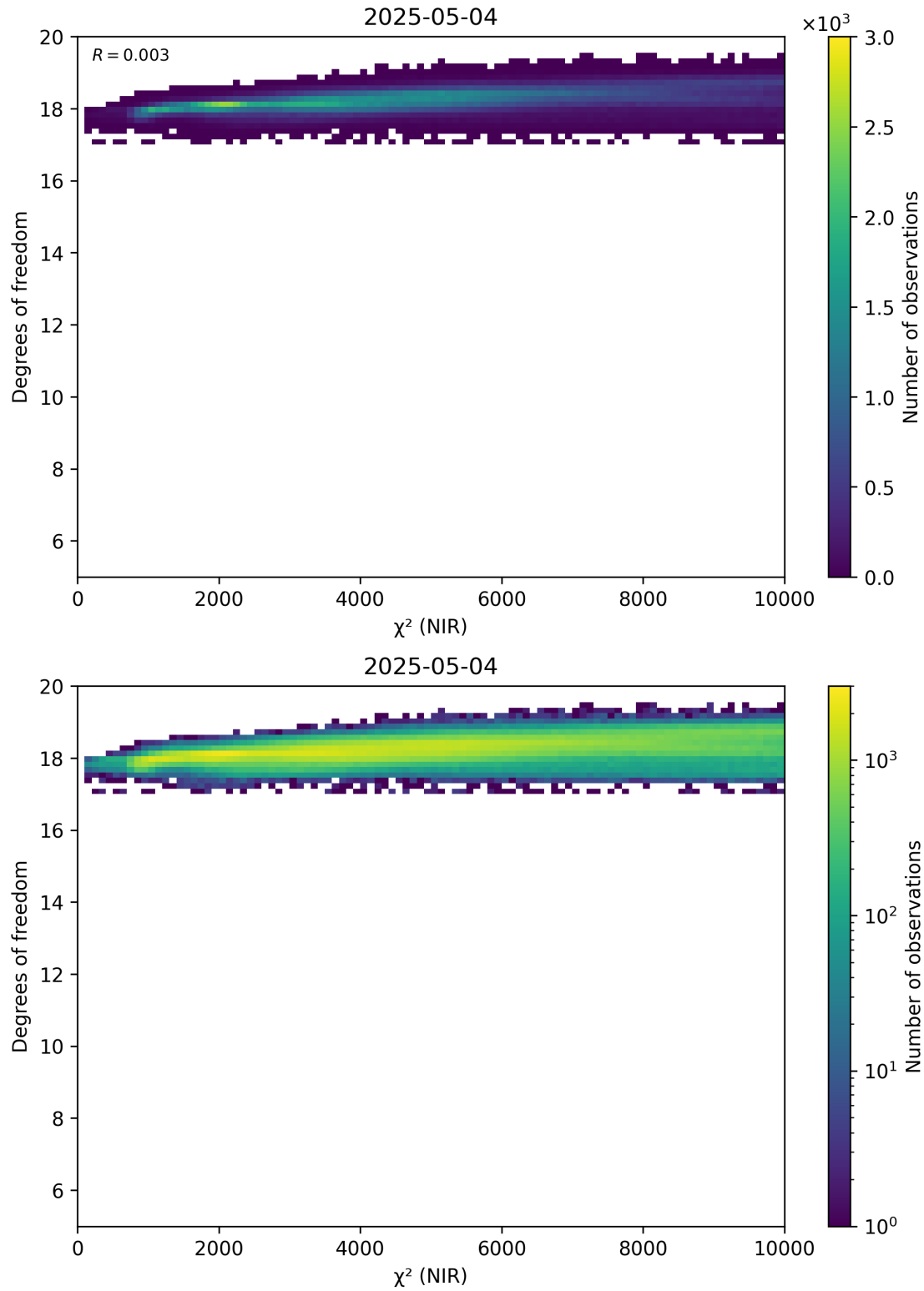
Figure 44: Scatter density plot of “ \chi^2 (NIR)” against “Degrees of freedom” for 2025-05-03 to 2025-05-05.
