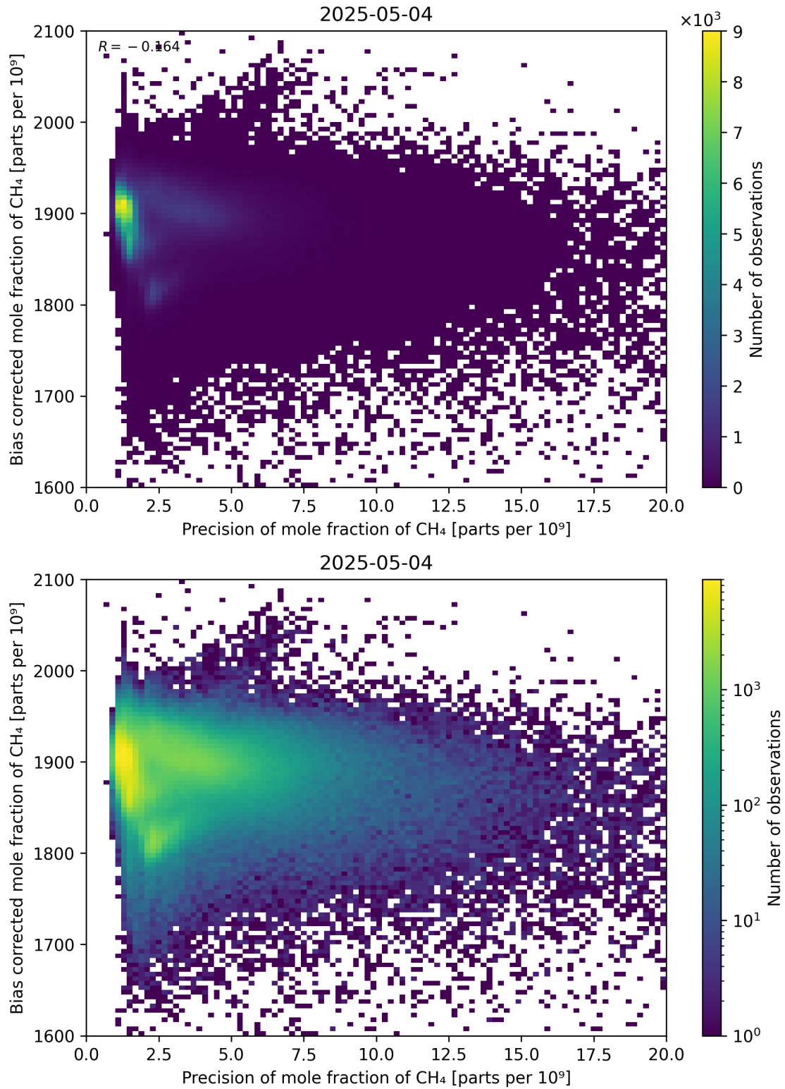
Figure 82: Scatter density plot of “Precision of mole fraction of CH 4 ” against “Bias corrected mole fraction of CH 4 ” for 2025-05-03 to 2025-05-05.
