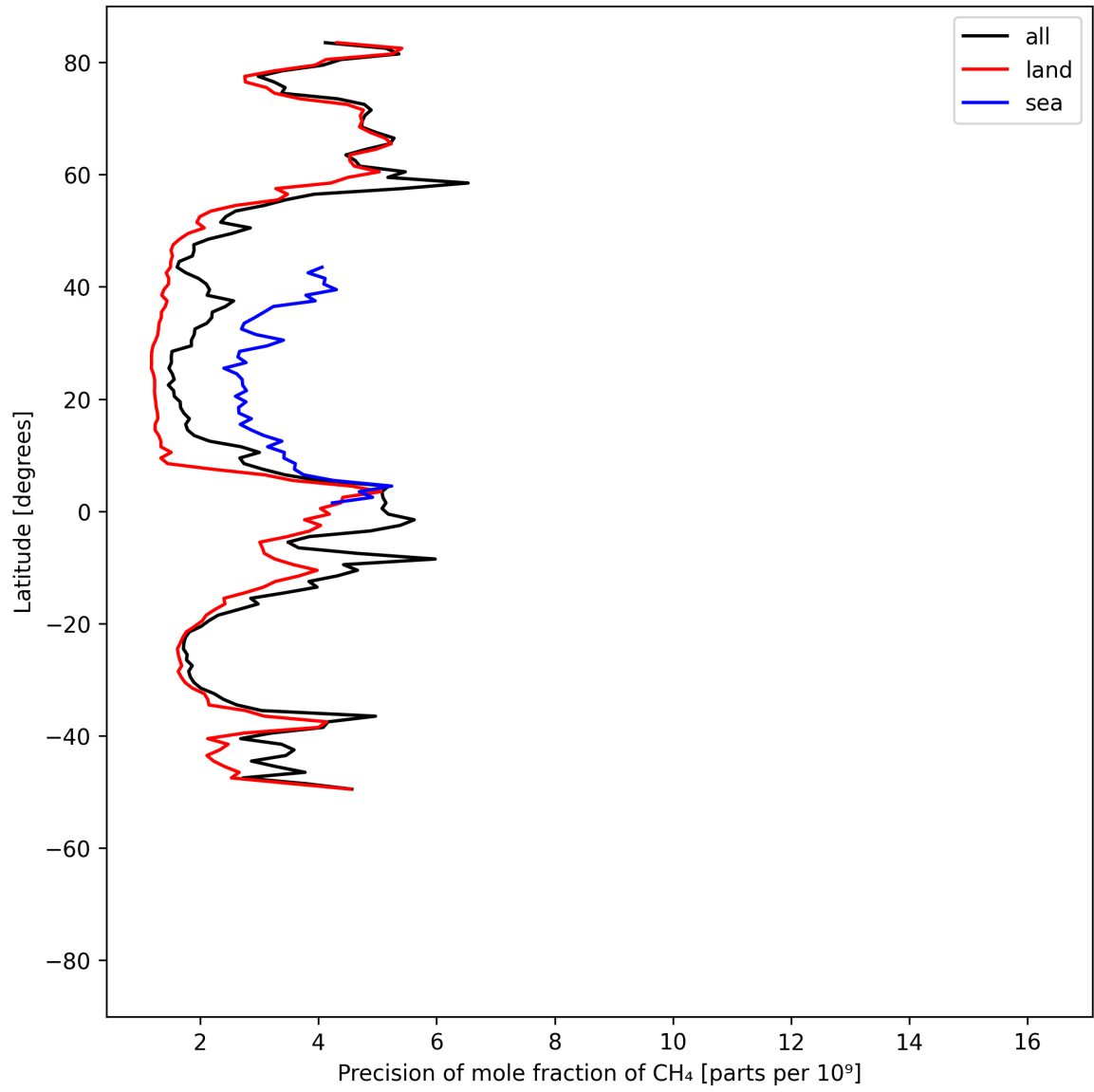
Figure 13: Zonal average of “Precision of mole fraction of CH 4 ” for 2025-05-03 to 2025-05-05.
