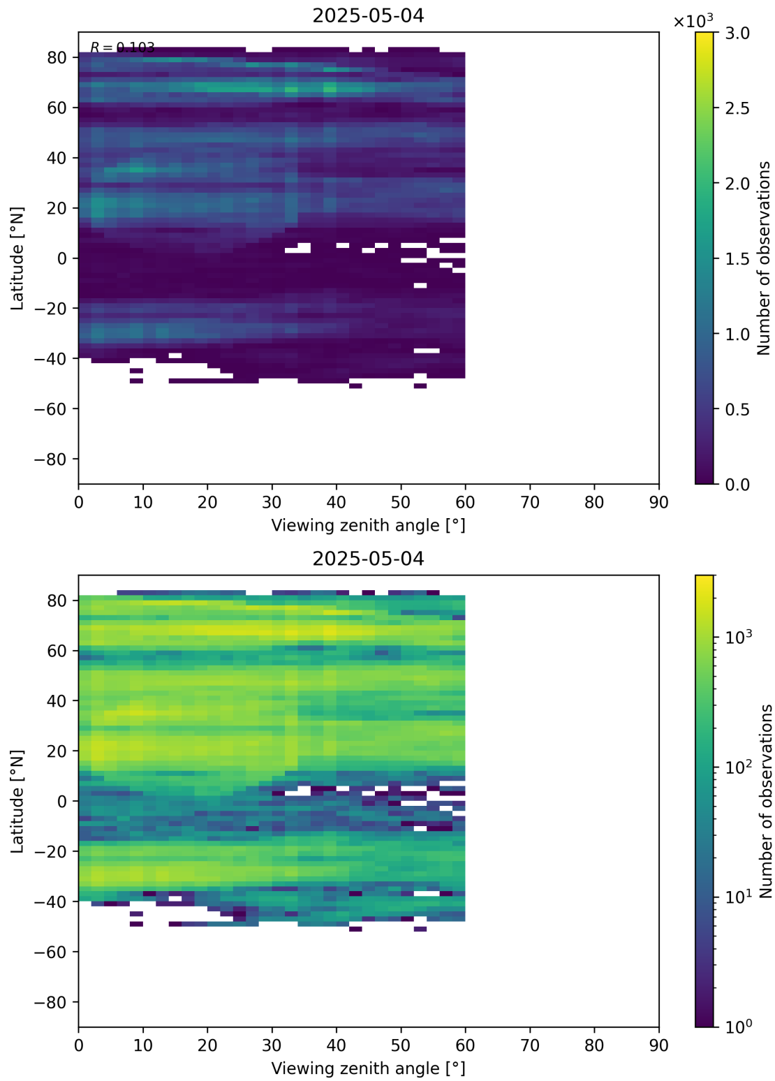
Figure 109: Scatter density plot of “Viewing zenith angle” against “Latitude” for 2025-05-03 to 2025-05-05.
