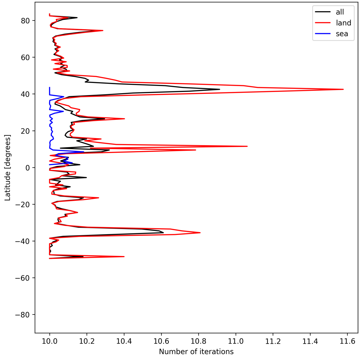
Figure 20: Zonal average of “Number of iterations” for 2025-05-03 to 2025-05-05.
