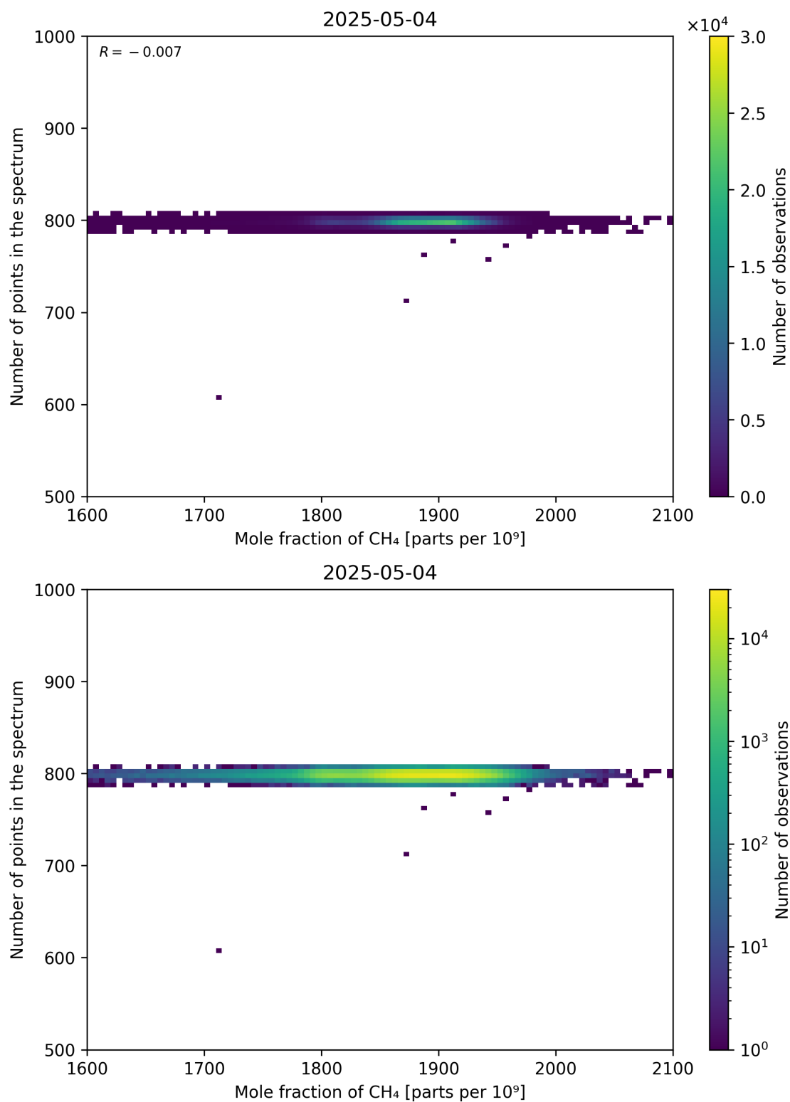
Figure 77: Scatter density plot of “Mole fraction of CH 4 ” against “Number of points in the spectrum” for 2025-05-03 to 2025-05-05.
