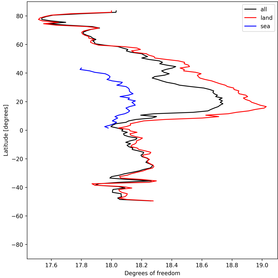
Figure 19: Zonal average of “Degrees of freedom” for 2025-05-03 to 2025-05-05.
