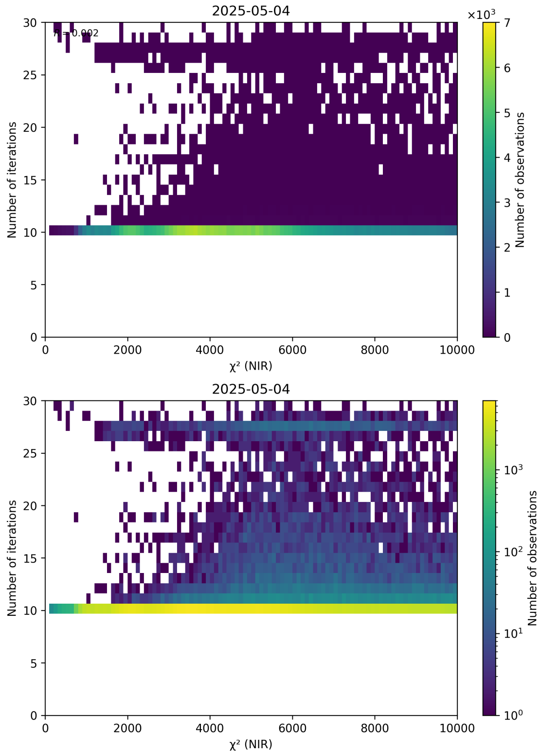
Figure 46: Scatter density plot of “ \chi^2 (NIR)” against “Number of iterations” for 2025-05-03 to 2025-05-05.
