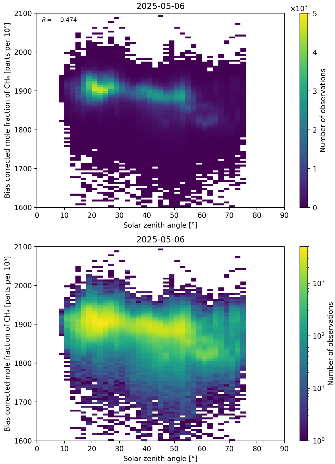
Figure 100: Scatter density plot of “Solar zenith angle” against “Bias corrected mole fraction of \text{CH}_4 ” for 2025-05-05 to 2025-05-07.
