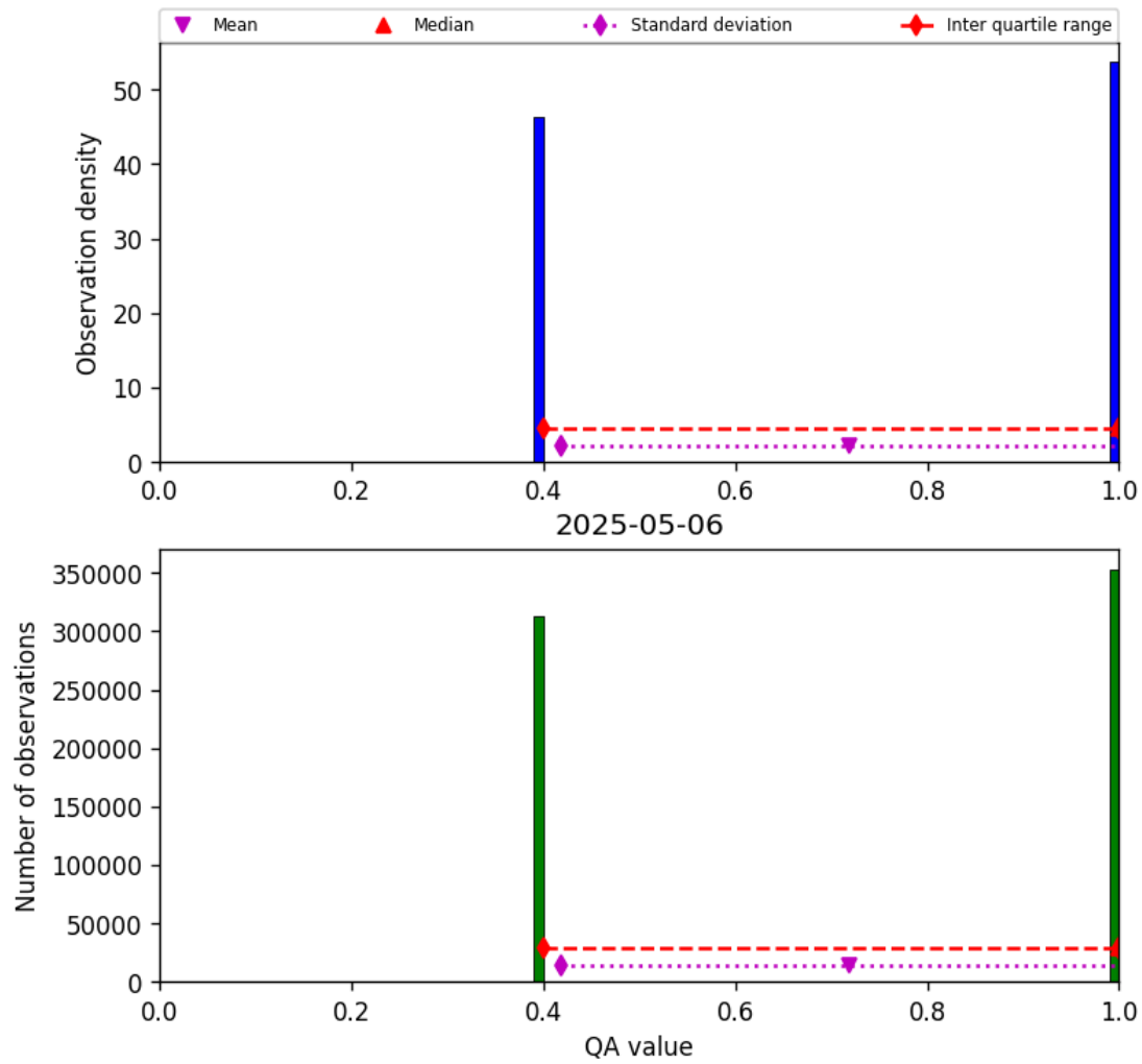
Figure 22: Histogram of “QA value” for 2025-05-05 to 2025-05-07
