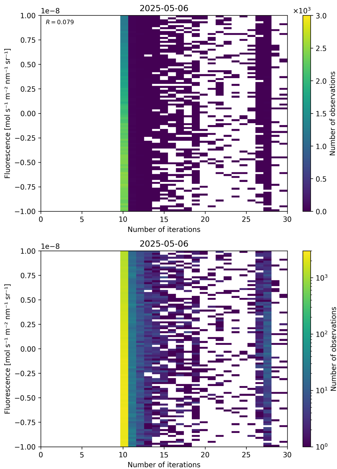
Figure 87: Scatter density plot of "Number of iterations" against "Fluorescence" for 2025-05-05 to 2025-05-07.
