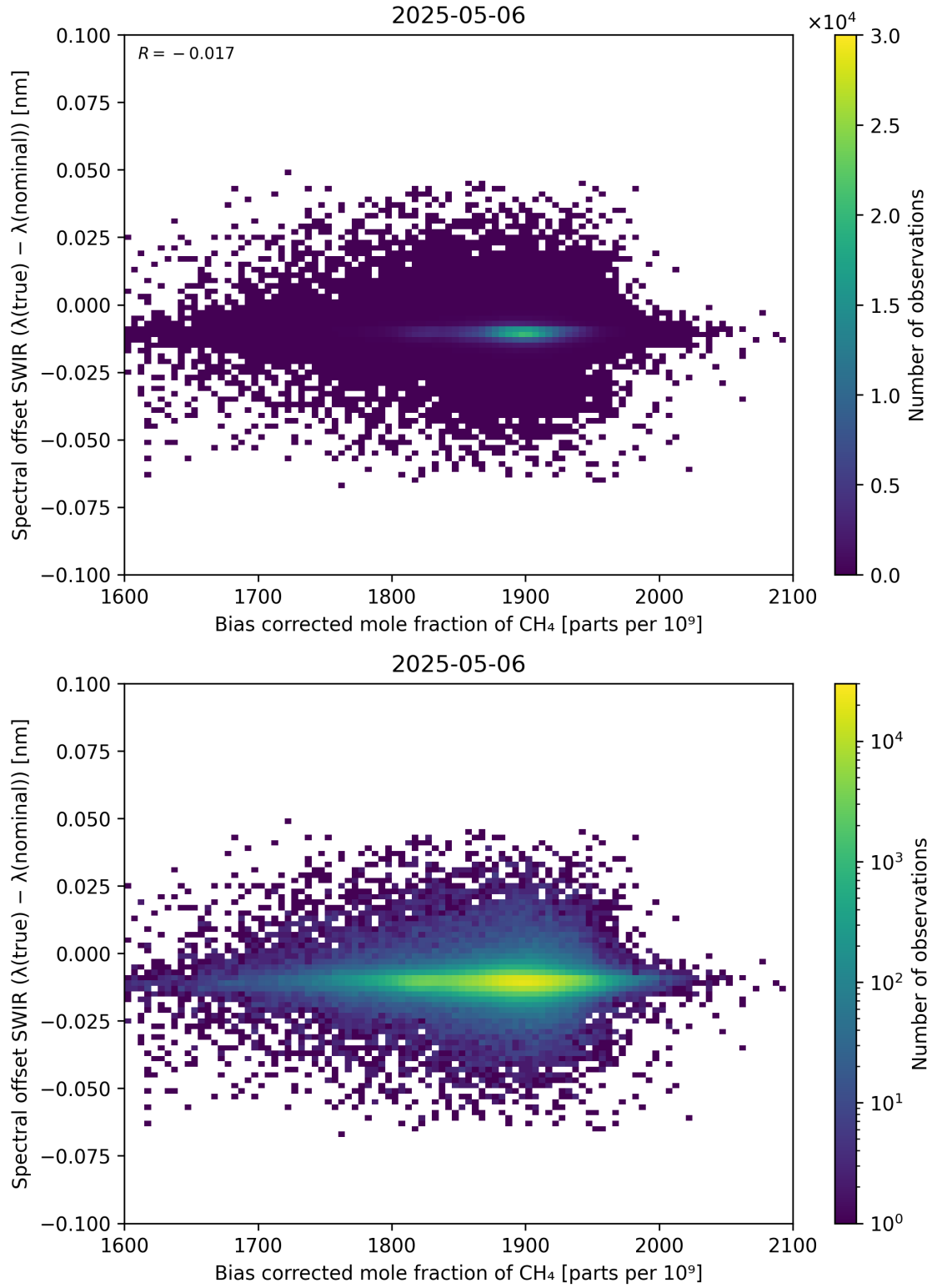
Figure 69: Scatter density plot of “Bias corrected mole fraction of \text{CH}_4 ” against “Spectral offset SWIR ( \lambda_{\text{true}} - \lambda_{\text{nominal}} )” for 2025-05-05 to 2025-05-07.
