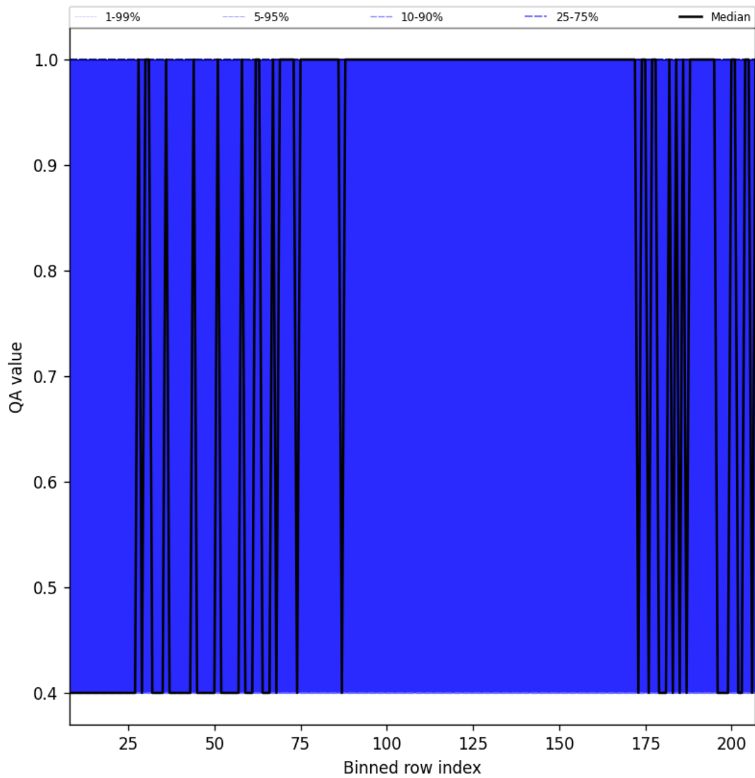
Figure 33: Along track statistics of “QA value” for 2025-05-05 to 2025-05-07
