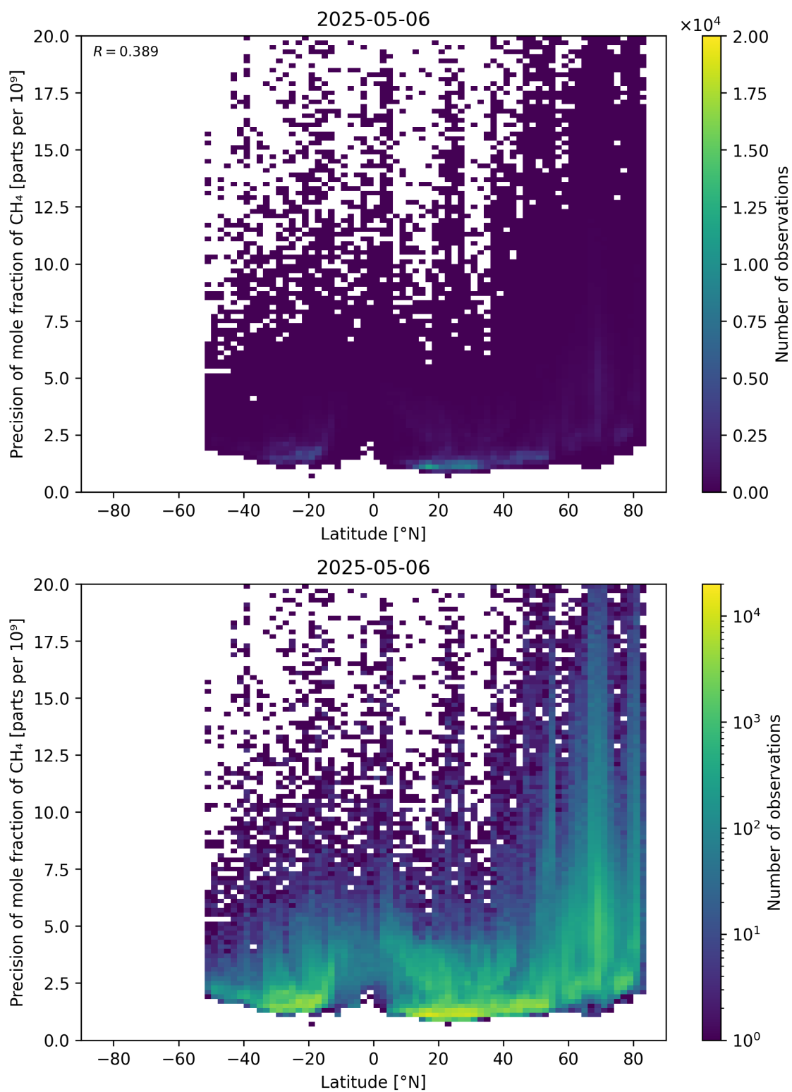
Figure 59: Scatter density plot of “Latitude” against “Precision of mole fraction of \text{CH}_4 ” for 2025-05-05 to 2025-05-07.
