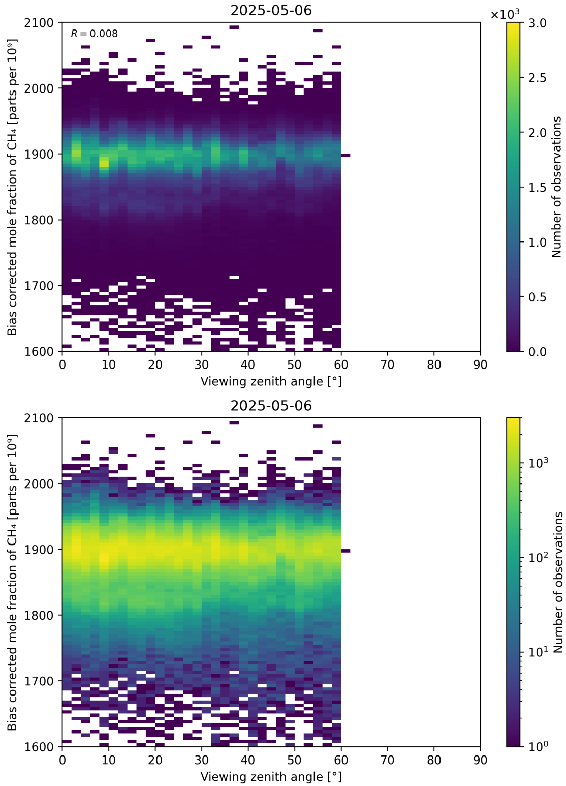
Figure 111: Scatter density plot of “Viewing zenith angle” against “Bias corrected mole fraction of CH 4 ” for 2025-05-05 to 2025-05-07.
