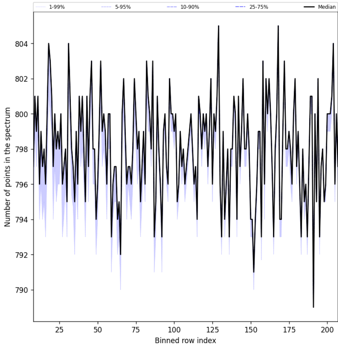
Figure 37: Along track statistics of “Number of points in the spectrum” for 2025-05-05 to 2025-05-07
