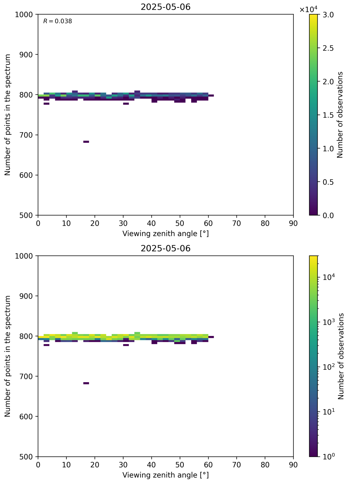
Figure 114: Scatter density plot of “Viewing zenith angle” against “Number of points in the spectrum” for 2025-05-05 to 2025-05-07.
