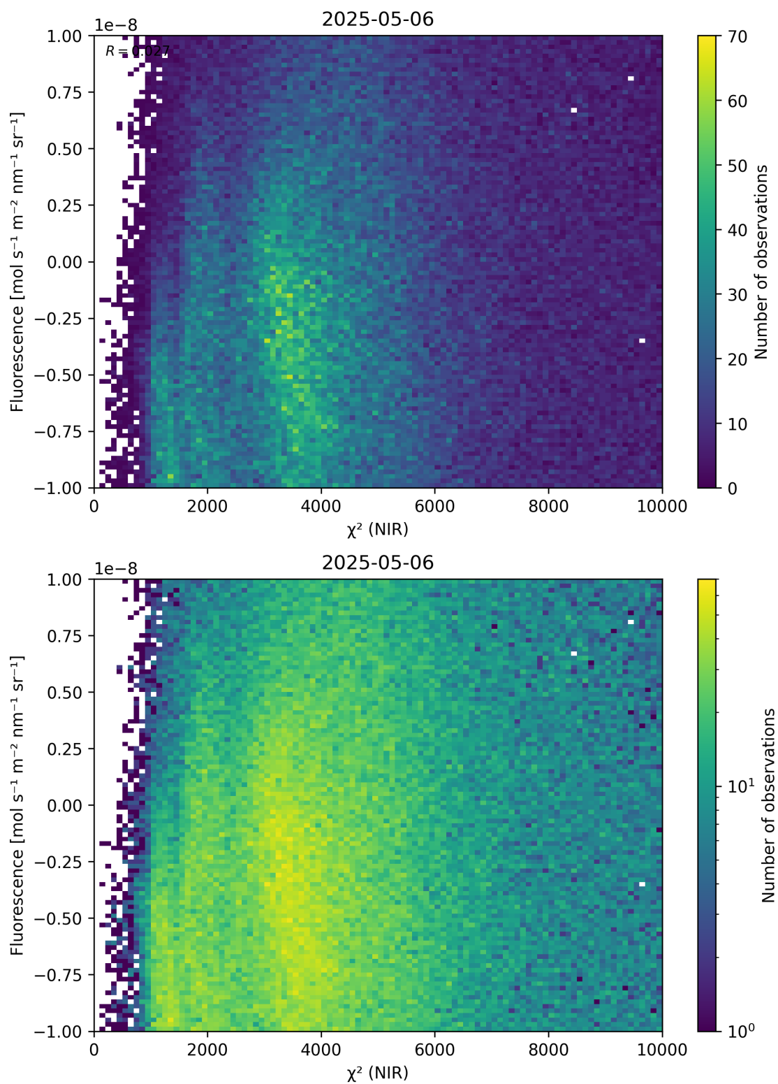
Figure 45: Scatter density plot of “ \chi^2 (NIR)” against “Fluorescence” for 2025-05-05 to 2025-05-07.
