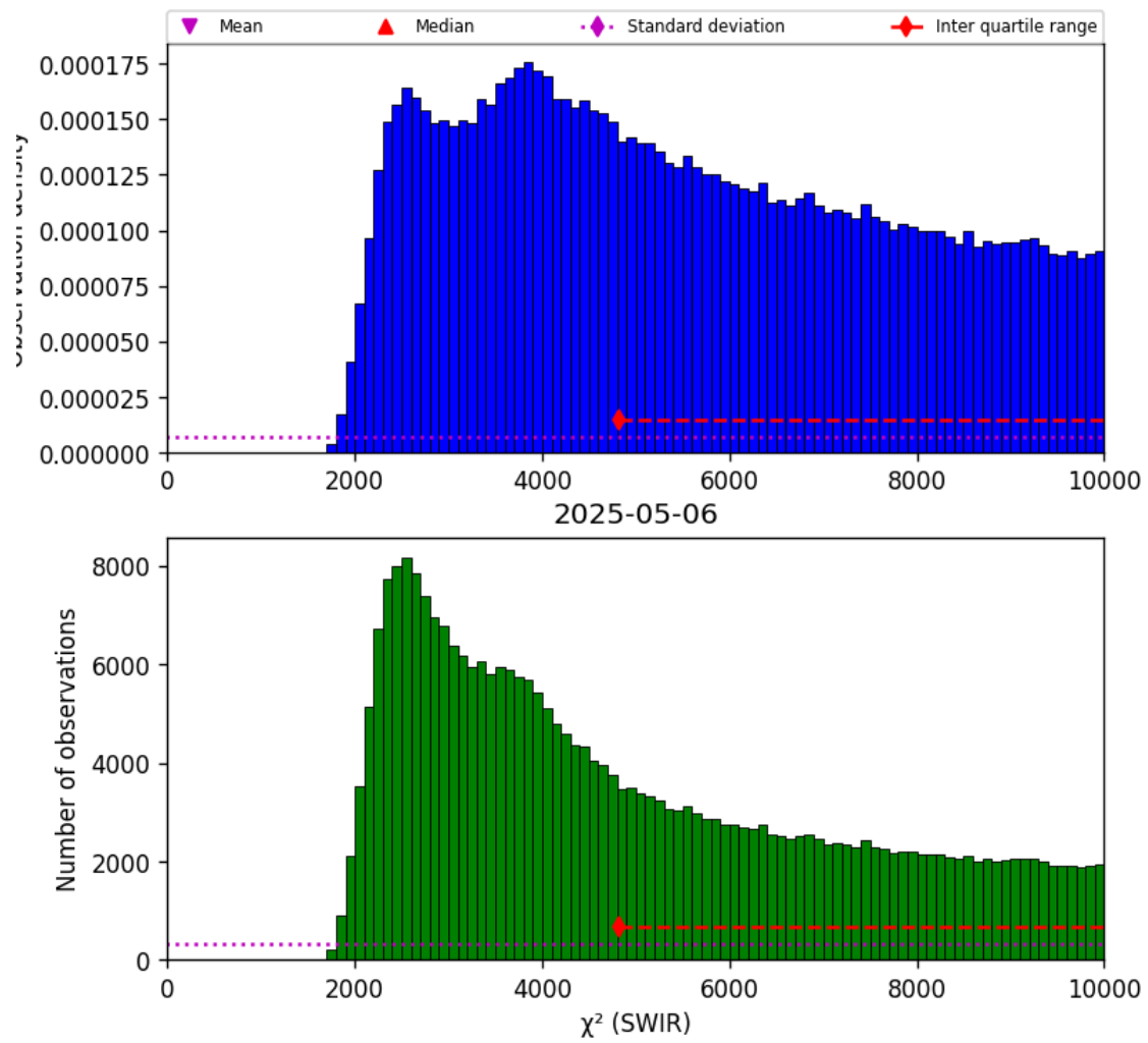
Figure 28: Histogram of “ \chi^2 (SWIR)” for 2025-05-05 to 2025-05-07
