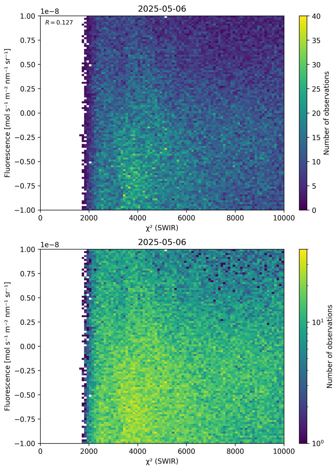
Figure 49: Scatter density plot of “ \chi^2 (SWIR)” against “Fluorescence” for 2025-05-05 to 2025-05-07.
