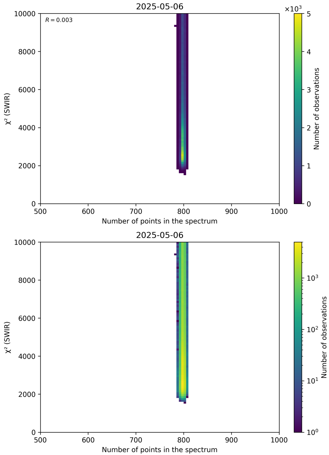
Figure 89: Scatter density plot of “Number of points in the spectrum” against “ \chi^2 (SWIR)” for 2025-05-05 to 2025-05-07.
