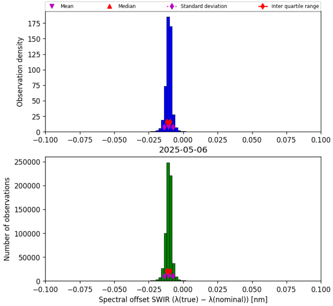
Figure 27: Histogram of “Spectral offset SWIR ( \lambda_{\text{true}} - \lambda_{\text{nominal}} )” for 2025-05-05 to 2025-05-07
