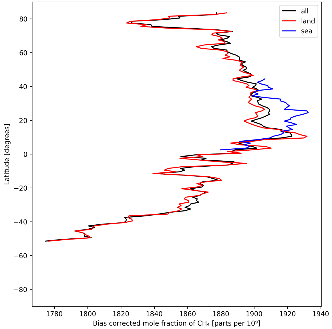
Figure 14: Zonal average of “Bias corrected mole fraction of CH 4 ” for 2025-05-05 to 2025-05-07.
