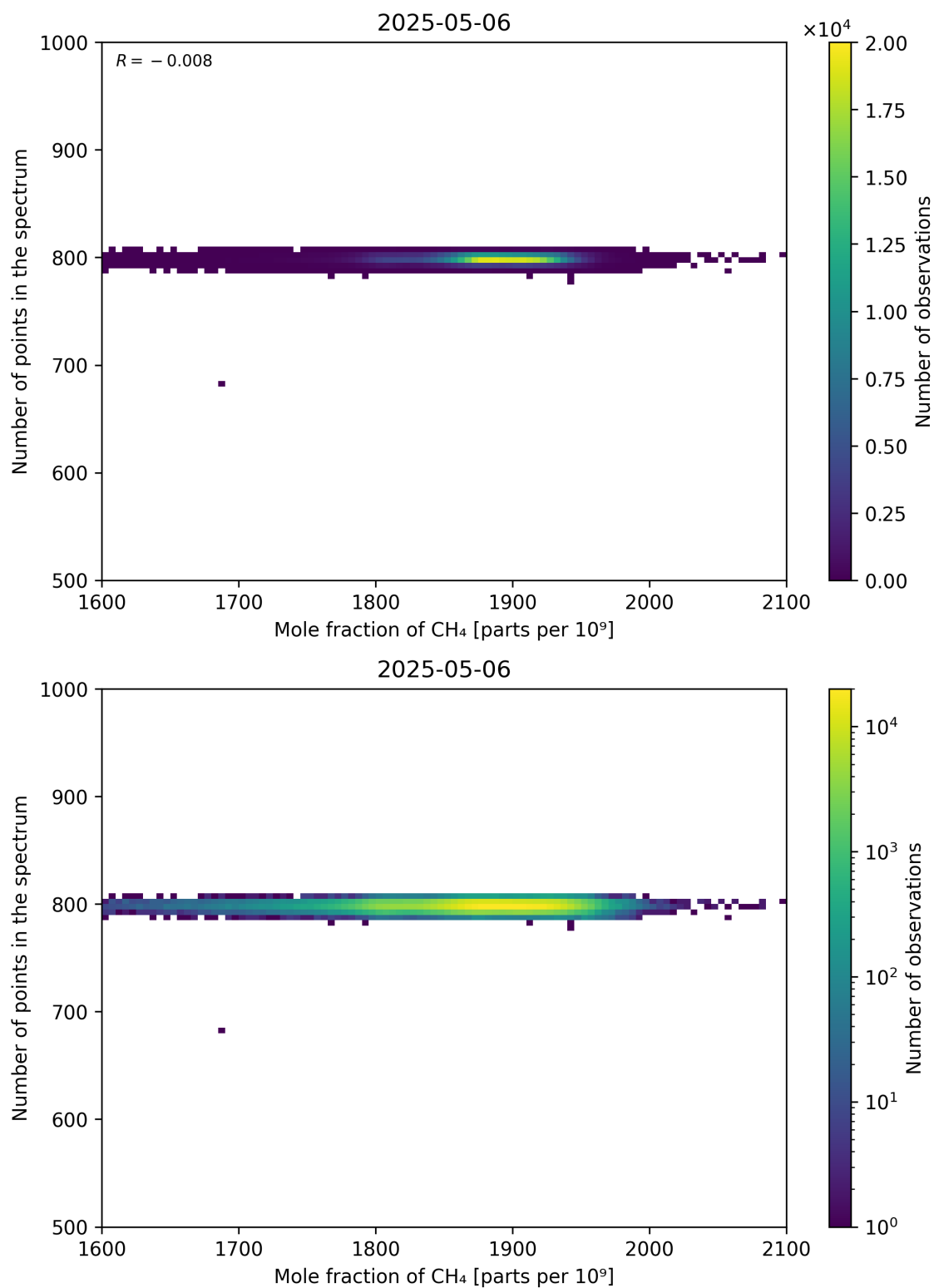
Figure 77: Scatter density plot of “Mole fraction of CH 4 ” against “Number of points in the spectrum” for 2025-05-05 to 2025-05-07.
