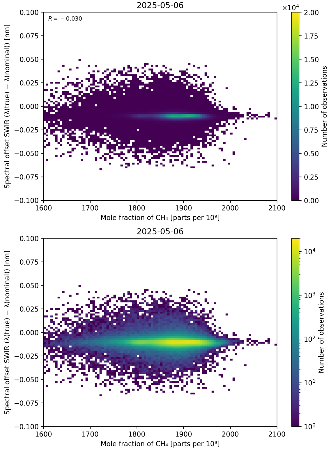
Figure 86: Scatter density plot of “Mole fraction of \text{CH}_4 ” against “Spectral offset SWIR ( \lambda_{\text{true}} - \lambda_{\text{nominal}} )” for 2025-05-05 to 2025-05-07.
