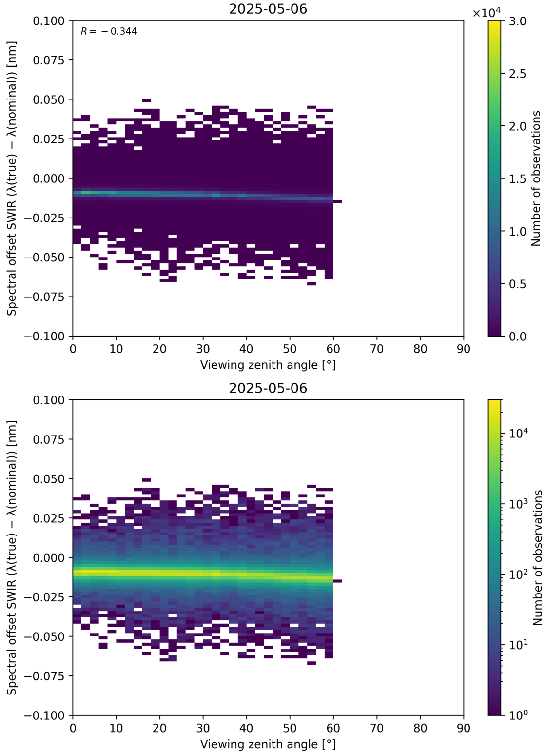
Figure 116: Scatter density plot of “Viewing zenith angle” against “Spectral offset SWIR ( \lambda_{\text{true}} - \lambda_{\text{nominal}} )” for 2025-05-05 to 2025-05-07.
