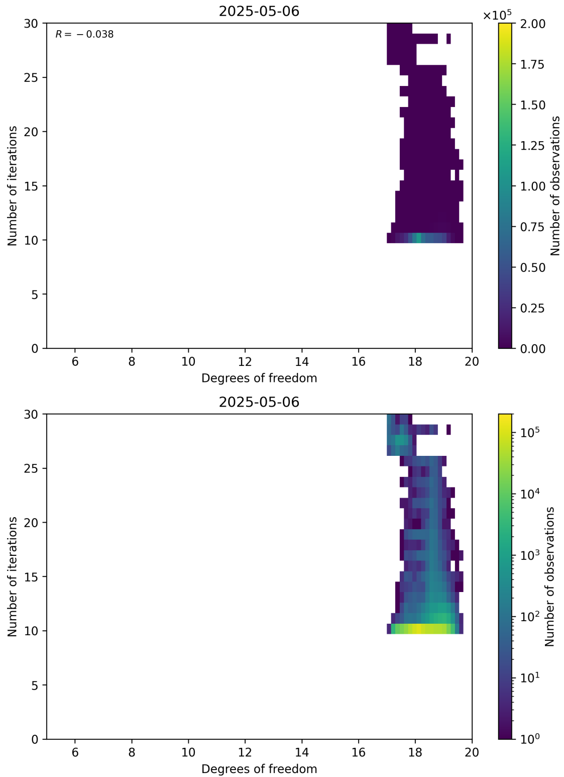
Figure 52: Scatter density plot of “Degrees of freedom” against “Number of iterations” for 2025-05-05 to 2025-05-07.
