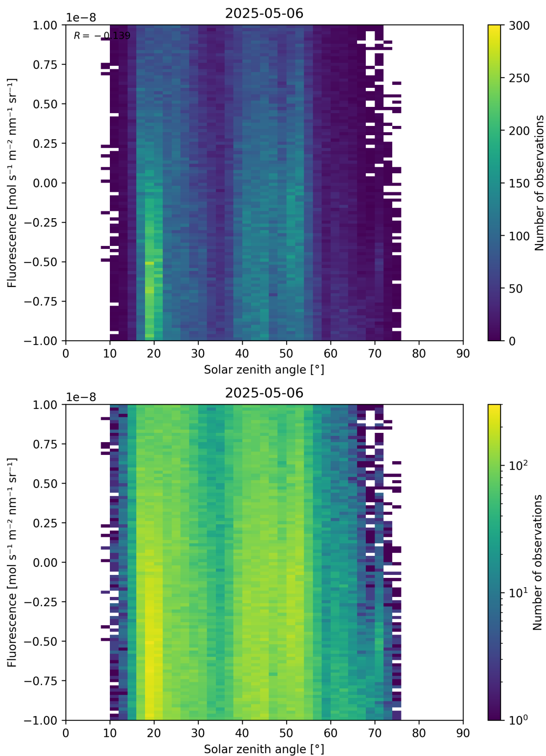
Figure 97: Scatter density plot of “Solar zenith angle” against “Fluorescence” for 2025-05-05 to 2025-05-07.
