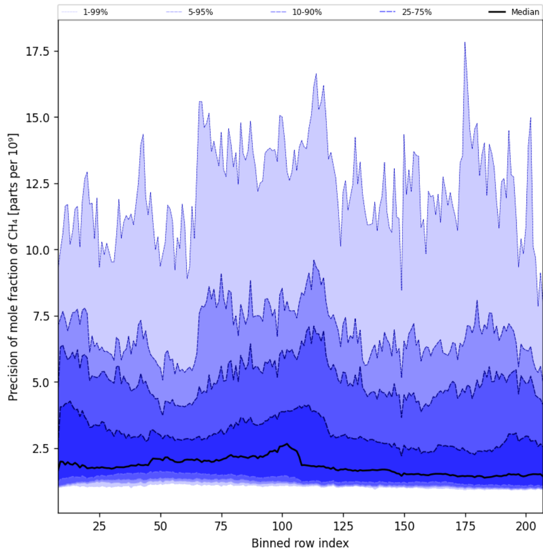
Figure 35: Along track statistics of “Precision of mole fraction of CH 4 ” for 2025-05-05 to 2025-05-07
