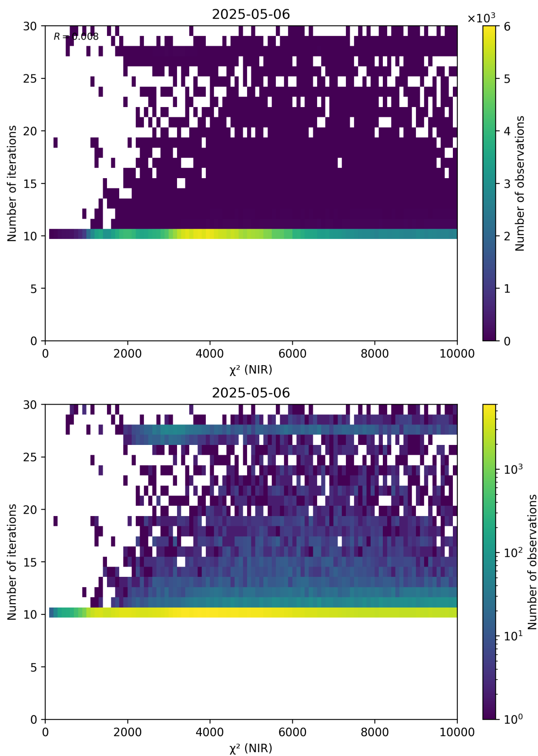
Figure 46: Scatter density plot of “ \chi^2 (NIR)” against “Number of iterations” for 2025-05-05 to 2025-05-07.
