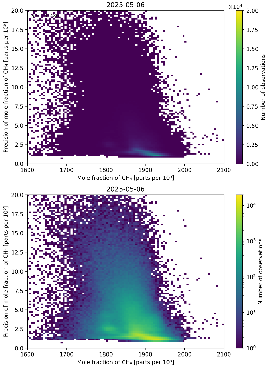
Figure 75: Scatter density plot of “Mole fraction of CH 4 ” against “Precision of mole fraction of CH 4 ” for 2025-05-05 to 2025-05-07.
