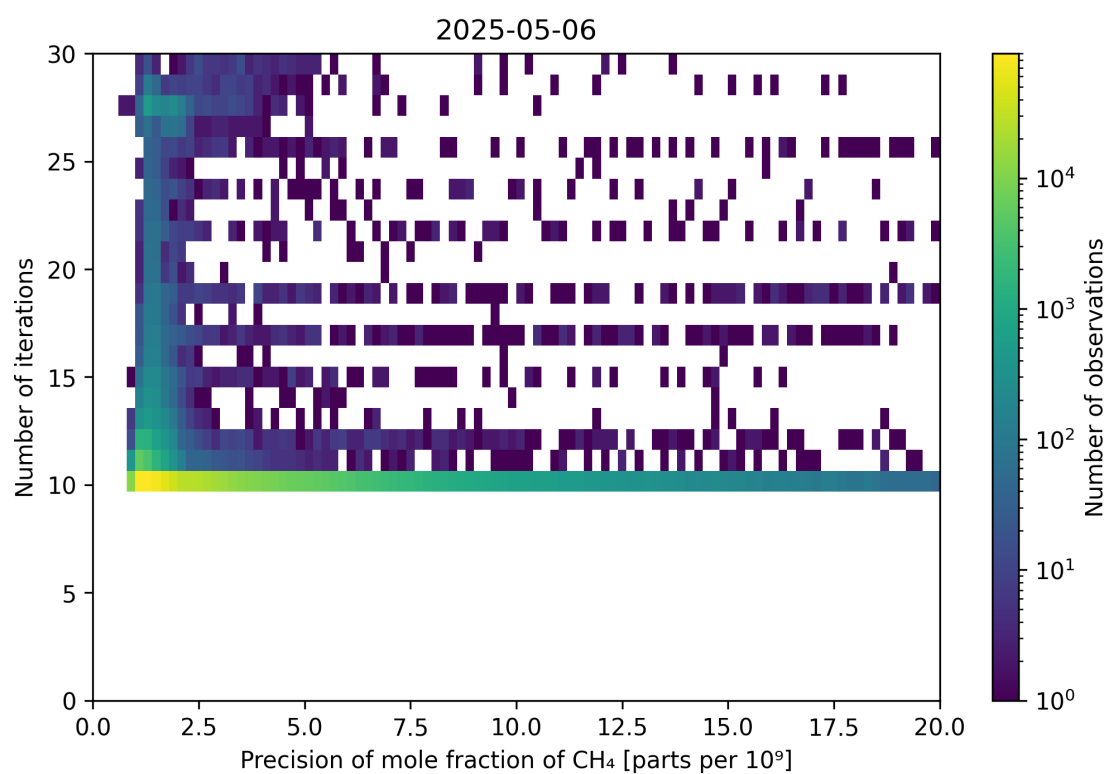
Figure 83: Scatter density plot of “Precision of mole fraction of CH 4 ” against “Number of iterations” for 2025-05-05 to 2025-05-07.
