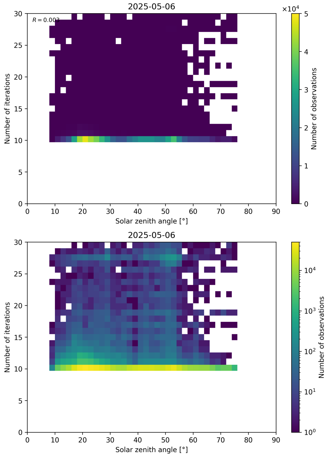
Figure 102: Scatter density plot of “Solar zenith angle” against “Number of iterations” for 2025-05-05 to 2025-05-07.
