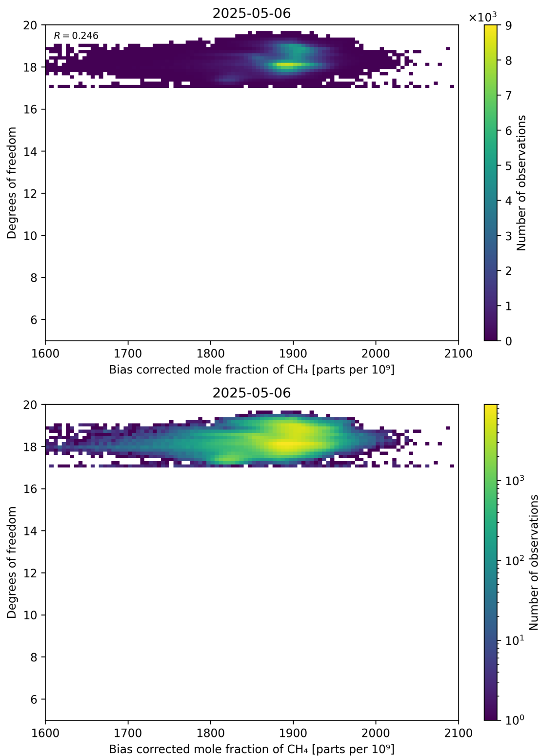
Figure 65: Scatter density plot of “Bias corrected mole fraction of CH 4 ” against “Degrees of freedom” for 2025-05-05 to 2025-05-07.
