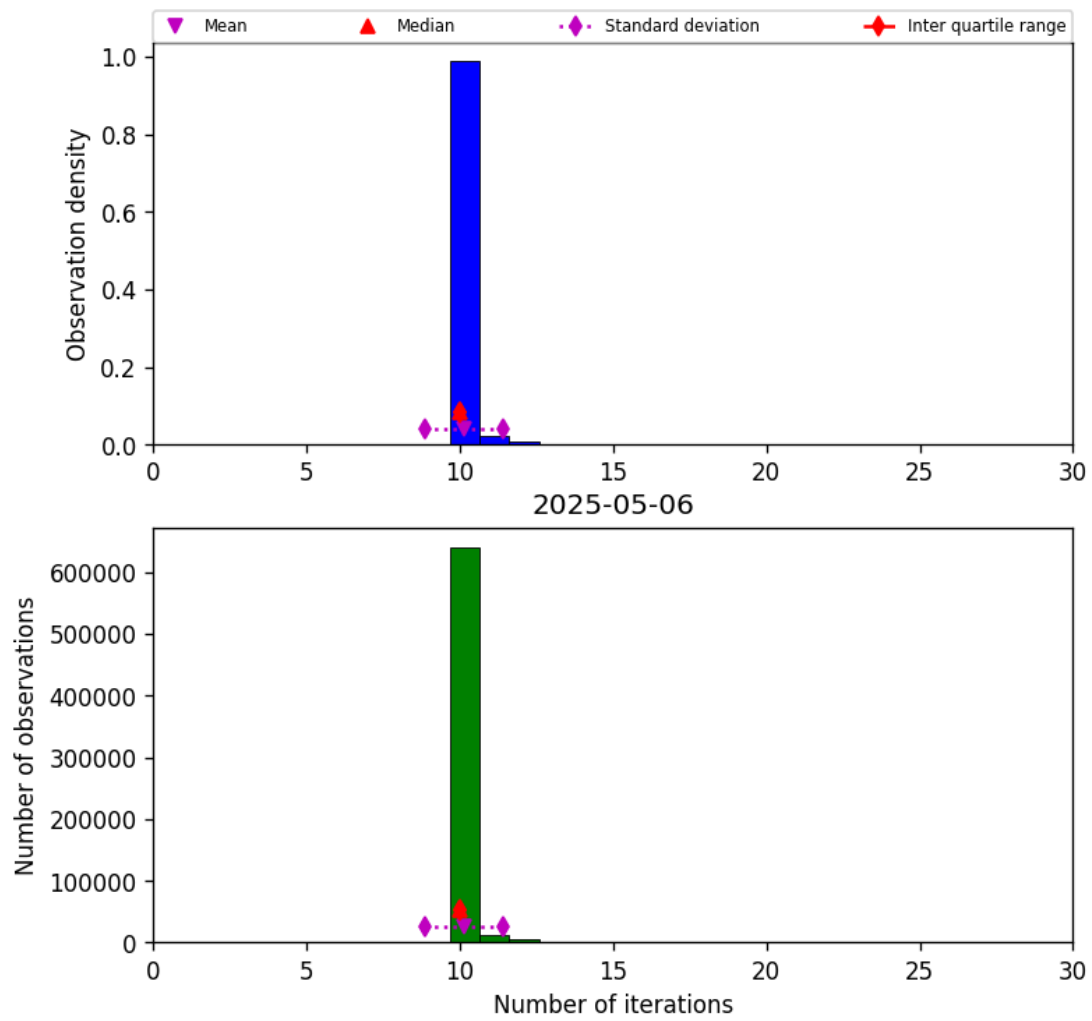
Figure 31: Histogram of “Number of iterations” for 2025-05-05 to 2025-05-07
