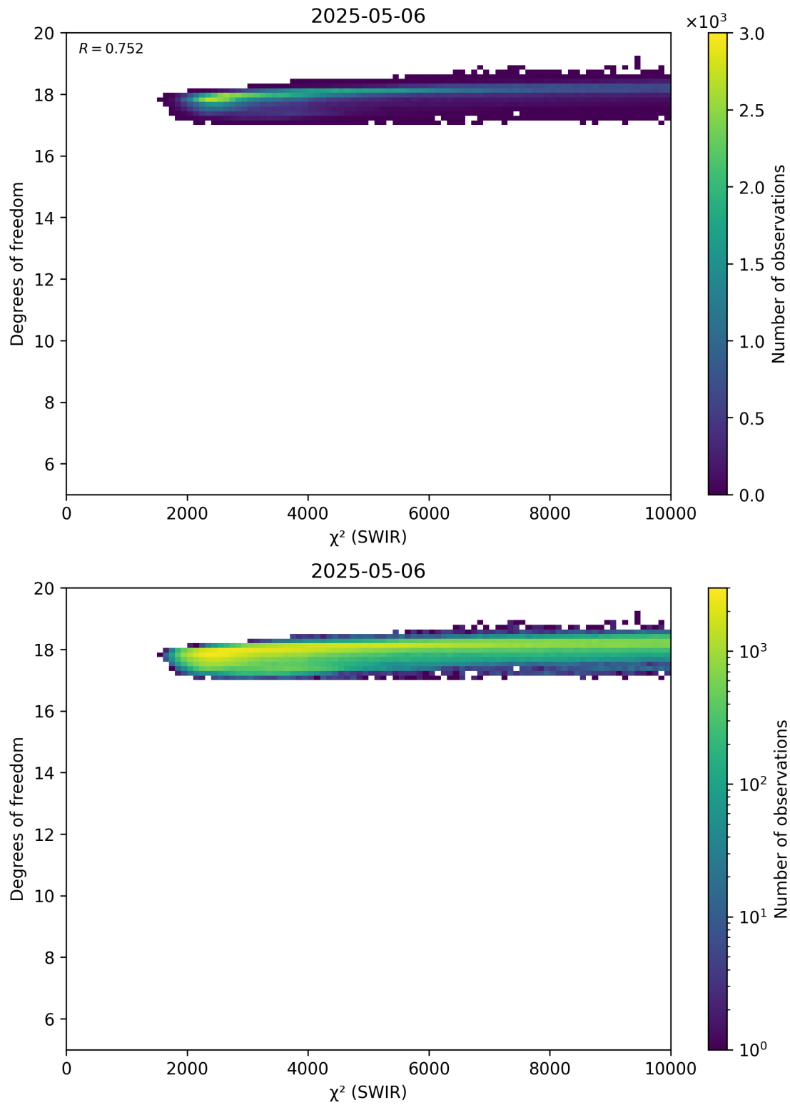
Figure 48: Scatter density plot of “ \chi^2 (SWIR)” against “Degrees of freedom” for 2025-05-05 to 2025-05-07.
