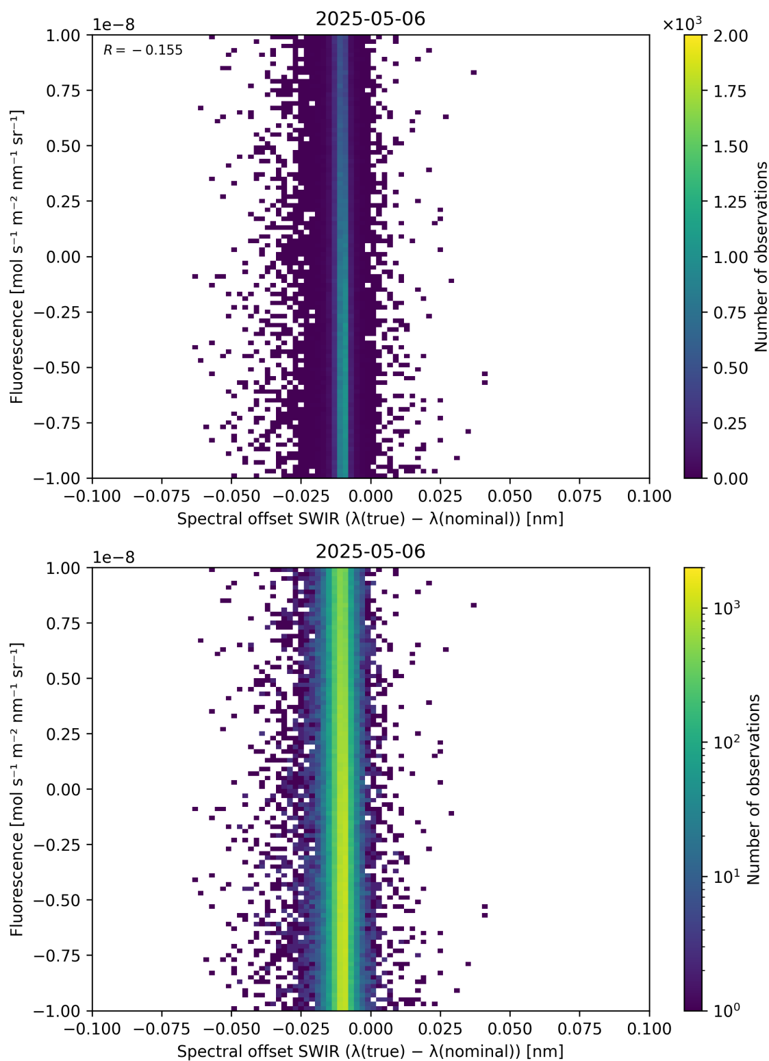
Figure 120: Scatter density plot of “Spectral offset SWIR ( \lambda_{\text{true}} - \lambda_{\text{nominal}} )” against “Fluorescence” for 2025-05-05 to 2025-05-07.
