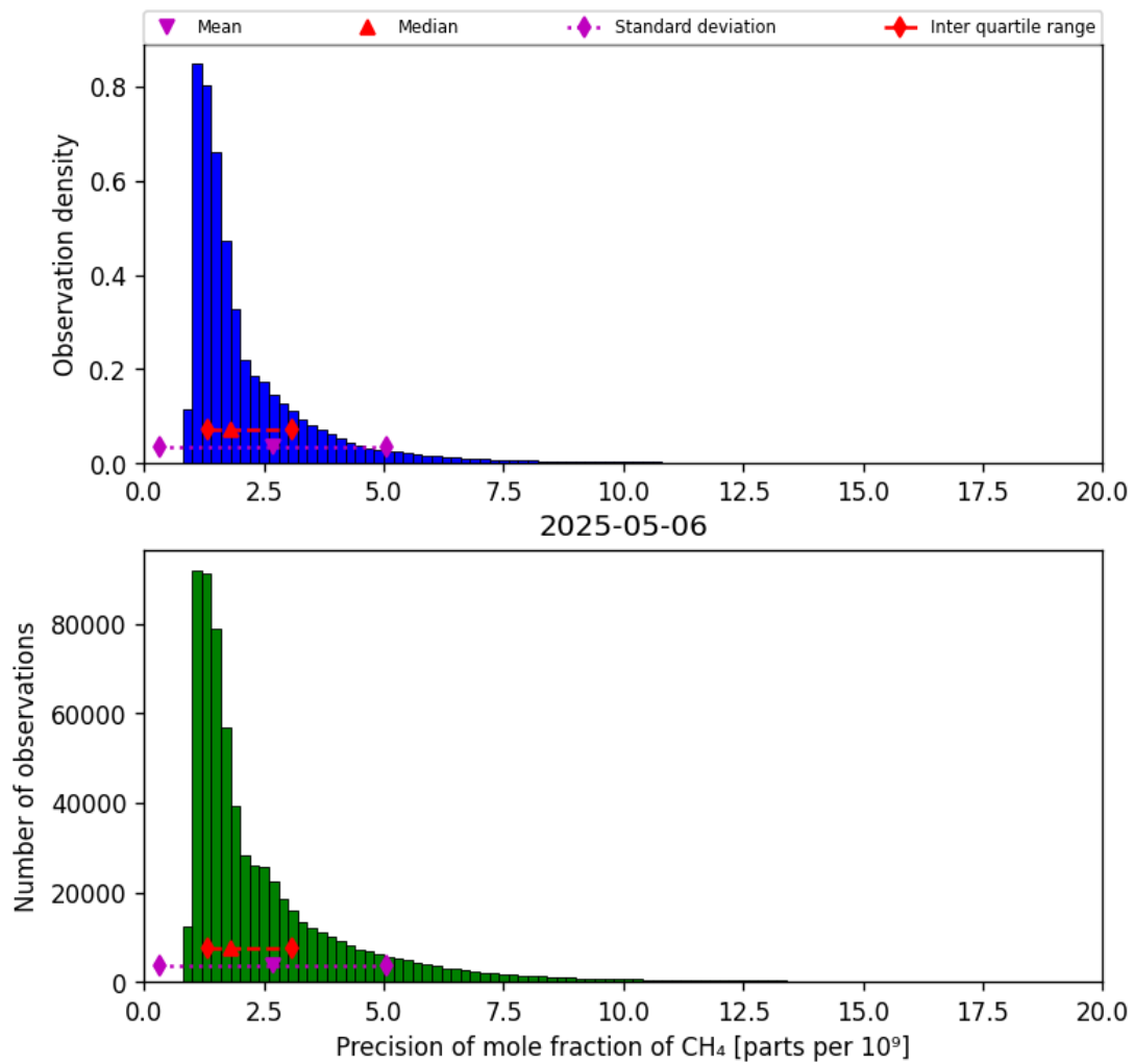
Figure 24: Histogram of “Precision of mole fraction of CH 4 ” for 2025-05-05 to 2025-05-07
