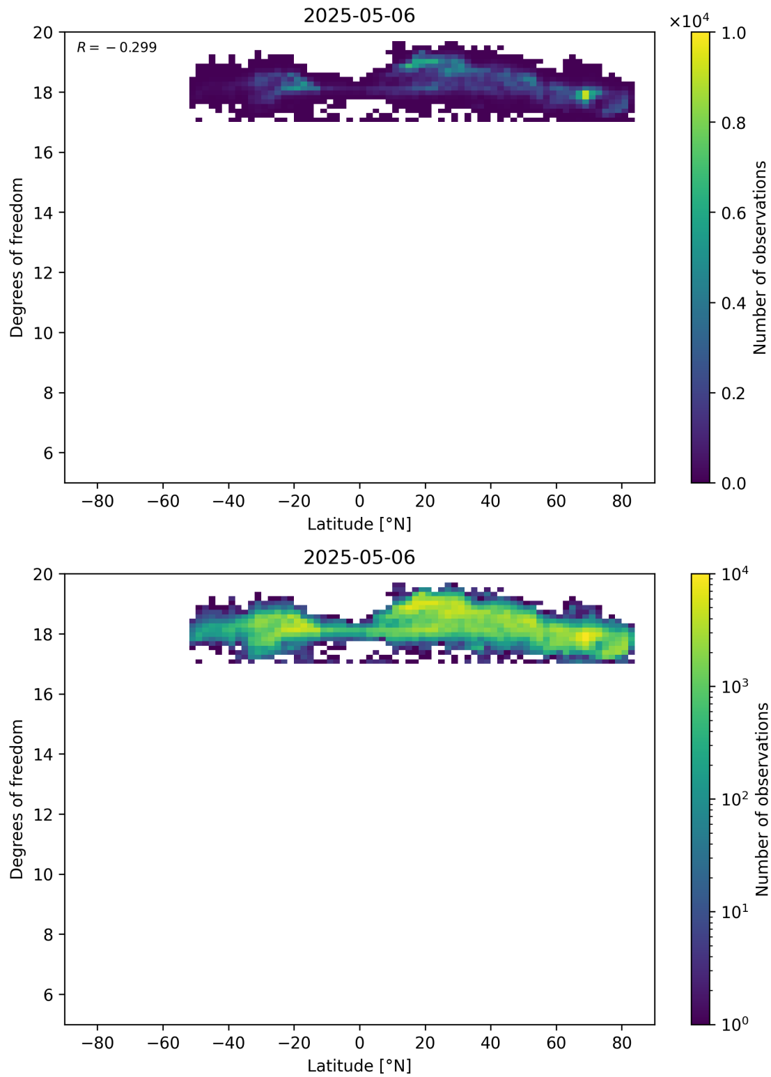
Figure 55: Scatter density plot of “Latitude” against “Degrees of freedom” for 2025-05-05 to 2025-05-07.
