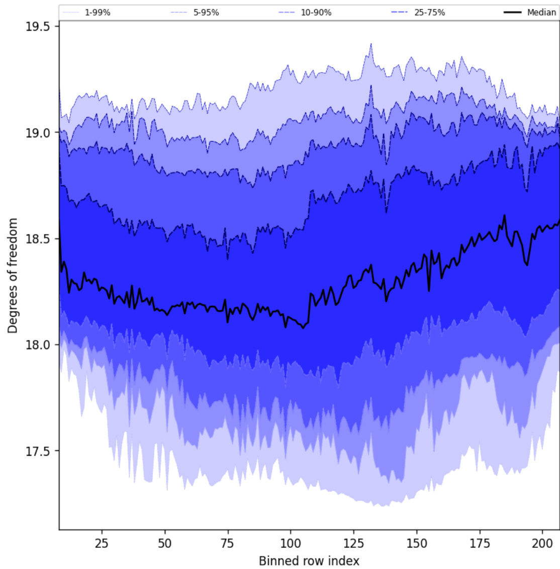
Figure 41: Along track statistics of “Degrees of freedom” for 2025-05-05 to 2025-05-07
