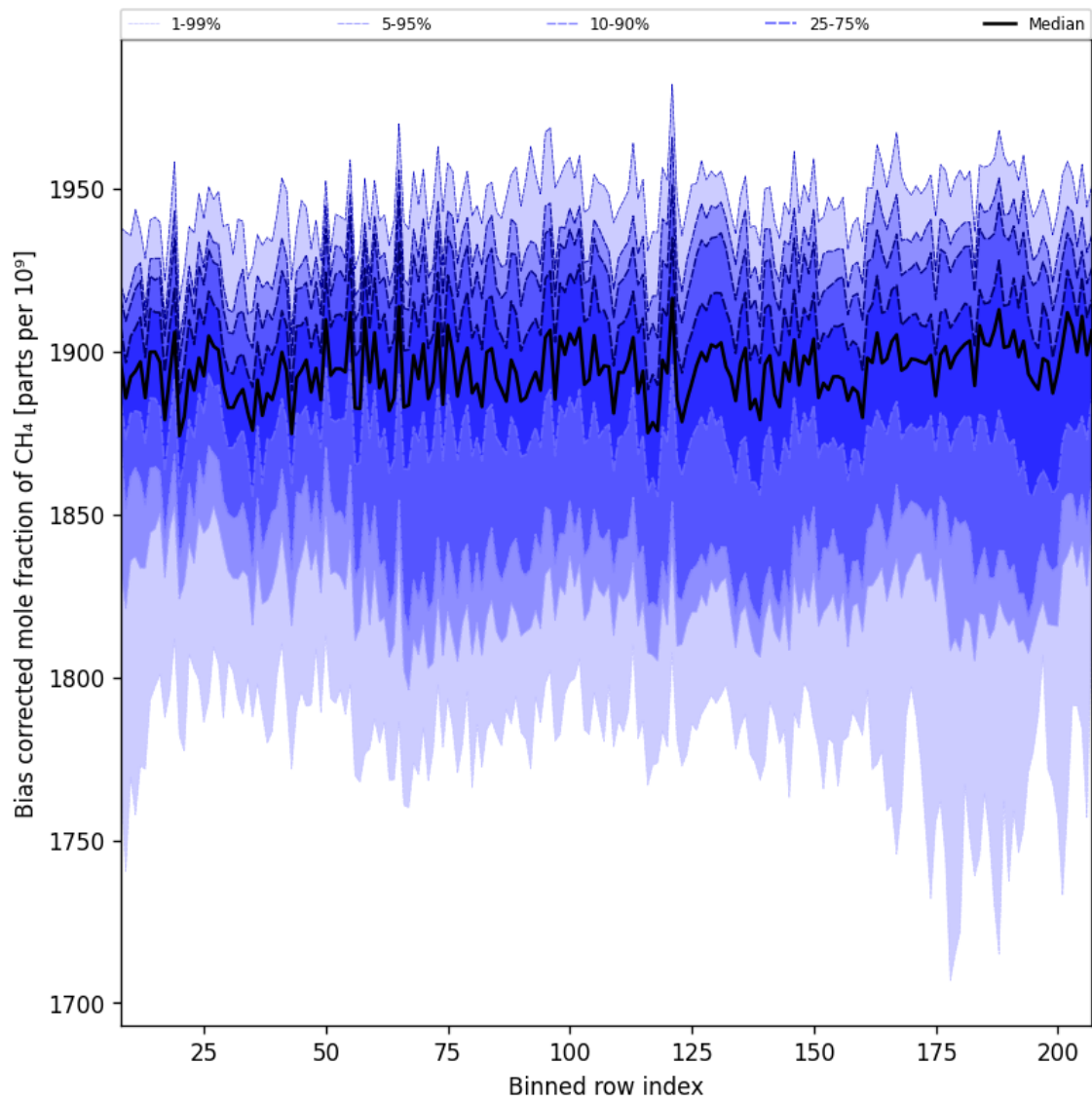
Figure 36: Along track statistics of “Bias corrected mole fraction of CH 4 ” for 2025-05-05 to 2025-05-07
