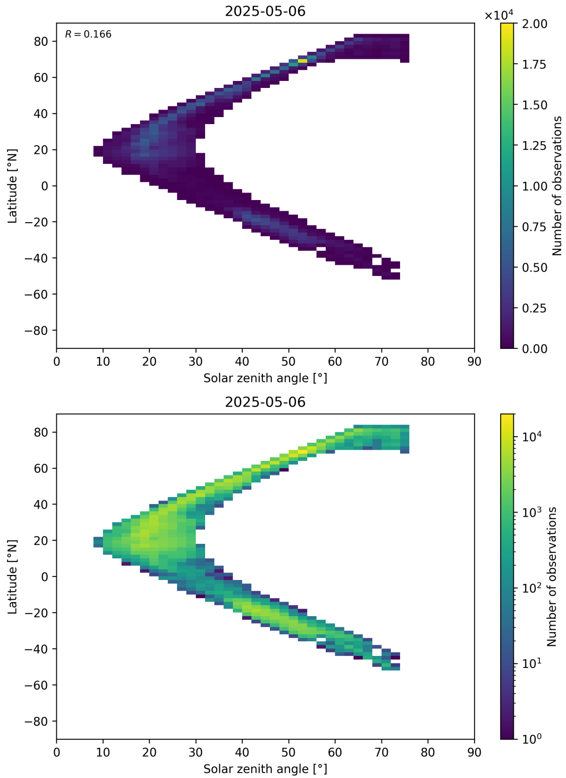
Figure 98: Scatter density plot of “Solar zenith angle” against “Latitude” for 2025-05-05 to 2025-05-07.
