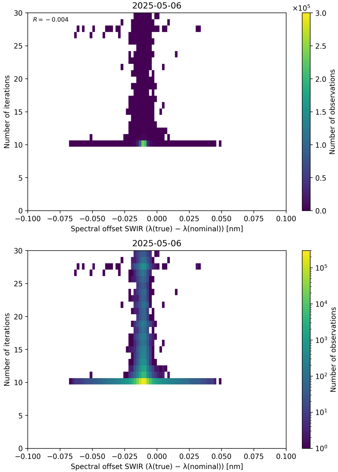
Figure 121: Scatter density plot of “Spectral offset SWIR ( \lambda_{\text{true}} - \lambda_{\text{nominal}} )” against “Number of iterations” for 2025-05-05 to 2025-05-07.
