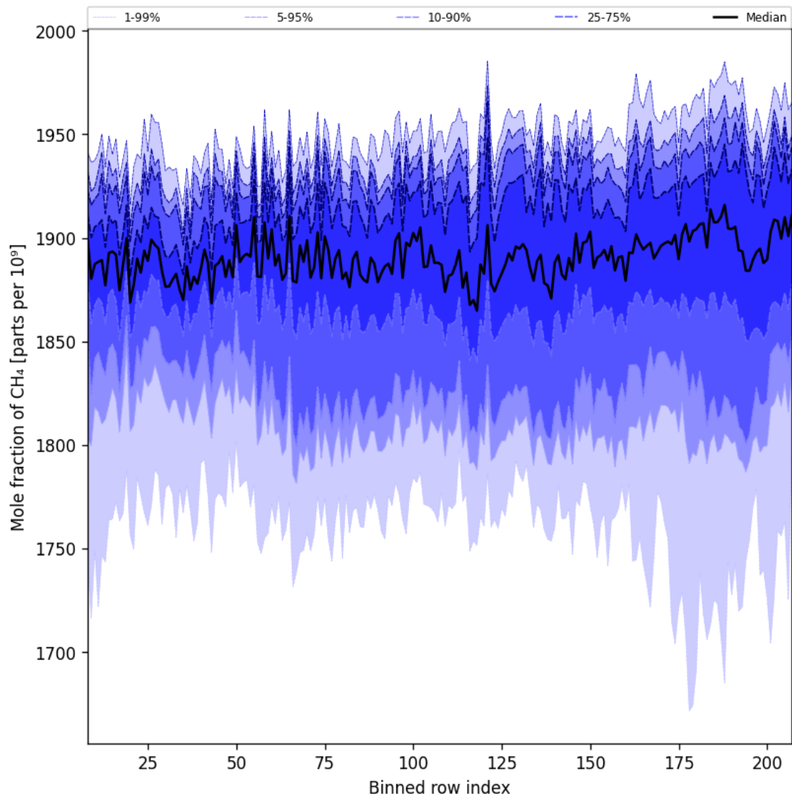
Figure 34: Along track statistics of “Mole fraction of CH 4 ” for 2025-05-05 to 2025-05-07
