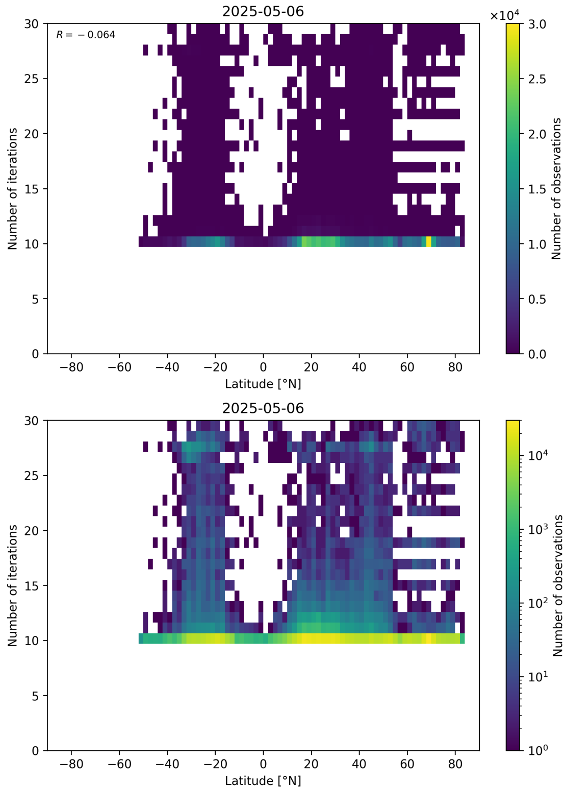
Figure 60: Scatter density plot of “Latitude” against “Number of iterations” for 2025-05-05 to 2025-05-07.
