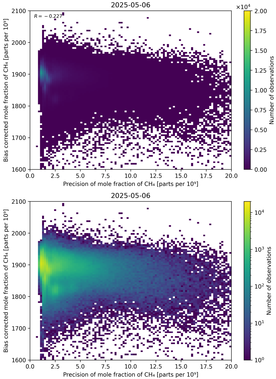
Figure 82: Scatter density plot of “Precision of mole fraction of CH 4 ” against “Bias corrected mole fraction of CH 4 ” for 2025-05-05 to 2025-05-07.
