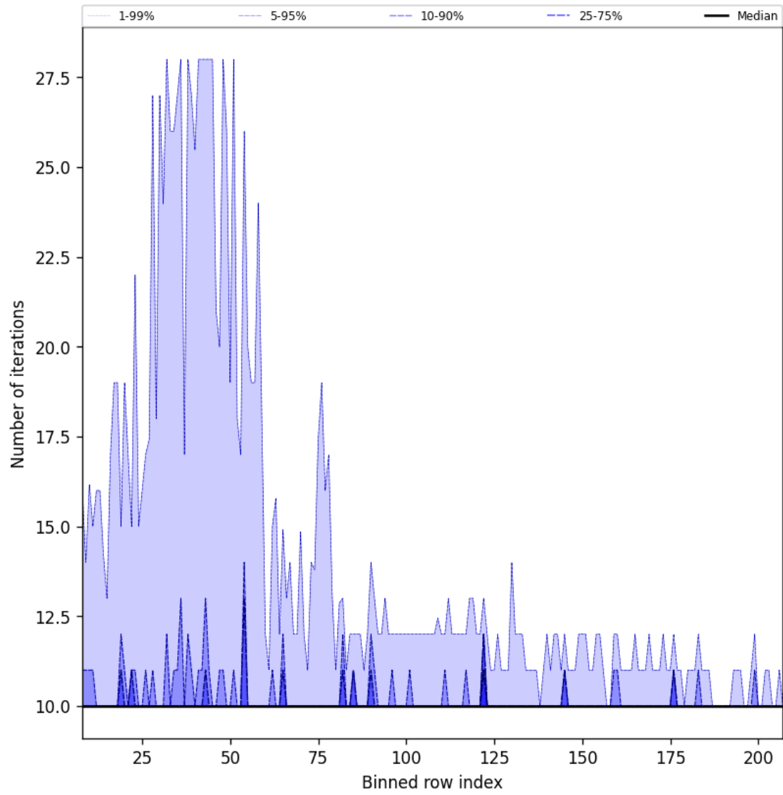
Figure 42: Along track statistics of “Number of iterations” for 2025-05-05 to 2025-05-07
