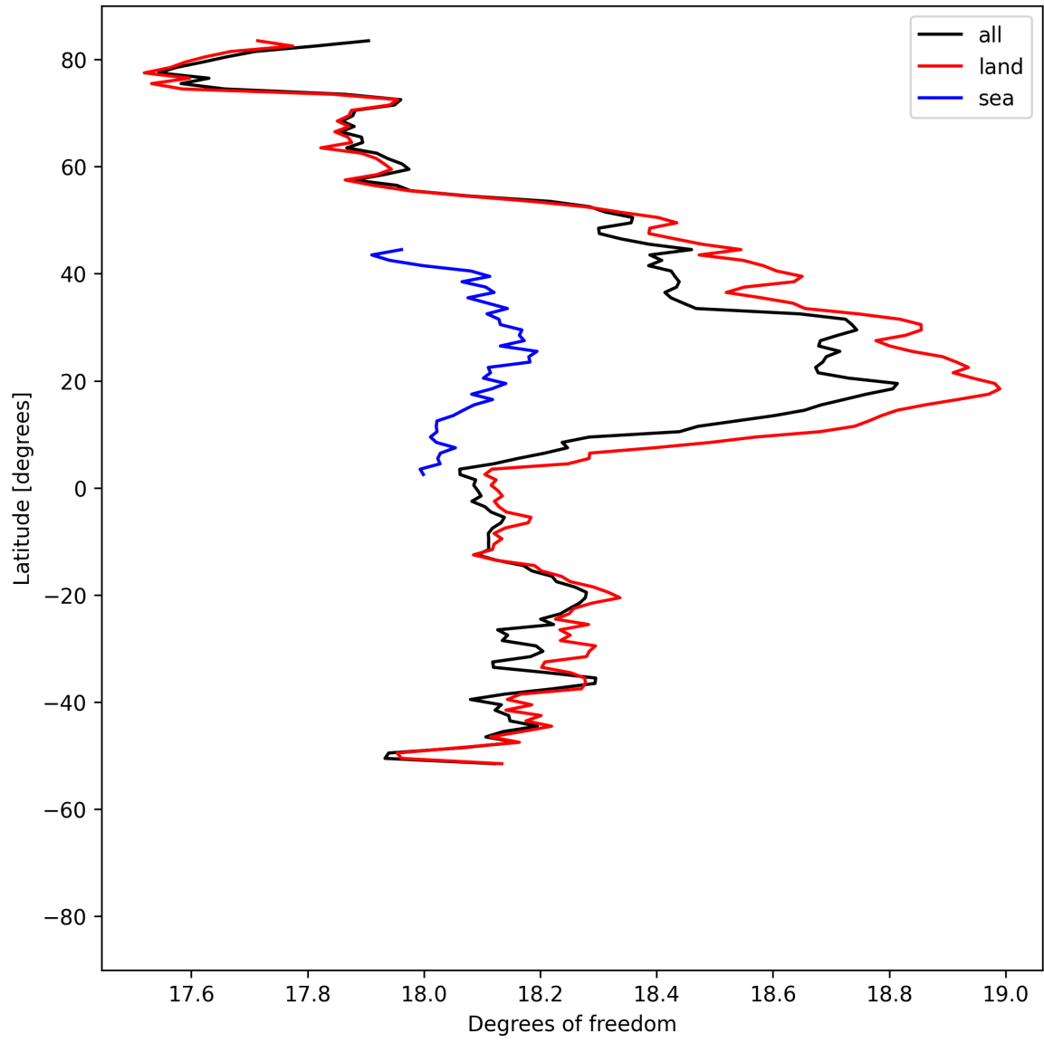
Figure 19: Zonal average of “Degrees of freedom” for 2025-05-05 to 2025-05-07.
