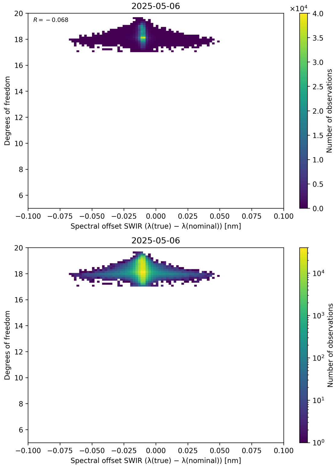
Figure 119: Scatter density plot of “Spectral offset SWIR ( \lambda_{\text{true}} - \lambda_{\text{nominal}} )” against “Degrees of freedom” for 2025-05-05 to 2025-05-07.
