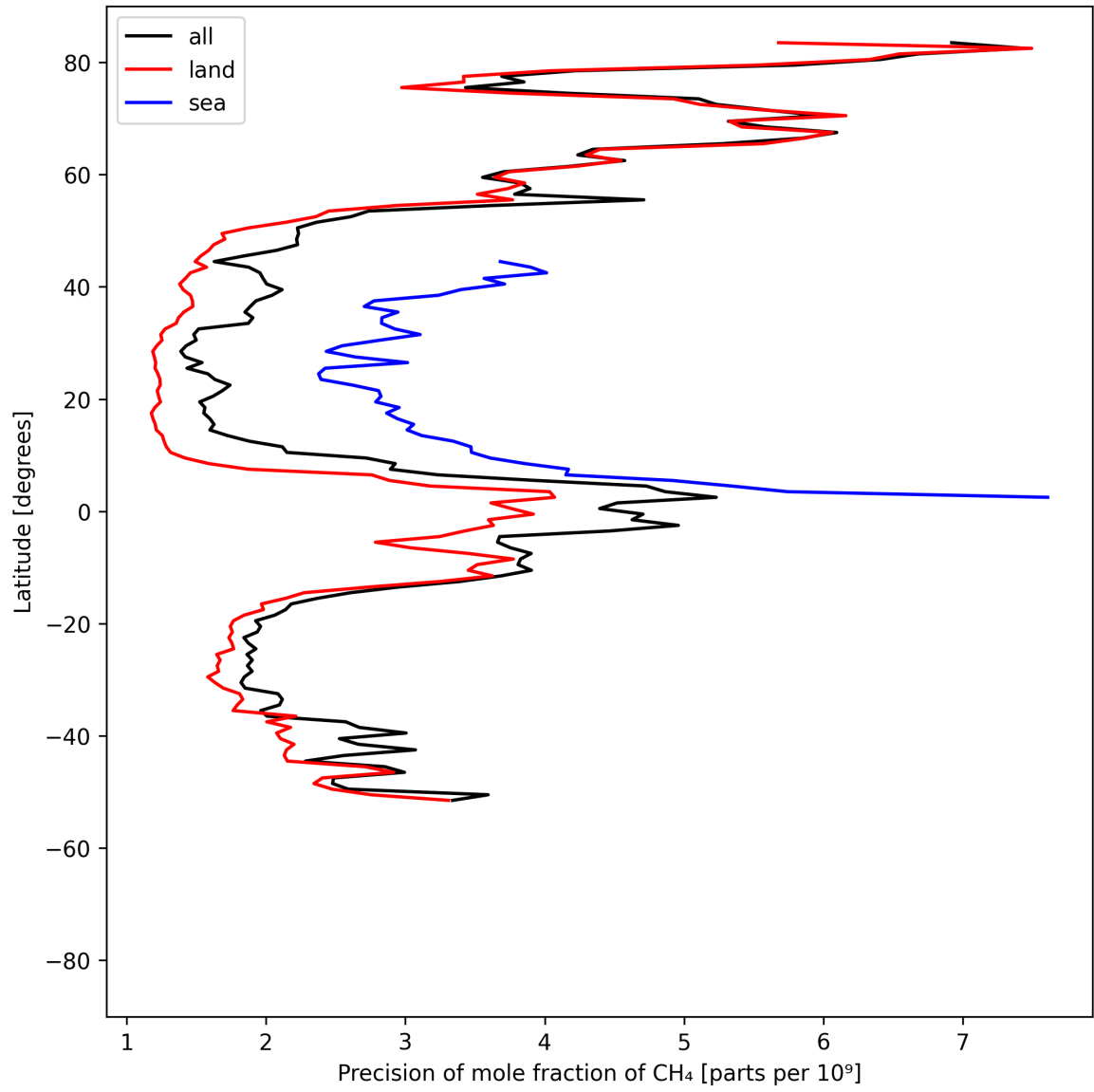
Figure 13: Zonal average of “Precision of mole fraction of CH 4 ” for 2025-05-05 to 2025-05-07.
