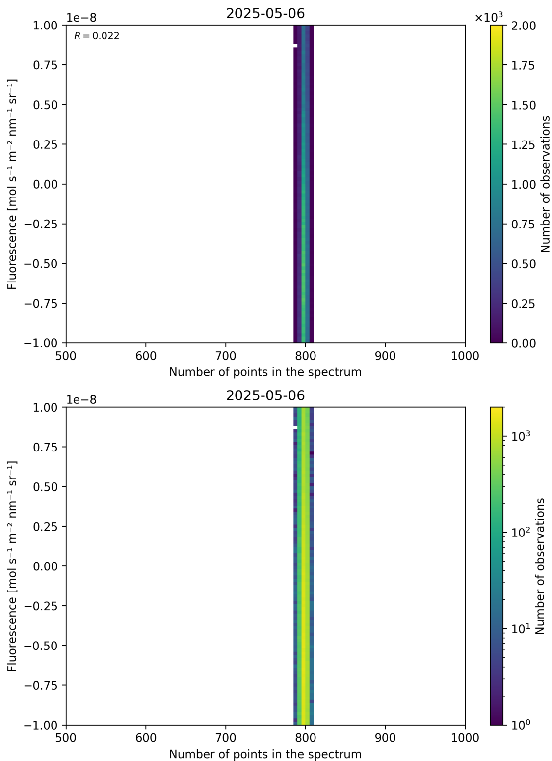
Figure 91: Scatter density plot of “Number of points in the spectrum” against “Fluorescence” for 2025-05-05 to 2025-05-07.
