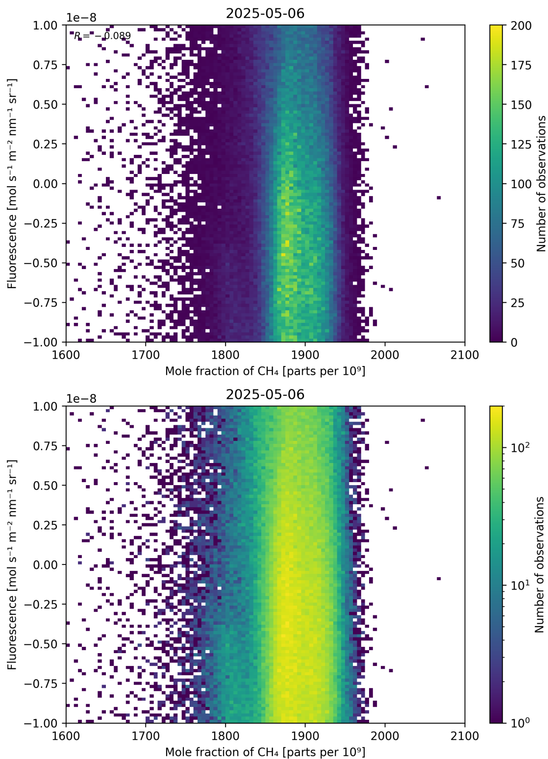
Figure 73: Scatter density plot of “Mole fraction of \text{CH}_4 ” against “Fluorescence” for 2025-05-05 to 2025-05-07.
