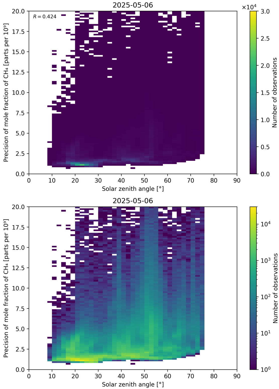
Figure 101: Scatter density plot of “Solar zenith angle” against “Precision of mole fraction of CH 4 ” for 2025-05-05 to 2025-05-07.
