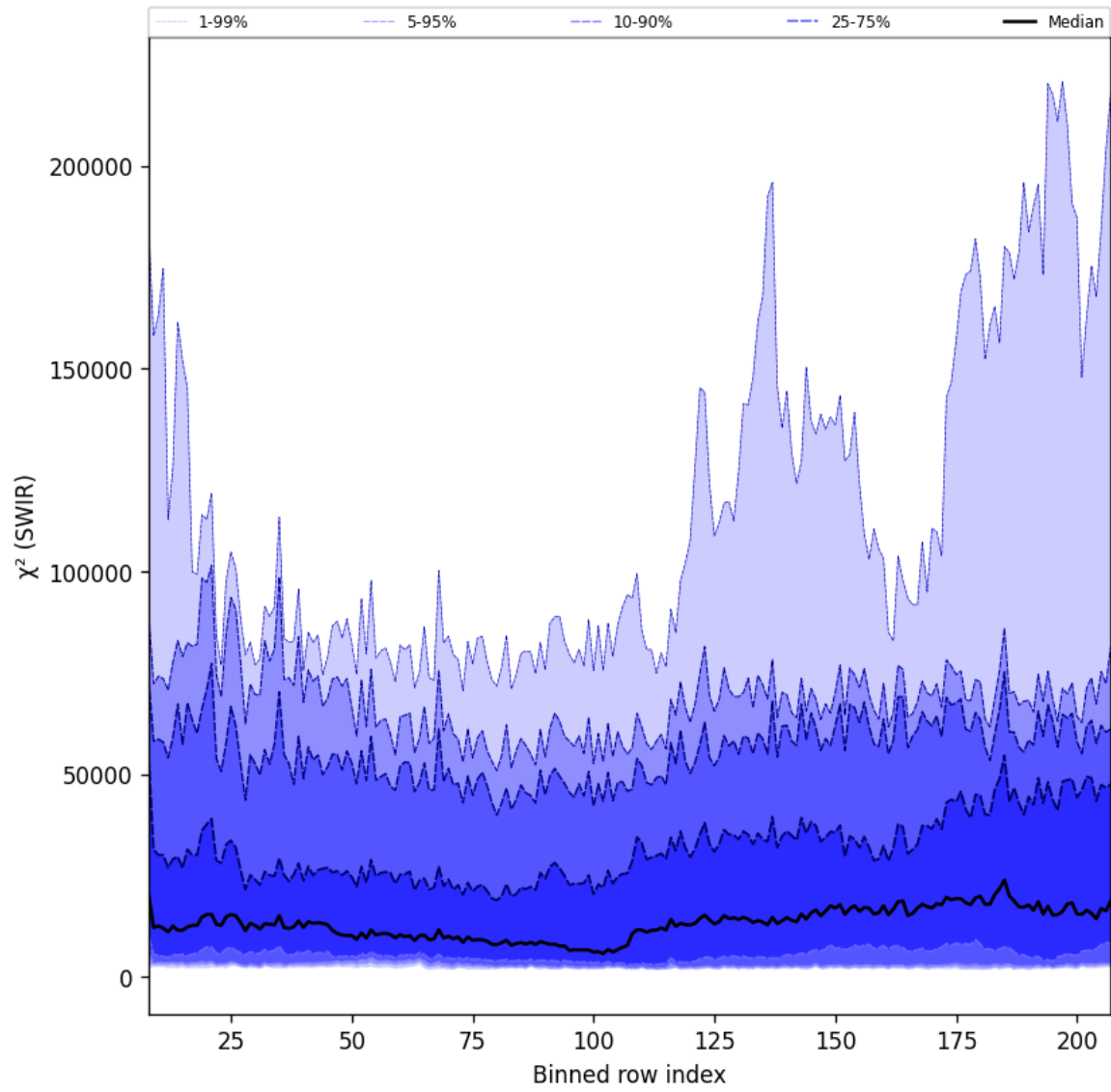
Figure 39: Along track statistics of “ \chi^2 (SWIR)” for 2025-05-05 to 2025-05-07
