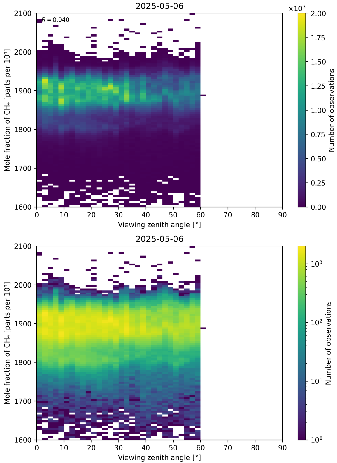
Figure 110: Scatter density plot of “Viewing zenith angle” against “Mole fraction of CH 4 ” for 2025-05-05 to 2025-05-07.
