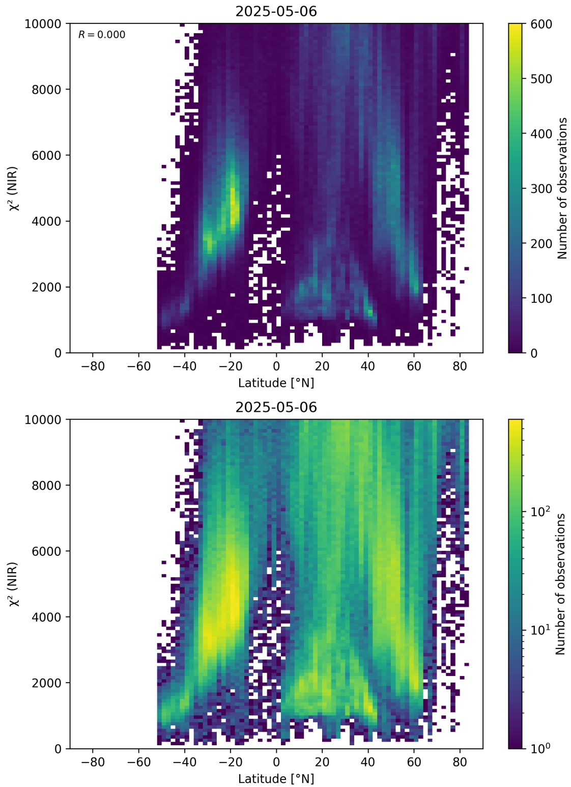
Figure 53: Scatter density plot of “Latitude” against “ \chi^2 (NIR)” for 2025-05-05 to 2025-05-07.
