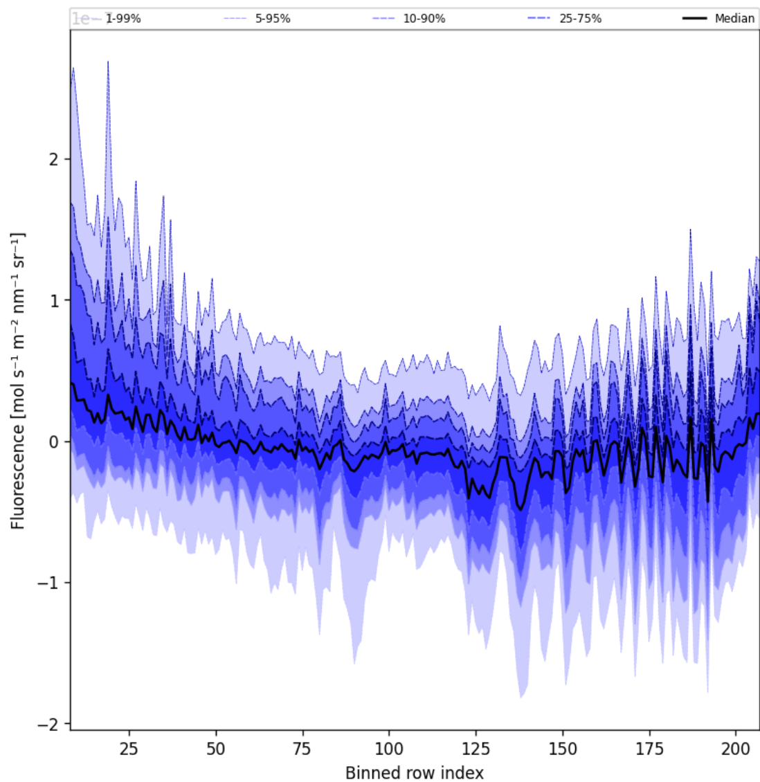
Figure 43: Along track statistics of “Fluorescence” for 2025-05-05 to 2025-05-07
