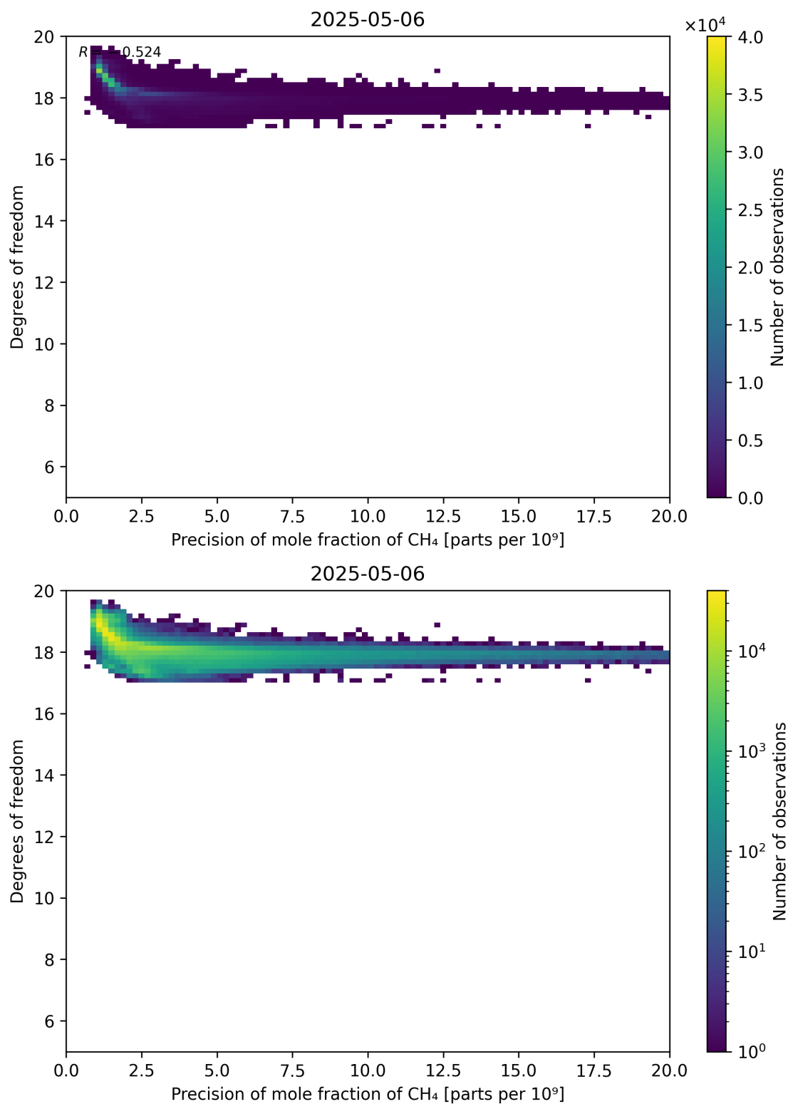
Figure 80: Scatter density plot of “Precision of mole fraction of CH 4 ” against “Degrees of freedom” for 2025-05-05 to 2025-05-07.
