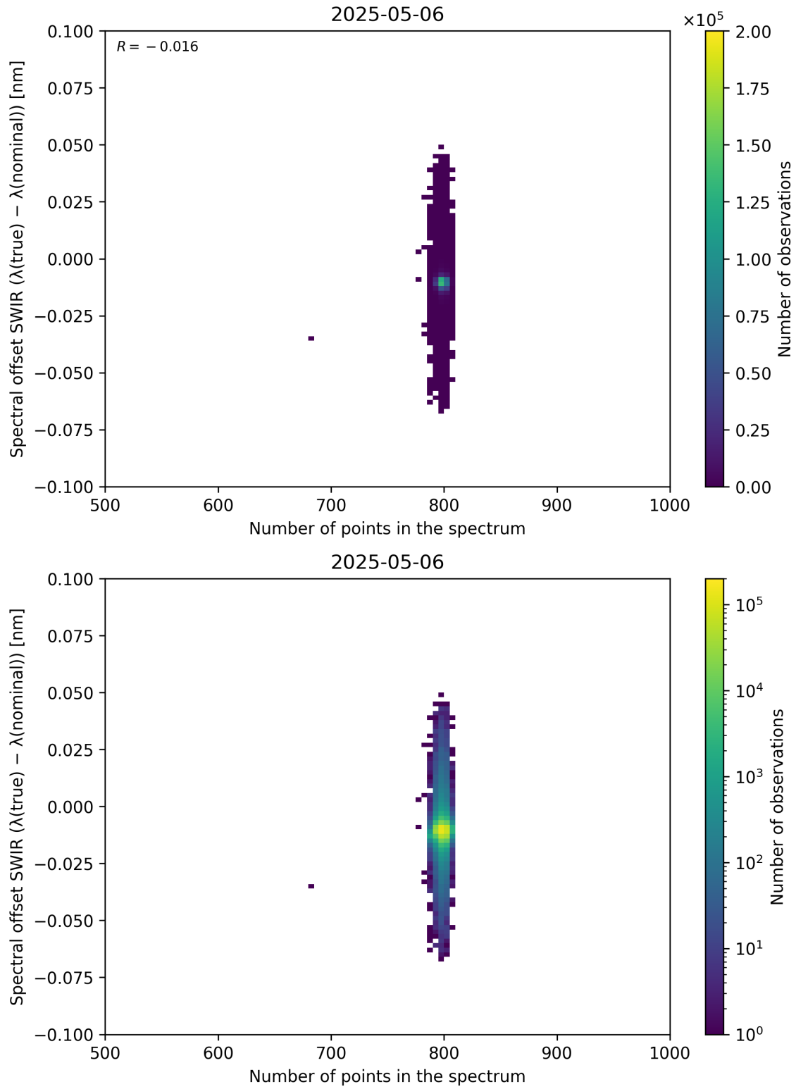
Figure 93: Scatter density plot of “Number of points in the spectrum” against “Spectral offset SWIR ( \lambda_{\text{true}} - \lambda_{\text{nominal}} )” for 2025-05-05 to 2025-05-07.
