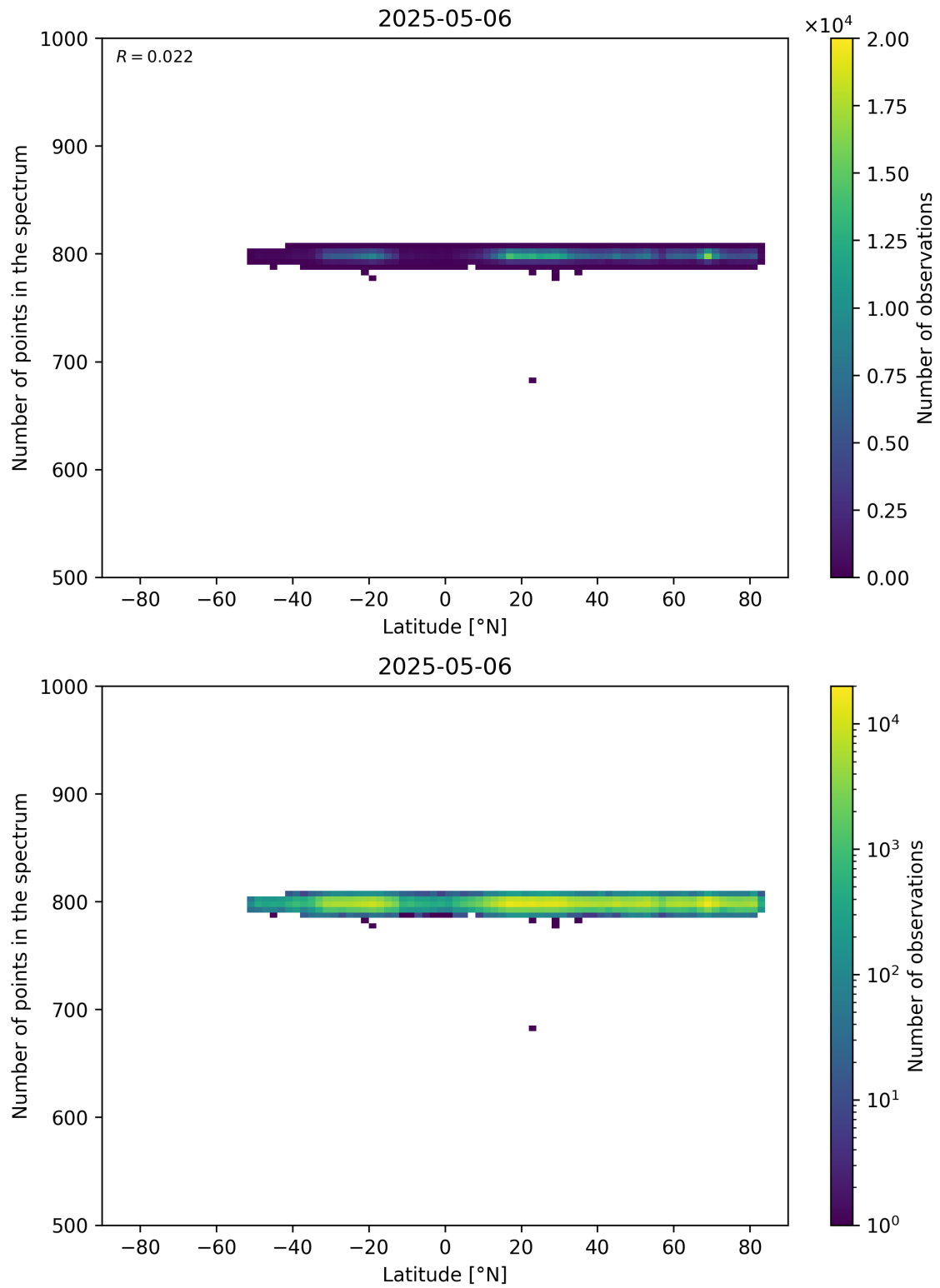
Figure 61: Scatter density plot of “Latitude” against “Number of points in the spectrum” for 2025-05-05 to 2025-05-07.
