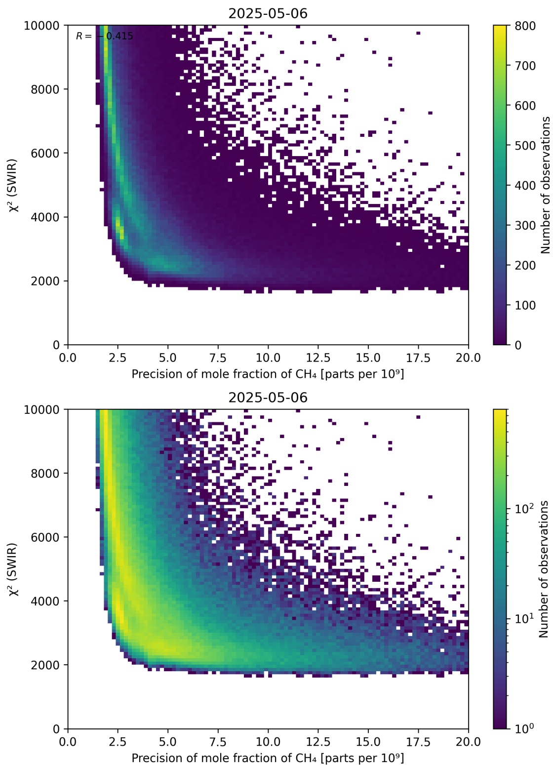
Figure 79: Scatter density plot of “Precision of mole fraction of \text{CH}_4 ” against “ \chi^2 (SWIR)” for 2025-05-05 to 2025-05-07.
