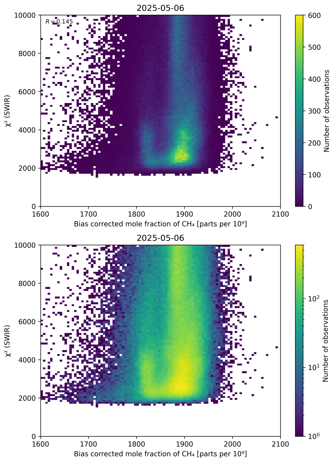
Figure 64: Scatter density plot of “Bias corrected mole fraction of \text{CH}_4 ” against “ \chi^2 (SWIR)” for 2025-05-05 to 2025-05-07.
