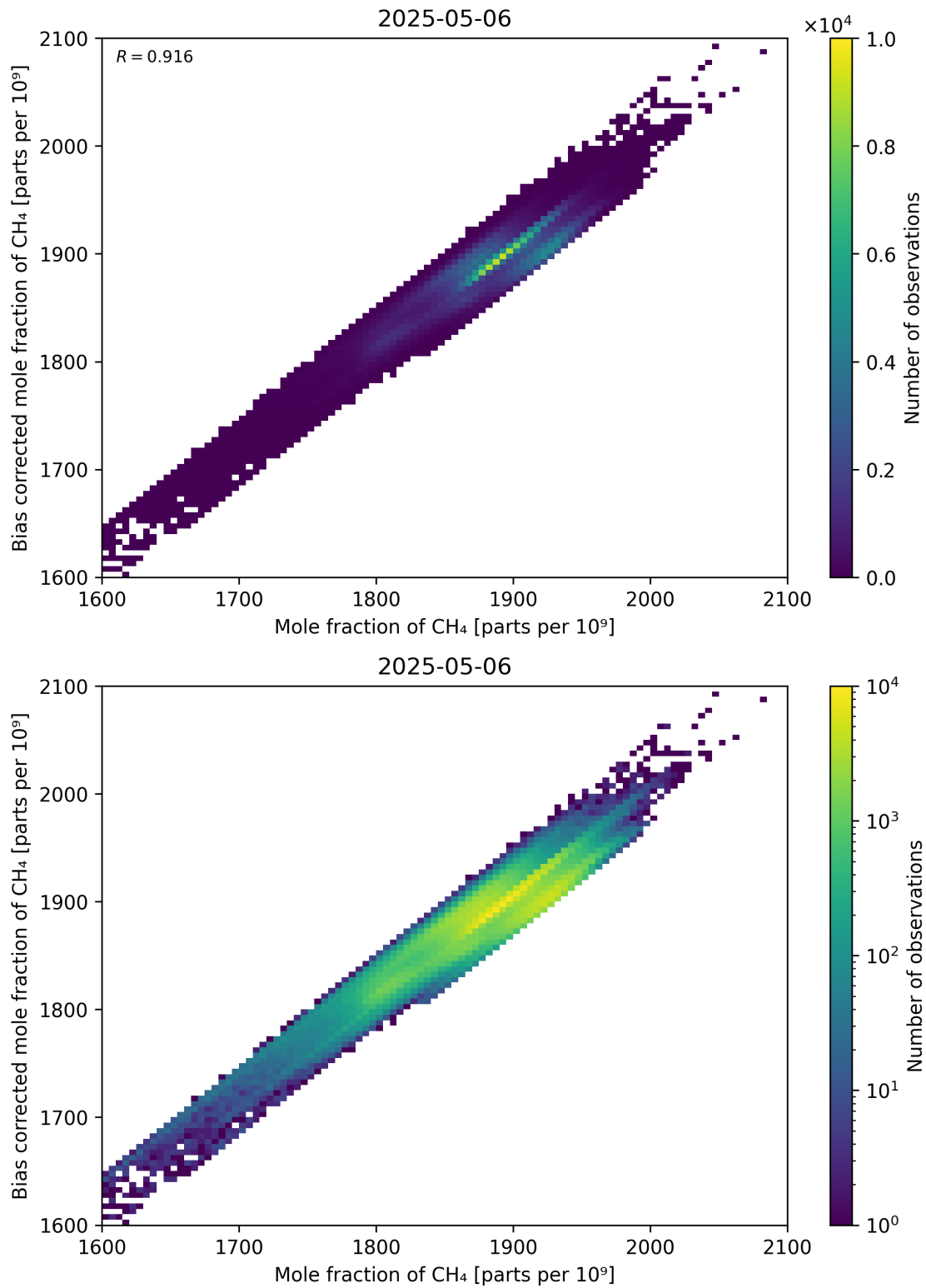
Figure 74: Scatter density plot of “Mole fraction of CH 4 ” against “Bias corrected mole fraction of CH 4 ” for 2025-05-05 to 2025-05-07.
