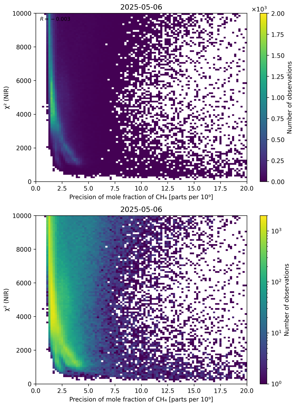
Figure 78: Scatter density plot of “Precision of mole fraction of CH 4 ” against “ \chi^2 (NIR)” for 2025-05-05 to 2025-05-07.
