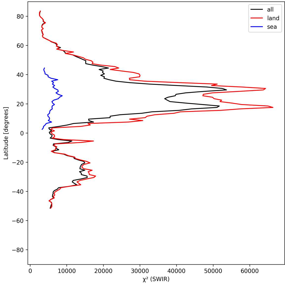
Figure 17: Zonal average of “ \chi^2 (SWIR)” for 2025-05-05 to 2025-05-07.
