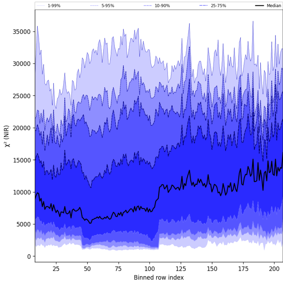
Figure 40: Along track statistics of “ \chi^2 (NIR)” for 2025-05-05 to 2025-05-07
