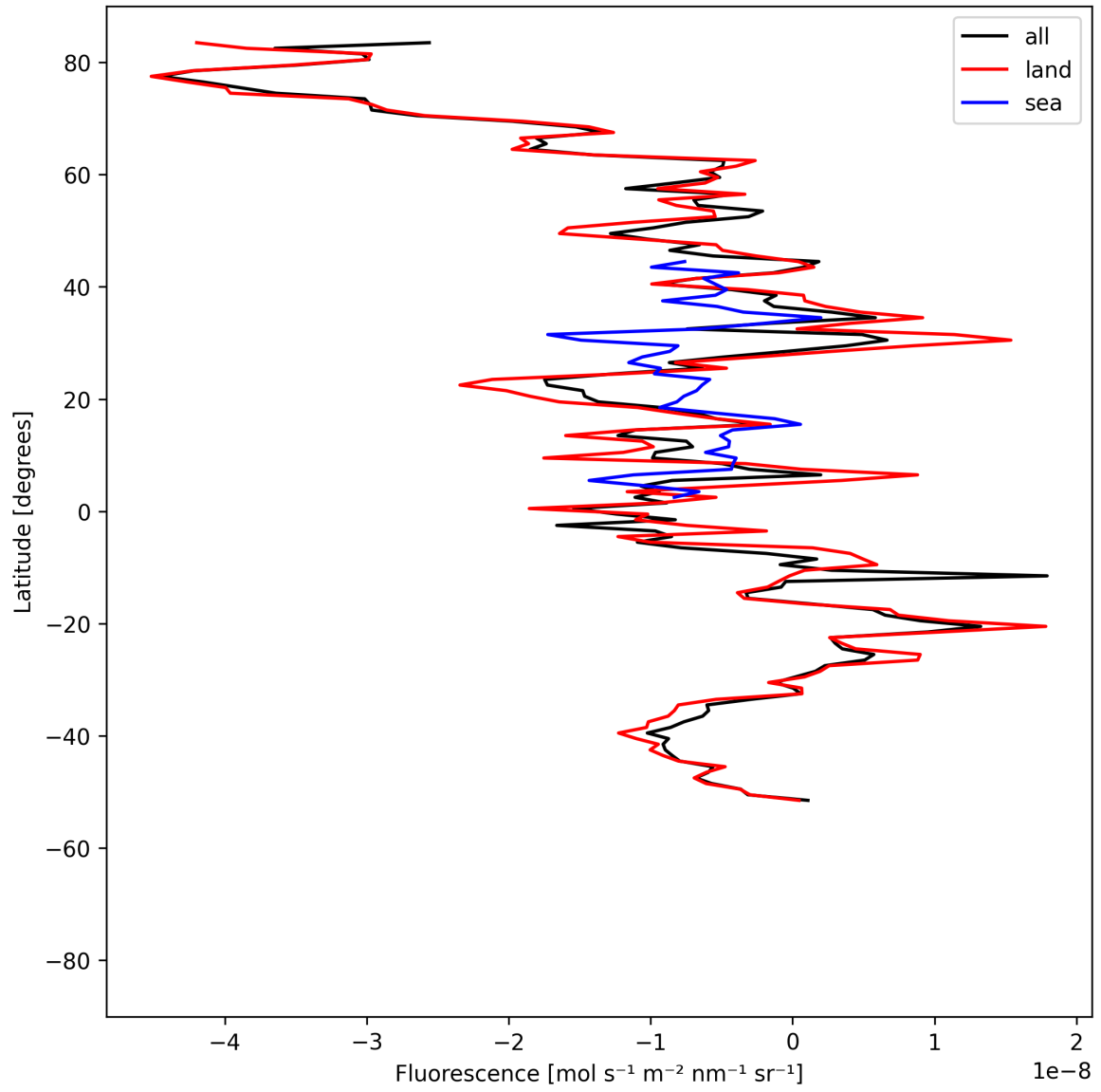
Figure 21: Zonal average of “Fluorescence” for 2025-05-05 to 2025-05-07.
