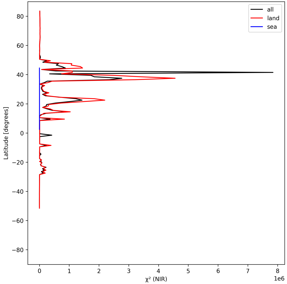
Figure 18: Zonal average of “ \chi^2 (NIR)” for 2025-05-05 to 2025-05-07.
