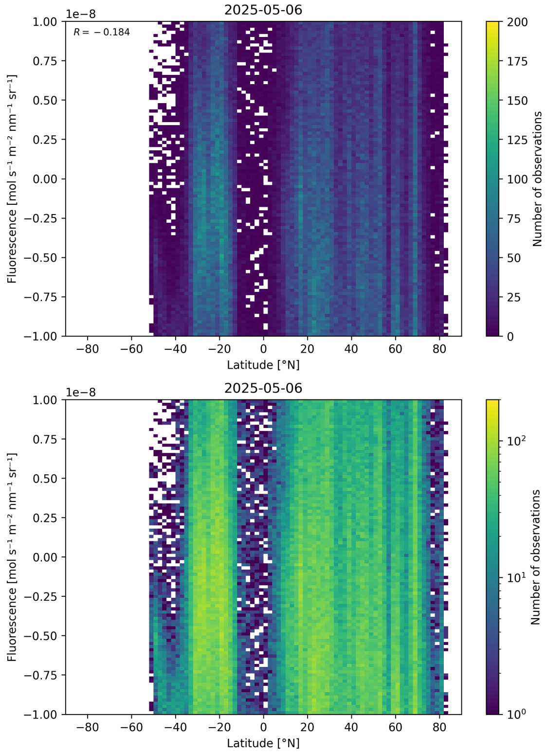
Figure 56: Scatter density plot of “Latitude” against “Fluorescence” for 2025-05-05 to 2025-05-07.
