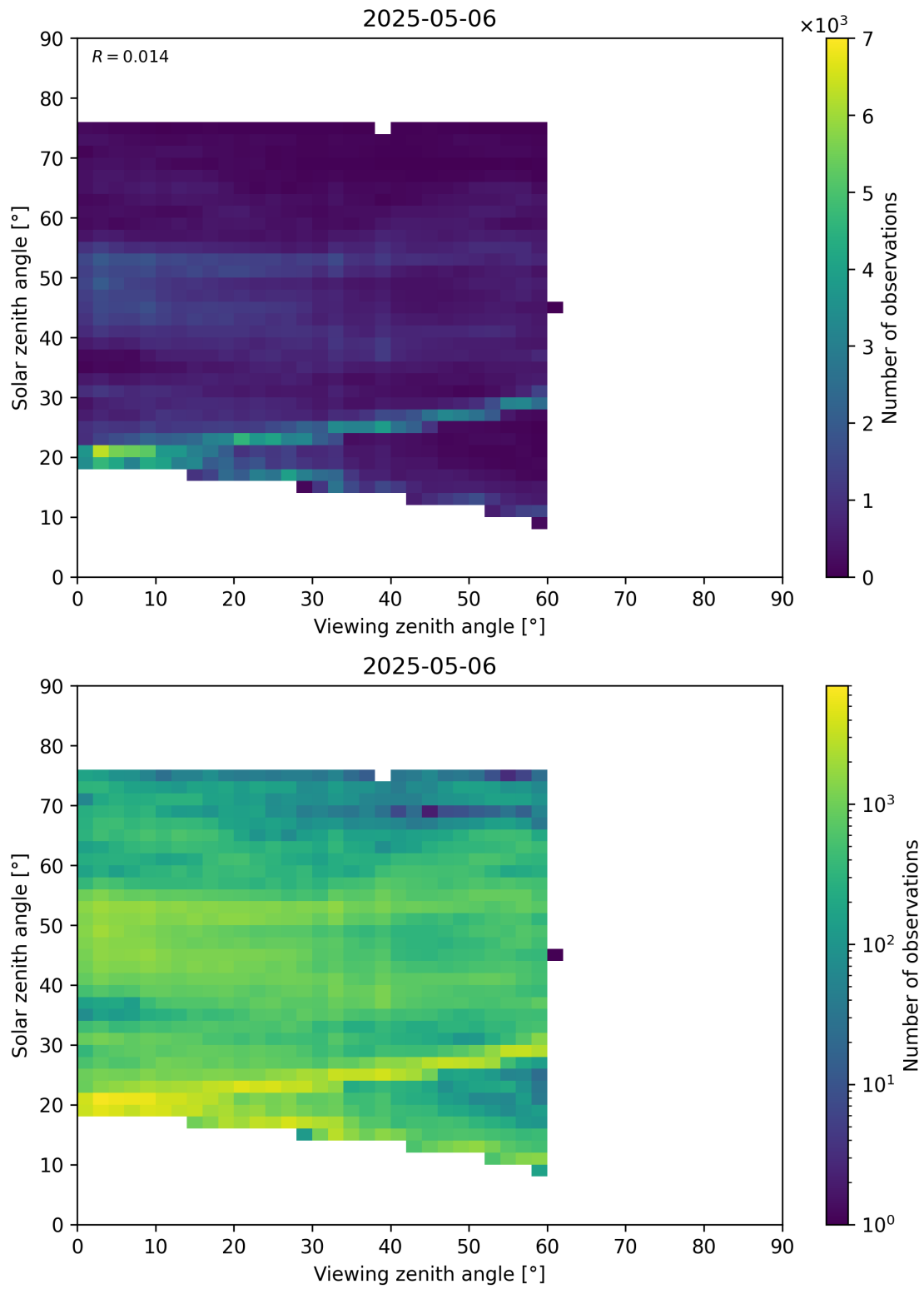
Figure 115: Scatter density plot of “Viewing zenith angle” against “Solar zenith angle” for 2025-05-05 to 2025-05-07.
