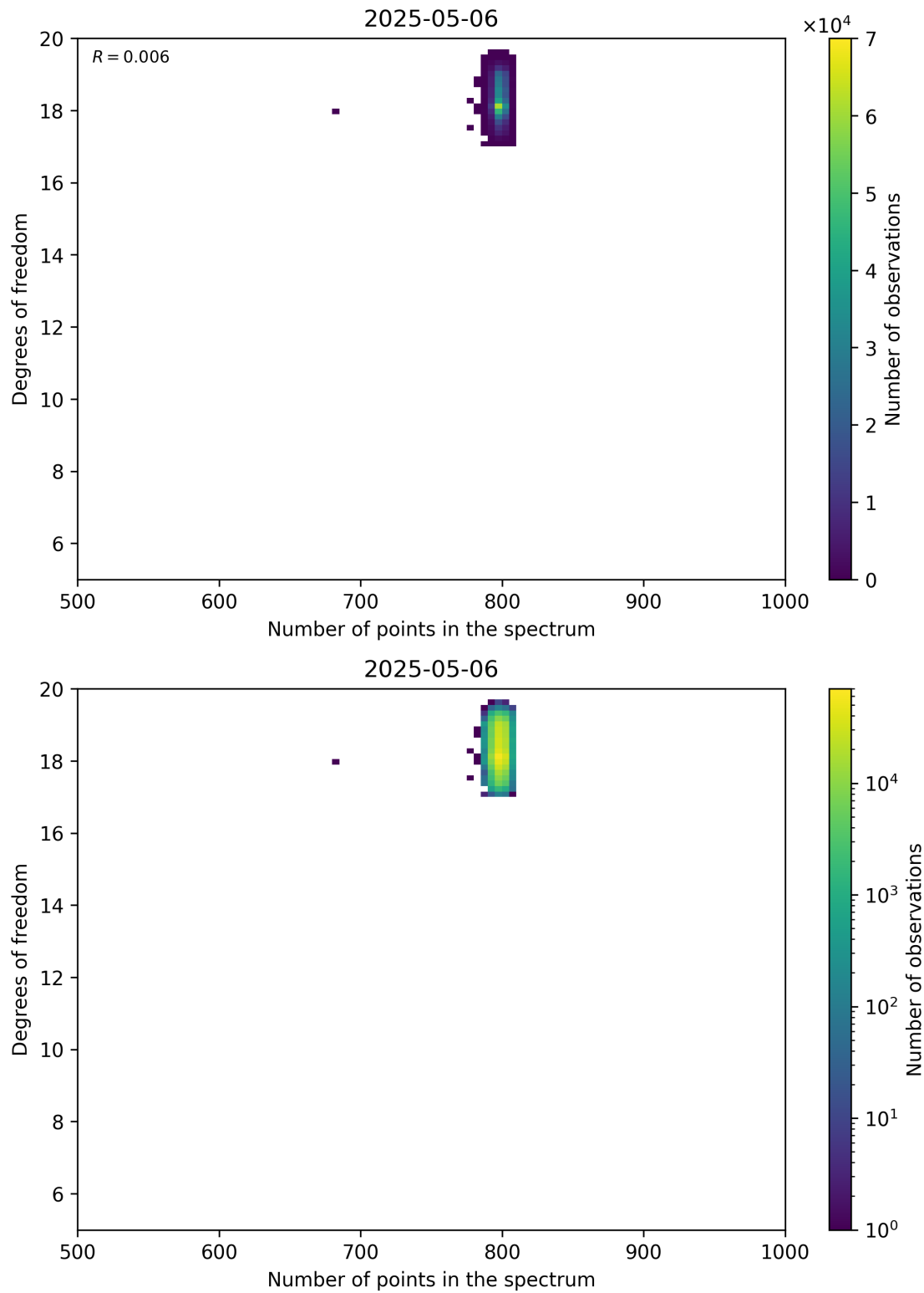
Figure 90: Scatter density plot of “Number of points in the spectrum” against “Degrees of freedom” for 2025-05-05 to 2025-05-07.
