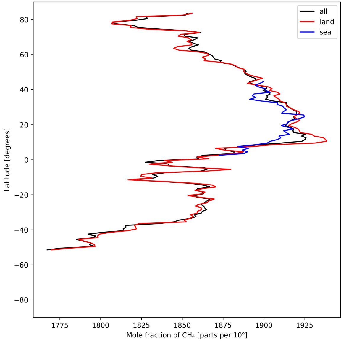
Figure 12: Zonal average of “Mole fraction of \text{CH}_4 ” for 2025-05-05 to 2025-05-07.
