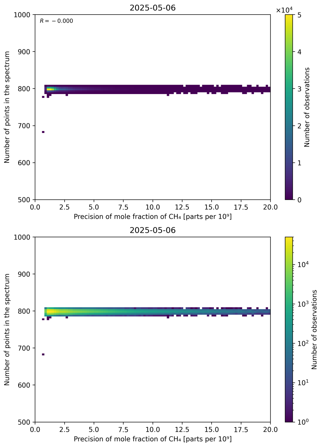
Figure 84: Scatter density plot of “Precision of mole fraction of CH 4 ” against “Number of points in the spectrum” for 2025-05-05 to 2025-05-07.
