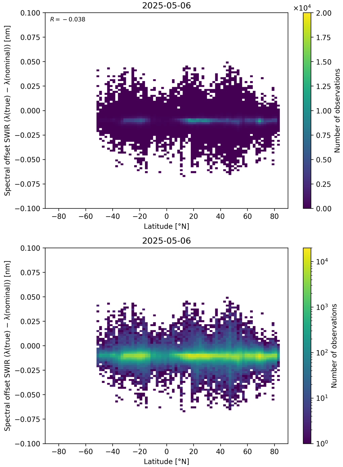
Figure 62: Scatter density plot of “Latitude” against “Spectral offset SWIR ( \lambda_{\text{true}} - \lambda_{\text{nominal}} )” for 2025-05-05 to 2025-05-07.
