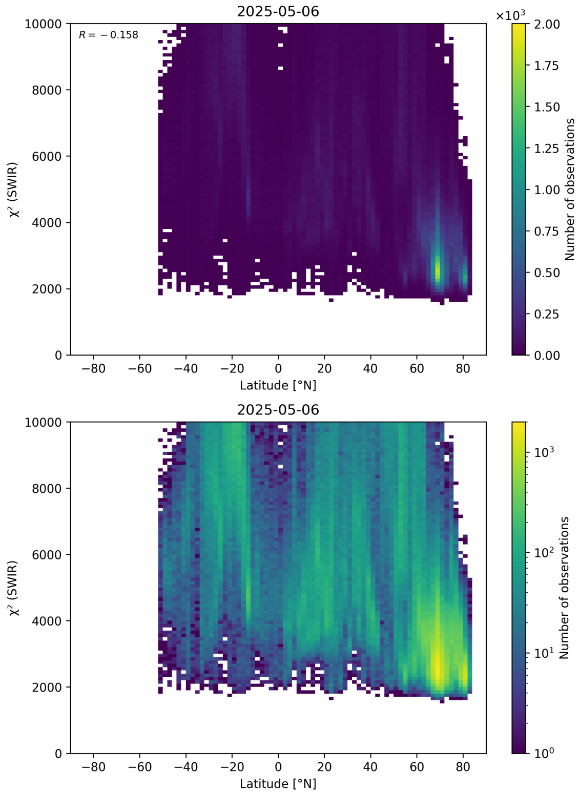
Figure 54: Scatter density plot of “Latitude” against “ \chi^2 (SWIR)” for 2025-05-05 to 2025-05-07.
