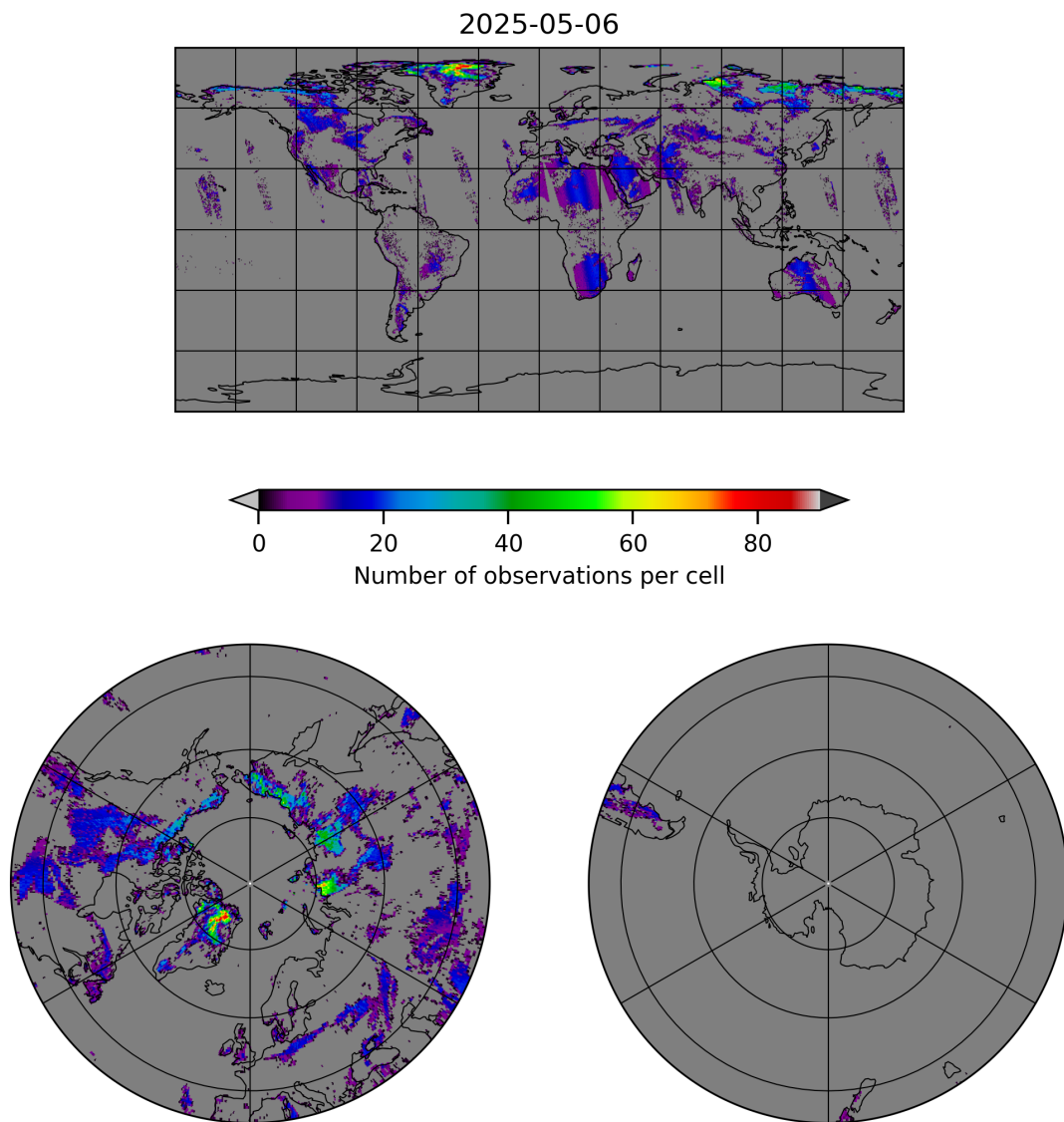
Figure 10: Map of the number of observations for 2025-05-05 to 2025-05-07
