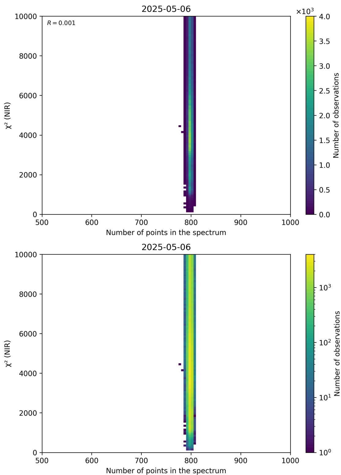
Figure 88: Scatter density plot of “Number of points in the spectrum” against “ \chi^2 (NIR)” for 2025-05-05 to 2025-05-07.
