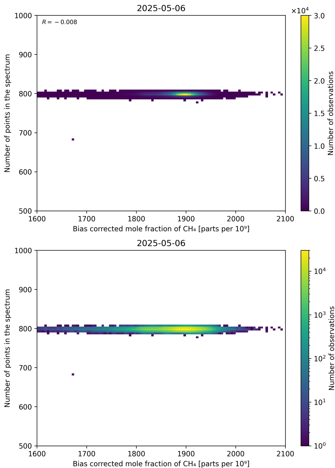
Figure 68: Scatter density plot of “Bias corrected mole fraction of CH 4 ” against “Number of points in the spectrum” for 2025-05-05 to 2025-05-07.
