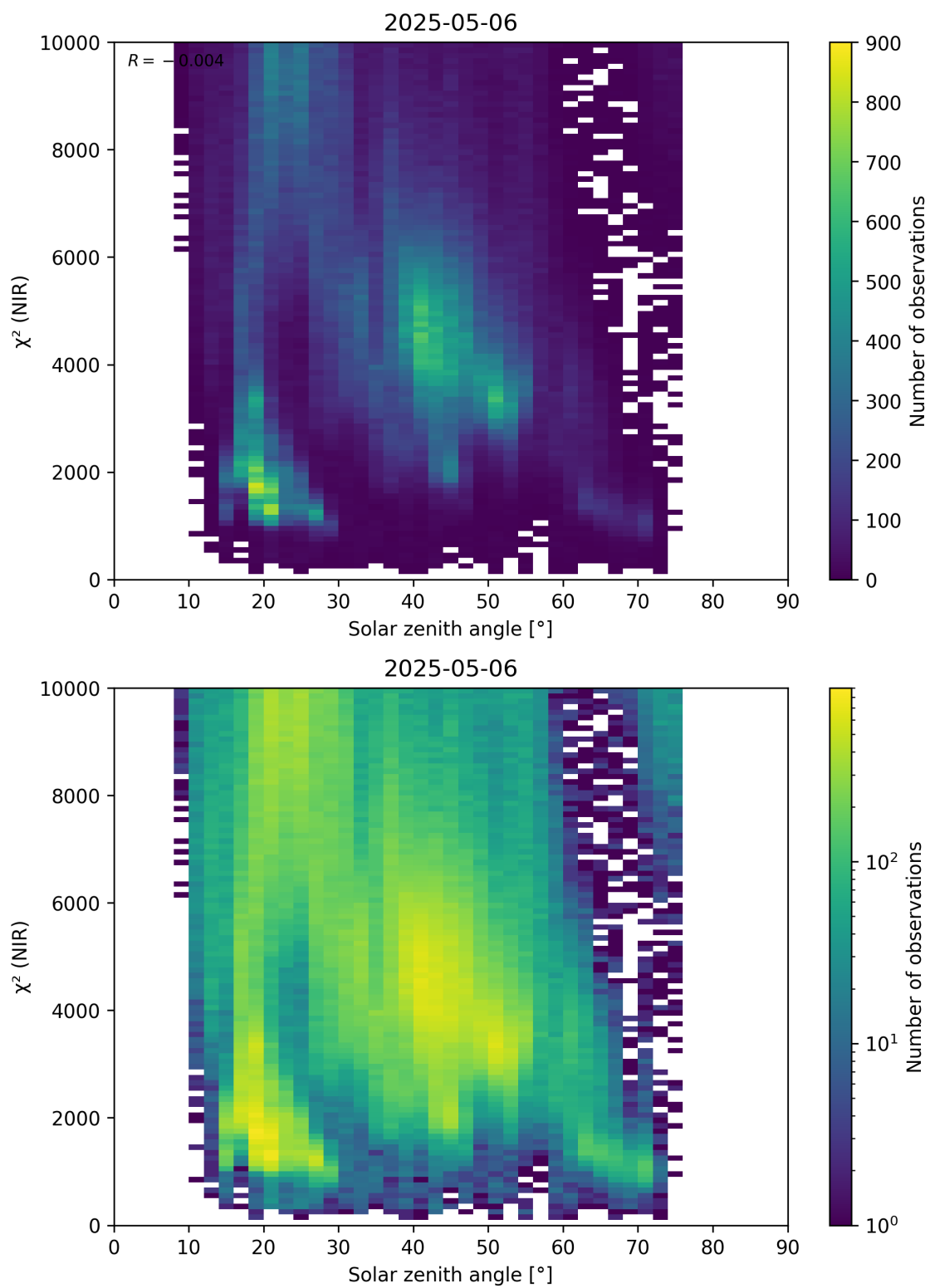
Figure 94: Scatter density plot of “Solar zenith angle” against “ \chi^2 (NIR)” for 2025-05-05 to 2025-05-07.
