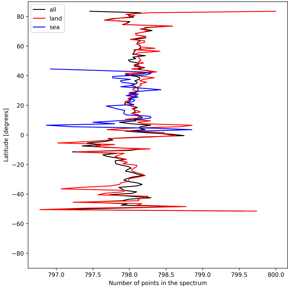
Figure 15: Zonal average of “Number of points in the spectrum” for 2025-05-05 to 2025-05-07.
