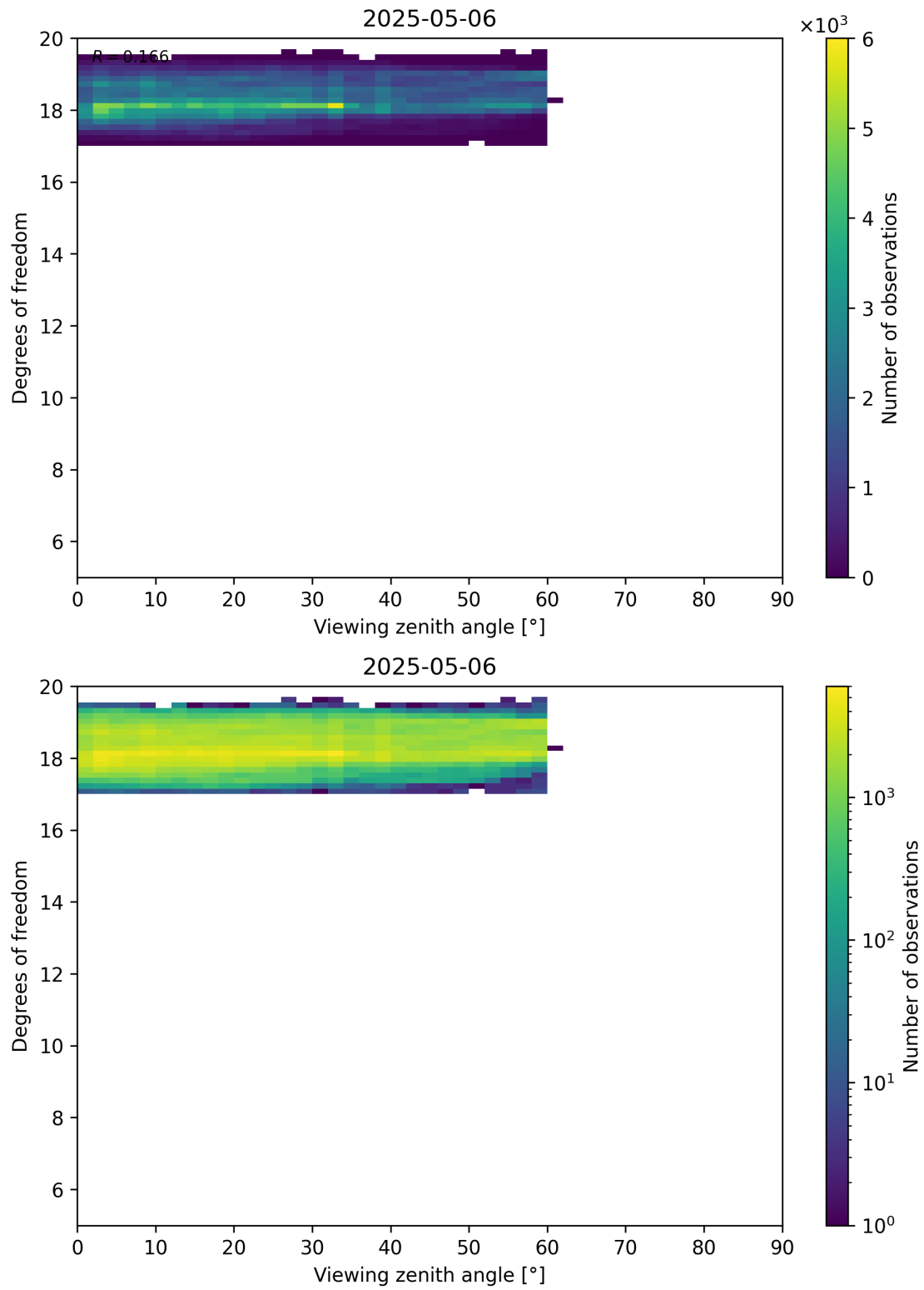
Figure 107: Scatter density plot of “Viewing zenith angle” against “Degrees of freedom” for 2025-05-05 to 2025-05-07.
