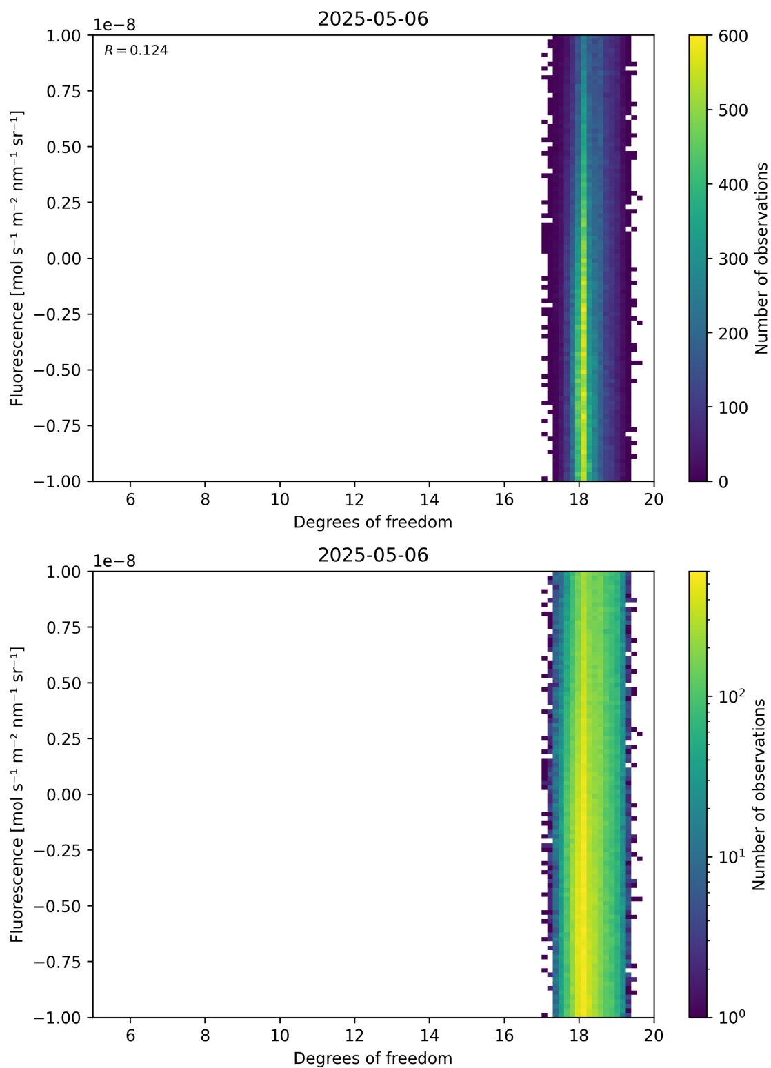
Figure 51: Scatter density plot of “Degrees of freedom” against “Fluorescence” for 2025-05-05 to 2025-05-07.
