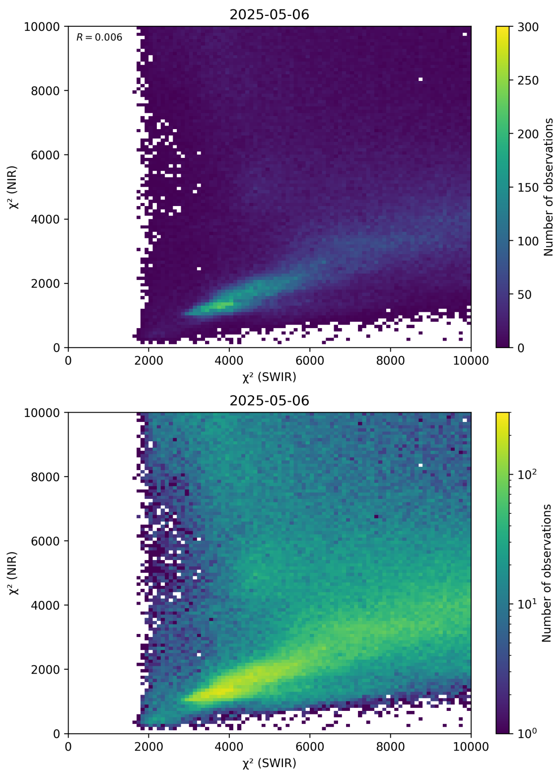
Figure 47: Scatter density plot of “ \chi^2 (SWIR)” against “ \chi^2 (NIR)” for 2025-05-05 to 2025-05-07.
