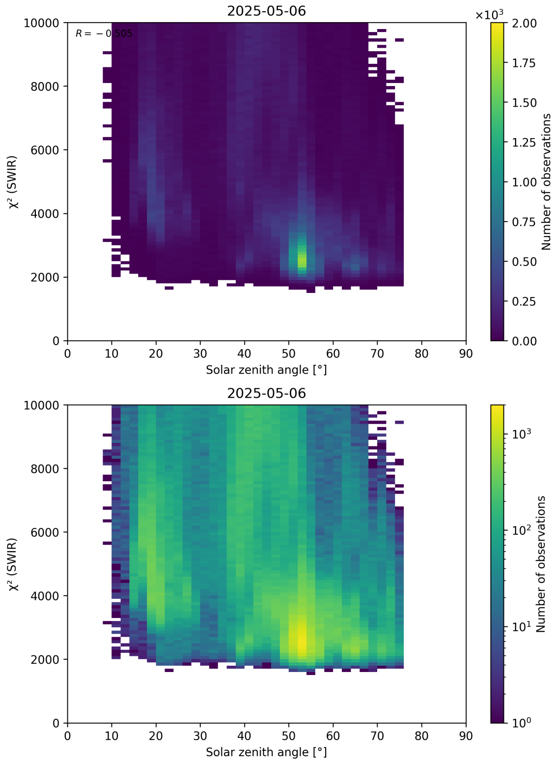
Figure 95: Scatter density plot of “Solar zenith angle” against “ \chi^2 (SWIR)” for 2025-05-05 to 2025-05-07.
