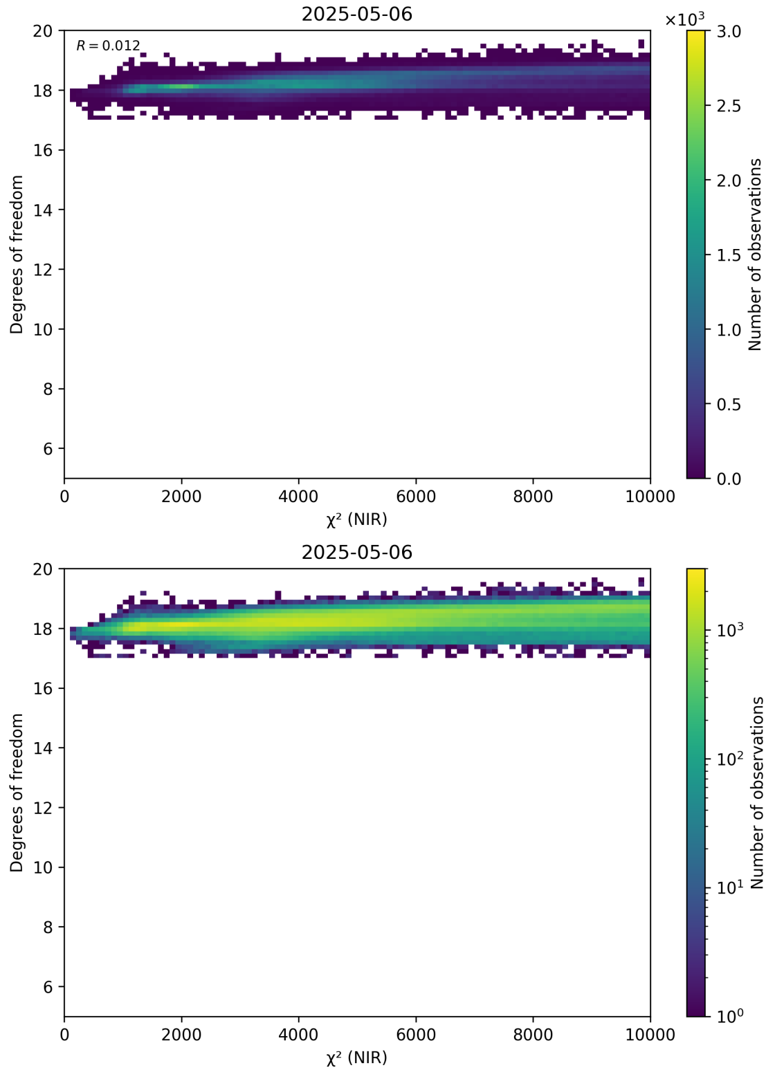
Figure 44: Scatter density plot of “ \chi^2 (NIR)” against “Degrees of freedom” for 2025-05-05 to 2025-05-07.
