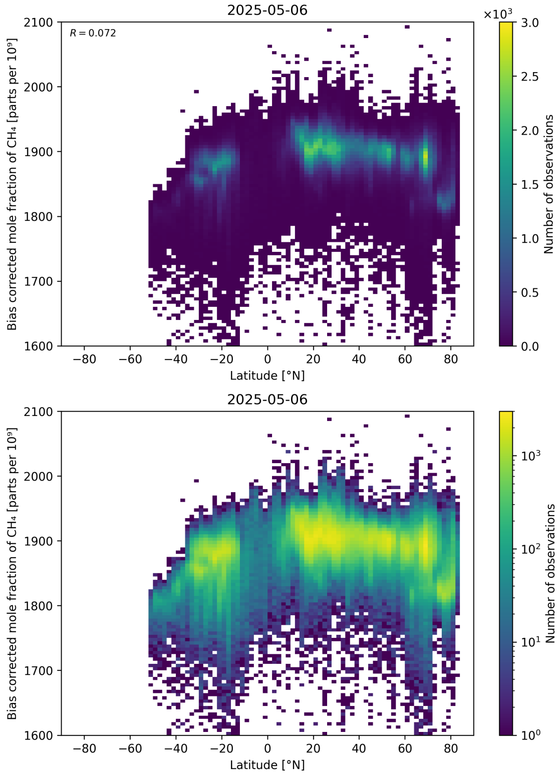
Figure 58: Scatter density plot of “Latitude” against “Bias corrected mole fraction of CH 4 ” for 2025-05-05 to 2025-05-07.
