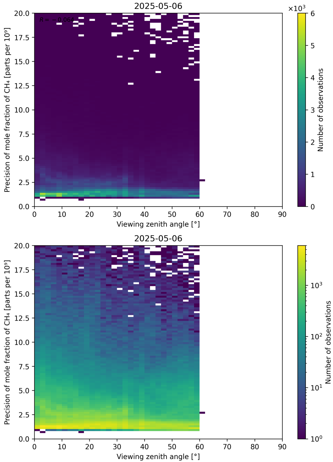
Figure 112: Scatter density plot of “Viewing zenith angle” against “Precision of mole fraction of CH 4 ” for 2025-05-05 to 2025-05-07.
