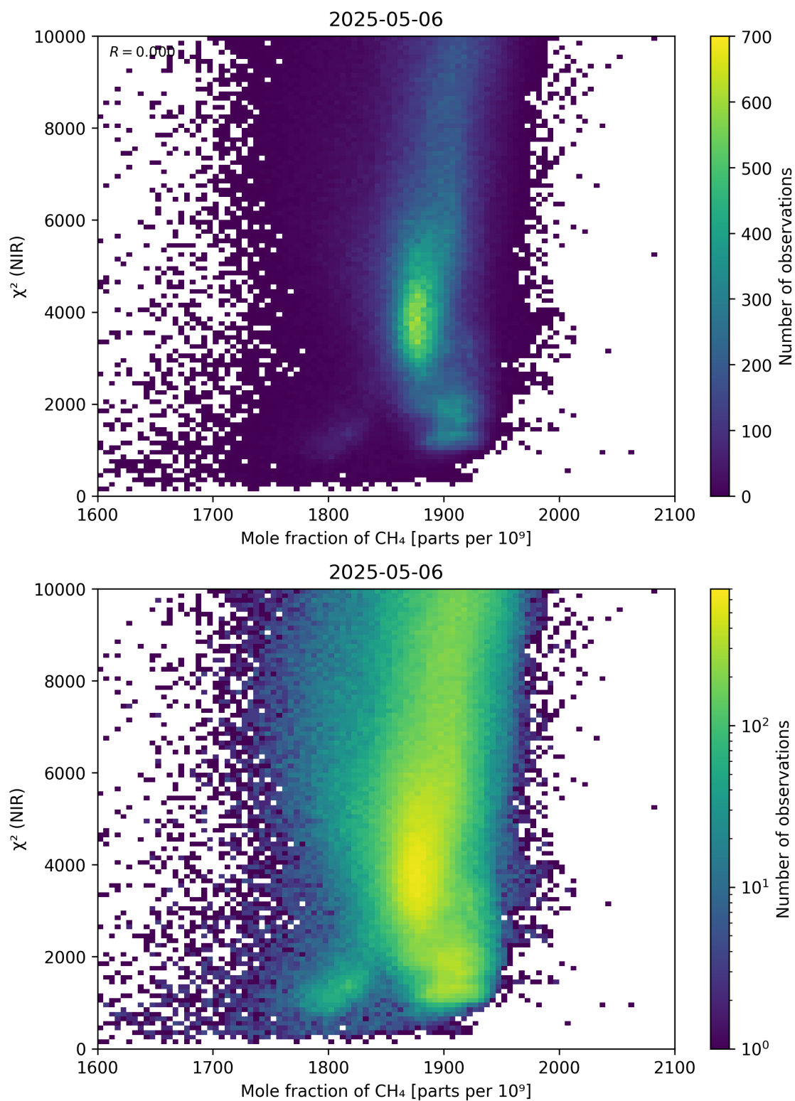
Figure 70: Scatter density plot of “Mole fraction of CH 4 ” against “ \chi^2 (NIR)” for 2025-05-05 to 2025-05-07.
