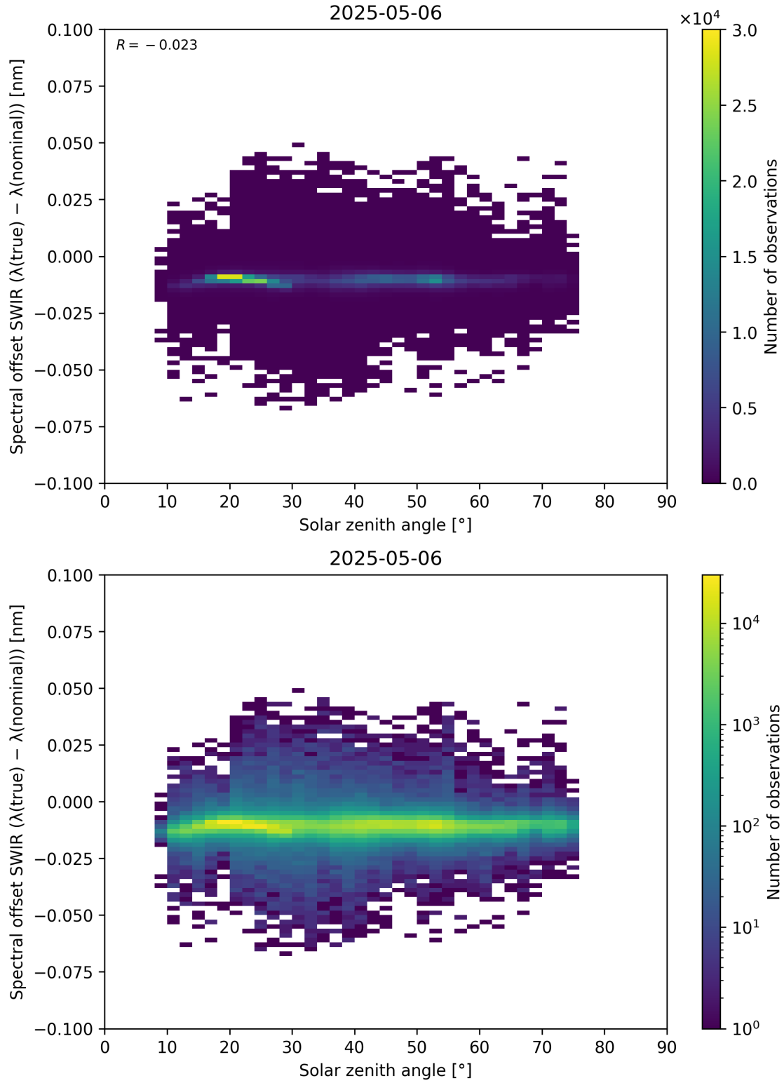
Figure 104: Scatter density plot of “Solar zenith angle” against “Spectral offset SWIR ( \lambda_{\text{true}} - \lambda_{\text{nominal}} )” for 2025-05-05 to 2025-05-07.
