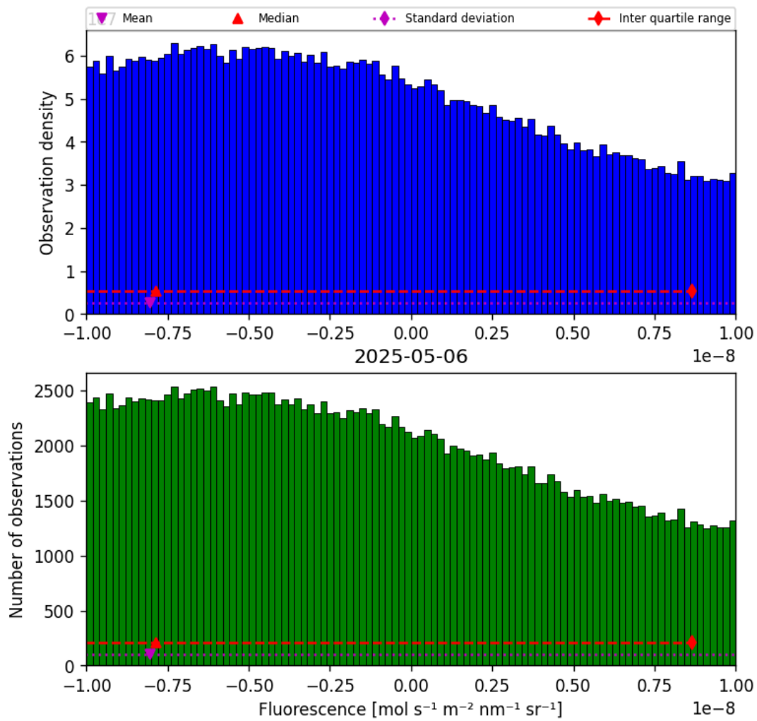
Figure 32: Histogram of “Fluorescence” for 2025-05-05 to 2025-05-07
