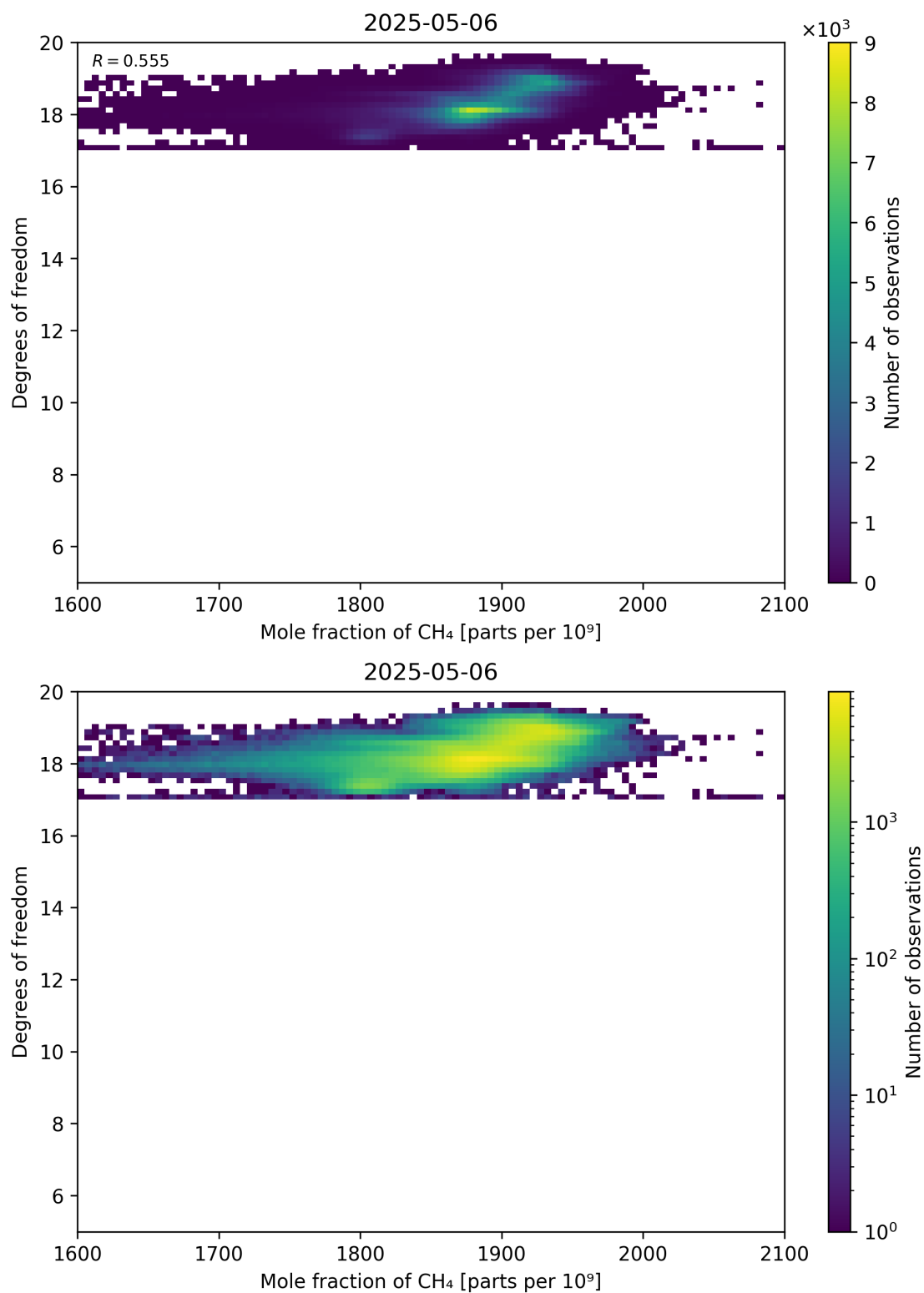
Figure 72: Scatter density plot of “Mole fraction of CH 4 ” against “Degrees of freedom” for 2025-05-05 to 2025-05-07.
