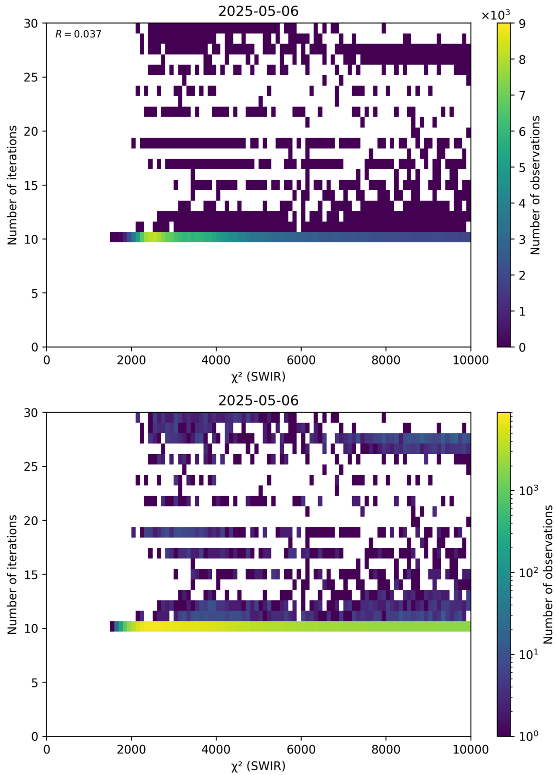
Figure 50: Scatter density plot of “ \chi^2 (SWIR)” against “Number of iterations” for 2025-05-05 to 2025-05-07.
