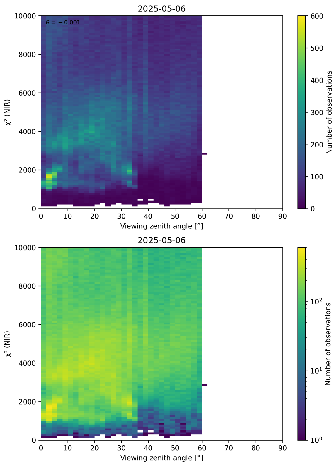
Figure 105: Scatter density plot of “Viewing zenith angle” against “ \chi^2 (NIR)” for 2025-05-05 to 2025-05-07.
