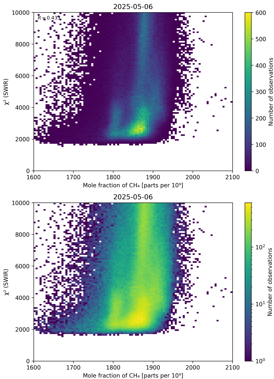
Figure 71: Scatter density plot of “Mole fraction of \text{CH}_4 ” against “ \chi^2 (SWIR)” for 2025-05-05 to 2025-05-07.
