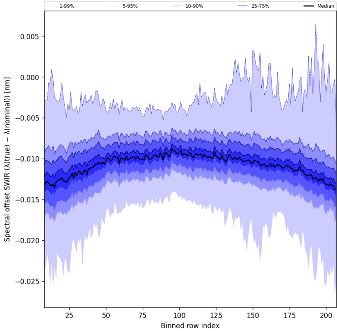
Figure 38: Along track statistics of “Spectral offset SWIR ( \lambda_{\text{true}} - \lambda_{\text{nominal}} )” for 2025-05-05 to 2025-05-07
