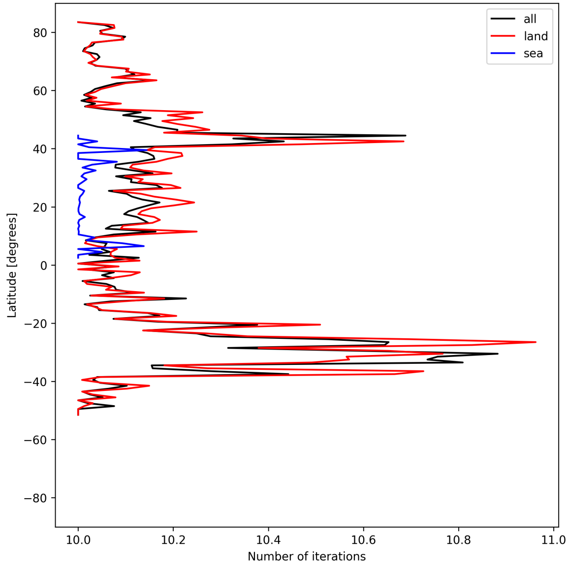
Figure 20: Zonal average of “Number of iterations” for 2025-05-05 to 2025-05-07.
