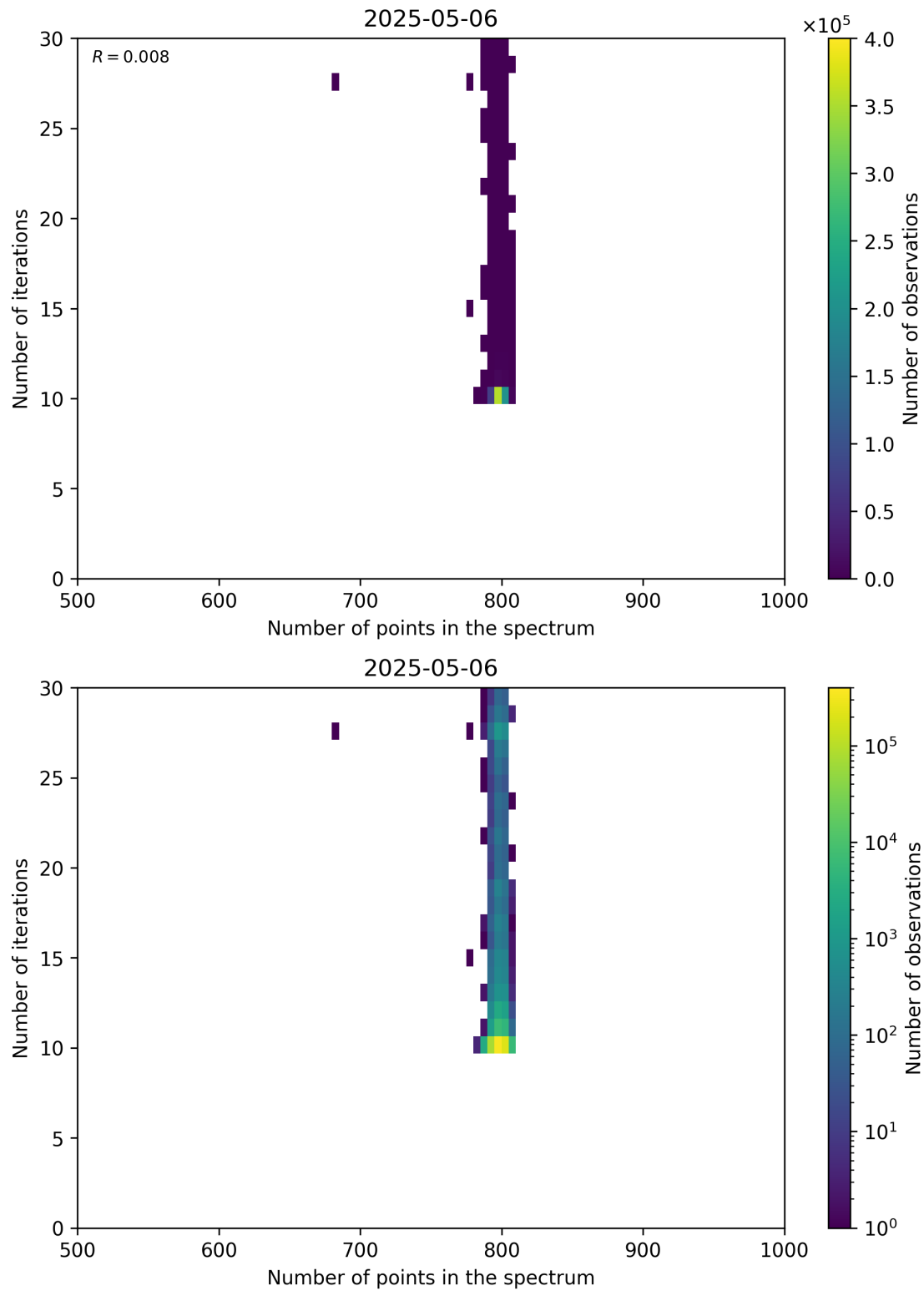
Figure 92: Scatter density plot of “Number of points in the spectrum” against “Number of iterations” for 2025-05-05 to 2025-05-07.
