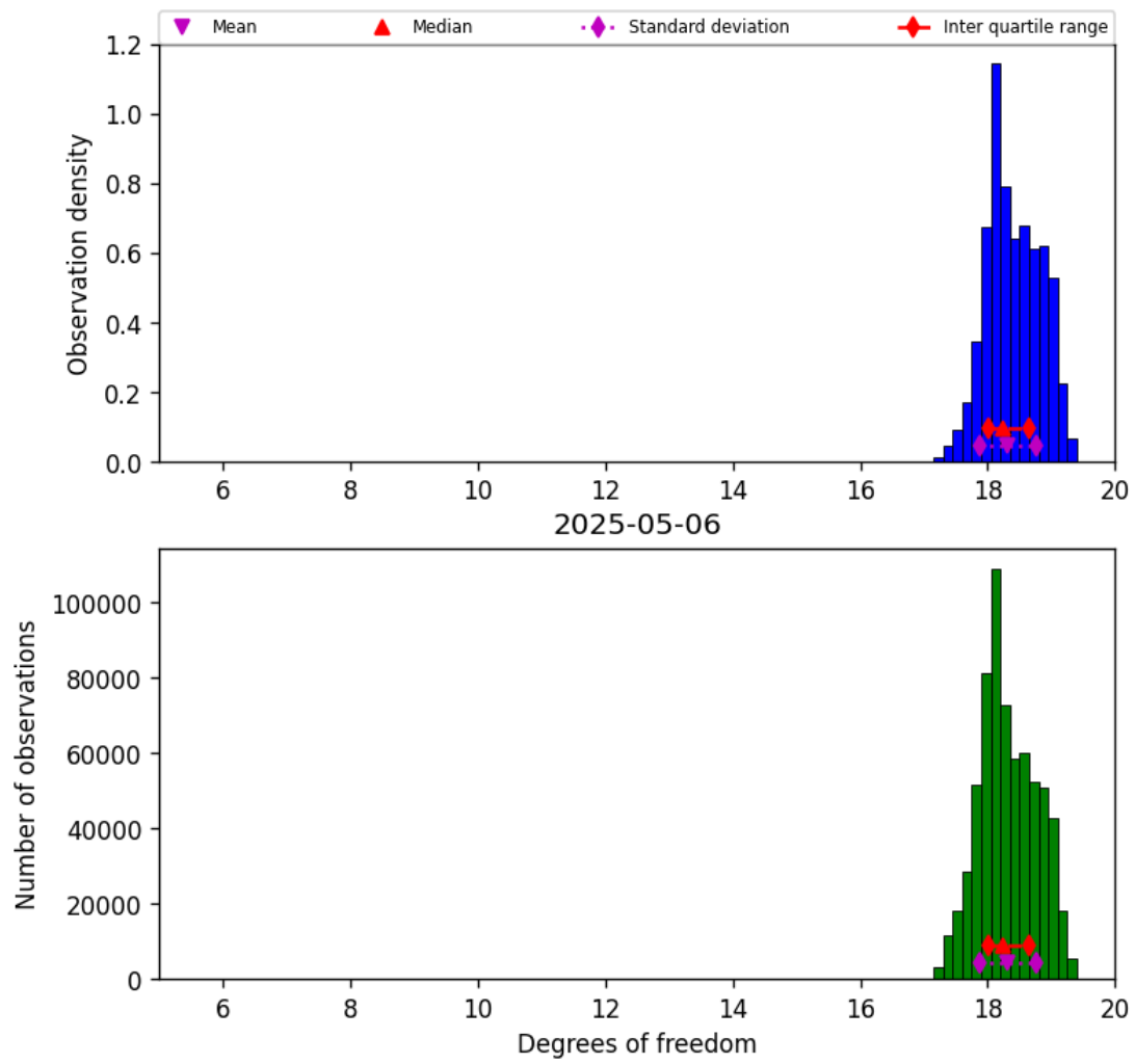
Figure 30: Histogram of “Degrees of freedom” for 2025-05-05 to 2025-05-07
