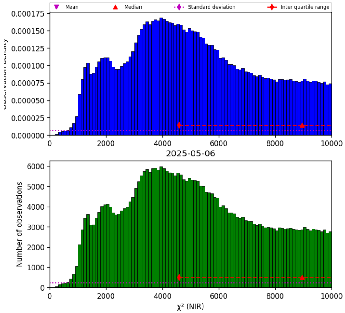
Figure 29: Histogram of “ \chi^2 (NIR)” for 2025-05-05 to 2025-05-07
