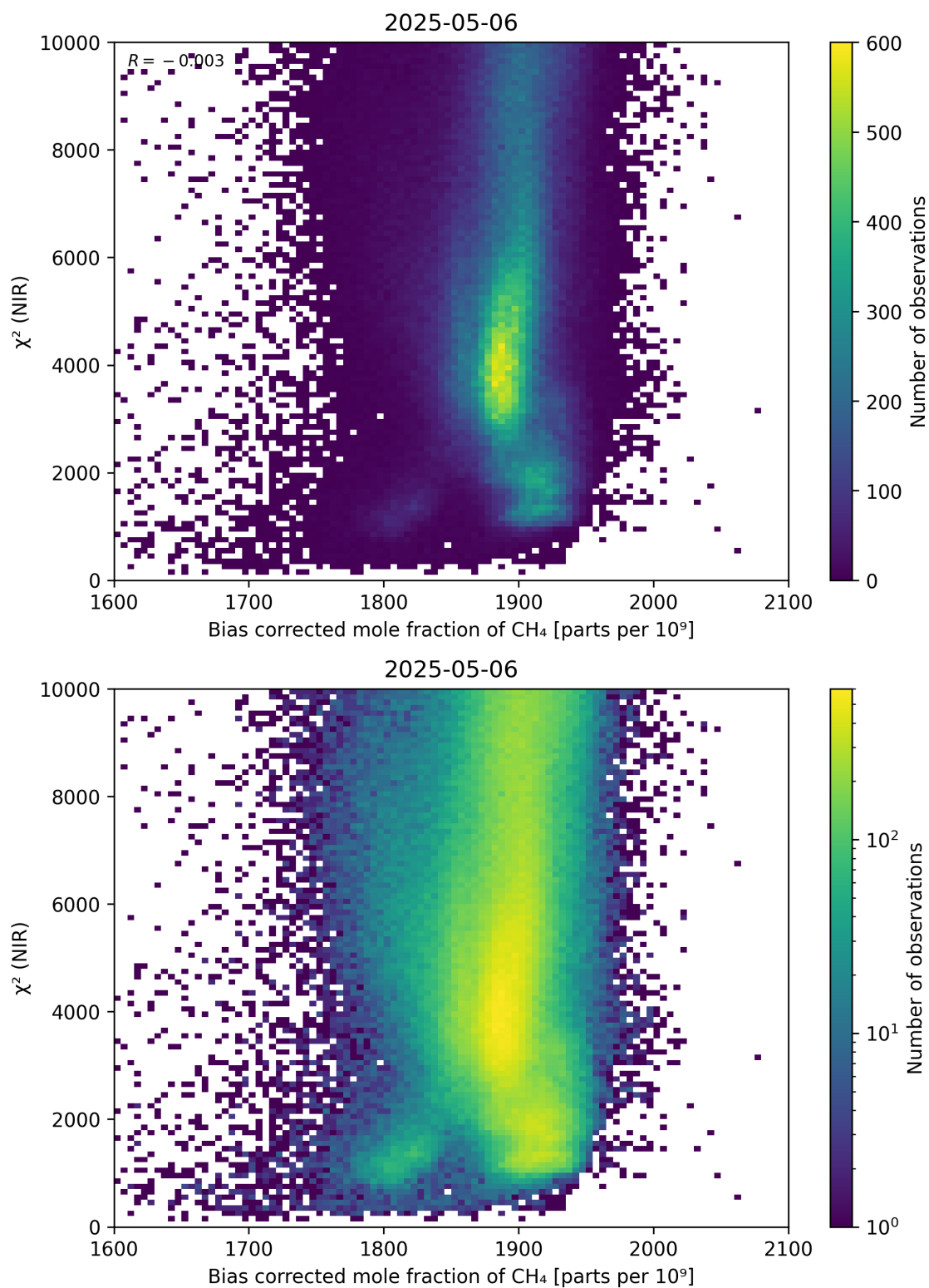
Figure 63: Scatter density plot of “Bias corrected mole fraction of CH 4 ” against “ \chi^2 (NIR)” for 2025-05-05 to 2025-05-07.
