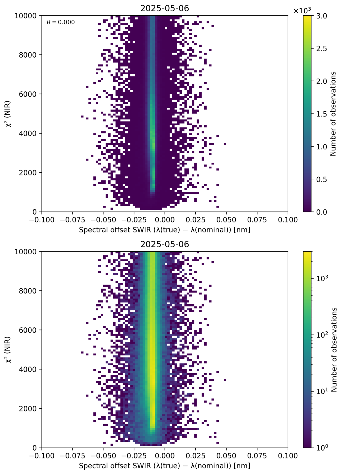
Figure 117: Scatter density plot of “Spectral offset SWIR ( \lambda_{\text{true}} - \lambda_{\text{nominal}} )” against “ \chi^2 (NIR)” for 2025-05-05 to 2025-05-07.
