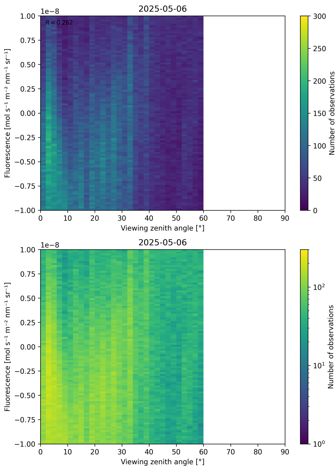
Figure 108: Scatter density plot of “Viewing zenith angle” against “Fluorescence” for 2025-05-05 to 2025-05-07.
