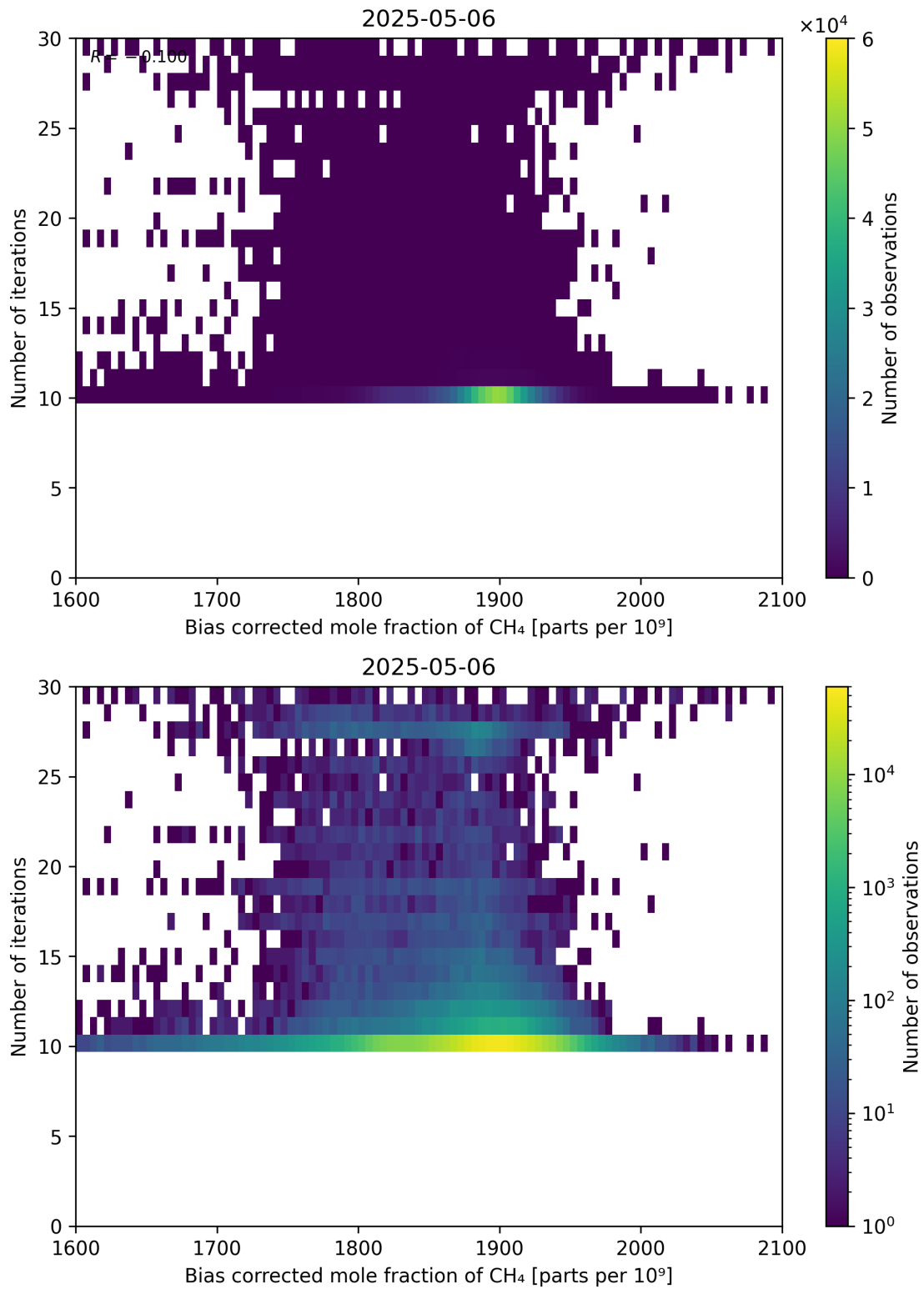
Figure 67: Scatter density plot of “Bias corrected mole fraction of CH 4 ” against “Number of iterations” for 2025-05-05 to 2025-05-07.
