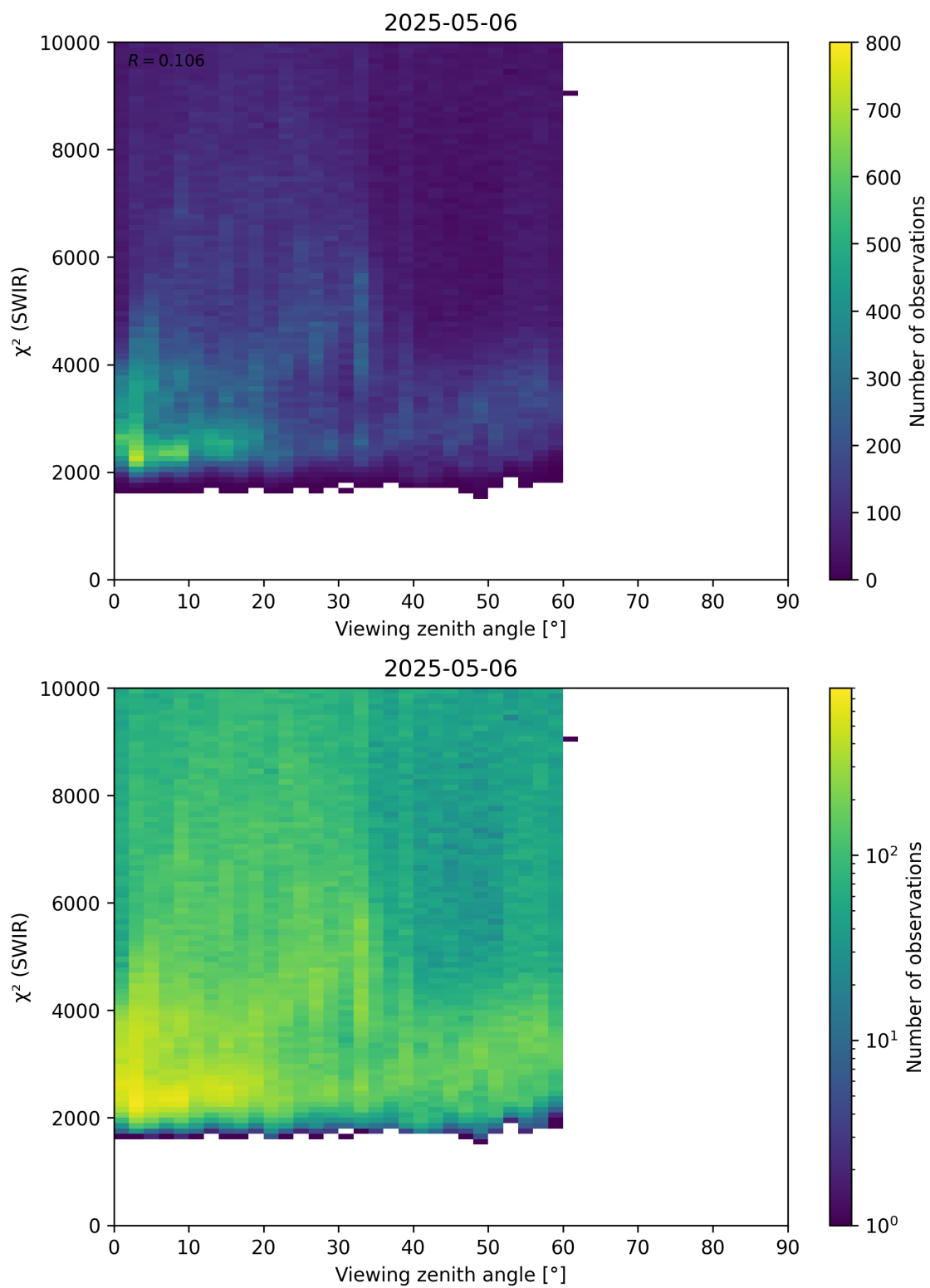
Figure 106: Scatter density plot of “Viewing zenith angle” against “ \chi^2 (SWIR)” for 2025-05-05 to 2025-05-07.
