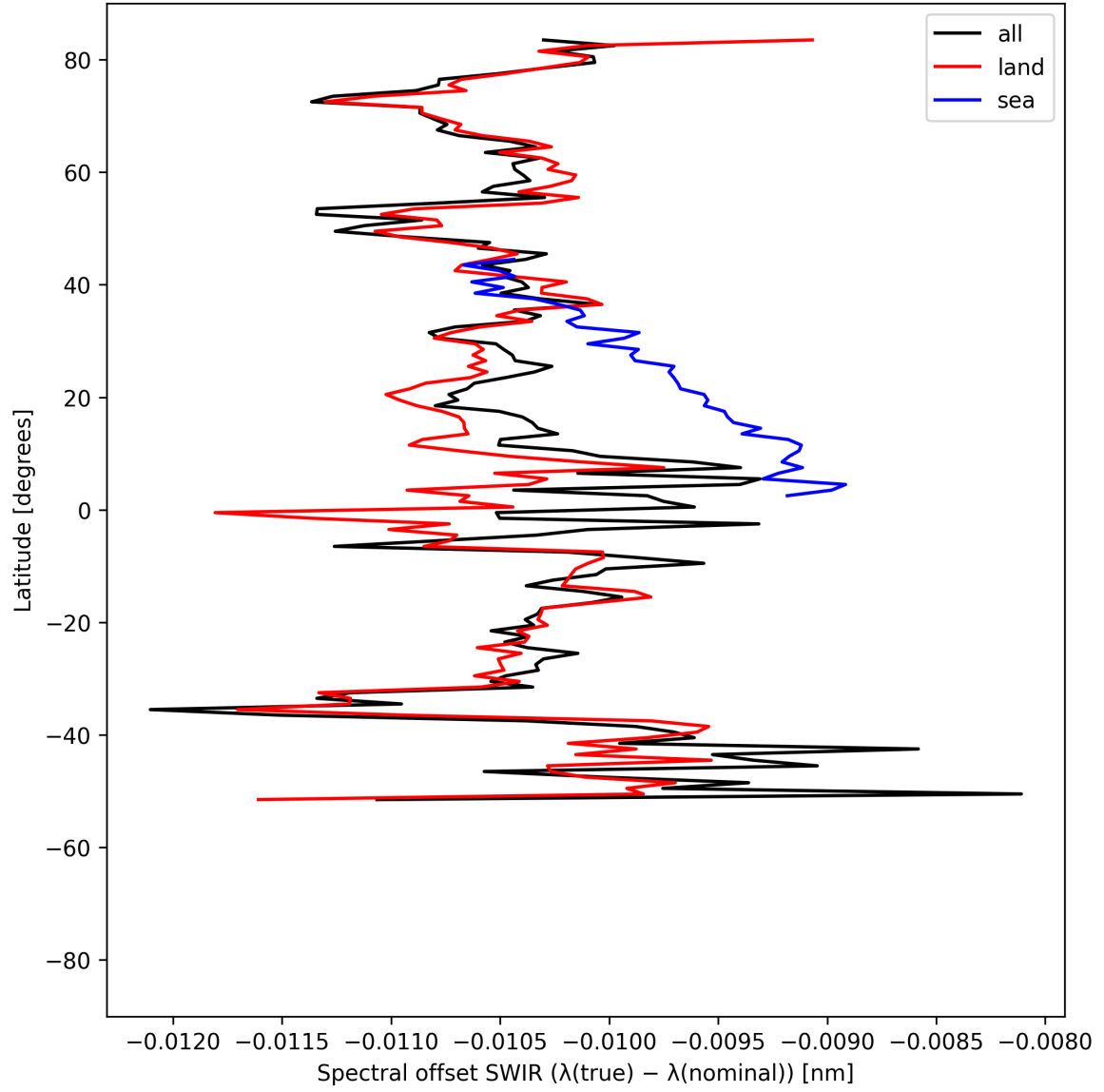
Figure 16: Zonal average of “Spectral offset SWIR ( \lambda_{\text{true}} - \lambda_{\text{nominal}} )” for 2025-05-05 to 2025-05-07.
