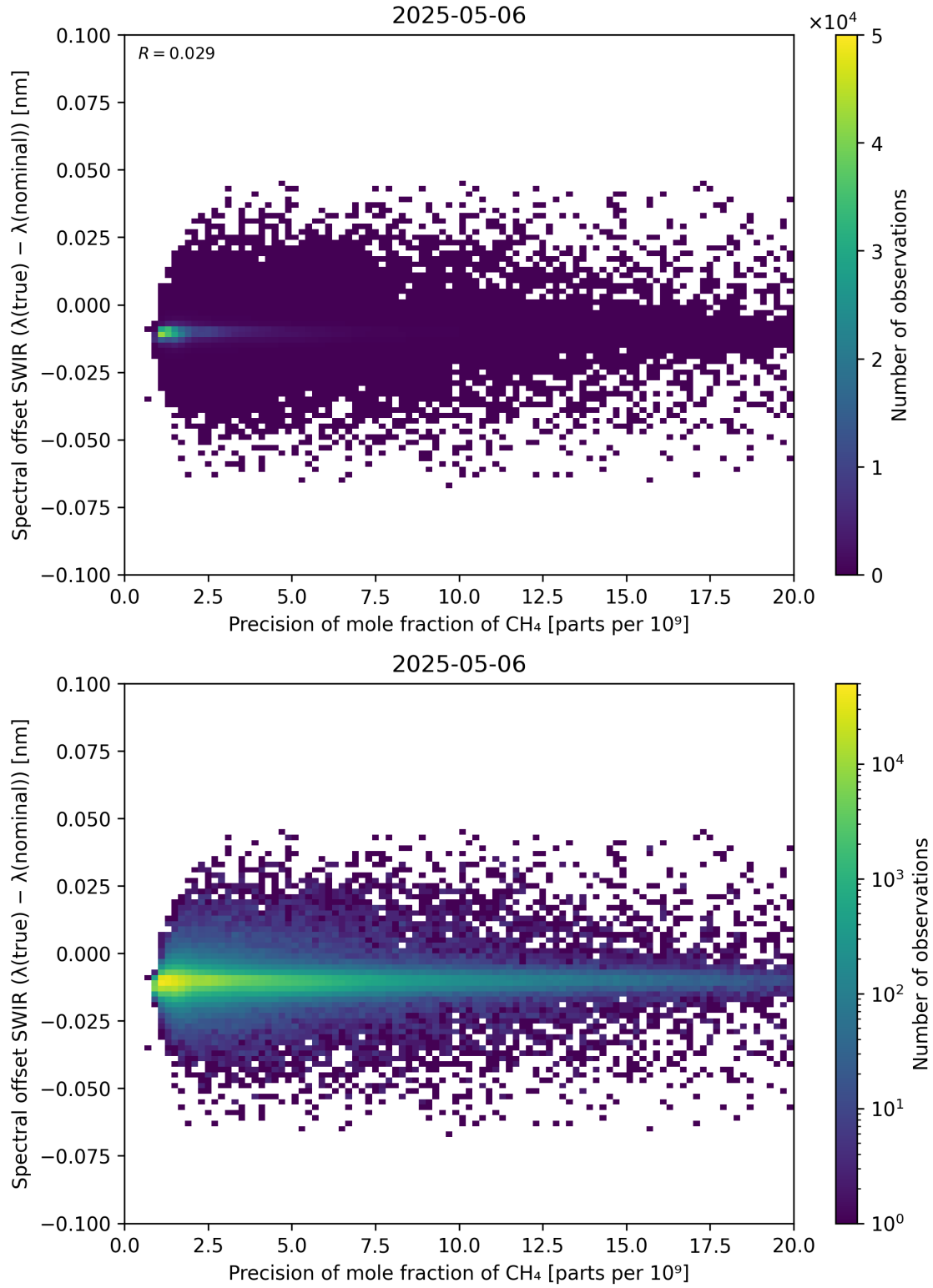
Figure 85: Scatter density plot of “Precision of mole fraction of \text{CH}_4 ” against “Spectral offset SWIR ( \lambda_{\text{true}} - \lambda_{\text{nominal}} )” for 2025-05-05 to 2025-05-07.
