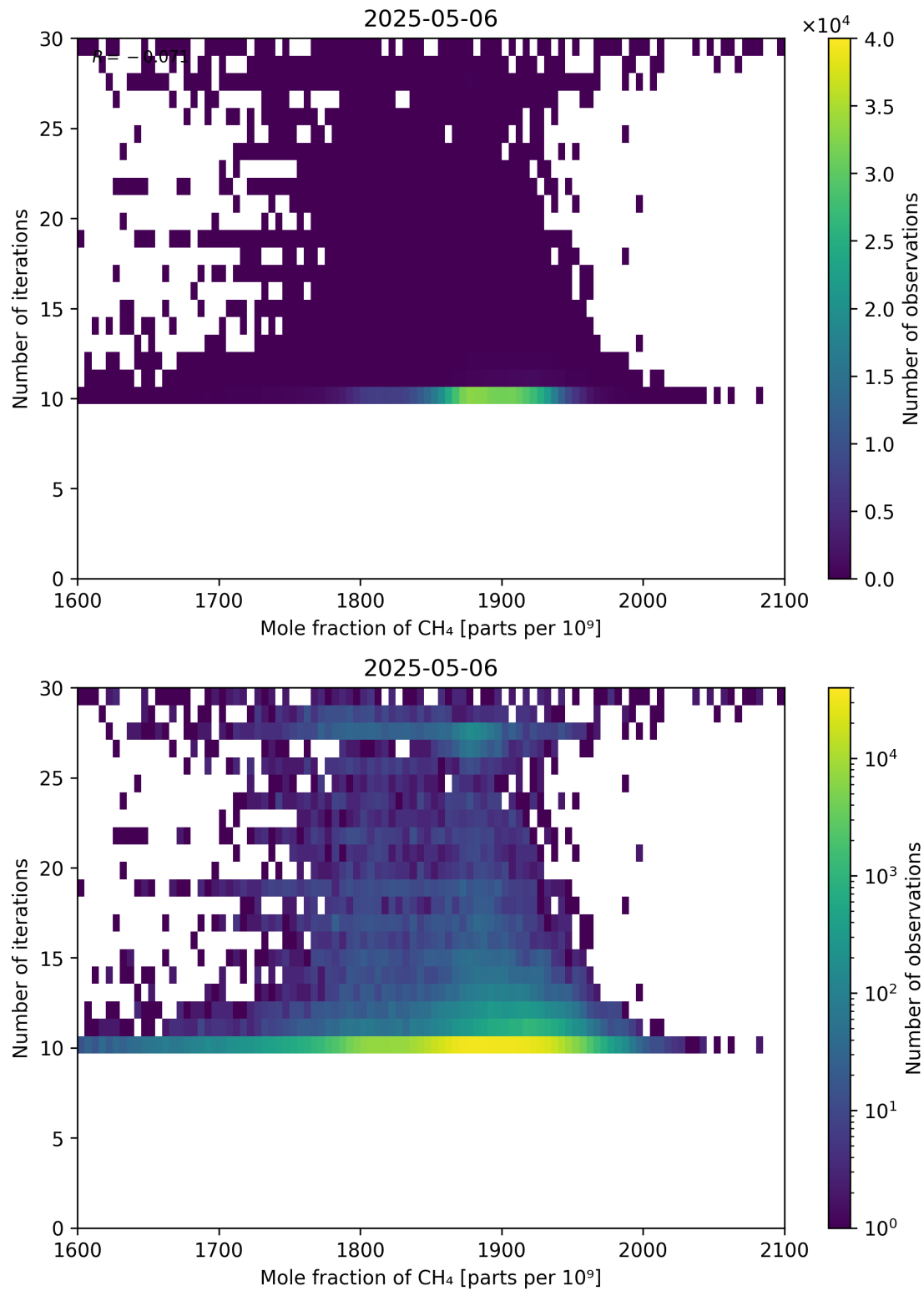
Figure 76: Scatter density plot of “Mole fraction of CH 4 ” against “Number of iterations” for 2025-05-05 to 2025-05-07.
