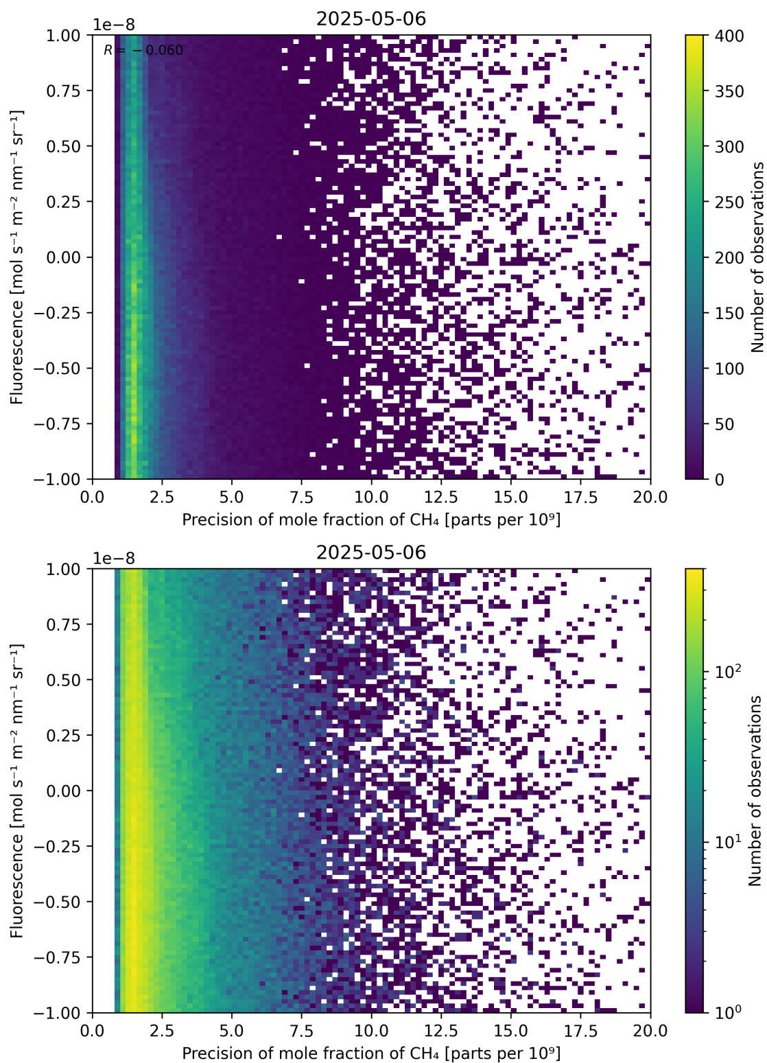
Figure 81: Scatter density plot of “Precision of mole fraction of \text{CH}_4 ” against “Fluorescence” for 2025-05-05 to 2025-05-07.
