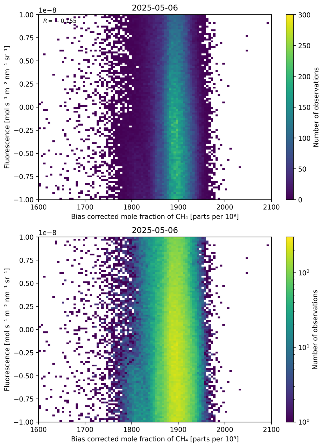
Figure 66: Scatter density plot of “Bias corrected mole fraction of CH 4 ” against “Fluorescence” for 2025-05-05 to 2025-05-07.
