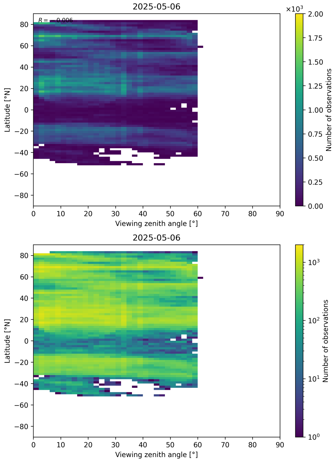
Figure 109: Scatter density plot of “Viewing zenith angle” against “Latitude” for 2025-05-05 to 2025-05-07.
