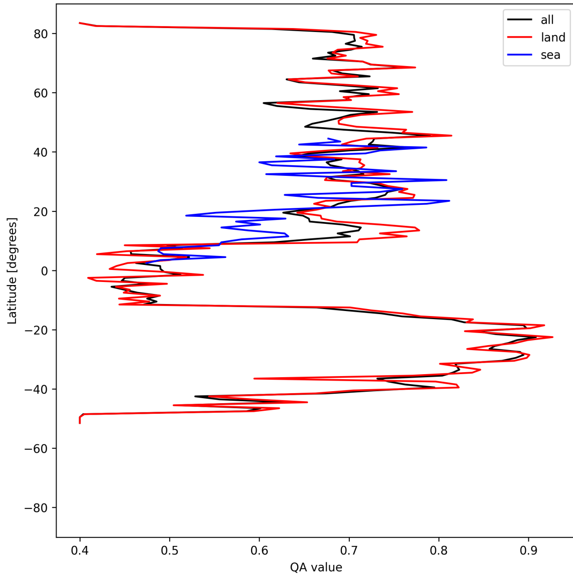
Figure 11: Zonal average of “QA value” for 2025-05-05 to 2025-05-07.
