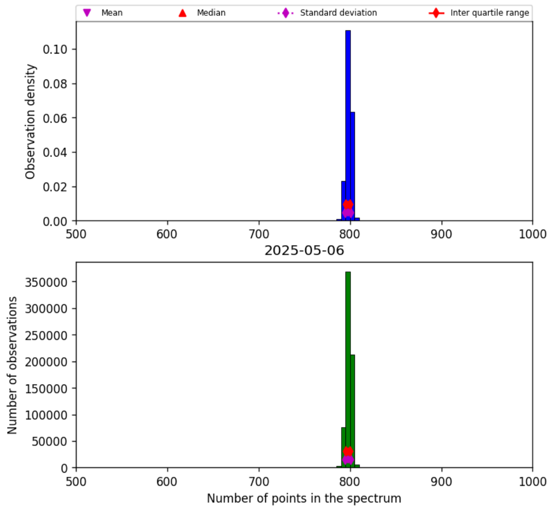
Figure 26: Histogram of “Number of points in the spectrum” for 2025-05-05 to 2025-05-07
