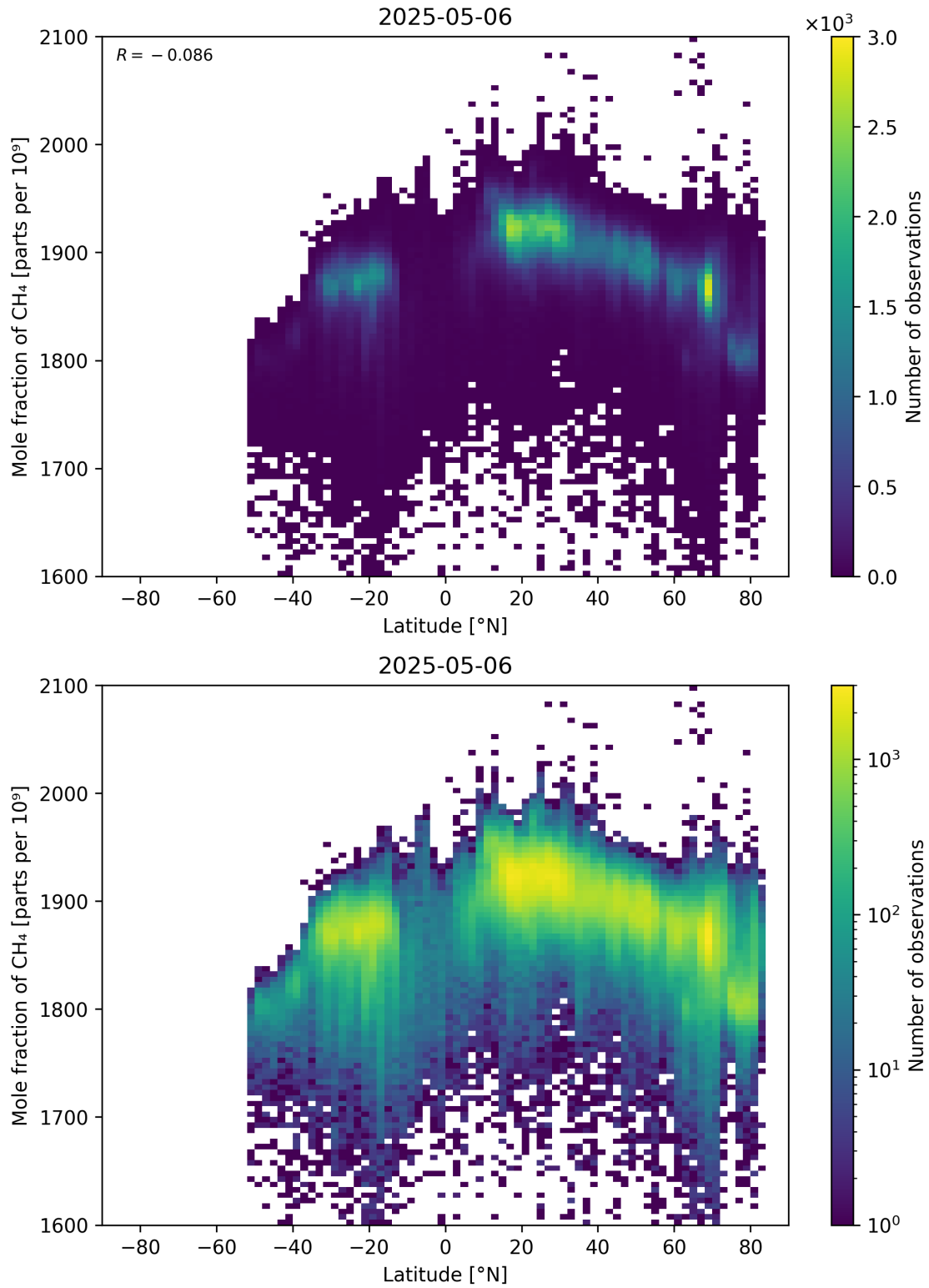
Figure 57: Scatter density plot of “Latitude” against “Mole fraction of CH 4 ” for 2025-05-05 to 2025-05-07.
