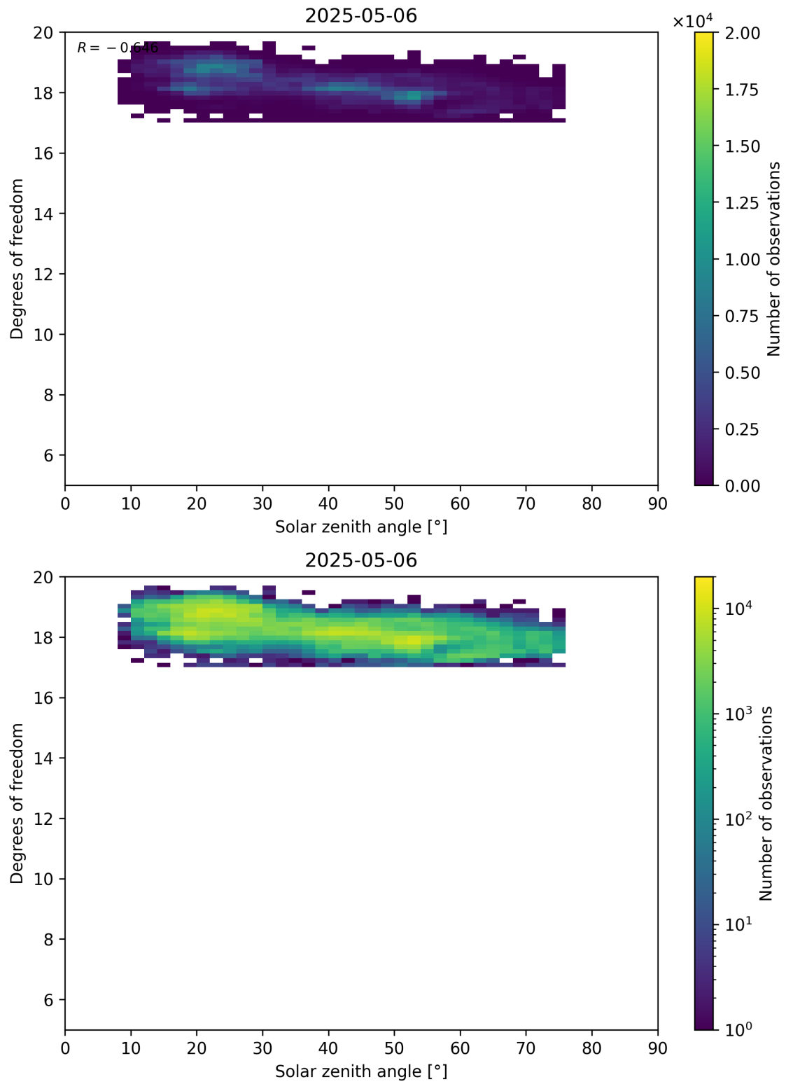
Figure 96: Scatter density plot of “Solar zenith angle” against “Degrees of freedom” for 2025-05-05 to 2025-05-07.
