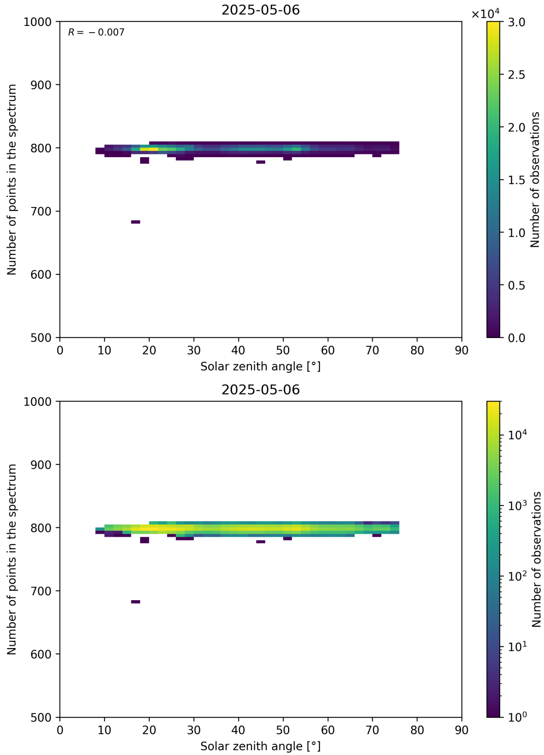
Figure 103: Scatter density plot of “Solar zenith angle” against “Number of points in the spectrum” for 2025-05-05 to 2025-05-07.
