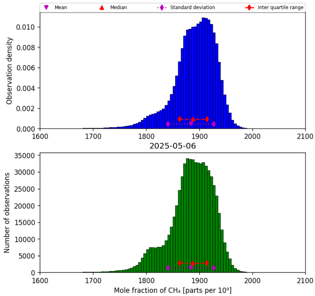
Figure 23: Histogram of “Mole fraction of CH 4 ” for 2025-05-05 to 2025-05-07
