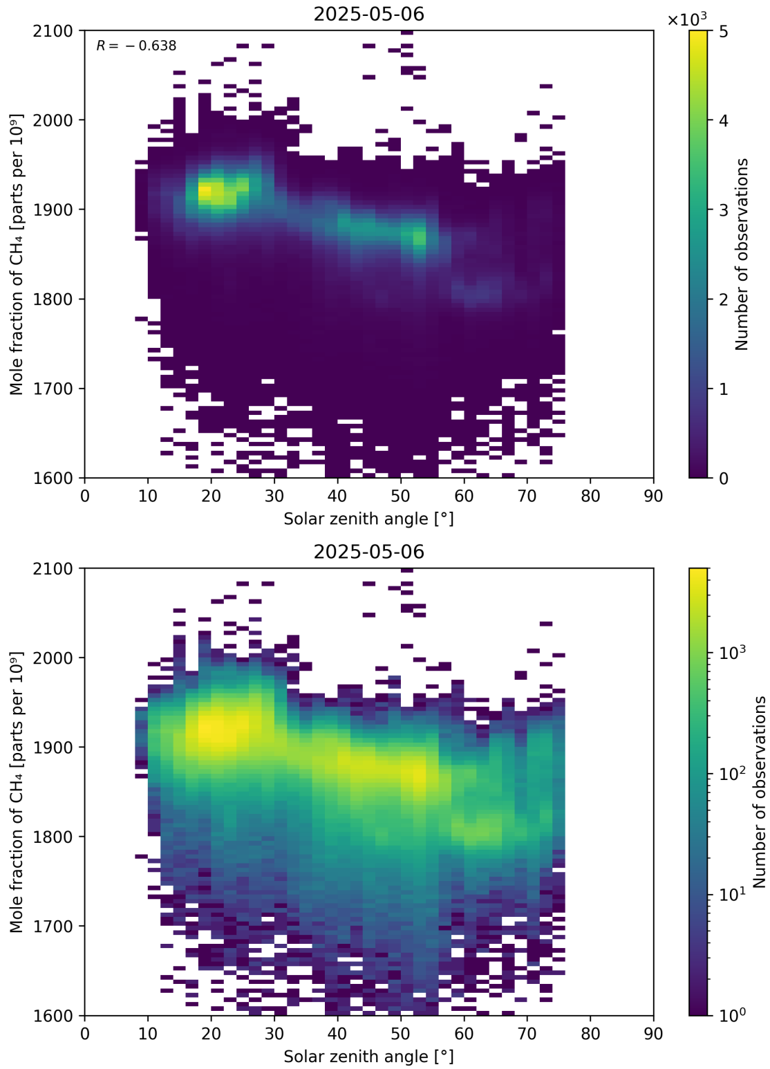
Figure 99: Scatter density plot of “Solar zenith angle” against “Mole fraction of CH 4 ” for 2025-05-05 to 2025-05-07.
