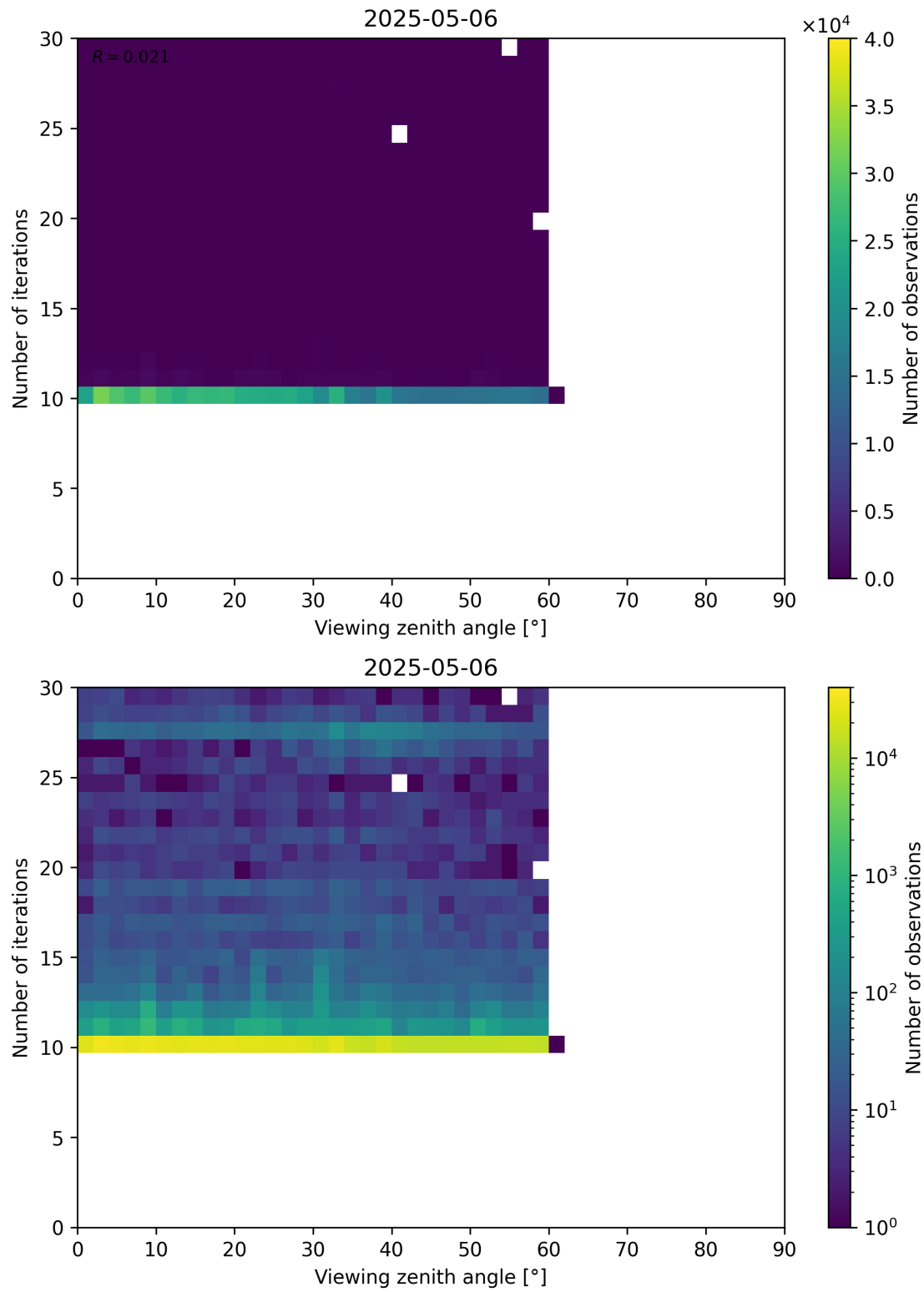
Figure 113: Scatter density plot of “Viewing zenith angle” against “Number of iterations” for 2025-05-05 to 2025-05-07.
