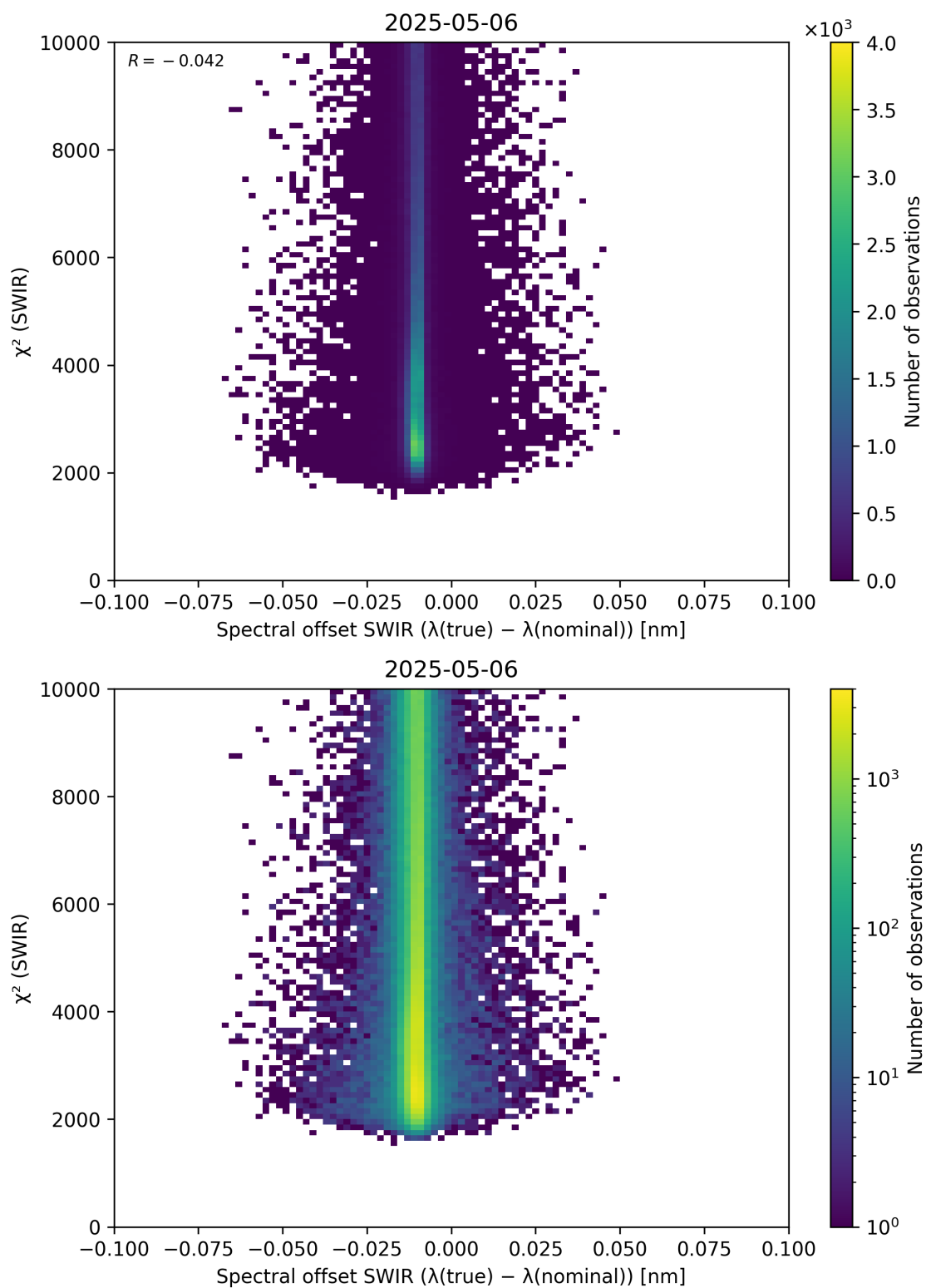
Figure 118: Scatter density plot of “Spectral offset SWIR ( \lambda_{\text{true}} - \lambda_{\text{nominal}} )” against “ \chi^2 (SWIR)” for 2025-05-05 to 2025-05-07.
