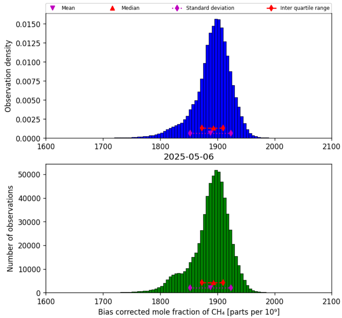
Figure 25: Histogram of “Bias corrected mole fraction of CH 4 ” for 2025-05-05 to 2025-05-07
