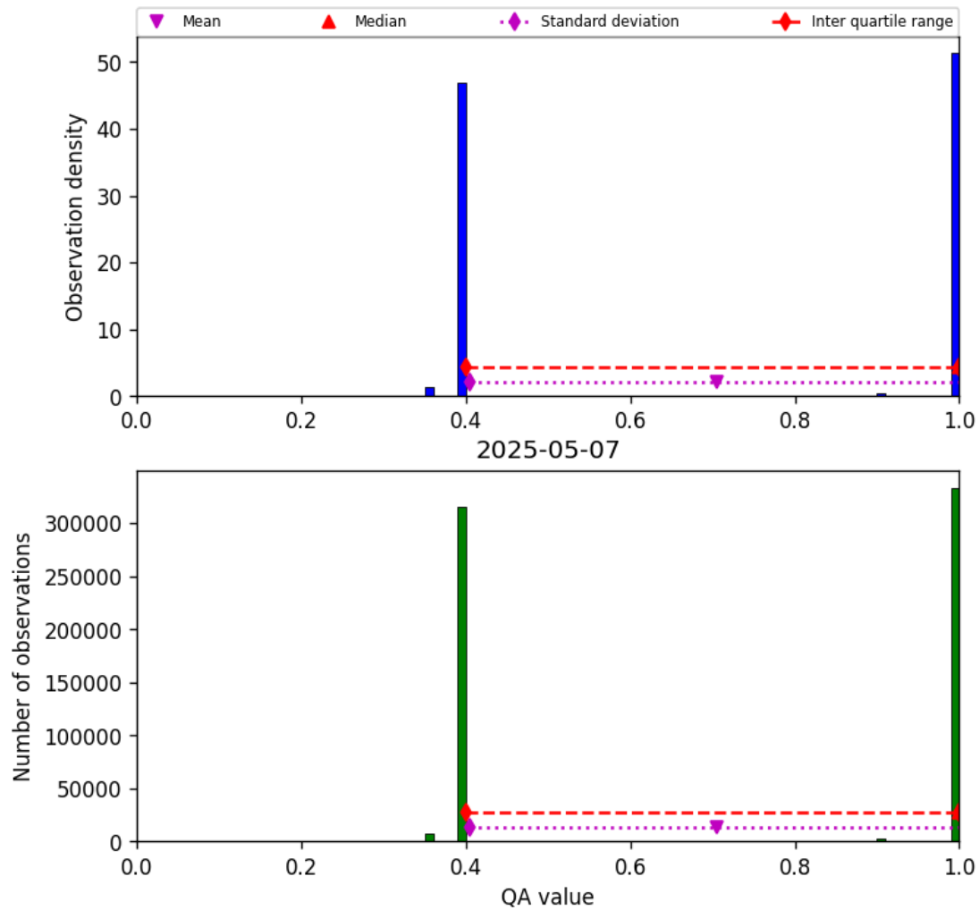
Figure 22: Histogram of “QA value” for 2025-05-06 to 2025-05-08
