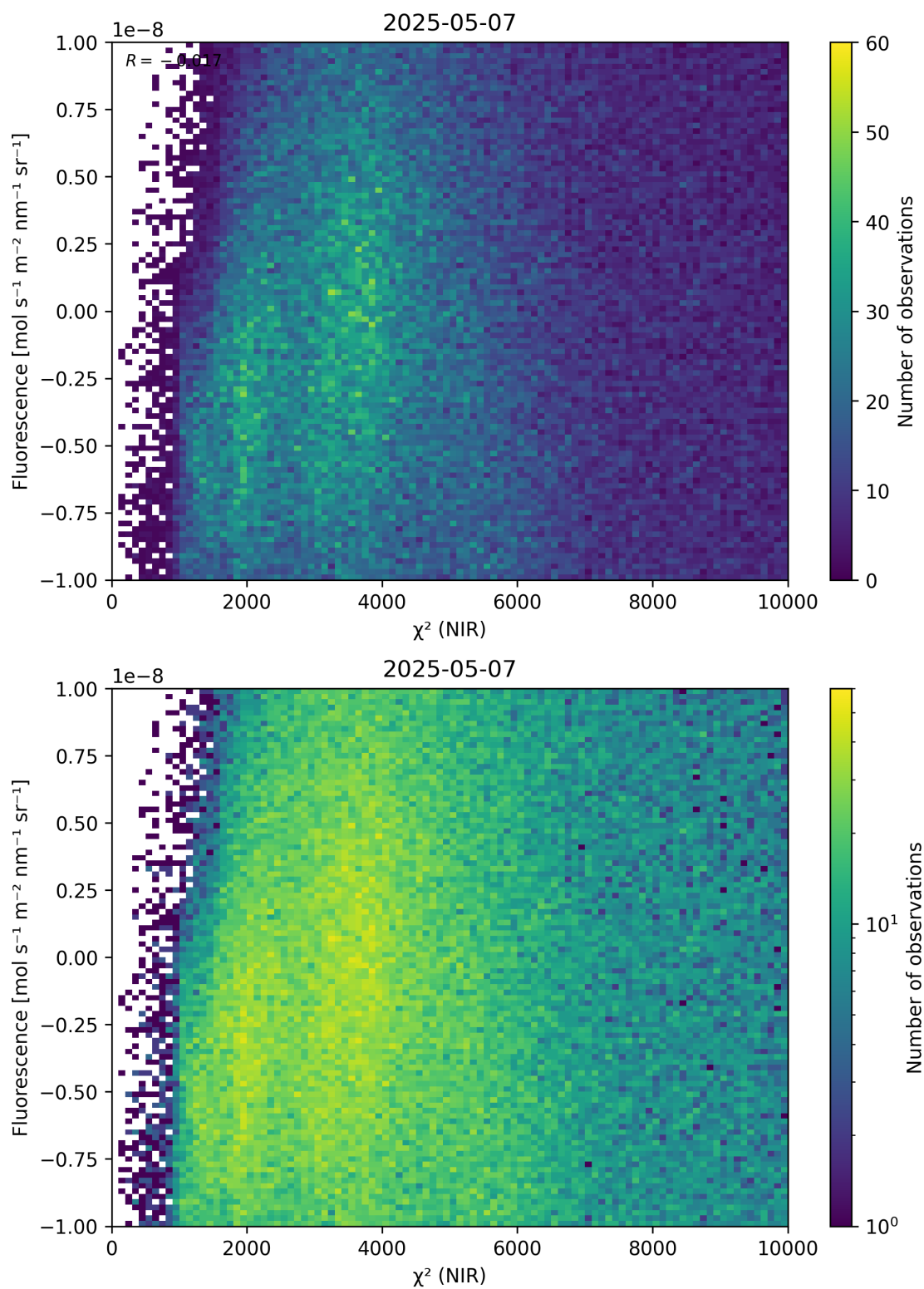
Figure 45: Scatter density plot of “ \chi^2 (NIR)” against “Fluorescence” for 2025-05-06 to 2025-05-08.
