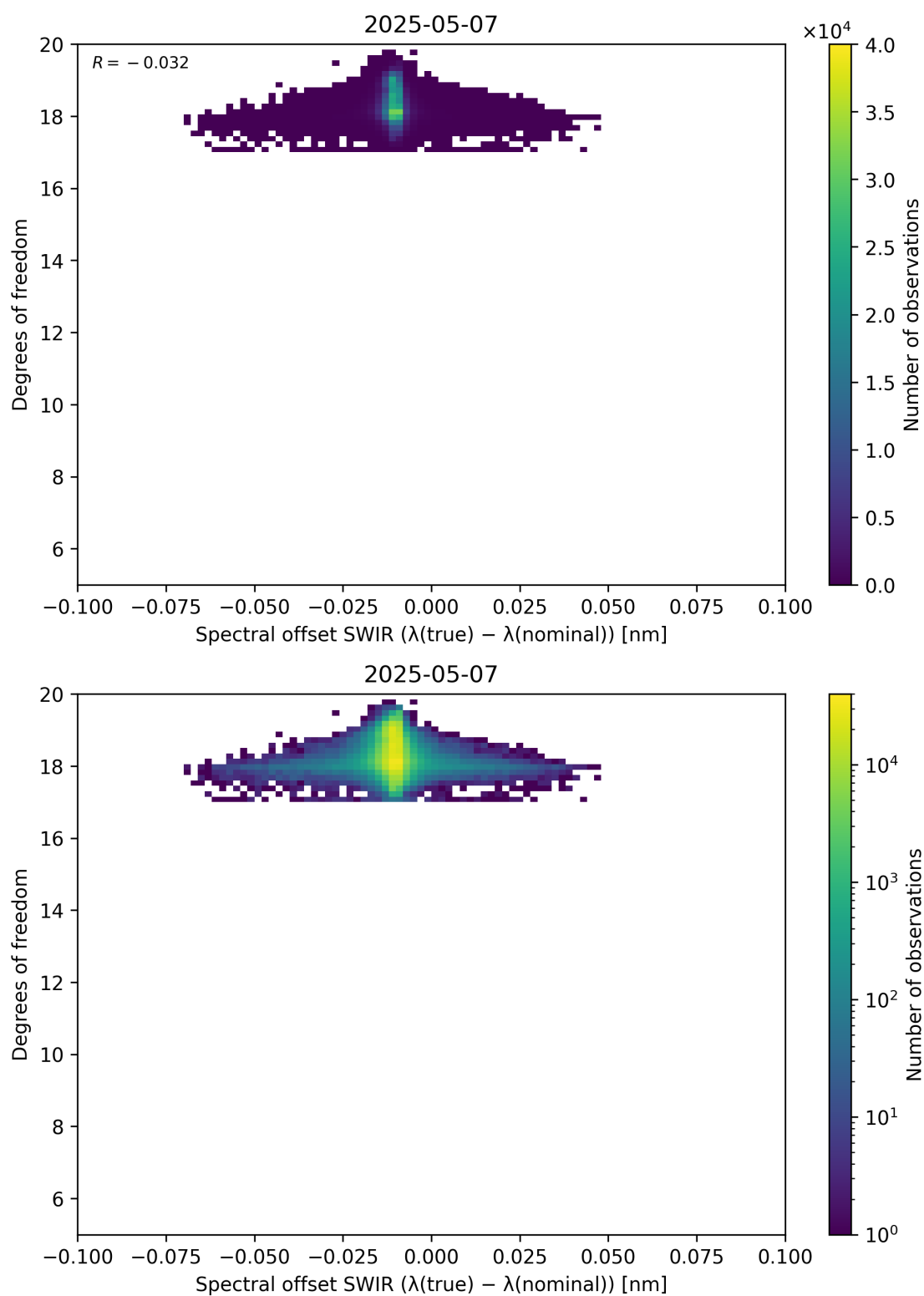
Figure 119: Scatter density plot of “Spectral offset SWIR ( \lambda_{\text{true}} - \lambda_{\text{nominal}} )” against “Degrees of freedom” for 2025-05-06 to 2025-05-08.
