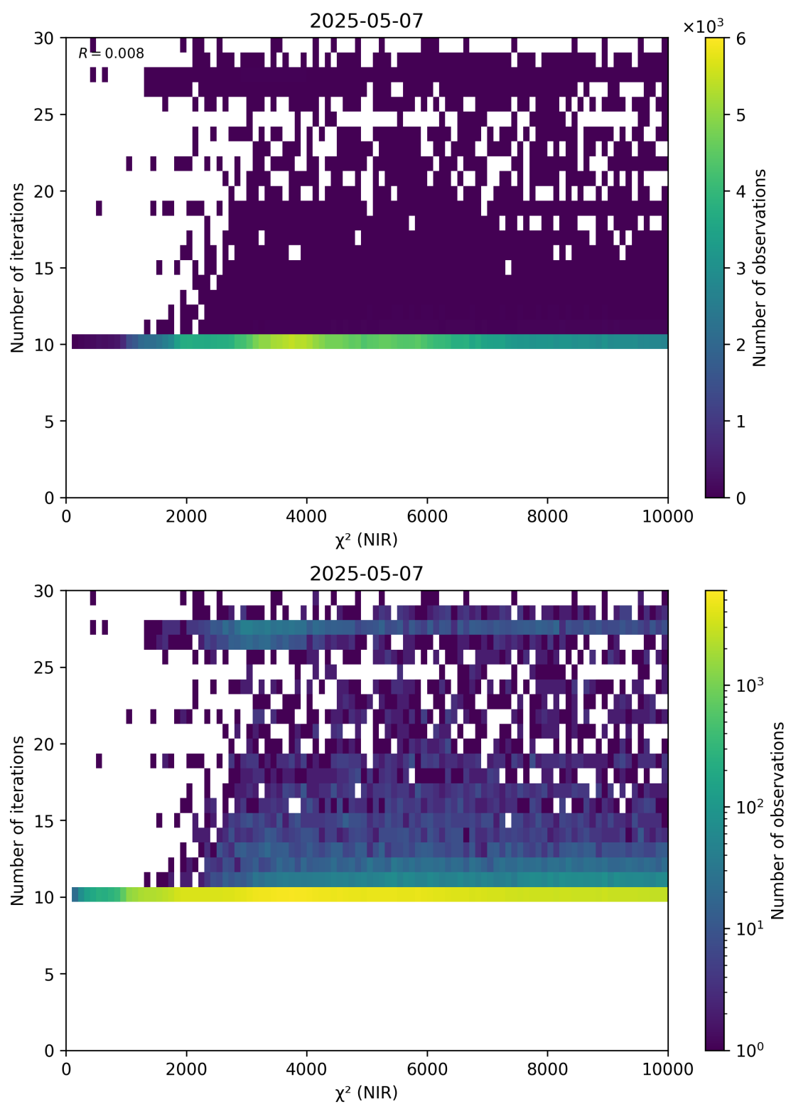
Figure 46: Scatter density plot of “ \chi^2 (NIR)” against “Number of iterations” for 2025-05-06 to 2025-05-08.
