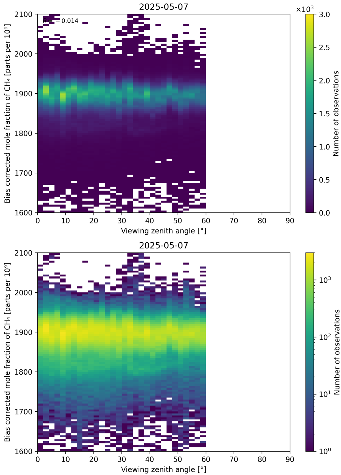
Figure 111: Scatter density plot of “Viewing zenith angle” against “Bias corrected mole fraction of CH 4 ” for 2025-05-06 to 2025-05-08.
