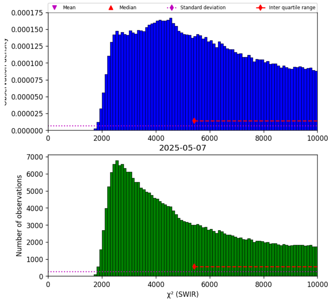
Figure 28: Histogram of “ \chi^2 (SWIR)” for 2025-05-06 to 2025-05-08
