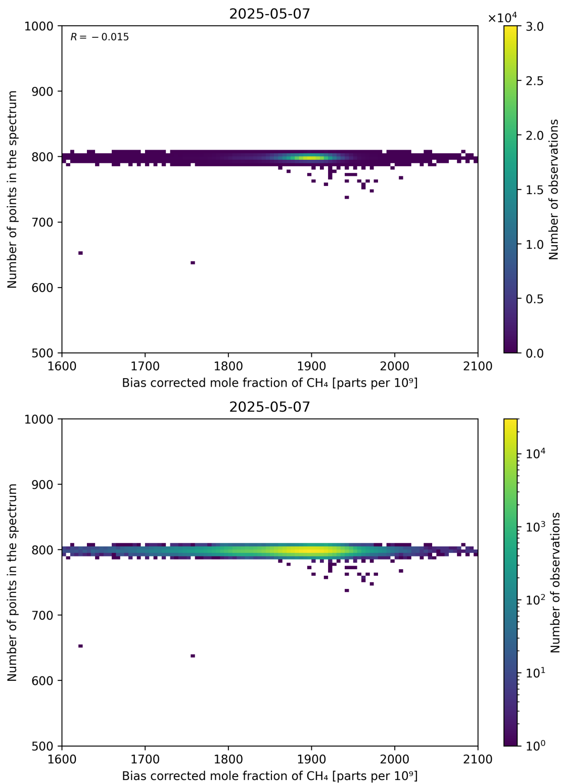
Figure 68: Scatter density plot of “Bias corrected mole fraction of CH 4 ” against “Number of points in the spectrum” for 2025-05-06 to 2025-05-08.
