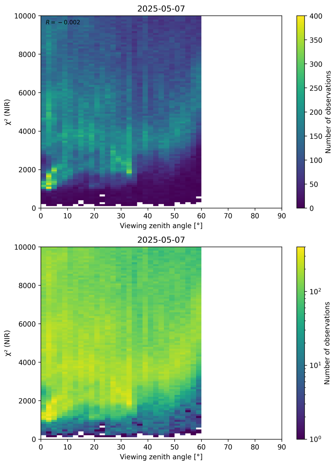
Figure 105: Scatter density plot of “Viewing zenith angle” against “ \chi^2 (NIR)” for 2025-05-06 to 2025-05-08.
