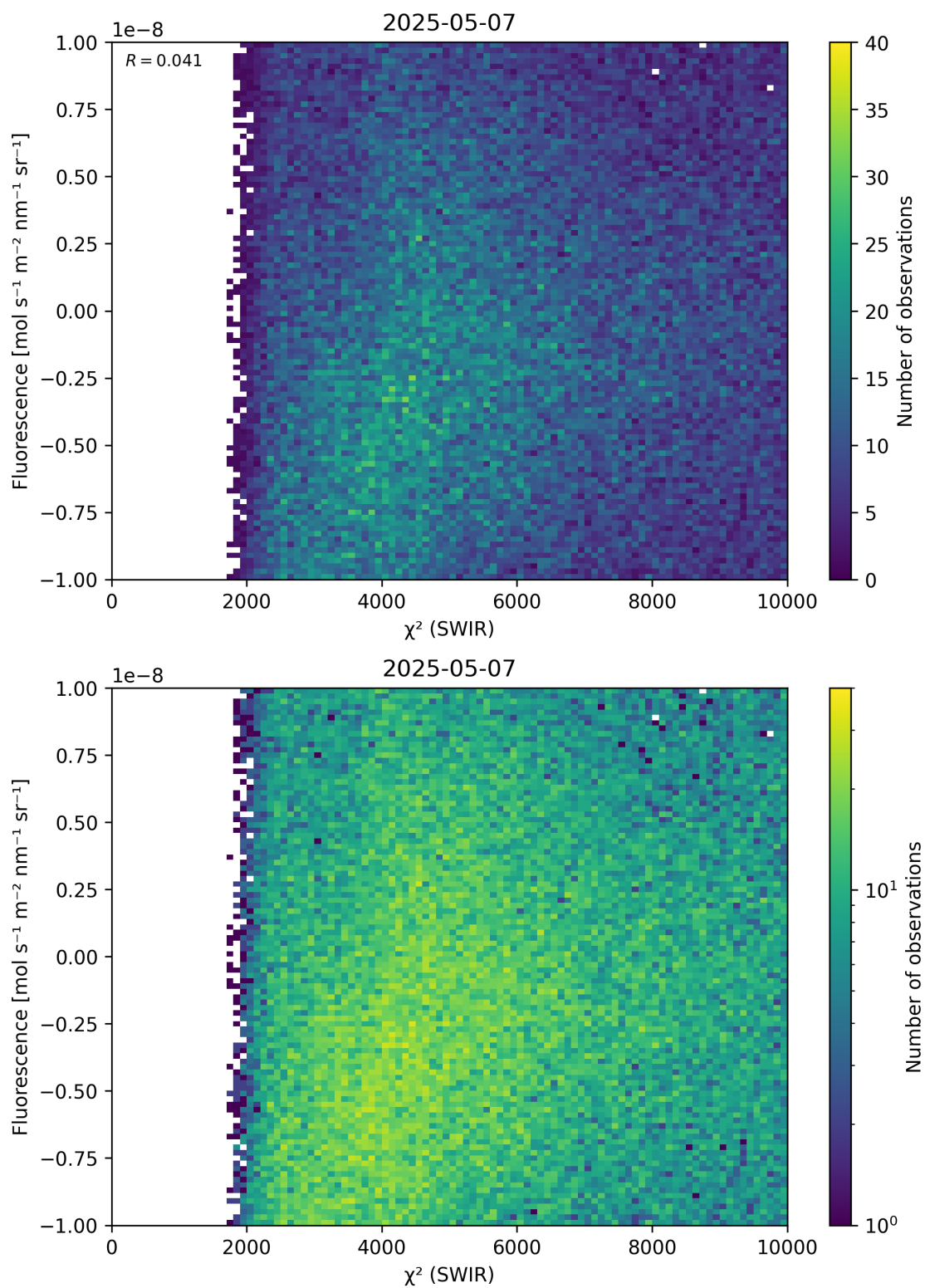
Figure 49: Scatter density plot of “ \chi^2 (SWIR)” against “Fluorescence” for 2025-05-06 to 2025-05-08.
