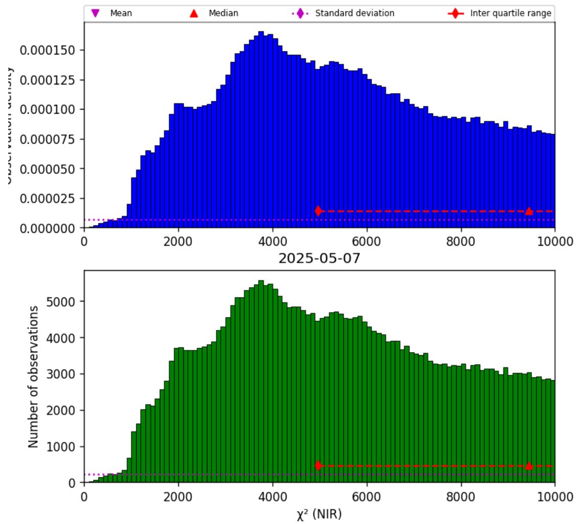
Figure 29: Histogram of “ \chi^2 (NIR)” for 2025-05-06 to 2025-05-08
