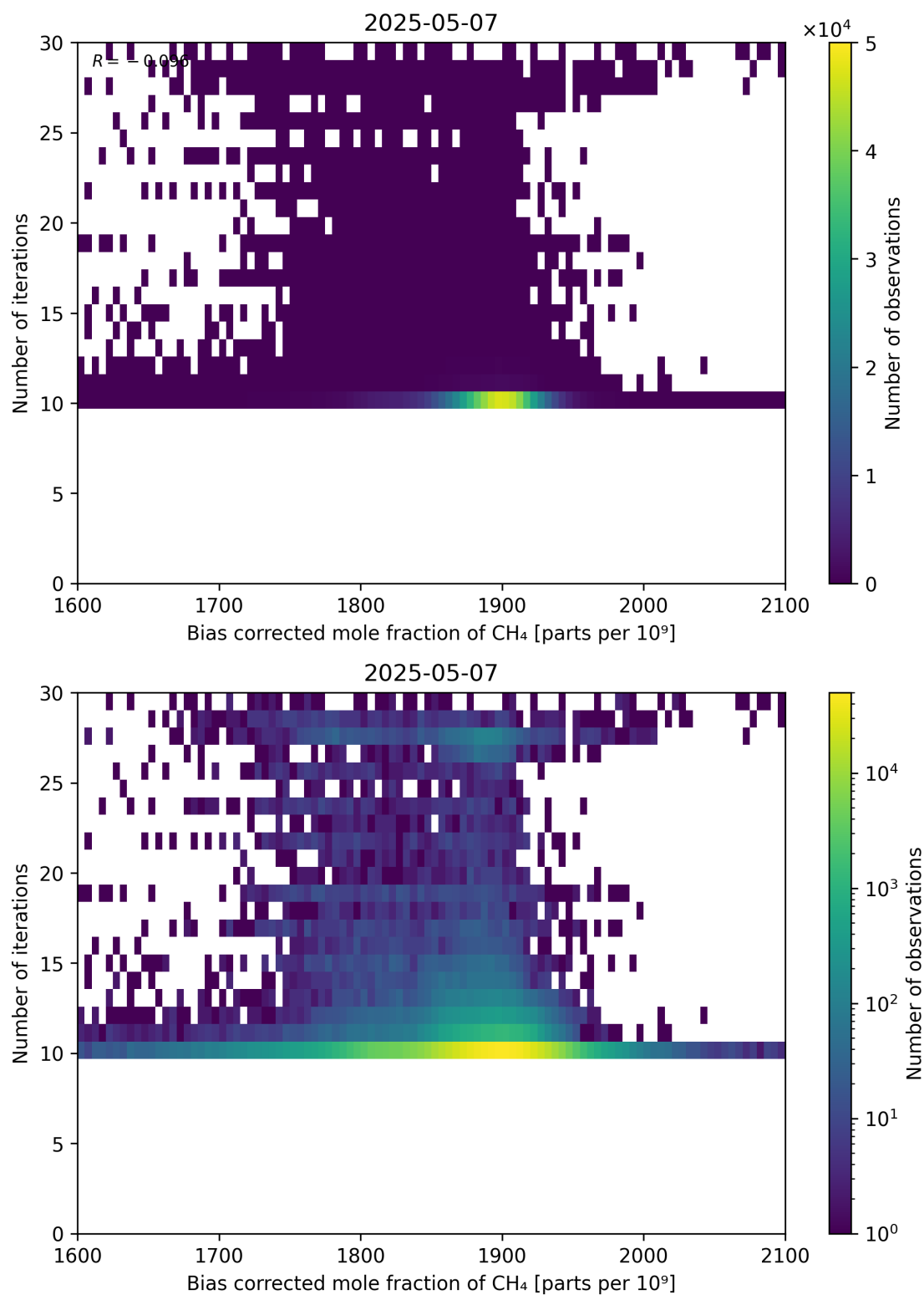
Figure 67: Scatter density plot of “Bias corrected mole fraction of CH 4 ” against “Number of iterations” for 2025-05-06 to 2025-05-08.
