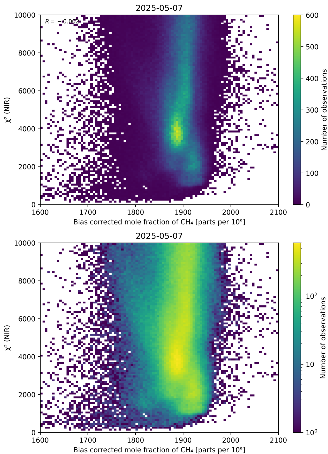
Figure 63: Scatter density plot of “Bias corrected mole fraction of CH 4 ” against “ \chi^2 (NIR)” for 2025-05-06 to 2025-05-08.
