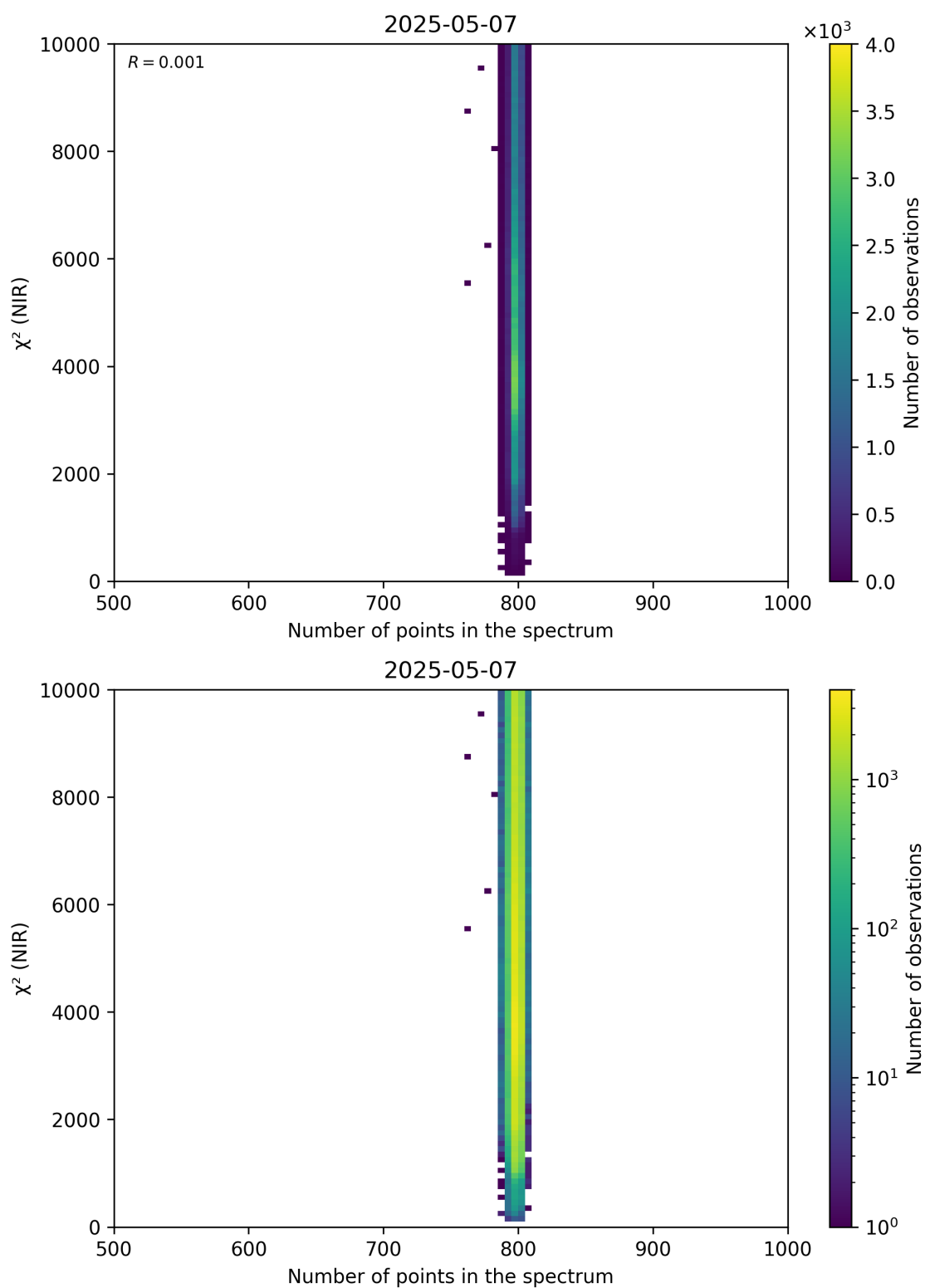
Figure 88: Scatter density plot of “Number of points in the spectrum” against “ \chi^2 (NIR)” for 2025-05-06 to 2025-05-08.
