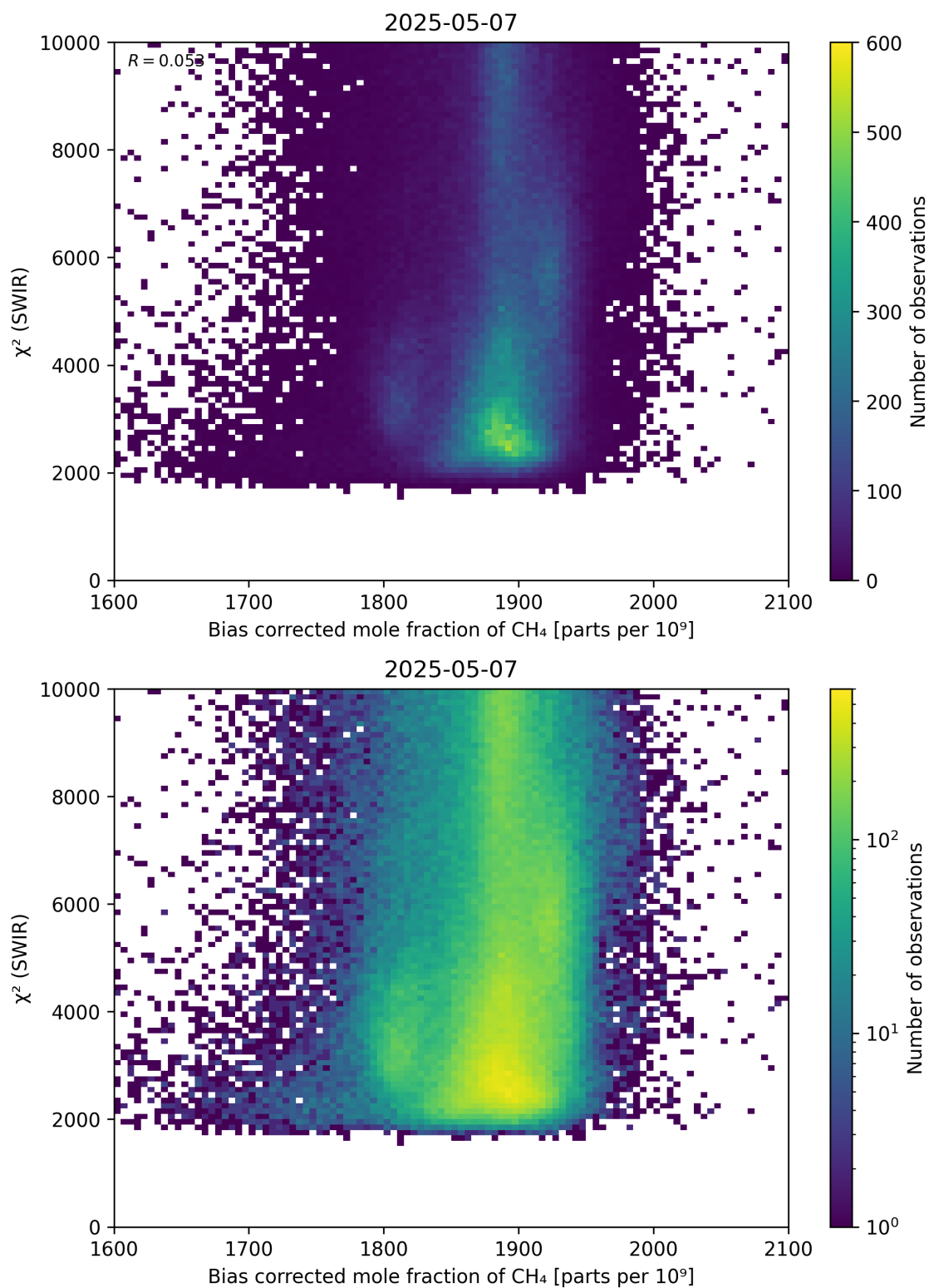
Figure 64: Scatter density plot of “Bias corrected mole fraction of \text{CH}_4 ” against “ \chi^2 (SWIR)” for 2025-05-06 to 2025-05-08.
