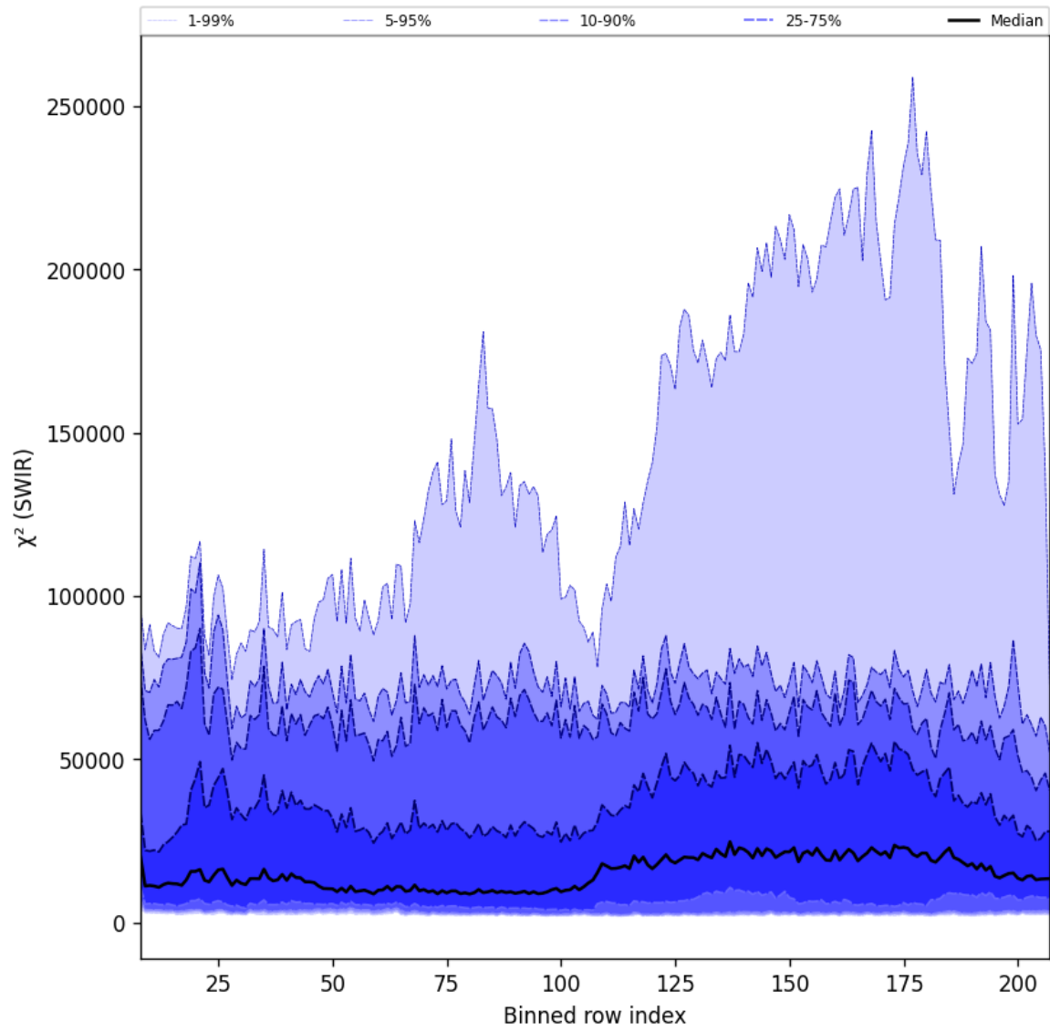
Figure 39: Along track statistics of " \chi^2 (SWIR)" for 2025-05-06 to 2025-05-08
