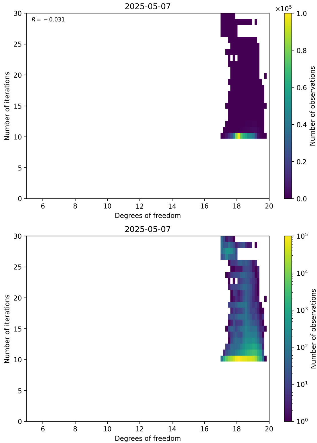
Figure 52: Scatter density plot of “Degrees of freedom” against “Number of iterations” for 2025-05-06 to 2025-05-08.
