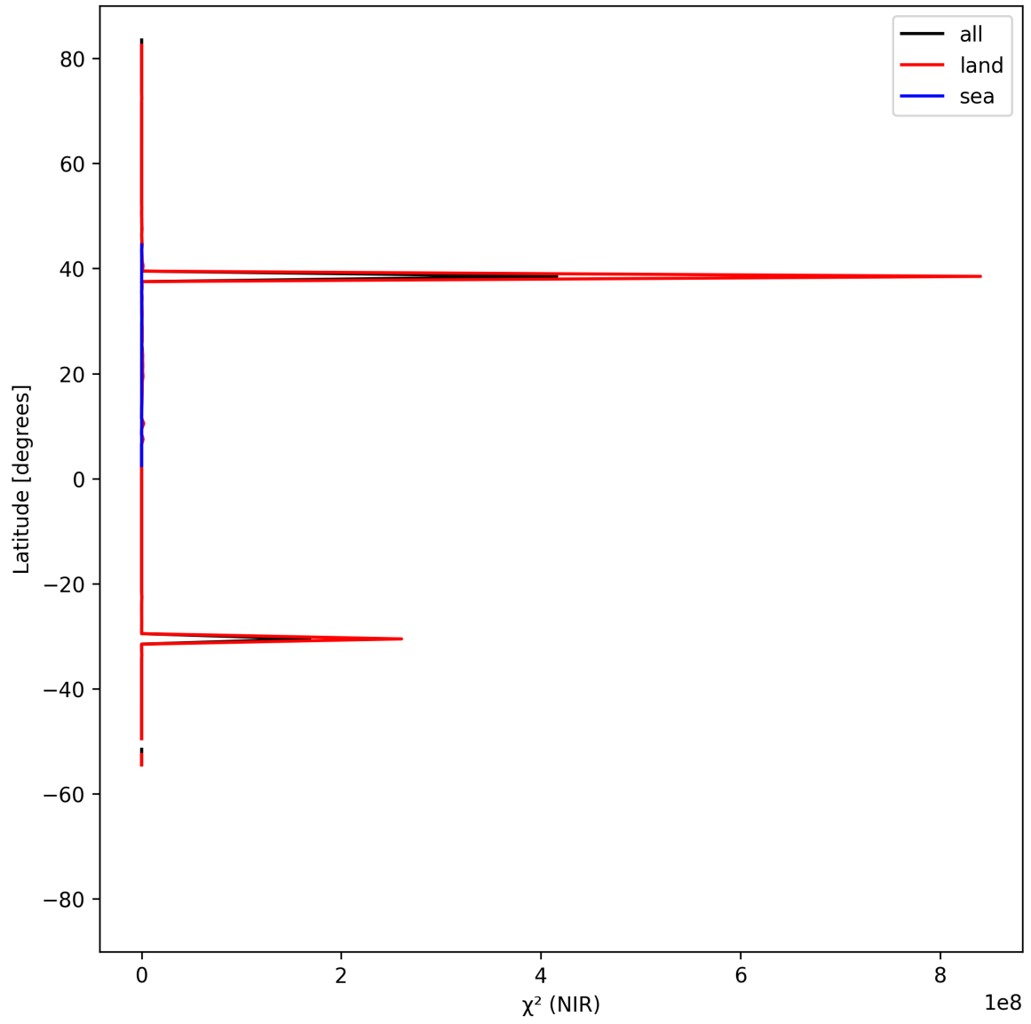
Figure 18: Zonal average of “ \chi^2 (NIR)” for 2025-05-06 to 2025-05-08.
