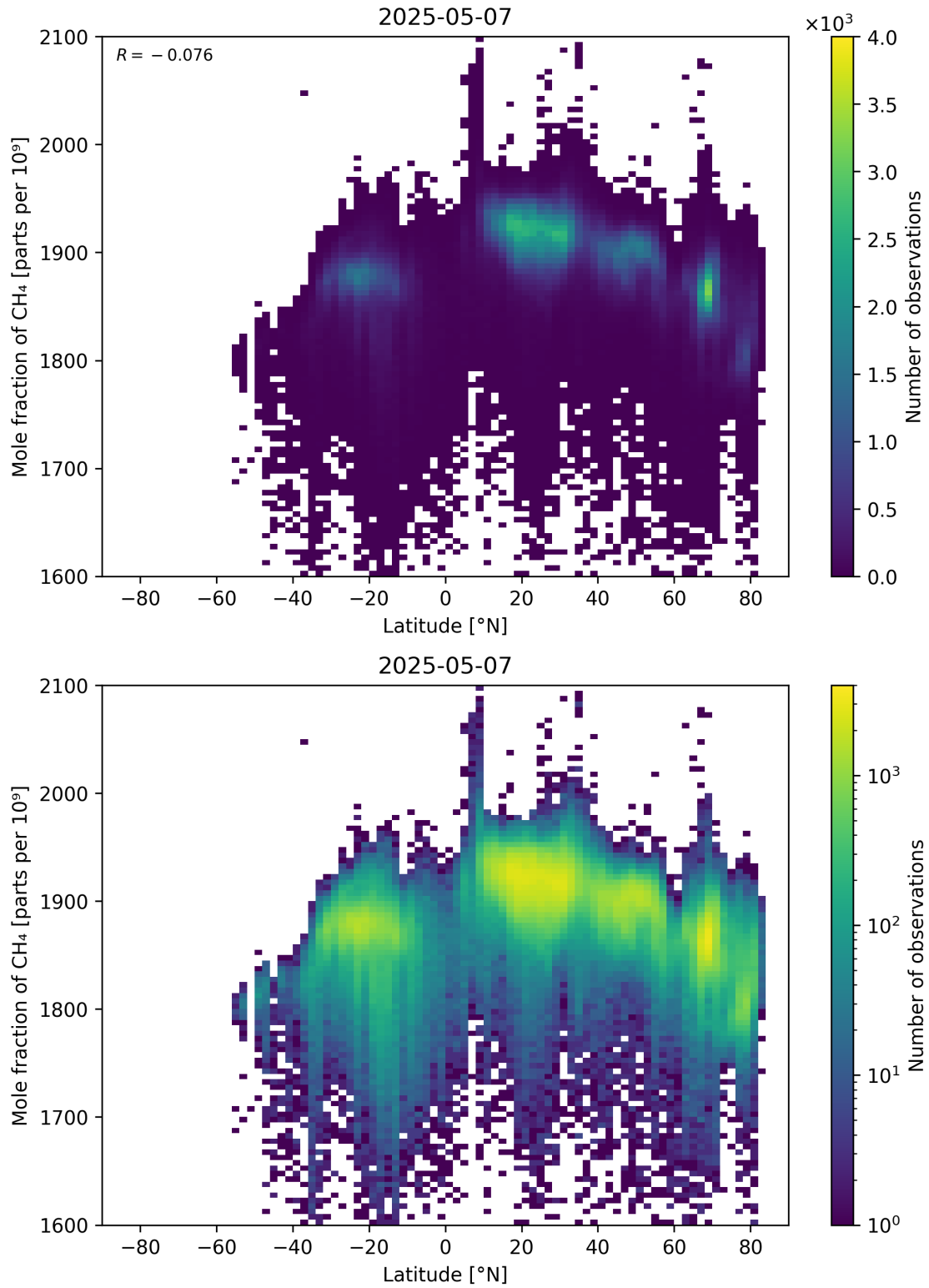
Figure 57: Scatter density plot of “Latitude” against “Mole fraction of CH 4 ” for 2025-05-06 to 2025-05-08.
