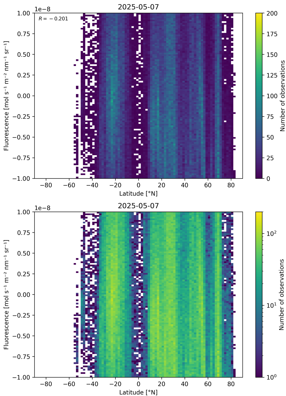
Figure 56: Scatter density plot of “Latitude” against “Fluorescence” for 2025-05-06 to 2025-05-08.
