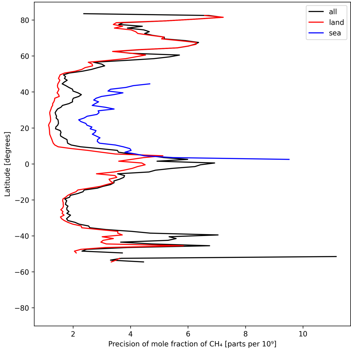
Figure 13: Zonal average of “Precision of mole fraction of CH 4 ” for 2025-05-06 to 2025-05-08.
