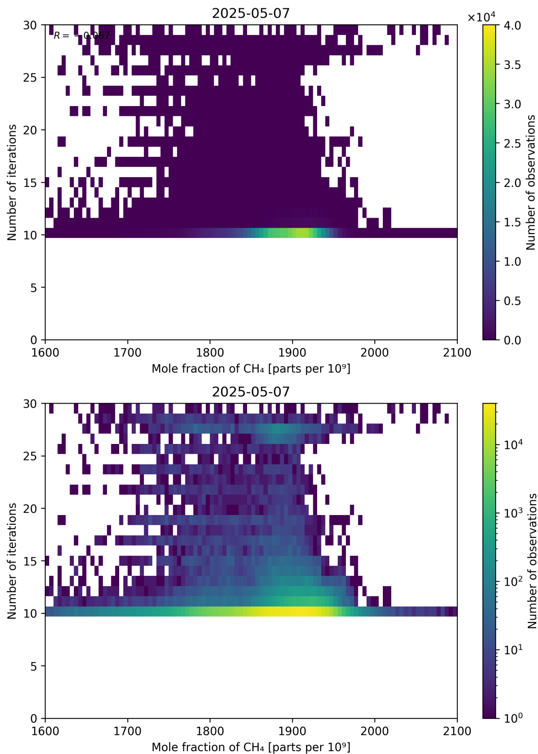
Figure 76: Scatter density plot of “Mole fraction of CH 4 ” against “Number of iterations” for 2025-05-06 to 2025-05-08.
