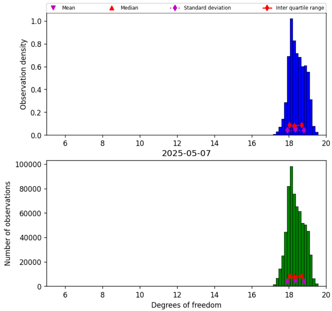
Figure 30: Histogram of "Degrees of freedom" for 2025-05-06 to 2025-05-08
