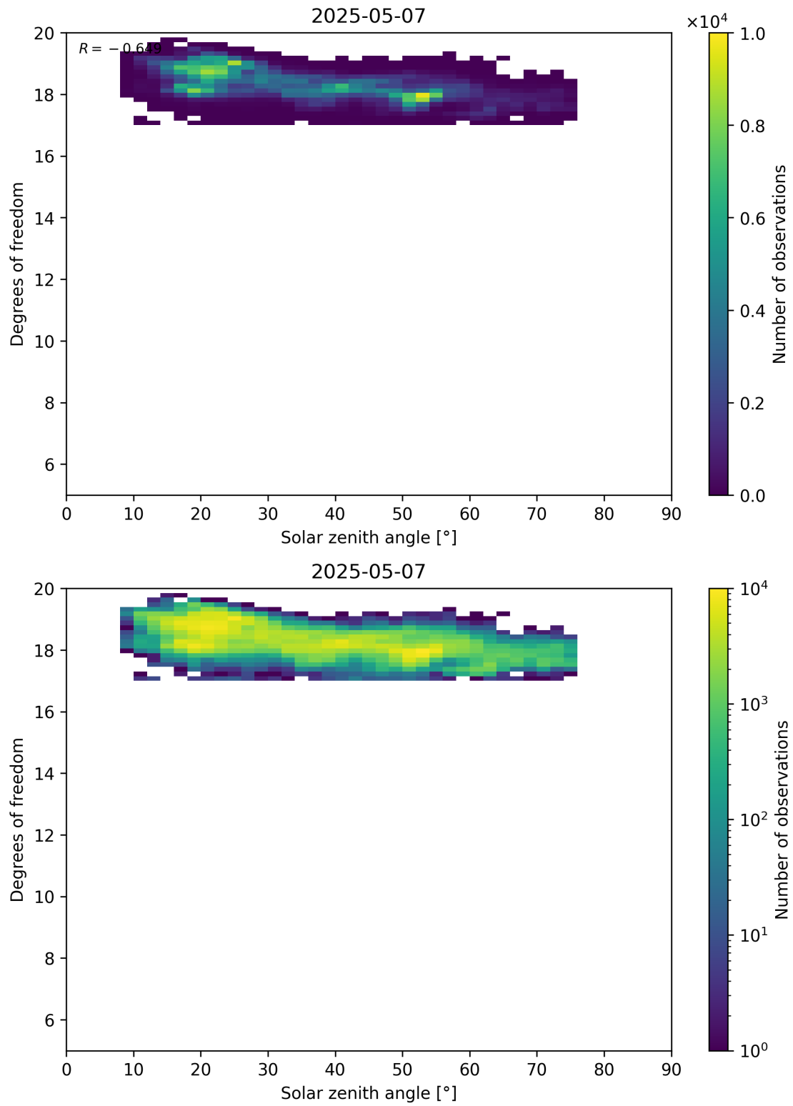
Figure 96: Scatter density plot of “Solar zenith angle” against “Degrees of freedom” for 2025-05-06 to 2025-05-08.
