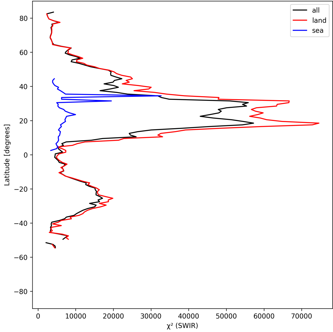
Figure 17: Zonal average of “ \chi^2 (SWIR)” for 2025-05-06 to 2025-05-08.
