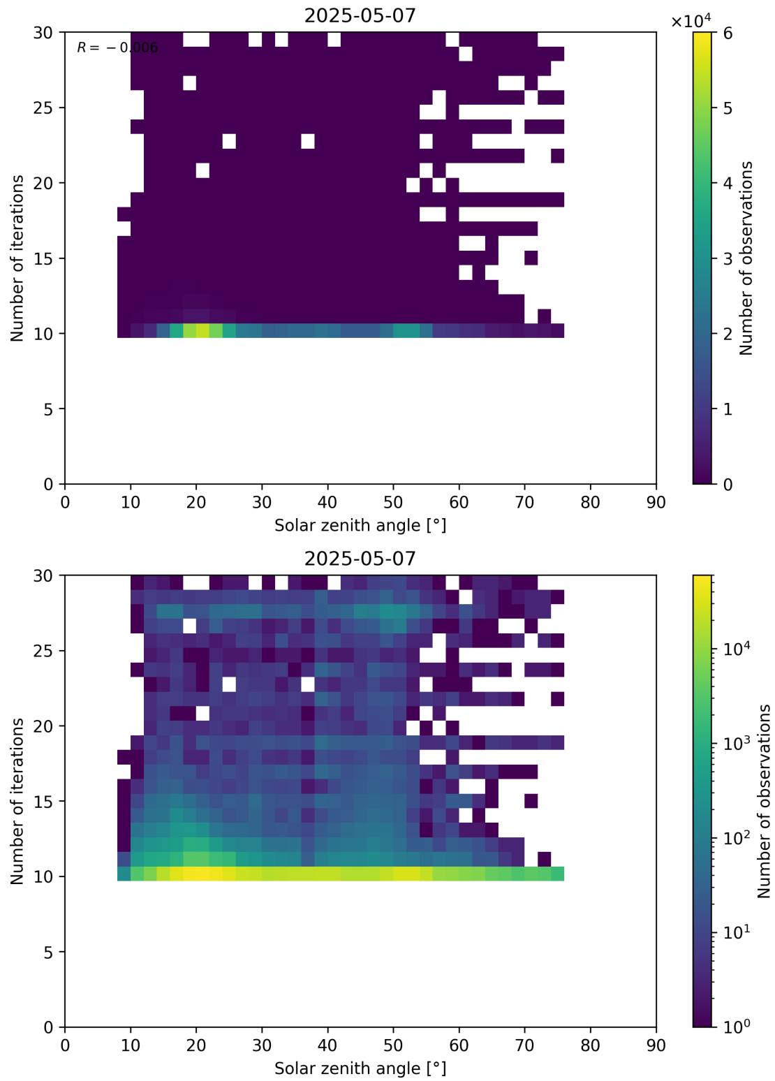
Figure 102: Scatter density plot of “Solar zenith angle” against “Number of iterations” for 2025-05-06 to 2025-05-08.
