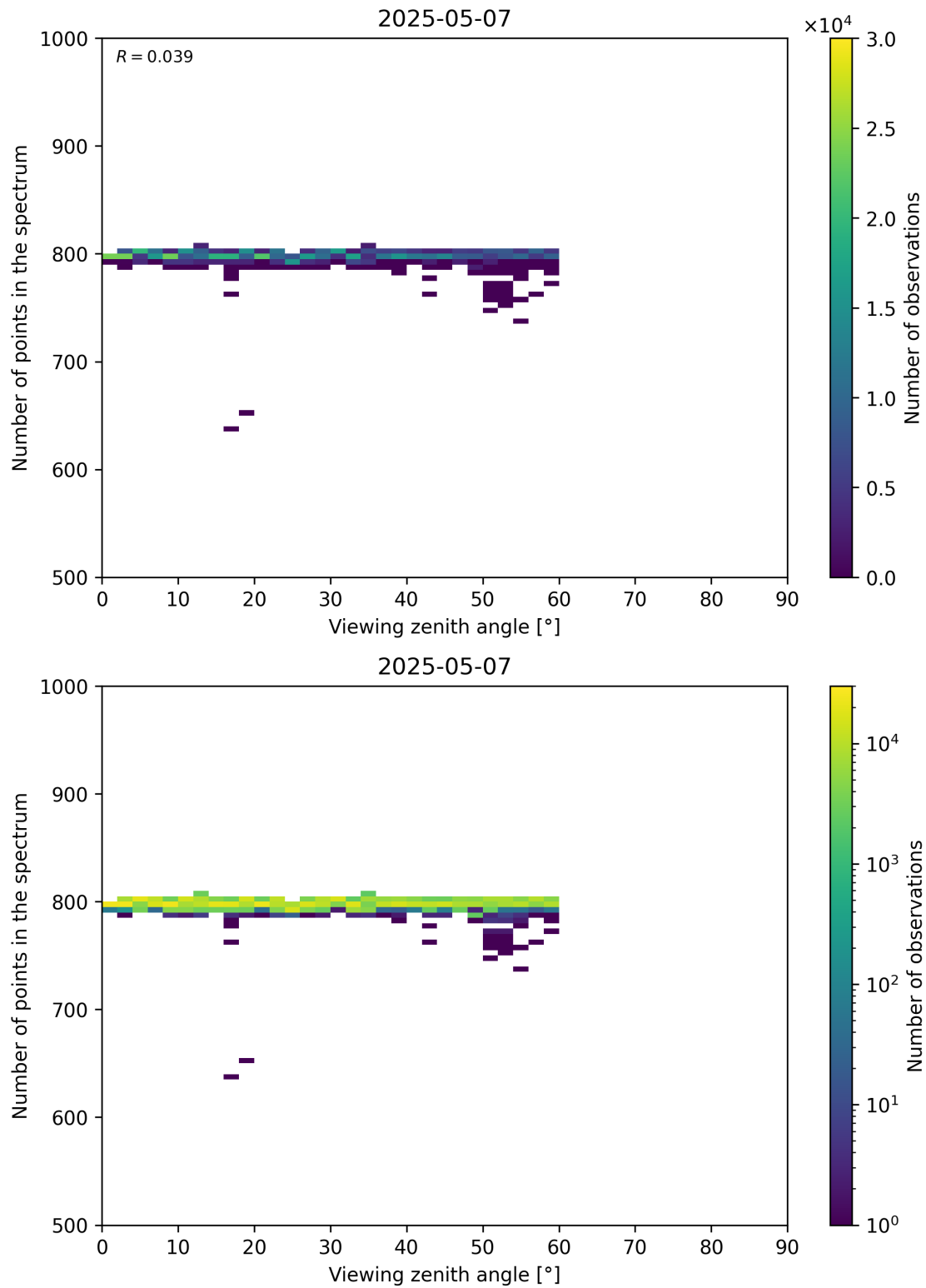
Figure 114: Scatter density plot of “Viewing zenith angle” against “Number of points in the spectrum” for 2025-05-06 to 2025-05-08.
