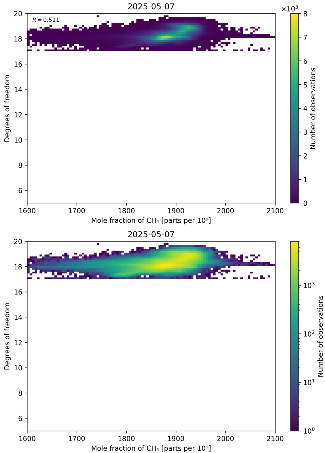
Figure 72: Scatter density plot of “Mole fraction of CH 4 ” against “Degrees of freedom” for 2025-05-06 to 2025-05-08.
