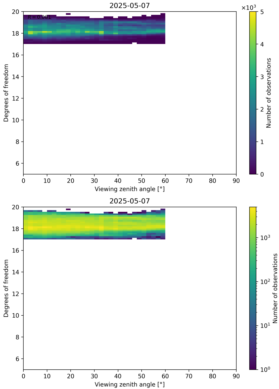
Figure 107: Scatter density plot of “Viewing zenith angle” against “Degrees of freedom” for 2025-05-06 to 2025-05-08.
