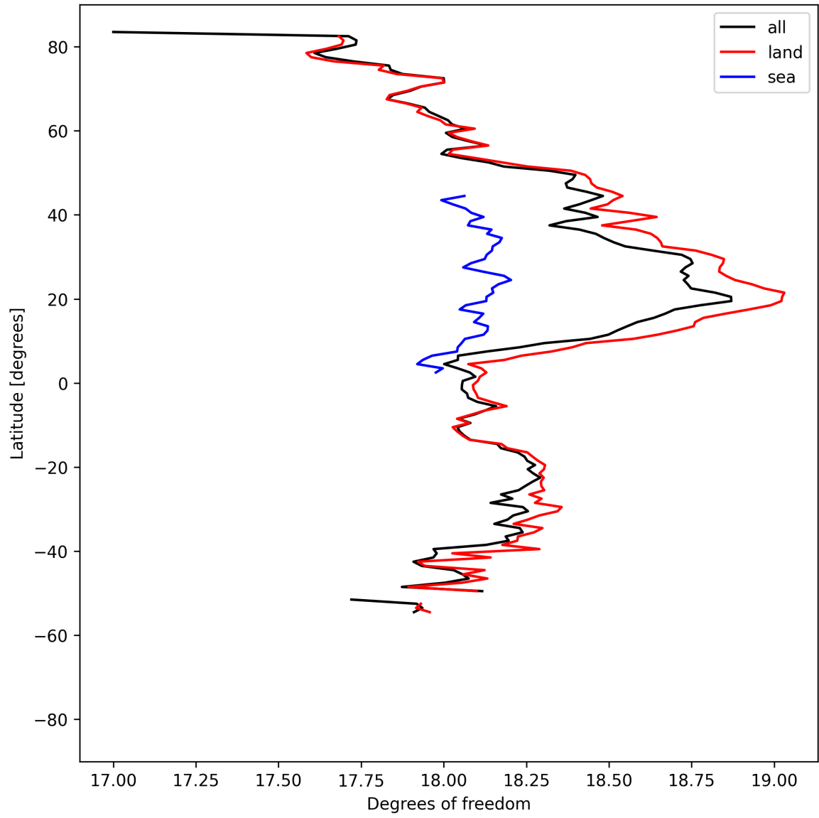
Figure 19: Zonal average of “Degrees of freedom” for 2025-05-06 to 2025-05-08.
