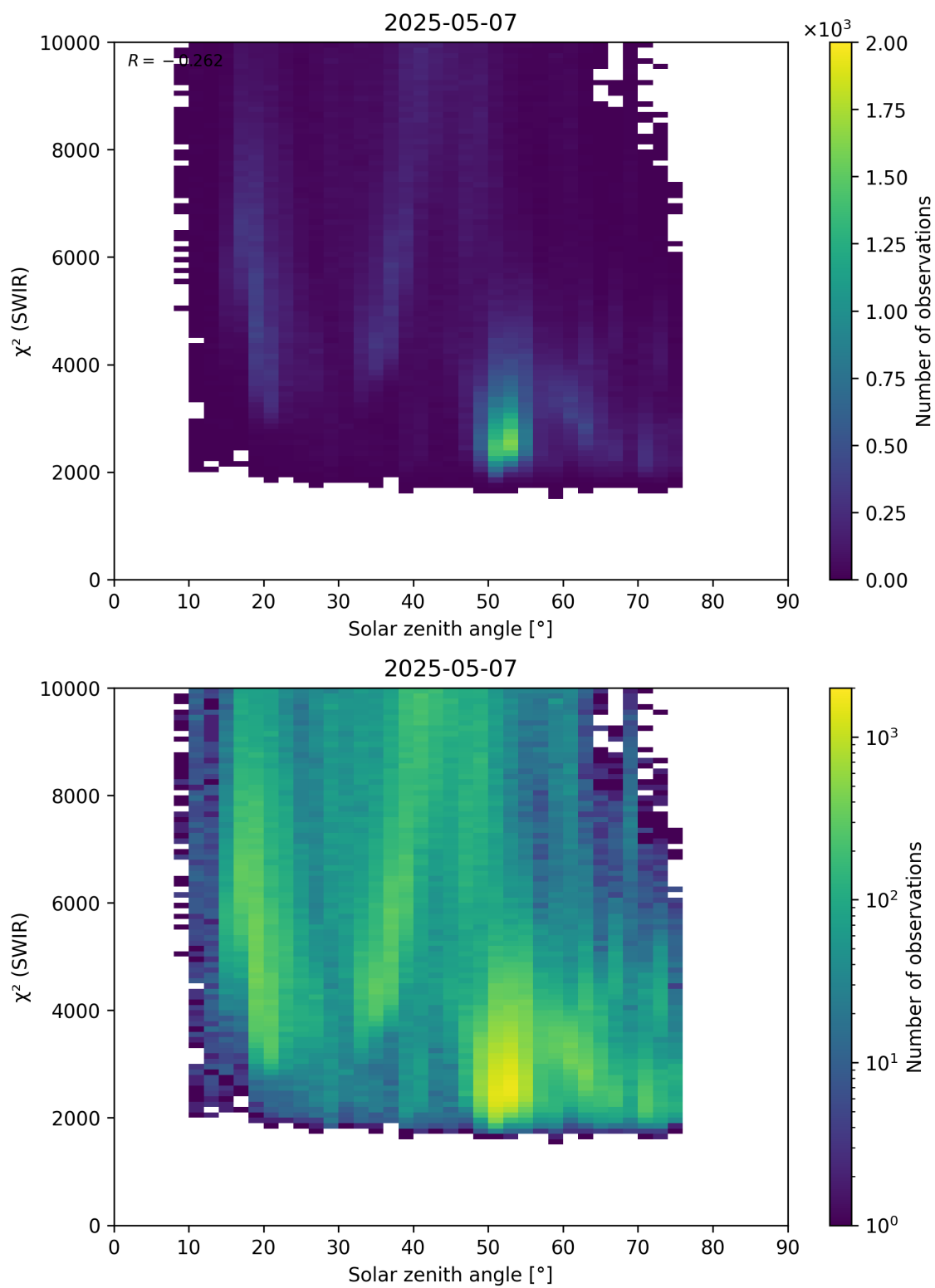
Figure 95: Scatter density plot of “Solar zenith angle” against “ \chi^2 (SWIR)” for 2025-05-06 to 2025-05-08.
