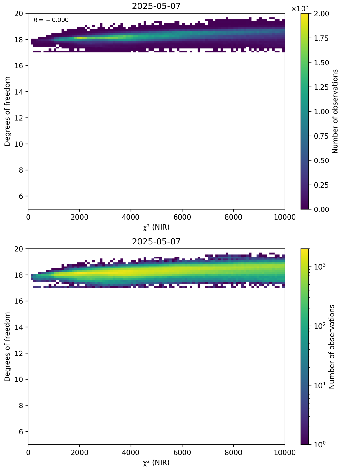
Figure 44: Scatter density plot of “ \chi^2 (NIR)” against “Degrees of freedom” for 2025-05-06 to 2025-05-08.
