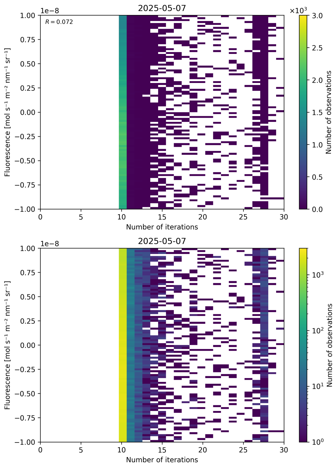
Figure 87: Scatter density plot of “Number of iterations” against “Fluorescence” for 2025-05-06 to 2025-05-08.
