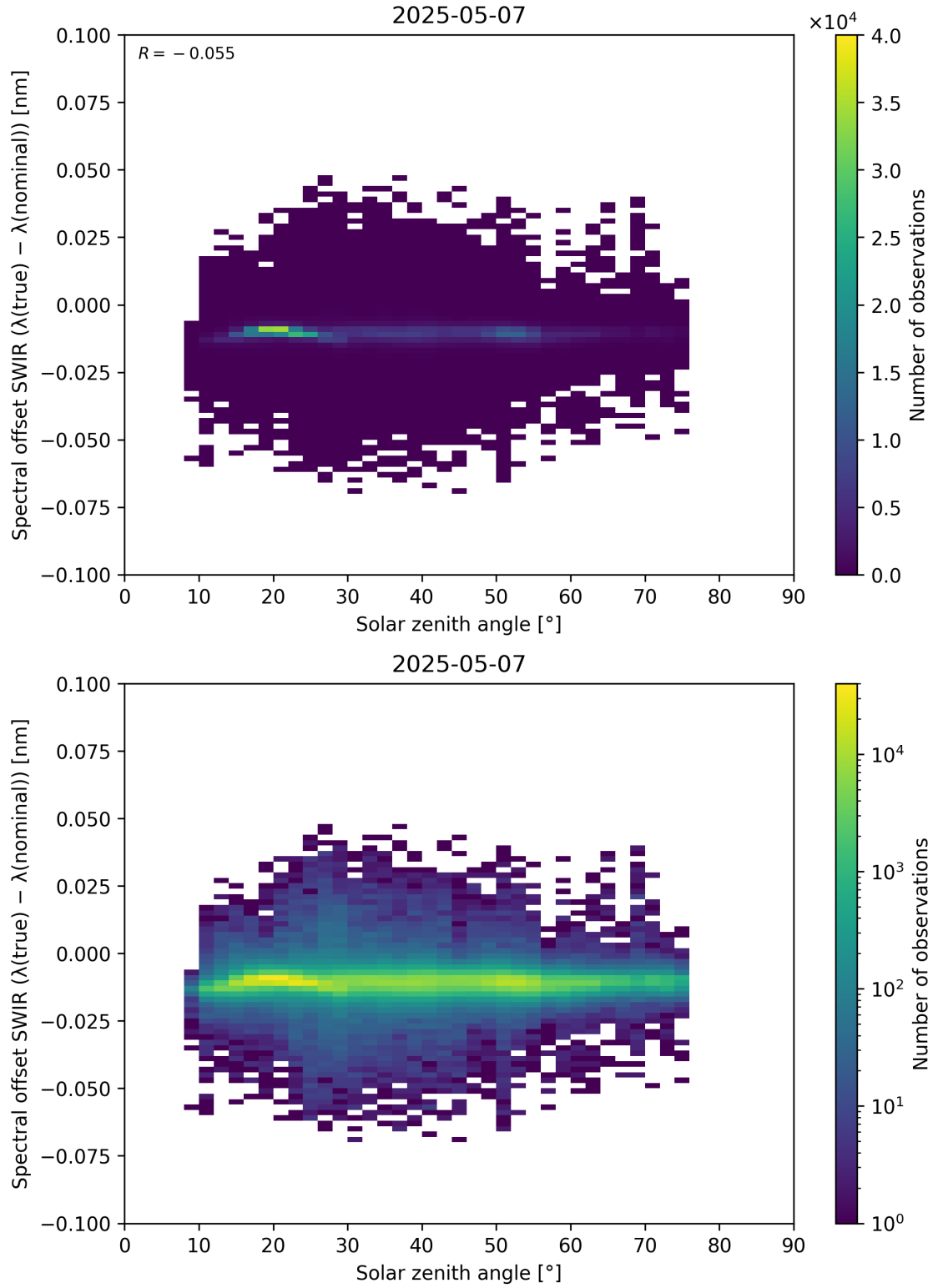
Figure 104: Scatter density plot of “Solar zenith angle” against “Spectral offset SWIR ( \lambda_{\text{true}} - \lambda_{\text{nominal}} )” for 2025-05-06 to 2025-05-08.
