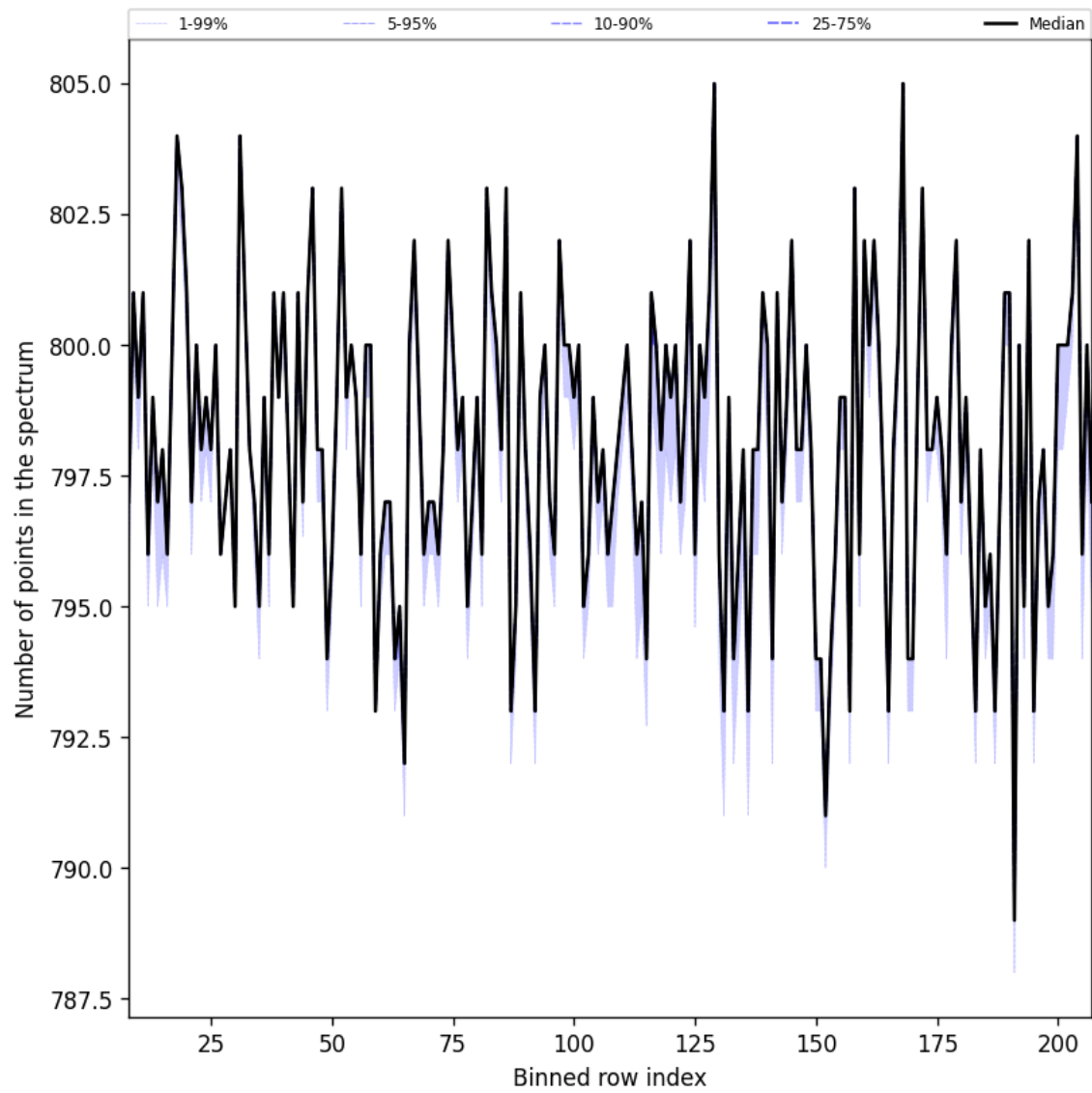
Figure 37: Along track statistics of “Number of points in the spectrum” for 2025-05-06 to 2025-05-08
