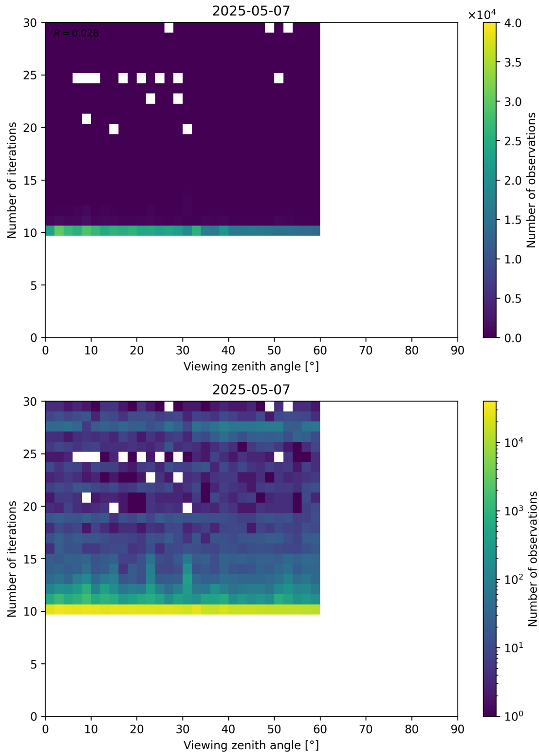
Figure 113: Scatter density plot of “Viewing zenith angle” against “Number of iterations” for 2025-05-06 to 2025-05-08.
