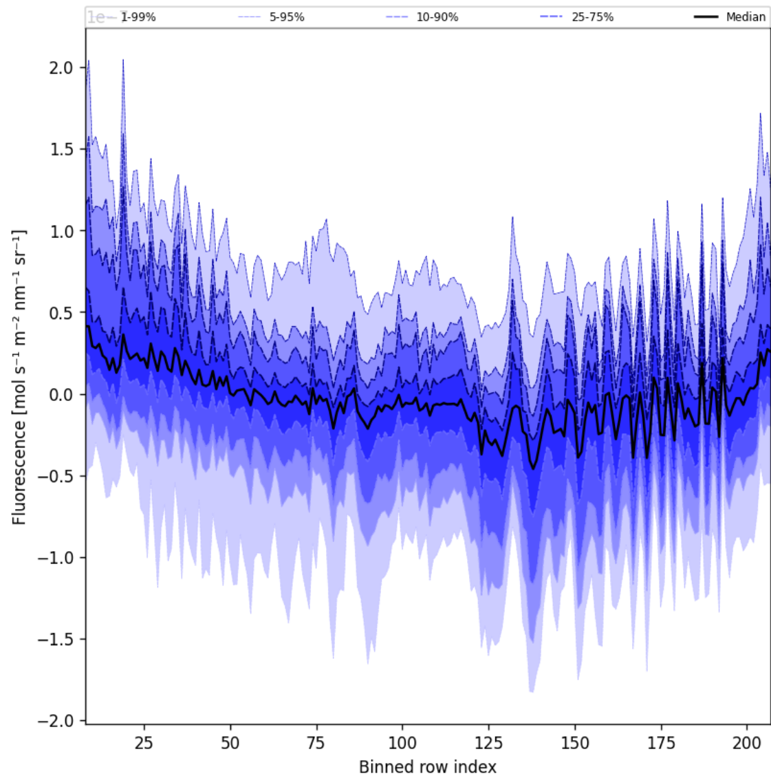
Figure 43: Along track statistics of “Fluorescence” for 2025-05-06 to 2025-05-08
