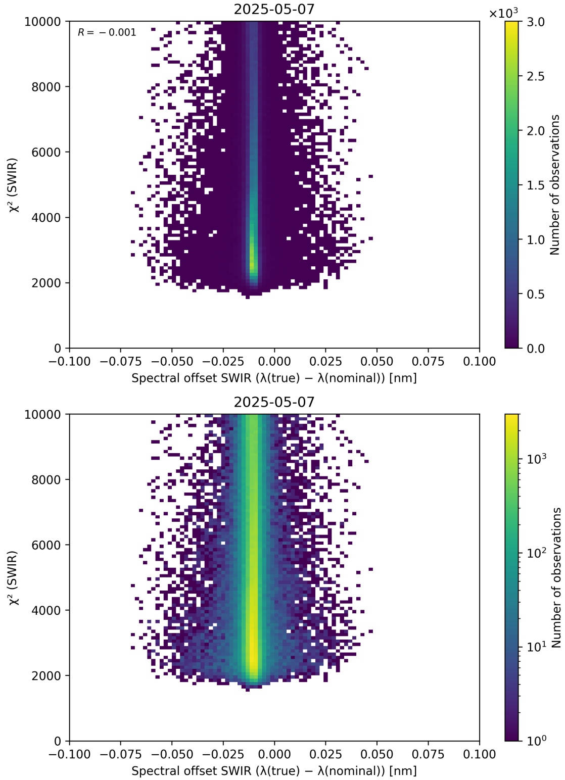
Figure 118: Scatter density plot of “Spectral offset SWIR ( \lambda_{\text{true}} - \lambda_{\text{nominal}} )” against “ \chi^2 (SWIR)” for 2025-05-06 to 2025-05-08.
