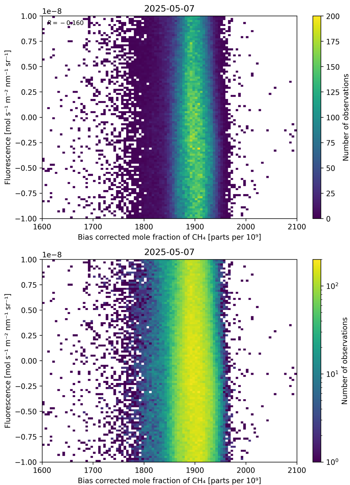
Figure 66: Scatter density plot of “Bias corrected mole fraction of \text{CH}_4 ” against “Fluorescence” for 2025-05-06 to 2025-05-08.
