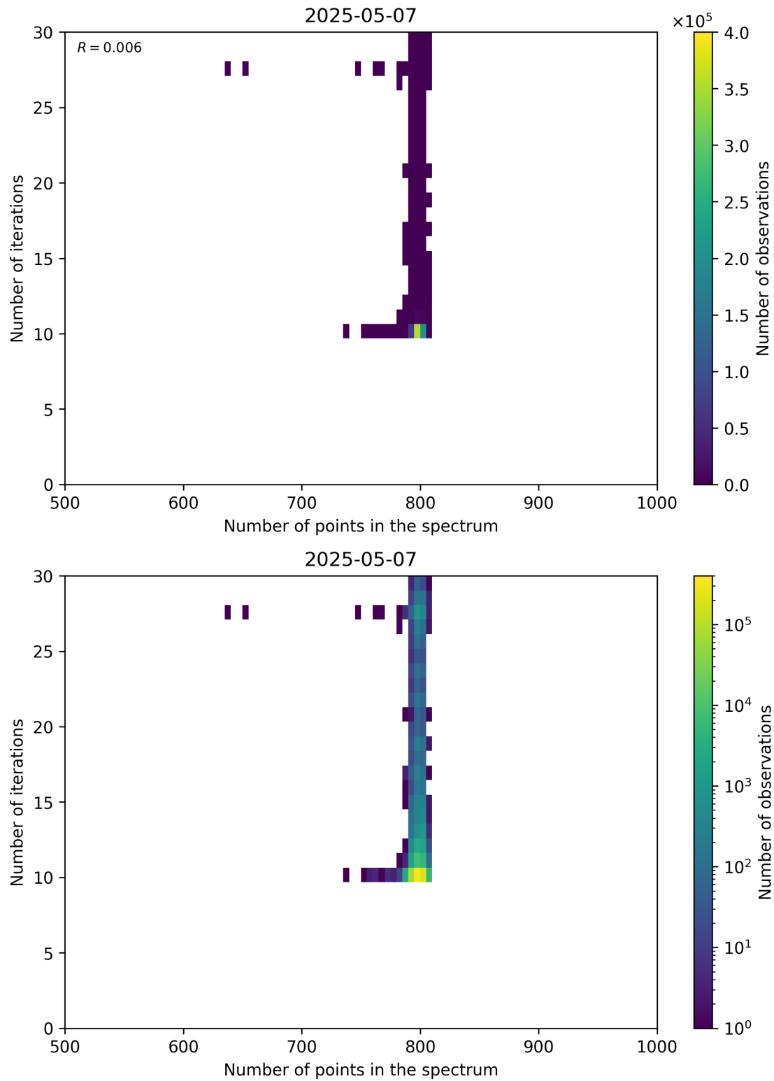
Figure 92: Scatter density plot of “Number of points in the spectrum” against “Number of iterations” for 2025-05-06 to 2025-05-08.
