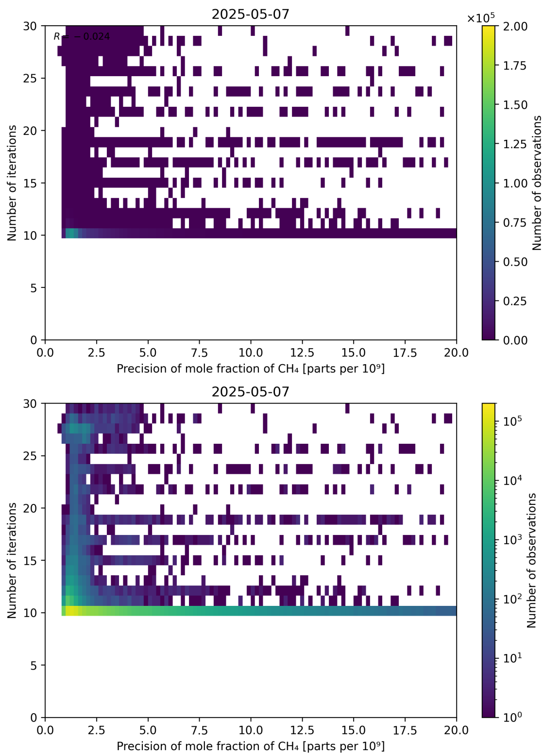
Figure 83: Scatter density plot of “Precision of mole fraction of CH 4 ” against “Number of iterations” for 2025-05-06 to 2025-05-08.
