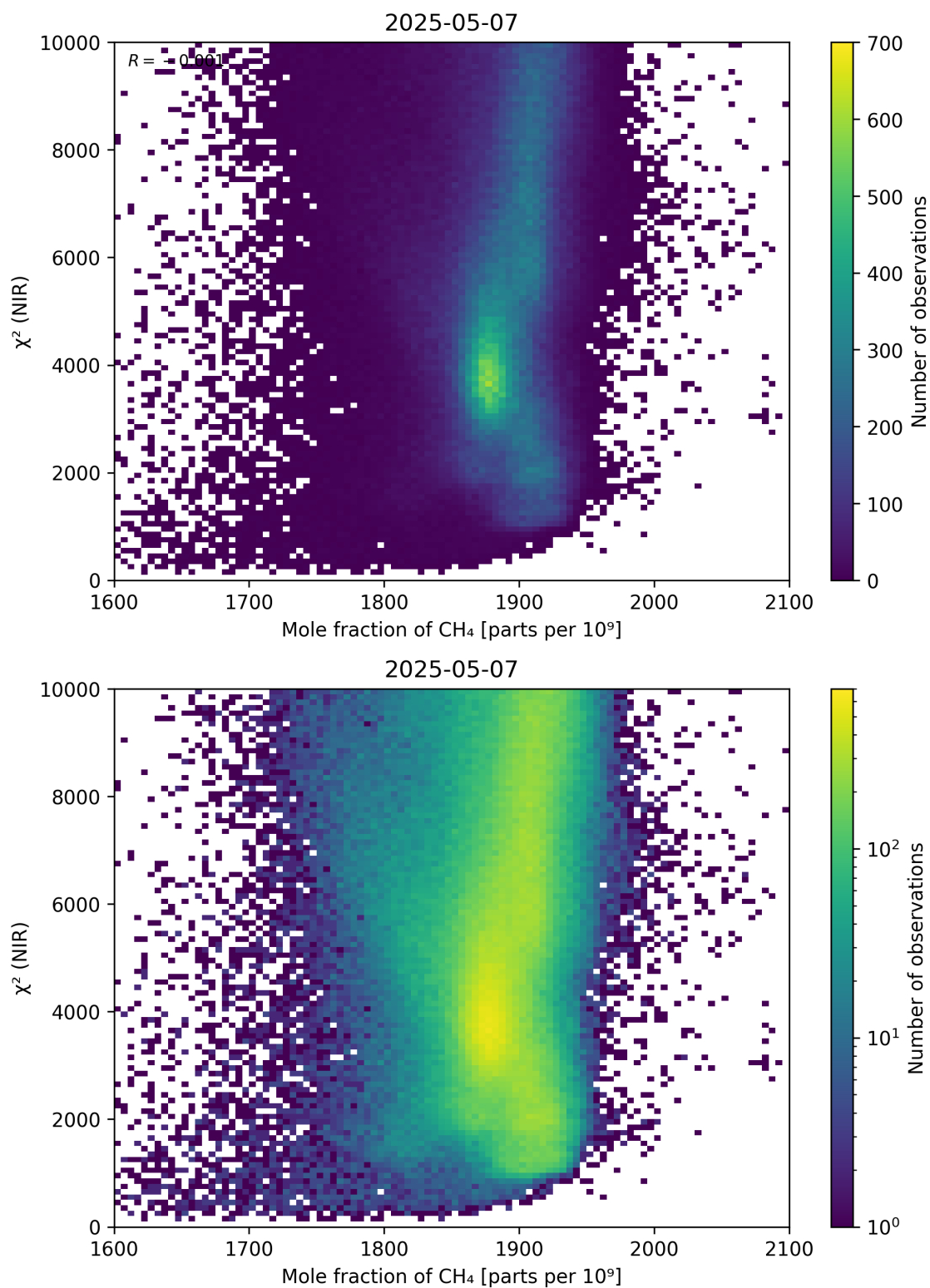
Figure 70: Scatter density plot of “Mole fraction of \text{CH}_4 ” against “ \chi^2 (NIR)” for 2025-05-06 to 2025-05-08.
