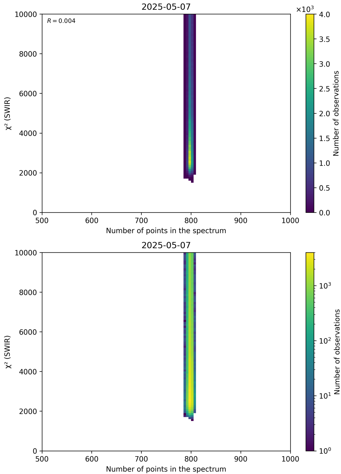
Figure 89: Scatter density plot of “Number of points in the spectrum” against “ \chi^2 (SWIR)” for 2025-05-06 to 2025-05-08.
