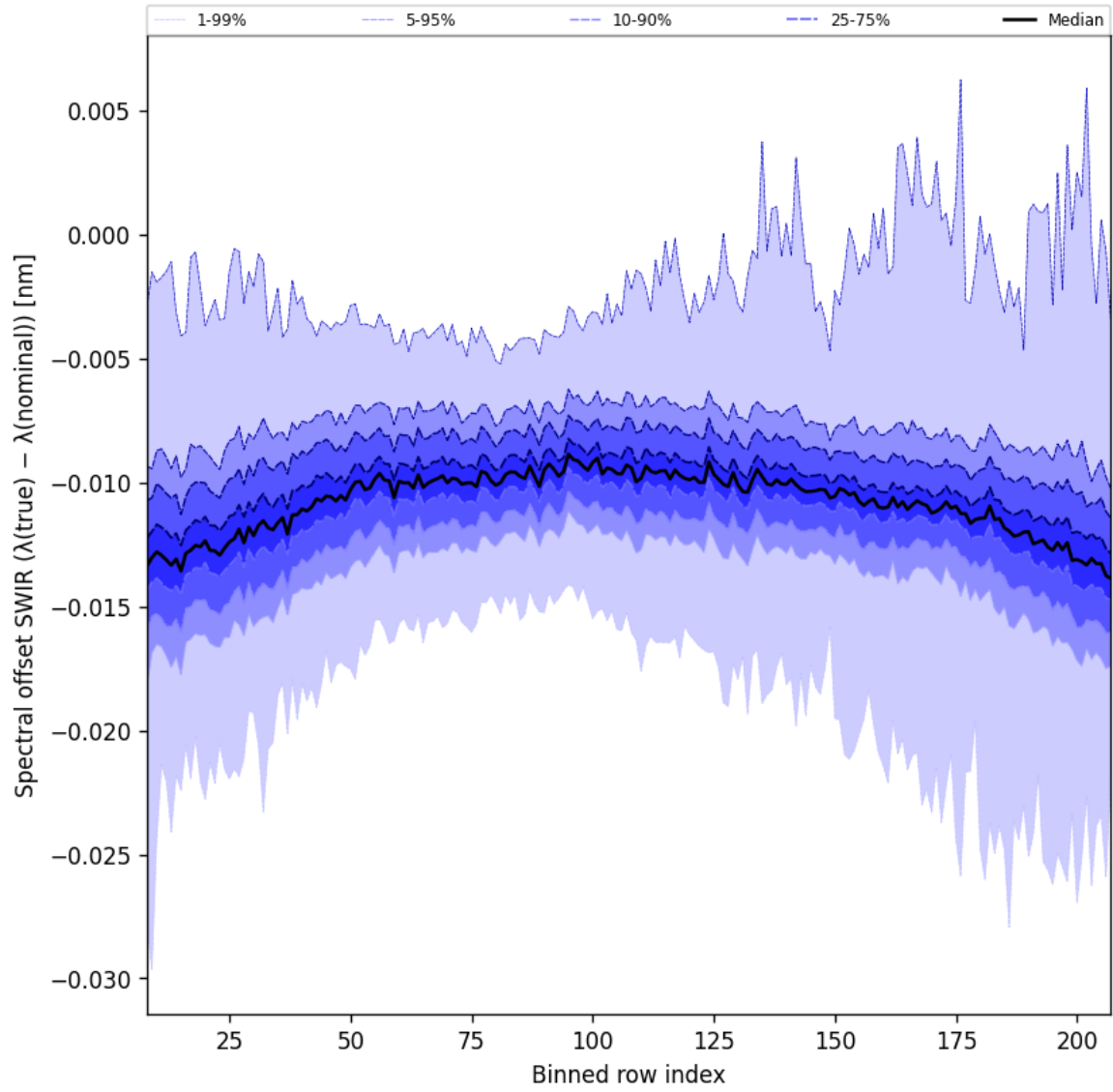
Figure 38: Along track statistics of “Spectral offset SWIR ( \lambda_{\text{true}} - \lambda_{\text{nominal}} )” for 2025-05-06 to 2025-05-08
