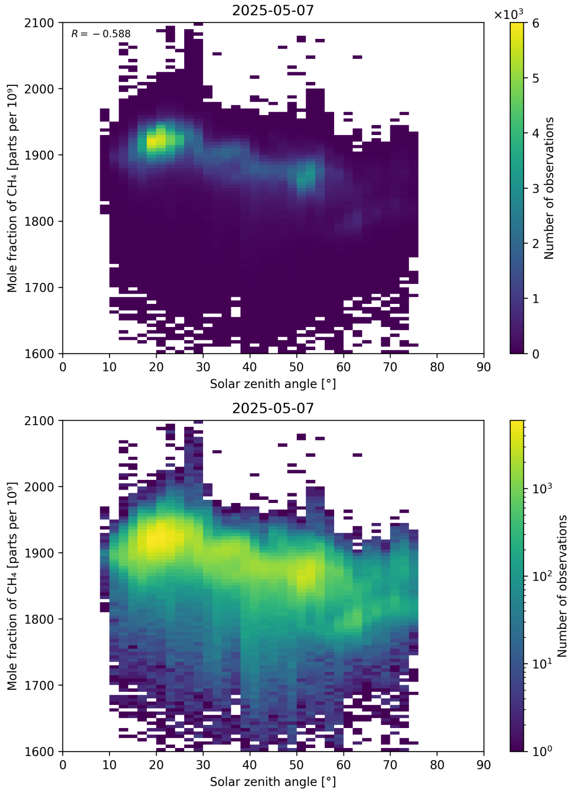
Figure 99: Scatter density plot of “Solar zenith angle” against “Mole fraction of \text{CH}_4 ” for 2025-05-06 to 2025-05-08.
