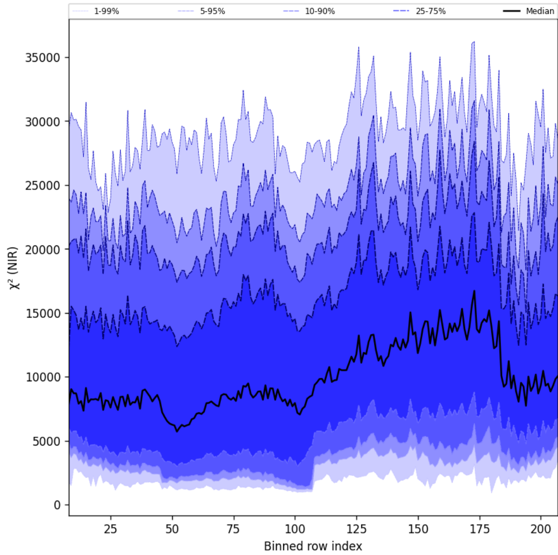
Figure 40: Along track statistics of “ \chi^2 (NIR)” for 2025-05-06 to 2025-05-08
