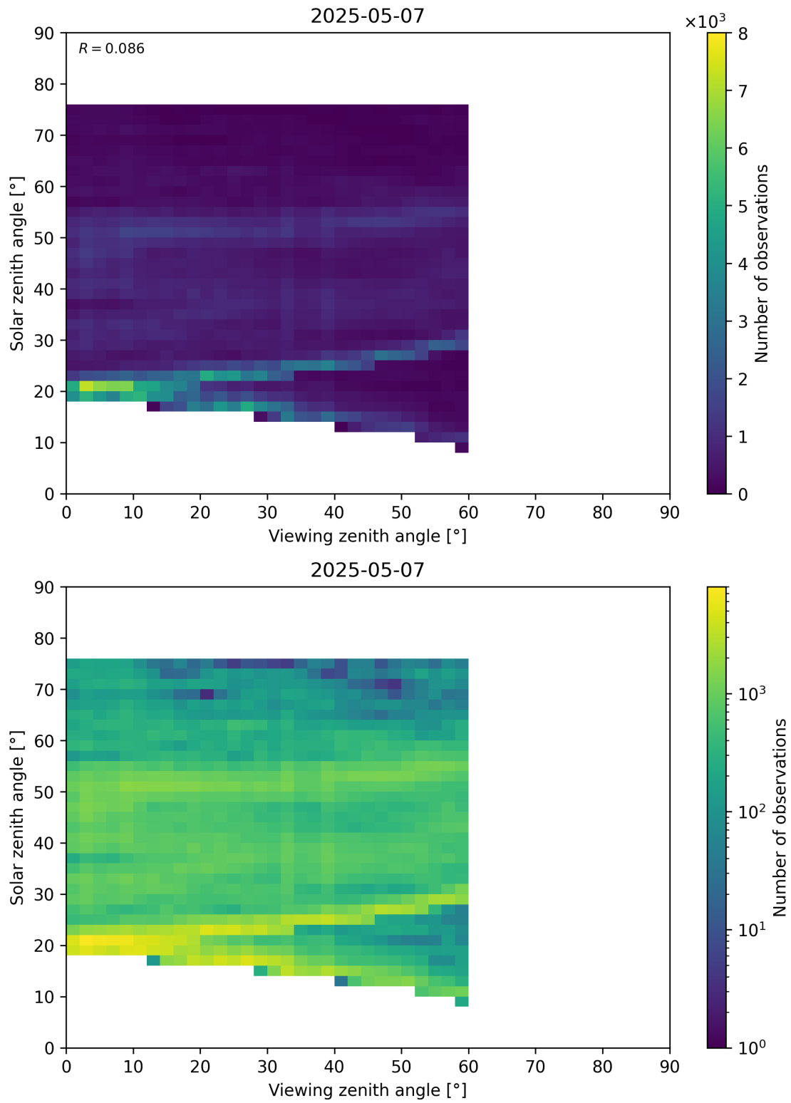
Figure 115: Scatter density plot of “Viewing zenith angle” against “Solar zenith angle” for 2025-05-06 to 2025-05-08.
