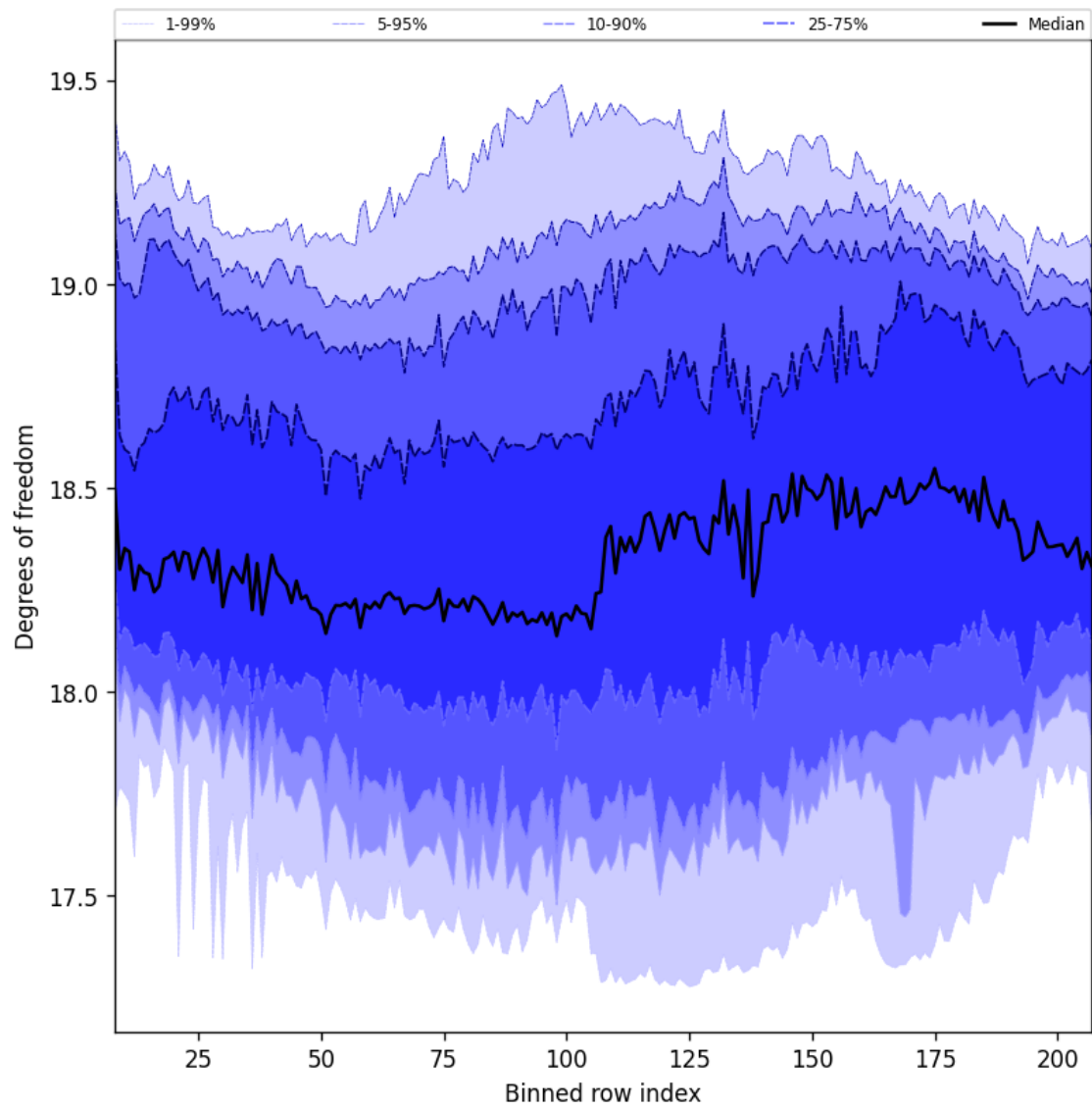
Figure 41: Along track statistics of “Degrees of freedom” for 2025-05-06 to 2025-05-08
