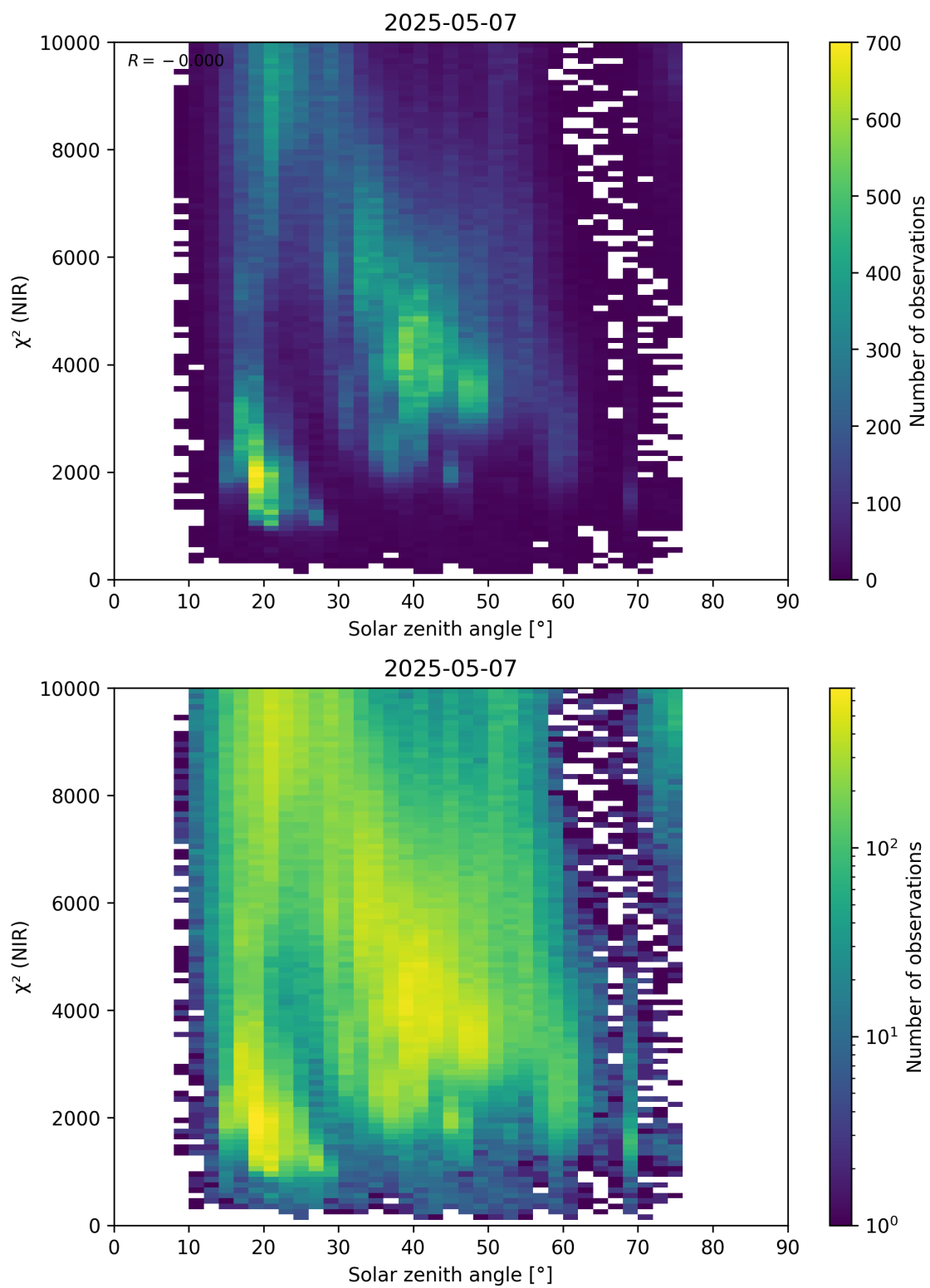
Figure 94: Scatter density plot of “Solar zenith angle” against “ \chi^2 (NIR)” for 2025-05-06 to 2025-05-08.
