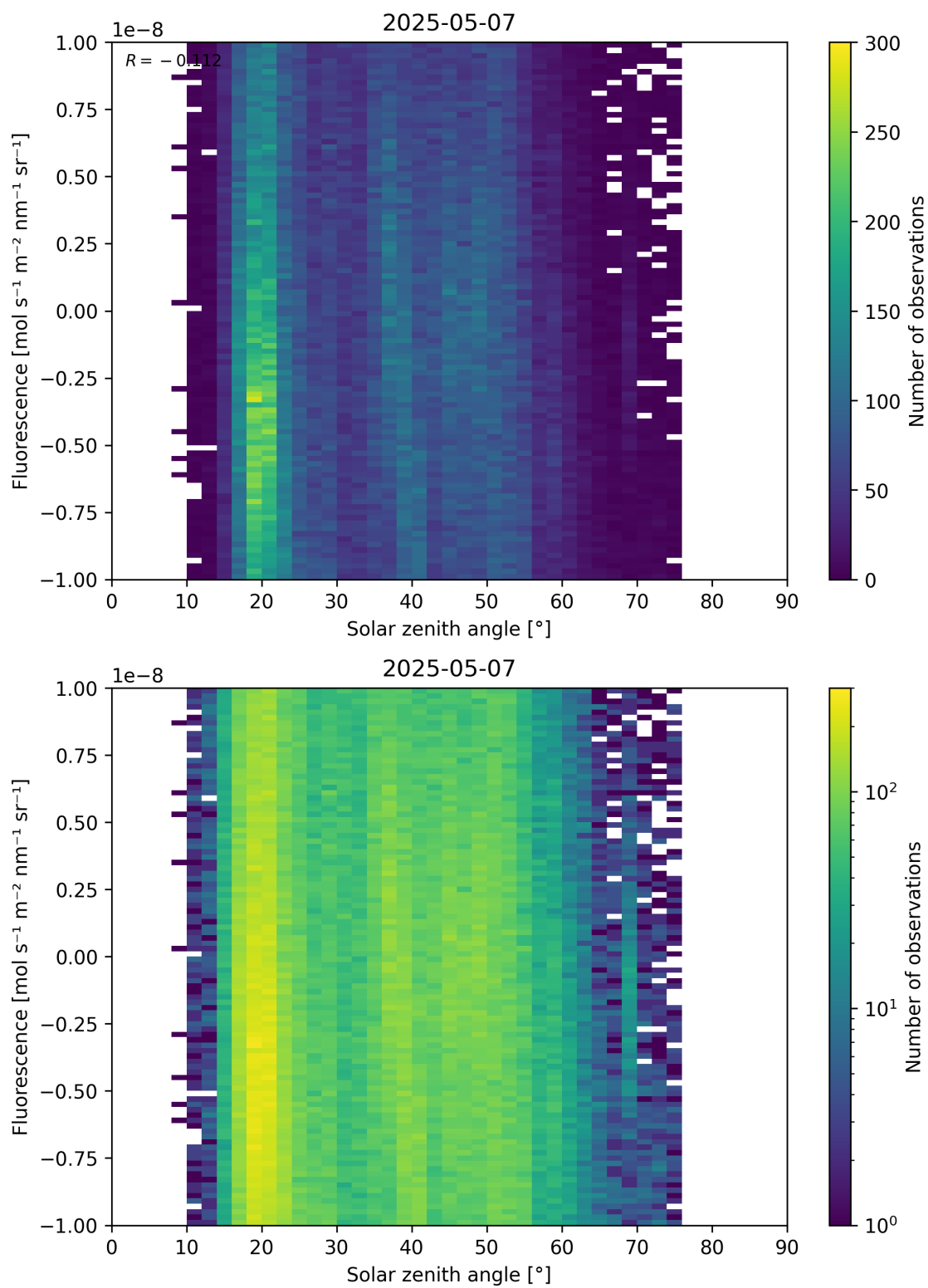
Figure 97: Scatter density plot of “Solar zenith angle” against “Fluorescence” for 2025-05-06 to 2025-05-08.
