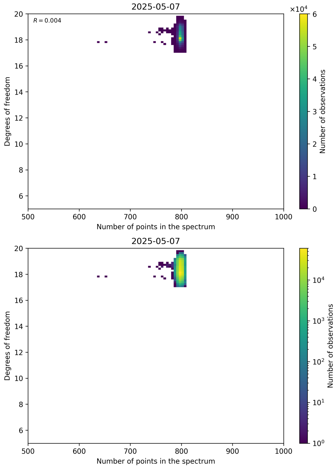
Figure 90: Scatter density plot of “Number of points in the spectrum” against “Degrees of freedom” for 2025-05-06 to 2025-05-08.
