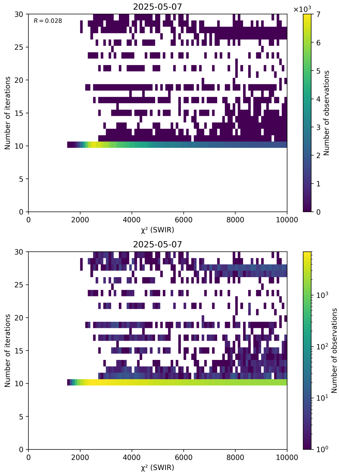
Figure 50: Scatter density plot of “ \chi^2 (SWIR)” against “Number of iterations” for 2025-05-06 to 2025-05-08.
