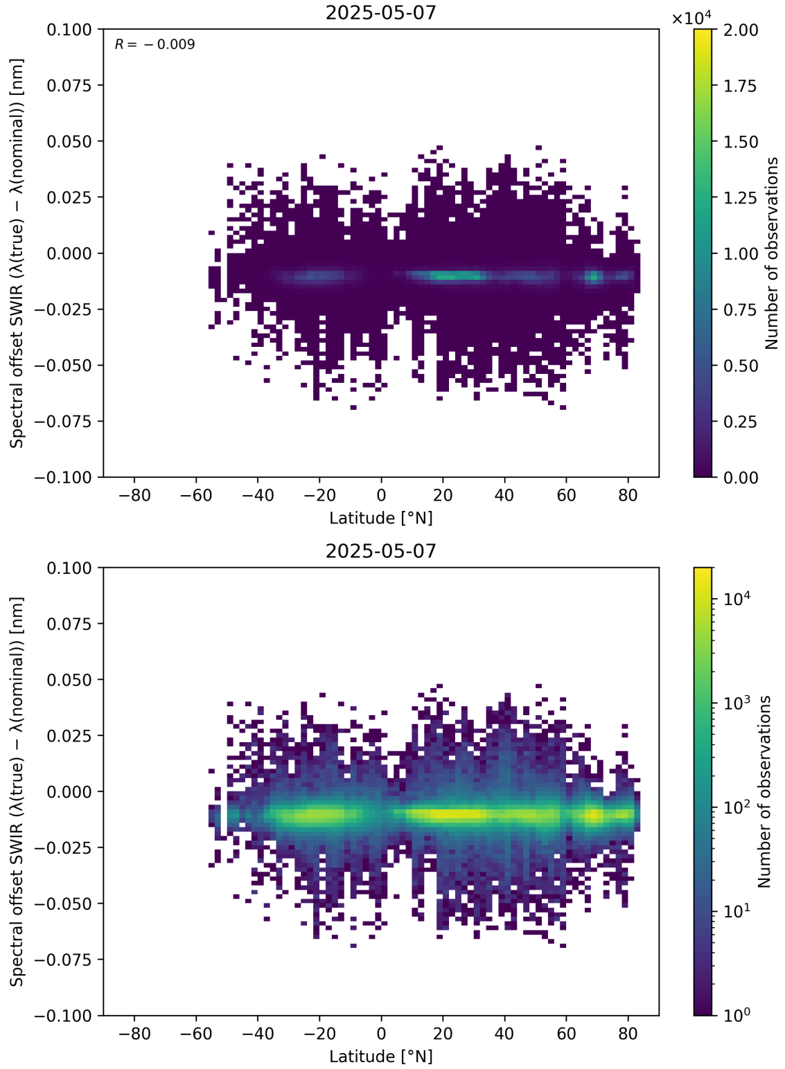
Figure 62: Scatter density plot of “Latitude” against “Spectral offset SWIR ( \lambda_{\text{true}} - \lambda_{\text{nominal}} )” for 2025-05-06 to 2025-05-08.
