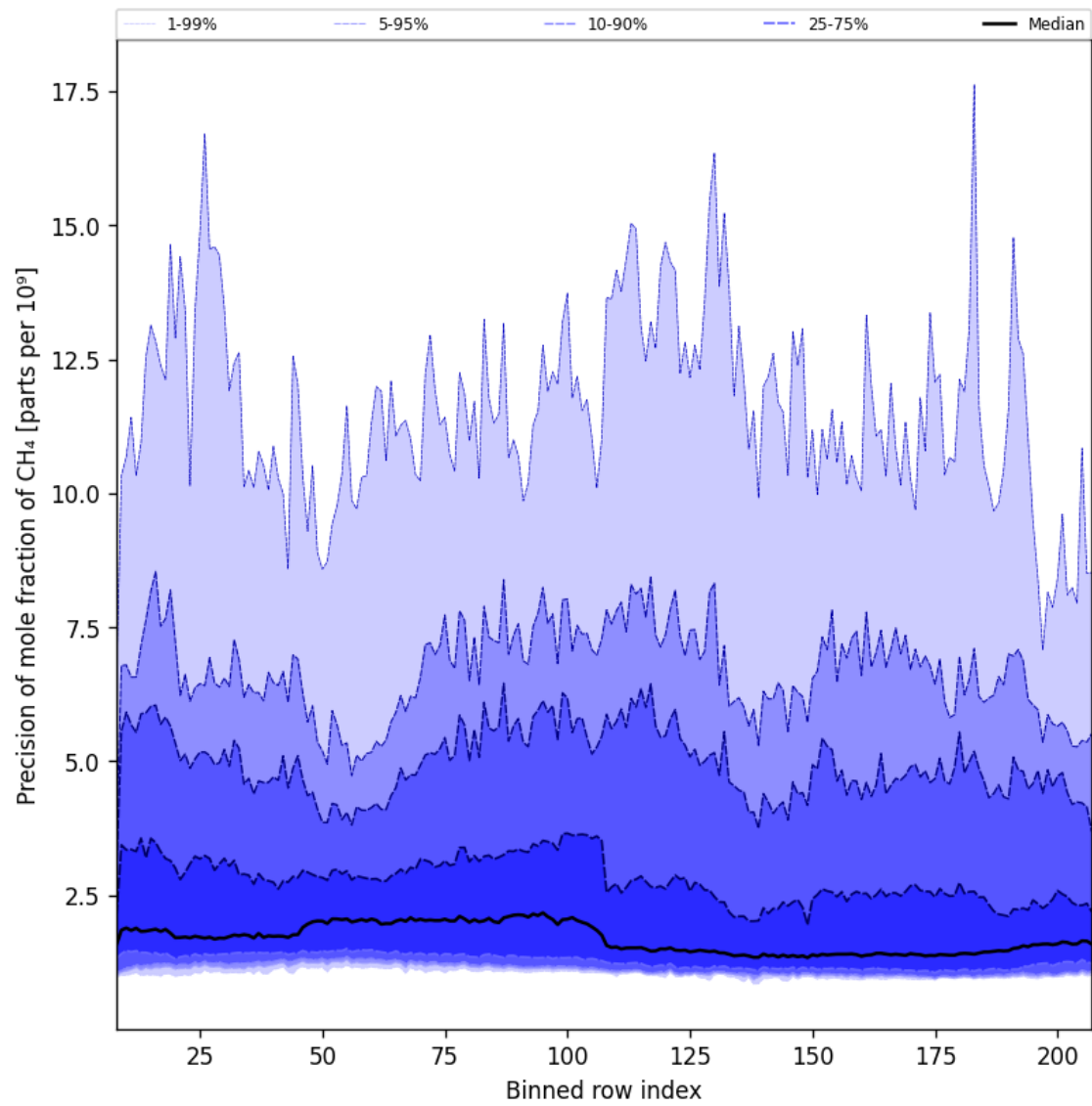
Figure 35: Along track statistics of “Precision of mole fraction of CH 4 ” for 2025-05-06 to 2025-05-08
