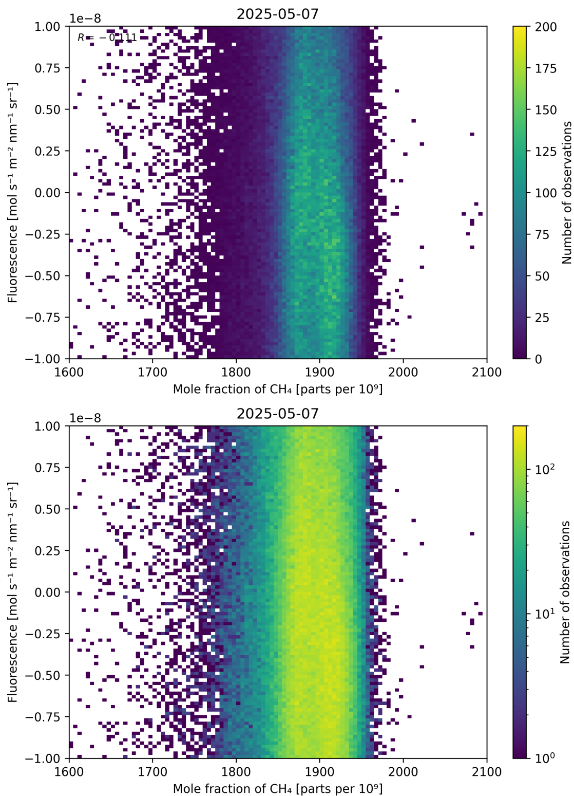
Figure 73: Scatter density plot of “Mole fraction of \text{CH}_4 ” against “Fluorescence” for 2025-05-06 to 2025-05-08.
