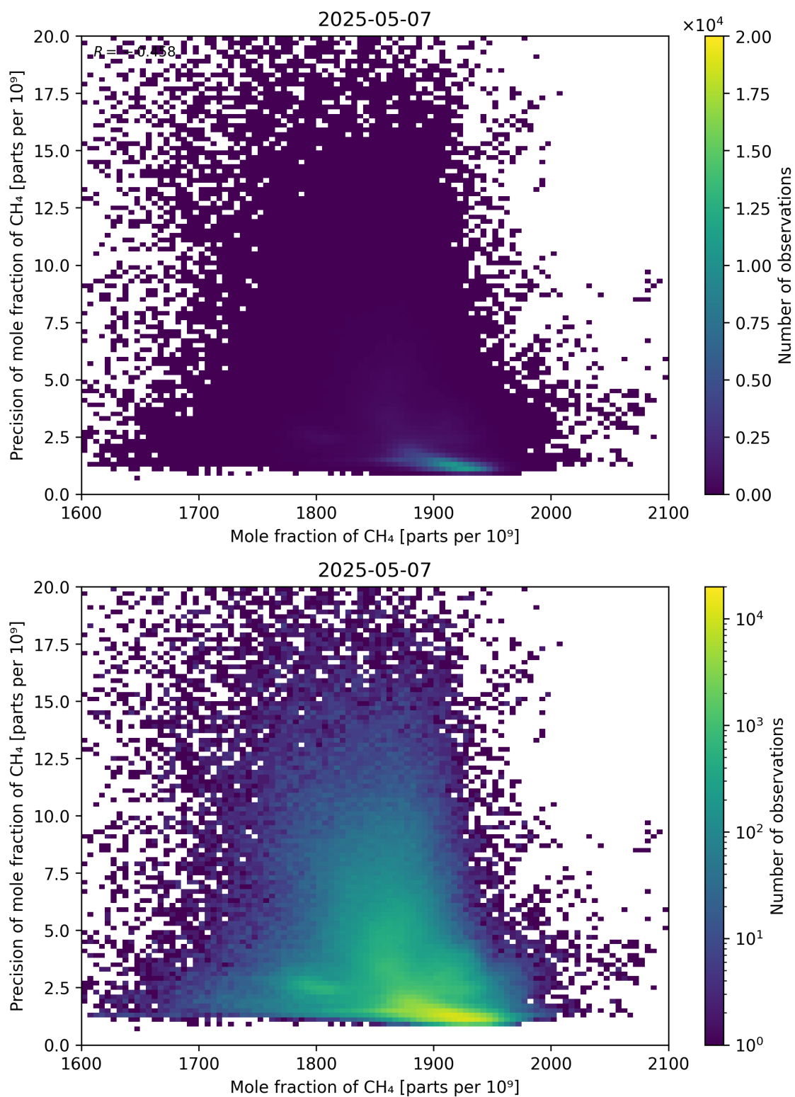
Figure 75: Scatter density plot of “Mole fraction of CH 4 ” against “Precision of mole fraction of CH 4 ” for 2025-05-06 to 2025-05-08.
