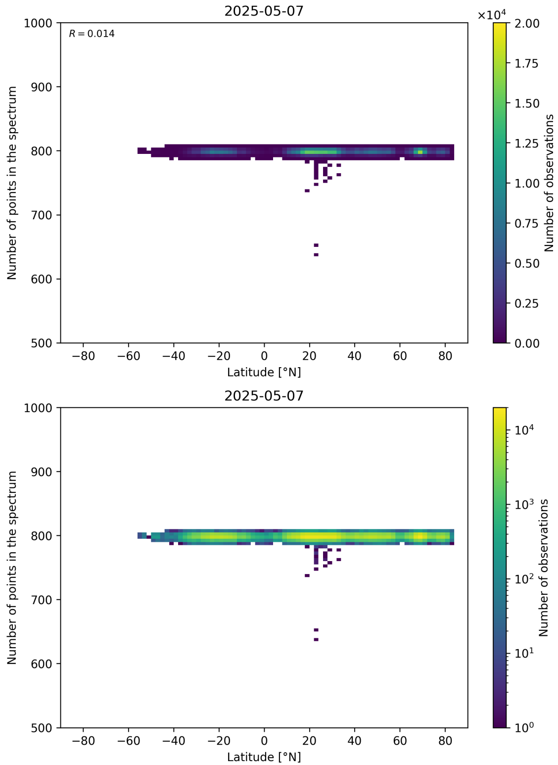
Figure 61: Scatter density plot of “Latitude” against “Number of points in the spectrum” for 2025-05-06 to 2025-05-08.
