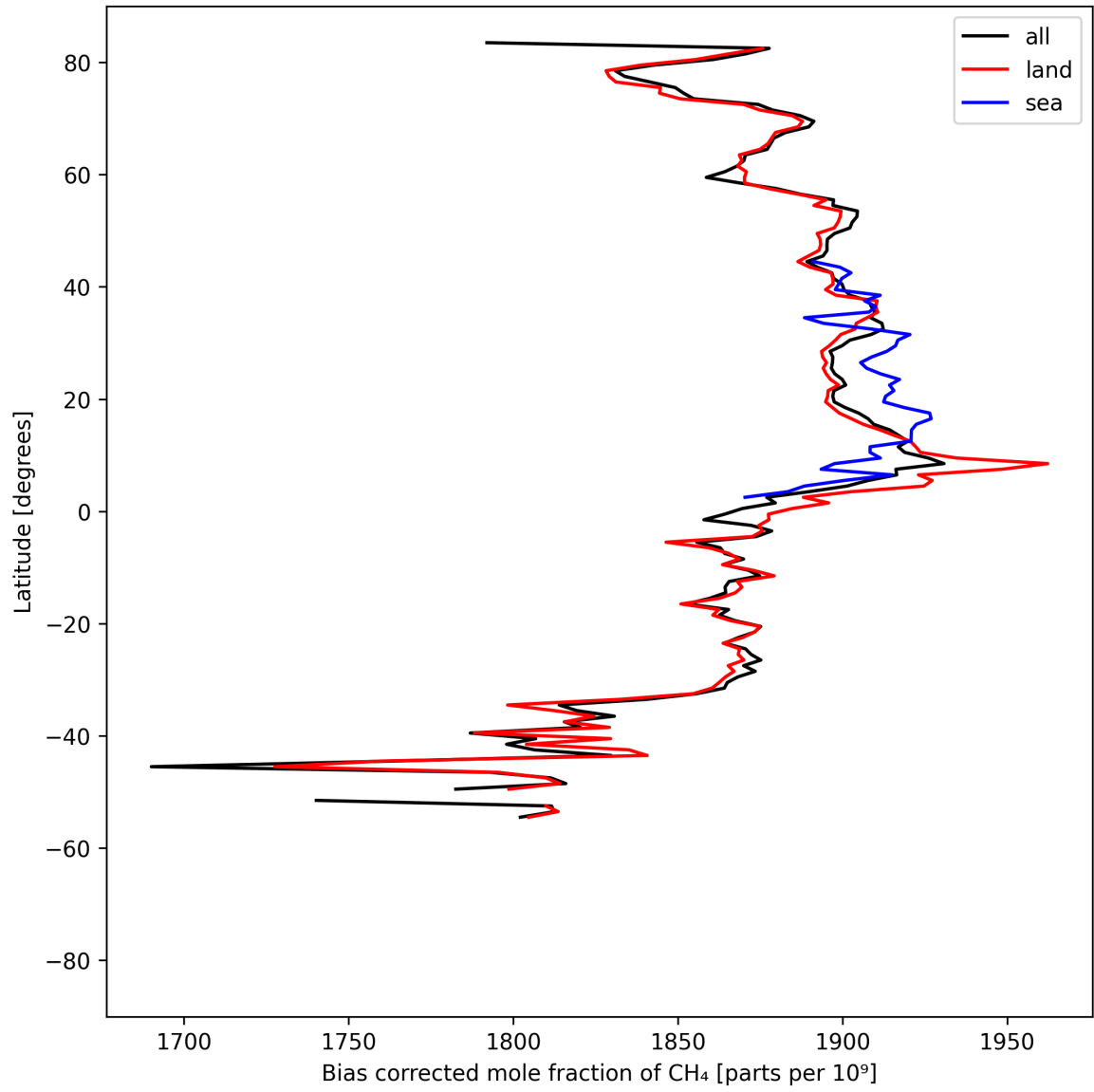
Figure 14: Zonal average of “Bias corrected mole fraction of CH 4 ” for 2025-05-06 to 2025-05-08.
