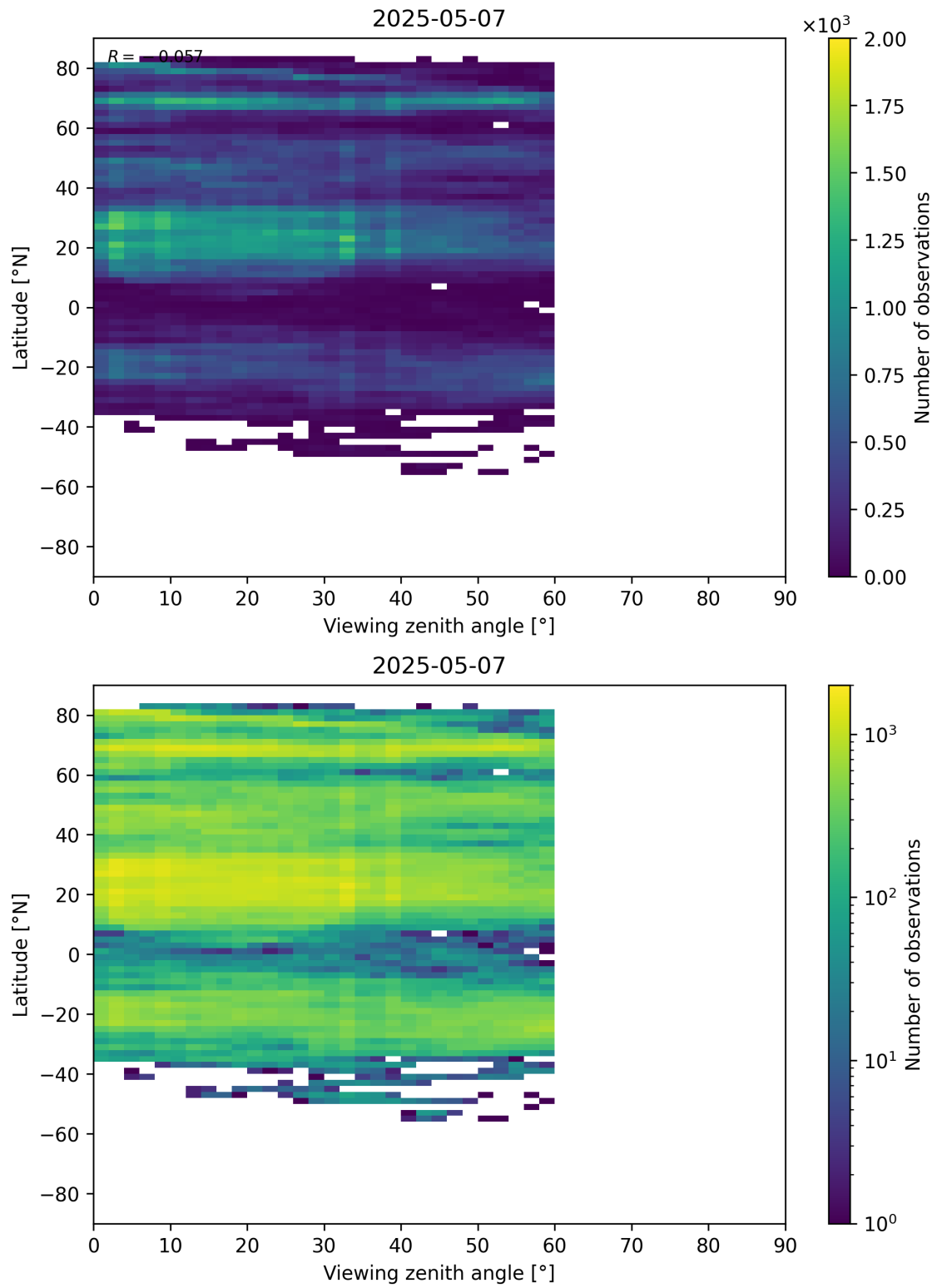
Figure 109: Scatter density plot of “Viewing zenith angle” against “Latitude” for 2025-05-06 to 2025-05-08.
