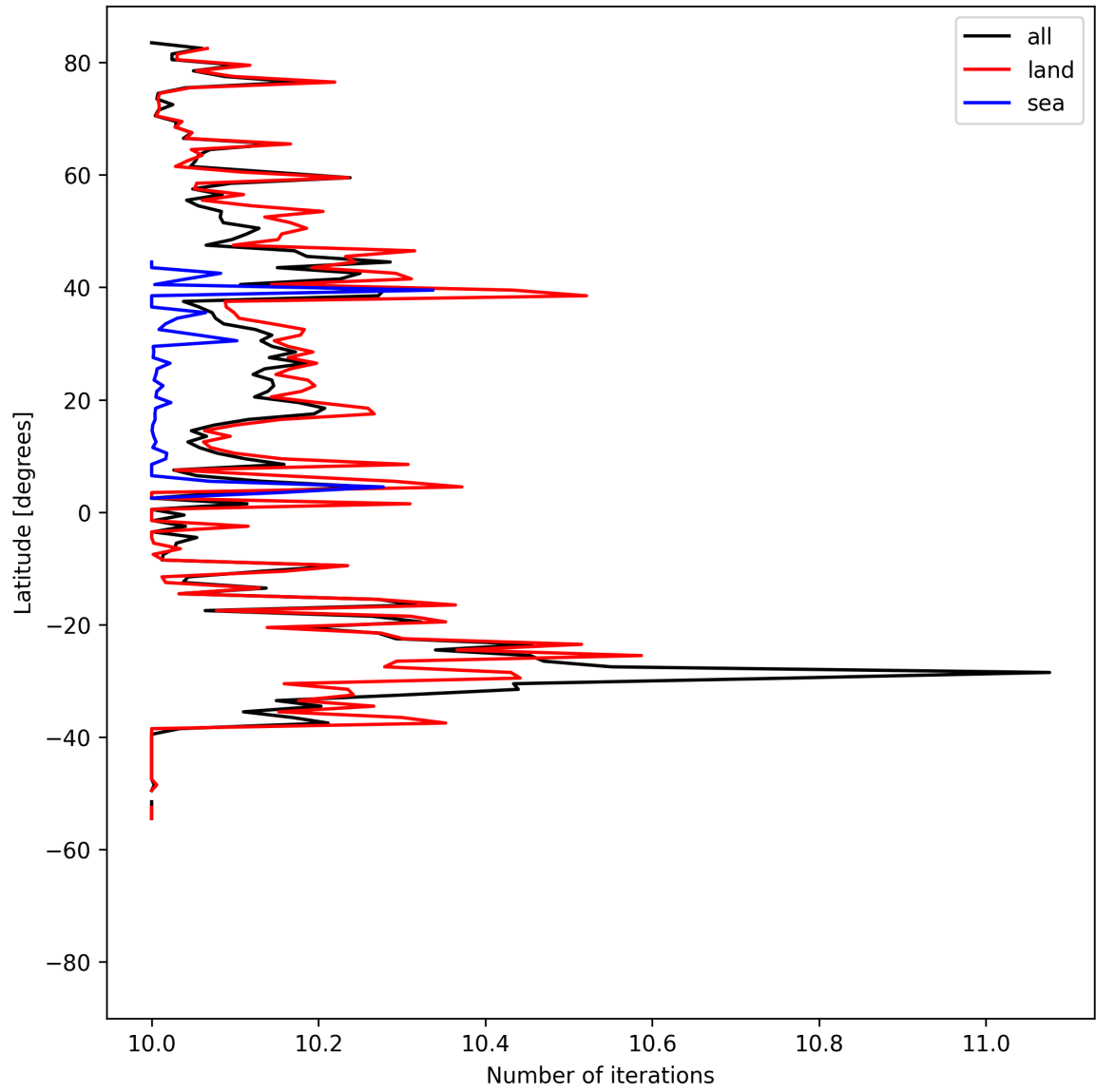
Figure 20: Zonal average of “Number of iterations” for 2025-05-06 to 2025-05-08.
