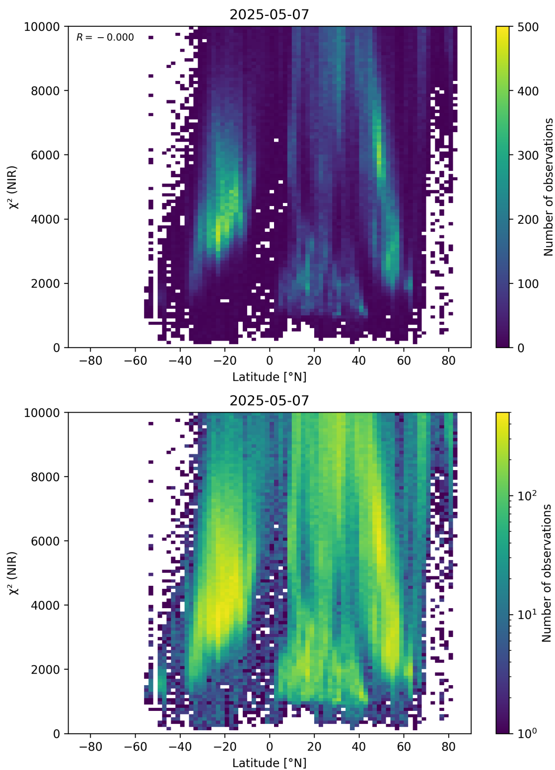
Figure 53: Scatter density plot of “Latitude” against “ \chi^2 (NIR)” for 2025-05-06 to 2025-05-08.
