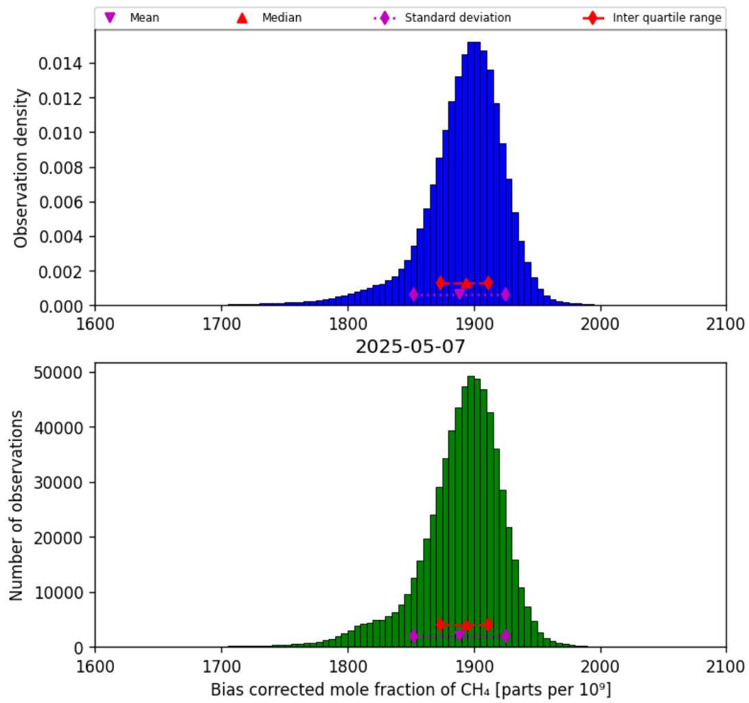
Figure 25: Histogram of “Bias corrected mole fraction of CH 4 ” for 2025-05-06 to 2025-05-08
