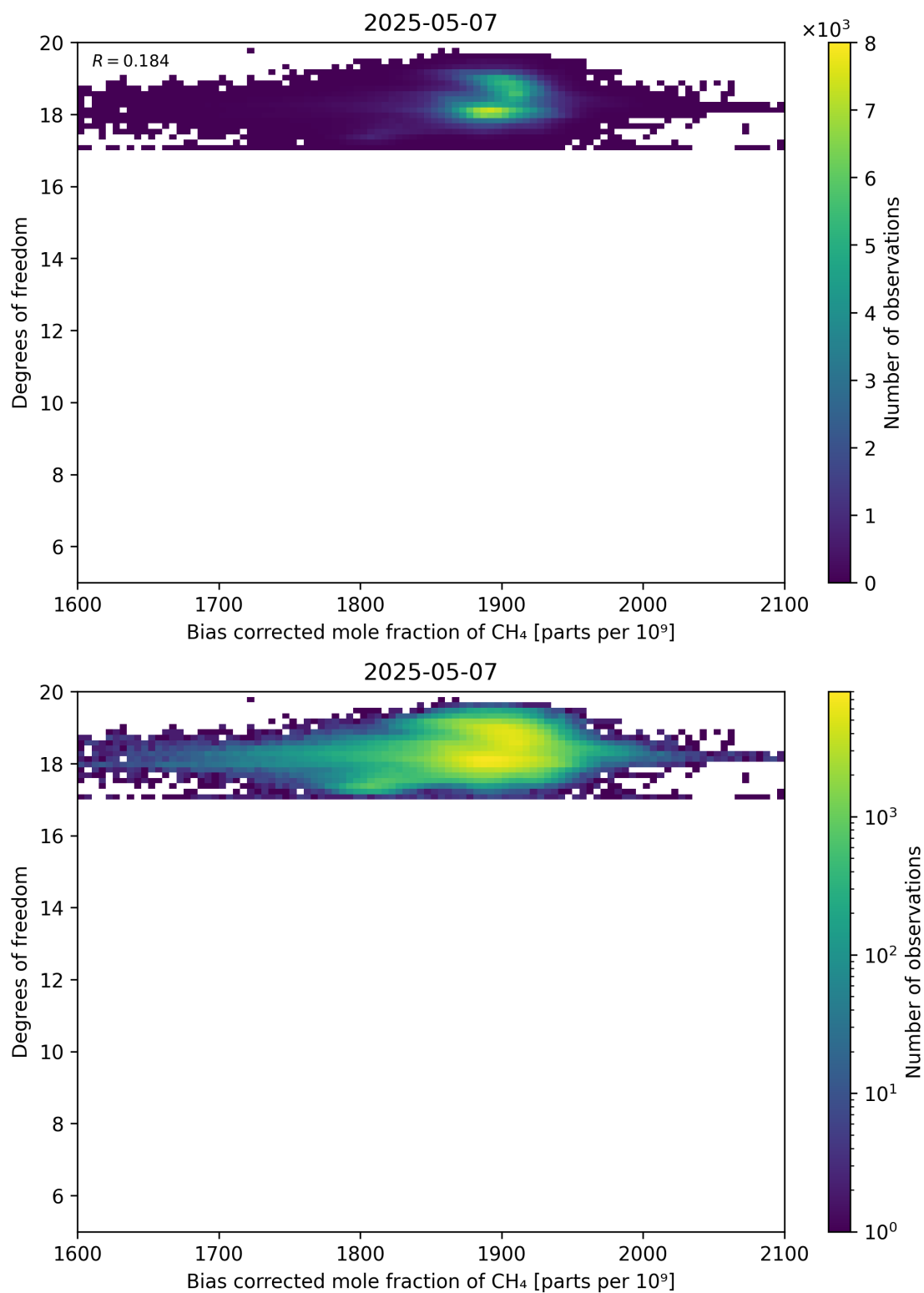
Figure 65: Scatter density plot of “Bias corrected mole fraction of CH 4 ” against “Degrees of freedom” for 2025-05-06 to 2025-05-08.
