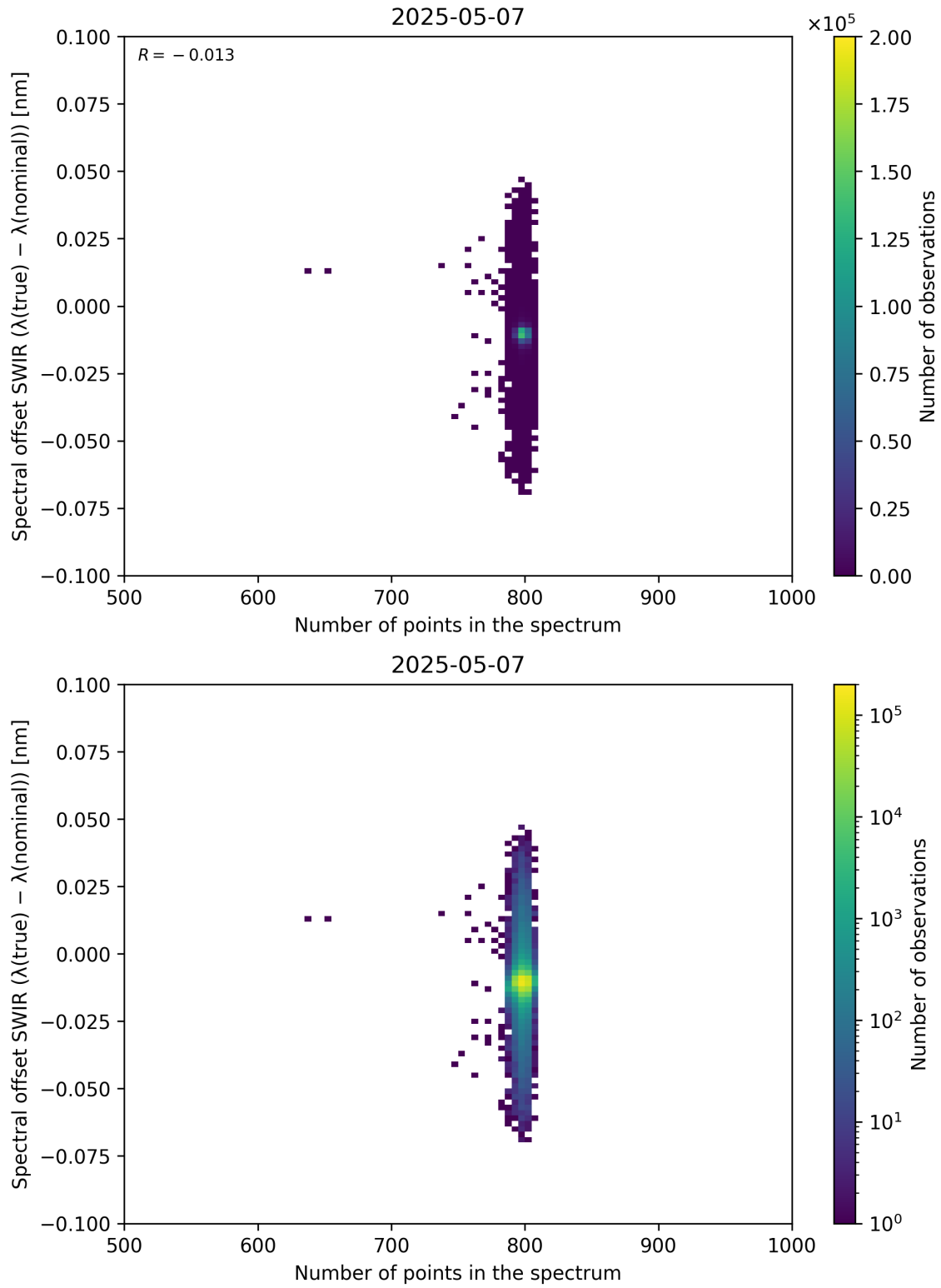
Figure 93: Scatter density plot of “Number of points in the spectrum” against “Spectral offset SWIR ( \lambda_{\text{true}} - \lambda_{\text{nominal}} )” for 2025-05-06 to 2025-05-08.
