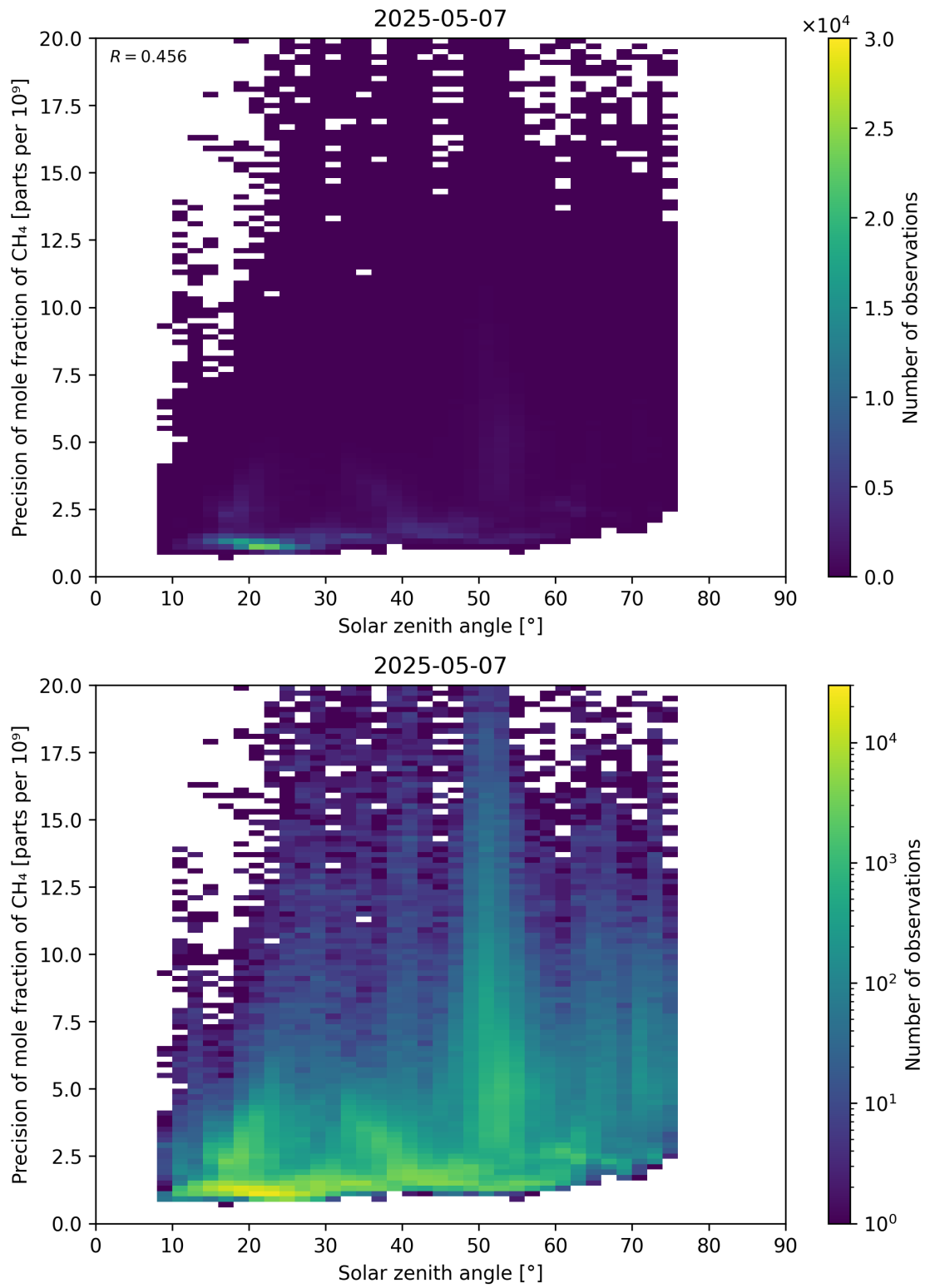
Figure 101: Scatter density plot of “Solar zenith angle” against “Precision of mole fraction of \text{CH}_4 ” for 2025-05-06 to 2025-05-08.
