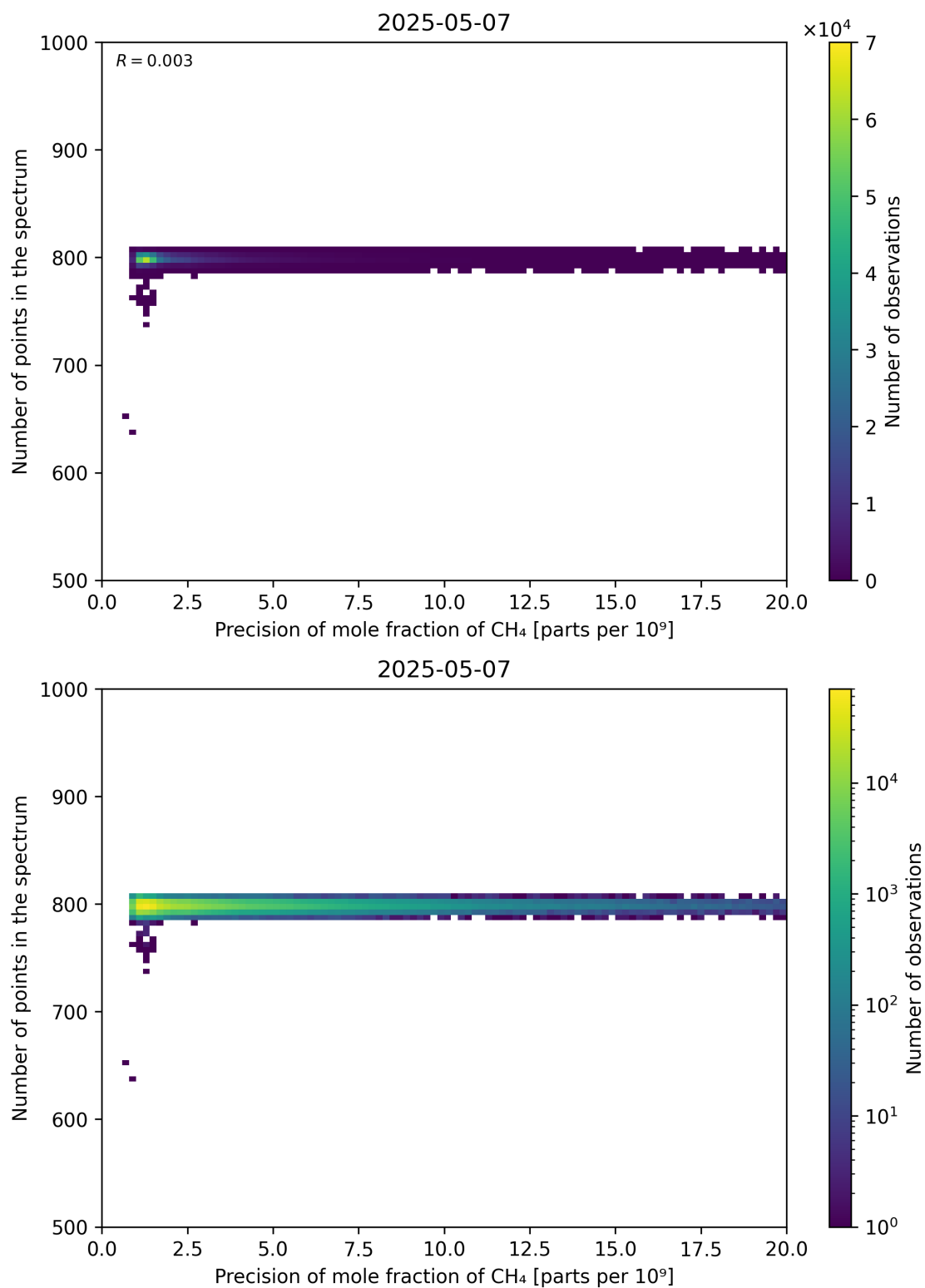
Figure 84: Scatter density plot of “Precision of mole fraction of CH 4 ” against “Number of points in the spectrum” for 2025-05-06 to 2025-05-08.
