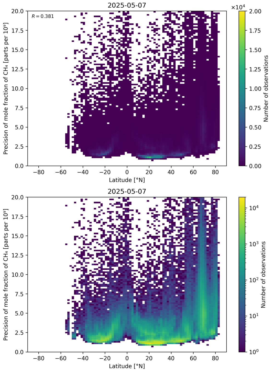
Figure 59: Scatter density plot of “Latitude” against “Precision of mole fraction of CH 4 ” for 2025-05-06 to 2025-05-08.
