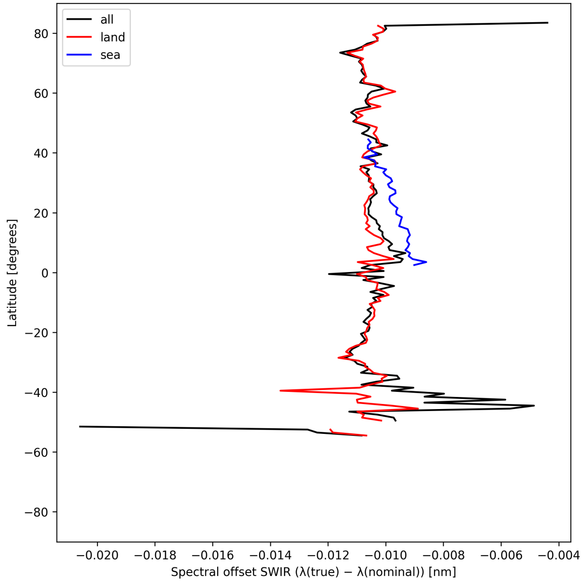
Figure 16: Zonal average of “Spectral offset SWIR ( \lambda_{\text{true}} - \lambda_{\text{nominal}} )” for 2025-05-06 to 2025-05-08.
