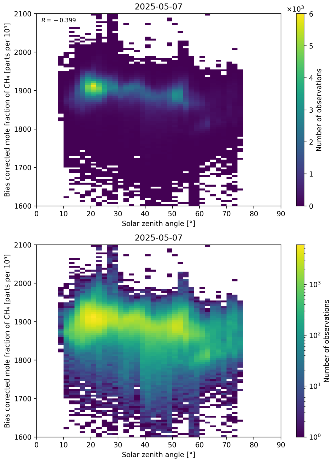
Figure 100: Scatter density plot of “Solar zenith angle” against “Bias corrected mole fraction of CH 4 ” for 2025-05-06 to 2025-05-08.
