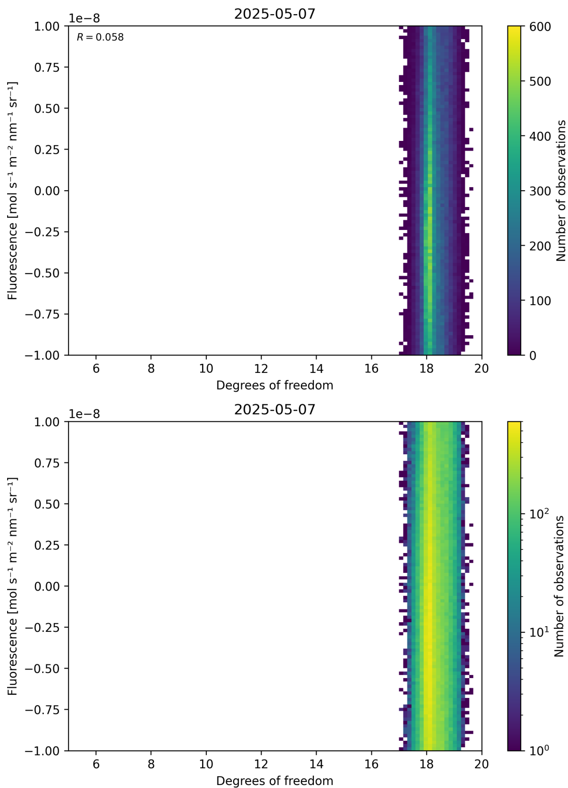
Figure 51: Scatter density plot of “Degrees of freedom” against “Fluorescence” for 2025-05-06 to 2025-05-08.
