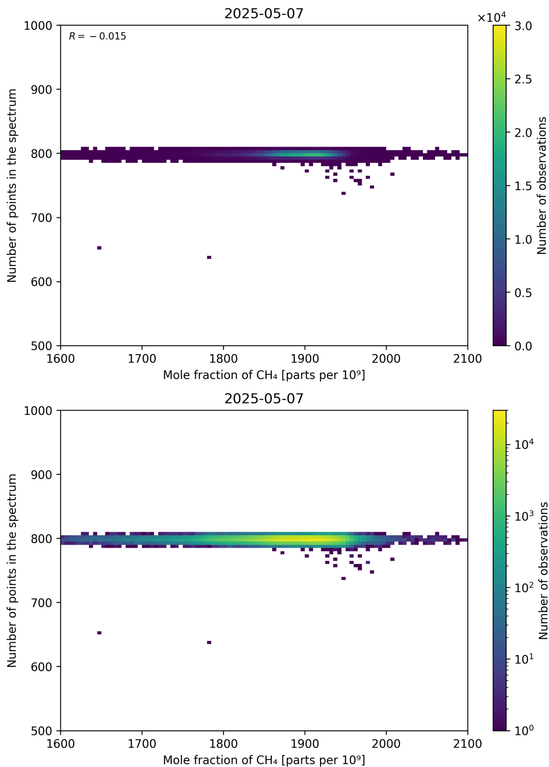
Figure 77: Scatter density plot of “Mole fraction of CH 4 ” against “Number of points in the spectrum” for 2025-05-06 to 2025-05-08.
