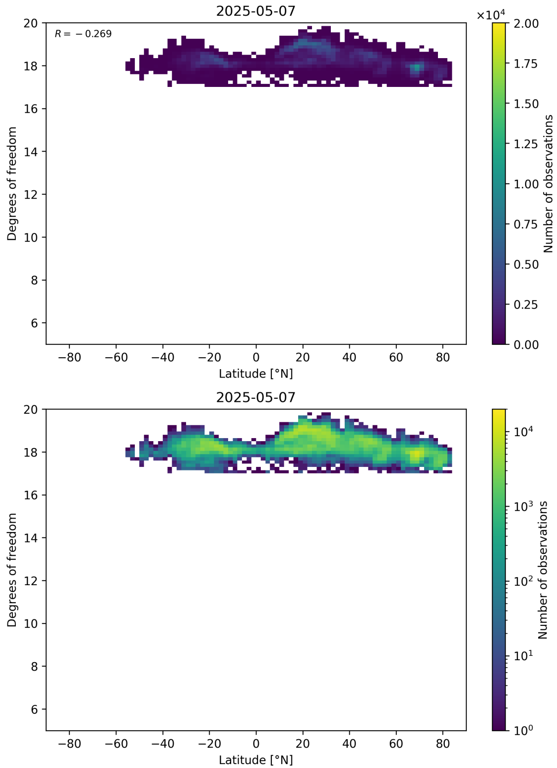
Figure 55: Scatter density plot of “Latitude” against “Degrees of freedom” for 2025-05-06 to 2025-05-08.
