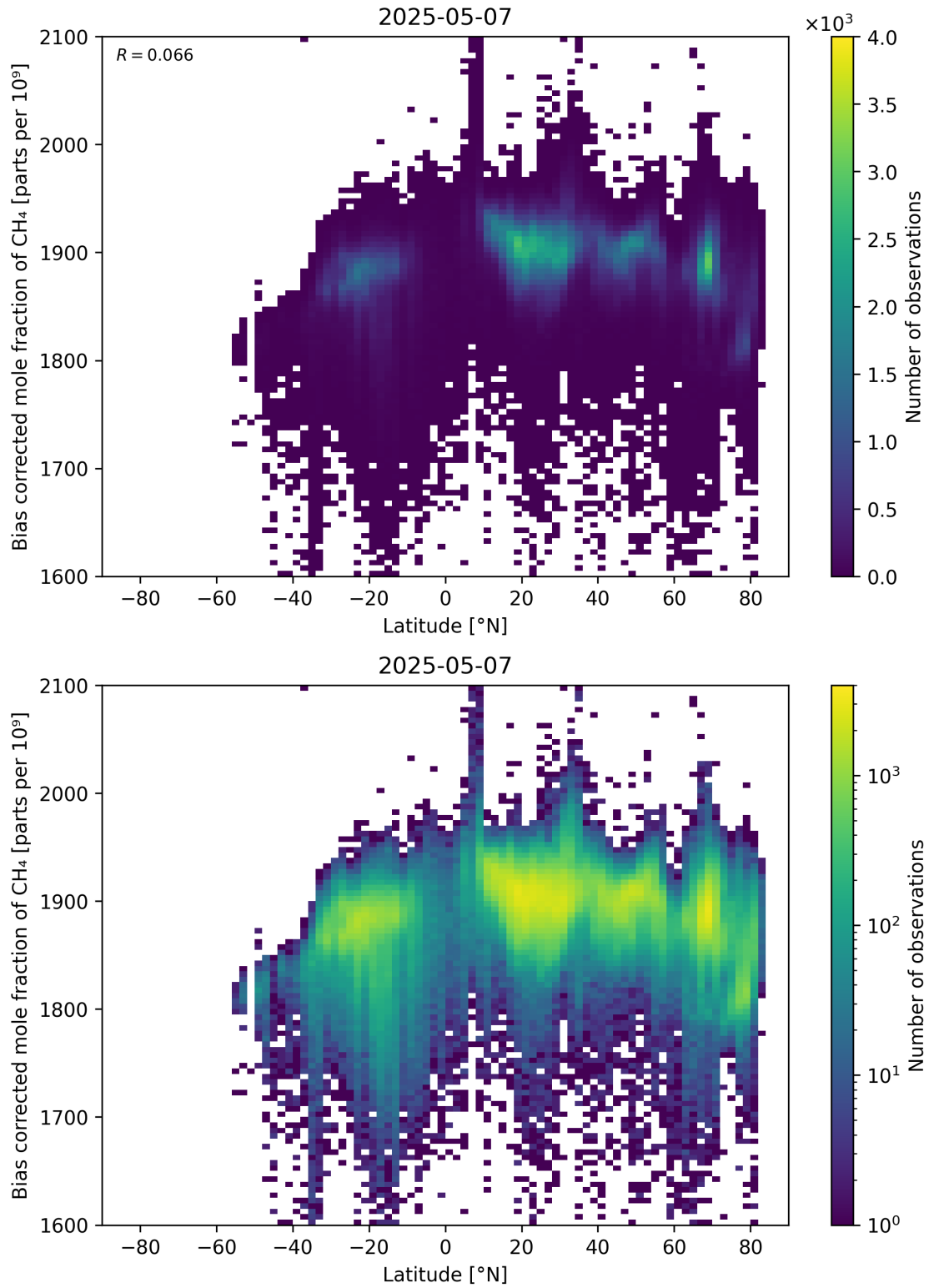
Figure 58: Scatter density plot of “Latitude” against “Bias corrected mole fraction of CH 4 ” for 2025-05-06 to 2025-05-08.
