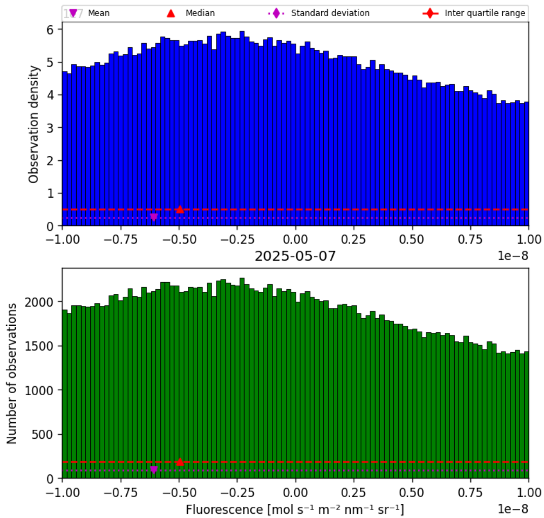
Figure 32: Histogram of “Fluorescence” for 2025-05-06 to 2025-05-08
