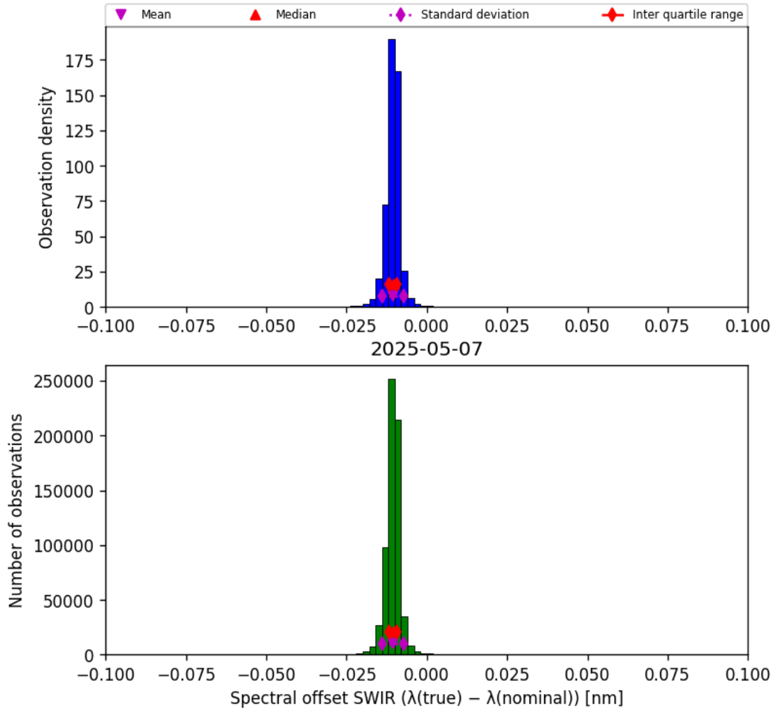
Figure 27: Histogram of “Spectral offset SWIR ( \lambda_{\text{true}} - \lambda_{\text{nominal}} )” for 2025-05-06 to 2025-05-08
