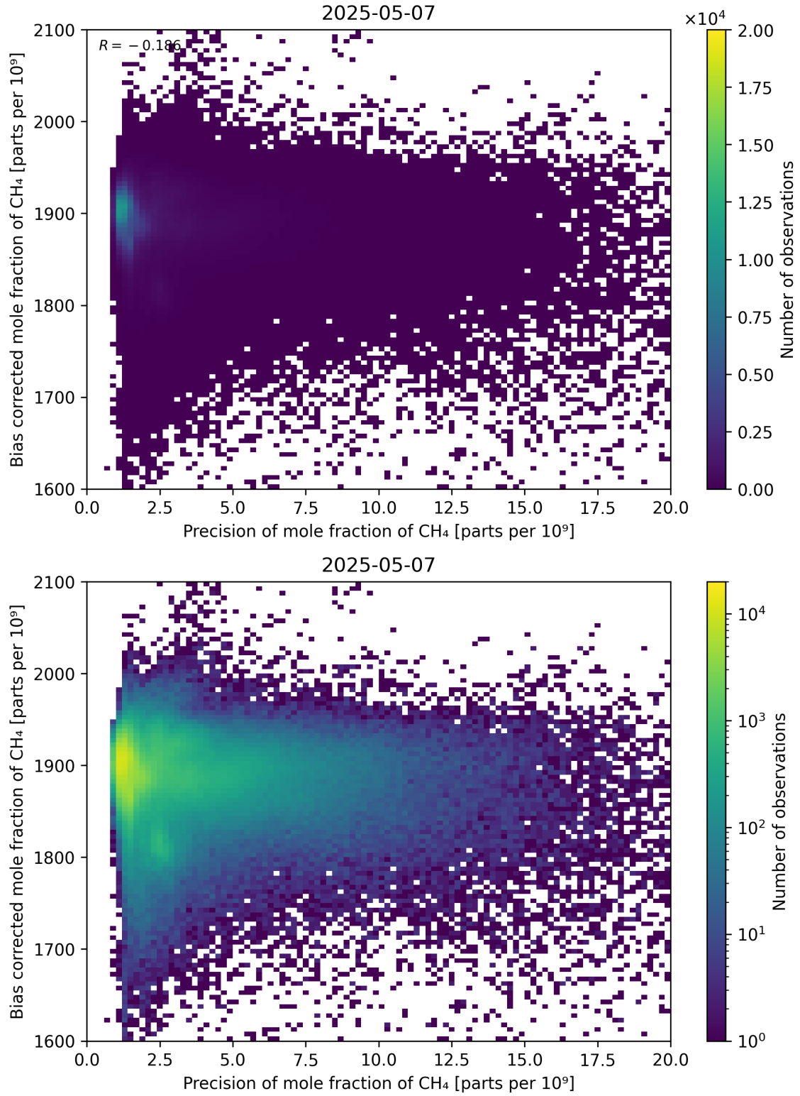
Figure 82: Scatter density plot of “Precision of mole fraction of CH 4 ” against “Bias corrected mole fraction of CH 4 ” for 2025-05-06 to 2025-05-08.
