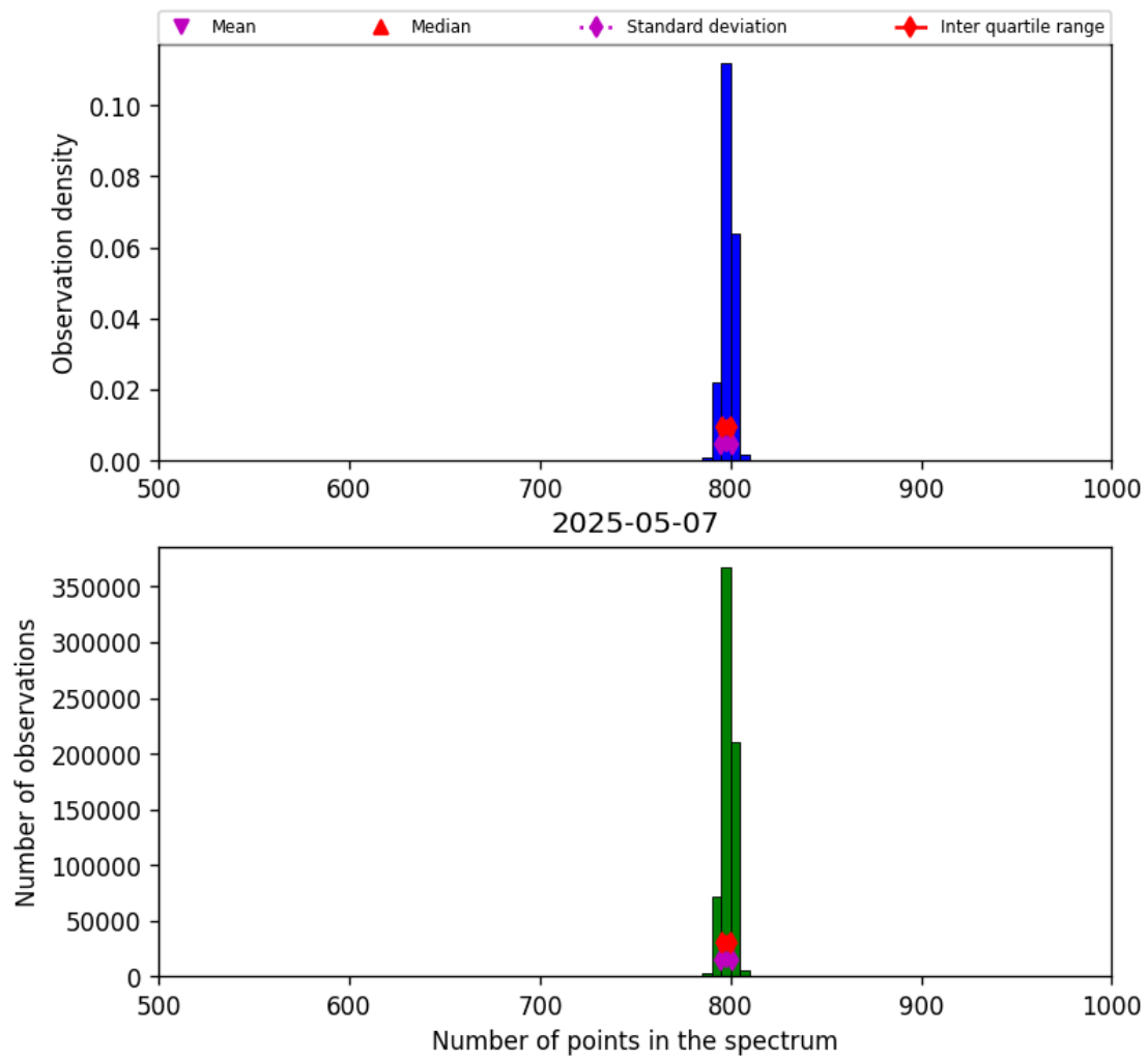
Figure 26: Histogram of “Number of points in the spectrum” for 2025-05-06 to 2025-05-08
