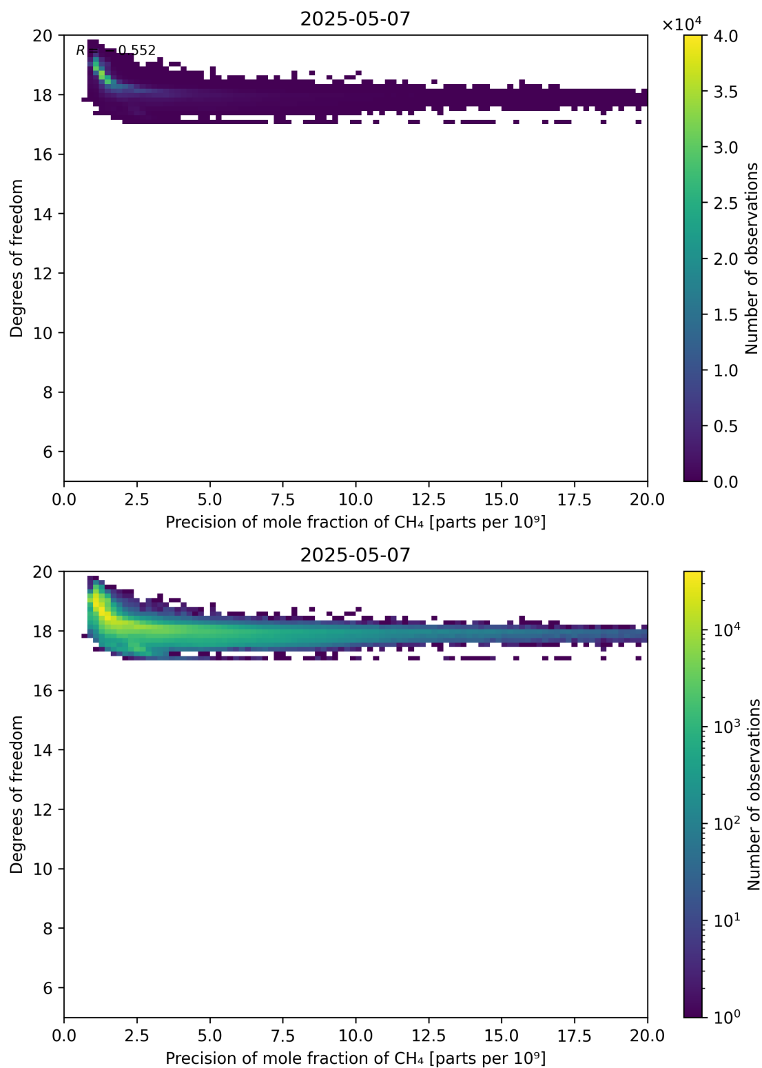
Figure 80: Scatter density plot of “Precision of mole fraction of CH 4 ” against “Degrees of freedom” for 2025-05-06 to 2025-05-08.
