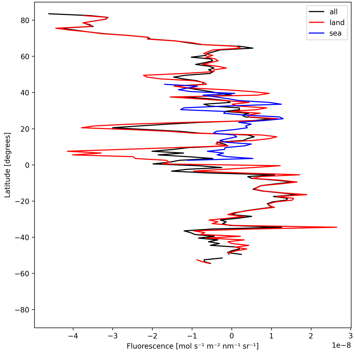
Figure 21: Zonal average of “Fluorescence” for 2025-05-06 to 2025-05-08.
