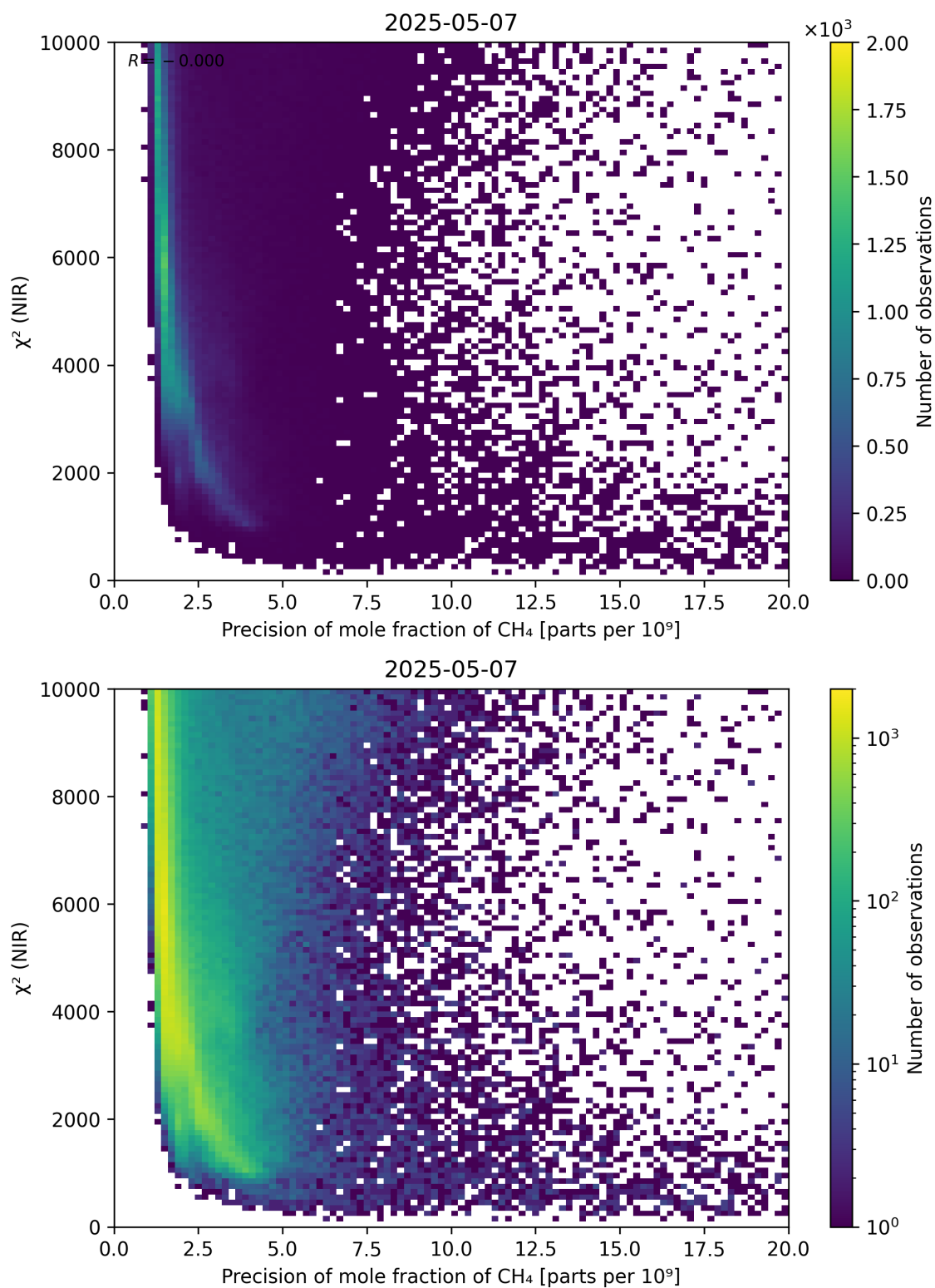
Figure 78: Scatter density plot of “Precision of mole fraction of \text{CH}_4 ” against “ \chi^2 (NIR)” for 2025-05-06 to 2025-05-08.
