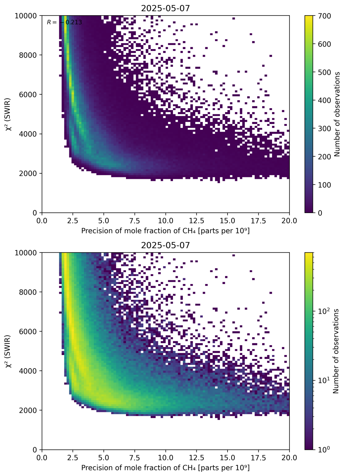
Figure 79: Scatter density plot of “Precision of mole fraction of \text{CH}_4 ” against “ \chi^2 (SWIR)” for 2025-05-06 to 2025-05-08.
