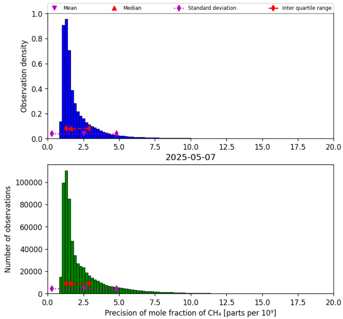
Figure 24: Histogram of “Precision of mole fraction of CH 4 ” for 2025-05-06 to 2025-05-08
