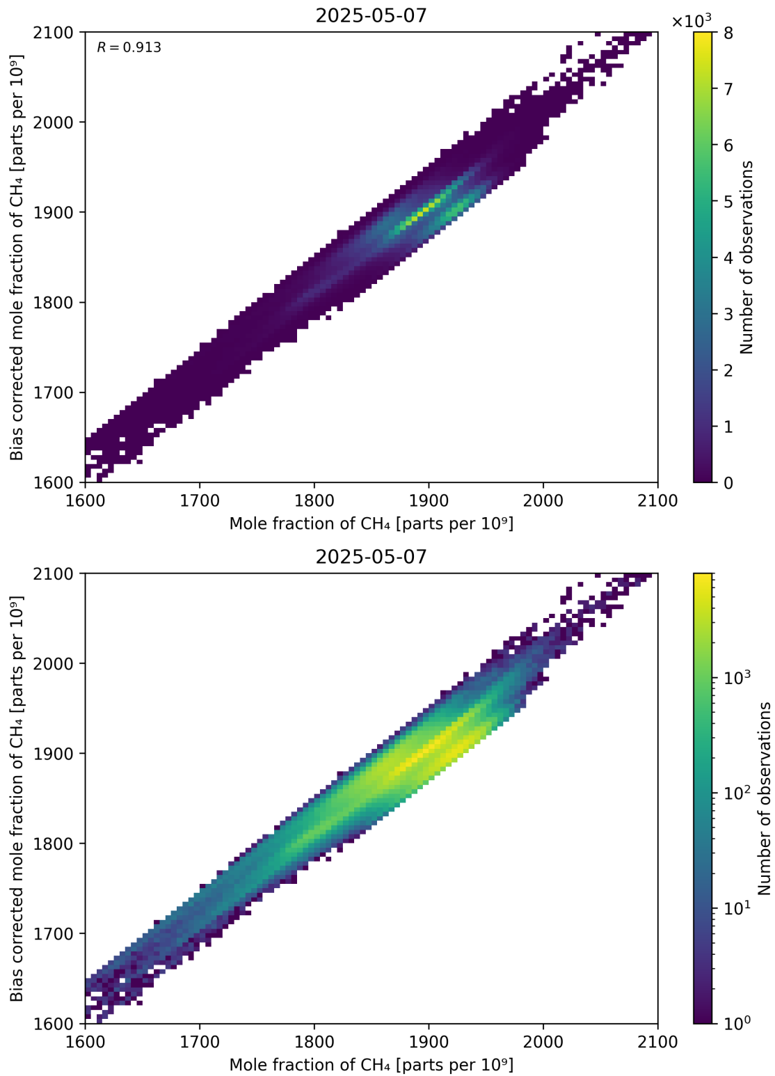
Figure 74: Scatter density plot of “Mole fraction of CH 4 ” against “Bias corrected mole fraction of CH 4 ” for 2025-05-06 to 2025-05-08.
