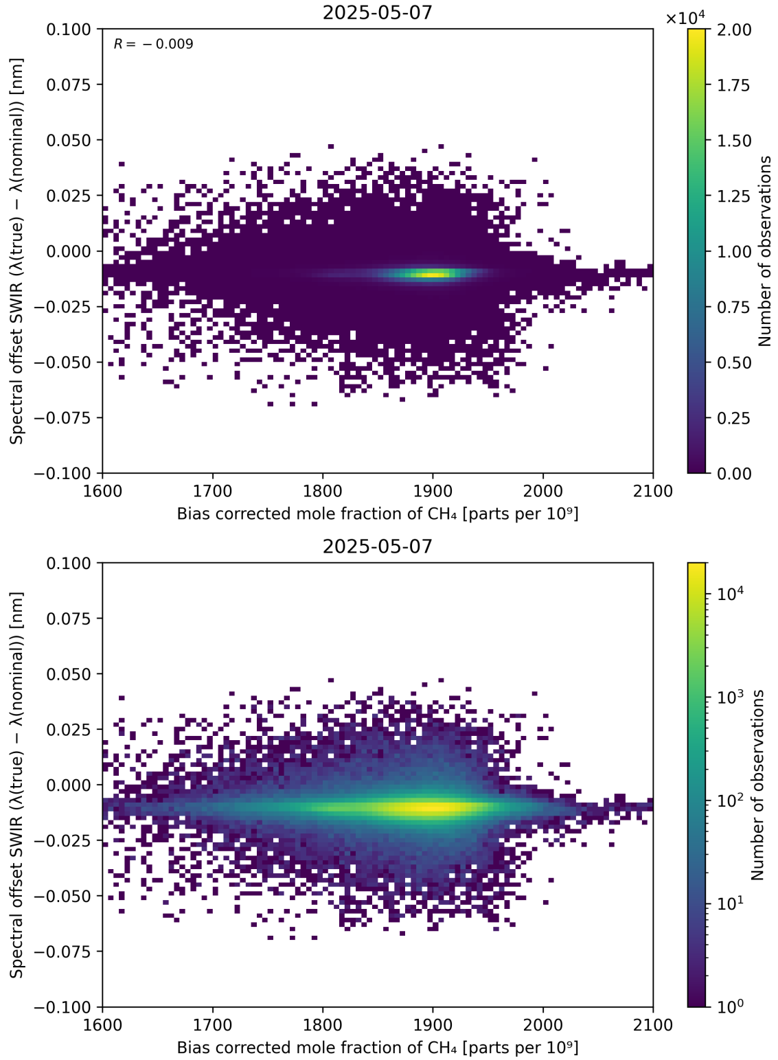
Figure 69: Scatter density plot of “Bias corrected mole fraction of \text{CH}_4 ” against “Spectral offset SWIR ( \lambda_{\text{true}} - \lambda_{\text{nominal}} )” for 2025-05-06 to 2025-05-08.
