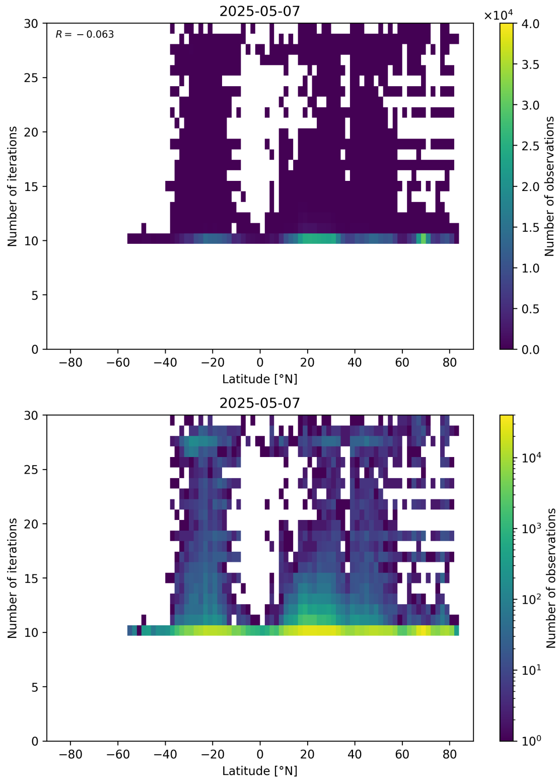
Figure 60: Scatter density plot of “Latitude” against “Number of iterations” for 2025-05-06 to 2025-05-08.
