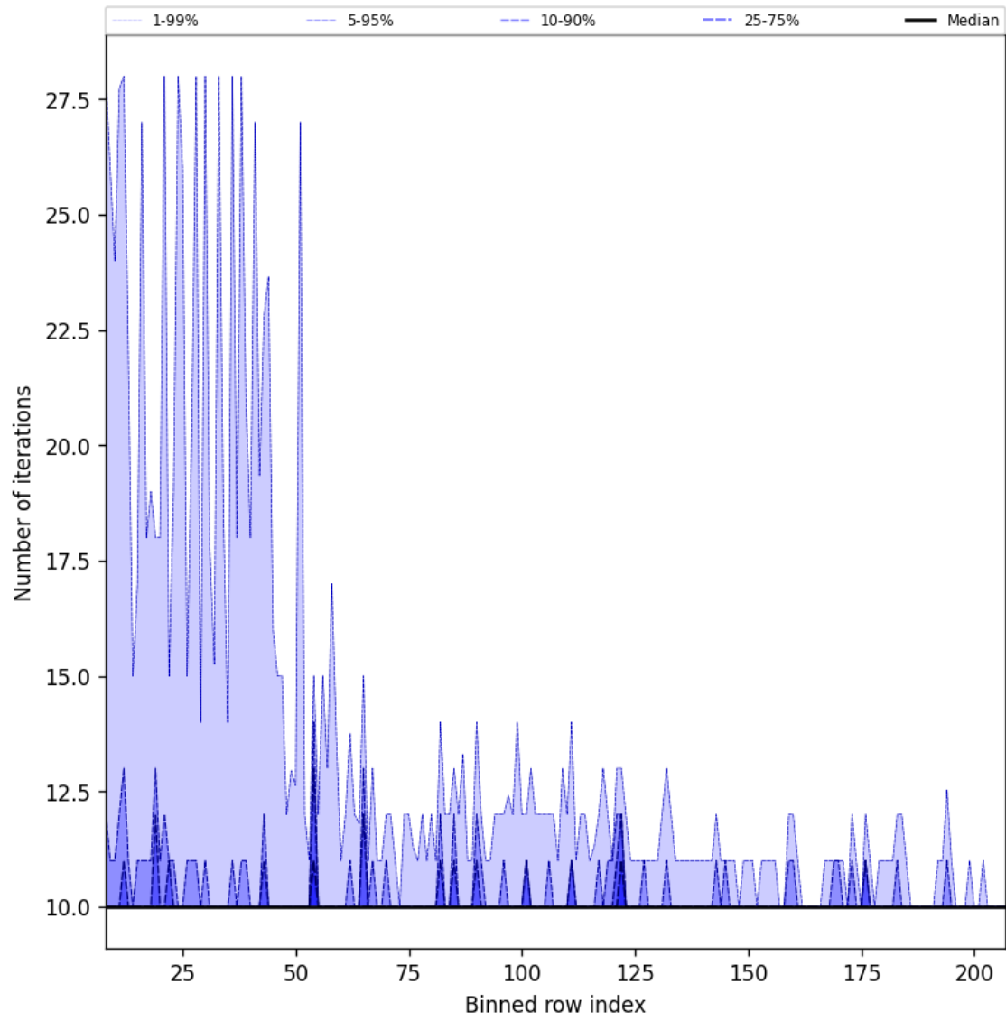
Figure 42: Along track statistics of “Number of iterations” for 2025-05-06 to 2025-05-08
