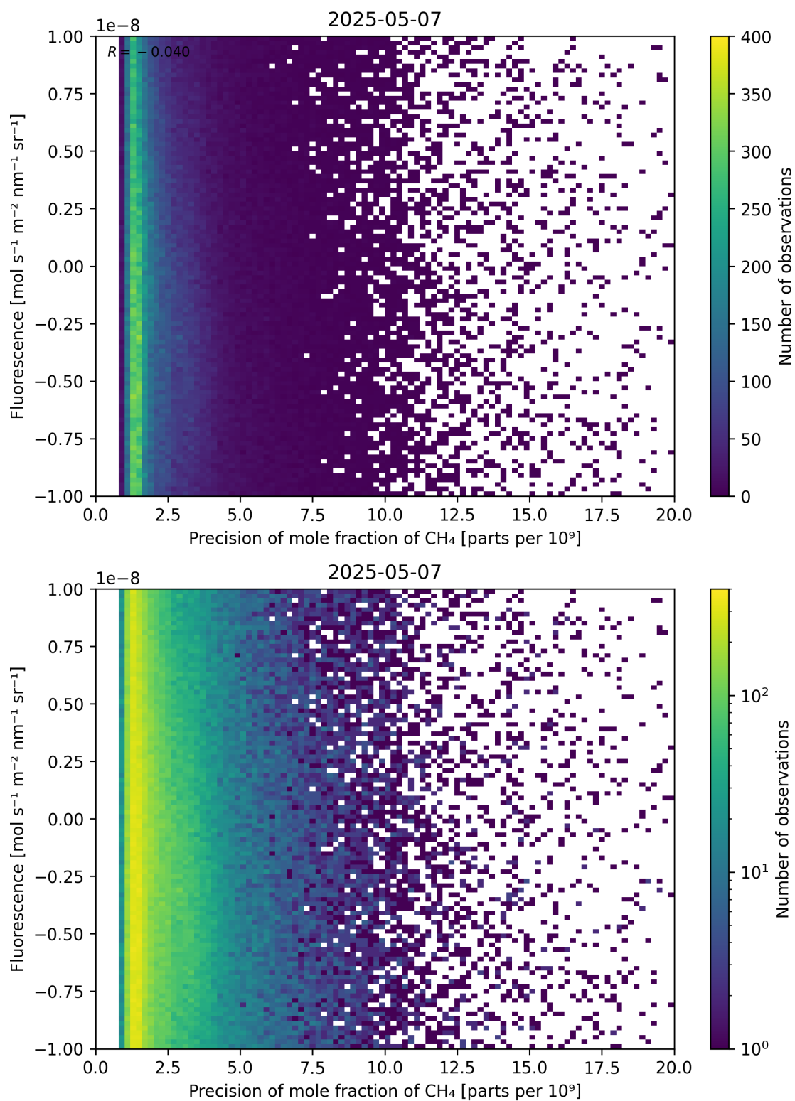
Figure 81: Scatter density plot of “Precision of mole fraction of CH 4 ” against “Fluorescence” for 2025-05-06 to 2025-05-08.
