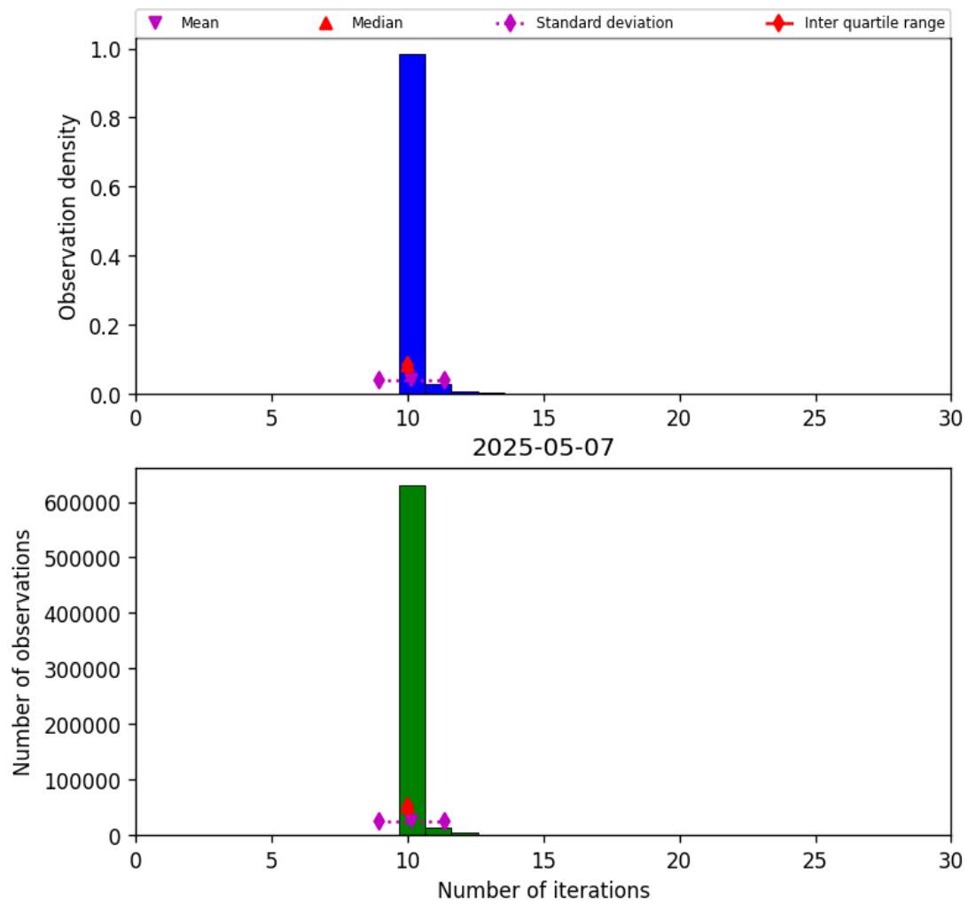
Figure 31: Histogram of “Number of iterations” for 2025-05-06 to 2025-05-08
