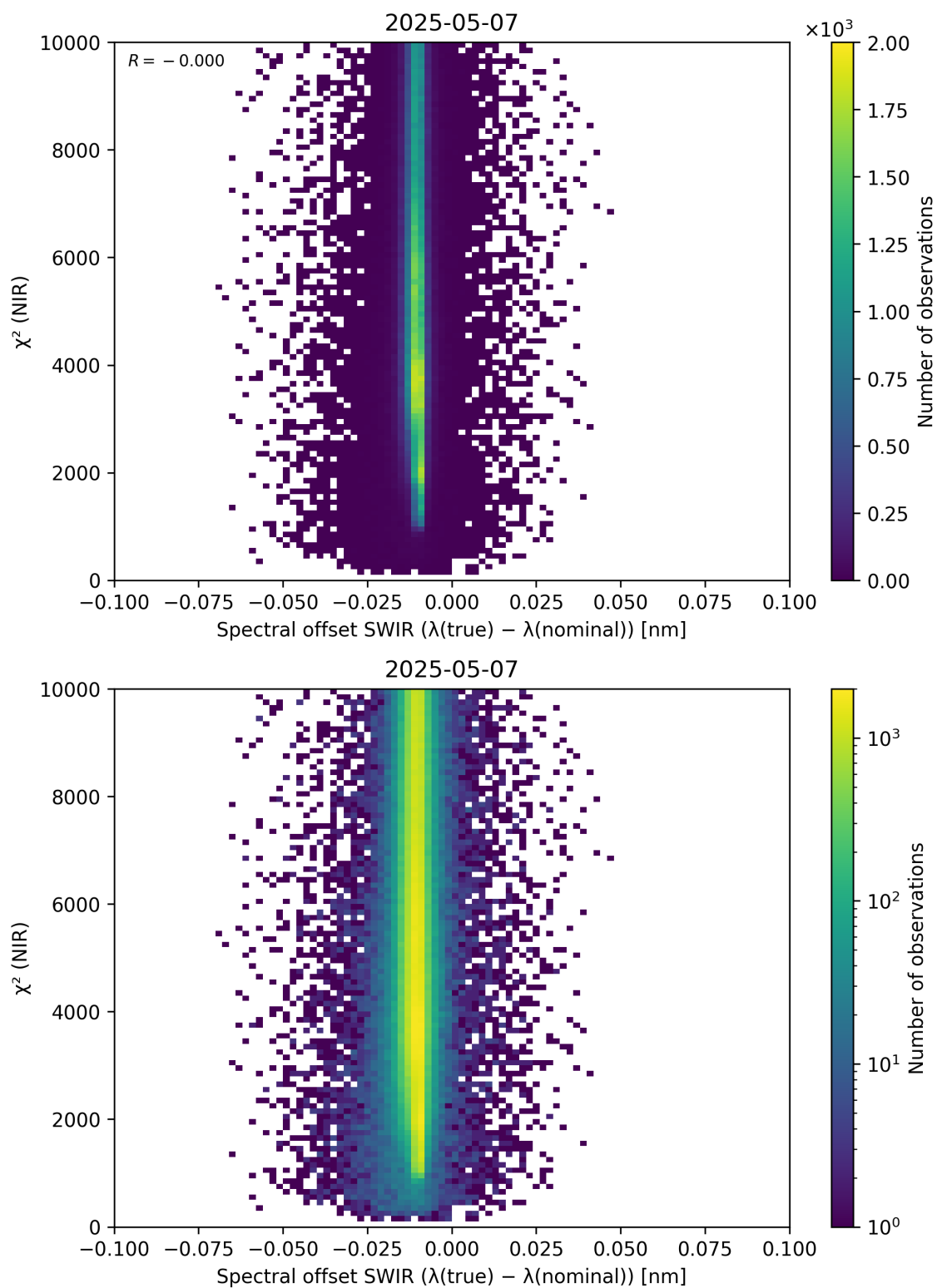
Figure 117: Scatter density plot of “Spectral offset SWIR ( \lambda_{\text{true}} - \lambda_{\text{nominal}} )” against “ \chi^2 (NIR)” for 2025-05-06 to 2025-05-08.
