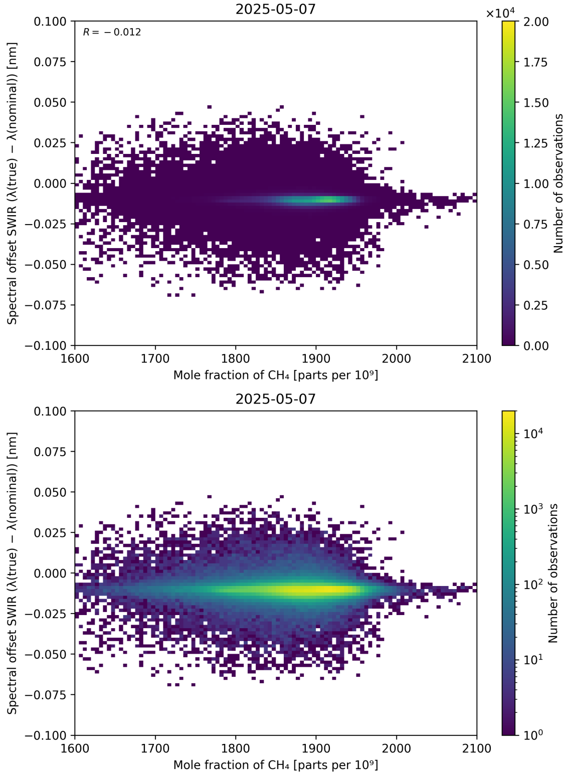
Figure 86: Scatter density plot of “Mole fraction of CH 4 ” against “Spectral offset SWIR ( \lambda_{\text{true}} - \lambda_{\text{nominal}} )” for 2025-05-06 to 2025-05-08.
