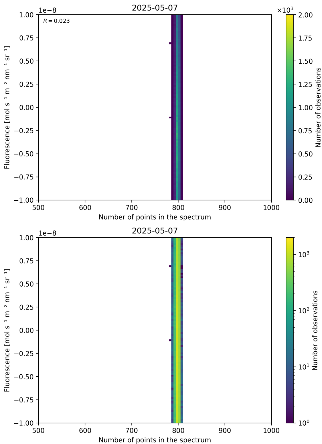
Figure 91: Scatter density plot of “Number of points in the spectrum” against “Fluorescence” for 2025-05-06 to 2025-05-08.
