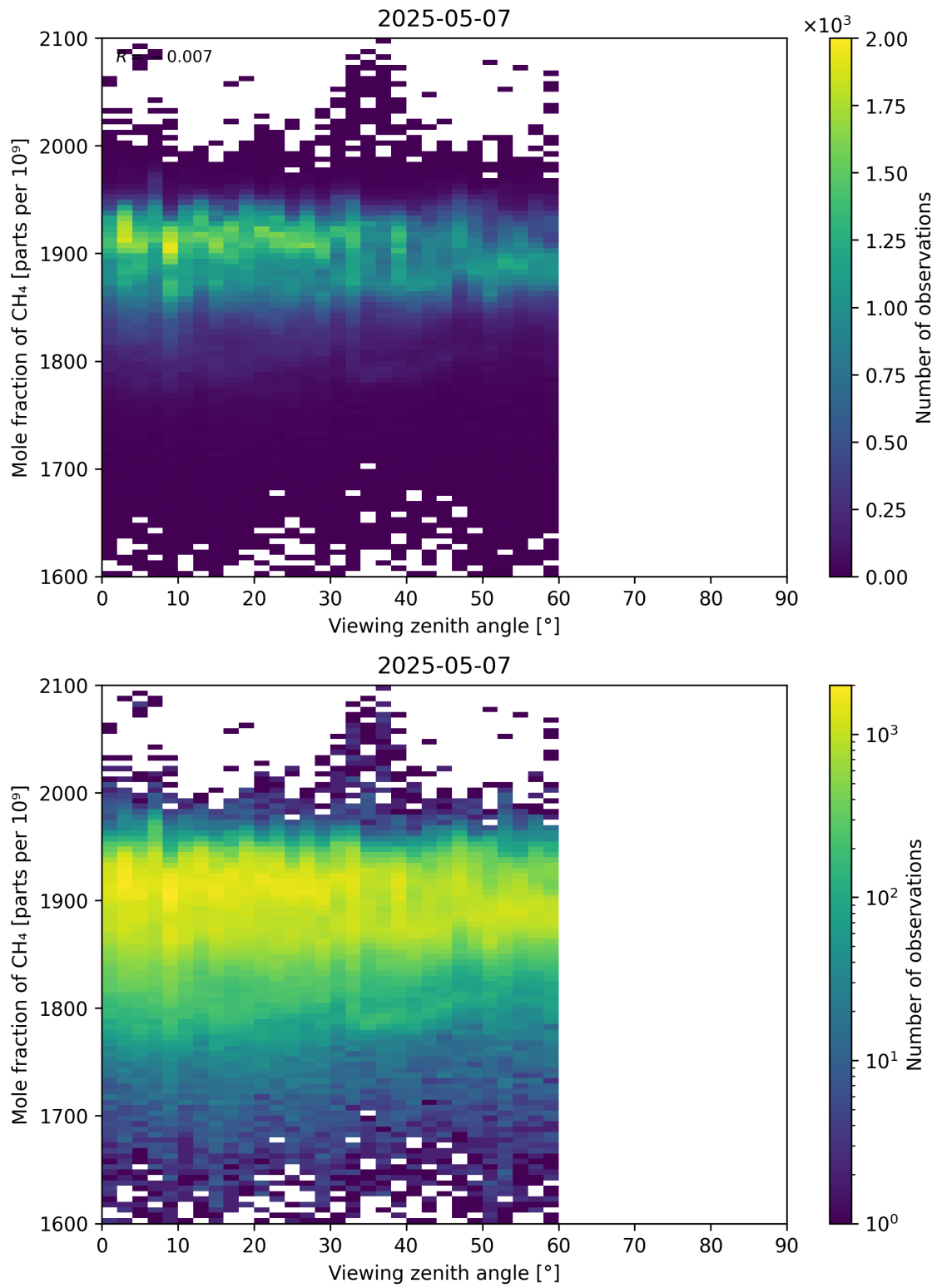
Figure 110: Scatter density plot of “Viewing zenith angle” against “Mole fraction of CH 4 ” for 2025-05-06 to 2025-05-08.
