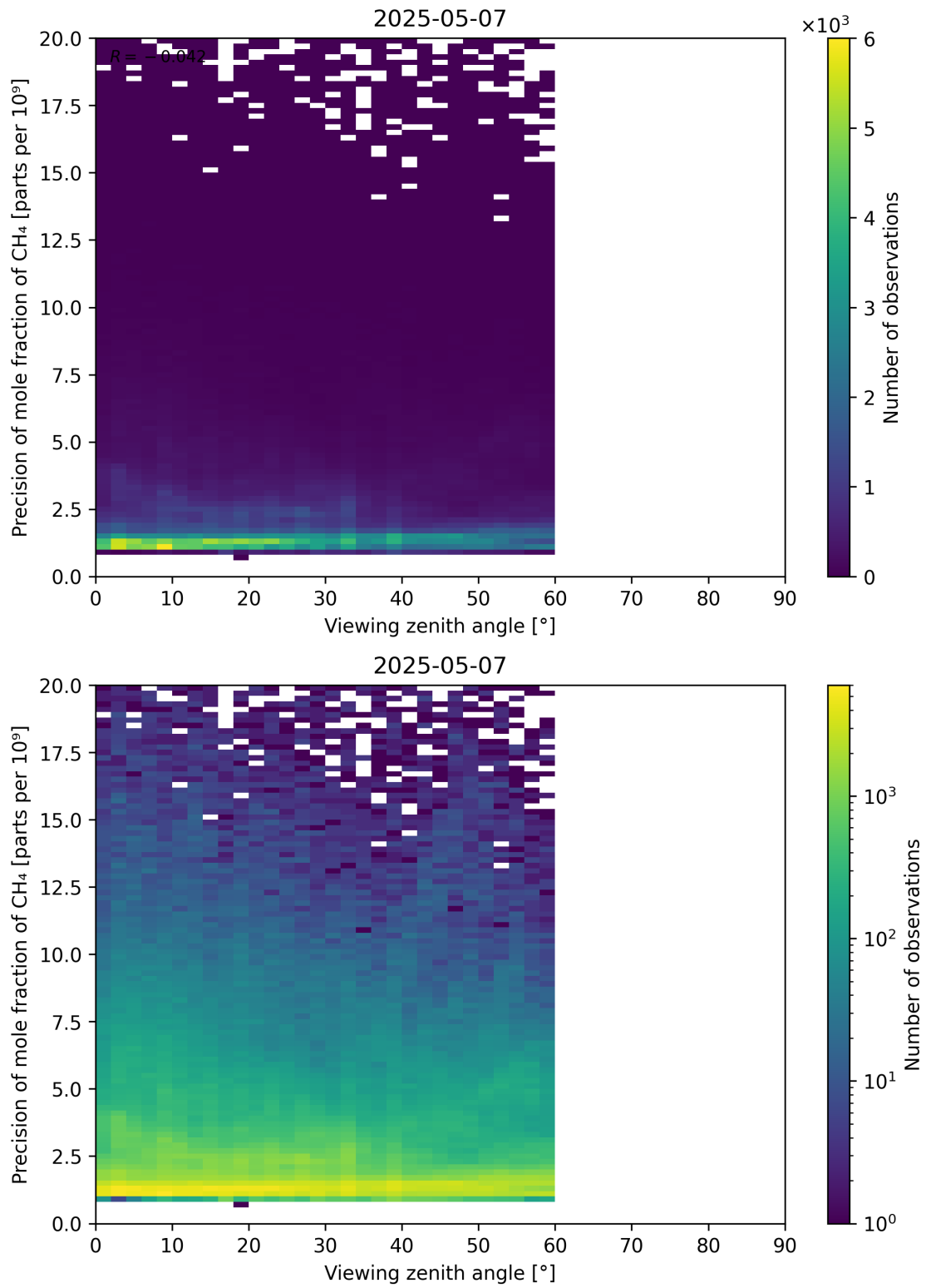
Figure 112: Scatter density plot of “Viewing zenith angle” against “Precision of mole fraction of CH 4 ” for 2025-05-06 to 2025-05-08.
