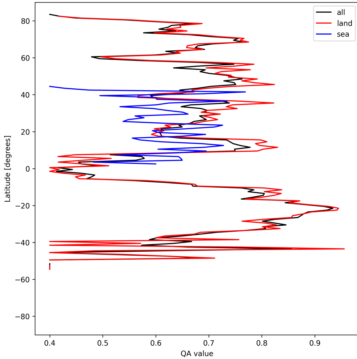
Figure 11: Zonal average of “QA value” for 2025-05-06 to 2025-05-08.
