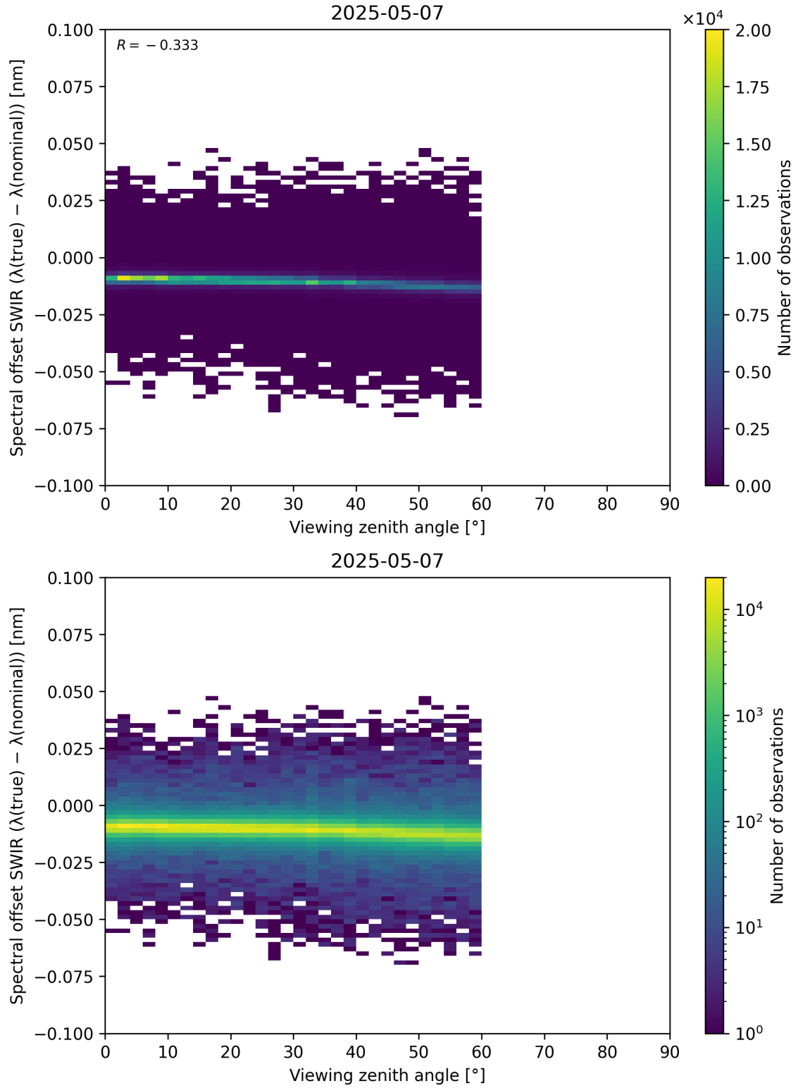
Figure 116: Scatter density plot of “Viewing zenith angle” against “Spectral offset SWIR ( \lambda_{\text{true}} - \lambda_{\text{nominal}} )” for 2025-05-06 to 2025-05-08.
