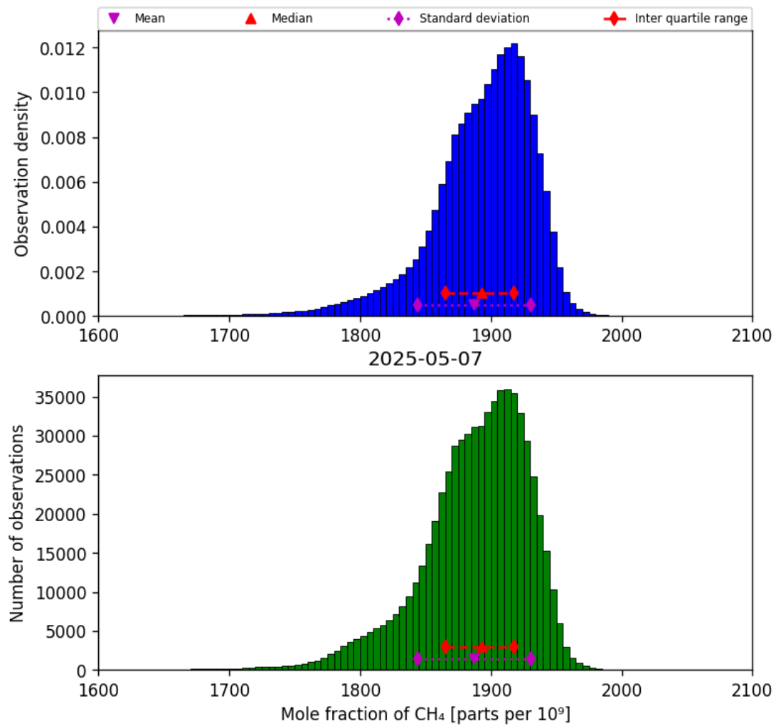
Figure 23: Histogram of “Mole fraction of CH 4 ” for 2025-05-06 to 2025-05-08
