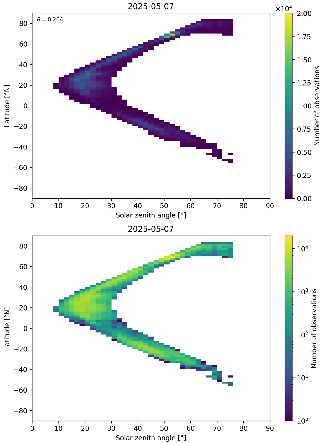
Figure 98: Scatter density plot of “Solar zenith angle” against “Latitude” for 2025-05-06 to 2025-05-08.
