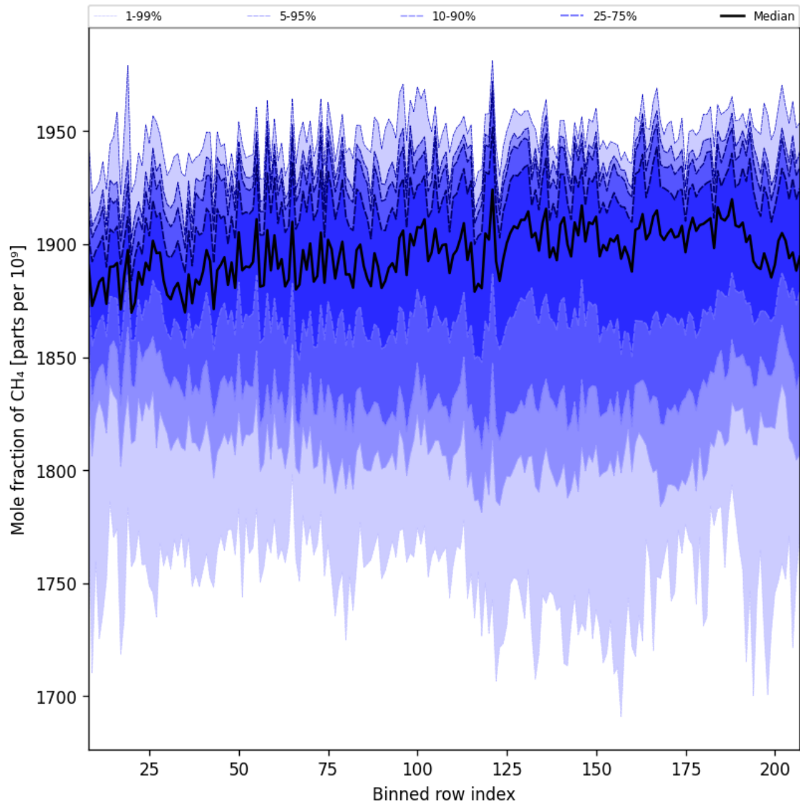
Figure 34: Along track statistics of “Mole fraction of CH 4 ” for 2025-05-06 to 2025-05-08
