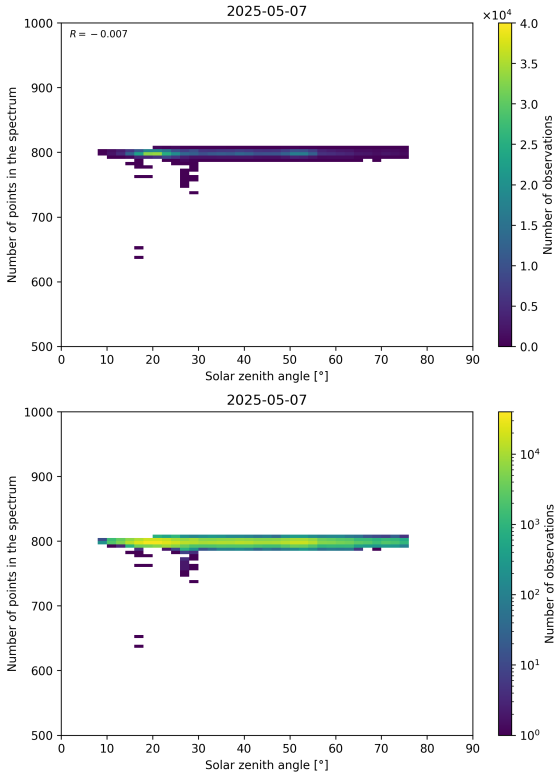
Figure 103: Scatter density plot of “Solar zenith angle” against “Number of points in the spectrum” for 2025-05-06 to 2025-05-08.
