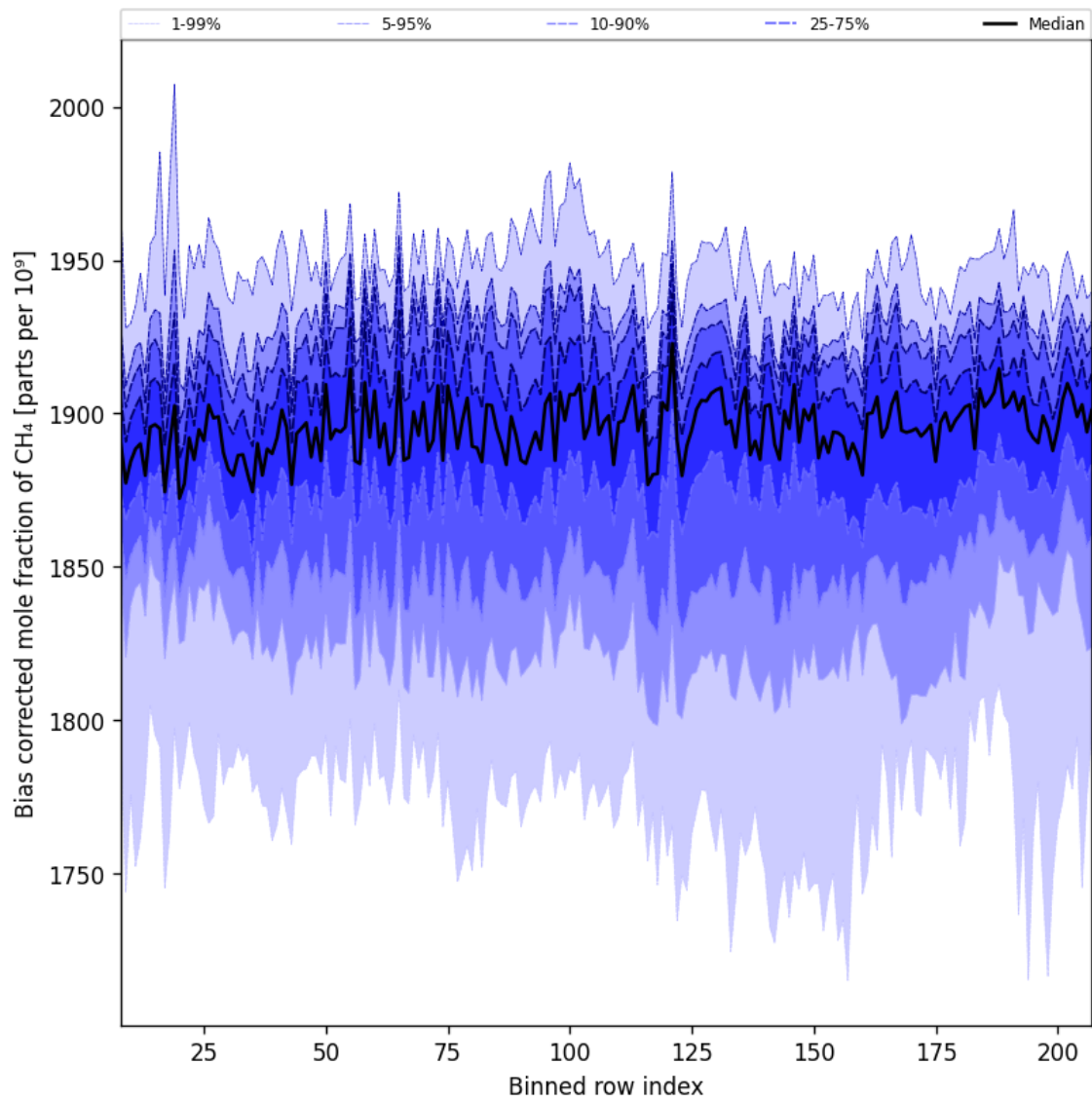
Figure 36: Along track statistics of “Bias corrected mole fraction of CH 4 ” for 2025-05-06 to 2025-05-08
