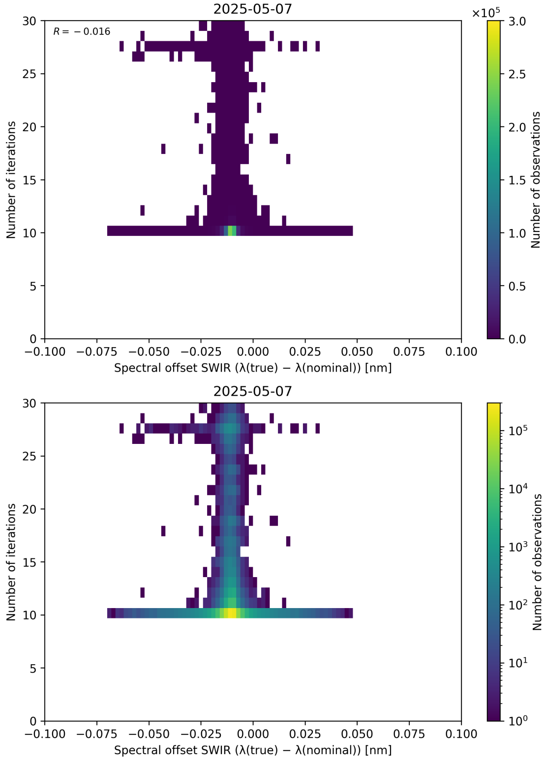
Figure 121: Scatter density plot of “Spectral offset SWIR ( \lambda_{\text{true}} - \lambda_{\text{nominal}} )” against “Number of iterations” for 2025-05-06 to 2025-05-08.
