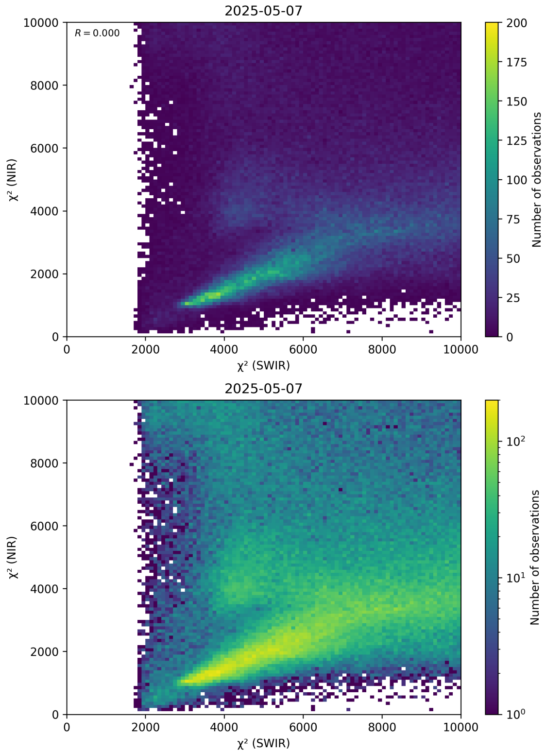
Figure 47: Scatter density plot of “ \chi^2 (SWIR)” against “ \chi^2 (NIR)” for 2025-05-06 to 2025-05-08.
