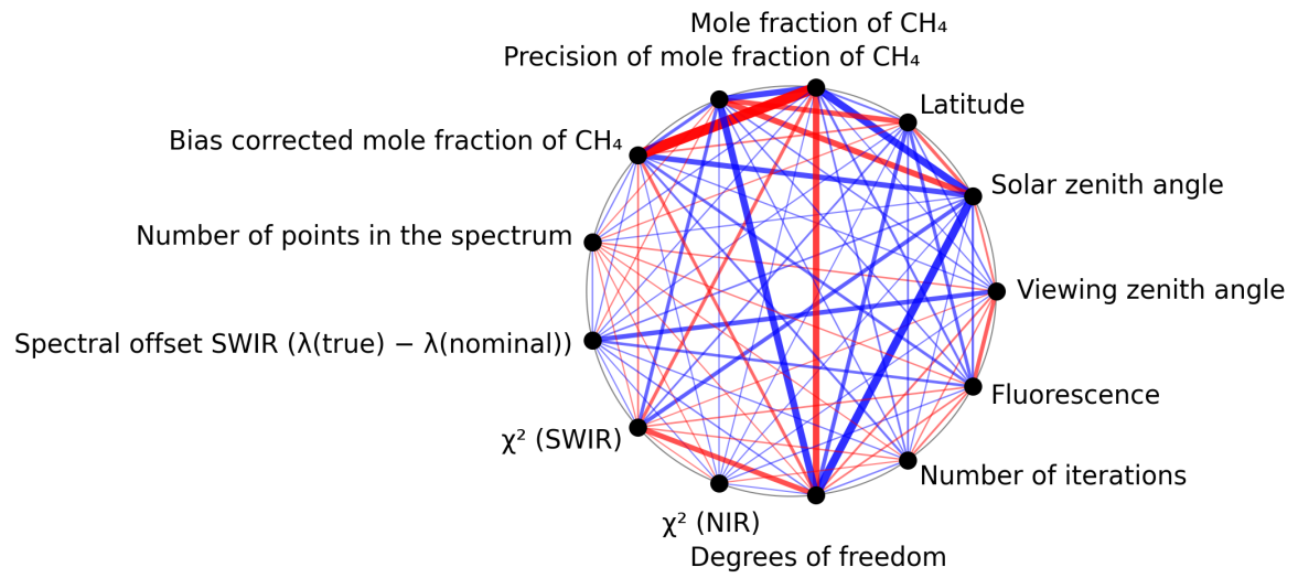
Figure 1: Map of correlation graph for 2025-05-06 to 2025-05-08.
