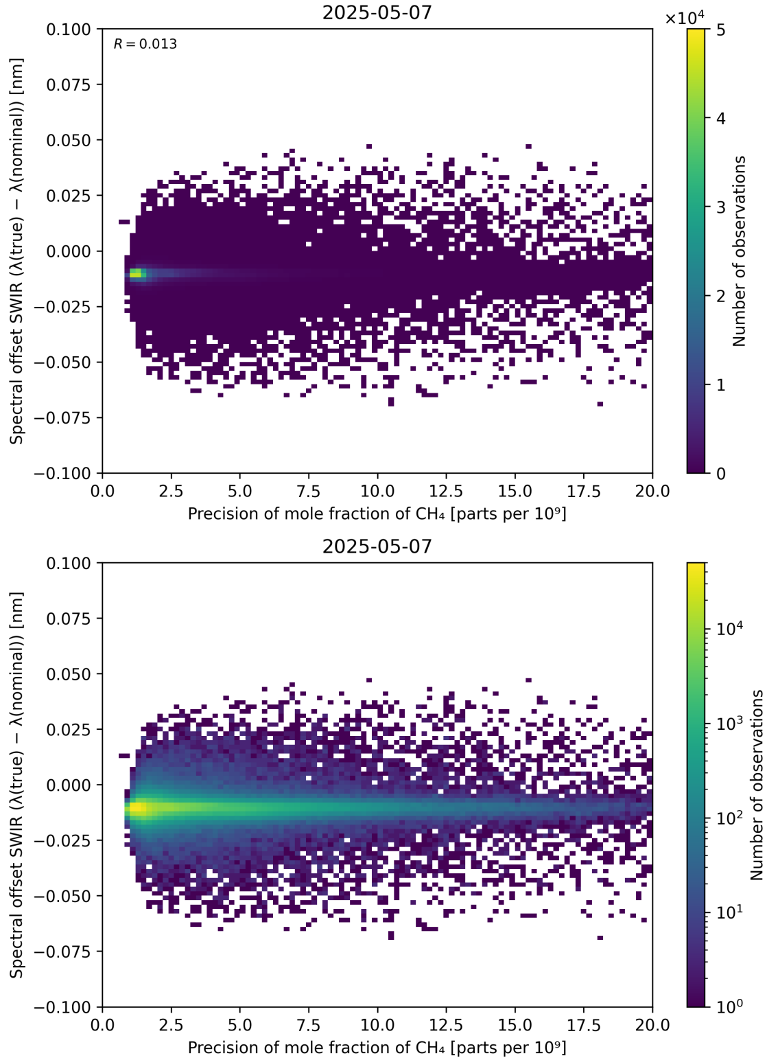
Figure 85: Scatter density plot of “Precision of mole fraction of CH 4 ” against “Spectral offset SWIR ( \lambda_{\text{true}} - \lambda_{\text{nominal}} )” for 2025-05-06 to 2025-05-08.
