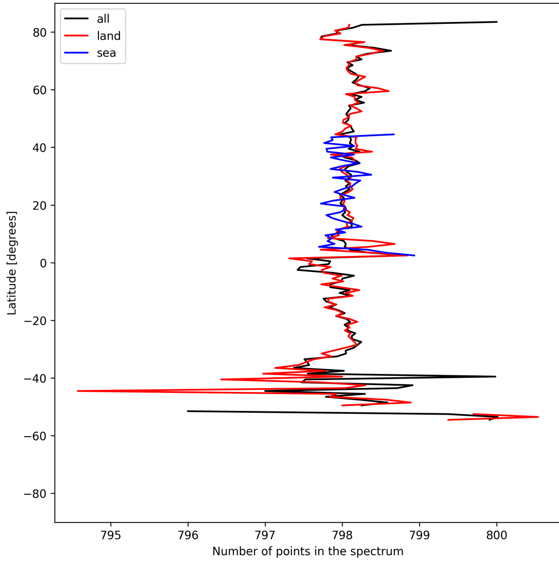
Figure 15: Zonal average of “Number of points in the spectrum” for 2025-05-06 to 2025-05-08.
