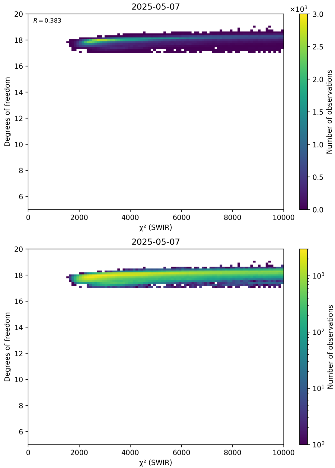
Figure 48: Scatter density plot of " \chi^2 (SWIR)" against "Degrees of freedom" for 2025-05-06 to 2025-05-08.
