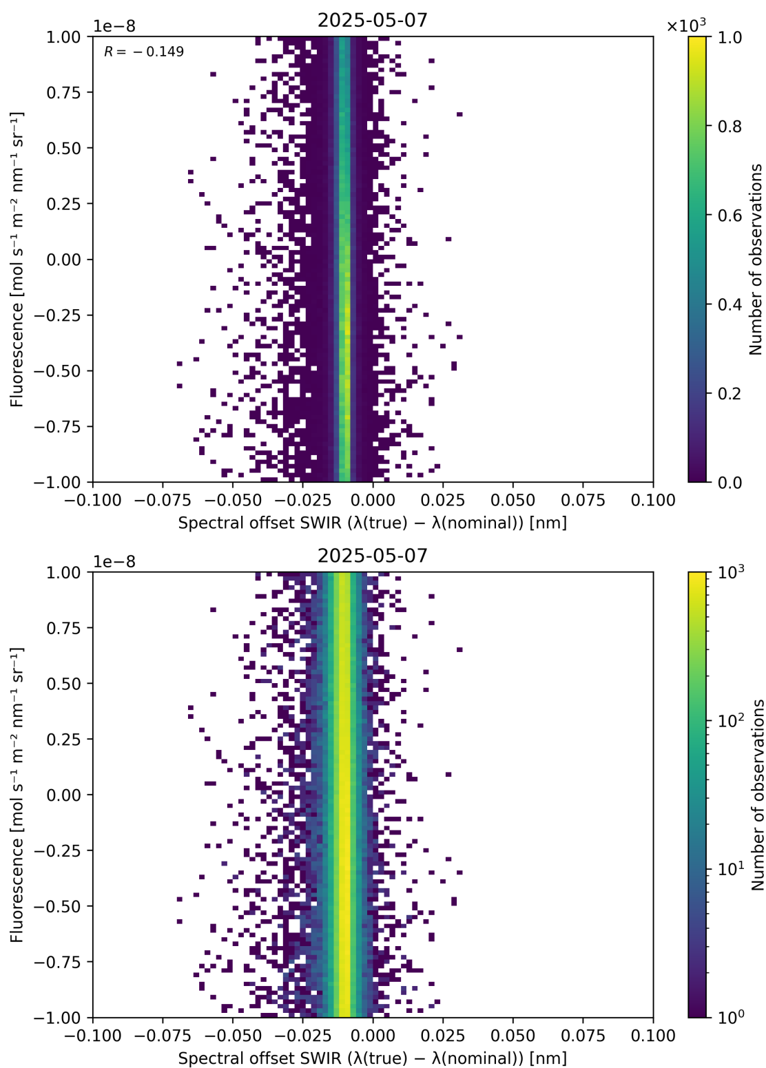
Figure 120: Scatter density plot of “Spectral offset SWIR ( \lambda_{\text{true}} - \lambda_{\text{nominal}} )” against “Fluorescence” for 2025-05-06 to 2025-05-08.
