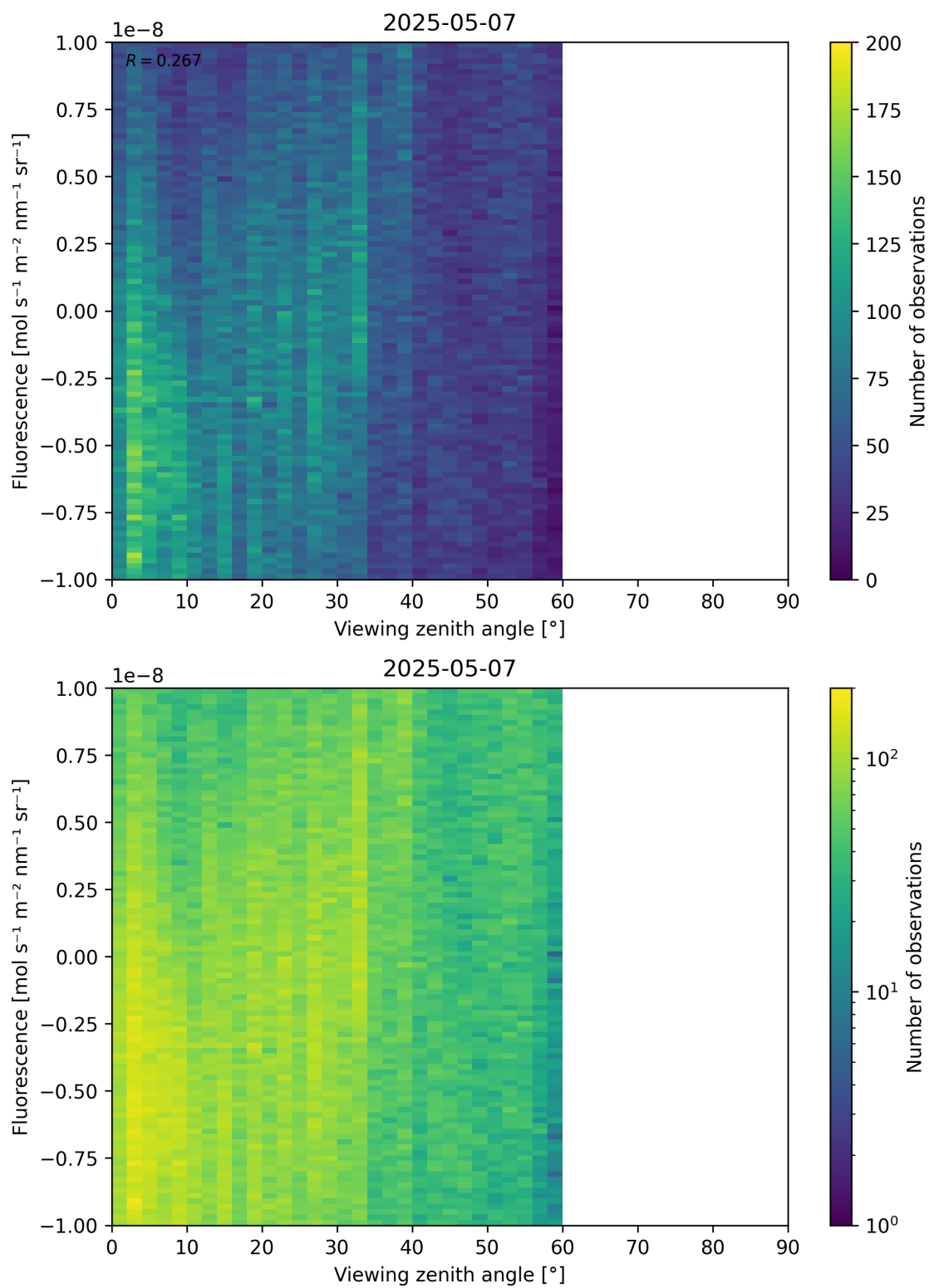
Figure 108: Scatter density plot of “Viewing zenith angle” against “Fluorescence” for 2025-05-06 to 2025-05-08.
