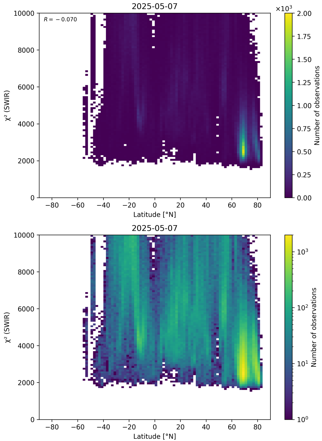
Figure 54: Scatter density plot of “Latitude” against “ \chi^2 (SWIR)” for 2025-05-06 to 2025-05-08.
