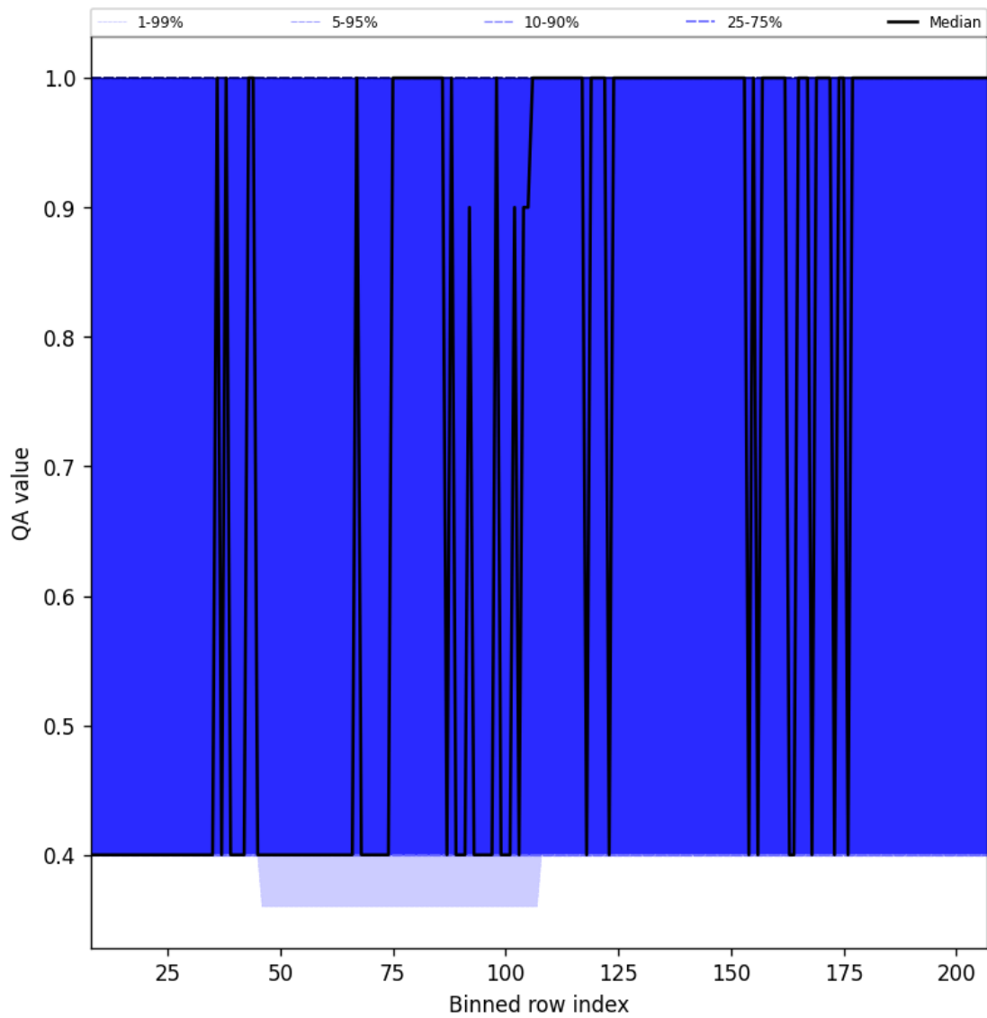
Figure 33: Along track statistics of “QA value” for 2025-05-06 to 2025-05-08
