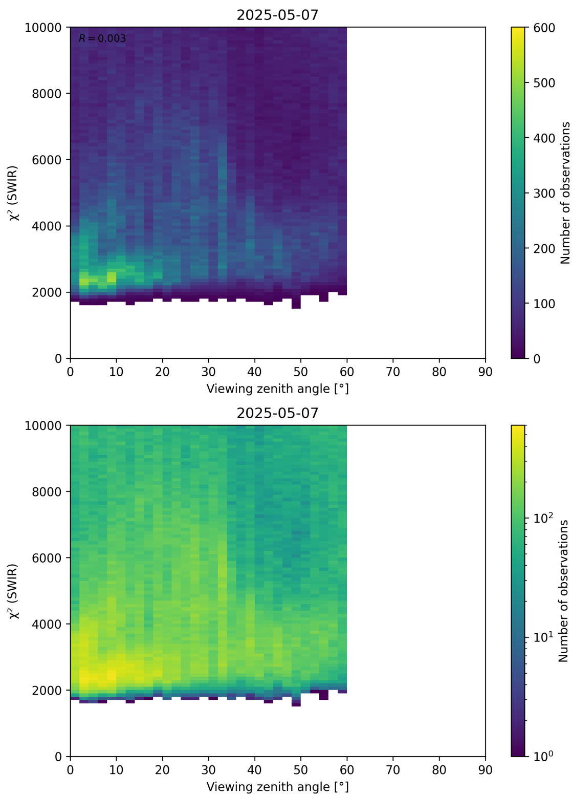
Figure 106: Scatter density plot of “Viewing zenith angle” against “ \chi^2 (SWIR)” for 2025-05-06 to 2025-05-08.
