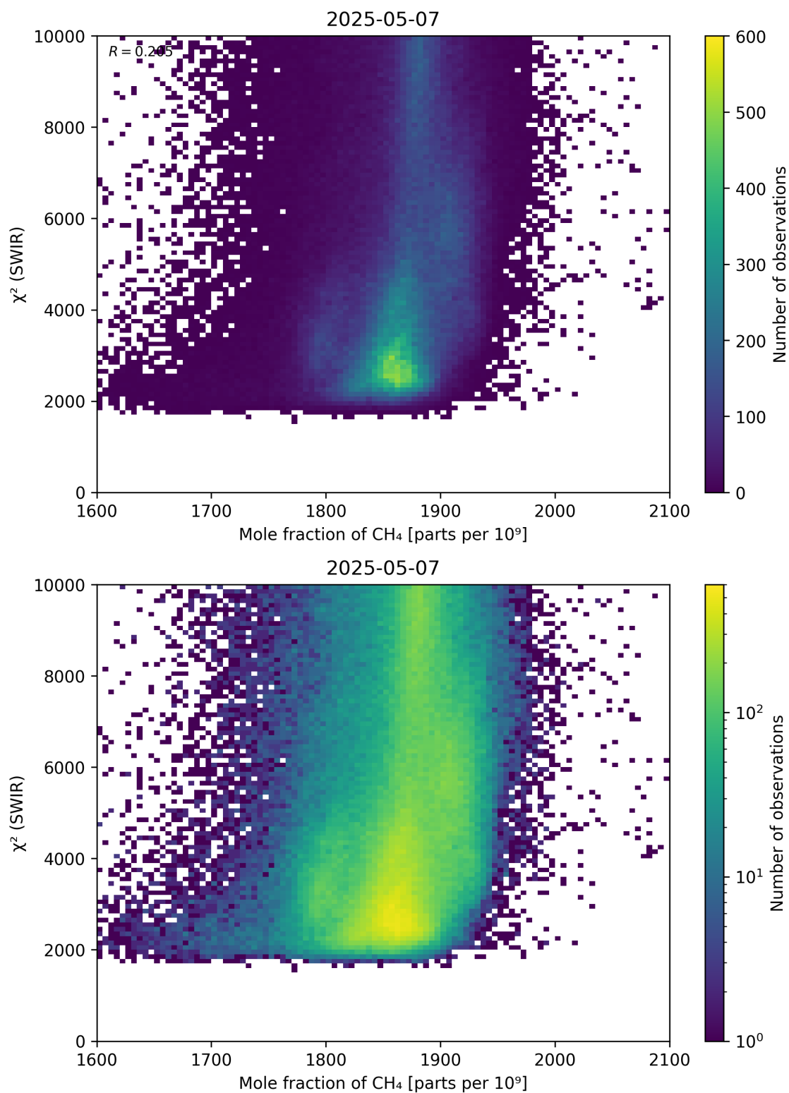
Figure 71: Scatter density plot of “Mole fraction of \text{CH}_4 ” against “ \chi^2 (SWIR)” for 2025-05-06 to 2025-05-08.
