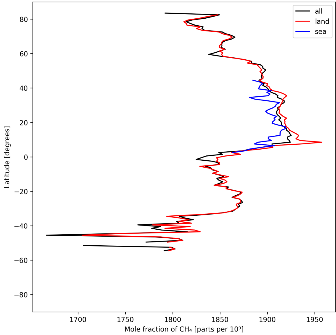
Figure 12: Zonal average of “Mole fraction of \text{CH}_4 ” for 2025-05-06 to 2025-05-08.
