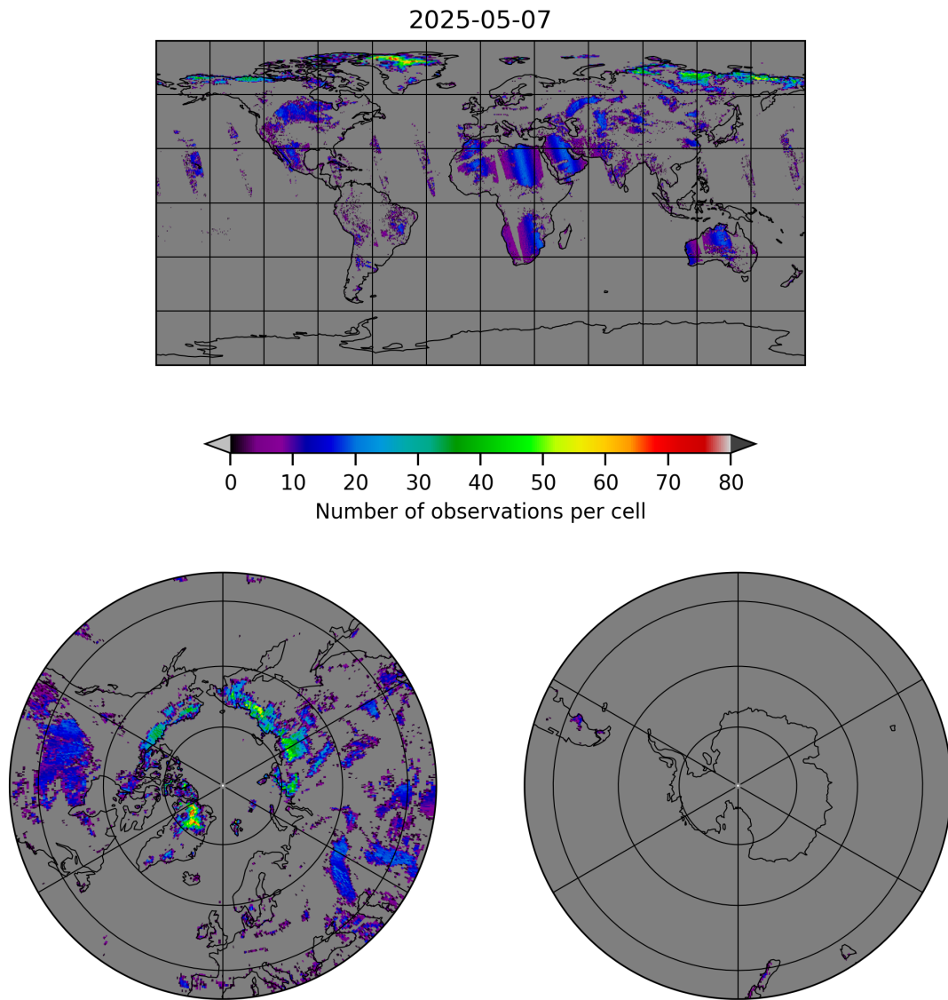
Figure 10: Map of the number of observations for 2025-05-06 to 2025-05-08
