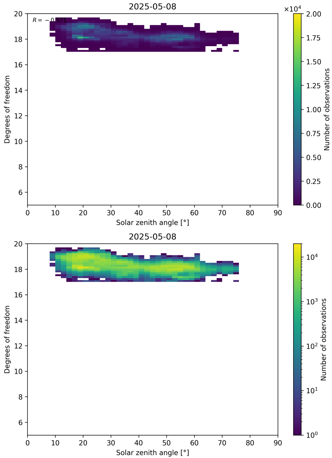
Figure 96: Scatter density plot of “Solar zenith angle” against “Degrees of freedom” for 2025-05-07 to 2025-05-09.
