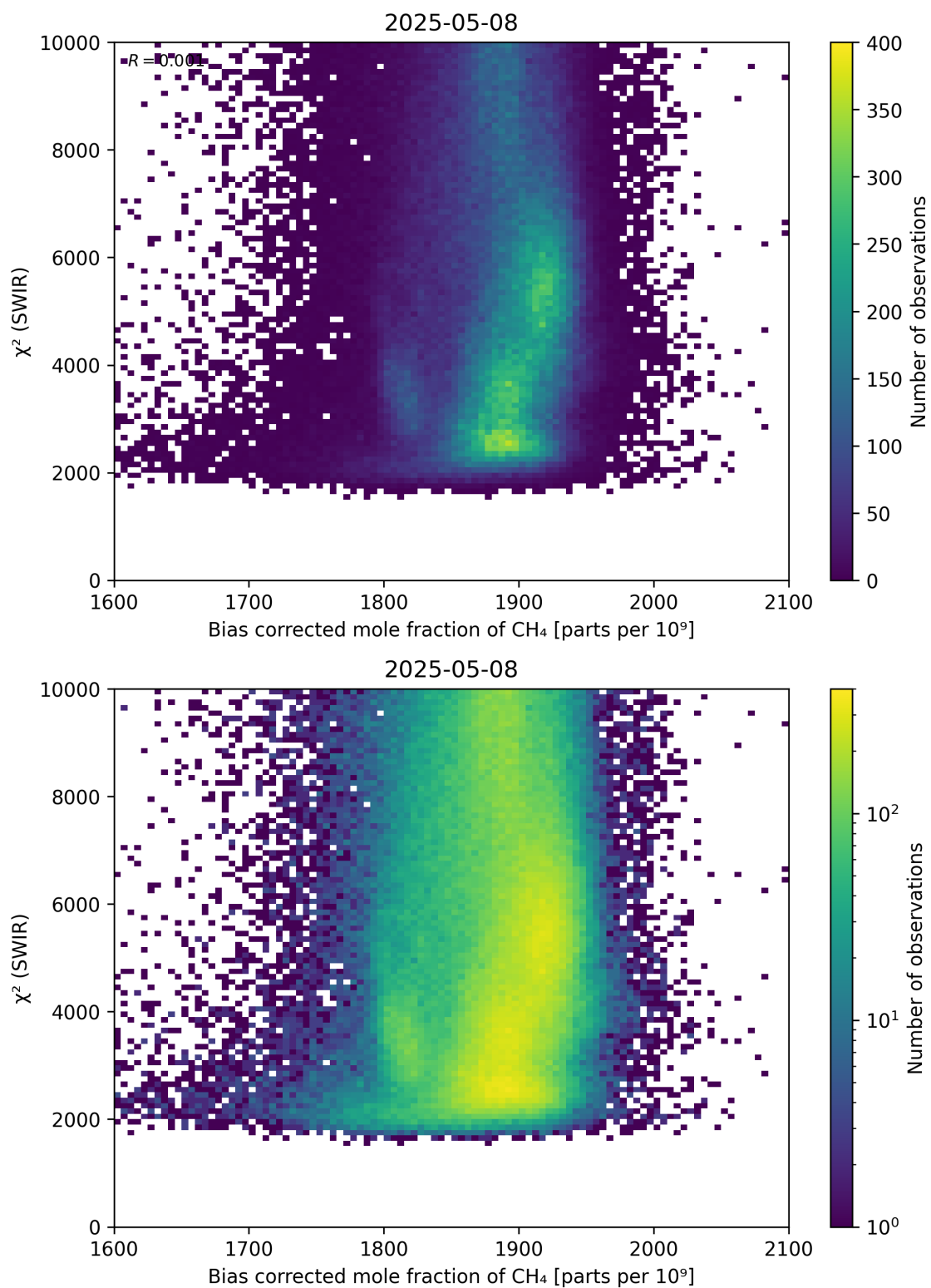
Figure 64: Scatter density plot of “Bias corrected mole fraction of CH 4 ” against “ \chi^2 (SWIR)” for 2025-05-07 to 2025-05-09.
