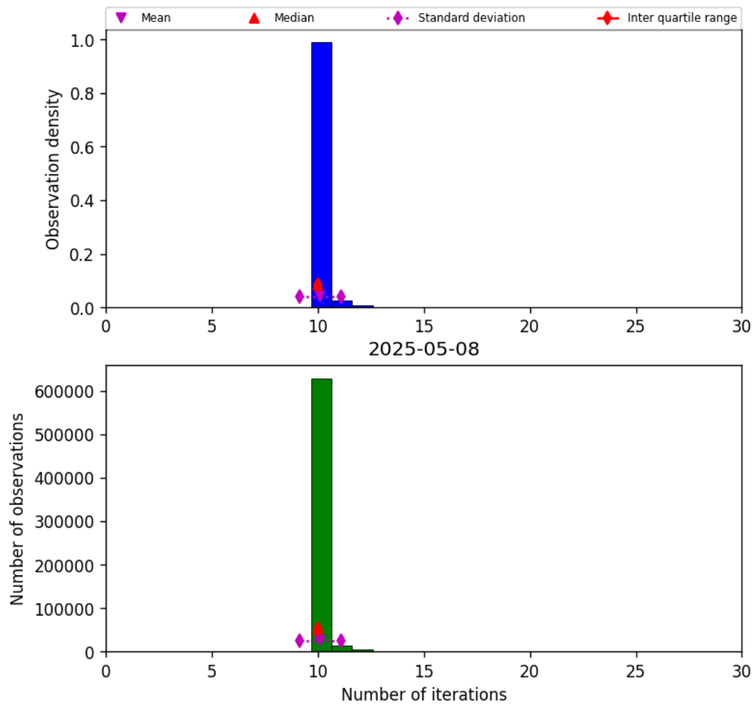
Figure 31: Histogram of “Number of iterations” for 2025-05-07 to 2025-05-09
