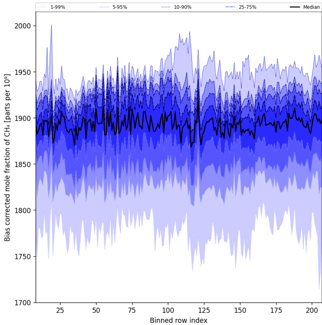
Figure 36: Along track statistics of “Bias corrected mole fraction of CH 4 ” for 2025-05-07 to 2025-05-09
