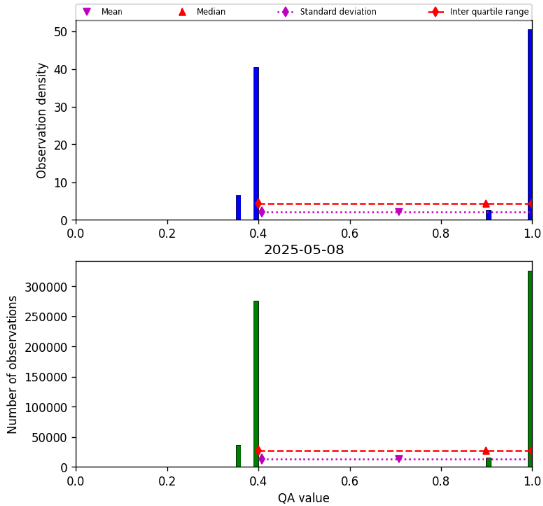
Figure 22: Histogram of “QA value” for 2025-05-07 to 2025-05-09
