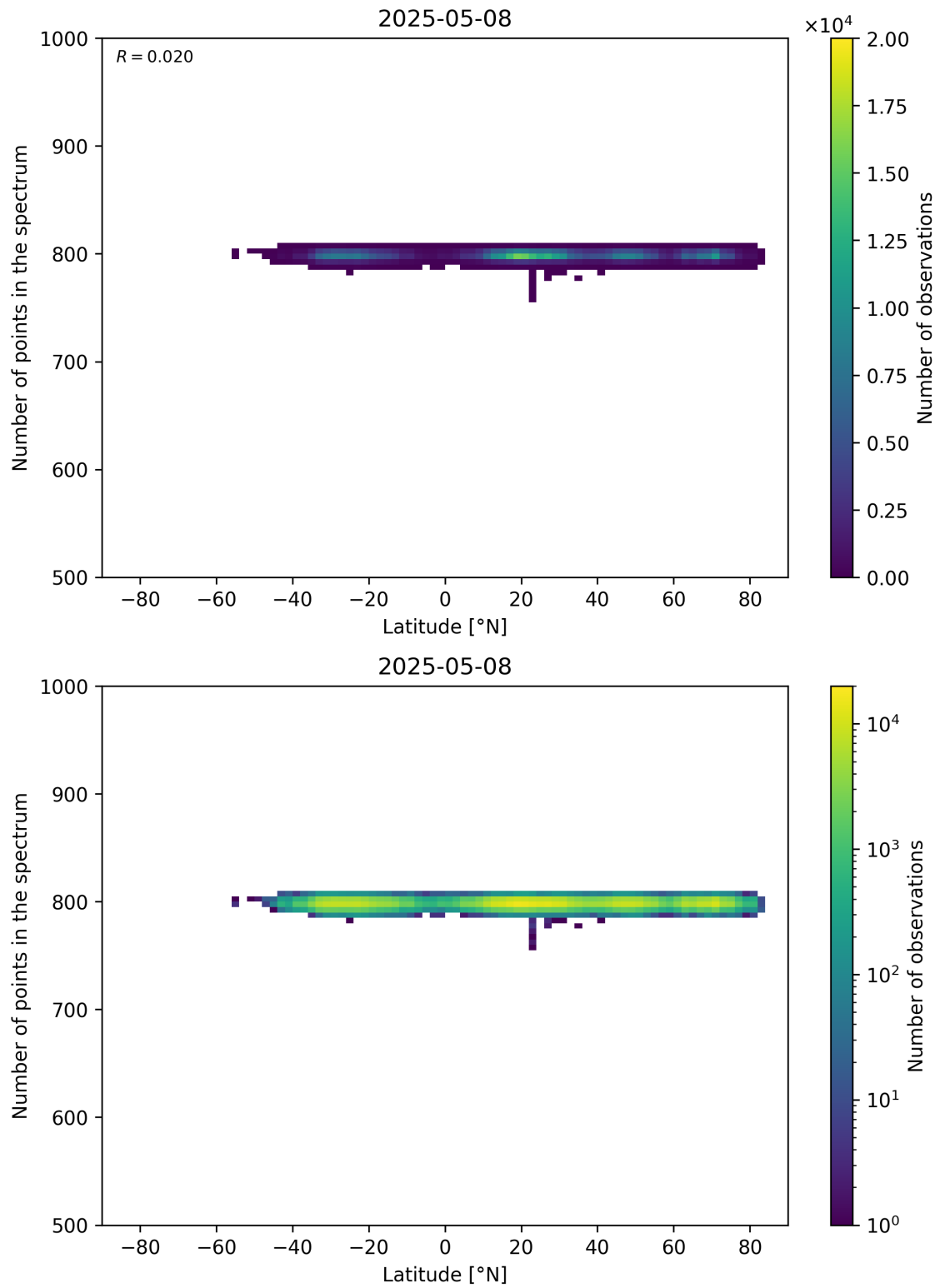
Figure 61: Scatter density plot of “Latitude” against “Number of points in the spectrum” for 2025-05-07 to 2025-05-09.
