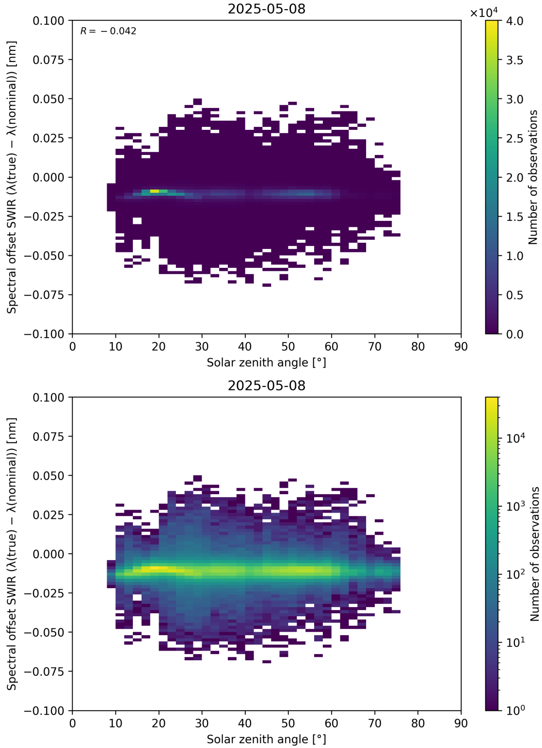
Figure 104: Scatter density plot of “Solar zenith angle” against “Spectral offset SWIR ( \lambda_{\text{true}} - \lambda_{\text{nominal}} )” for 2025-05-07 to 2025-05-09.
