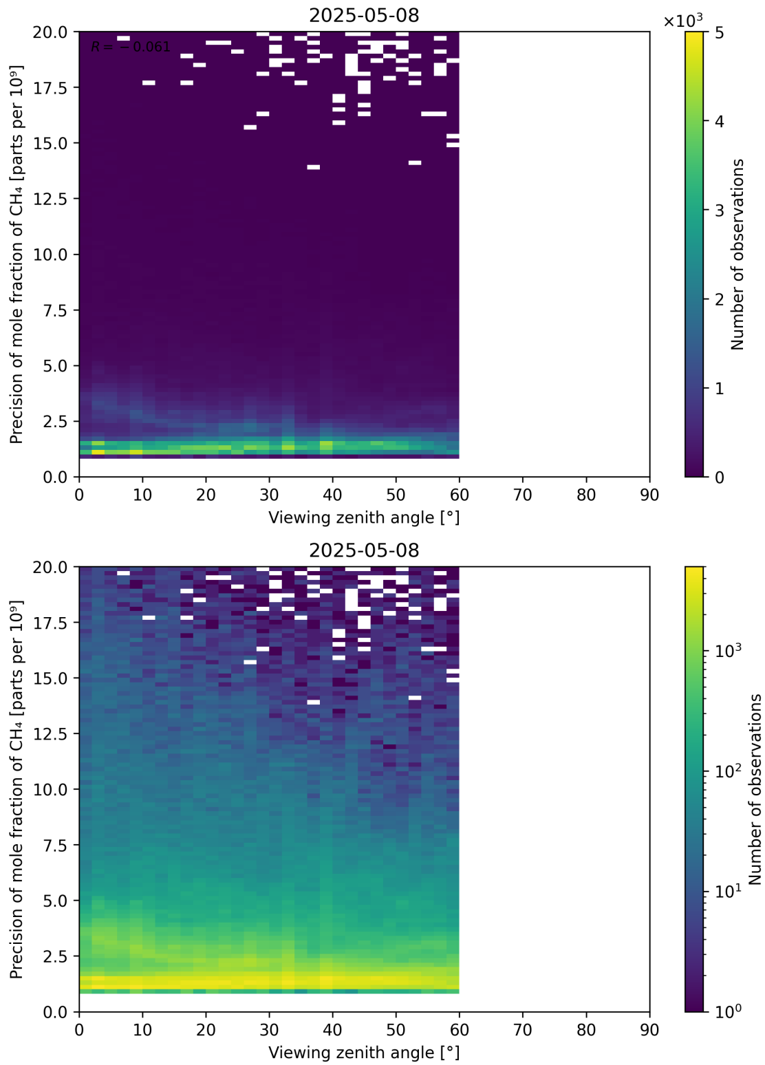
Figure 112: Scatter density plot of “Viewing zenith angle” against “Precision of mole fraction of CH 4 ” for 2025-05-07 to 2025-05-09.
