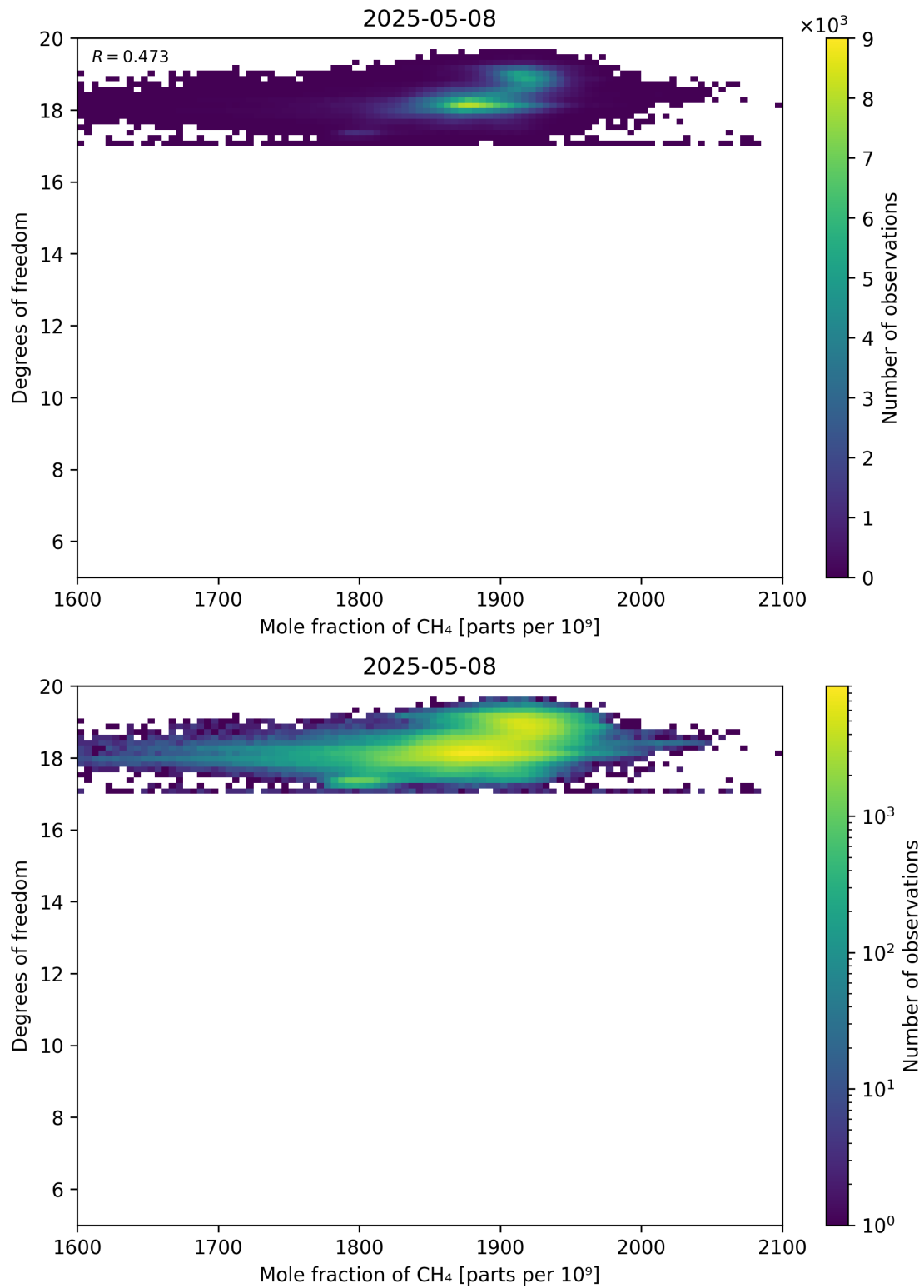
Figure 72: Scatter density plot of “Mole fraction of CH 4 ” against “Degrees of freedom” for 2025-05-07 to 2025-05-09.
