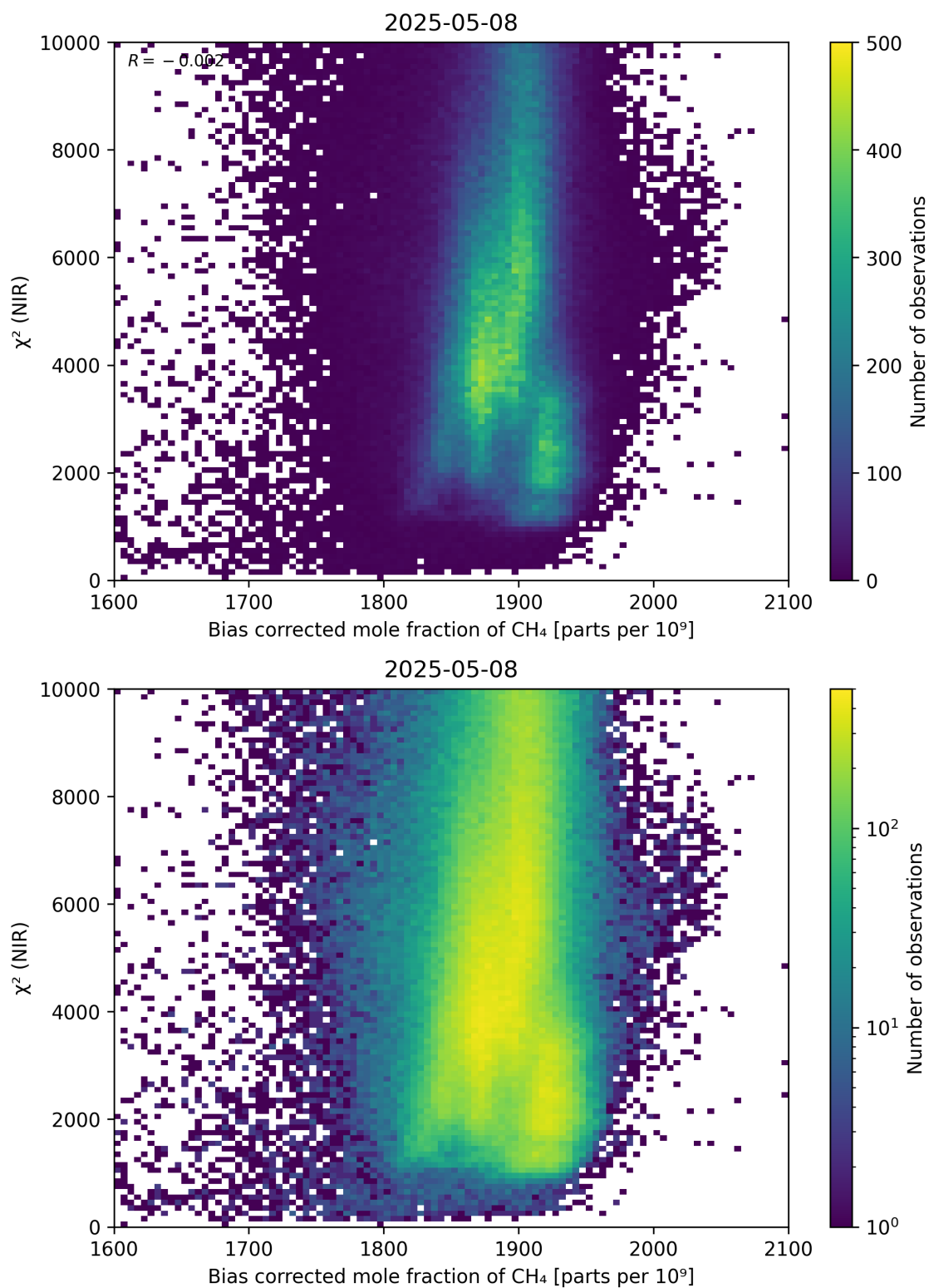
Figure 63: Scatter density plot of “Bias corrected mole fraction of CH 4 ” against “ \chi^2 (NIR)” for 2025-05-07 to 2025-05-09.
