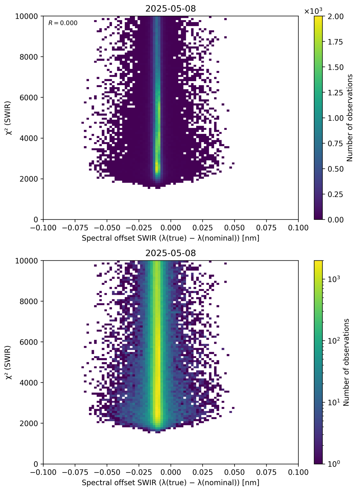
Figure 118: Scatter density plot of “Spectral offset SWIR ( \lambda_{\text{true}} - \lambda_{\text{nominal}} )” against “ \chi^2 (SWIR)” for 2025-05-07 to 2025-05-09.
