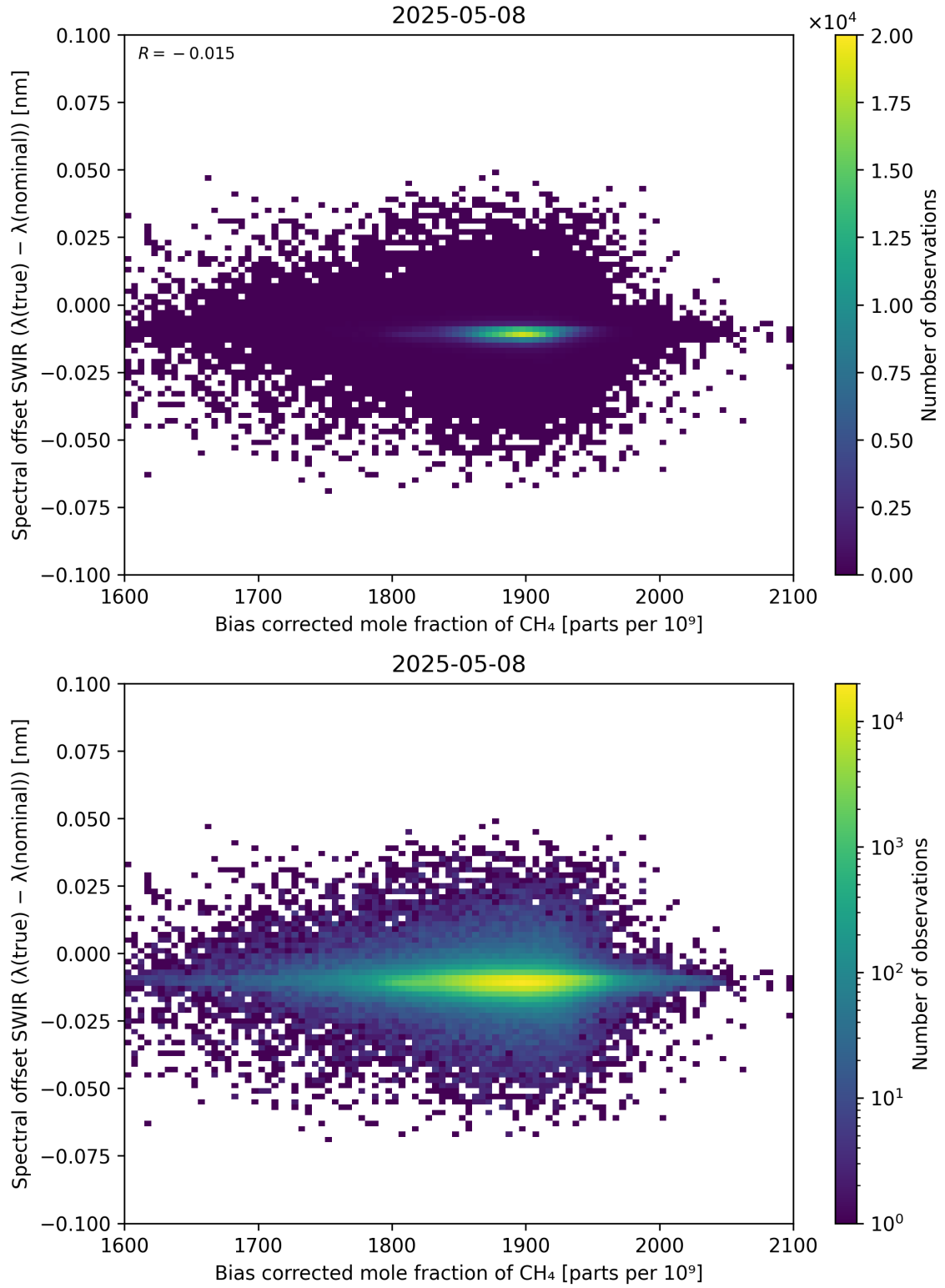
Figure 69: Scatter density plot of “Bias corrected mole fraction of \text{CH}_4 ” against “Spectral offset SWIR ( \lambda_{\text{true}} - \lambda_{\text{nominal}} )” for 2025-05-07 to 2025-05-09.
