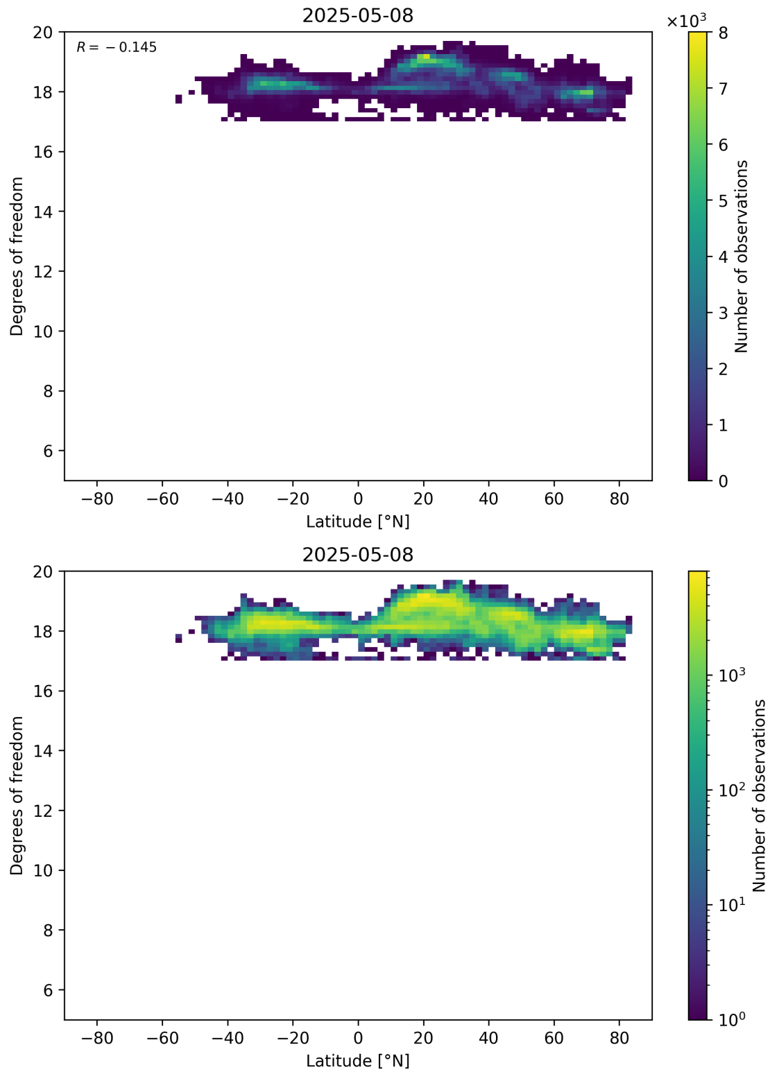
Figure 55: Scatter density plot of “Latitude” against “Degrees of freedom” for 2025-05-07 to 2025-05-09.
