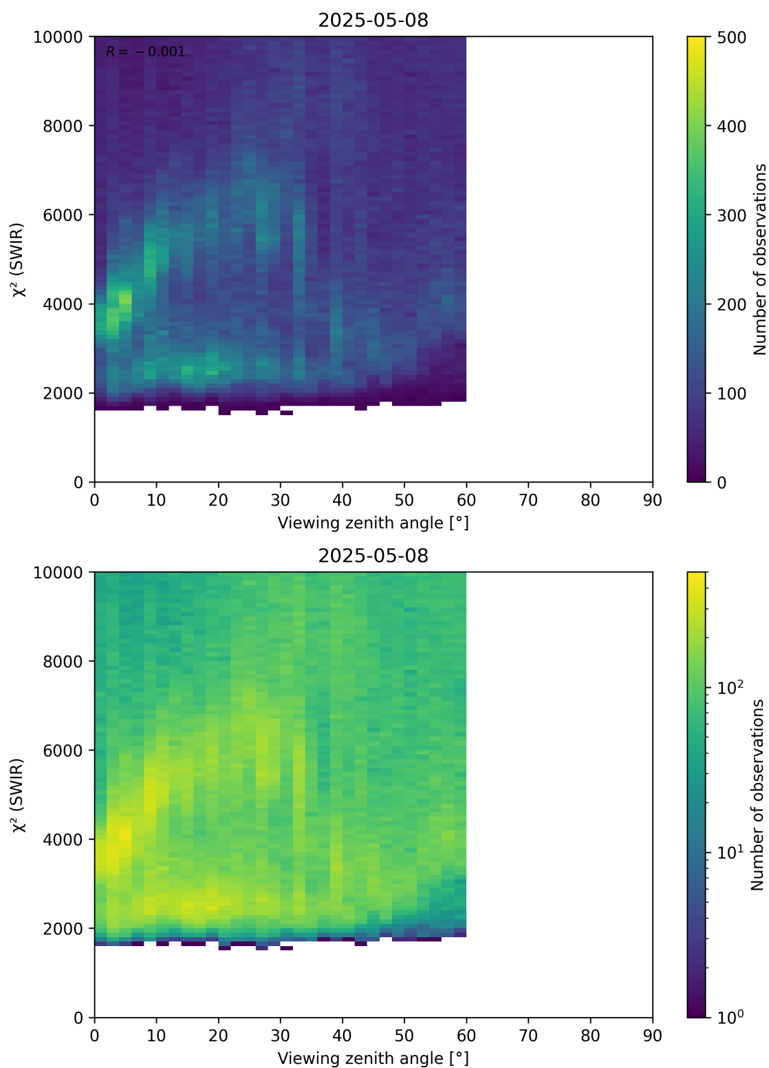
Figure 106: Scatter density plot of “Viewing zenith angle” against “ \chi^2 (SWIR)” for 2025-05-07 to 2025-05-09.
