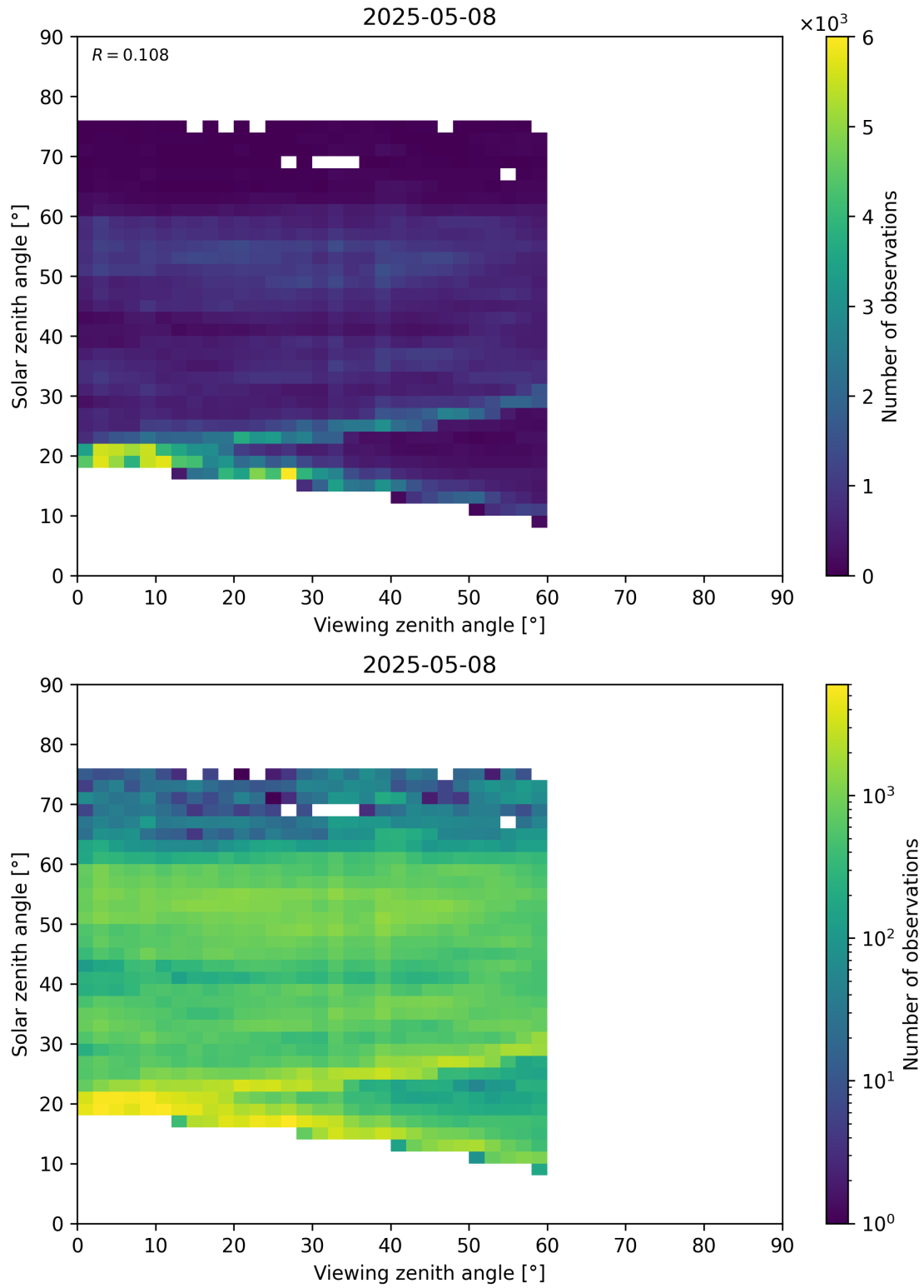
Figure 115: Scatter density plot of “Viewing zenith angle” against “Solar zenith angle” for 2025-05-07 to 2025-05-09.
