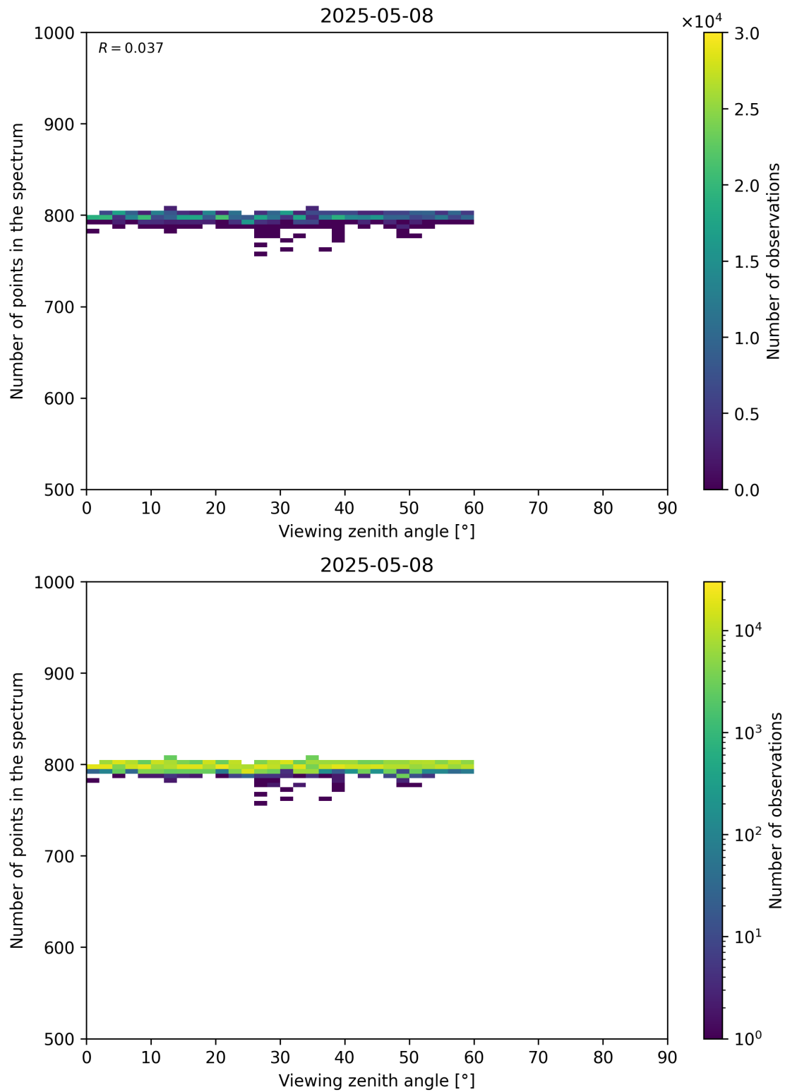
Figure 114: Scatter density plot of “Viewing zenith angle” against “Number of points in the spectrum” for 2025-05-07 to 2025-05-09.
