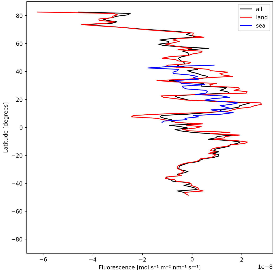
Figure 21: Zonal average of “Fluorescence” for 2025-05-07 to 2025-05-09.
