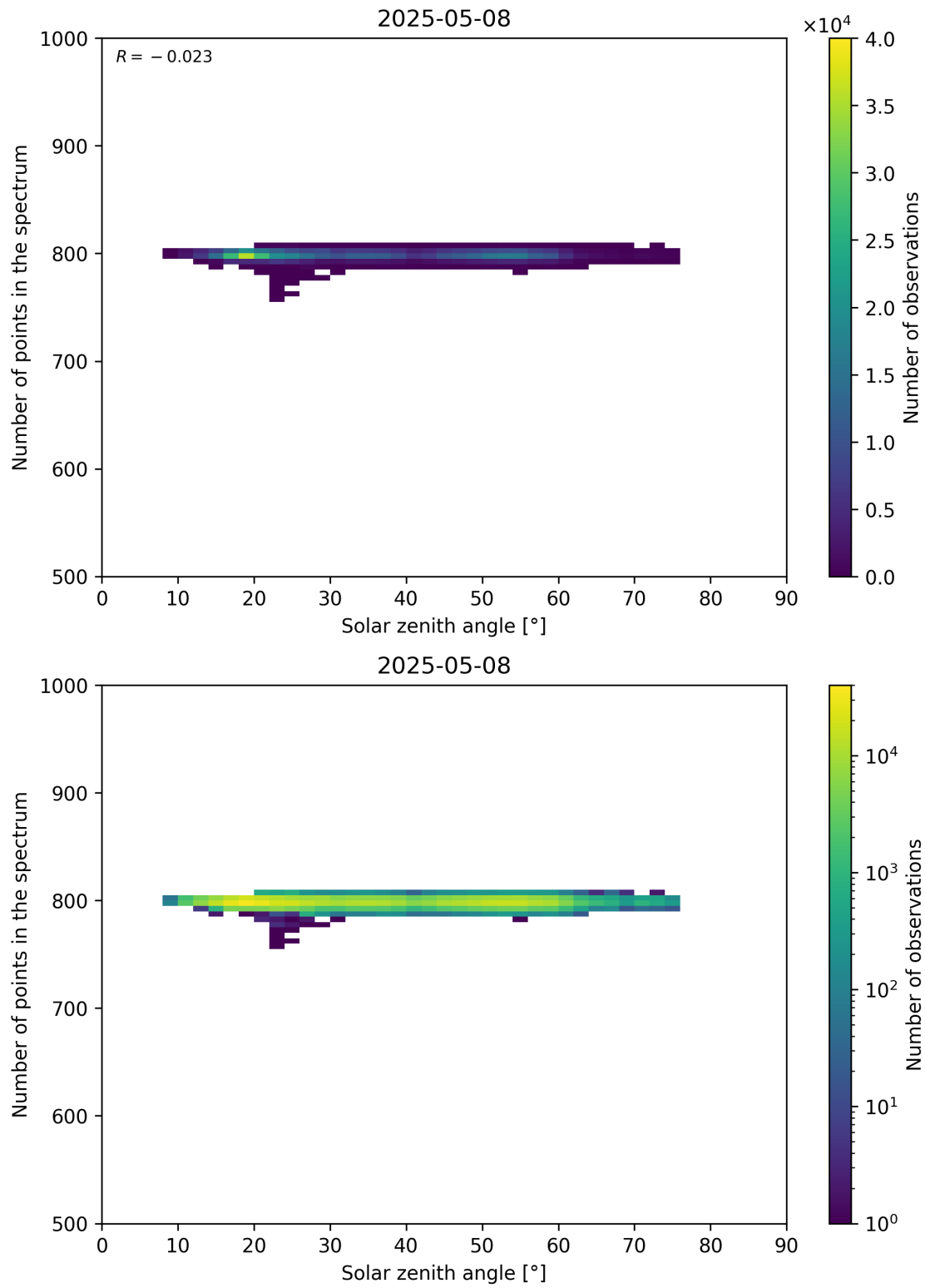
Figure 103: Scatter density plot of “Solar zenith angle” against “Number of points in the spectrum” for 2025-05-07 to 2025-05-09.
