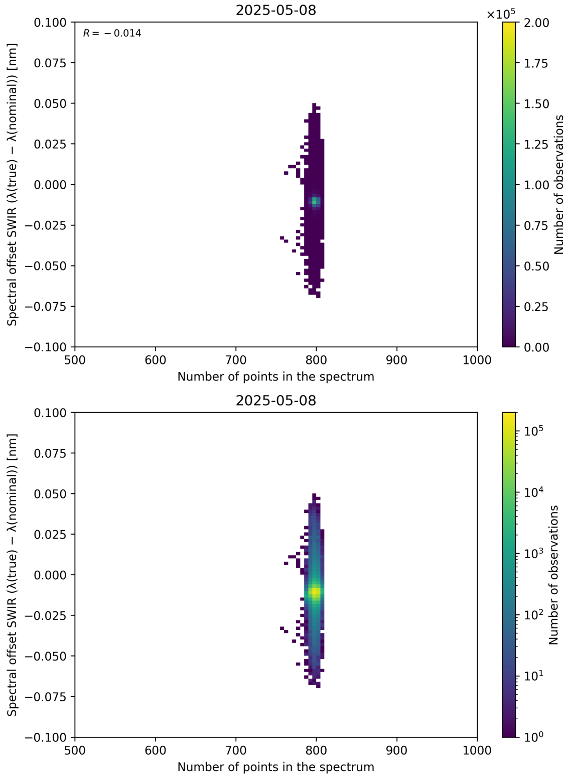
Figure 93: Scatter density plot of “Number of points in the spectrum” against “Spectral offset SWIR ( \lambda_{\text{true}} - \lambda_{\text{nominal}} )” for 2025-05-07 to 2025-05-09.
