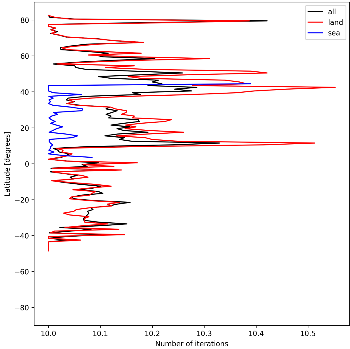
Figure 20: Zonal average of “Number of iterations” for 2025-05-07 to 2025-05-09.
