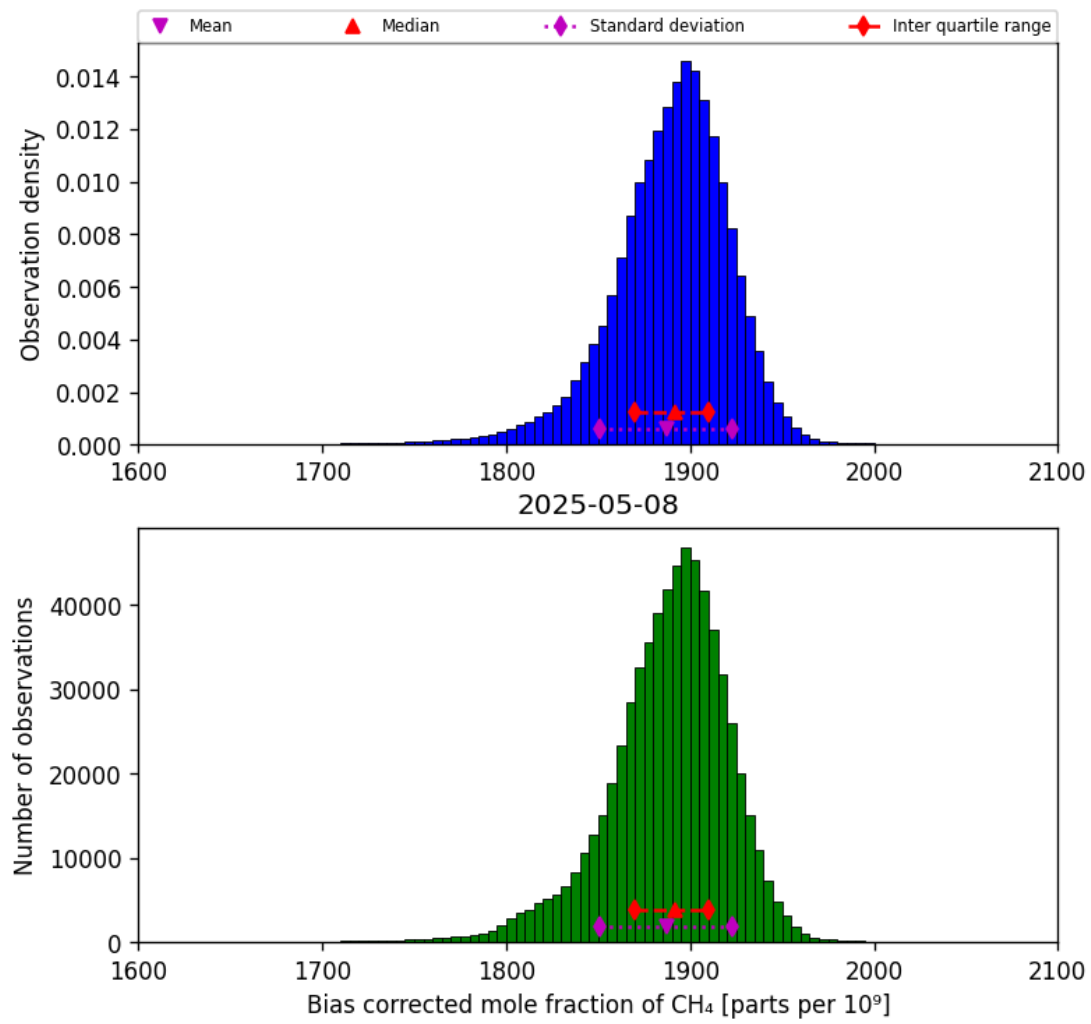
Figure 25: Histogram of “Bias corrected mole fraction of CH 4 ” for 2025-05-07 to 2025-05-09
