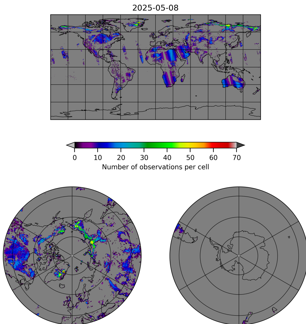
Figure 10: Map of the number of observations for 2025-05-07 to 2025-05-09
