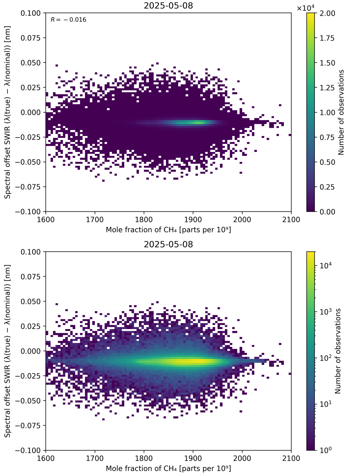
Figure 86: Scatter density plot of “Mole fraction of CH 4 ” against “Spectral offset SWIR ( \lambda_{\text{true}} - \lambda_{\text{nominal}} )” for 2025-05-07 to 2025-05-09.
