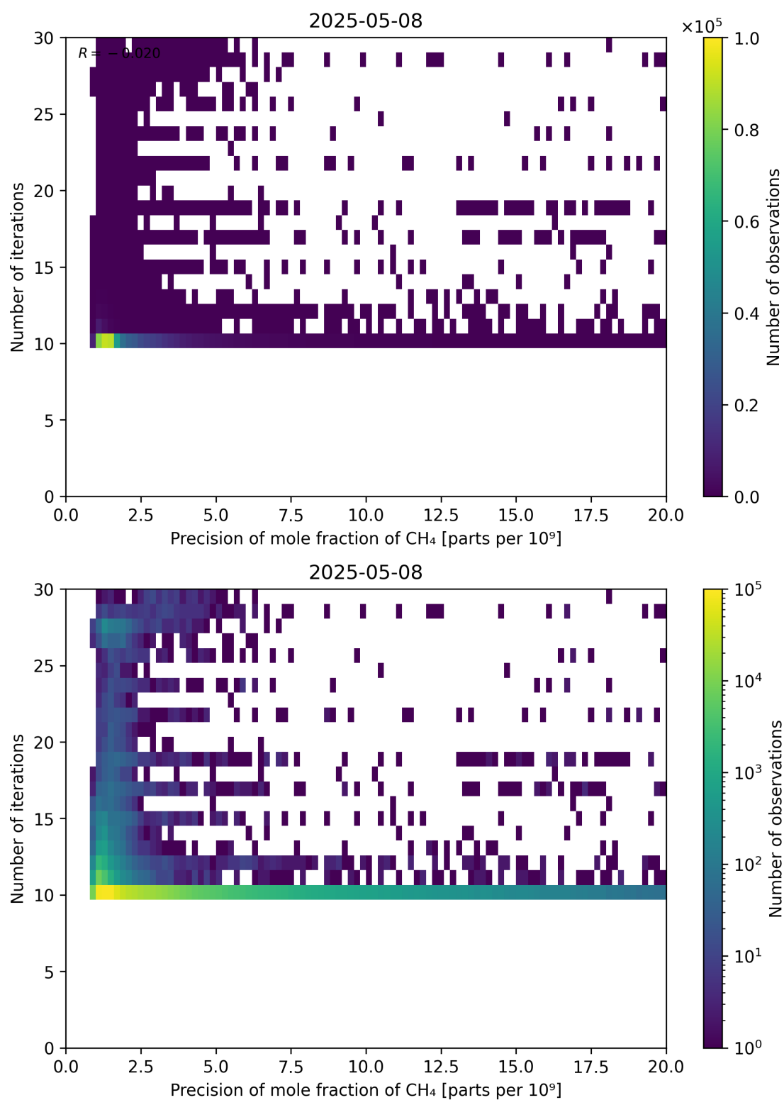
Figure 83: Scatter density plot of “Precision of mole fraction of CH 4 ” against “Number of iterations” for 2025-05-07 to 2025-05-09.
