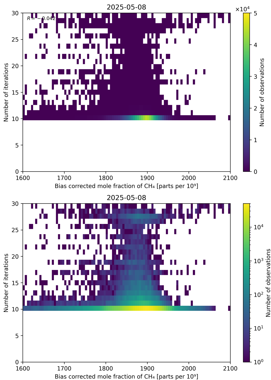
Figure 67: Scatter density plot of “Bias corrected mole fraction of \text{CH}_4 ” against “Number of iterations” for 2025-05-07 to 2025-05-09.
