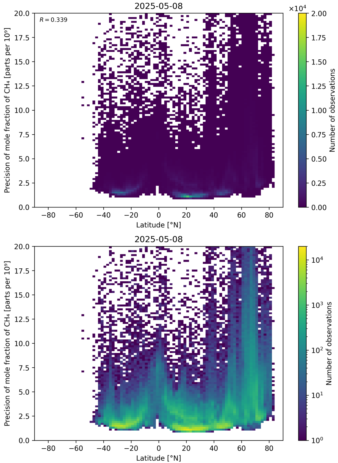
Figure 59: Scatter density plot of “Latitude” against “Precision of mole fraction of \text{CH}_4 ” for 2025-05-07 to 2025-05-09.
