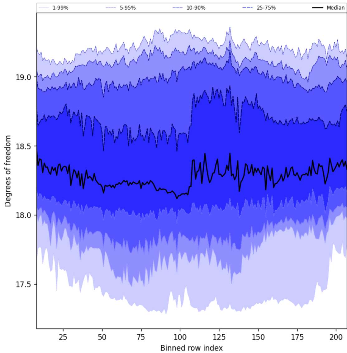
Figure 41: Along track statistics of “Degrees of freedom” for 2025-05-07 to 2025-05-09
