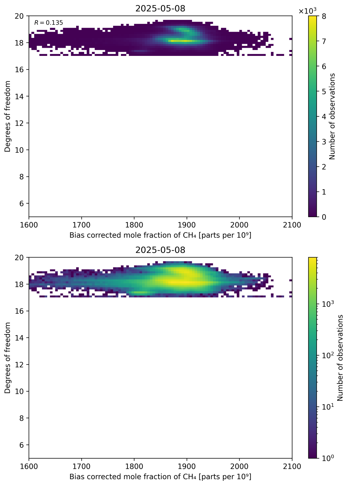
Figure 65: Scatter density plot of “Bias corrected mole fraction of CH 4 ” against “Degrees of freedom” for 2025-05-07 to 2025-05-09.
