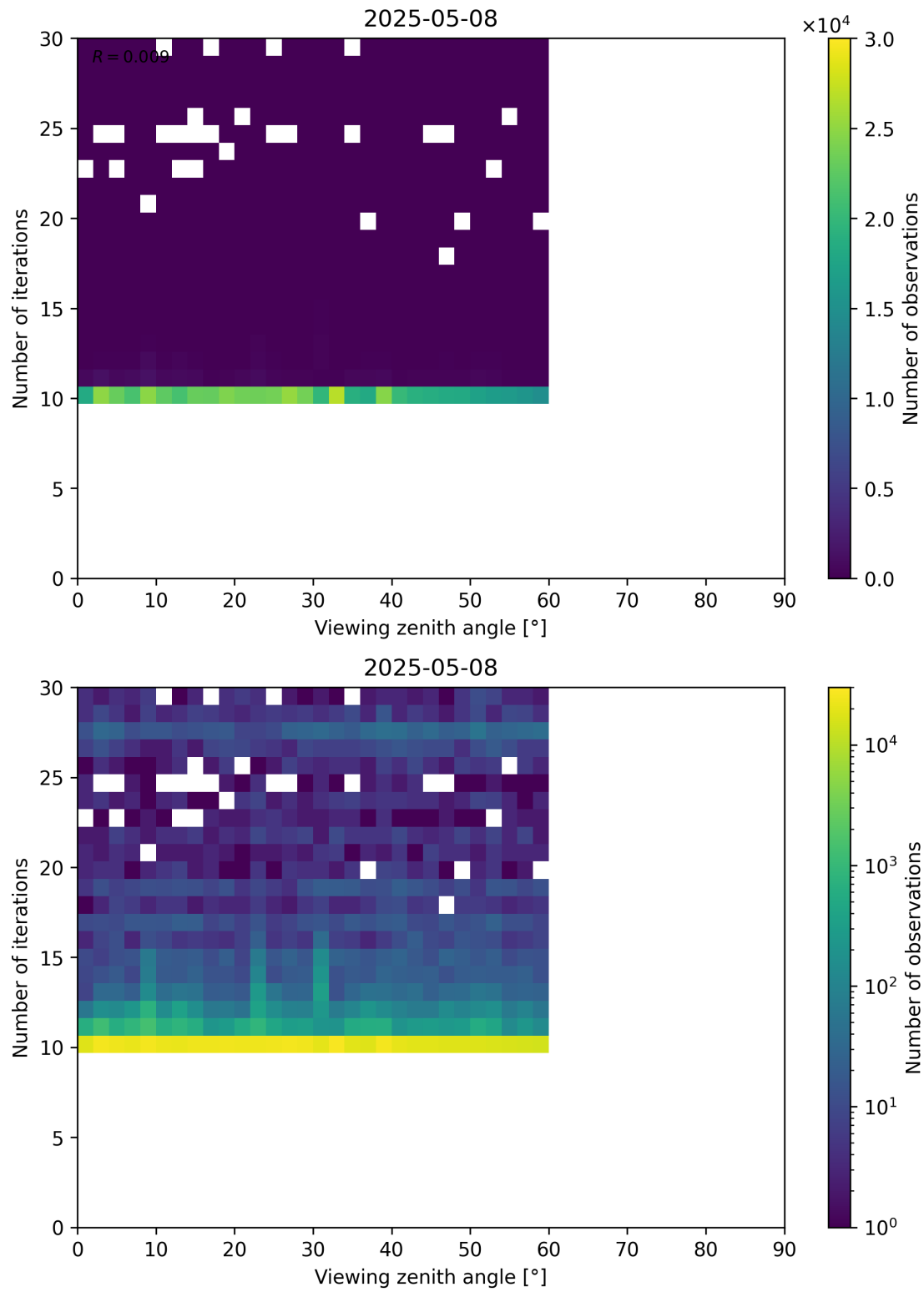
Figure 113: Scatter density plot of “Viewing zenith angle” against “Number of iterations” for 2025-05-07 to 2025-05-09.
