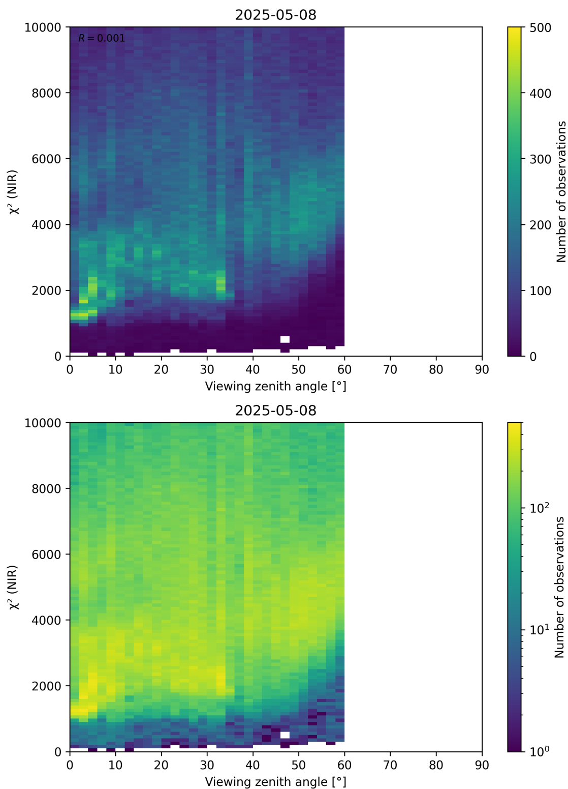
Figure 105: Scatter density plot of “Viewing zenith angle” against “ \chi^2 (NIR)” for 2025-05-07 to 2025-05-09.
