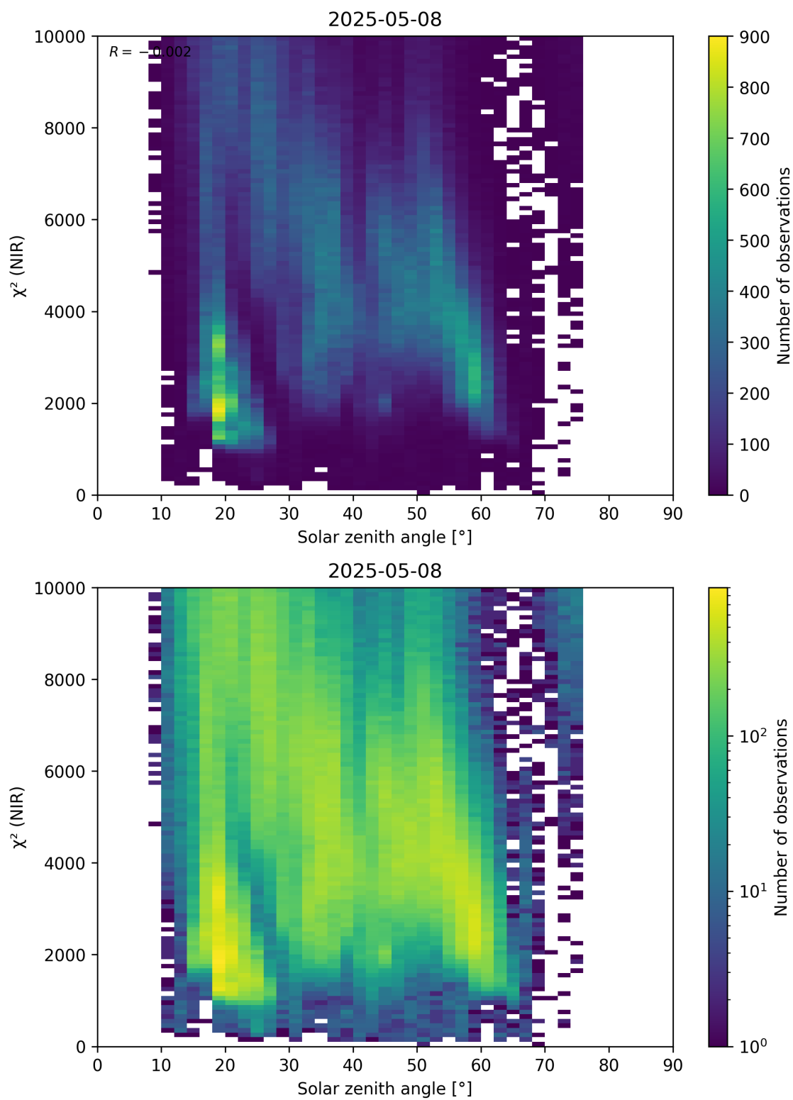
Figure 94: Scatter density plot of “Solar zenith angle” against “ \chi^2 (NIR)” for 2025-05-07 to 2025-05-09.
