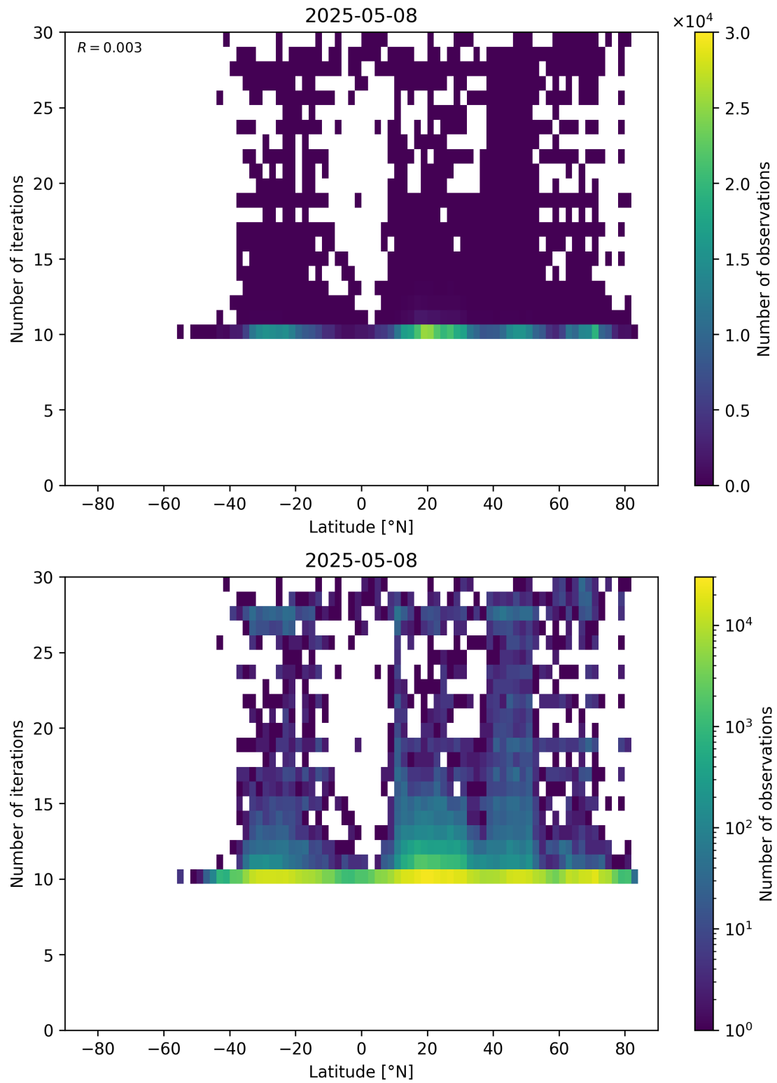
Figure 60: Scatter density plot of “Latitude” against “Number of iterations” for 2025-05-07 to 2025-05-09.
