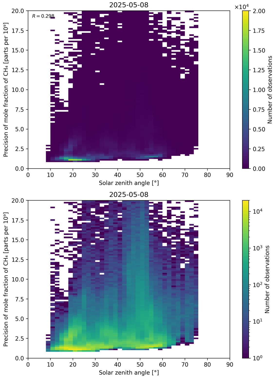
Figure 101: Scatter density plot of “Solar zenith angle” against “Precision of mole fraction of CH 4 ” for 2025-05-07 to 2025-05-09.
