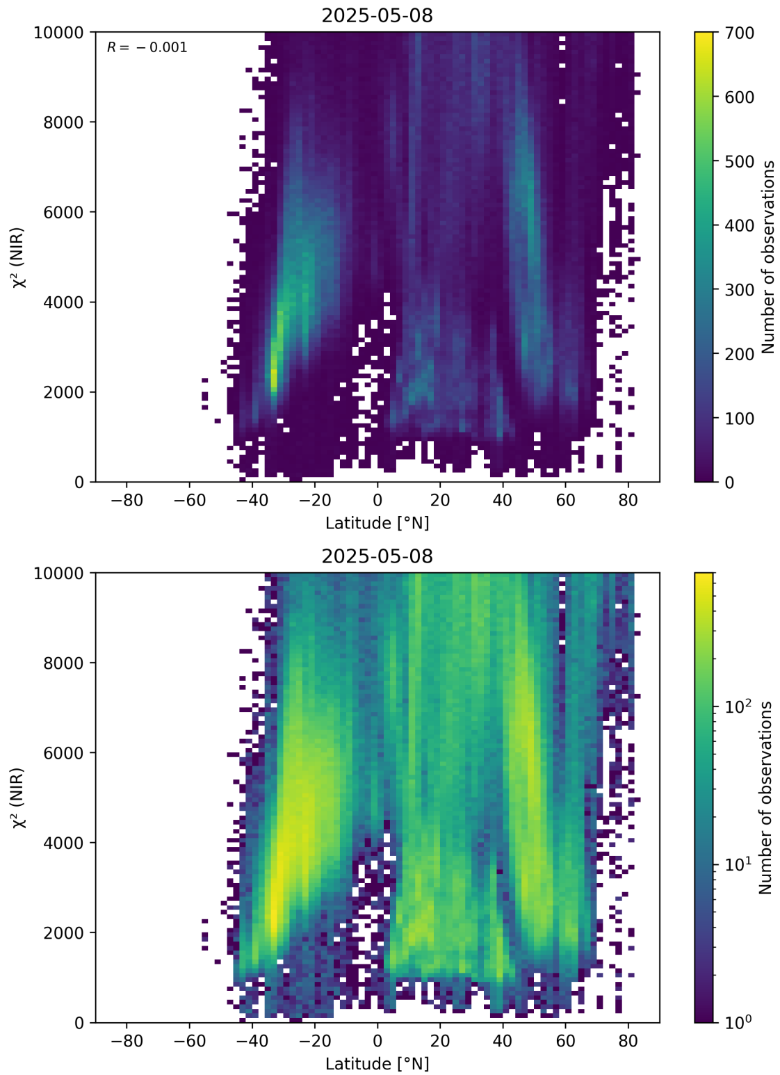
Figure 53: Scatter density plot of “Latitude” against “ \chi^2 (NIR)” for 2025-05-07 to 2025-05-09.
