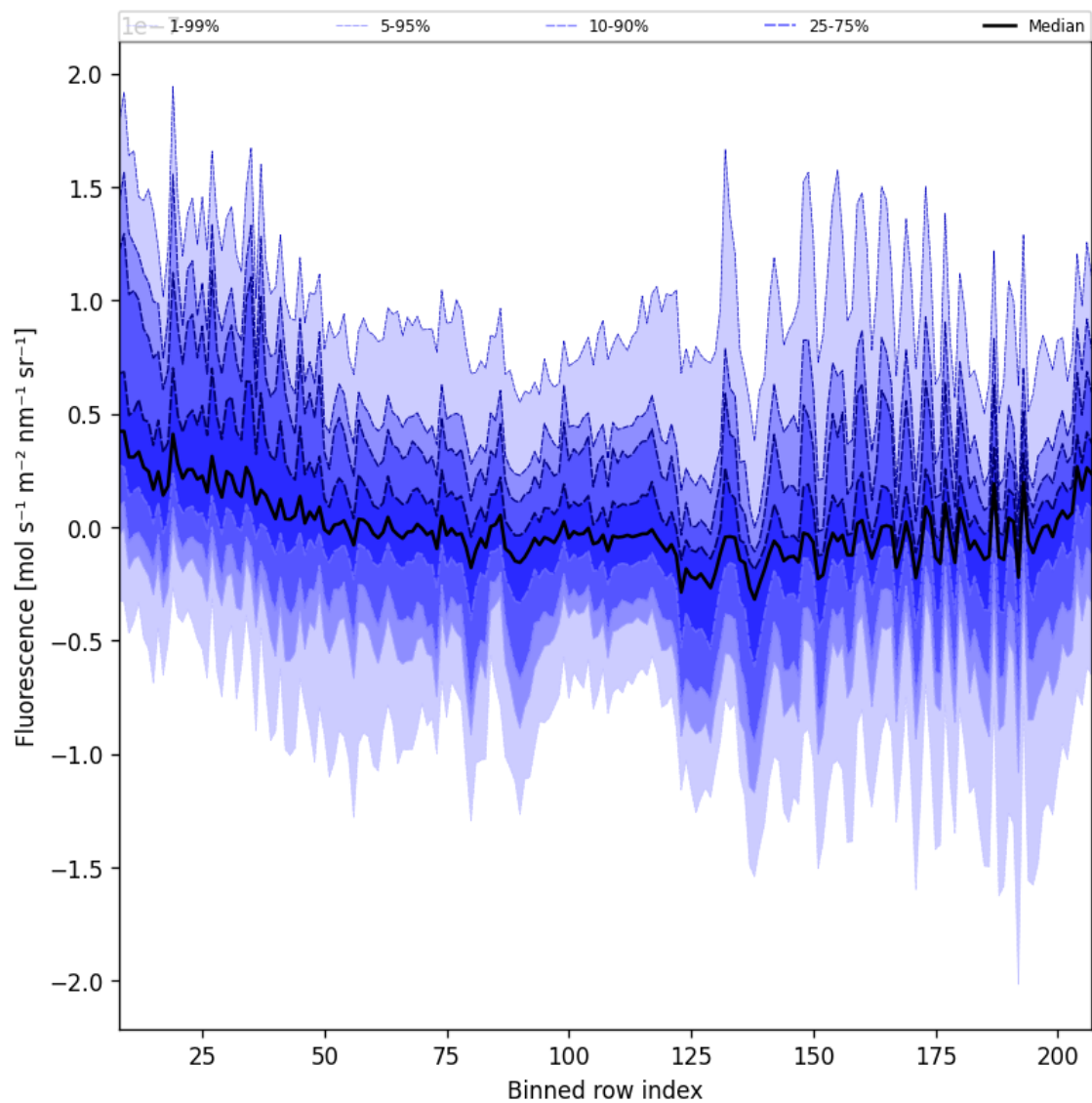
Figure 43: Along track statistics of "Fluorescence" for 2025-05-07 to 2025-05-09
