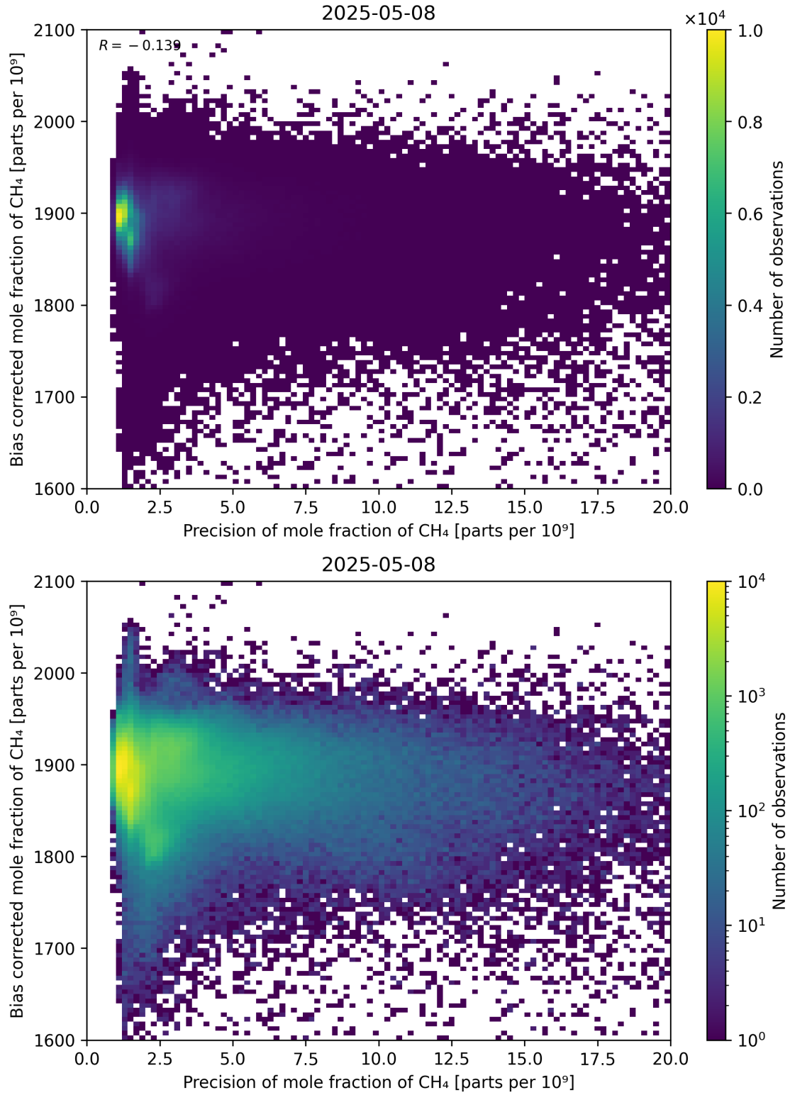
Figure 82: Scatter density plot of “Precision of mole fraction of CH 4 ” against “Bias corrected mole fraction of CH 4 ” for 2025-05-07 to 2025-05-09.
