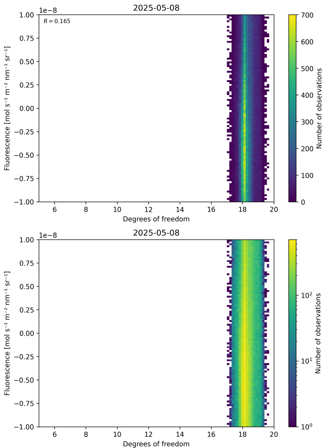
Figure 51: Scatter density plot of “Degrees of freedom” against “Fluorescence” for 2025-05-07 to 2025-05-09.
