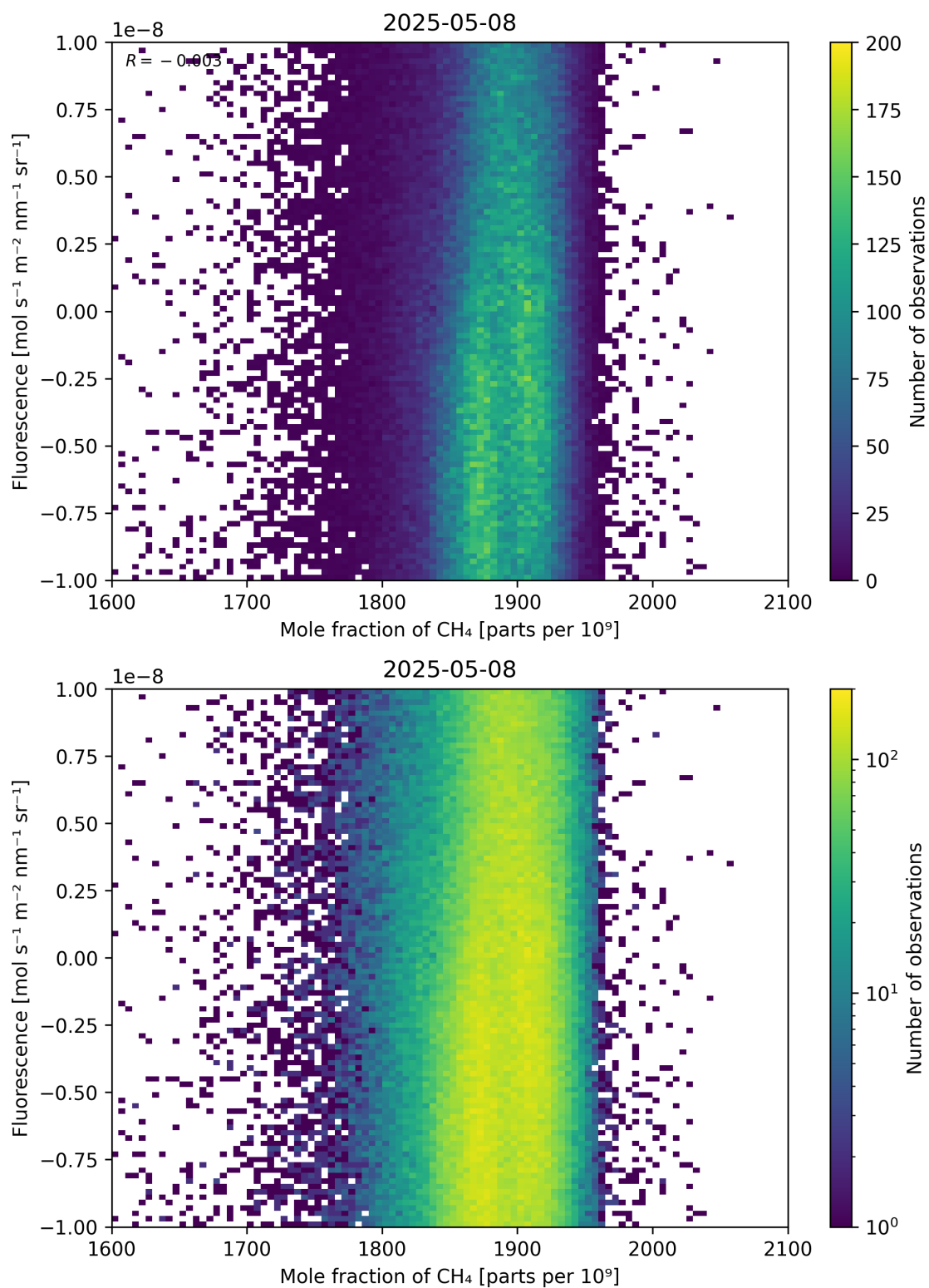
Figure 73: Scatter density plot of “Mole fraction of CH 4 ” against “Fluorescence” for 2025-05-07 to 2025-05-09.
