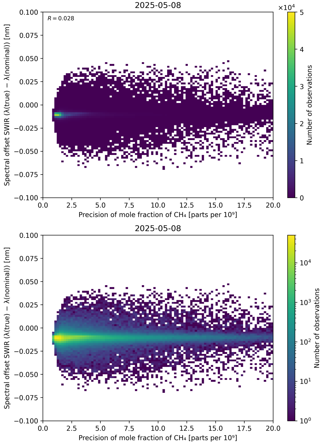
Figure 85: Scatter density plot of “Precision of mole fraction of CH 4 ” against “Spectral offset SWIR ( \lambda_{\text{true}} - \lambda_{\text{nominal}} )” for 2025-05-07 to 2025-05-09.
