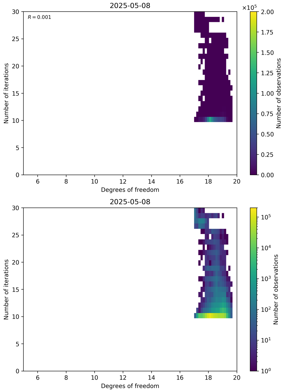
Figure 52: Scatter density plot of “Degrees of freedom” against “Number of iterations” for 2025-05-07 to 2025-05-09.
