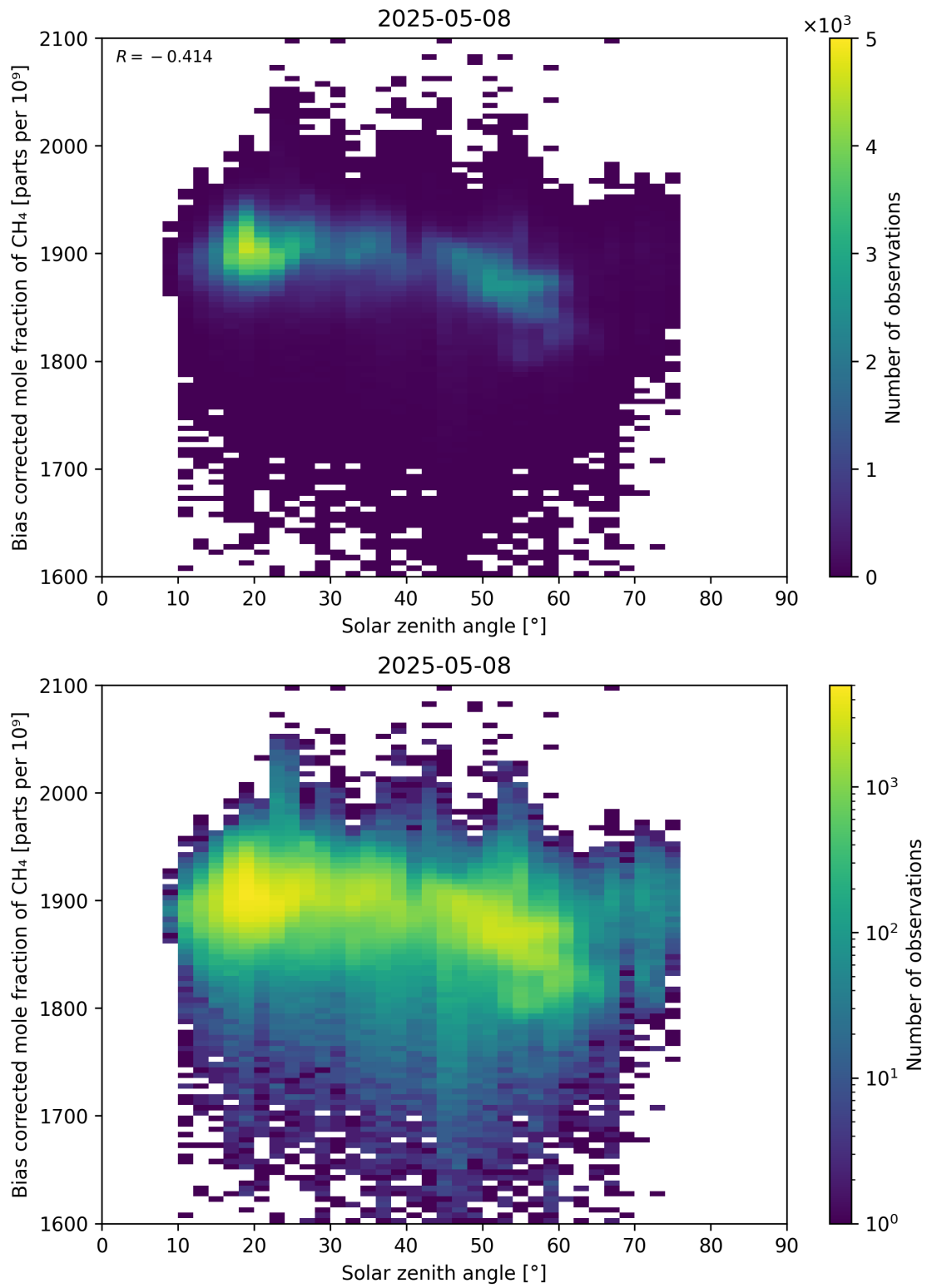
Figure 100: Scatter density plot of “Solar zenith angle” against “Bias corrected mole fraction of \text{CH}_4 ” for 2025-05-07 to 2025-05-09.
