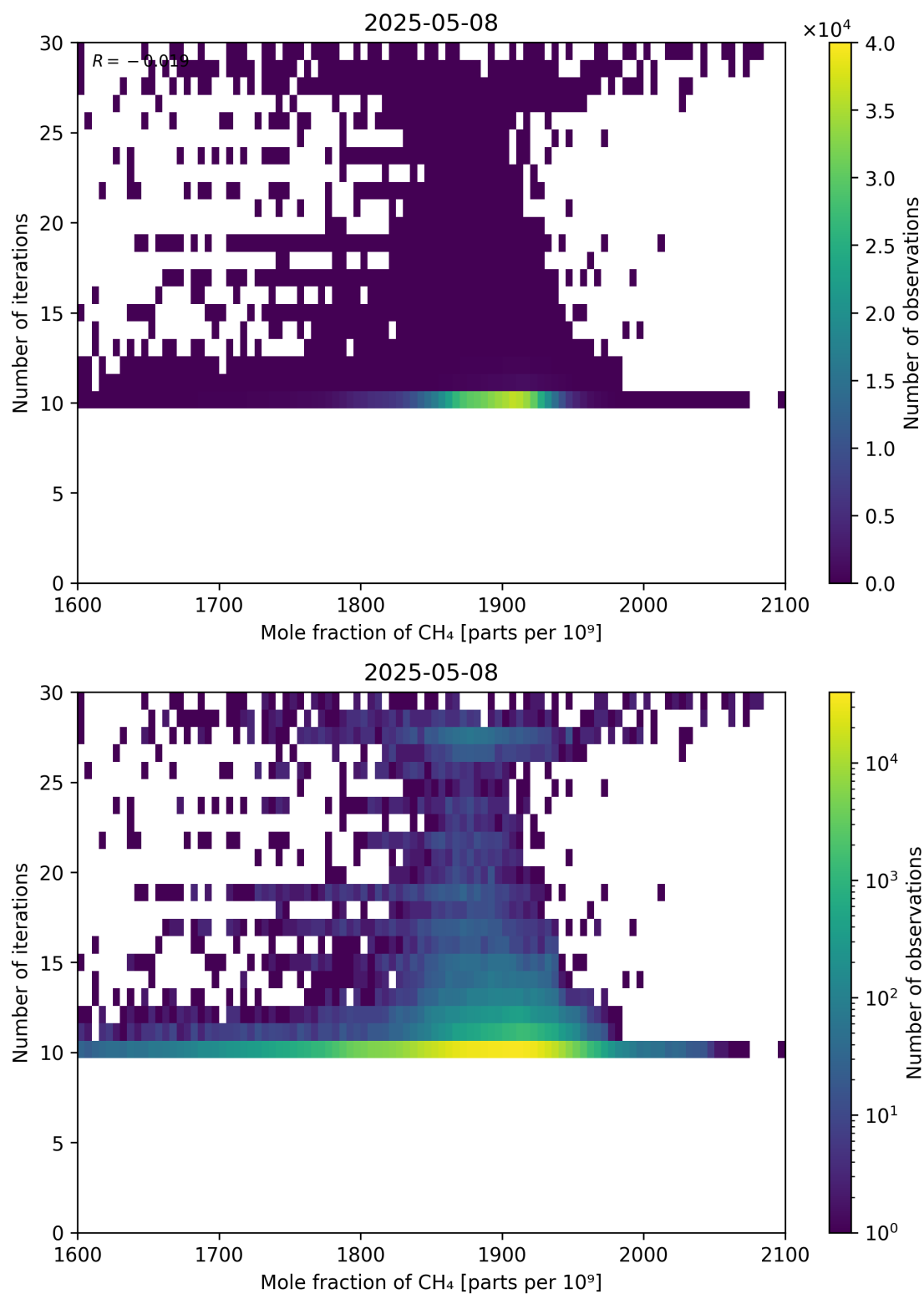
Figure 76: Scatter density plot of “Mole fraction of CH 4 ” against “Number of iterations” for 2025-05-07 to 2025-05-09.
