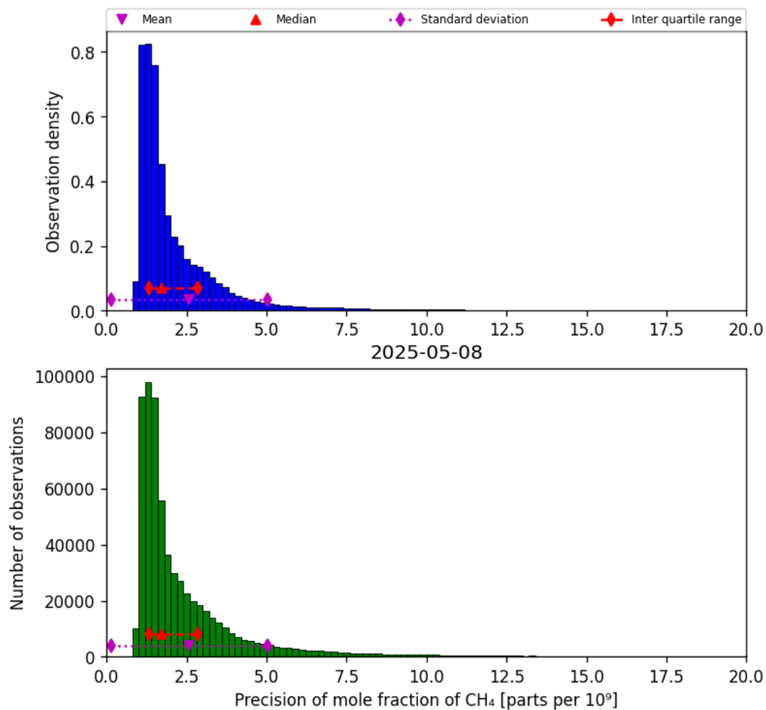
Figure 24: Histogram of “Precision of mole fraction of CH 4 ” for 2025-05-07 to 2025-05-09
