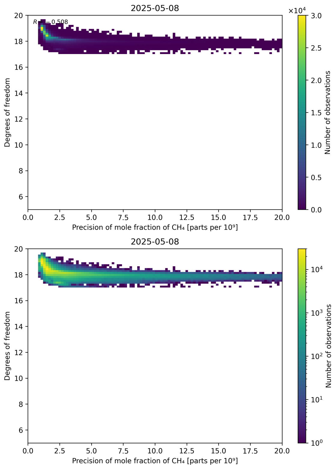
Figure 80: Scatter density plot of “Precision of mole fraction of CH 4 ” against “Degrees of freedom” for 2025-05-07 to 2025-05-09.
