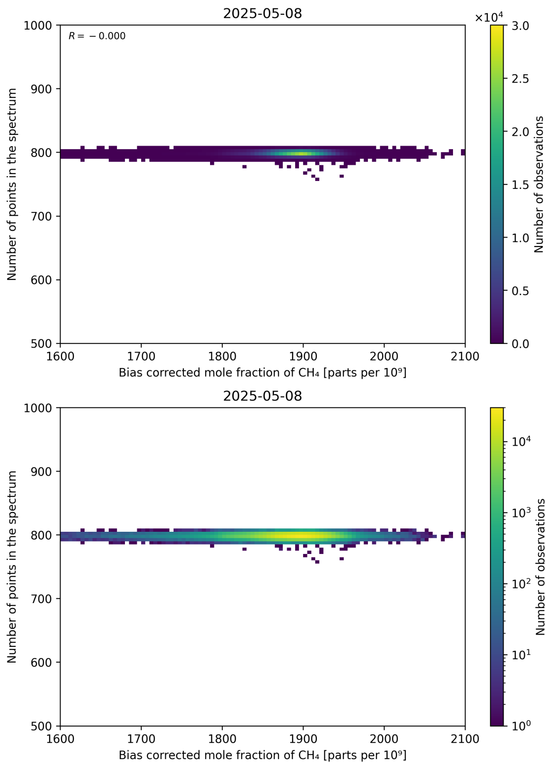
Figure 68: Scatter density plot of “Bias corrected mole fraction of CH 4 ” against “Number of points in the spectrum” for 2025-05-07 to 2025-05-09.
