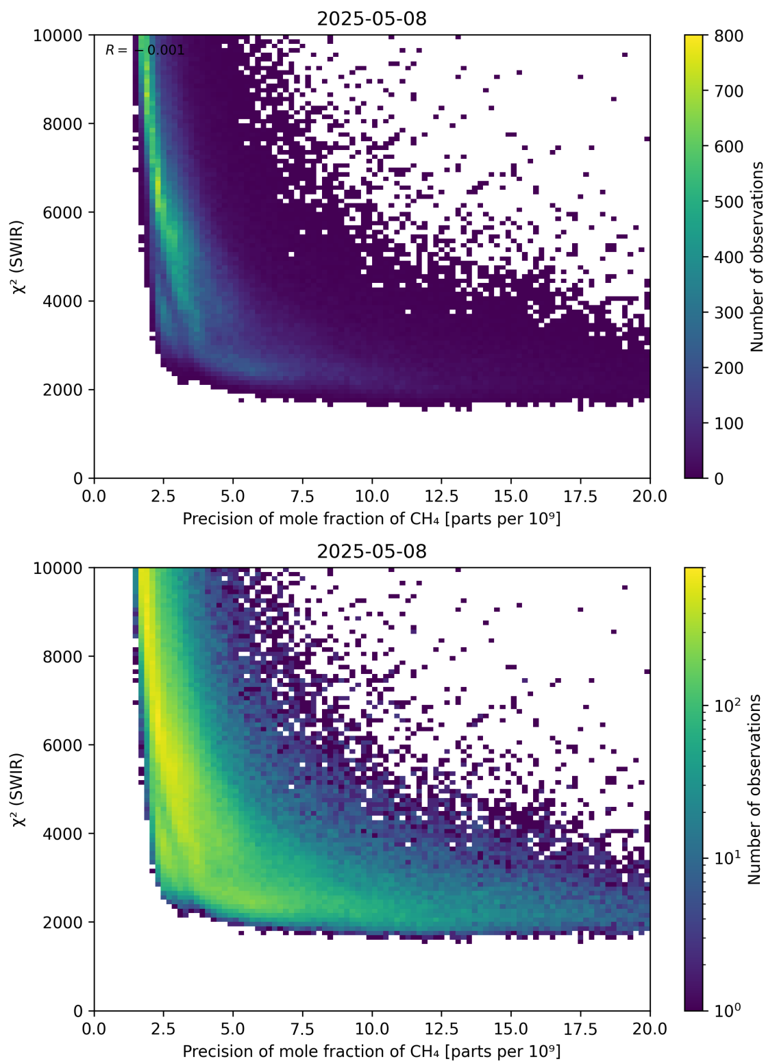
Figure 79: Scatter density plot of “Precision of mole fraction of \text{CH}_4 ” against “ \chi^2 (SWIR)” for 2025-05-07 to 2025-05-09.
