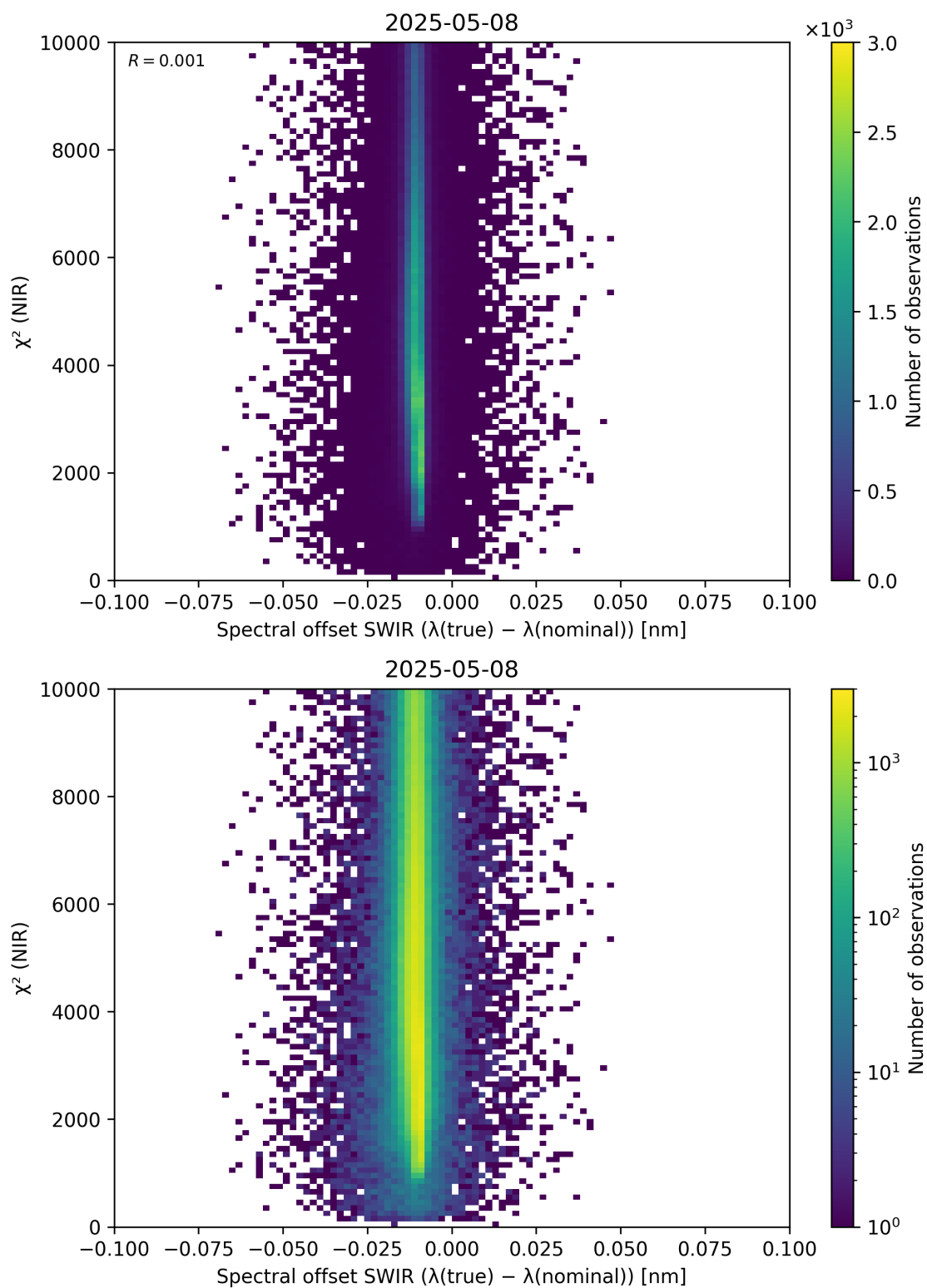
Figure 117: Scatter density plot of “Spectral offset SWIR ( \lambda_{\text{true}} - \lambda_{\text{nominal}} )” against “ \chi^2 (NIR)” for 2025-05-07 to 2025-05-09.
