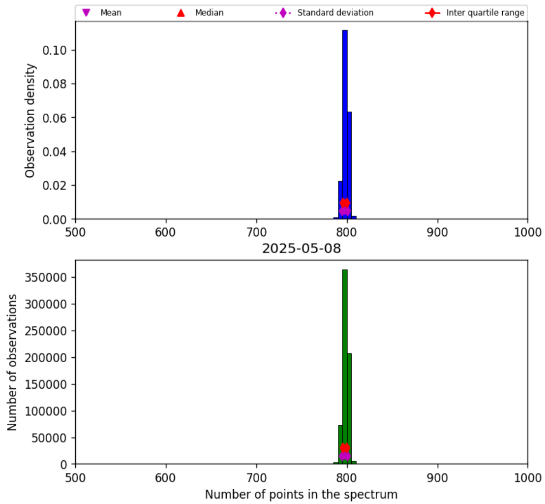
Figure 26: Histogram of “Number of points in the spectrum” for 2025-05-07 to 2025-05-09
