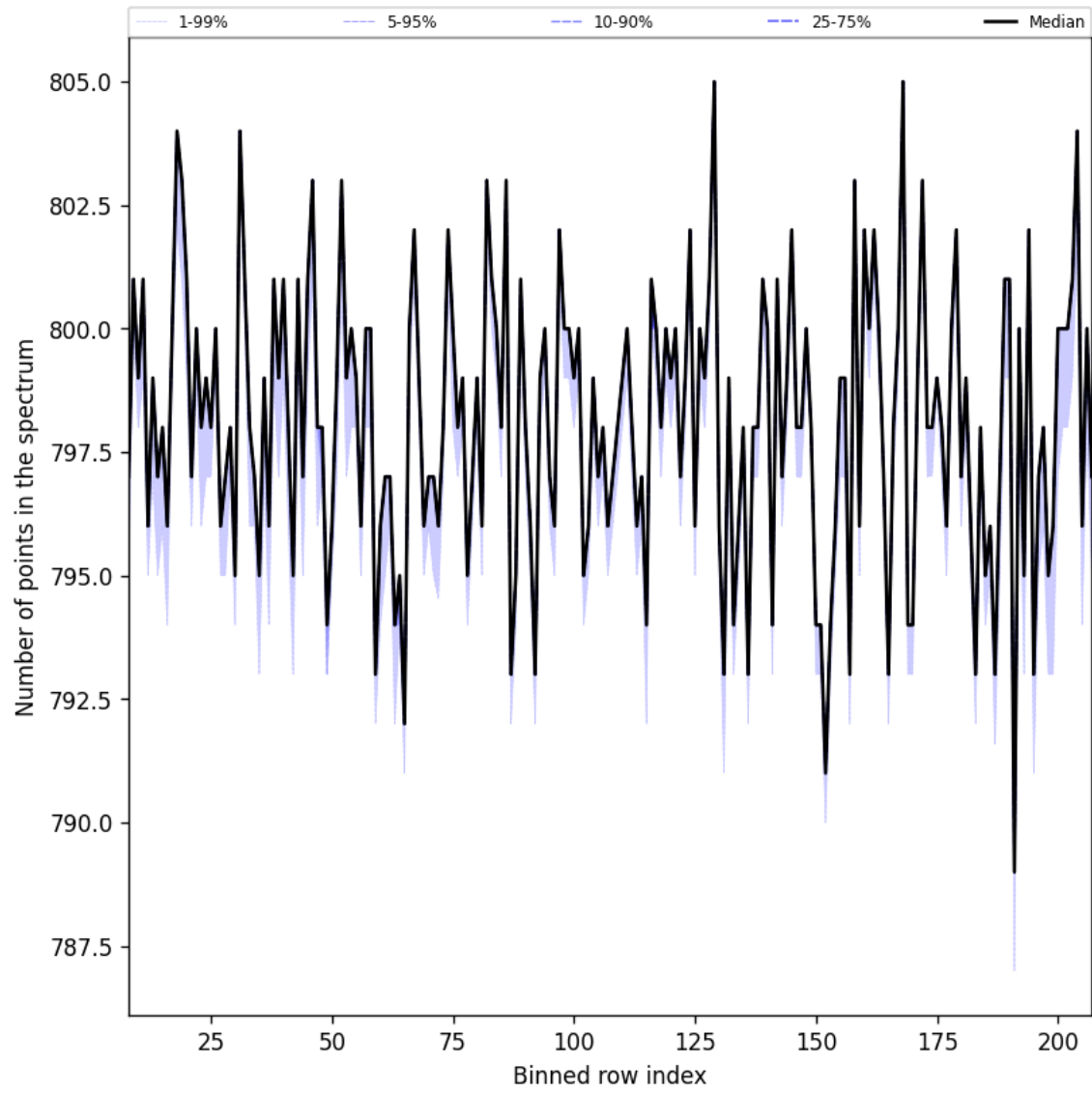
Figure 37: Along track statistics of “Number of points in the spectrum” for 2025-05-07 to 2025-05-09
