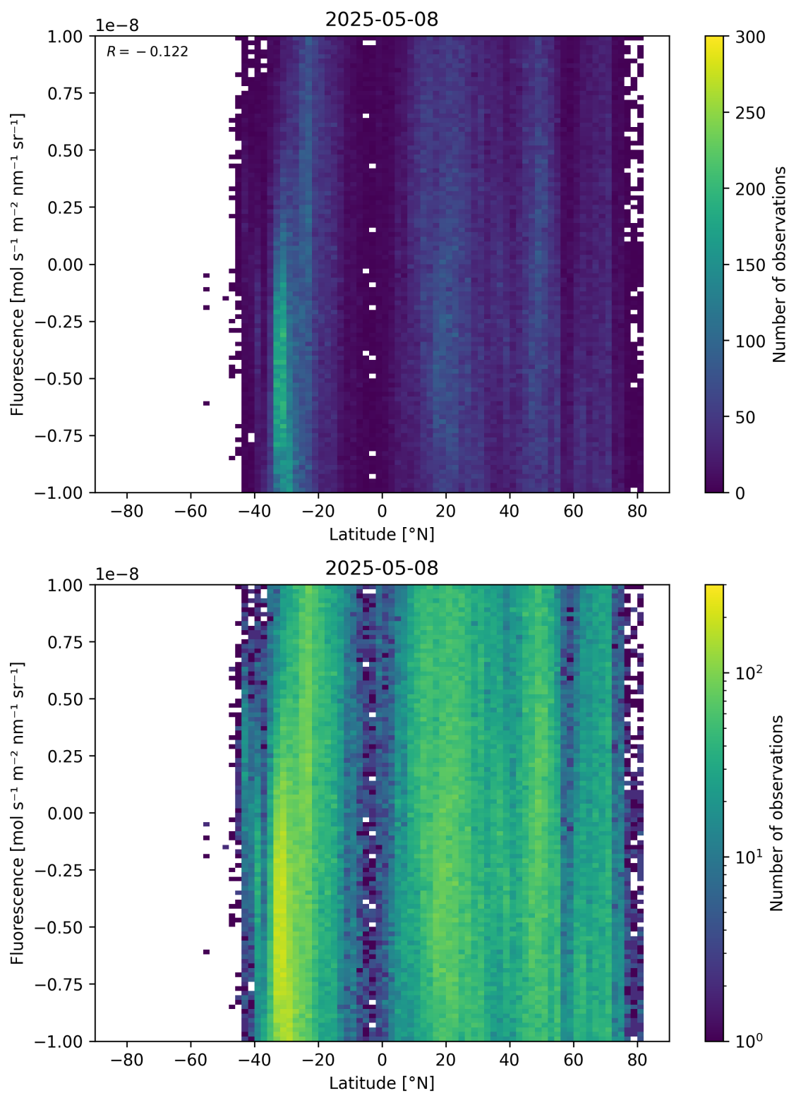
Figure 56: Scatter density plot of “Latitude” against “Fluorescence” for 2025-05-07 to 2025-05-09.
