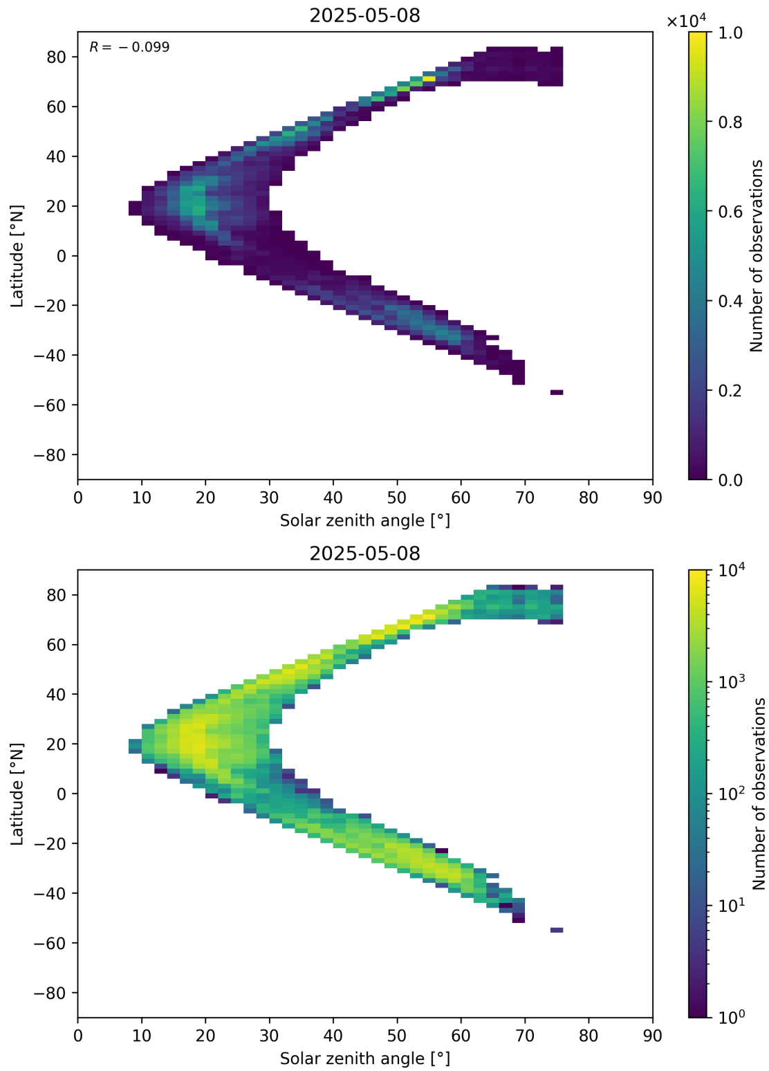
Figure 98: Scatter density plot of “Solar zenith angle” against “Latitude” for 2025-05-07 to 2025-05-09.
