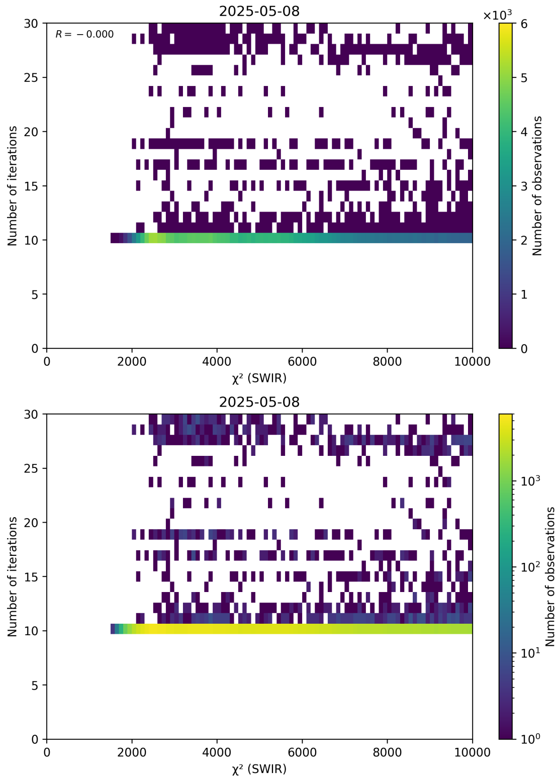
Figure 50: Scatter density plot of “ \chi^2 (SWIR)” against “Number of iterations” for 2025-05-07 to 2025-05-09.
