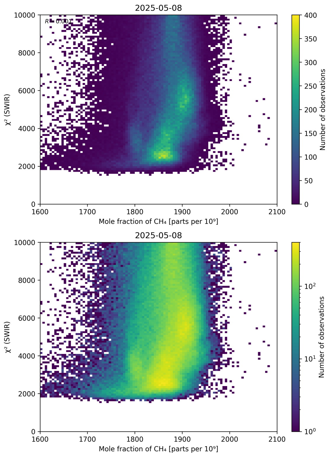
Figure 71: Scatter density plot of “Mole fraction of \text{CH}_4 ” against “ \chi^2 (SWIR)” for 2025-05-07 to 2025-05-09.
