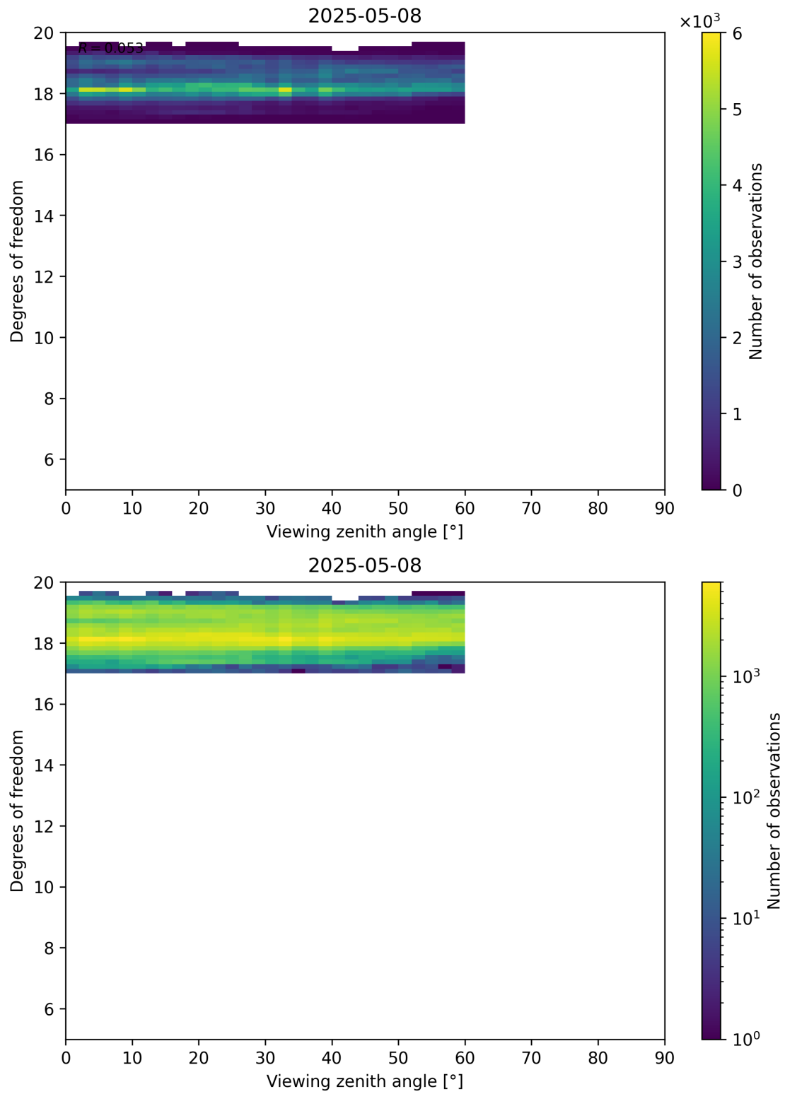
Figure 107: Scatter density plot of “Viewing zenith angle” against “Degrees of freedom” for 2025-05-07 to 2025-05-09.
