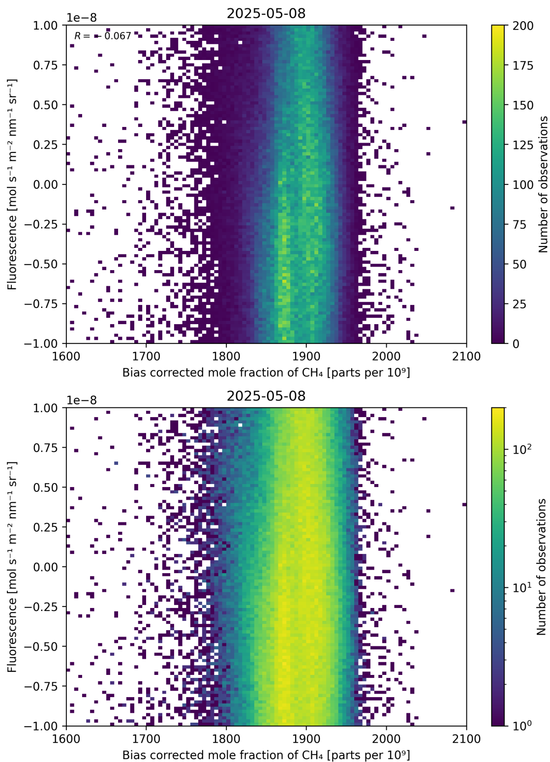
Figure 66: Scatter density plot of “Bias corrected mole fraction of \text{CH}_4 ” against “Fluorescence” for 2025-05-07 to 2025-05-09.
