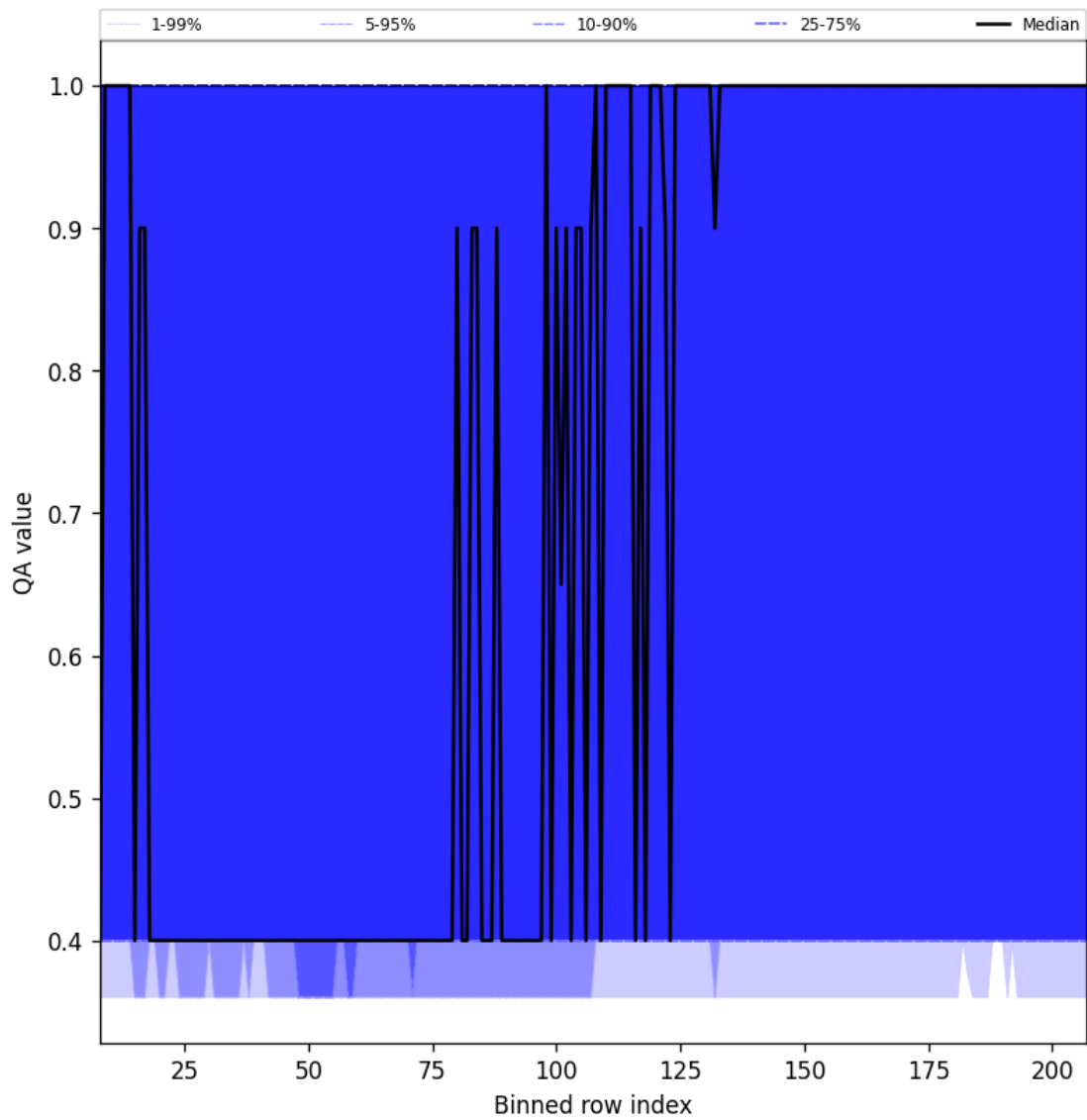
Figure 33: Along track statistics of “QA value” for 2025-05-07 to 2025-05-09
