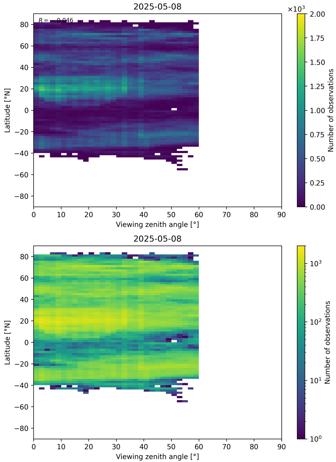
Figure 109: Scatter density plot of “Viewing zenith angle” against “Latitude” for 2025-05-07 to 2025-05-09.
