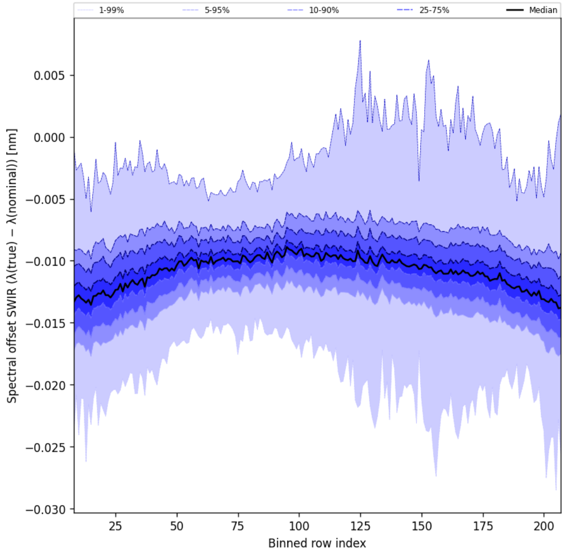
Figure 38: Along track statistics of “Spectral offset SWIR ( \lambda_{\text{true}} - \lambda_{\text{nominal}} )” for 2025-05-07 to 2025-05-09
