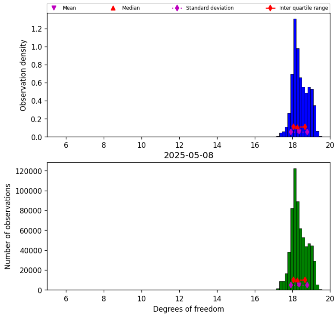
Figure 30: Histogram of “Degrees of freedom” for 2025-05-07 to 2025-05-09
