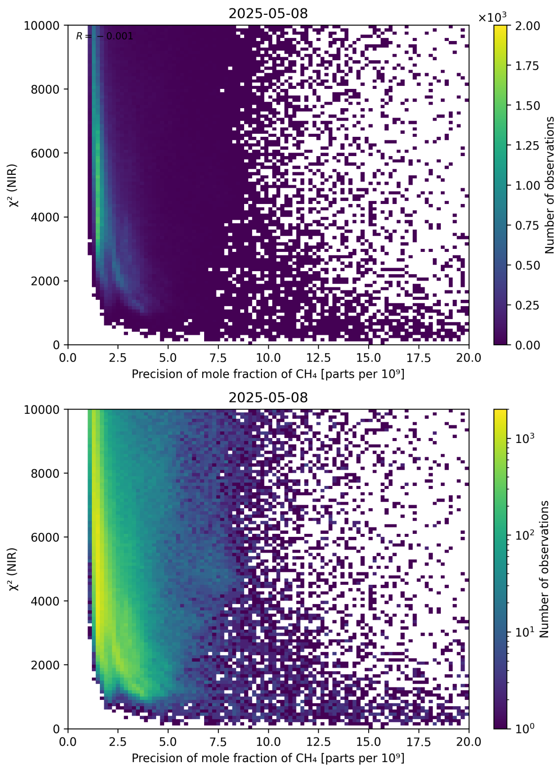
Figure 78: Scatter density plot of “Precision of mole fraction of CH 4 ” against “ \chi^2 (NIR)” for 2025-05-07 to 2025-05-09.
