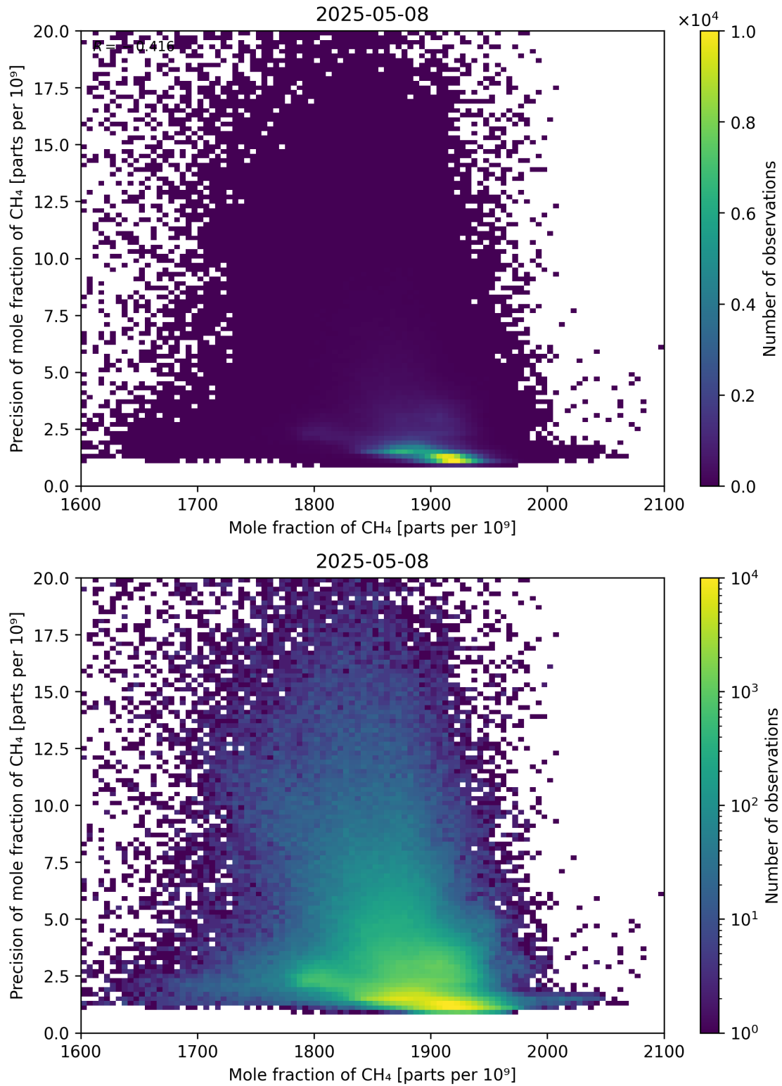
Figure 75: Scatter density plot of “Mole fraction of CH 4 ” against “Precision of mole fraction of CH 4 ” for 2025-05-07 to 2025-05-09.
