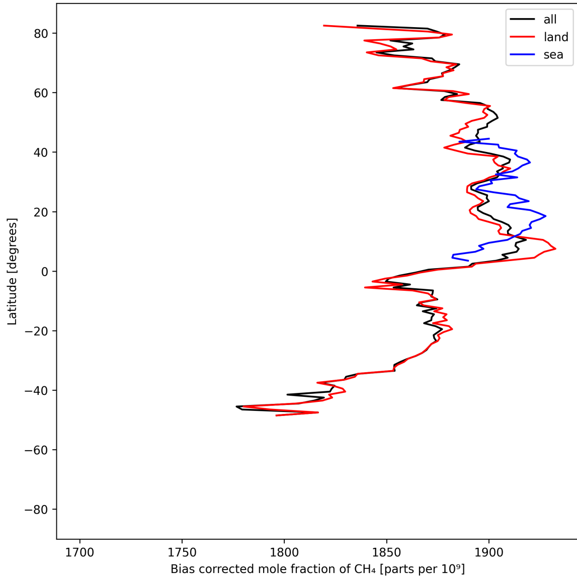
Figure 14: Zonal average of “Bias corrected mole fraction of CH 4 ” for 2025-05-07 to 2025-05-09.
