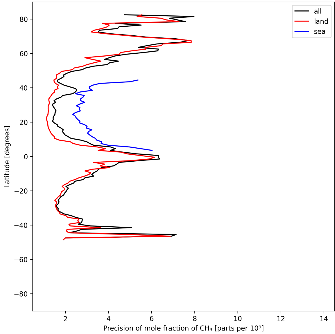
Figure 13: Zonal average of “Precision of mole fraction of CH 4 ” for 2025-05-07 to 2025-05-09.
