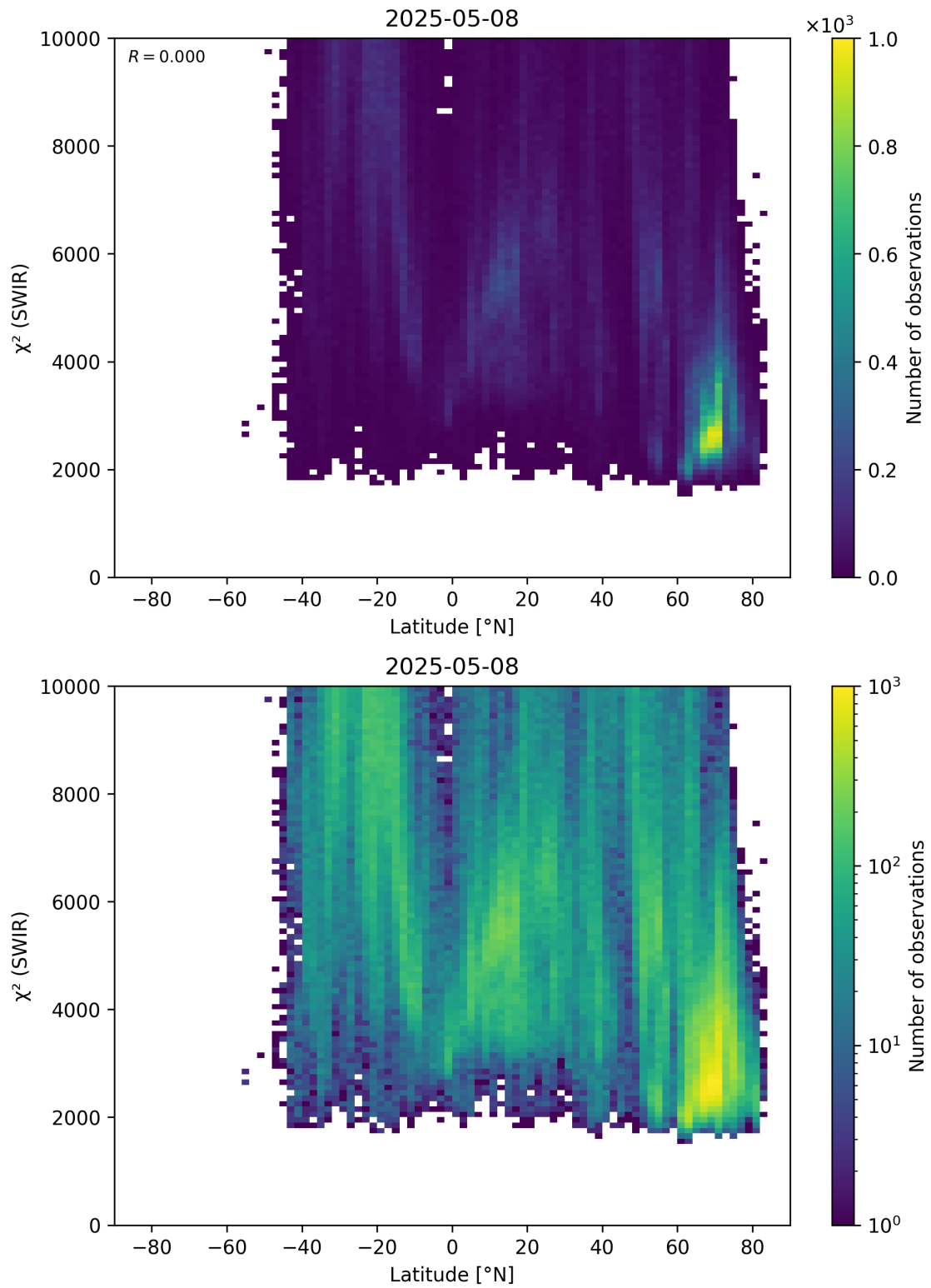
Figure 54: Scatter density plot of “Latitude” against “ \chi^2 (SWIR)” for 2025-05-07 to 2025-05-09.
