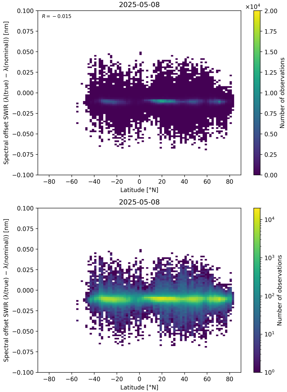
Figure 62: Scatter density plot of “Latitude” against “Spectral offset SWIR ( \lambda_{\text{true}} - \lambda_{\text{nominal}} )” for 2025-05-07 to 2025-05-09.
