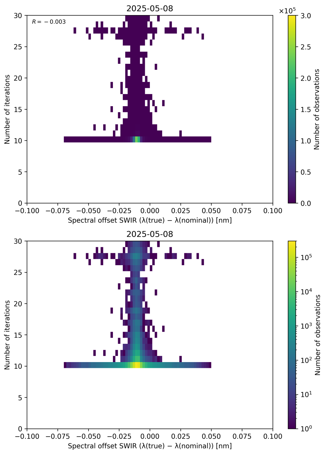
Figure 121: Scatter density plot of “Spectral offset SWIR ( \lambda_{\text{true}} - \lambda_{\text{nominal}} )” against “Number of iterations” for 2025-05-07 to 2025-05-09.
