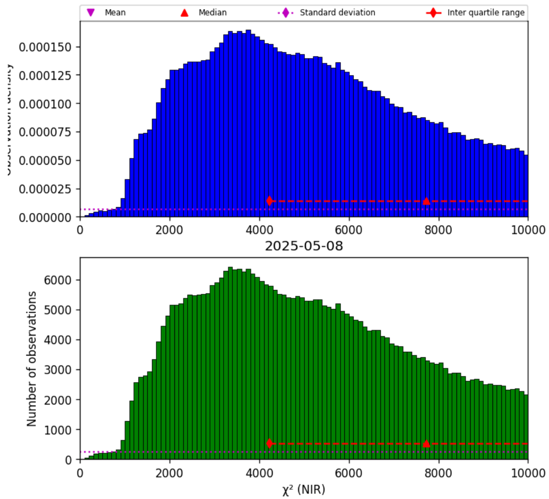
Figure 29: Histogram of “ \chi^2 (NIR)” for 2025-05-07 to 2025-05-09
