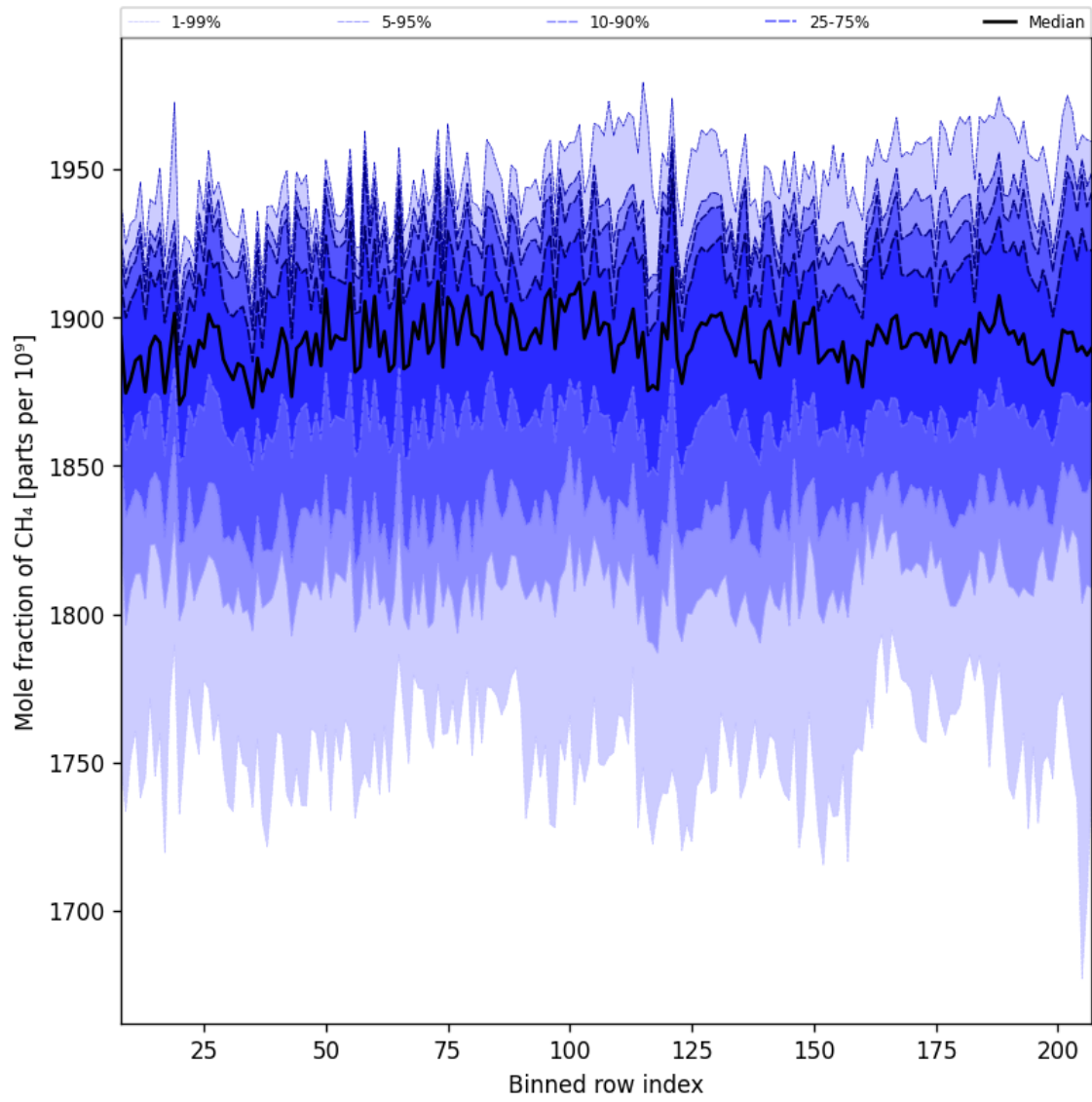
Figure 34: Along track statistics of “Mole fraction of CH 4 ” for 2025-05-07 to 2025-05-09
