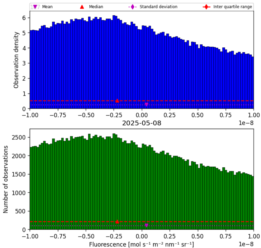
Figure 32: Histogram of “Fluorescence” for 2025-05-07 to 2025-05-09
