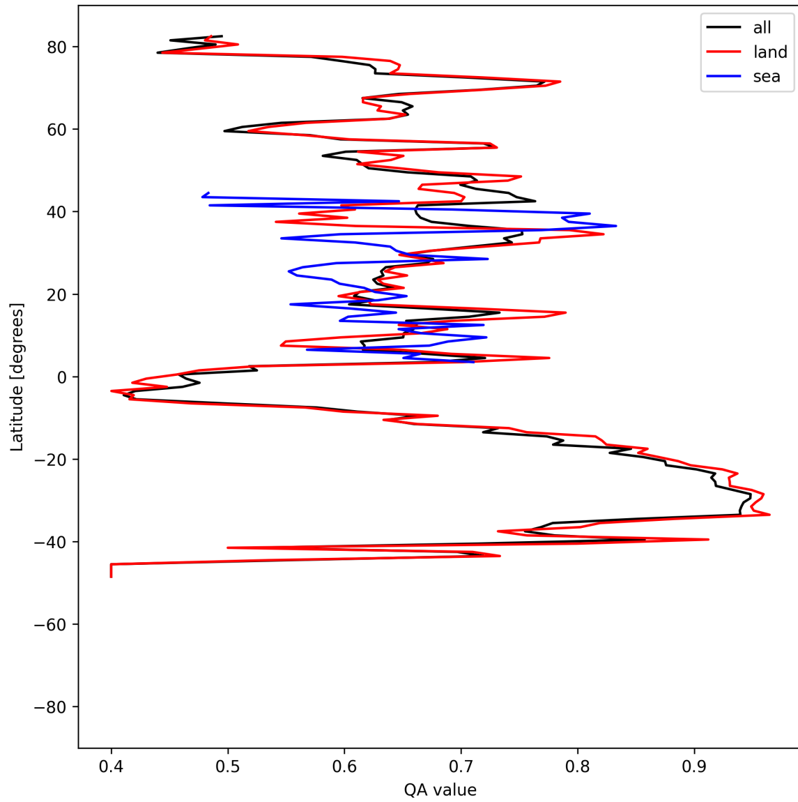
Figure 11: Zonal average of “QA value” for 2025-05-07 to 2025-05-09.
