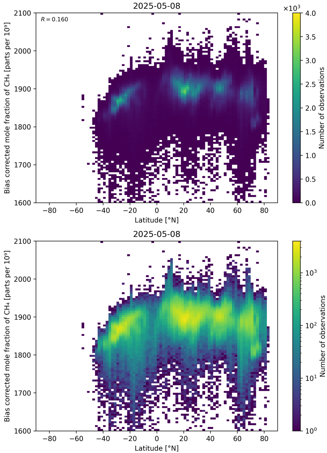
Figure 58: Scatter density plot of “Latitude” against “Bias corrected mole fraction of CH 4 ” for 2025-05-07 to 2025-05-09.
