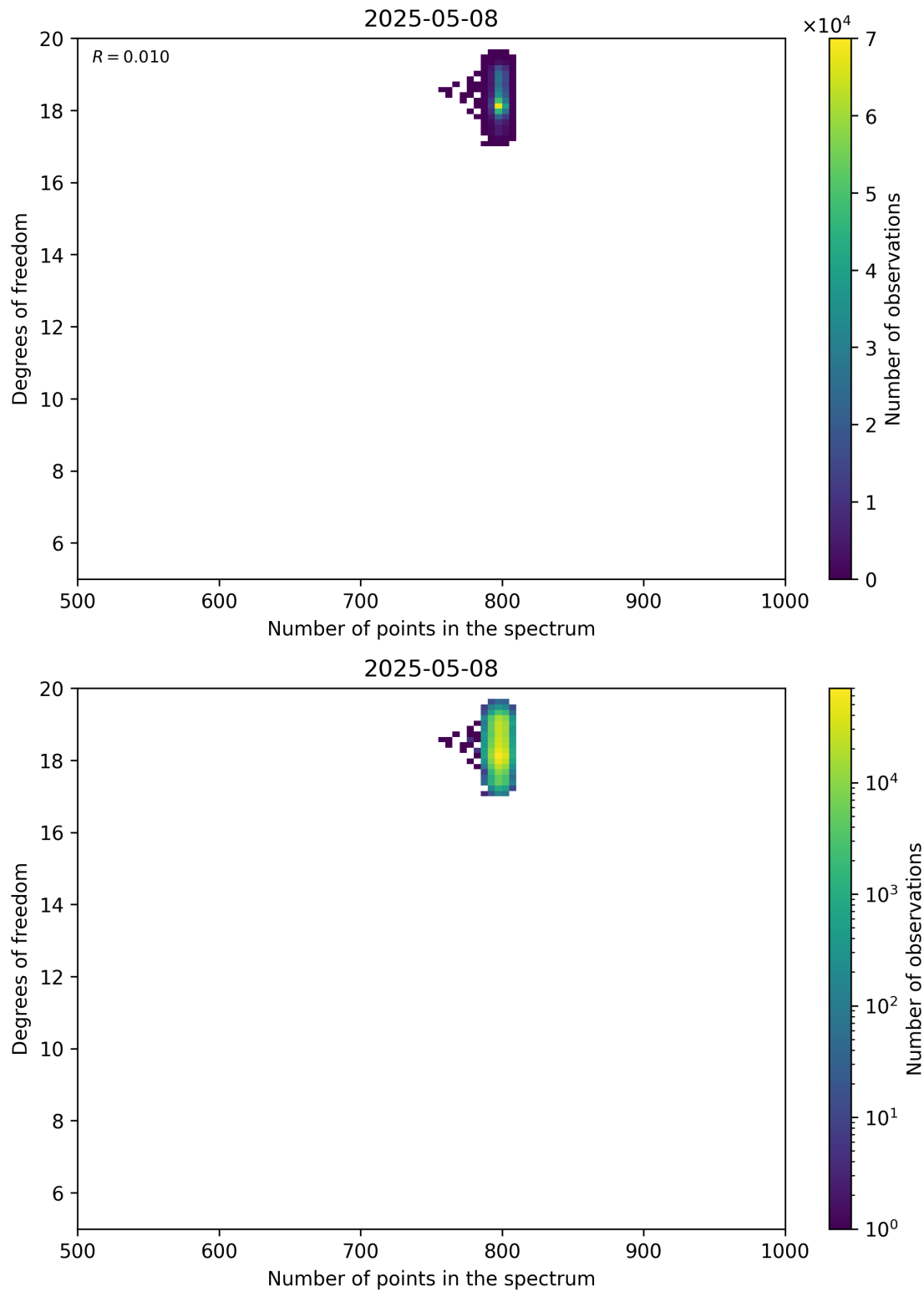
Figure 90: Scatter density plot of “Number of points in the spectrum” against “Degrees of freedom” for 2025-05-07 to 2025-05-09.
