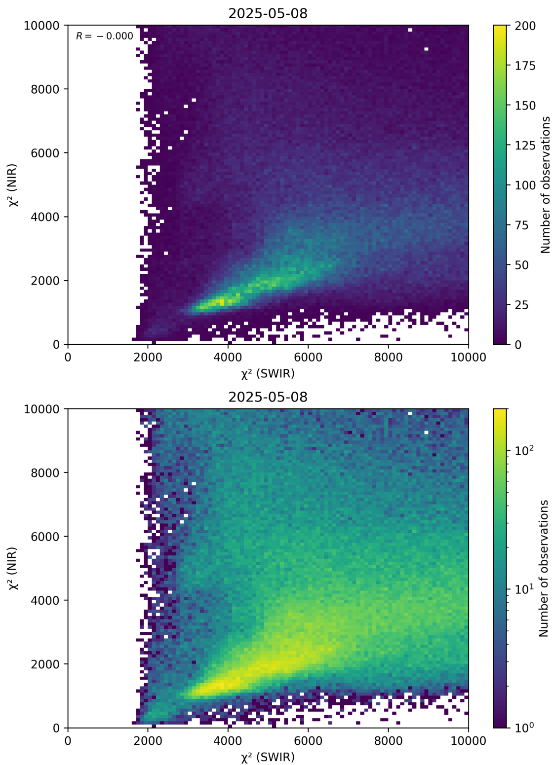
Figure 47: Scatter density plot of “ \chi^2 (SWIR)” against “ \chi^2 (NIR)” for 2025-05-07 to 2025-05-09.
