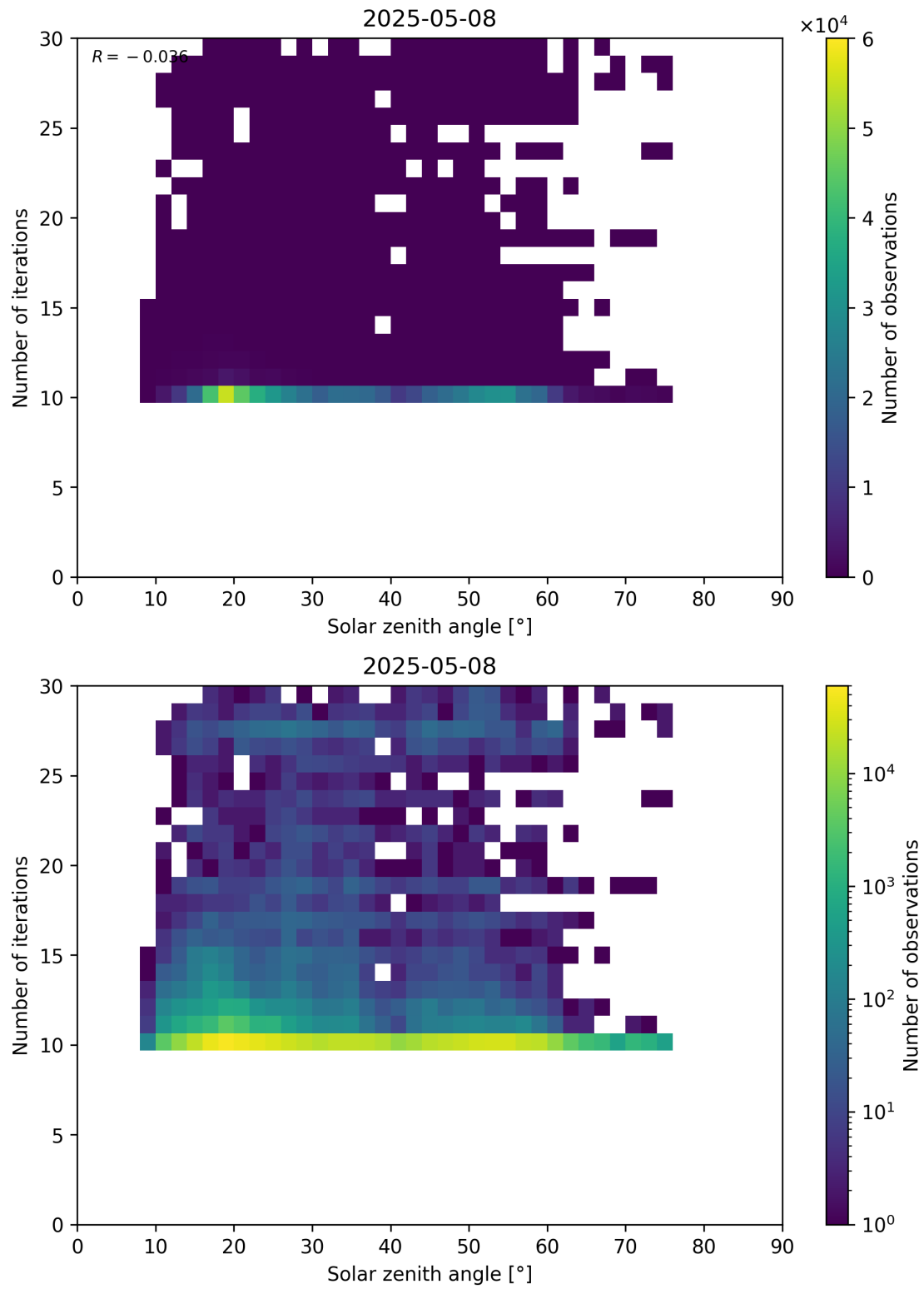
Figure 102: Scatter density plot of “Solar zenith angle” against “Number of iterations” for 2025-05-07 to 2025-05-09.
