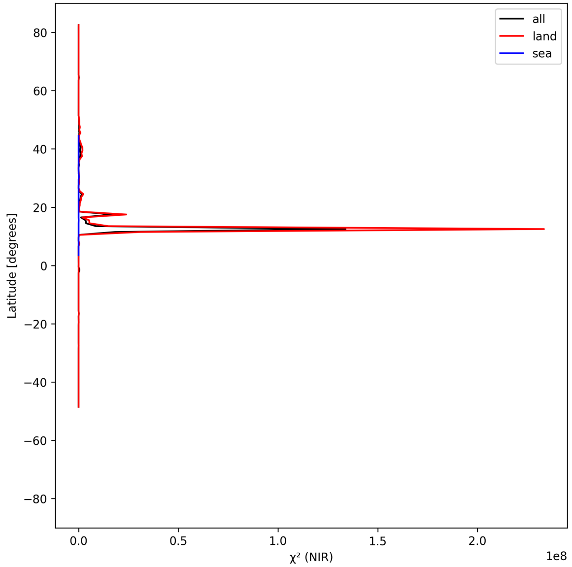
Figure 18: Zonal average of “ \chi^2 (NIR)” for 2025-05-07 to 2025-05-09.
