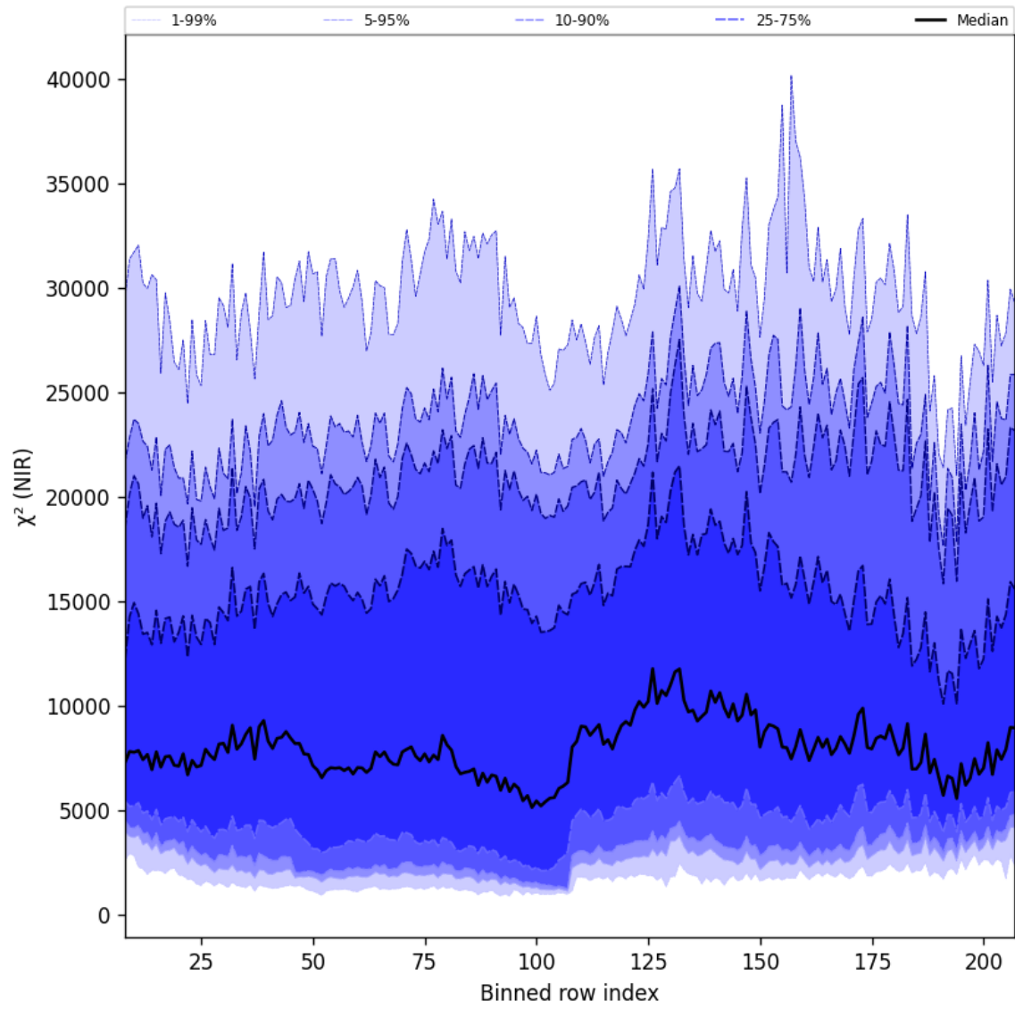
Figure 40: Along track statistics of “ \chi^2 (NIR)” for 2025-05-07 to 2025-05-09
