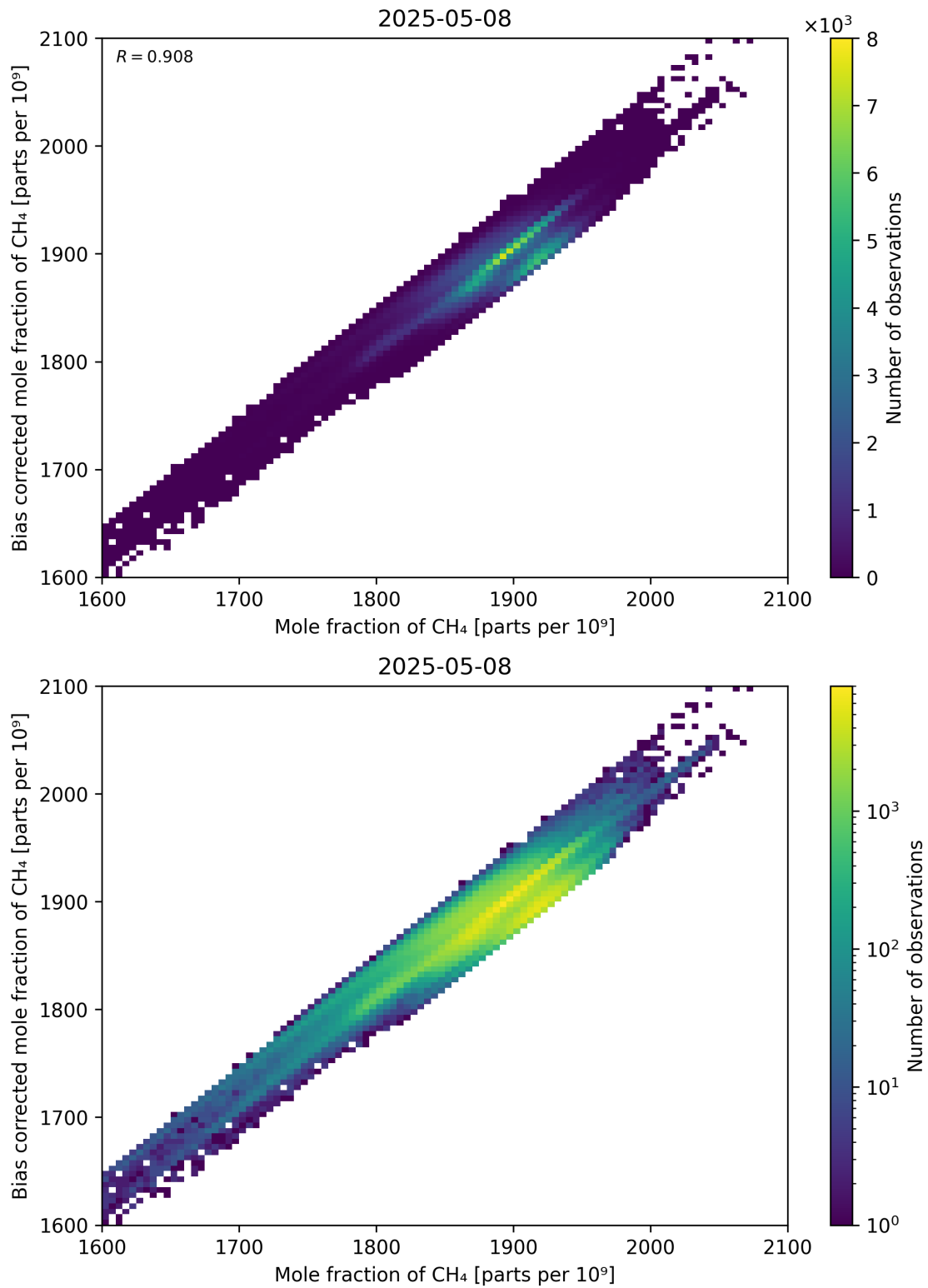
Figure 74: Scatter density plot of “Mole fraction of CH 4 ” against “Bias corrected mole fraction of CH 4 ” for 2025-05-07 to 2025-05-09.
