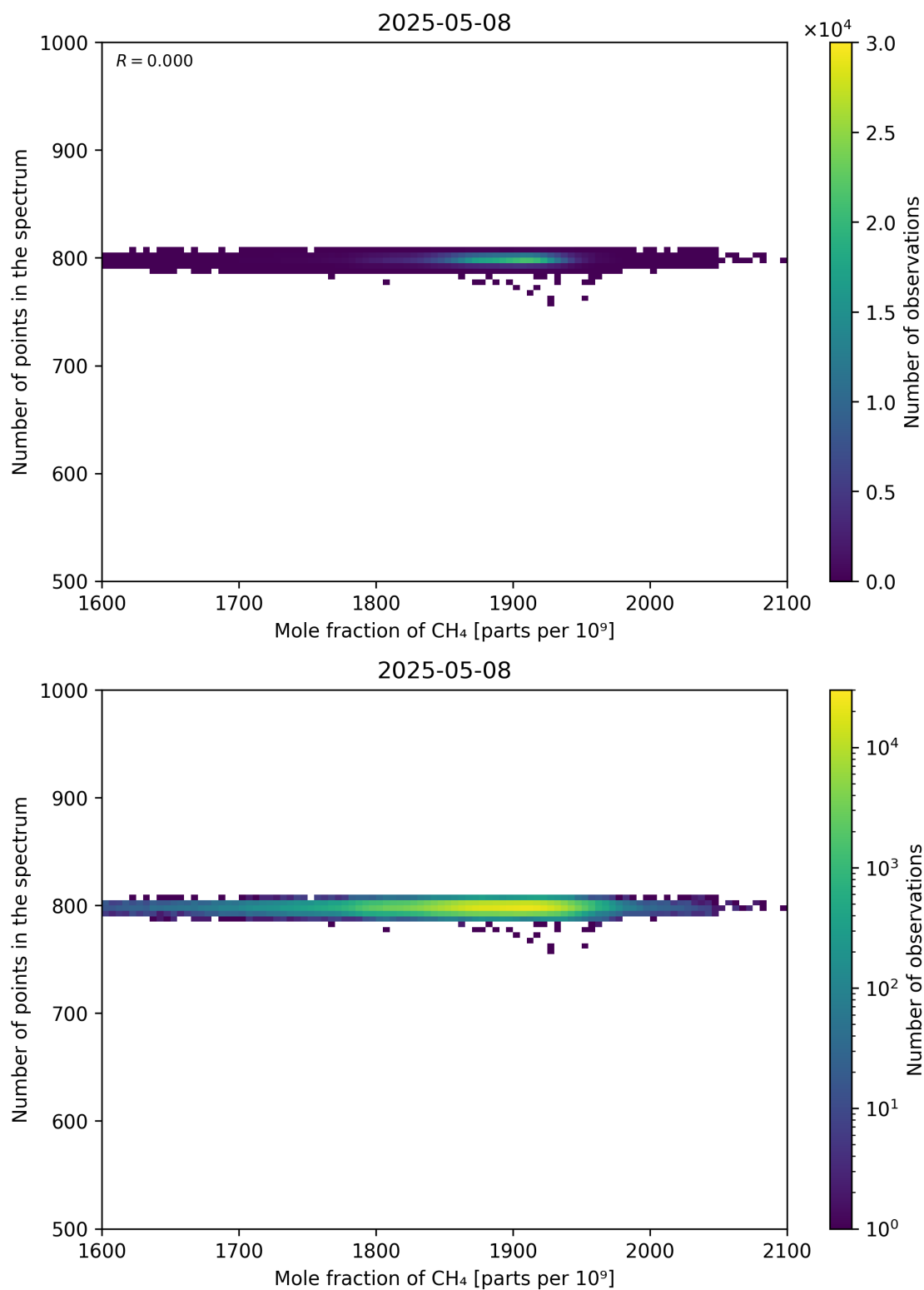
Figure 77: Scatter density plot of “Mole fraction of CH 4 ” against “Number of points in the spectrum” for 2025-05-07 to 2025-05-09.
