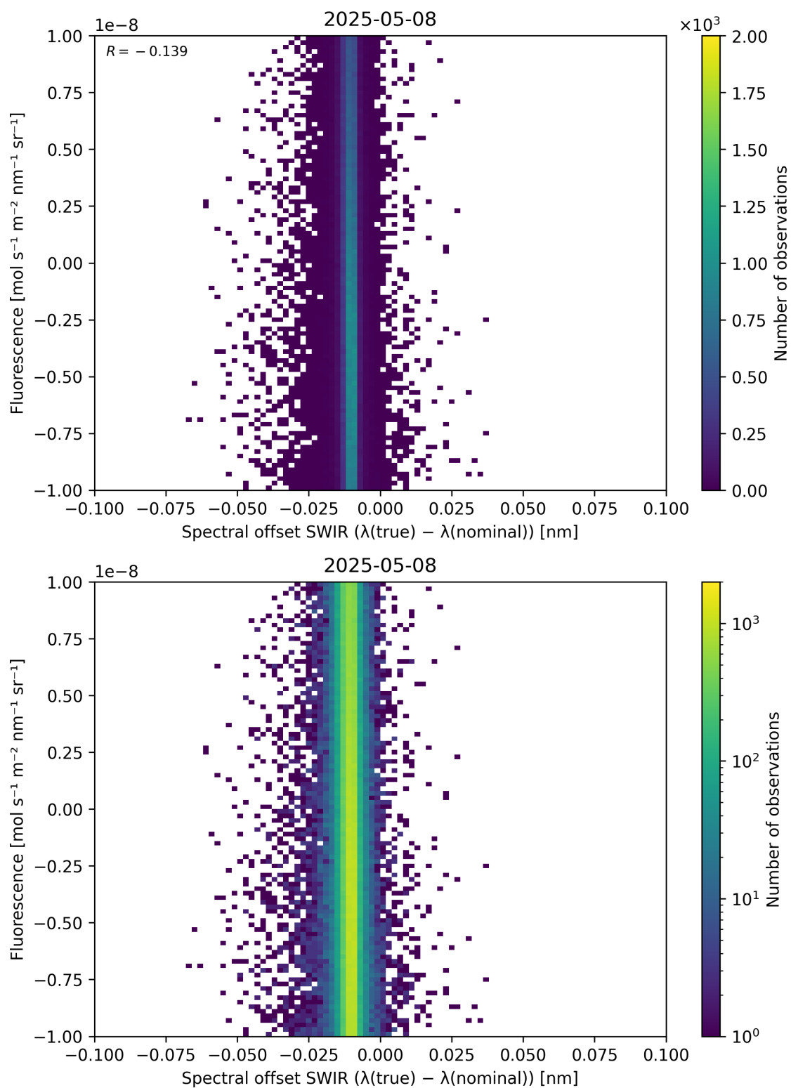
Figure 120: Scatter density plot of “Spectral offset SWIR ( \lambda_{\text{true}} - \lambda_{\text{nominal}} )” against “Fluorescence” for 2025-05-07 to 2025-05-09.
