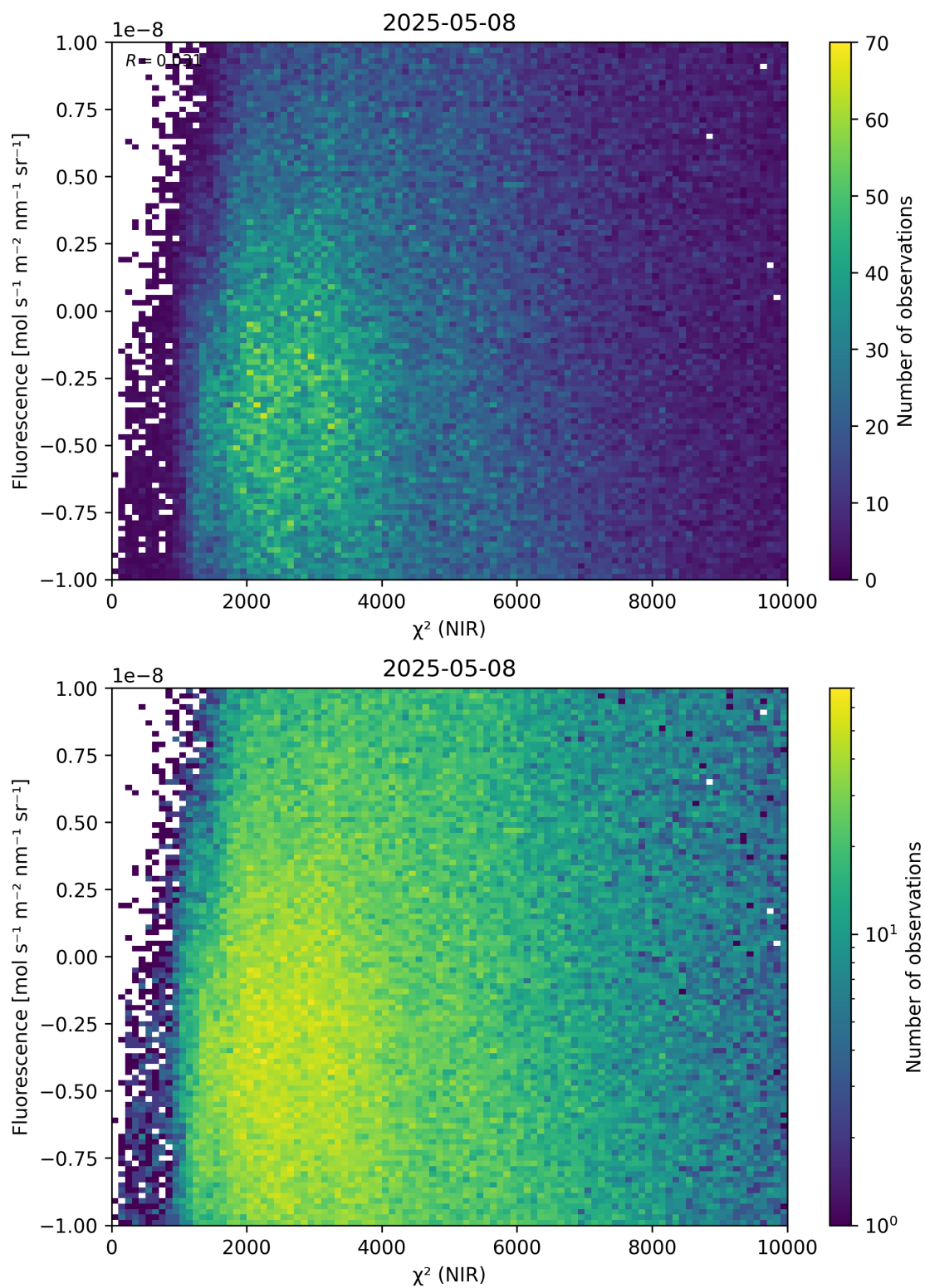
Figure 45: Scatter density plot of “ \chi^2 (NIR)” against “Fluorescence” for 2025-05-07 to 2025-05-09.
