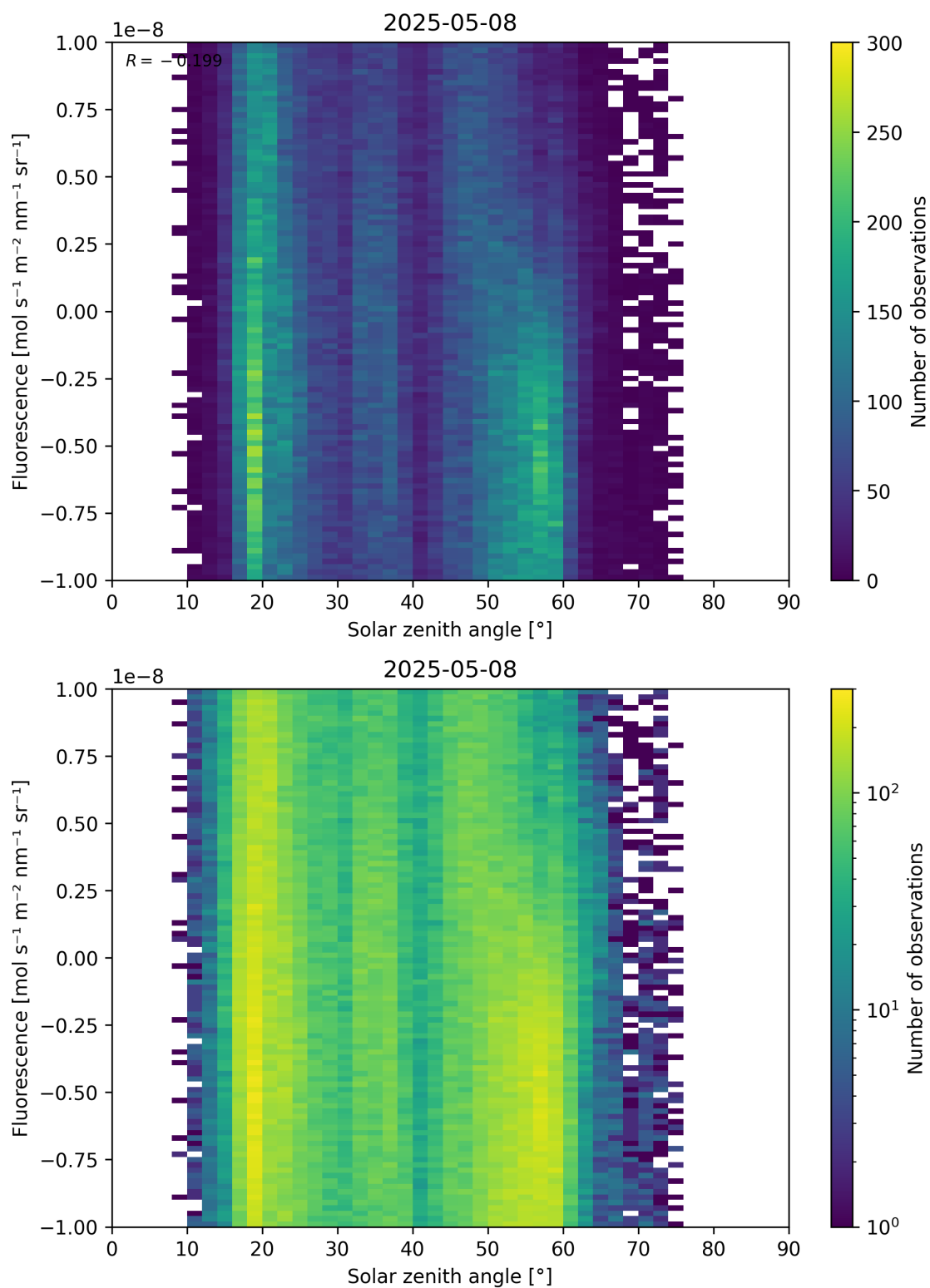
Figure 97: Scatter density plot of “Solar zenith angle” against “Fluorescence” for 2025-05-07 to 2025-05-09.
