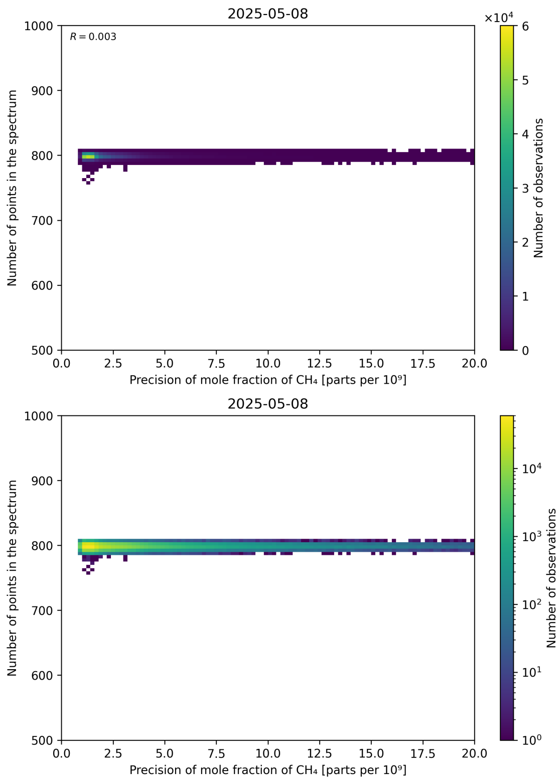
Figure 84: Scatter density plot of “Precision of mole fraction of CH 4 ” against “Number of points in the spectrum” for 2025-05-07 to 2025-05-09.
