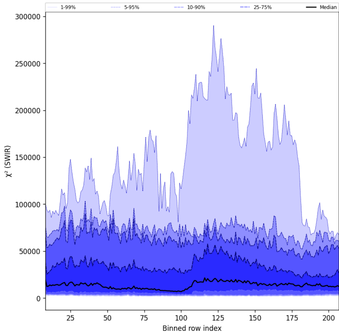
Figure 39: Along track statistics of " \chi^2 (SWIR)" for 2025-05-07 to 2025-05-09
