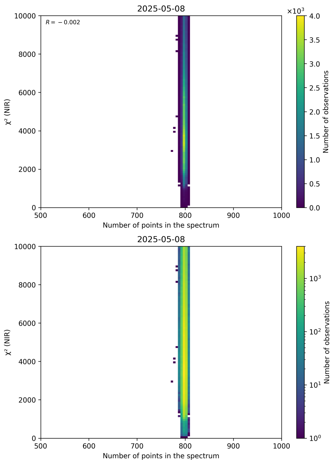
Figure 88: Scatter density plot of “Number of points in the spectrum” against “ \chi^2 (NIR)” for 2025-05-07 to 2025-05-09.
