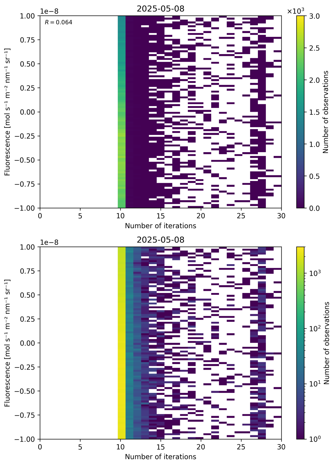
Figure 87: Scatter density plot of “Number of iterations” against “Fluorescence” for 2025-05-07 to 2025-05-09.
