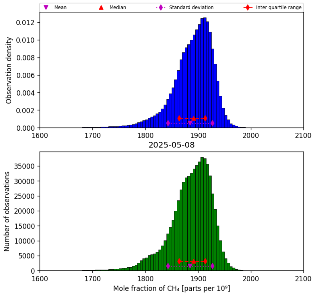
Figure 23: Histogram of “Mole fraction of CH 4 ” for 2025-05-07 to 2025-05-09
