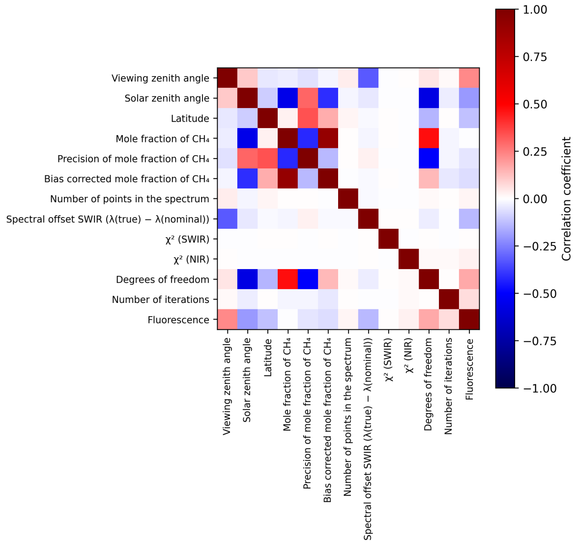
Figure 2: Map of correlation matrix for 2025-05-07 to 2025-05-09.
