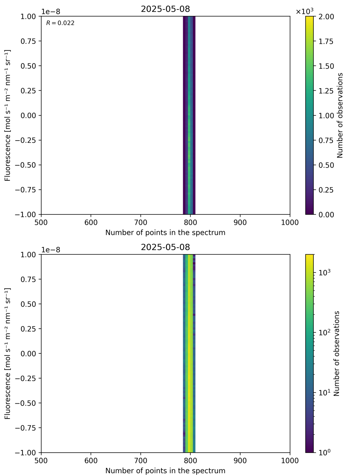
Figure 91: Scatter density plot of “Number of points in the spectrum” against “Fluorescence” for 2025-05-07 to 2025-05-09.
