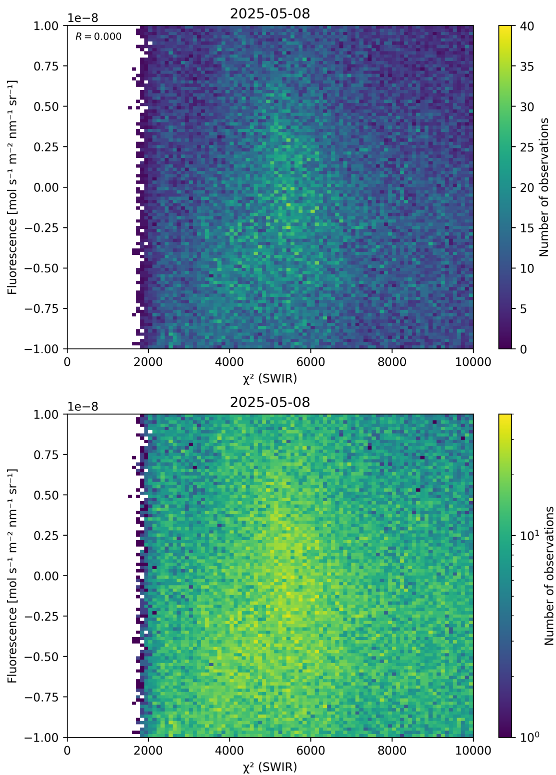
Figure 49: Scatter density plot of “ \chi^2 (SWIR)” against “Fluorescence” for 2025-05-07 to 2025-05-09.
