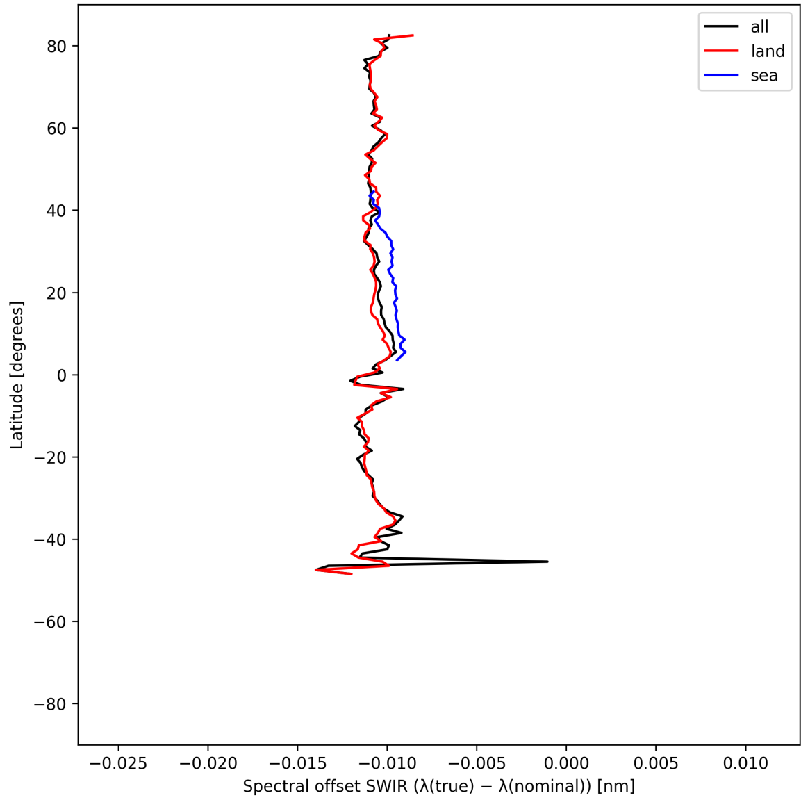
Figure 16: Zonal average of “Spectral offset SWIR ( \lambda_{\text{true}} - \lambda_{\text{nominal}} )” for 2025-05-07 to 2025-05-09.
