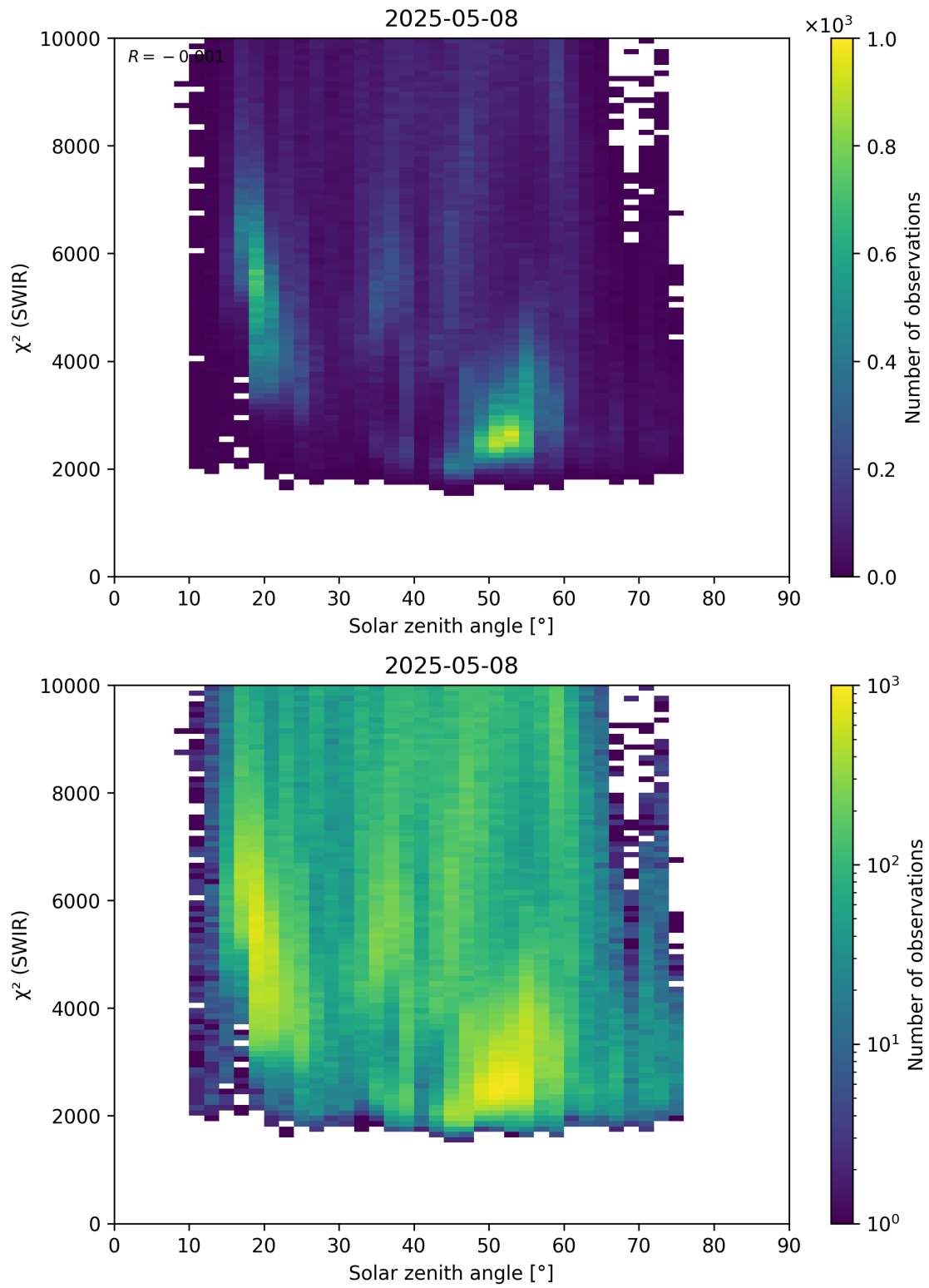
Figure 95: Scatter density plot of “Solar zenith angle” against “ \chi^2 (SWIR)” for 2025-05-07 to 2025-05-09.
