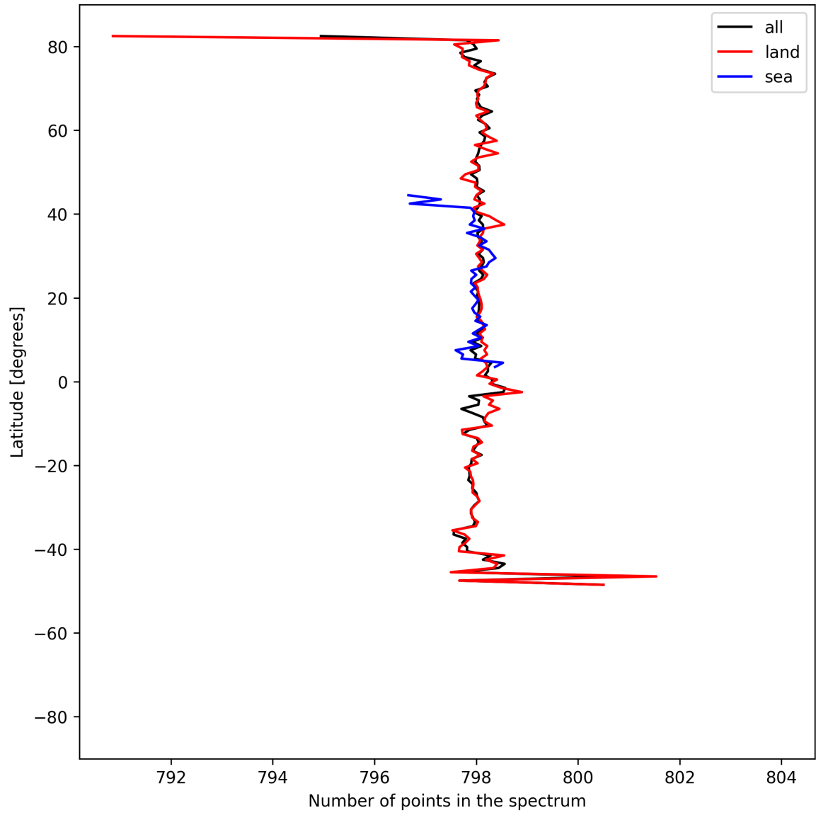
Figure 15: Zonal average of “Number of points in the spectrum” for 2025-05-07 to 2025-05-09.
