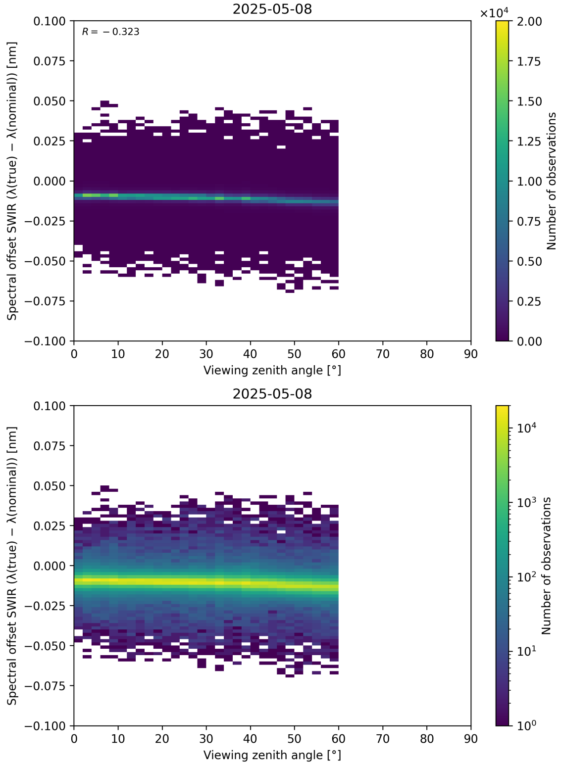
Figure 116: Scatter density plot of “Viewing zenith angle” against “Spectral offset SWIR ( \lambda_{\text{true}} - \lambda_{\text{nominal}} )” for 2025-05-07 to 2025-05-09.
