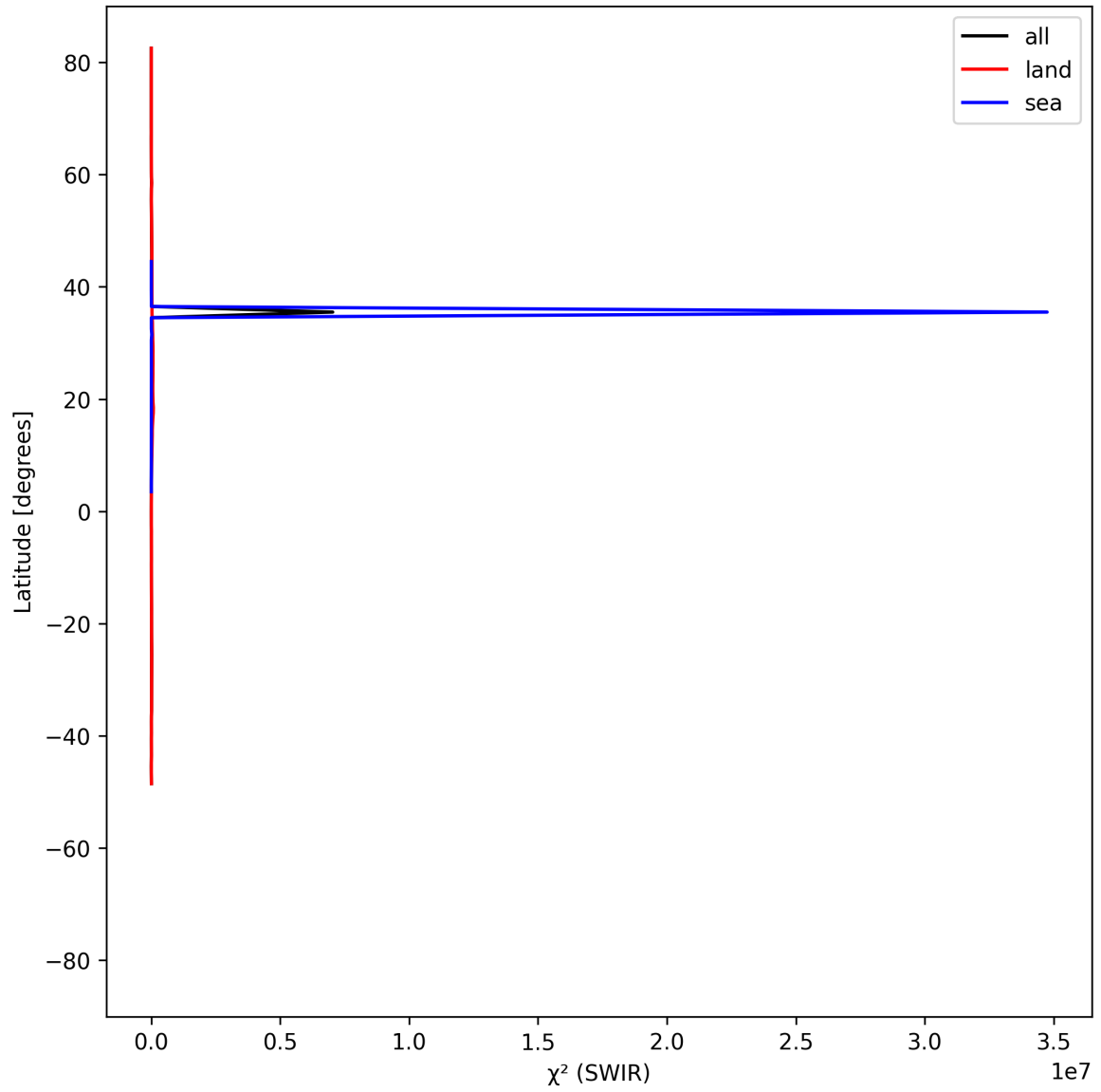
Figure 17: Zonal average of “ \chi^2 (SWIR)” for 2025-05-07 to 2025-05-09.
