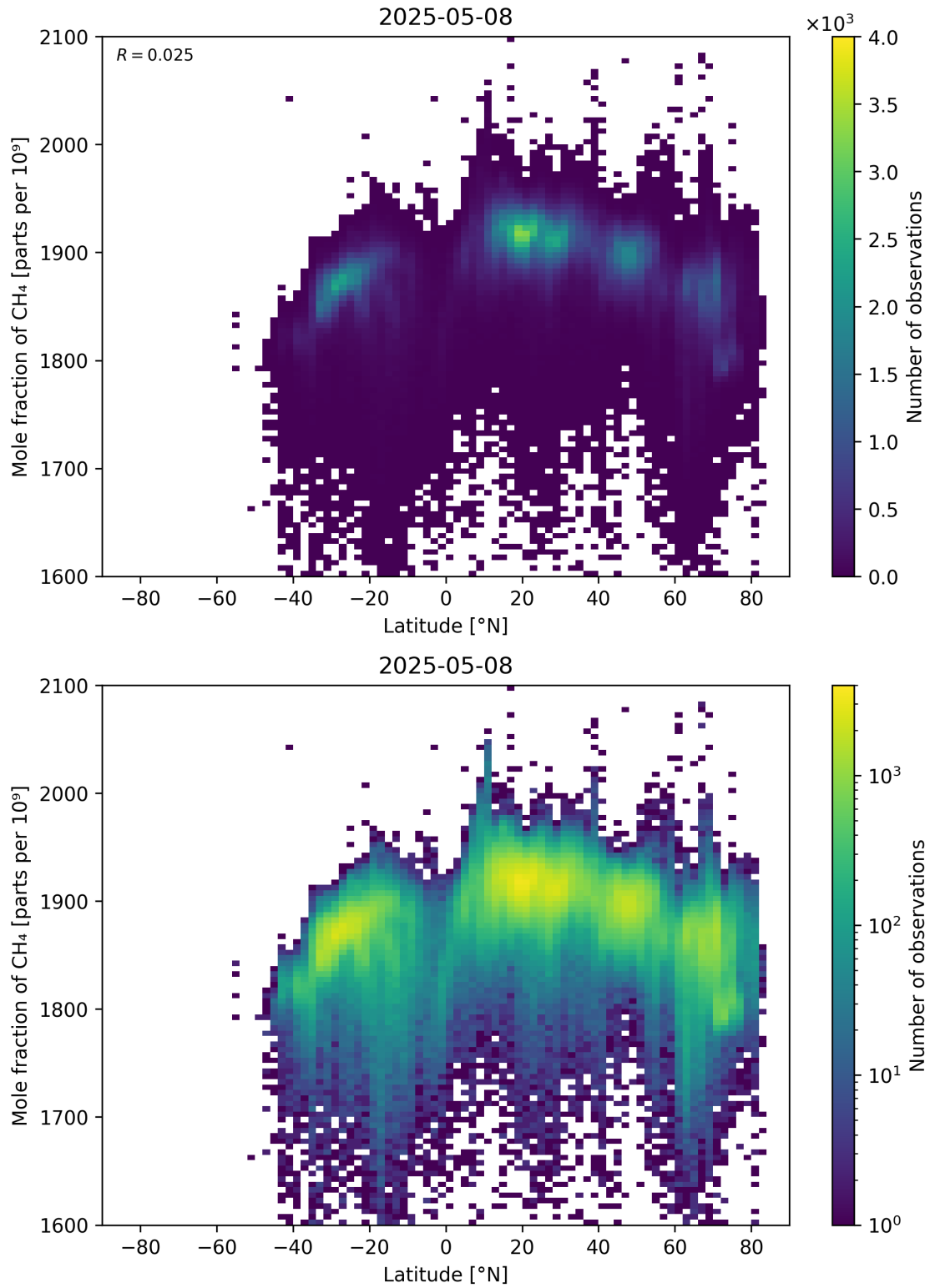
Figure 57: Scatter density plot of “Latitude” against “Mole fraction of \text{CH}_4 ” for 2025-05-07 to 2025-05-09.
