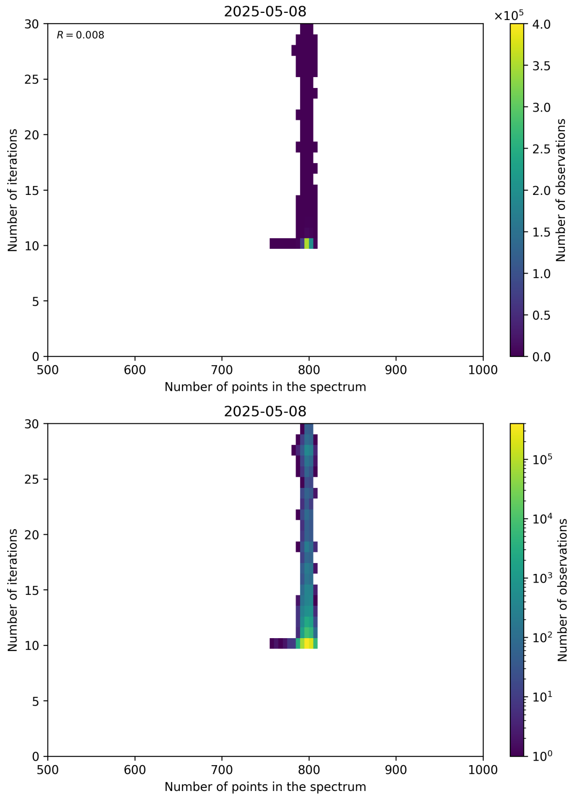
Figure 92: Scatter density plot of “Number of points in the spectrum” against “Number of iterations” for 2025-05-07 to 2025-05-09.
