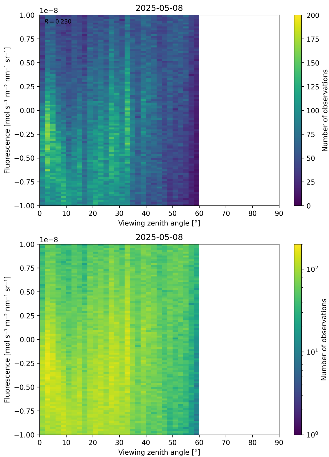
Figure 108: Scatter density plot of “Viewing zenith angle” against “Fluorescence” for 2025-05-07 to 2025-05-09.
