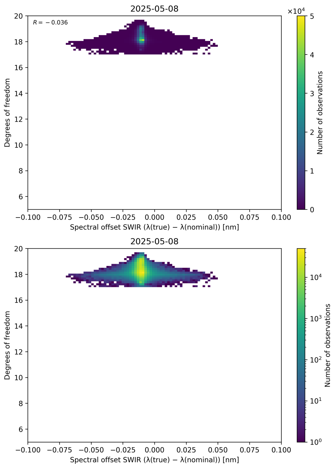
Figure 119: Scatter density plot of “Spectral offset SWIR ( \lambda_{\text{true}} - \lambda_{\text{nominal}} )” against “Degrees of freedom” for 2025-05-07 to 2025-05-09.
