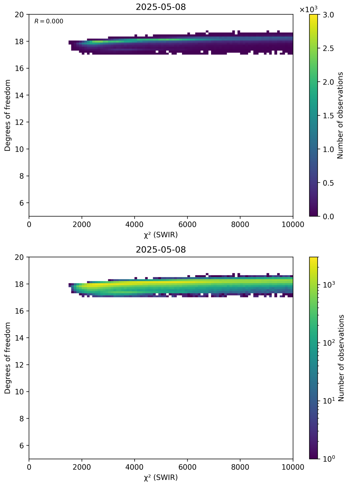
Figure 48: Scatter density plot of “ \chi^2 (SWIR)” against “Degrees of freedom” for 2025-05-07 to 2025-05-09.
