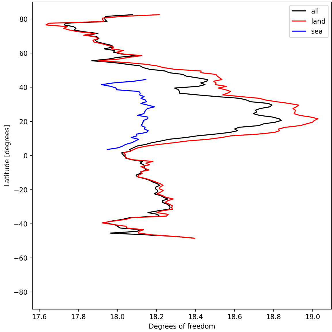
Figure 19: Zonal average of “Degrees of freedom” for 2025-05-07 to 2025-05-09.
