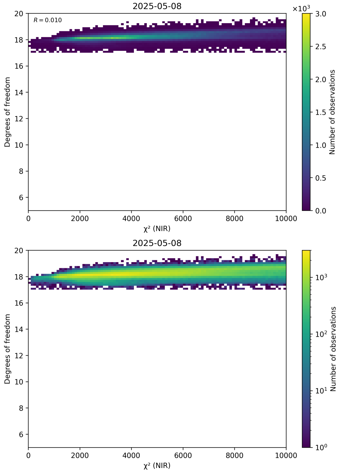
Figure 44: Scatter density plot of “ \chi^2 (NIR)” against “Degrees of freedom” for 2025-05-07 to 2025-05-09.
