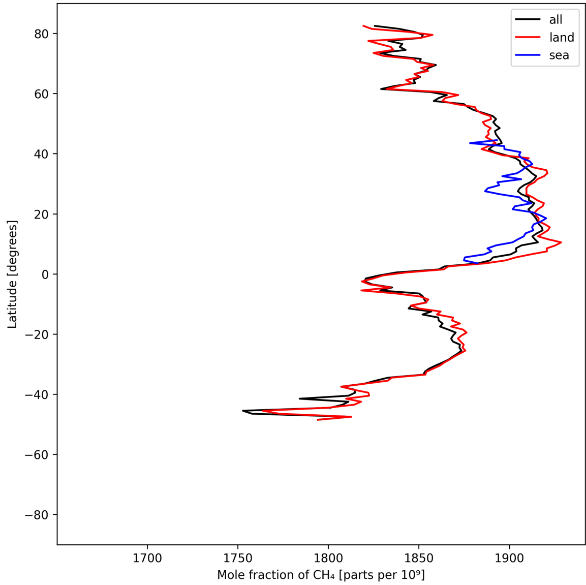
Figure 12: Zonal average of “Mole fraction of \text{CH}_4 ” for 2025-05-07 to 2025-05-09.
