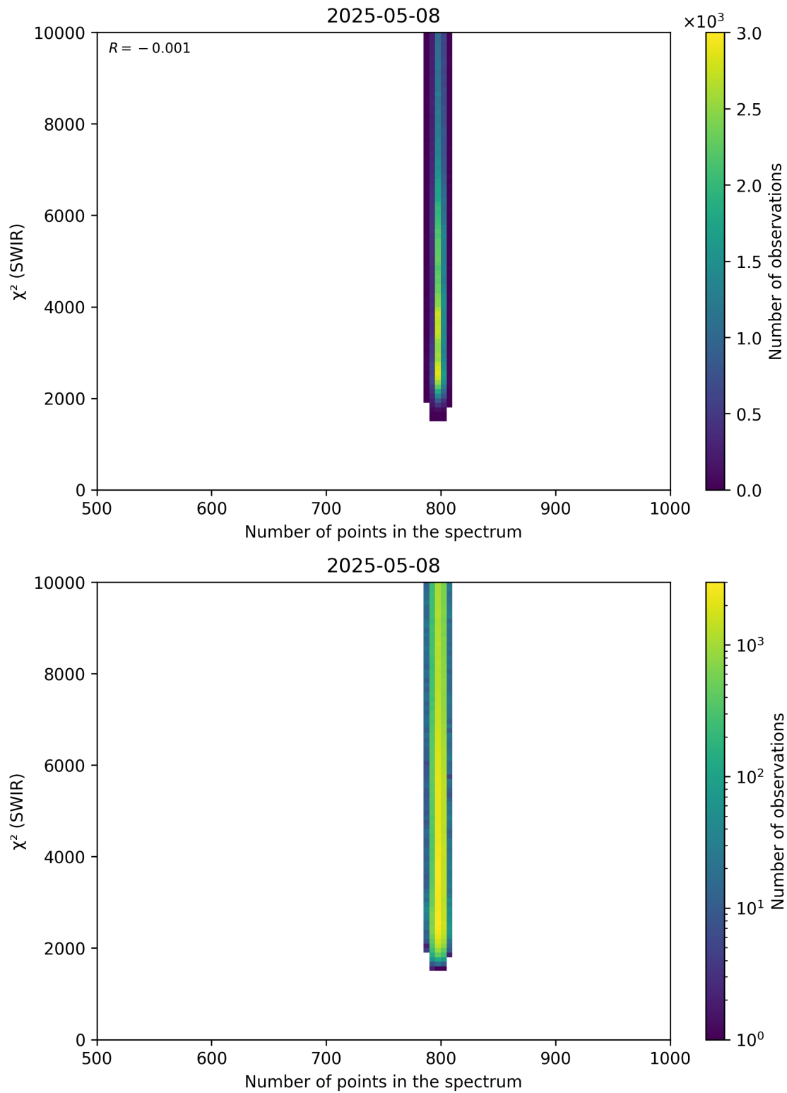
Figure 89: Scatter density plot of “Number of points in the spectrum” against “ \chi^2 (SWIR)” for 2025-05-07 to 2025-05-09.
