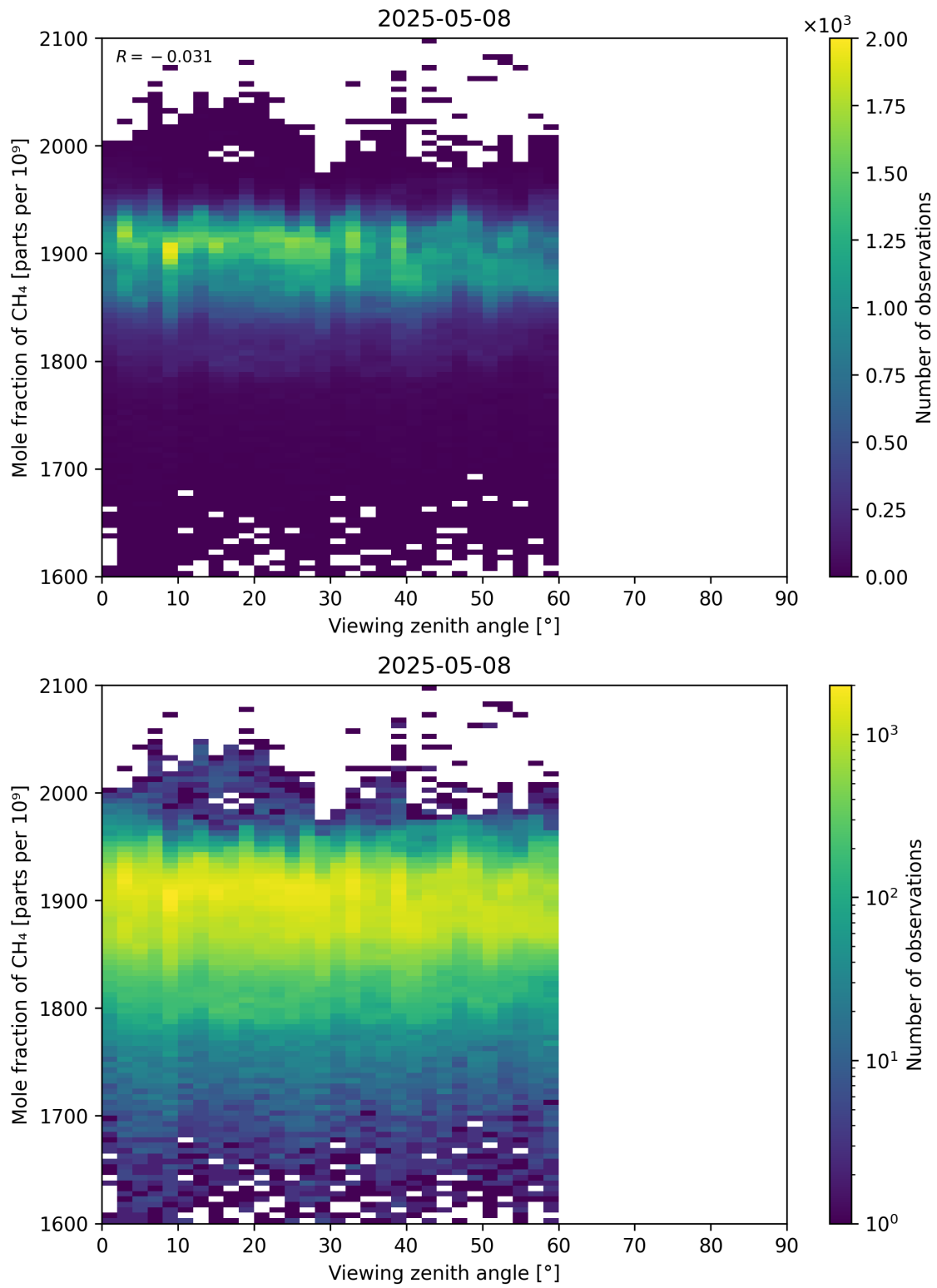
Figure 110: Scatter density plot of “Viewing zenith angle” against “Mole fraction of CH 4 ” for 2025-05-07 to 2025-05-09.
