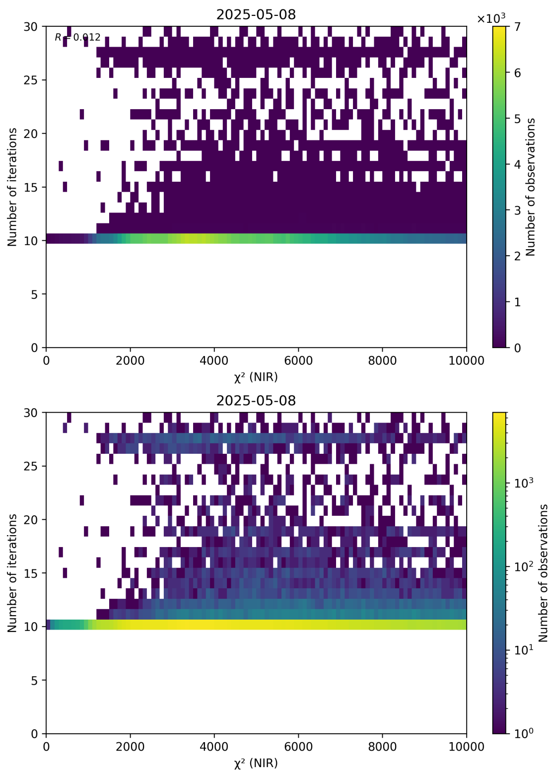
Figure 46: Scatter density plot of “ \chi^2 (NIR)” against “Number of iterations” for 2025-05-07 to 2025-05-09.
