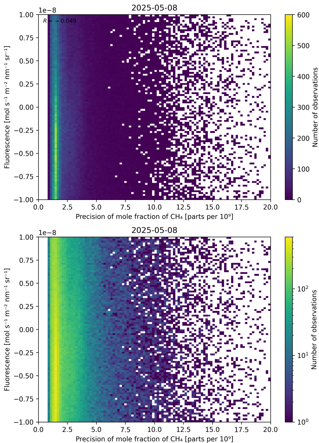
Figure 81: Scatter density plot of “Precision of mole fraction of \text{CH}_4 ” against “Fluorescence” for 2025-05-07 to 2025-05-09.
