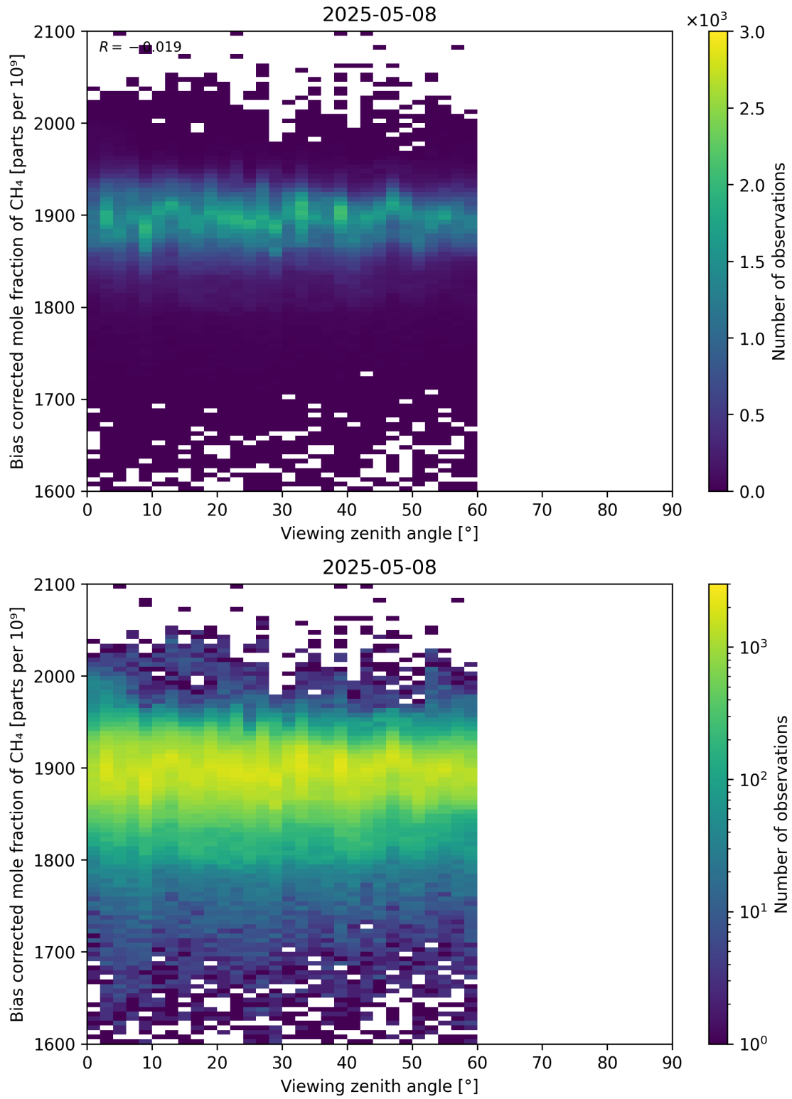
Figure 111: Scatter density plot of “Viewing zenith angle” against “Bias corrected mole fraction of CH 4 ” for 2025-05-07 to 2025-05-09.
