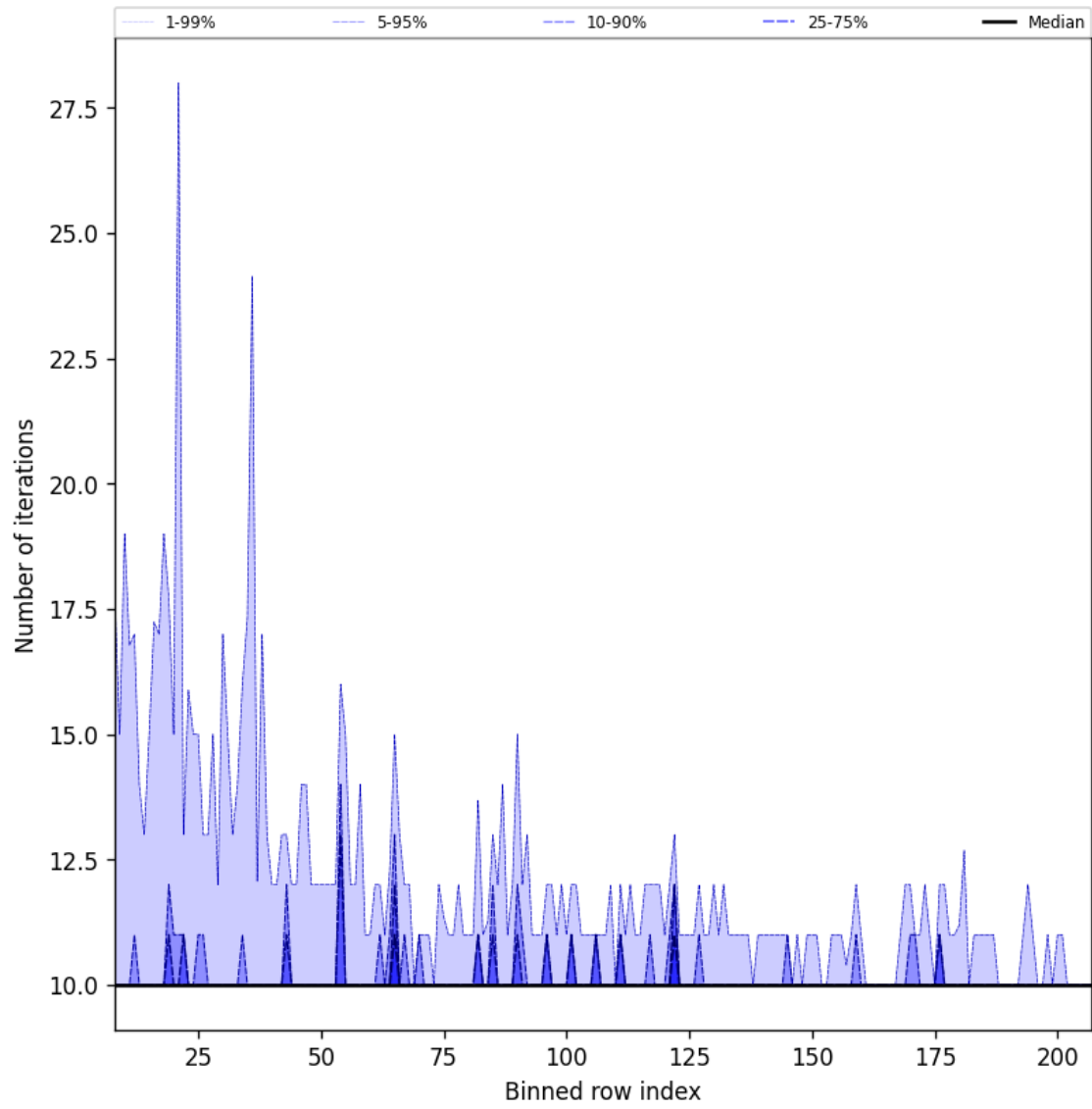
Figure 42: Along track statistics of “Number of iterations” for 2025-05-07 to 2025-05-09
