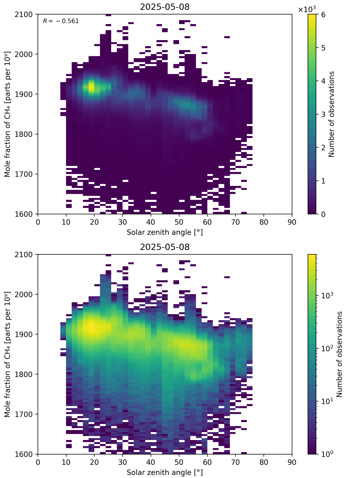
Figure 99: Scatter density plot of “Solar zenith angle” against “Mole fraction of CH 4 ” for 2025-05-07 to 2025-05-09.
