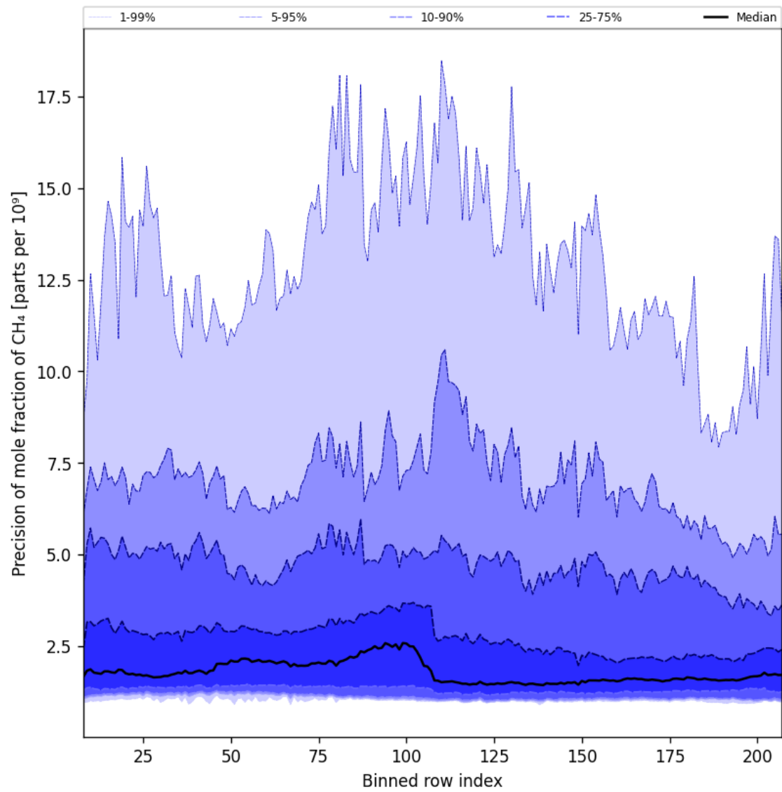
Figure 35: Along track statistics of “Precision of mole fraction of CH 4 ” for 2025-05-07 to 2025-05-09
