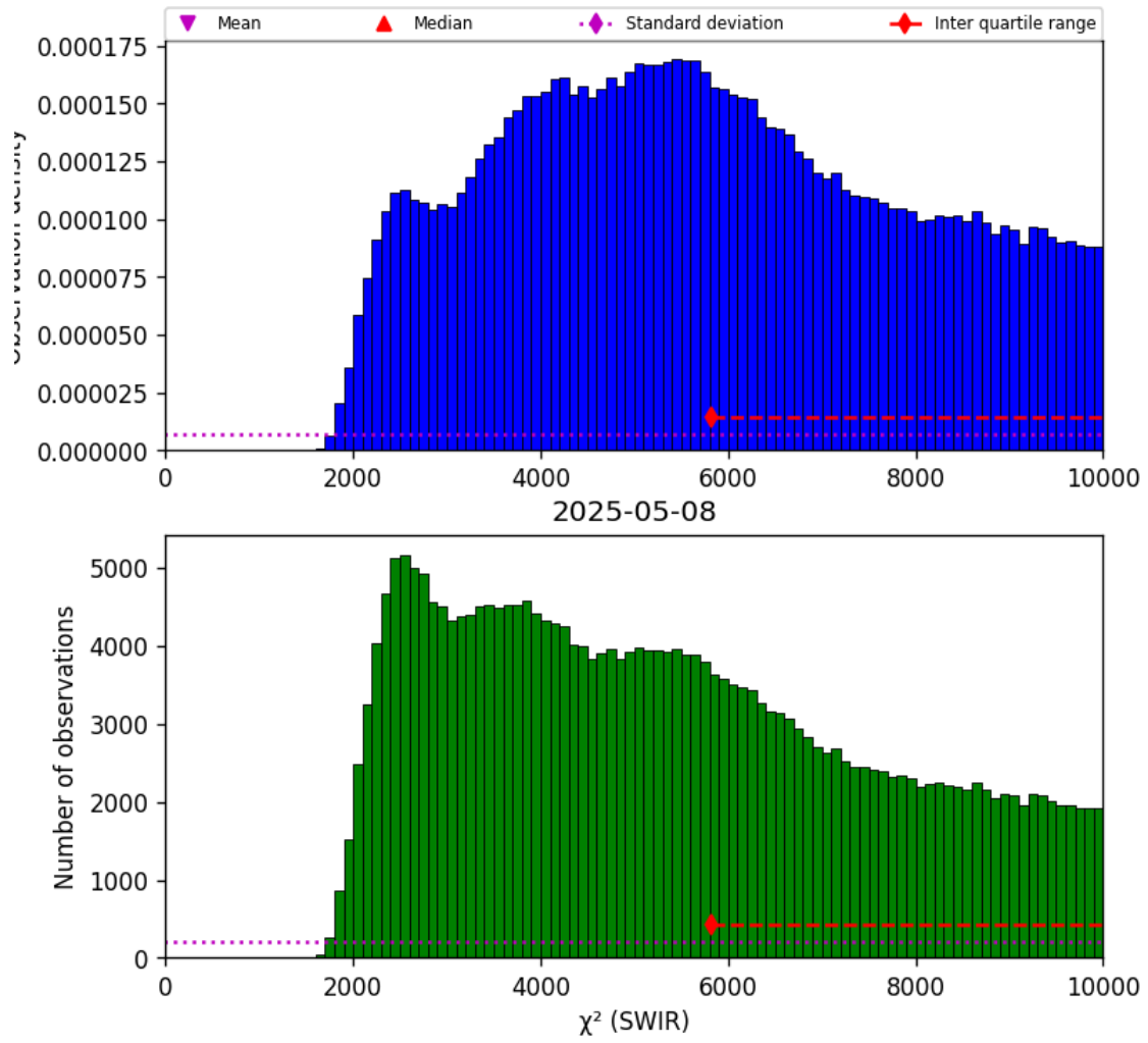
Figure 28: Histogram of “ \chi^2 (SWIR)” for 2025-05-07 to 2025-05-09
