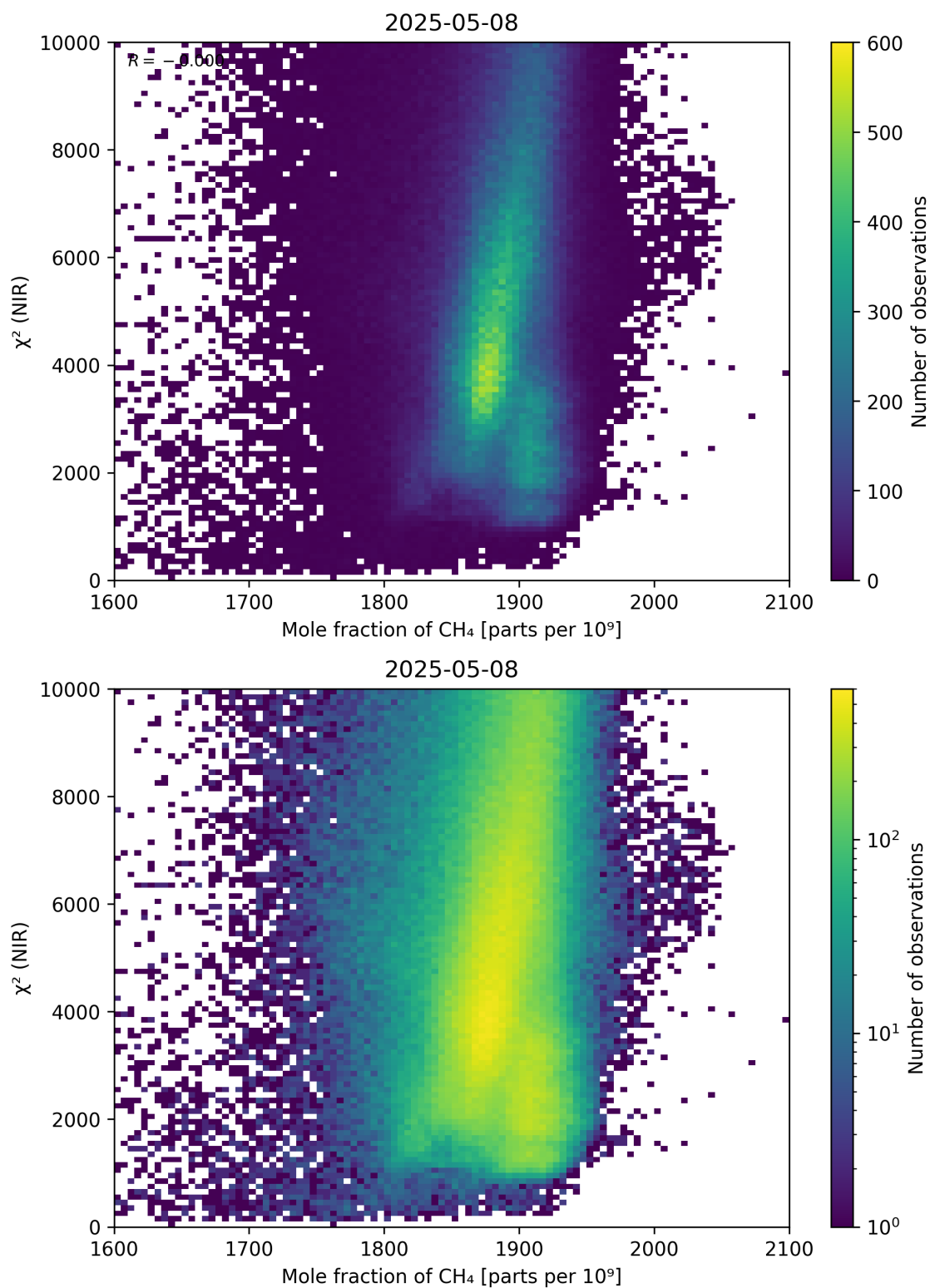
Figure 70: Scatter density plot of “Mole fraction of CH 4 ” against “ \chi^2 (NIR)” for 2025-05-07 to 2025-05-09.
