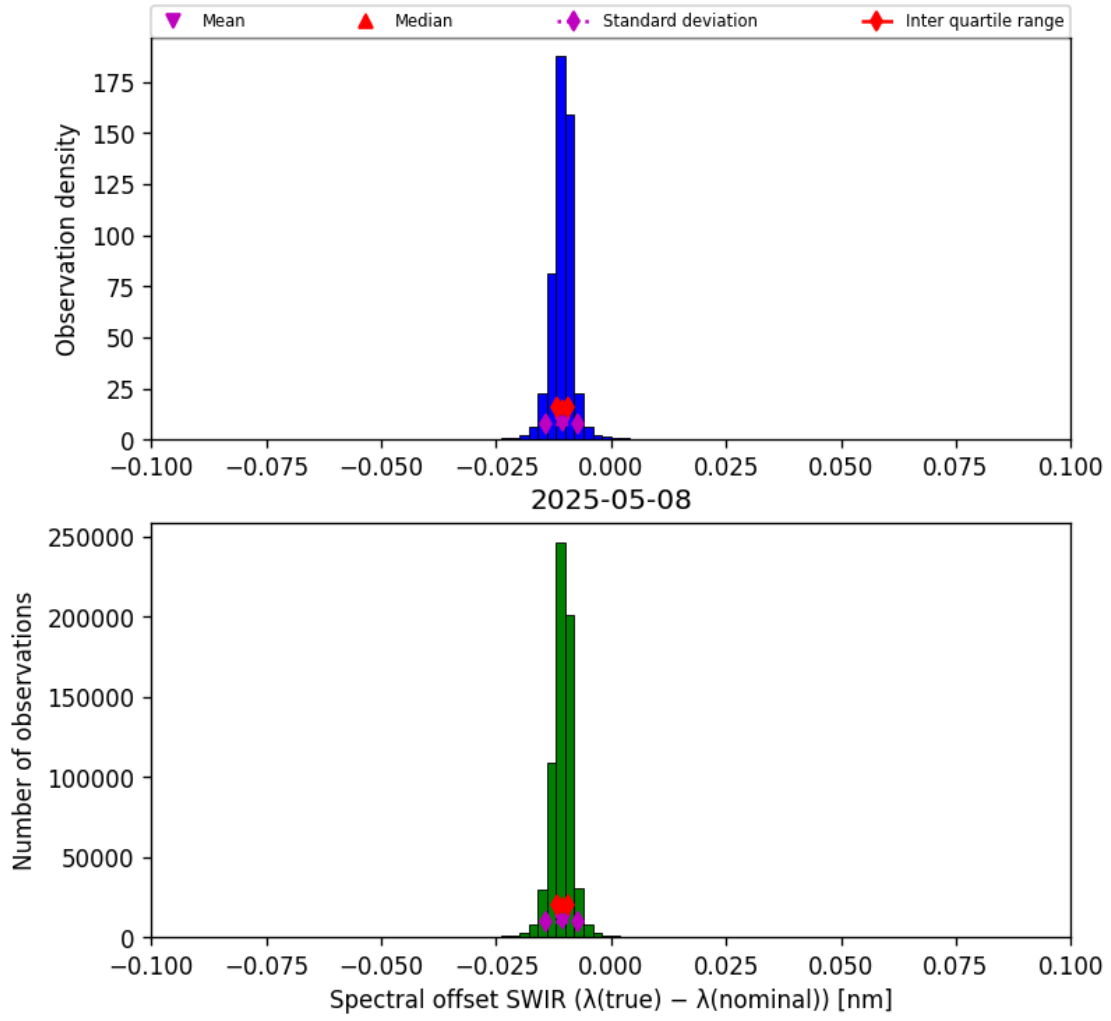
Figure 27: Histogram of “Spectral offset SWIR ( \lambda_{\text{true}} - \lambda_{\text{nominal}} )” for 2025-05-07 to 2025-05-09
