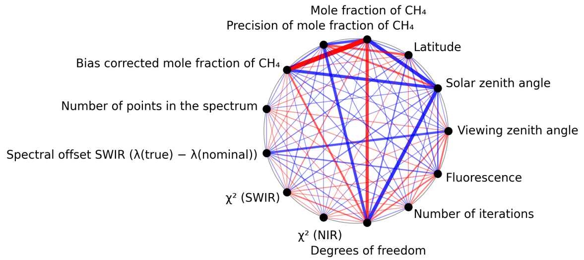
Figure 1: Map of correlation graph for 2025-05-08 to 2025-05-10.
