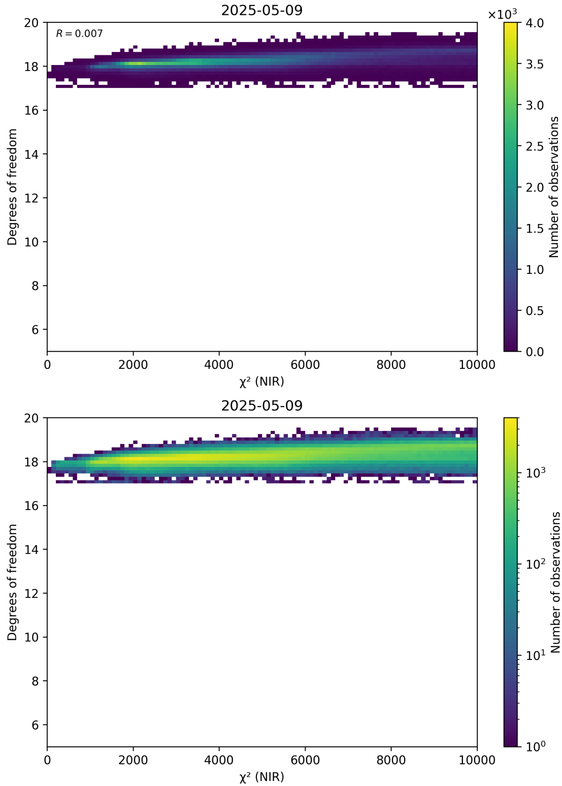
Figure 44: Scatter density plot of “ \chi^2 (NIR)” against “Degrees of freedom” for 2025-05-08 to 2025-05-10.
