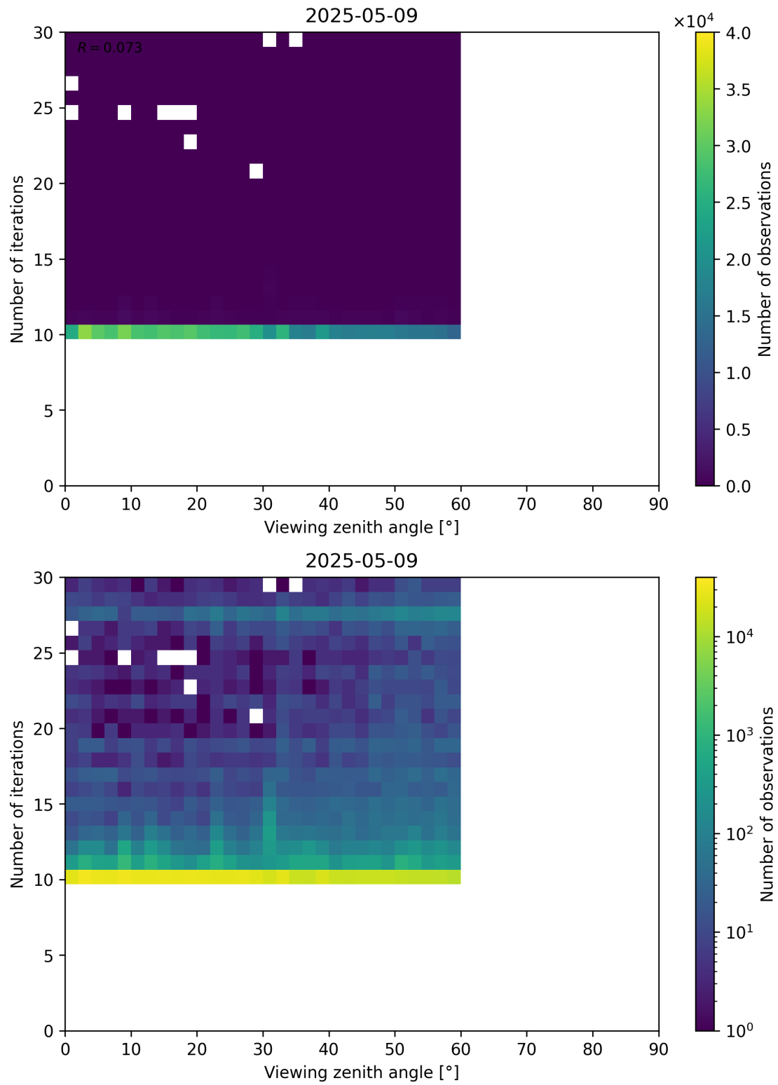
Figure 113: Scatter density plot of “Viewing zenith angle” against “Number of iterations” for 2025-05-08 to 2025-05-10.
