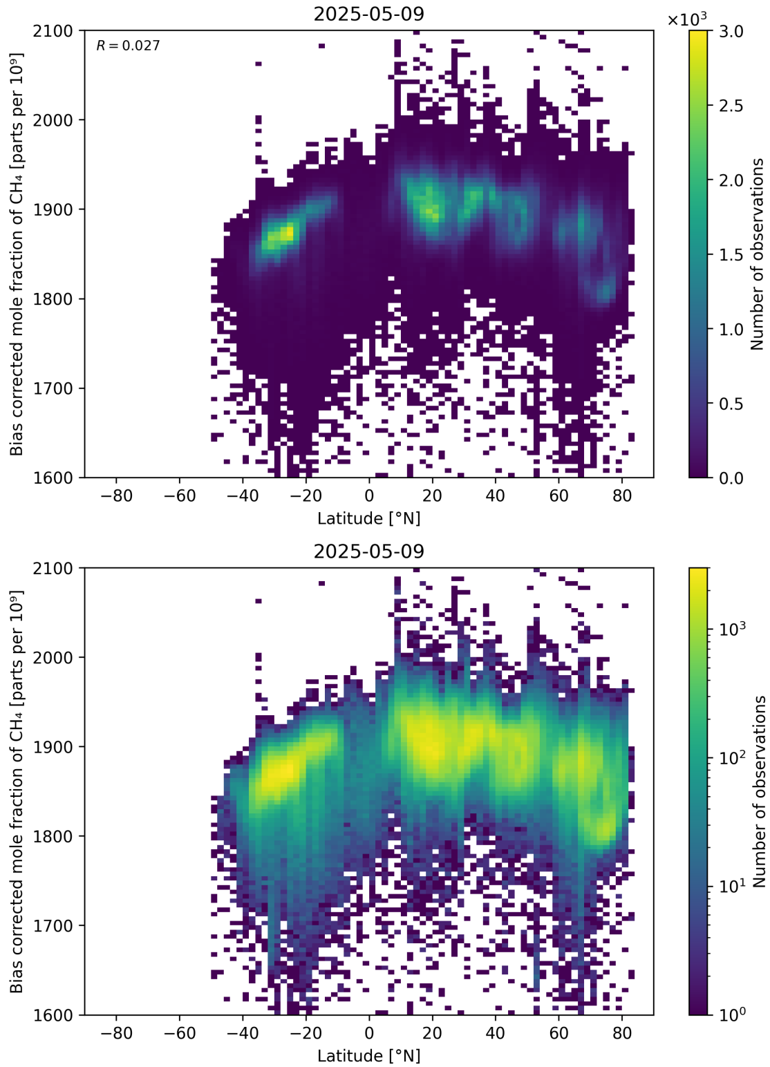
Figure 58: Scatter density plot of “Latitude” against “Bias corrected mole fraction of CH 4 ” for 2025-05-08 to 2025-05-10.
