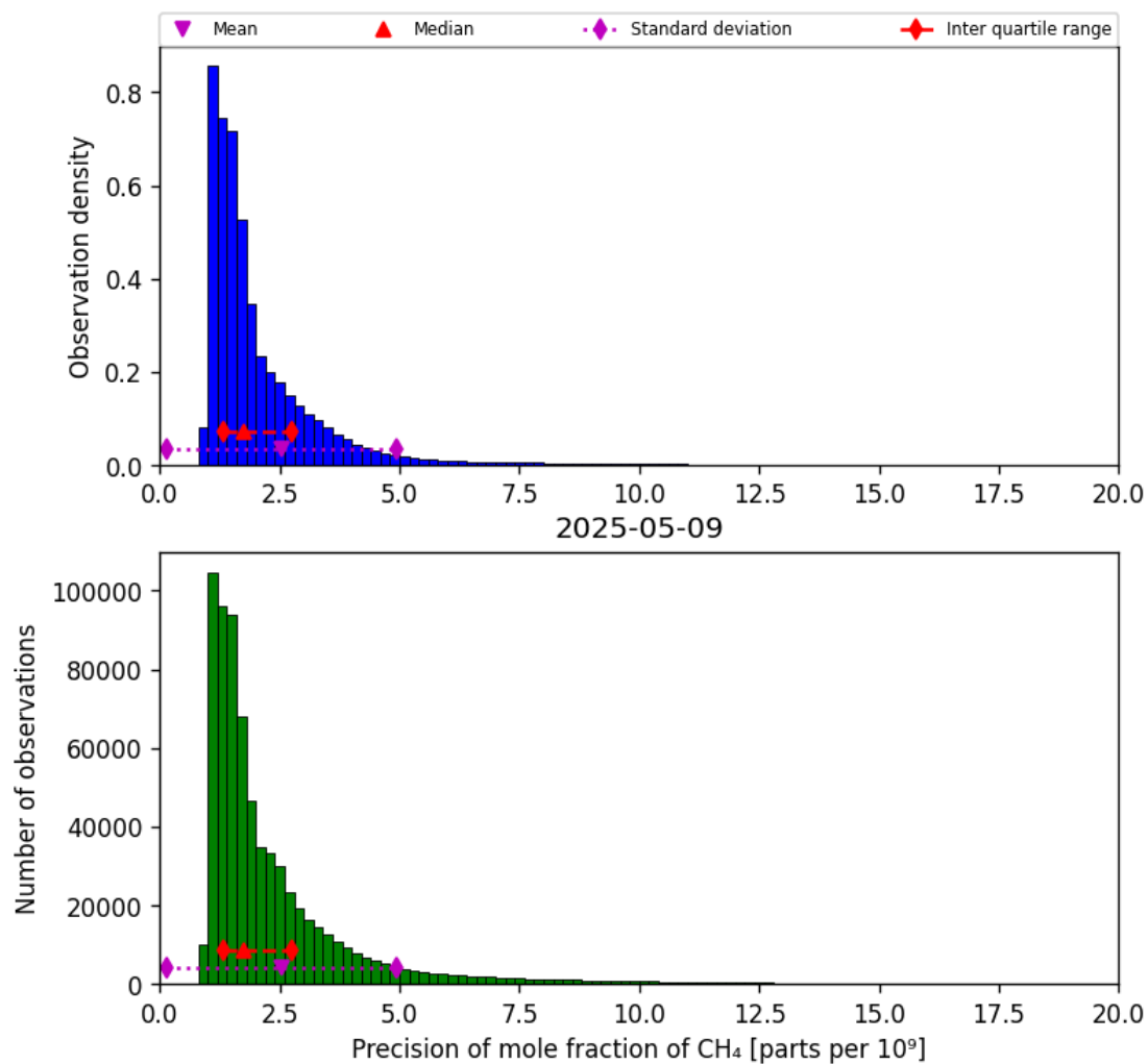
Figure 24: Histogram of “Precision of mole fraction of CH 4 ” for 2025-05-08 to 2025-05-10
