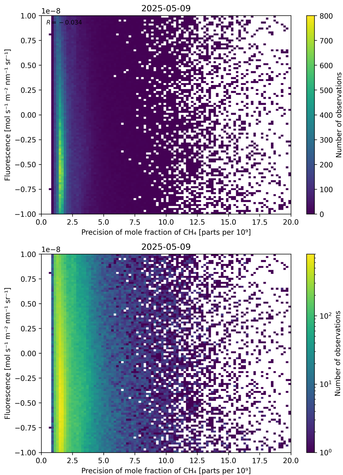
Figure 81: Scatter density plot of “Precision of mole fraction of CH 4 ” against “Fluorescence” for 2025-05-08 to 2025-05-10.
