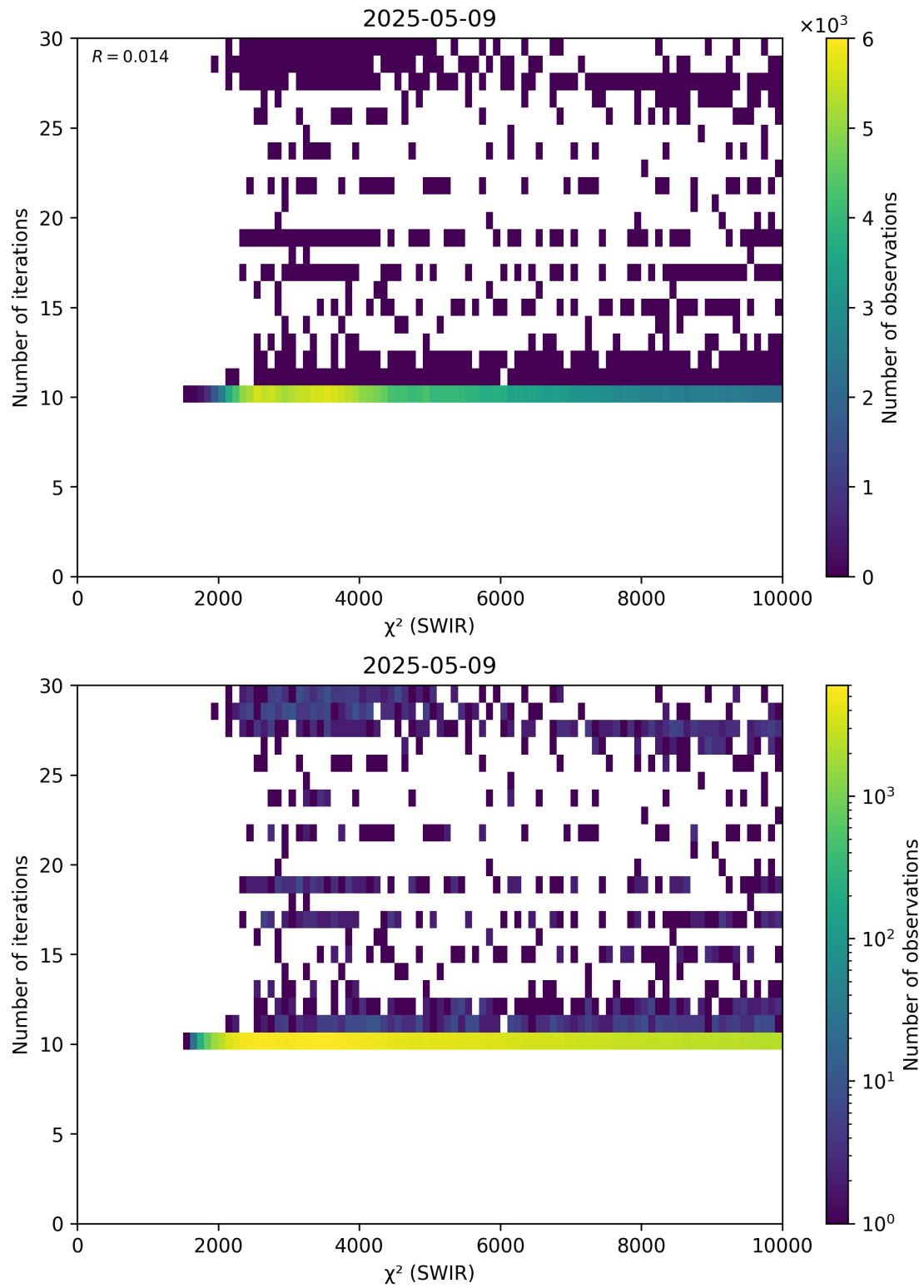
Figure 50: Scatter density plot of “ \chi^2 (SWIR)” against “Number of iterations” for 2025-05-08 to 2025-05-10.
