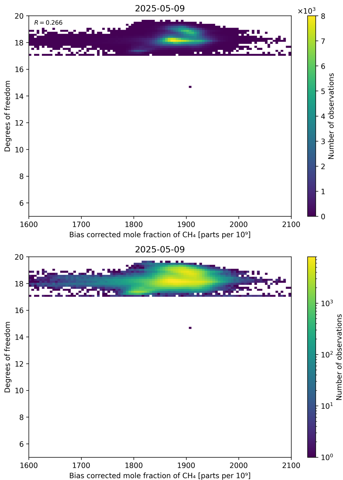
Figure 65: Scatter density plot of “Bias corrected mole fraction of CH 4 ” against “Degrees of freedom” for 2025-05-08 to 2025-05-10.
