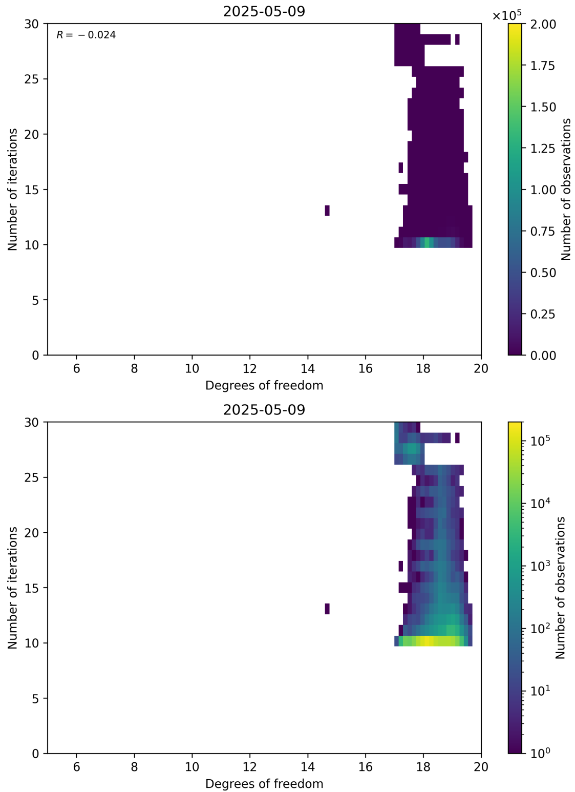
Figure 52: Scatter density plot of “Degrees of freedom” against “Number of iterations” for 2025-05-08 to 2025-05-10.
