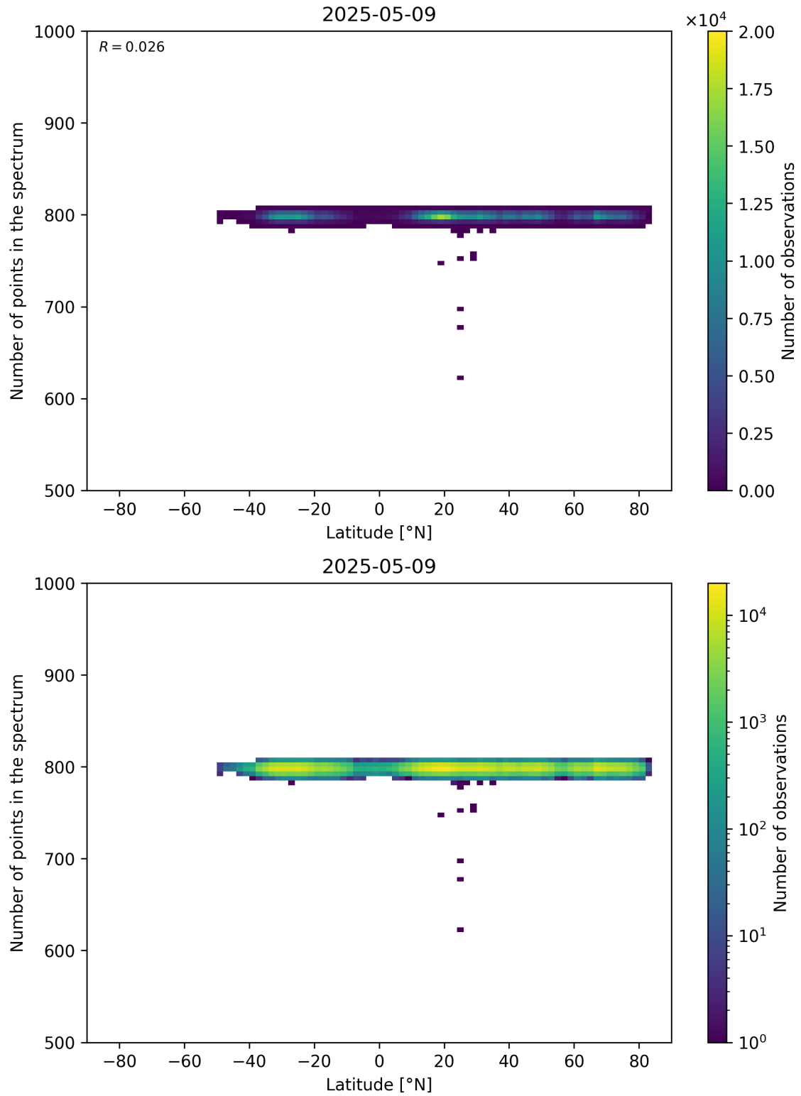
Figure 61: Scatter density plot of “Latitude” against “Number of points in the spectrum” for 2025-05-08 to 2025-05-10.
