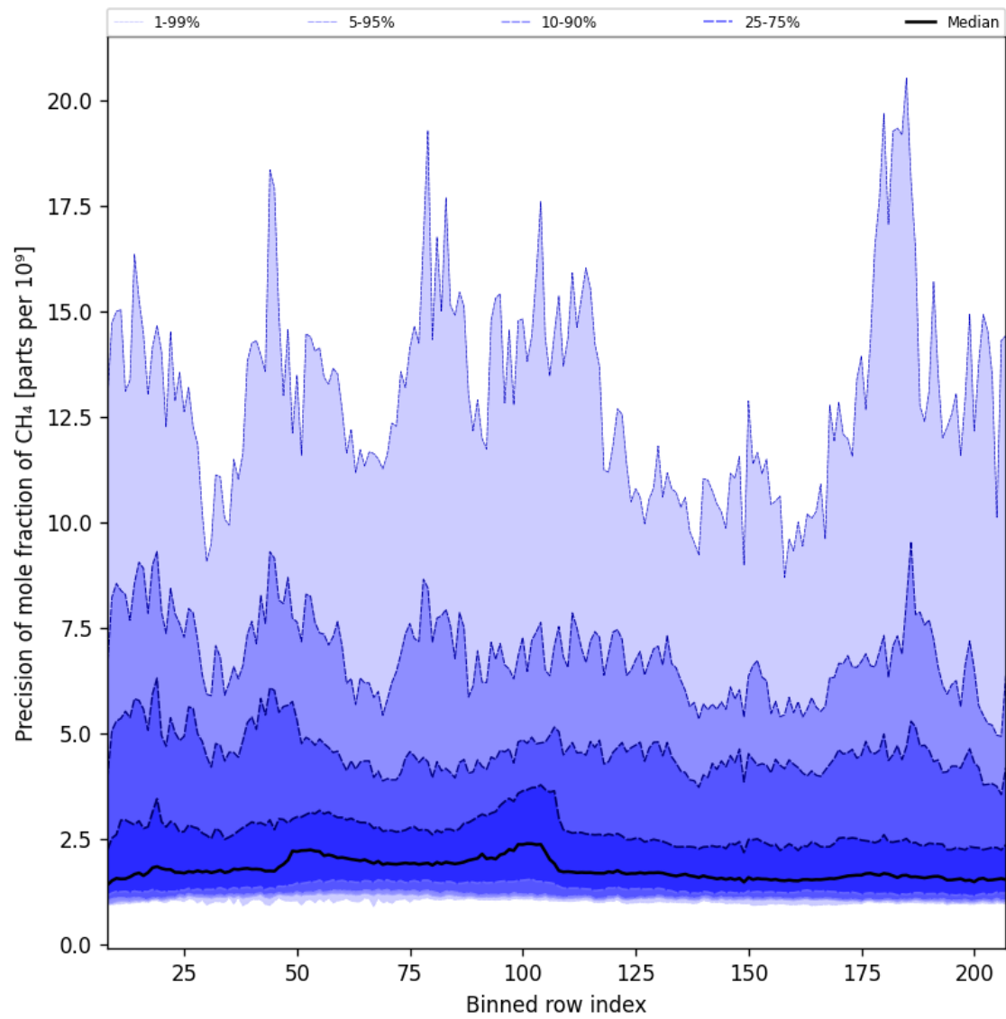
Figure 35: Along track statistics of “Precision of mole fraction of CH 4 ” for 2025-05-08 to 2025-05-10
