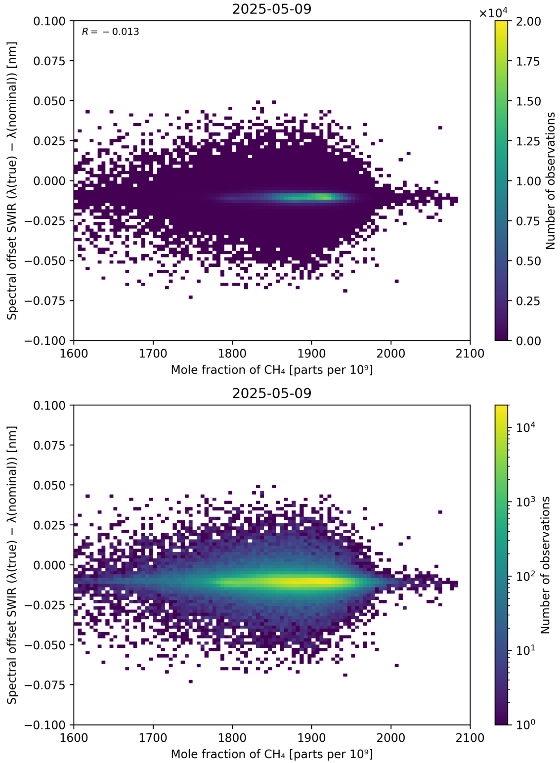
Figure 86: Scatter density plot of “Mole fraction of CH 4 ” against “Spectral offset SWIR ( \lambda_{\text{true}} - \lambda_{\text{nominal}} )” for 2025-05-08 to 2025-05-10.
