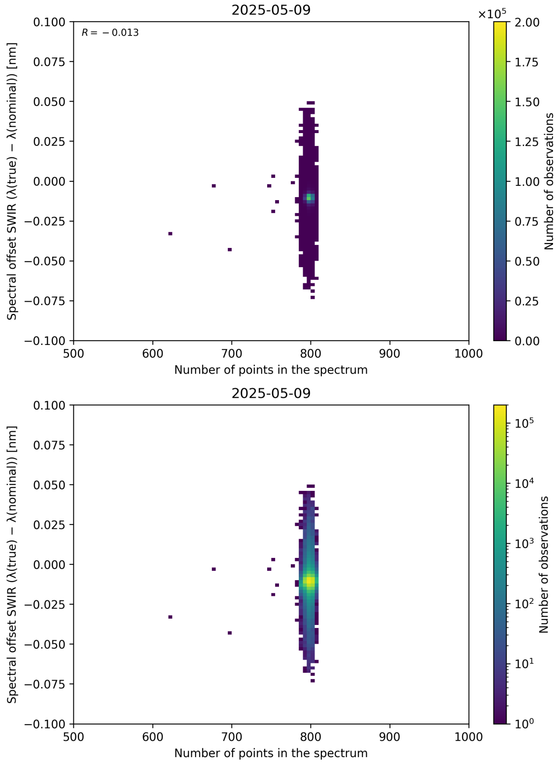
Figure 93: Scatter density plot of “Number of points in the spectrum” against “Spectral offset SWIR ( \lambda_{\text{true}} - \lambda_{\text{nominal}} )” for 2025-05-08 to 2025-05-10.
