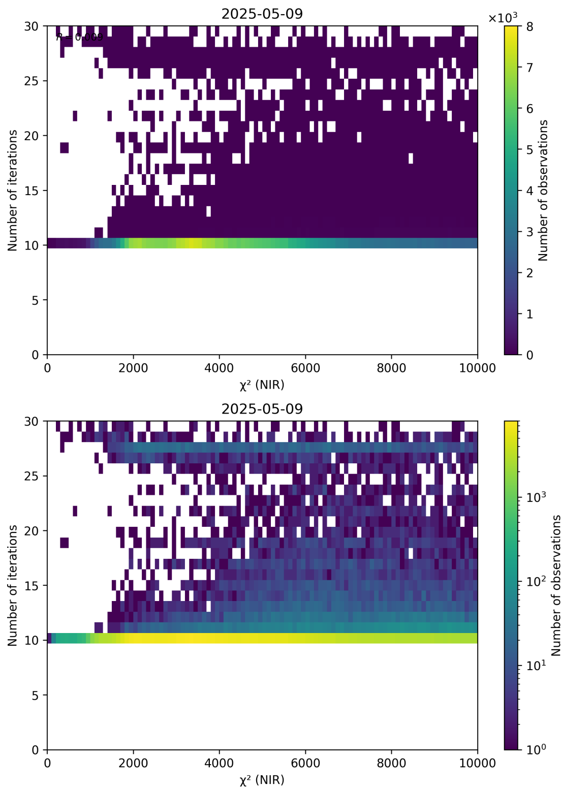
Figure 46: Scatter density plot of “ \chi^2 (NIR)” against “Number of iterations” for 2025-05-08 to 2025-05-10.
