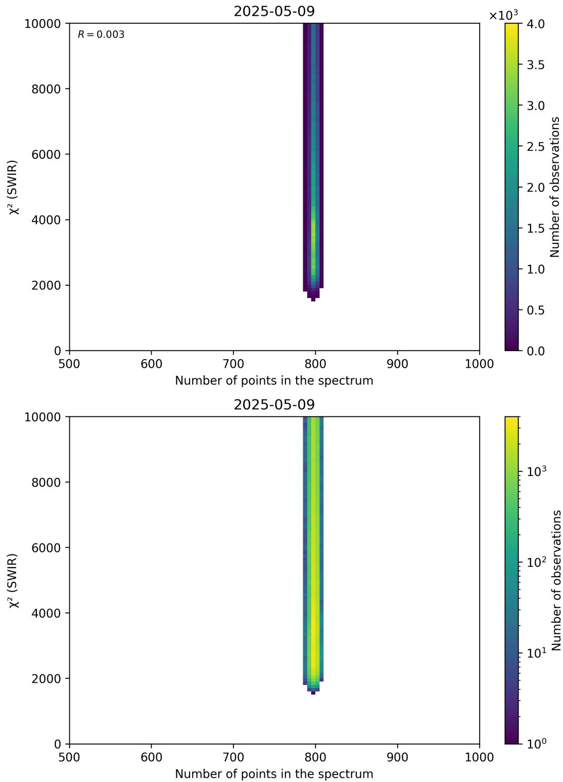
Figure 89: Scatter density plot of “Number of points in the spectrum” against “ \chi^2 (SWIR)” for 2025-05-08 to 2025-05-10.
