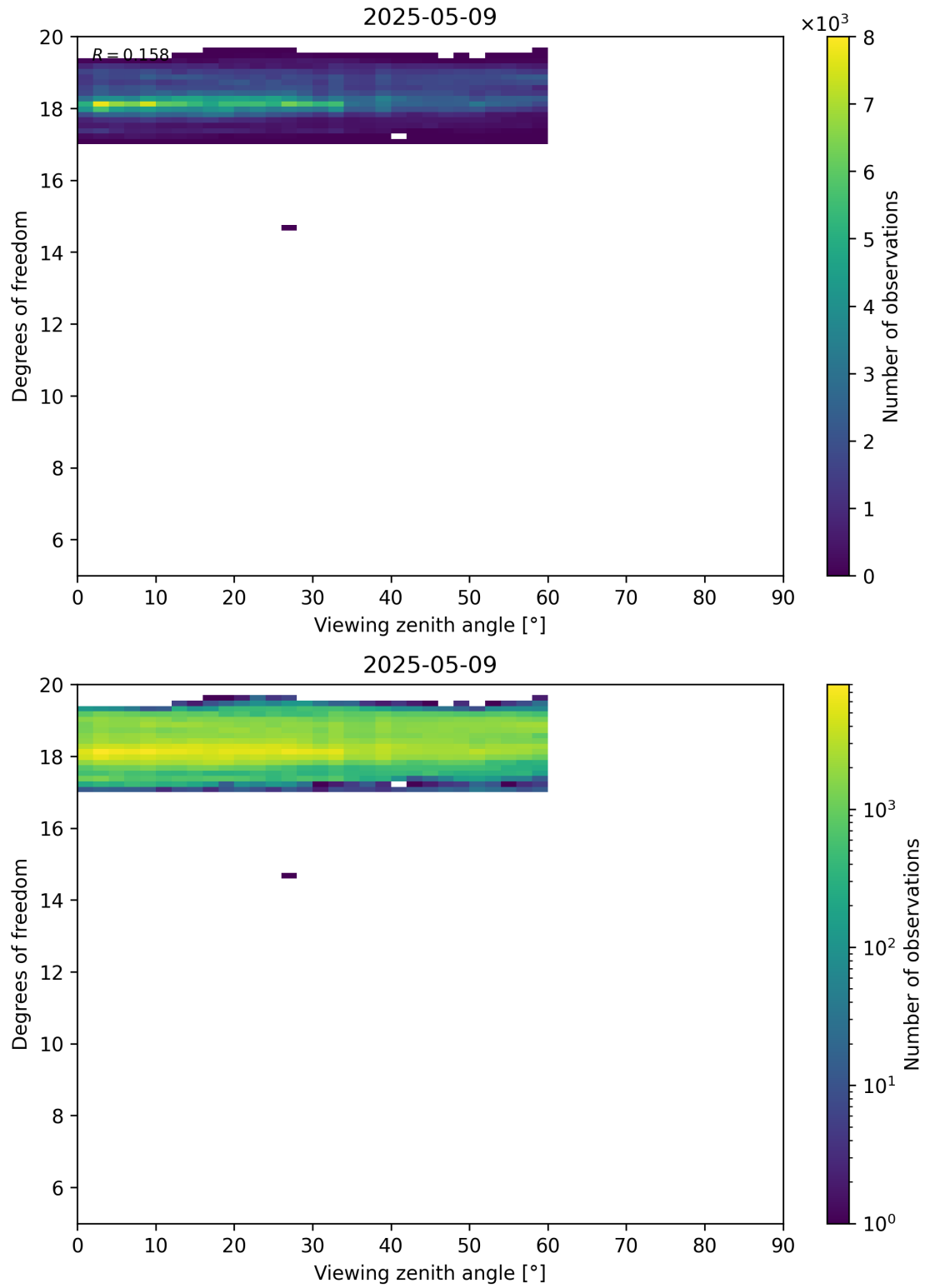
Figure 107: Scatter density plot of “Viewing zenith angle” against “Degrees of freedom” for 2025-05-08 to 2025-05-10.
