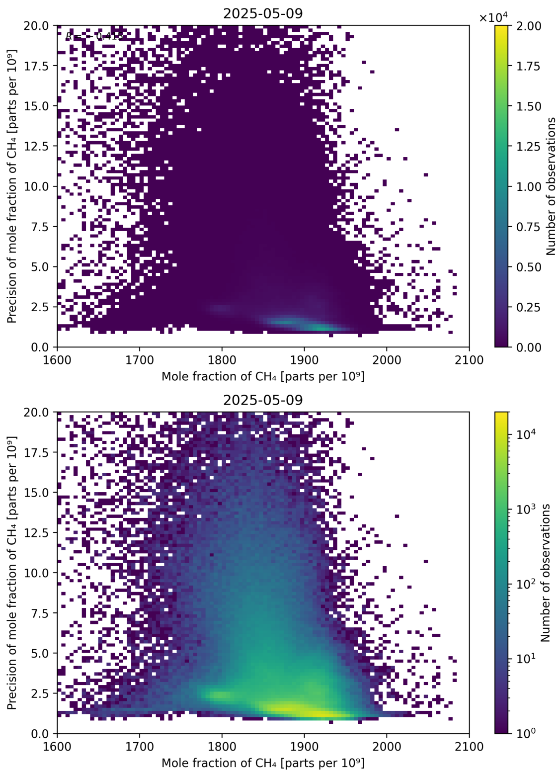
Figure 75: Scatter density plot of “Mole fraction of CH 4 ” against “Precision of mole fraction of CH 4 ” for 2025-05-08 to 2025-05-10.
