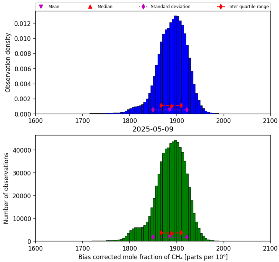
Figure 25: Histogram of “Bias corrected mole fraction of CH 4 ” for 2025-05-08 to 2025-05-10
