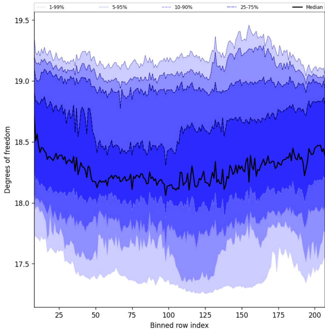
Figure 41: Along track statistics of “Degrees of freedom” for 2025-05-08 to 2025-05-10
