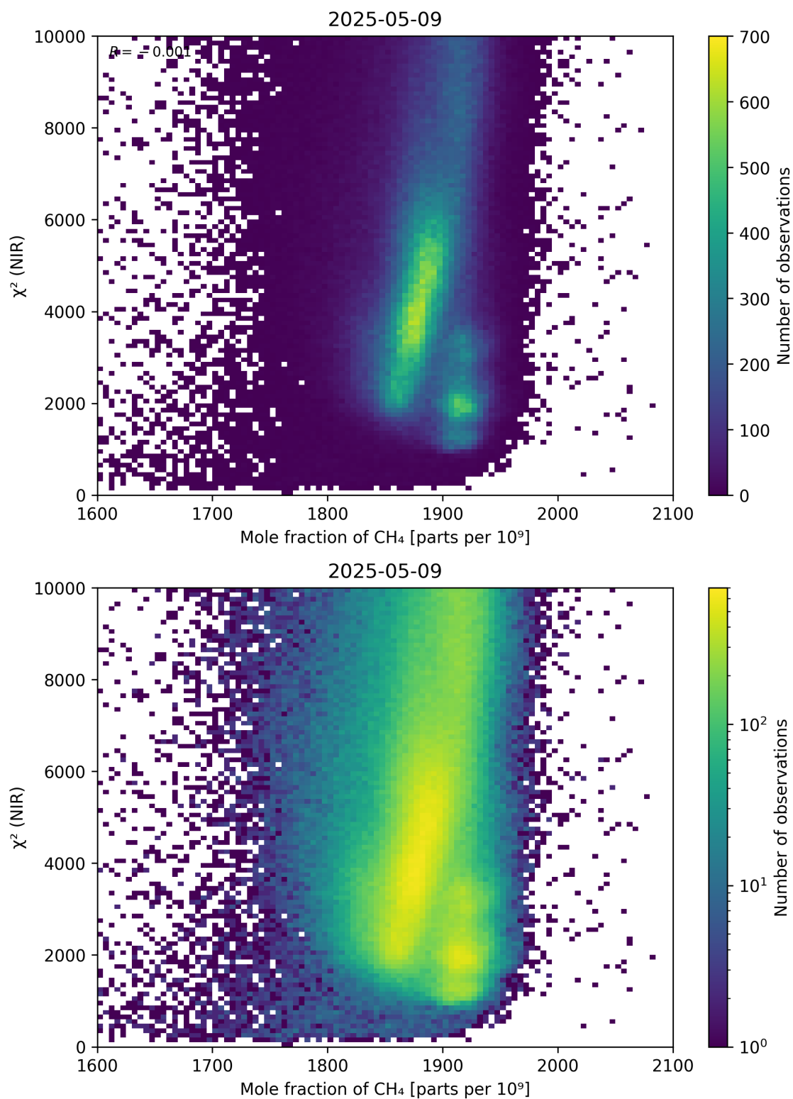
Figure 70: Scatter density plot of “Mole fraction of \text{CH}_4 ” against “ \chi^2 (NIR)” for 2025-05-08 to 2025-05-10.
