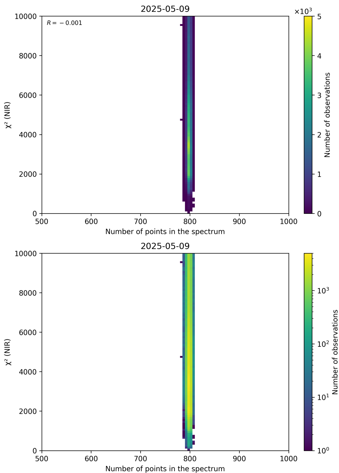
Figure 88: Scatter density plot of “Number of points in the spectrum” against “ \chi^2 (NIR)” for 2025-05-08 to 2025-05-10.
