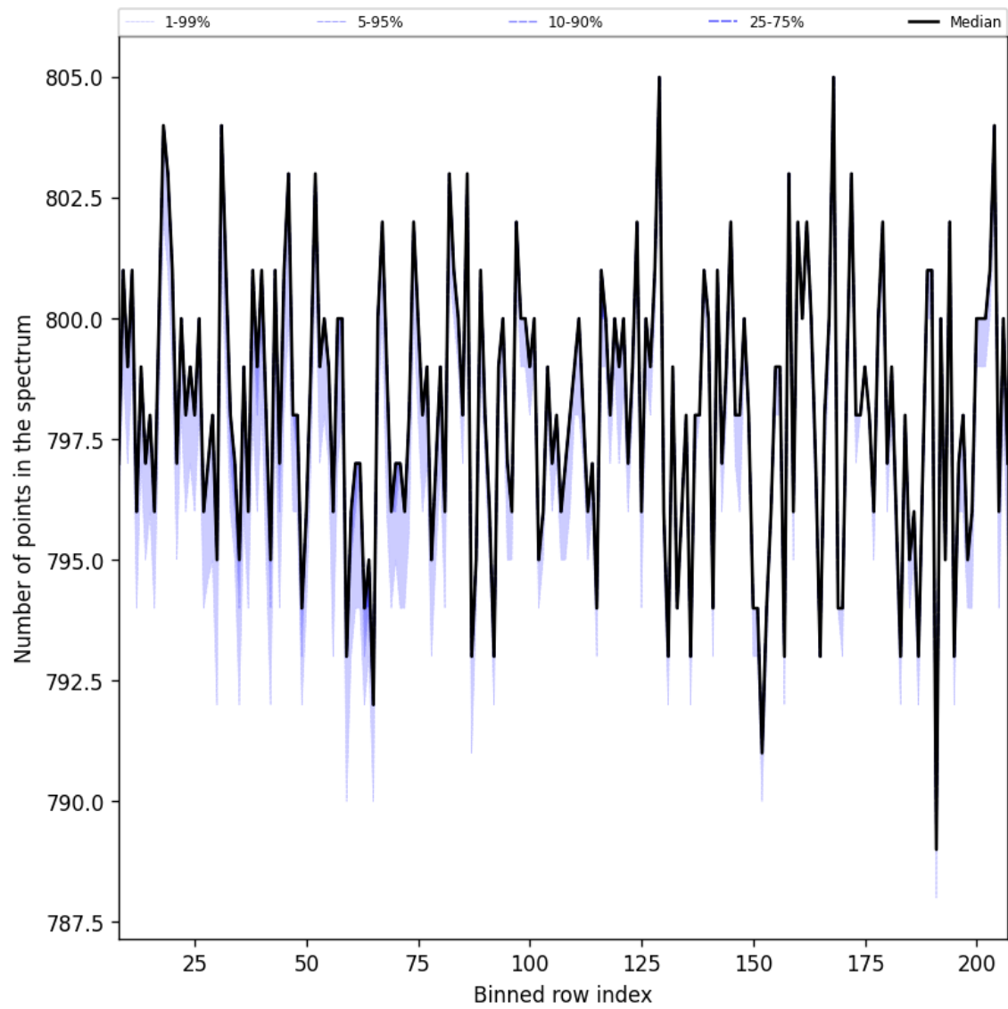
Figure 37: Along track statistics of “Number of points in the spectrum” for 2025-05-08 to 2025-05-10
