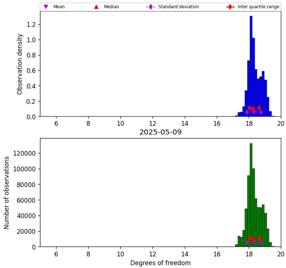
Figure 30: Histogram of “Degrees of freedom” for 2025-05-08 to 2025-05-10
