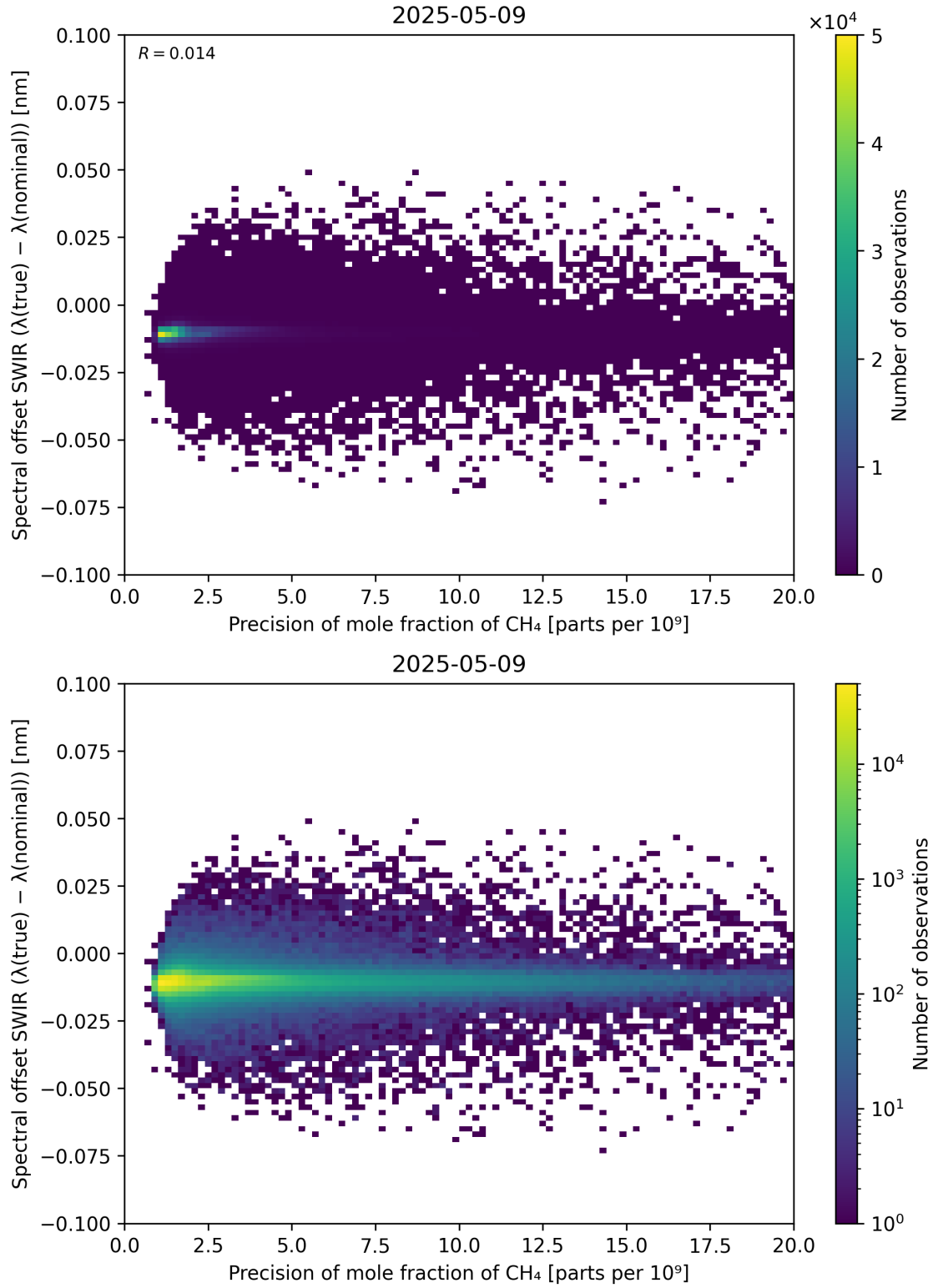
Figure 85: Scatter density plot of “Precision of mole fraction of CH 4 ” against “Spectral offset SWIR ( \lambda_{\text{true}} - \lambda_{\text{nominal}} )” for 2025-05-08 to 2025-05-10.
