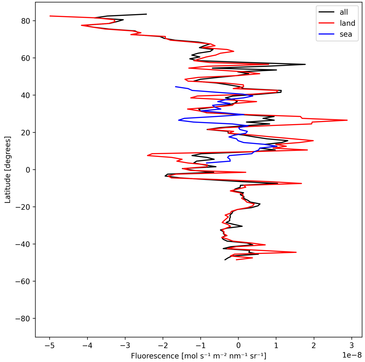
Figure 21: Zonal average of “Fluorescence” for 2025-05-08 to 2025-05-10.
