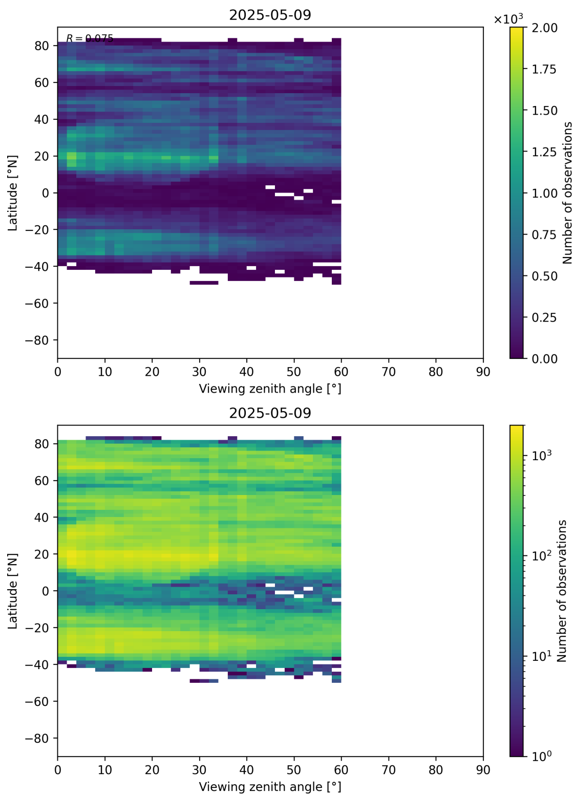
Figure 109: Scatter density plot of “Viewing zenith angle” against “Latitude” for 2025-05-08 to 2025-05-10.
