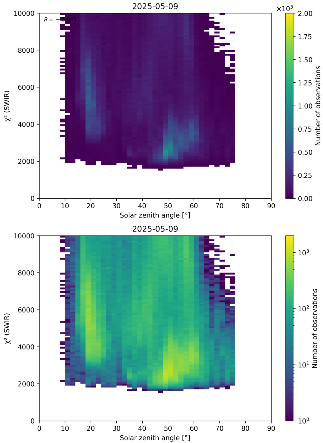
Figure 95: Scatter density plot of “Solar zenith angle” against “ \chi^2 (SWIR)” for 2025-05-08 to 2025-05-10.
