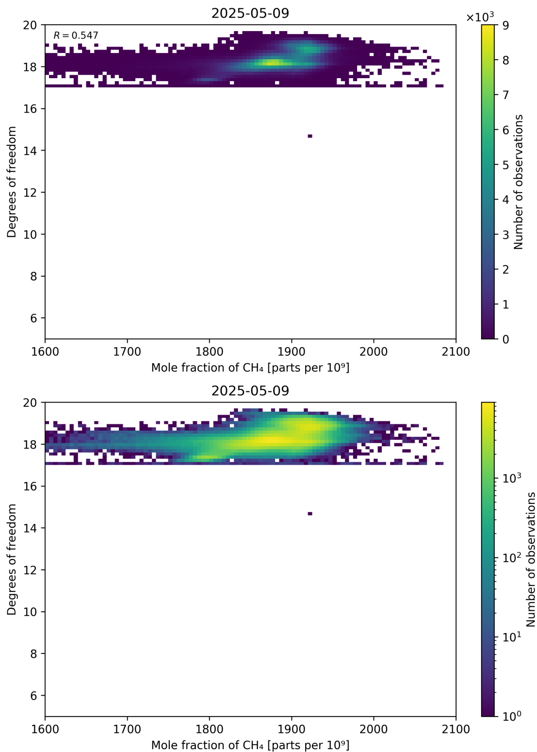
Figure 72: Scatter density plot of “Mole fraction of CH 4 ” against “Degrees of freedom” for 2025-05-08 to 2025-05-10.
