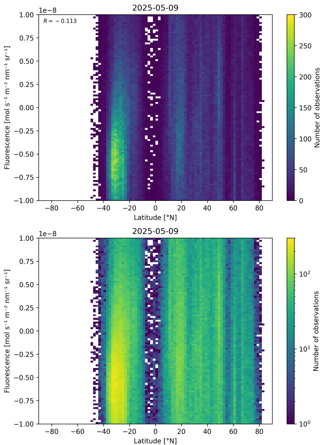
Figure 56: Scatter density plot of “Latitude” against “Fluorescence” for 2025-05-08 to 2025-05-10.
