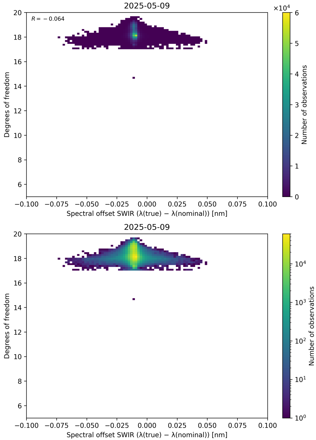
Figure 119: Scatter density plot of “Spectral offset SWIR ( \lambda_{\text{true}} - \lambda_{\text{nominal}} )” against “Degrees of freedom” for 2025-05-08 to 2025-05-10.
