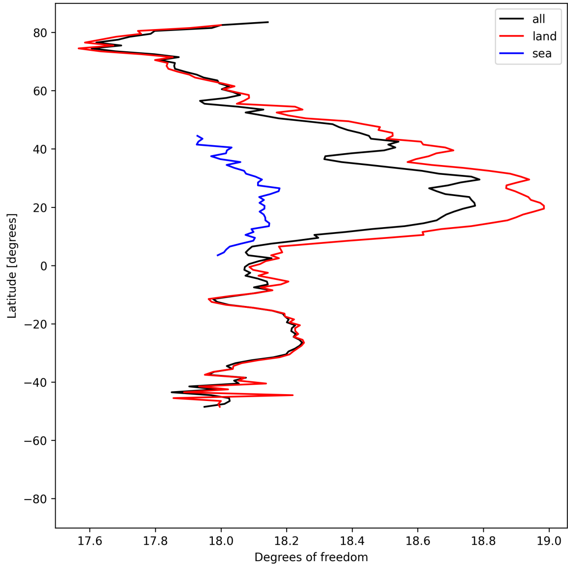
Figure 19: Zonal average of “Degrees of freedom” for 2025-05-08 to 2025-05-10.
