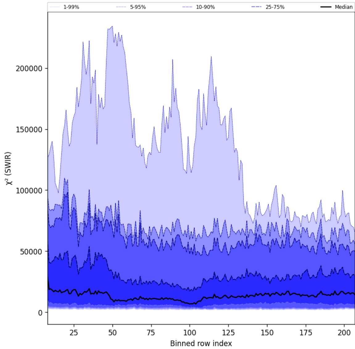
Figure 39: Along track statistics of “ \chi^2 (SWIR)” for 2025-05-08 to 2025-05-10
