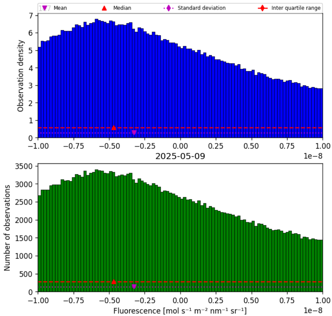
Figure 32: Histogram of “Fluorescence” for 2025-05-08 to 2025-05-10
