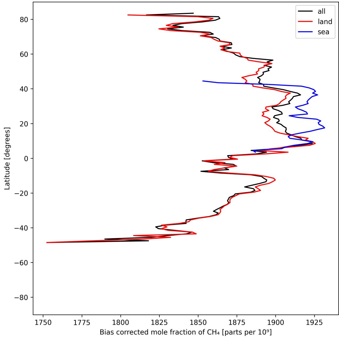
Figure 14: Zonal average of “Bias corrected mole fraction of \text{CH}_4 ” for 2025-05-08 to 2025-05-10.
