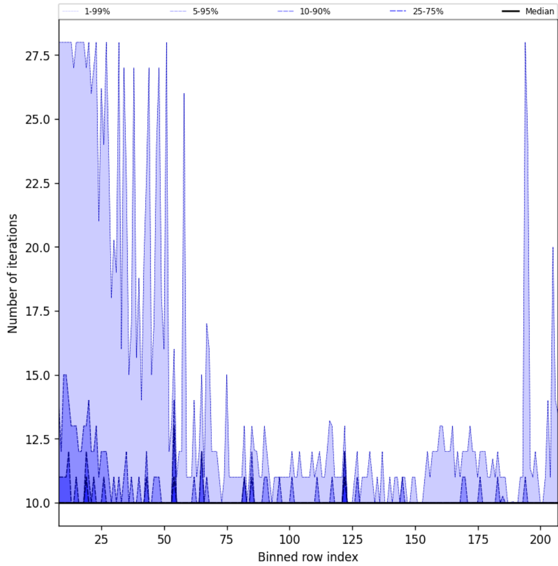
Figure 42: Along track statistics of “Number of iterations” for 2025-05-08 to 2025-05-10
