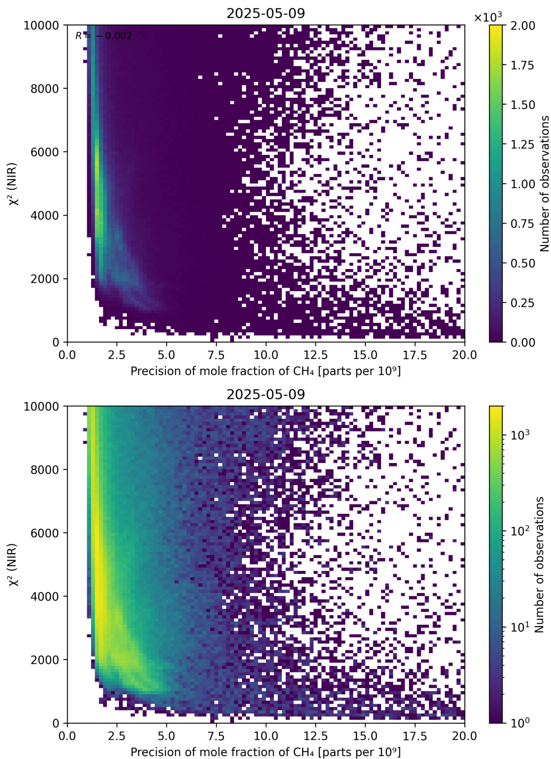
Figure 78: Scatter density plot of “Precision of mole fraction of \text{CH}_4 ” against “ \chi^2 (NIR)” for 2025-05-08 to 2025-05-10.
