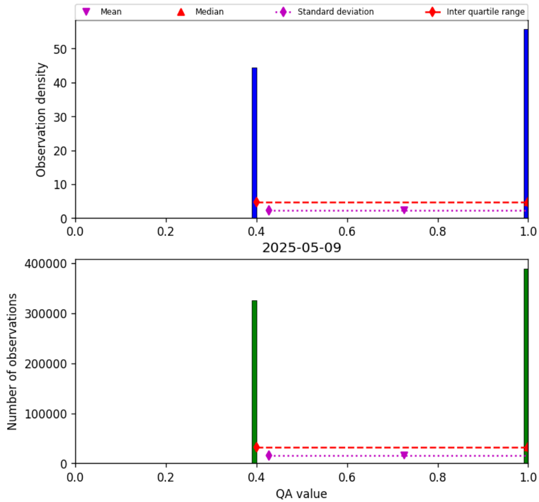
Figure 22: Histogram of “QA value” for 2025-05-08 to 2025-05-10
