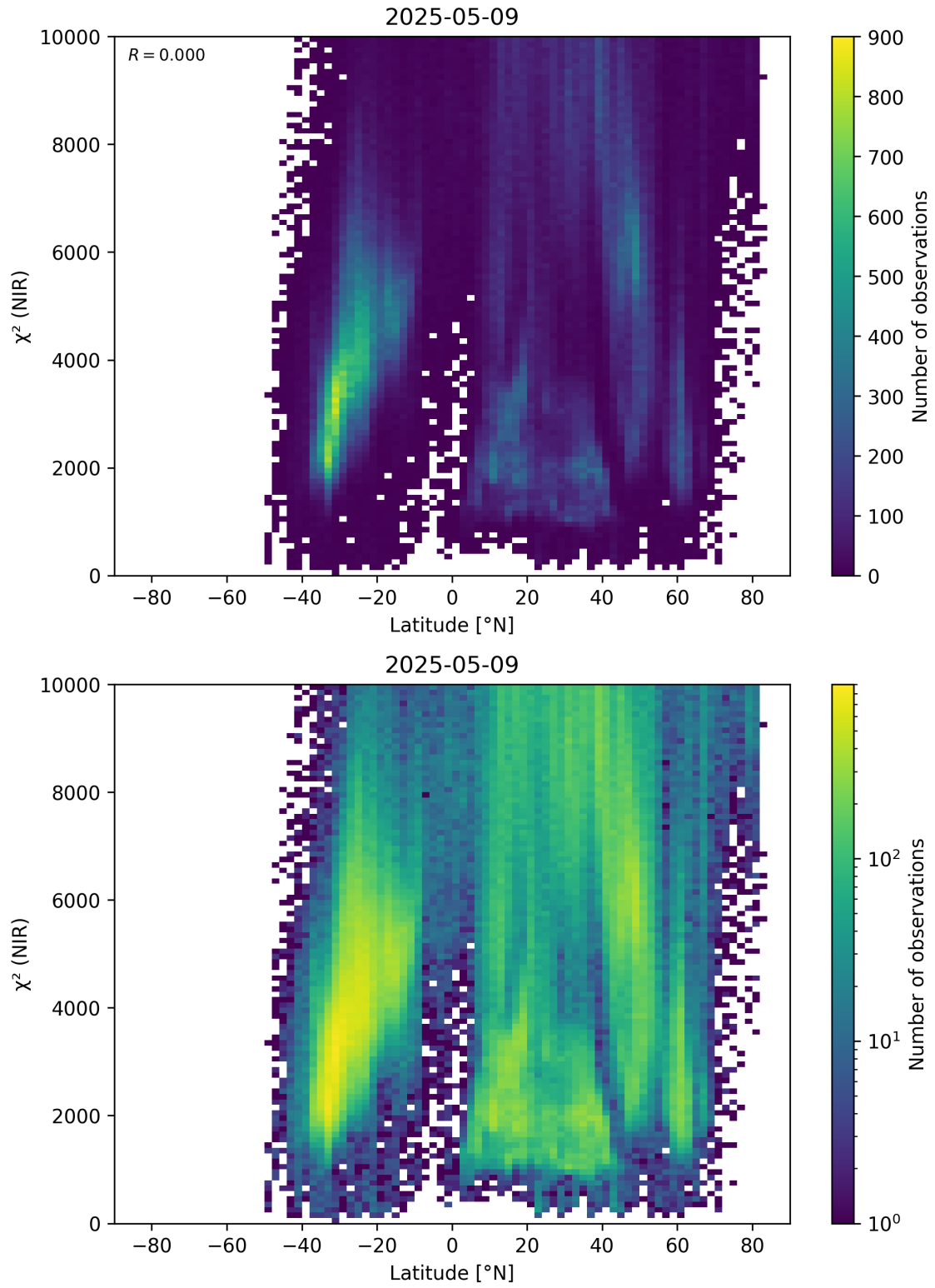
Figure 53: Scatter density plot of “Latitude” against “ \chi^2 (NIR)” for 2025-05-08 to 2025-05-10.
