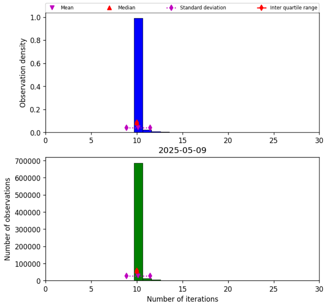
Figure 31: Histogram of "Number of iterations" for 2025-05-08 to 2025-05-10
