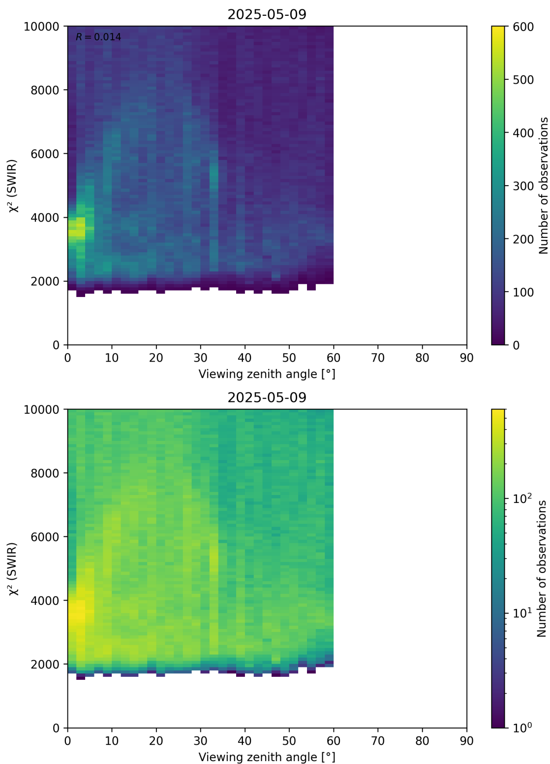
Figure 106: Scatter density plot of “Viewing zenith angle” against “ \chi^2 (SWIR)” for 2025-05-08 to 2025-05-10.
