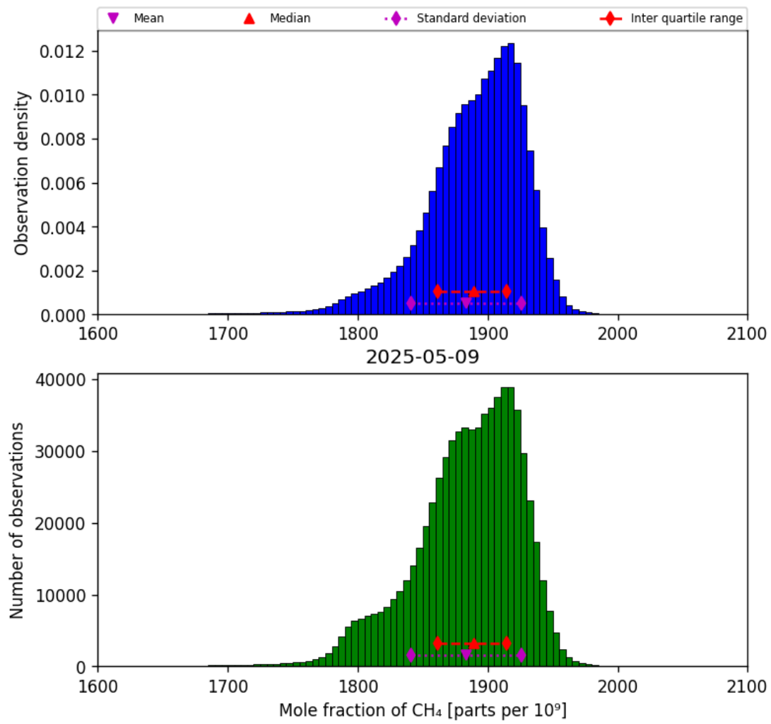
Figure 23: Histogram of “Mole fraction of CH 4 ” for 2025-05-08 to 2025-05-10
