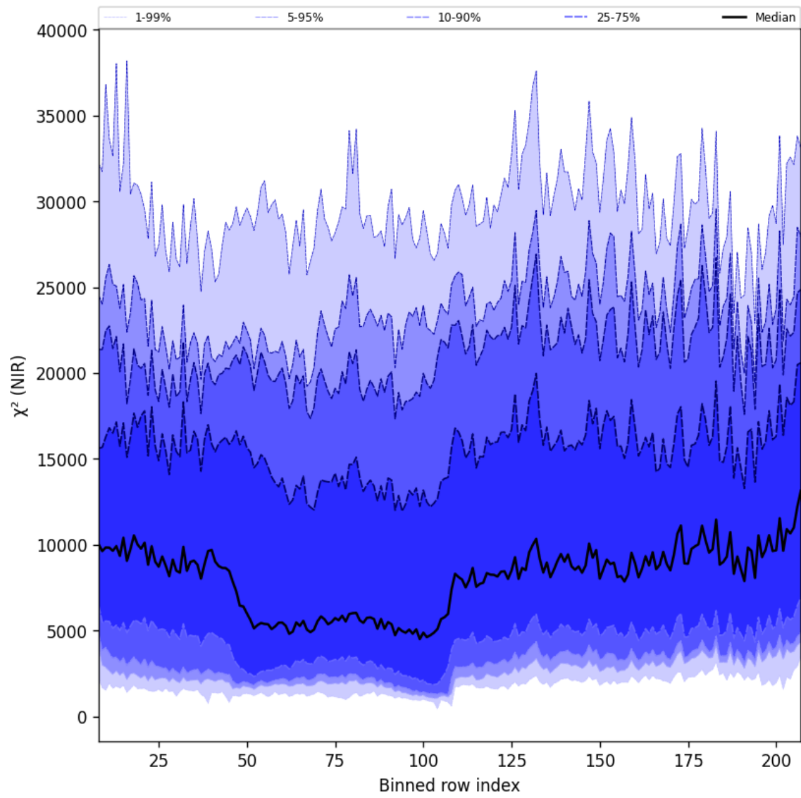
Figure 40: Along track statistics of “ \chi^2 (NIR)” for 2025-05-08 to 2025-05-10
