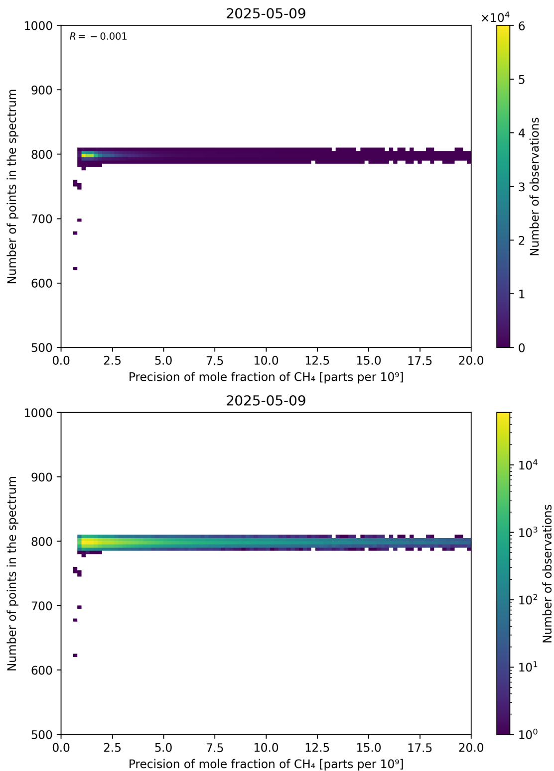
Figure 84: Scatter density plot of “Precision of mole fraction of CH 4 ” against “Number of points in the spectrum” for 2025-05-08 to 2025-05-10.
