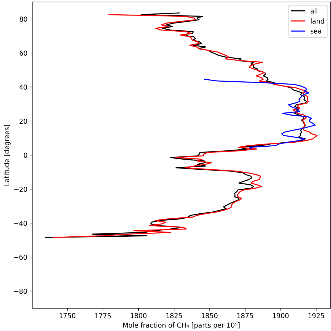
Figure 12: Zonal average of “Mole fraction of \text{CH}_4 ” for 2025-05-08 to 2025-05-10.
