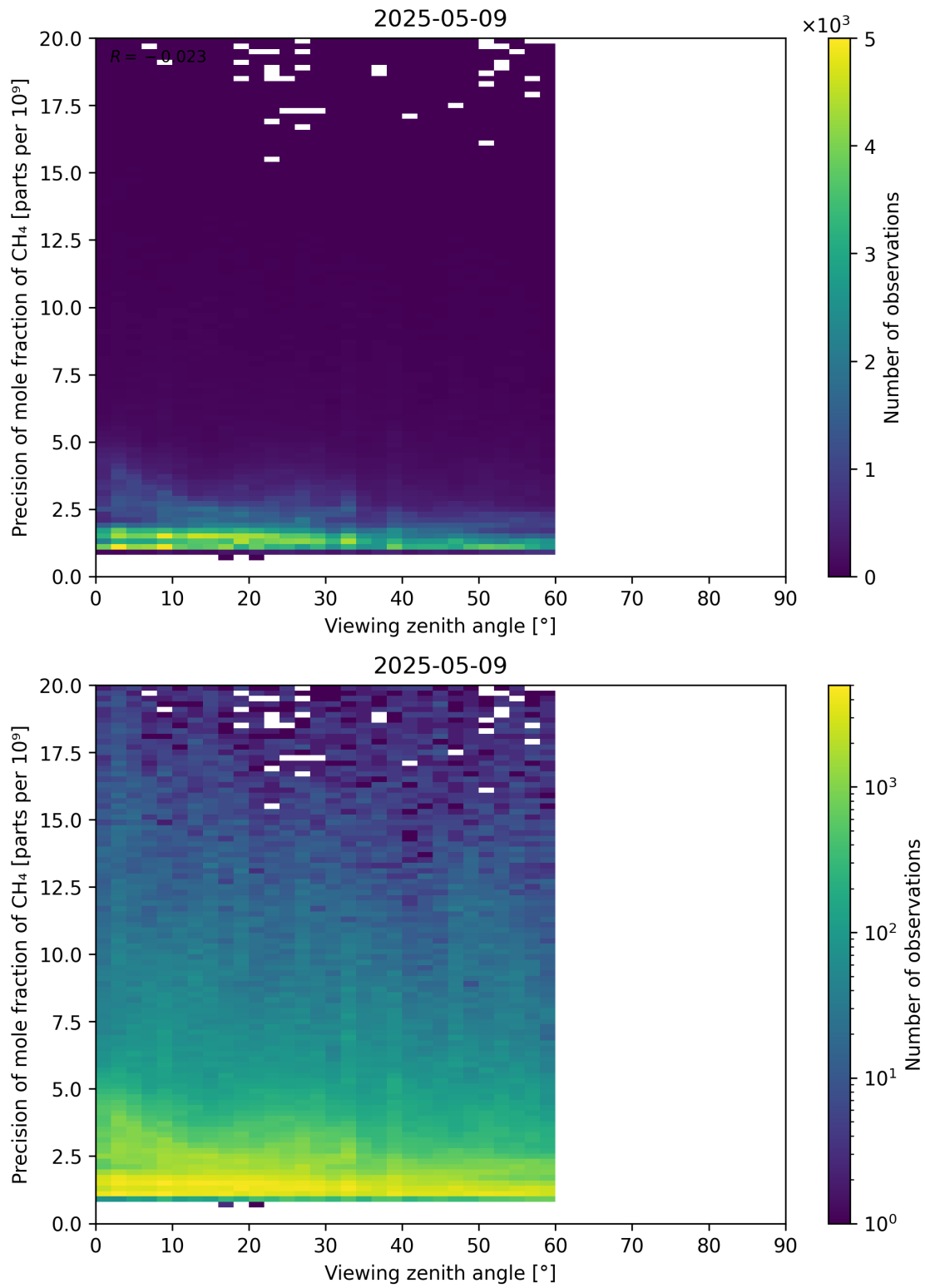
Figure 112: Scatter density plot of “Viewing zenith angle” against “Precision of mole fraction of CH 4 ” for 2025-05-08 to 2025-05-10.
