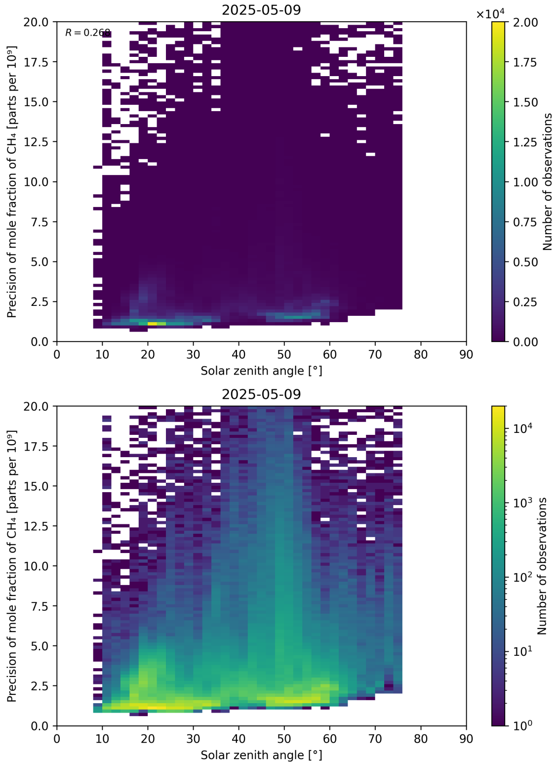
Figure 101: Scatter density plot of “Solar zenith angle” against “Precision of mole fraction of CH 4 ” for 2025-05-08 to 2025-05-10.
