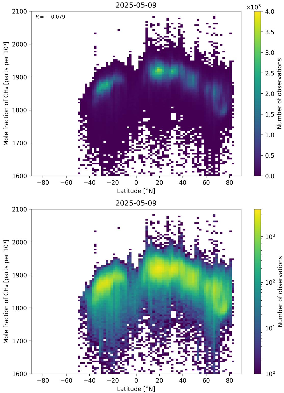
Figure 57: Scatter density plot of “Latitude” against “Mole fraction of CH 4 ” for 2025-05-08 to 2025-05-10.
