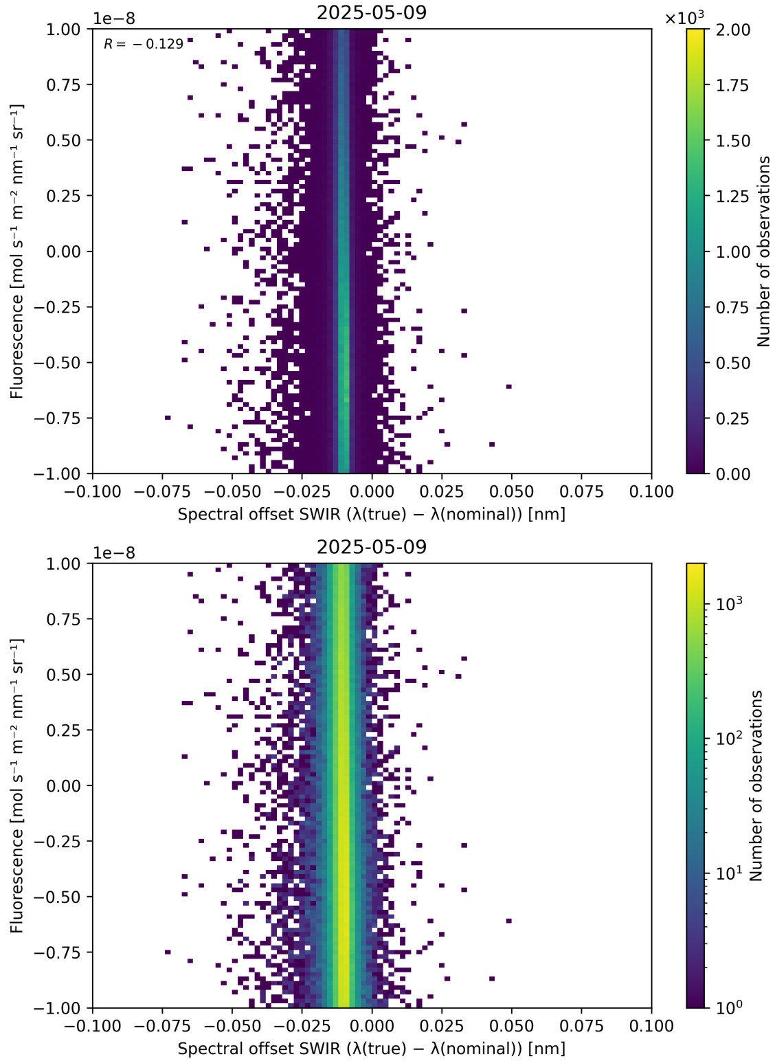
Figure 120: Scatter density plot of “Spectral offset SWIR ( \lambda_{\text{true}} - \lambda_{\text{nominal}} )” against “Fluorescence” for 2025-05-08 to 2025-05-10.
