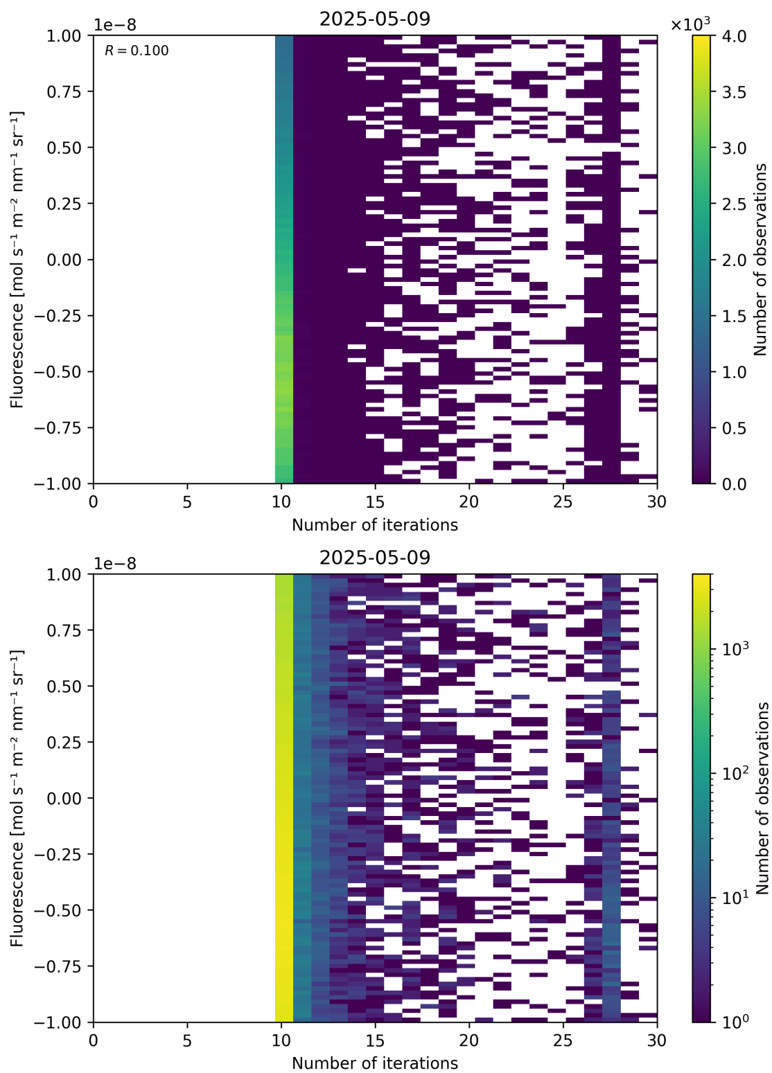
Figure 87: Scatter density plot of “Number of iterations” against “Fluorescence” for 2025-05-08 to 2025-05-10.
