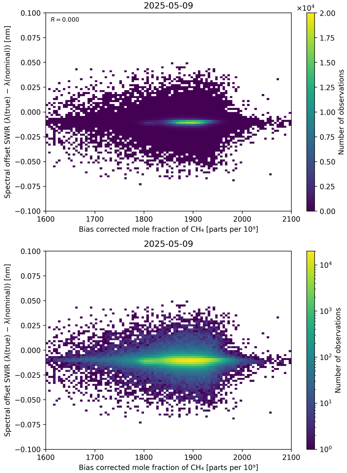
Figure 69: Scatter density plot of “Bias corrected mole fraction of \text{CH}_4 ” against “Spectral offset SWIR ( \lambda_{\text{true}} - \lambda_{\text{nominal}} )” for 2025-05-08 to 2025-05-10.
