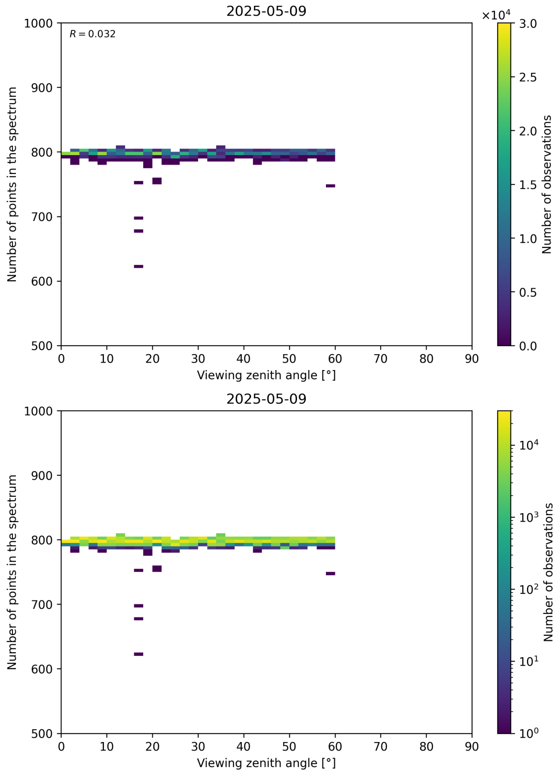
Figure 114: Scatter density plot of “Viewing zenith angle” against “Number of points in the spectrum” for 2025-05-08 to 2025-05-10.
