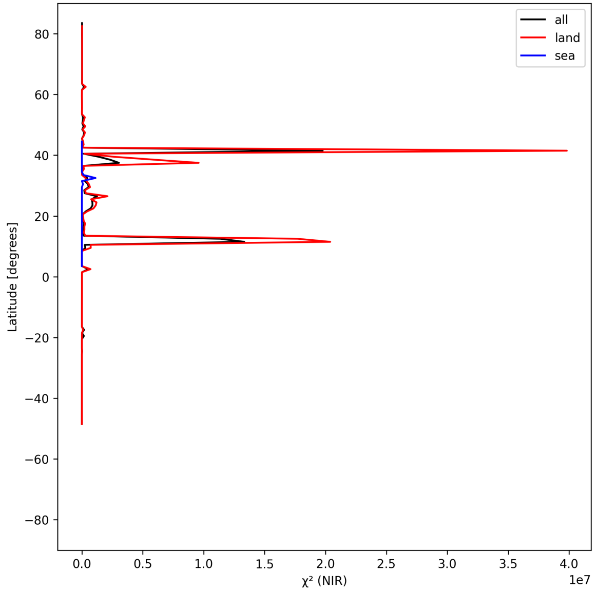
Figure 18: Zonal average of “ \chi^2 (NIR)” for 2025-05-08 to 2025-05-10.
