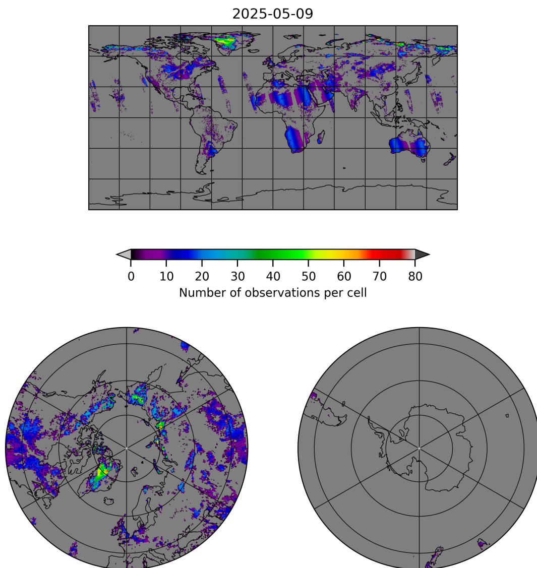
Figure 10: Map of the number of observations for 2025-05-08 to 2025-05-10
