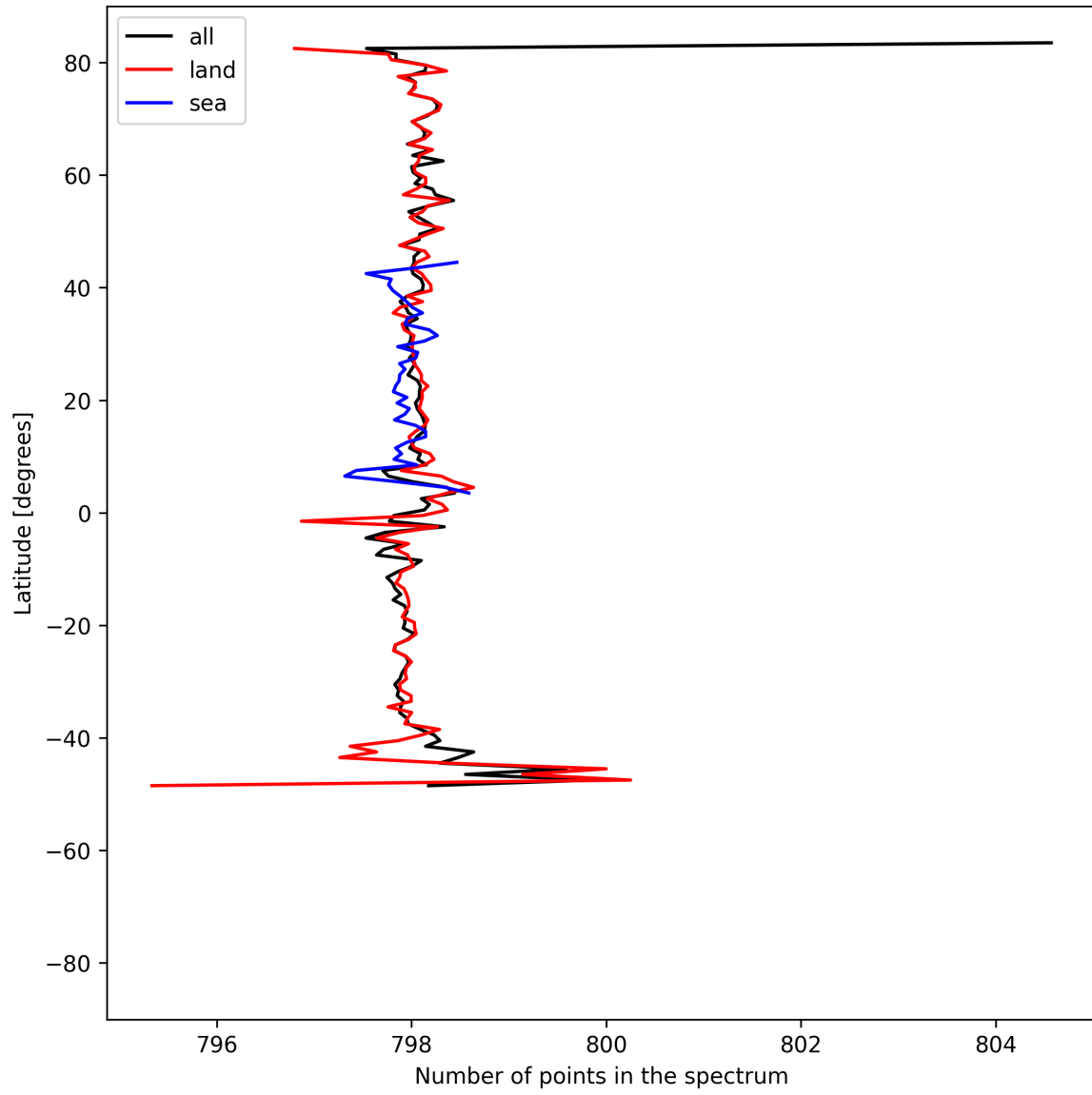
Figure 15: Zonal average of “Number of points in the spectrum” for 2025-05-08 to 2025-05-10.
