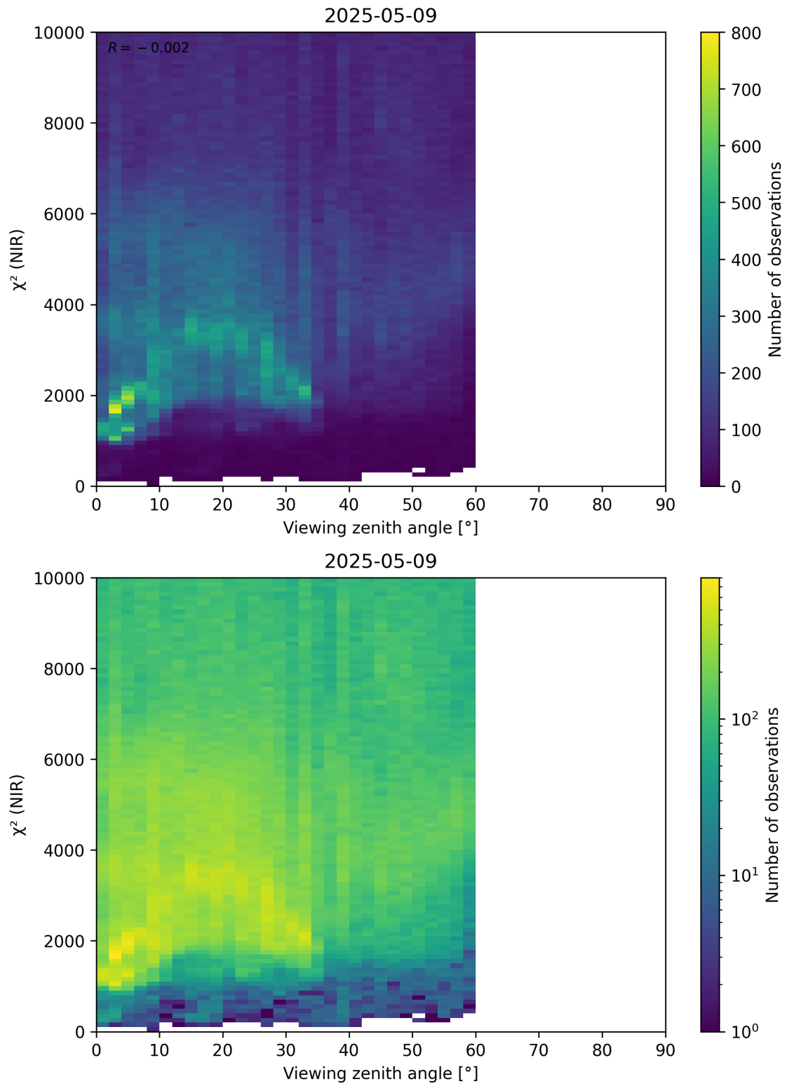
Figure 105: Scatter density plot of “Viewing zenith angle” against “ \chi^2 (NIR)” for 2025-05-08 to 2025-05-10.
