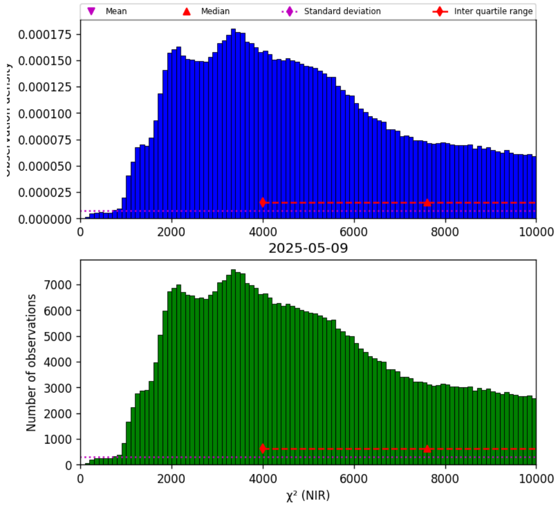
Figure 29: Histogram of “ \chi^2 (NIR)” for 2025-05-08 to 2025-05-10
