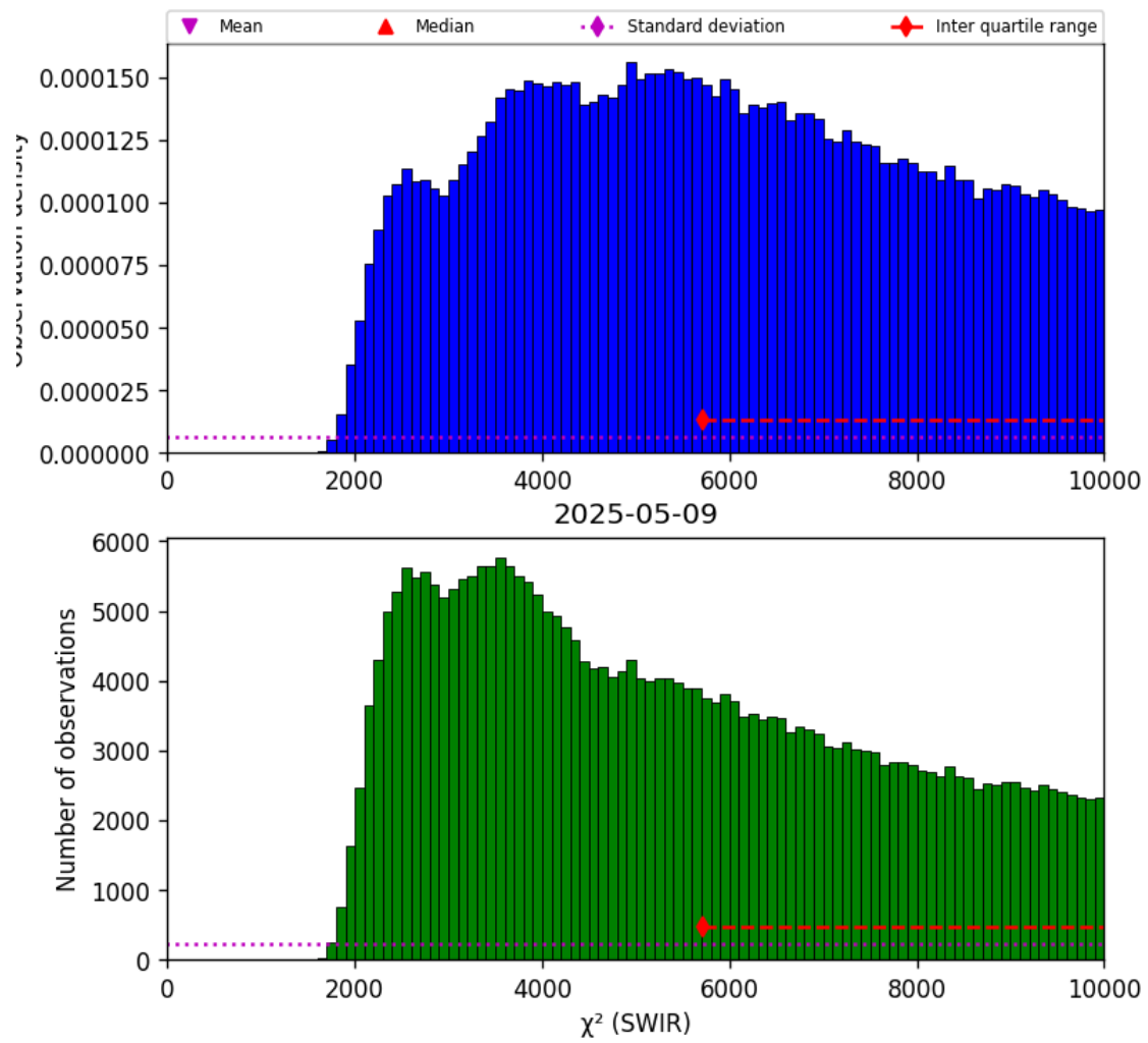
Figure 28: Histogram of “ \chi^2 (SWIR)” for 2025-05-08 to 2025-05-10
