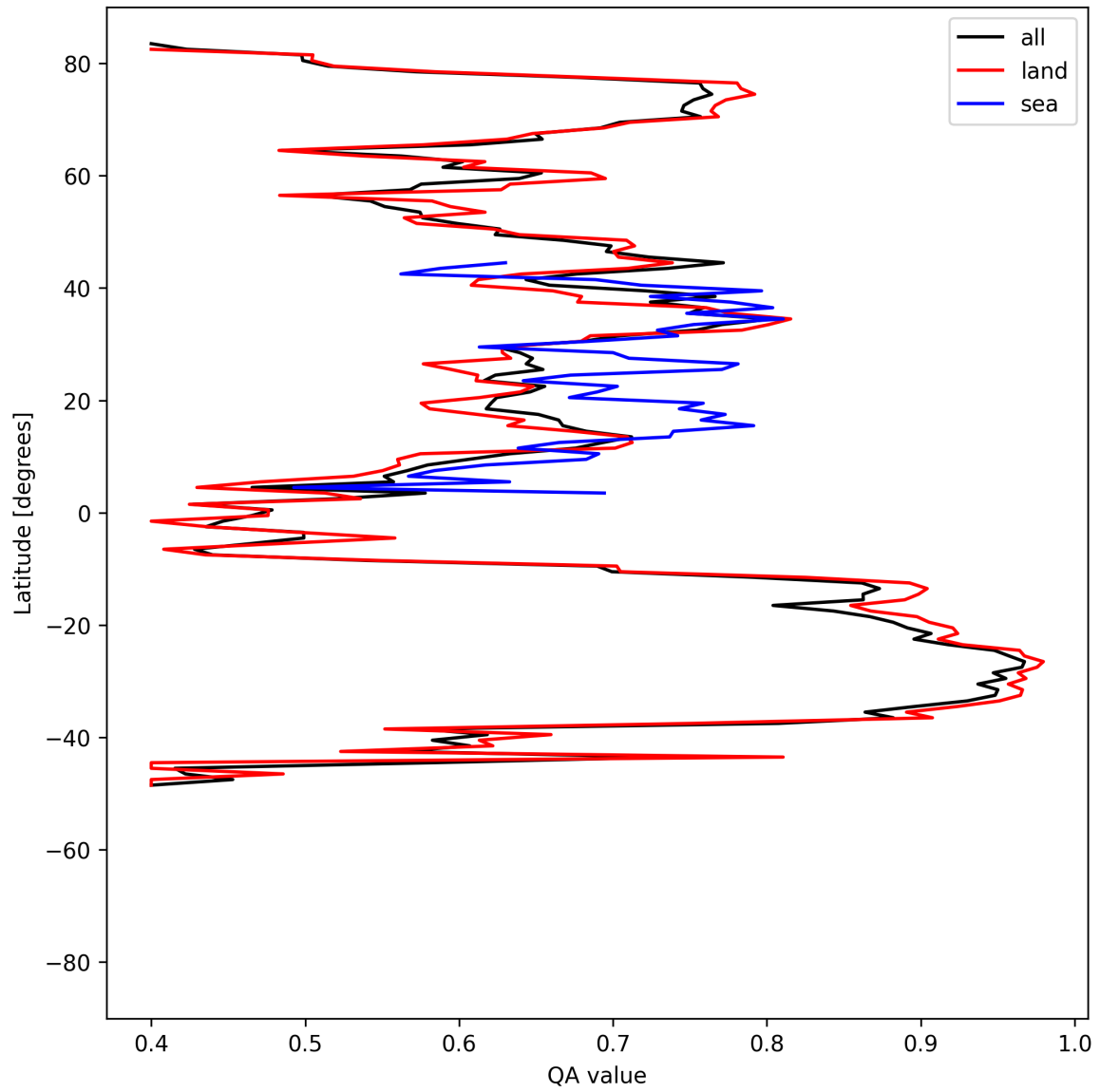
Figure 11: Zonal average of “QA value” for 2025-05-08 to 2025-05-10.
