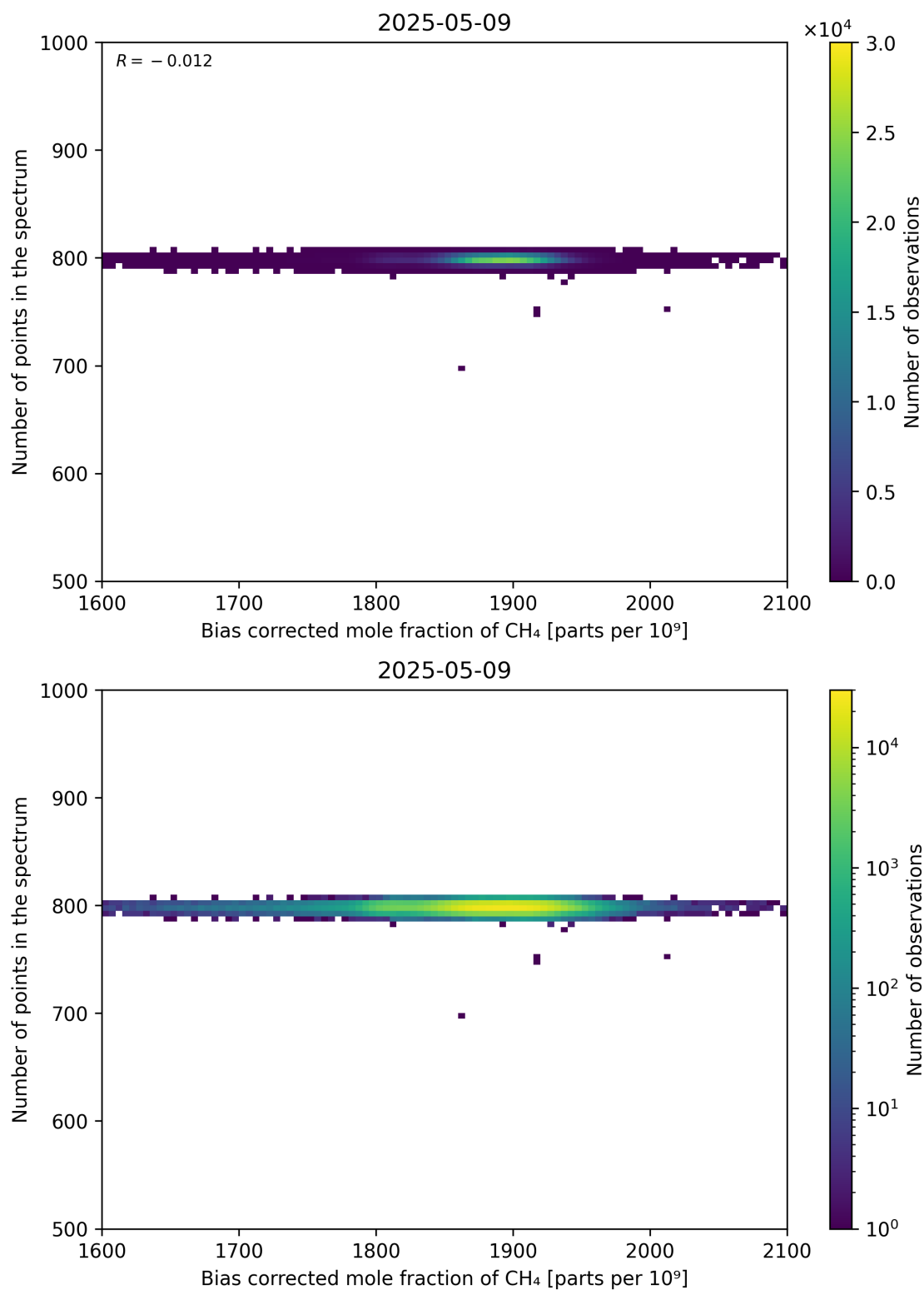
Figure 68: Scatter density plot of “Bias corrected mole fraction of CH 4 ” against “Number of points in the spectrum” for 2025-05-08 to 2025-05-10.
