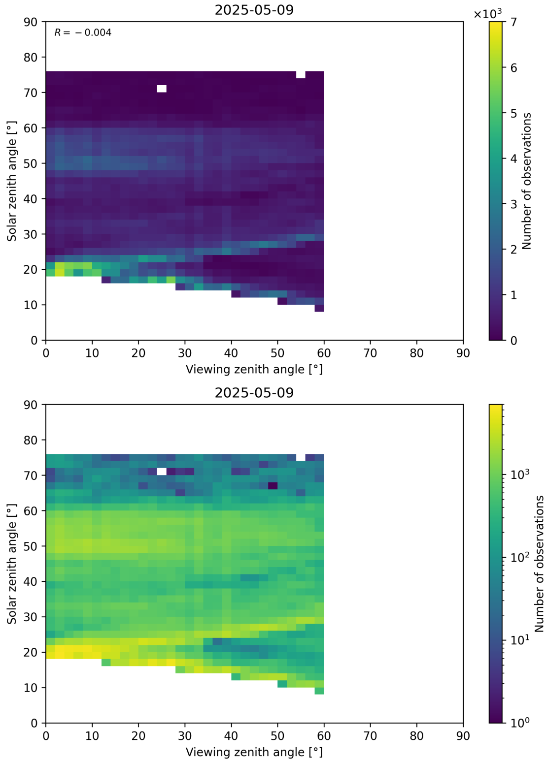
Figure 115: Scatter density plot of “Viewing zenith angle” against “Solar zenith angle” for 2025-05-08 to 2025-05-10.
