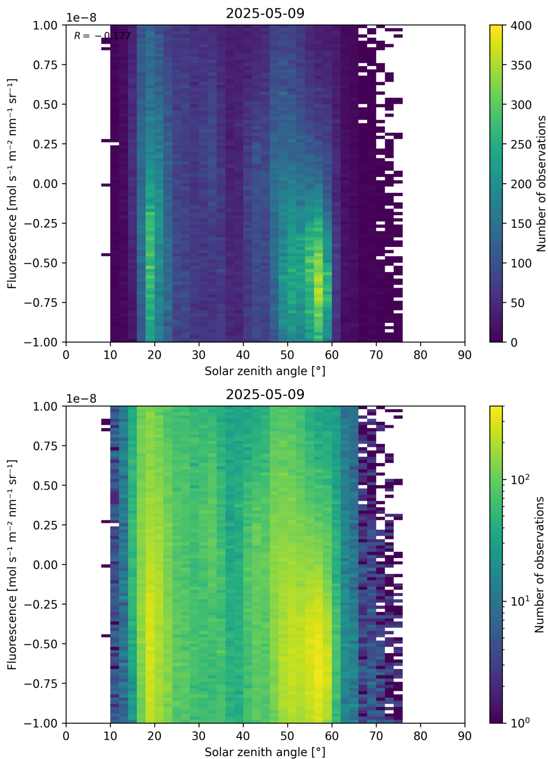
Figure 97: Scatter density plot of “Solar zenith angle” against “Fluorescence” for 2025-05-08 to 2025-05-10.
