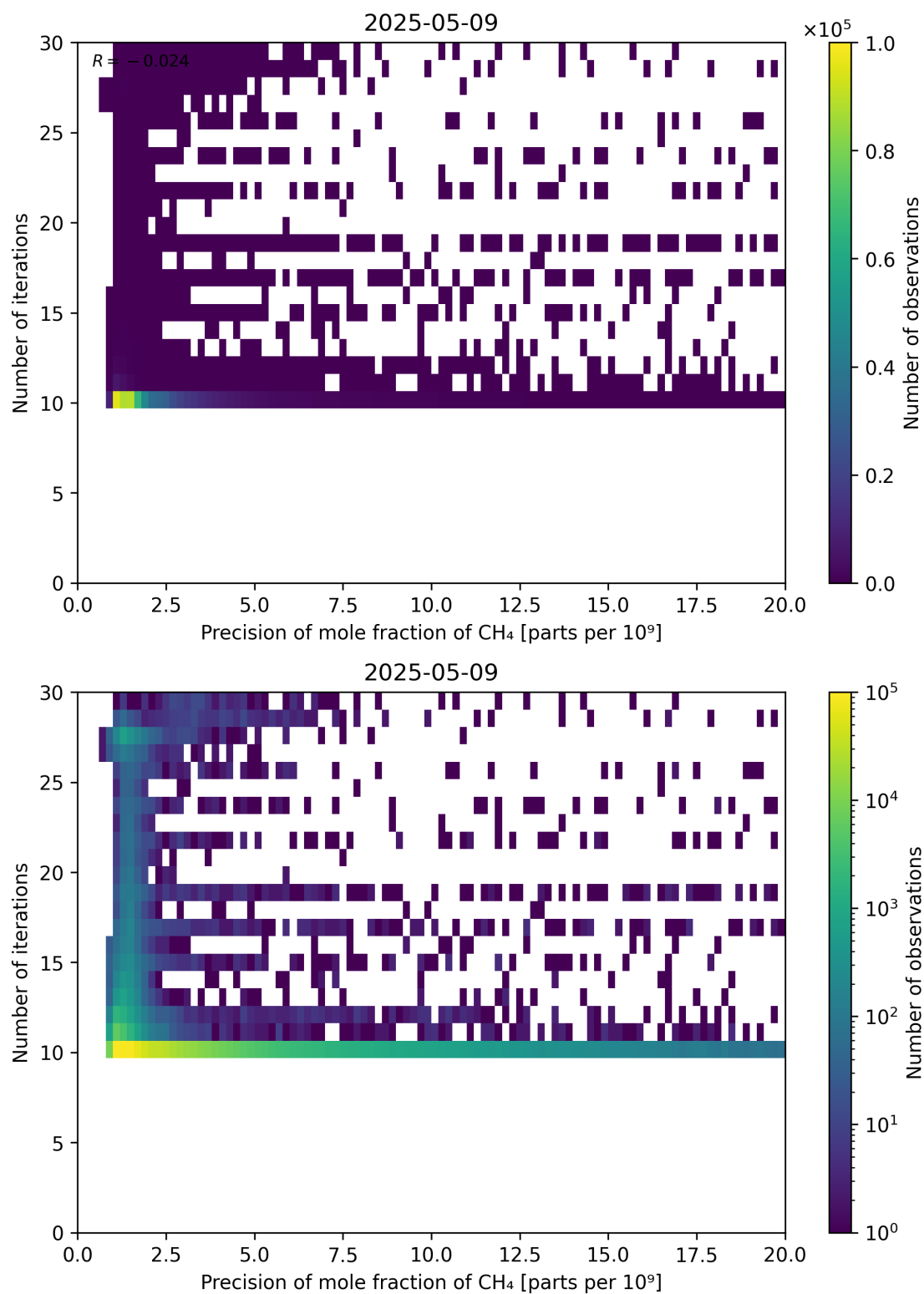
Figure 83: Scatter density plot of “Precision of mole fraction of CH 4 ” against “Number of iterations” for 2025-05-08 to 2025-05-10.
