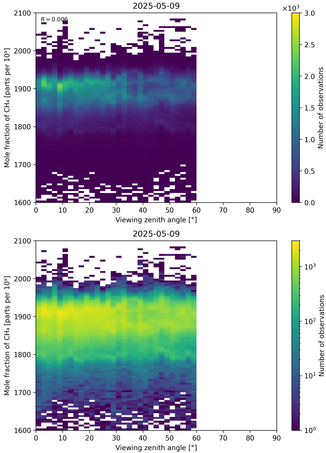
Figure 110: Scatter density plot of “Viewing zenith angle” against “Mole fraction of CH 4 ” for 2025-05-08 to 2025-05-10.
