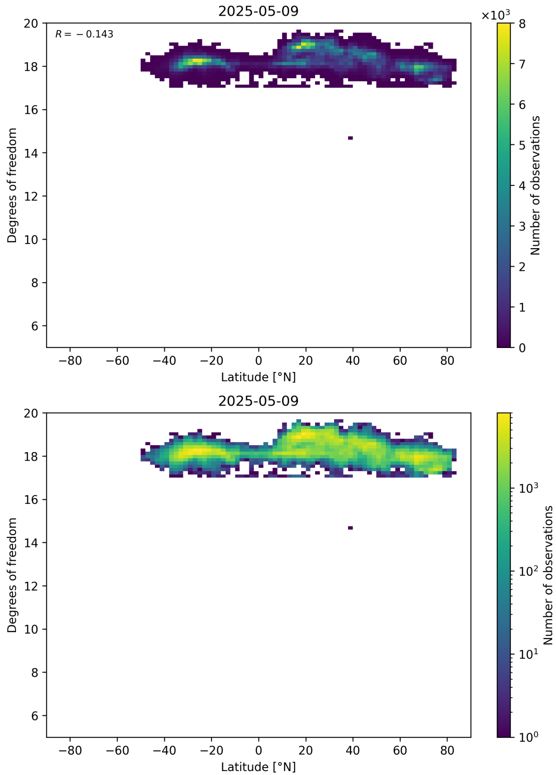
Figure 55: Scatter density plot of “Latitude” against “Degrees of freedom” for 2025-05-08 to 2025-05-10.
