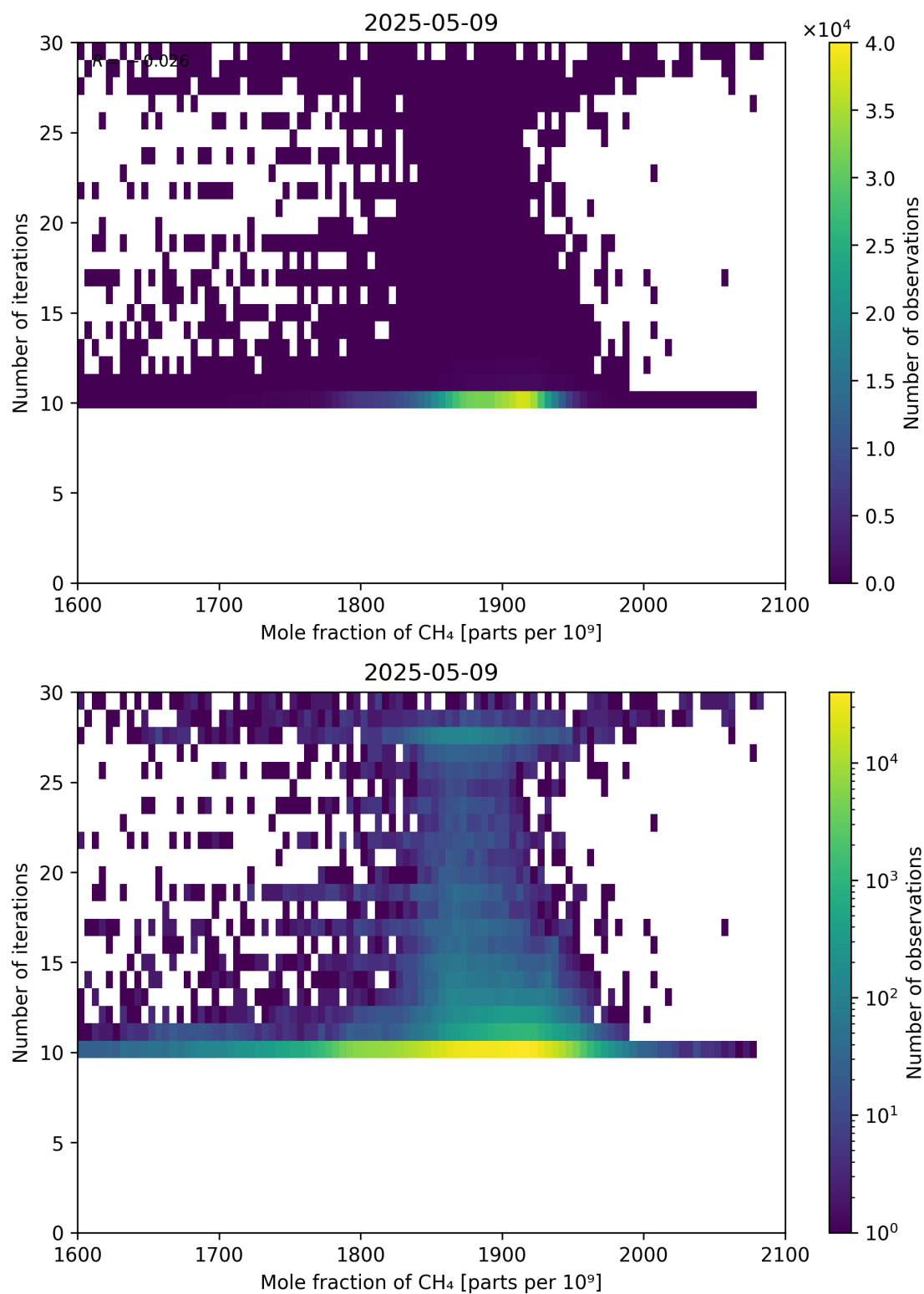
Figure 76: Scatter density plot of “Mole fraction of CH 4 ” against “Number of iterations” for 2025-05-08 to 2025-05-10.
