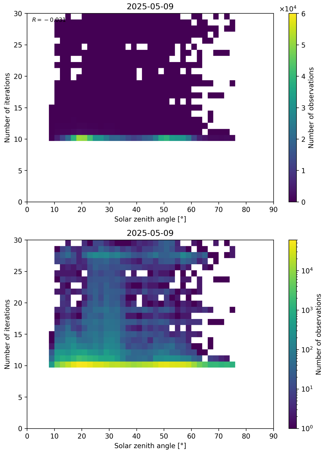
Figure 102: Scatter density plot of “Solar zenith angle” against “Number of iterations” for 2025-05-08 to 2025-05-10.
