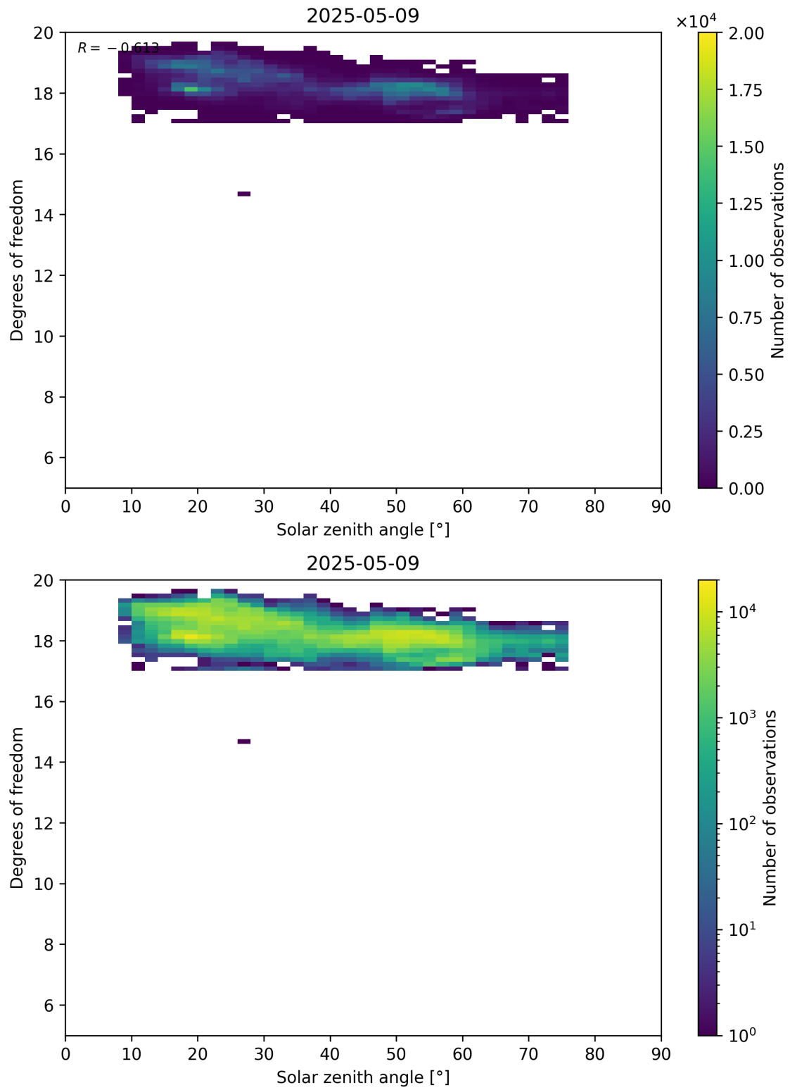
Figure 96: Scatter density plot of “Solar zenith angle” against “Degrees of freedom” for 2025-05-08 to 2025-05-10.
