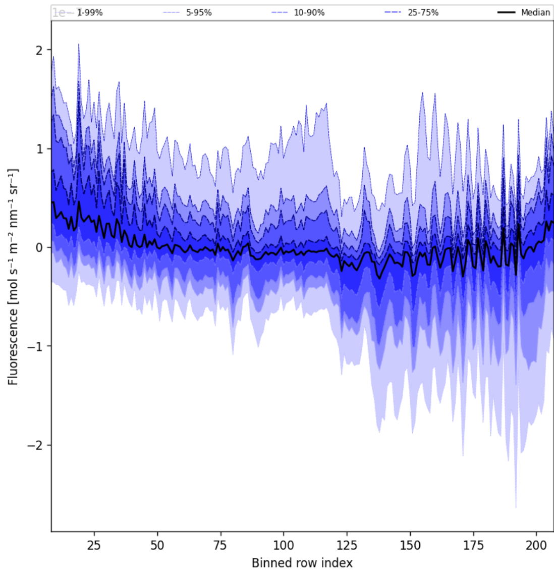
Figure 43: Along track statistics of “Fluorescence” for 2025-05-08 to 2025-05-10
