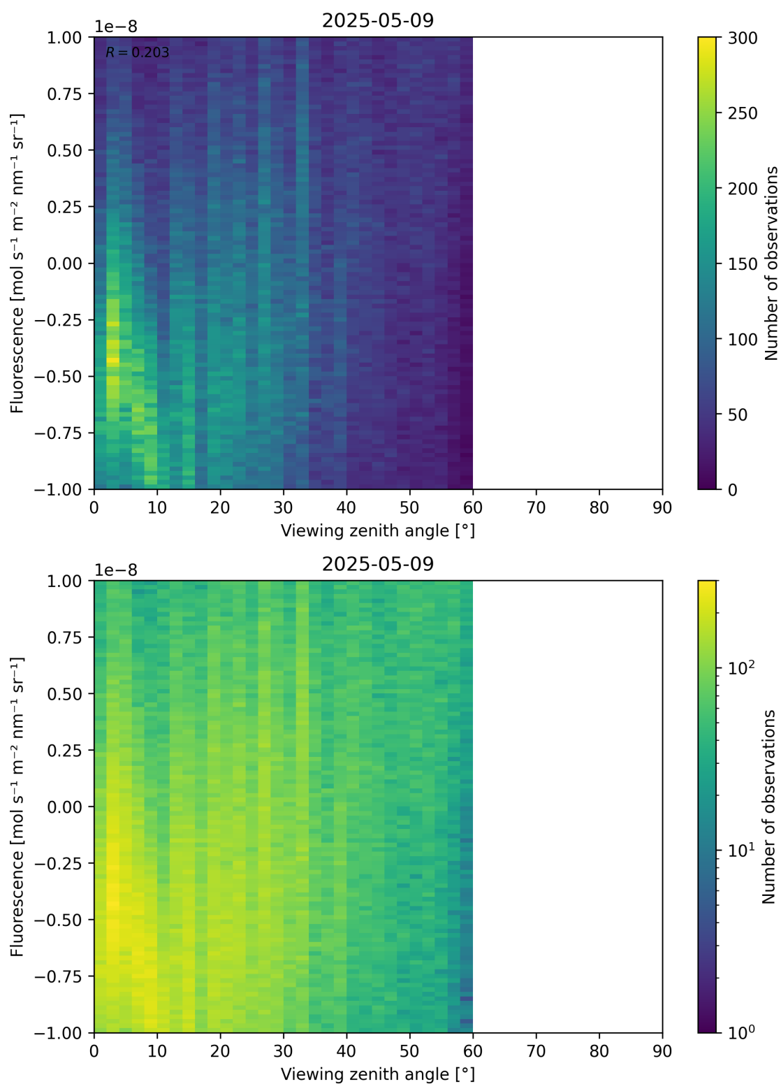
Figure 108: Scatter density plot of “Viewing zenith angle” against “Fluorescence” for 2025-05-08 to 2025-05-10.
