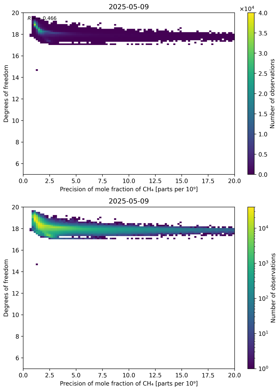
Figure 80: Scatter density plot of “Precision of mole fraction of CH 4 ” against “Degrees of freedom” for 2025-05-08 to 2025-05-10.
