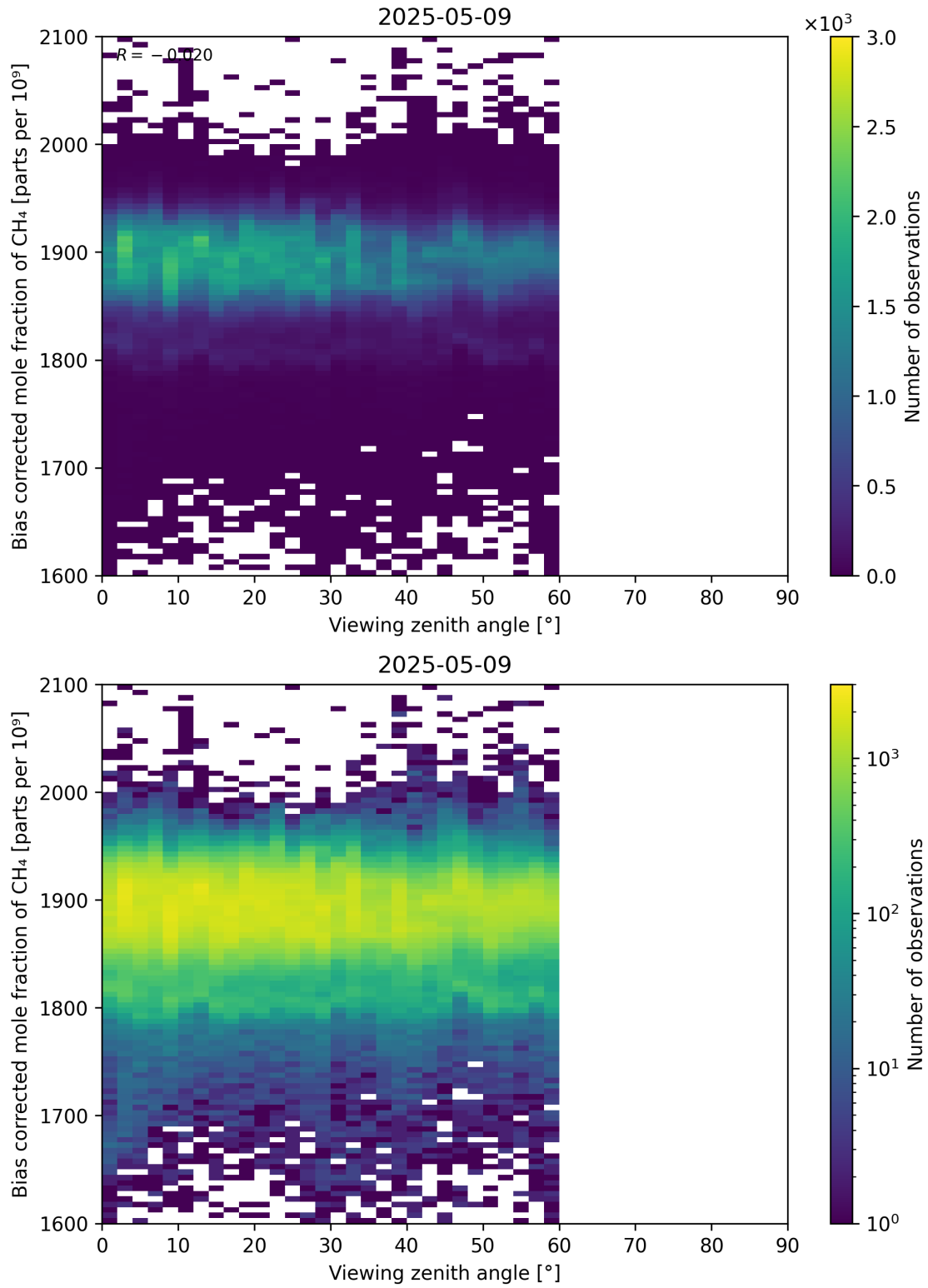
Figure 111: Scatter density plot of “Viewing zenith angle” against “Bias corrected mole fraction of CH 4 ” for 2025-05-08 to 2025-05-10.
