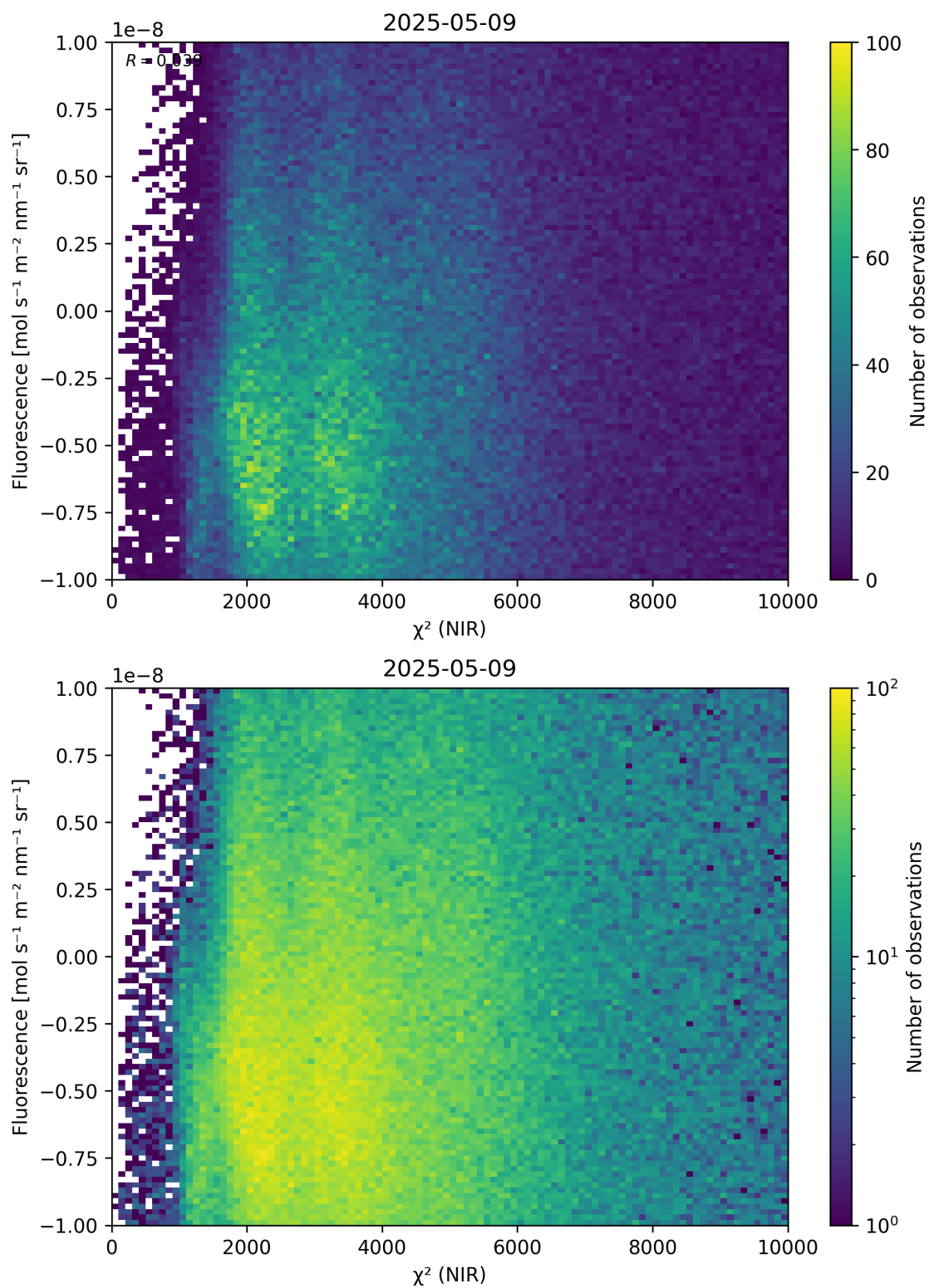
Figure 45: Scatter density plot of “ \chi^2 (NIR)” against “Fluorescence” for 2025-05-08 to 2025-05-10.
