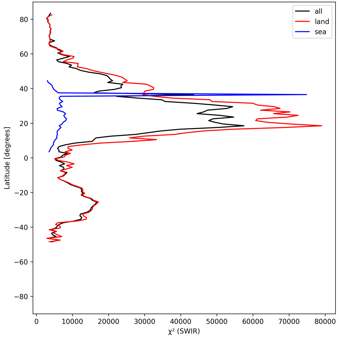
Figure 17: Zonal average of “ \chi^2 (SWIR)” for 2025-05-08 to 2025-05-10.
