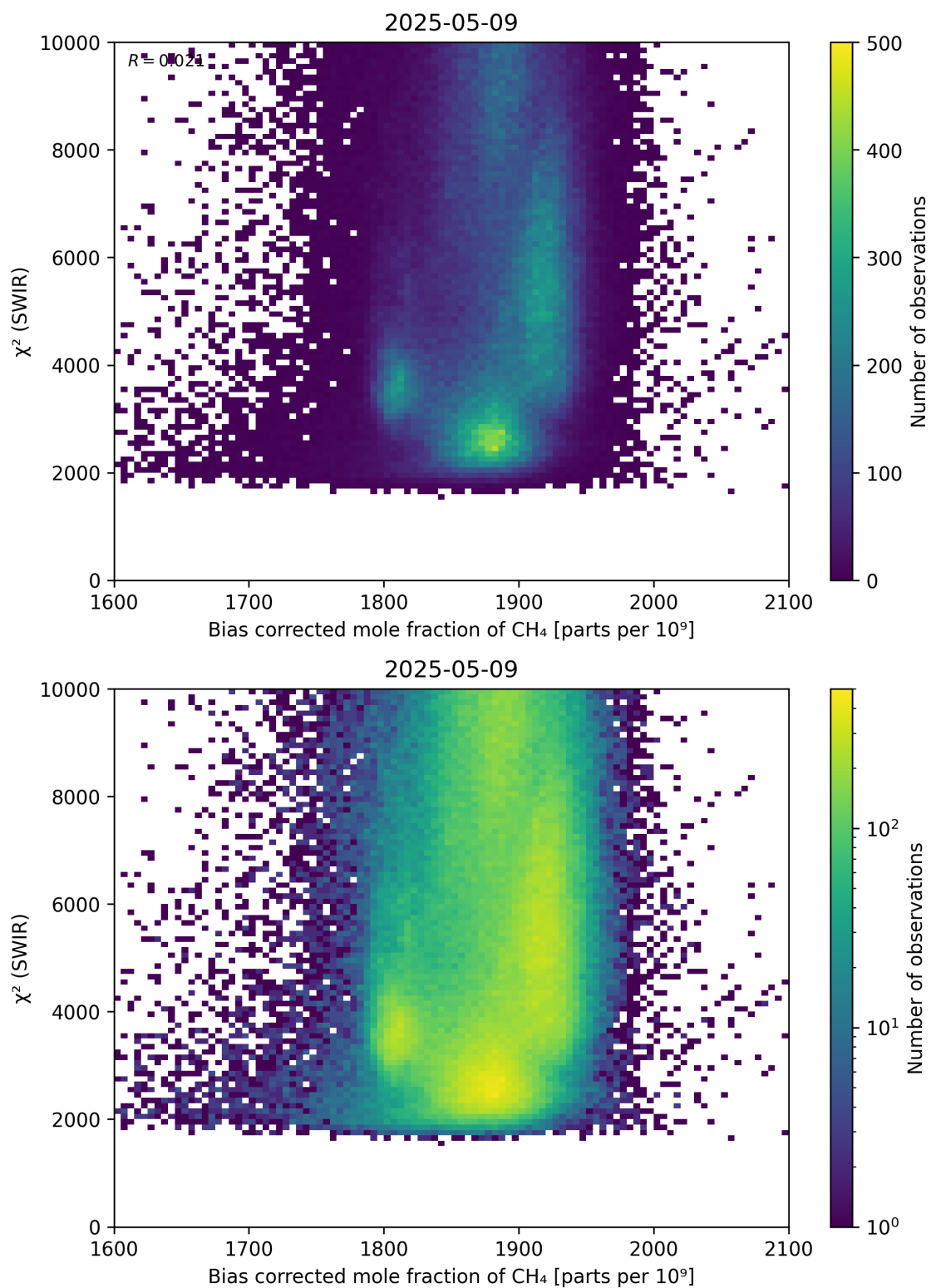
Figure 64: Scatter density plot of “Bias corrected mole fraction of \text{CH}_4 ” against “ \chi^2 (SWIR)” for 2025-05-08 to 2025-05-10.
