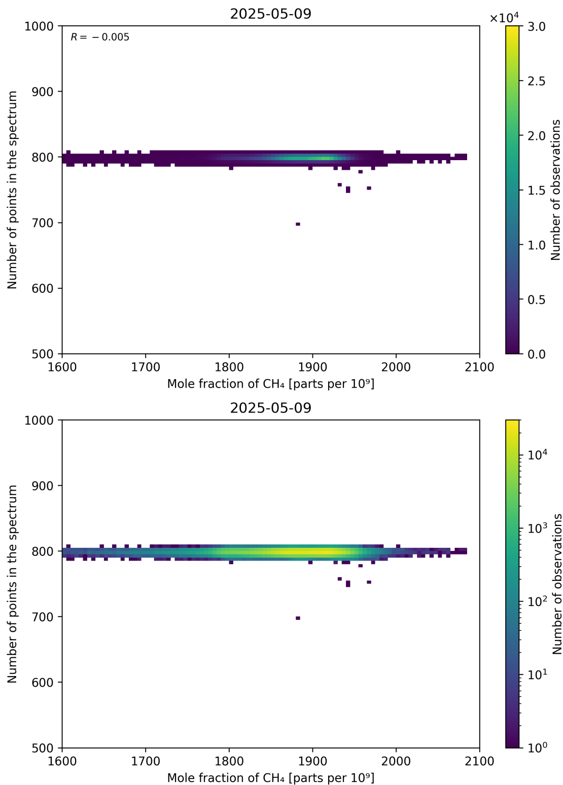
Figure 77: Scatter density plot of “Mole fraction of CH 4 ” against “Number of points in the spectrum” for 2025-05-08 to 2025-05-10.
