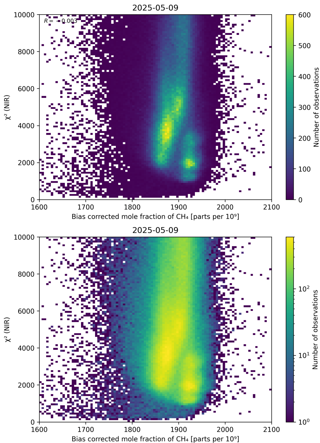
Figure 63: Scatter density plot of “Bias corrected mole fraction of CH 4 ” against “ \chi^2 (NIR)” for 2025-05-08 to 2025-05-10.
