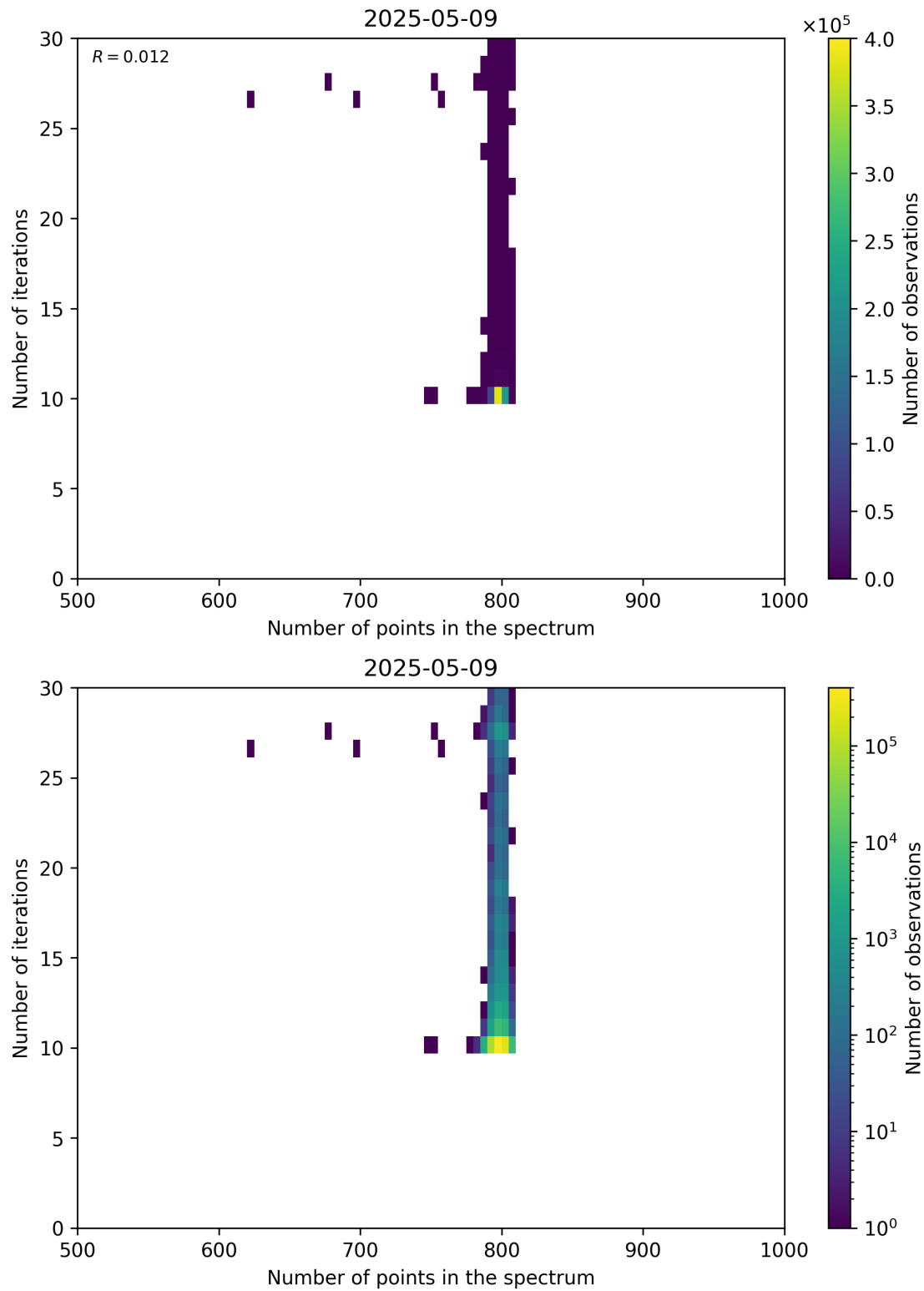
Figure 92: Scatter density plot of “Number of points in the spectrum” against “Number of iterations” for 2025-05-08 to 2025-05-10.
