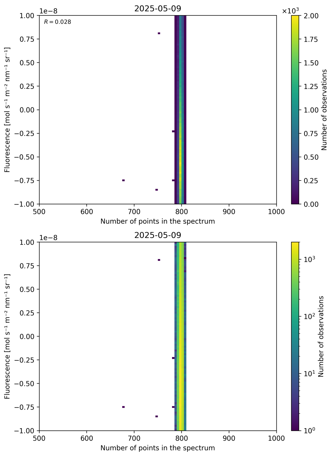
Figure 91: Scatter density plot of “Number of points in the spectrum” against “Fluorescence” for 2025-05-08 to 2025-05-10.
