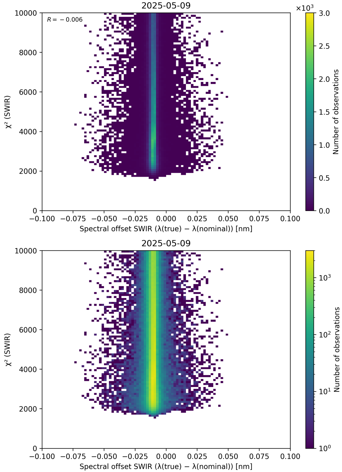
Figure 118: Scatter density plot of “Spectral offset SWIR ( \lambda_{\text{true}} - \lambda_{\text{nominal}} )” against “ \chi^2 (SWIR)” for 2025-05-08 to 2025-05-10.
