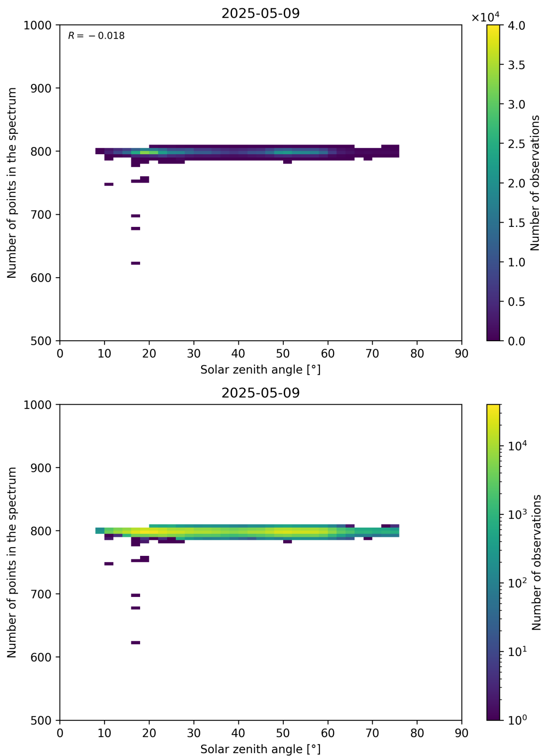
Figure 103: Scatter density plot of “Solar zenith angle” against “Number of points in the spectrum” for 2025-05-08 to 2025-05-10.
