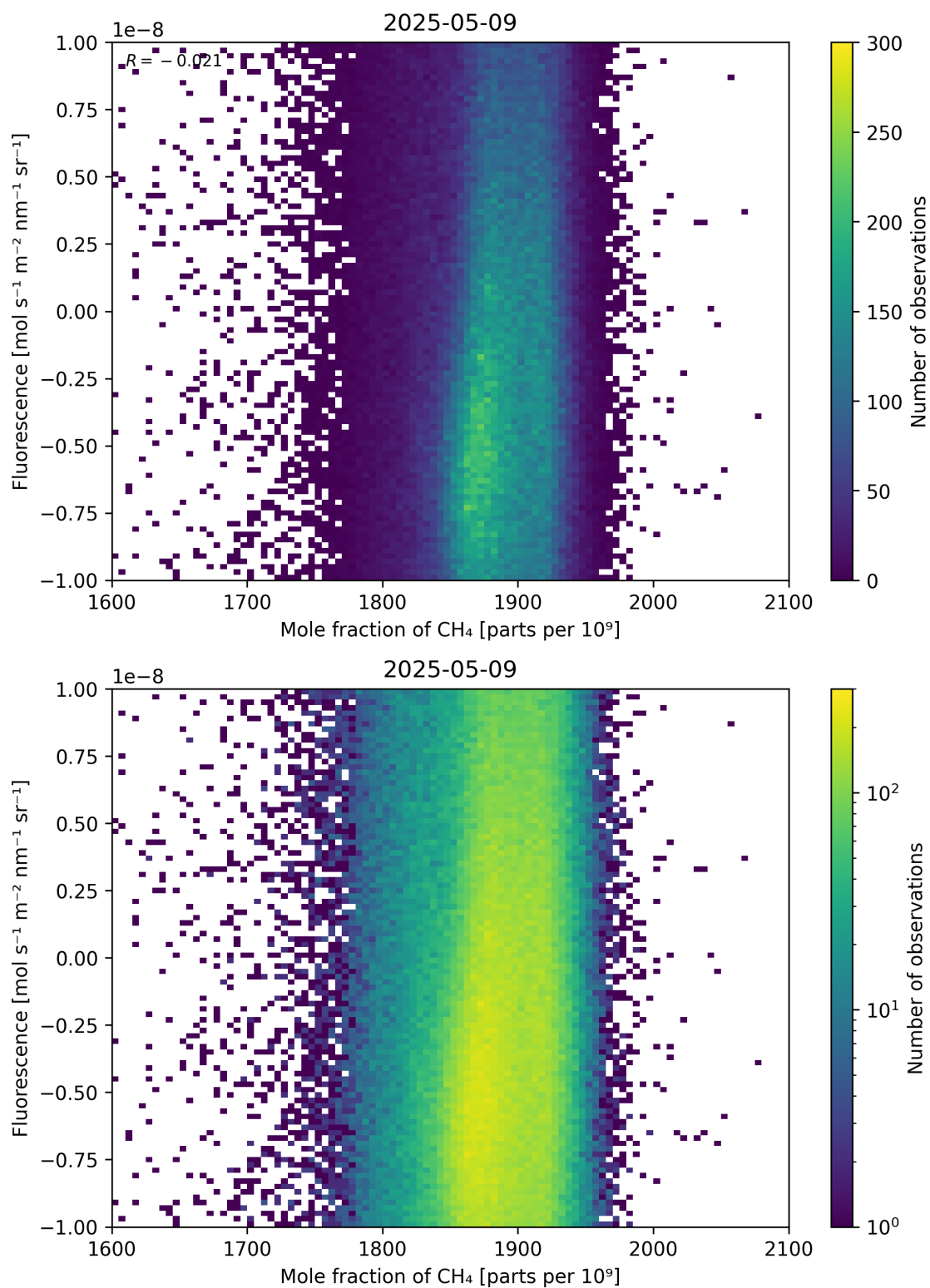
Figure 73: Scatter density plot of “Mole fraction of \text{CH}_4 ” against “Fluorescence” for 2025-05-08 to 2025-05-10.
