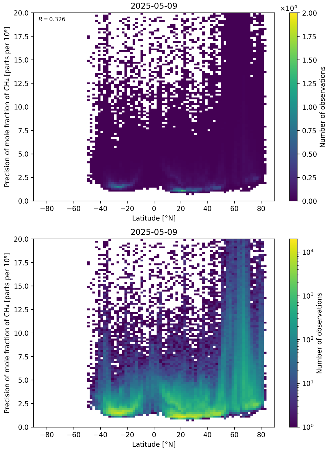
Figure 59: Scatter density plot of “Latitude” against “Precision of mole fraction of \text{CH}_4 ” for 2025-05-08 to 2025-05-10.
