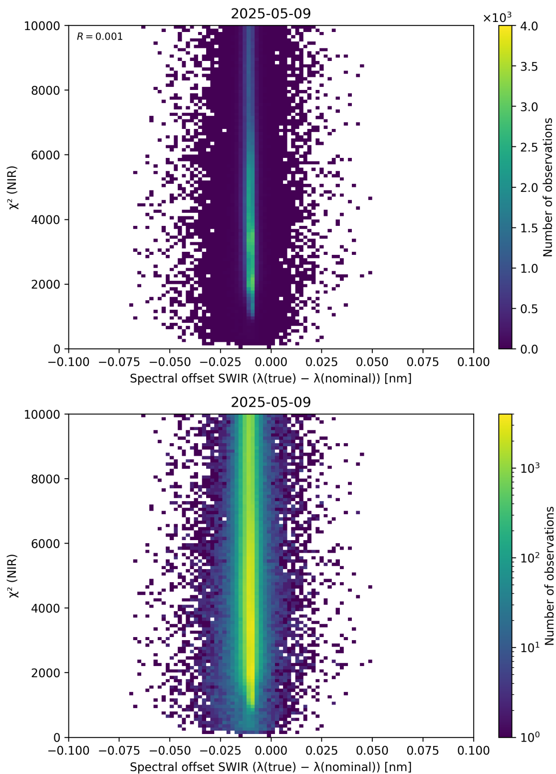
Figure 117: Scatter density plot of “Spectral offset SWIR ( \lambda_{\text{true}} - \lambda_{\text{nominal}} )” against “ \chi^2 (NIR)” for 2025-05-08 to 2025-05-10.
