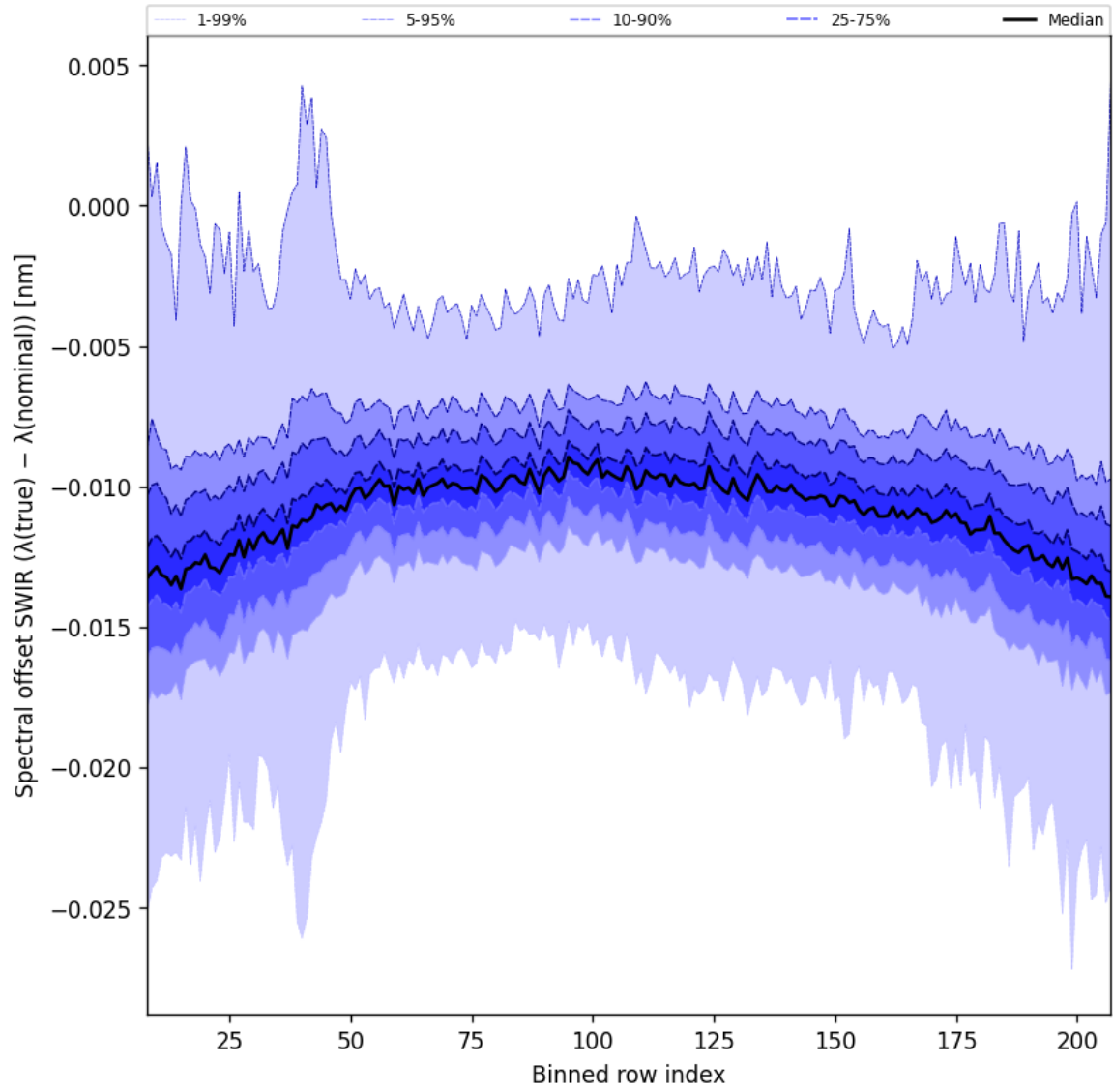
Figure 38: Along track statistics of “Spectral offset SWIR ( \lambda_{\text{true}} - \lambda_{\text{nominal}} )” for 2025-05-08 to 2025-05-10
