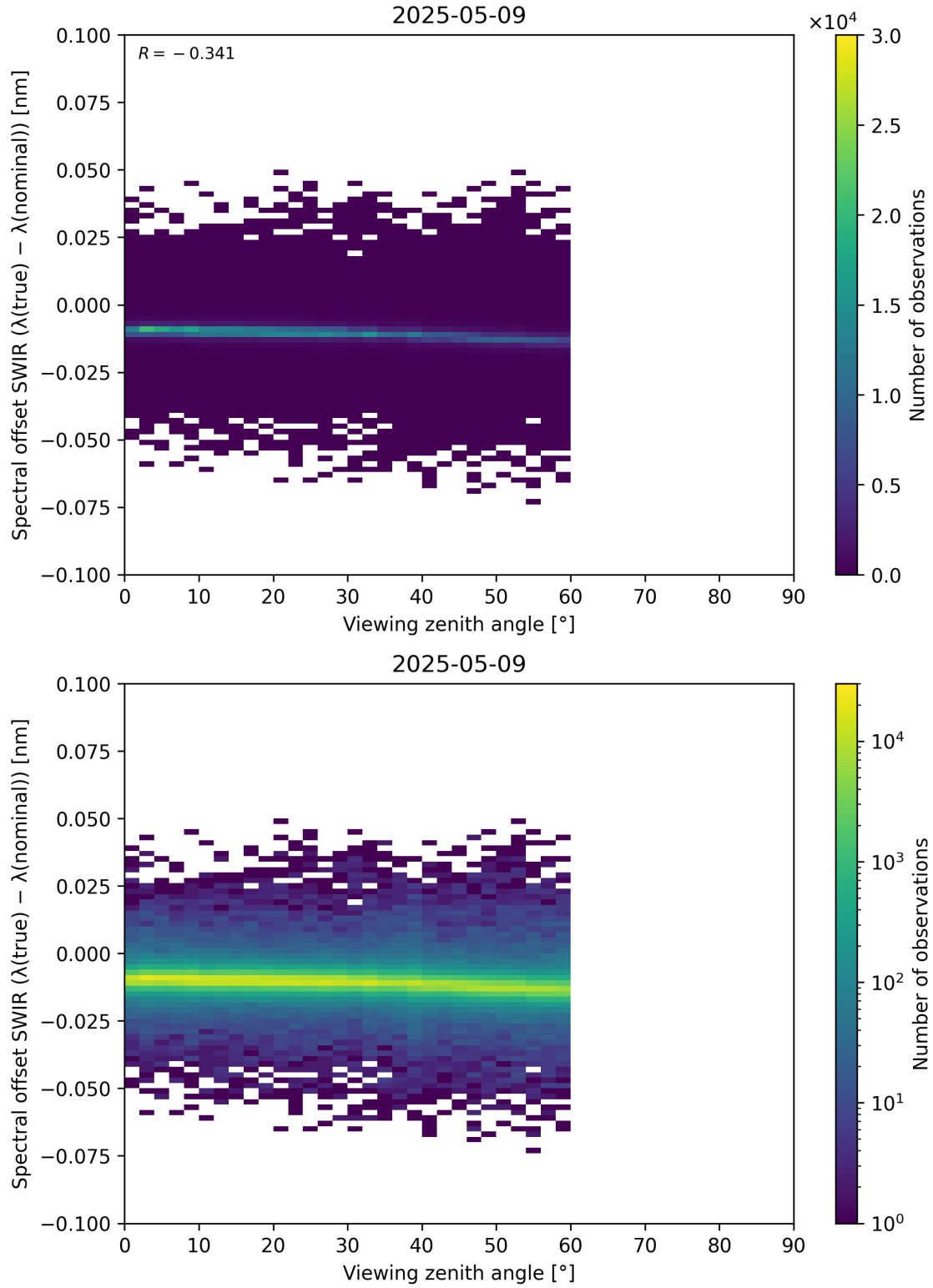
Figure 116: Scatter density plot of “Viewing zenith angle” against “Spectral offset SWIR ( \lambda_{\text{true}} - \lambda_{\text{nominal}} )” for 2025-05-08 to 2025-05-10.
