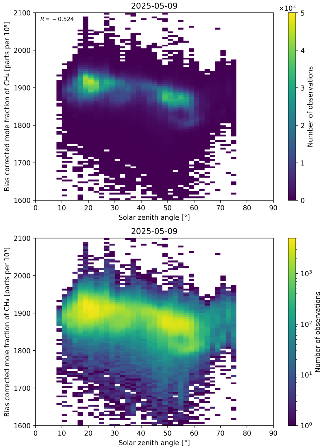
Figure 100: Scatter density plot of “Solar zenith angle” against “Bias corrected mole fraction of CH 4 ” for 2025-05-08 to 2025-05-10.
