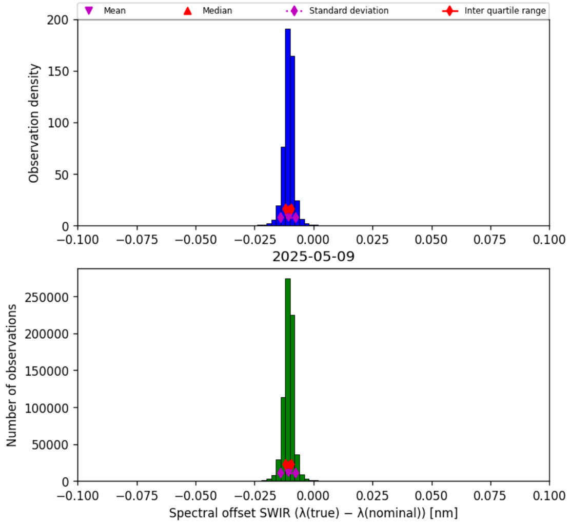
Figure 27: Histogram of “Spectral offset SWIR ( \lambda_{\text{true}} - \lambda_{\text{nominal}} )” for 2025-05-08 to 2025-05-10
