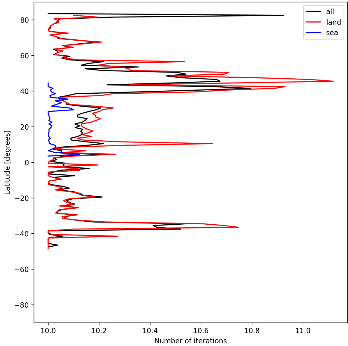
Figure 20: Zonal average of “Number of iterations” for 2025-05-08 to 2025-05-10.
