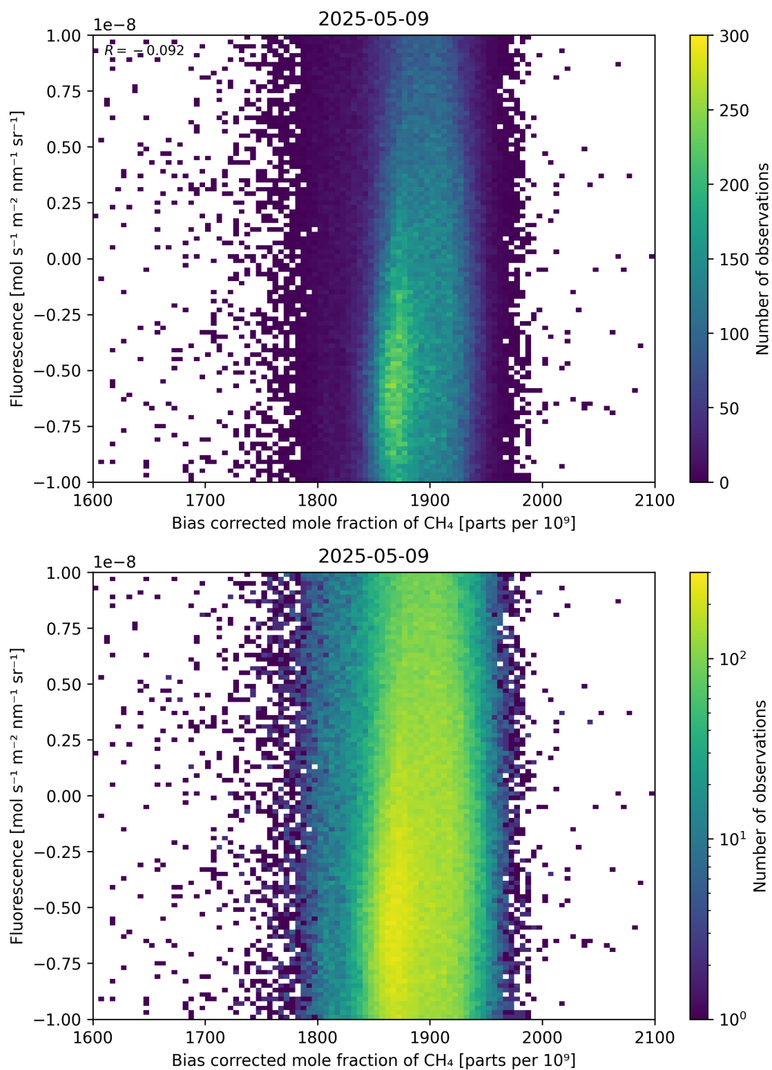
Figure 66: Scatter density plot of “Bias corrected mole fraction of \text{CH}_4 ” against “Fluorescence” for 2025-05-08 to 2025-05-10.
