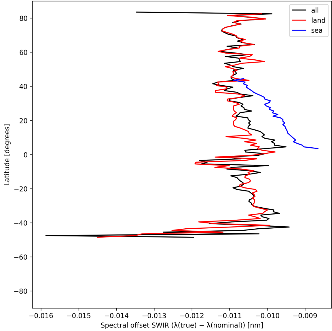
Figure 16: Zonal average of “Spectral offset SWIR ( \lambda_{\text{true}} - \lambda_{\text{nominal}} )” for 2025-05-08 to 2025-05-10.
