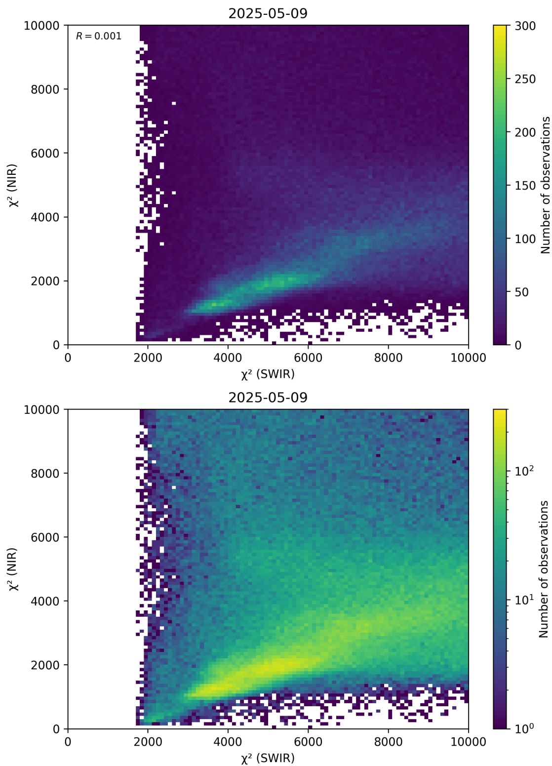
Figure 47: Scatter density plot of “ \chi^2 (SWIR)” against “ \chi^2 (NIR)” for 2025-05-08 to 2025-05-10.
