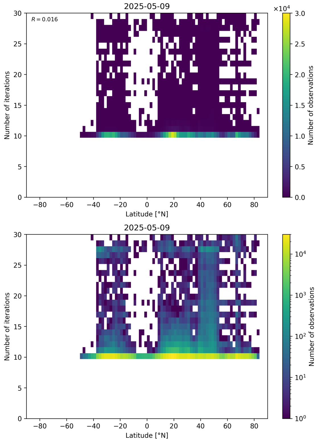
Figure 60: Scatter density plot of “Latitude” against “Number of iterations” for 2025-05-08 to 2025-05-10.
