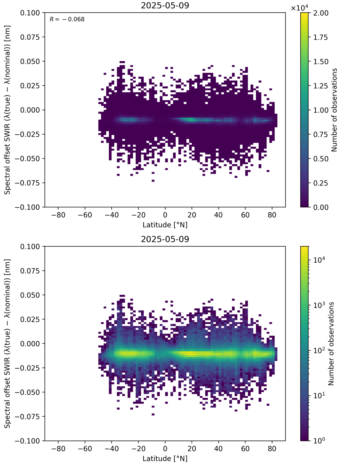
Figure 62: Scatter density plot of “Latitude” against “Spectral offset SWIR ( \lambda_{\text{true}} - \lambda_{\text{nominal}} )” for 2025-05-08 to 2025-05-10.
