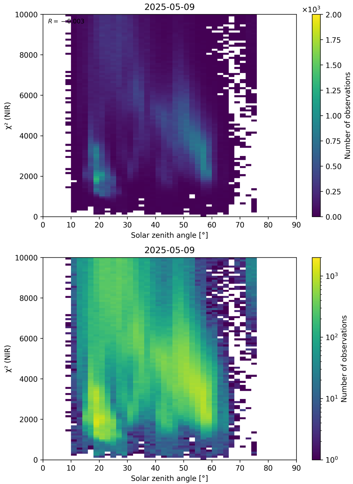
Figure 94: Scatter density plot of “Solar zenith angle” against “ \chi^2 (NIR)” for 2025-05-08 to 2025-05-10.
