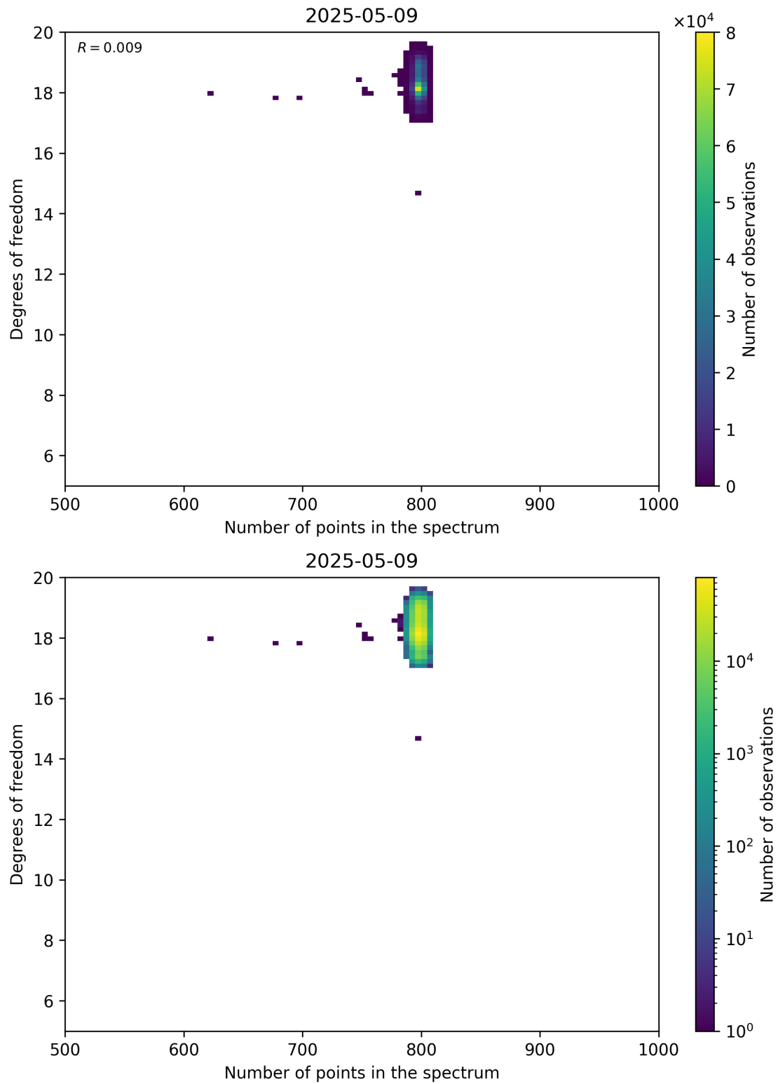
Figure 90: Scatter density plot of “Number of points in the spectrum” against “Degrees of freedom” for 2025-05-08 to 2025-05-10.
