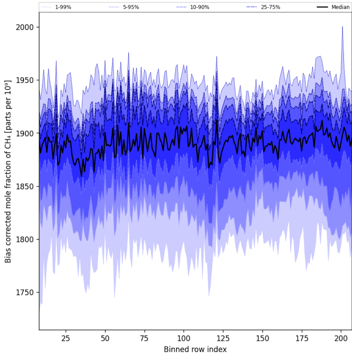
Figure 36: Along track statistics of “Bias corrected mole fraction of CH 4 ” for 2025-05-08 to 2025-05-10
