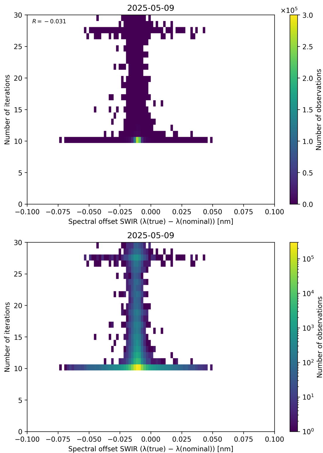
Figure 121: Scatter density plot of “Spectral offset SWIR ( \lambda_{\text{true}} - \lambda_{\text{nominal}} )” against “Number of iterations” for 2025-05-08 to 2025-05-10.
