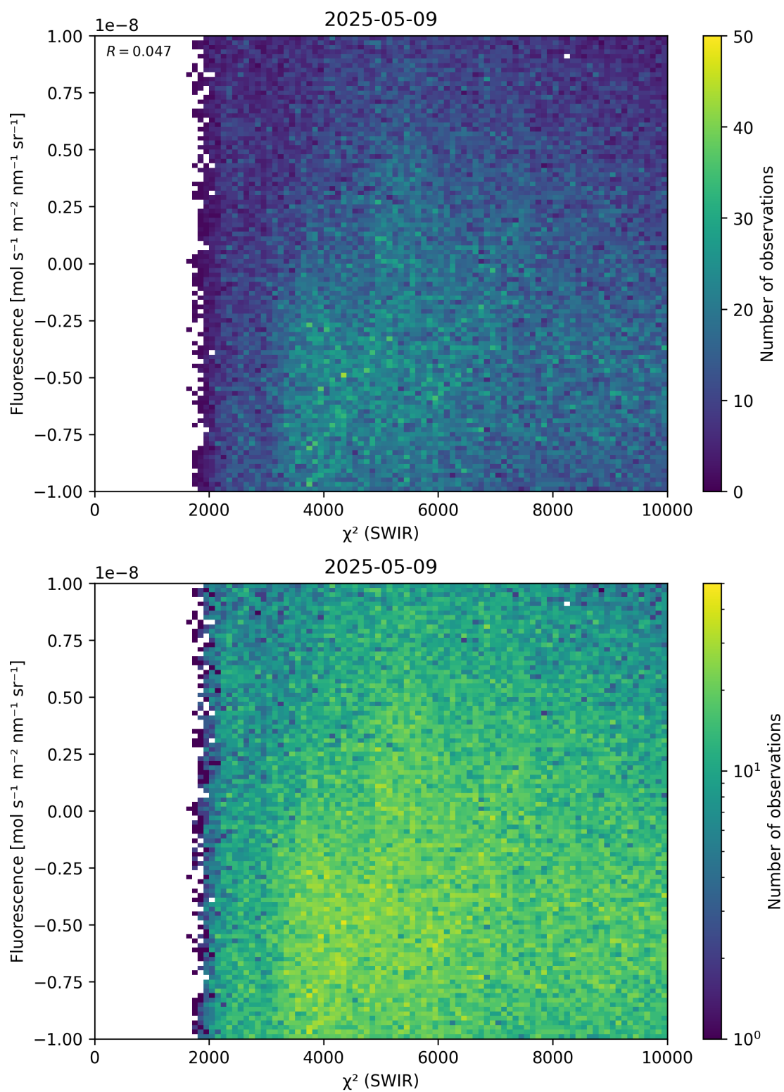
Figure 49: Scatter density plot of “ \chi^2 (SWIR)” against “Fluorescence” for 2025-05-08 to 2025-05-10.
