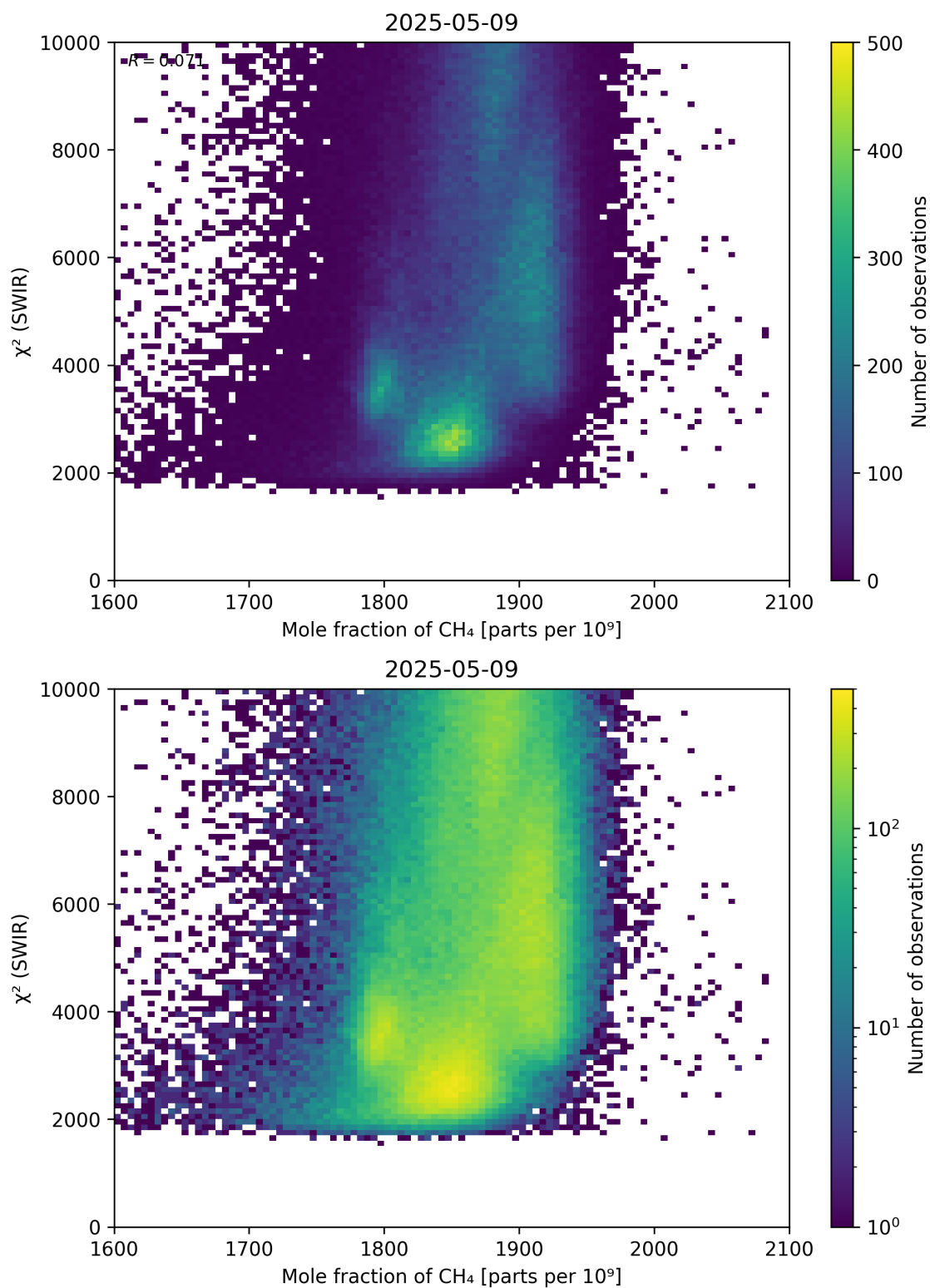
Figure 71: Scatter density plot of “Mole fraction of CH 4 ” against “ \chi^2 (SWIR)” for 2025-05-08 to 2025-05-10.
