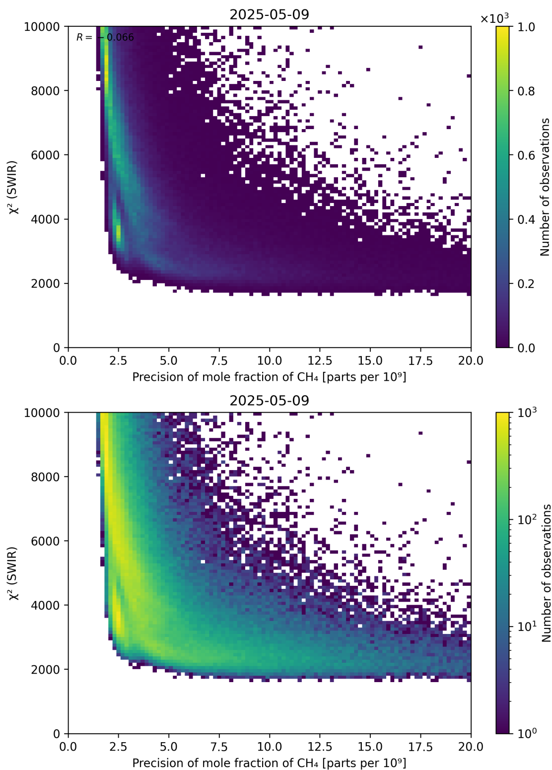
Figure 79: Scatter density plot of “Precision of mole fraction of \text{CH}_4 ” against “ \chi^2 (SWIR)” for 2025-05-08 to 2025-05-10.
