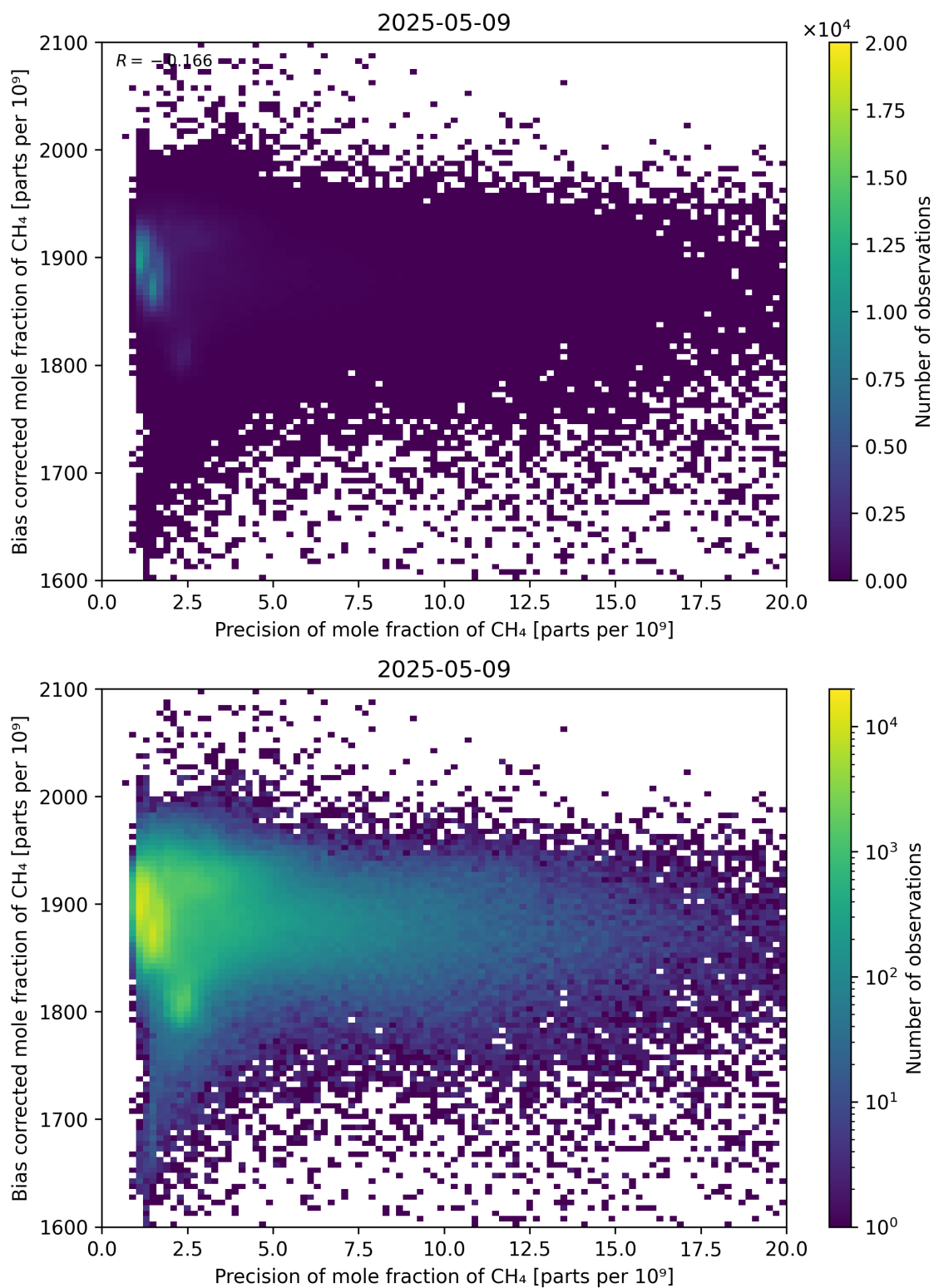
Figure 82: Scatter density plot of “Precision of mole fraction of CH 4 ” against “Bias corrected mole fraction of CH 4 ” for 2025-05-08 to 2025-05-10.
