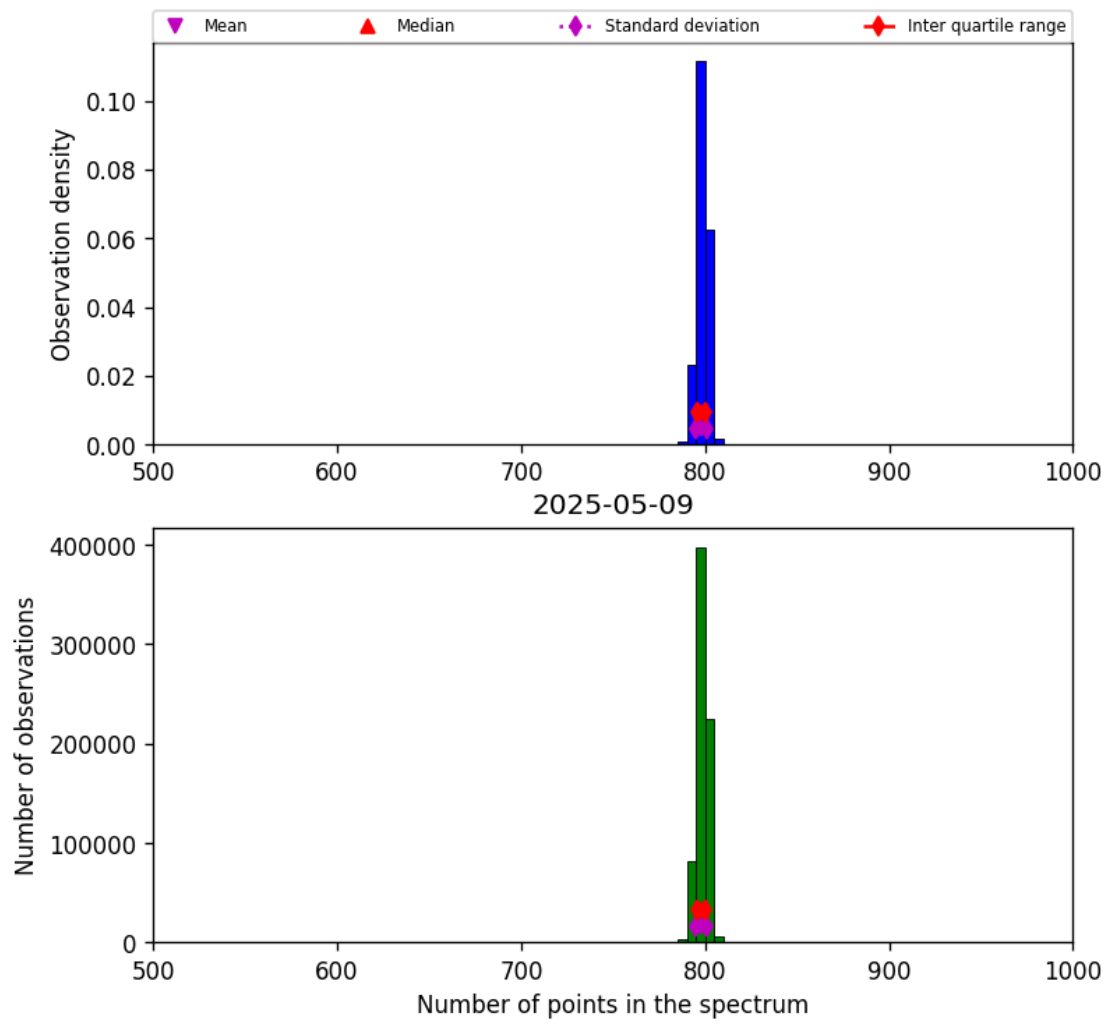
Figure 26: Histogram of “Number of points in the spectrum” for 2025-05-08 to 2025-05-10
