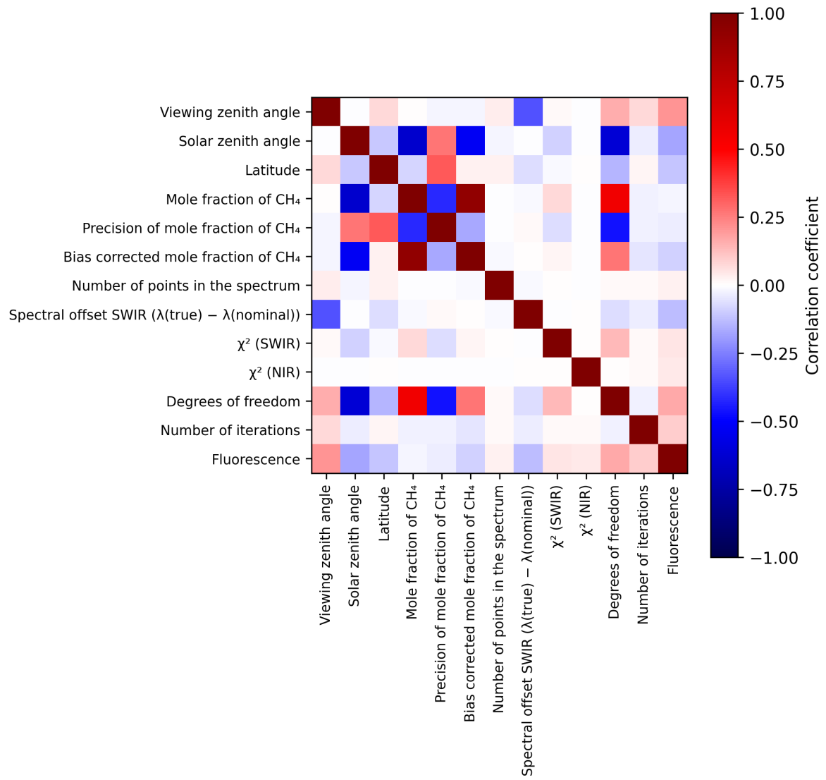
Figure 2: Map of correlation matrix for 2025-05-08 to 2025-05-10.
