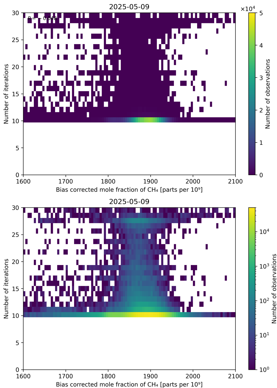
Figure 67: Scatter density plot of “Bias corrected mole fraction of \text{CH}_4 ” against “Number of iterations” for 2025-05-08 to 2025-05-10.
