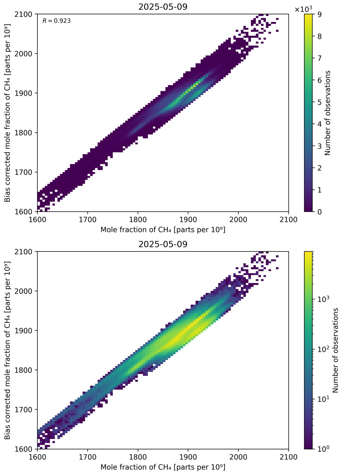
Figure 74: Scatter density plot of “Mole fraction of CH 4 ” against “Bias corrected mole fraction of CH 4 ” for 2025-05-08 to 2025-05-10.
