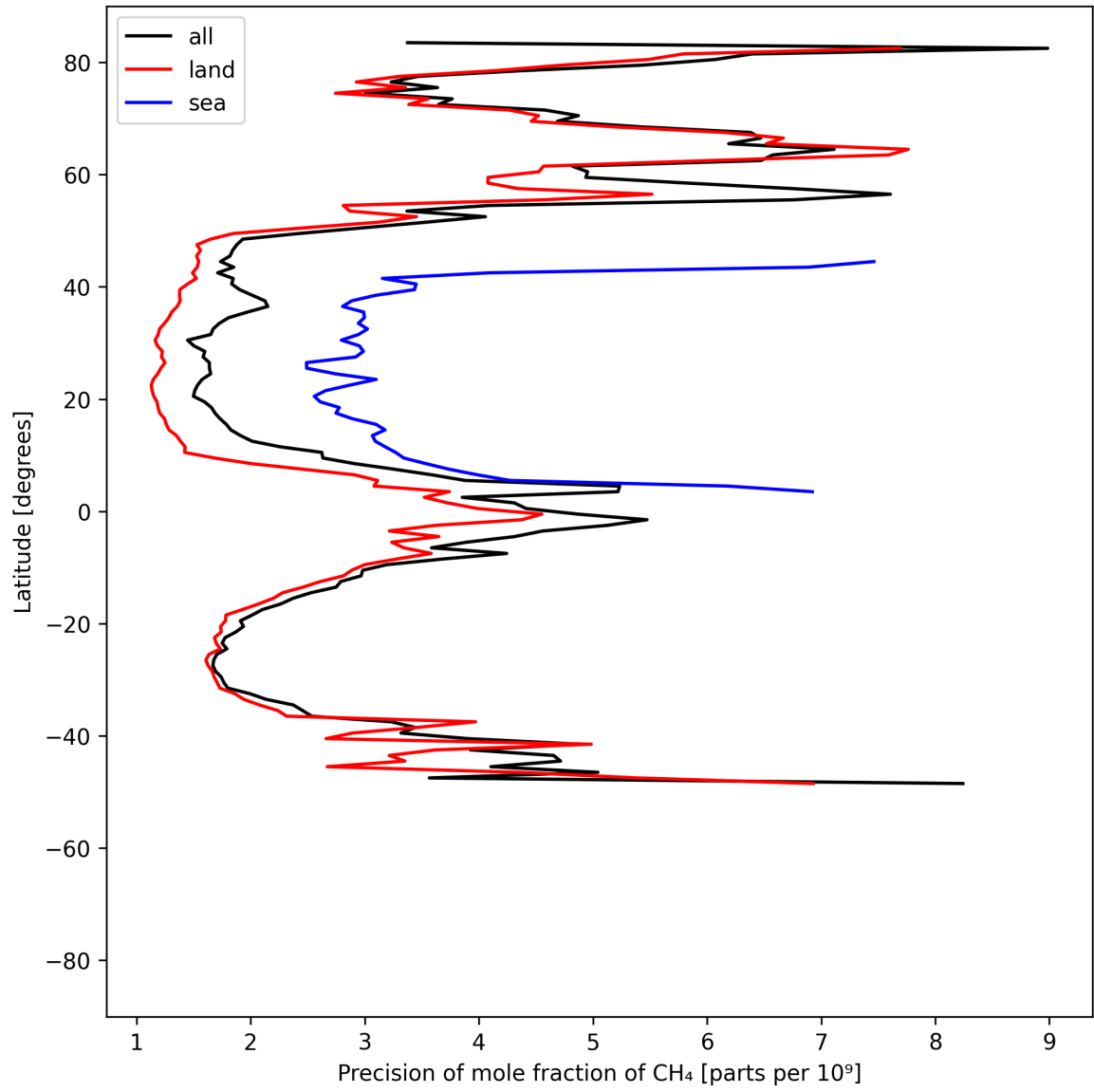
Figure 13: Zonal average of “Precision of mole fraction of CH 4 ” for 2025-05-08 to 2025-05-10.
