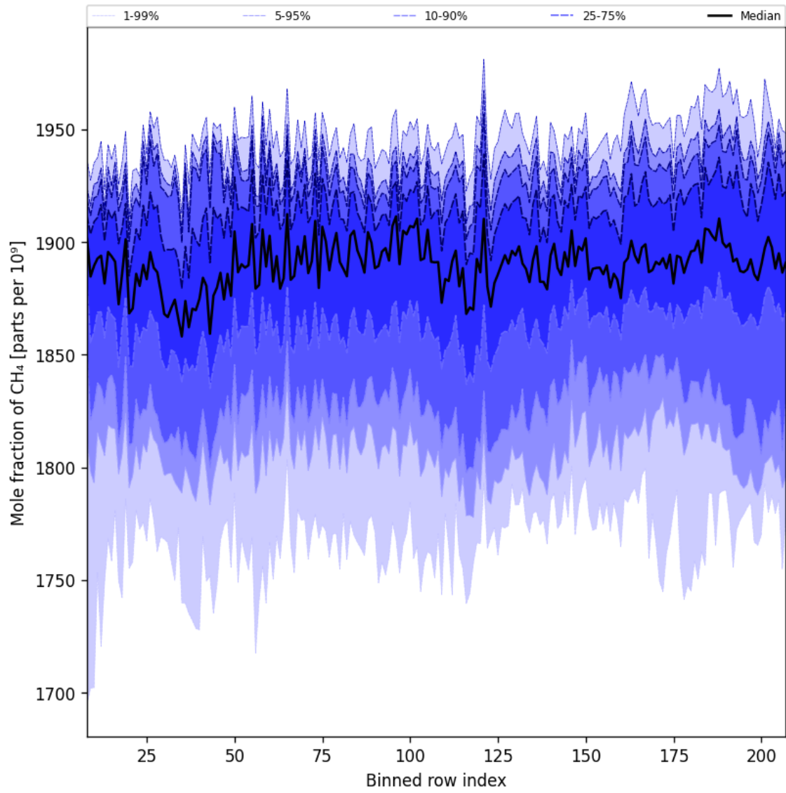
Figure 34: Along track statistics of “Mole fraction of CH 4 ” for 2025-05-08 to 2025-05-10
