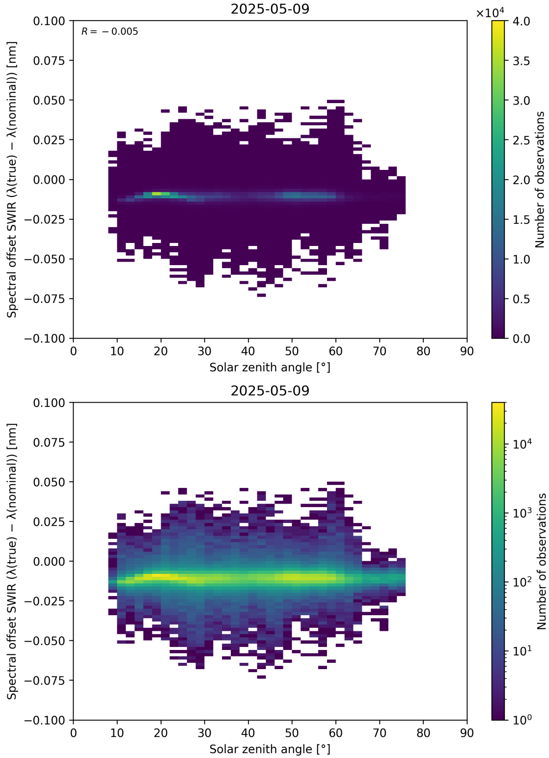
Figure 104: Scatter density plot of “Solar zenith angle” against “Spectral offset SWIR ( \lambda_{\text{true}} - \lambda_{\text{nominal}} )” for 2025-05-08 to 2025-05-10.
