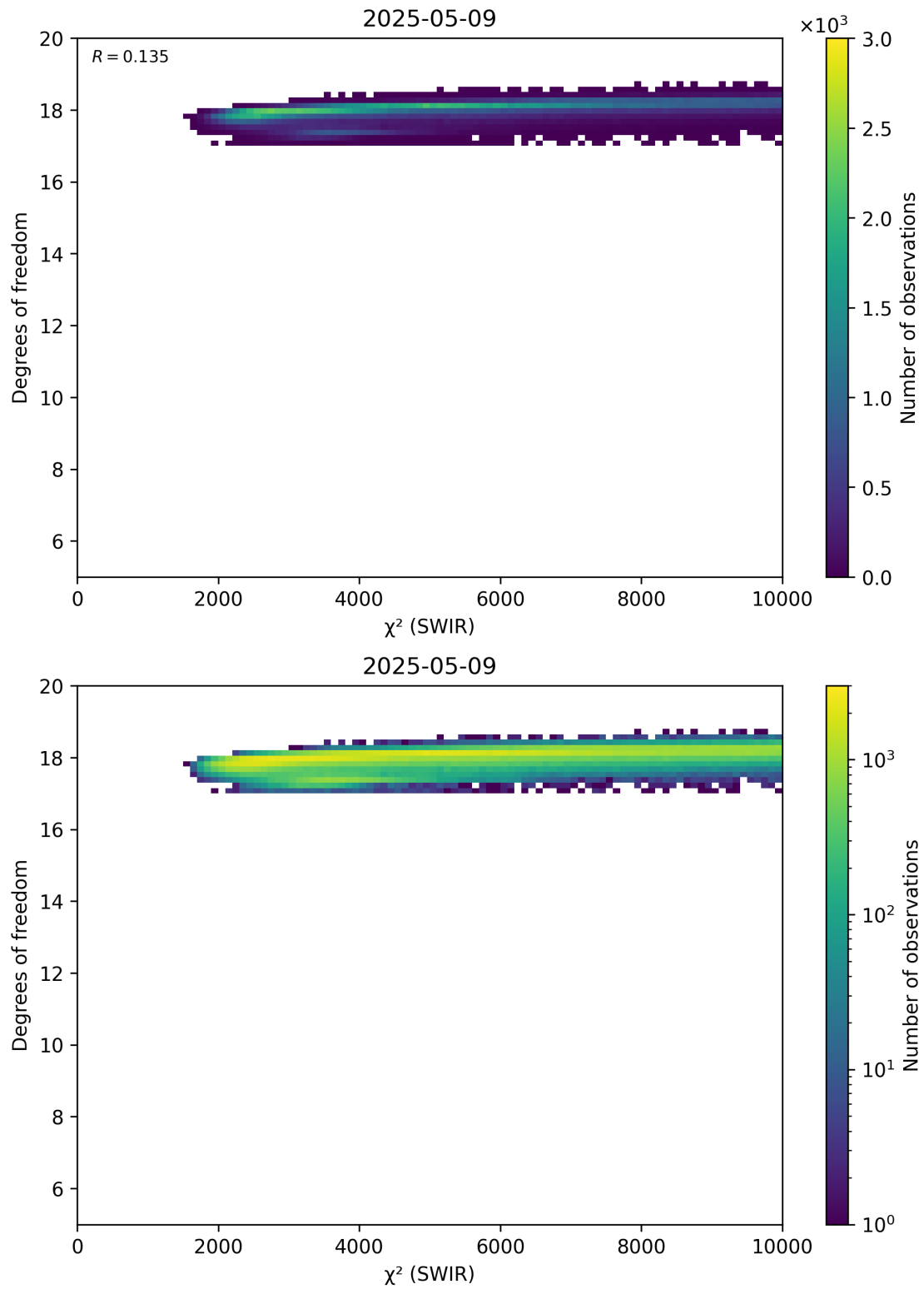
Figure 48: Scatter density plot of “ \chi^2 (SWIR)” against “Degrees of freedom” for 2025-05-08 to 2025-05-10.
