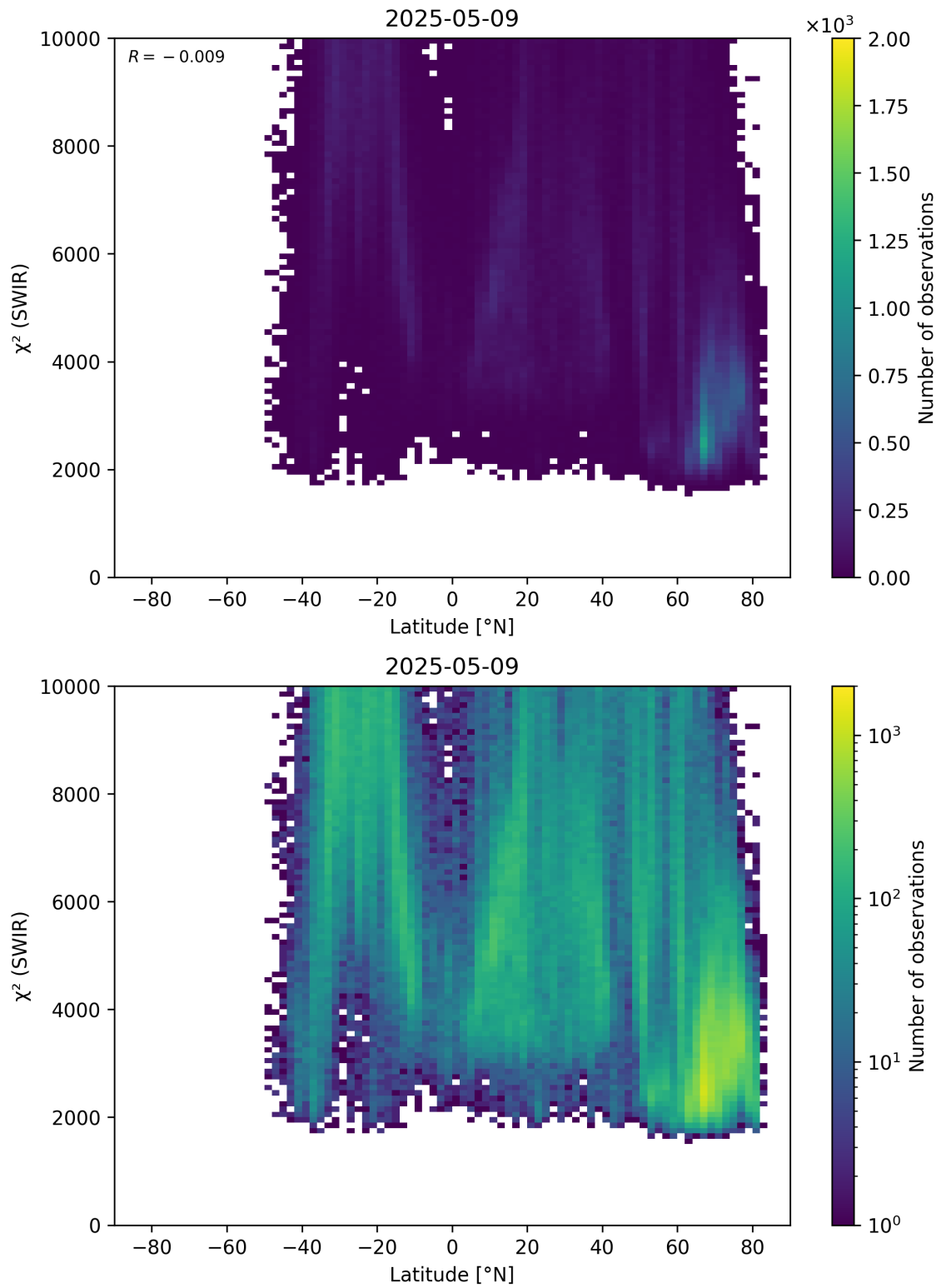
Figure 54: Scatter density plot of “Latitude” against “ \chi^2 (SWIR)” for 2025-05-08 to 2025-05-10.
