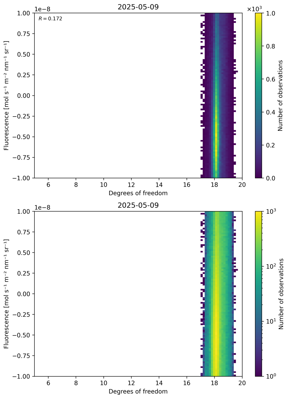
Figure 51: Scatter density plot of “Degrees of freedom” against “Fluorescence” for 2025-05-08 to 2025-05-10.
