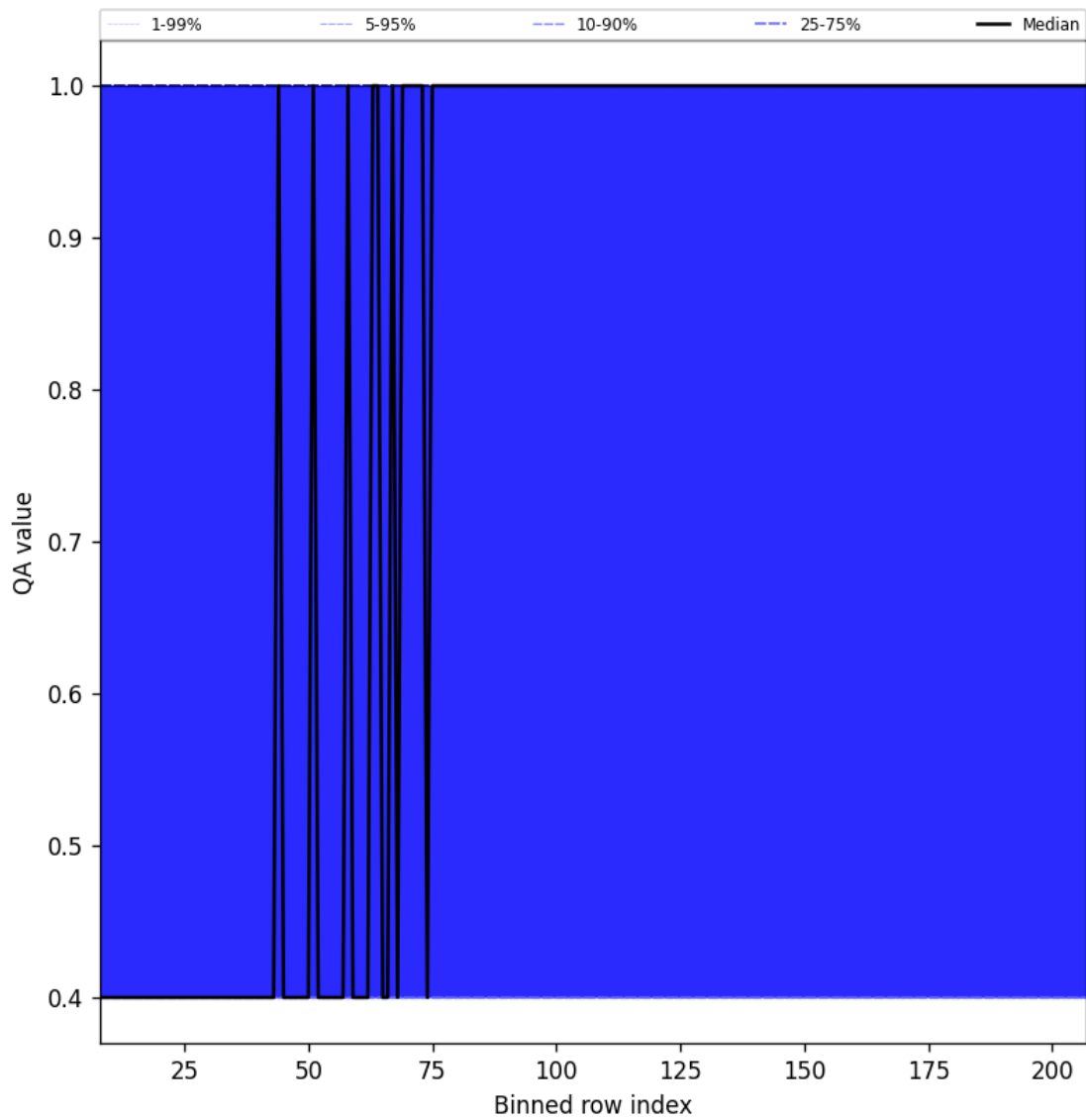
Figure 33: Along track statistics of “QA value” for 2025-05-08 to 2025-05-10
