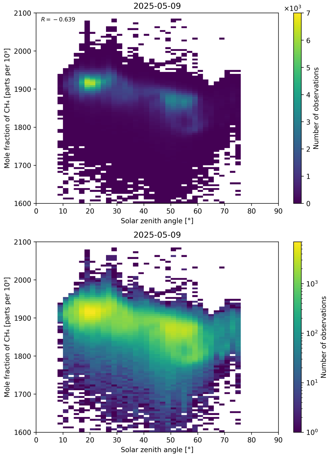
Figure 99: Scatter density plot of “Solar zenith angle” against “Mole fraction of \text{CH}_4 ” for 2025-05-08 to 2025-05-10.
