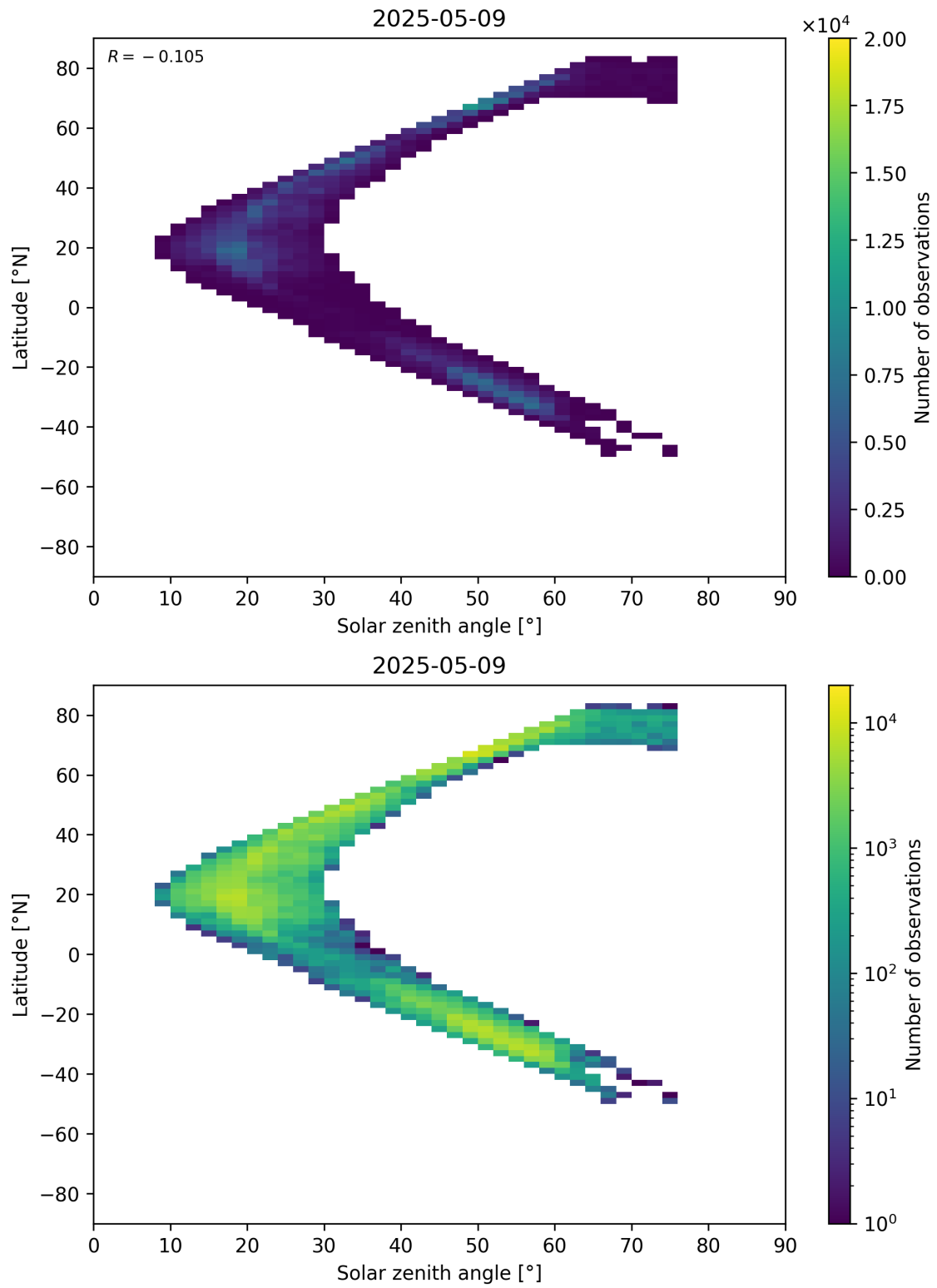
Figure 98: Scatter density plot of “Solar zenith angle” against “Latitude” for 2025-05-08 to 2025-05-10.
