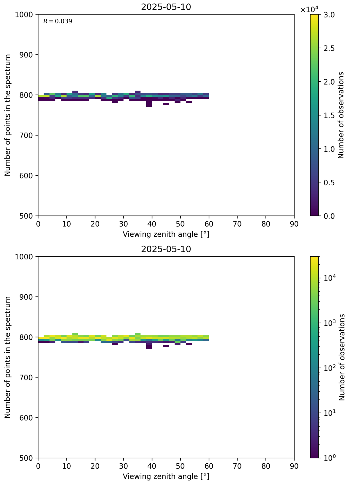
Figure 114: Scatter density plot of “Viewing zenith angle” against “Number of points in the spectrum” for 2025-05-10 to 2025-05-11.
