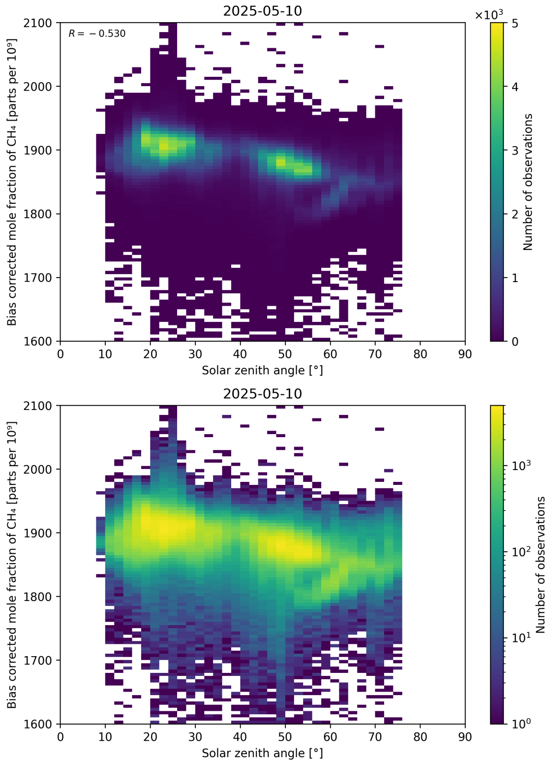
Figure 100: Scatter density plot of “Solar zenith angle” against “Bias corrected mole fraction of CH 4 ” for 2025-05-10 to 2025-05-11.
