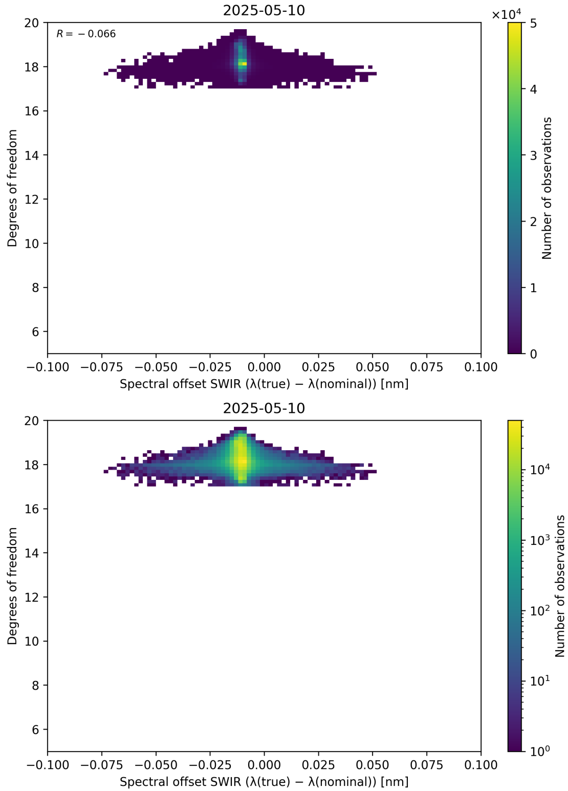
Figure 119: Scatter density plot of “Spectral offset SWIR ( \lambda_{\text{true}} - \lambda_{\text{nominal}} )” against “Degrees of freedom” for 2025-05-10 to 2025-05-11.
