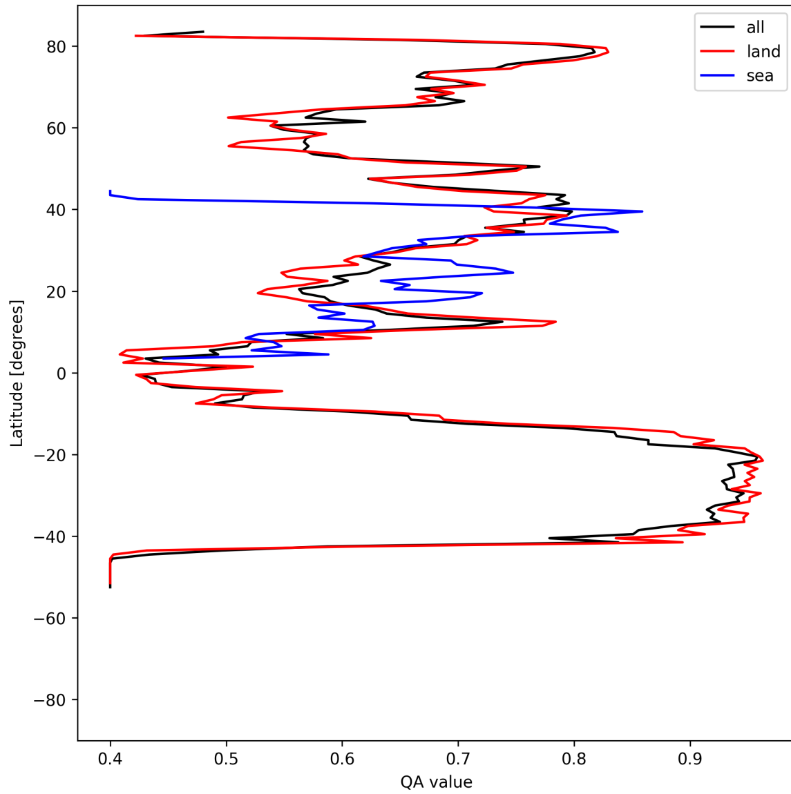
Figure 11: Zonal average of “QA value” for 2025-05-10 to 2025-05-11.
