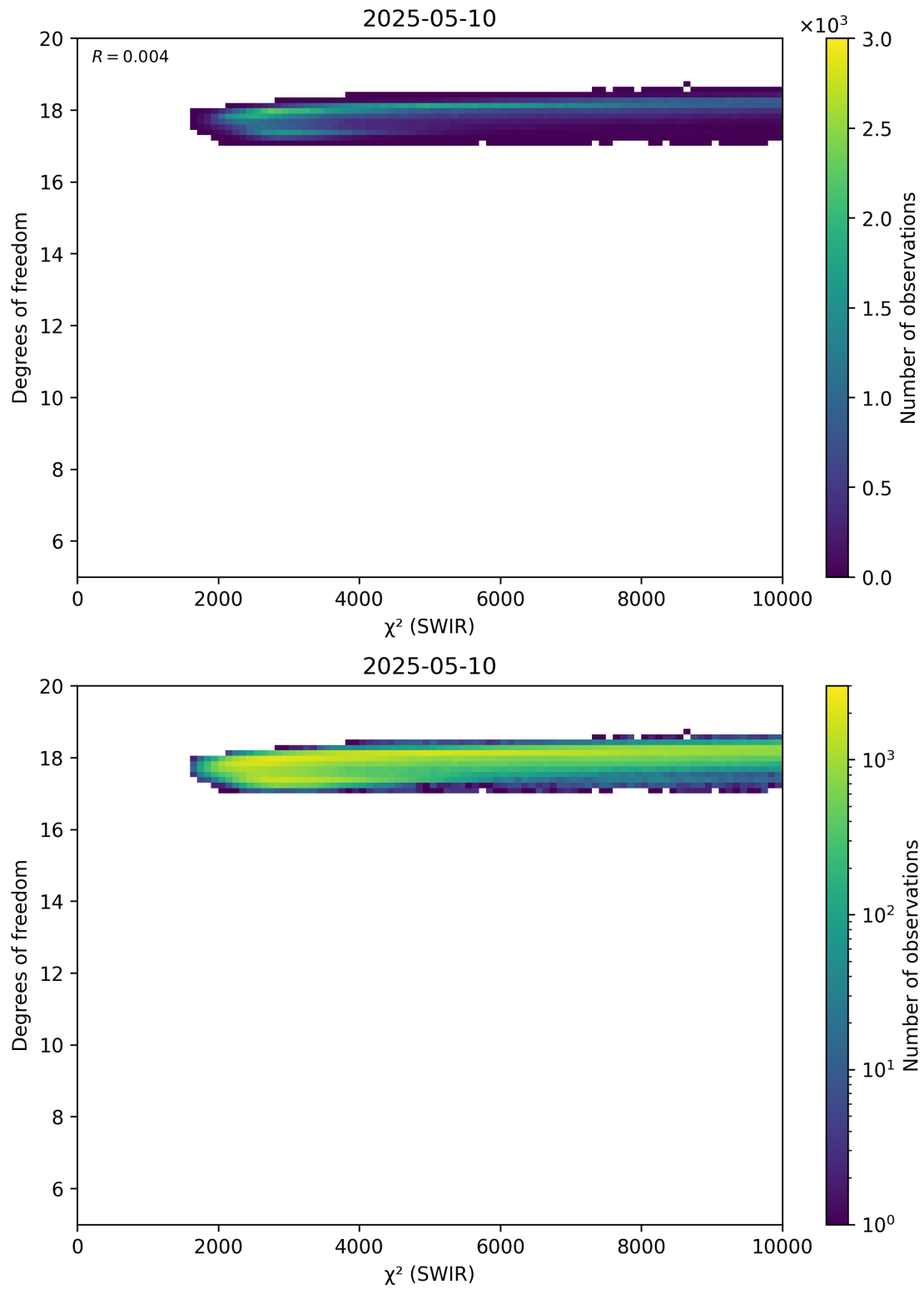
Figure 48: Scatter density plot of “ \chi^2 (SWIR)” against “Degrees of freedom” for 2025-05-10 to 2025-05-11.
