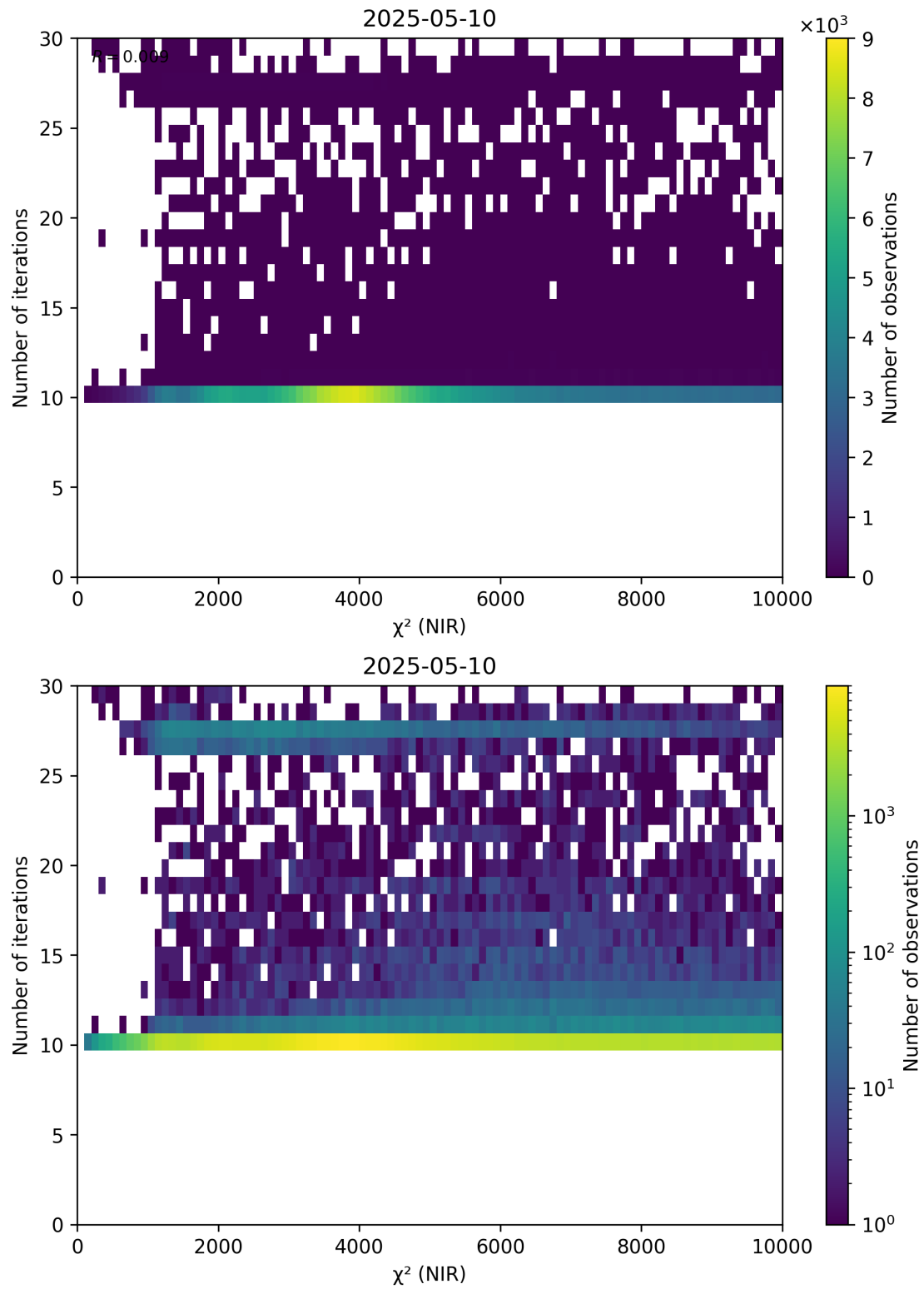
Figure 46: Scatter density plot of “ \chi^2 (NIR)” against “Number of iterations” for 2025-05-10 to 2025-05-11.
