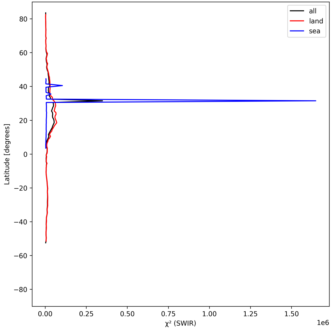
Figure 17: Zonal average of “ \chi^2 (SWIR)” for 2025-05-10 to 2025-05-11.
