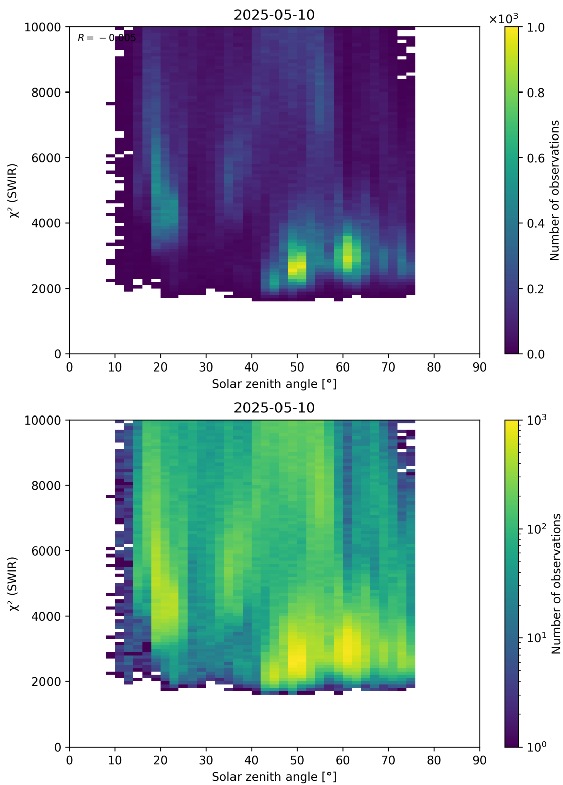
Figure 95: Scatter density plot of “Solar zenith angle” against “ \chi^2 (SWIR)” for 2025-05-10 to 2025-05-11.
