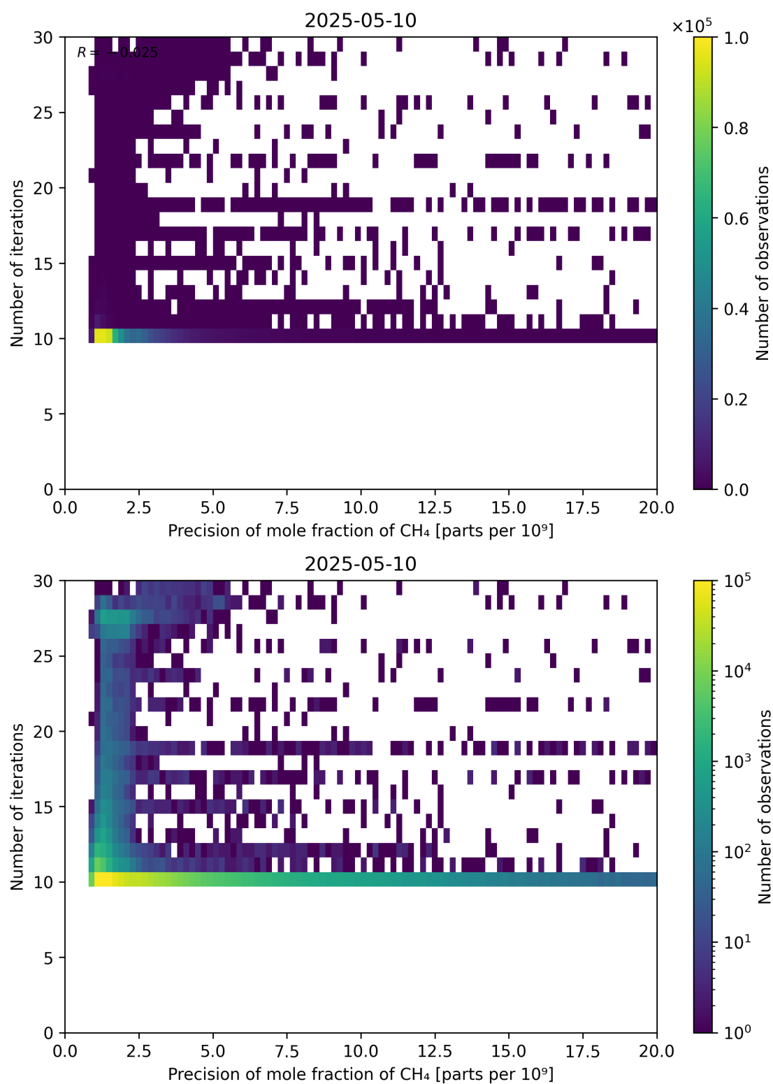
Figure 83: Scatter density plot of “Precision of mole fraction of CH 4 ” against “Number of iterations” for 2025-05-10 to 2025-05-11.
