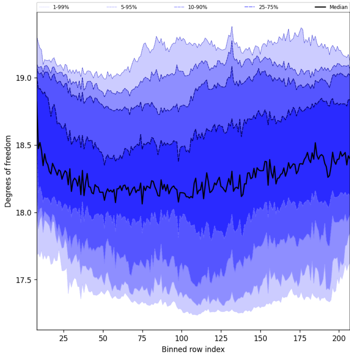
Figure 41: Along track statistics of “Degrees of freedom” for 2025-05-10 to 2025-05-11
