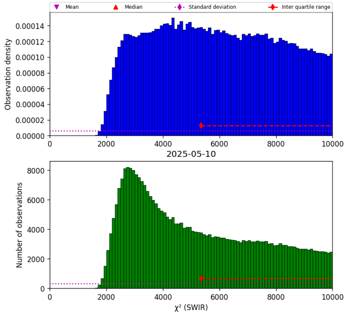
Figure 28: Histogram of “ \chi^2 (SWIR)” for 2025-05-10 to 2025-05-11
