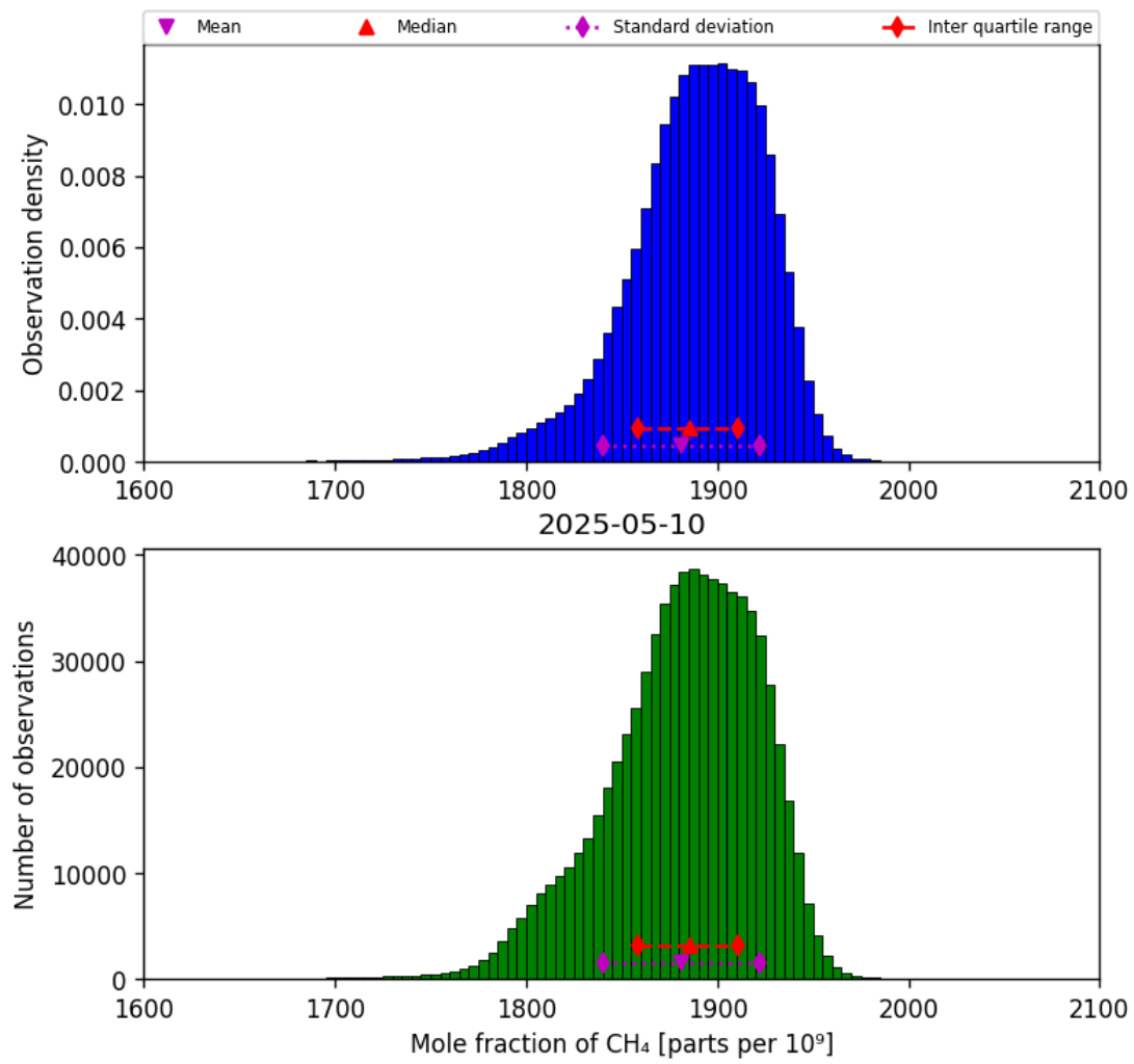
Figure 23: Histogram of “Mole fraction of CH 4 ” for 2025-05-10 to 2025-05-11
