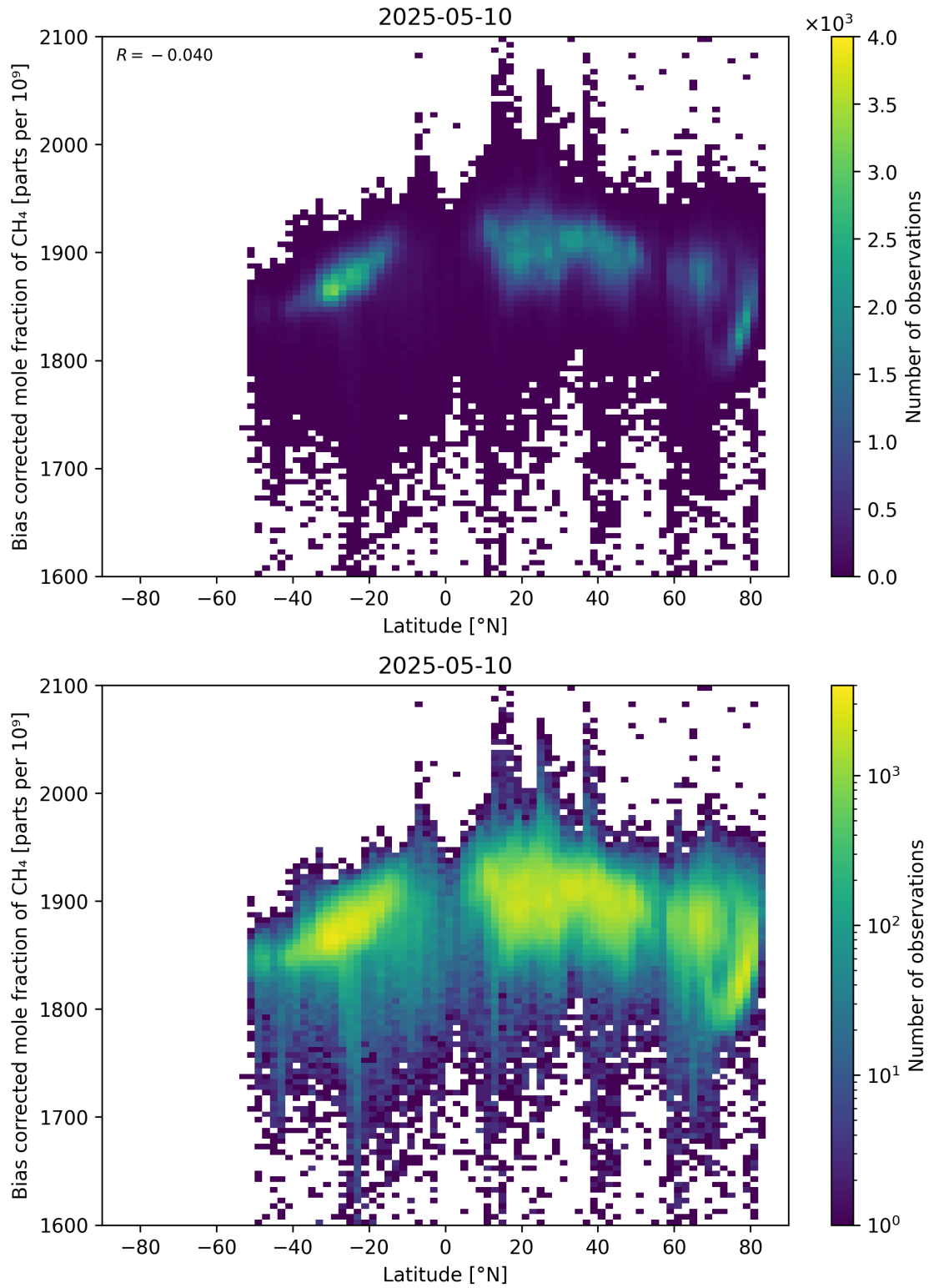
Figure 58: Scatter density plot of “Latitude” against “Bias corrected mole fraction of \text{CH}_4 ” for 2025-05-10 to 2025-05-11.
