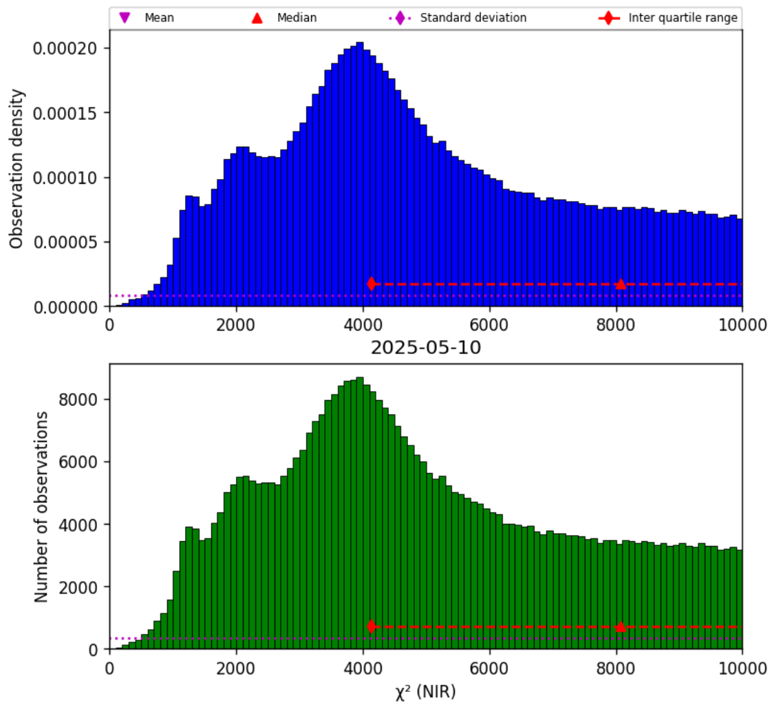
Figure 29: Histogram of “ \chi^2 (NIR)” for 2025-05-10 to 2025-05-11
