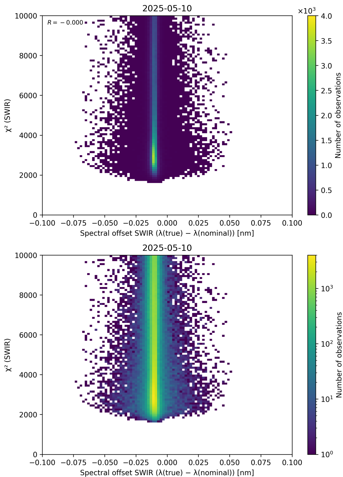
Figure 118: Scatter density plot of “Spectral offset SWIR ( \lambda_{\text{true}} - \lambda_{\text{nominal}} )” against “ \chi^2 (SWIR)” for 2025-05-10 to 2025-05-11.
