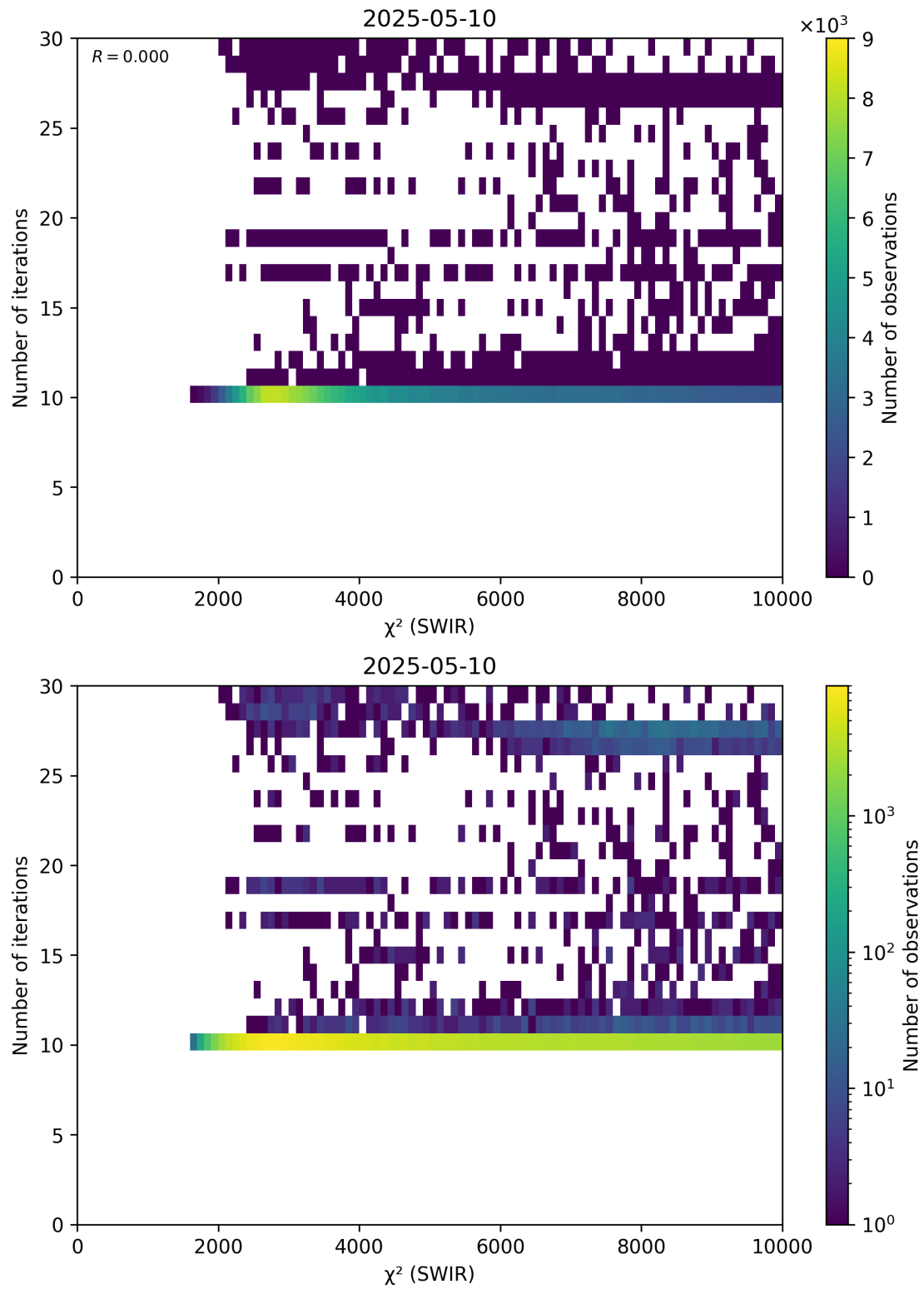
Figure 50: Scatter density plot of “ \chi^2 (SWIR)” against “Number of iterations” for 2025-05-10 to 2025-05-11.
