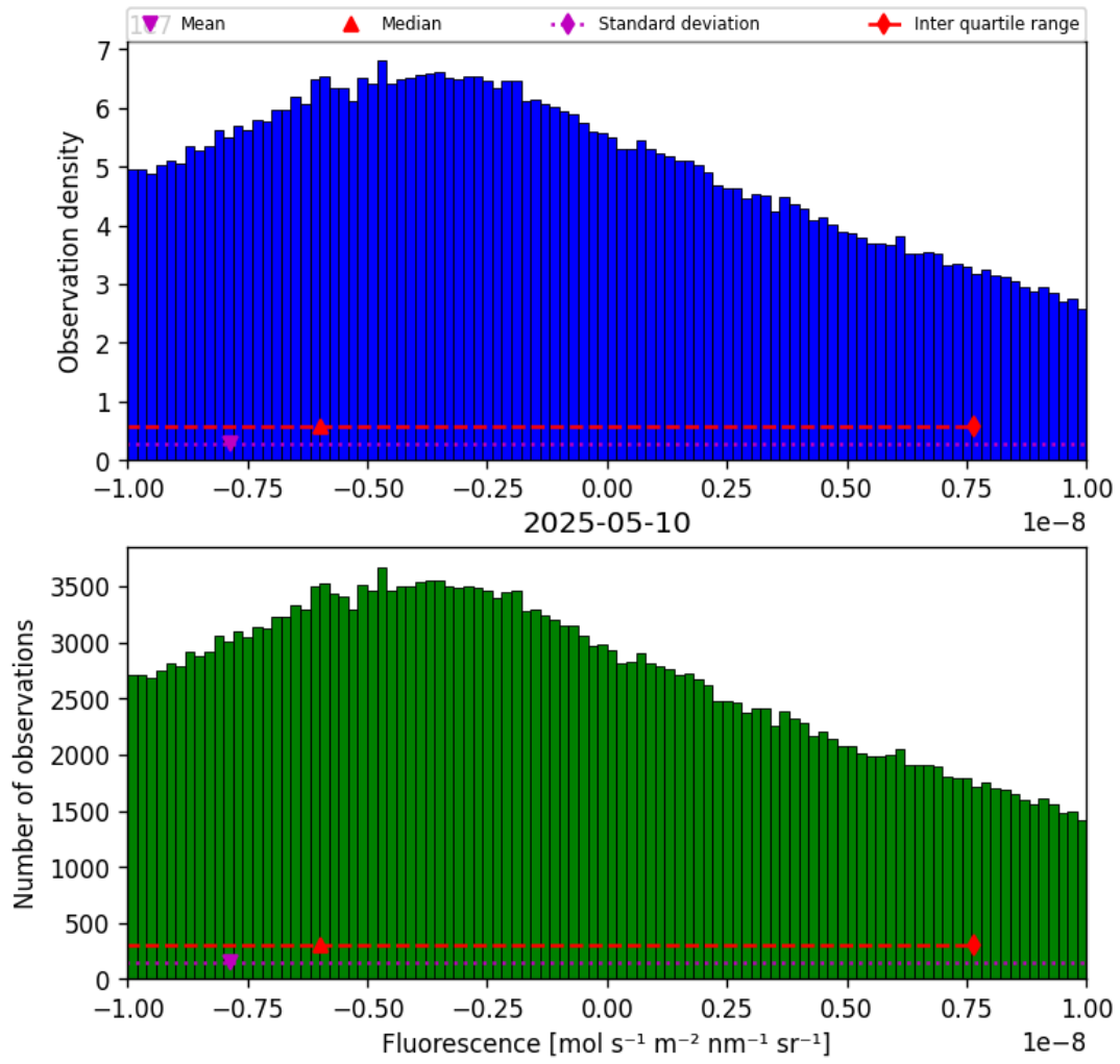
Figure 32: Histogram of “Fluorescence” for 2025-05-10 to 2025-05-11
