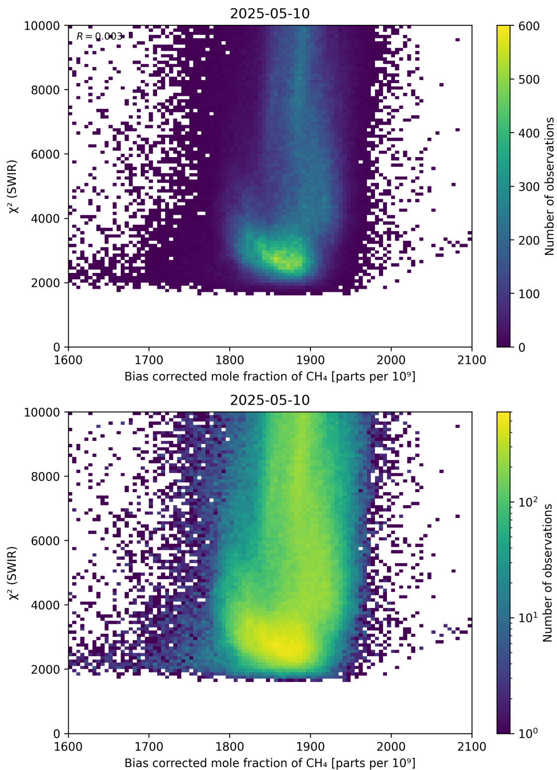
Figure 64: Scatter density plot of “Bias corrected mole fraction of \text{CH}_4 ” against “ \chi^2 (SWIR)” for 2025-05-10 to 2025-05-11.
