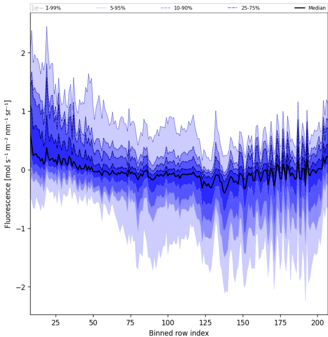
Figure 43: Along track statistics of “Fluorescence” for 2025-05-10 to 2025-05-11
