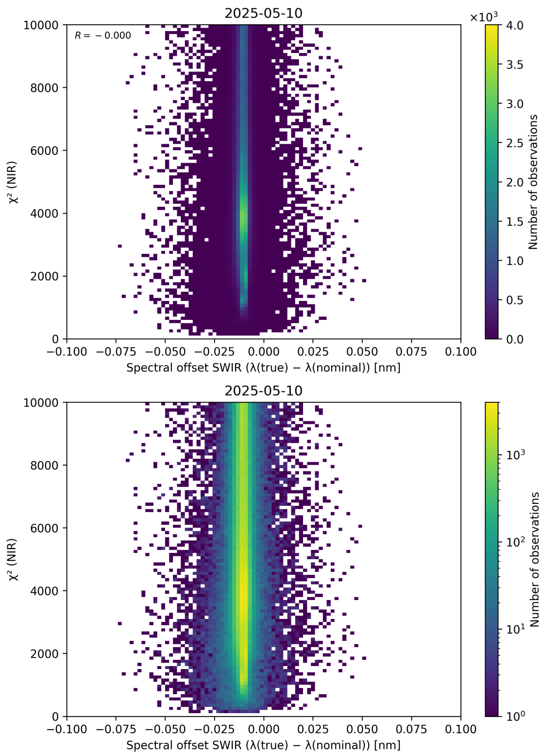
Figure 117: Scatter density plot of “Spectral offset SWIR ( \lambda_{\text{true}} - \lambda_{\text{nominal}} )” against “ \chi^2 (NIR)” for 2025-05-10 to 2025-05-11.
