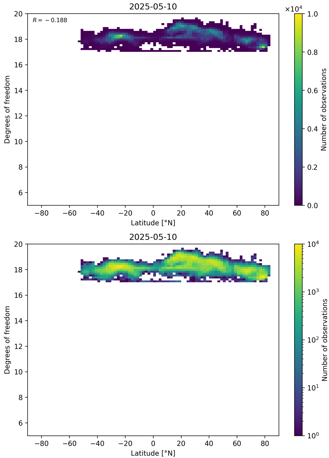
Figure 55: Scatter density plot of “Latitude” against “Degrees of freedom” for 2025-05-10 to 2025-05-11.
