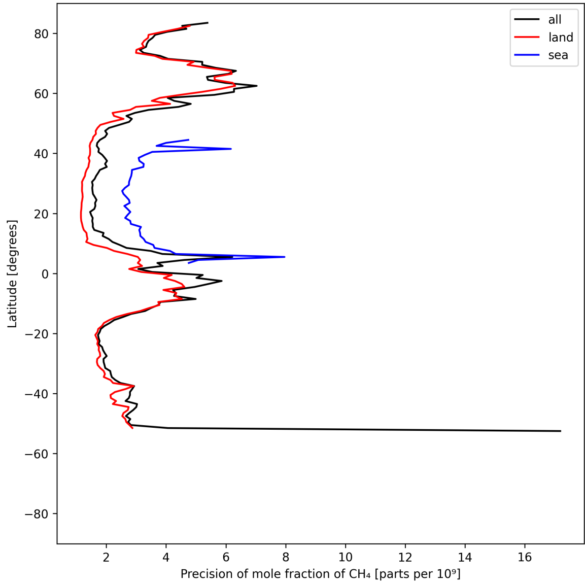
Figure 13: Zonal average of “Precision of mole fraction of CH 4 ” for 2025-05-10 to 2025-05-11.
