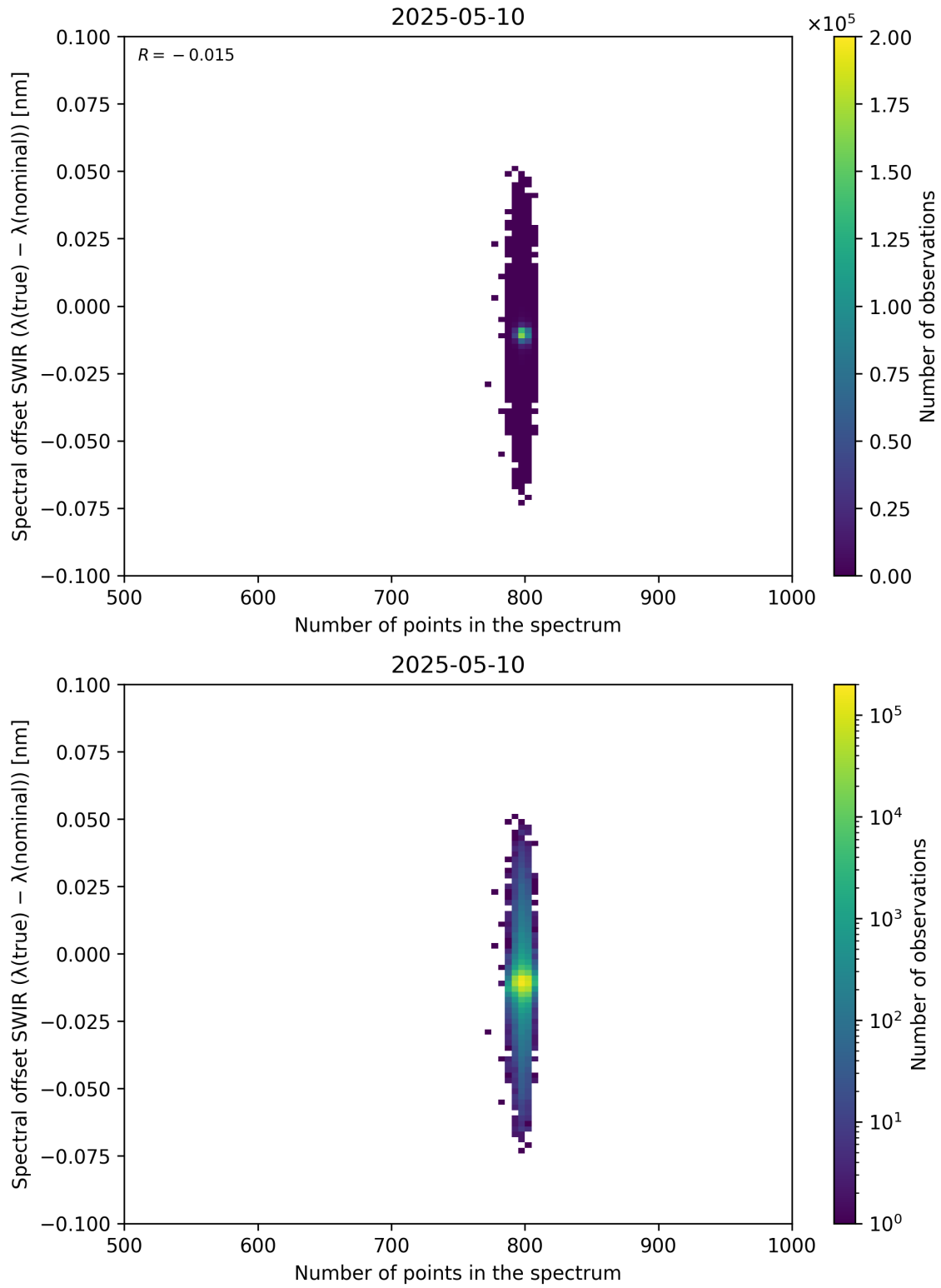
Figure 93: Scatter density plot of “Number of points in the spectrum” against “Spectral offset SWIR ( \lambda_{\text{true}} - \lambda_{\text{nominal}} )” for 2025-05-10 to 2025-05-11.
