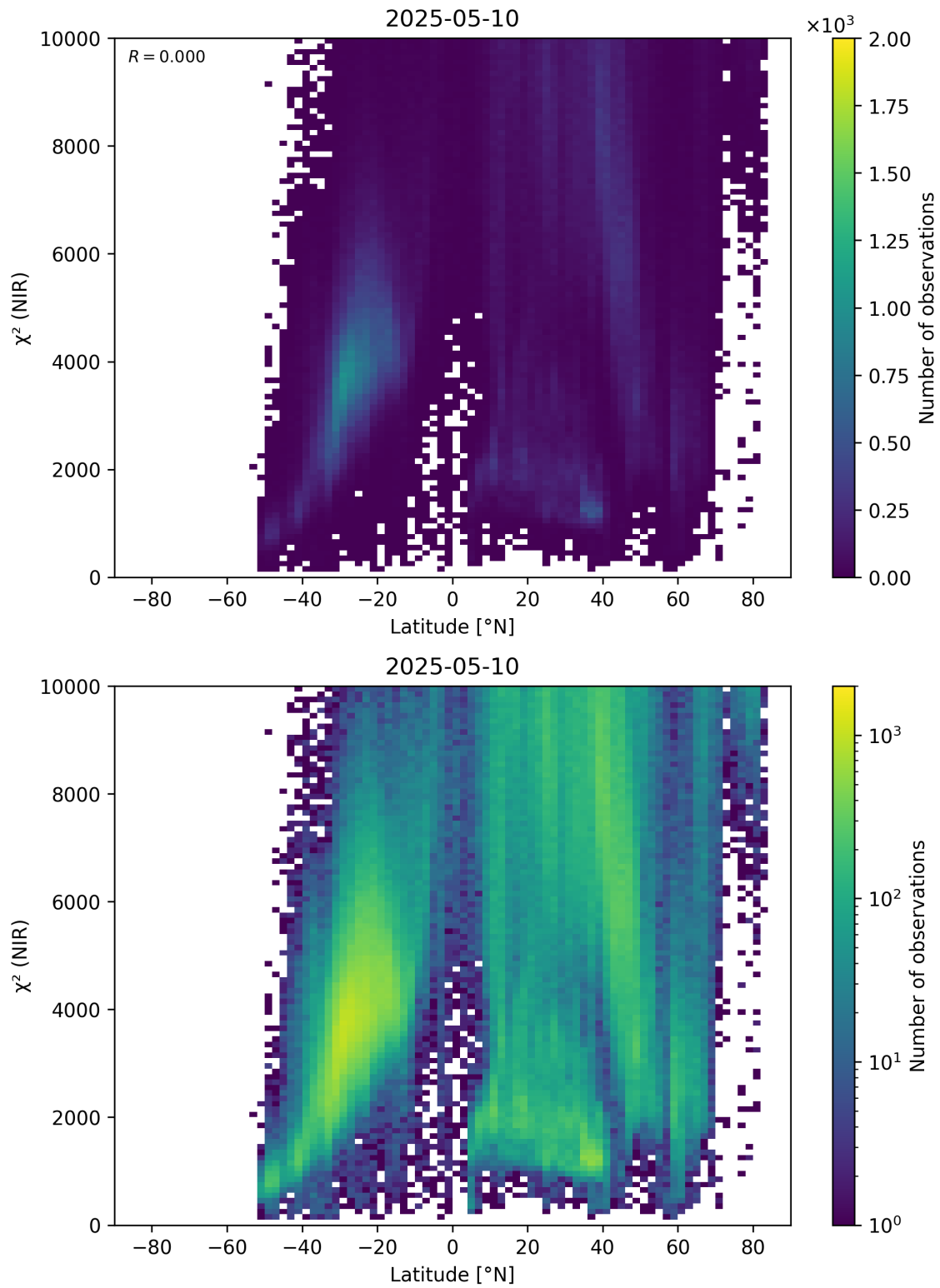
Figure 53: Scatter density plot of “Latitude” against “ \chi^2 (NIR)” for 2025-05-10 to 2025-05-11.
