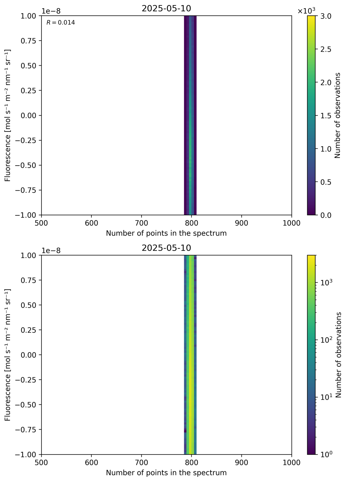
Figure 91: Scatter density plot of “Number of points in the spectrum” against “Fluorescence” for 2025-05-10 to 2025-05-11.
