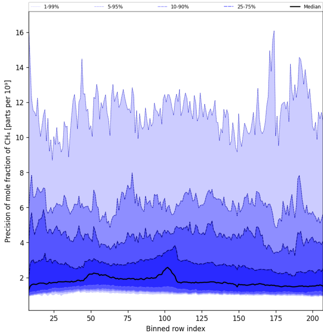
Figure 35: Along track statistics of “Precision of mole fraction of CH 4 ” for 2025-05-10 to 2025-05-11
