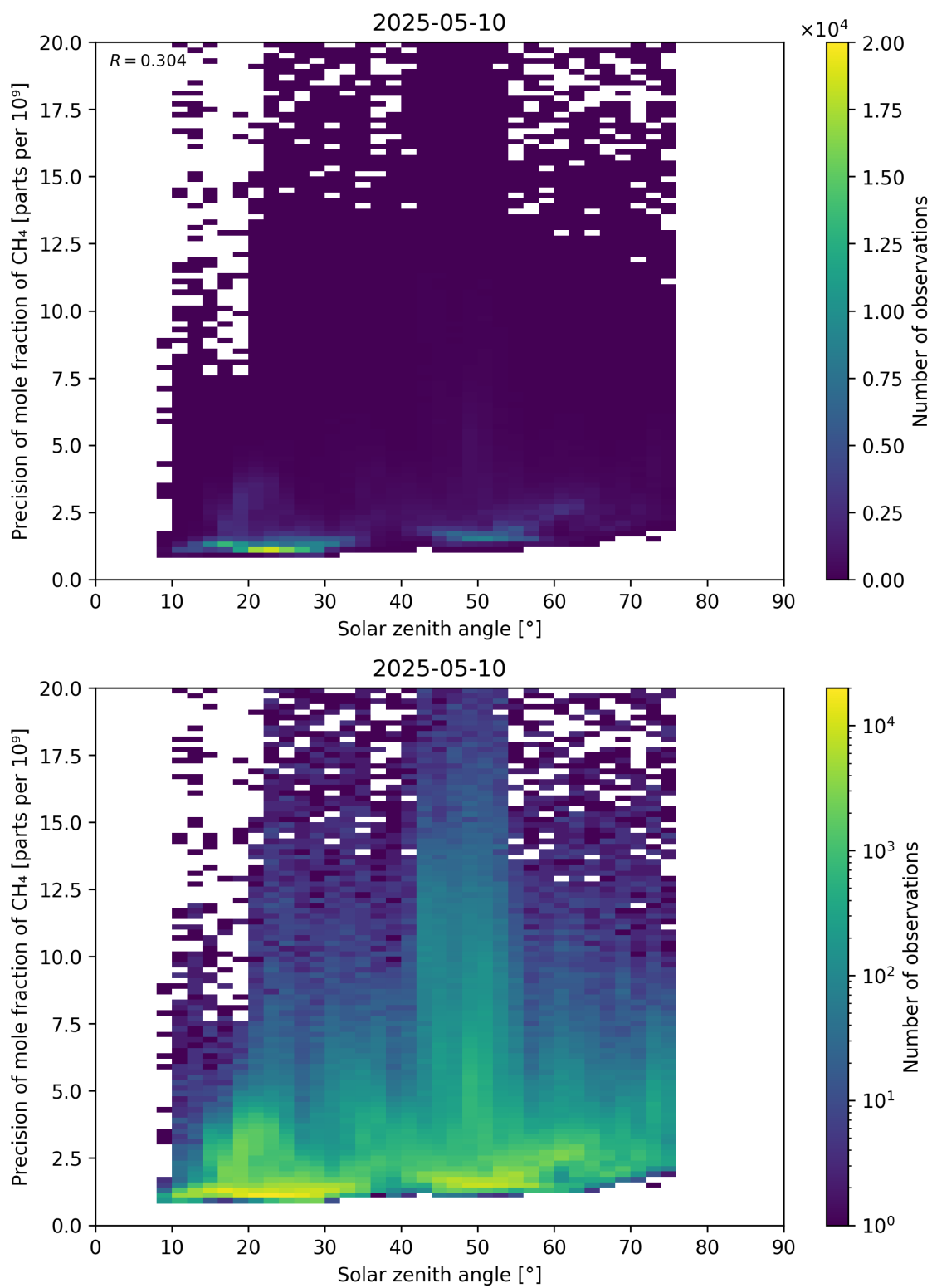
Figure 101: Scatter density plot of “Solar zenith angle” against “Precision of mole fraction of CH 4 ” for 2025-05-10 to 2025-05-11.
