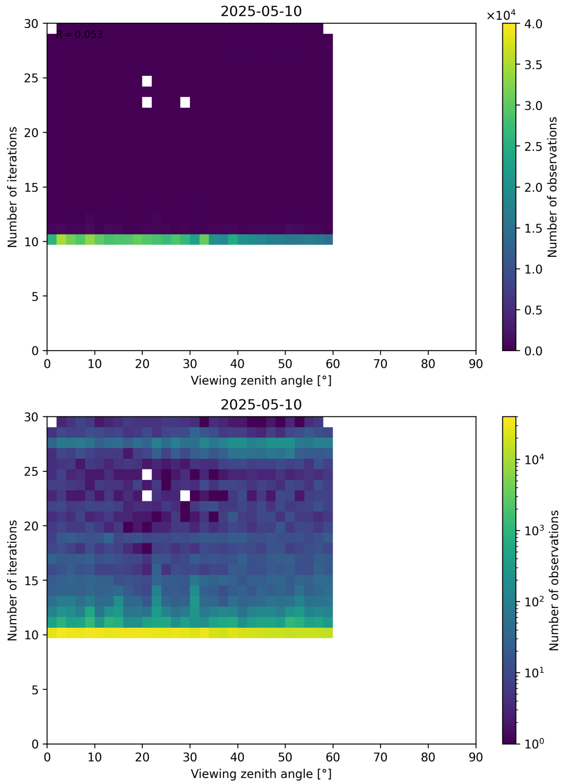
Figure 113: Scatter density plot of “Viewing zenith angle” against “Number of iterations” for 2025-05-10 to 2025-05-11.
