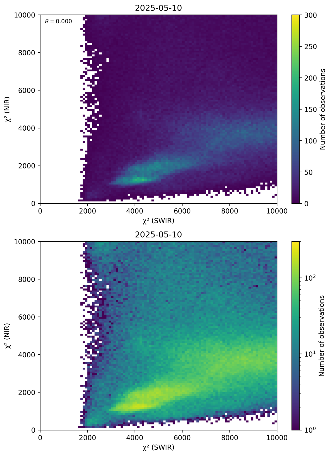
Figure 47: Scatter density plot of “ \chi^2 (SWIR)” against “ \chi^2 (NIR)” for 2025-05-10 to 2025-05-11.
