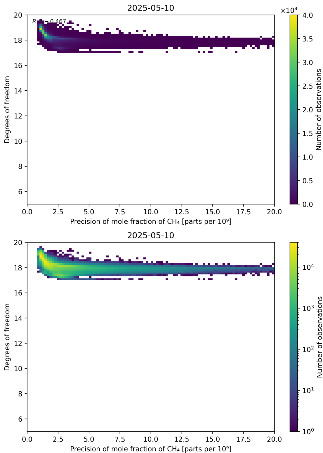
Figure 80: Scatter density plot of “Precision of mole fraction of CH 4 ” against “Degrees of freedom” for 2025-05-10 to 2025-05-11.
