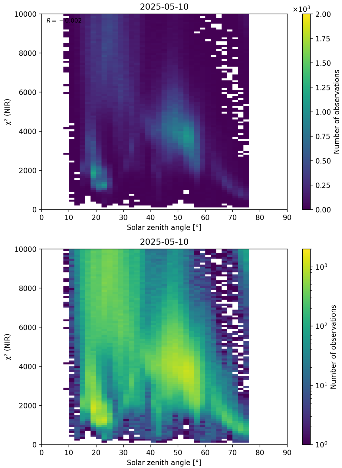
Figure 94: Scatter density plot of “Solar zenith angle” against “ \chi^2 (NIR)” for 2025-05-10 to 2025-05-11.
