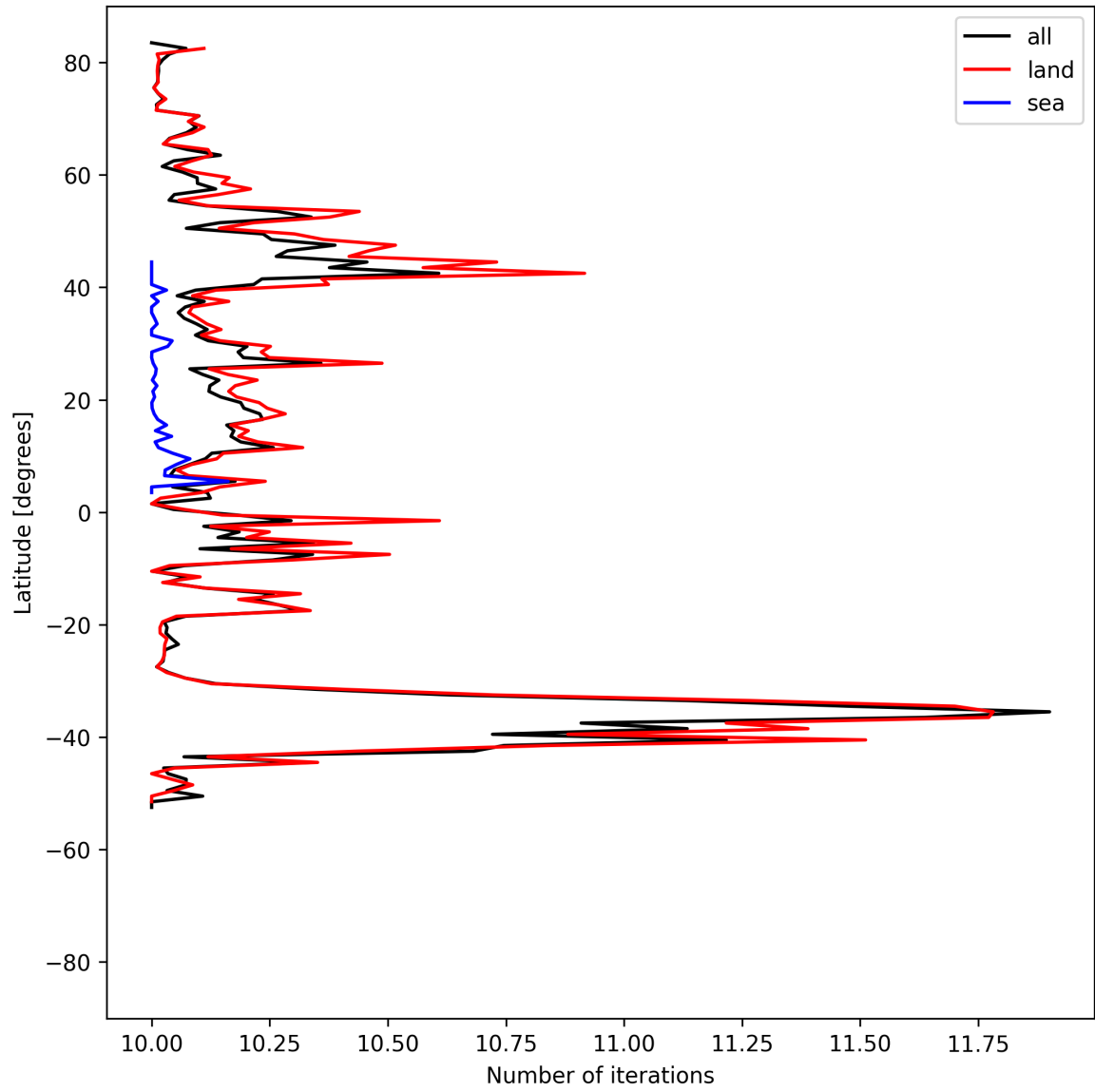
Figure 20: Zonal average of “Number of iterations” for 2025-05-10 to 2025-05-11.
