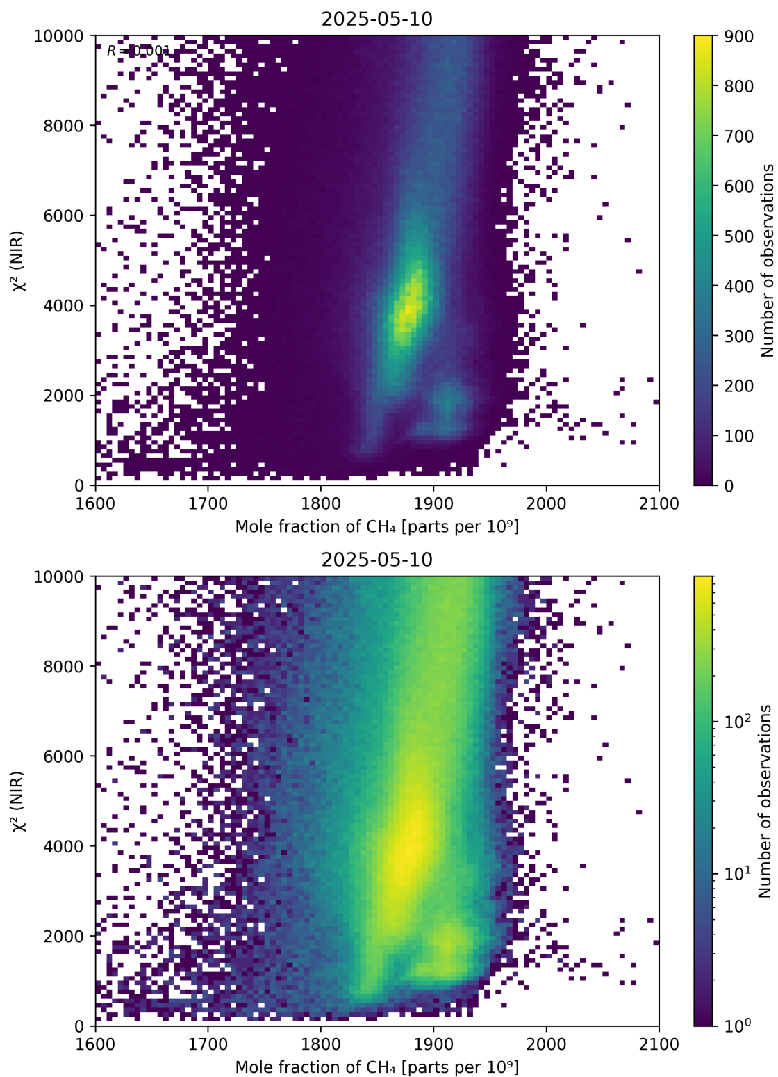
Figure 70: Scatter density plot of “Mole fraction of \text{CH}_4 ” against “ \chi^2 (NIR)” for 2025-05-10 to 2025-05-11.
