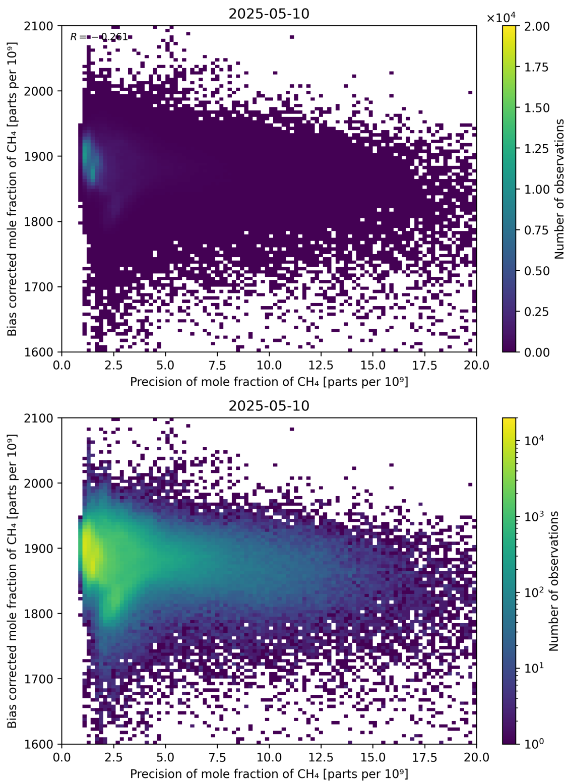
Figure 82: Scatter density plot of “Precision of mole fraction of CH 4 ” against “Bias corrected mole fraction of CH 4 ” for 2025-05-10 to 2025-05-11.
