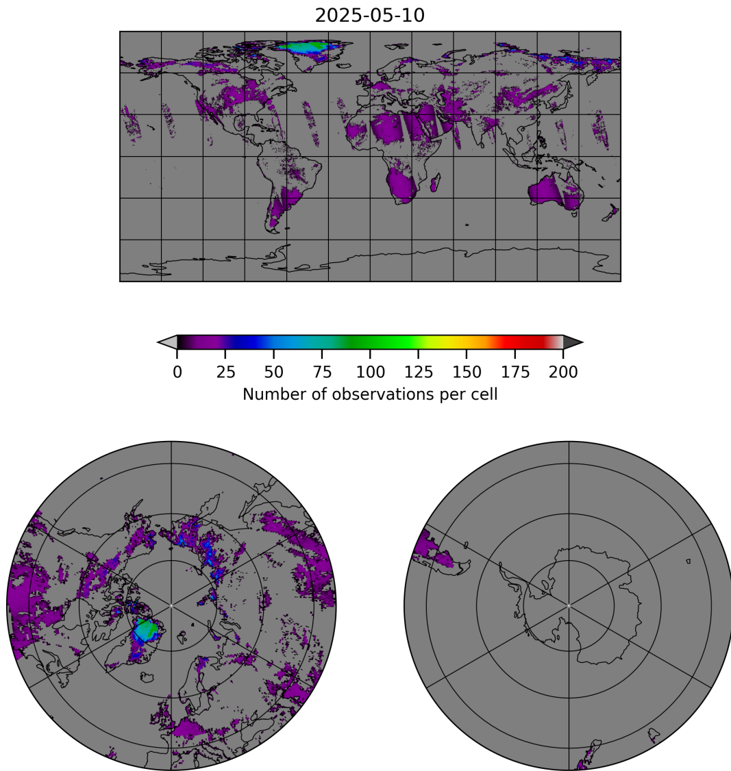
Figure 10: Map of the number of observations for 2025-05-10 to 2025-05-11
