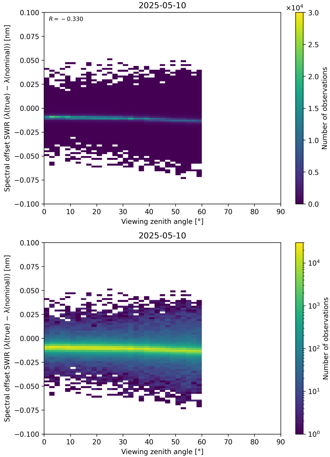
Figure 116: Scatter density plot of “Viewing zenith angle” against “Spectral offset SWIR ( \lambda_{\text{true}} - \lambda_{\text{nominal}} )” for 2025-05-10 to 2025-05-11.
