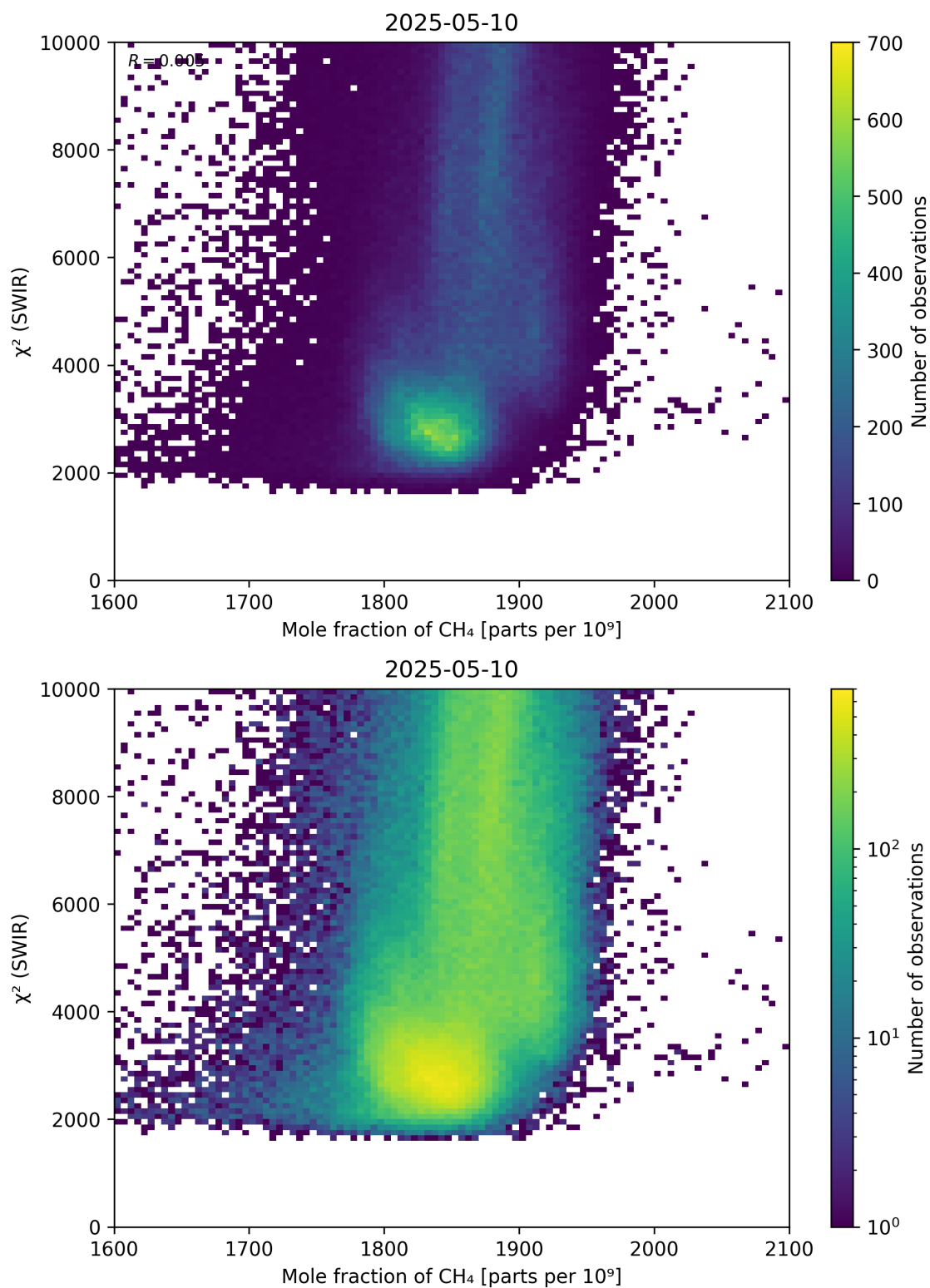
Figure 71: Scatter density plot of “Mole fraction of \text{CH}_4 ” against “ \chi^2 (SWIR)” for 2025-05-10 to 2025-05-11.
