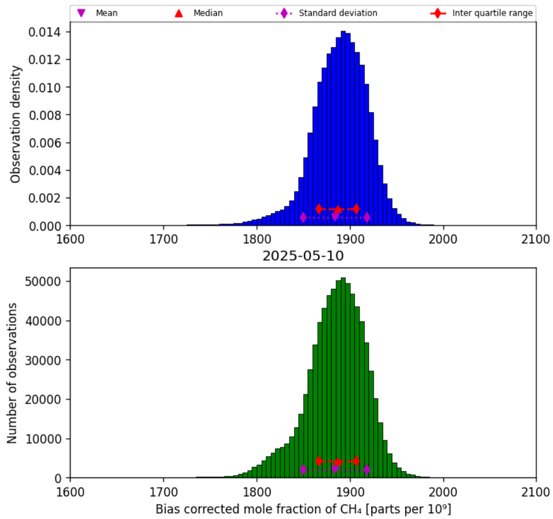
Figure 25: Histogram of “Bias corrected mole fraction of CH 4 ” for 2025-05-10 to 2025-05-11
