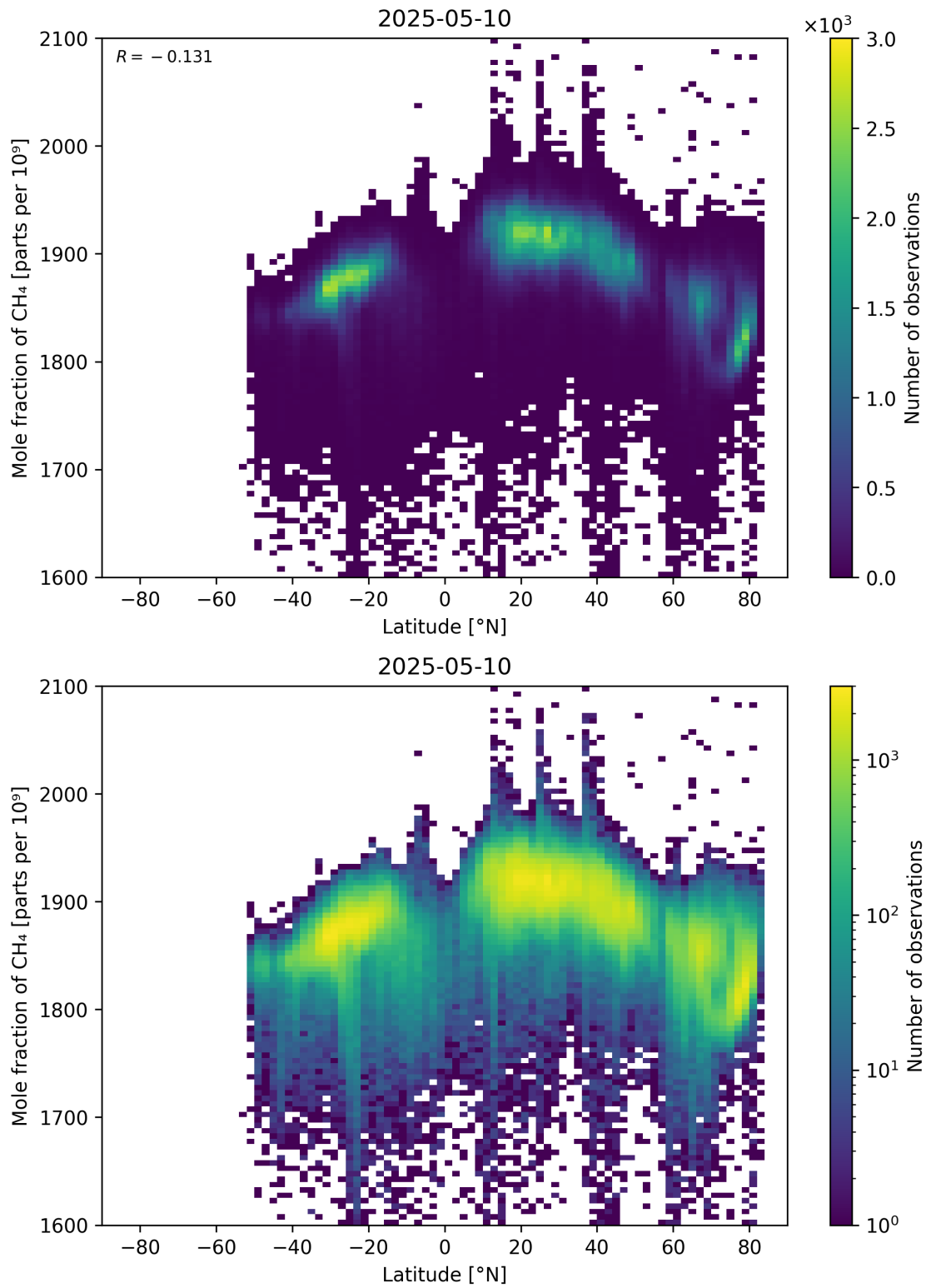
Figure 57: Scatter density plot of “Latitude” against “Mole fraction of CH 4 ” for 2025-05-10 to 2025-05-11.
