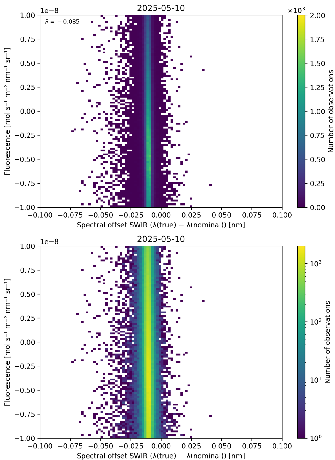
Figure 120: Scatter density plot of “Spectral offset SWIR ( \lambda_{\text{true}} - \lambda_{\text{nominal}} )” against “Fluorescence” for 2025-05-10 to 2025-05-11.
