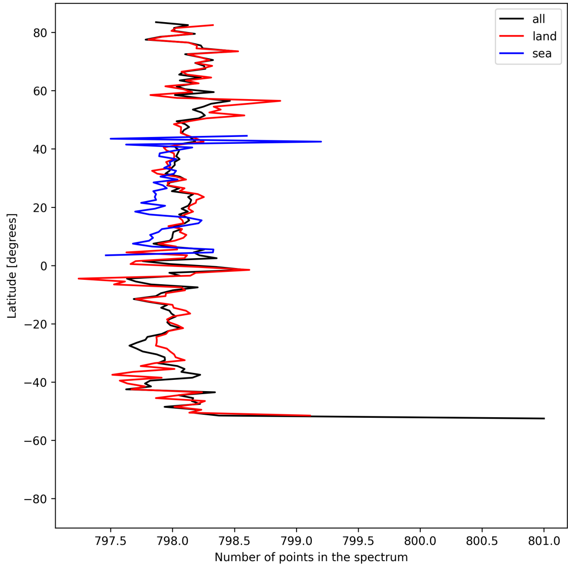
Figure 15: Zonal average of “Number of points in the spectrum” for 2025-05-10 to 2025-05-11.
