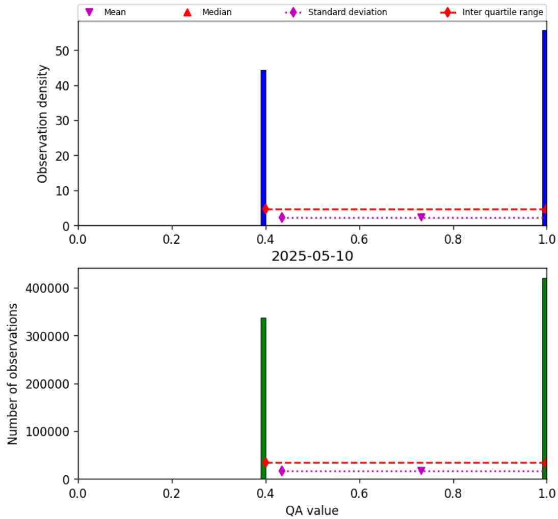
Figure 22: Histogram of “QA value” for 2025-05-10 to 2025-05-11
