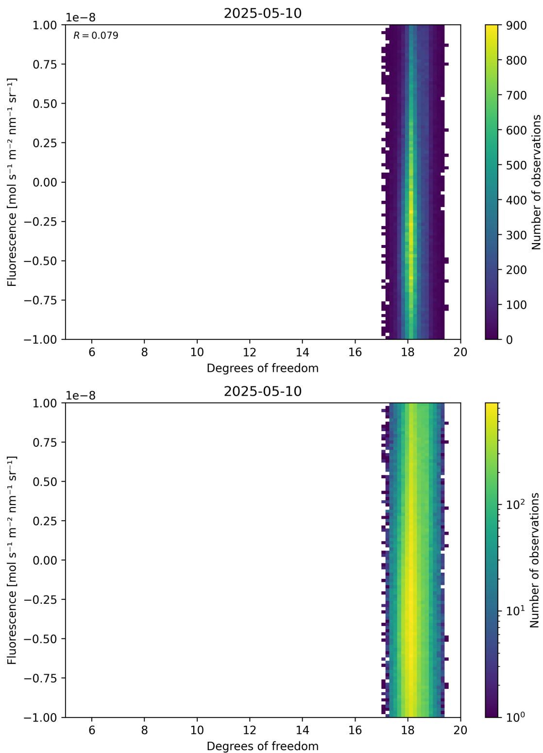
Figure 51: Scatter density plot of “Degrees of freedom” against “Fluorescence” for 2025-05-10 to 2025-05-11.
