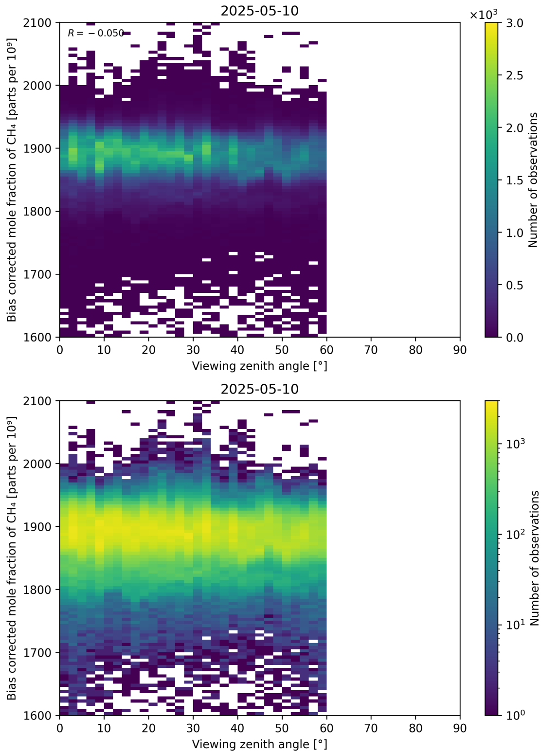
Figure 111: Scatter density plot of “Viewing zenith angle” against “Bias corrected mole fraction of CH 4 ” for 2025-05-10 to 2025-05-11.
