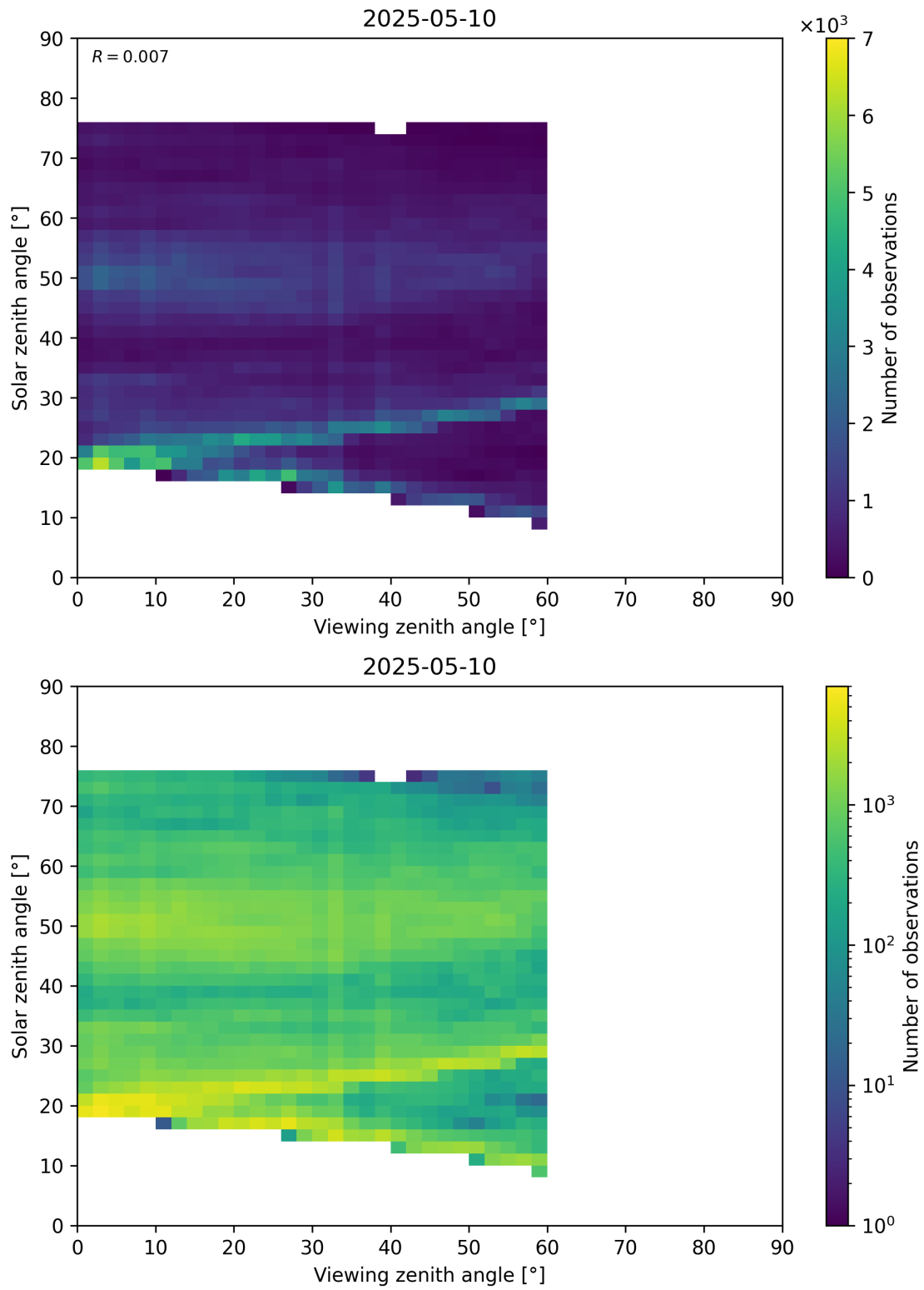
Figure 115: Scatter density plot of “Viewing zenith angle” against “Solar zenith angle” for 2025-05-10 to 2025-05-11.
