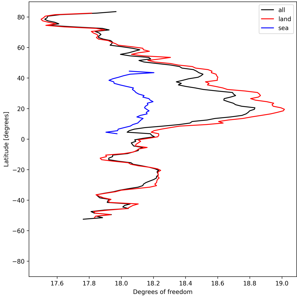
Figure 19: Zonal average of “Degrees of freedom” for 2025-05-10 to 2025-05-11.
