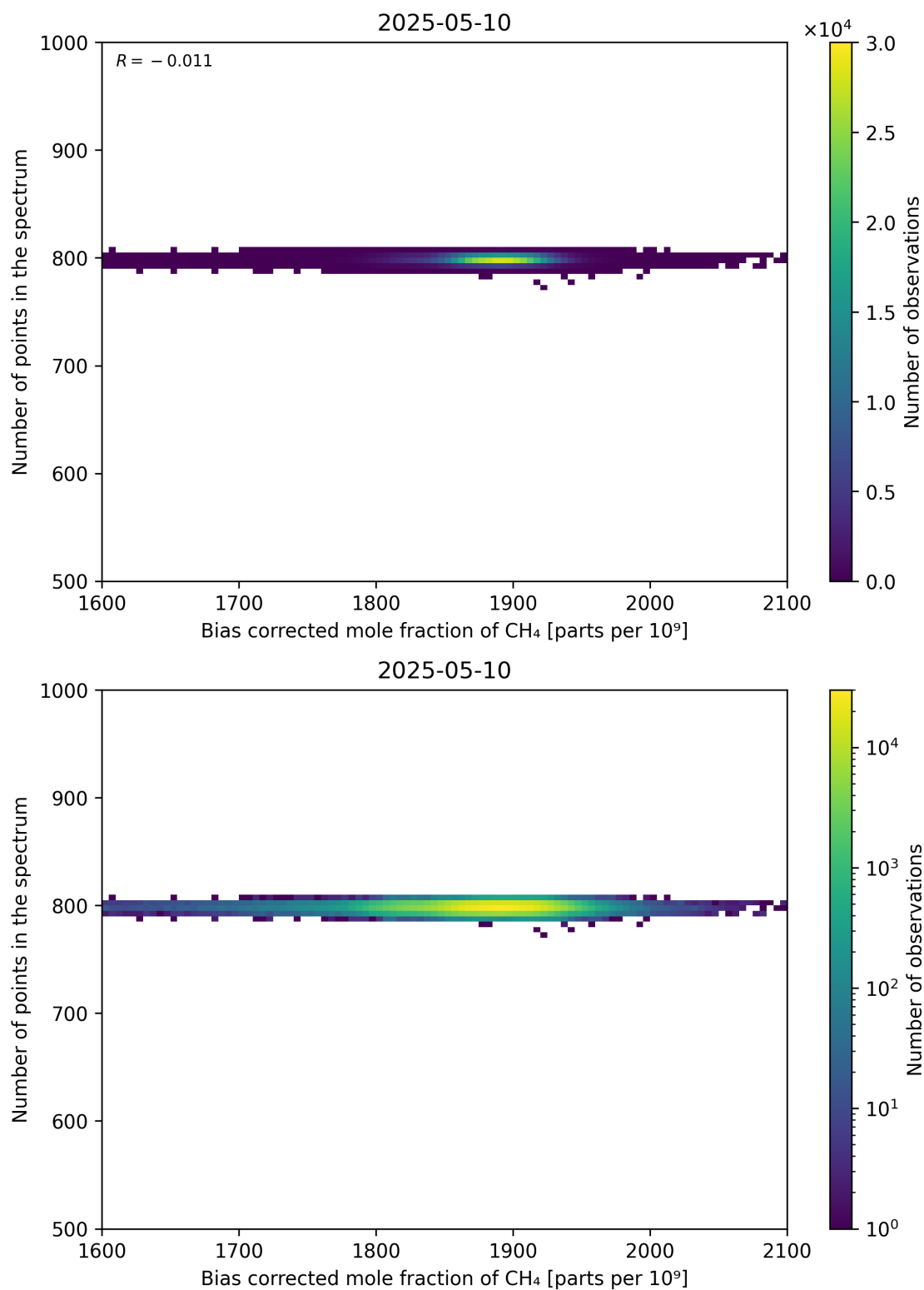
Figure 68: Scatter density plot of “Bias corrected mole fraction of CH 4 ” against “Number of points in the spectrum” for 2025-05-10 to 2025-05-11.
