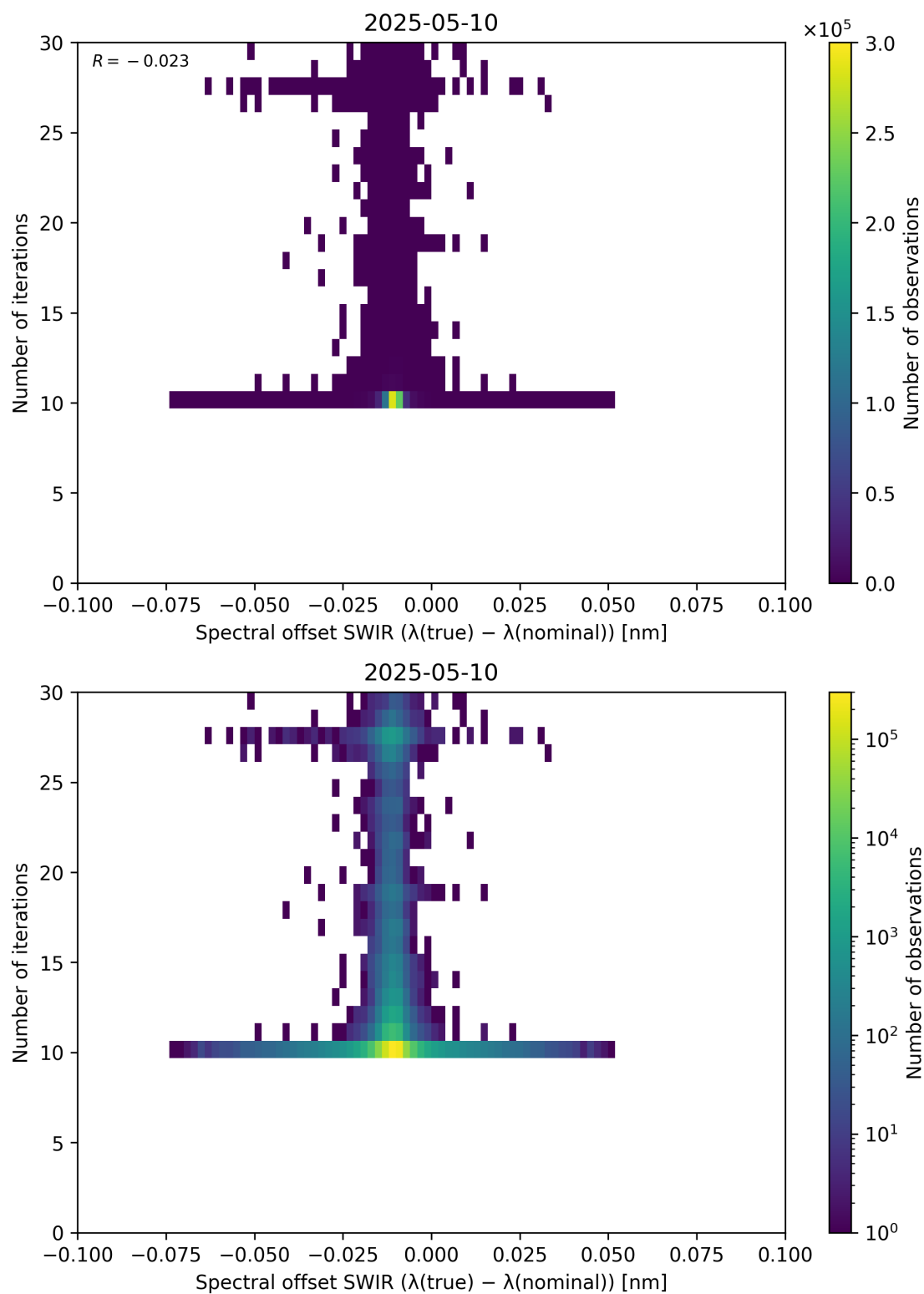
Figure 121: Scatter density plot of “Spectral offset SWIR ( \lambda_{\text{true}} - \lambda_{\text{nominal}} )” against “Number of iterations” for 2025-05-10 to 2025-05-11.
