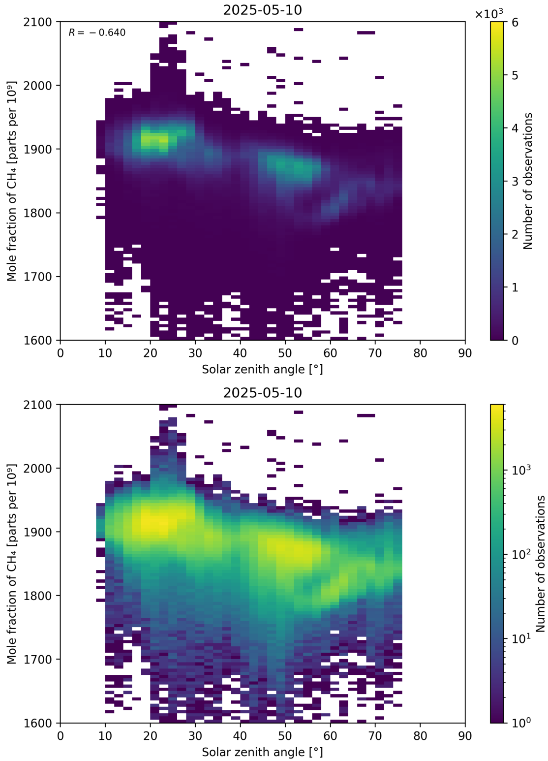
Figure 99: Scatter density plot of “Solar zenith angle” against “Mole fraction of CH 4 ” for 2025-05-10 to 2025-05-11.
