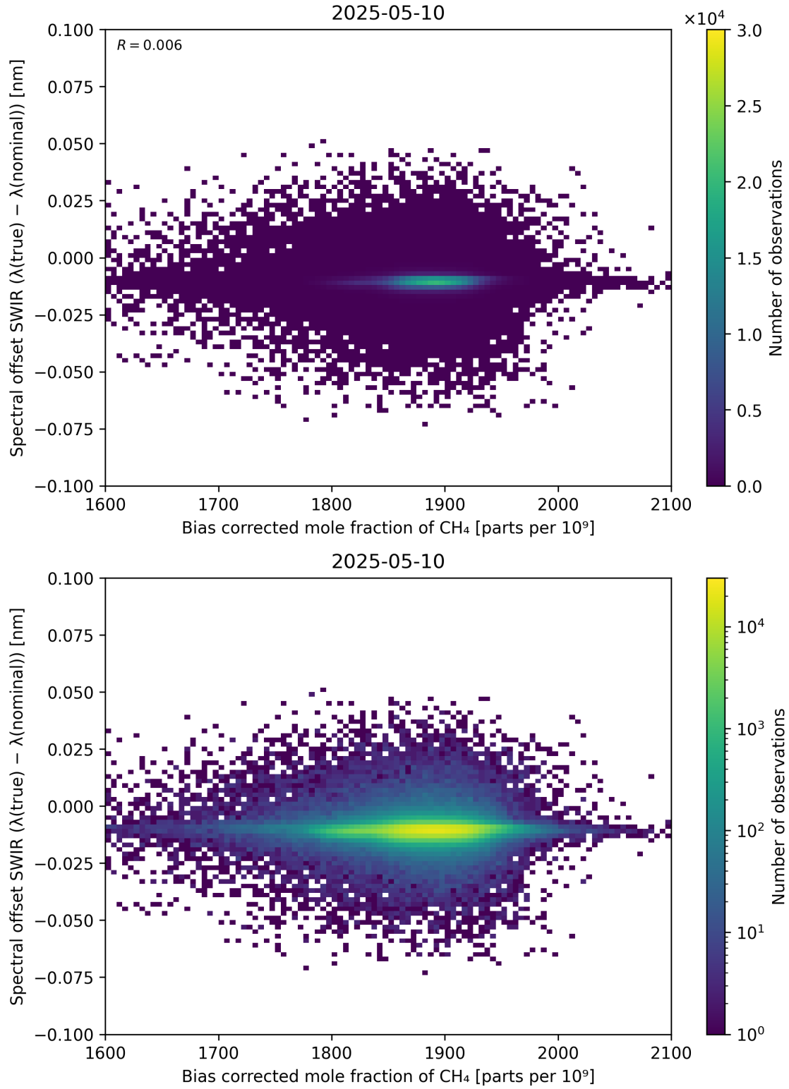
Figure 69: Scatter density plot of “Bias corrected mole fraction of CH 4 ” against “Spectral offset SWIR ( \lambda_{\text{true}} - \lambda_{\text{nominal}} )” for 2025-05-10 to 2025-05-11.
