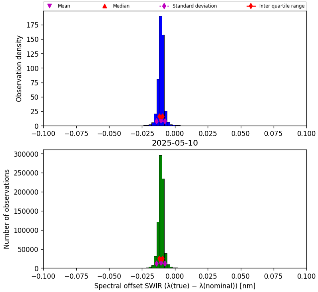
Figure 27: Histogram of “Spectral offset SWIR ( \lambda_{\text{true}} - \lambda_{\text{nominal}} )” for 2025-05-10 to 2025-05-11
