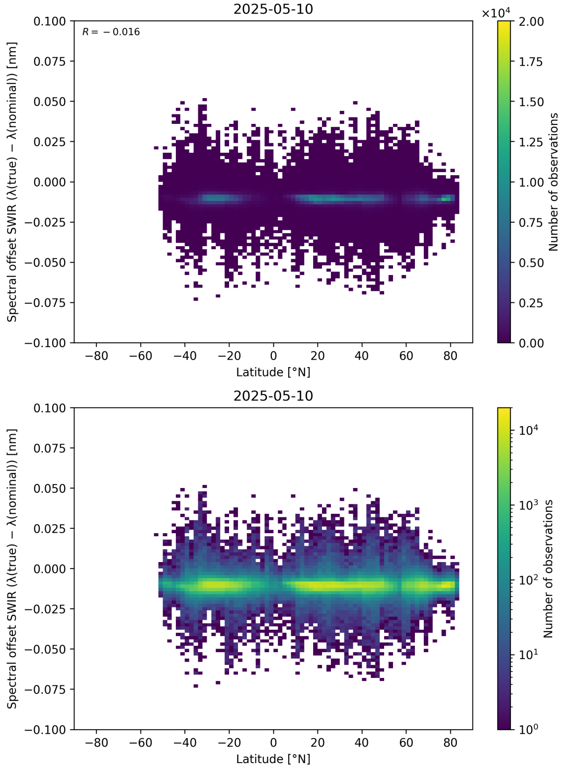
Figure 62: Scatter density plot of “Latitude” against “Spectral offset SWIR ( \lambda_{\text{true}} - \lambda_{\text{nominal}} )” for 2025-05-10 to 2025-05-11.
