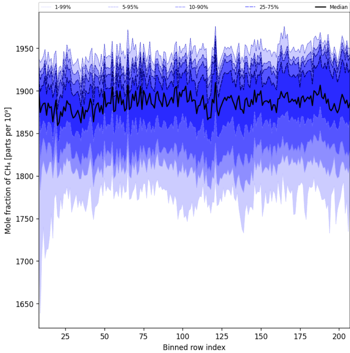
Figure 34: Along track statistics of “Mole fraction of CH 4 ” for 2025-05-10 to 2025-05-11
