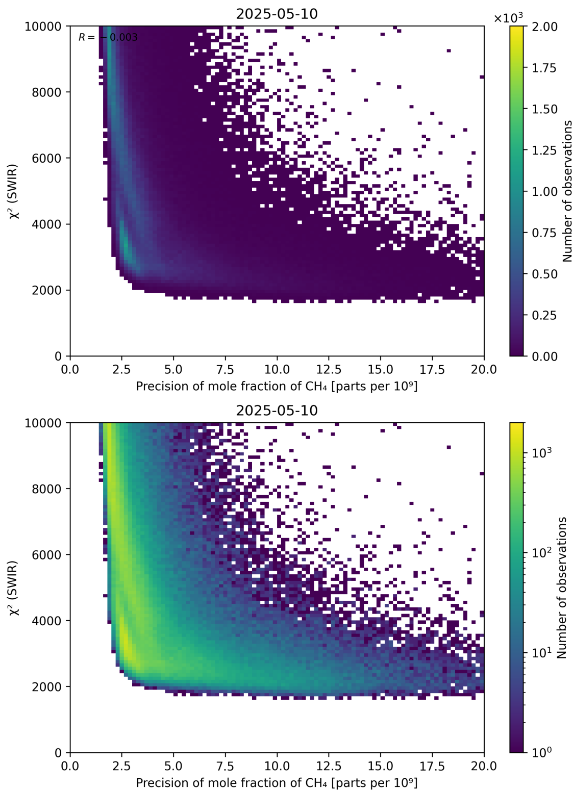
Figure 79: Scatter density plot of “Precision of mole fraction of \text{CH}_4 ” against “ \chi^2 (SWIR)” for 2025-05-10 to 2025-05-11.
