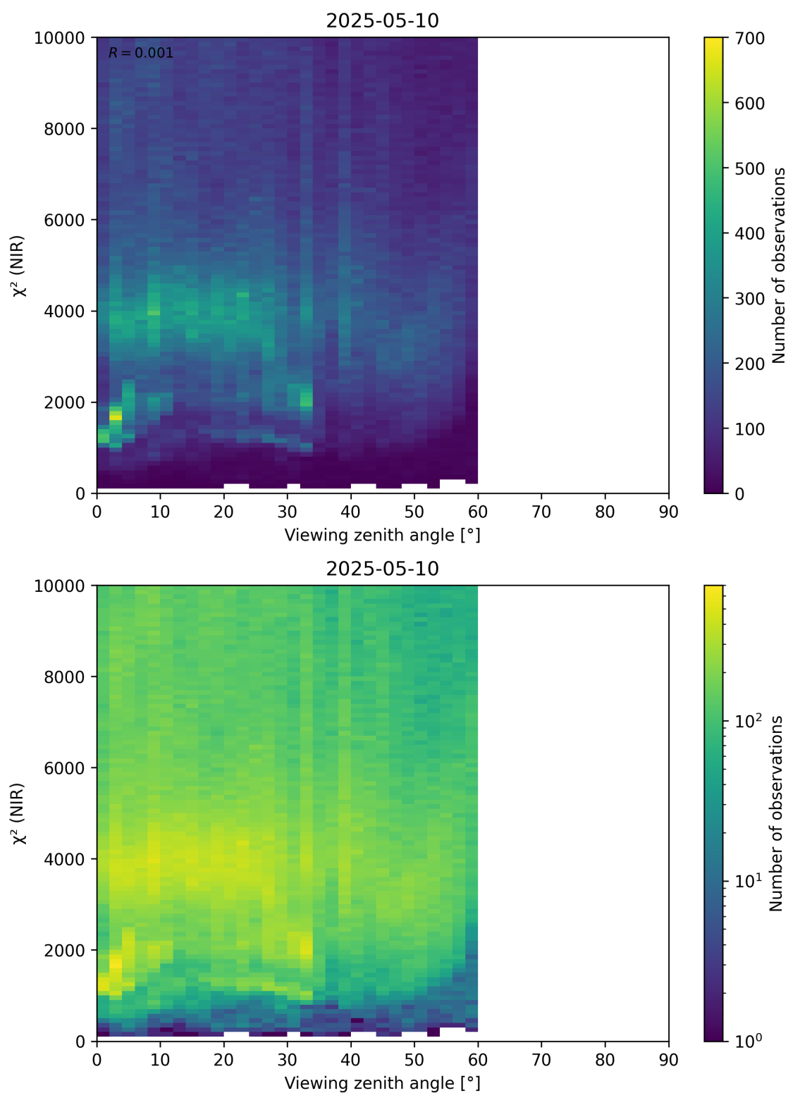
Figure 105: Scatter density plot of “Viewing zenith angle” against “ \chi^2 (NIR)” for 2025-05-10 to 2025-05-11.
