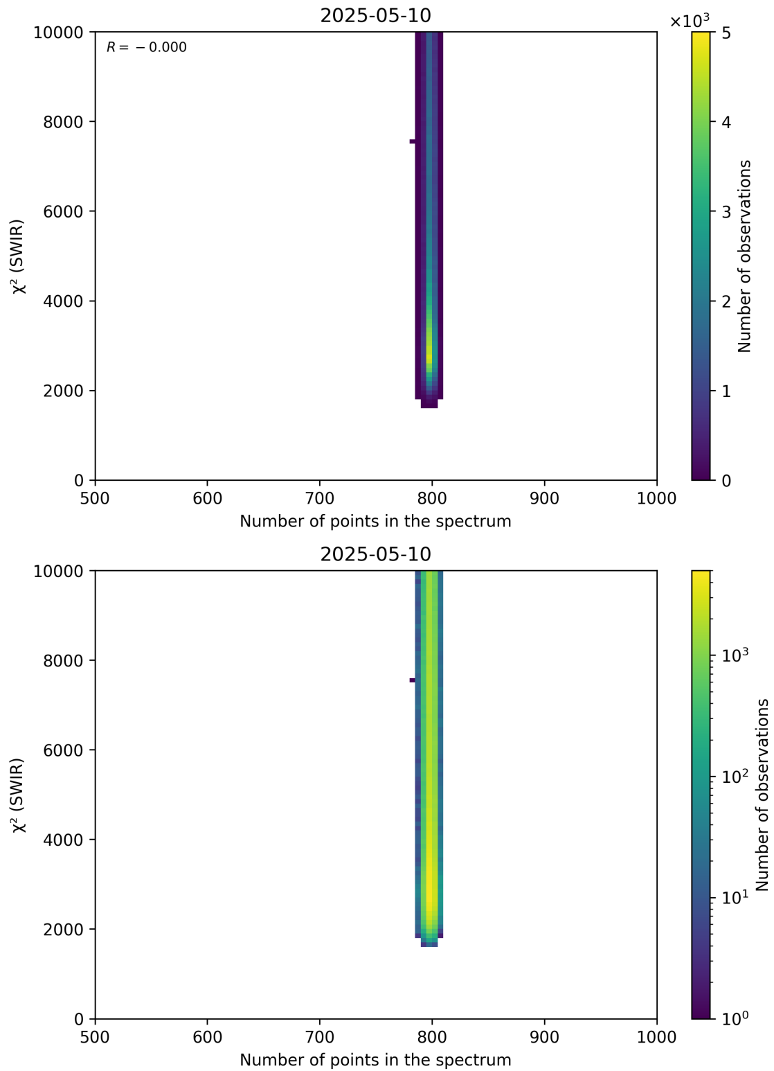
Figure 89: Scatter density plot of “Number of points in the spectrum” against “ \chi^2 (SWIR)” for 2025-05-10 to 2025-05-11.
