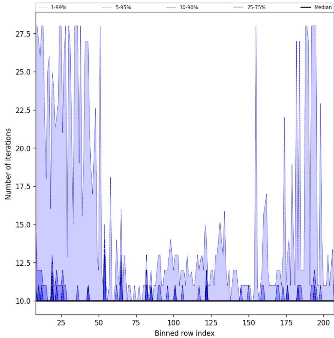
Figure 42: Along track statistics of “Number of iterations” for 2025-05-10 to 2025-05-11
