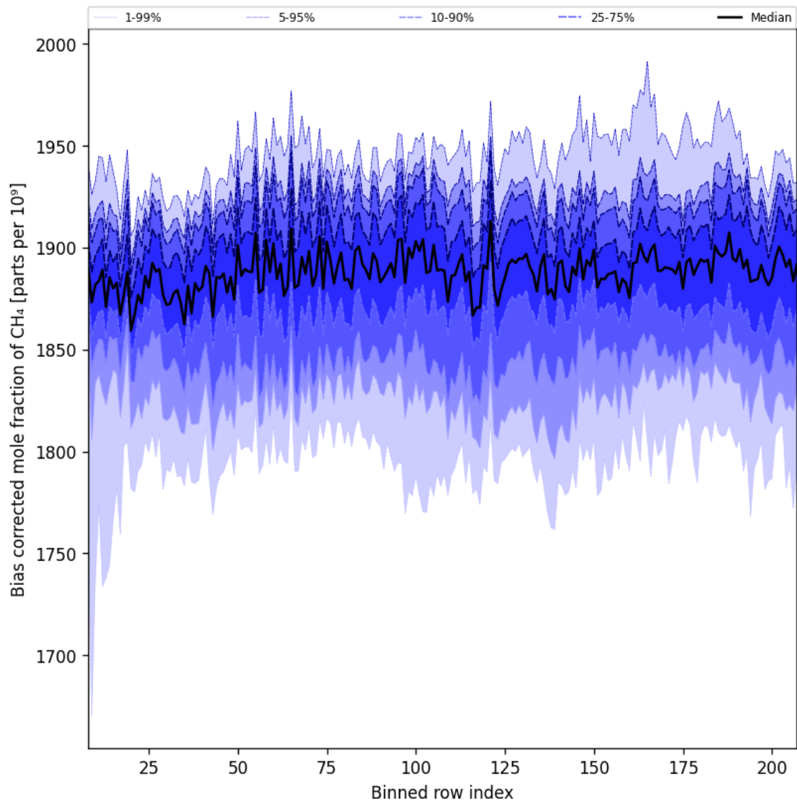
Figure 36: Along track statistics of “Bias corrected mole fraction of CH 4 ” for 2025-05-10 to 2025-05-11
