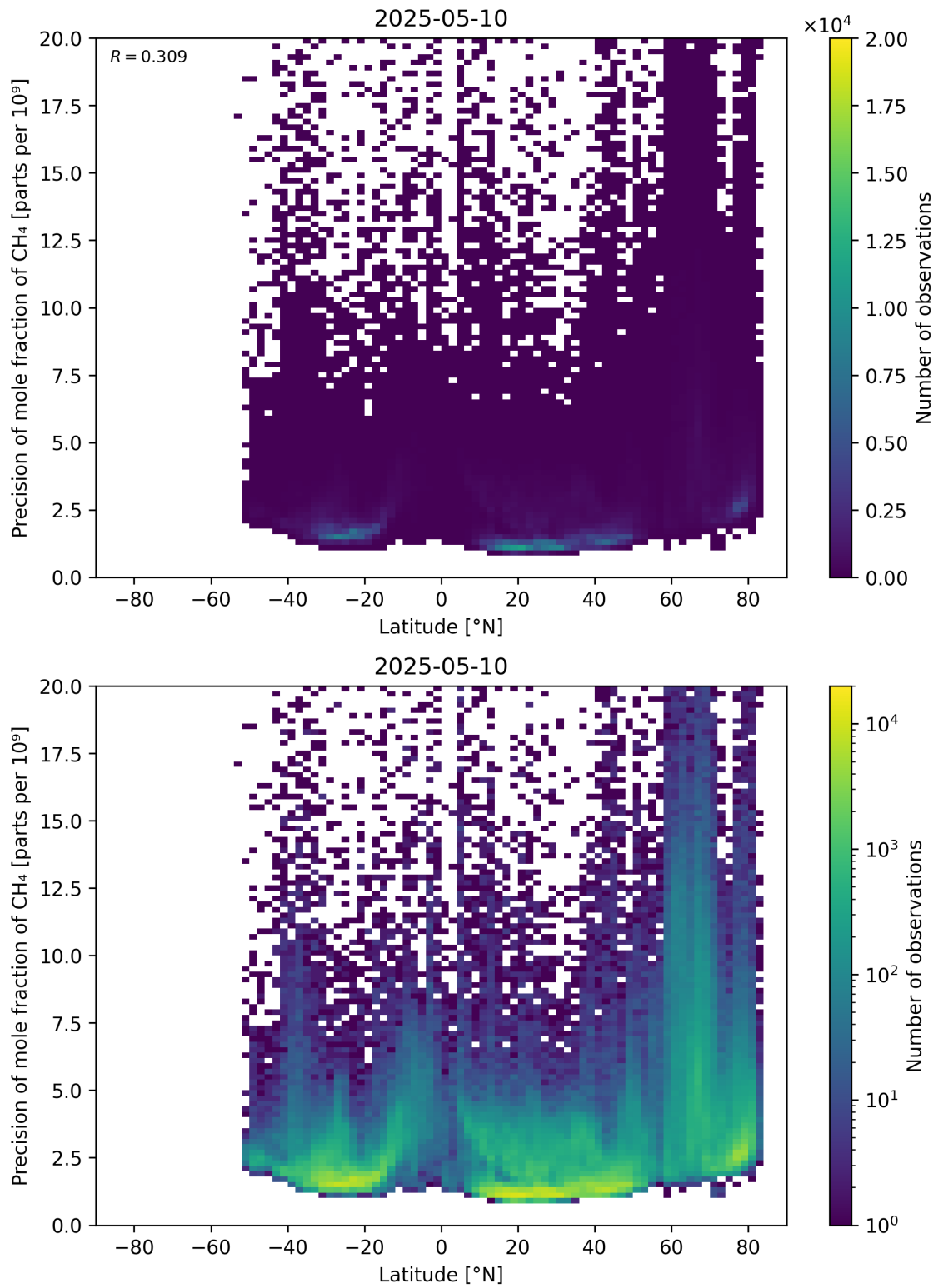
Figure 59: Scatter density plot of “Latitude” against “Precision of mole fraction of \text{CH}_4 ” for 2025-05-10 to 2025-05-11.
