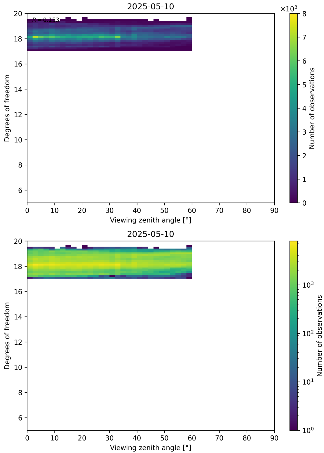
Figure 107: Scatter density plot of “Viewing zenith angle” against “Degrees of freedom” for 2025-05-10 to 2025-05-11.
