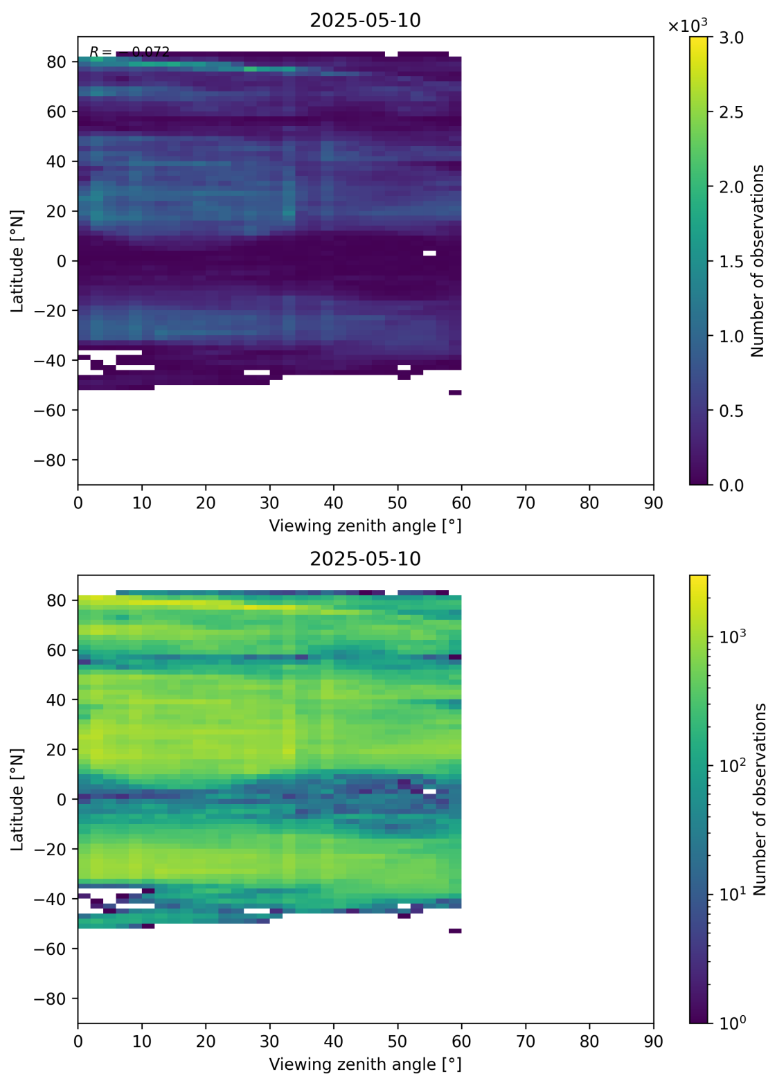
Figure 109: Scatter density plot of “Viewing zenith angle” against “Latitude” for 2025-05-10 to 2025-05-11.
