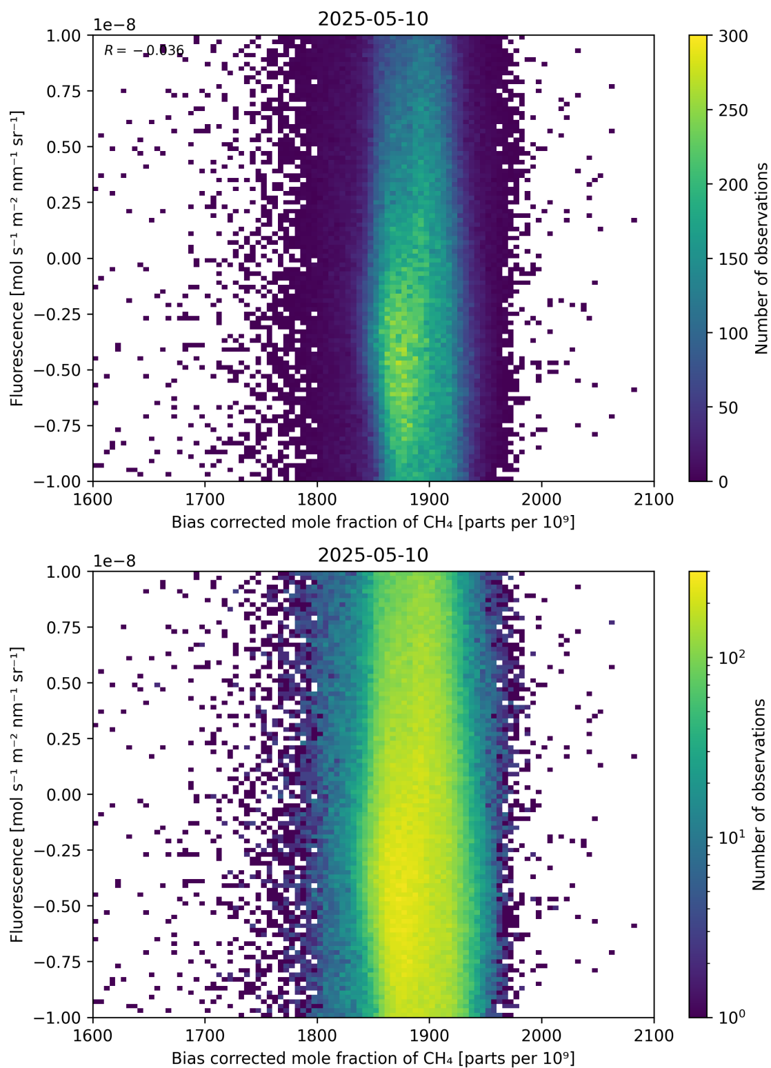
Figure 66: Scatter density plot of “Bias corrected mole fraction of \text{CH}_4 ” against “Fluorescence” for 2025-05-10 to 2025-05-11.
