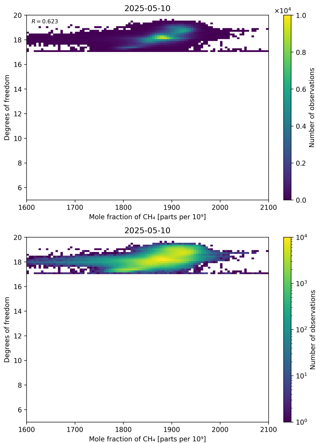
Figure 72: Scatter density plot of “Mole fraction of CH 4 ” against “Degrees of freedom” for 2025-05-10 to 2025-05-11.
