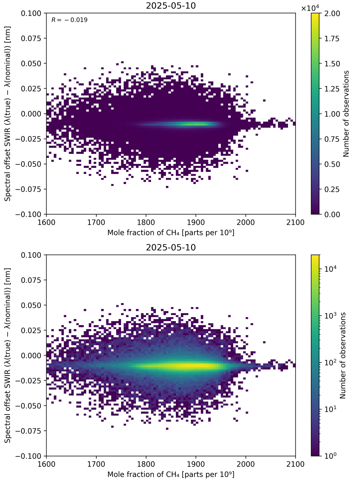
Figure 86: Scatter density plot of “Mole fraction of \text{CH}_4 ” against “Spectral offset SWIR ( \lambda_{\text{true}} - \lambda_{\text{nominal}} )” for 2025-05-10 to 2025-05-11.
