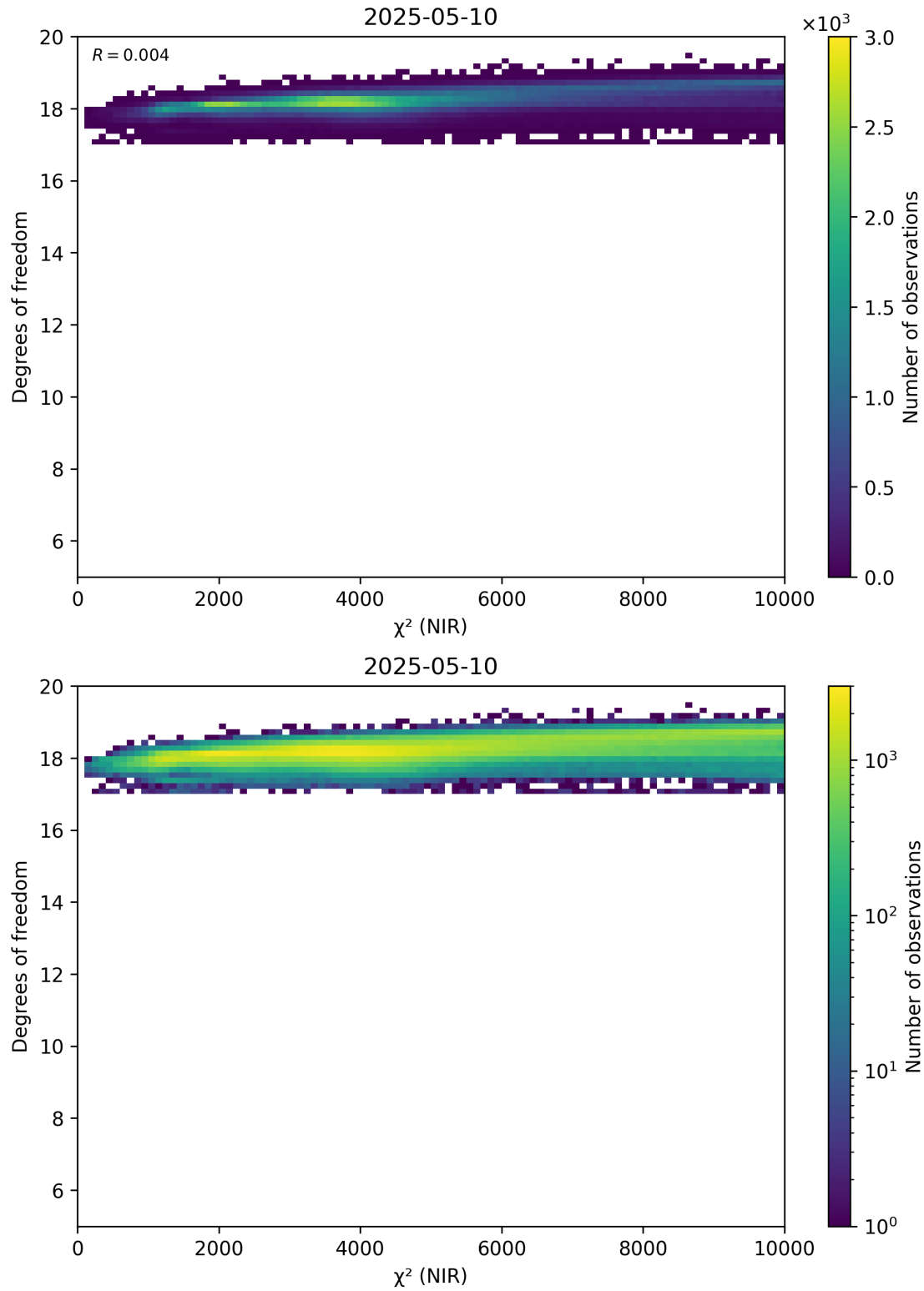
Figure 44: Scatter density plot of “ \chi^2 (NIR)” against “Degrees of freedom” for 2025-05-10 to 2025-05-11.
