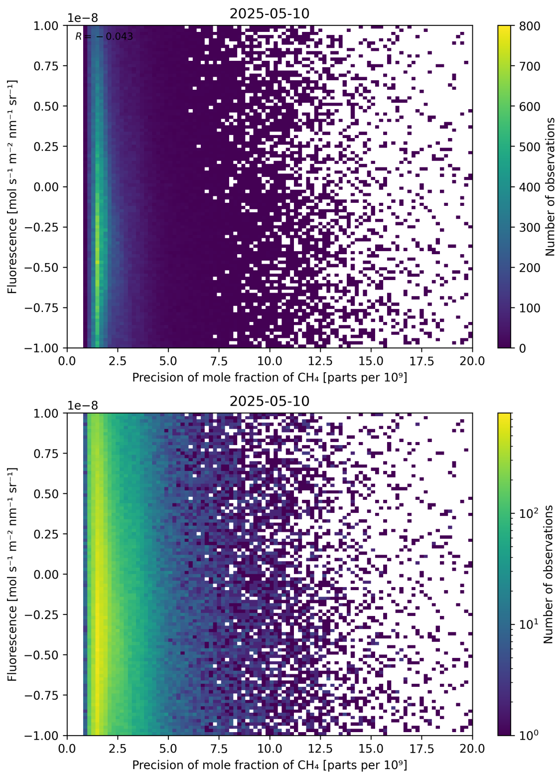
Figure 81: Scatter density plot of “Precision of mole fraction of \text{CH}_4 ” against “Fluorescence” for 2025-05-10 to 2025-05-11.
