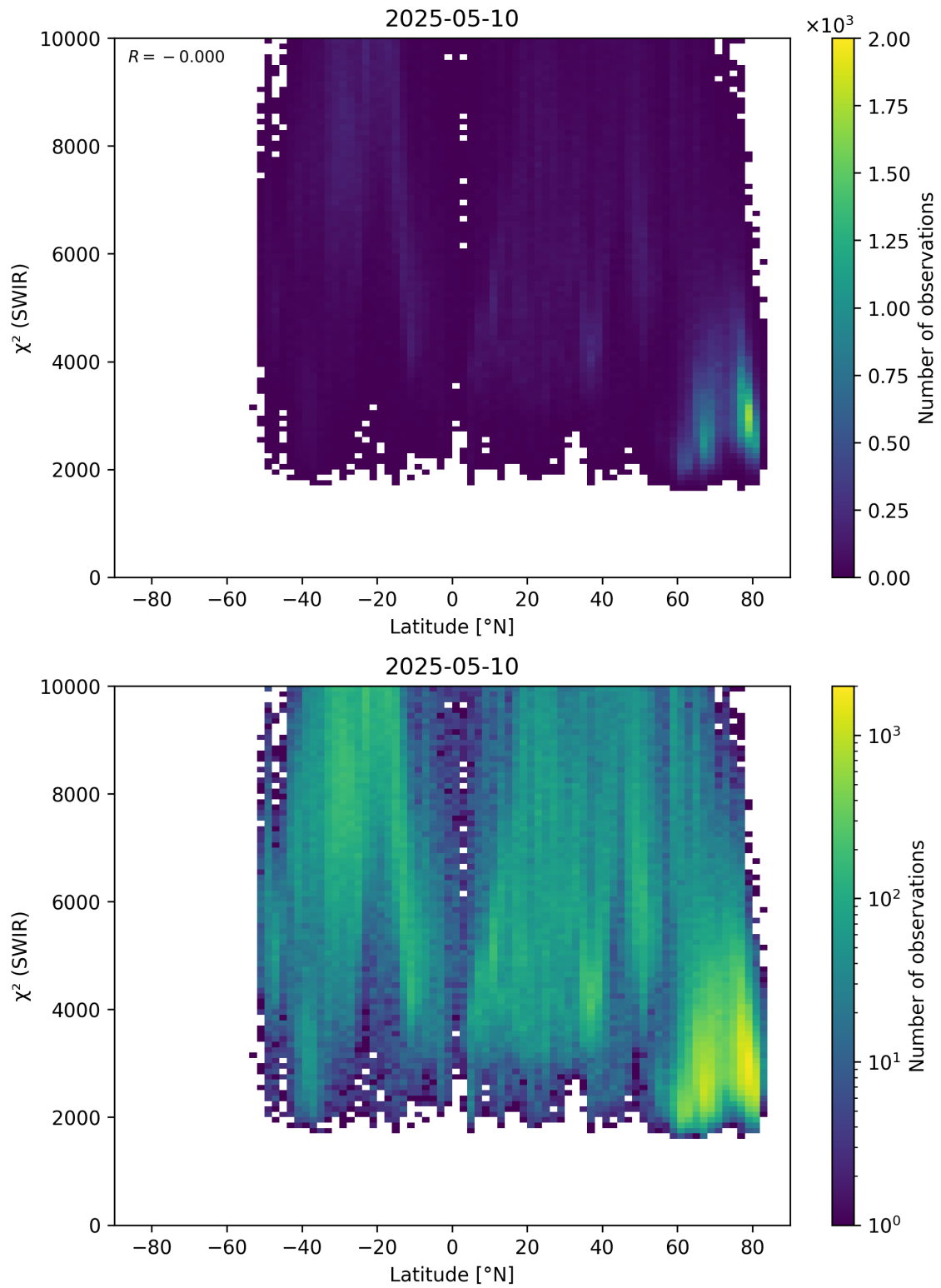
Figure 54: Scatter density plot of “Latitude” against “ \chi^2 (SWIR)” for 2025-05-10 to 2025-05-11.
