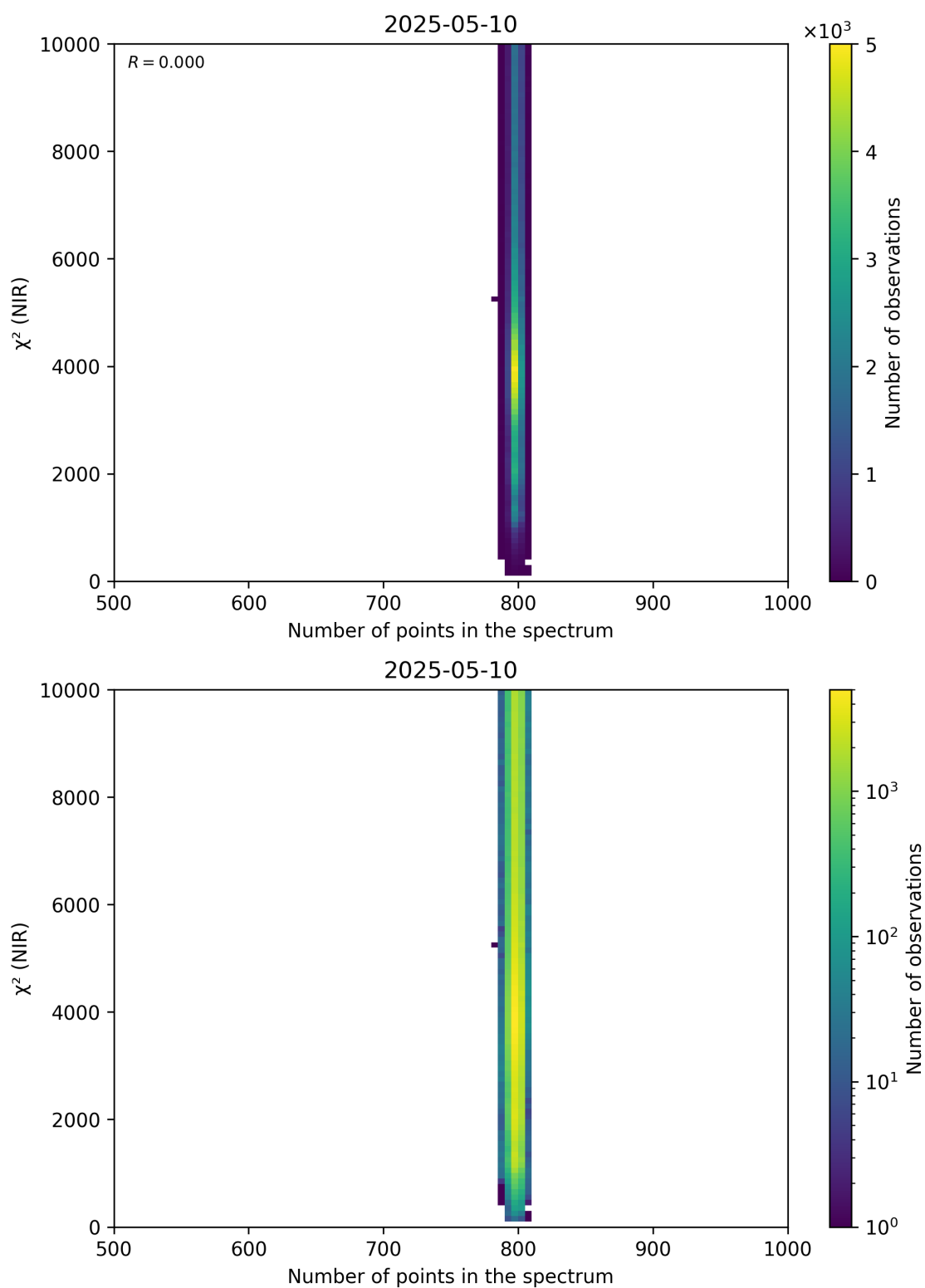
Figure 88: Scatter density plot of “Number of points in the spectrum” against “ \chi^2 (NIR)” for 2025-05-10 to 2025-05-11.
