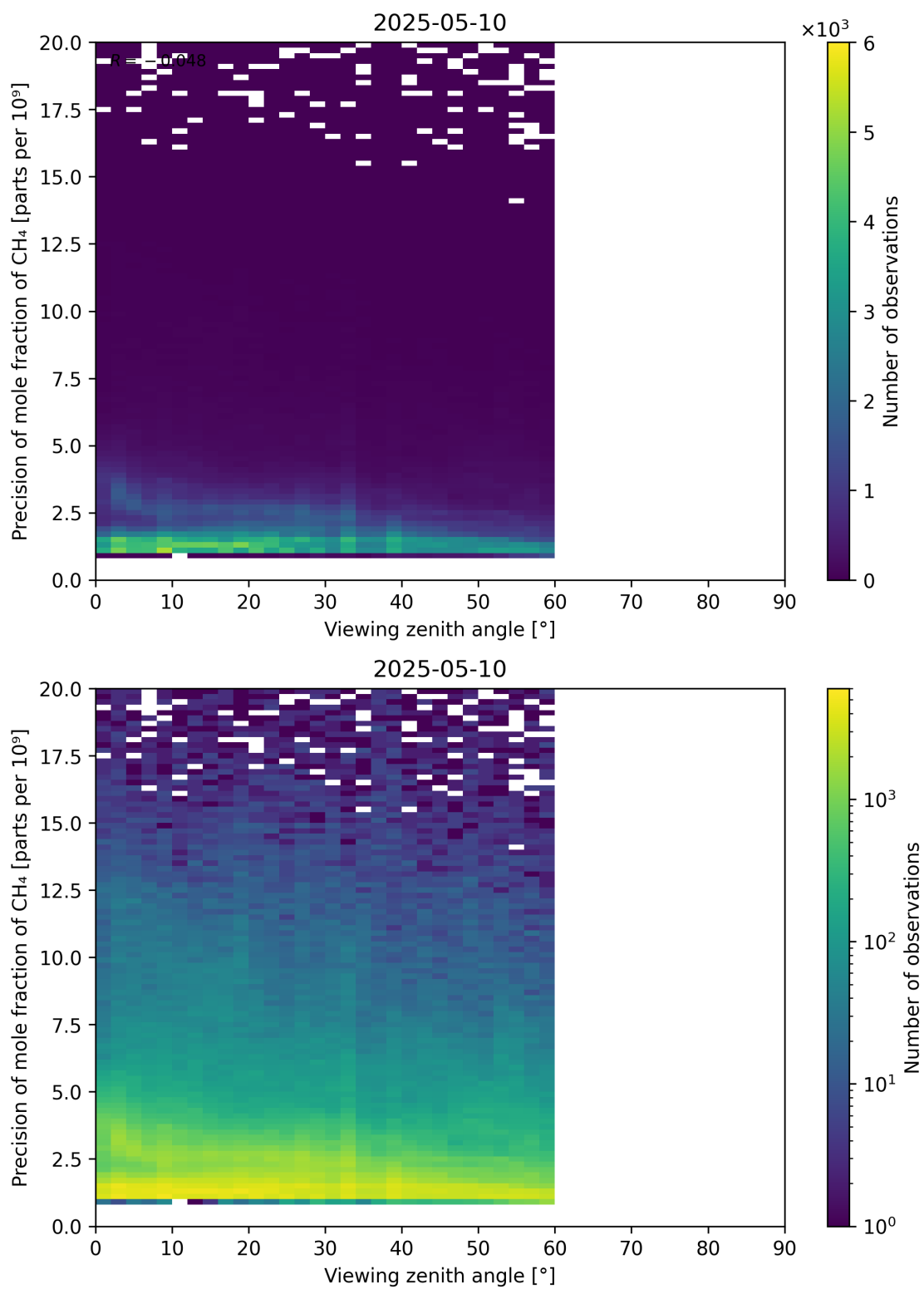
Figure 112: Scatter density plot of “Viewing zenith angle” against “Precision of mole fraction of CH 4 ” for 2025-05-10 to 2025-05-11.
