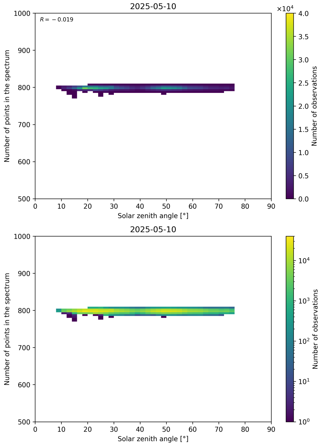
Figure 103: Scatter density plot of “Solar zenith angle” against “Number of points in the spectrum” for 2025-05-10 to 2025-05-11.
