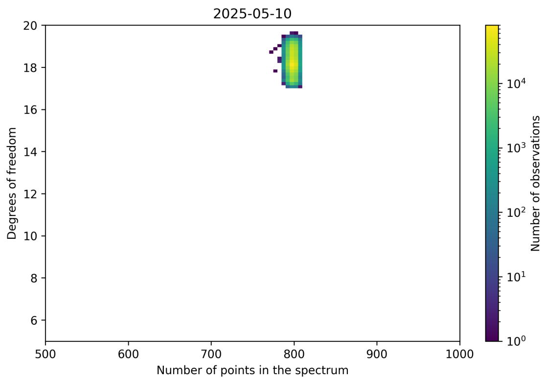
Figure 90: Scatter density plot of “Number of points in the spectrum” against “Degrees of freedom” for 2025-05-10 to 2025-05-11.
