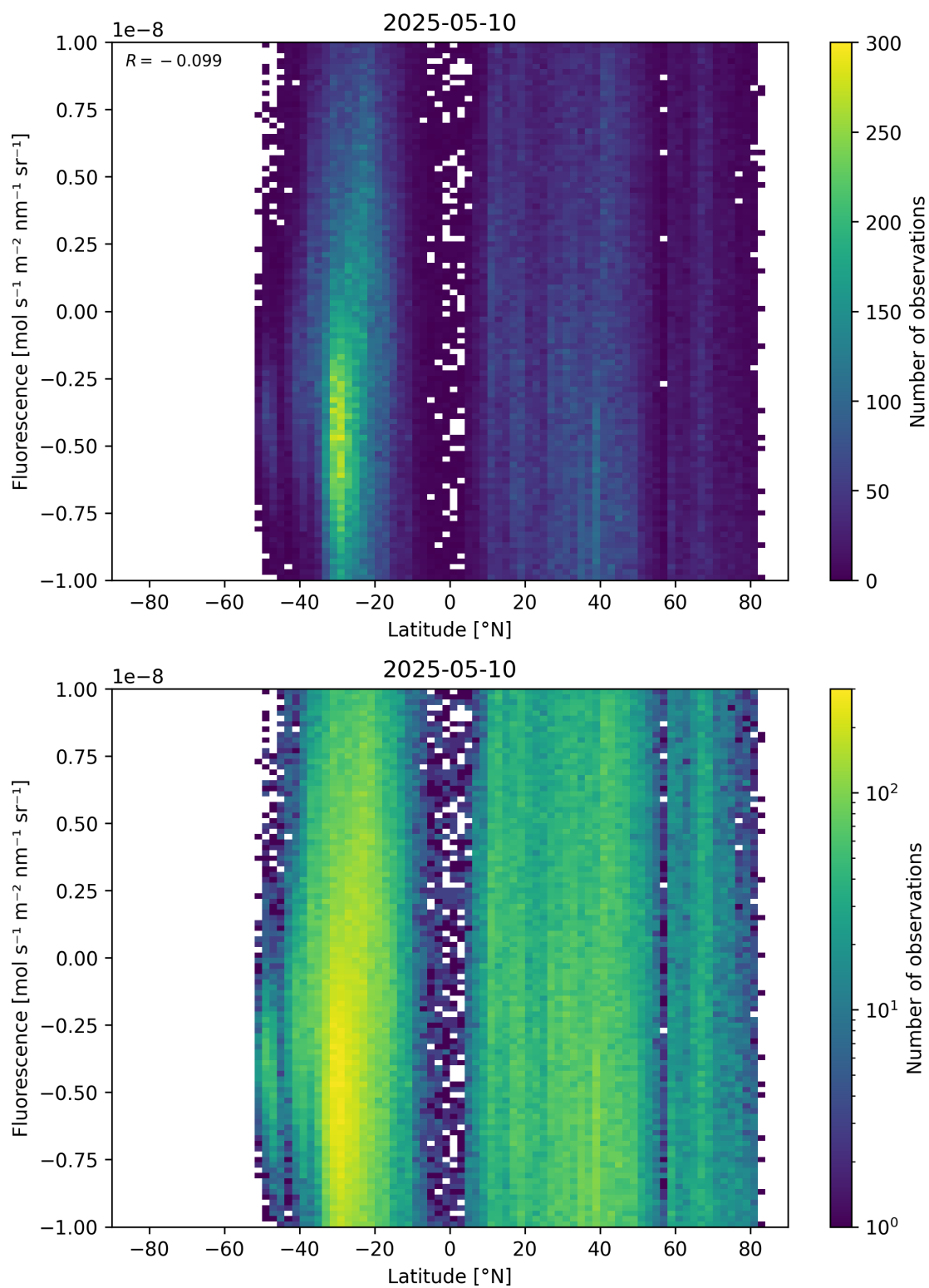
Figure 56: Scatter density plot of “Latitude” against “Fluorescence” for 2025-05-10 to 2025-05-11.
