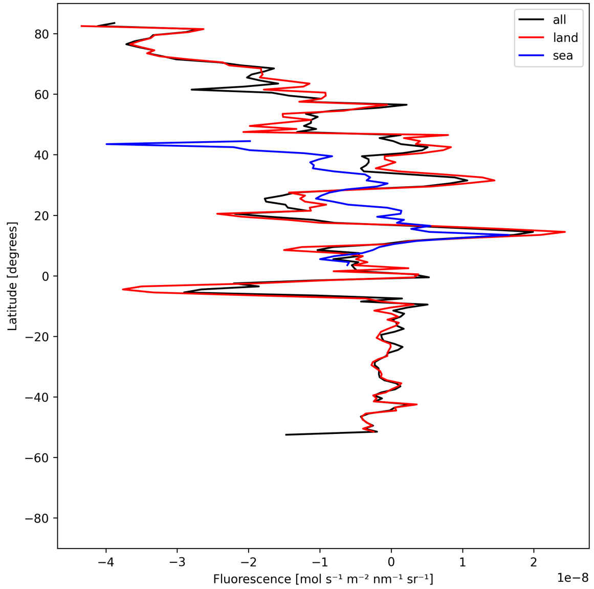
Figure 21: Zonal average of “Fluorescence” for 2025-05-10 to 2025-05-11.
