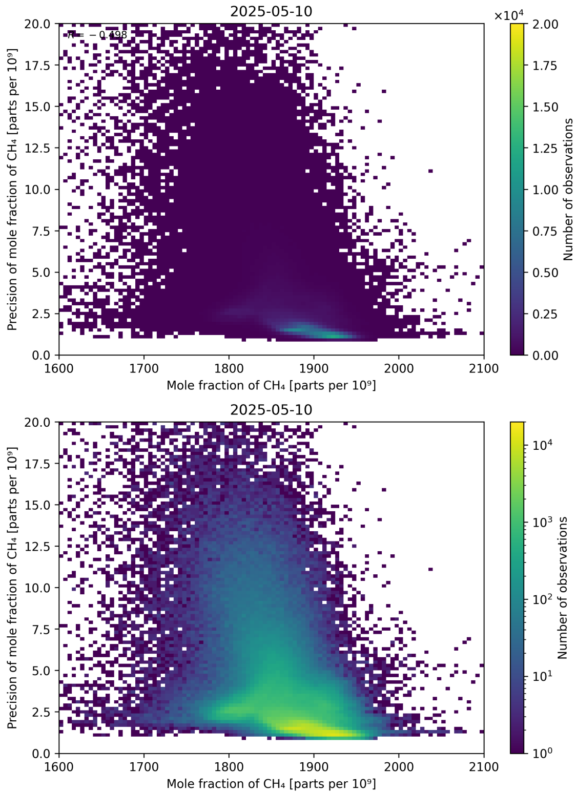
Figure 75: Scatter density plot of “Mole fraction of CH 4 ” against “Precision of mole fraction of CH 4 ” for 2025-05-10 to 2025-05-11.
