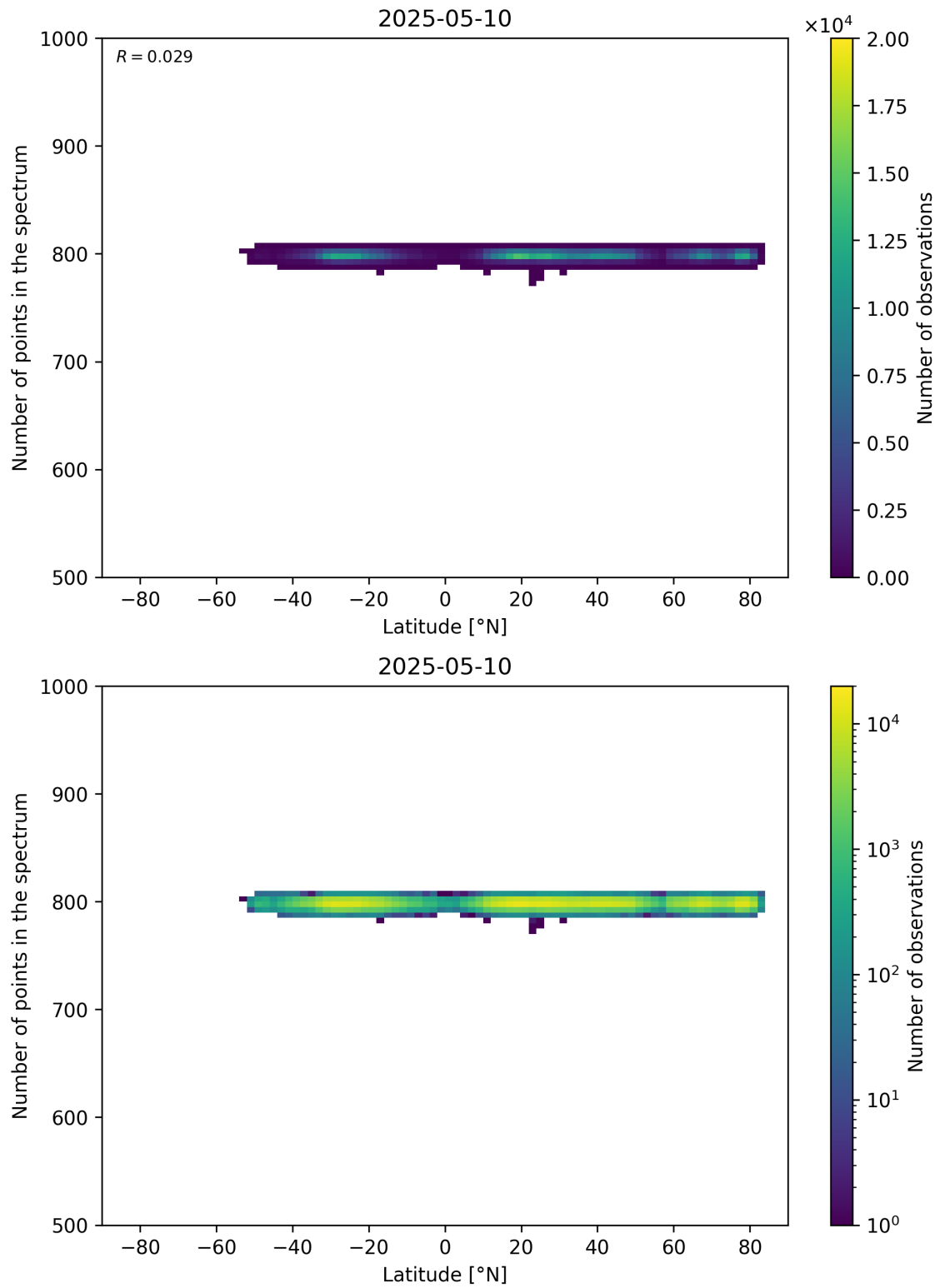
Figure 61: Scatter density plot of “Latitude” against “Number of points in the spectrum” for 2025-05-10 to 2025-05-11.
