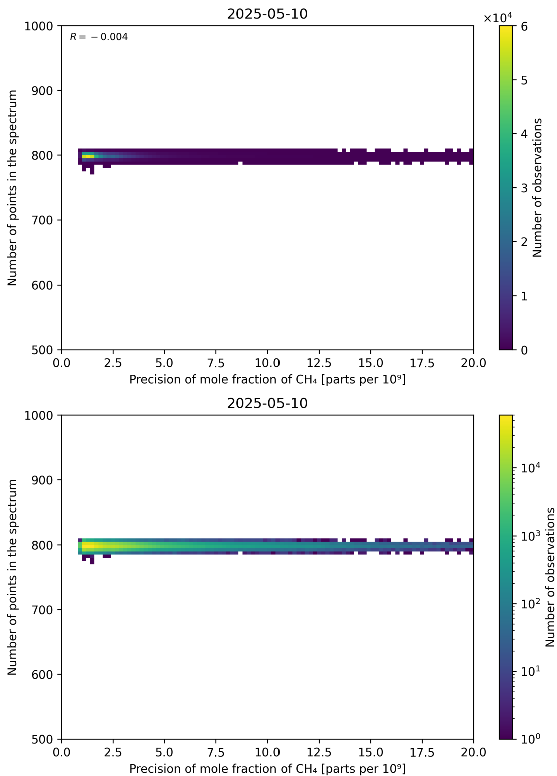
Figure 84: Scatter density plot of “Precision of mole fraction of CH 4 ” against “Number of points in the spectrum” for 2025-05-10 to 2025-05-11.
