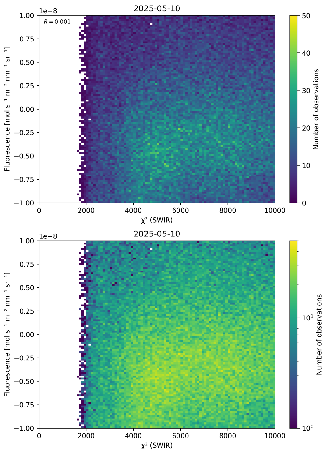
Figure 49: Scatter density plot of “ \chi^2 (SWIR)” against “Fluorescence” for 2025-05-10 to 2025-05-11.
