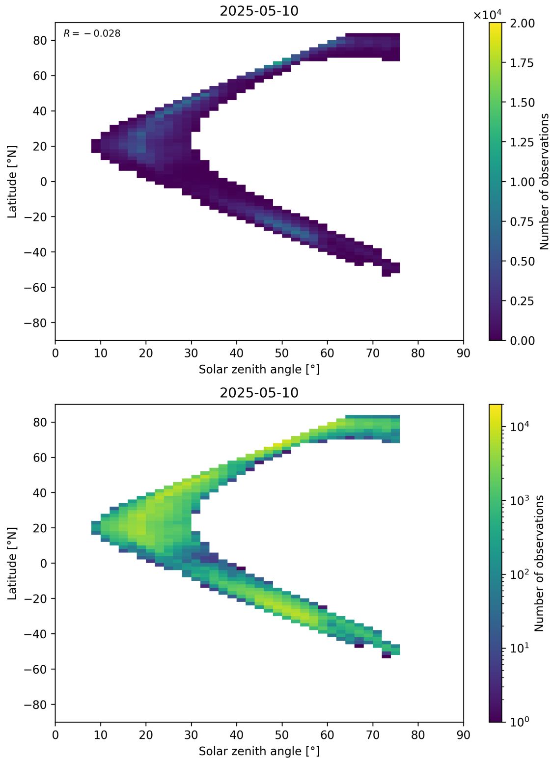
Figure 98: Scatter density plot of “Solar zenith angle” against “Latitude” for 2025-05-10 to 2025-05-11.
