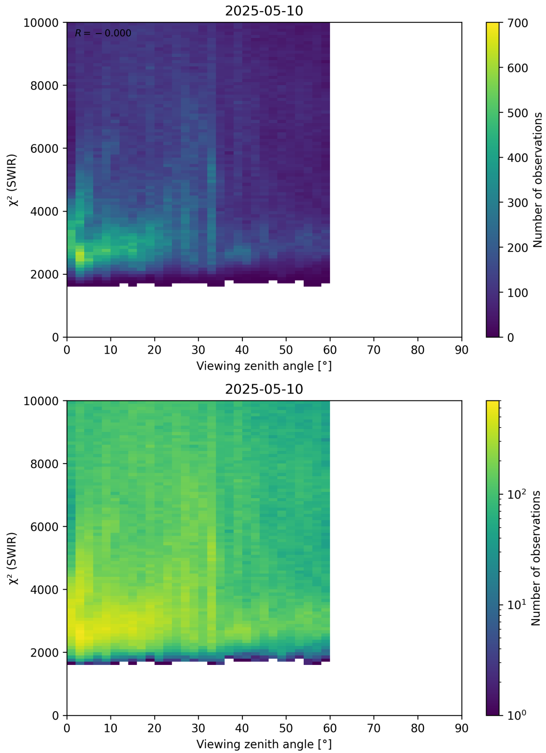
Figure 106: Scatter density plot of “Viewing zenith angle” against “ \chi^2 (SWIR)” for 2025-05-10 to 2025-05-11.
