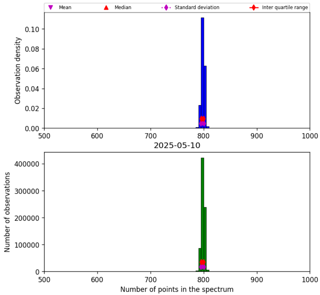
Figure 26: Histogram of “Number of points in the spectrum” for 2025-05-10 to 2025-05-11
