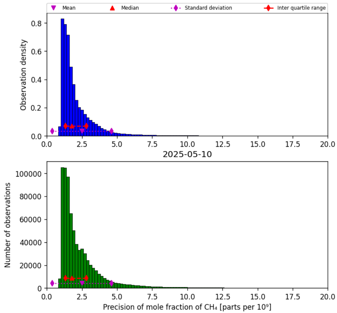
Figure 24: Histogram of “Precision of mole fraction of CH 4 ” for 2025-05-10 to 2025-05-11
