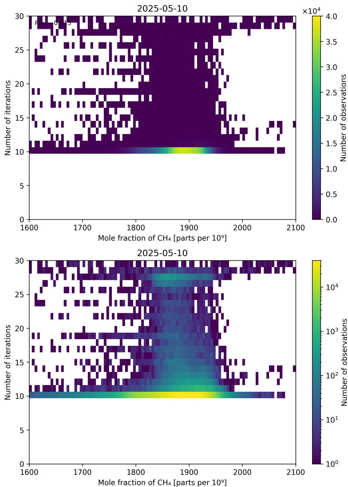
Figure 76: Scatter density plot of “Mole fraction of CH 4 ” against “Number of iterations” for 2025-05-10 to 2025-05-11.
