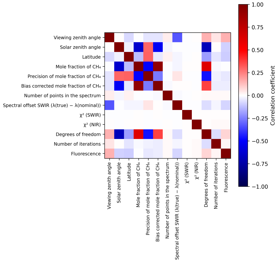
Figure 2: Map of correlation matrix for 2025-05-10 to 2025-05-11.
