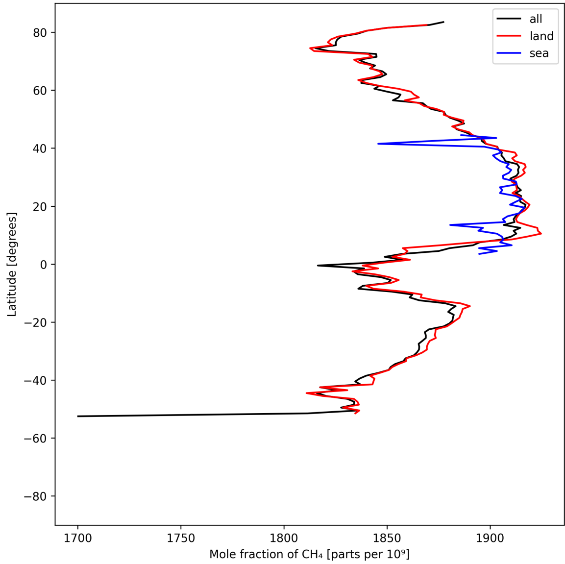
Figure 12: Zonal average of “Mole fraction of CH 4 ” for 2025-05-10 to 2025-05-11.
