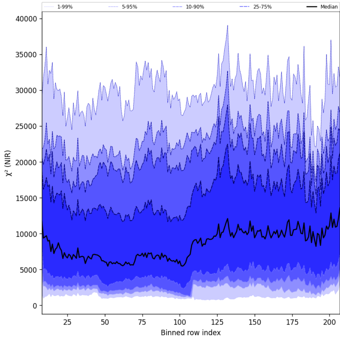
Figure 40: Along track statistics of “ \chi^2 (NIR)” for 2025-05-10 to 2025-05-11
