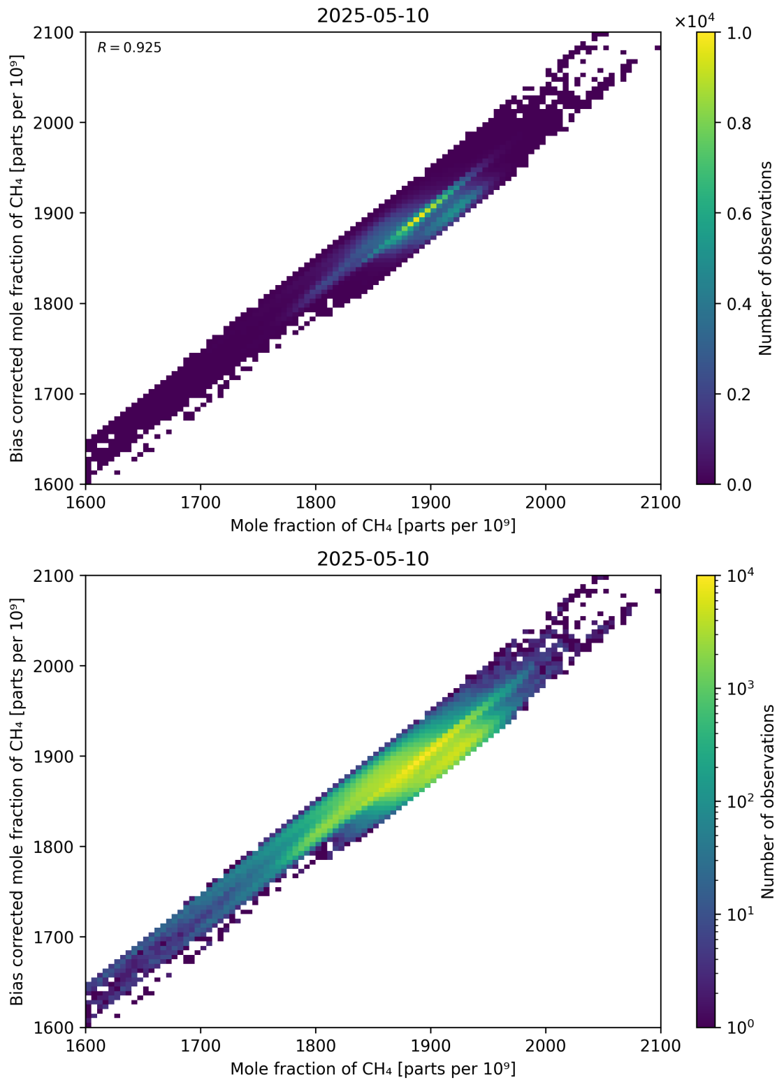
Figure 74: Scatter density plot of “Mole fraction of CH 4 ” against “Bias corrected mole fraction of CH 4 ” for 2025-05-10 to 2025-05-11.
