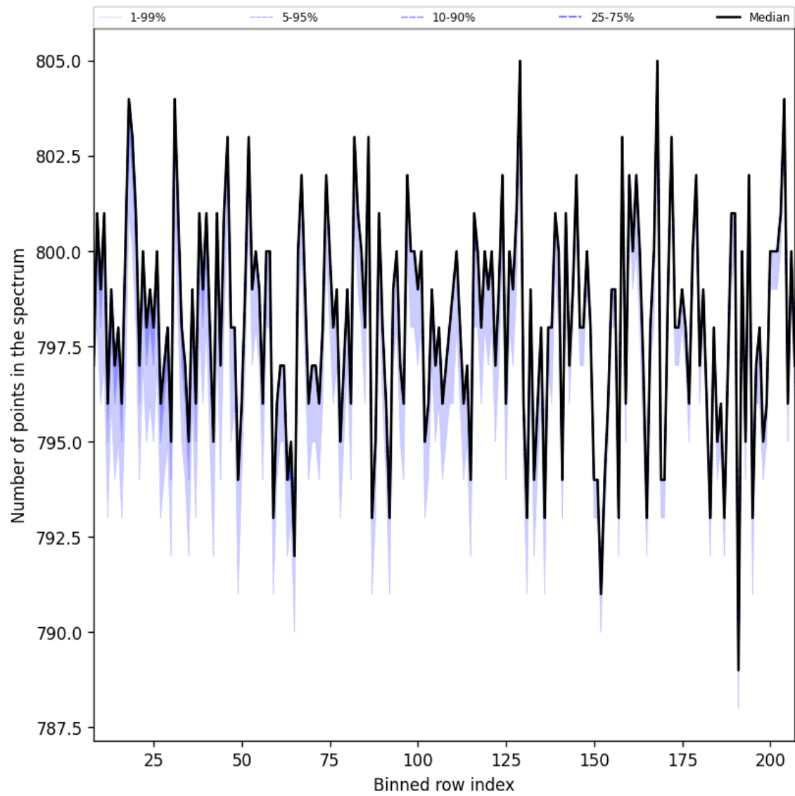
Figure 37: Along track statistics of “Number of points in the spectrum” for 2025-05-10 to 2025-05-11
