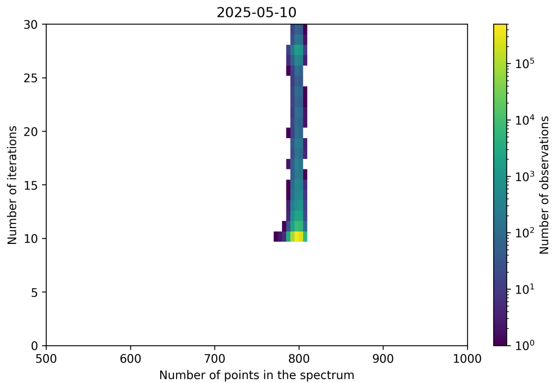
Figure 92: Scatter density plot of “Number of points in the spectrum” against “Number of iterations” for 2025-05-10 to 2025-05-11.
