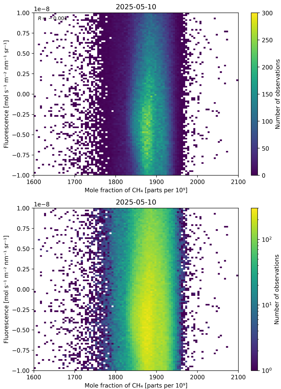
Figure 73: Scatter density plot of “Mole fraction of \text{CH}_4 ” against “Fluorescence” for 2025-05-10 to 2025-05-11.
