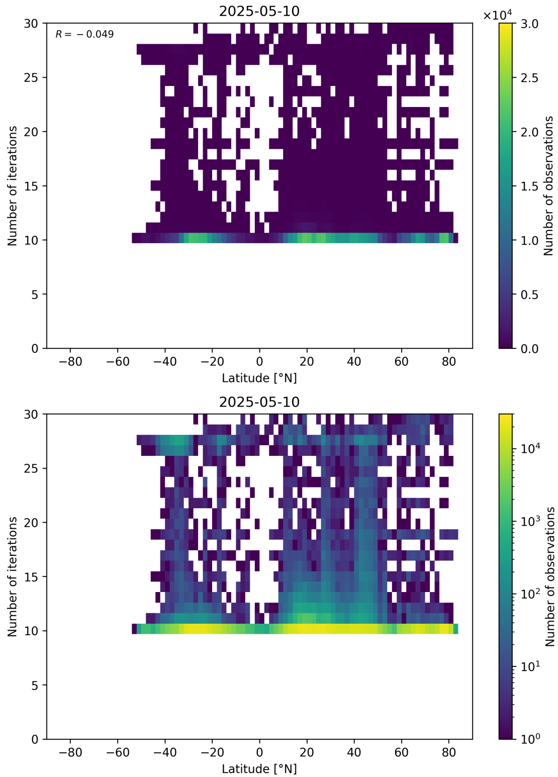
Figure 60: Scatter density plot of “Latitude” against “Number of iterations” for 2025-05-10 to 2025-05-11.
