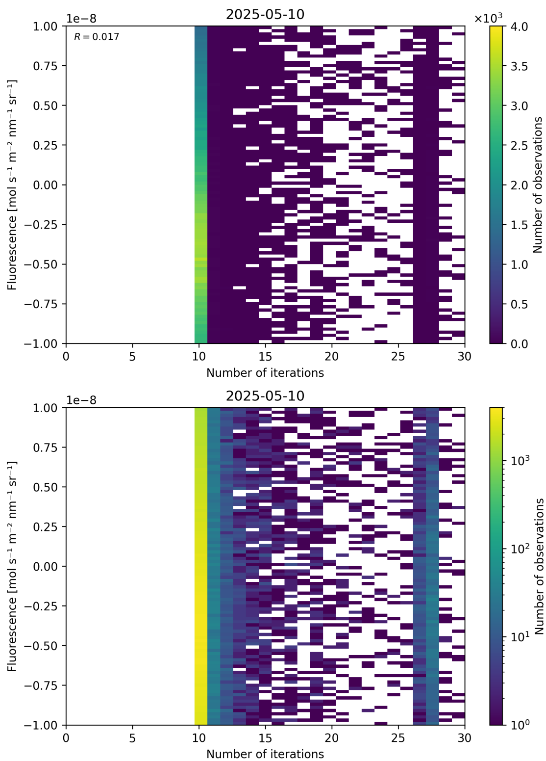
Figure 87: Scatter density plot of “Number of iterations” against “Fluorescence” for 2025-05-10 to 2025-05-11.
