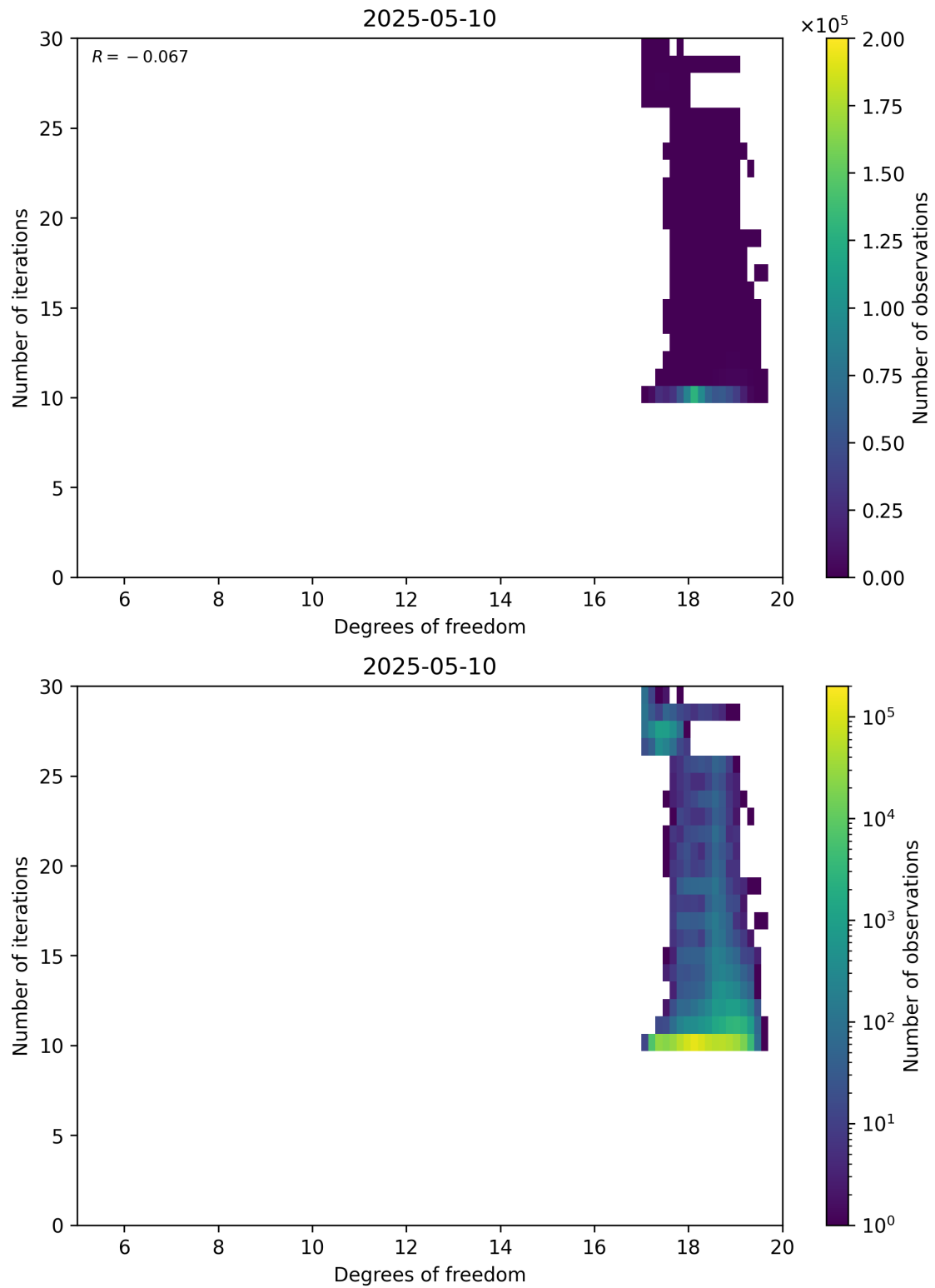
Figure 52: Scatter density plot of “Degrees of freedom” against “Number of iterations” for 2025-05-10 to 2025-05-11.
