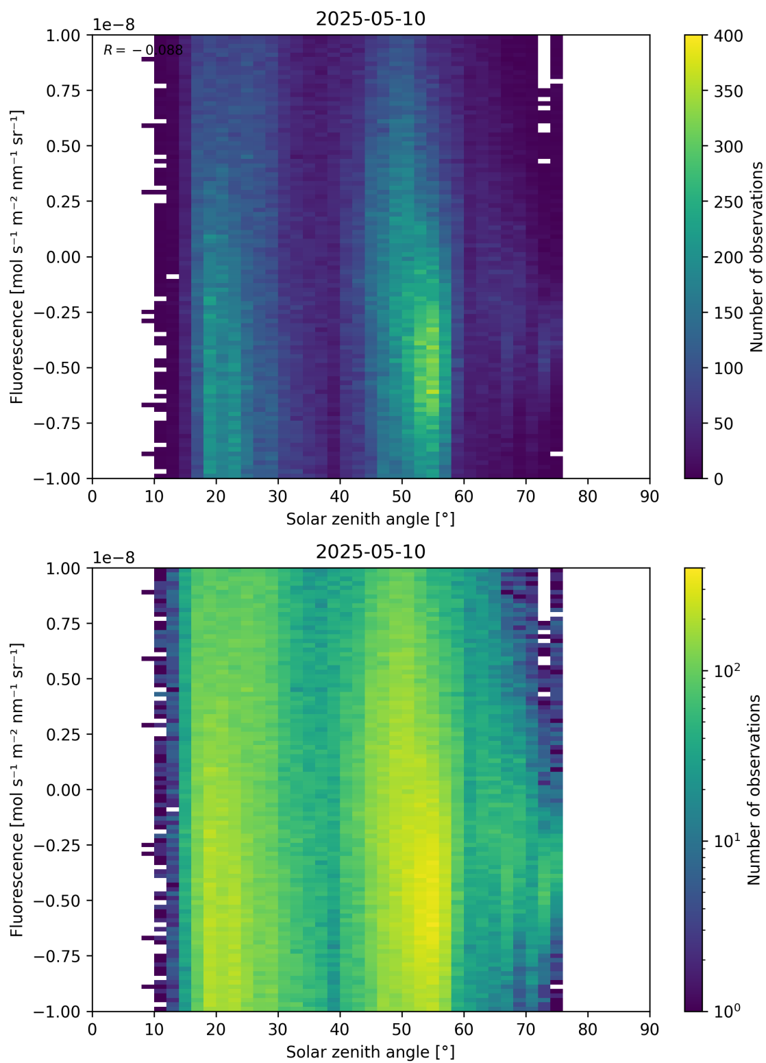
Figure 97: Scatter density plot of “Solar zenith angle” against “Fluorescence” for 2025-05-10 to 2025-05-11.
