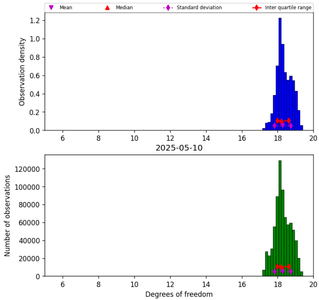
Figure 30: Histogram of “Degrees of freedom” for 2025-05-10 to 2025-05-11
