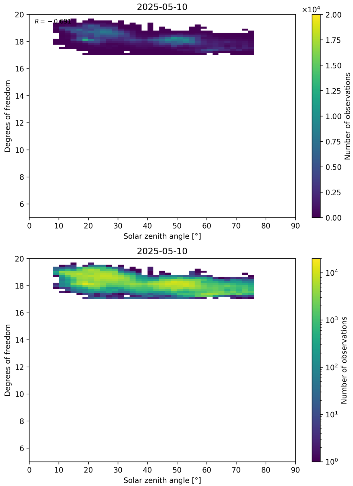
Figure 96: Scatter density plot of “Solar zenith angle” against “Degrees of freedom” for 2025-05-10 to 2025-05-11.
