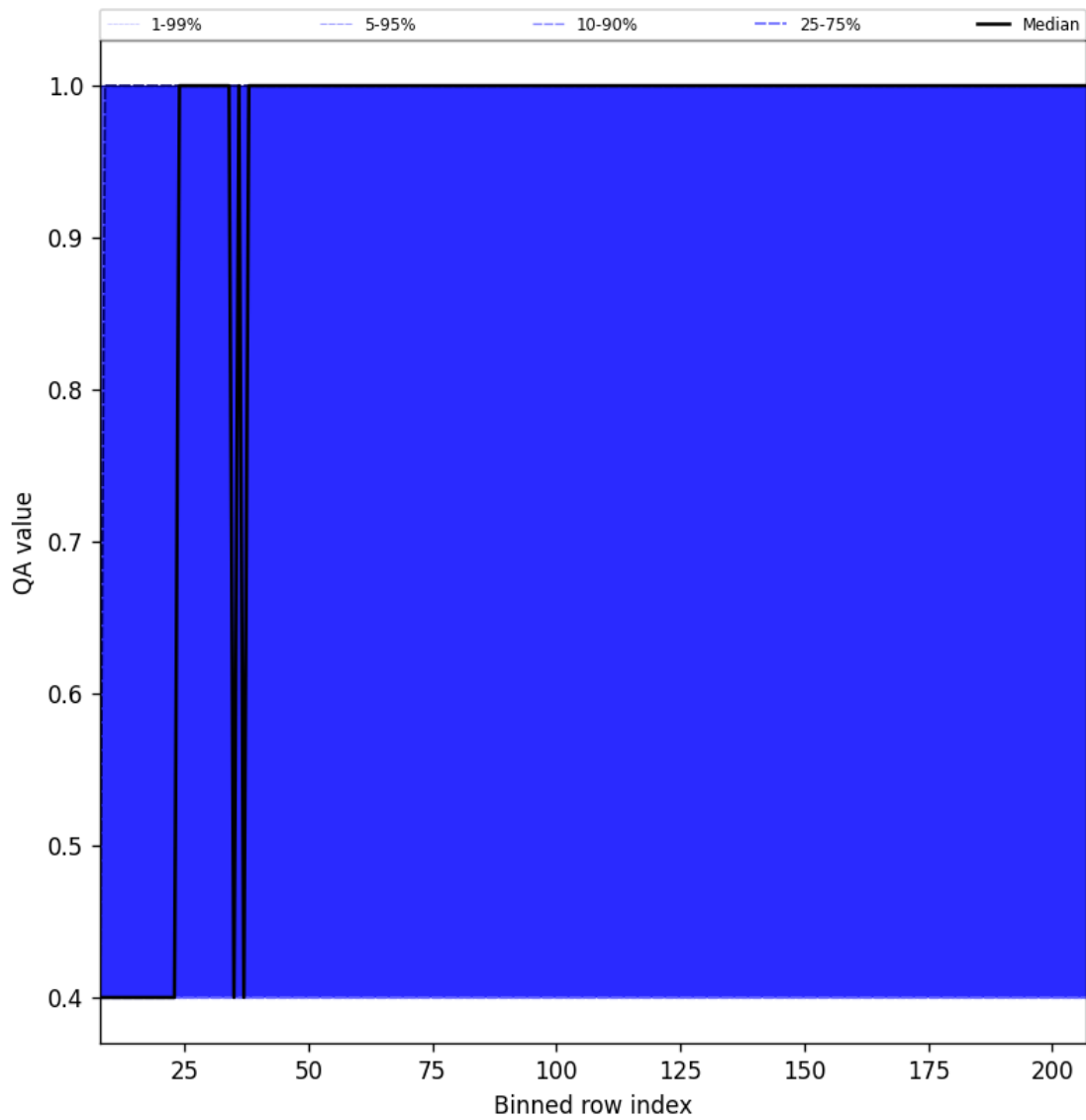
Figure 33: Along track statistics of “QA value” for 2025-05-10 to 2025-05-11
