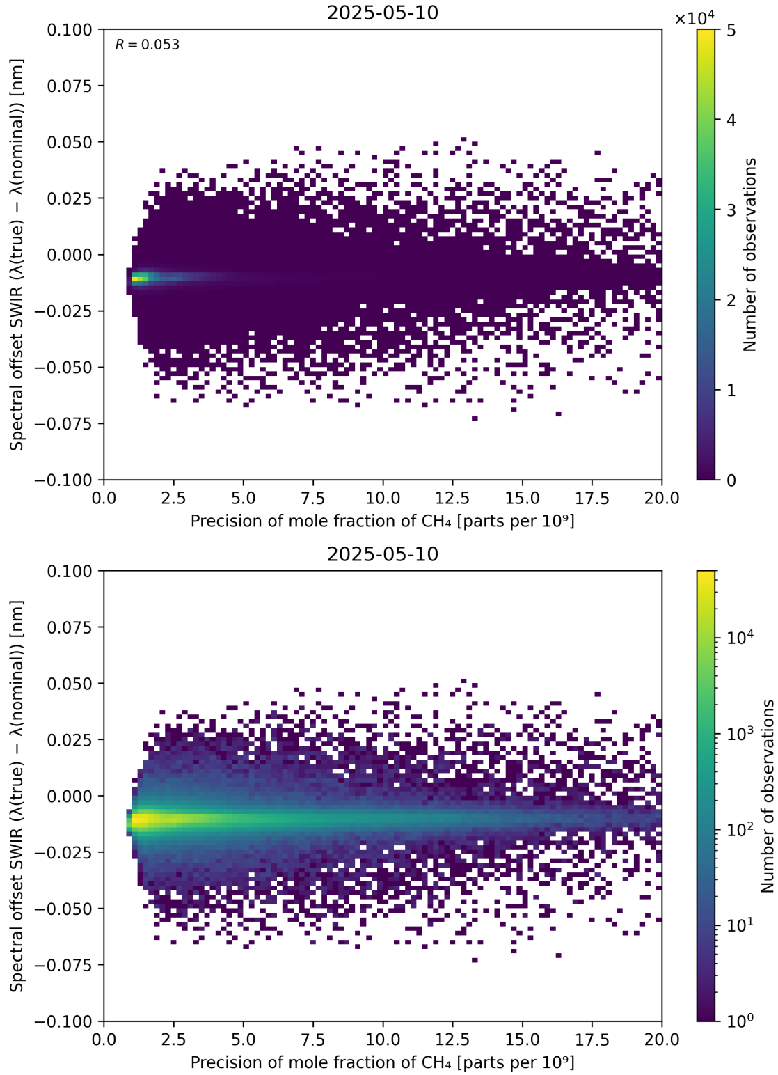
Figure 85: Scatter density plot of “Precision of mole fraction of \text{CH}_4 ” against “Spectral offset SWIR ( \lambda_{\text{true}} - \lambda_{\text{nominal}} )” for 2025-05-10 to 2025-05-11.
