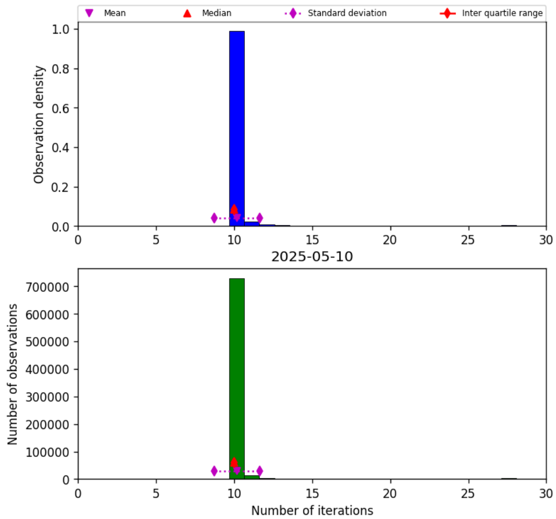
Figure 31: Histogram of “Number of iterations” for 2025-05-10 to 2025-05-11
