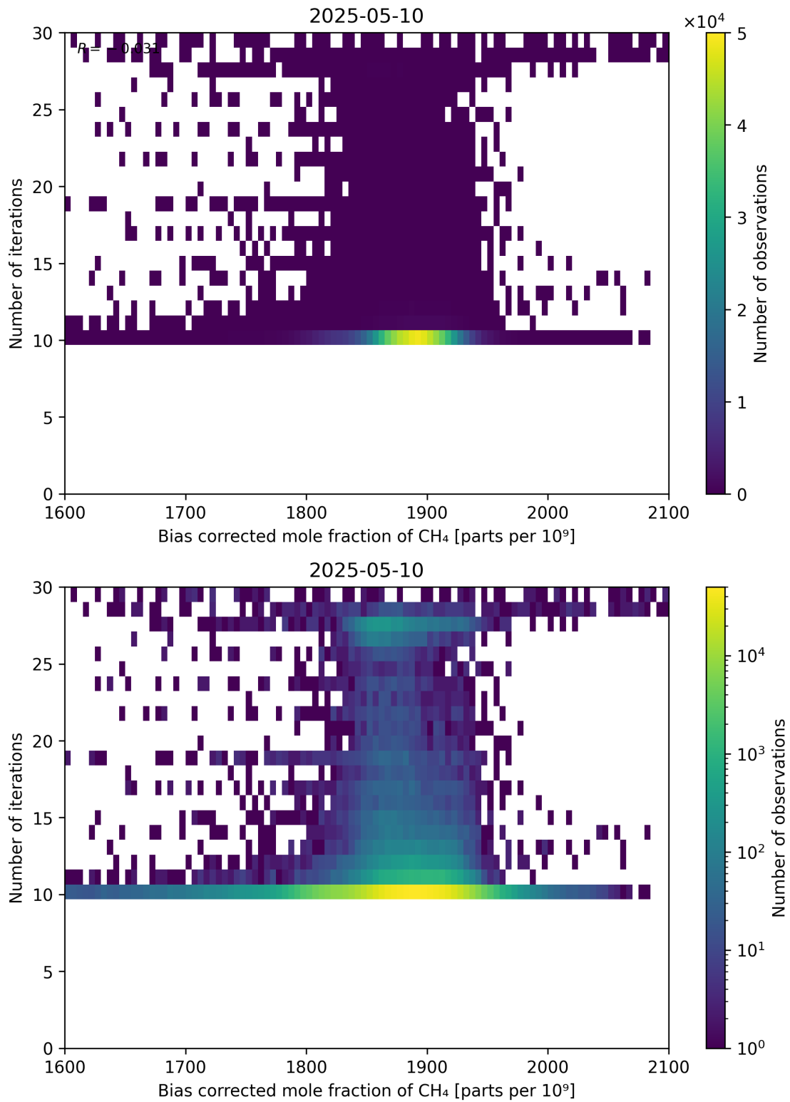
Figure 67: Scatter density plot of “Bias corrected mole fraction of \text{CH}_4 ” against “Number of iterations” for 2025-05-10 to 2025-05-11.
