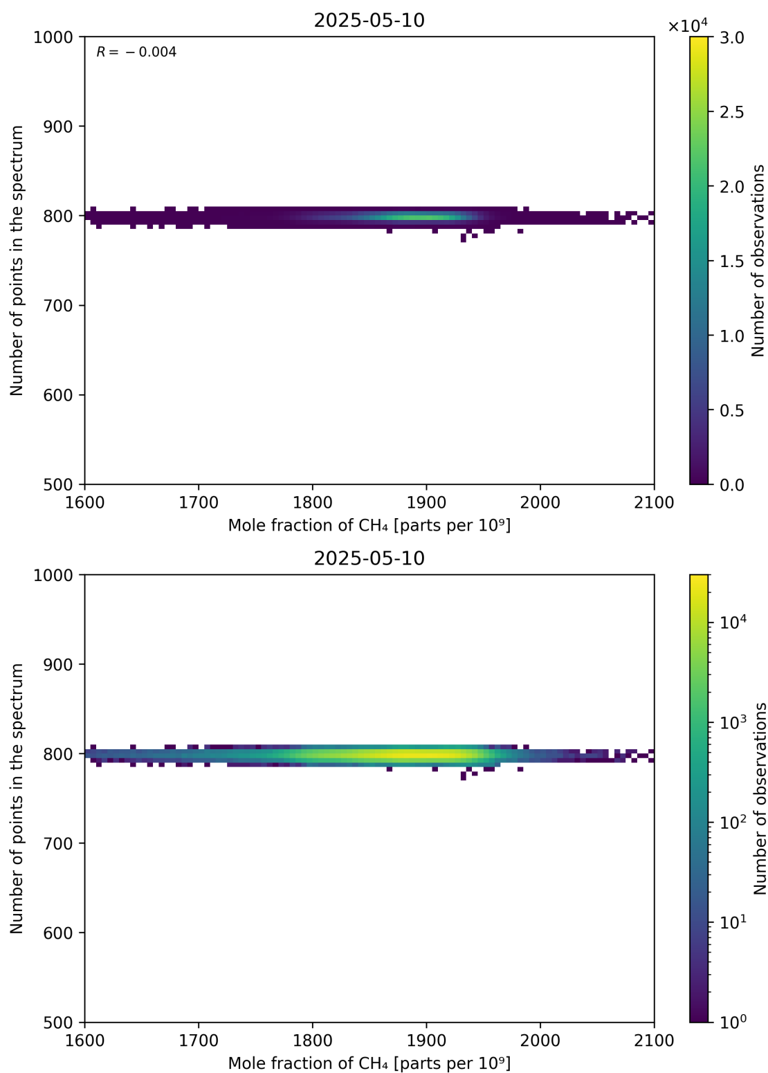
Figure 77: Scatter density plot of “Mole fraction of CH 4 ” against “Number of points in the spectrum” for 2025-05-10 to 2025-05-11.
