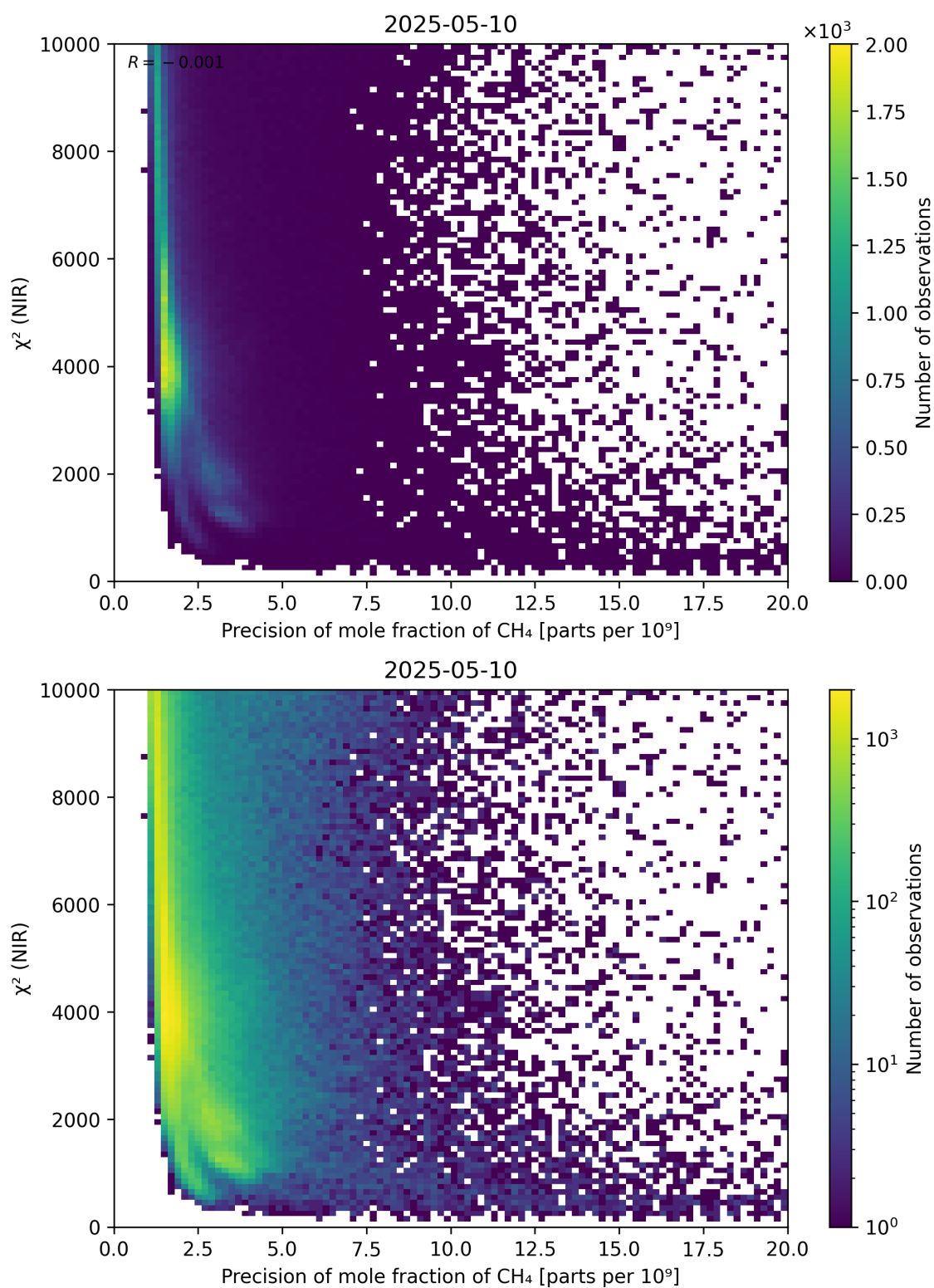
Figure 78: Scatter density plot of “Precision of mole fraction of CH 4 ” against “ \chi^2 (NIR)” for 2025-05-10 to 2025-05-11.
