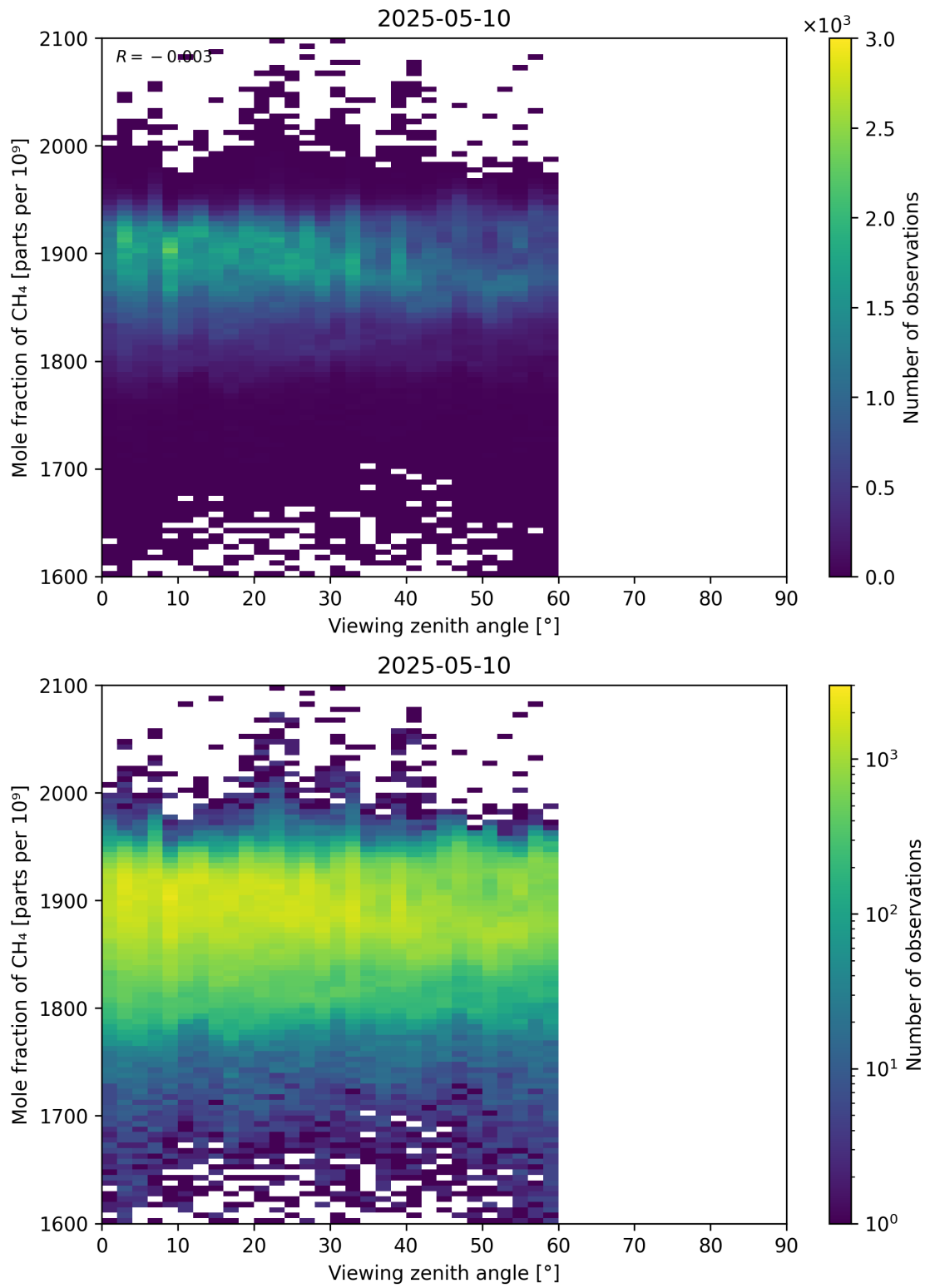
Figure 110: Scatter density plot of “Viewing zenith angle” against “Mole fraction of CH 4 ” for 2025-05-10 to 2025-05-11.
