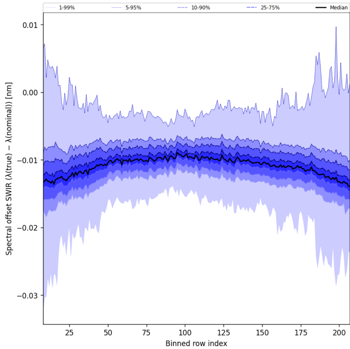
Figure 38: Along track statistics of “Spectral offset SWIR ( \lambda_{\text{true}} - \lambda_{\text{nominal}} )” for 2025-05-10 to 2025-05-11
