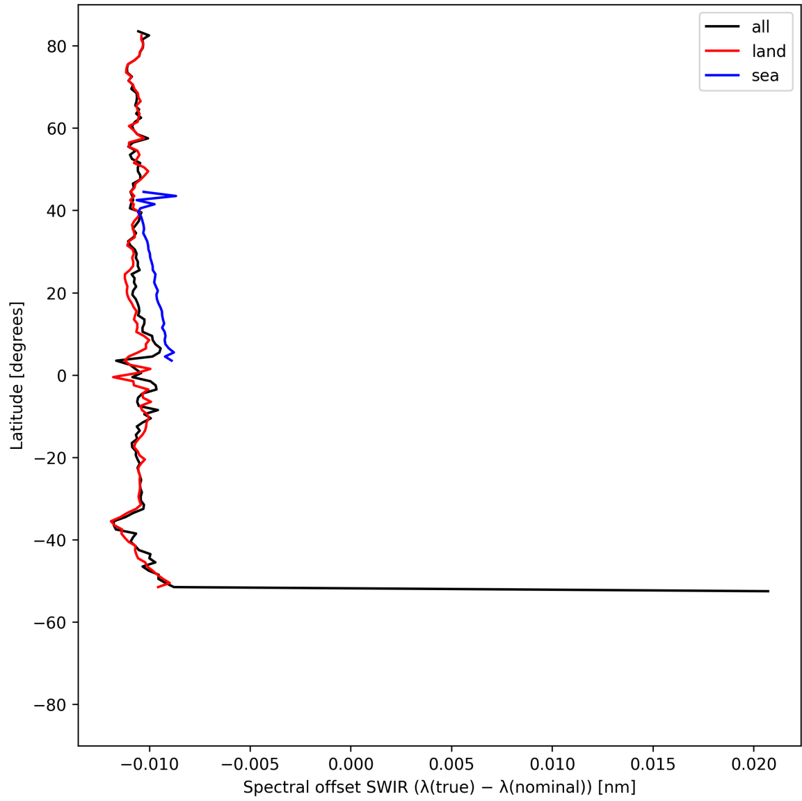
Figure 16: Zonal average of “Spectral offset SWIR ( \lambda_{\text{true}} - \lambda_{\text{nominal}} )” for 2025-05-10 to 2025-05-11.
