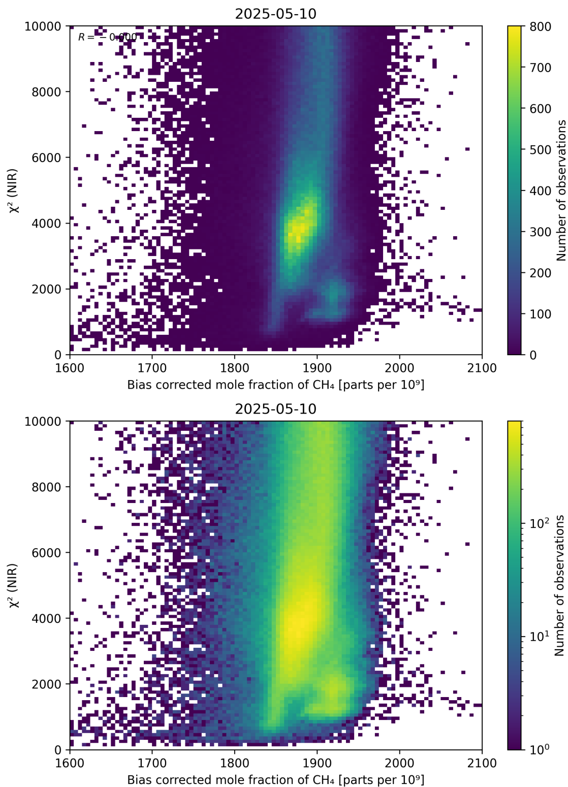
Figure 63: Scatter density plot of “Bias corrected mole fraction of CH 4 ” against “ \chi^2 (NIR)” for 2025-05-10 to 2025-05-11.
