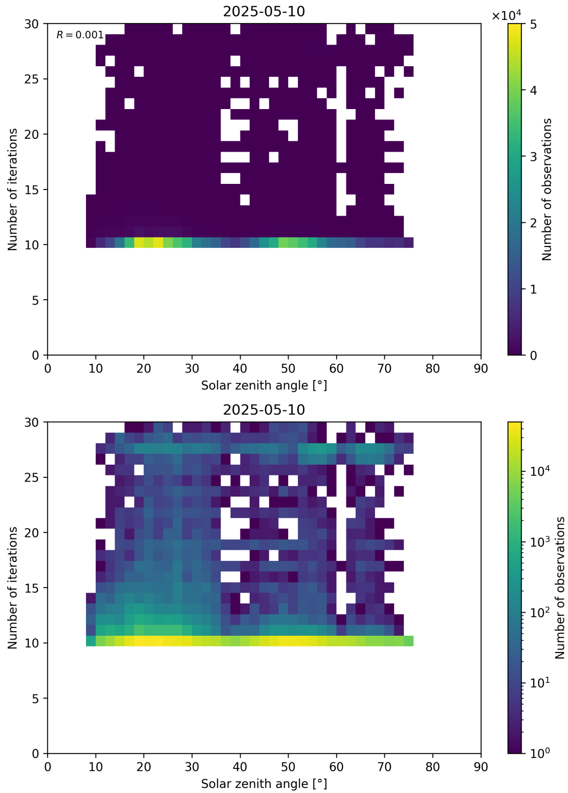
Figure 102: Scatter density plot of “Solar zenith angle” against “Number of iterations” for 2025-05-10 to 2025-05-11.
