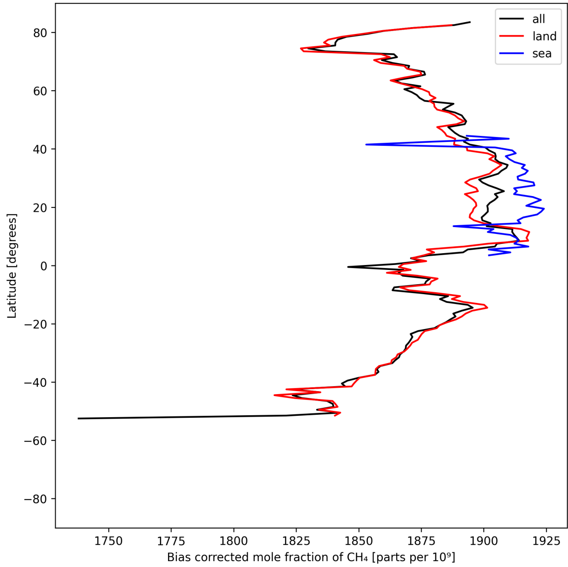
Figure 14: Zonal average of “Bias corrected mole fraction of CH 4 ” for 2025-05-10 to 2025-05-11.
