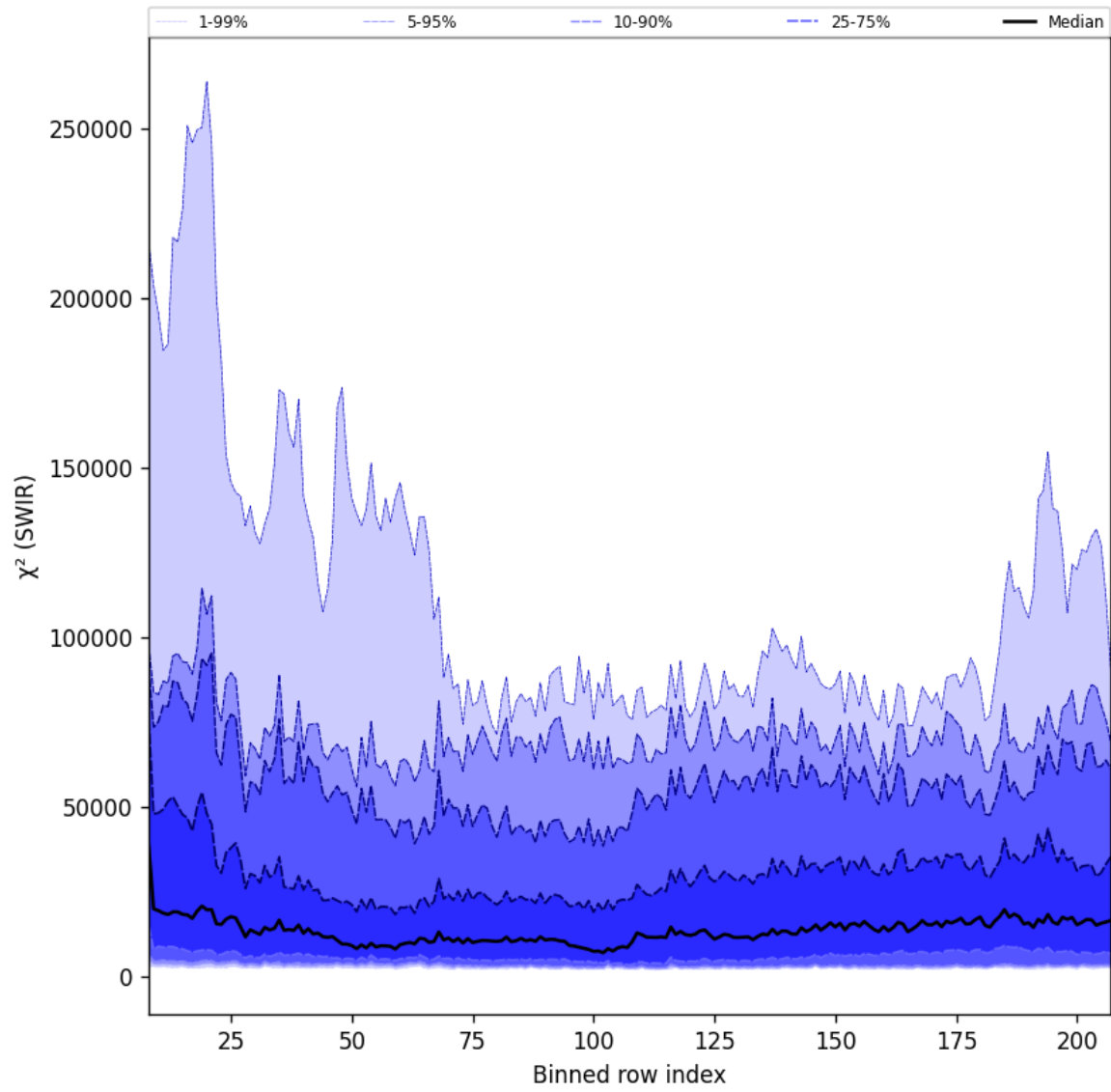
Figure 39: Along track statistics of “ \chi^2 (SWIR)” for 2025-05-10 to 2025-05-11
