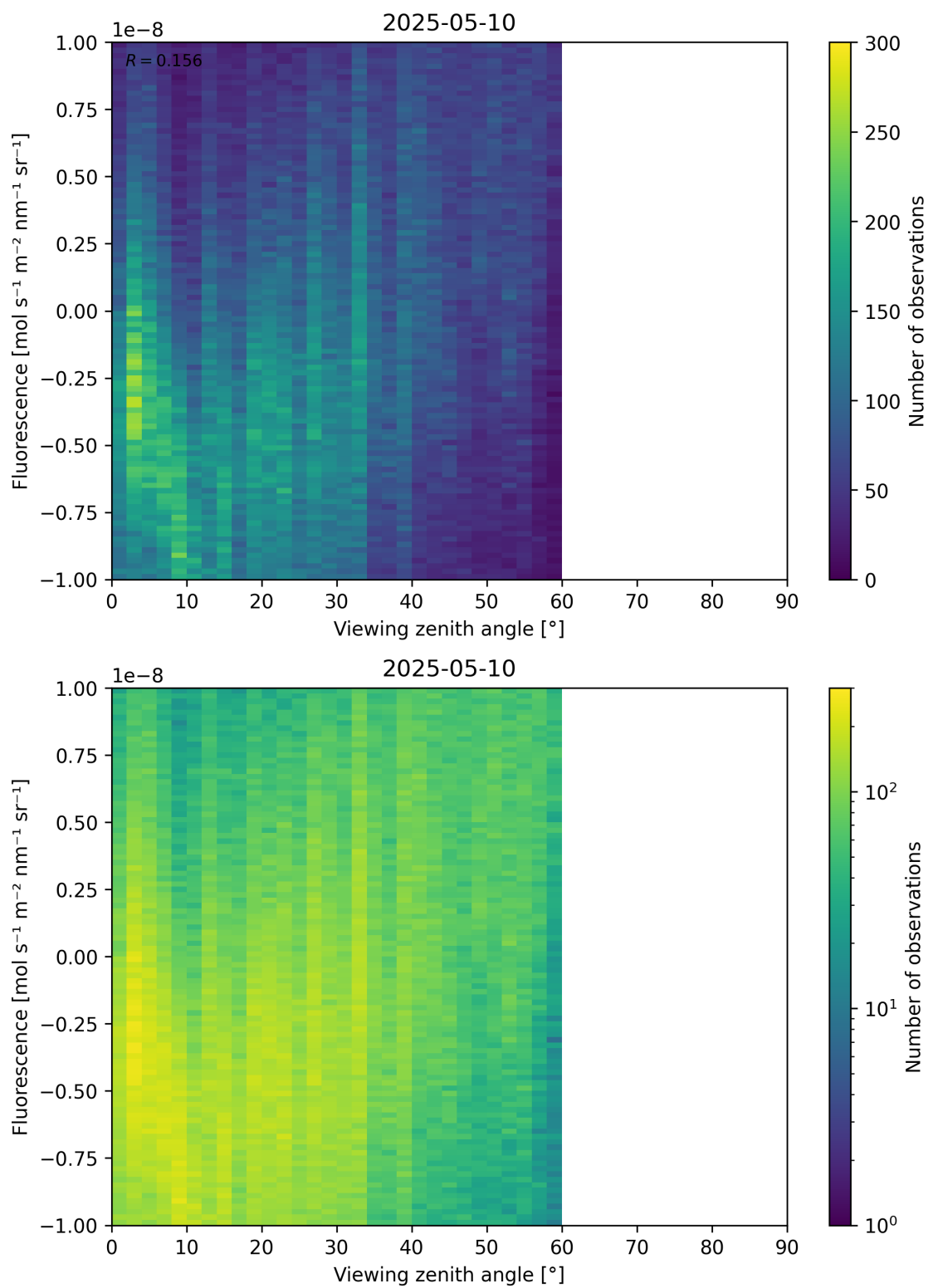
Figure 108: Scatter density plot of “Viewing zenith angle” against “Fluorescence” for 2025-05-10 to 2025-05-11.
