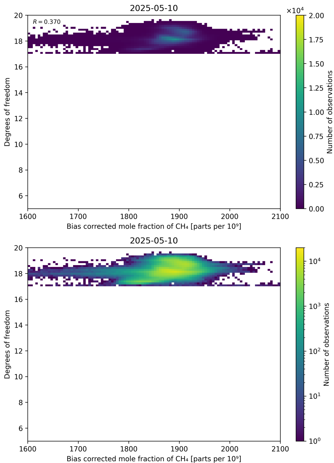
Figure 65: Scatter density plot of “Bias corrected mole fraction of CH 4 ” against “Degrees of freedom” for 2025-05-10 to 2025-05-11.
