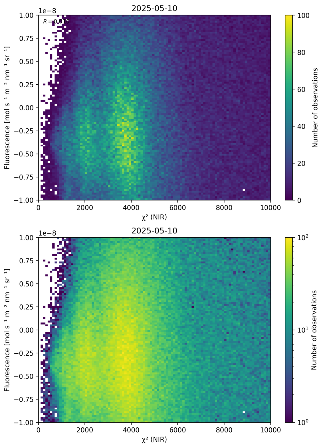
Figure 45: Scatter density plot of “ \chi^2 (NIR)” against “Fluorescence” for 2025-05-10 to 2025-05-11.
