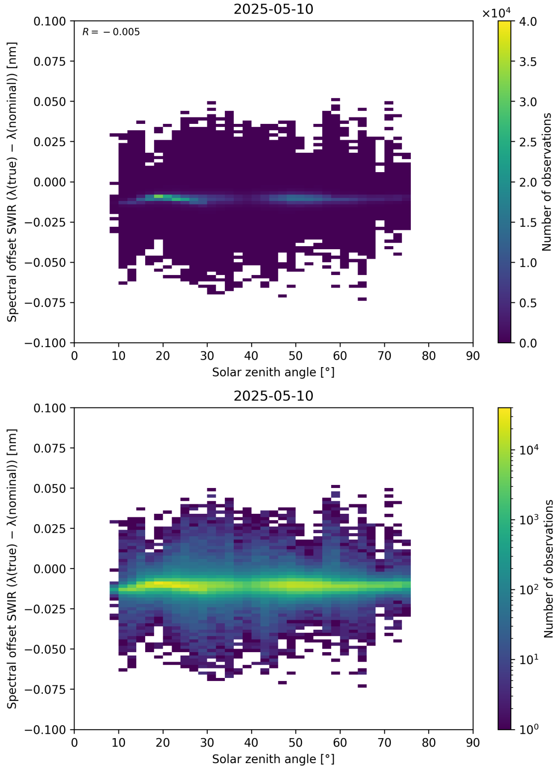
Figure 104: Scatter density plot of “Solar zenith angle” against “Spectral offset SWIR ( \lambda_{\text{true}} - \lambda_{\text{nominal}} )” for 2025-05-10 to 2025-05-11.
