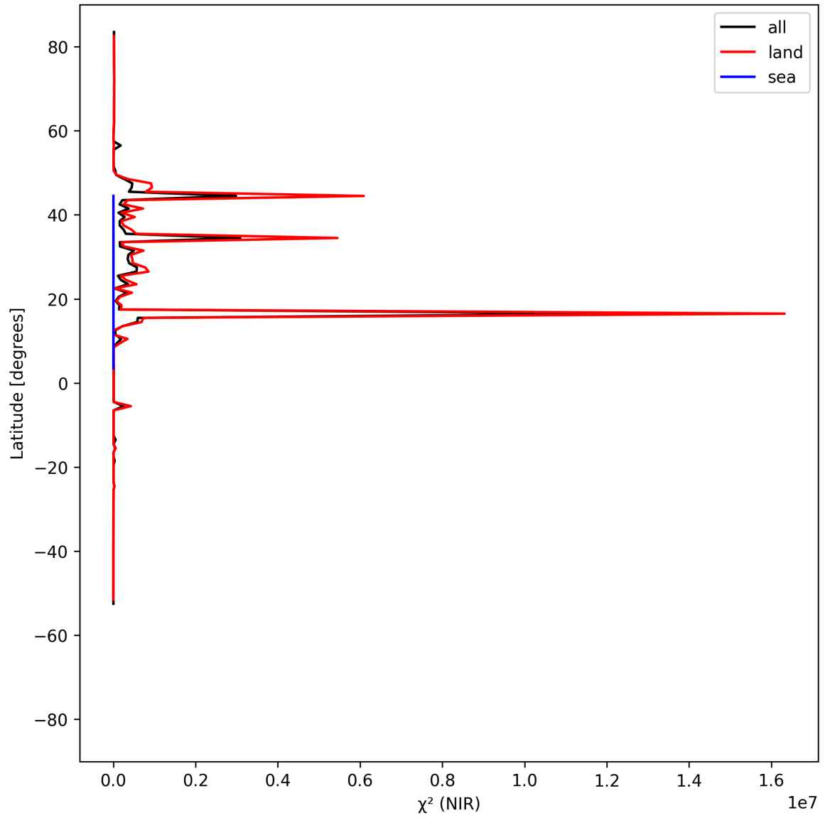
Figure 18: Zonal average of “ \chi^2 (NIR)” for 2025-05-10 to 2025-05-11.
