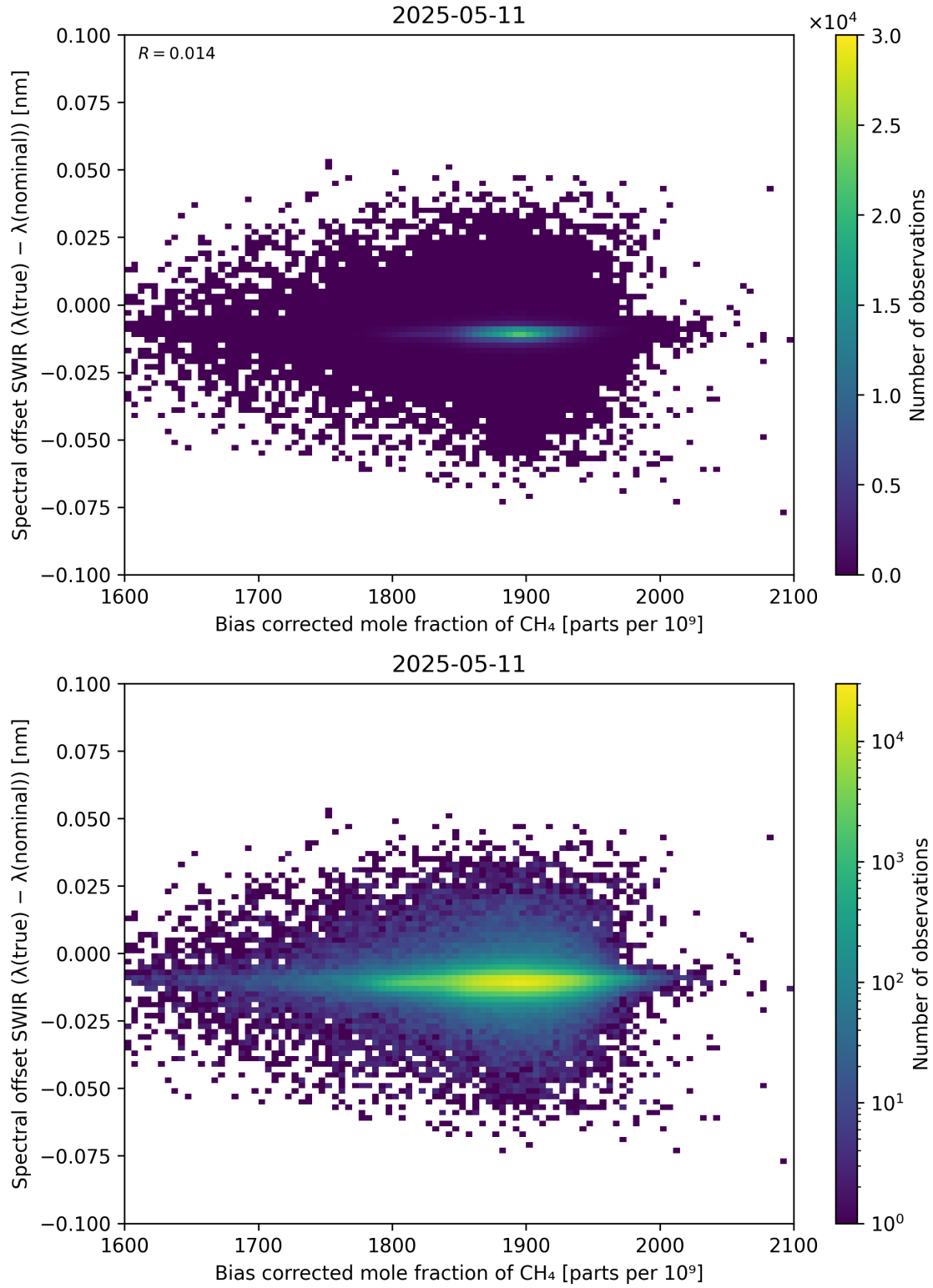
Figure 69: Scatter density plot of “Bias corrected mole fraction of \text{CH}_4 ” against “Spectral offset SWIR ( \lambda_{\text{true}} - \lambda_{\text{nominal}} )” for 2025-05-10 to 2025-05-12.
