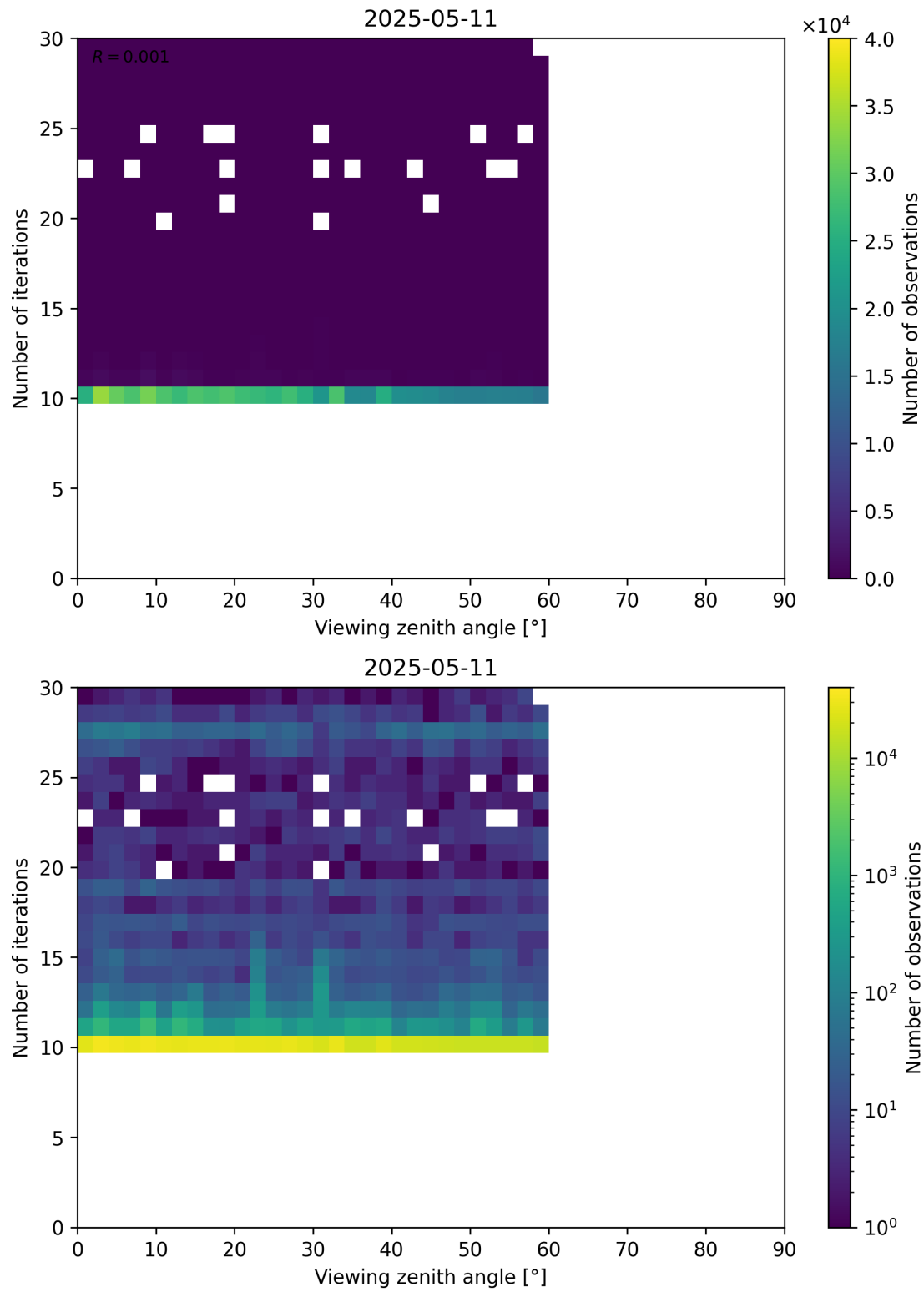
Figure 113: Scatter density plot of “Viewing zenith angle” against “Number of iterations” for 2025-05-10 to 2025-05-12.
