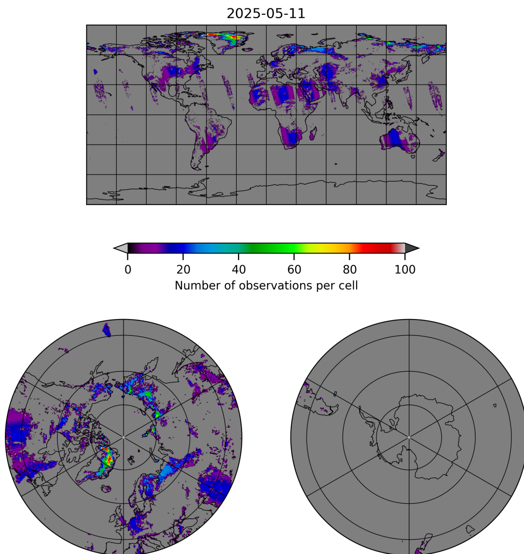
Figure 10: Map of the number of observations for 2025-05-10 to 2025-05-12
