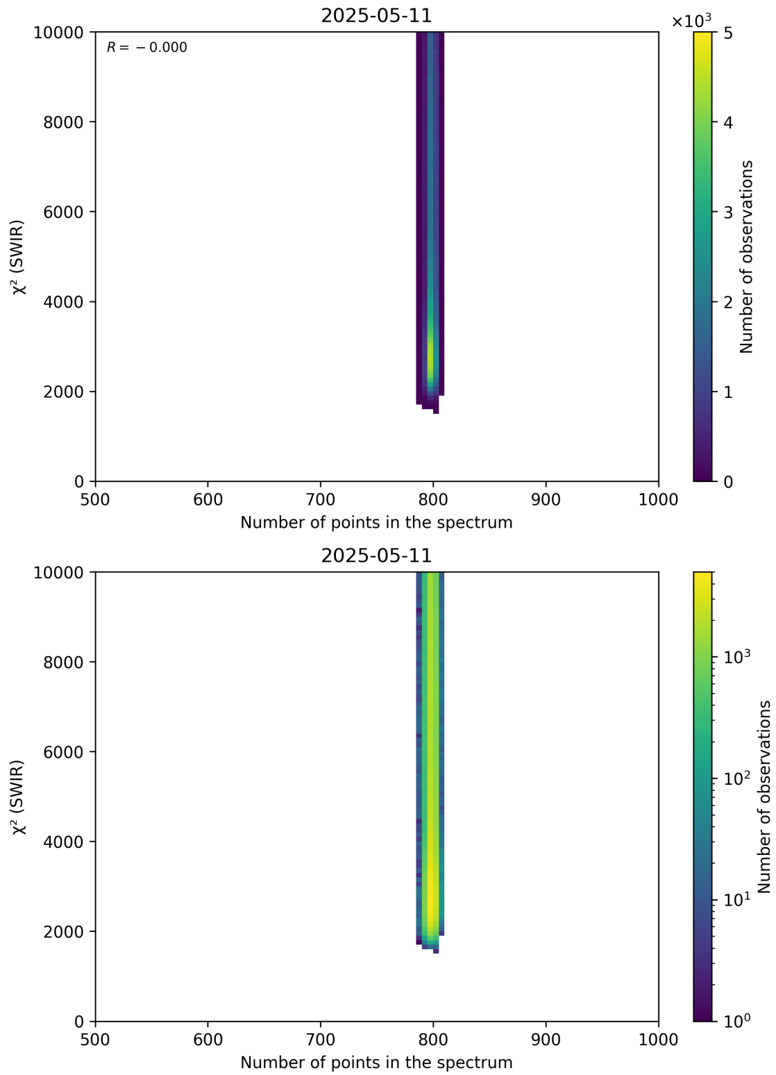
Figure 89: Scatter density plot of “Number of points in the spectrum” against “ \chi^2 (SWIR)” for 2025-05-10 to 2025-05-12.
