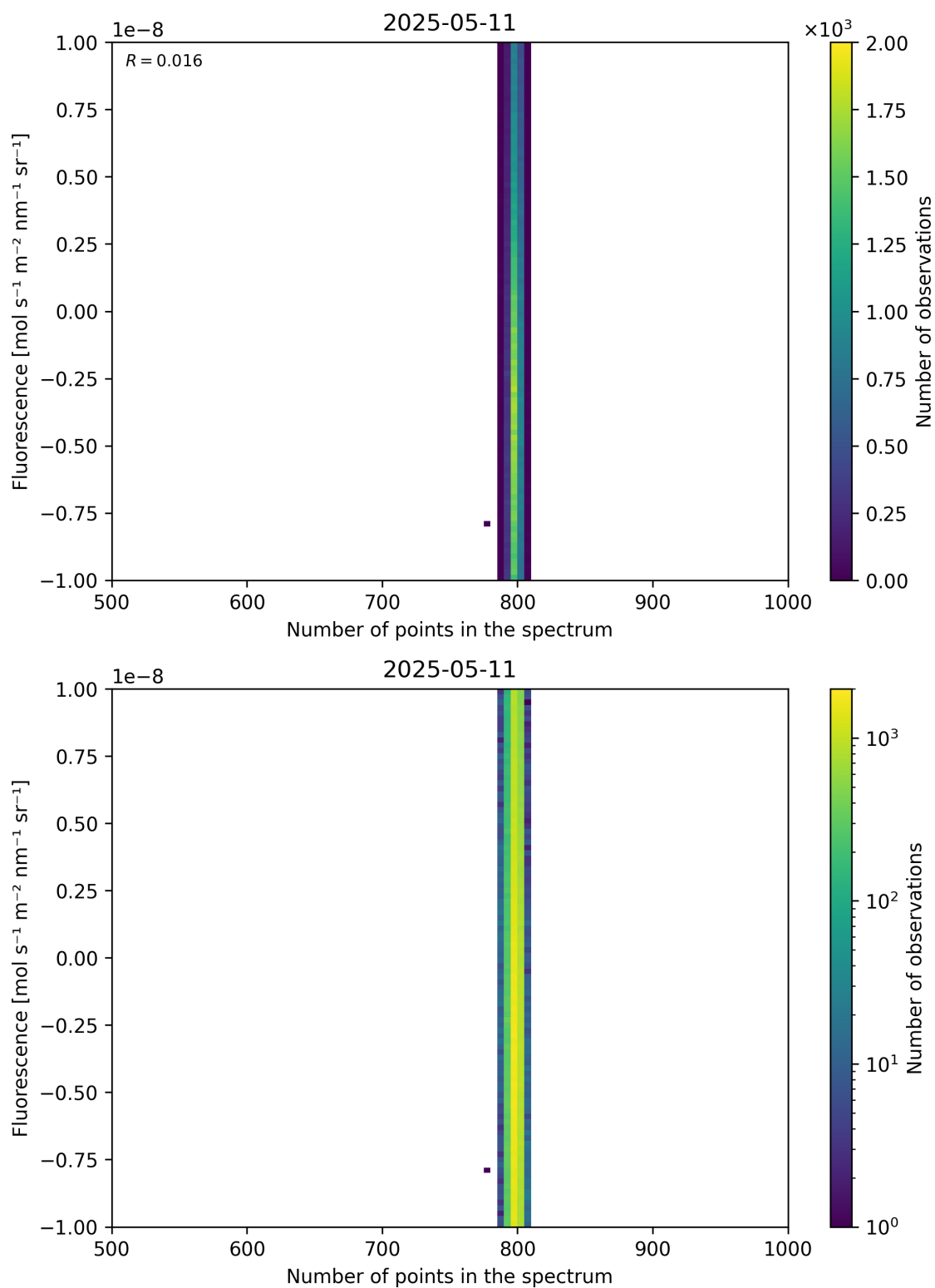
Figure 91: Scatter density plot of “Number of points in the spectrum” against “Fluorescence” for 2025-05-10 to 2025-05-12.
