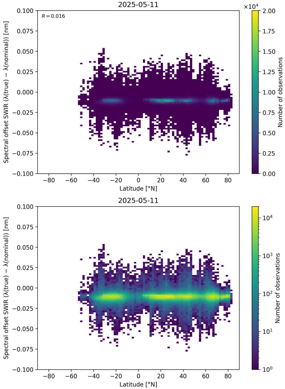
Figure 62: Scatter density plot of “Latitude” against “Spectral offset SWIR ( \lambda_{\text{true}} - \lambda_{\text{nominal}} )” for 2025-05-10 to 2025-05-12.
