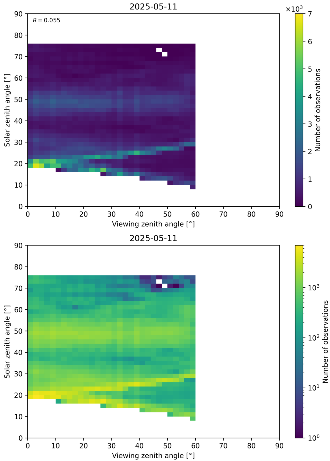
Figure 115: Scatter density plot of “Viewing zenith angle” against “Solar zenith angle” for 2025-05-10 to 2025-05-12.
