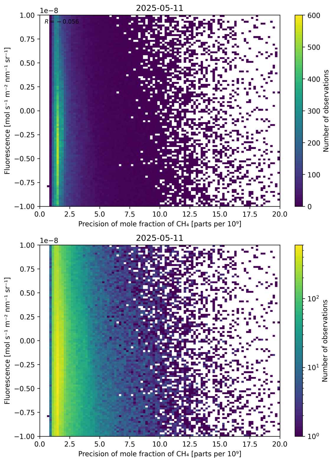
Figure 81: Scatter density plot of “Precision of mole fraction of CH 4 ” against “Fluorescence” for 2025-05-10 to 2025-05-12.
