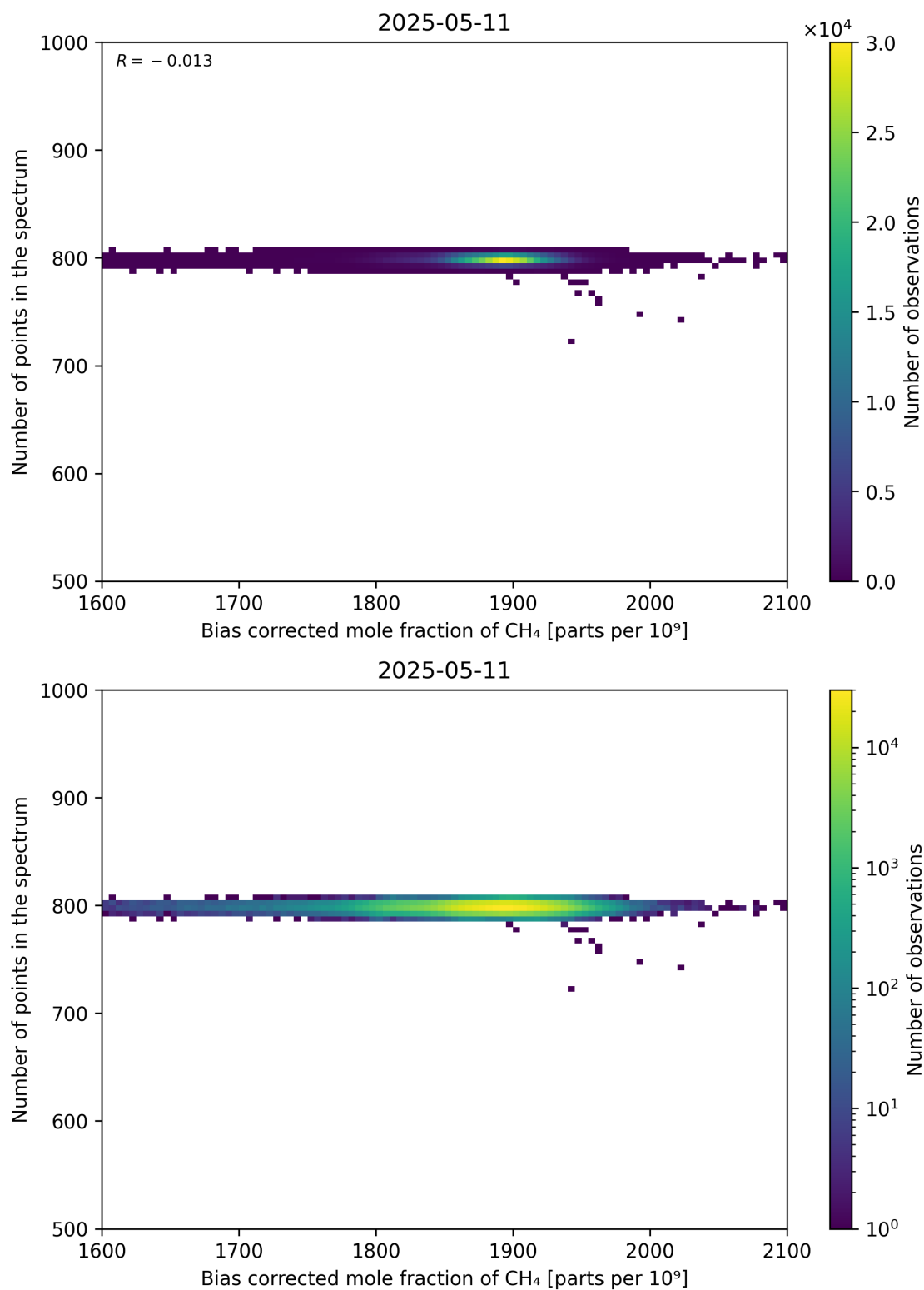
Figure 68: Scatter density plot of “Bias corrected mole fraction of CH 4 ” against “Number of points in the spectrum” for 2025-05-10 to 2025-05-12.
