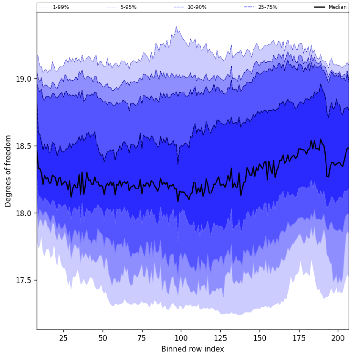
Figure 41: Along track statistics of “Degrees of freedom” for 2025-05-10 to 2025-05-12
