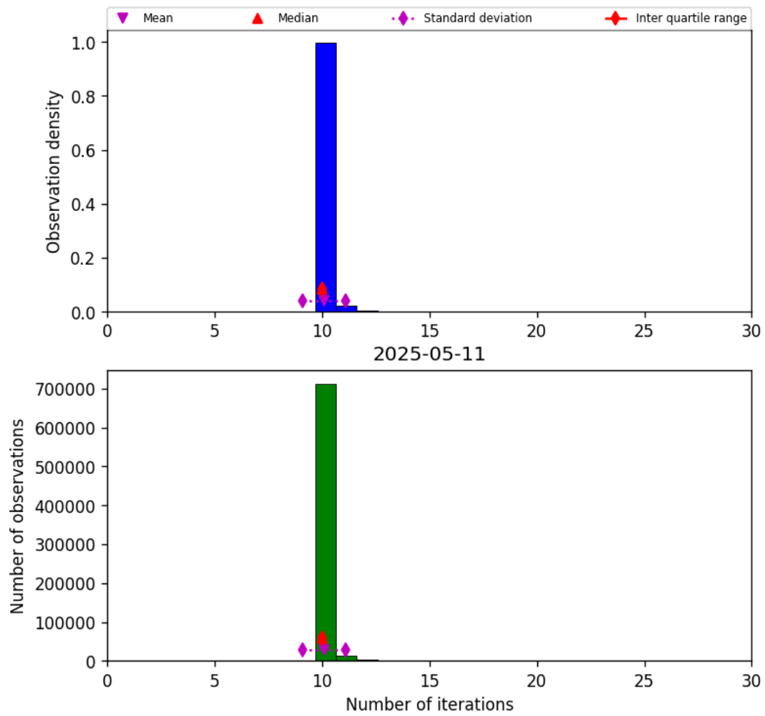
Figure 31: Histogram of “Number of iterations” for 2025-05-10 to 2025-05-12
