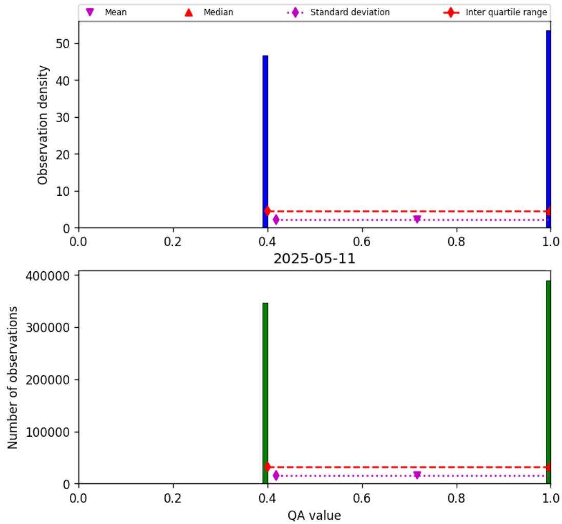
Figure 22: Histogram of “QA value” for 2025-05-10 to 2025-05-12
