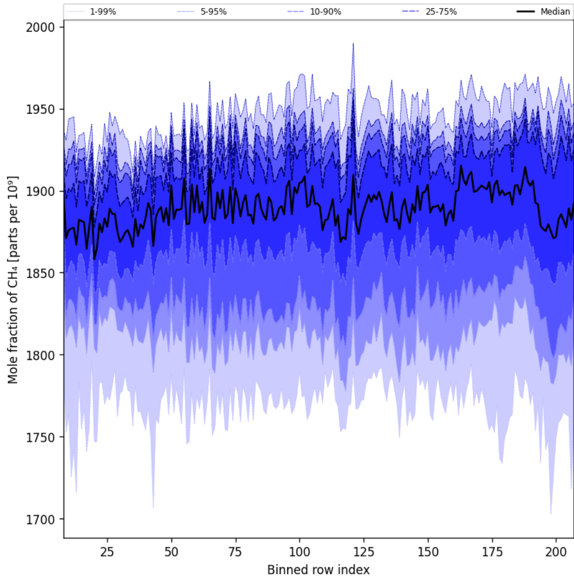
Figure 34: Along track statistics of “Mole fraction of CH 4 ” for 2025-05-10 to 2025-05-12
