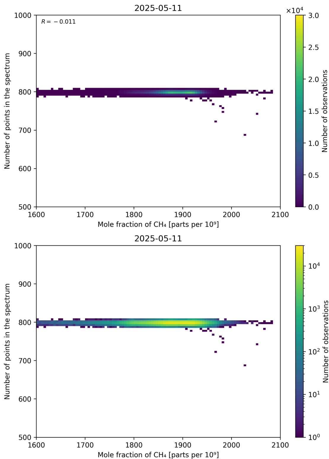
Figure 77: Scatter density plot of “Mole fraction of CH 4 ” against “Number of points in the spectrum” for 2025-05-10 to 2025-05-12.
