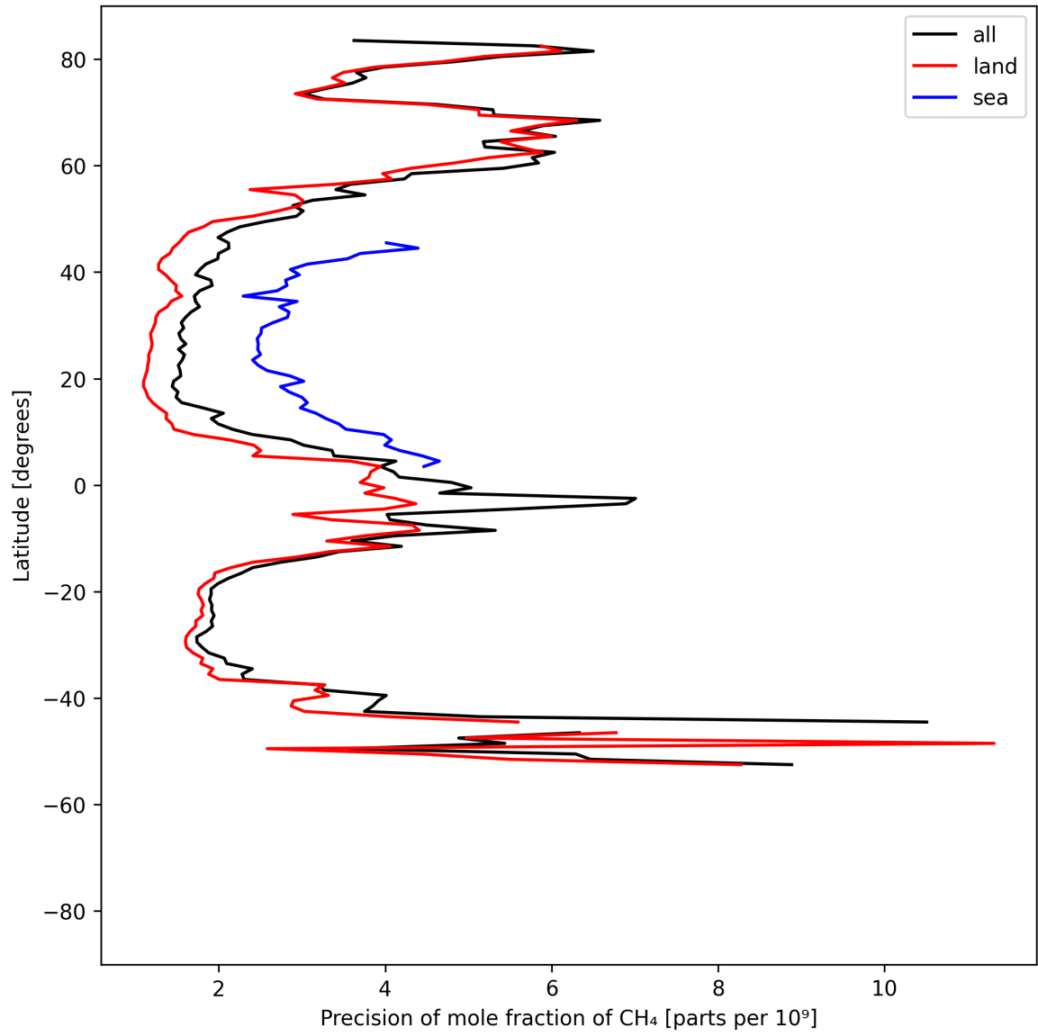
Figure 13: Zonal average of “Precision of mole fraction of CH 4 ” for 2025-05-10 to 2025-05-12.
