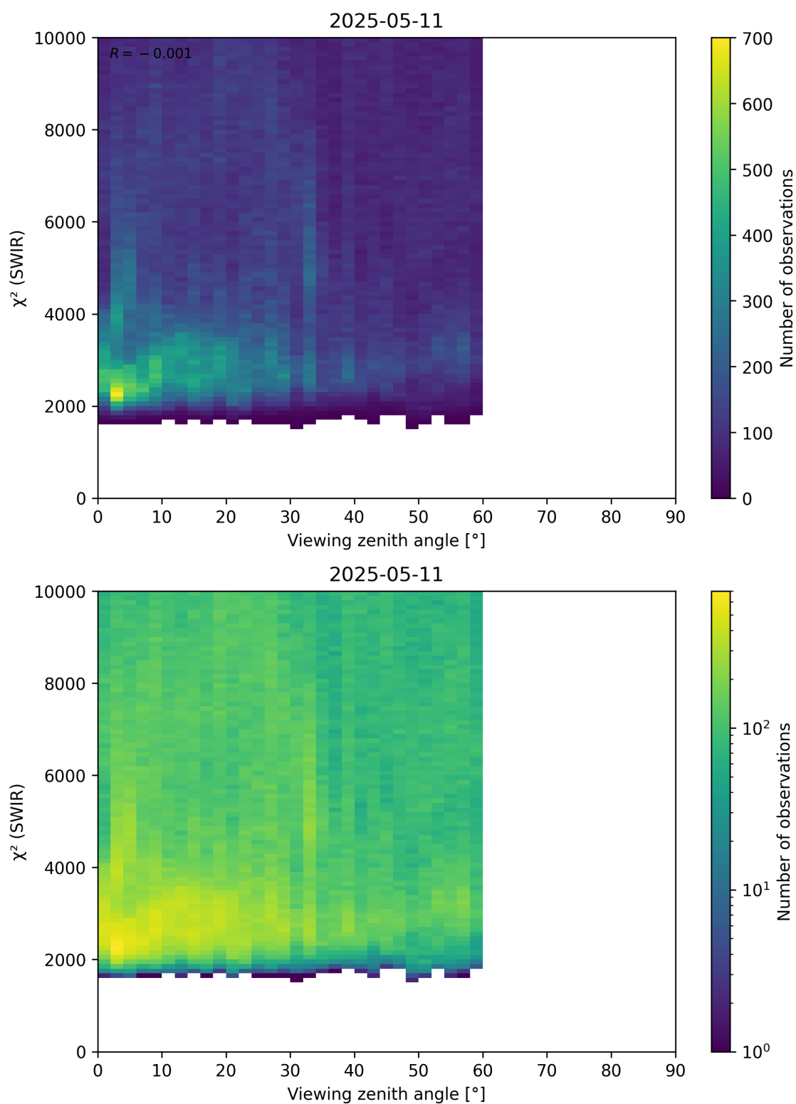
Figure 106: Scatter density plot of “Viewing zenith angle” against “ \chi^2 (SWIR)” for 2025-05-10 to 2025-05-12.
