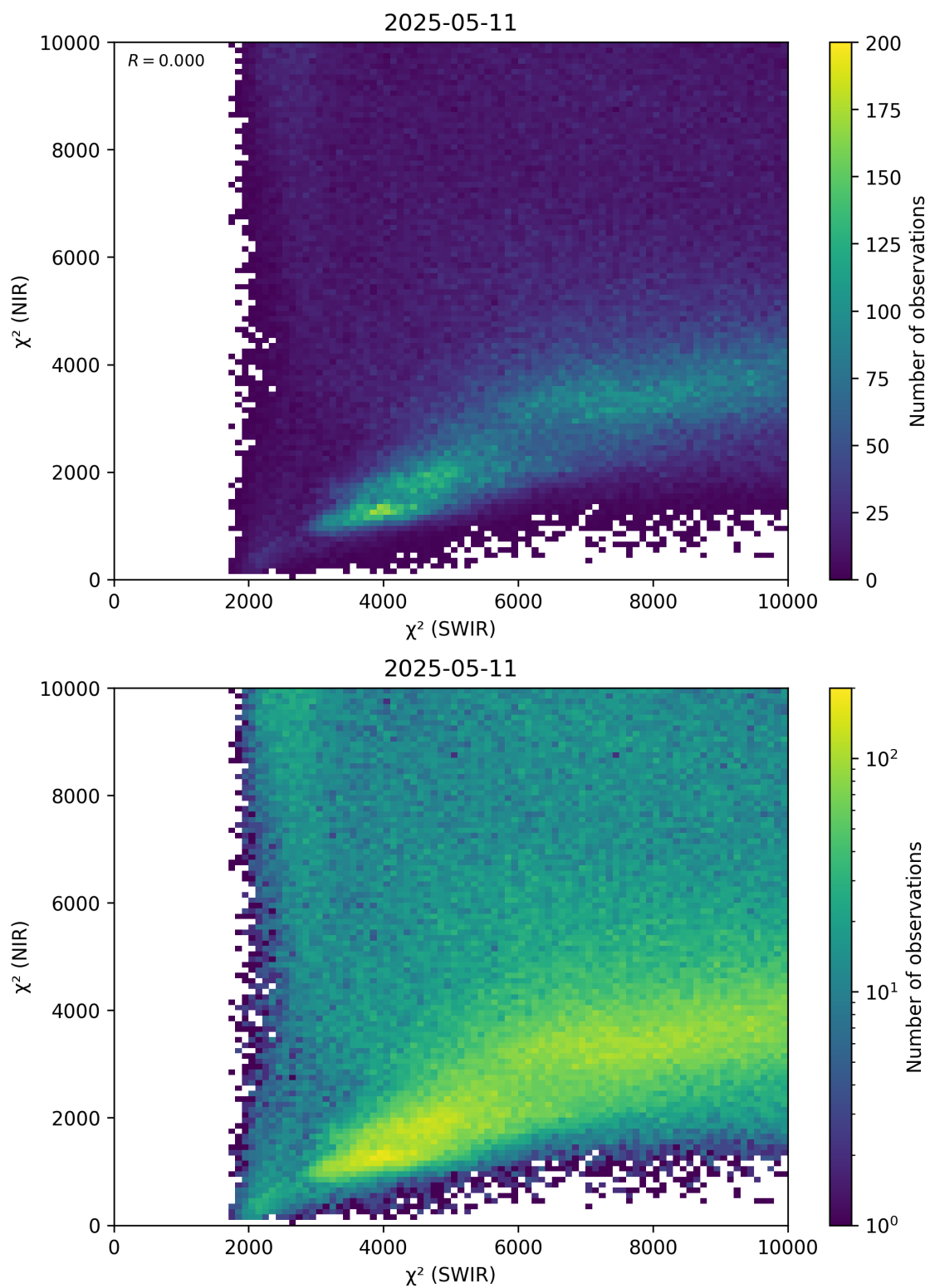
Figure 47: Scatter density plot of “ \chi^2 (SWIR)” against “ \chi^2 (NIR)” for 2025-05-10 to 2025-05-12.
