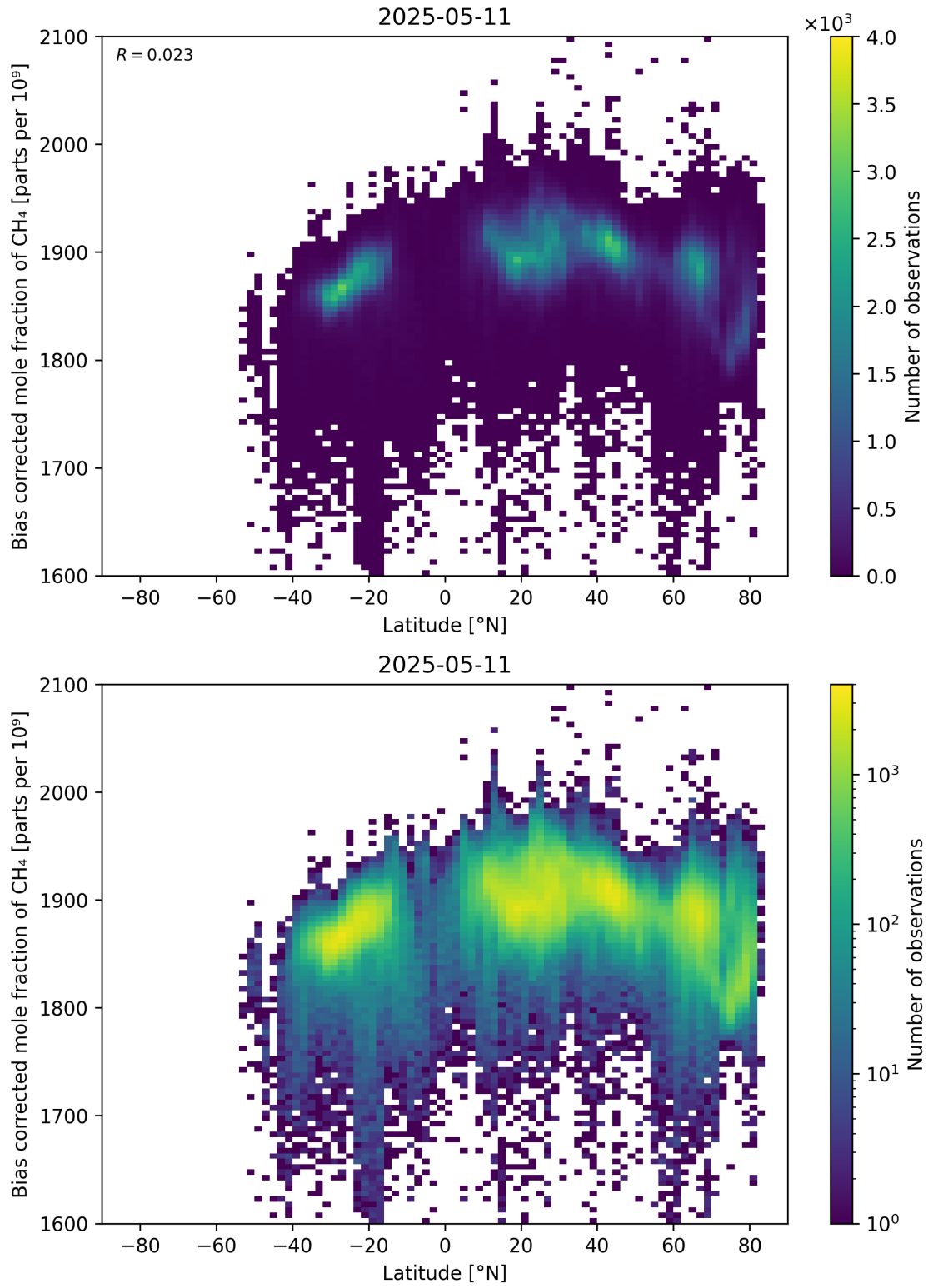
Figure 58: Scatter density plot of “Latitude” against “Bias corrected mole fraction of \text{CH}_4 ” for 2025-05-10 to 2025-05-12.
