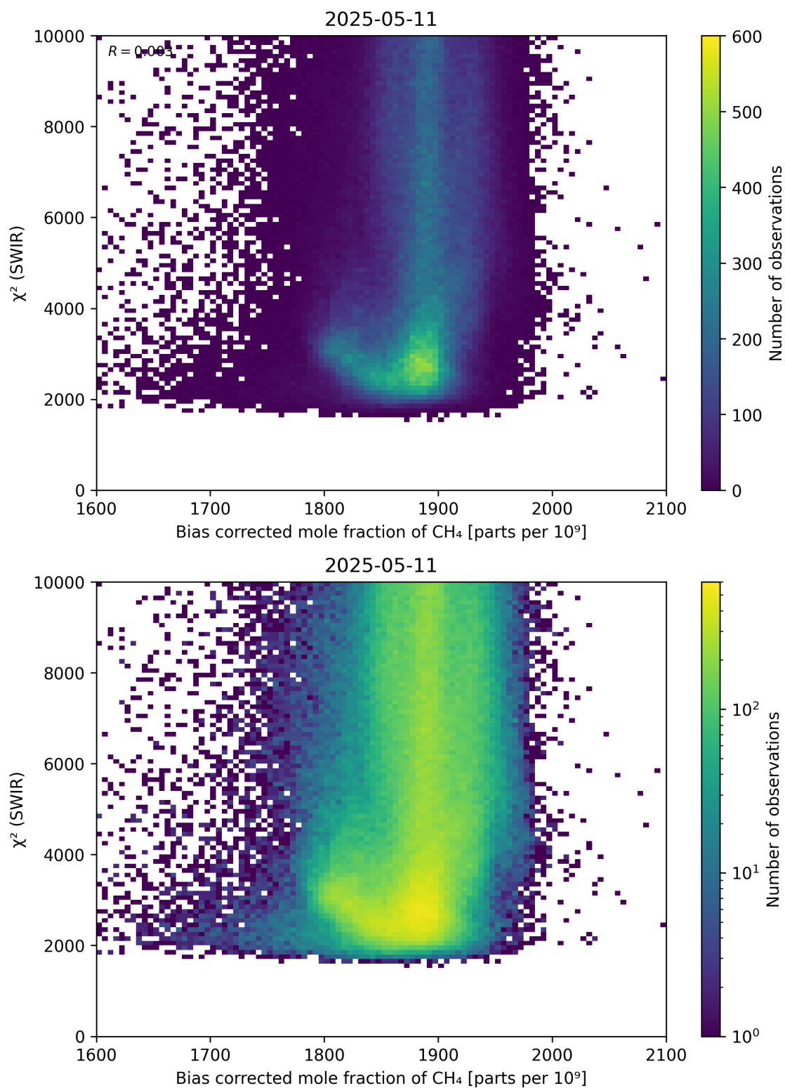
Figure 64: Scatter density plot of “Bias corrected mole fraction of \text{CH}_4 ” against “ \chi^2 (SWIR)” for 2025-05-10 to 2025-05-12.
