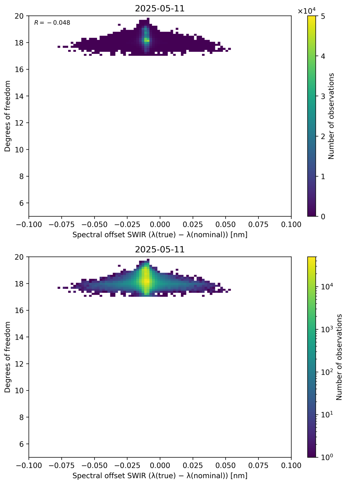
Figure 119: Scatter density plot of “Spectral offset SWIR ( \lambda_{\text{true}} - \lambda_{\text{nominal}} )” against “Degrees of freedom” for 2025-05-10 to 2025-05-12.
