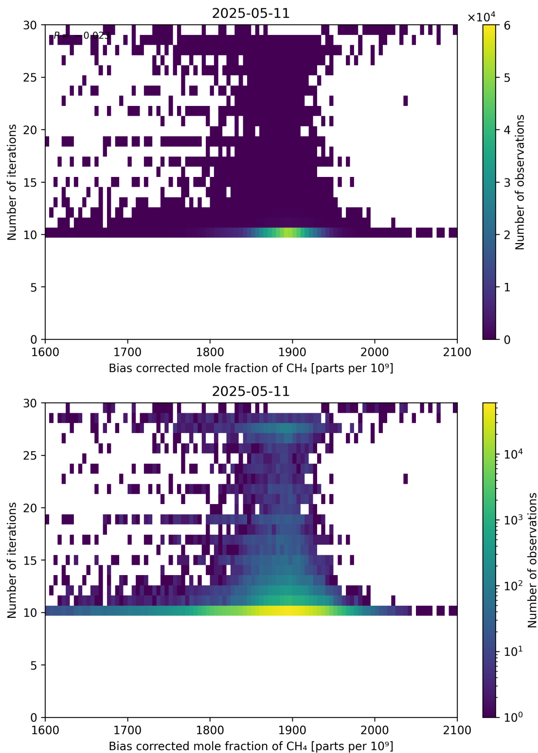
Figure 67: Scatter density plot of “Bias corrected mole fraction of CH 4 ” against “Number of iterations” for 2025-05-10 to 2025-05-12.
