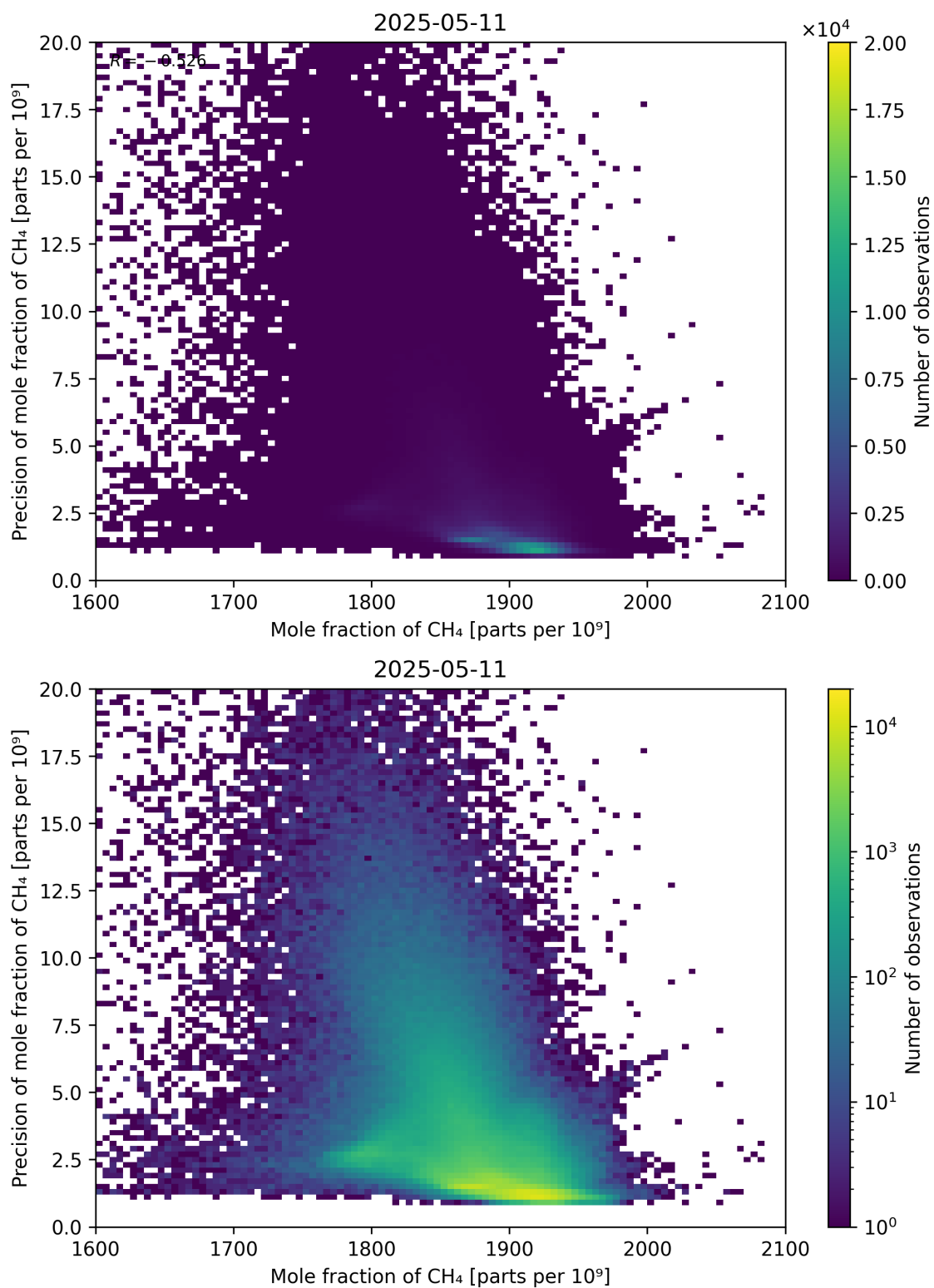
Figure 75: Scatter density plot of “Mole fraction of CH 4 ” against “Precision of mole fraction of CH 4 ” for 2025-05-10 to 2025-05-12.
