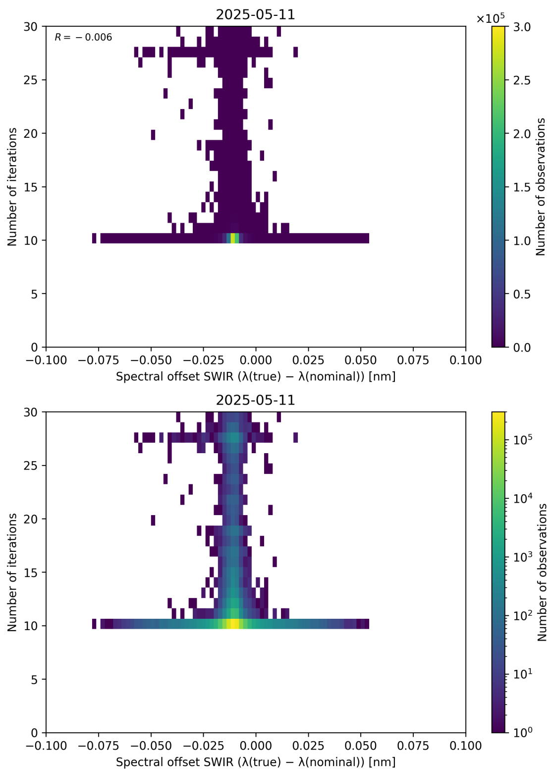
Figure 121: Scatter density plot of “Spectral offset SWIR ( \lambda_{\text{true}} - \lambda_{\text{nominal}} )” against “Number of iterations” for 2025-05-10 to 2025-05-12.
