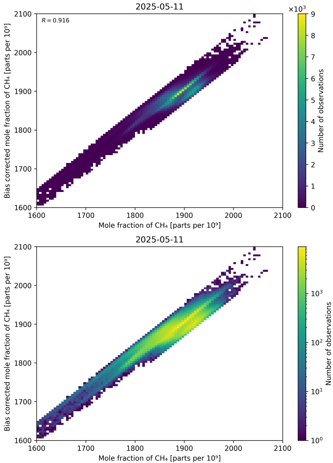
Figure 74: Scatter density plot of “Mole fraction of CH 4 ” against “Bias corrected mole fraction of CH 4 ” for 2025-05-10 to 2025-05-12.
