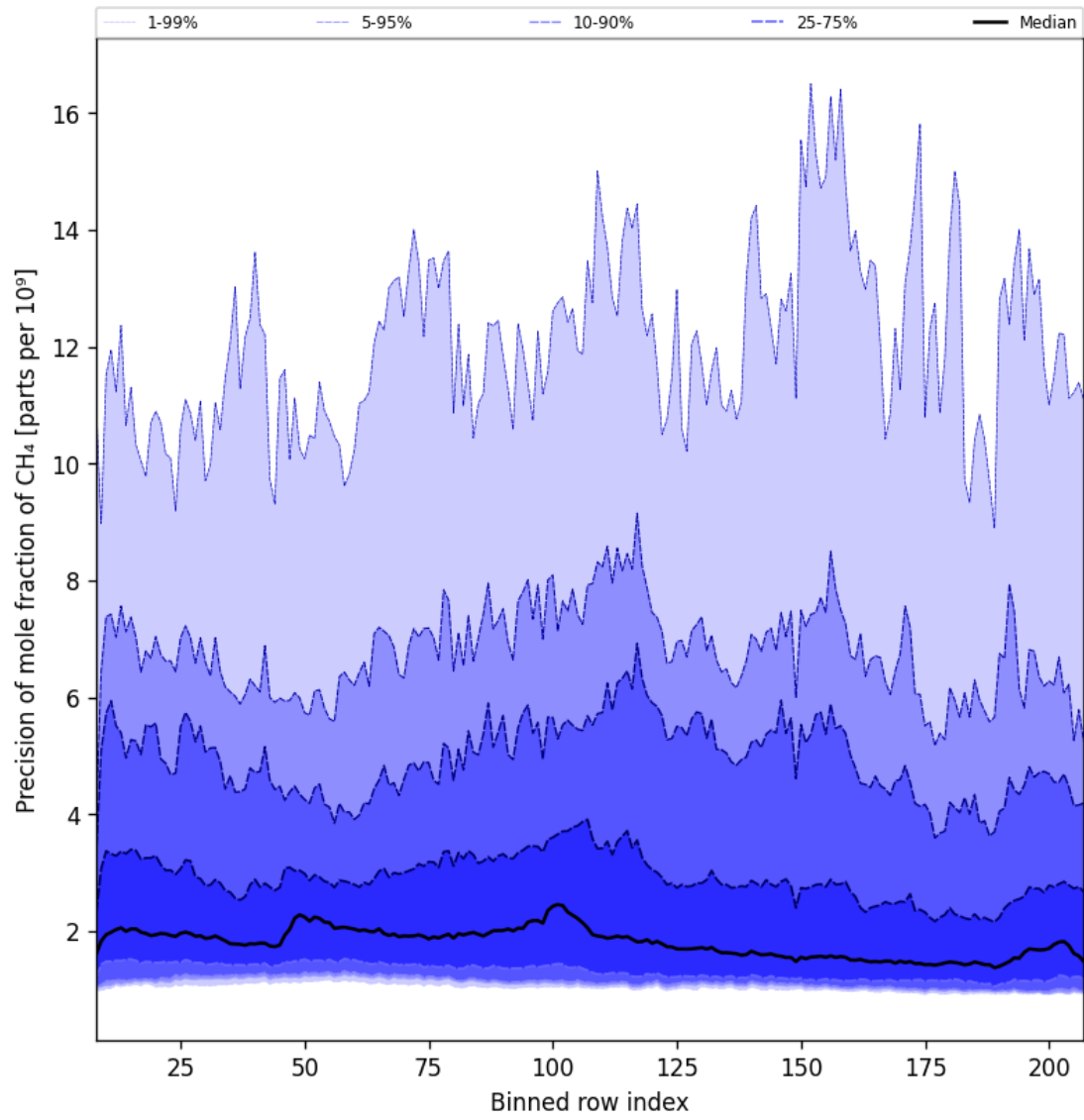
Figure 35: Along track statistics of “Precision of mole fraction of CH 4 ” for 2025-05-10 to 2025-05-12
