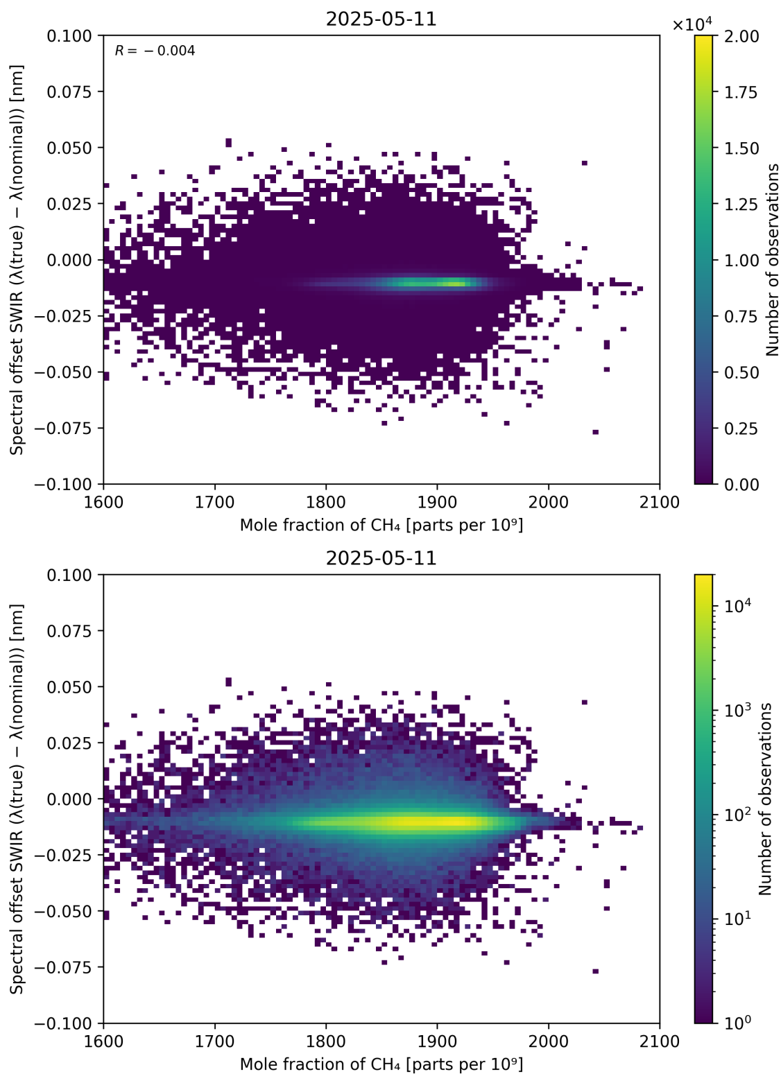
Figure 86: Scatter density plot of “Mole fraction of CH 4 ” against “Spectral offset SWIR ( \lambda_{\text{true}} - \lambda_{\text{nominal}} )” for 2025-05-10 to 2025-05-12.
