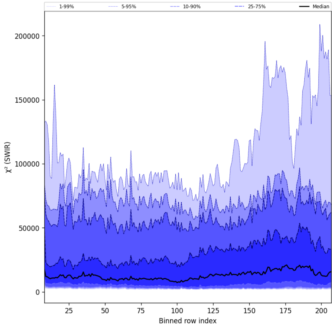
Figure 39: Along track statistics of “ \chi^2 (SWIR)” for 2025-05-10 to 2025-05-12
