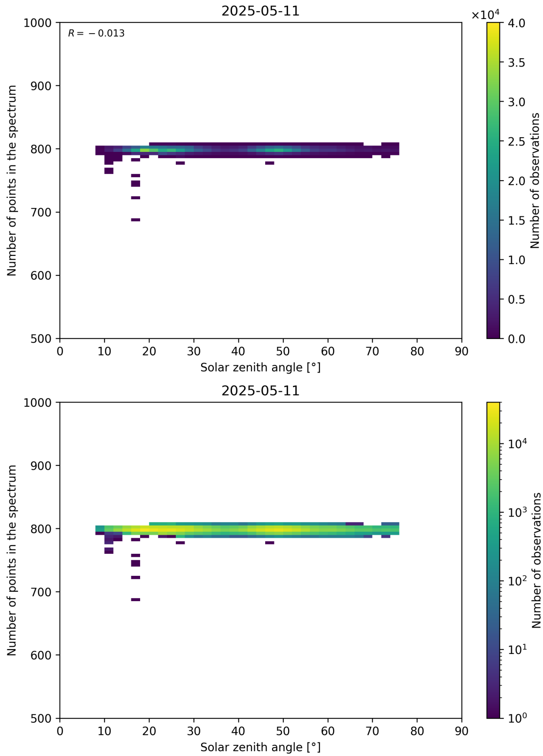
Figure 103: Scatter density plot of “Solar zenith angle” against “Number of points in the spectrum” for 2025-05-10 to 2025-05-12.
