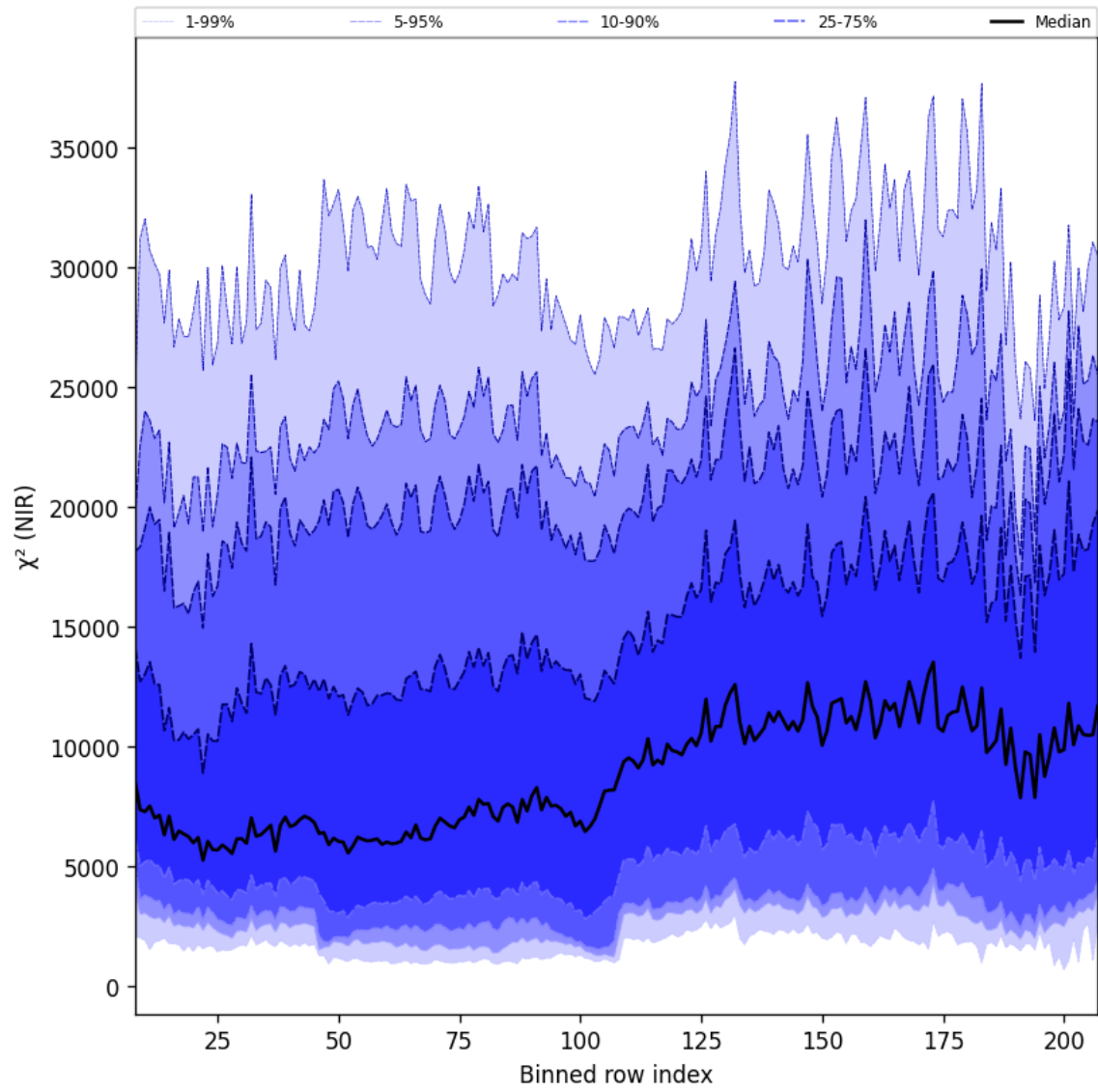
Figure 40: Along track statistics of “ \chi^2 (NIR)” for 2025-05-10 to 2025-05-12
