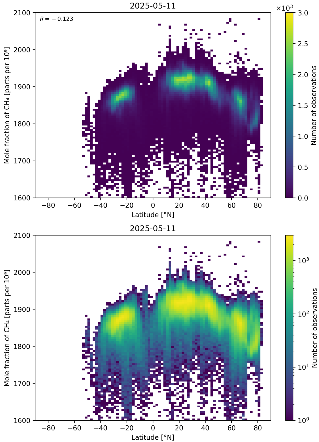
Figure 57: Scatter density plot of “Latitude” against “Mole fraction of CH 4 ” for 2025-05-10 to 2025-05-12.
