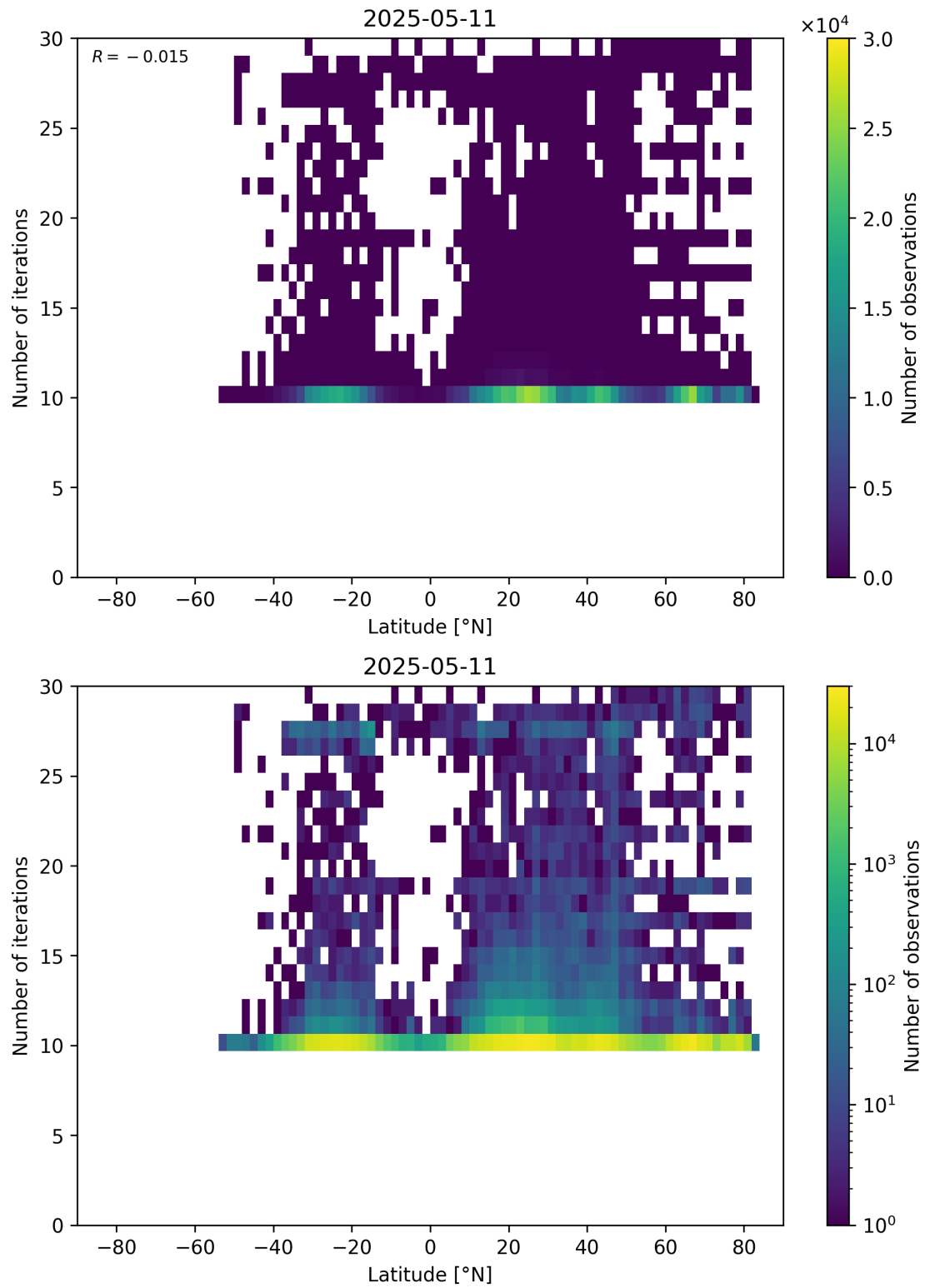
Figure 60: Scatter density plot of “Latitude” against “Number of iterations” for 2025-05-10 to 2025-05-12.
