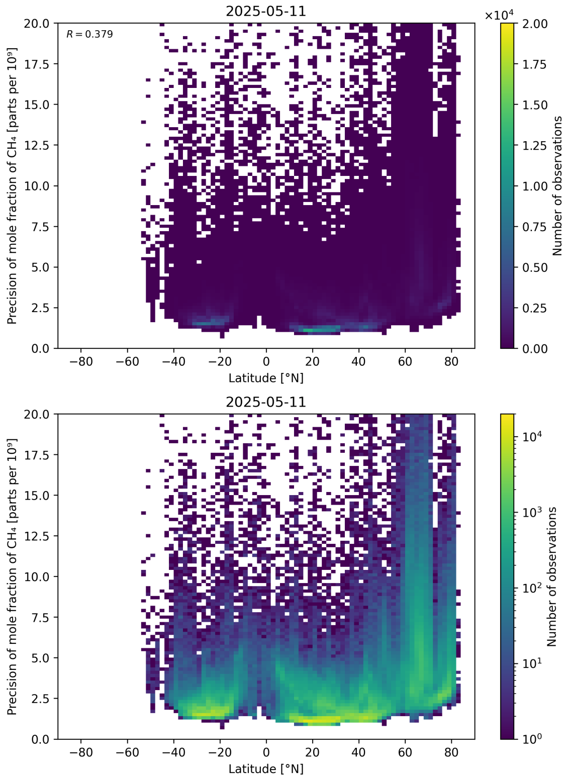
Figure 59: Scatter density plot of “Latitude” against “Precision of mole fraction of \text{CH}_4 ” for 2025-05-10 to 2025-05-12.
