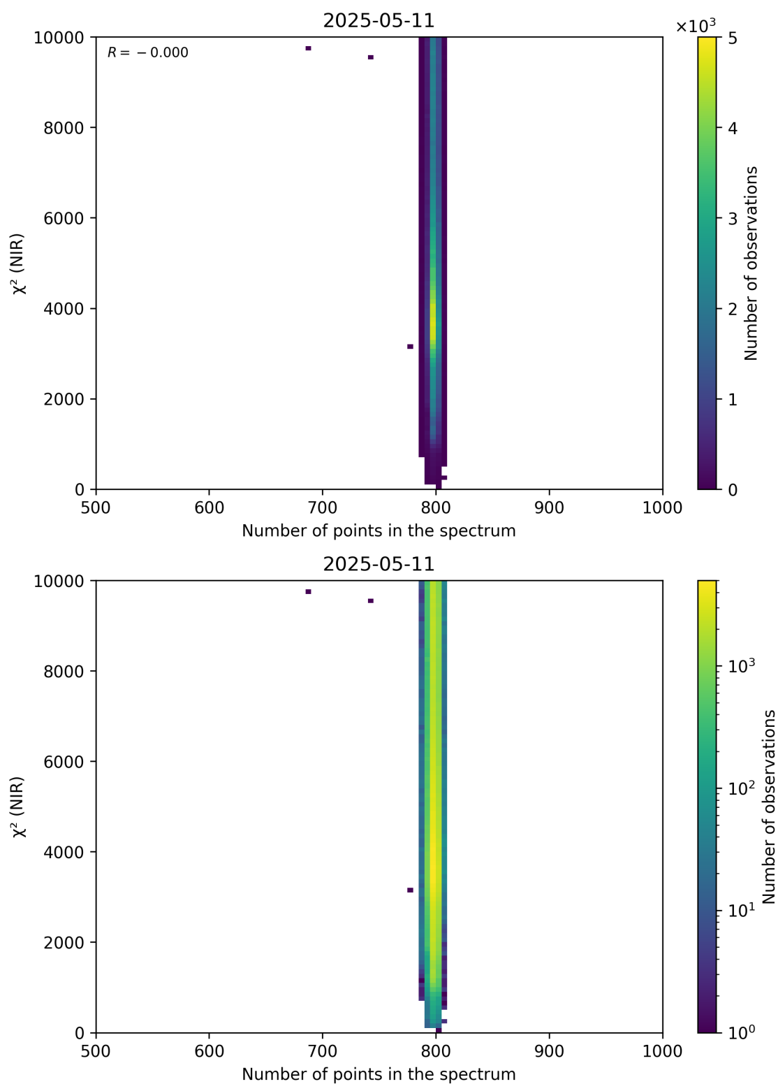
Figure 88: Scatter density plot of “Number of points in the spectrum” against “ \chi^2 (NIR)” for 2025-05-10 to 2025-05-12.
