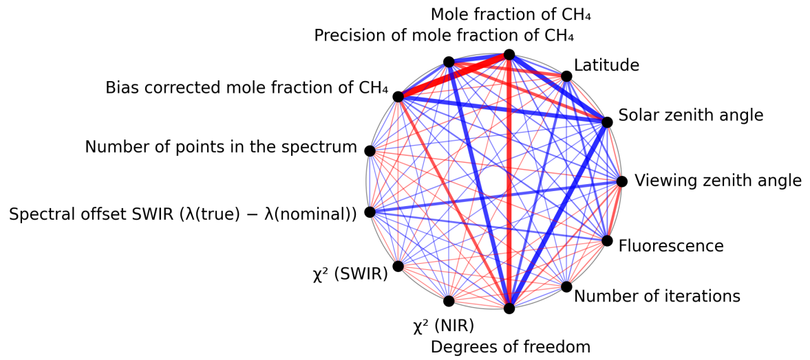
Figure 1: Map of correlation graph for 2025-05-10 to 2025-05-12.
