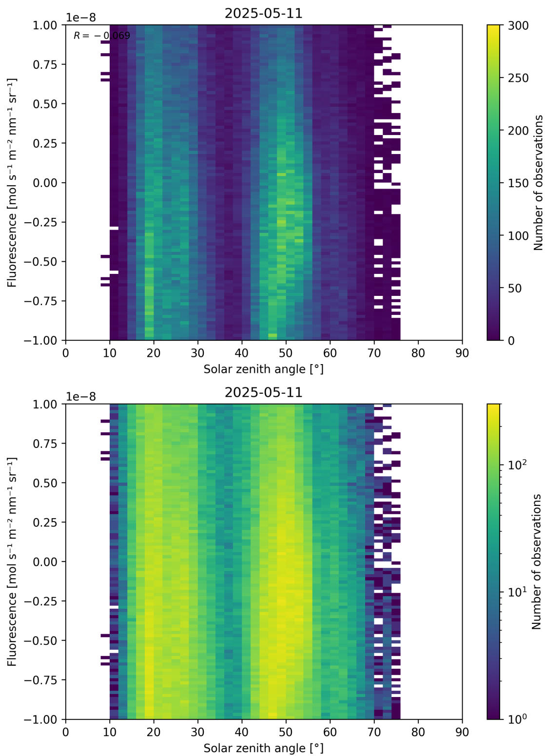
Figure 97: Scatter density plot of “Solar zenith angle” against “Fluorescence” for 2025-05-10 to 2025-05-12.
