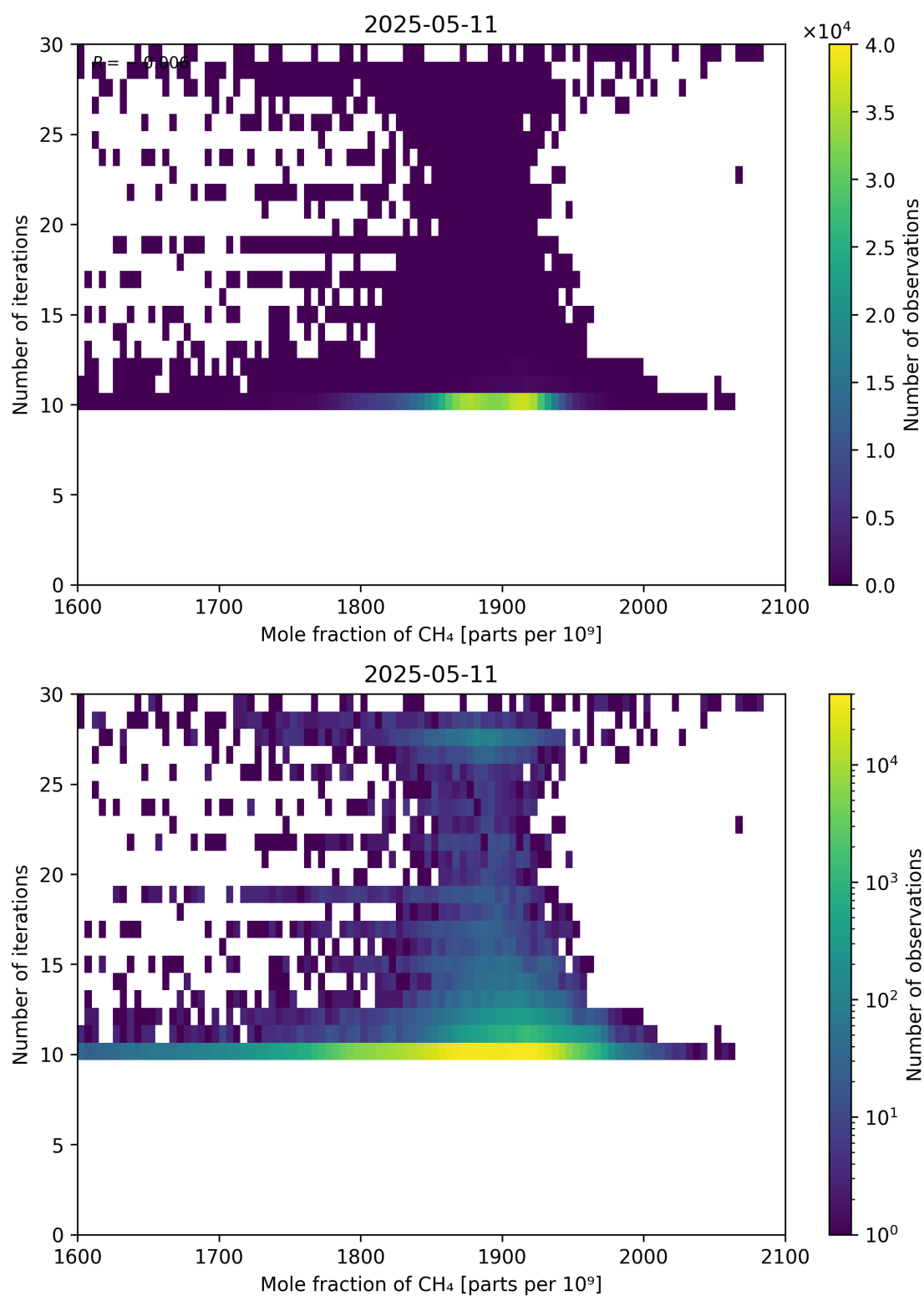
Figure 76: Scatter density plot of “Mole fraction of CH 4 ” against “Number of iterations” for 2025-05-10 to 2025-05-12.
