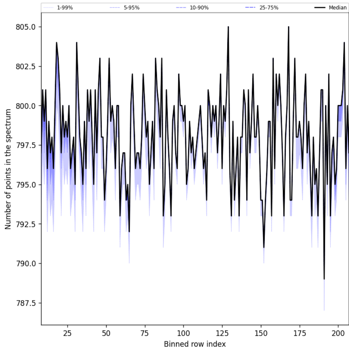
Figure 37: Along track statistics of “Number of points in the spectrum” for 2025-05-10 to 2025-05-12
