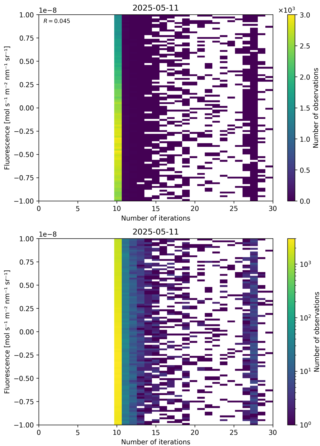
Figure 87: Scatter density plot of "Number of iterations" against "Fluorescence" for 2025-05-10 to 2025-05-12.
