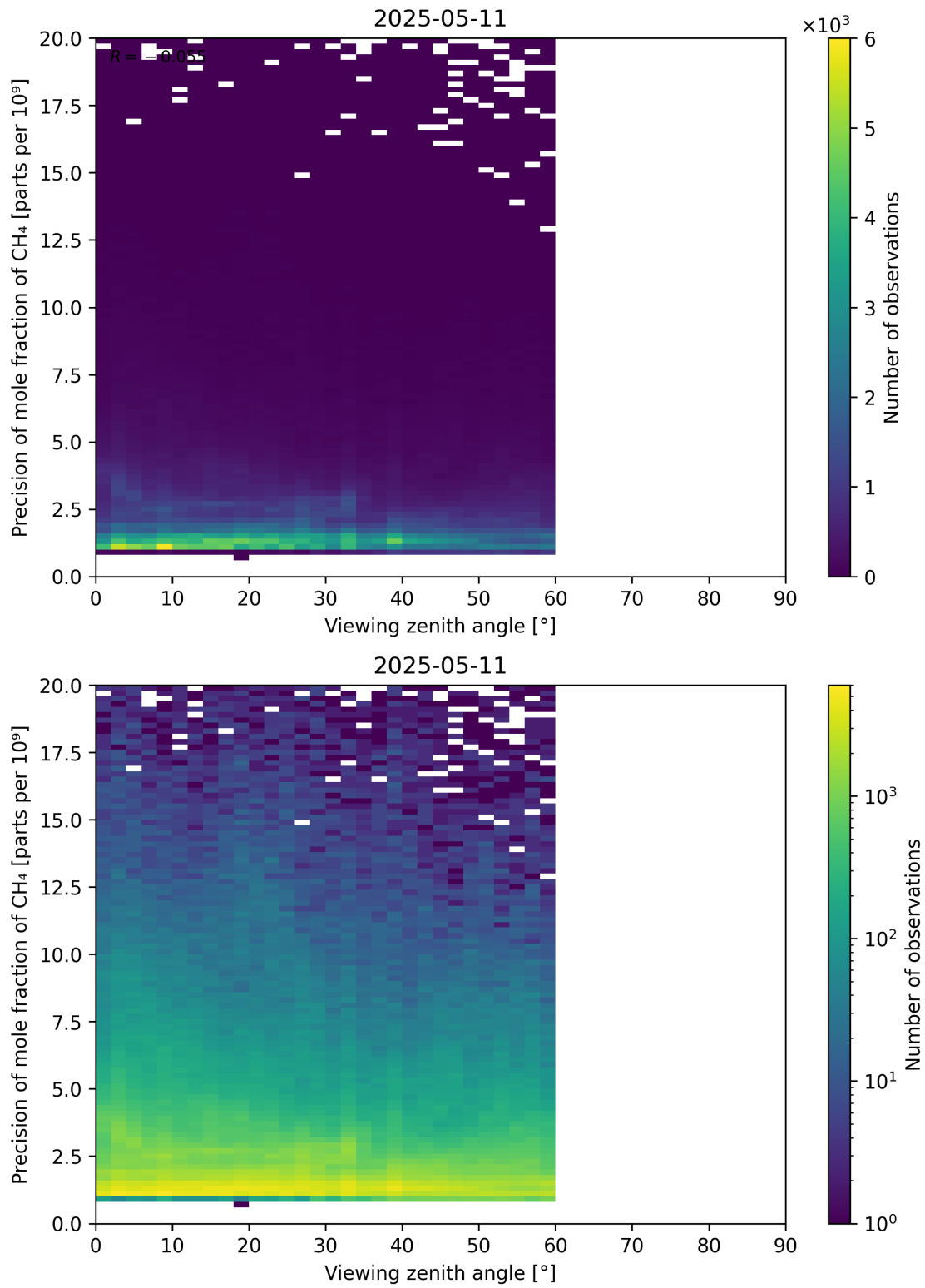
Figure 112: Scatter density plot of “Viewing zenith angle” against “Precision of mole fraction of CH 4 ” for 2025-05-10 to 2025-05-12.
