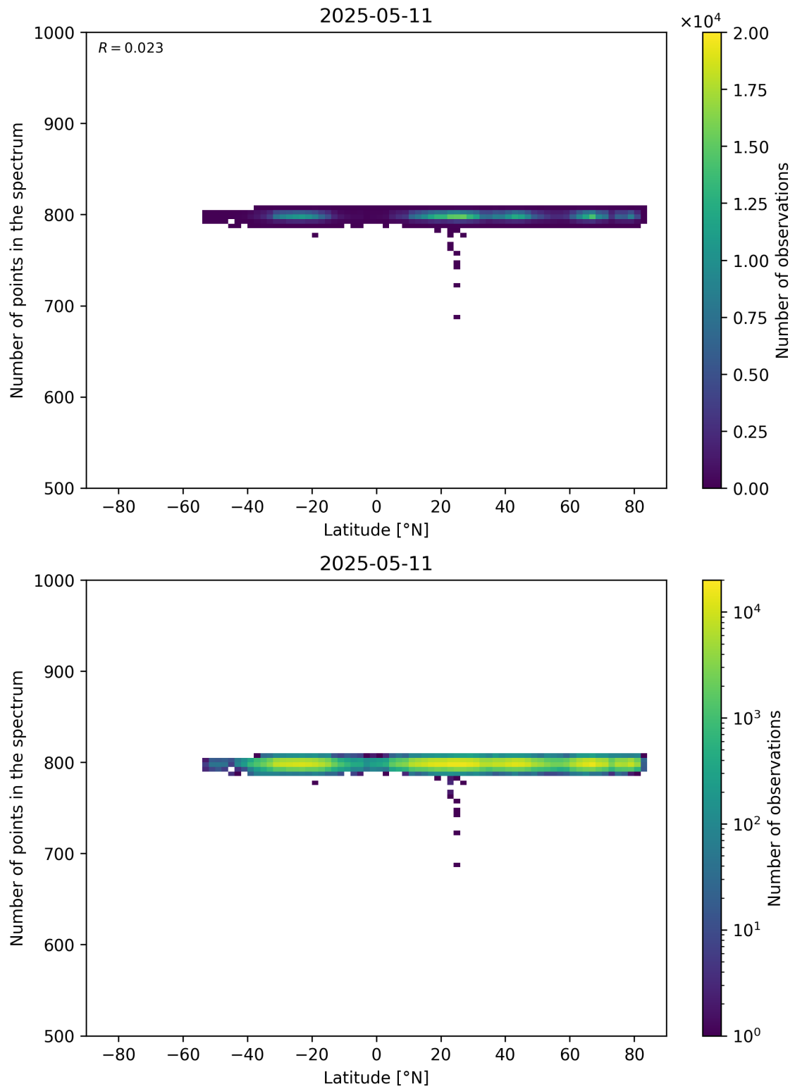
Figure 61: Scatter density plot of “Latitude” against “Number of points in the spectrum” for 2025-05-10 to 2025-05-12.
