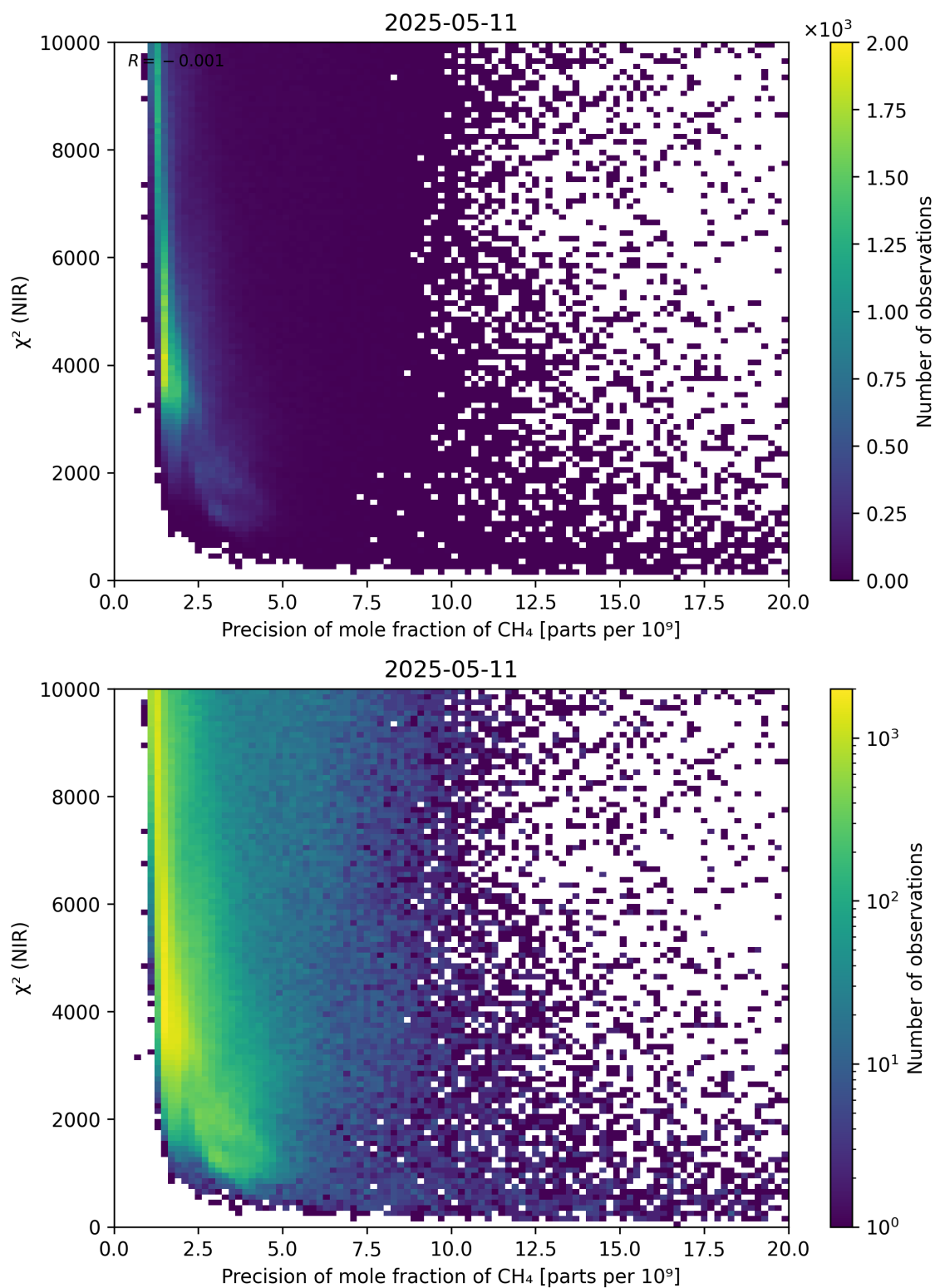
Figure 78: Scatter density plot of “Precision of mole fraction of CH 4 ” against “ \chi^2 (NIR)” for 2025-05-10 to 2025-05-12.
