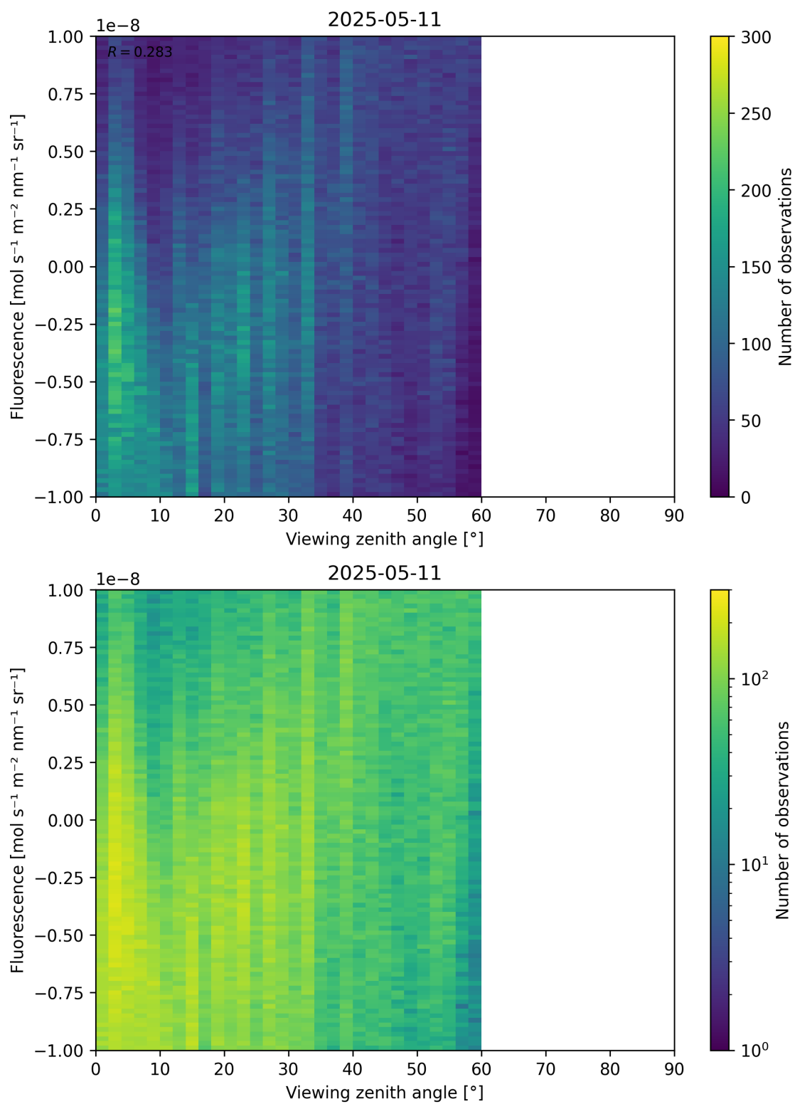
Figure 108: Scatter density plot of “Viewing zenith angle” against “Fluorescence” for 2025-05-10 to 2025-05-12.
