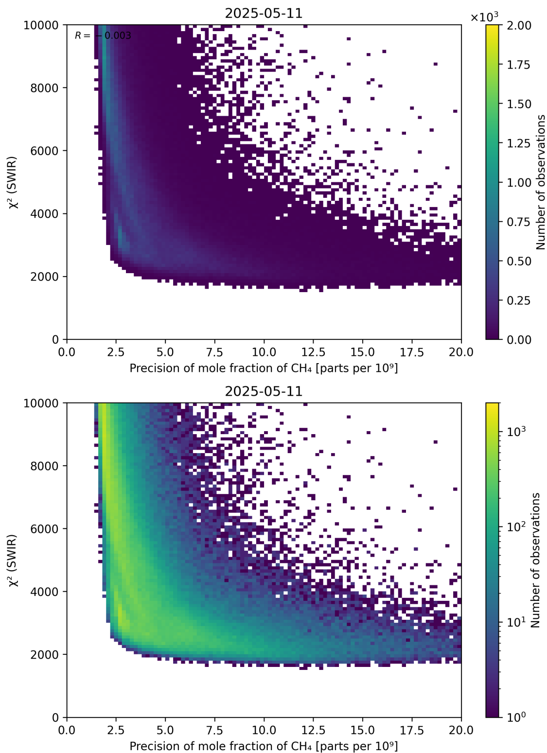
Figure 79: Scatter density plot of “Precision of mole fraction of CH 4 ” against “ \chi^2 (SWIR)” for 2025-05-10 to 2025-05-12.
