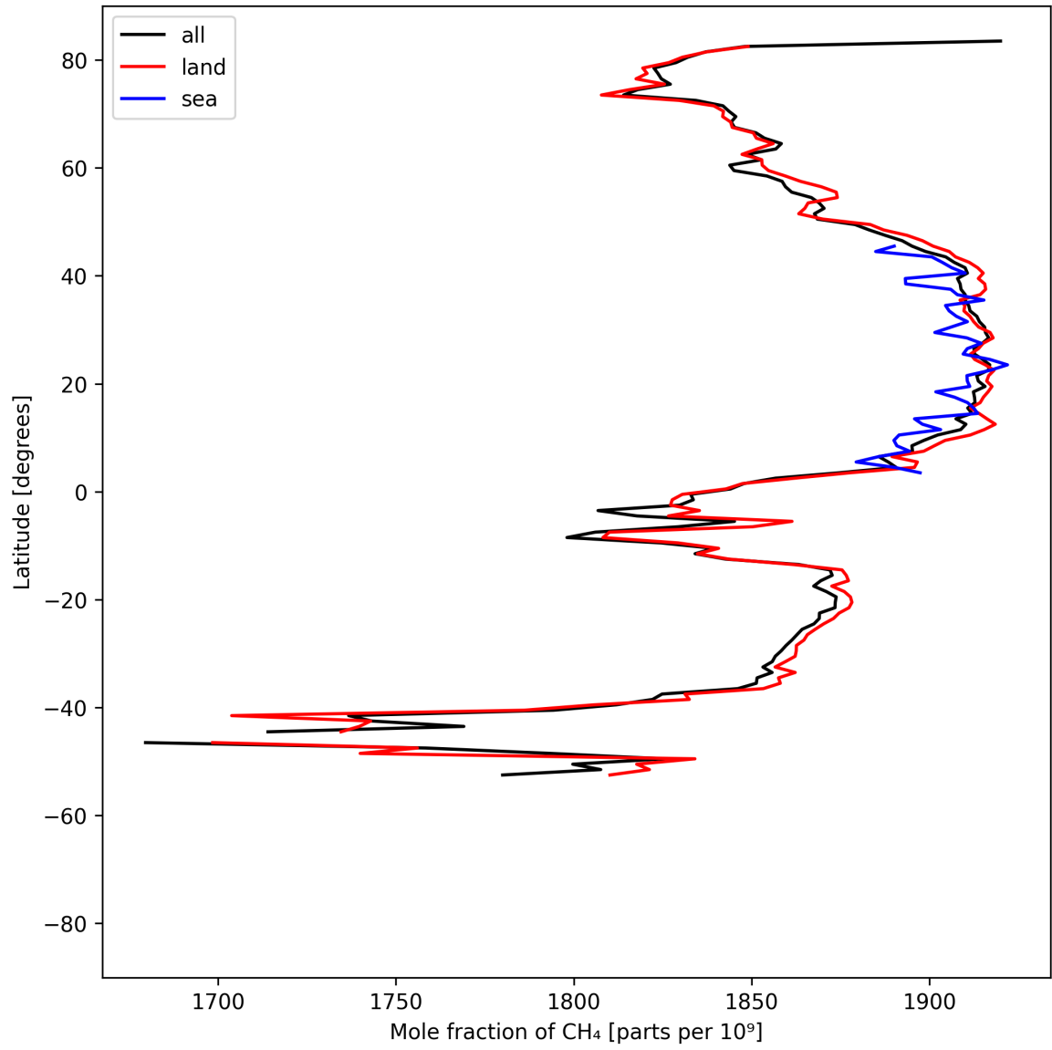
Figure 12: Zonal average of “Mole fraction of \text{CH}_4 ” for 2025-05-10 to 2025-05-12.
