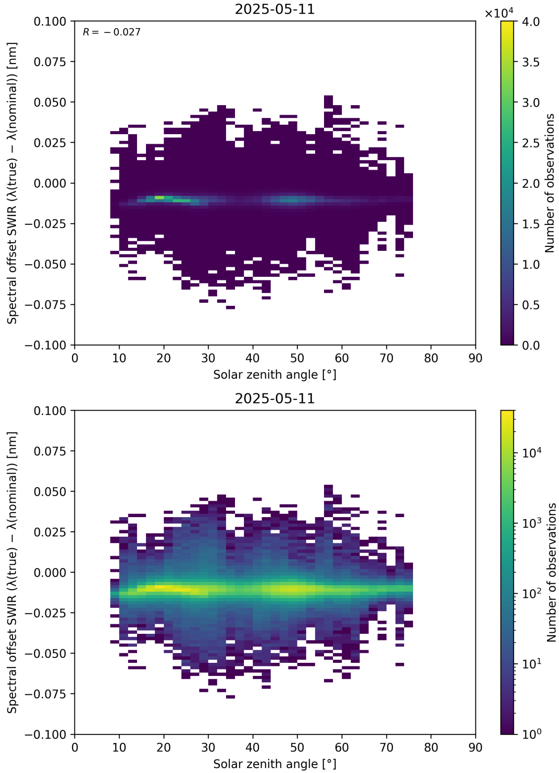
Figure 104: Scatter density plot of “Solar zenith angle” against “Spectral offset SWIR ( \lambda_{\text{true}} - \lambda_{\text{nominal}} )” for 2025-05-10 to 2025-05-12.
