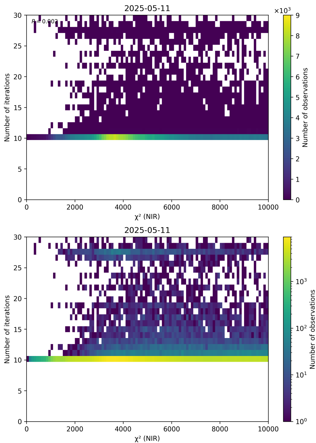
Figure 46: Scatter density plot of “ \chi^2 (NIR)” against “Number of iterations” for 2025-05-10 to 2025-05-12.
