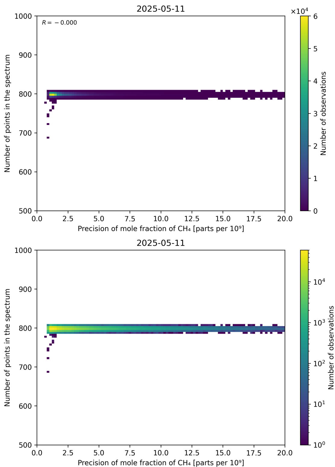
Figure 84: Scatter density plot of “Precision of mole fraction of CH 4 ” against “Number of points in the spectrum” for 2025-05-10 to 2025-05-12.
