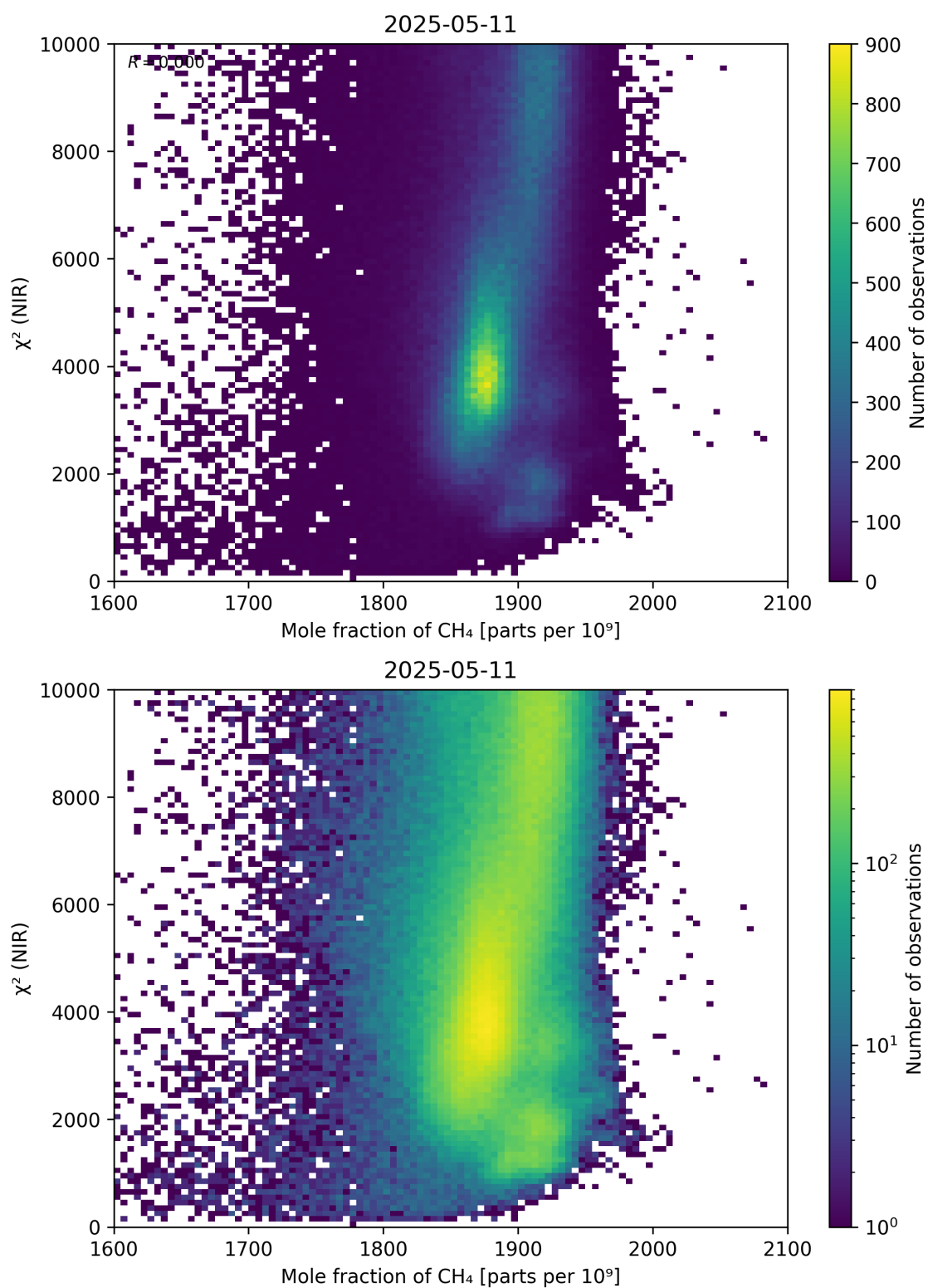
Figure 70: Scatter density plot of “Mole fraction of \text{CH}_4 ” against “ \chi^2 (NIR)” for 2025-05-10 to 2025-05-12.
