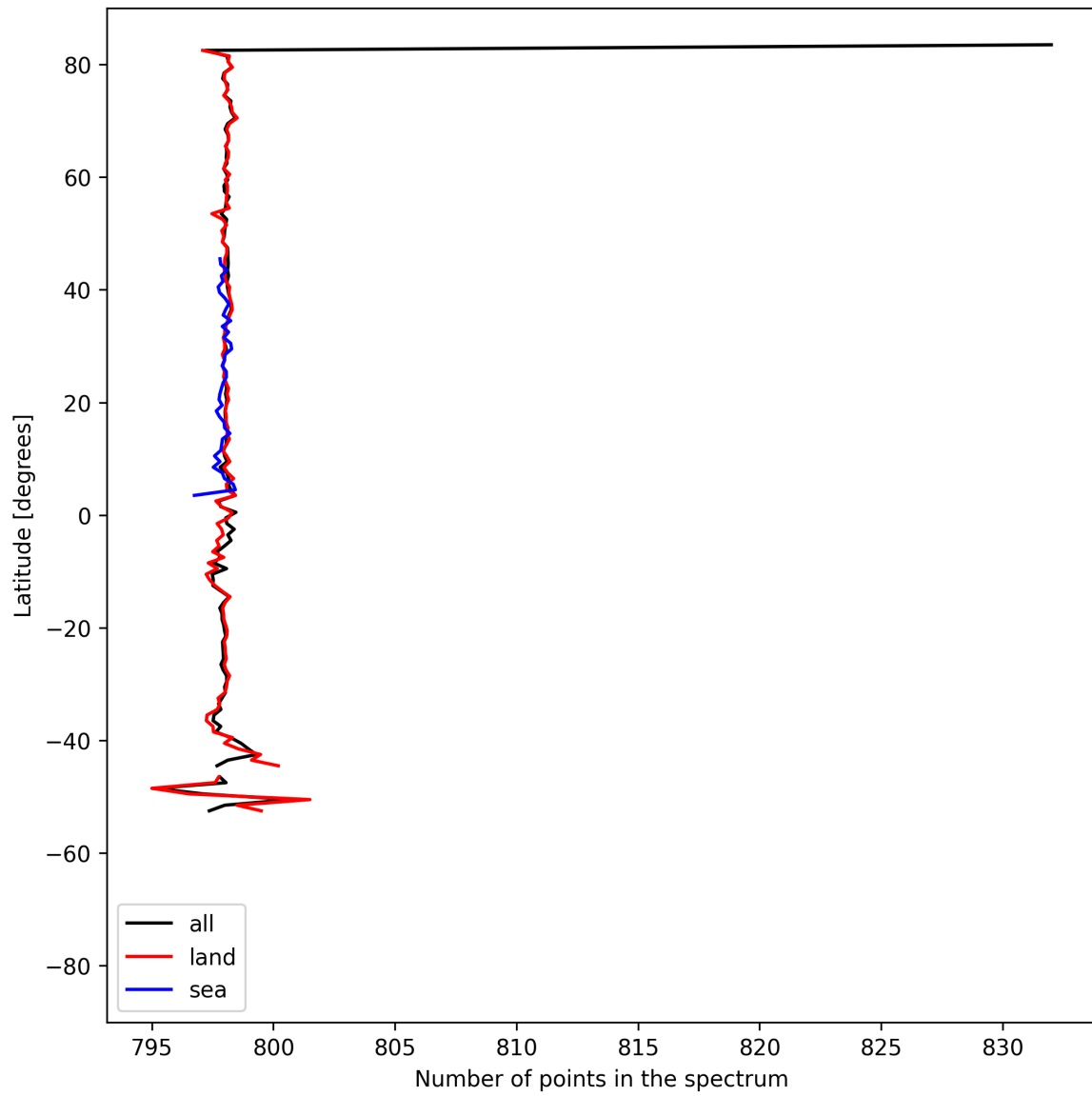
Figure 15: Zonal average of “Number of points in the spectrum” for 2025-05-10 to 2025-05-12.
