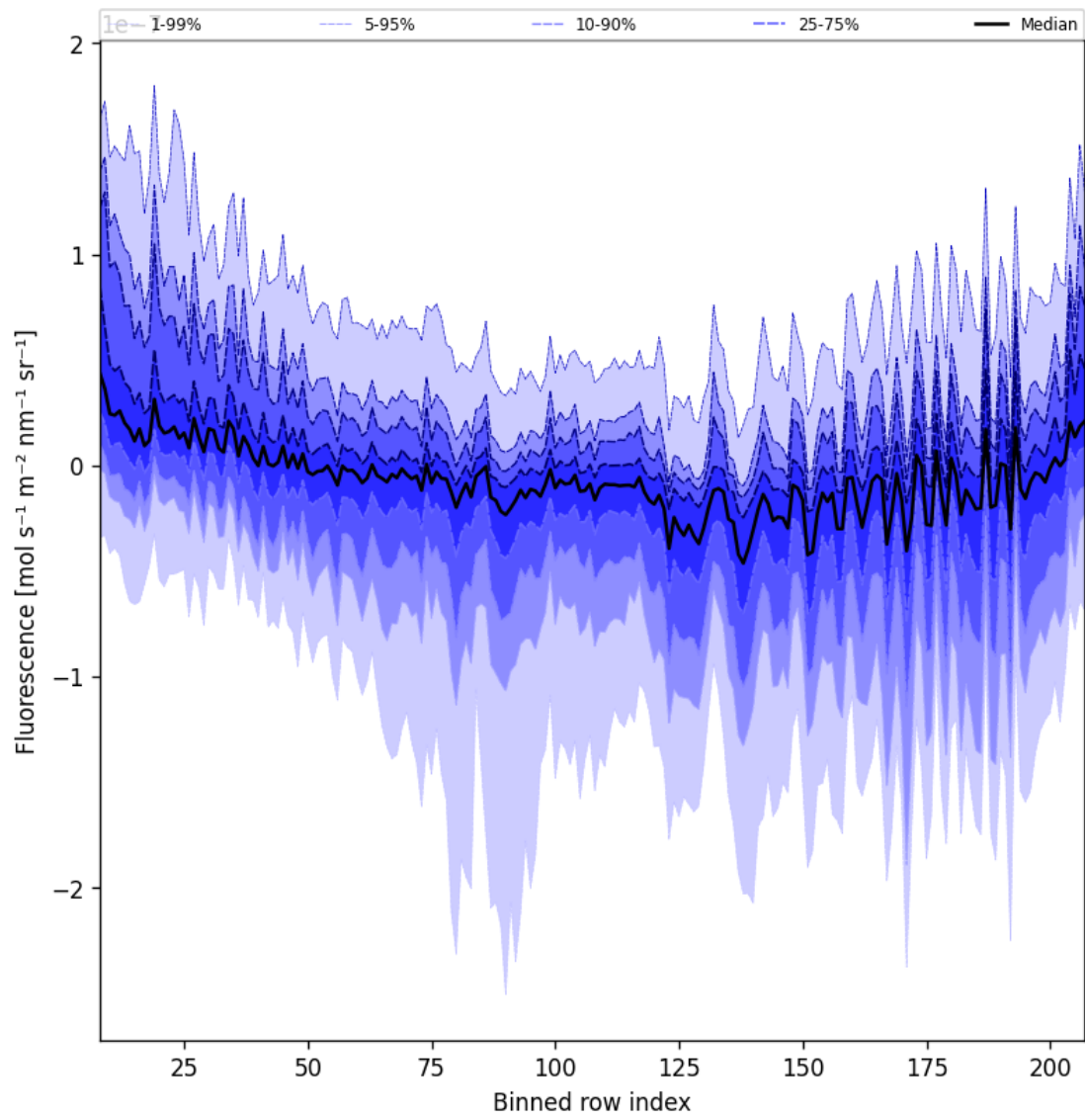
Figure 43: Along track statistics of “Fluorescence” for 2025-05-10 to 2025-05-12
