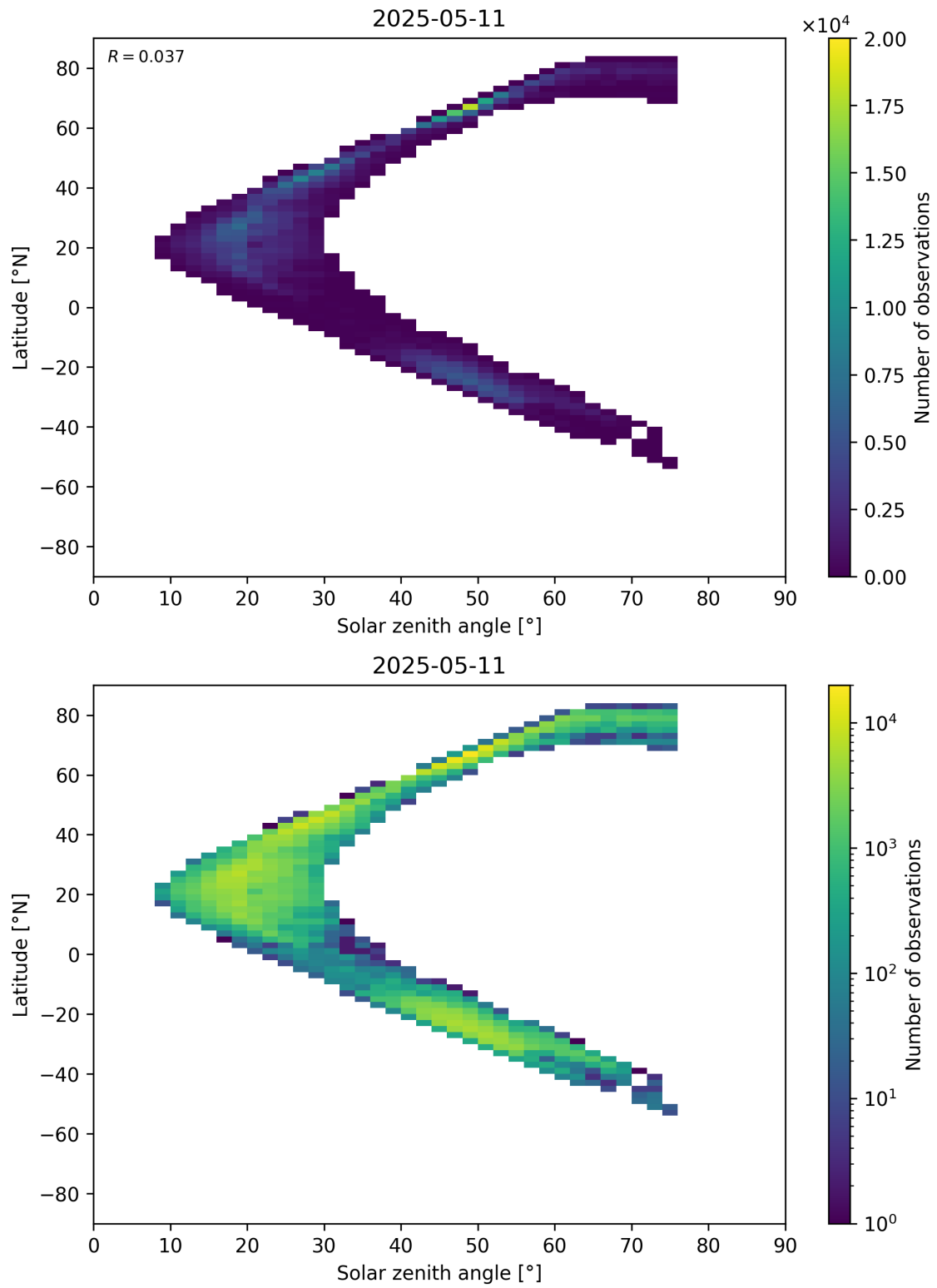
Figure 98: Scatter density plot of “Solar zenith angle” against “Latitude” for 2025-05-10 to 2025-05-12.
