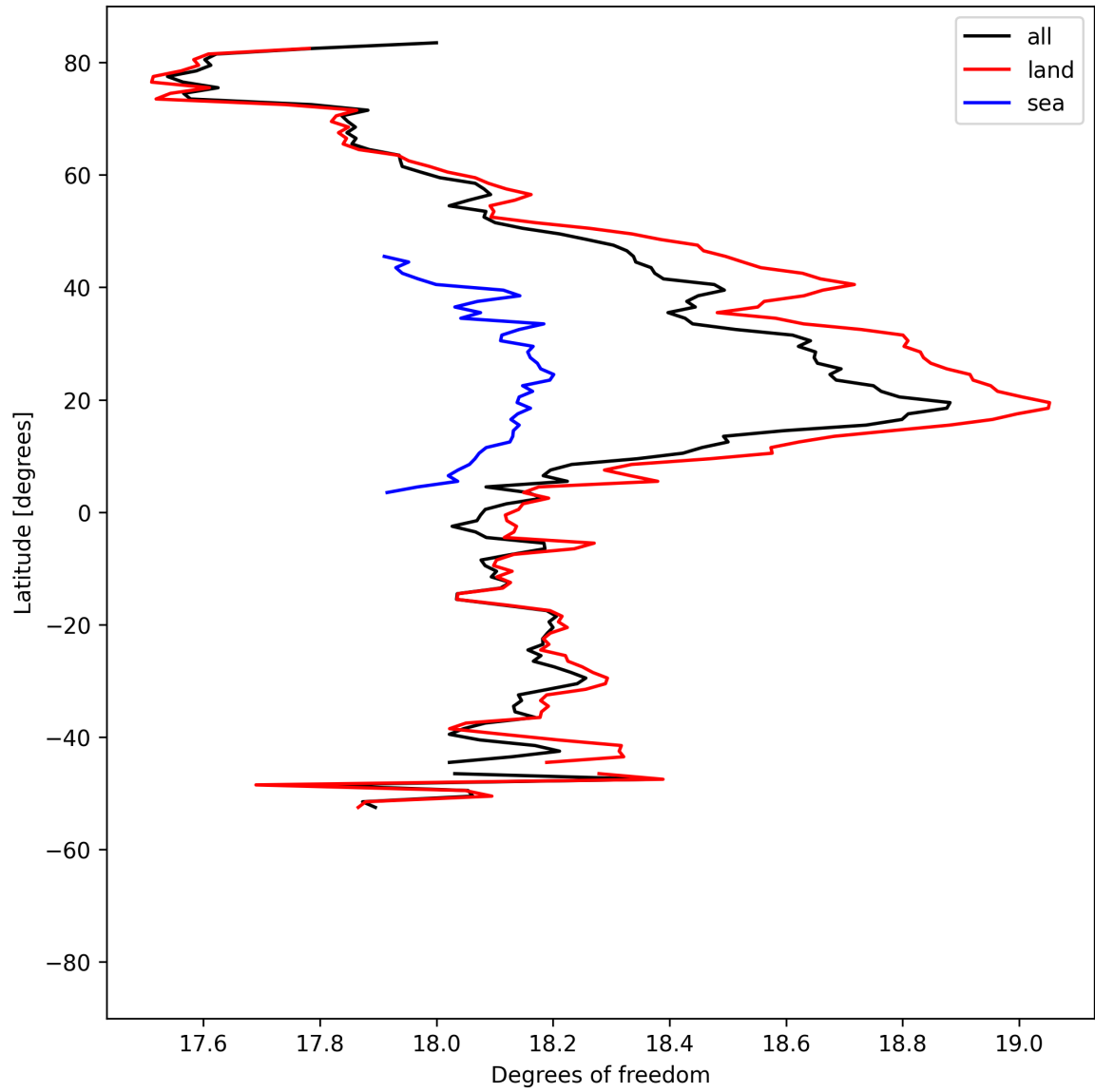
Figure 19: Zonal average of “Degrees of freedom” for 2025-05-10 to 2025-05-12.
