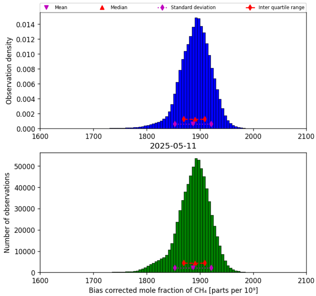
Figure 25: Histogram of “Bias corrected mole fraction of CH 4 ” for 2025-05-10 to 2025-05-12
