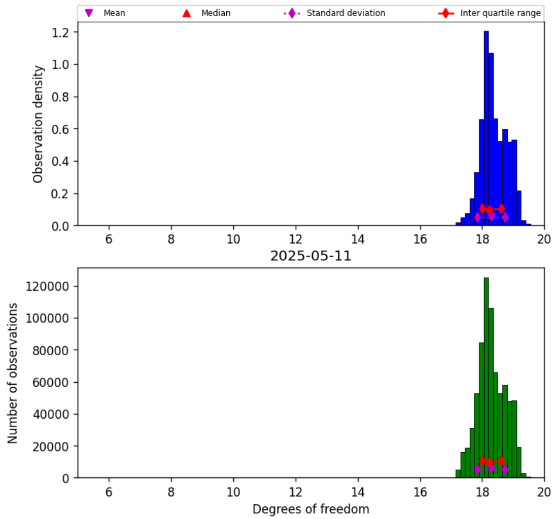
Figure 30: Histogram of “Degrees of freedom” for 2025-05-10 to 2025-05-12
