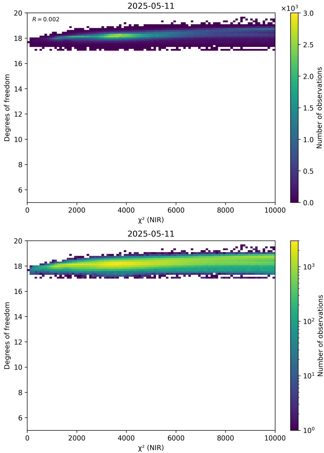
Figure 44: Scatter density plot of “ \chi^2 (NIR)” against “Degrees of freedom” for 2025-05-10 to 2025-05-12.
