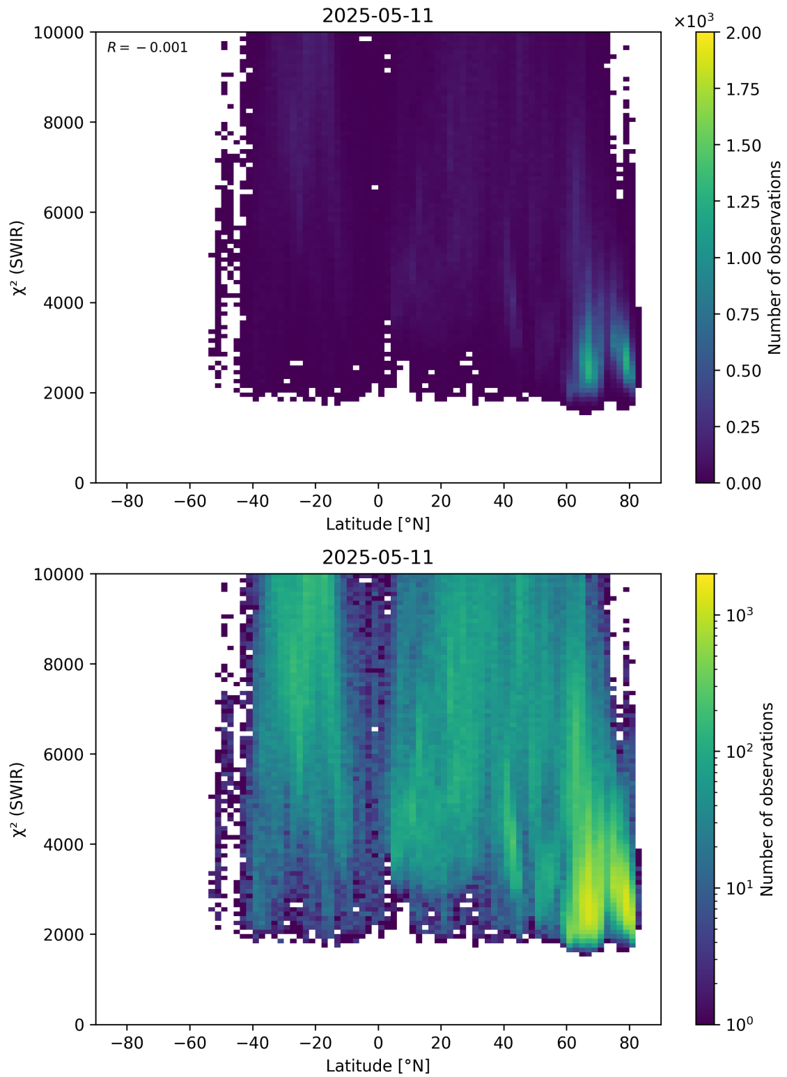
Figure 54: Scatter density plot of “Latitude” against “ \chi^2 (SWIR)” for 2025-05-10 to 2025-05-12.
