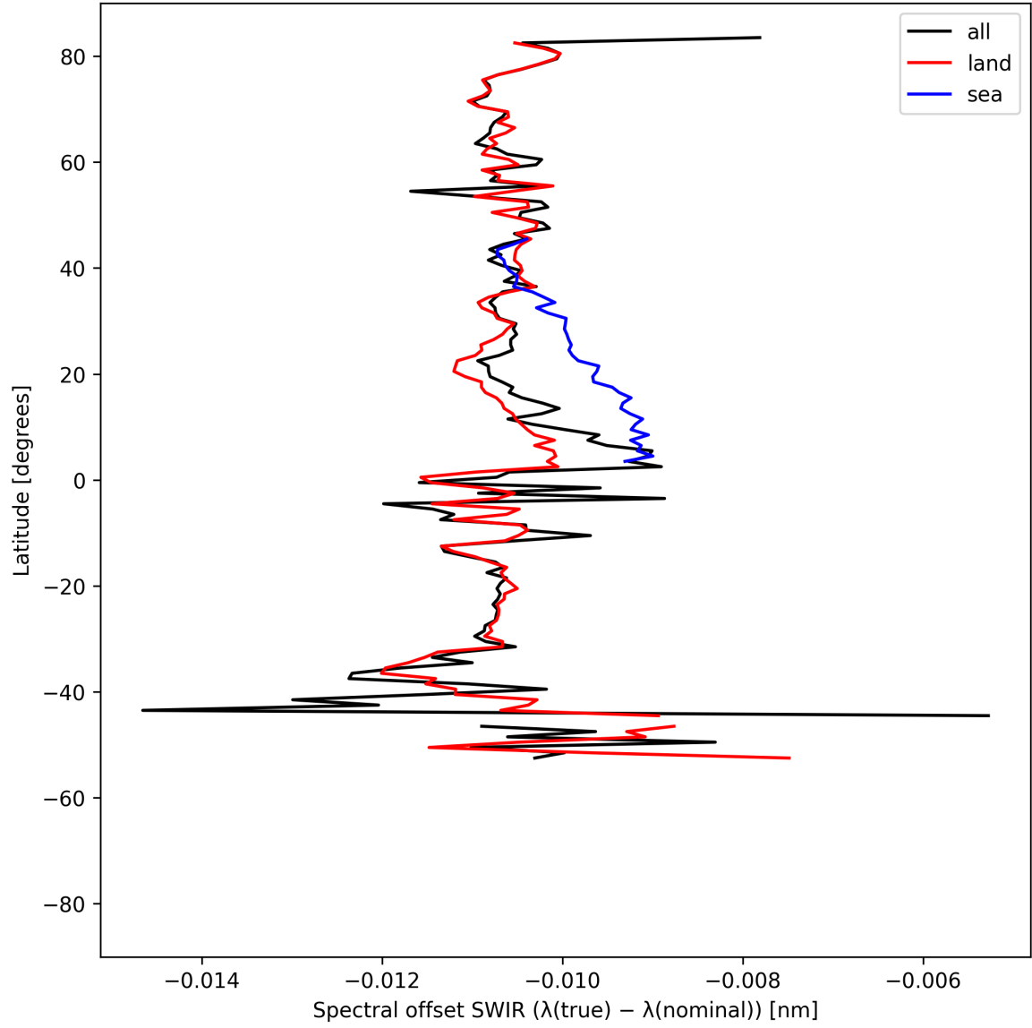
Figure 16: Zonal average of “Spectral offset SWIR ( \lambda_{\text{true}} - \lambda_{\text{nominal}} )” for 2025-05-10 to 2025-05-12.
