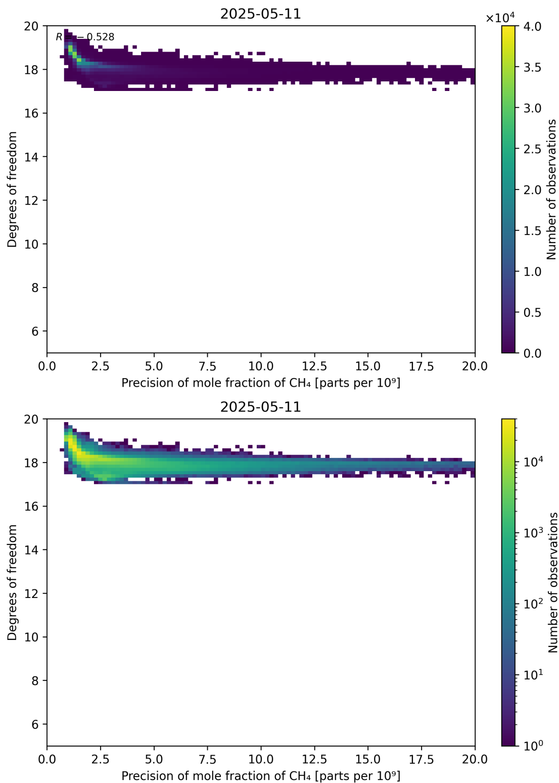
Figure 80: Scatter density plot of “Precision of mole fraction of CH 4 ” against “Degrees of freedom” for 2025-05-10 to 2025-05-12.
