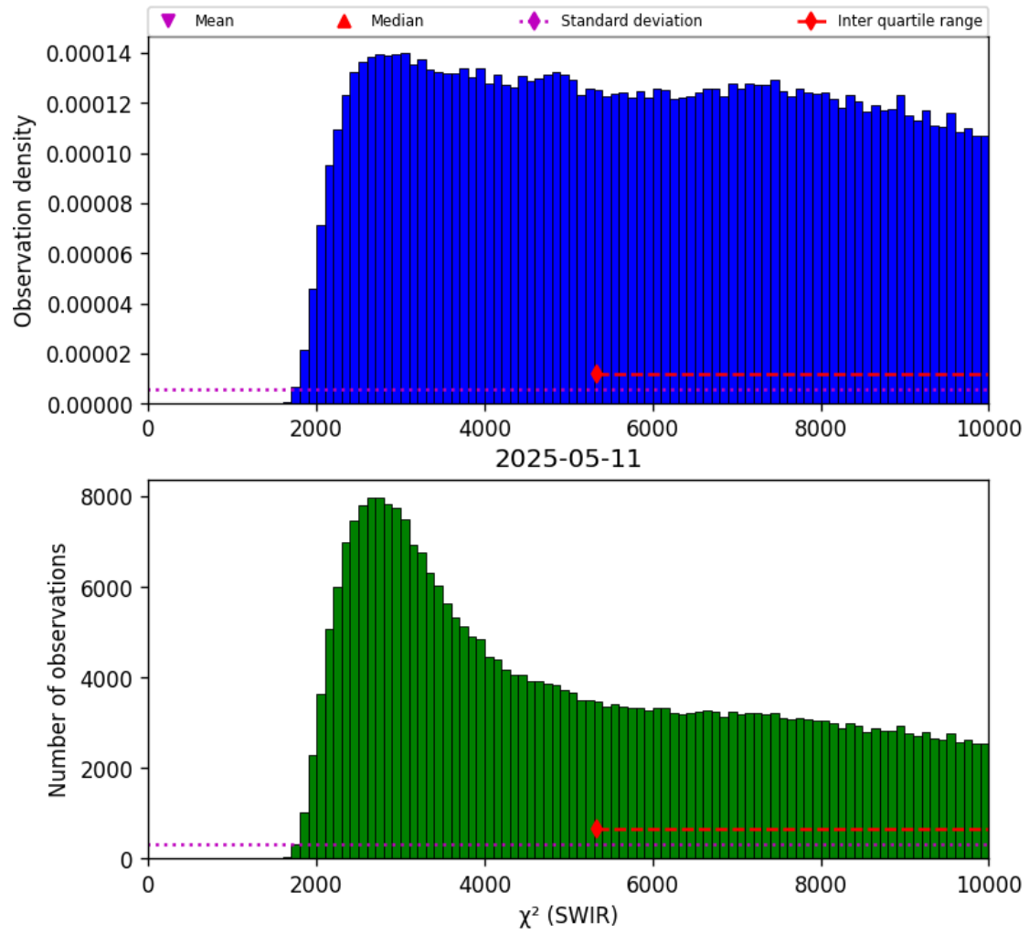
Figure 28: Histogram of “ \chi^2 (SWIR)” for 2025-05-10 to 2025-05-12
