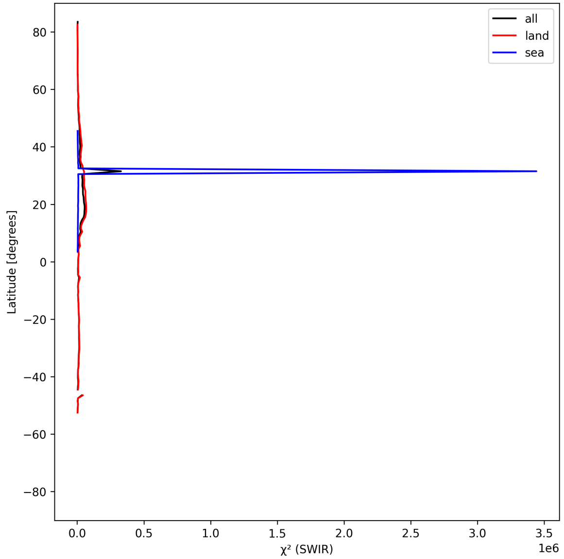
Figure 17: Zonal average of “ \chi^2 (SWIR)” for 2025-05-10 to 2025-05-12.
