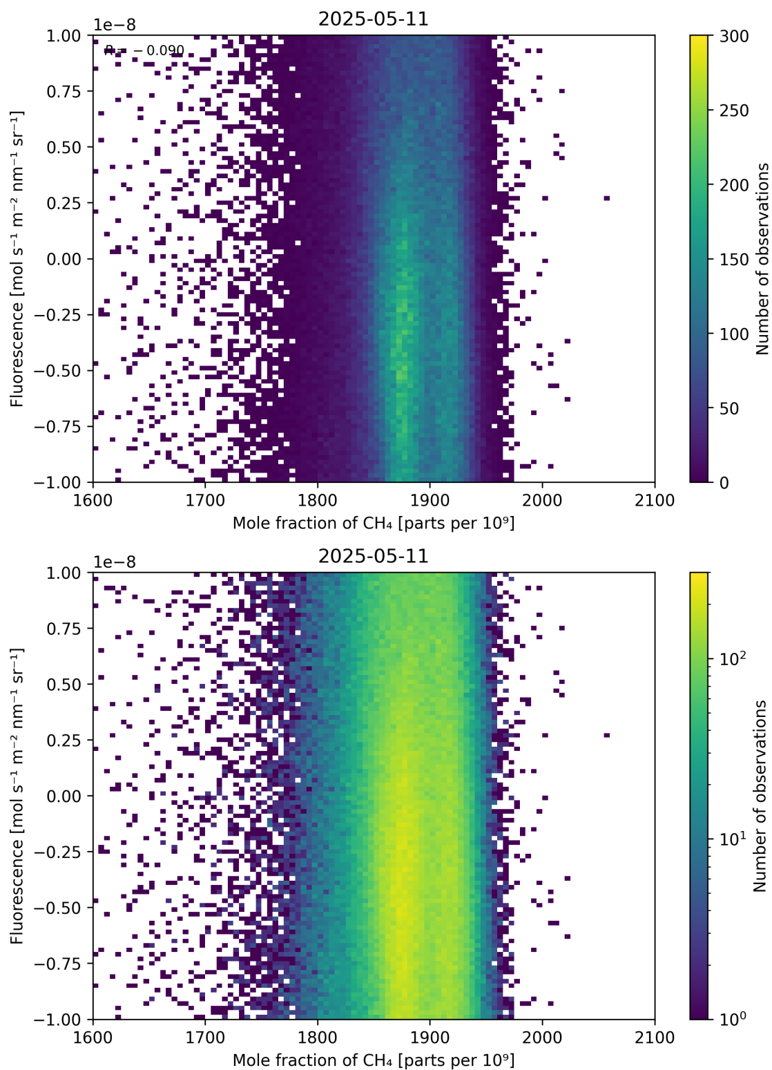
Figure 73: Scatter density plot of “Mole fraction of CH 4 ” against “Fluorescence” for 2025-05-10 to 2025-05-12.
