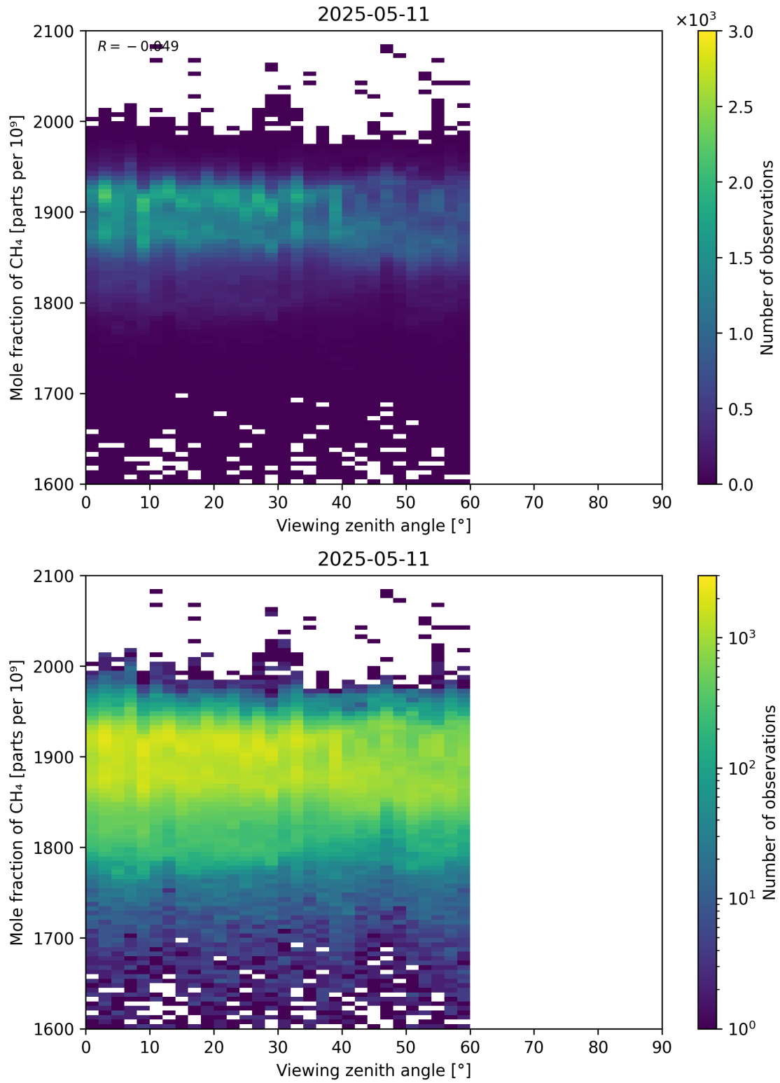
Figure 110: Scatter density plot of “Viewing zenith angle” against “Mole fraction of CH 4 ” for 2025-05-10 to 2025-05-12.
