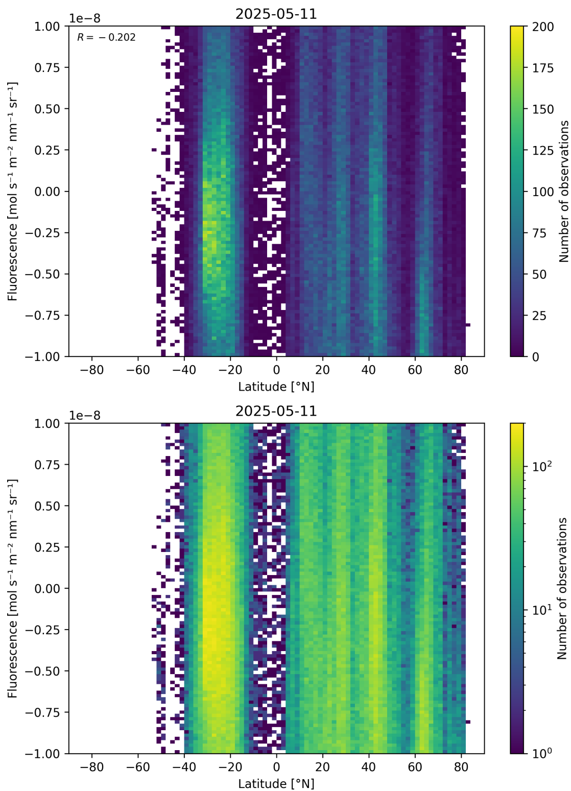
Figure 56: Scatter density plot of “Latitude” against “Fluorescence” for 2025-05-10 to 2025-05-12.
