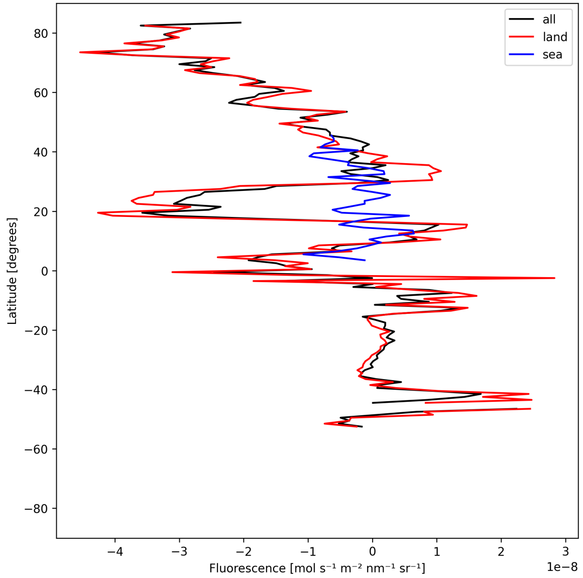
Figure 21: Zonal average of “Fluorescence” for 2025-05-10 to 2025-05-12.
