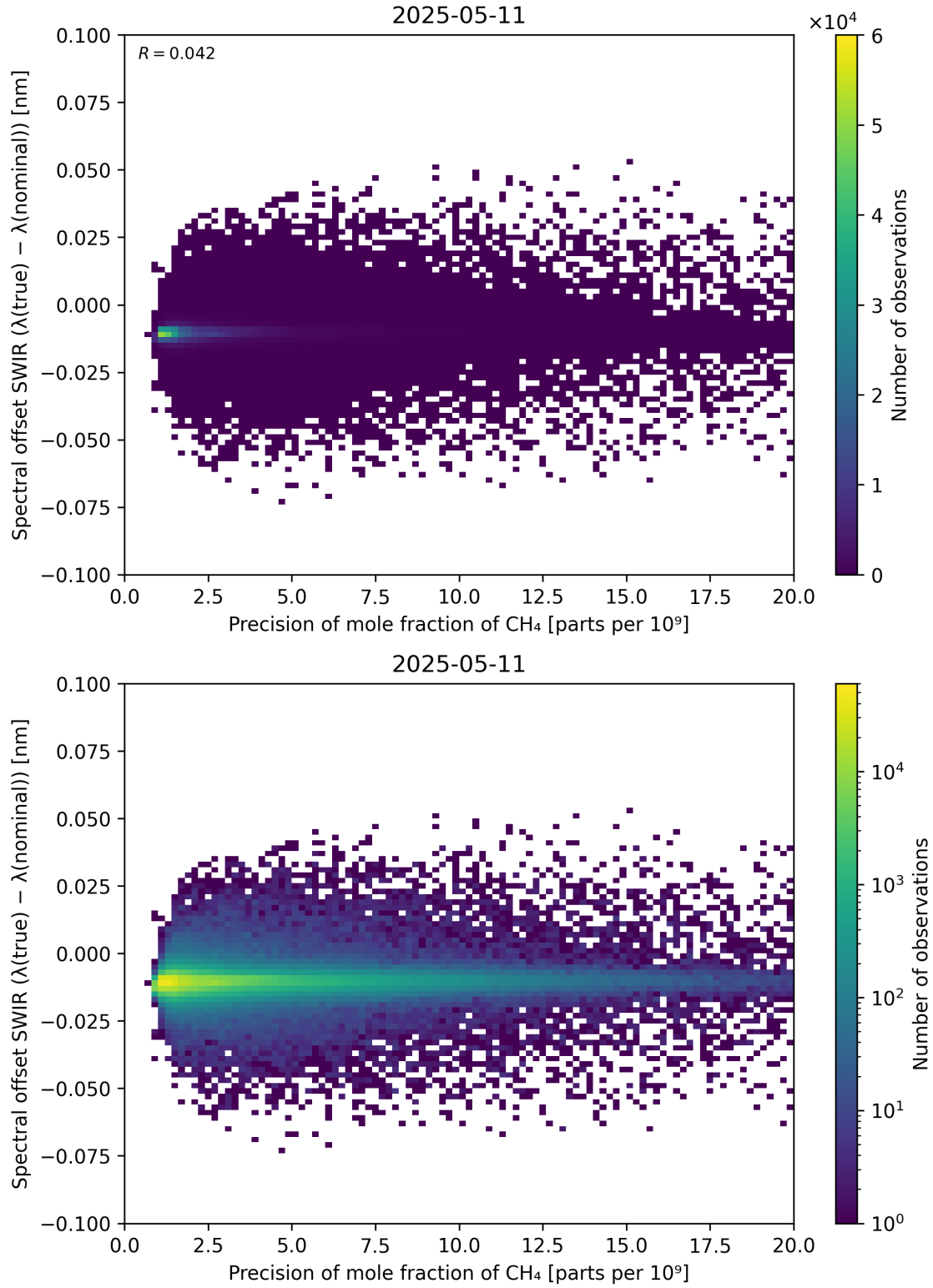
Figure 85: Scatter density plot of “Precision of mole fraction of \text{CH}_4 ” against “Spectral offset SWIR ( \lambda_{\text{true}} - \lambda_{\text{nominal}} )” for 2025-05-10 to 2025-05-12.
