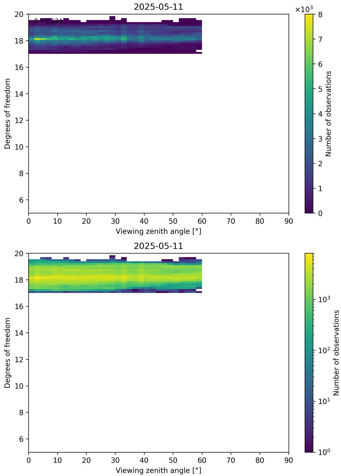
Figure 107: Scatter density plot of “Viewing zenith angle” against “Degrees of freedom” for 2025-05-10 to 2025-05-12.
