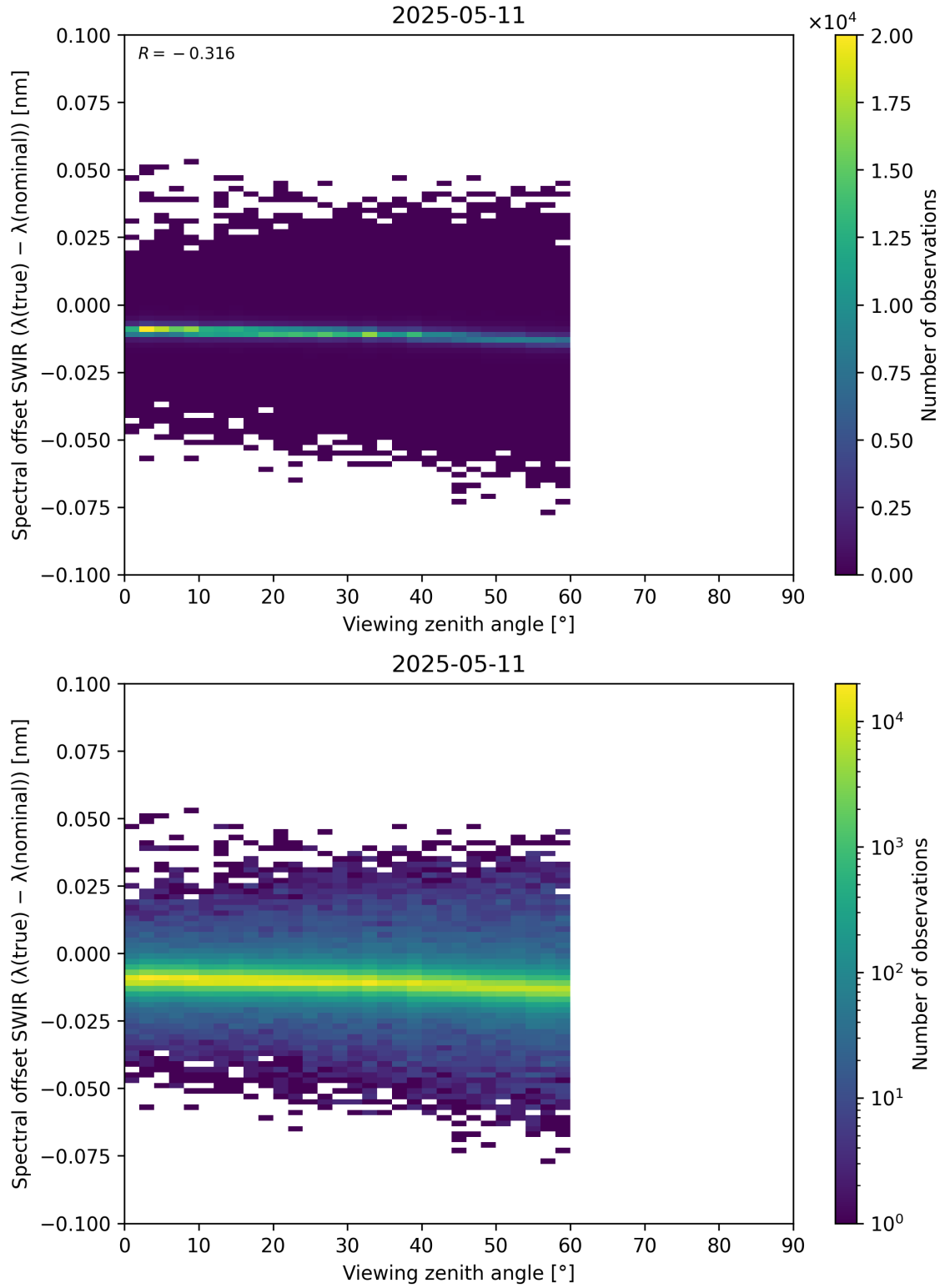
Figure 116: Scatter density plot of “Viewing zenith angle” against “Spectral offset SWIR ( \lambda_{\text{true}} - \lambda_{\text{nominal}} )” for 2025-05-10 to 2025-05-12.
