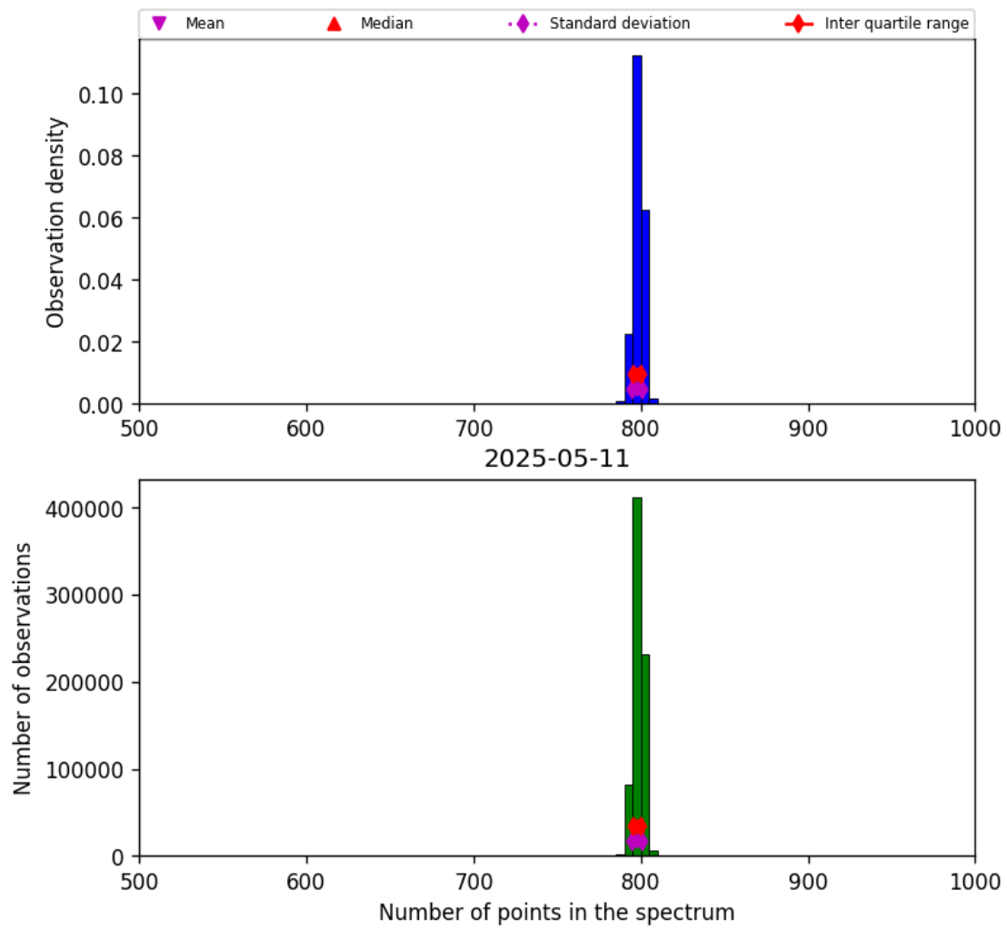
Figure 26: Histogram of “Number of points in the spectrum” for 2025-05-10 to 2025-05-12
