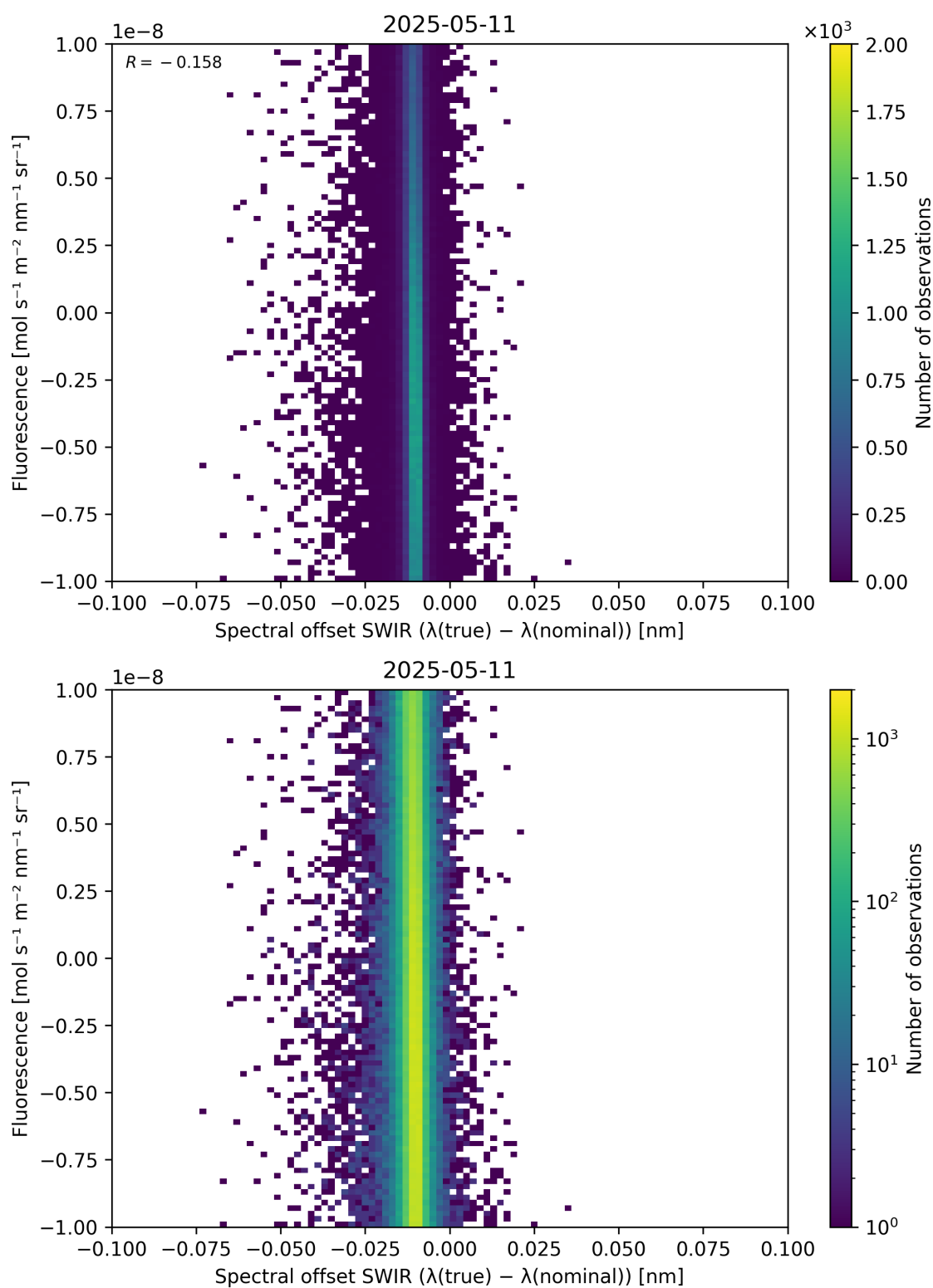
Figure 120: Scatter density plot of “Spectral offset SWIR ( \lambda_{\text{true}} - \lambda_{\text{nominal}} )” against “Fluorescence” for 2025-05-10 to 2025-05-12.
