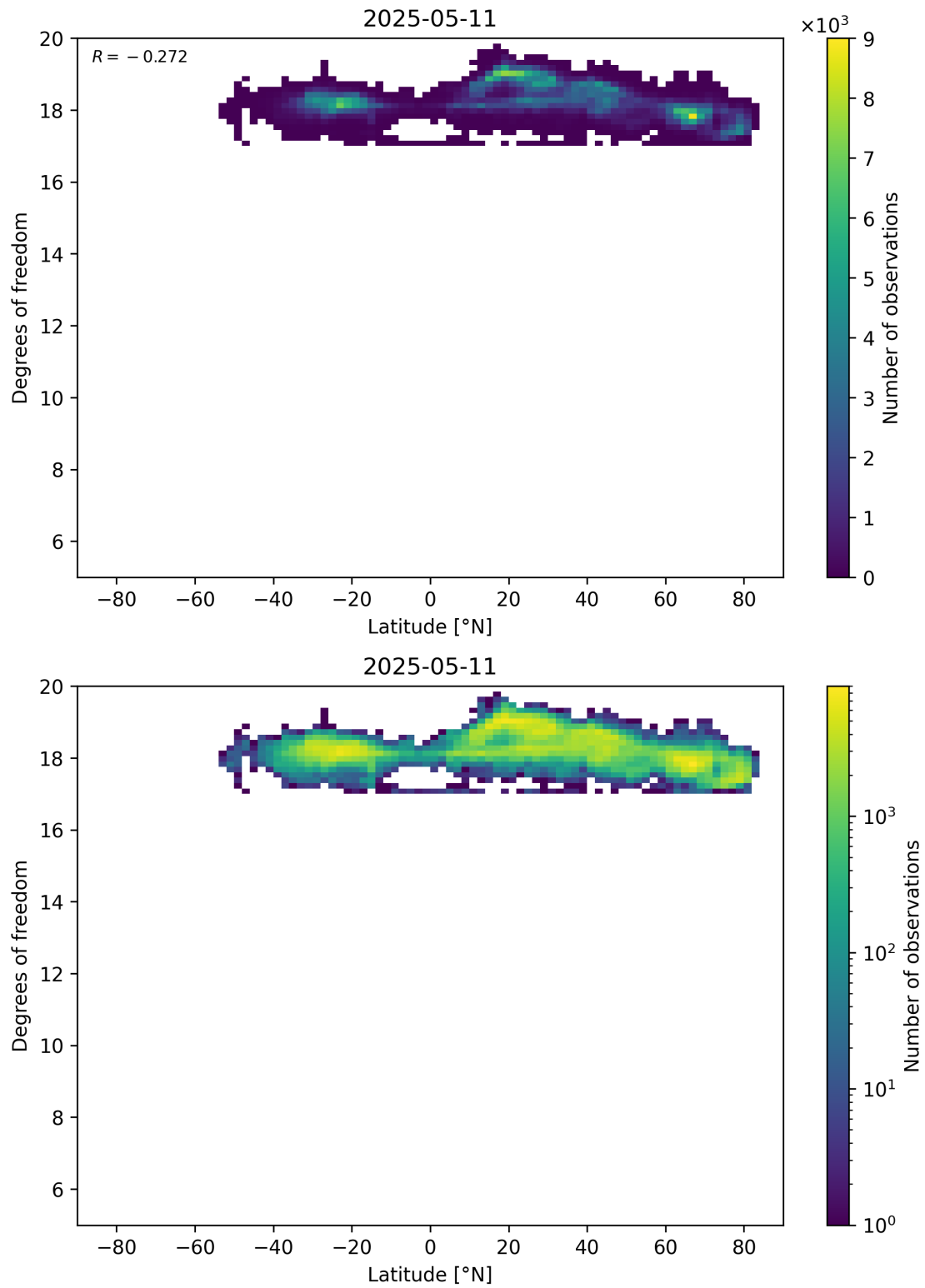
Figure 55: Scatter density plot of “Latitude” against “Degrees of freedom” for 2025-05-10 to 2025-05-12.
