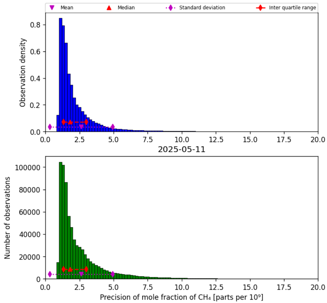
Figure 24: Histogram of “Precision of mole fraction of CH 4 ” for 2025-05-10 to 2025-05-12
