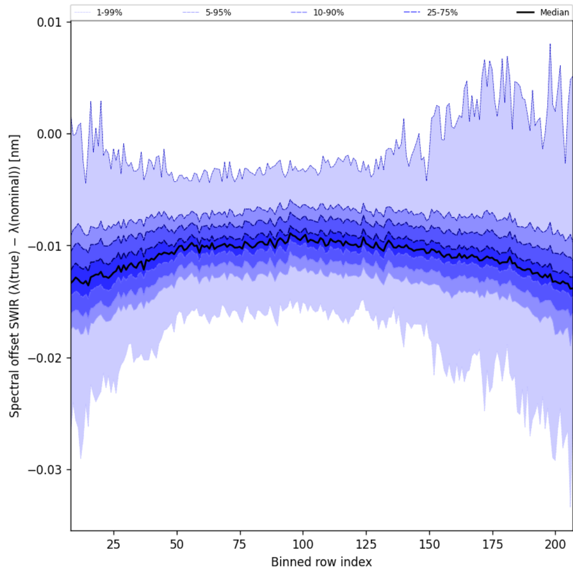
Figure 38: Along track statistics of “Spectral offset SWIR ( \lambda_{\text{true}} - \lambda_{\text{nominal}} )” for 2025-05-10 to 2025-05-12
