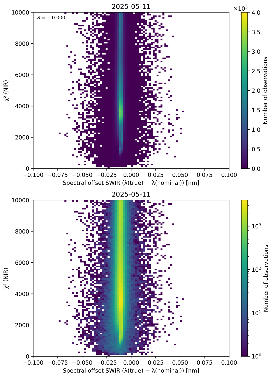
Figure 117: Scatter density plot of “Spectral offset SWIR ( \lambda_{\text{true}} - \lambda_{\text{nominal}} )” against “ \chi^2 (NIR)” for 2025-05-10 to 2025-05-12.
