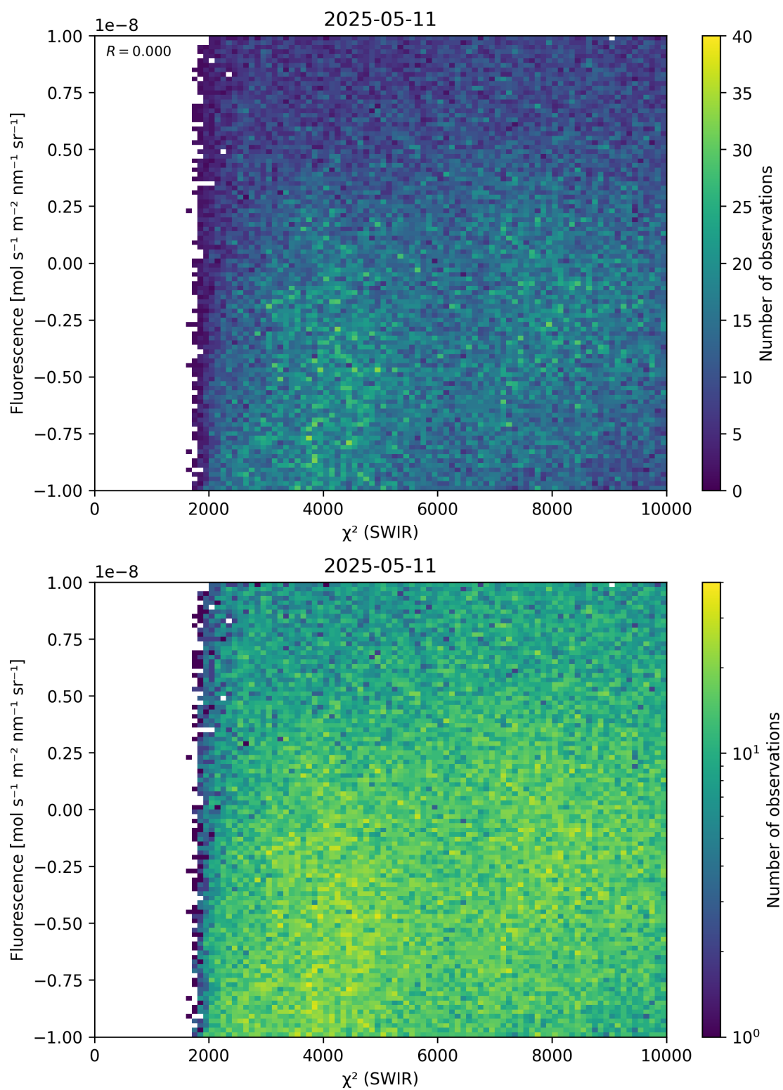
Figure 49: Scatter density plot of “ \chi^2 (SWIR)” against “Fluorescence” for 2025-05-10 to 2025-05-12.
