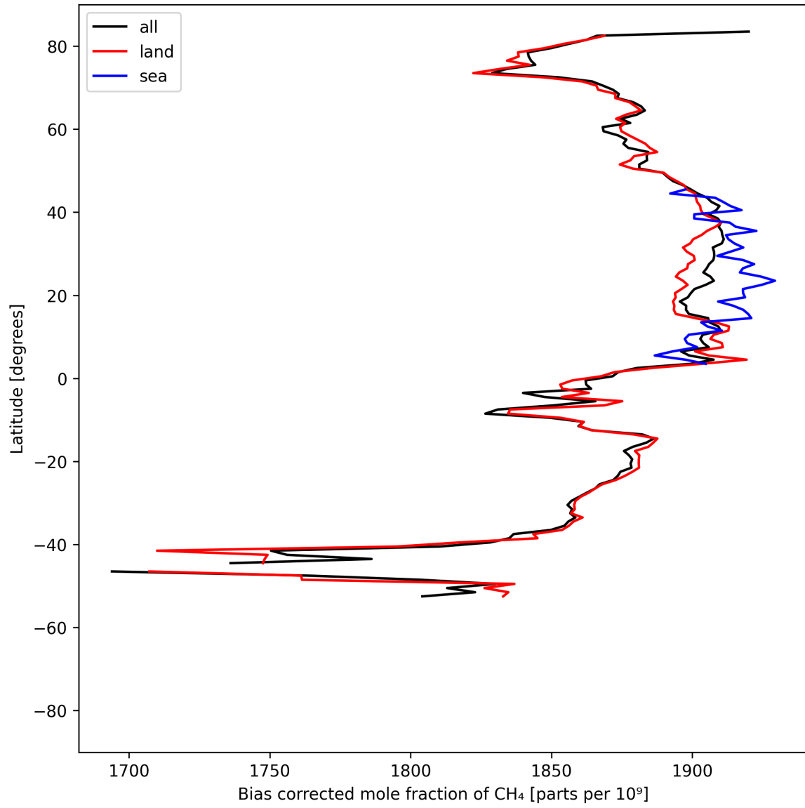
Figure 14: Zonal average of “Bias corrected mole fraction of \text{CH}_4 ” for 2025-05-10 to 2025-05-12.
