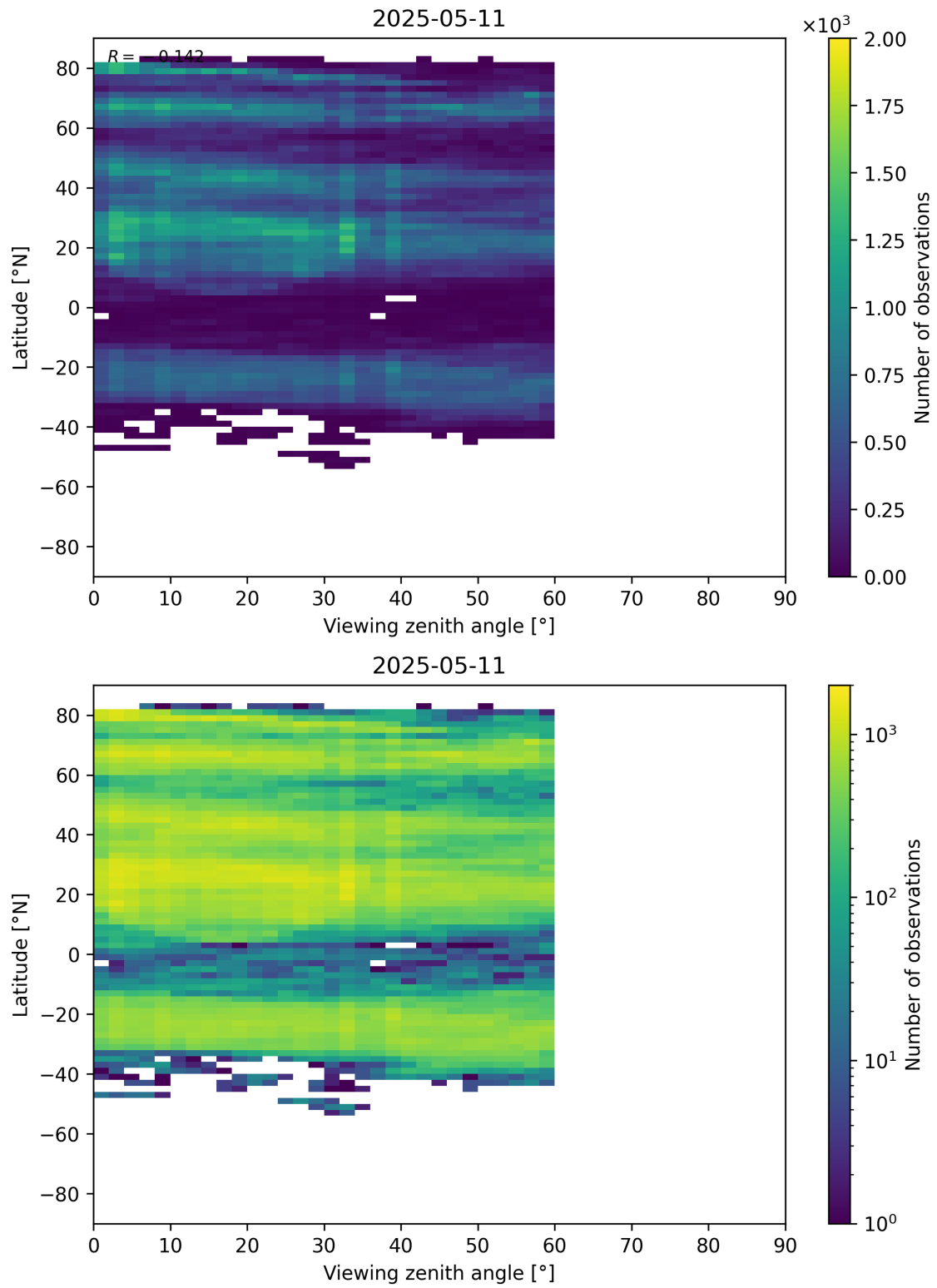
Figure 109: Scatter density plot of “Viewing zenith angle” against “Latitude” for 2025-05-10 to 2025-05-12.
