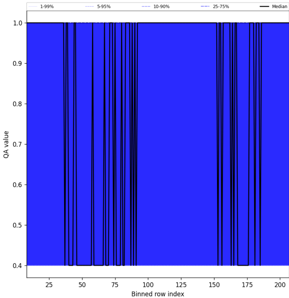
Figure 33: Along track statistics of “QA value” for 2025-05-10 to 2025-05-12
