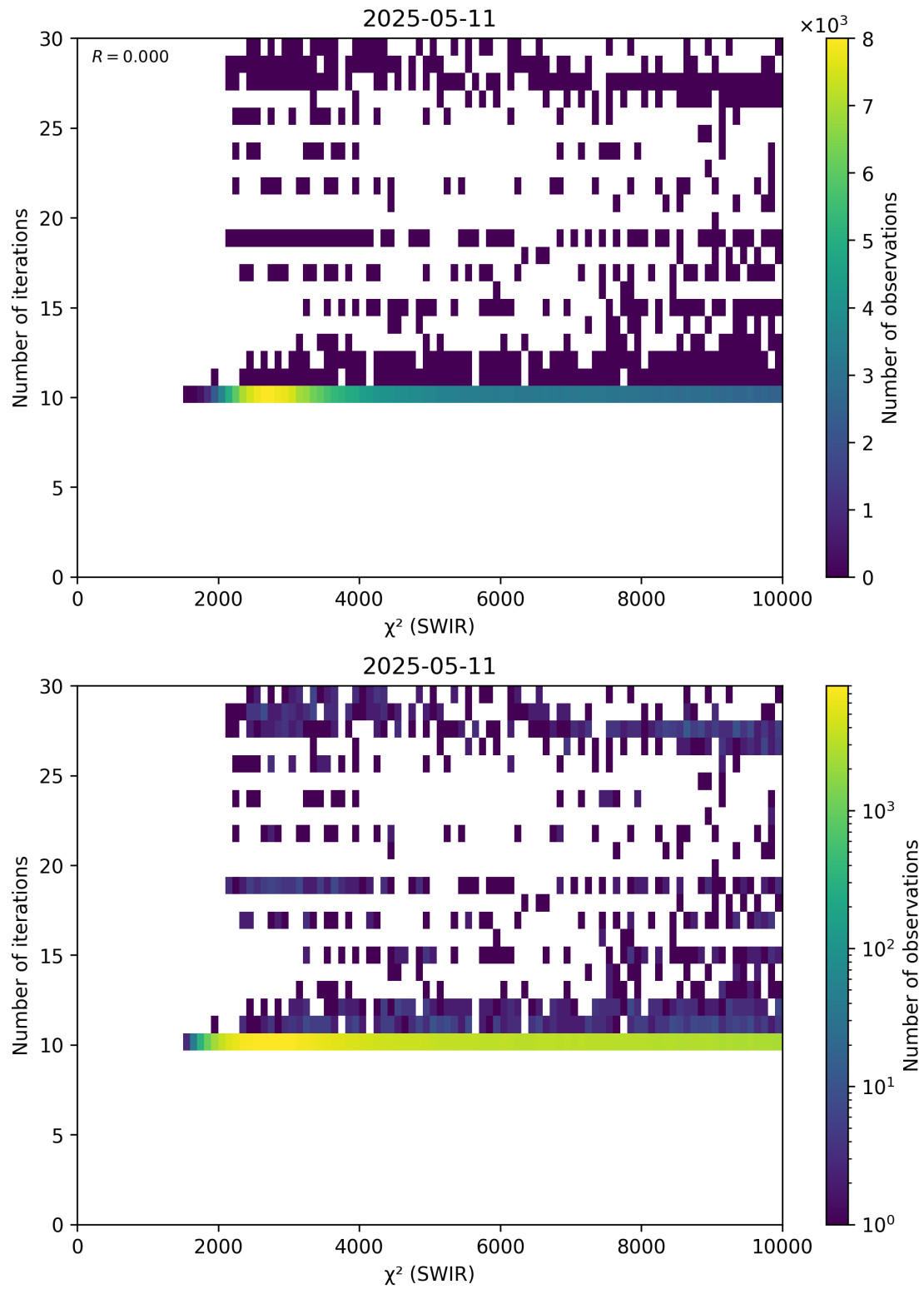
Figure 50: Scatter density plot of “ \chi^2 (SWIR)” against “Number of iterations” for 2025-05-10 to 2025-05-12.
