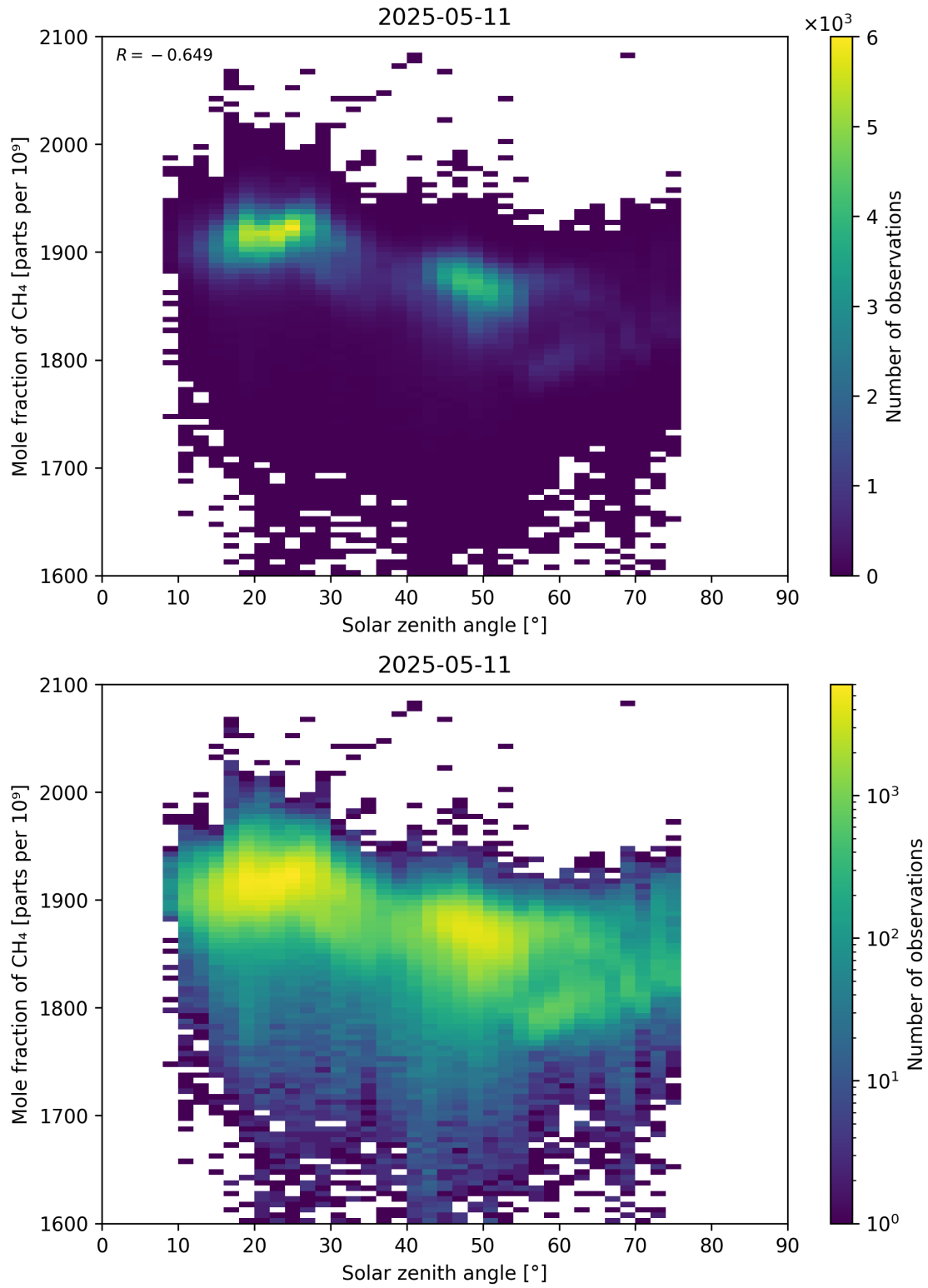
Figure 99: Scatter density plot of “Solar zenith angle” against “Mole fraction of CH 4 ” for 2025-05-10 to 2025-05-12.
