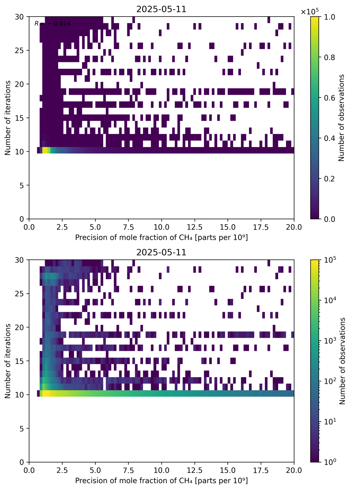
Figure 83: Scatter density plot of “Precision of mole fraction of CH 4 ” against “Number of iterations” for 2025-05-10 to 2025-05-12.
