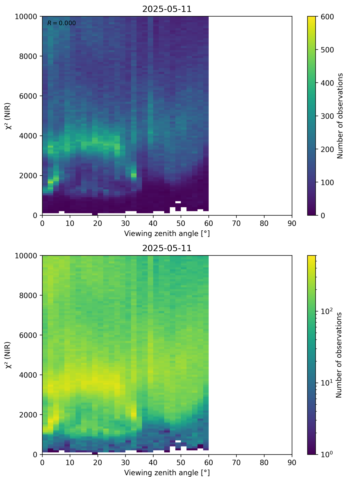
Figure 105: Scatter density plot of “Viewing zenith angle” against “ \chi^2 (NIR)” for 2025-05-10 to 2025-05-12.
