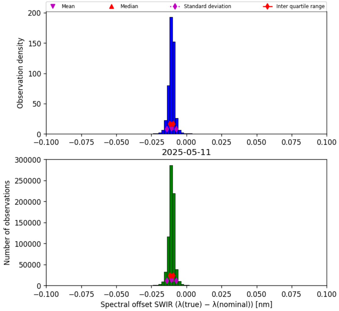
Figure 27: Histogram of “Spectral offset SWIR ( \lambda_{\text{true}} - \lambda_{\text{nominal}} )” for 2025-05-10 to 2025-05-12
