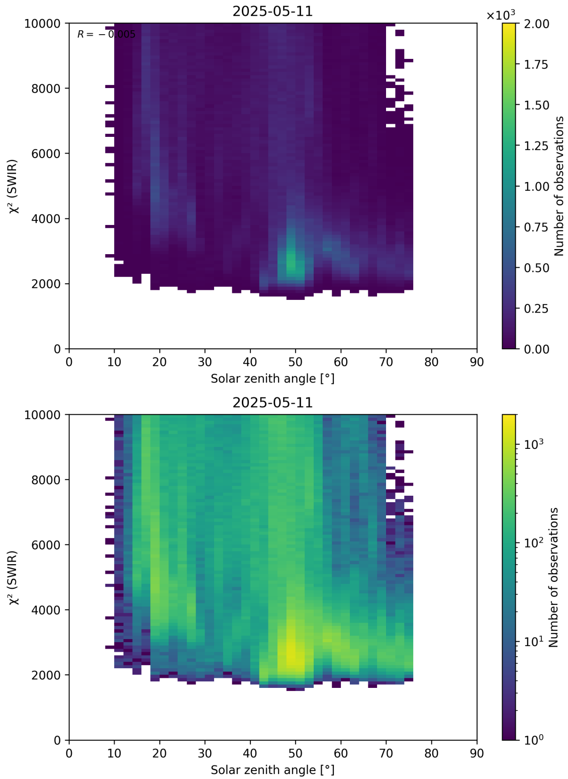
Figure 95: Scatter density plot of “Solar zenith angle” against “ \chi^2 (SWIR)” for 2025-05-10 to 2025-05-12.
