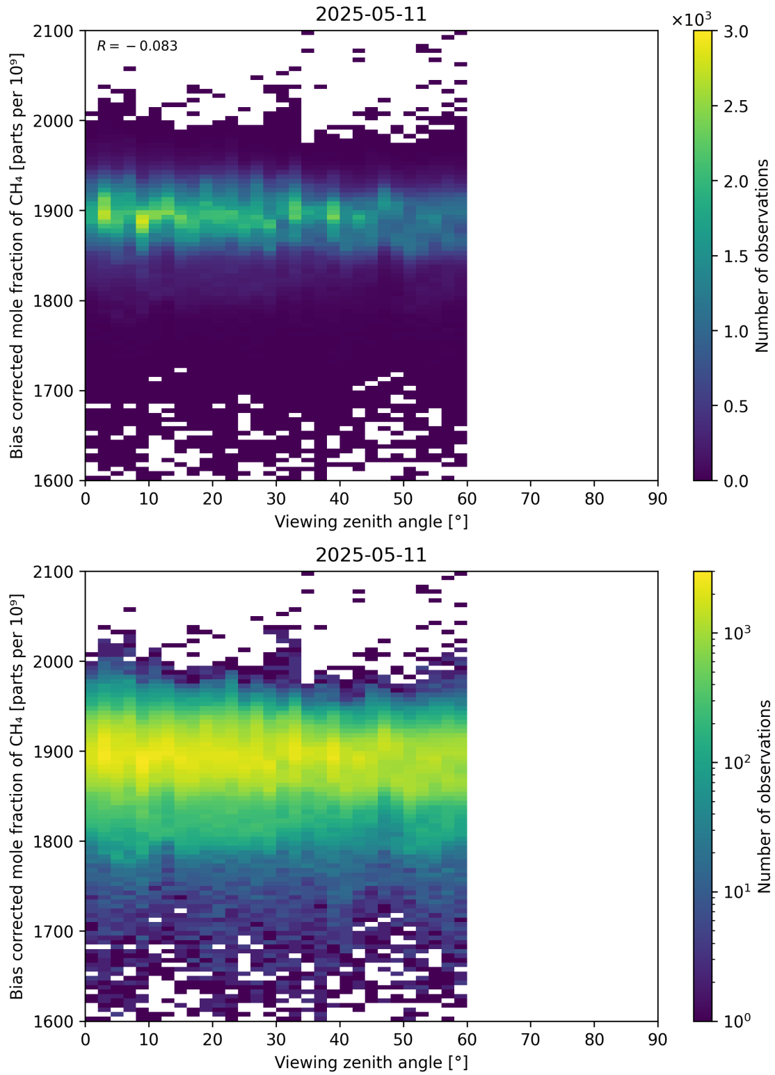
Figure 111: Scatter density plot of “Viewing zenith angle” against “Bias corrected mole fraction of CH 4 ” for 2025-05-10 to 2025-05-12.
