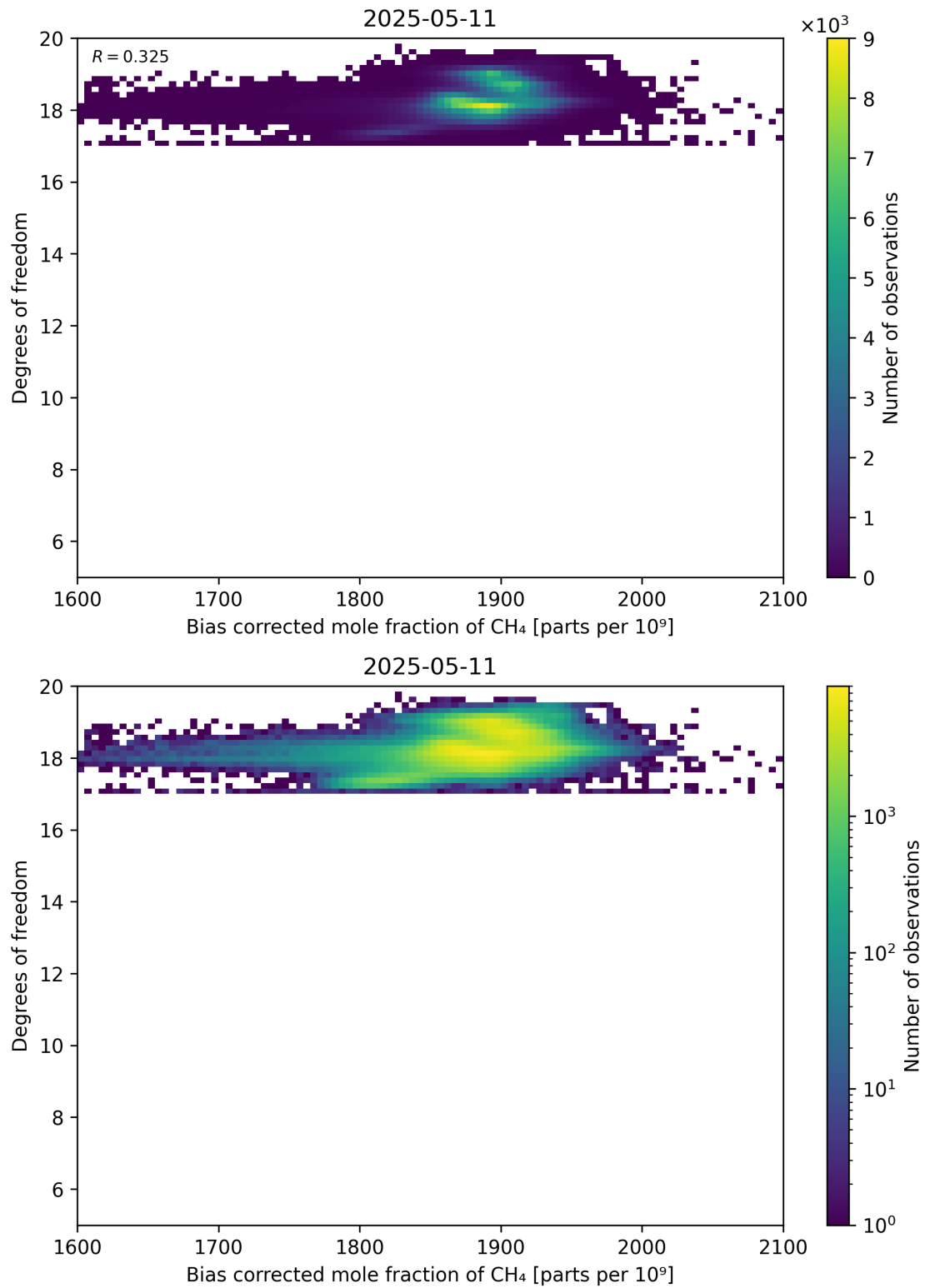
Figure 65: Scatter density plot of “Bias corrected mole fraction of CH 4 ” against “Degrees of freedom” for 2025-05-10 to 2025-05-12.
