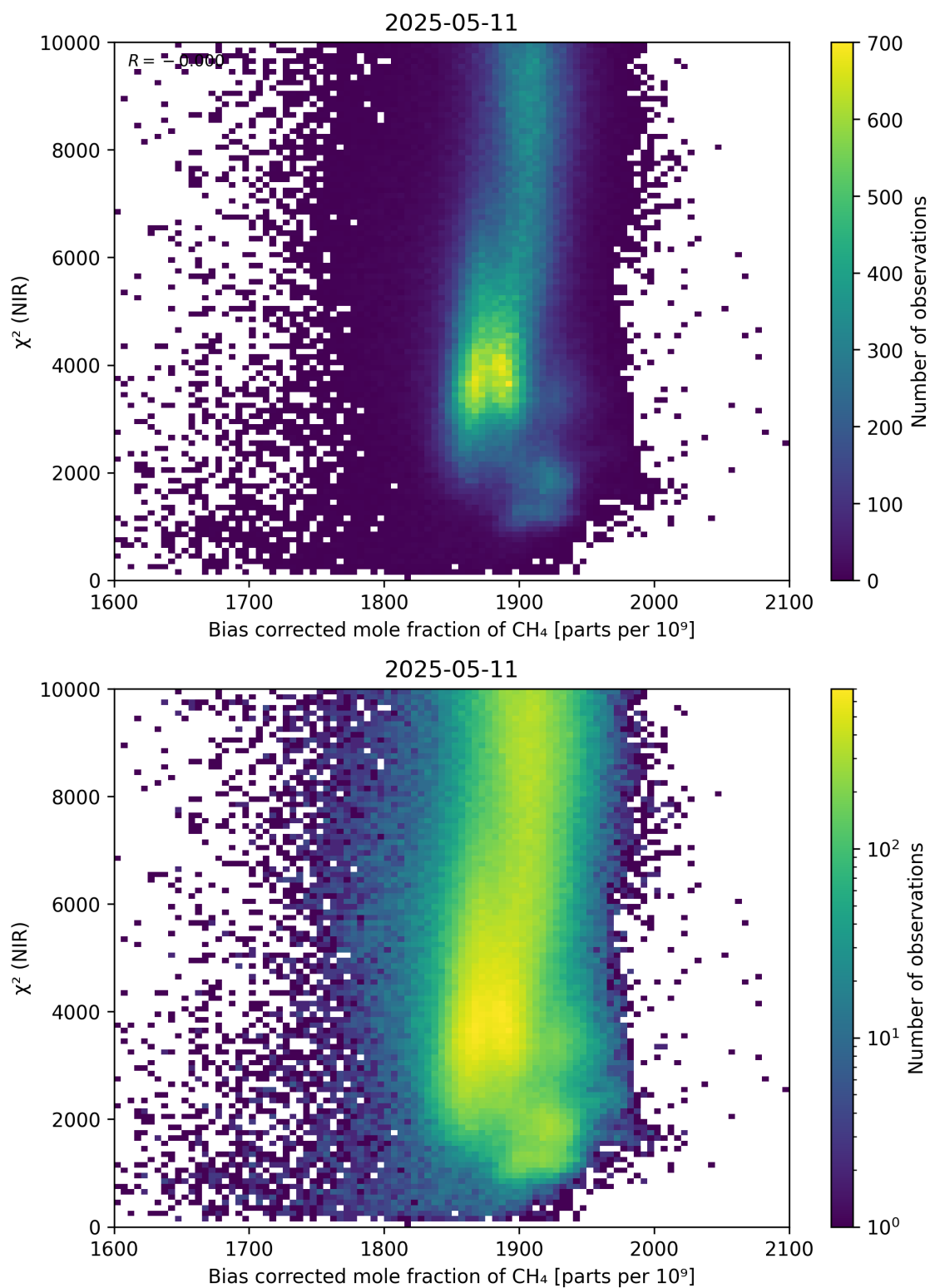
Figure 63: Scatter density plot of “Bias corrected mole fraction of \text{CH}_4 ” against “ \chi^2 (NIR)” for 2025-05-10 to 2025-05-12.
