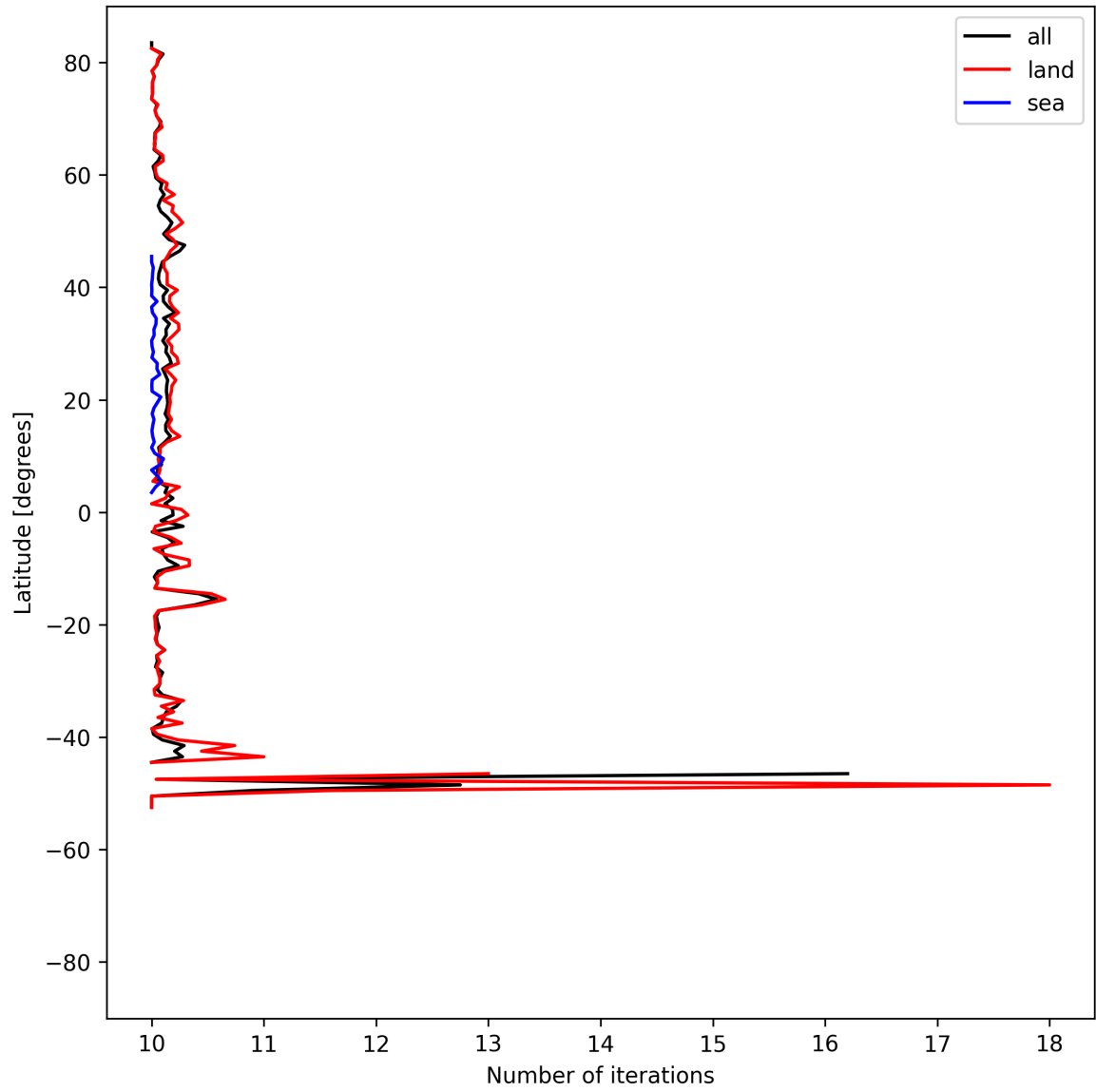
Figure 20: Zonal average of “Number of iterations” for 2025-05-10 to 2025-05-12.
