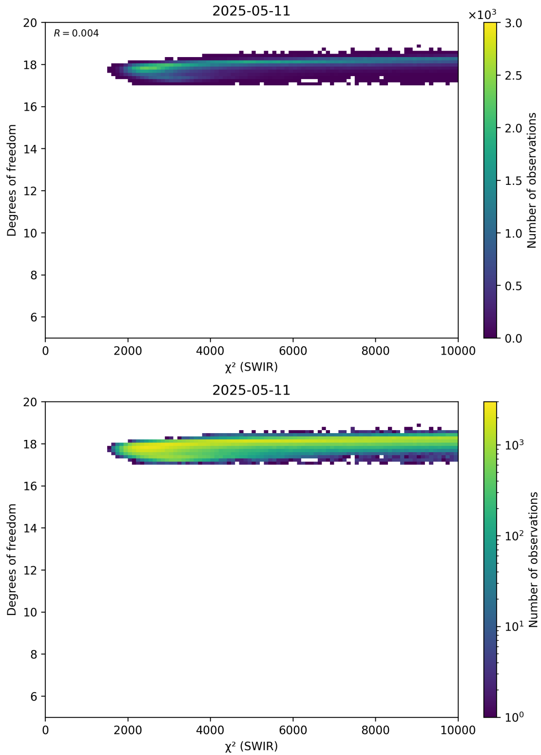
Figure 48: Scatter density plot of “ \chi^2 (SWIR)” against “Degrees of freedom” for 2025-05-10 to 2025-05-12.
