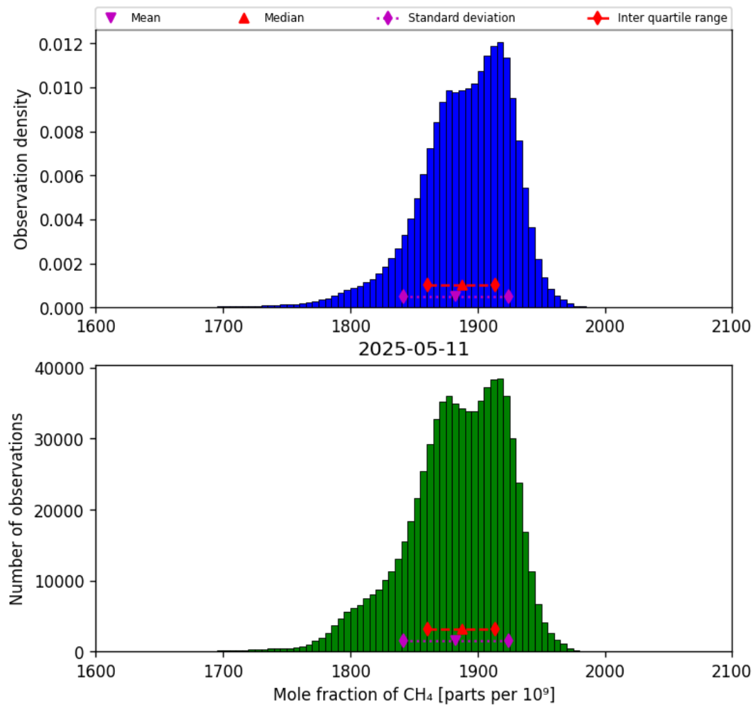
Figure 23: Histogram of “Mole fraction of CH 4 ” for 2025-05-10 to 2025-05-12
