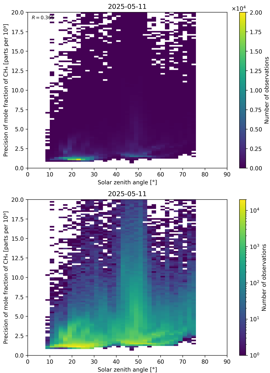
Figure 101: Scatter density plot of “Solar zenith angle” against “Precision of mole fraction of CH 4 ” for 2025-05-10 to 2025-05-12.
