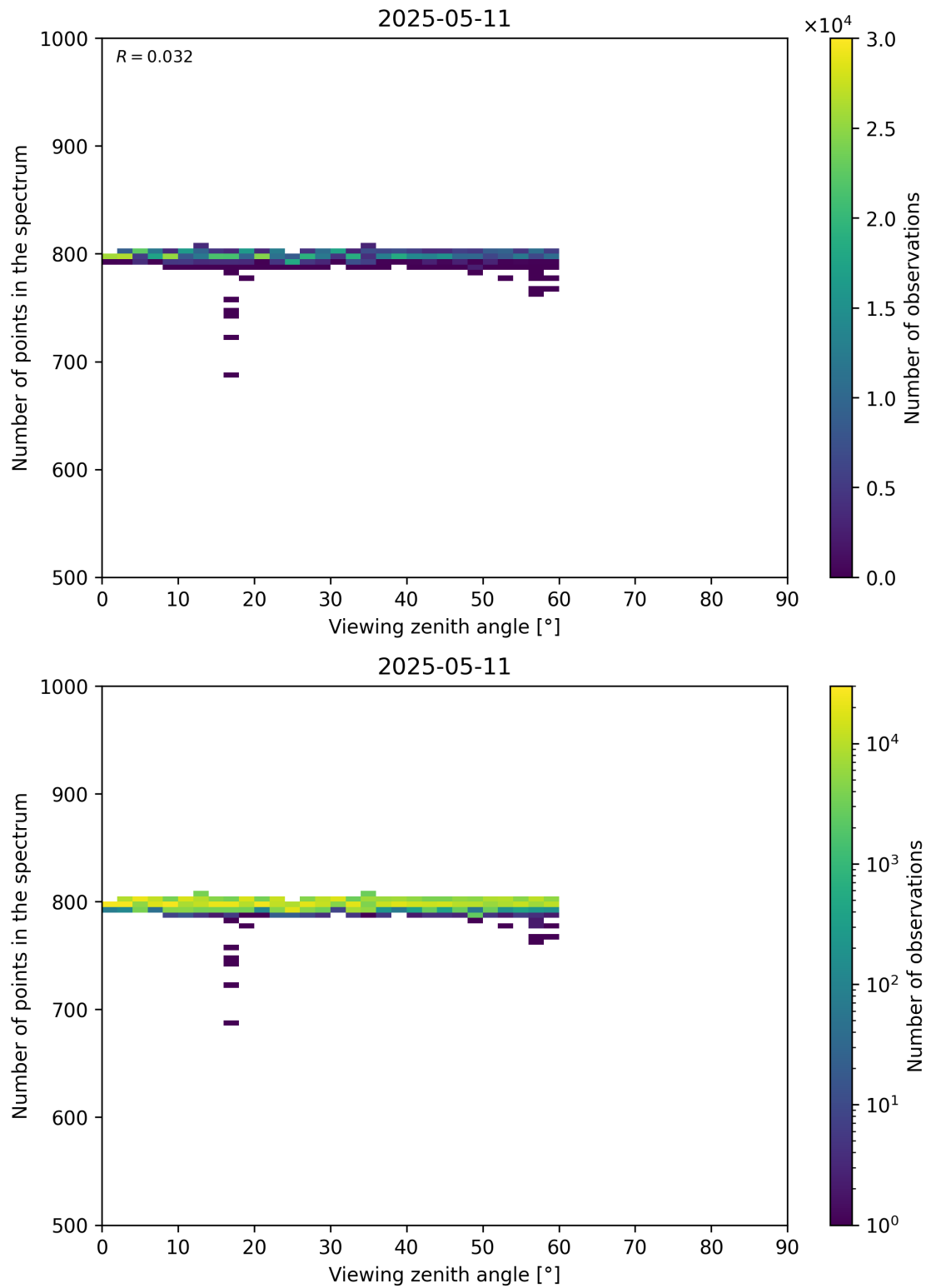
Figure 114: Scatter density plot of “Viewing zenith angle” against “Number of points in the spectrum” for 2025-05-10 to 2025-05-12.
