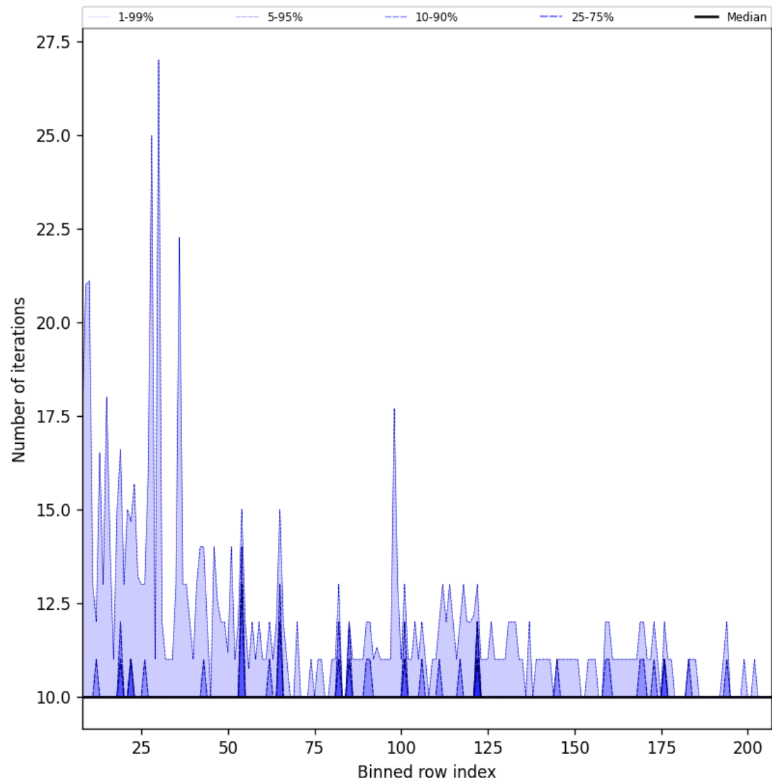
Figure 42: Along track statistics of “Number of iterations” for 2025-05-10 to 2025-05-12
