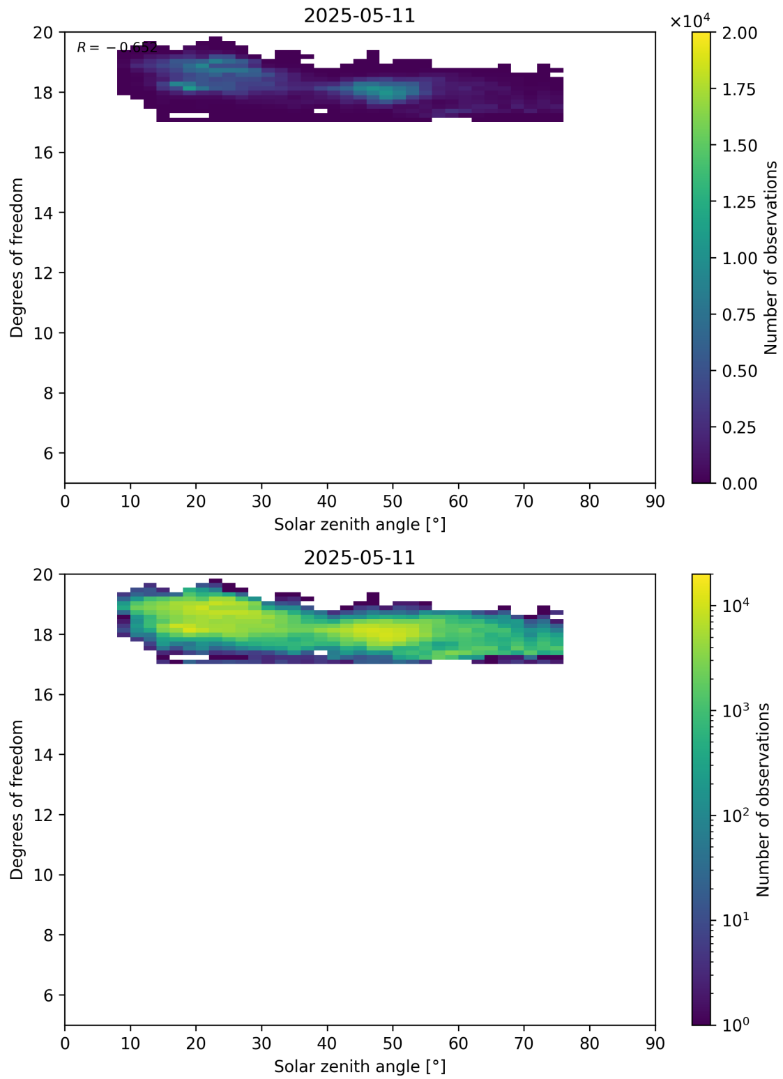
Figure 96: Scatter density plot of “Solar zenith angle” against “Degrees of freedom” for 2025-05-10 to 2025-05-12.
