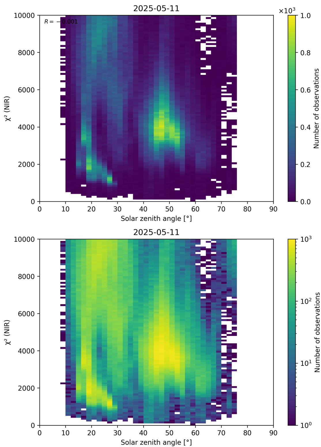
Figure 94: Scatter density plot of “Solar zenith angle” against “ \chi^2 (NIR)” for 2025-05-10 to 2025-05-12.
