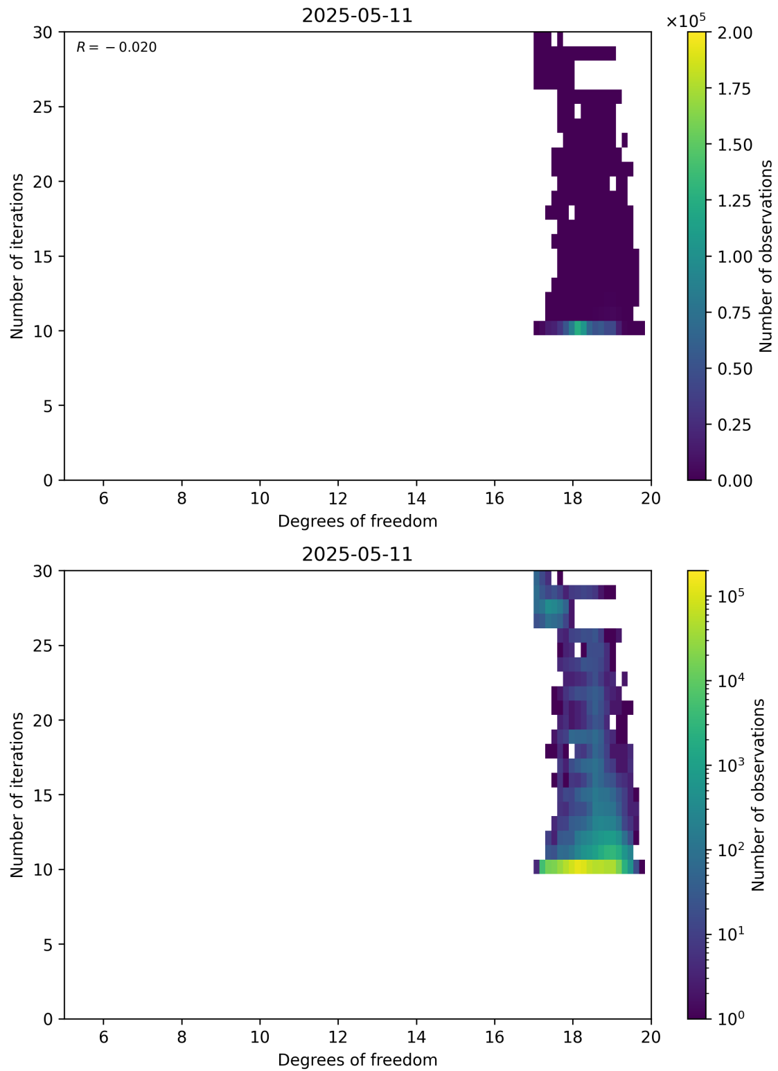
Figure 52: Scatter density plot of “Degrees of freedom” against “Number of iterations” for 2025-05-10 to 2025-05-12.
