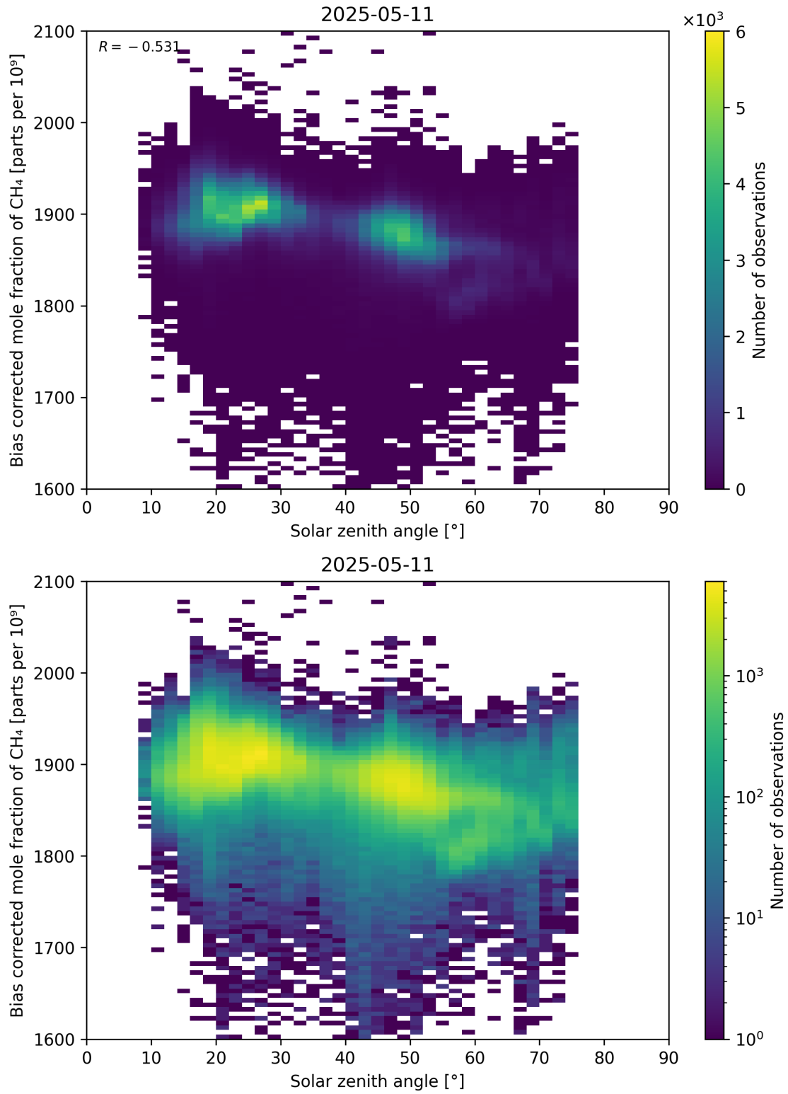
Figure 100: Scatter density plot of “Solar zenith angle” against “Bias corrected mole fraction of CH 4 ” for 2025-05-10 to 2025-05-12.
