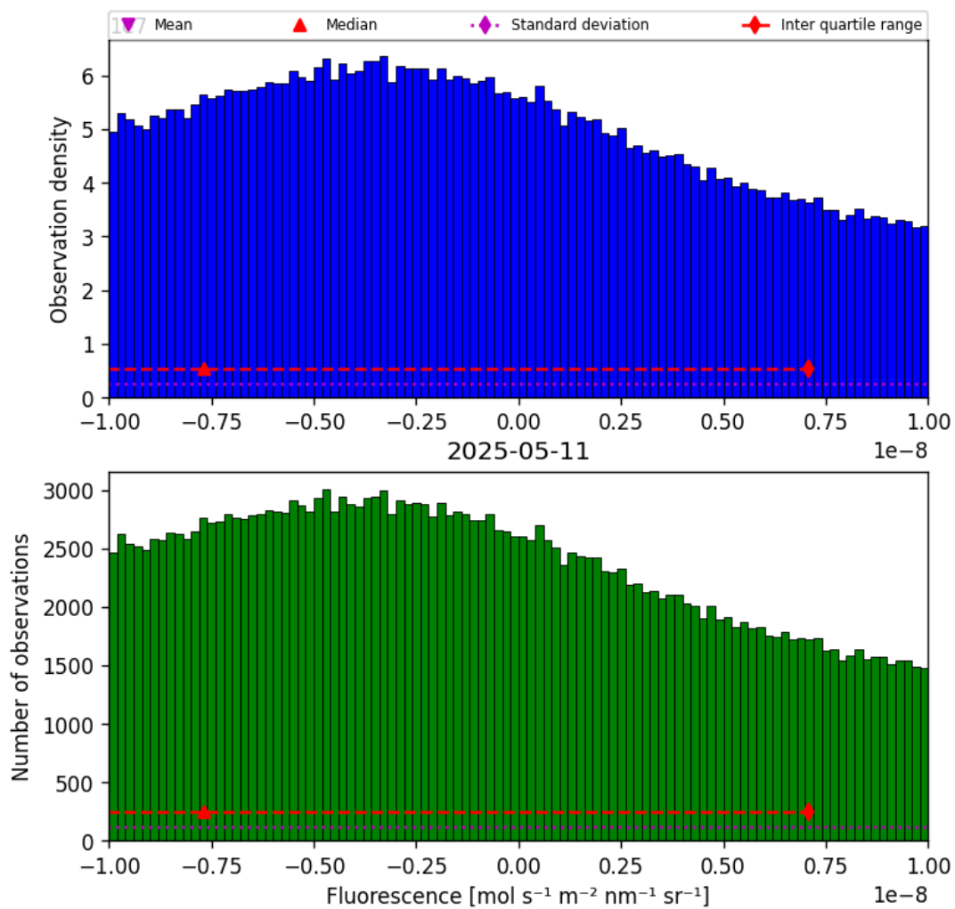
Figure 32: Histogram of “Fluorescence” for 2025-05-10 to 2025-05-12
