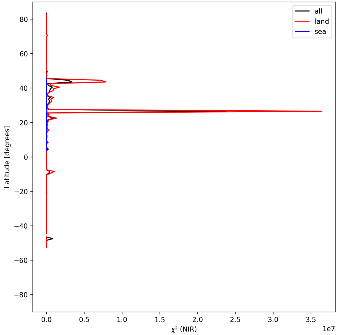
Figure 18: Zonal average of “ \chi^2 (NIR)” for 2025-05-10 to 2025-05-12.
