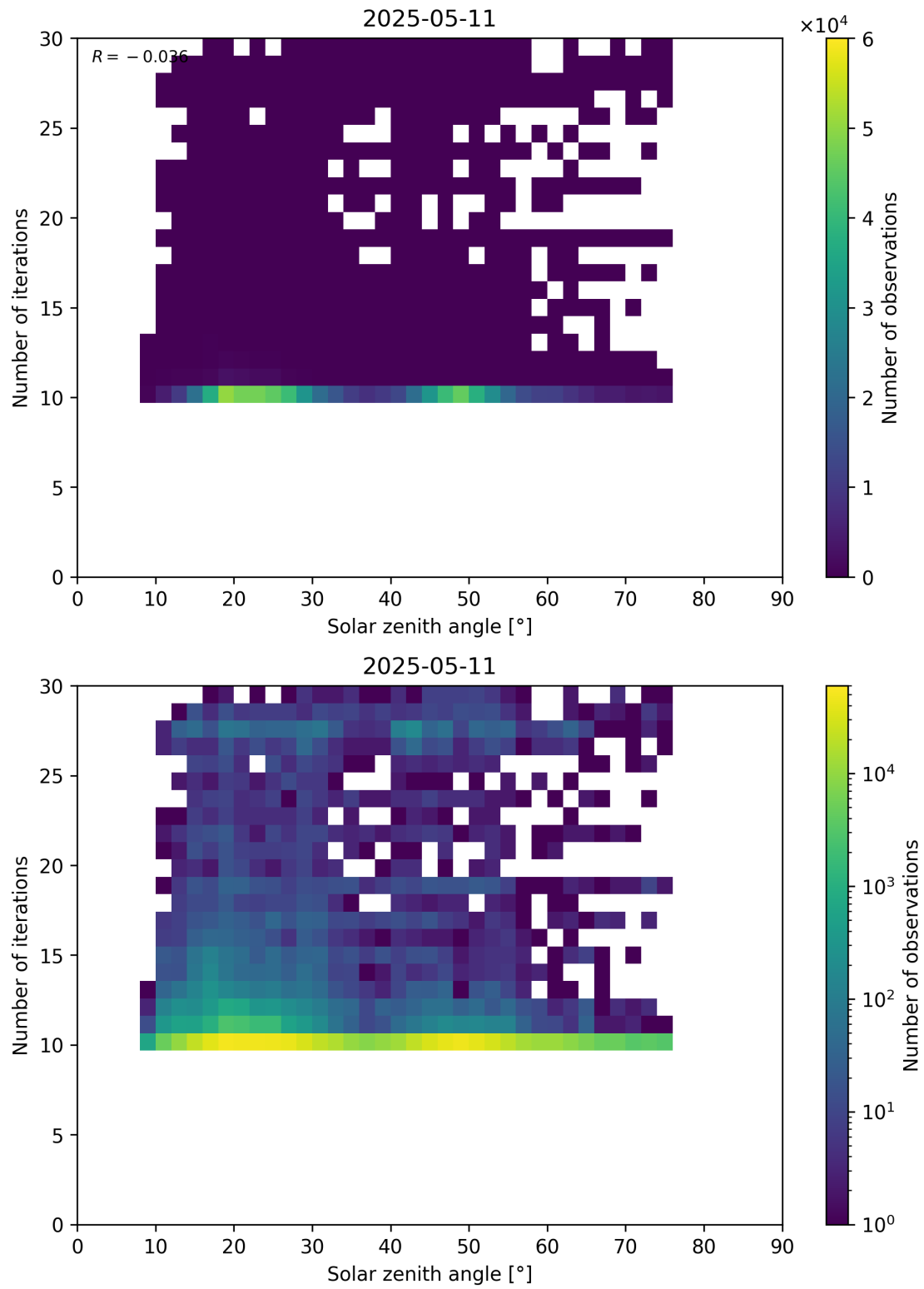
Figure 102: Scatter density plot of “Solar zenith angle” against “Number of iterations” for 2025-05-10 to 2025-05-12.
