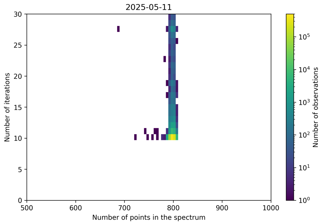
Figure 92: Scatter density plot of “Number of points in the spectrum” against “Number of iterations” for 2025-05-10 to 2025-05-12.
