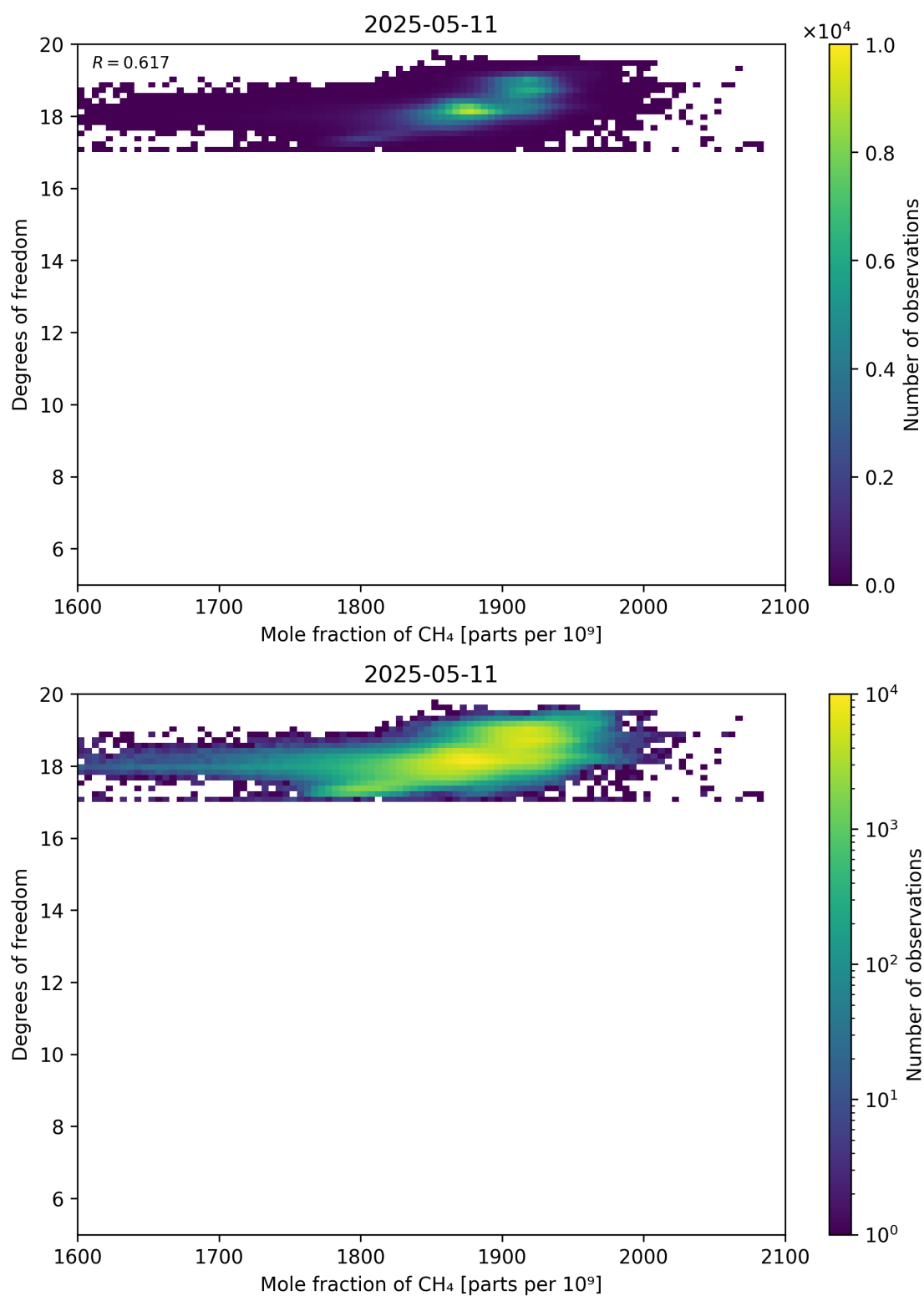
Figure 72: Scatter density plot of “Mole fraction of CH 4 ” against “Degrees of freedom” for 2025-05-10 to 2025-05-12.
