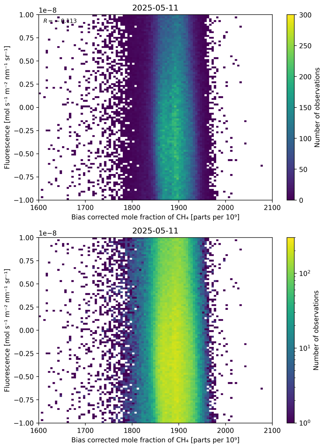
Figure 66: Scatter density plot of “Bias corrected mole fraction of \text{CH}_4 ” against “Fluorescence” for 2025-05-10 to 2025-05-12.
