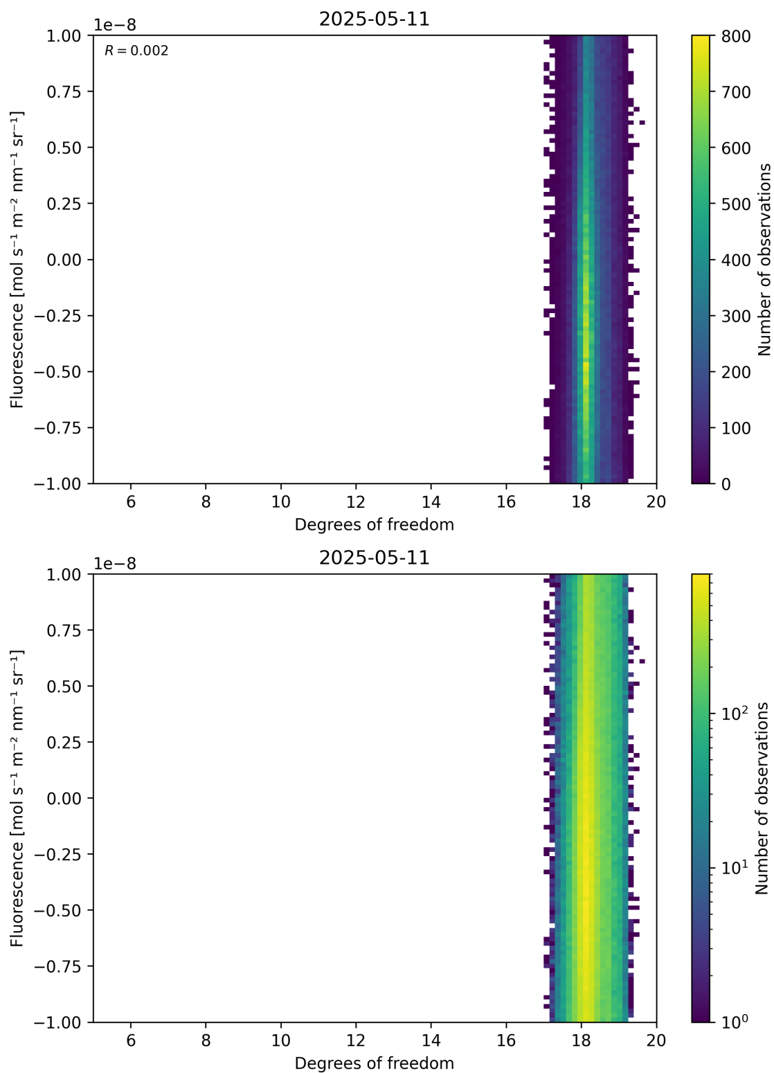
Figure 51: Scatter density plot of “Degrees of freedom” against “Fluorescence” for 2025-05-10 to 2025-05-12.
