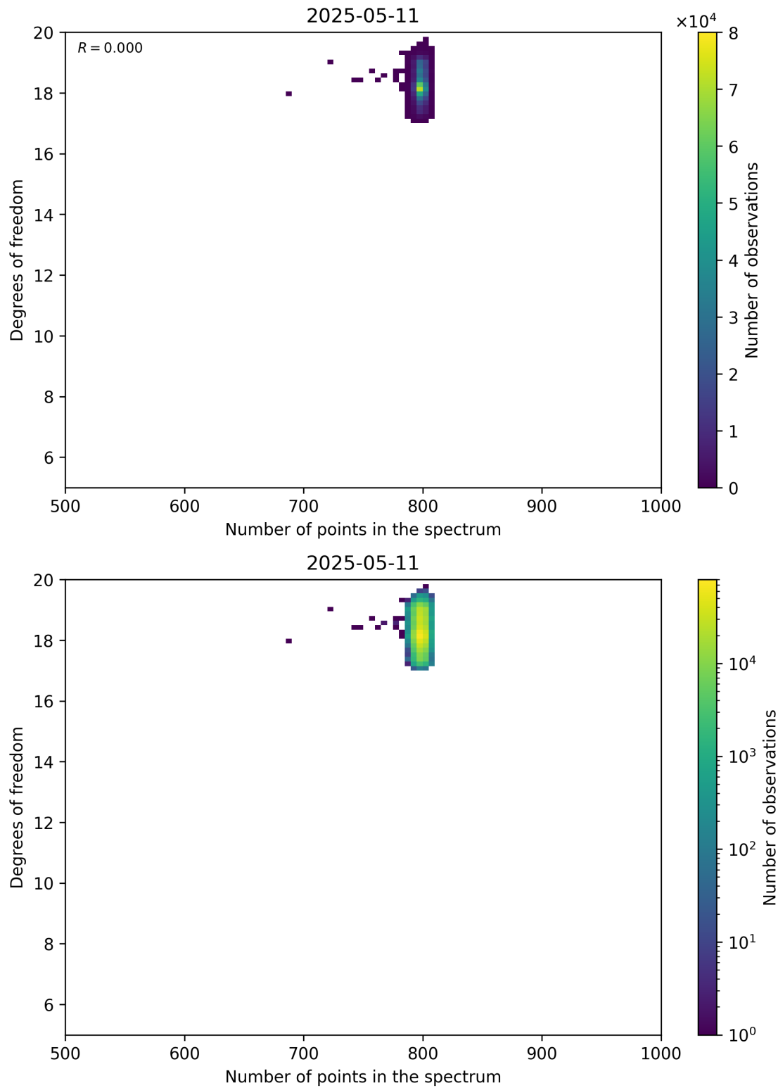
Figure 90: Scatter density plot of “Number of points in the spectrum” against “Degrees of freedom” for 2025-05-10 to 2025-05-12.
