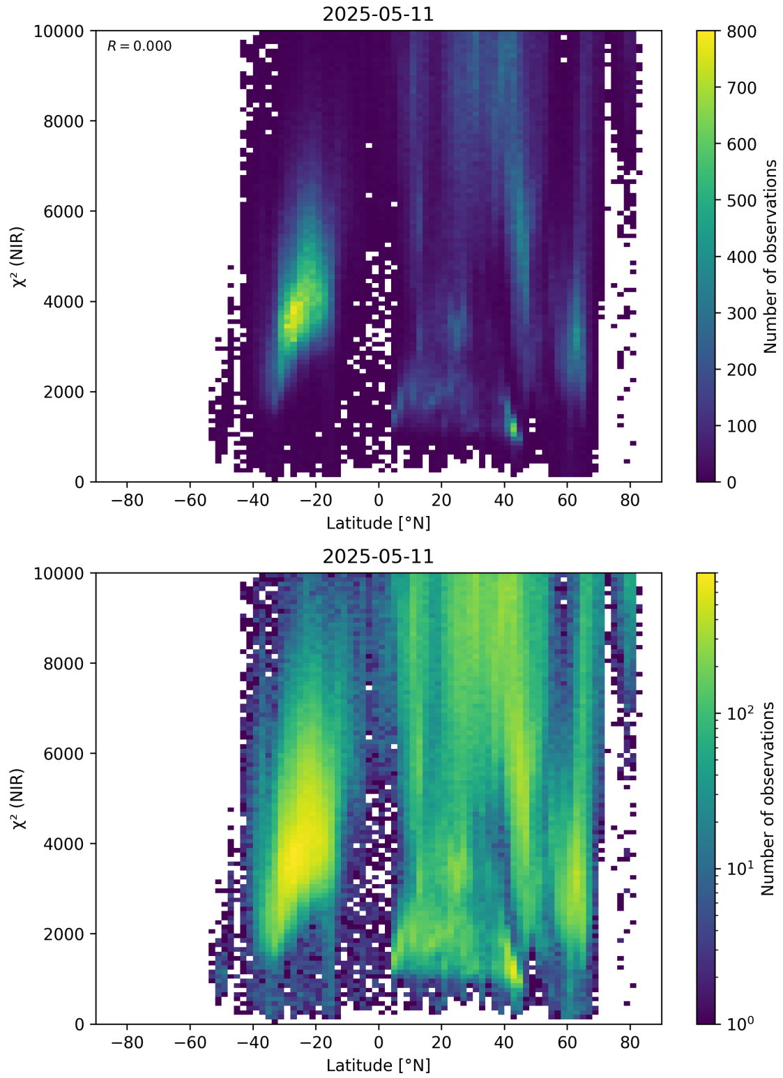
Figure 53: Scatter density plot of “Latitude” against “ \chi^2 (NIR)” for 2025-05-10 to 2025-05-12.
