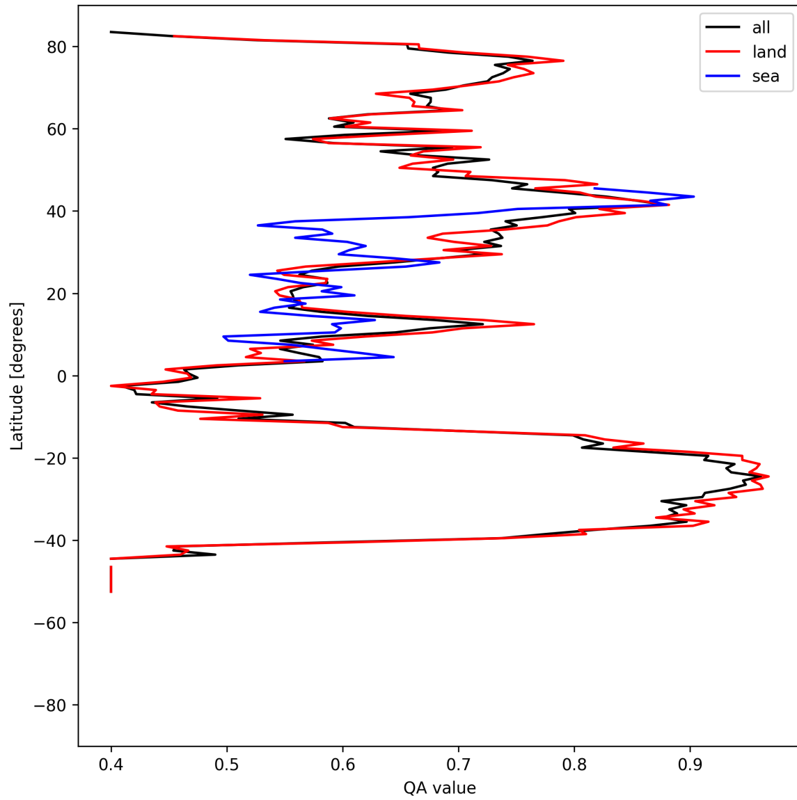
Figure 11: Zonal average of “QA value” for 2025-05-10 to 2025-05-12.
