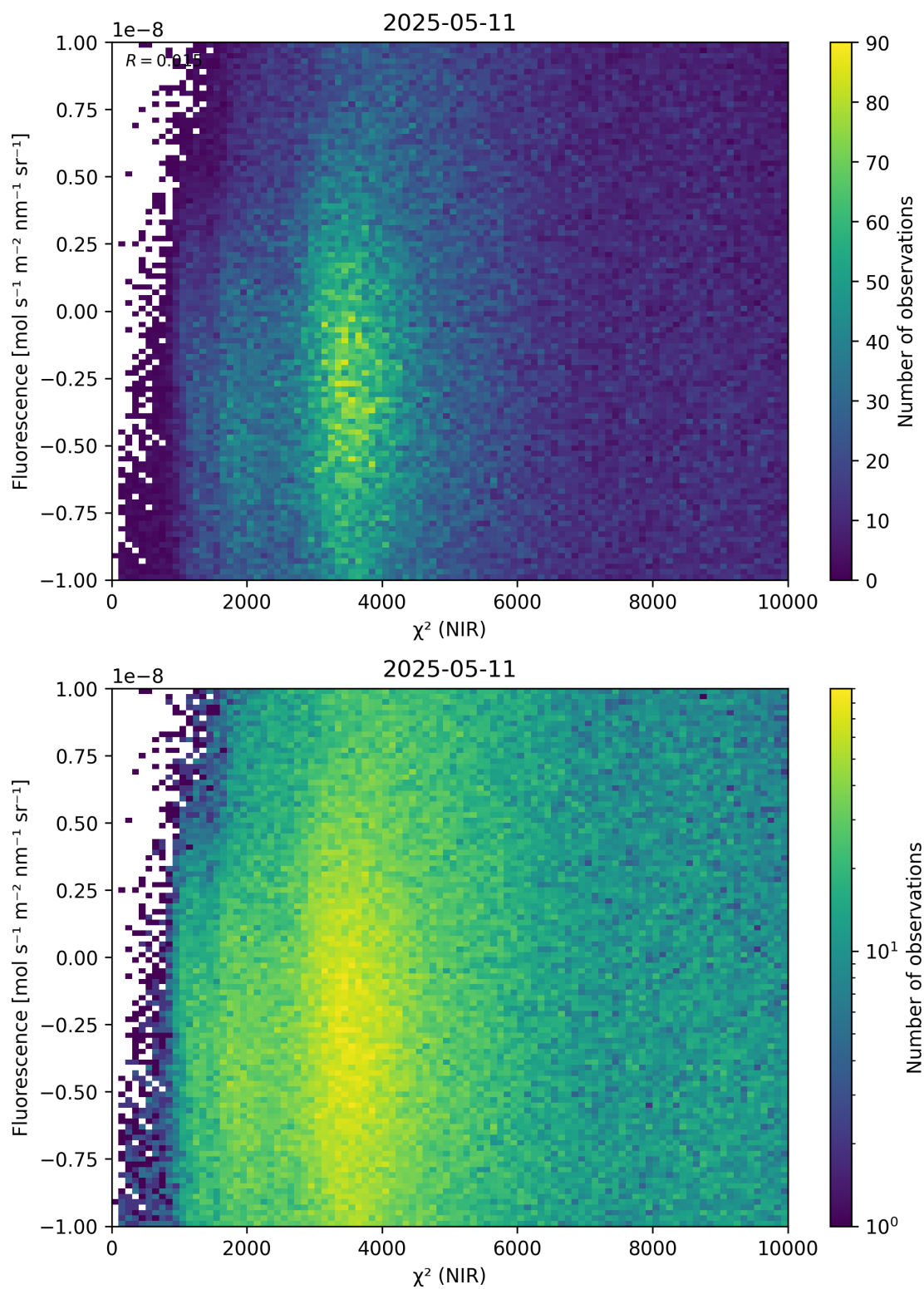
Figure 45: Scatter density plot of “ \chi^2 (NIR)” against “Fluorescence” for 2025-05-10 to 2025-05-12.
