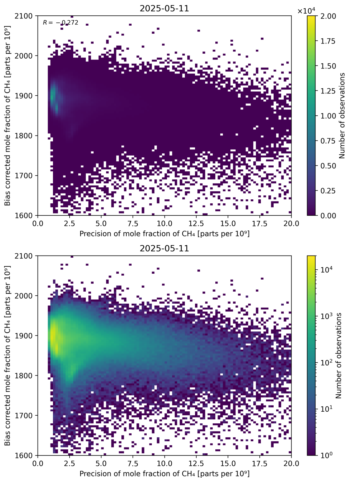
Figure 82: Scatter density plot of “Precision of mole fraction of CH 4 ” against “Bias corrected mole fraction of CH 4 ” for 2025-05-10 to 2025-05-12.
