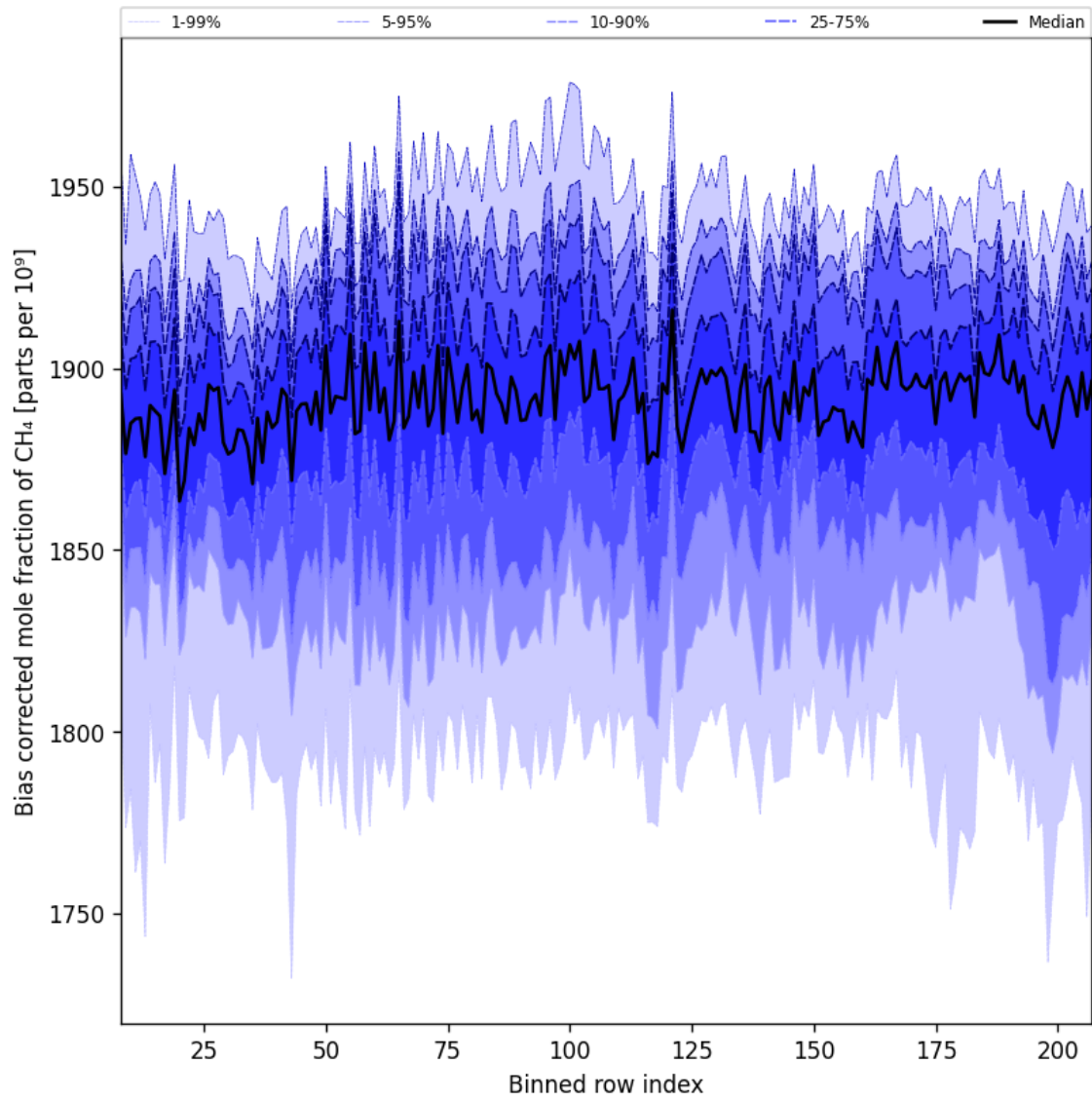
Figure 36: Along track statistics of “Bias corrected mole fraction of CH 4 ” for 2025-05-10 to 2025-05-12
