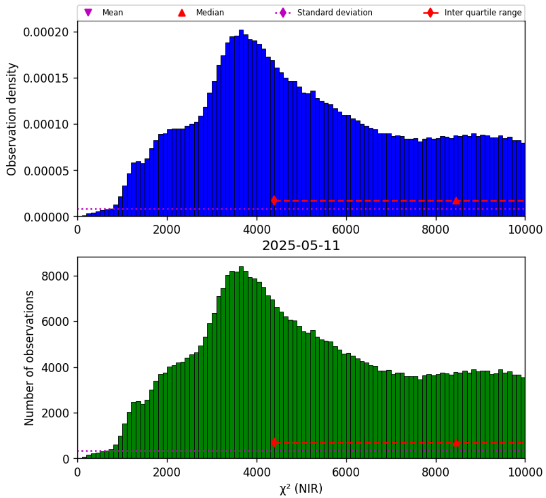
Figure 29: Histogram of " \chi^2 (NIR)" for 2025-05-10 to 2025-05-12
