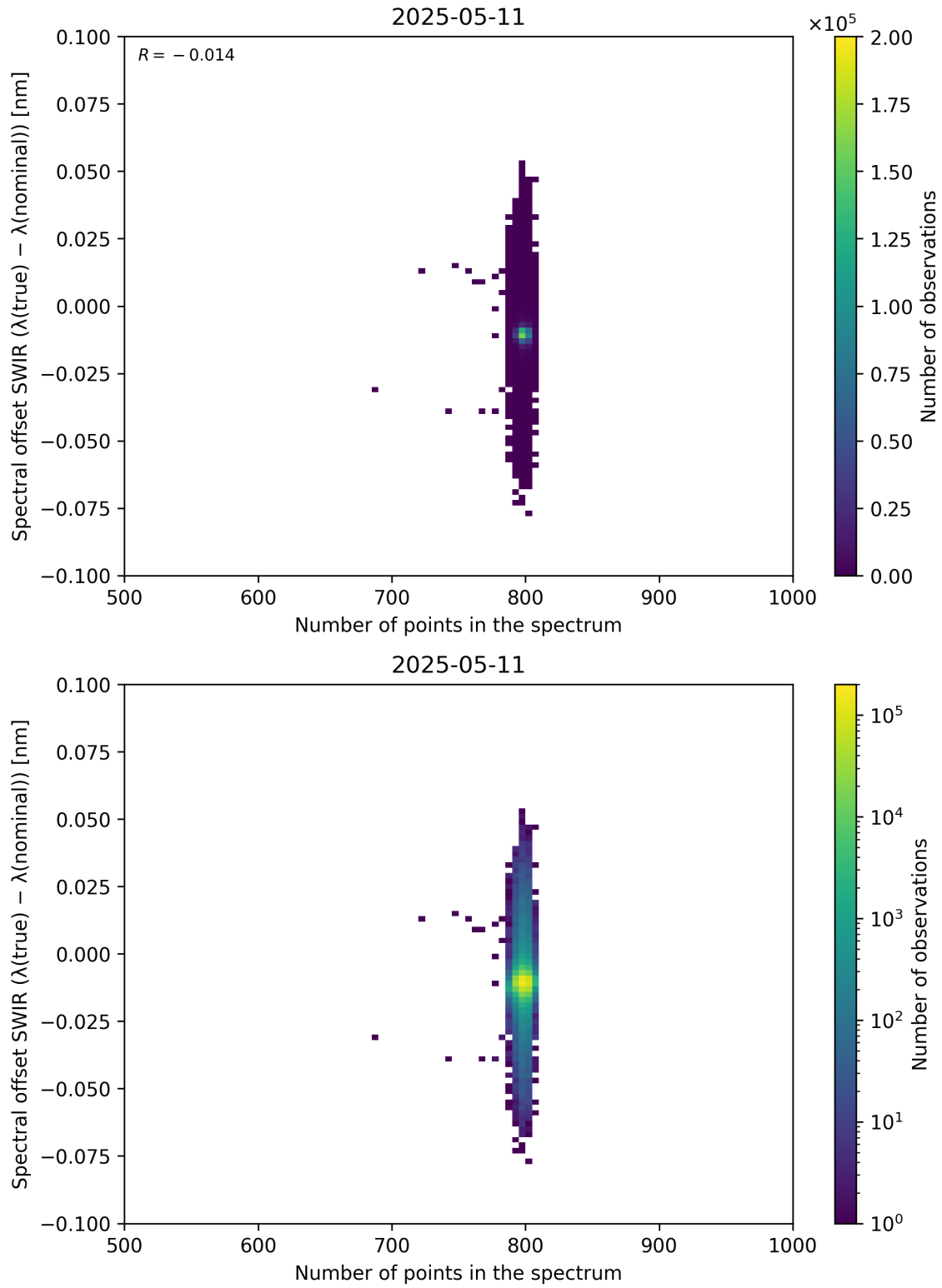
Figure 93: Scatter density plot of “Number of points in the spectrum” against “Spectral offset SWIR ( \lambda_{\text{true}} - \lambda_{\text{nominal}} )” for 2025-05-10 to 2025-05-12.
