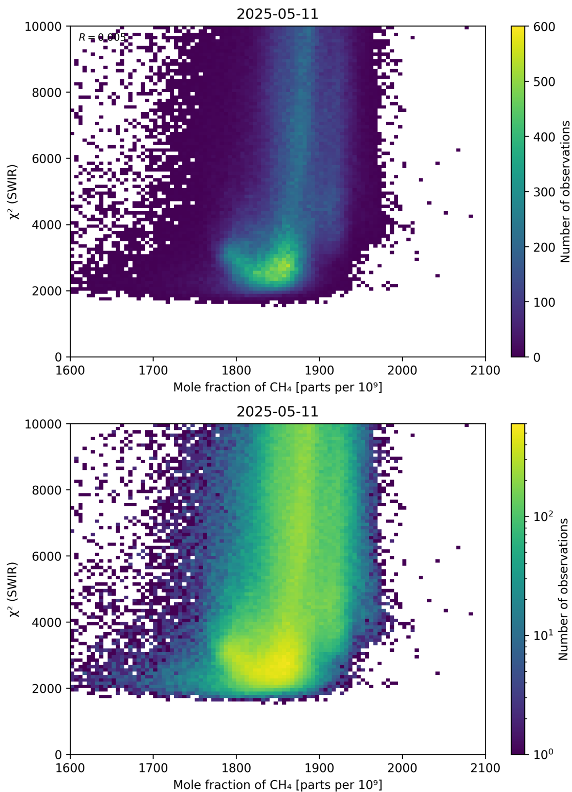
Figure 71: Scatter density plot of “Mole fraction of \text{CH}_4 ” against “ \chi^2 (SWIR)” for 2025-05-10 to 2025-05-12.
