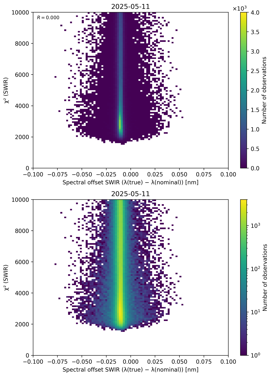
Figure 118: Scatter density plot of “Spectral offset SWIR ( \lambda_{\text{true}} - \lambda_{\text{nominal}} )” against “ \chi^2 (SWIR)” for 2025-05-10 to 2025-05-12.
