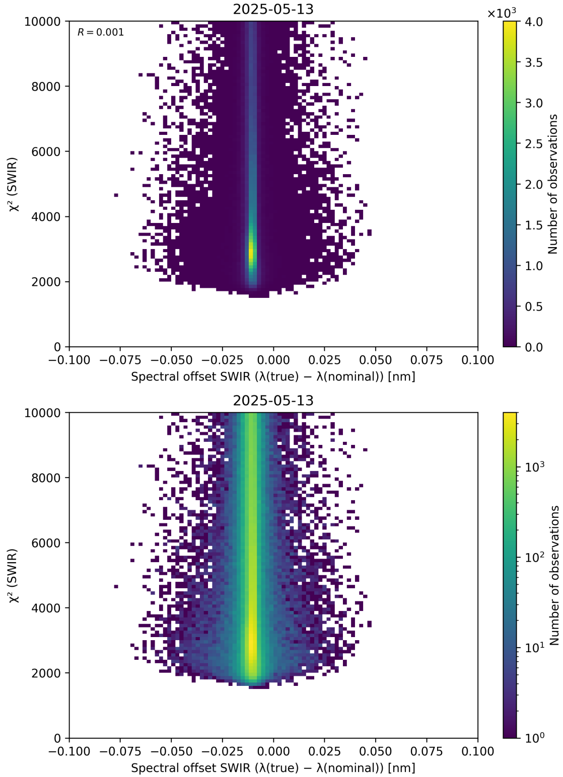
Figure 118: Scatter density plot of “Spectral offset SWIR ( \lambda_{\text{true}} - \lambda_{\text{nominal}} )” against “ \chi^2 (SWIR)” for 2025-05-12 to 2025-05-14.
