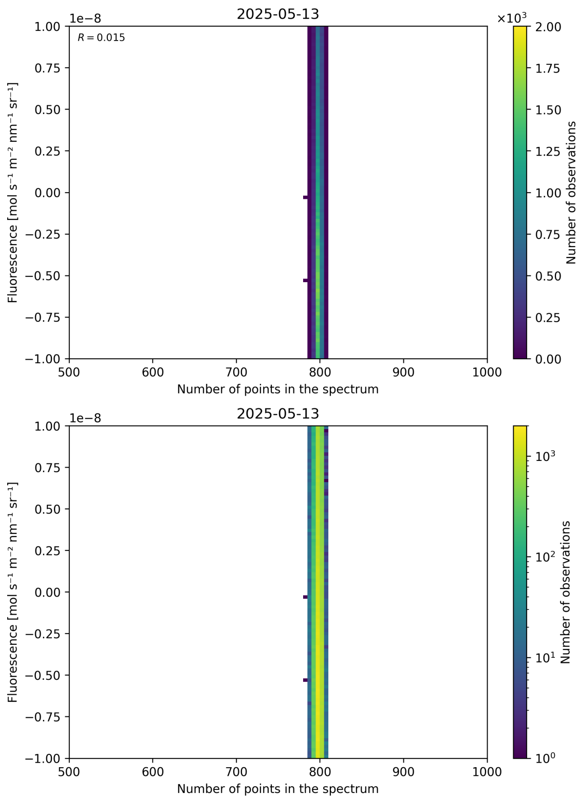
Figure 91: Scatter density plot of “Number of points in the spectrum” against “Fluorescence” for 2025-05-12 to 2025-05-14.
