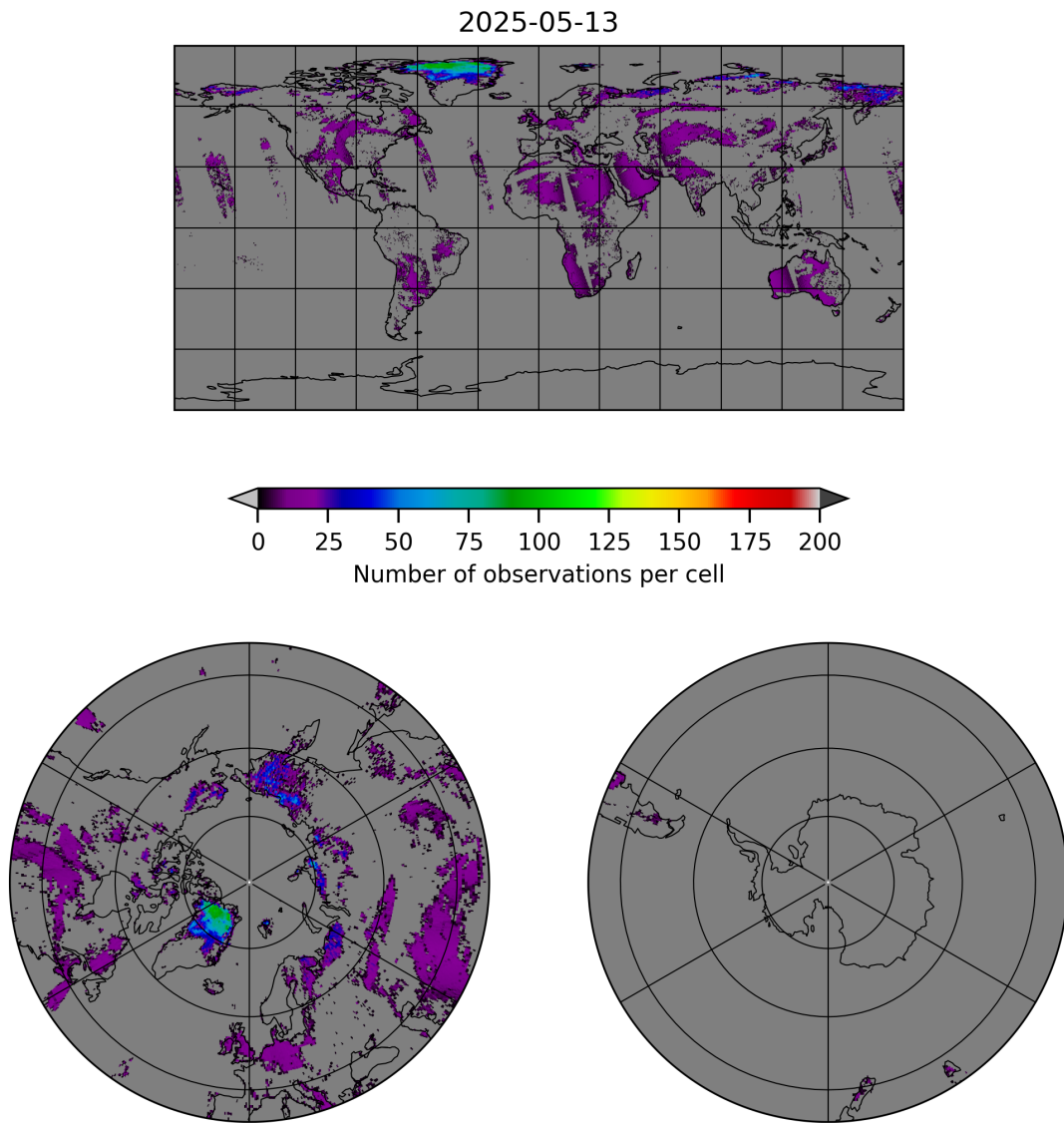
Figure 10: Map of the number of observations for 2025-05-12 to 2025-05-14
