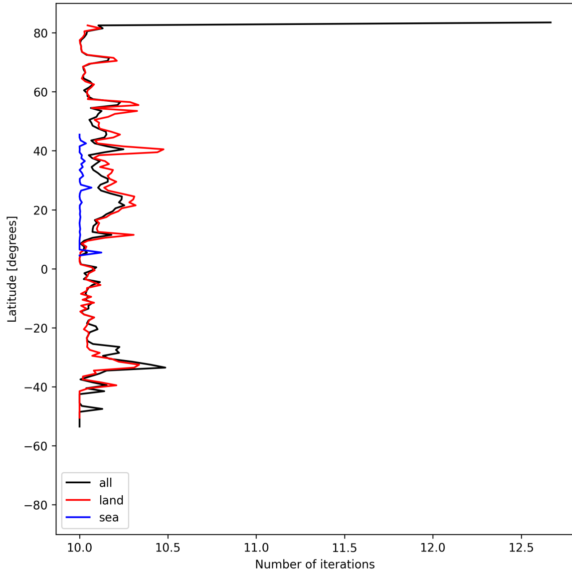
Figure 20: Zonal average of “Number of iterations” for 2025-05-12 to 2025-05-14.
