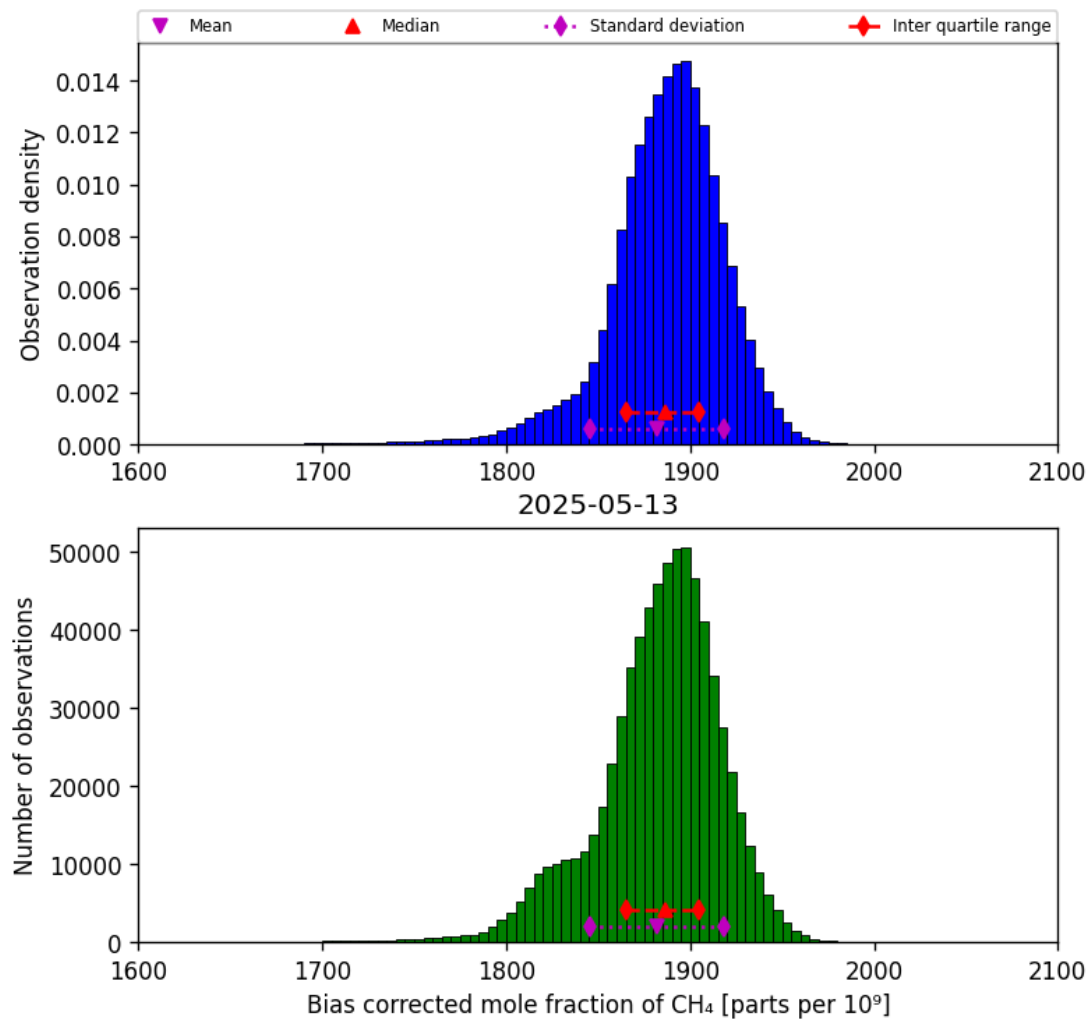
Figure 25: Histogram of “Bias corrected mole fraction of CH 4 ” for 2025-05-12 to 2025-05-14
