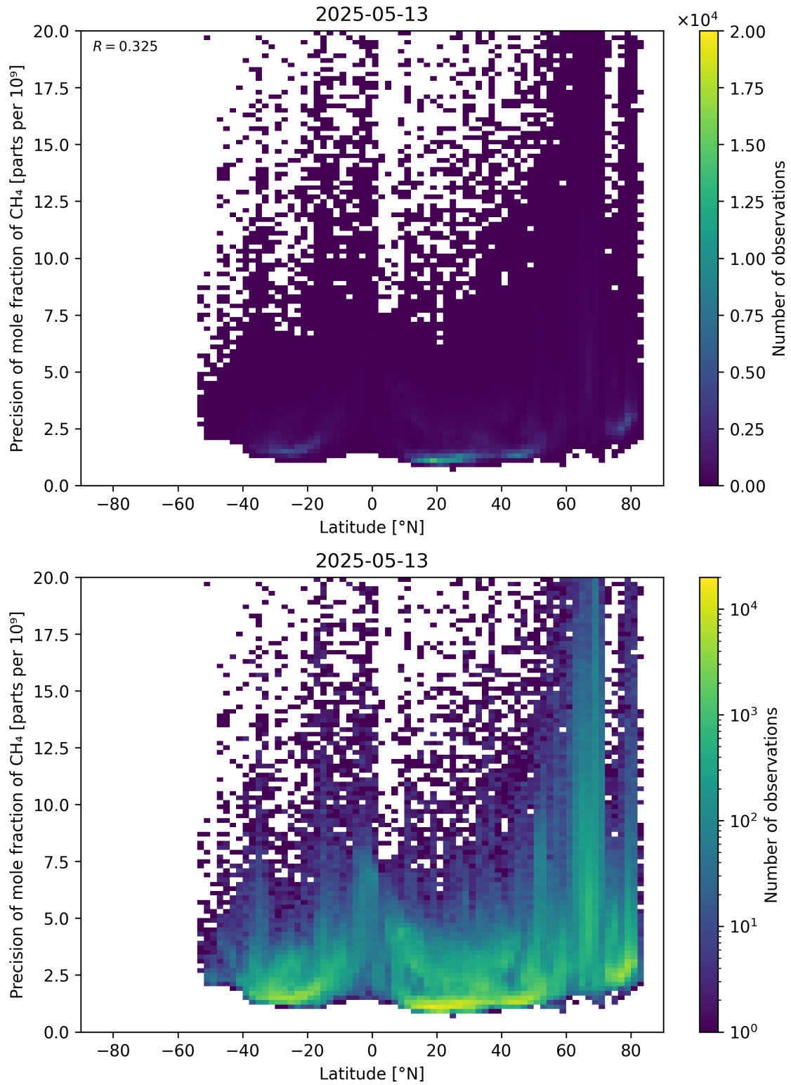
Figure 59: Scatter density plot of “Latitude” against “Precision of mole fraction of \text{CH}_4 ” for 2025-05-12 to 2025-05-14.
