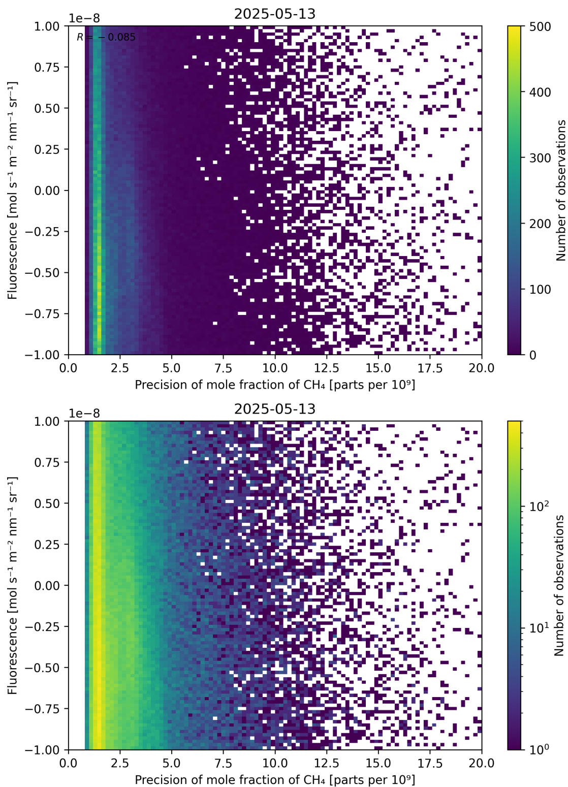
Figure 81: Scatter density plot of “Precision of mole fraction of \text{CH}_4 ” against “Fluorescence” for 2025-05-12 to 2025-05-14.
