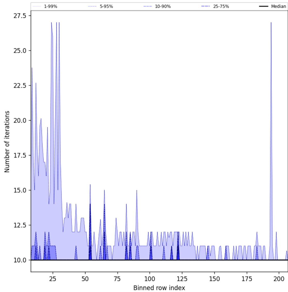
Figure 42: Along track statistics of “Number of iterations” for 2025-05-12 to 2025-05-14
