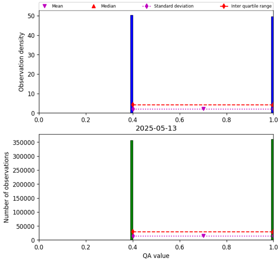
Figure 22: Histogram of “QA value” for 2025-05-12 to 2025-05-14
