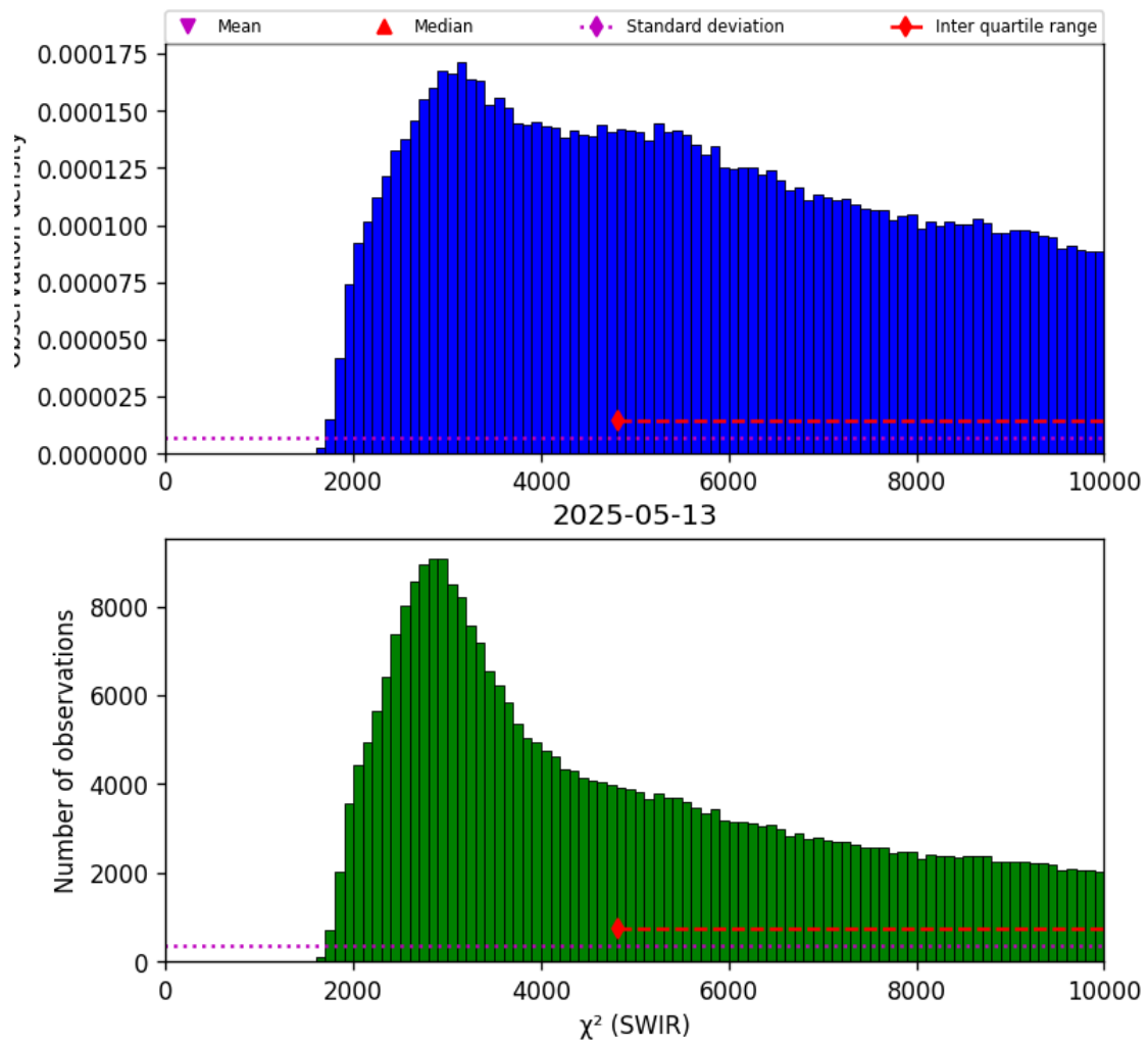
Figure 28: Histogram of “ \chi^2 (SWIR)” for 2025-05-12 to 2025-05-14
