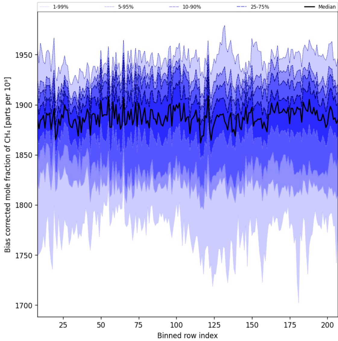
Figure 36: Along track statistics of “Bias corrected mole fraction of CH 4 ” for 2025-05-12 to 2025-05-14
