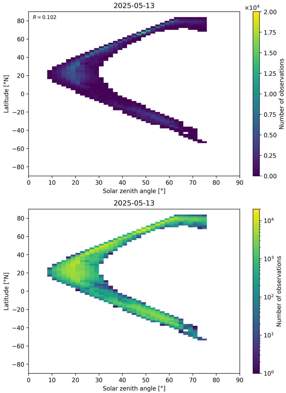
Figure 98: Scatter density plot of “Solar zenith angle” against “Latitude” for 2025-05-12 to 2025-05-14.
