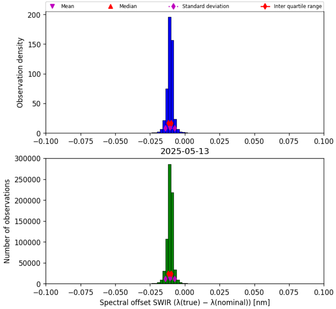
Figure 27: Histogram of “Spectral offset SWIR ( \lambda_{\text{true}} - \lambda_{\text{nominal}} )” for 2025-05-12 to 2025-05-14
