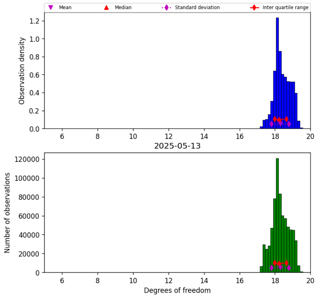
Figure 30: Histogram of “Degrees of freedom” for 2025-05-12 to 2025-05-14
