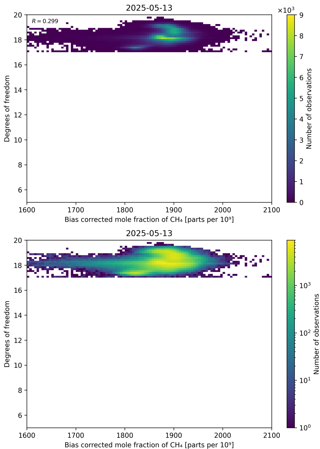
Figure 65: Scatter density plot of “Bias corrected mole fraction of CH 4 ” against “Degrees of freedom” for 2025-05-12 to 2025-05-14.
