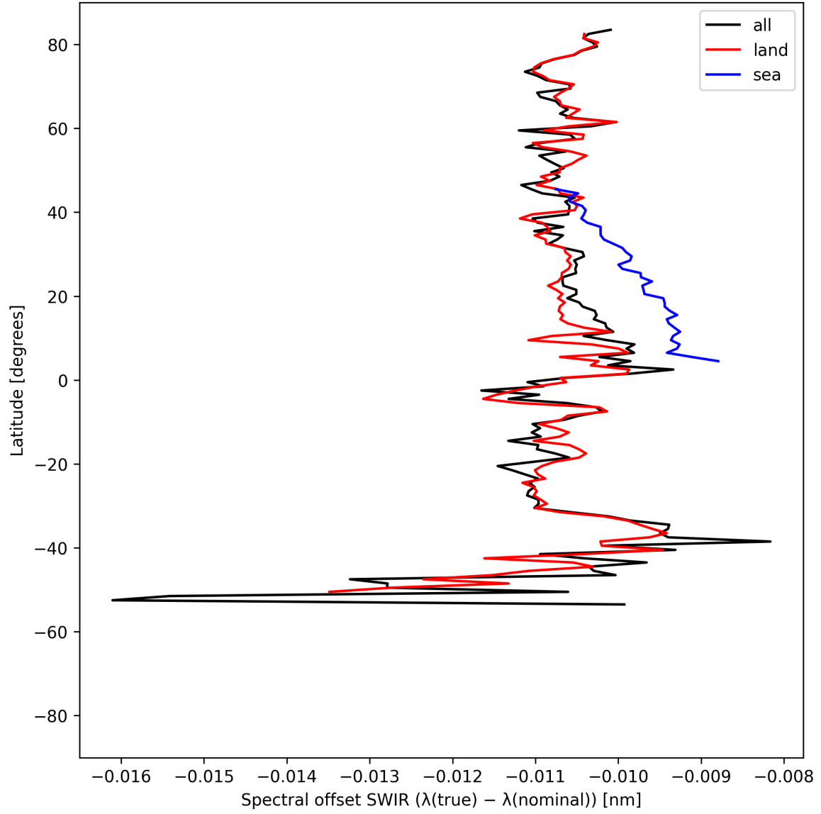
Figure 16: Zonal average of “Spectral offset SWIR ( \lambda_{\text{true}} - \lambda_{\text{nominal}} )” for 2025-05-12 to 2025-05-14.
