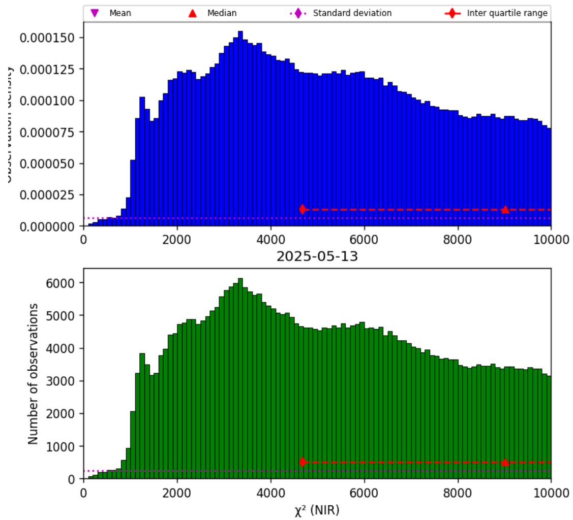
Figure 29: Histogram of “ \chi^2 (NIR)” for 2025-05-12 to 2025-05-14
