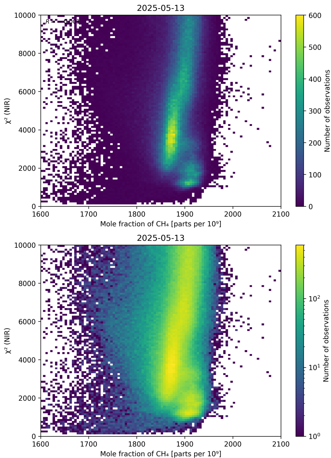
Figure 70: Scatter density plot of “Mole fraction of \text{CH}_4 ” against “ \chi^2 (NIR)” for 2025-05-12 to 2025-05-14.
