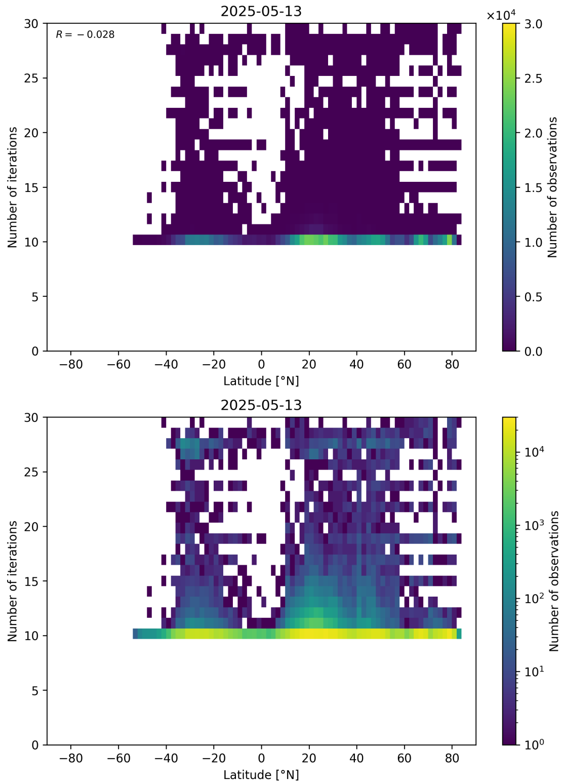
Figure 60: Scatter density plot of “Latitude” against “Number of iterations” for 2025-05-12 to 2025-05-14.
