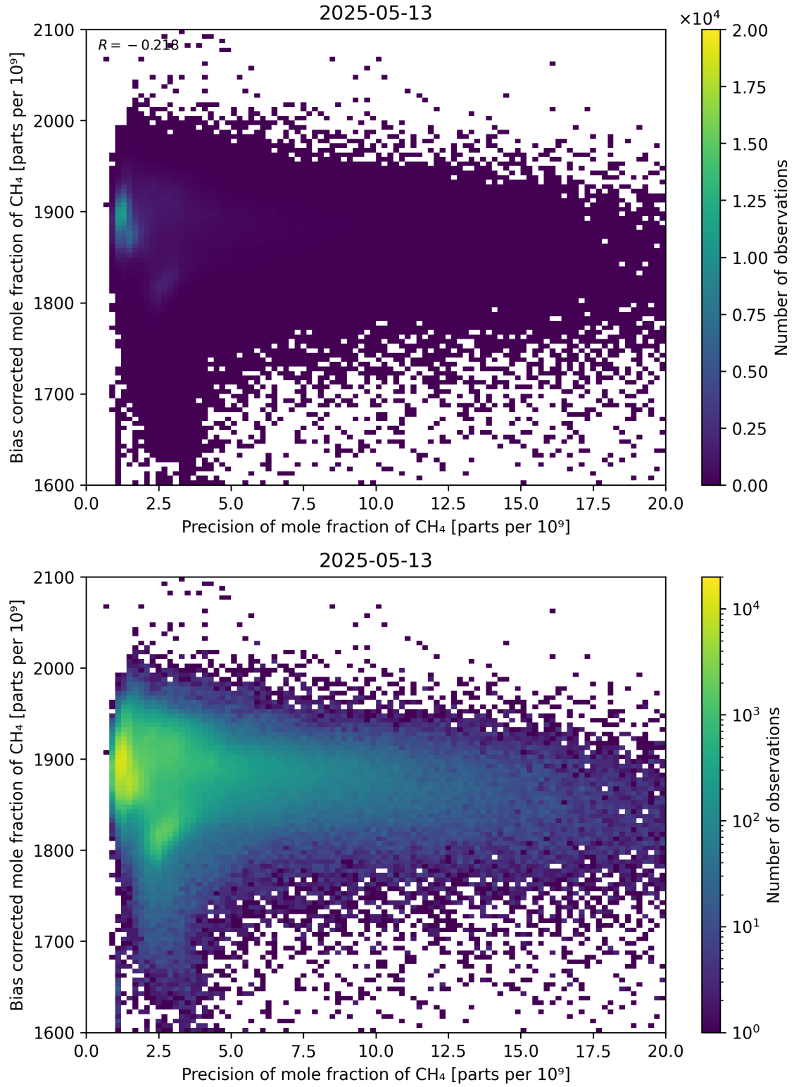
Figure 82: Scatter density plot of “Precision of mole fraction of CH 4 ” against “Bias corrected mole fraction of CH 4 ” for 2025-05-12 to 2025-05-14.
