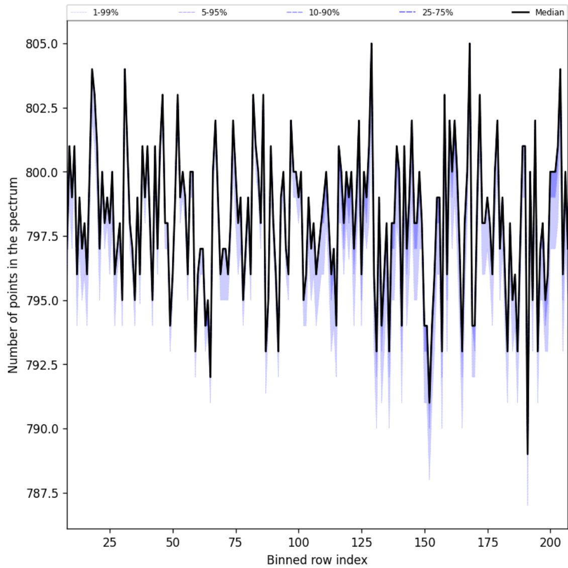
Figure 37: Along track statistics of “Number of points in the spectrum” for 2025-05-12 to 2025-05-14
