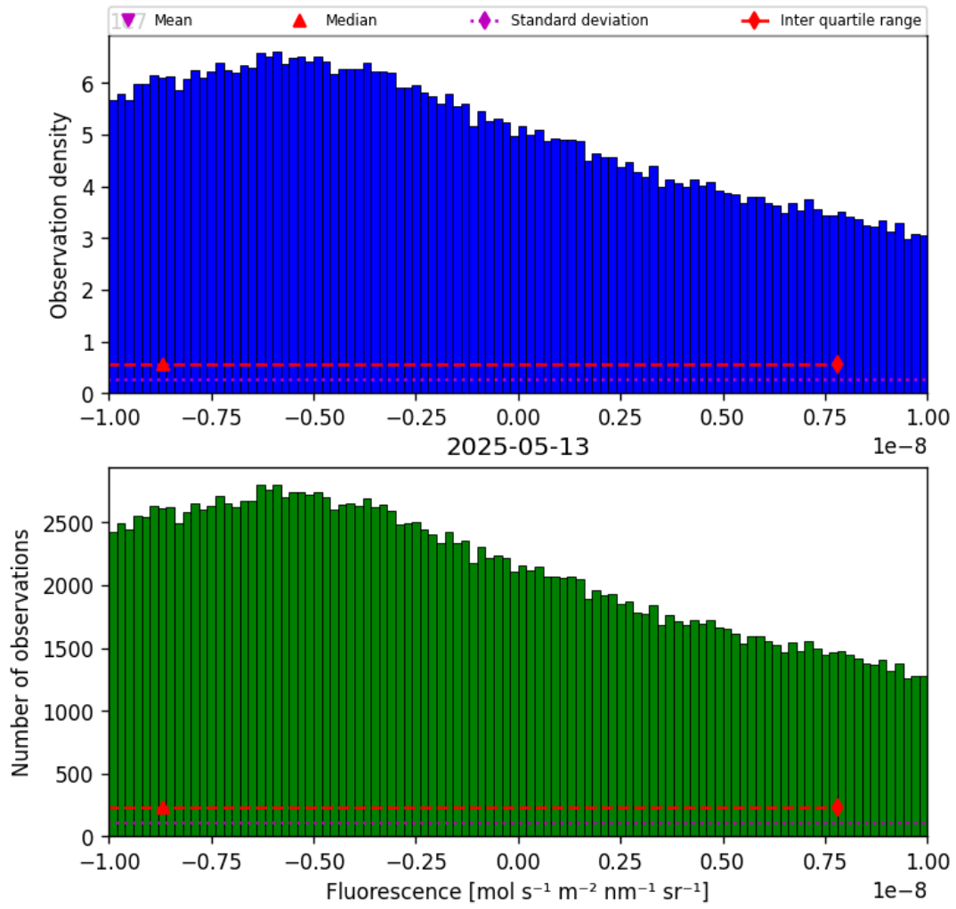
Figure 32: Histogram of “Fluorescence” for 2025-05-12 to 2025-05-14
