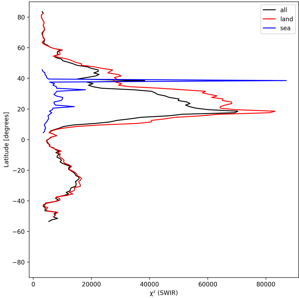
Figure 17: Zonal average of “ \chi^2 (SWIR)” for 2025-05-12 to 2025-05-14.
