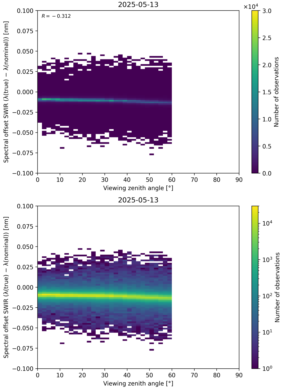
Figure 116: Scatter density plot of “Viewing zenith angle” against “Spectral offset SWIR ( \lambda_{\text{true}} - \lambda_{\text{nominal}} )” for 2025-05-12 to 2025-05-14.
