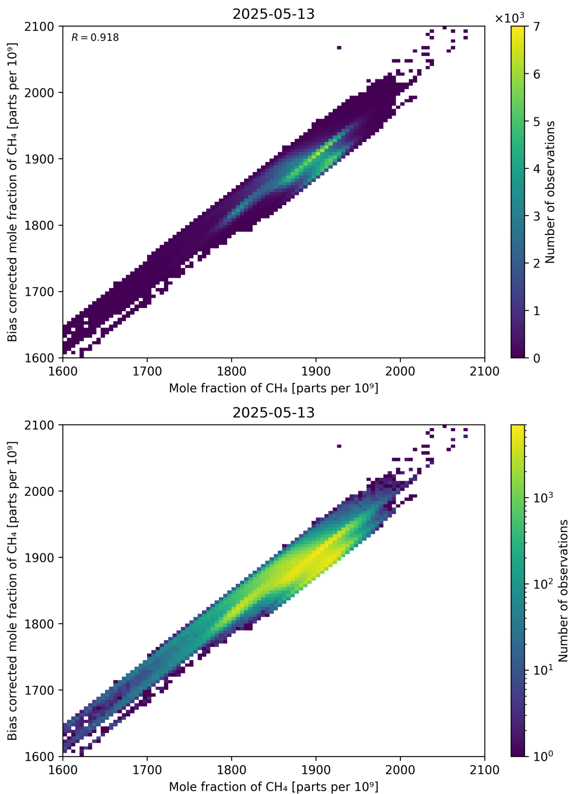
Figure 74: Scatter density plot of “Mole fraction of CH 4 ” against “Bias corrected mole fraction of CH 4 ” for 2025-05-12 to 2025-05-14.
