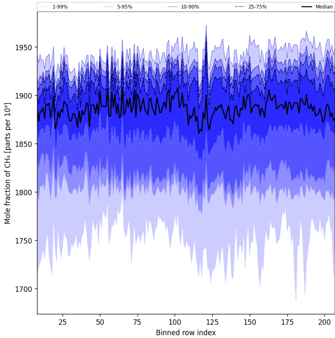
Figure 34: Along track statistics of “Mole fraction of CH 4 ” for 2025-05-12 to 2025-05-14
