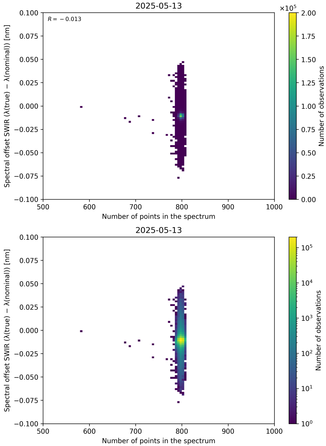
Figure 93: Scatter density plot of “Number of points in the spectrum” against “Spectral offset SWIR ( \lambda_{\text{true}} - \lambda_{\text{nominal}} )” for 2025-05-12 to 2025-05-14.
