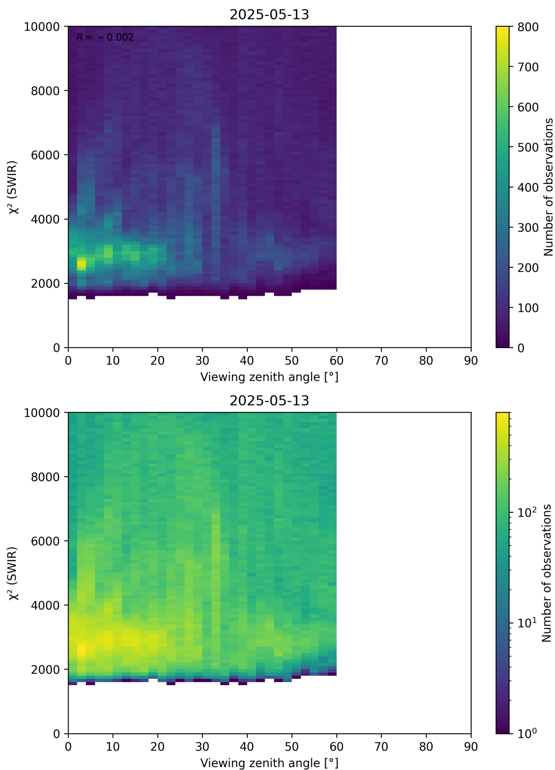
Figure 106: Scatter density plot of “Viewing zenith angle” against “ \chi^2 (SWIR)” for 2025-05-12 to 2025-05-14.
