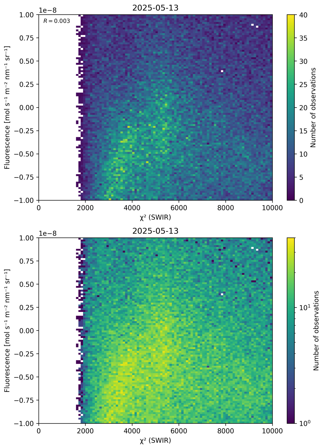
Figure 49: Scatter density plot of “ \chi^2 (SWIR)” against “Fluorescence” for 2025-05-12 to 2025-05-14.
