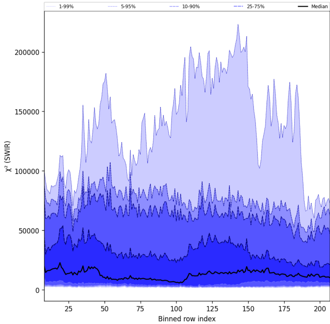
Figure 39: Along track statistics of “ \chi^2 (SWIR)” for 2025-05-12 to 2025-05-14
