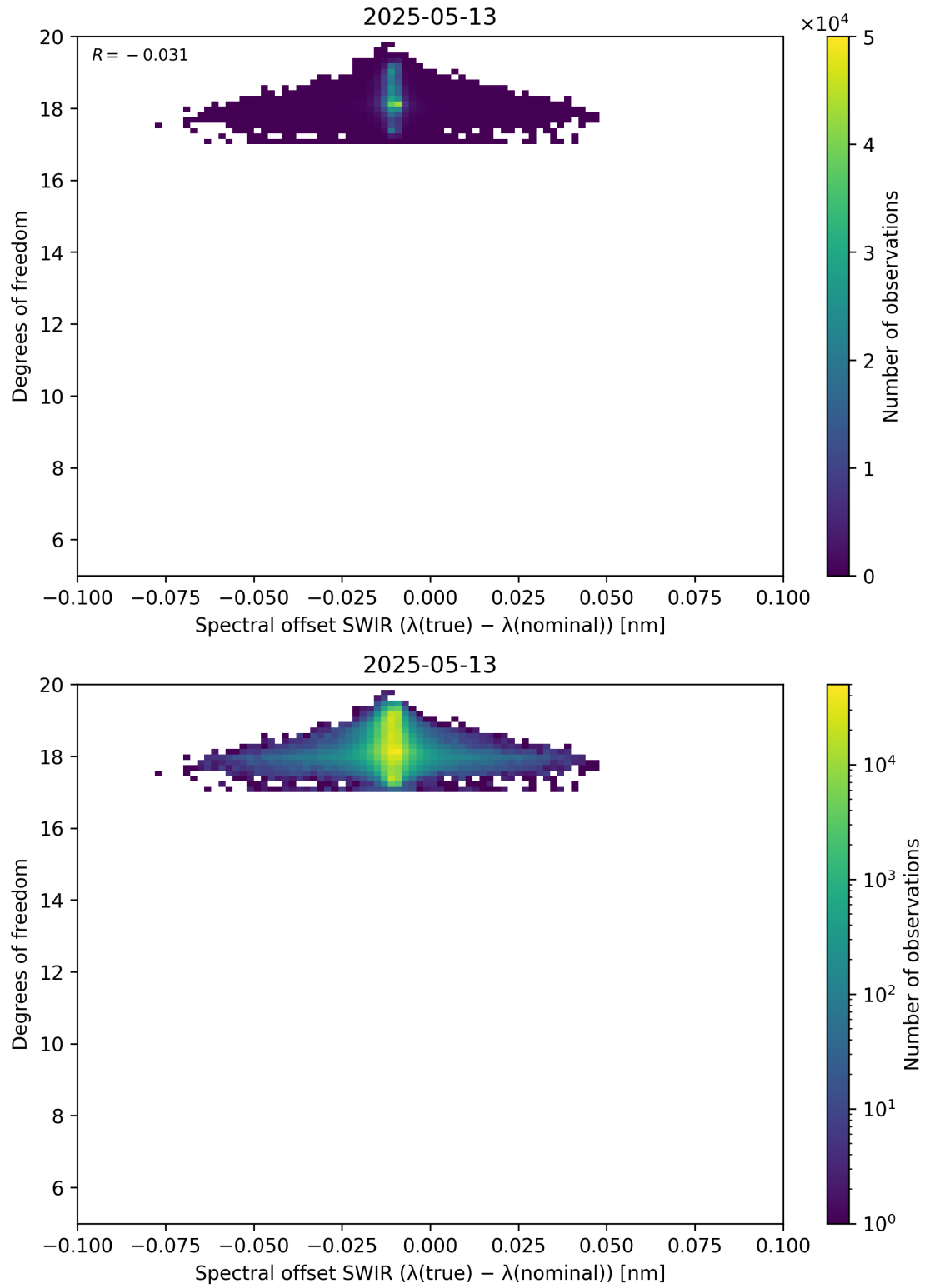
Figure 119: Scatter density plot of “Spectral offset SWIR ( \lambda_{\text{true}} - \lambda_{\text{nominal}} )” against “Degrees of freedom” for 2025-05-12 to 2025-05-14.
