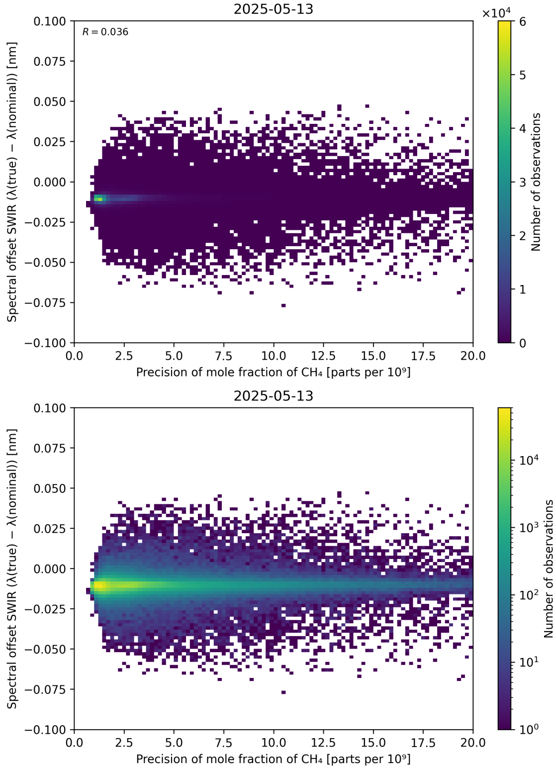
Figure 85: Scatter density plot of “Precision of mole fraction of CH 4 ” against “Spectral offset SWIR ( \lambda_{\text{true}} - \lambda_{\text{nominal}} )” for 2025-05-12 to 2025-05-14.
