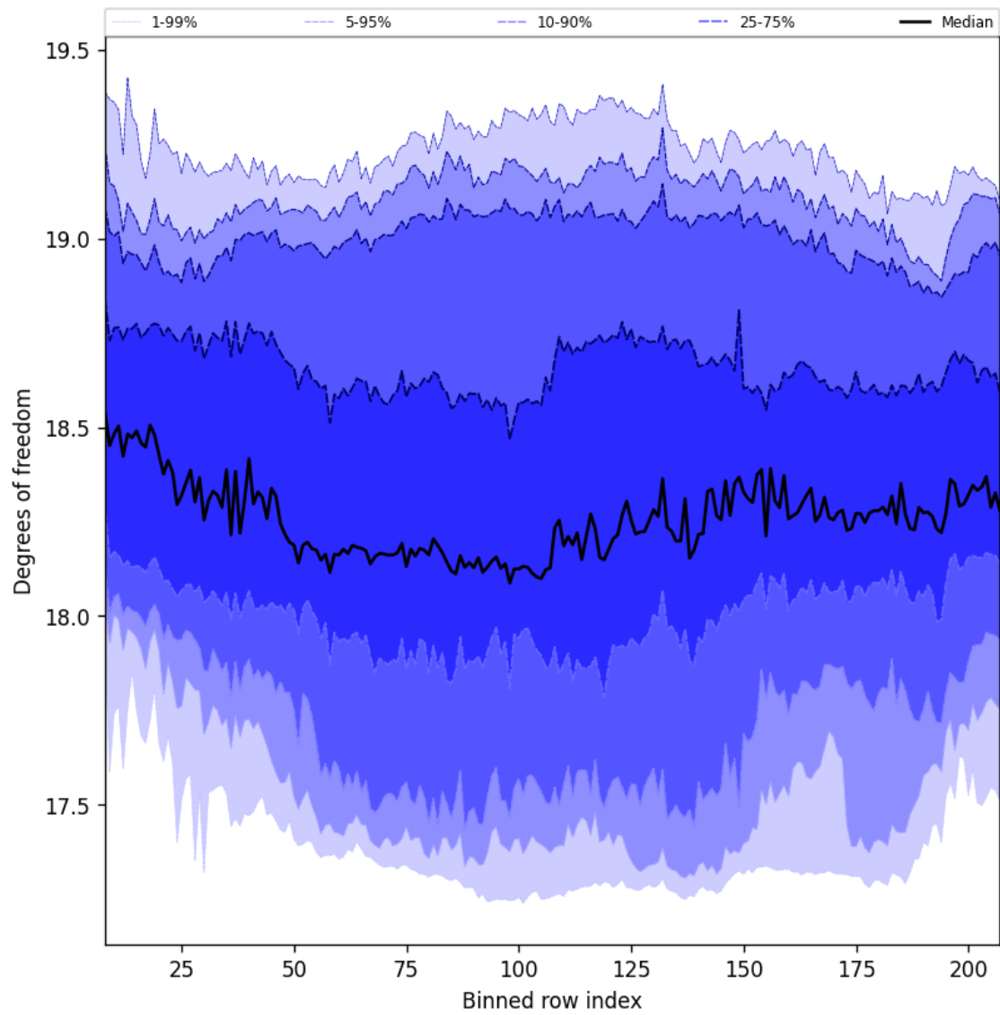
Figure 41: Along track statistics of “Degrees of freedom” for 2025-05-12 to 2025-05-14
