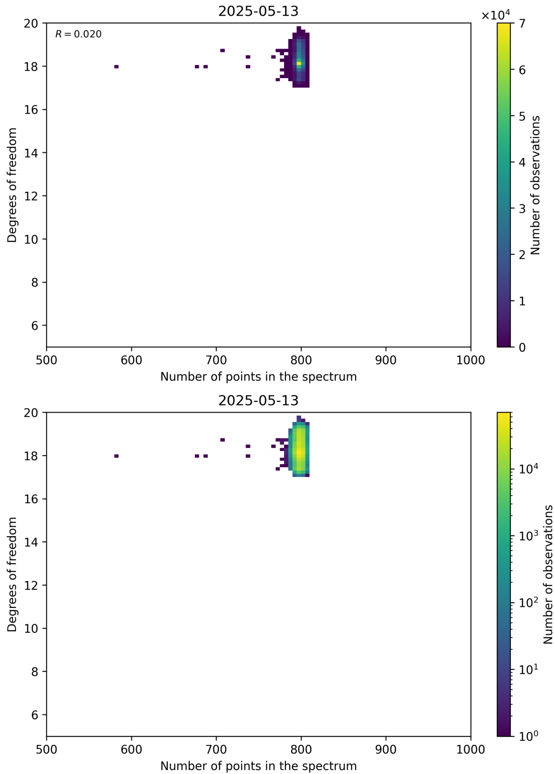
Figure 90: Scatter density plot of “Number of points in the spectrum” against “Degrees of freedom” for 2025-05-12 to 2025-05-14.
