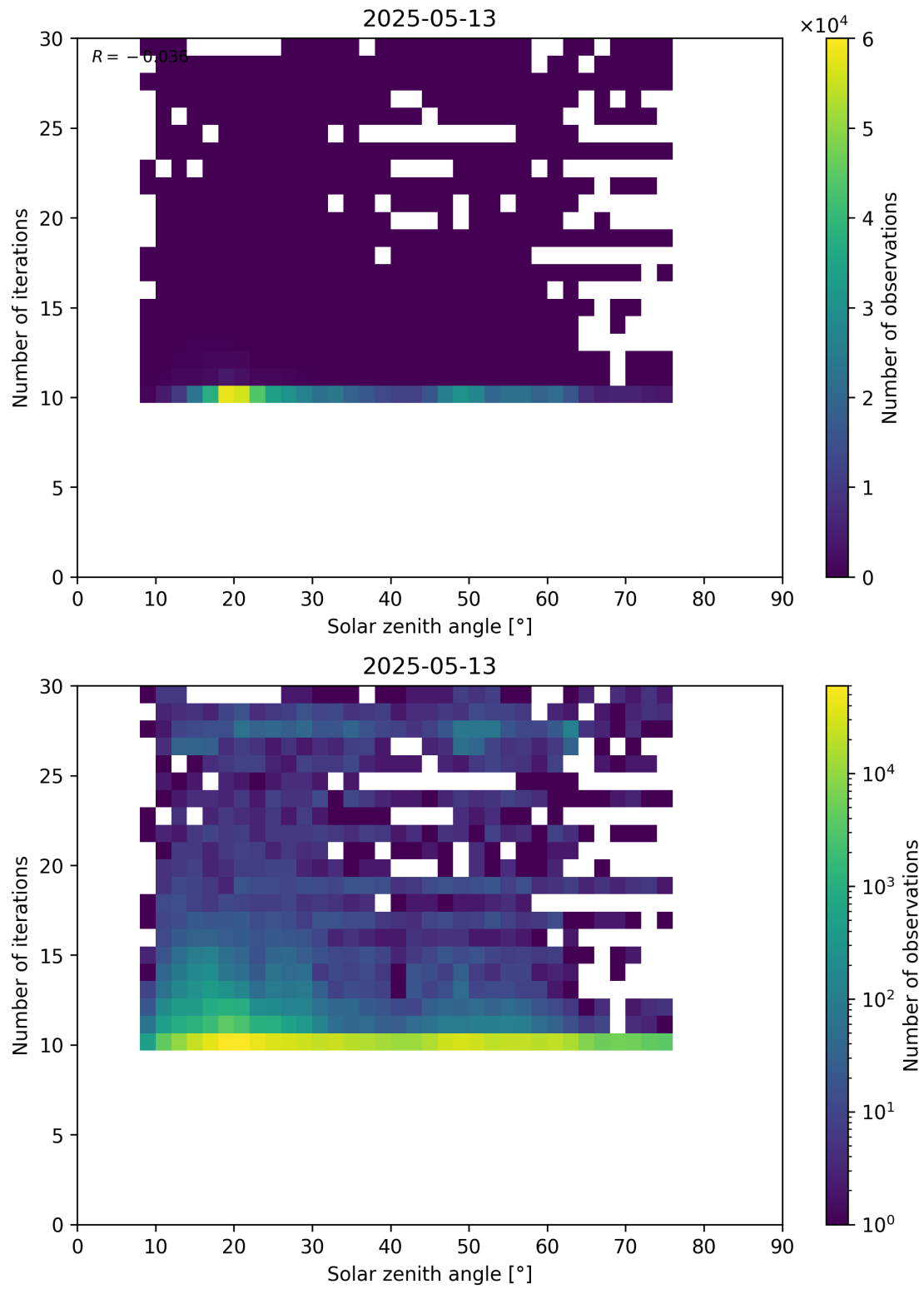
Figure 102: Scatter density plot of “Solar zenith angle” against “Number of iterations” for 2025-05-12 to 2025-05-14.
