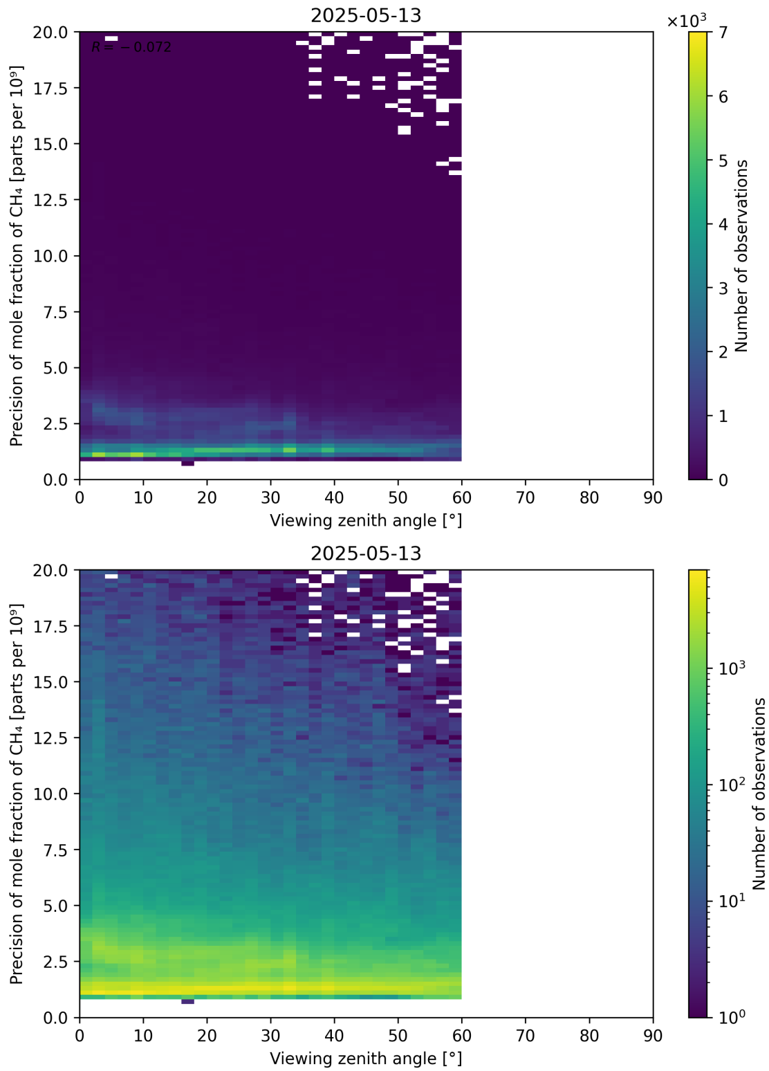
Figure 112: Scatter density plot of “Viewing zenith angle” against “Precision of mole fraction of CH 4 ” for 2025-05-12 to 2025-05-14.
