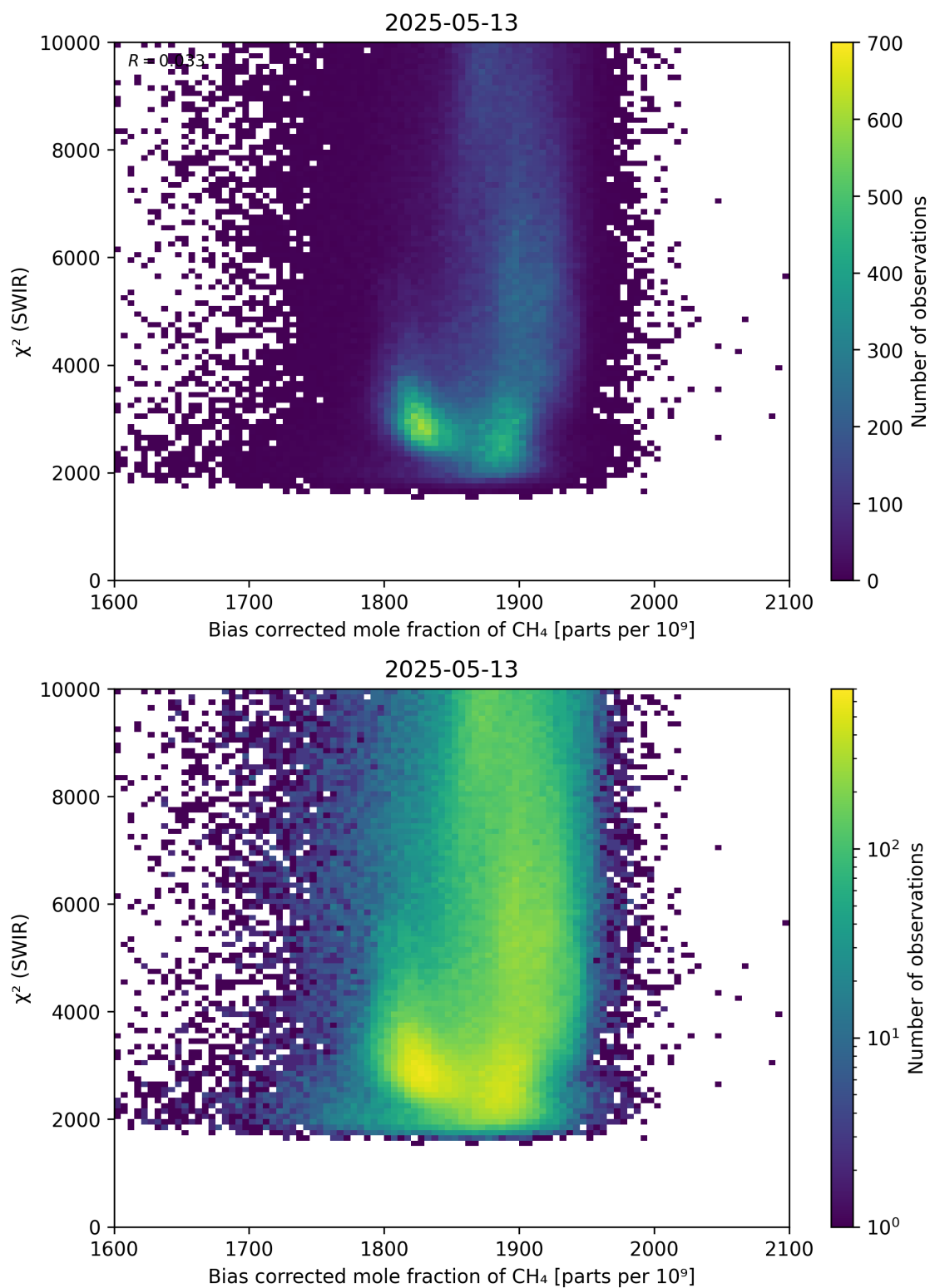
Figure 64: Scatter density plot of “Bias corrected mole fraction of CH 4 ” against “ \chi^2 (SWIR)” for 2025-05-12 to 2025-05-14.
