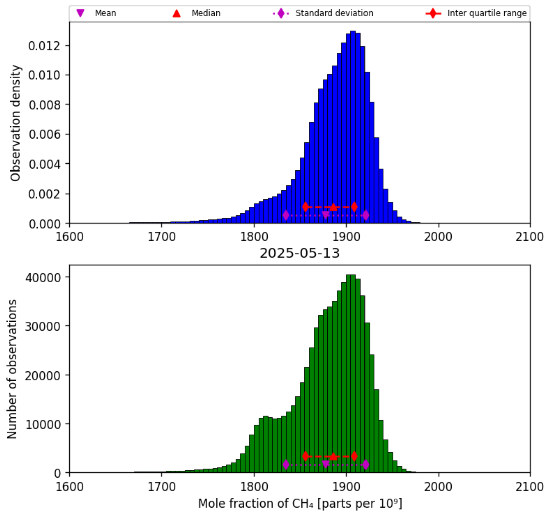
Figure 23: Histogram of “Mole fraction of CH 4 ” for 2025-05-12 to 2025-05-14
