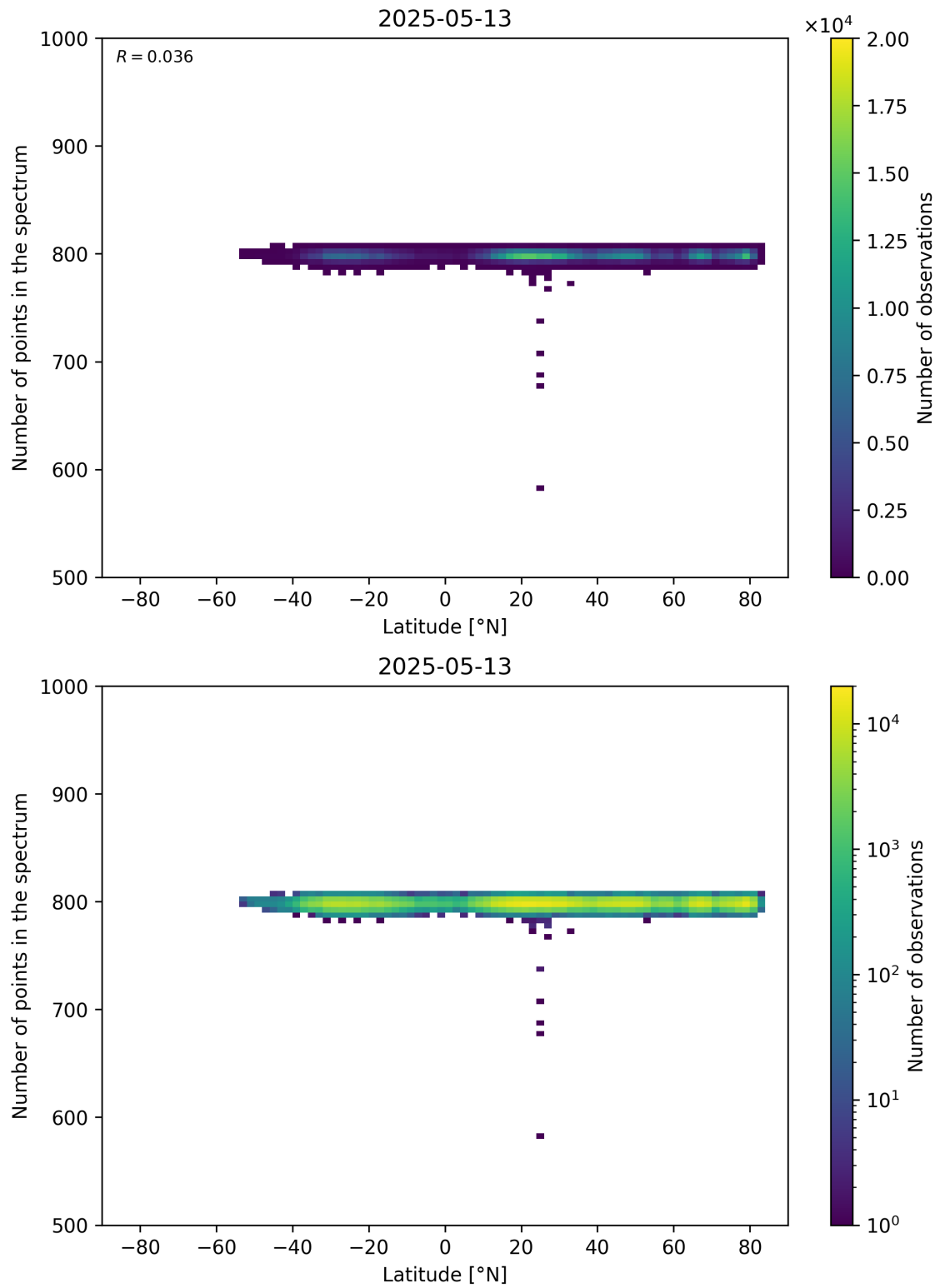
Figure 61: Scatter density plot of “Latitude” against “Number of points in the spectrum” for 2025-05-12 to 2025-05-14.
