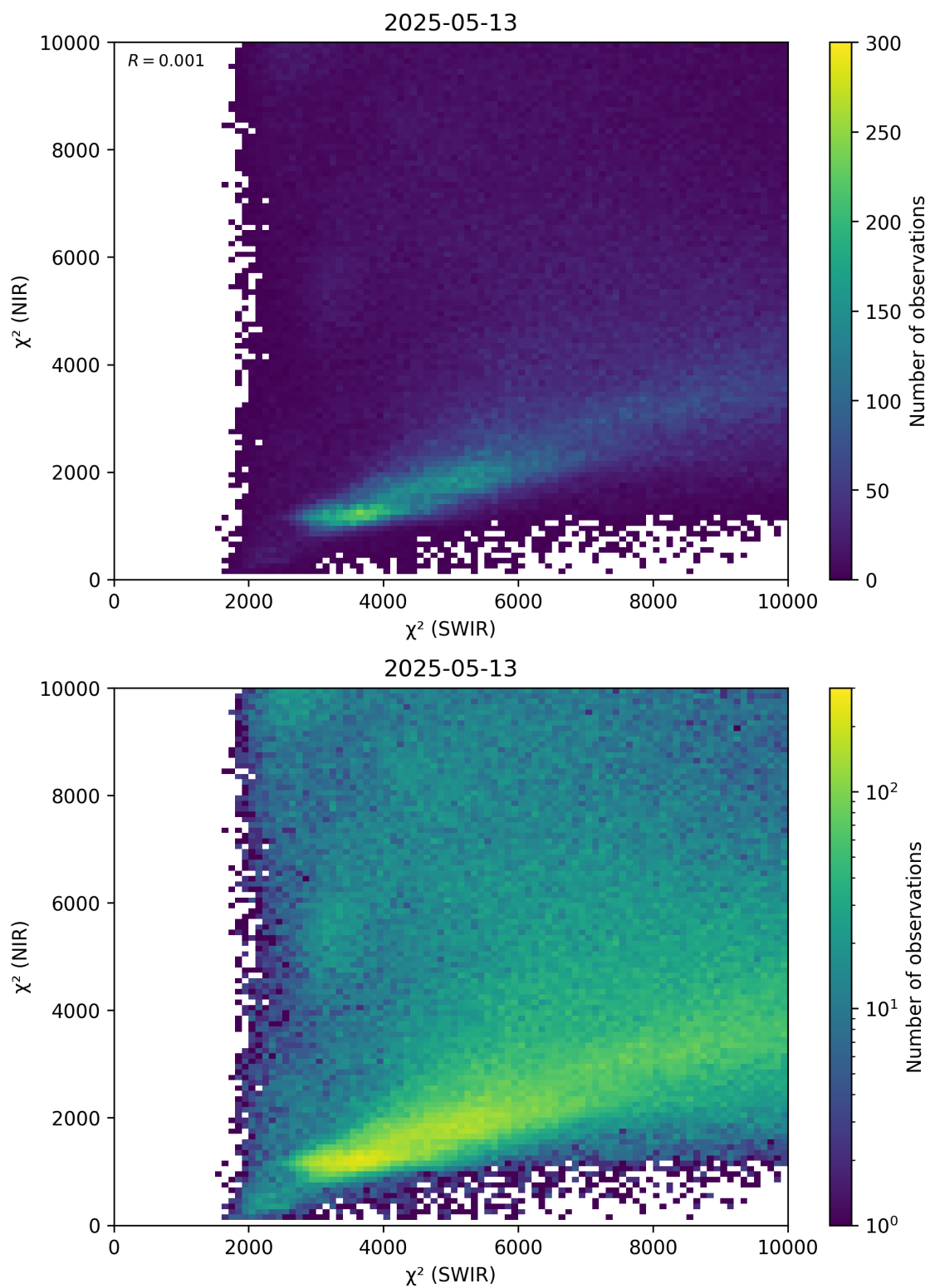
Figure 47: Scatter density plot of “ \chi^2 (SWIR)” against “ \chi^2 (NIR)” for 2025-05-12 to 2025-05-14.
