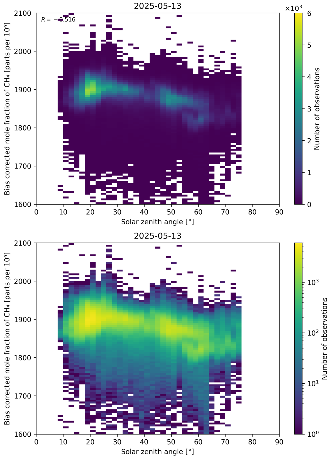
Figure 100: Scatter density plot of “Solar zenith angle” against “Bias corrected mole fraction of CH 4 ” for 2025-05-12 to 2025-05-14.
