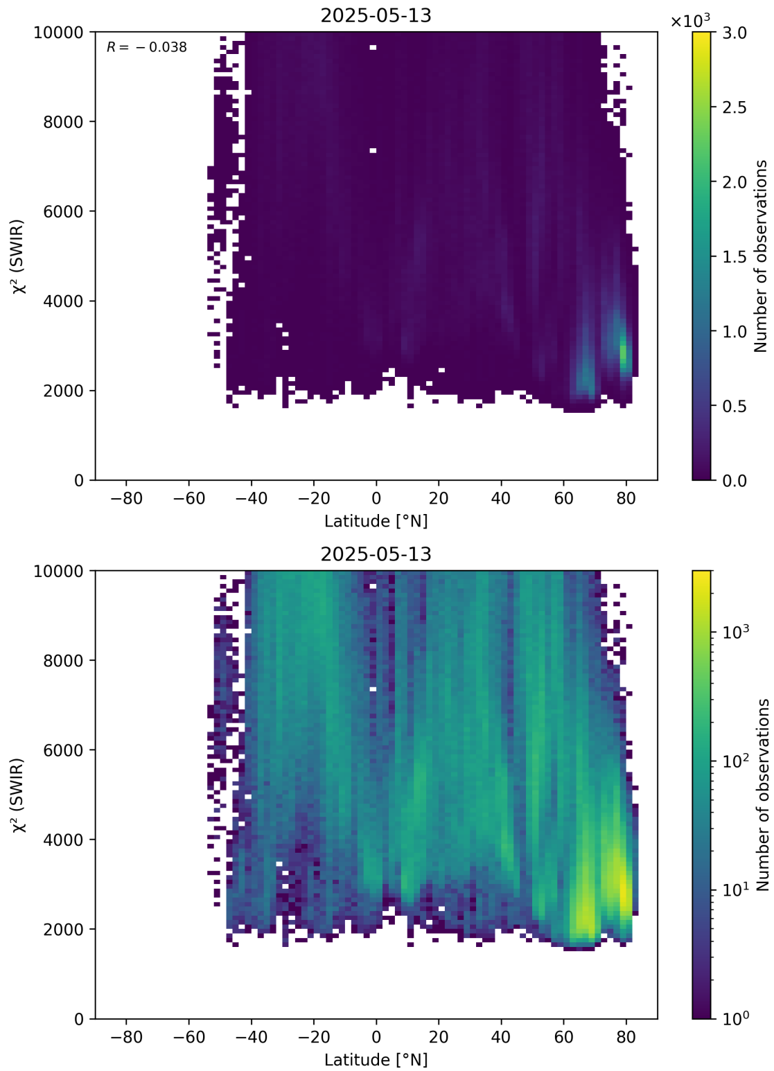
Figure 54: Scatter density plot of “Latitude” against “ \chi^2 (SWIR)” for 2025-05-12 to 2025-05-14.
