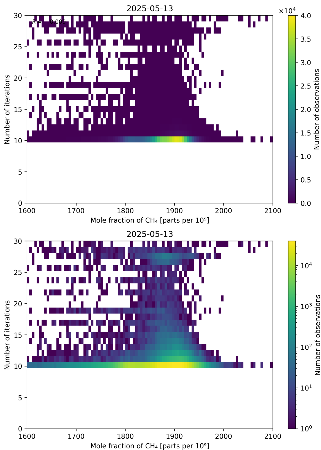
Figure 76: Scatter density plot of “Mole fraction of CH 4 ” against “Number of iterations” for 2025-05-12 to 2025-05-14.
