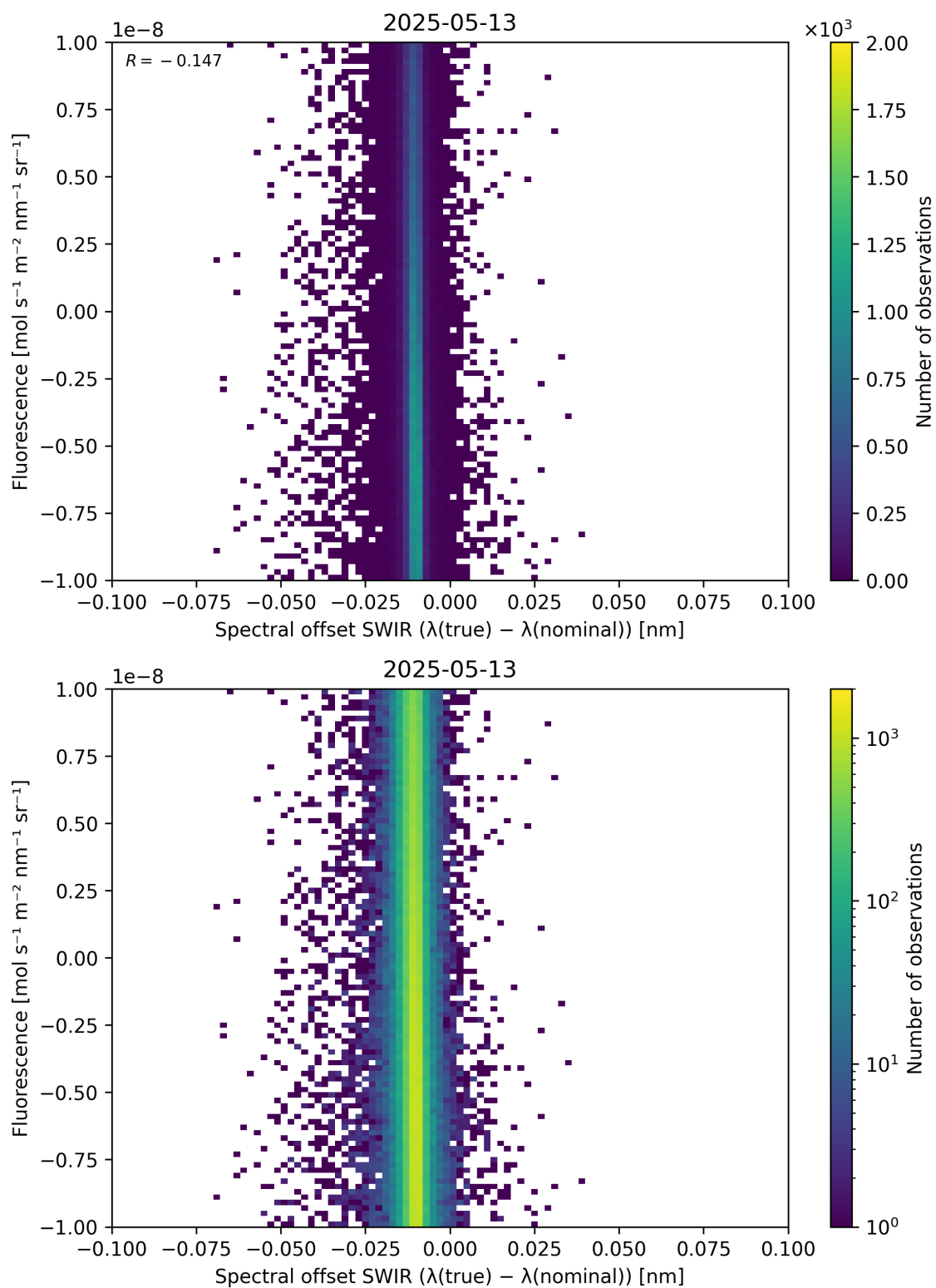
Figure 120: Scatter density plot of “Spectral offset SWIR ( \lambda_{\text{true}} - \lambda_{\text{nominal}} )” against “Fluorescence” for 2025-05-12 to 2025-05-14.
