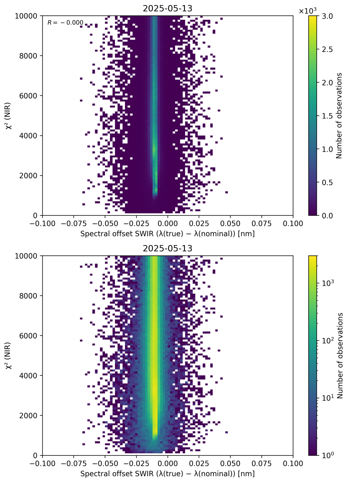
Figure 117: Scatter density plot of “Spectral offset SWIR ( \lambda_{\text{true}} - \lambda_{\text{nominal}} )” against “ \chi^2 (NIR)” for 2025-05-12 to 2025-05-14.
