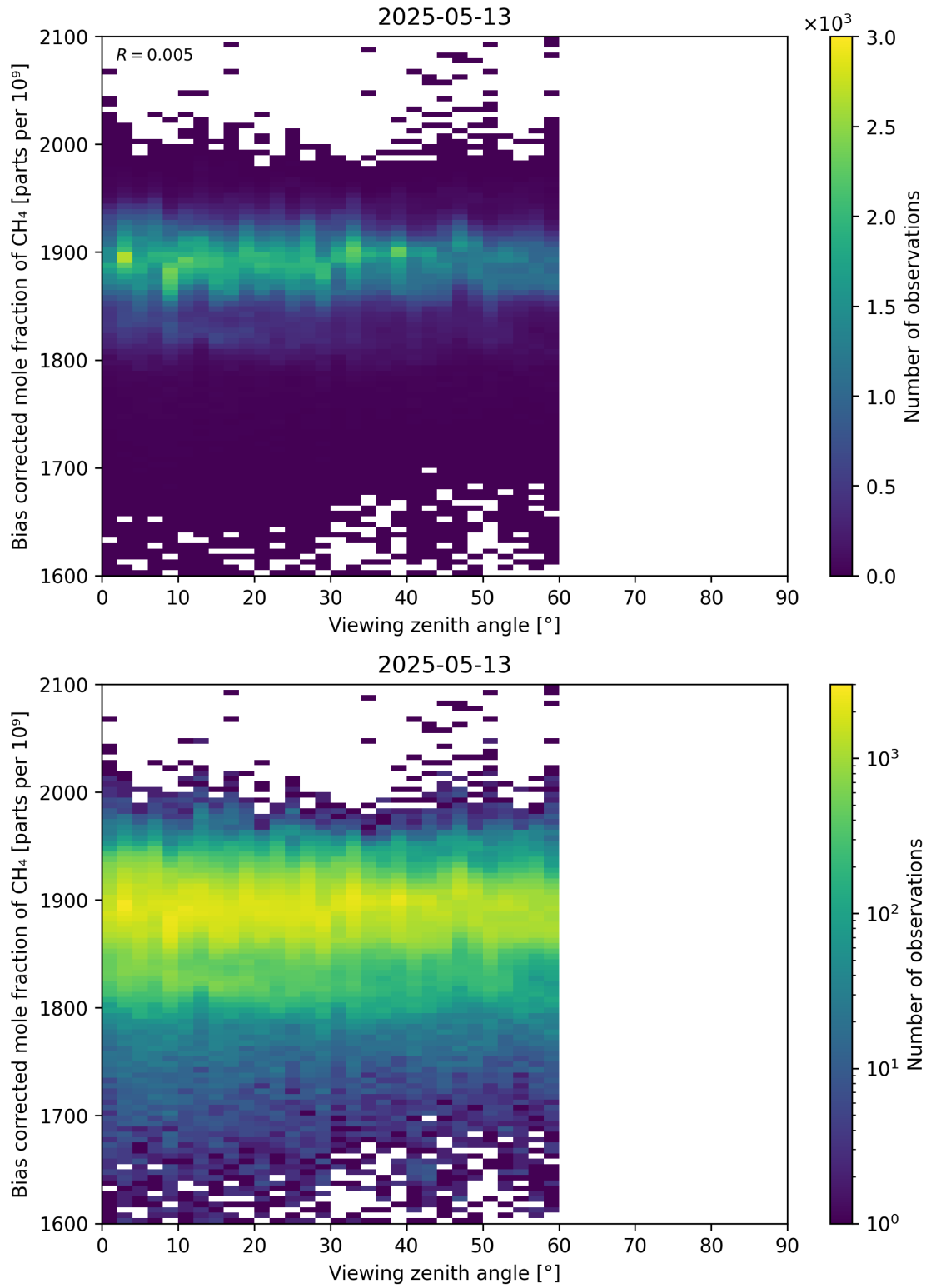
Figure 111: Scatter density plot of “Viewing zenith angle” against “Bias corrected mole fraction of CH 4 ” for 2025-05-12 to 2025-05-14.
