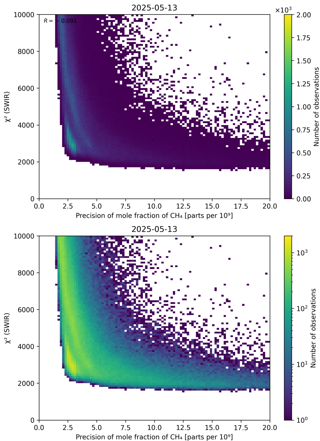
Figure 79: Scatter density plot of “Precision of mole fraction of \text{CH}_4 ” against “ \chi^2 (SWIR)” for 2025-05-12 to 2025-05-14.
