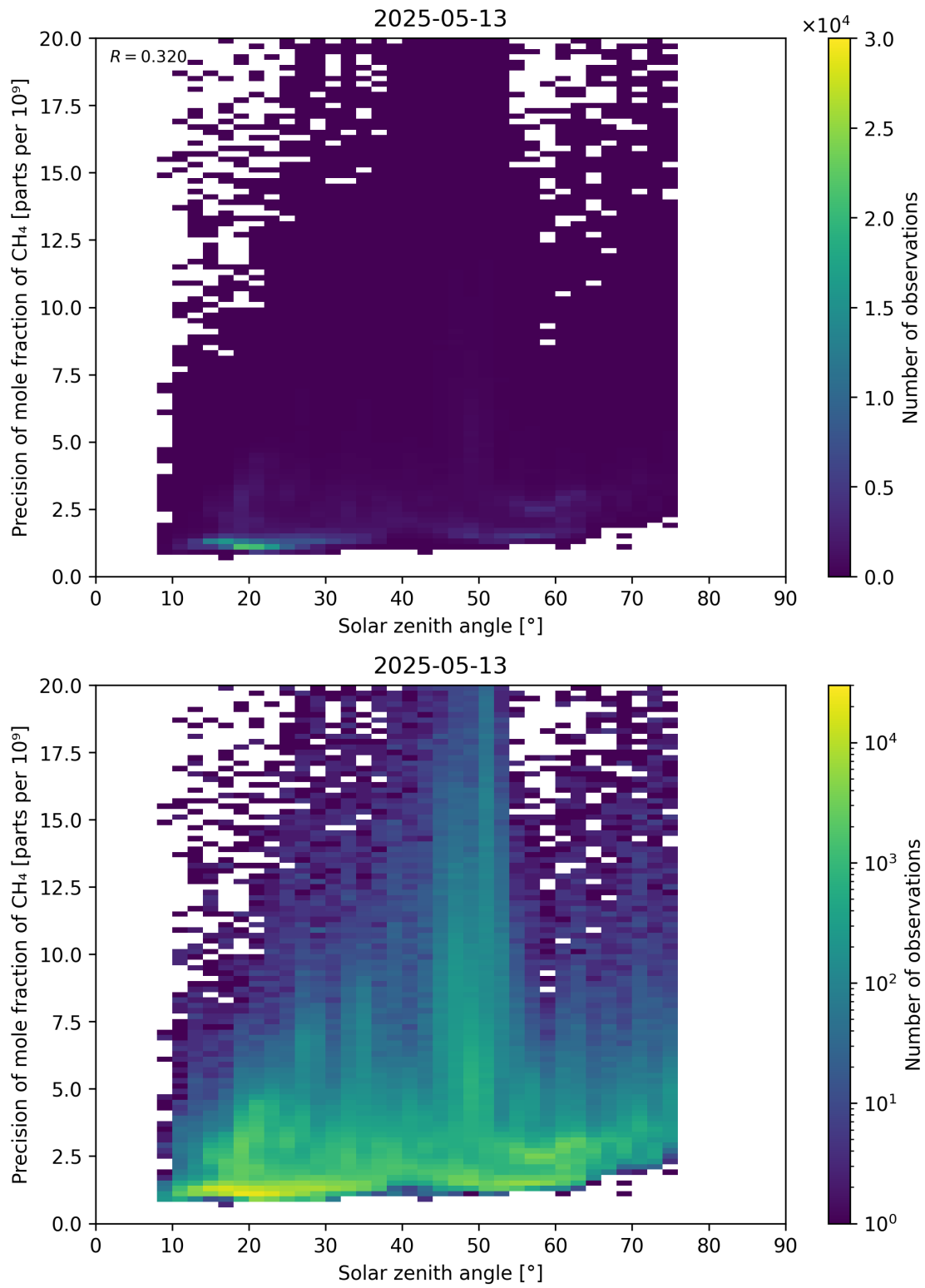
Figure 101: Scatter density plot of “Solar zenith angle” against “Precision of mole fraction of CH 4 ” for 2025-05-12 to 2025-05-14.
