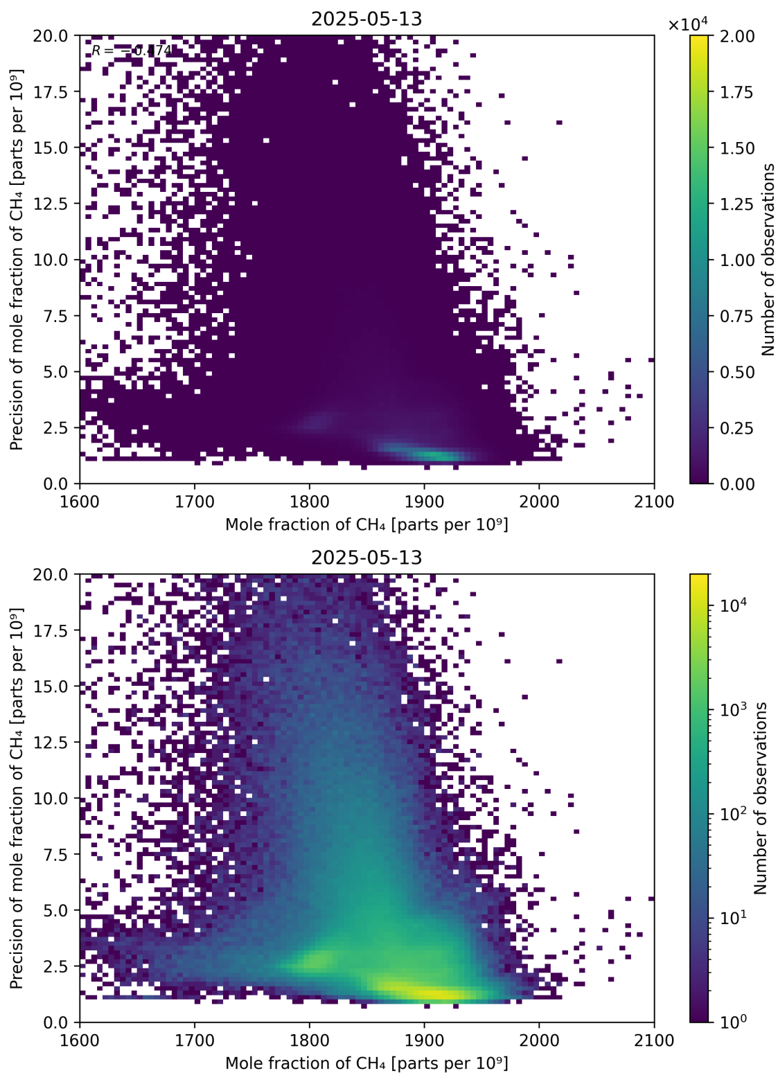
Figure 75: Scatter density plot of “Mole fraction of CH 4 ” against “Precision of mole fraction of CH 4 ” for 2025-05-12 to 2025-05-14.
