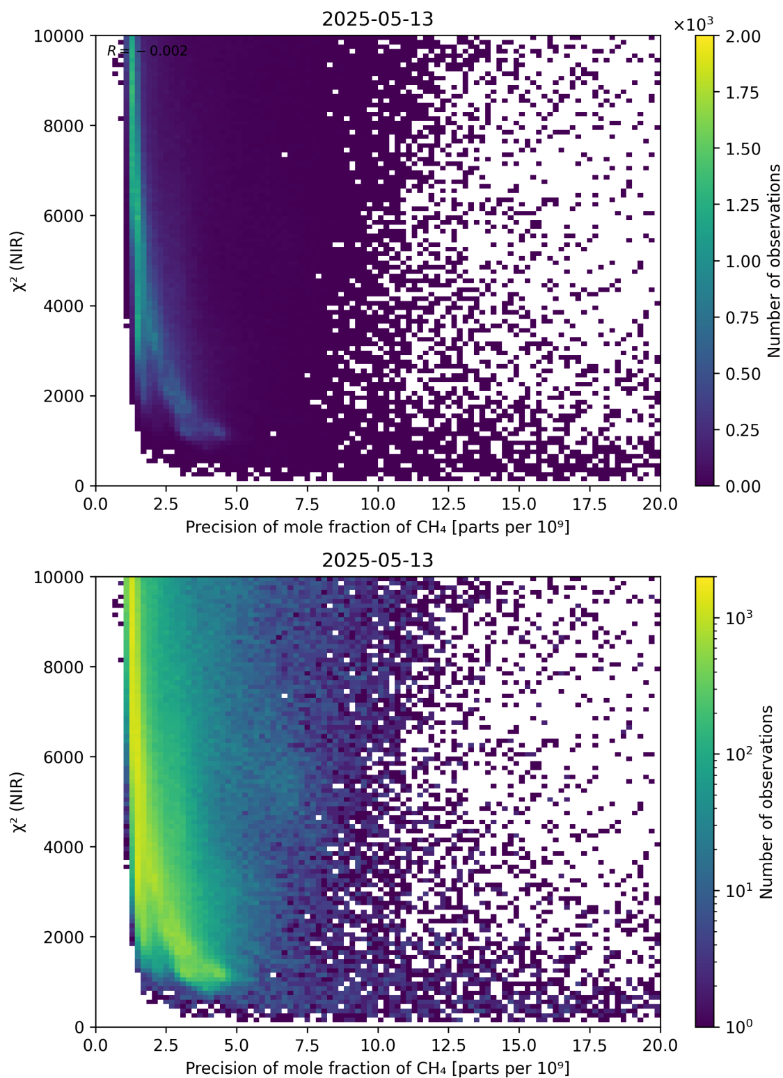
Figure 78: Scatter density plot of “Precision of mole fraction of CH 4 ” against “ \chi^2 (NIR)” for 2025-05-12 to 2025-05-14.
