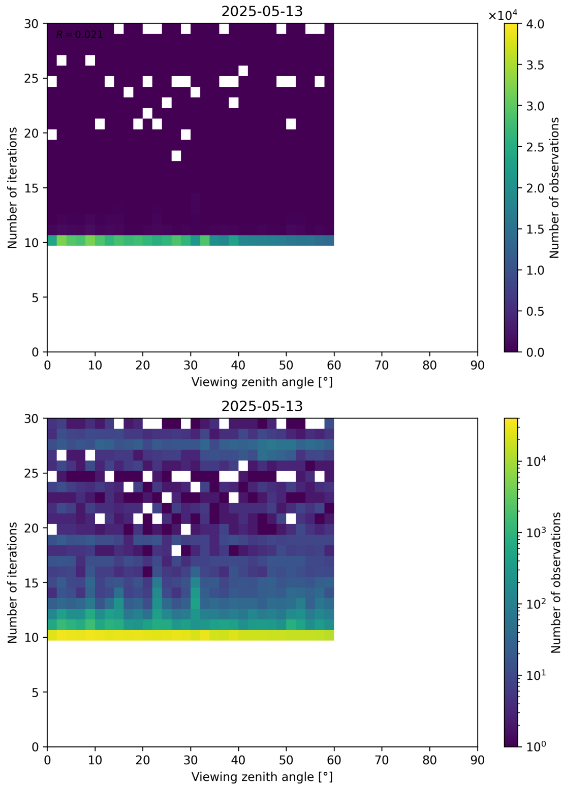
Figure 113: Scatter density plot of “Viewing zenith angle” against “Number of iterations” for 2025-05-12 to 2025-05-14.
