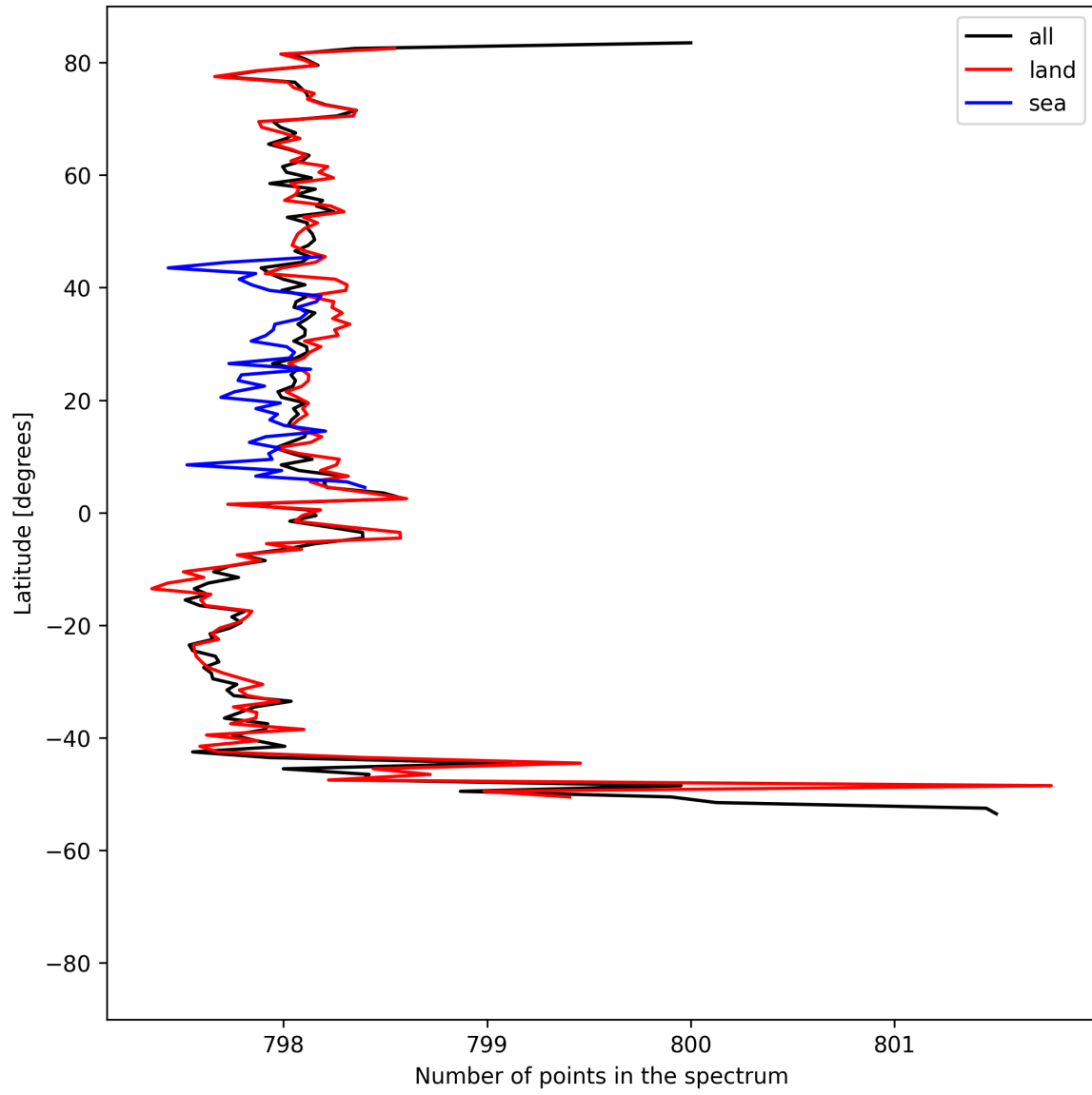
Figure 15: Zonal average of “Number of points in the spectrum” for 2025-05-12 to 2025-05-14.
