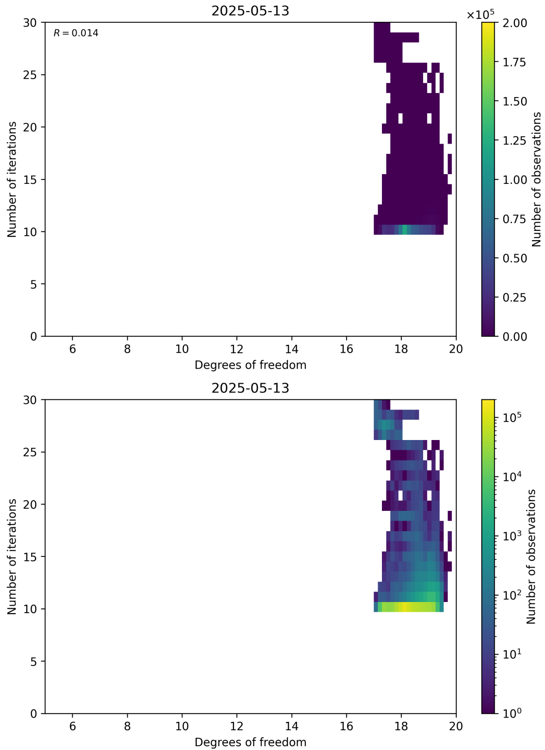
Figure 52: Scatter density plot of “Degrees of freedom” against “Number of iterations” for 2025-05-12 to 2025-05-14.
