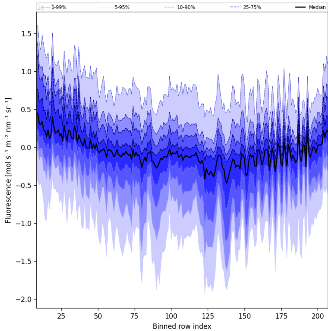
Figure 43: Along track statistics of “Fluorescence” for 2025-05-12 to 2025-05-14
