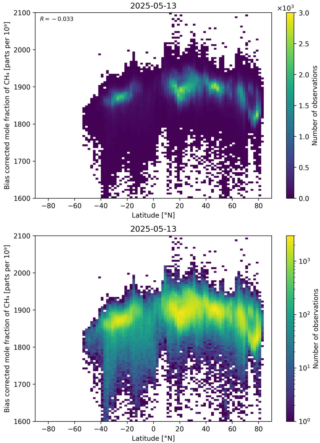
Figure 58: Scatter density plot of “Latitude” against “Bias corrected mole fraction of CH 4 ” for 2025-05-12 to 2025-05-14.
