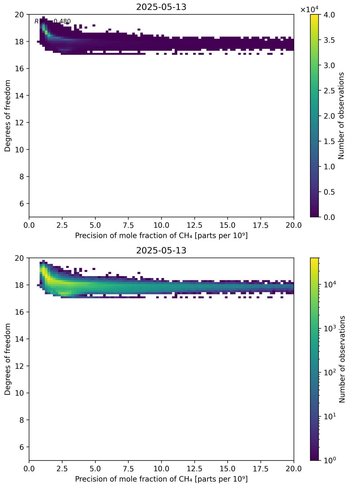
Figure 80: Scatter density plot of “Precision of mole fraction of CH 4 ” against “Degrees of freedom” for 2025-05-12 to 2025-05-14.
