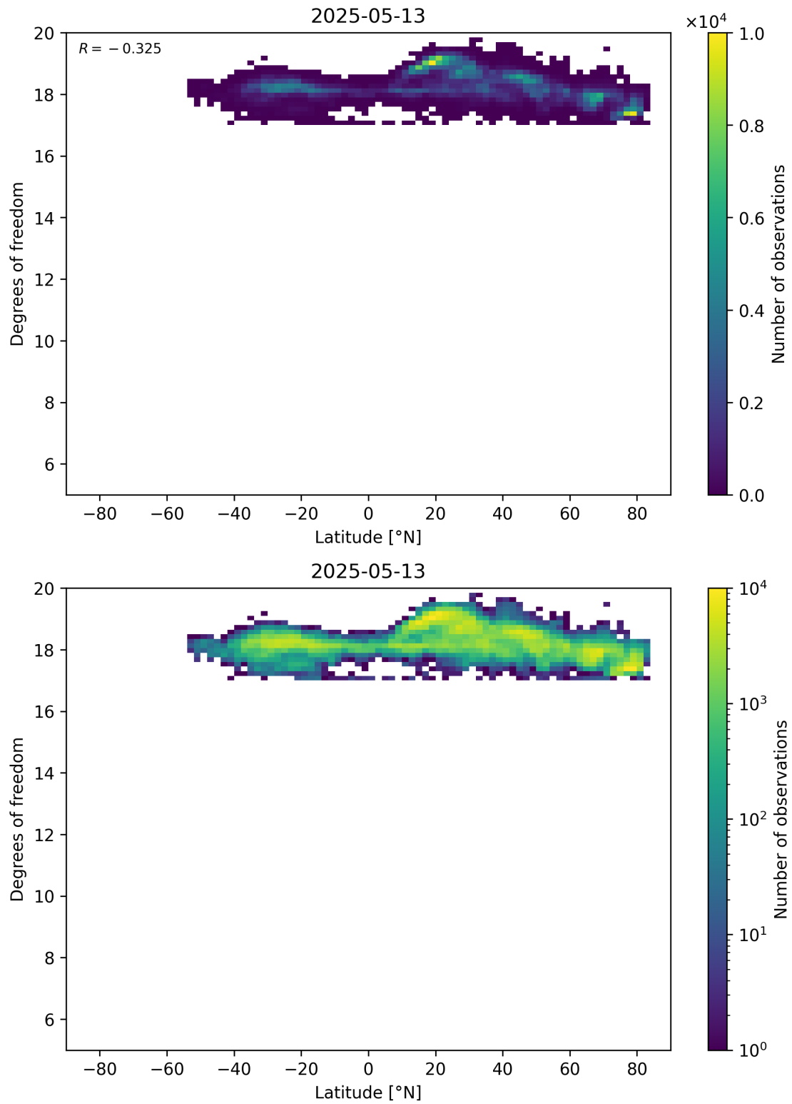
Figure 55: Scatter density plot of “Latitude” against “Degrees of freedom” for 2025-05-12 to 2025-05-14.
