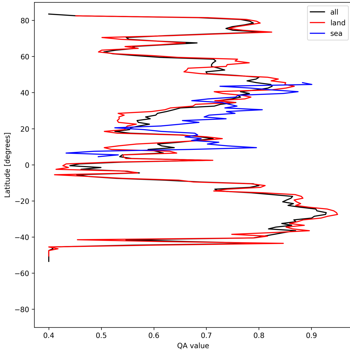
Figure 11: Zonal average of “QA value” for 2025-05-12 to 2025-05-14.
