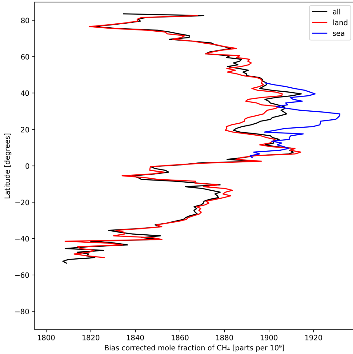
Figure 14: Zonal average of “Bias corrected mole fraction of \text{CH}_4 ” for 2025-05-12 to 2025-05-14.
