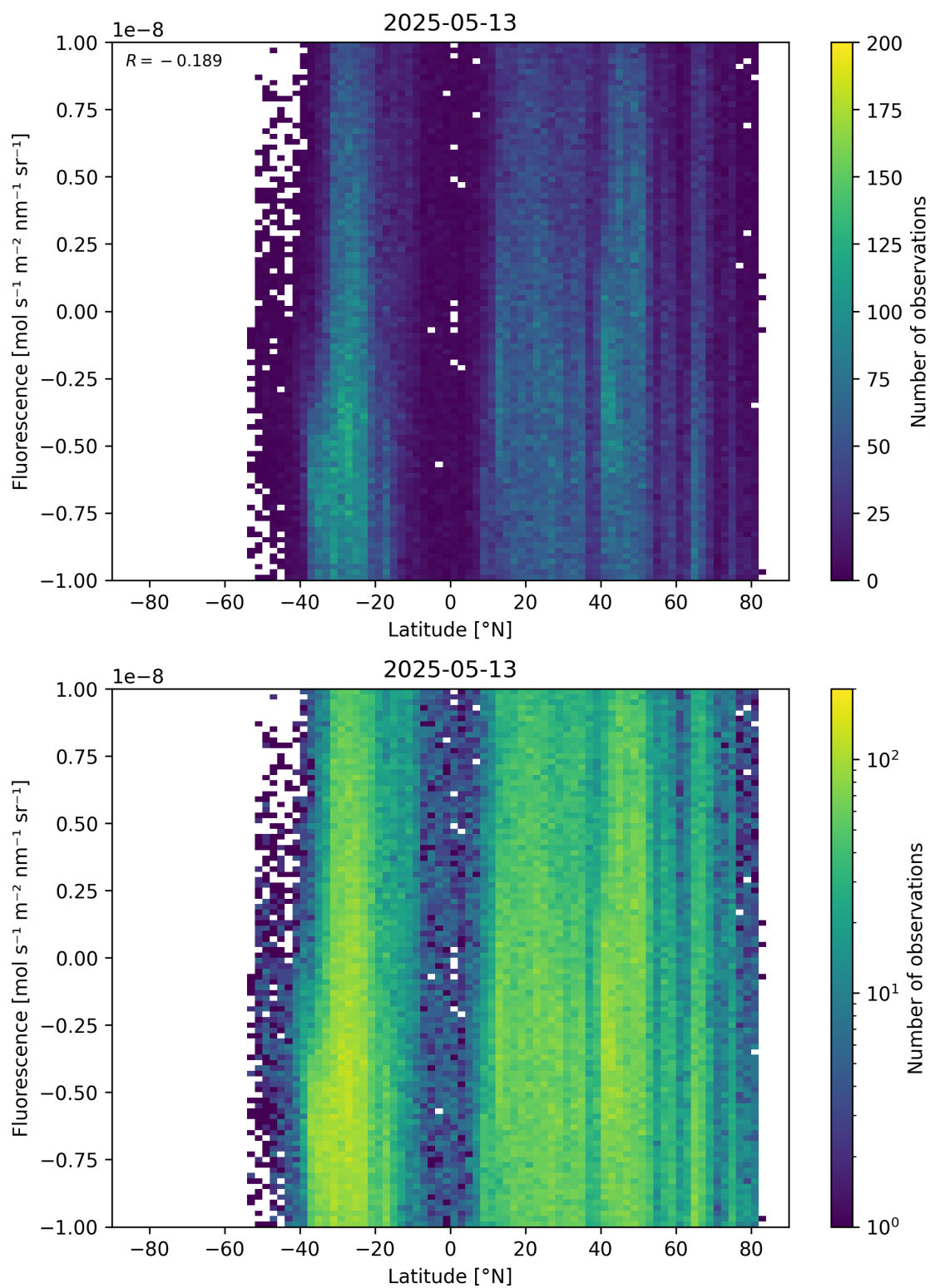
Figure 56: Scatter density plot of “Latitude” against “Fluorescence” for 2025-05-12 to 2025-05-14.
