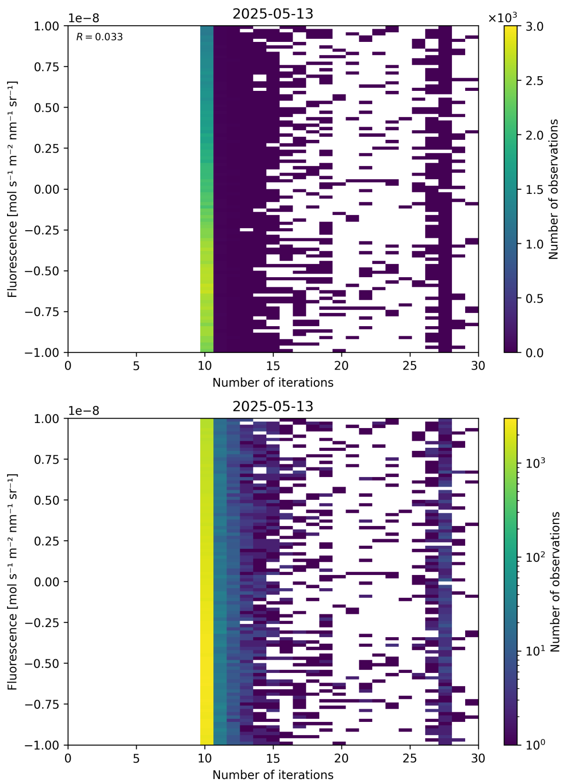
Figure 87: Scatter density plot of “Number of iterations” against “Fluorescence” for 2025-05-12 to 2025-05-14.
