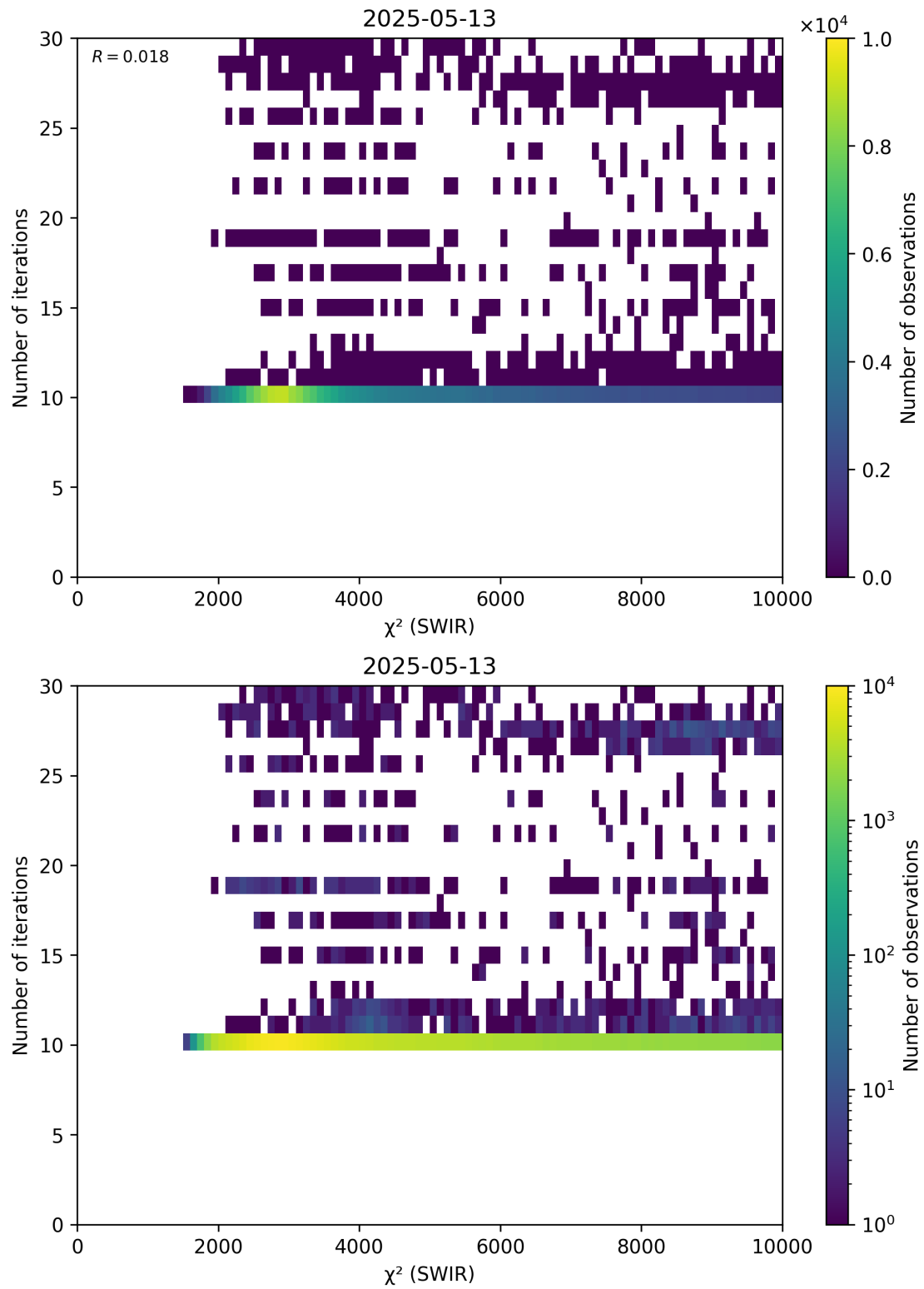
Figure 50: Scatter density plot of “ \chi^2 (SWIR)” against “Number of iterations” for 2025-05-12 to 2025-05-14.
