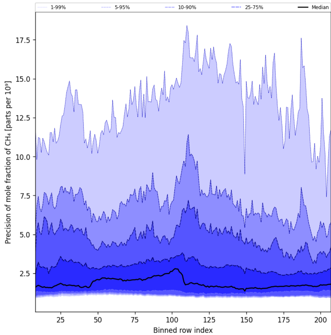
Figure 35: Along track statistics of “Precision of mole fraction of CH 4 ” for 2025-05-12 to 2025-05-14
