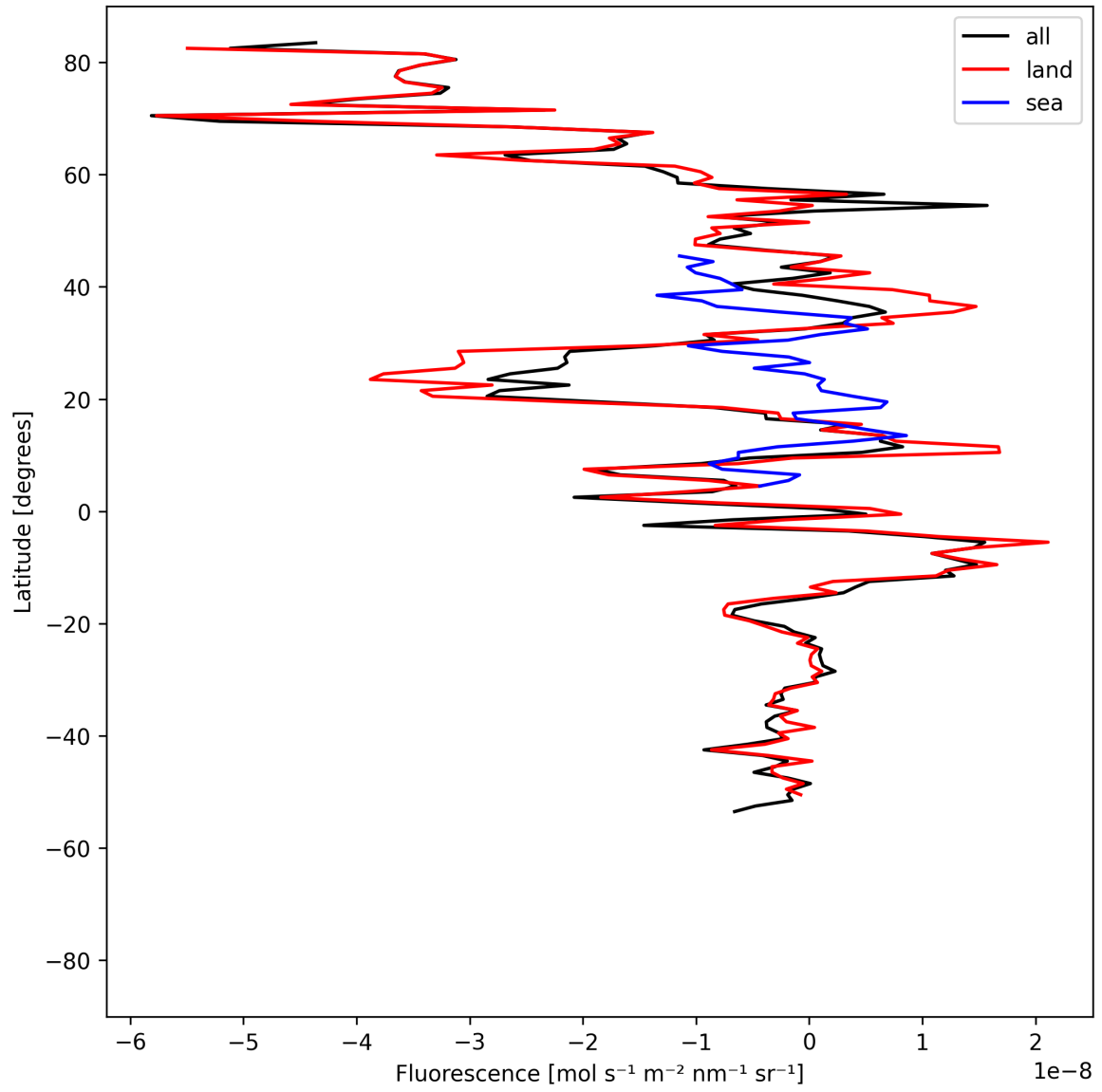
Figure 21: Zonal average of “Fluorescence” for 2025-05-12 to 2025-05-14.
