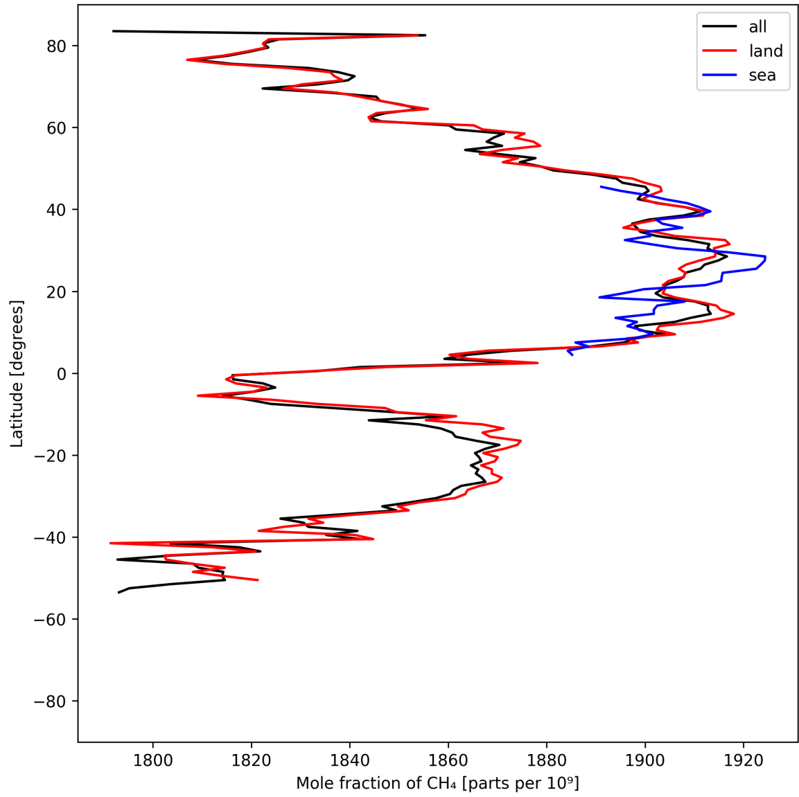
Figure 12: Zonal average of “Mole fraction of \text{CH}_4 ” for 2025-05-12 to 2025-05-14.
