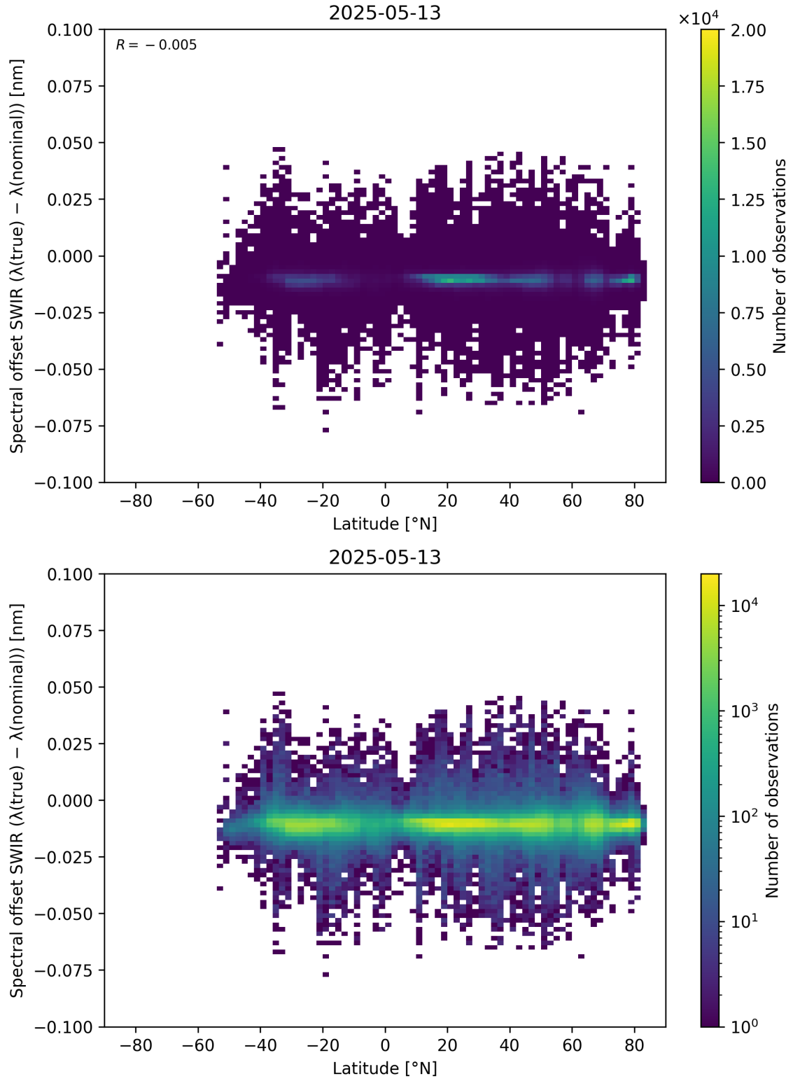
Figure 62: Scatter density plot of “Latitude” against “Spectral offset SWIR ( \lambda_{\text{true}} - \lambda_{\text{nominal}} )” for 2025-05-12 to 2025-05-14.
