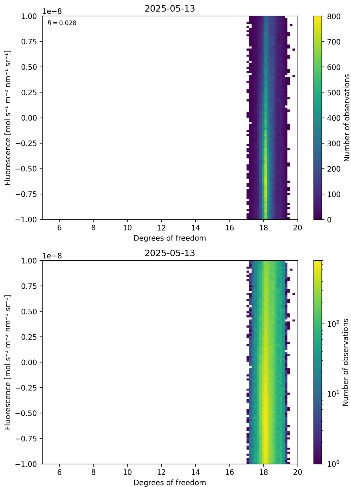
Figure 51: Scatter density plot of “Degrees of freedom” against “Fluorescence” for 2025-05-12 to 2025-05-14.
