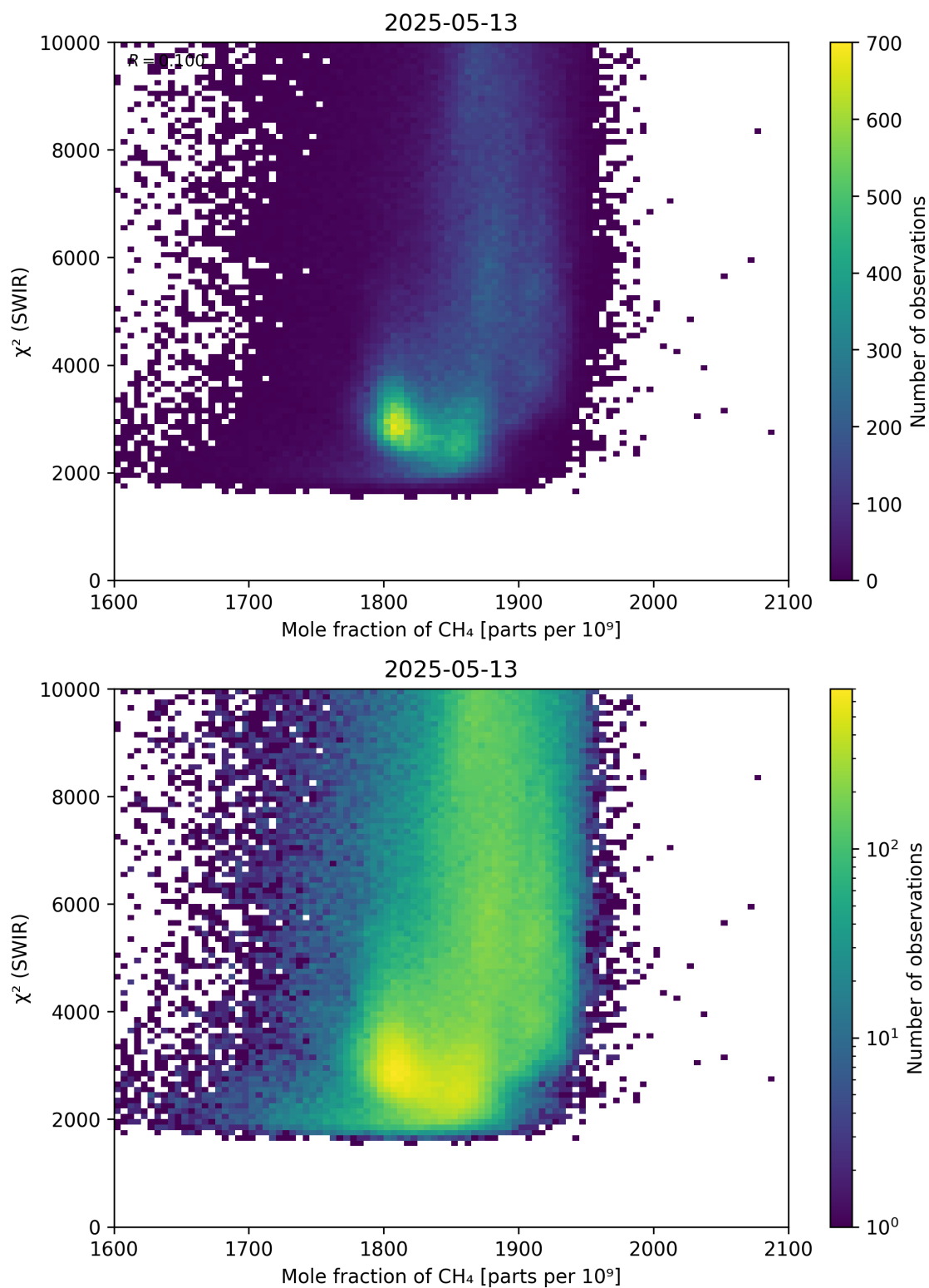
Figure 71: Scatter density plot of “Mole fraction of CH 4 ” against “ \chi^2 (SWIR)” for 2025-05-12 to 2025-05-14.
