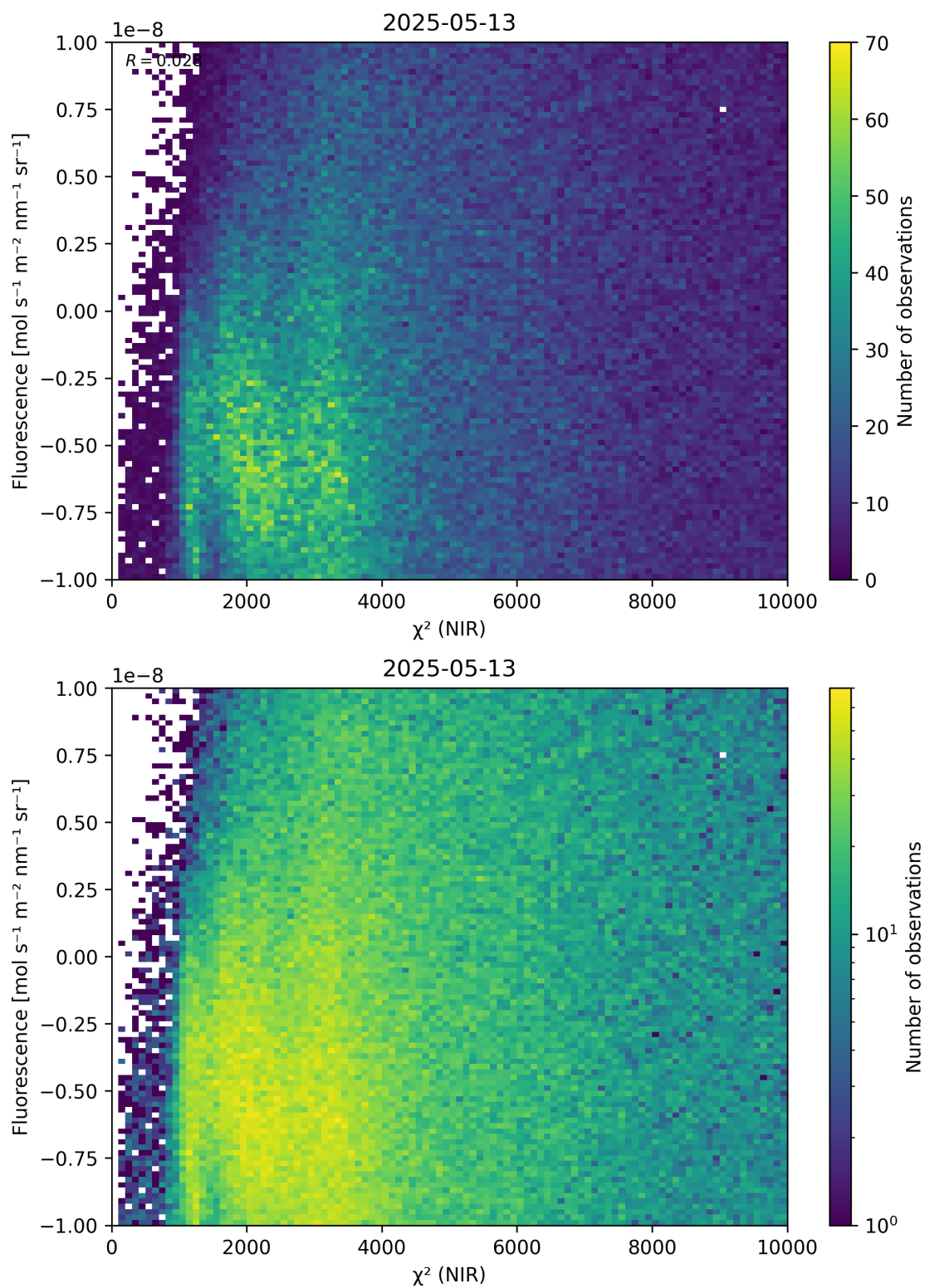
Figure 45: Scatter density plot of “ \chi^2 (NIR)” against “Fluorescence” for 2025-05-12 to 2025-05-14.
