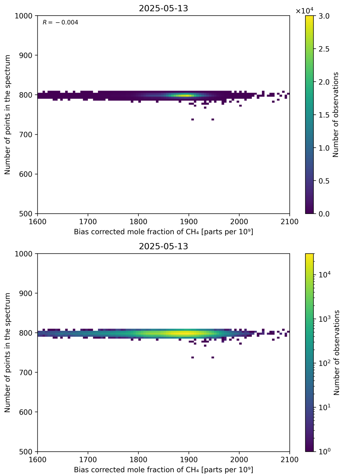
Figure 68: Scatter density plot of “Bias corrected mole fraction of CH 4 ” against “Number of points in the spectrum” for 2025-05-12 to 2025-05-14.
