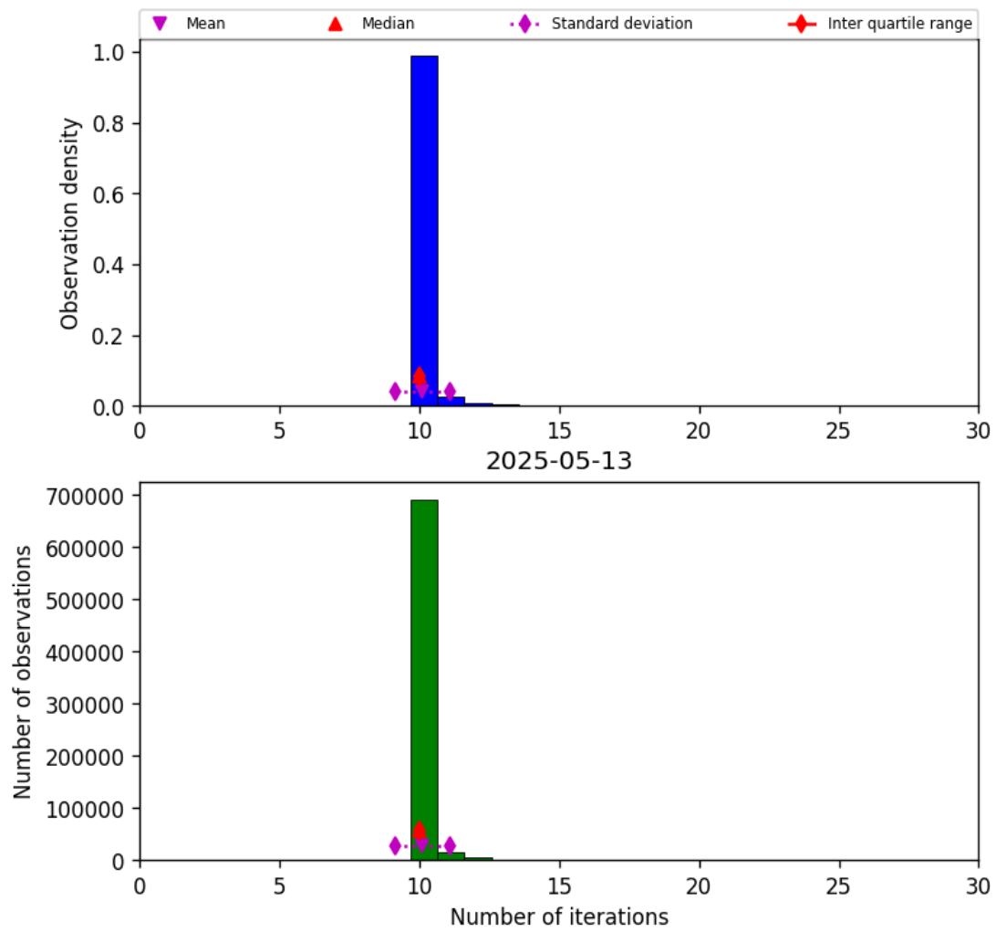
Figure 31: Histogram of “Number of iterations” for 2025-05-12 to 2025-05-14
