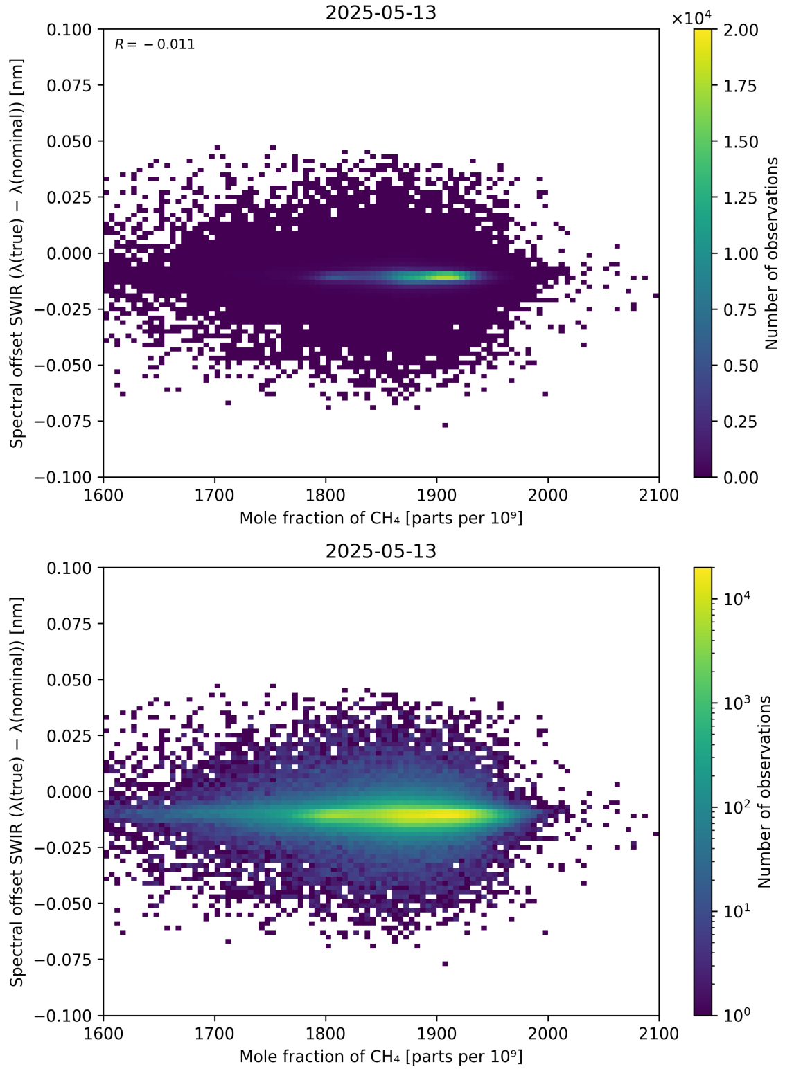
Figure 86: Scatter density plot of “Mole fraction of CH 4 ” against “Spectral offset SWIR ( \lambda_{\text{true}} - \lambda_{\text{nominal}} )” for 2025-05-12 to 2025-05-14.
