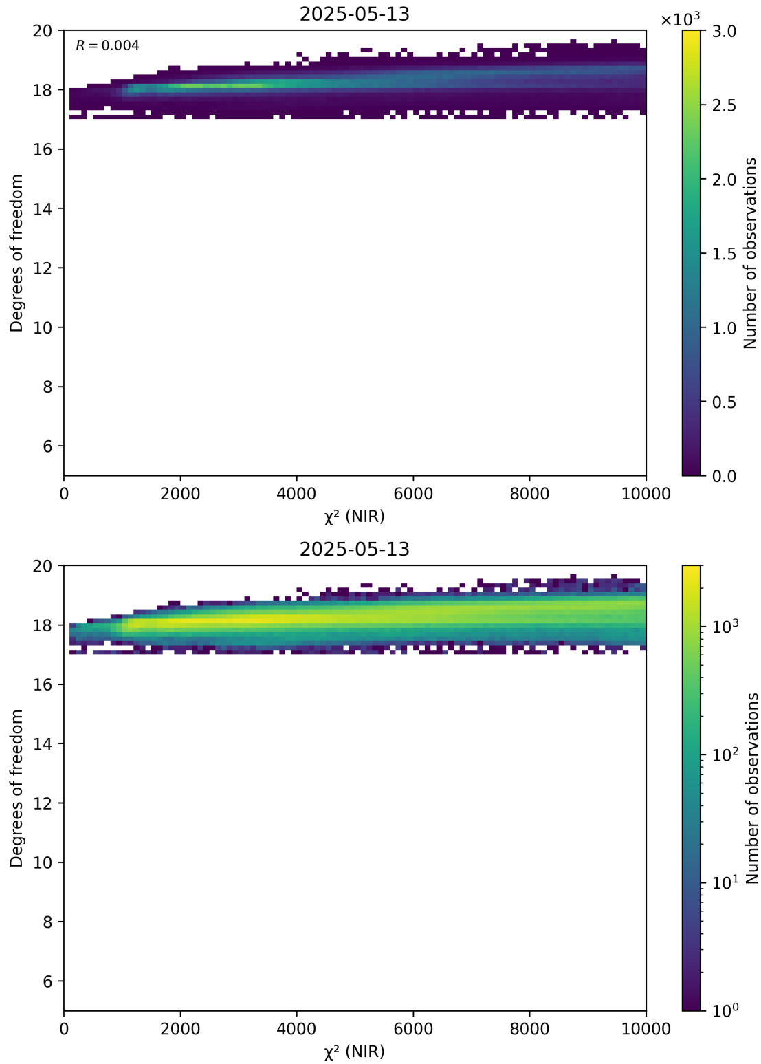
Figure 44: Scatter density plot of “ \chi^2 (NIR)” against “Degrees of freedom” for 2025-05-12 to 2025-05-14.
