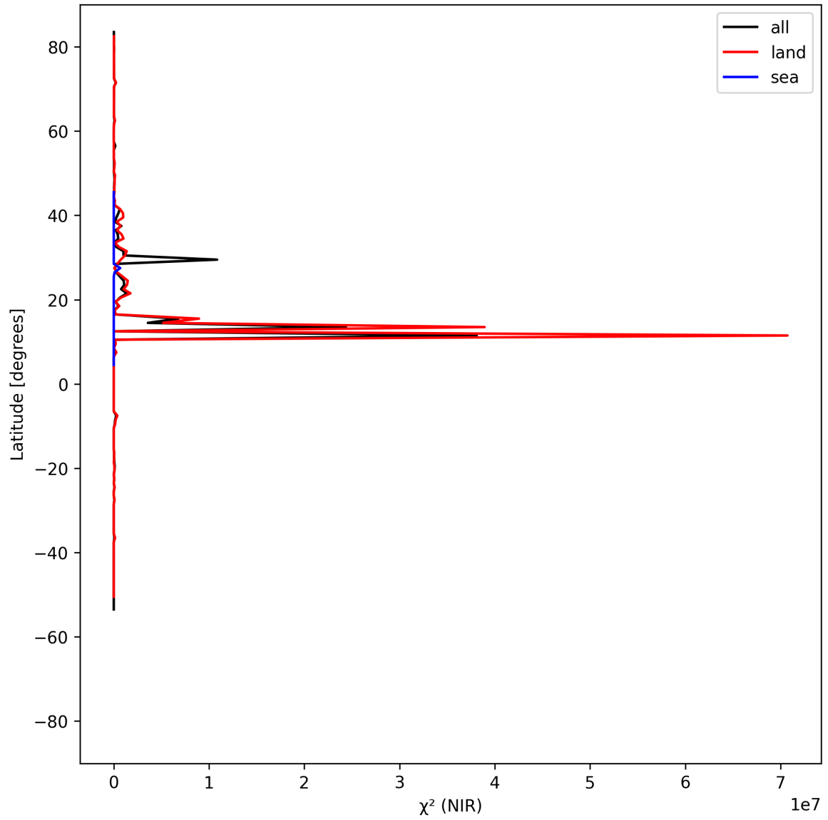
Figure 18: Zonal average of “ \chi^2 (NIR)” for 2025-05-12 to 2025-05-14.
