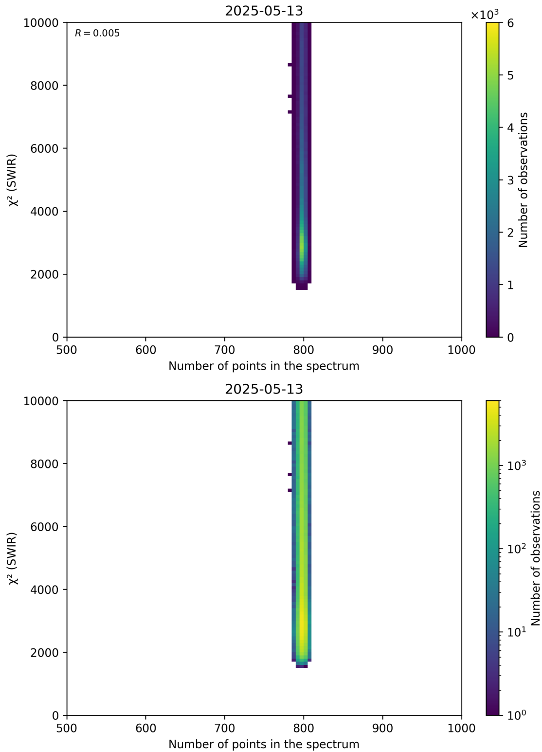
Figure 89: Scatter density plot of “Number of points in the spectrum” against “ \chi^2 (SWIR)” for 2025-05-12 to 2025-05-14.
