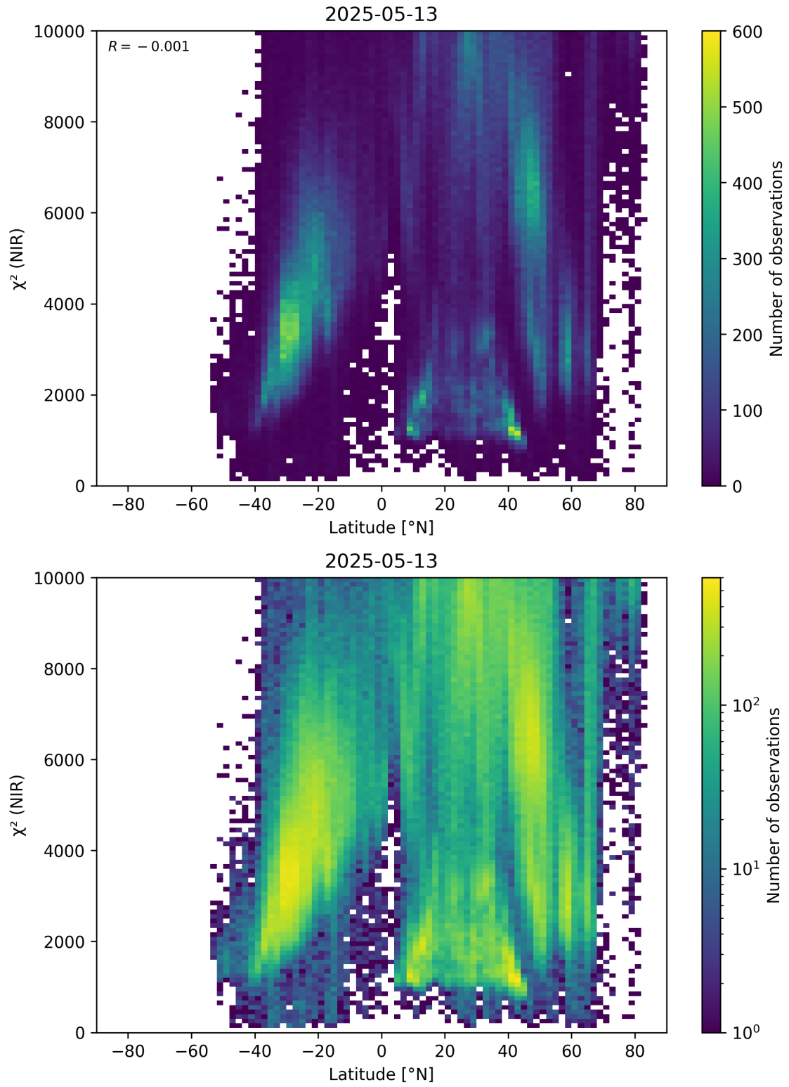
Figure 53: Scatter density plot of “Latitude” against “ \chi^2 (NIR)” for 2025-05-12 to 2025-05-14.
