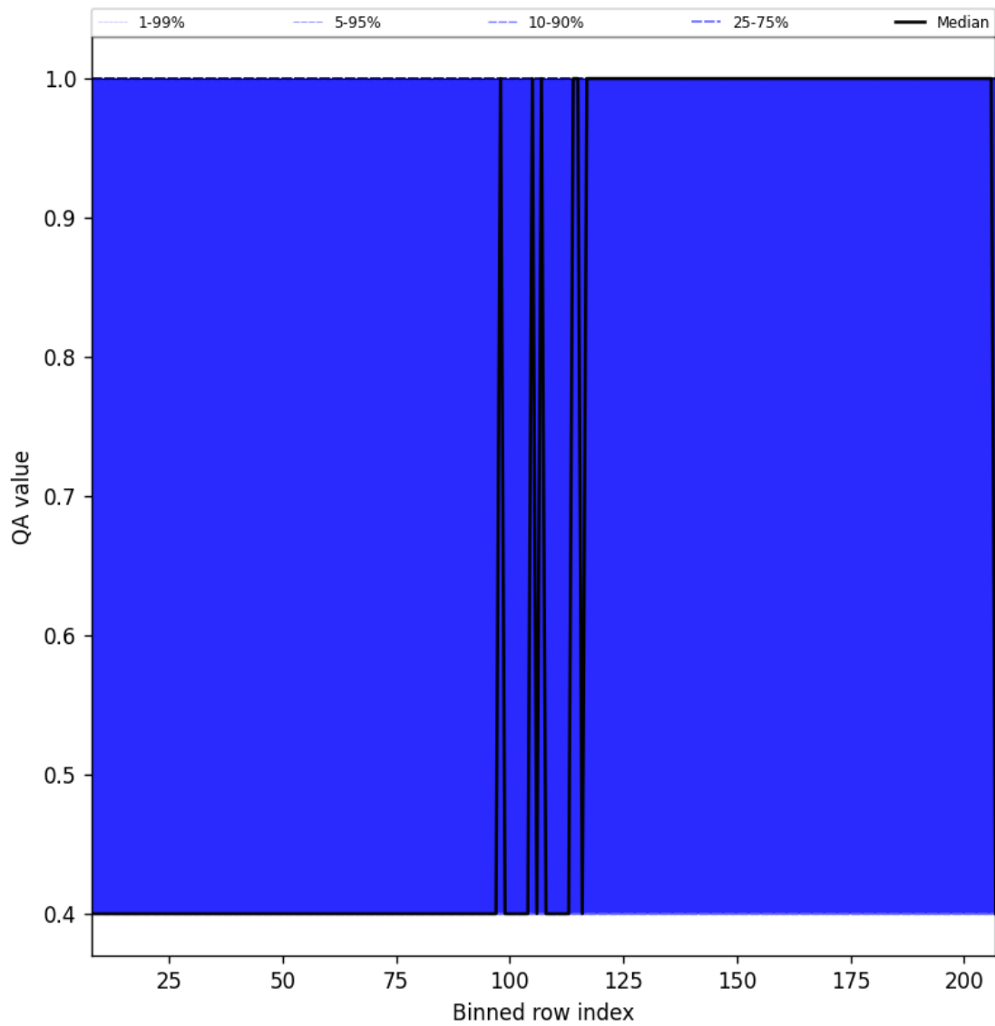
Figure 33: Along track statistics of “QA value” for 2025-05-12 to 2025-05-14
