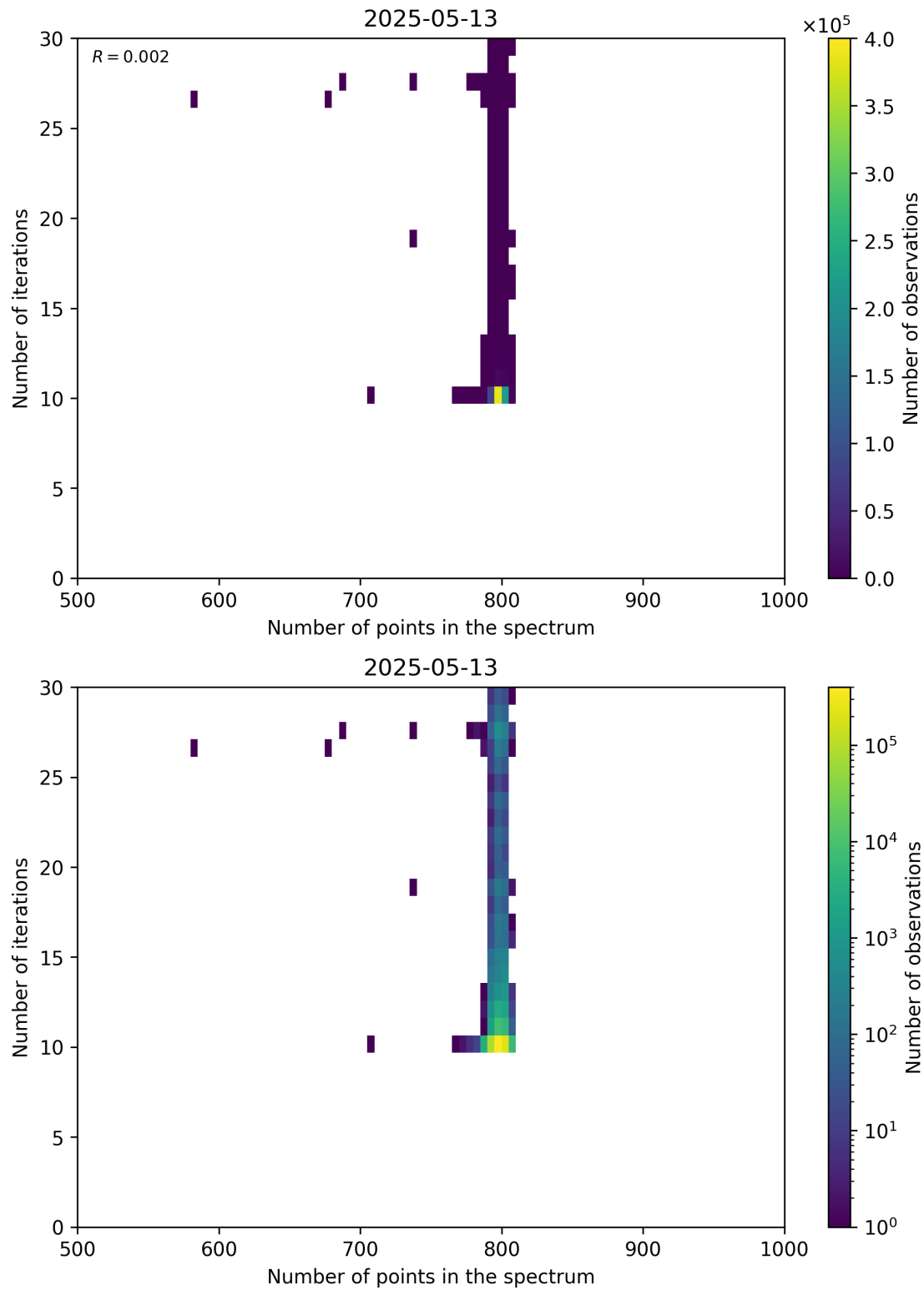
Figure 92: Scatter density plot of “Number of points in the spectrum” against “Number of iterations” for 2025-05-12 to 2025-05-14.
