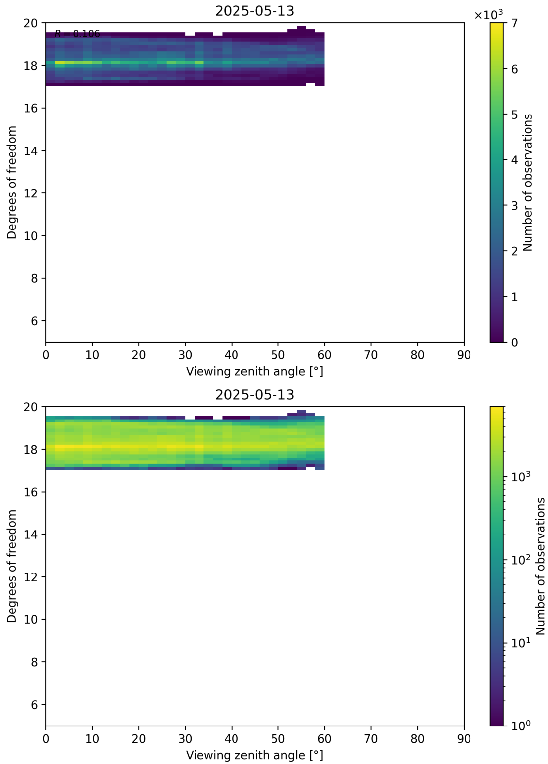
Figure 107: Scatter density plot of “Viewing zenith angle” against “Degrees of freedom” for 2025-05-12 to 2025-05-14.
