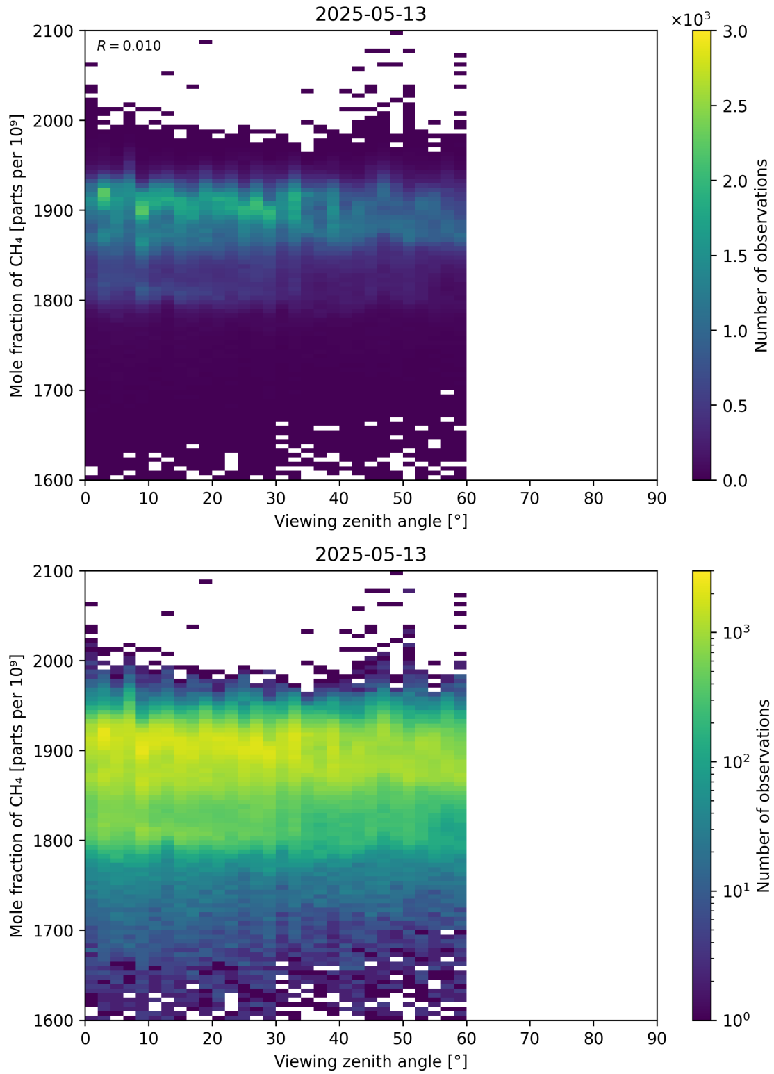
Figure 110: Scatter density plot of “Viewing zenith angle” against “Mole fraction of CH 4 ” for 2025-05-12 to 2025-05-14.
