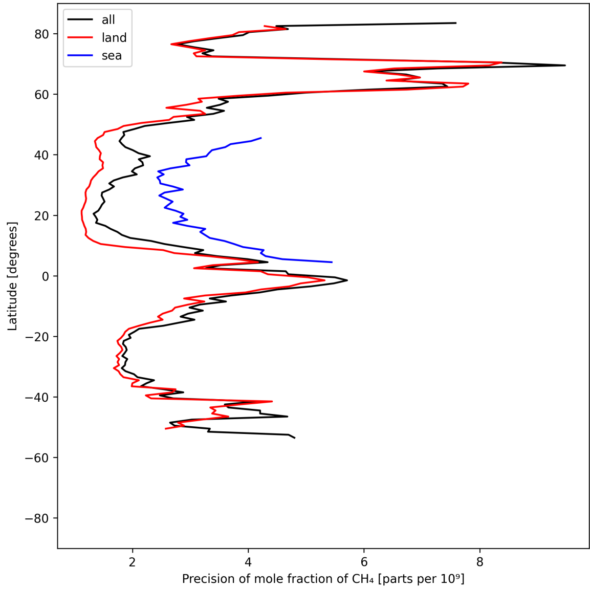
Figure 13: Zonal average of “Precision of mole fraction of CH 4 ” for 2025-05-12 to 2025-05-14.
