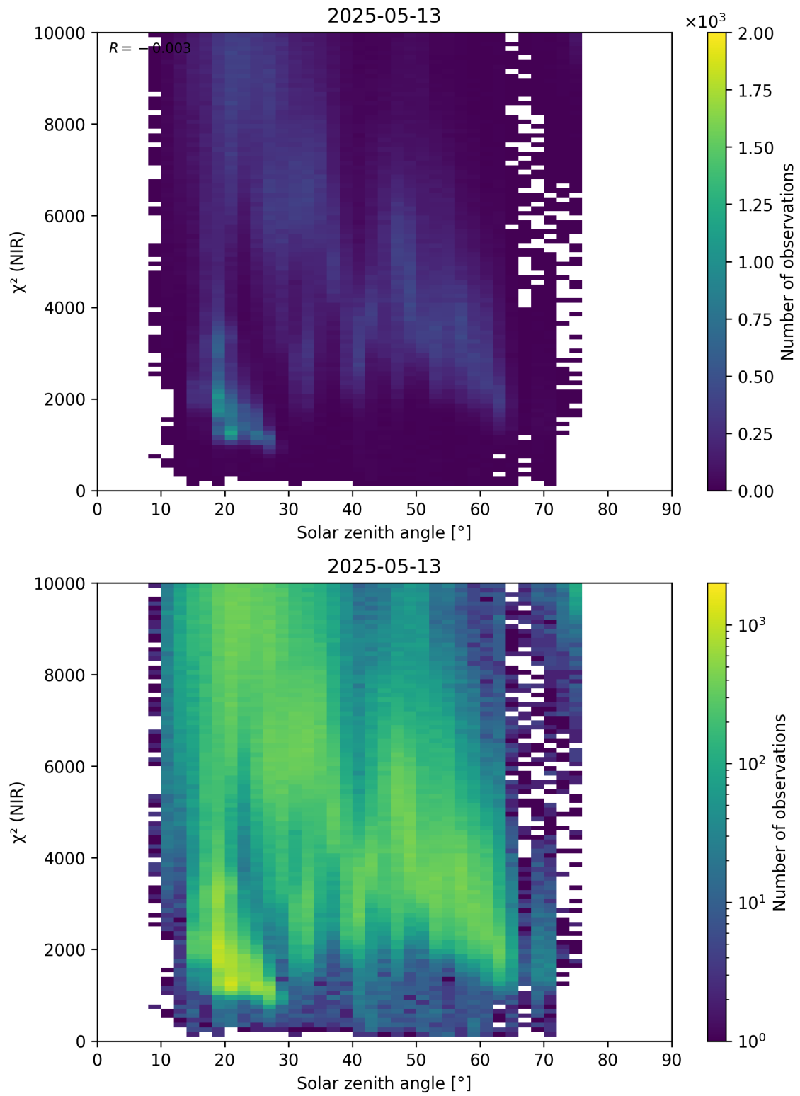
Figure 94: Scatter density plot of “Solar zenith angle” against “ \chi^2 (NIR)” for 2025-05-12 to 2025-05-14.
