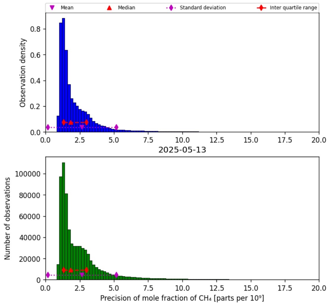
Figure 24: Histogram of “Precision of mole fraction of CH 4 ” for 2025-05-12 to 2025-05-14
