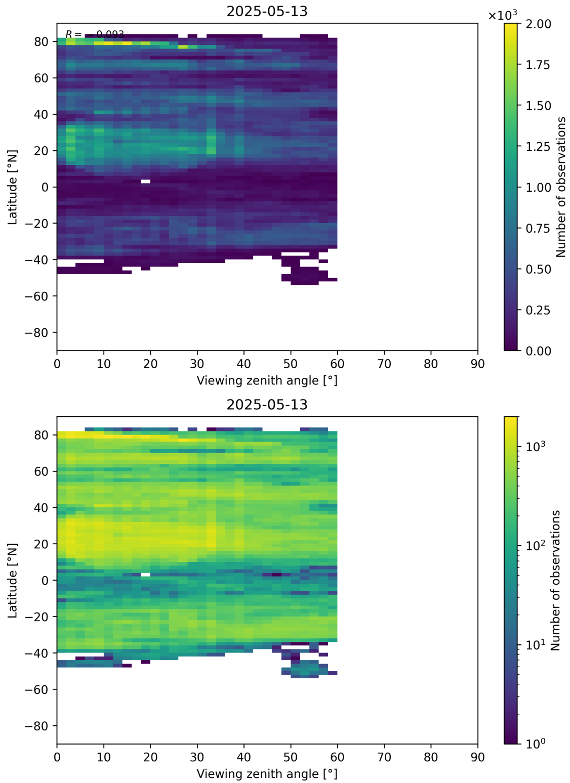
Figure 109: Scatter density plot of “Viewing zenith angle” against “Latitude” for 2025-05-12 to 2025-05-14.
