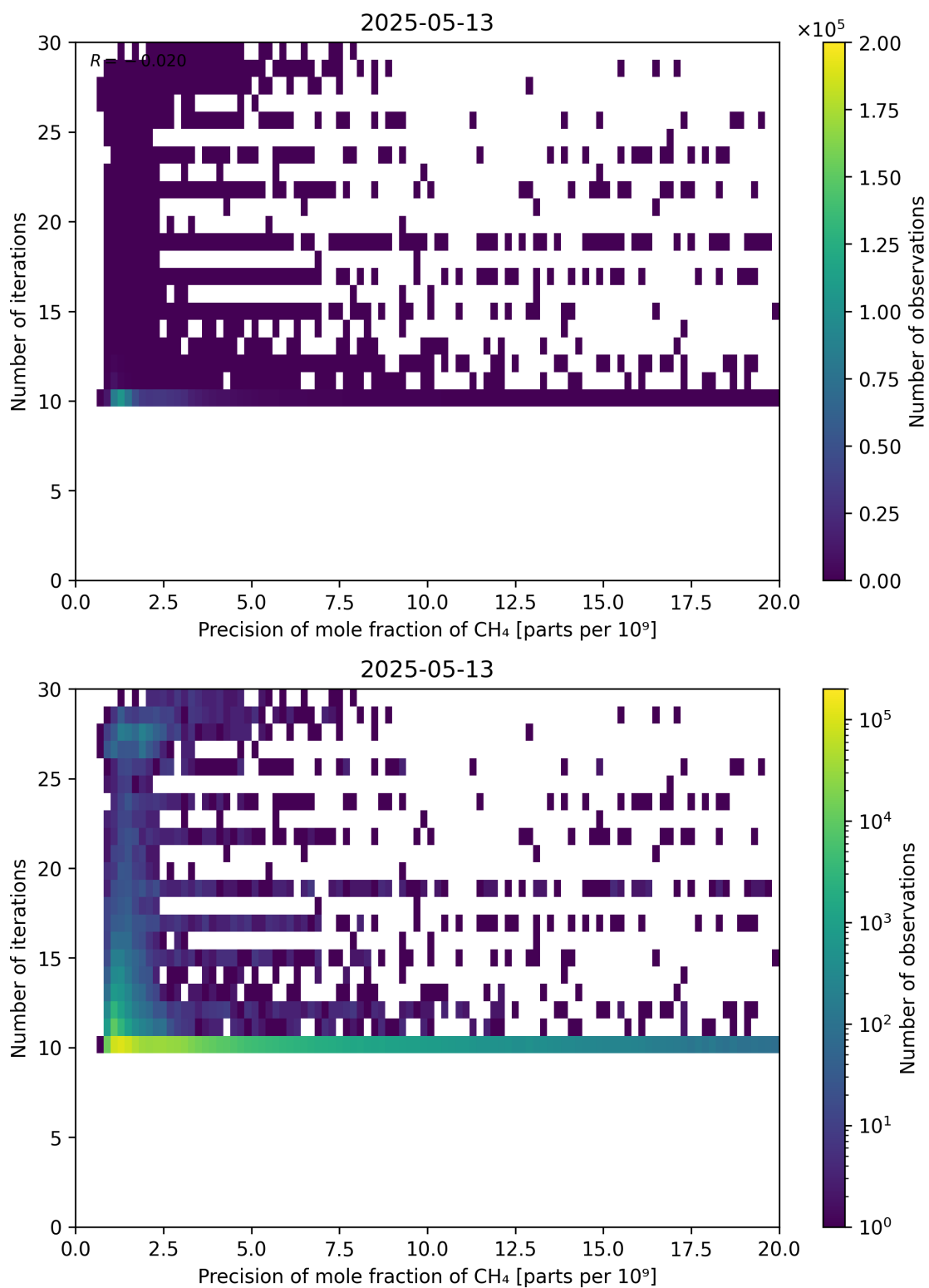
Figure 83: Scatter density plot of “Precision of mole fraction of CH 4 ” against “Number of iterations” for 2025-05-12 to 2025-05-14.
