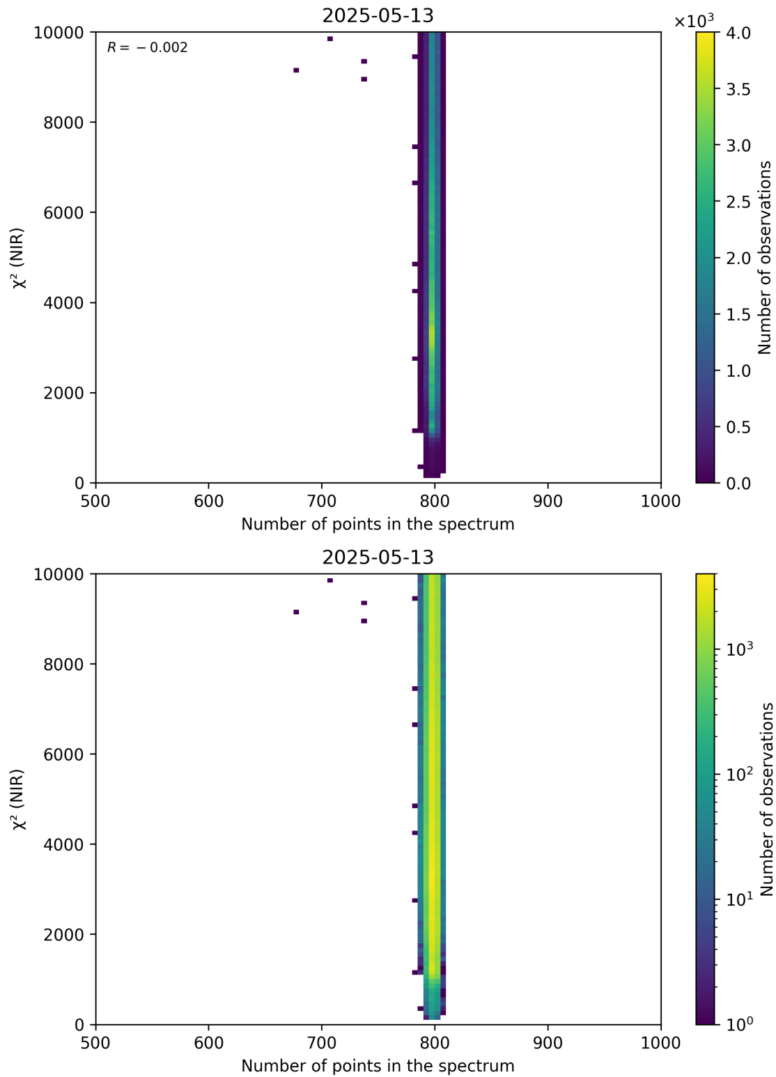
Figure 88: Scatter density plot of “Number of points in the spectrum” against “ \chi^2 (NIR)” for 2025-05-12 to 2025-05-14.
