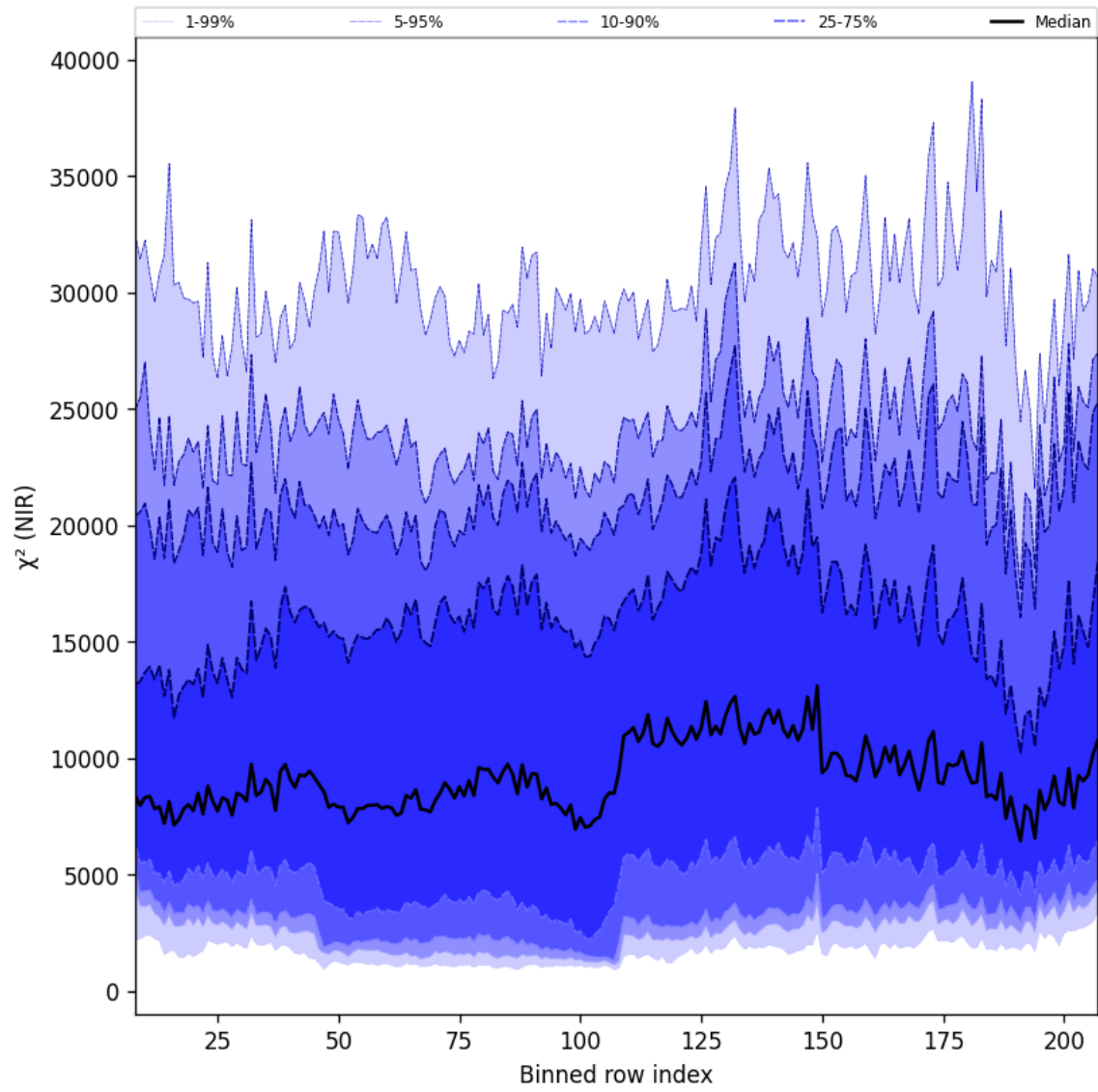
Figure 40: Along track statistics of “ \chi^2 (NIR)” for 2025-05-12 to 2025-05-14
