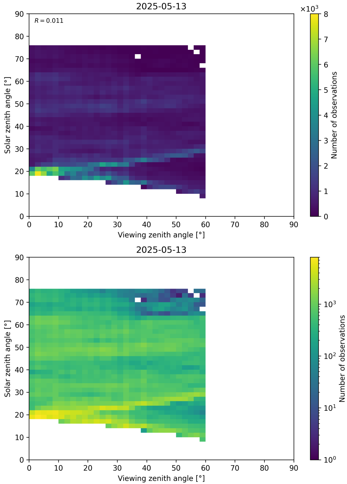
Figure 115: Scatter density plot of “Viewing zenith angle” against “Solar zenith angle” for 2025-05-12 to 2025-05-14.
