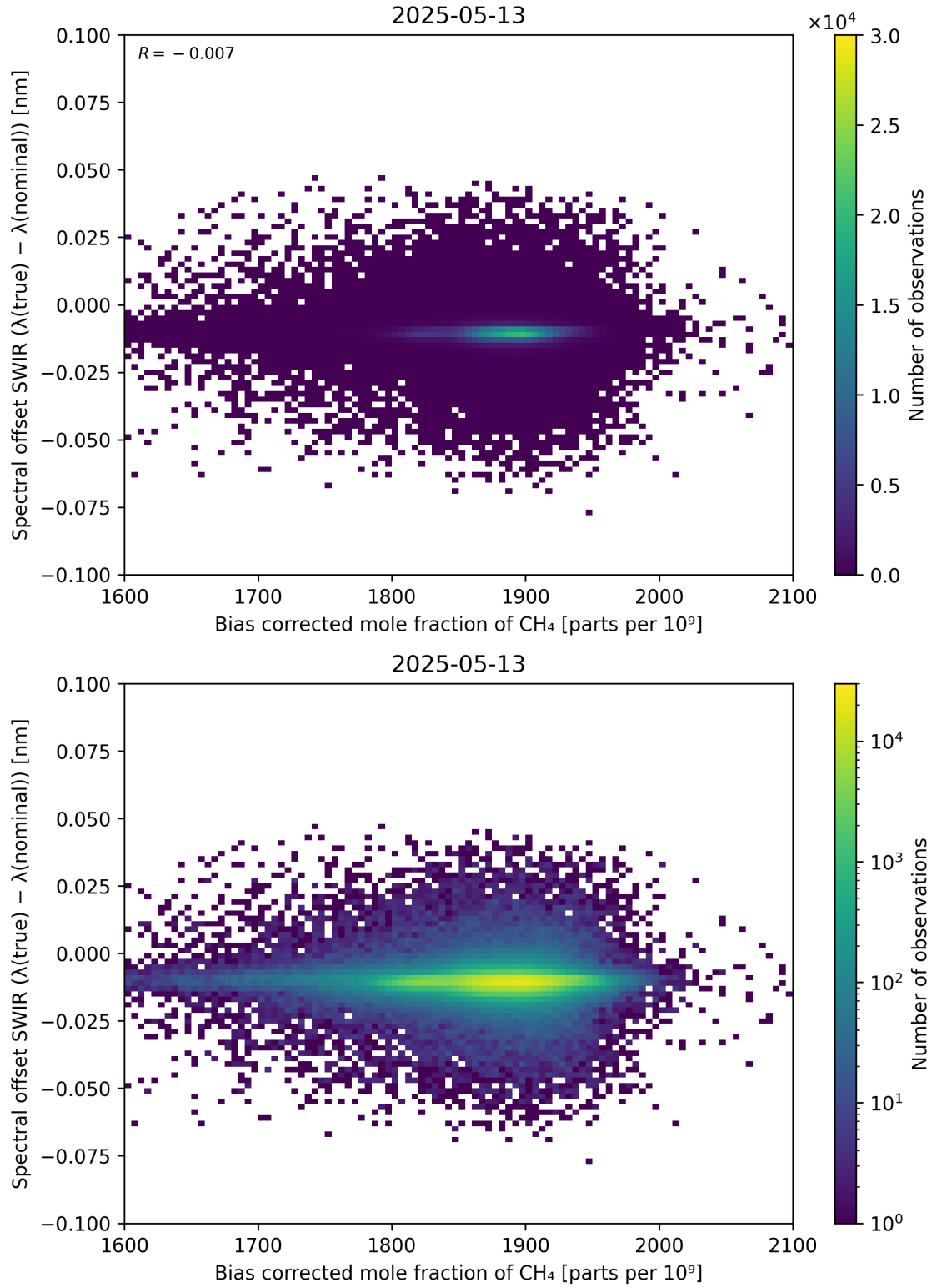
Figure 69: Scatter density plot of “Bias corrected mole fraction of CH 4 ” against “Spectral offset SWIR ( \lambda_{\text{true}} - \lambda_{\text{nominal}} )” for 2025-05-12 to 2025-05-14.
