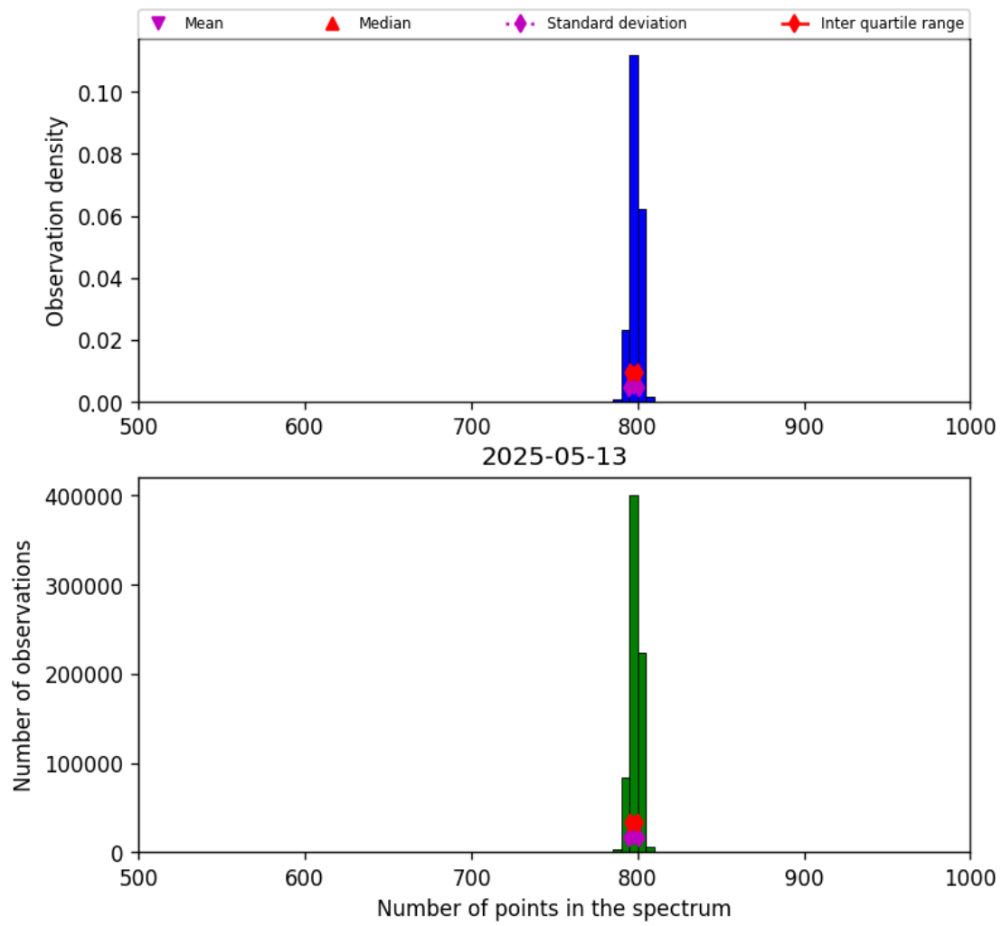
Figure 26: Histogram of “Number of points in the spectrum” for 2025-05-12 to 2025-05-14
