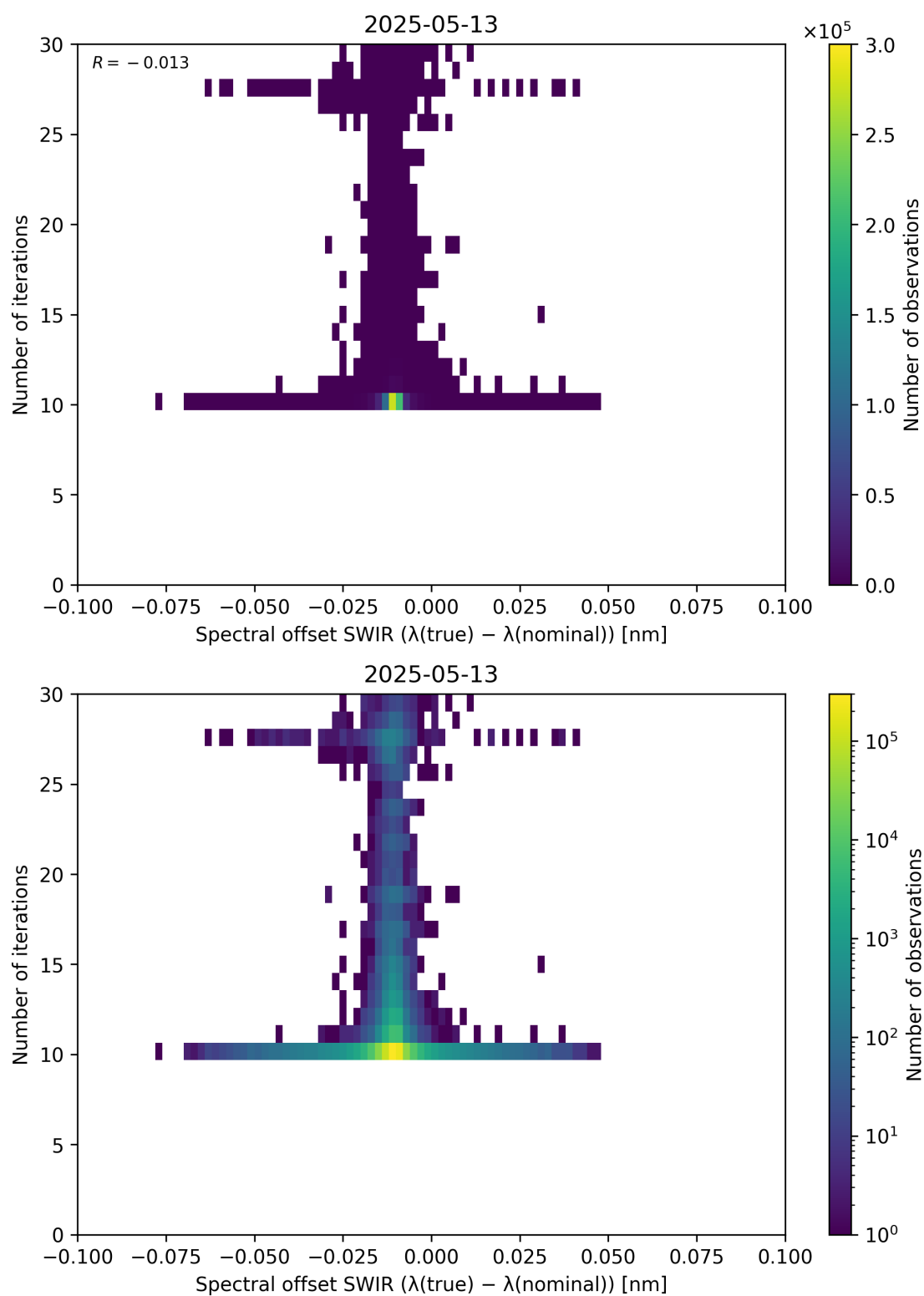
Figure 121: Scatter density plot of “Spectral offset SWIR ( \lambda_{\text{true}} - \lambda_{\text{nominal}} )” against “Number of iterations” for 2025-05-12 to 2025-05-14.
