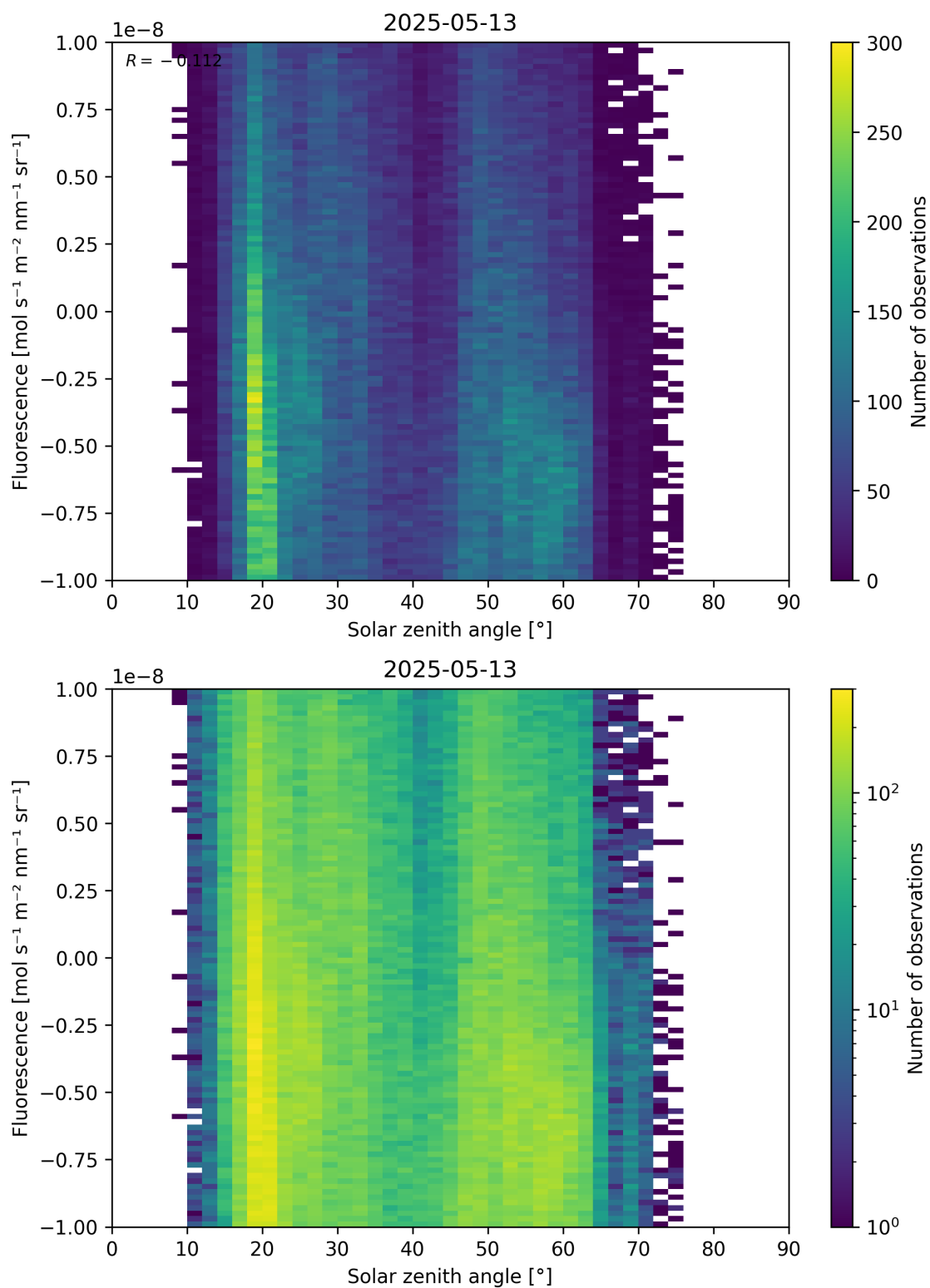
Figure 97: Scatter density plot of “Solar zenith angle” against “Fluorescence” for 2025-05-12 to 2025-05-14.
