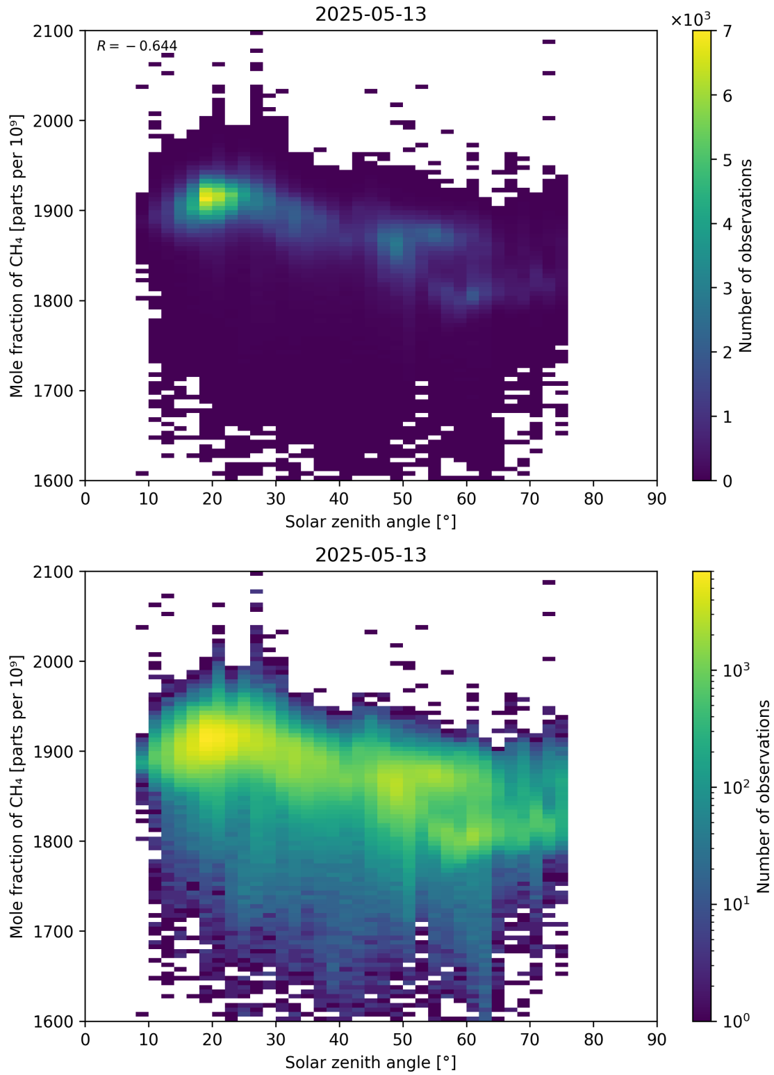
Figure 99: Scatter density plot of “Solar zenith angle” against “Mole fraction of CH 4 ” for 2025-05-12 to 2025-05-14.
