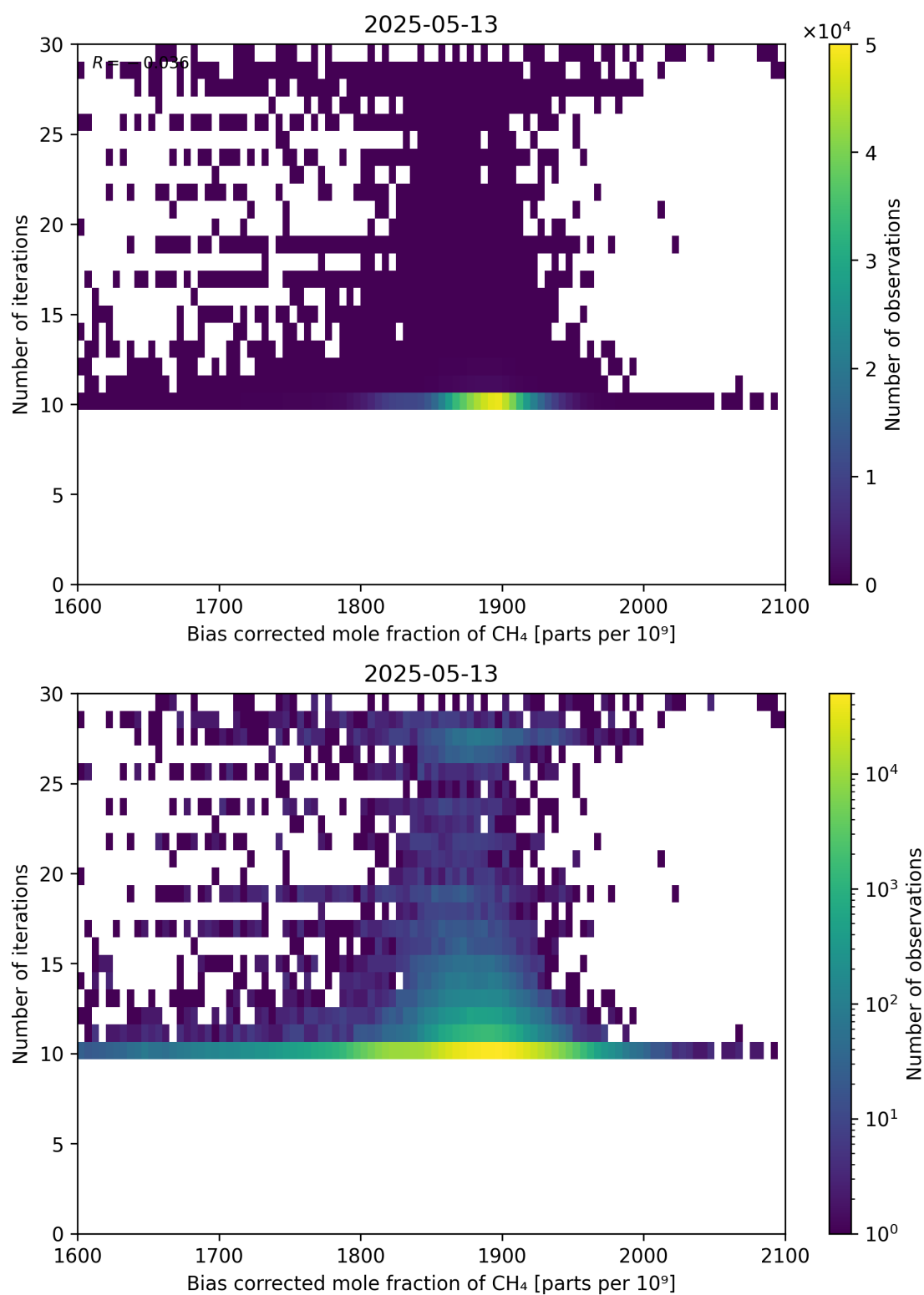
Figure 67: Scatter density plot of “Bias corrected mole fraction of \text{CH}_4 ” against “Number of iterations” for 2025-05-12 to 2025-05-14.
