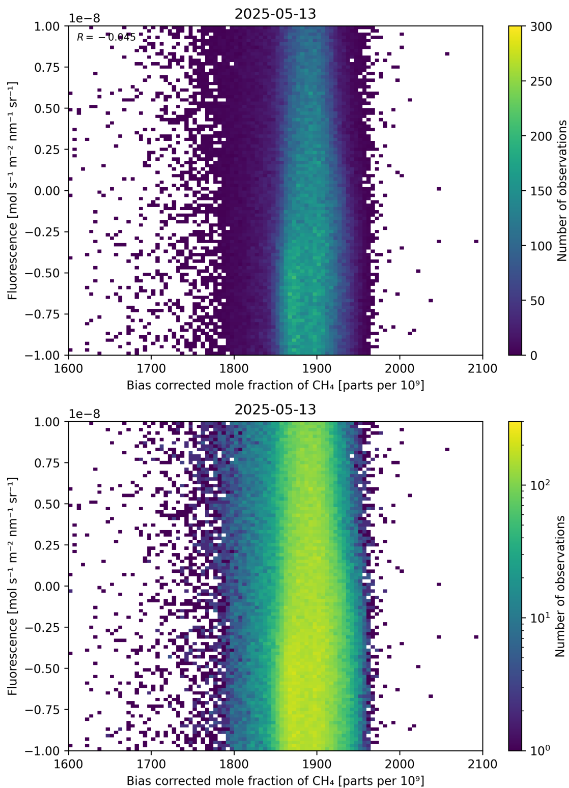
Figure 66: Scatter density plot of “Bias corrected mole fraction of \text{CH}_4 ” against “Fluorescence” for 2025-05-12 to 2025-05-14.
