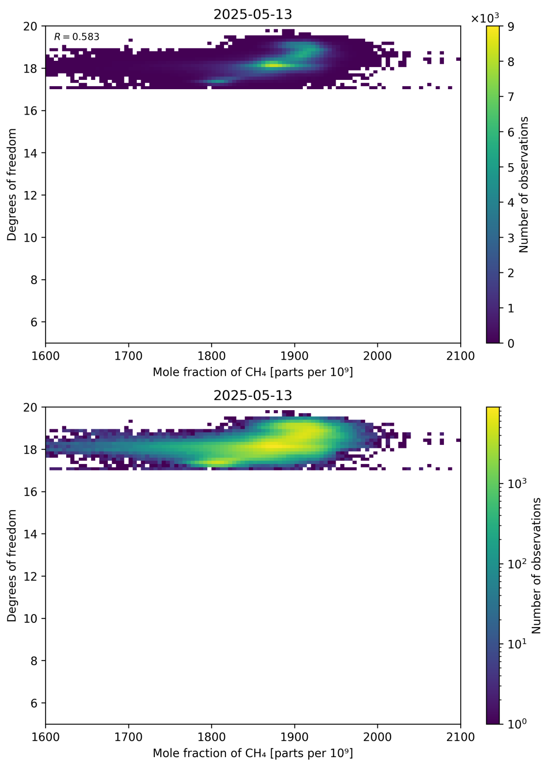
Figure 72: Scatter density plot of “Mole fraction of CH 4 ” against “Degrees of freedom” for 2025-05-12 to 2025-05-14.
