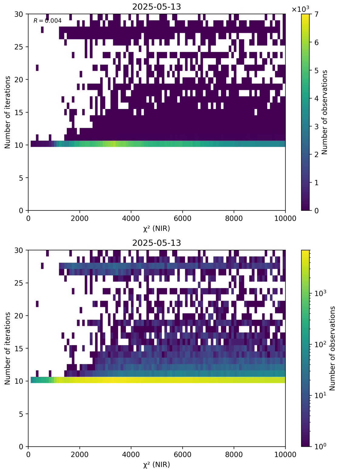
Figure 46: Scatter density plot of “ \chi^2 (NIR)” against “Number of iterations” for 2025-05-12 to 2025-05-14.
