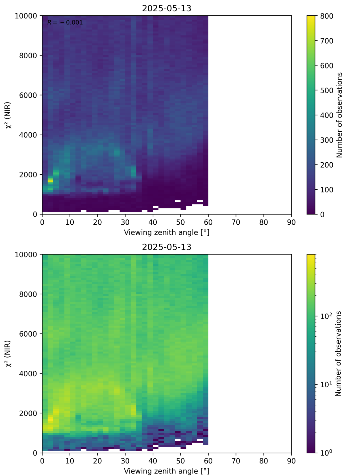
Figure 105: Scatter density plot of “Viewing zenith angle” against “ \chi^2 (NIR)” for 2025-05-12 to 2025-05-14.
