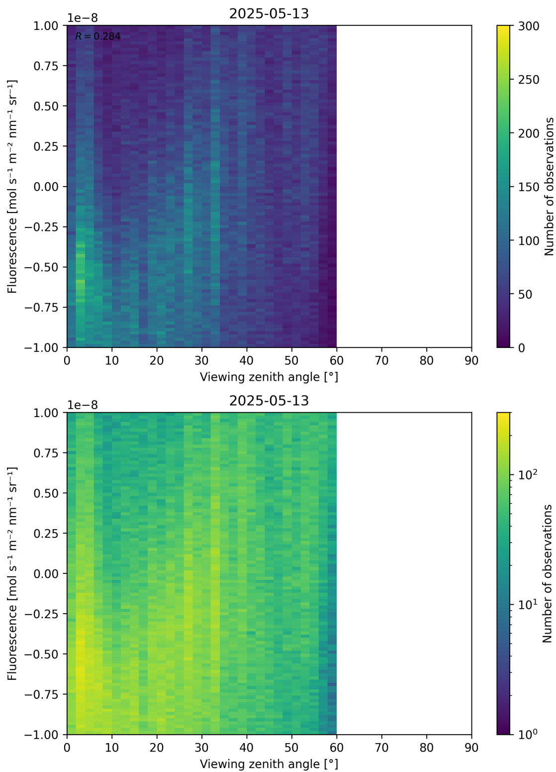
Figure 108: Scatter density plot of “Viewing zenith angle” against “Fluorescence” for 2025-05-12 to 2025-05-14.
