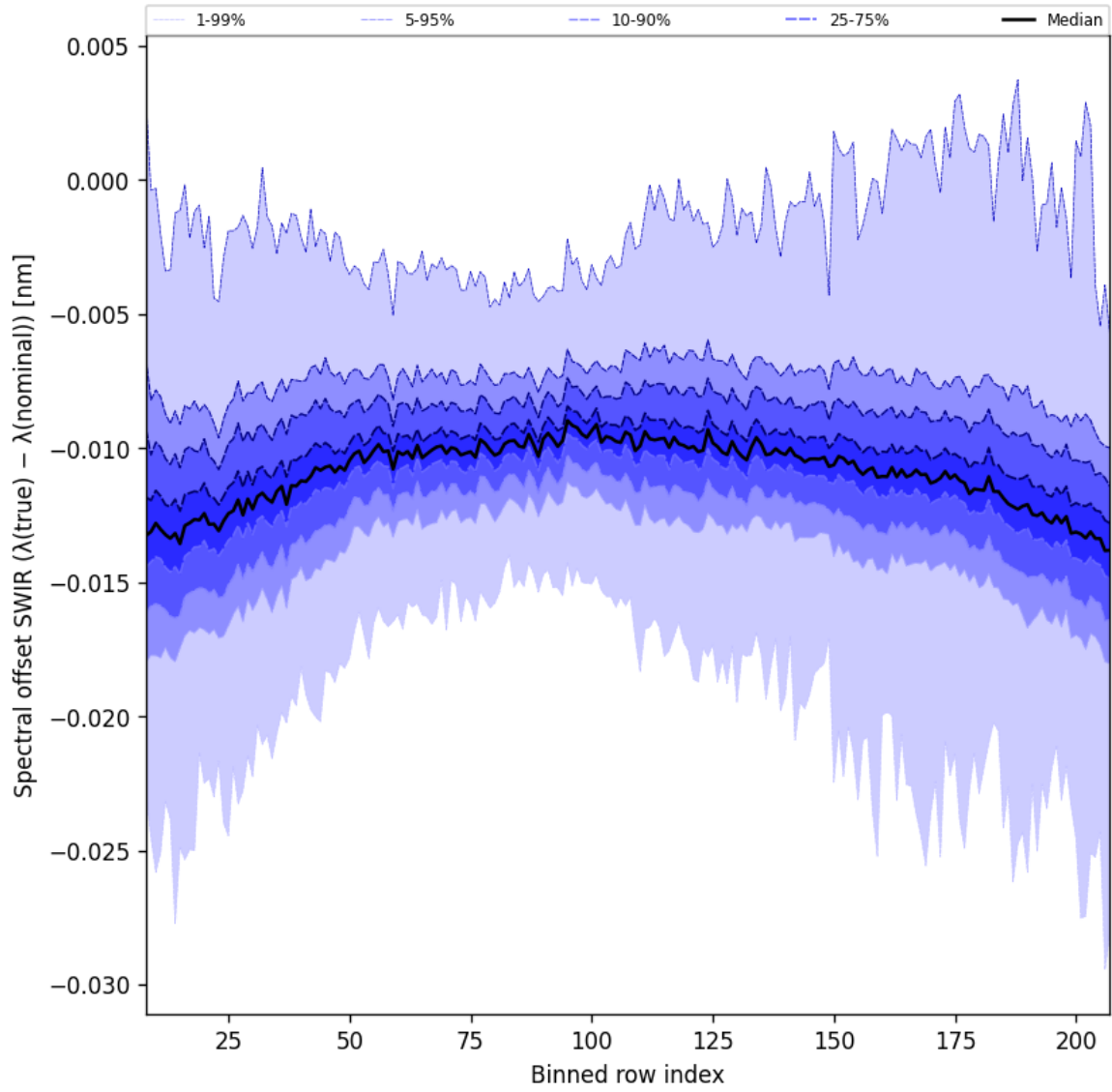
Figure 38: Along track statistics of “Spectral offset SWIR ( \lambda_{\text{true}} - \lambda_{\text{nominal}} )” for 2025-05-12 to 2025-05-14
