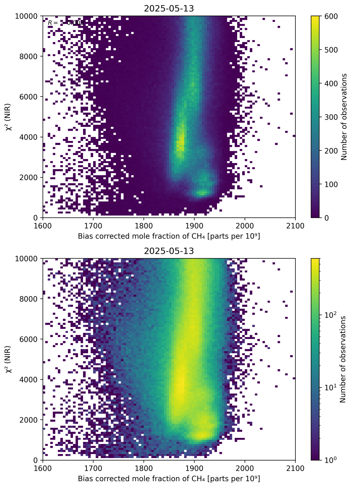
Figure 63: Scatter density plot of “Bias corrected mole fraction of CH 4 ” against “ \chi^2 (NIR)” for 2025-05-12 to 2025-05-14.
