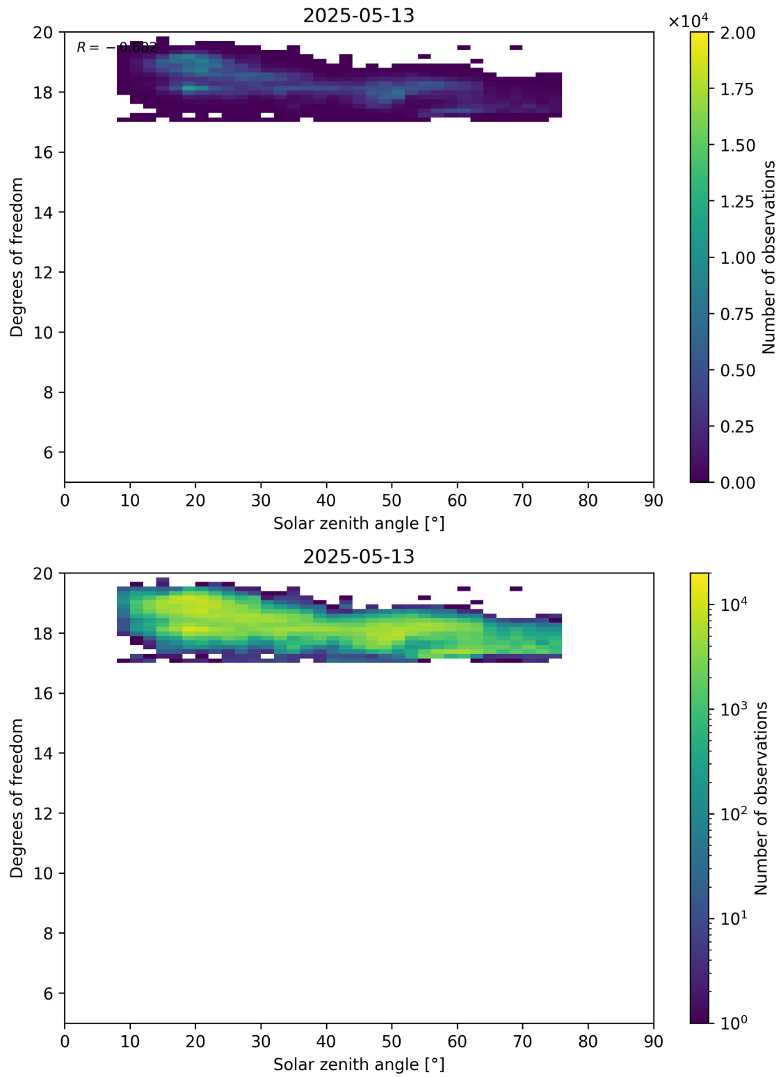
Figure 96: Scatter density plot of “Solar zenith angle” against “Degrees of freedom” for 2025-05-12 to 2025-05-14.
