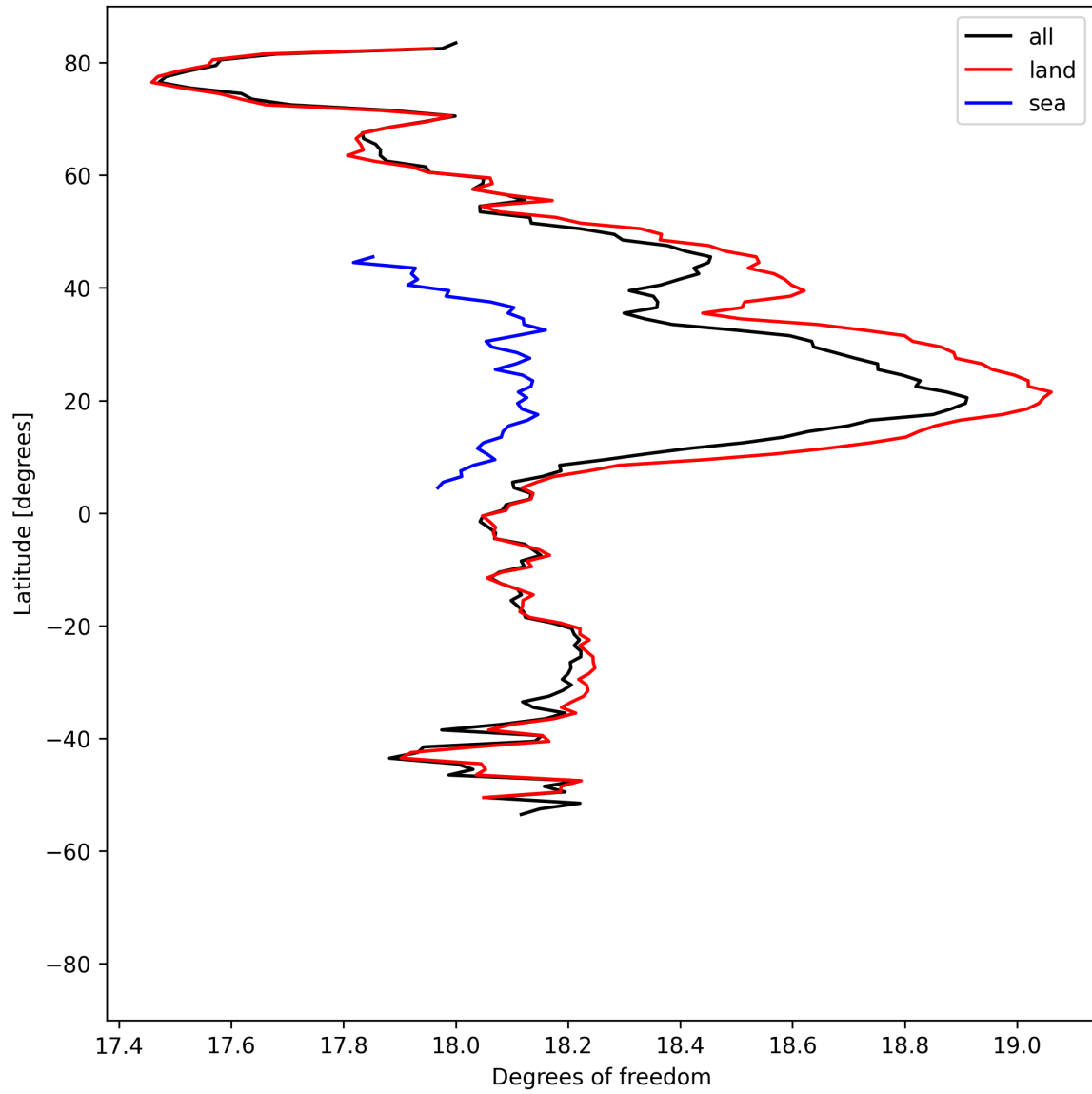
Figure 19: Zonal average of “Degrees of freedom” for 2025-05-12 to 2025-05-14.
