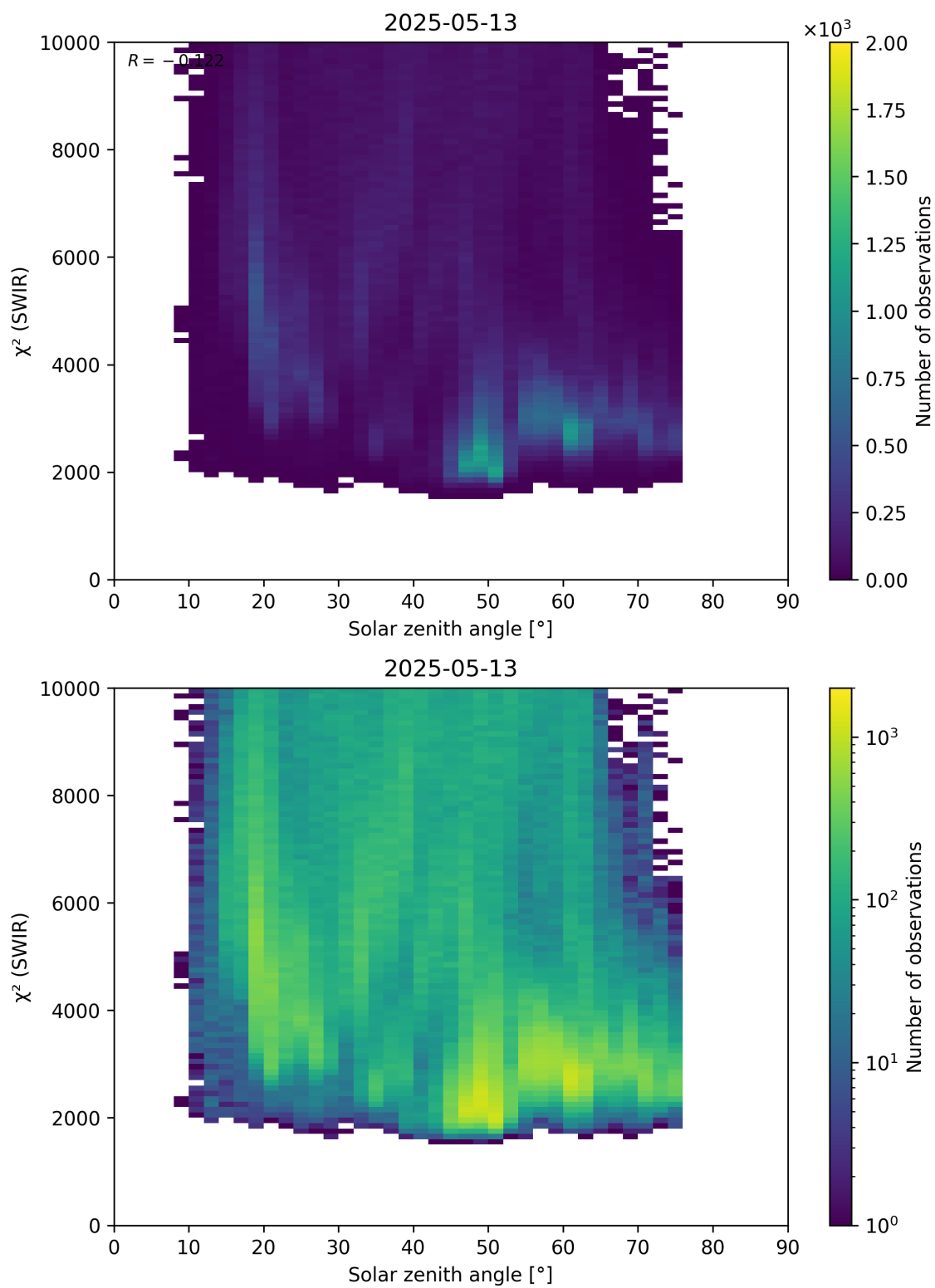
Figure 95: Scatter density plot of “Solar zenith angle” against “ \chi^2 (SWIR)” for 2025-05-12 to 2025-05-14.
