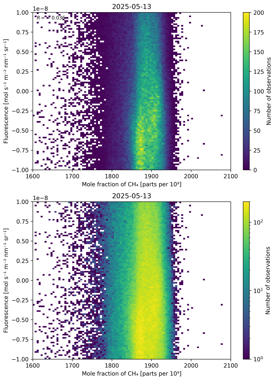
Figure 73: Scatter density plot of “Mole fraction of \text{CH}_4 ” against “Fluorescence” for 2025-05-12 to 2025-05-14.
