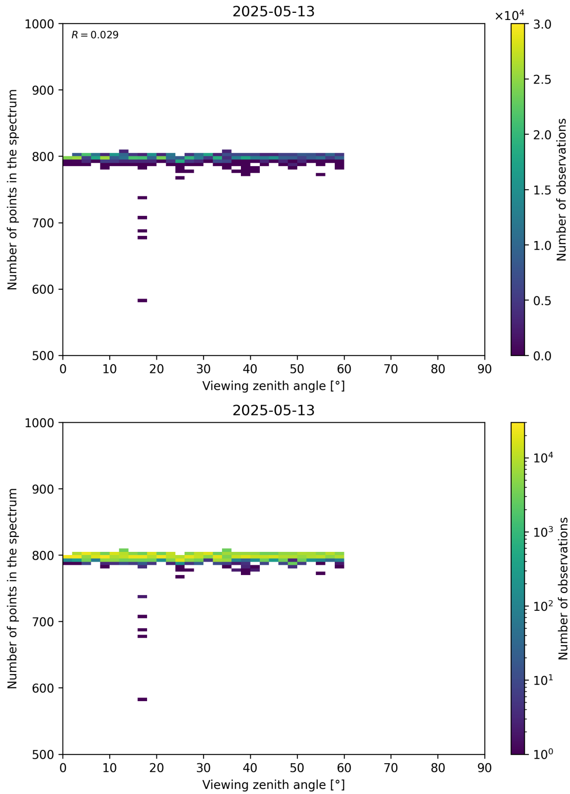
Figure 114: Scatter density plot of “Viewing zenith angle” against “Number of points in the spectrum” for 2025-05-12 to 2025-05-14.
