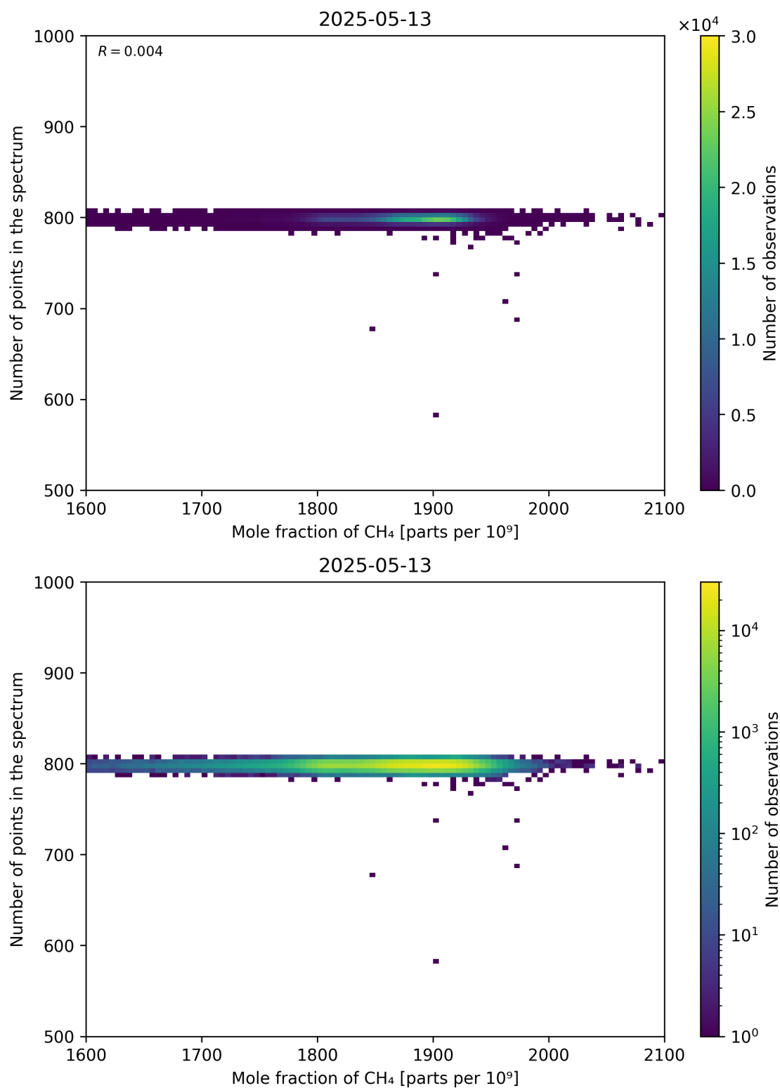
Figure 77: Scatter density plot of “Mole fraction of CH 4 ” against “Number of points in the spectrum” for 2025-05-12 to 2025-05-14.
