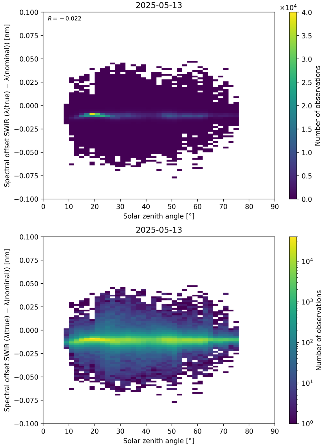
Figure 104: Scatter density plot of “Solar zenith angle” against “Spectral offset SWIR ( \lambda_{\text{true}} - \lambda_{\text{nominal}} )” for 2025-05-12 to 2025-05-14.
