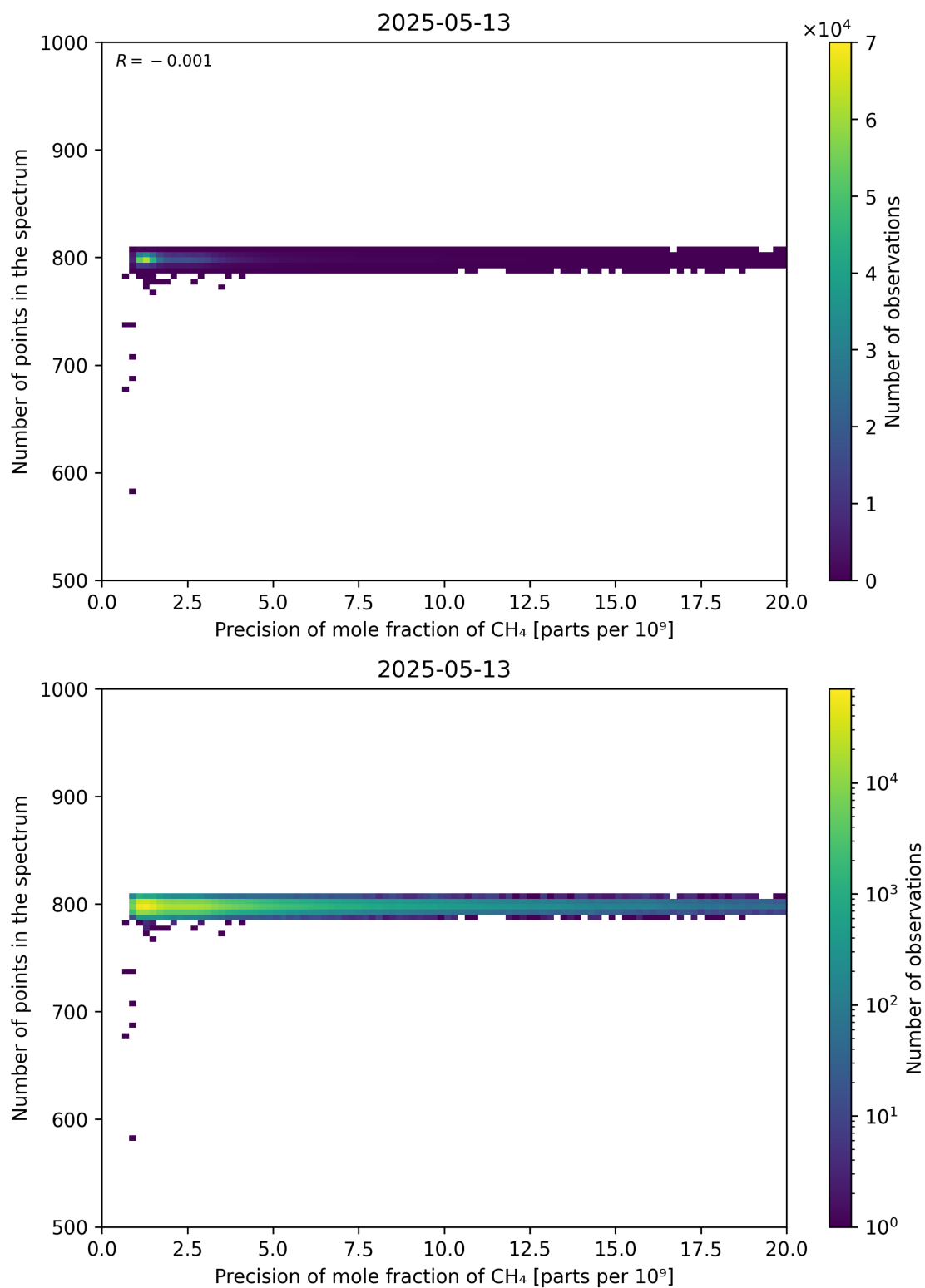
Figure 84: Scatter density plot of “Precision of mole fraction of CH 4 ” against “Number of points in the spectrum” for 2025-05-12 to 2025-05-14.
