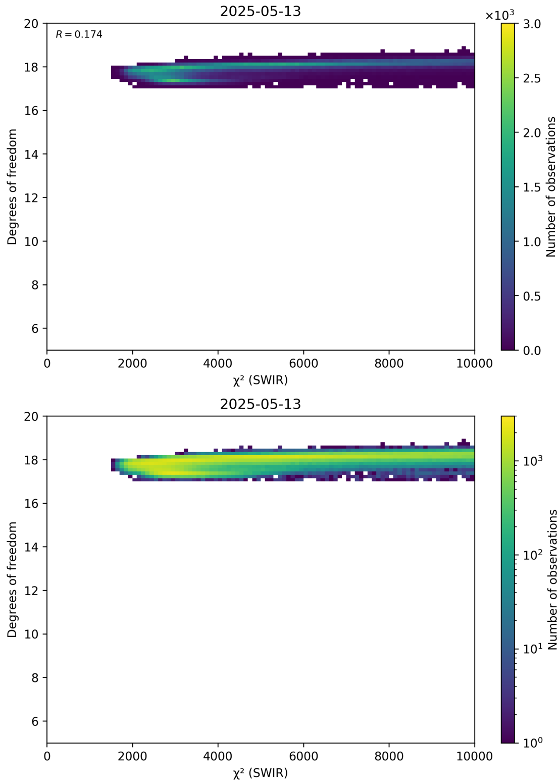
Figure 48: Scatter density plot of “ \chi^2 (SWIR)” against “Degrees of freedom” for 2025-05-12 to 2025-05-14.
