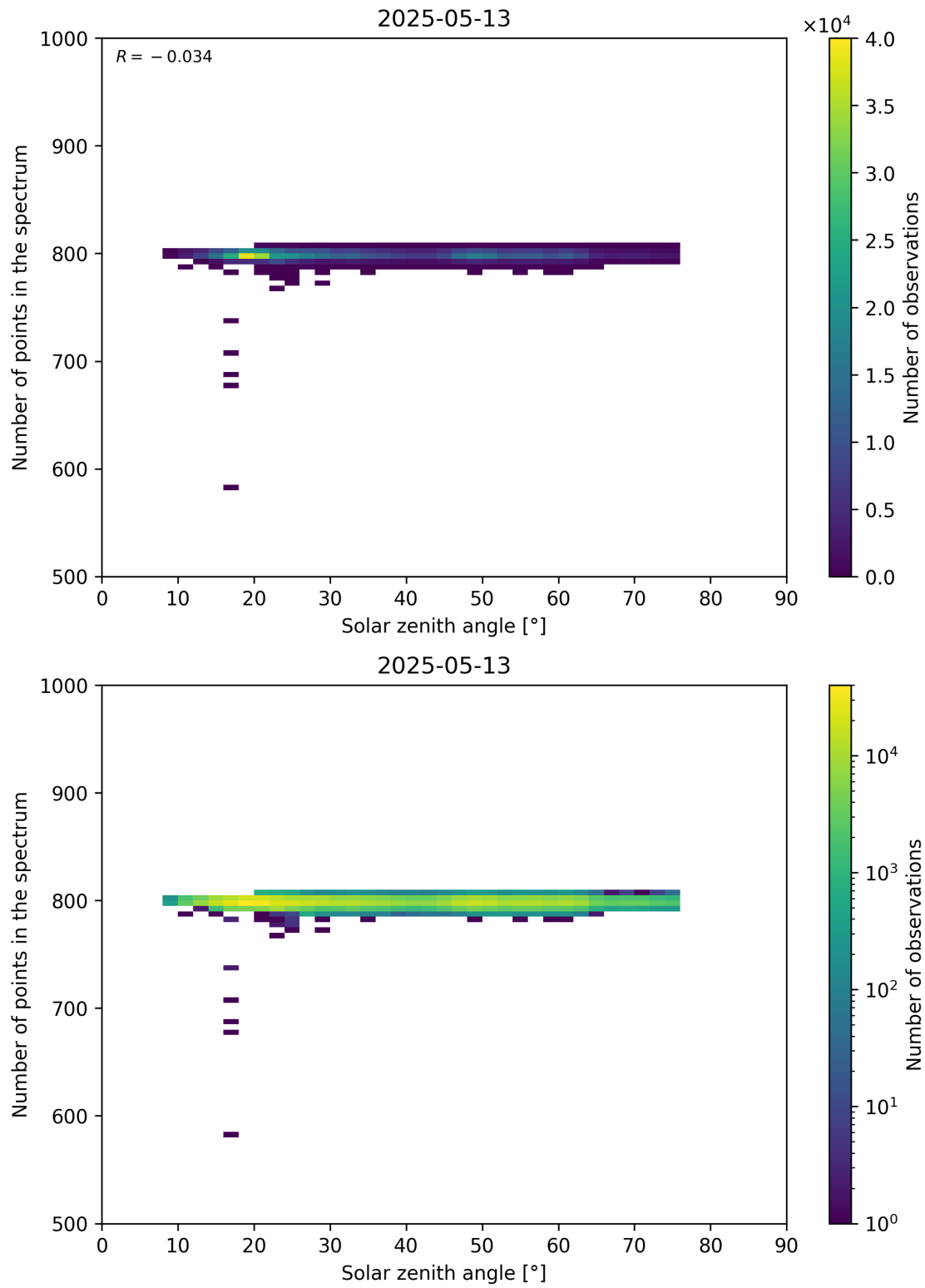
Figure 103: Scatter density plot of “Solar zenith angle” against “Number of points in the spectrum” for 2025-05-12 to 2025-05-14.
