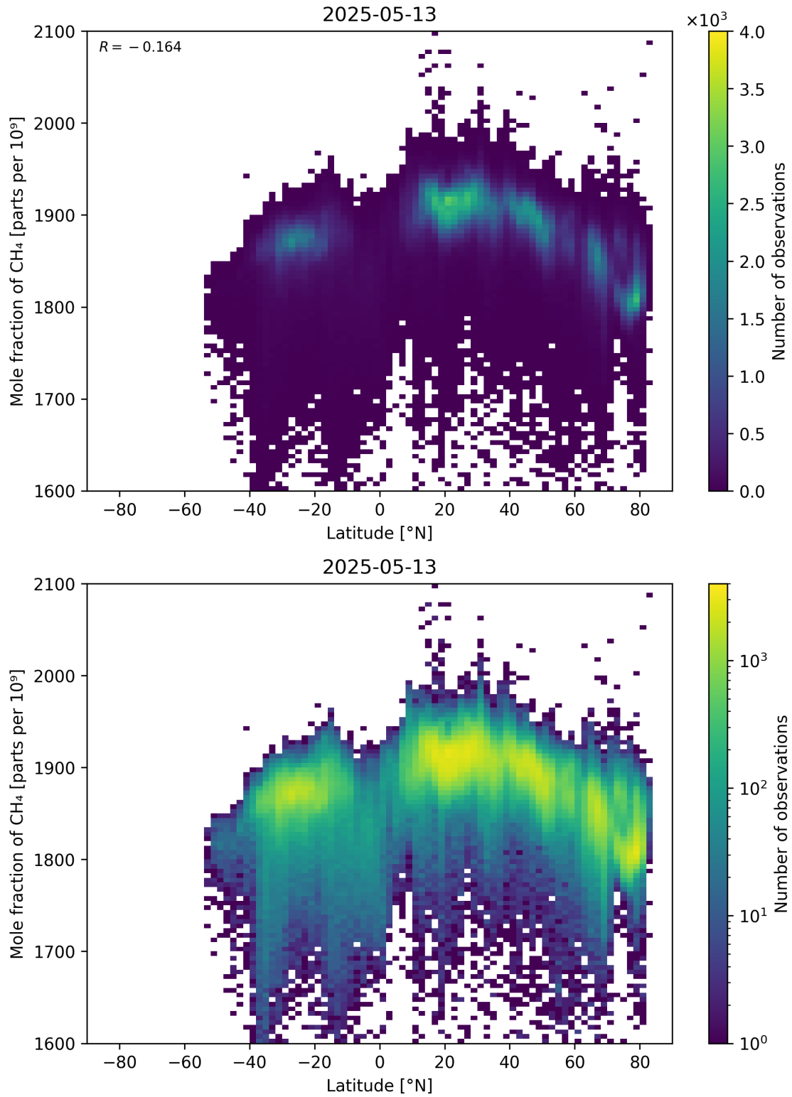
Figure 57: Scatter density plot of “Latitude” against “Mole fraction of CH 4 ” for 2025-05-12 to 2025-05-14.
