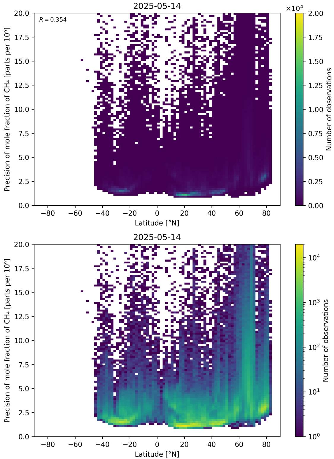
Figure 59: Scatter density plot of “Latitude” against “Precision of mole fraction of \text{CH}_4 ” for 2025-05-13 to 2025-05-15.
