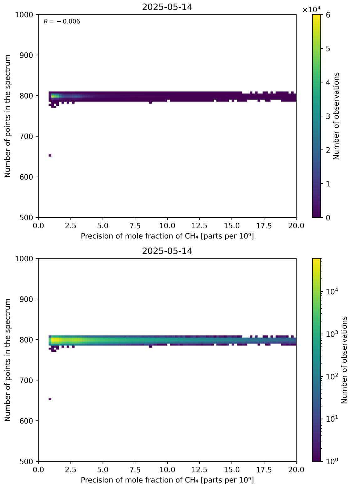
Figure 84: Scatter density plot of “Precision of mole fraction of CH 4 ” against “Number of points in the spectrum” for 2025-05-13 to 2025-05-15.
