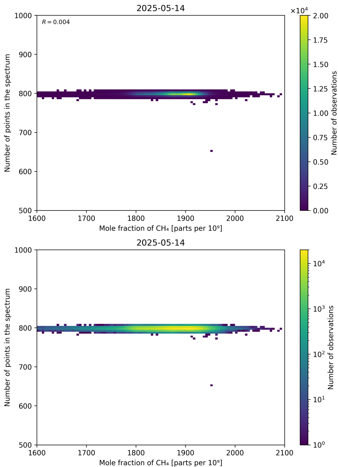
Figure 77: Scatter density plot of “Mole fraction of CH 4 ” against “Number of points in the spectrum” for 2025-05-13 to 2025-05-15.
