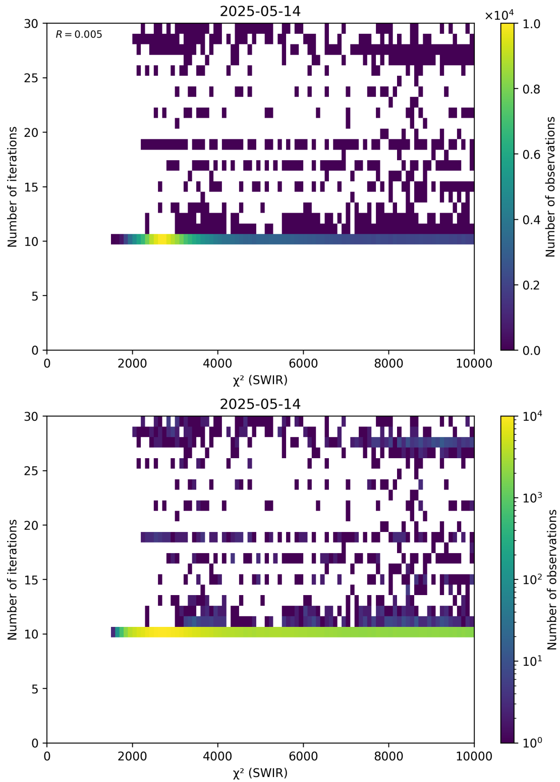
Figure 50: Scatter density plot of “ \chi^2 (SWIR)” against “Number of iterations” for 2025-05-13 to 2025-05-15.
