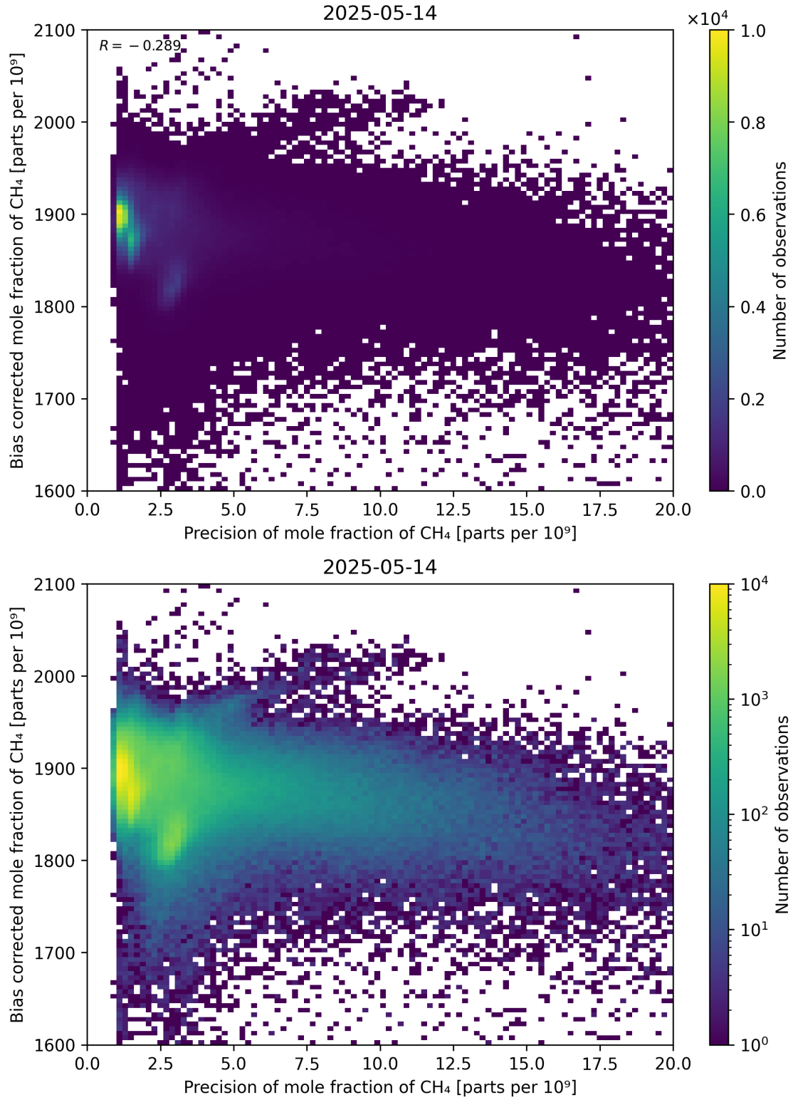
Figure 82: Scatter density plot of “Precision of mole fraction of CH 4 ” against “Bias corrected mole fraction of CH 4 ” for 2025-05-13 to 2025-05-15.
