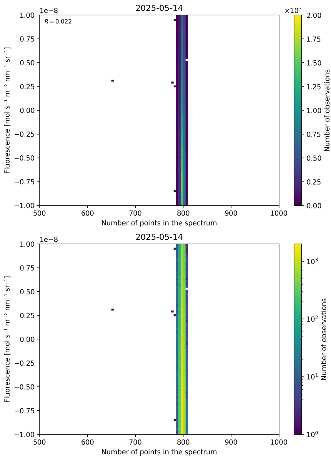
Figure 91: Scatter density plot of “Number of points in the spectrum” against “Fluorescence” for 2025-05-13 to 2025-05-15.
