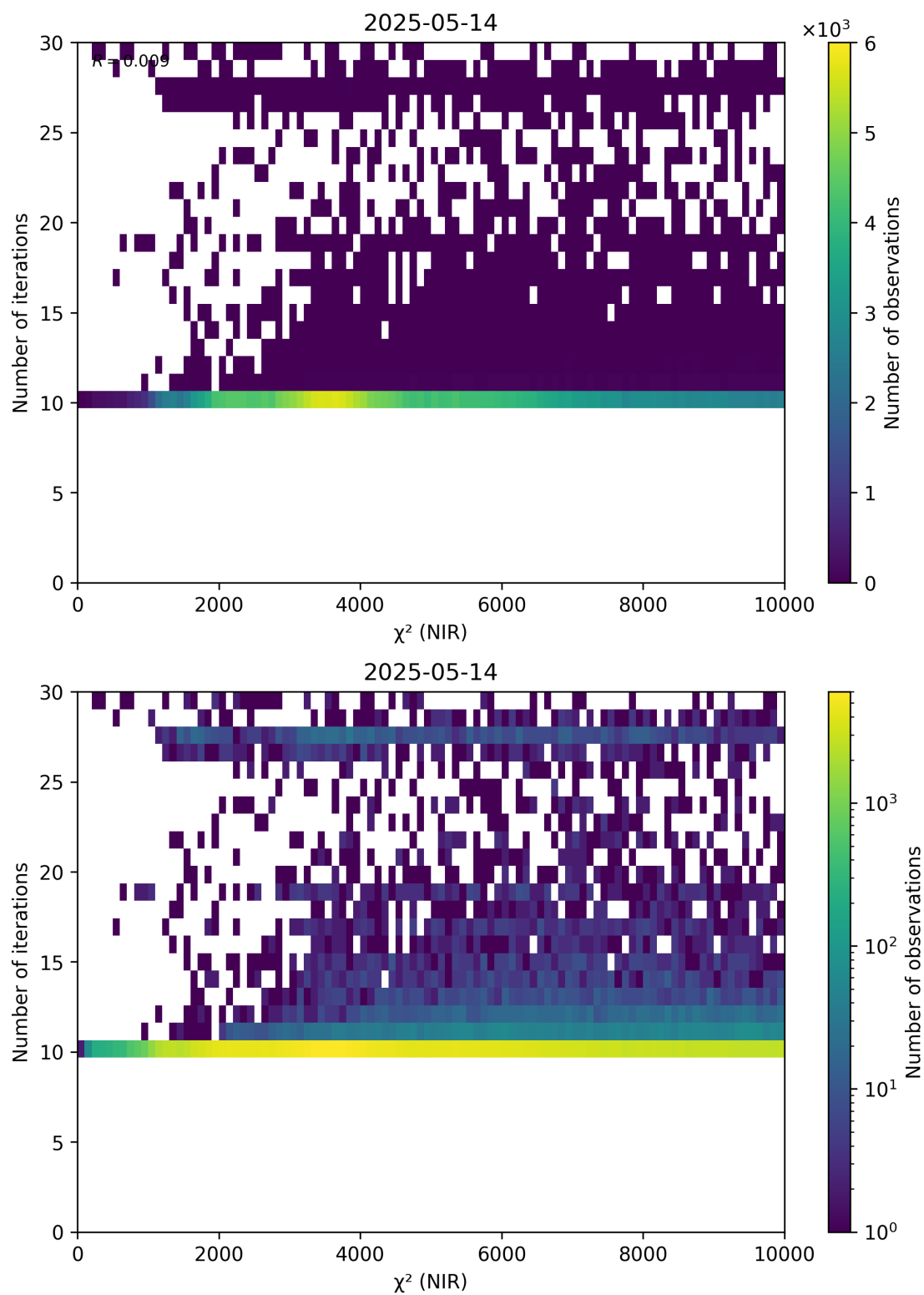
Figure 46: Scatter density plot of “ \chi^2 (NIR)” against “Number of iterations” for 2025-05-13 to 2025-05-15.
