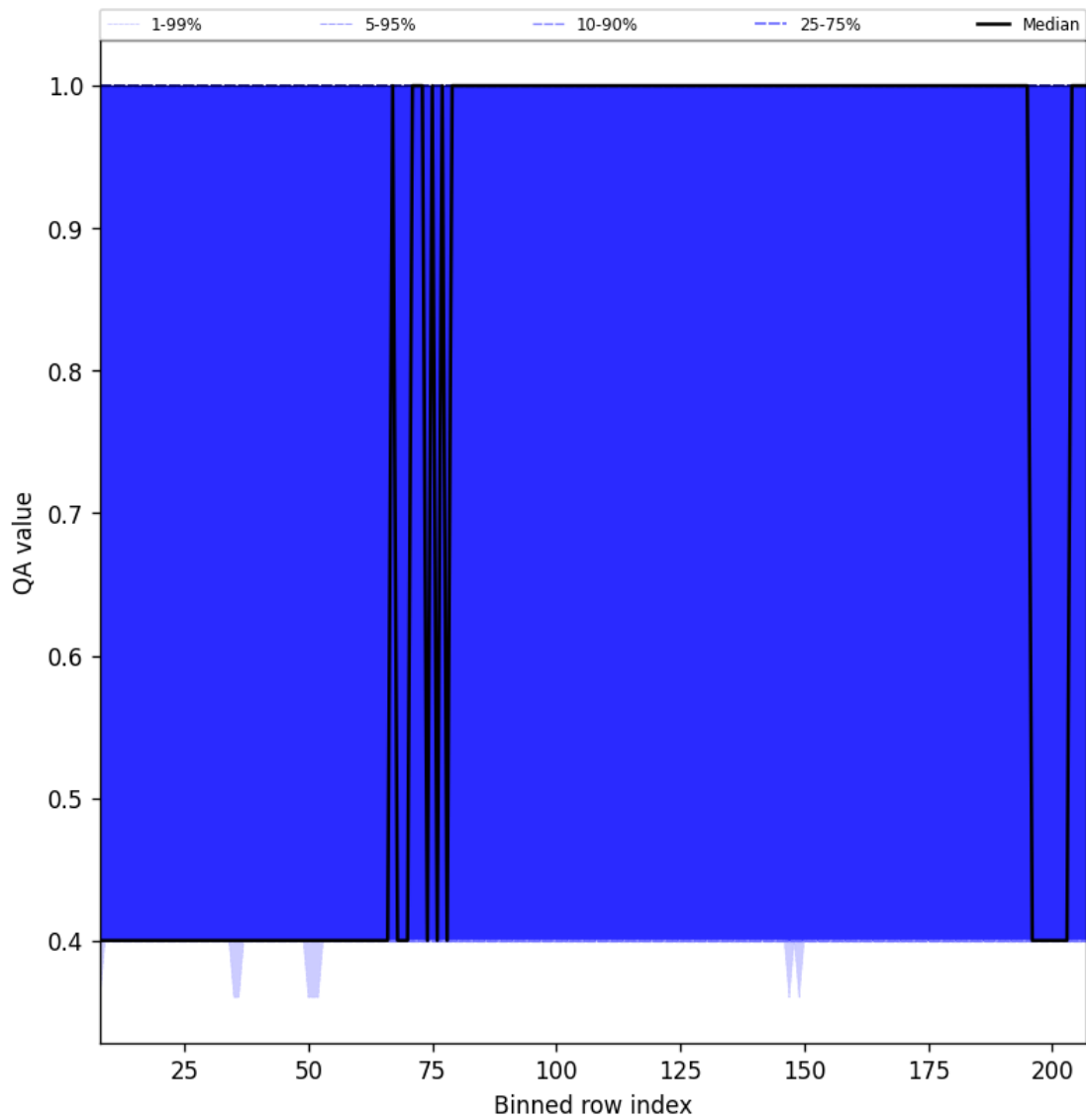
Figure 33: Along track statistics of “QA value” for 2025-05-13 to 2025-05-15
