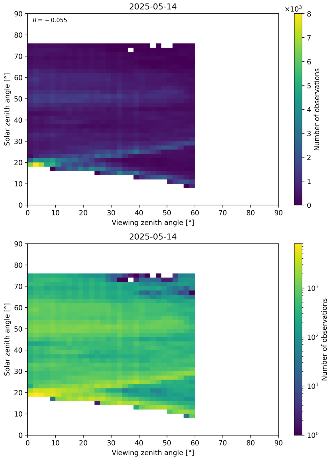
Figure 115: Scatter density plot of “Viewing zenith angle” against “Solar zenith angle” for 2025-05-13 to 2025-05-15.
