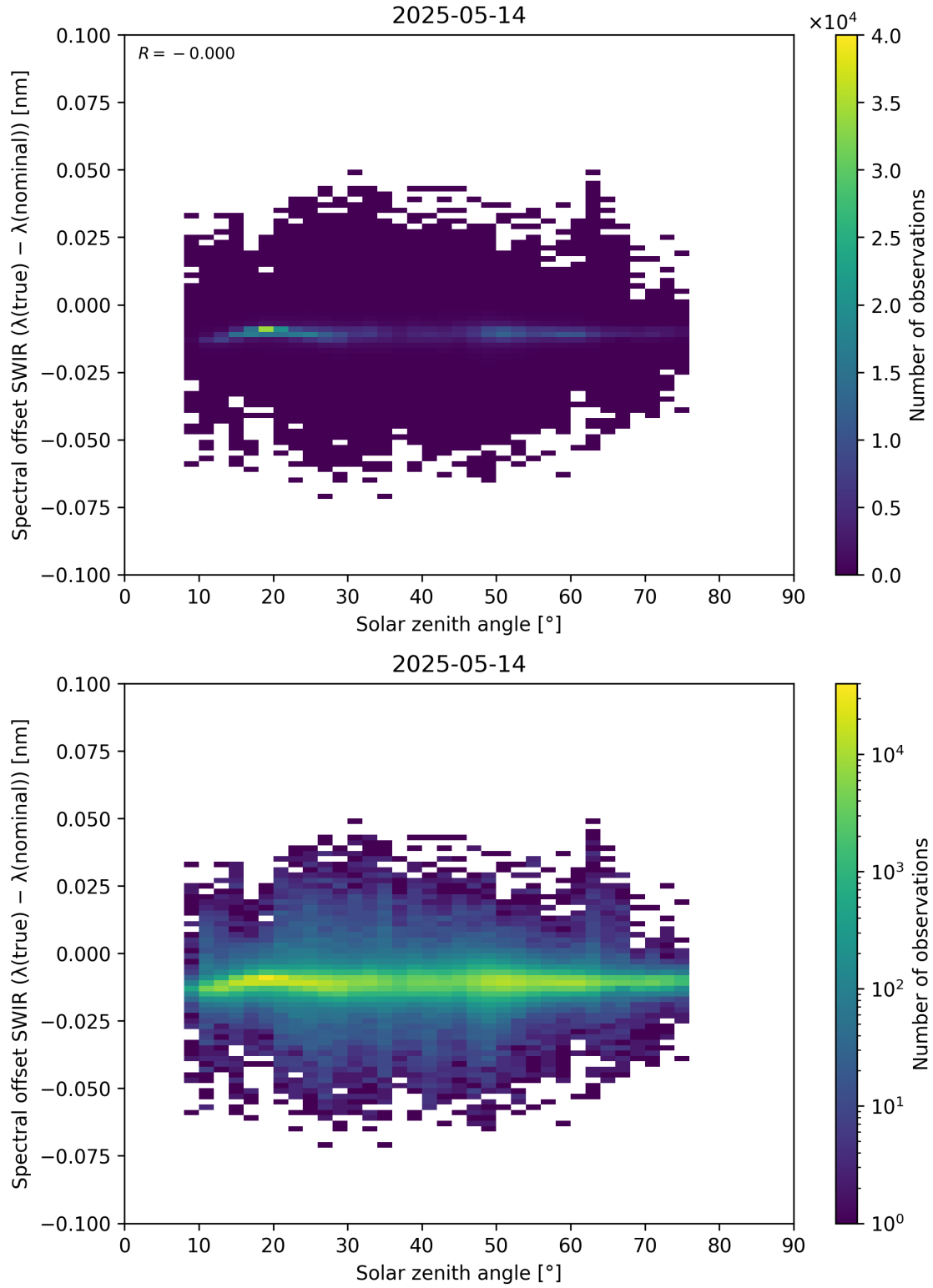
Figure 104: Scatter density plot of “Solar zenith angle” against “Spectral offset SWIR ( \lambda_{\text{true}} - \lambda_{\text{nominal}} )” for 2025-05-13 to 2025-05-15.
