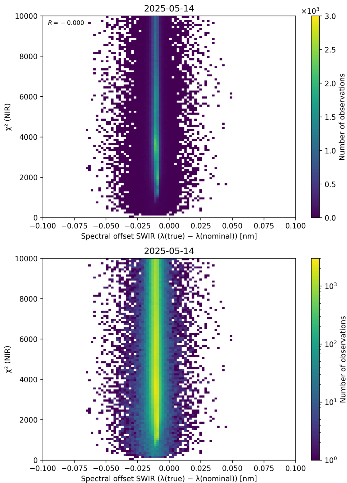
Figure 117: Scatter density plot of “Spectral offset SWIR ( \lambda_{\text{true}} - \lambda_{\text{nominal}} )” against “ \chi^2 (NIR)” for 2025-05-13 to 2025-05-15.
