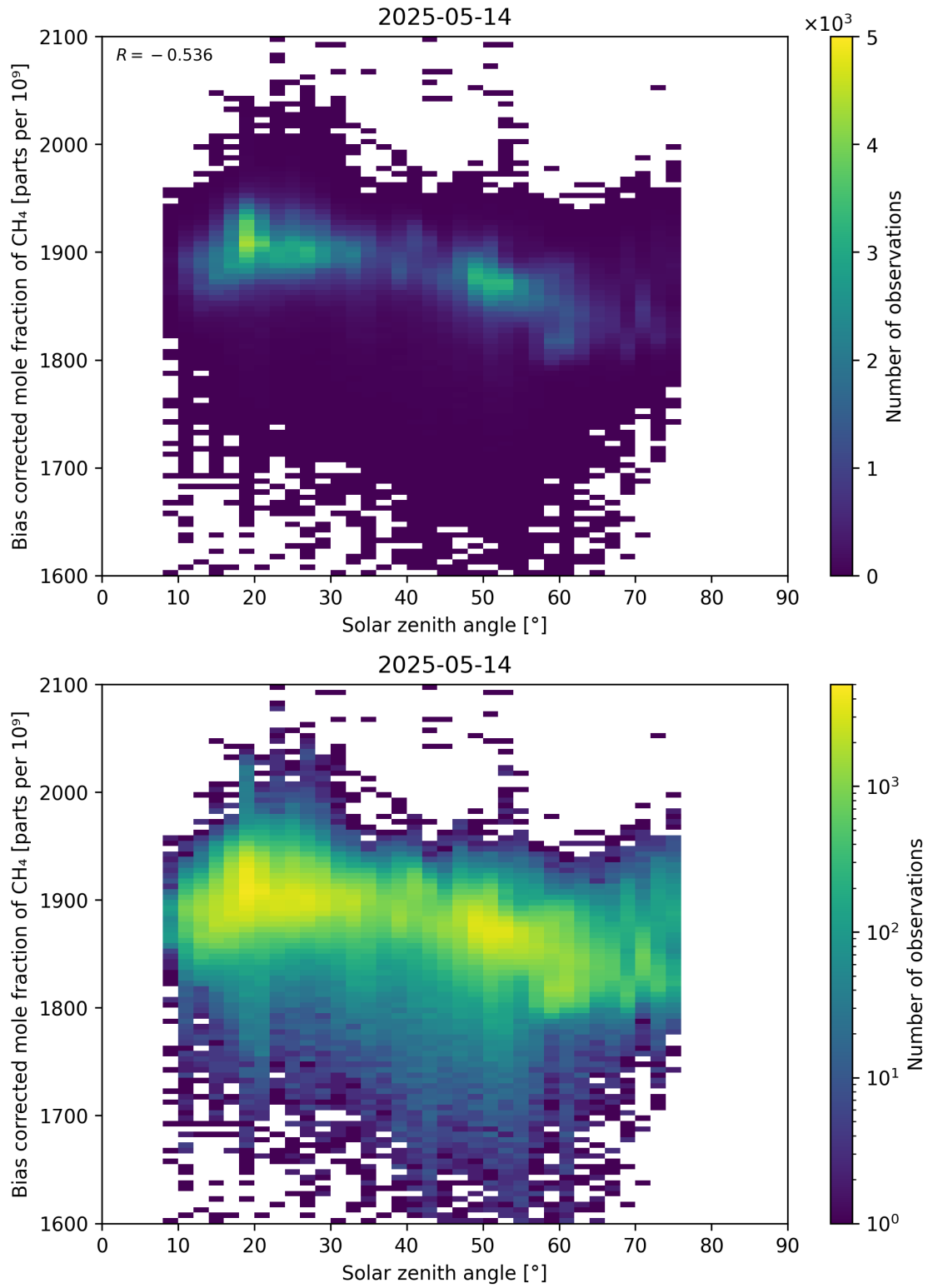
Figure 100: Scatter density plot of “Solar zenith angle” against “Bias corrected mole fraction of CH 4 ” for 2025-05-13 to 2025-05-15.
