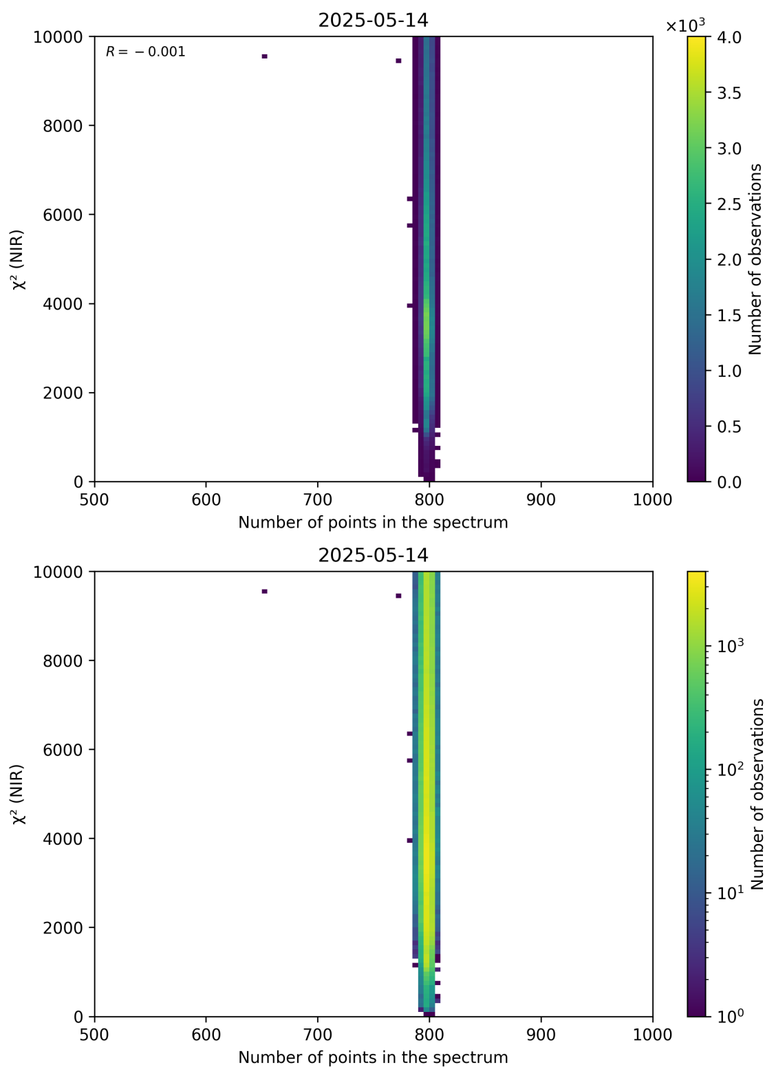
Figure 88: Scatter density plot of “Number of points in the spectrum” against “ \chi^2 (NIR)” for 2025-05-13 to 2025-05-15.
