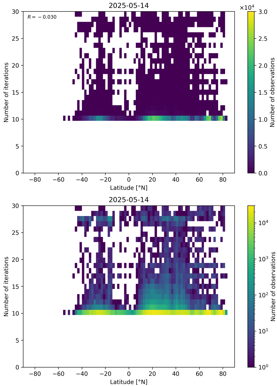
Figure 60: Scatter density plot of “Latitude” against “Number of iterations” for 2025-05-13 to 2025-05-15.
