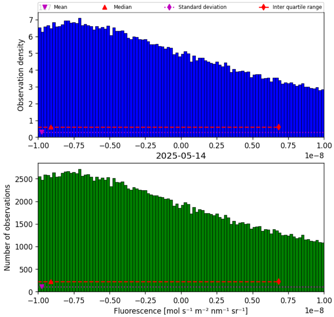
Figure 32: Histogram of “Fluorescence” for 2025-05-13 to 2025-05-15
