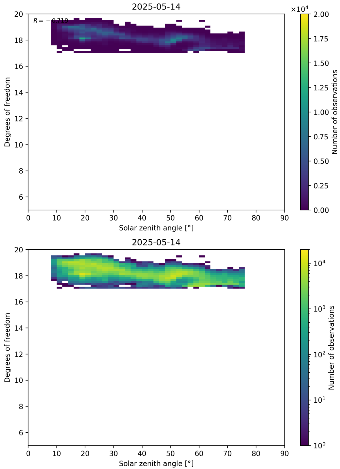
Figure 96: Scatter density plot of “Solar zenith angle” against “Degrees of freedom” for 2025-05-13 to 2025-05-15.
