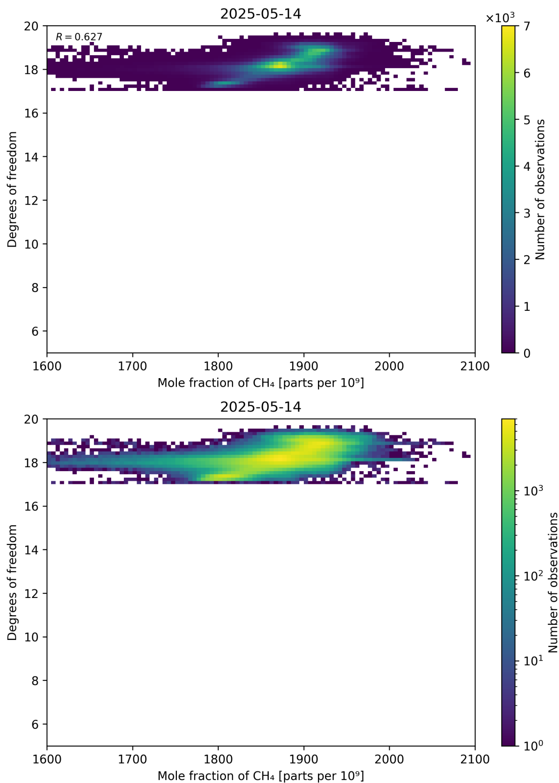
Figure 72: Scatter density plot of “Mole fraction of CH 4 ” against “Degrees of freedom” for 2025-05-13 to 2025-05-15.
