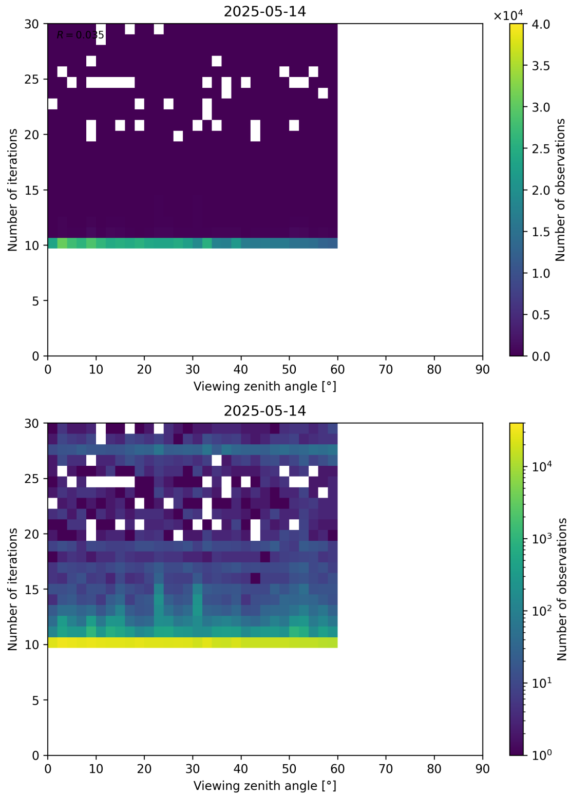
Figure 113: Scatter density plot of “Viewing zenith angle” against “Number of iterations” for 2025-05-13 to 2025-05-15.
