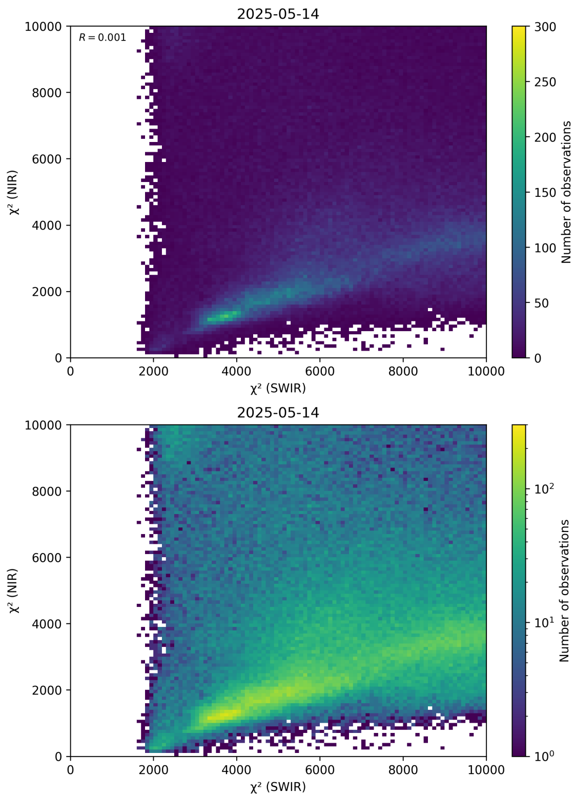
Figure 47: Scatter density plot of “ \chi^2 (SWIR)” against “ \chi^2 (NIR)” for 2025-05-13 to 2025-05-15.
