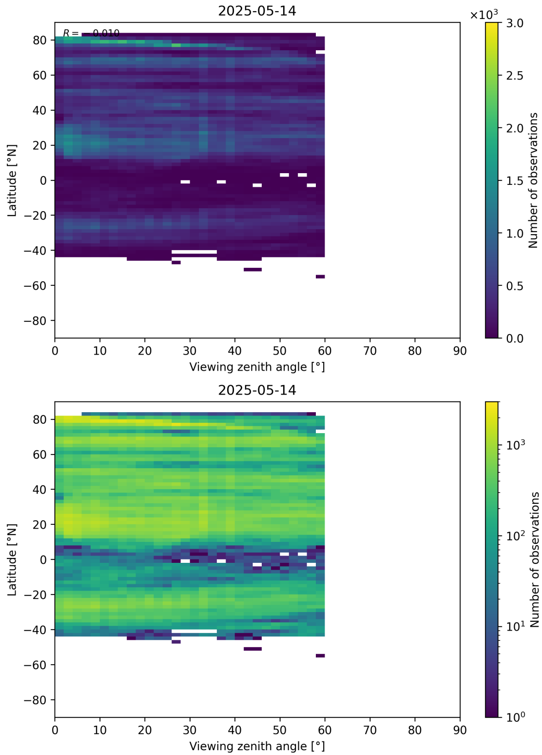
Figure 109: Scatter density plot of “Viewing zenith angle” against “Latitude” for 2025-05-13 to 2025-05-15.
