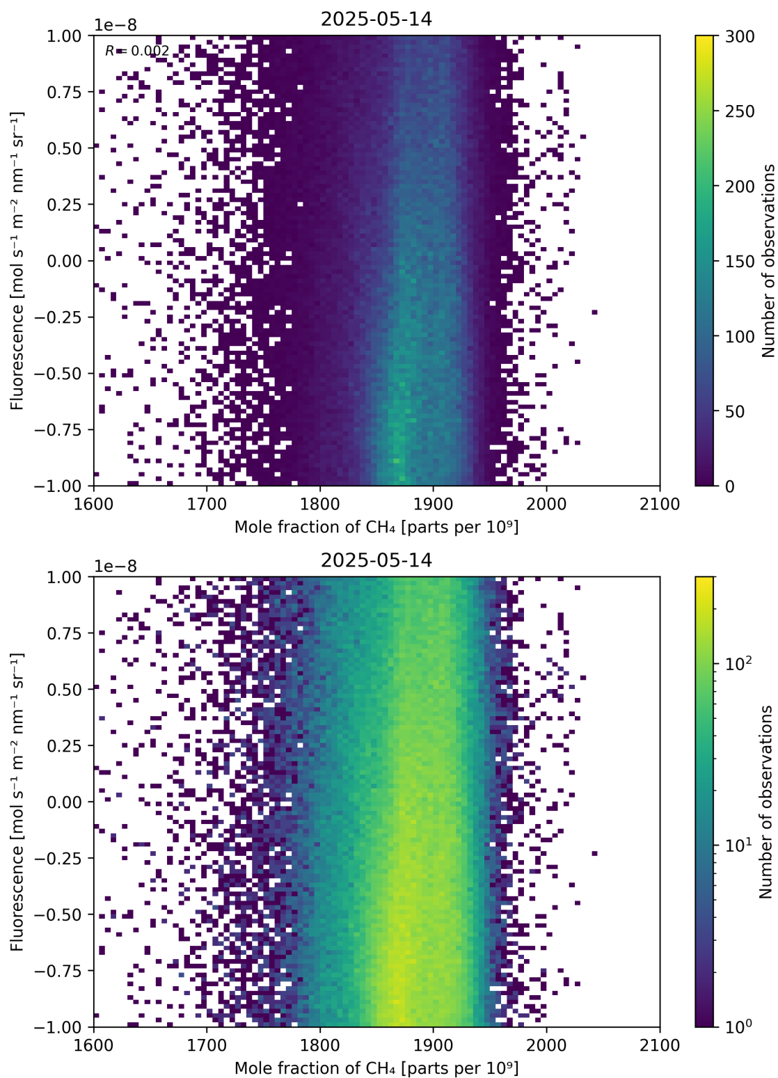
Figure 73: Scatter density plot of “Mole fraction of \text{CH}_4 ” against “Fluorescence” for 2025-05-13 to 2025-05-15.
