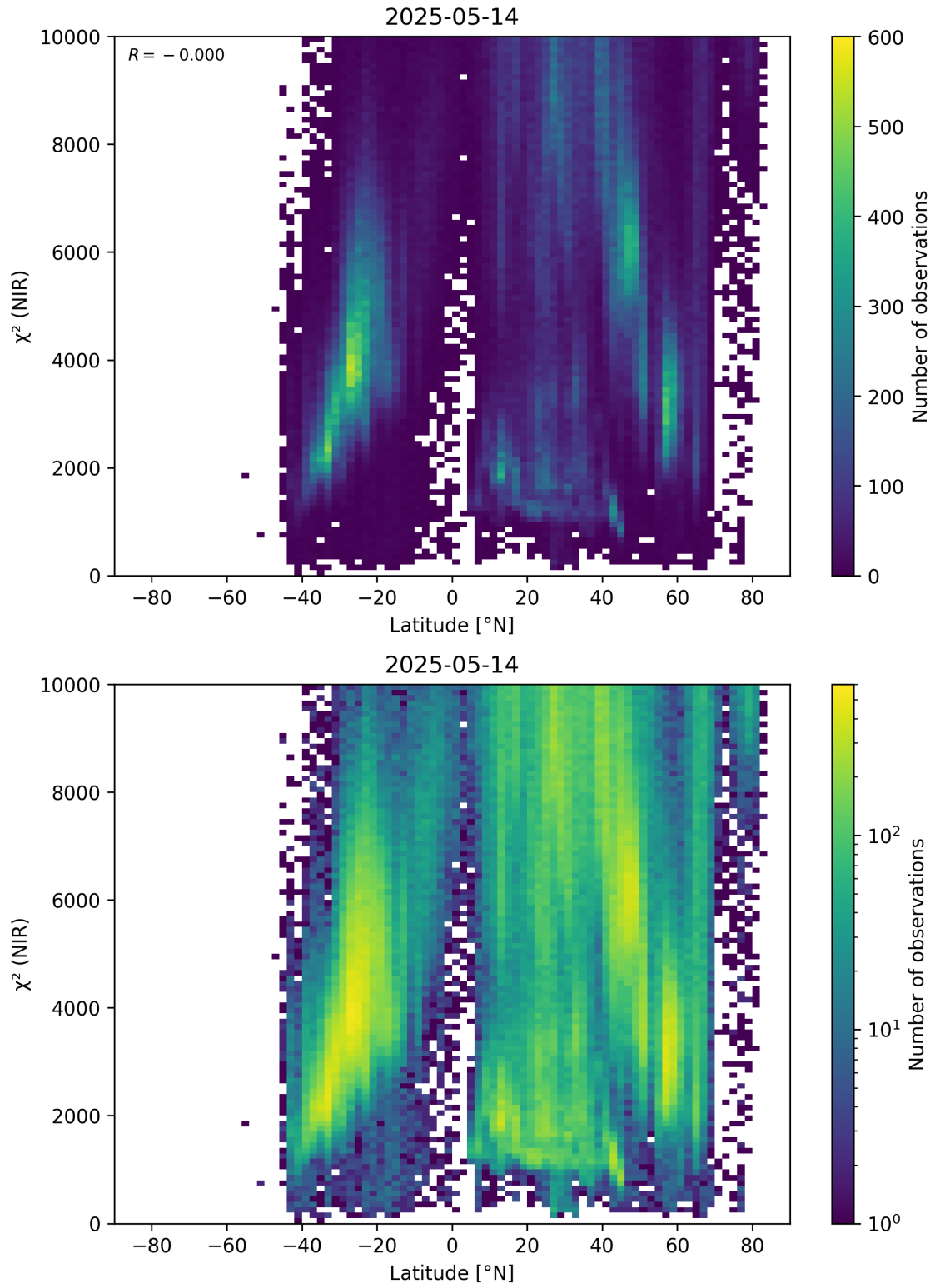
Figure 53: Scatter density plot of “Latitude” against “ \chi^2 (NIR)” for 2025-05-13 to 2025-05-15.
