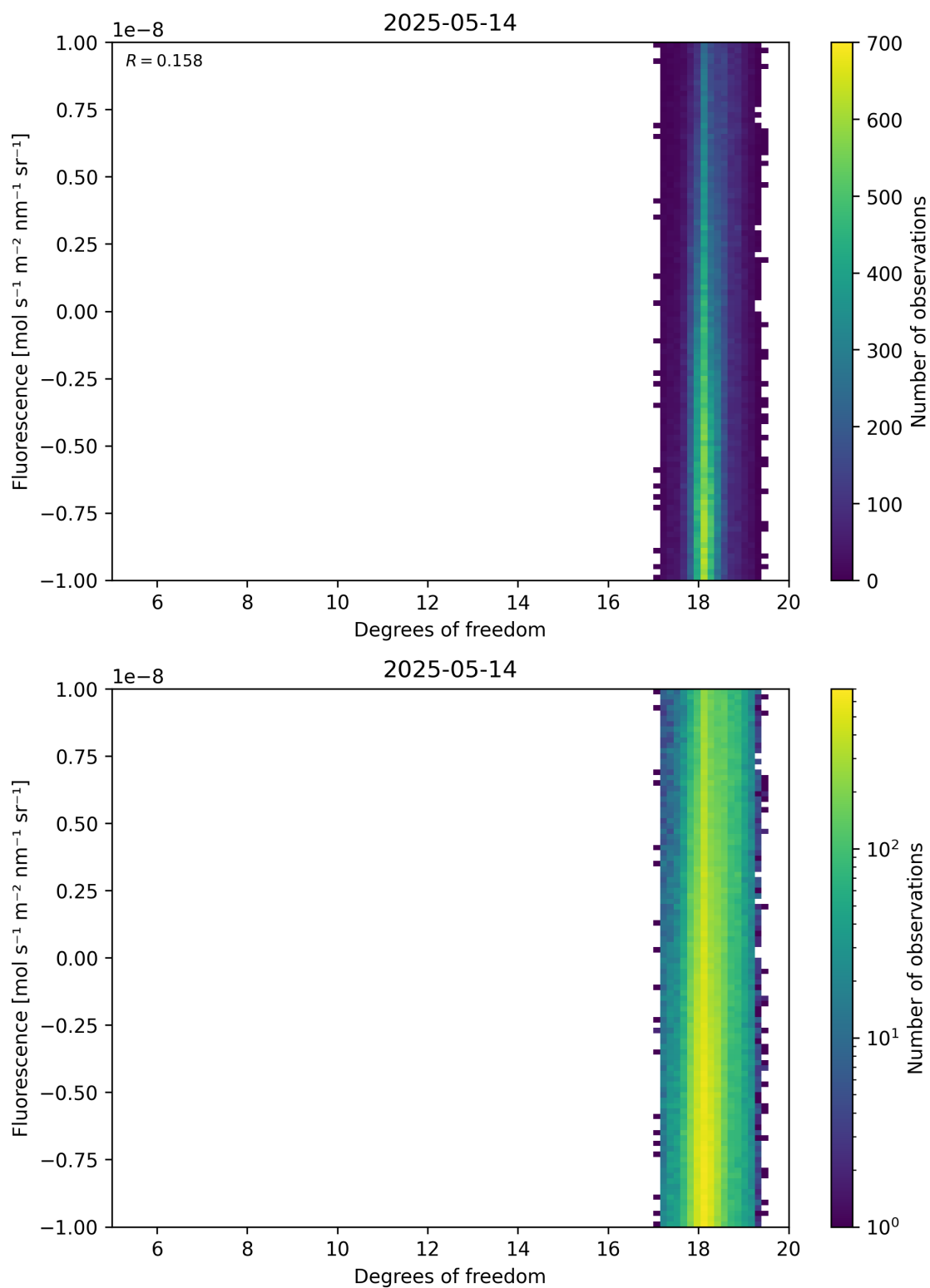
Figure 51: Scatter density plot of “Degrees of freedom” against “Fluorescence” for 2025-05-13 to 2025-05-15.
