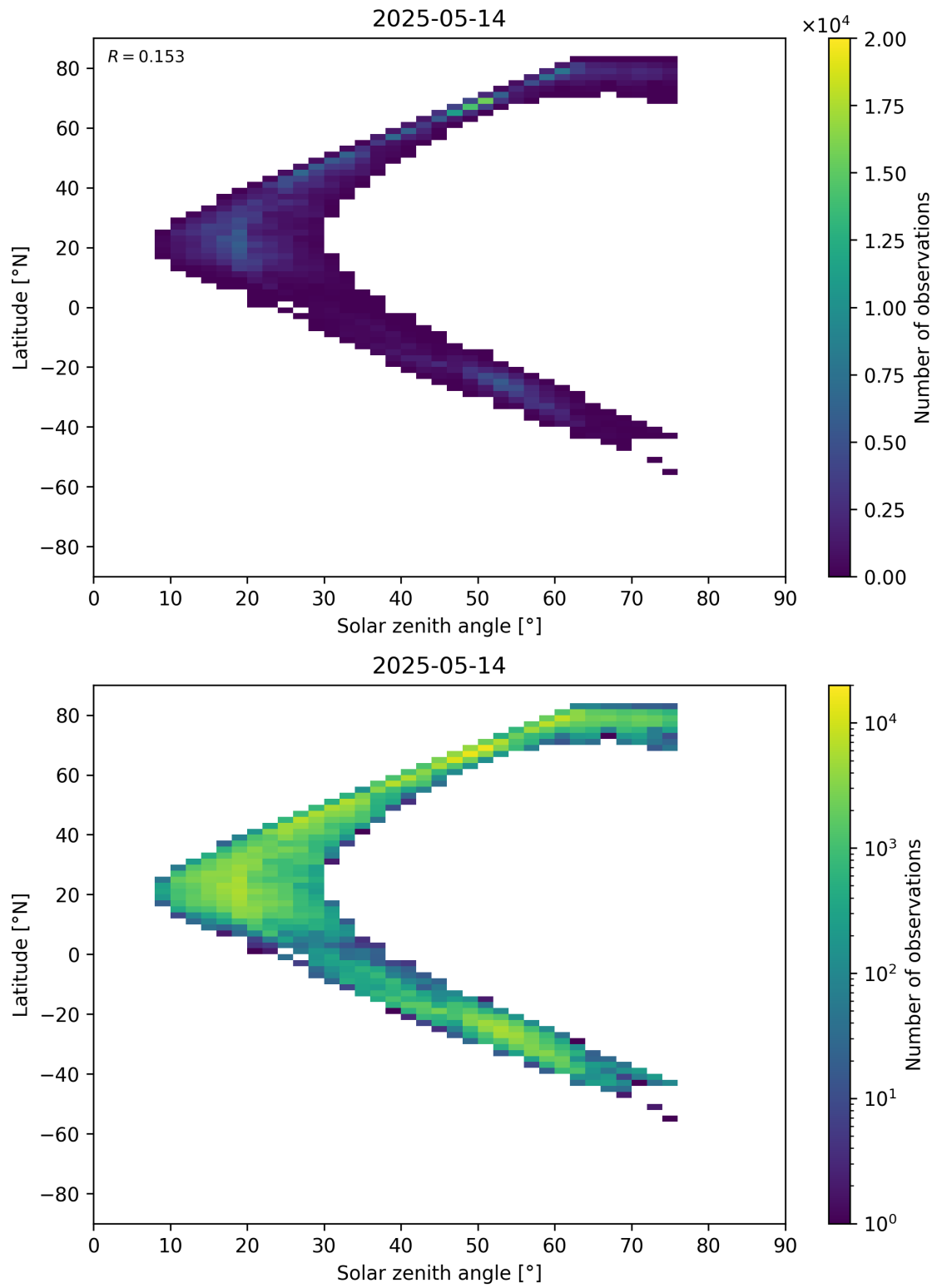
Figure 98: Scatter density plot of “Solar zenith angle” against “Latitude” for 2025-05-13 to 2025-05-15.
