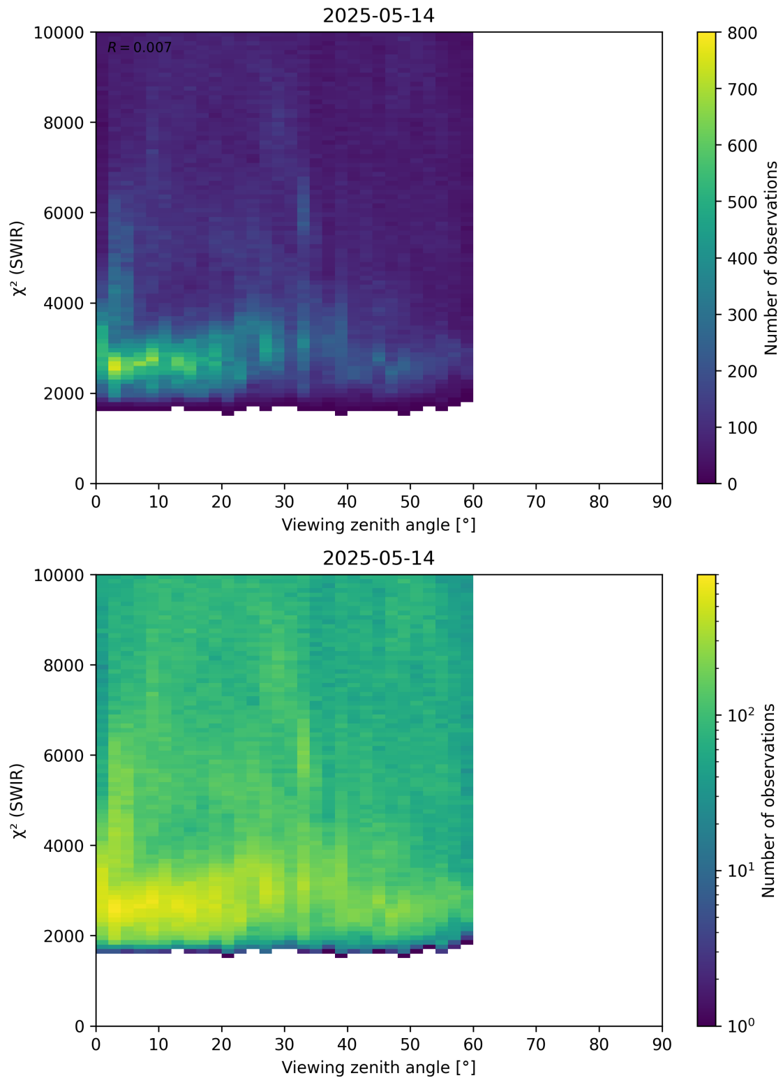
Figure 106: Scatter density plot of “Viewing zenith angle” against “ \chi^2 (SWIR)” for 2025-05-13 to 2025-05-15.
