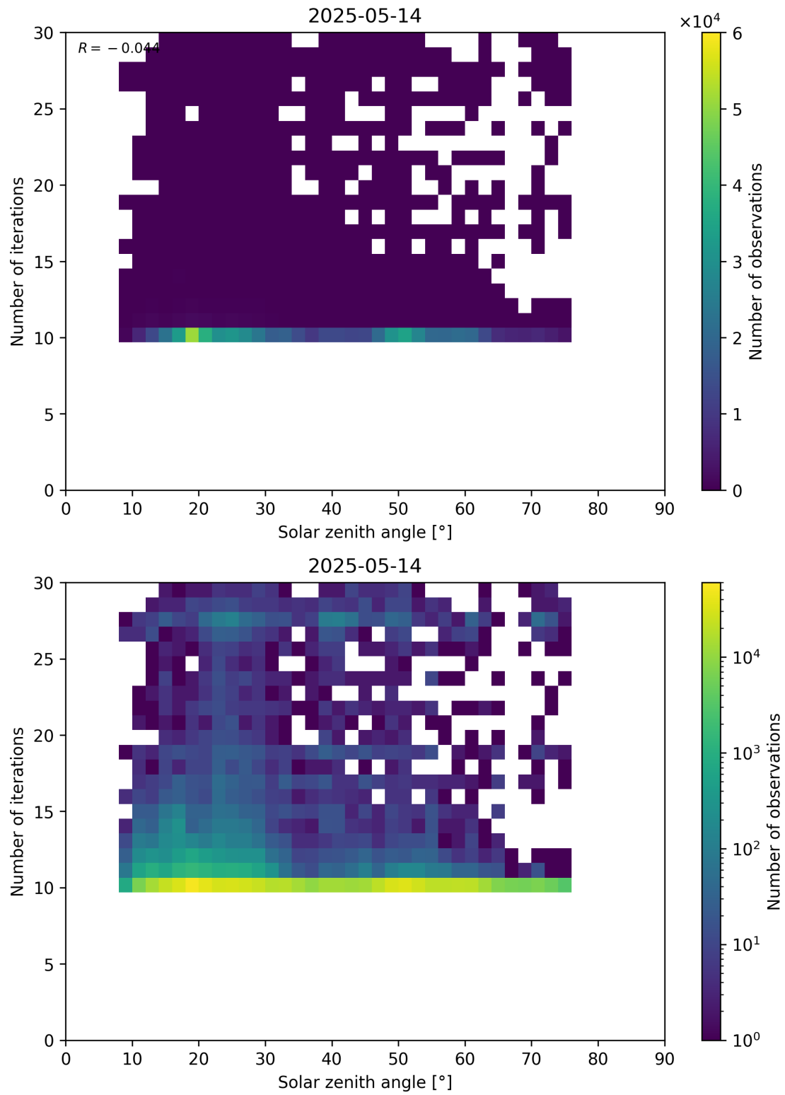
Figure 102: Scatter density plot of “Solar zenith angle” against “Number of iterations” for 2025-05-13 to 2025-05-15.
