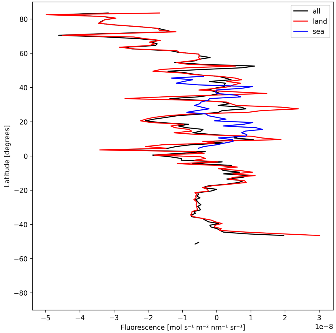
Figure 21: Zonal average of “Fluorescence” for 2025-05-13 to 2025-05-15.
