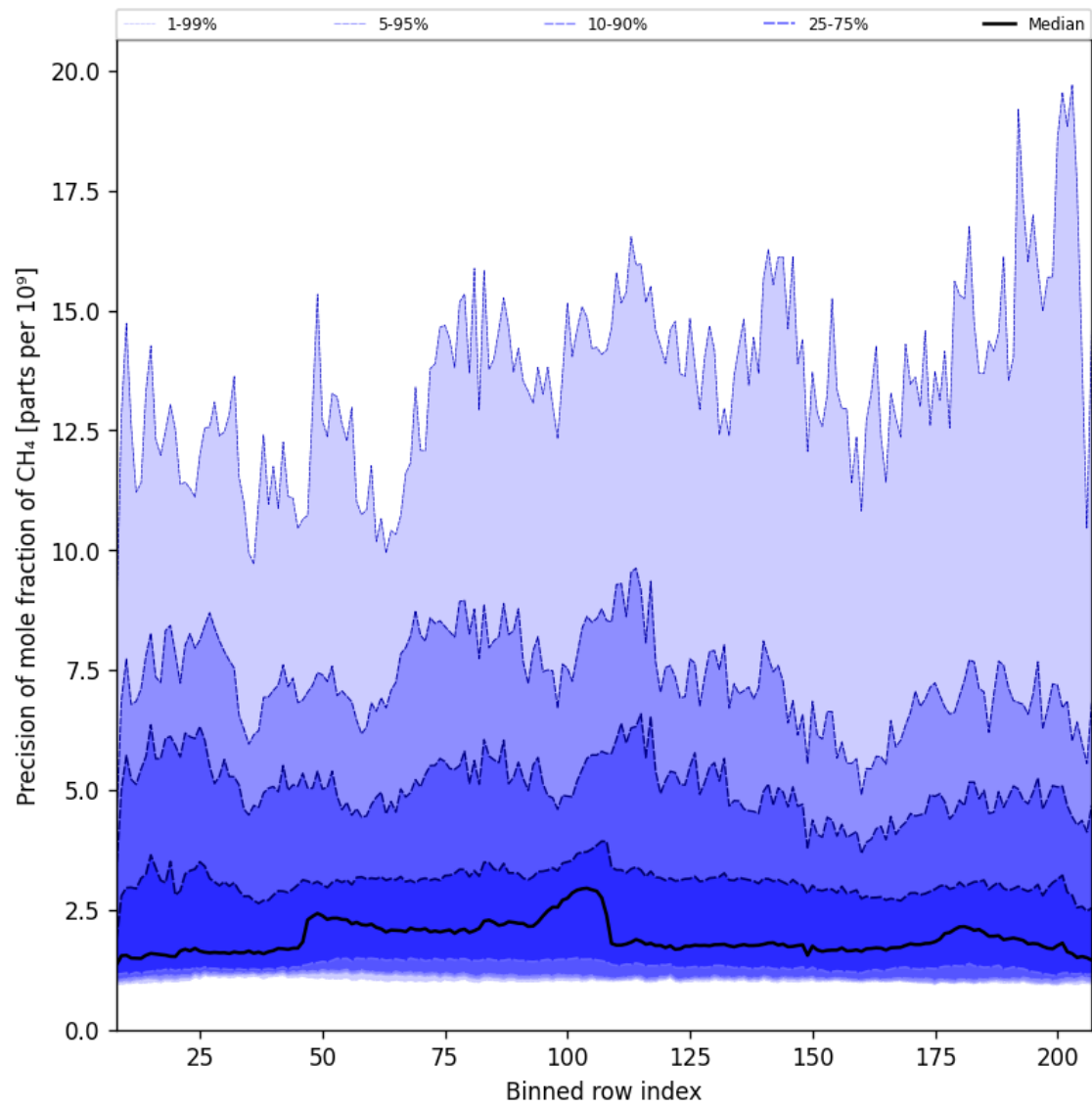
Figure 35: Along track statistics of “Precision of mole fraction of CH 4 ” for 2025-05-13 to 2025-05-15
