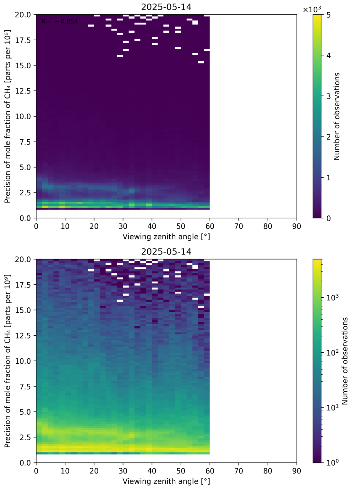
Figure 112: Scatter density plot of “Viewing zenith angle” against “Precision of mole fraction of \text{CH}_4 ” for 2025-05-13 to 2025-05-15.
