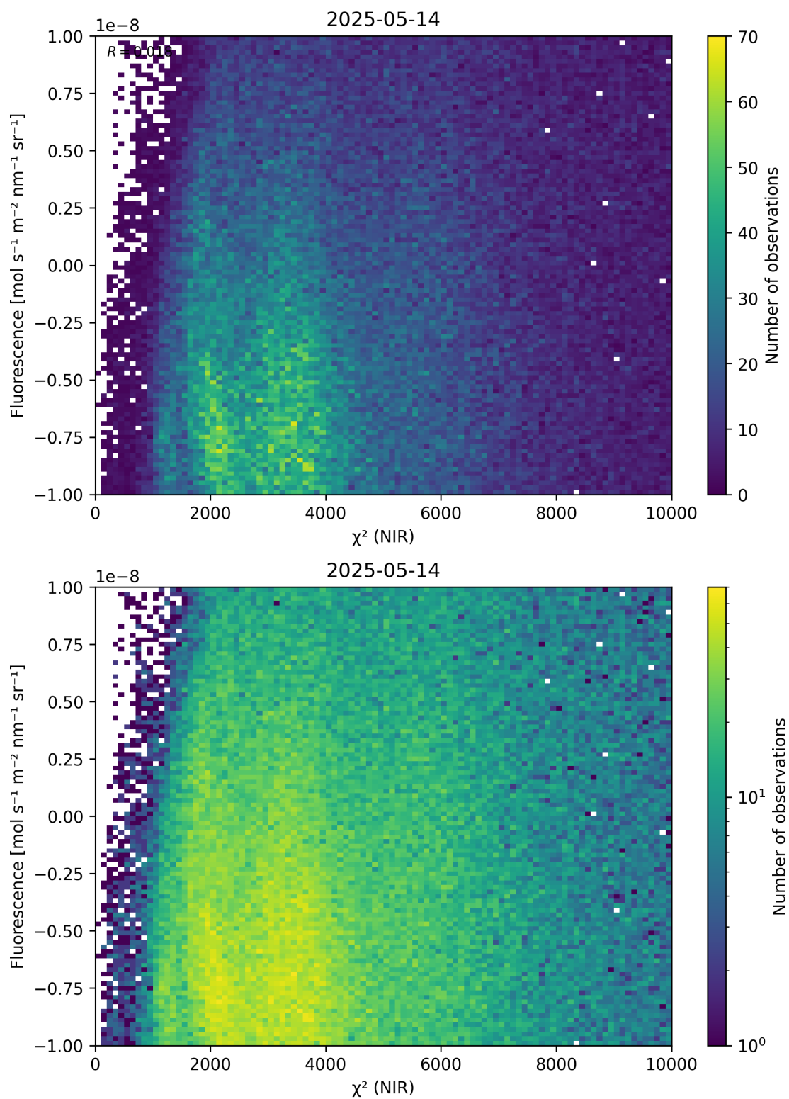
Figure 45: Scatter density plot of “ \chi^2 (NIR)” against “Fluorescence” for 2025-05-13 to 2025-05-15.
