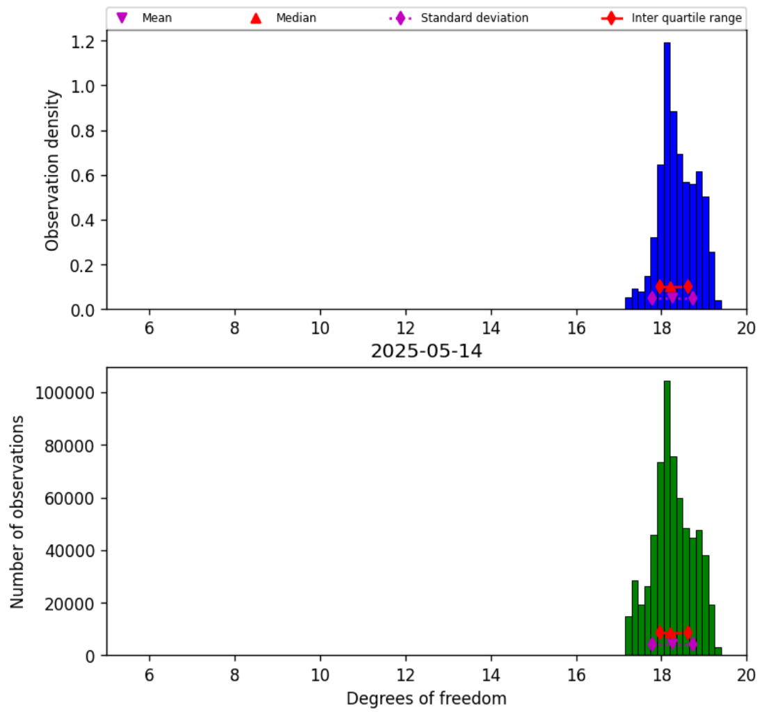
Figure 30: Histogram of "Degrees of freedom" for 2025-05-13 to 2025-05-15
