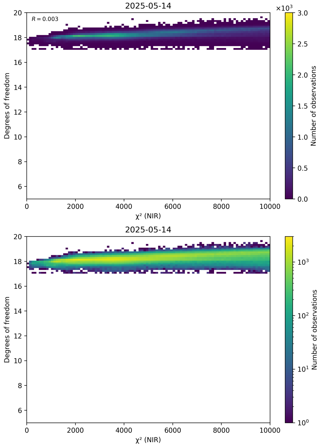
Figure 44: Scatter density plot of “ \chi^2 (NIR)” against “Degrees of freedom” for 2025-05-13 to 2025-05-15.
