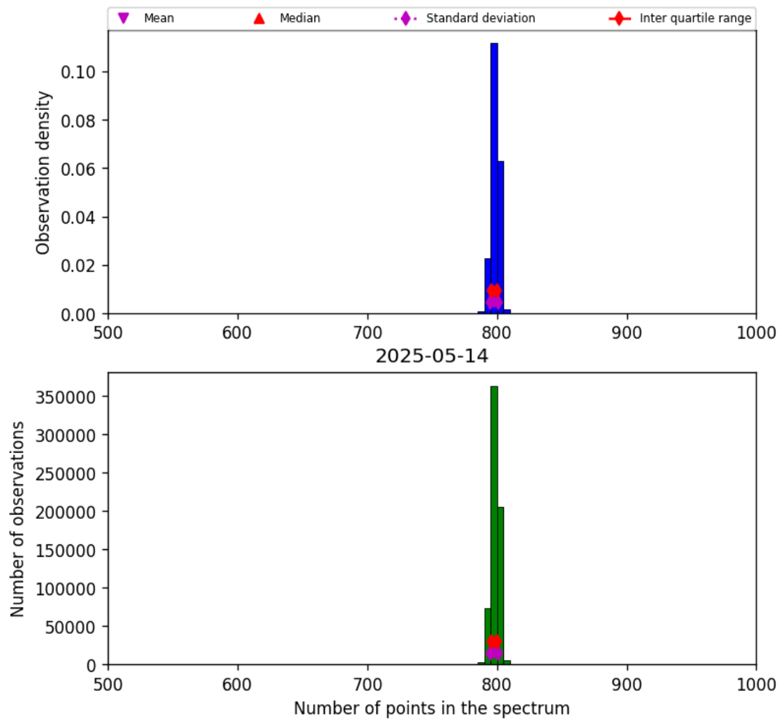
Figure 26: Histogram of “Number of points in the spectrum” for 2025-05-13 to 2025-05-15
