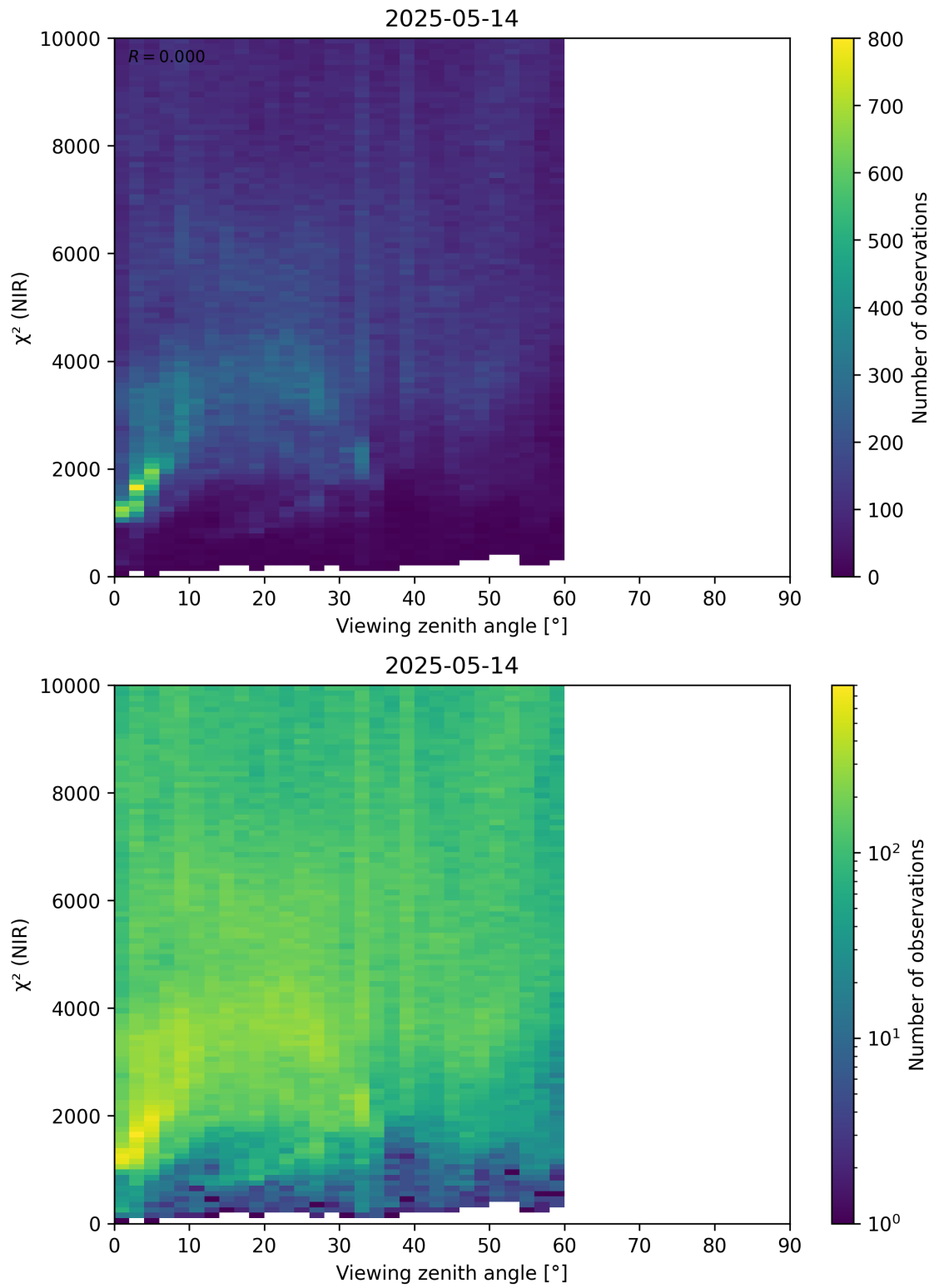
Figure 105: Scatter density plot of “Viewing zenith angle” against “ \chi^2 (NIR)” for 2025-05-13 to 2025-05-15.
