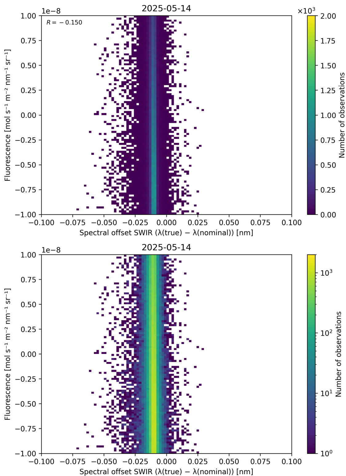
Figure 120: Scatter density plot of “Spectral offset SWIR ( \lambda_{\text{true}} - \lambda_{\text{nominal}} )” against “Fluorescence” for 2025-05-13 to 2025-05-15.
