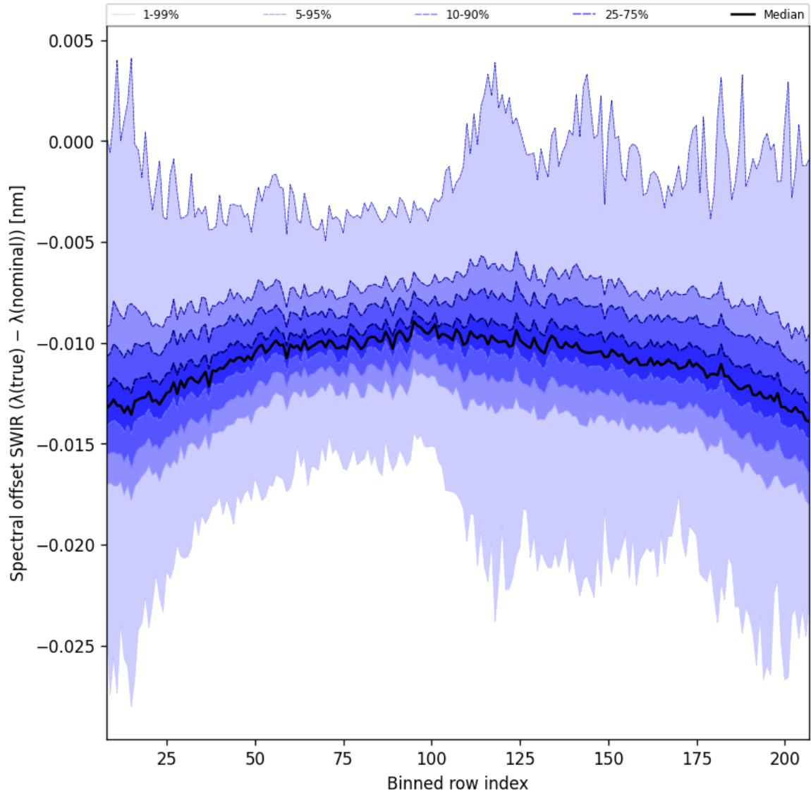
Figure 38: Along track statistics of “Spectral offset SWIR ( \lambda_{\text{true}} - \lambda_{\text{nominal}} )” for 2025-05-13 to 2025-05-15
