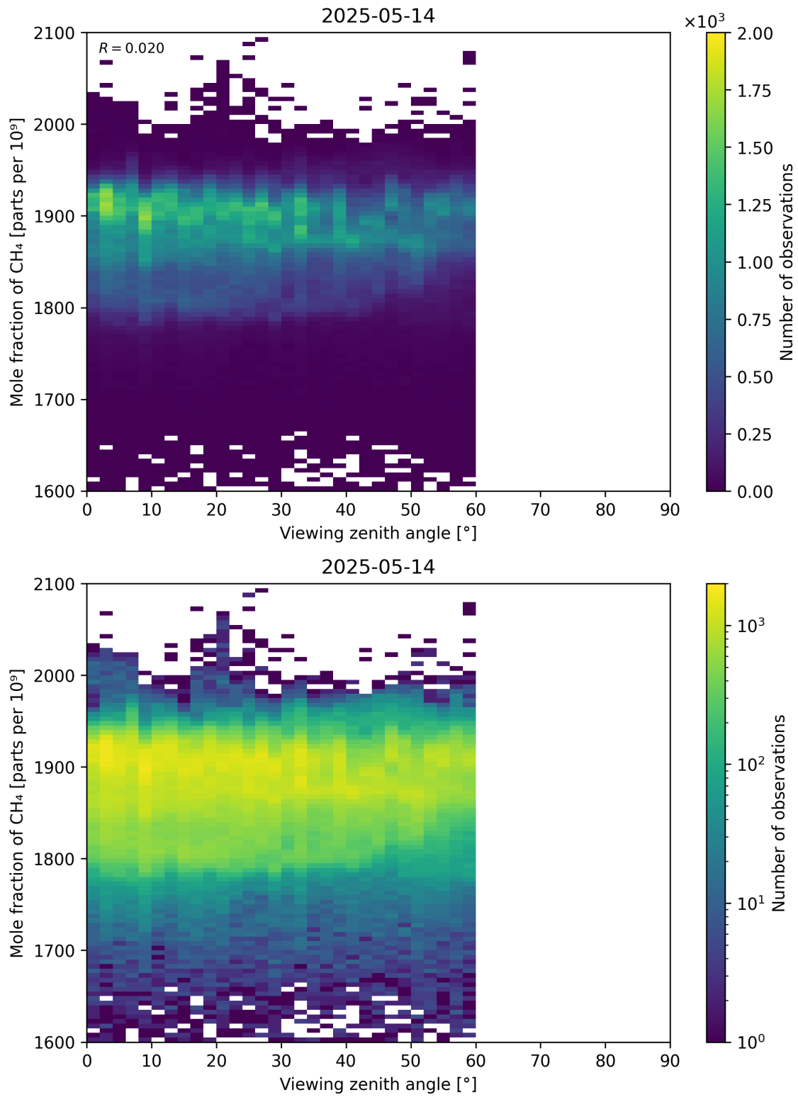
Figure 110: Scatter density plot of “Viewing zenith angle” against “Mole fraction of CH 4 ” for 2025-05-13 to 2025-05-15.
