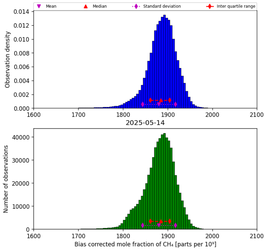
Figure 25: Histogram of “Bias corrected mole fraction of CH 4 ” for 2025-05-13 to 2025-05-15
