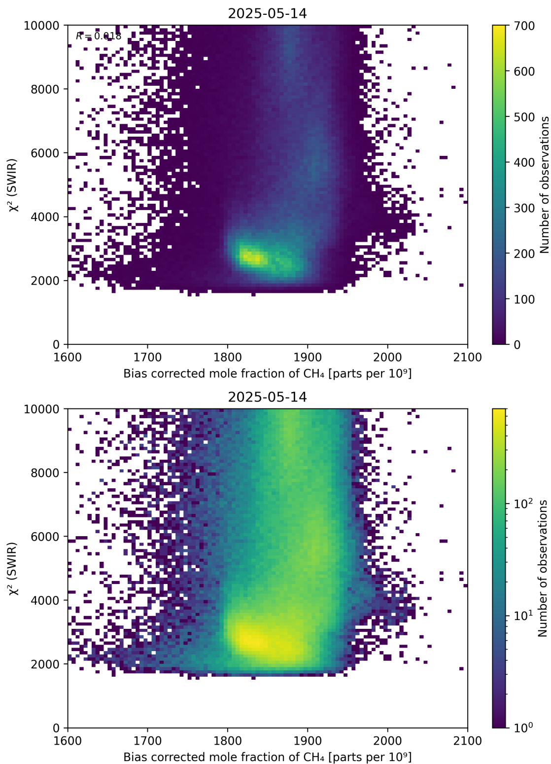
Figure 64: Scatter density plot of “Bias corrected mole fraction of CH 4 ” against “ \chi^2 (SWIR)” for 2025-05-13 to 2025-05-15.
