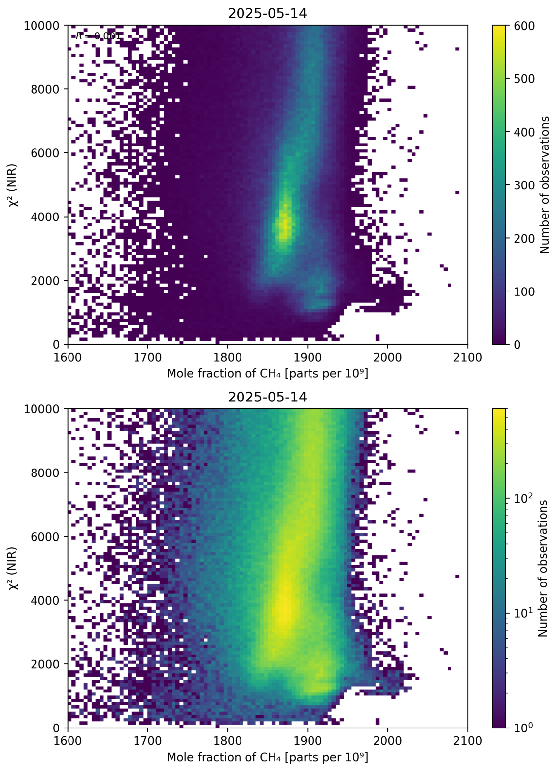
Figure 70: Scatter density plot of “Mole fraction of \text{CH}_4 ” against “ \chi^2 (NIR)” for 2025-05-13 to 2025-05-15.
