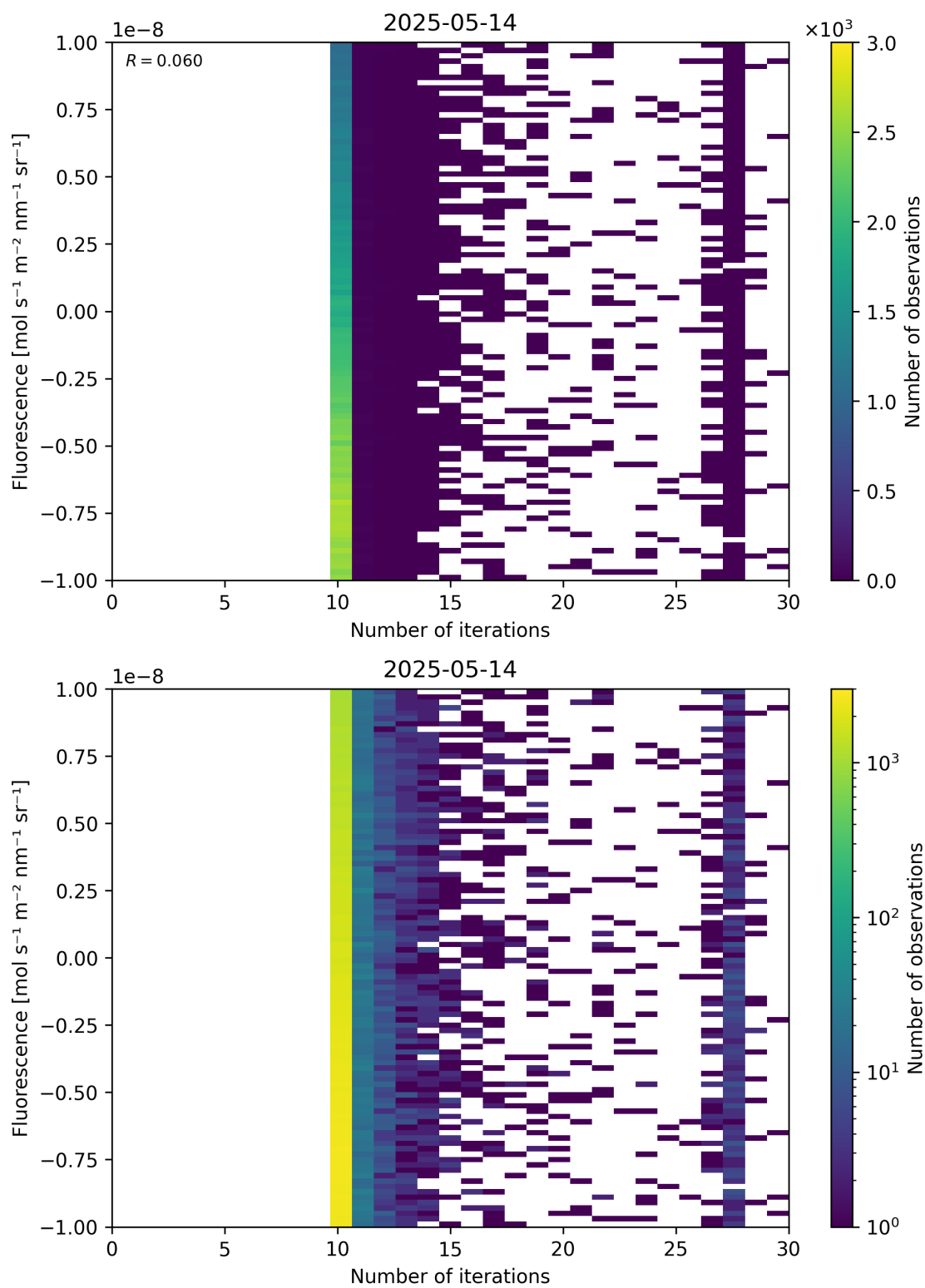
Figure 87: Scatter density plot of “Number of iterations” against “Fluorescence” for 2025-05-13 to 2025-05-15.
