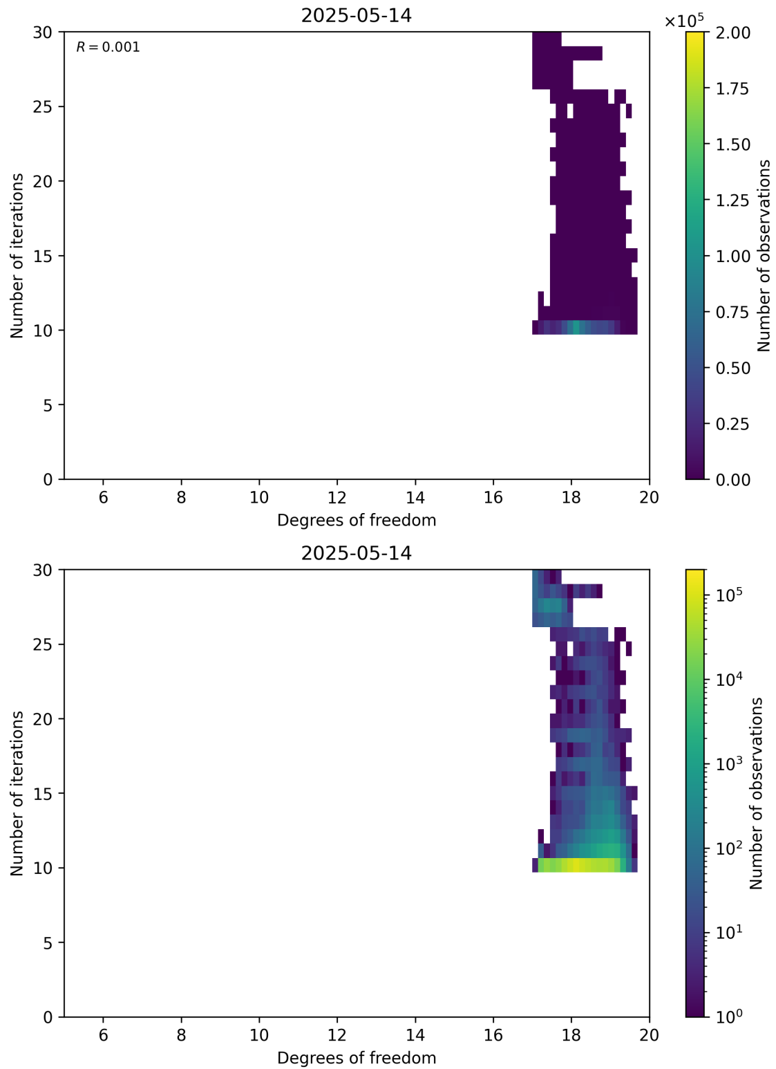
Figure 52: Scatter density plot of “Degrees of freedom” against “Number of iterations” for 2025-05-13 to 2025-05-15.
