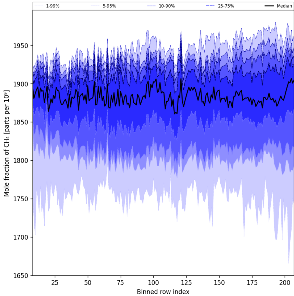
Figure 34: Along track statistics of “Mole fraction of CH 4 ” for 2025-05-13 to 2025-05-15
