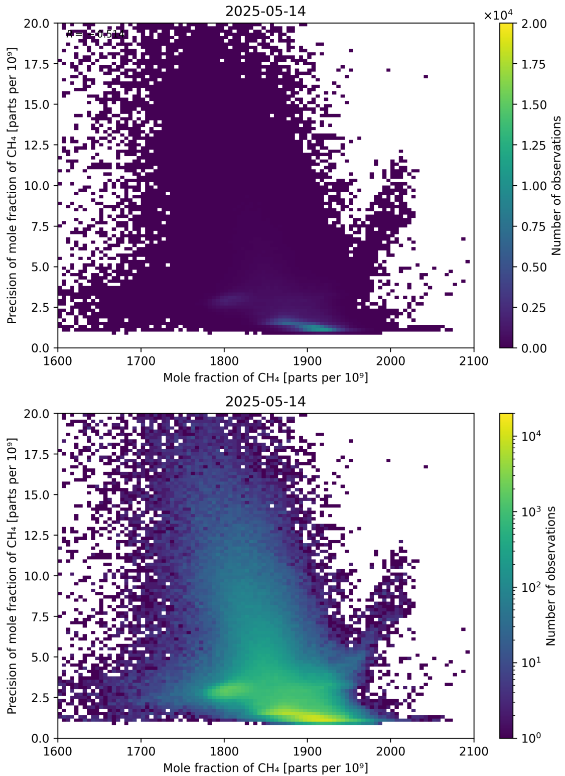
Figure 75: Scatter density plot of “Mole fraction of CH 4 ” against “Precision of mole fraction of CH 4 ” for 2025-05-13 to 2025-05-15.
