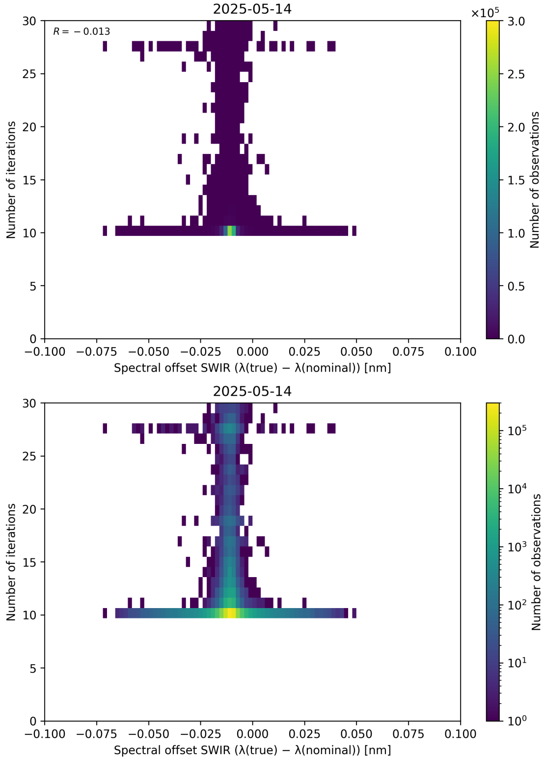
Figure 121: Scatter density plot of “Spectral offset SWIR ( \lambda_{\text{true}} - \lambda_{\text{nominal}} )” against “Number of iterations” for 2025-05-13 to 2025-05-15.
