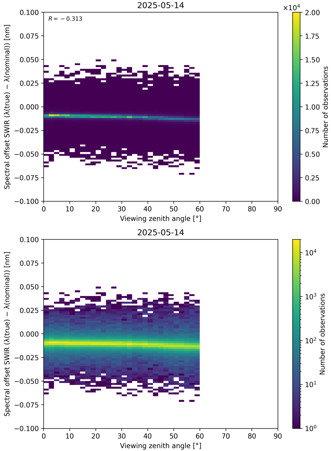
Figure 116: Scatter density plot of “Viewing zenith angle” against “Spectral offset SWIR ( \lambda_{\text{true}} - \lambda_{\text{nominal}} )” for 2025-05-13 to 2025-05-15.
