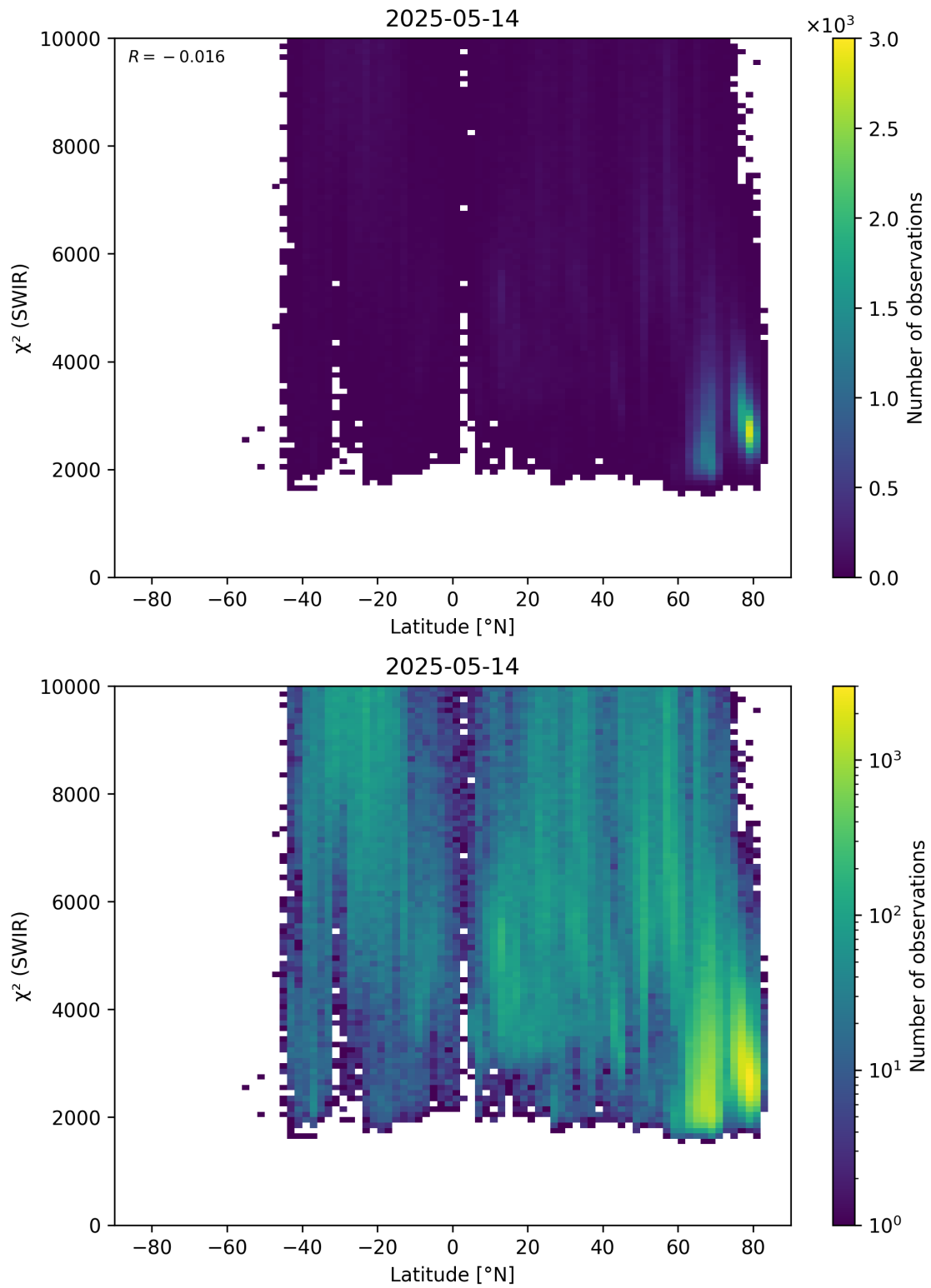
Figure 54: Scatter density plot of “Latitude” against “ \chi^2 (SWIR)” for 2025-05-13 to 2025-05-15.
