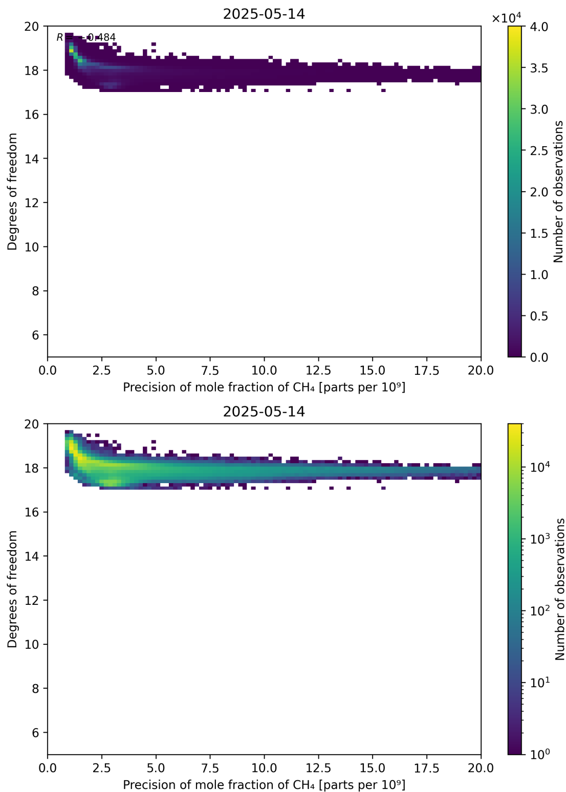
Figure 80: Scatter density plot of “Precision of mole fraction of CH 4 ” against “Degrees of freedom” for 2025-05-13 to 2025-05-15.
