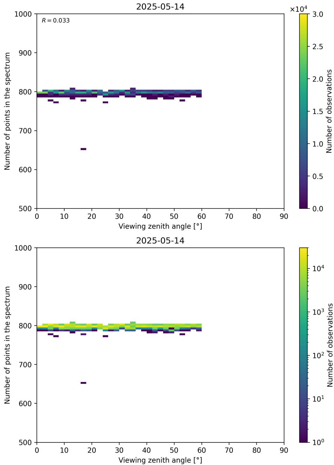
Figure 114: Scatter density plot of “Viewing zenith angle” against “Number of points in the spectrum” for 2025-05-13 to 2025-05-15.
