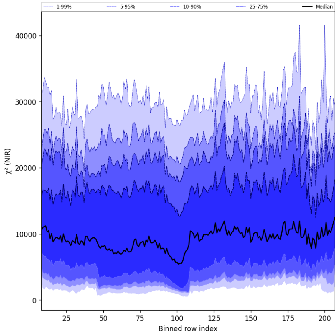
Figure 40: Along track statistics of “ \chi^2 (NIR)” for 2025-05-13 to 2025-05-15
