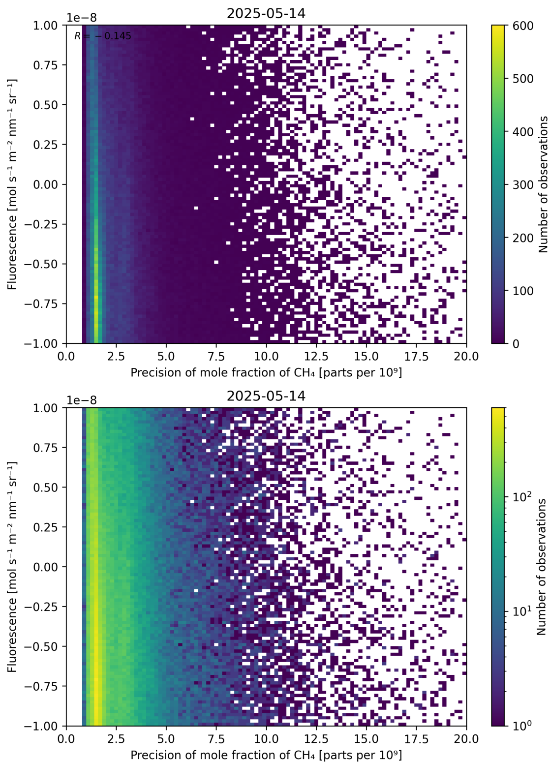
Figure 81: Scatter density plot of “Precision of mole fraction of \text{CH}_4 ” against “Fluorescence” for 2025-05-13 to 2025-05-15.
