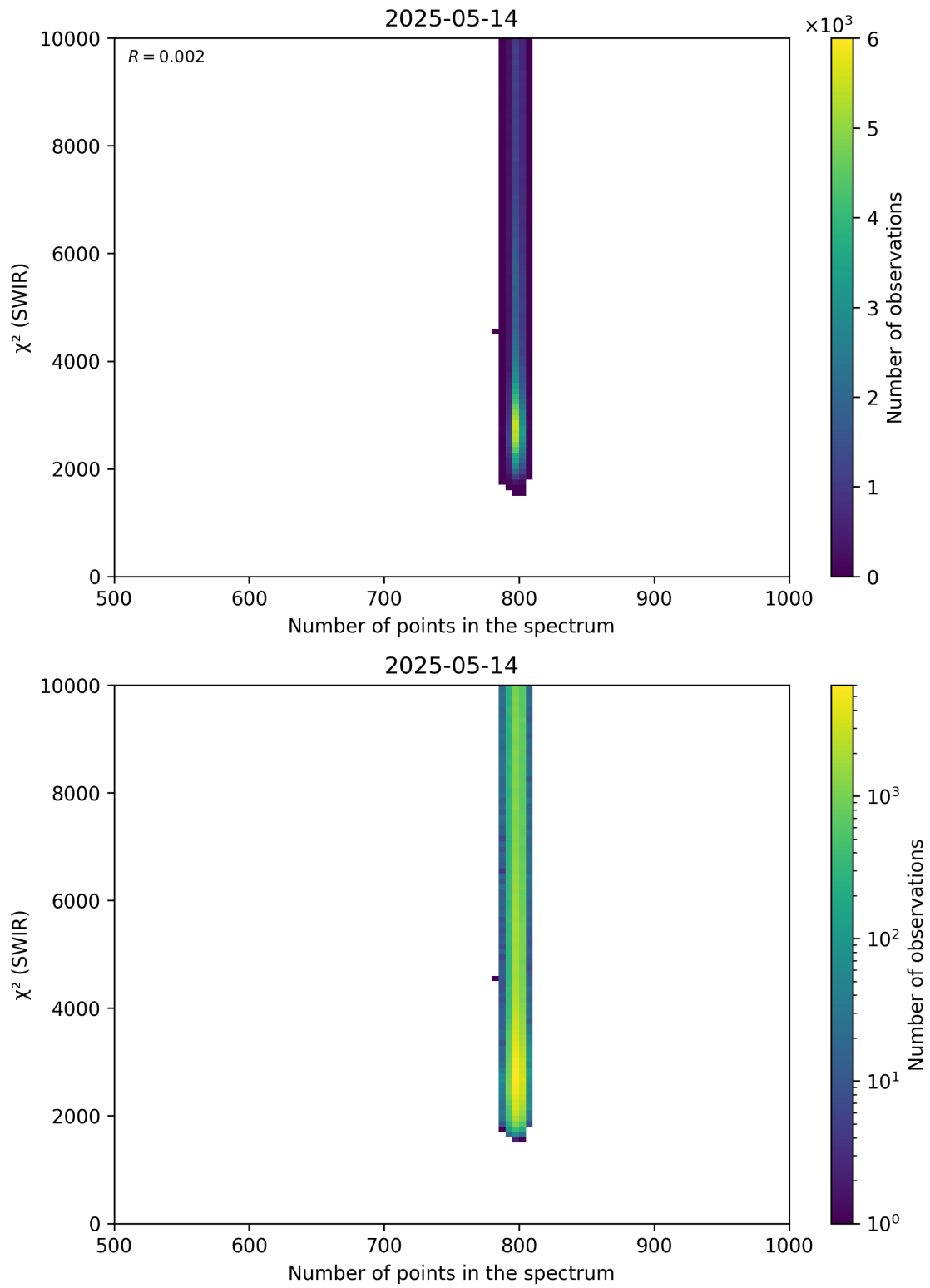
Figure 89: Scatter density plot of “Number of points in the spectrum” against “ \chi^2 (SWIR)” for 2025-05-13 to 2025-05-15.
