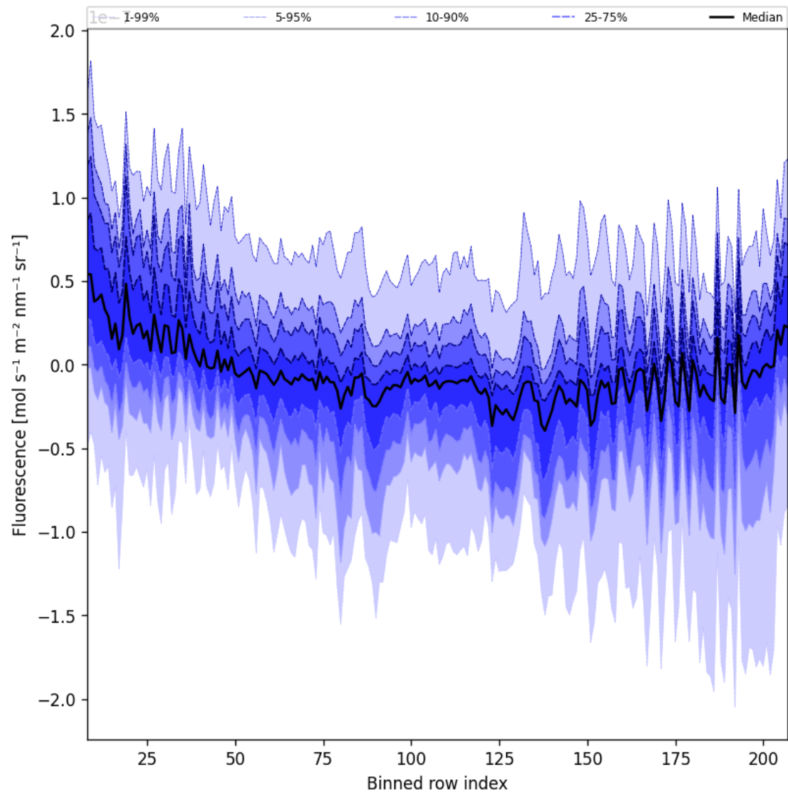
Figure 43: Along track statistics of “Fluorescence” for 2025-05-13 to 2025-05-15
