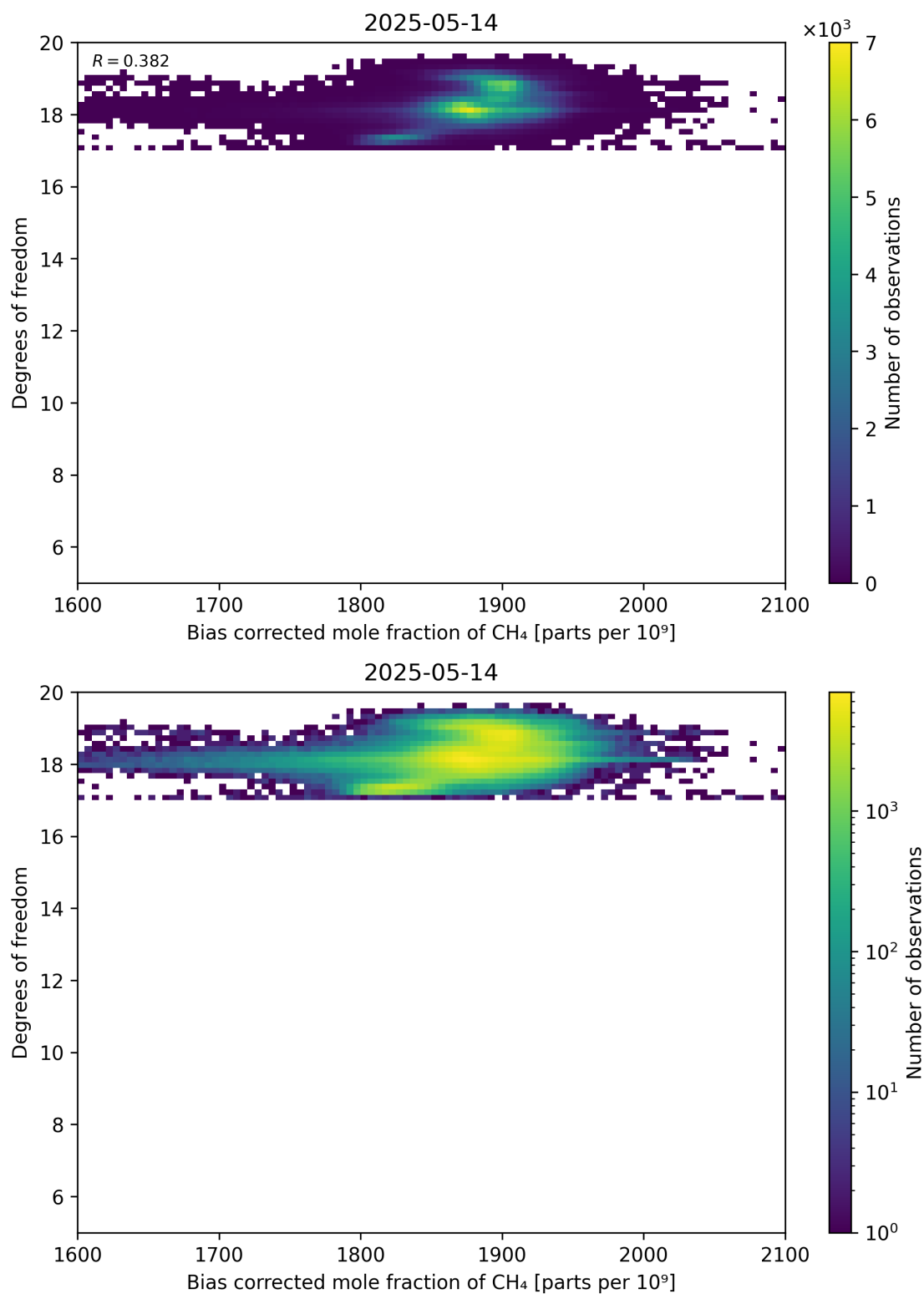
Figure 65: Scatter density plot of “Bias corrected mole fraction of CH 4 ” against “Degrees of freedom” for 2025-05-13 to 2025-05-15.
