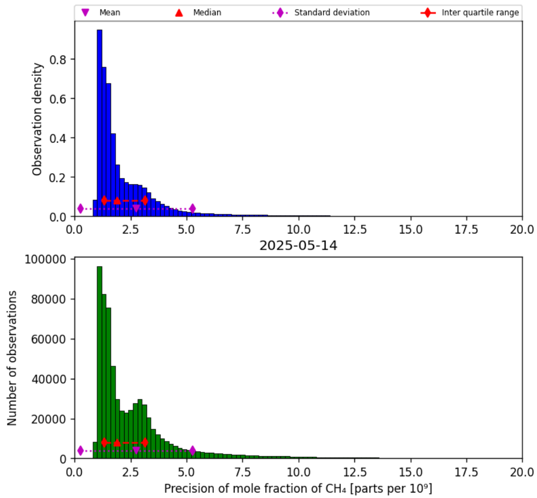
Figure 24: Histogram of “Precision of mole fraction of CH 4 ” for 2025-05-13 to 2025-05-15
