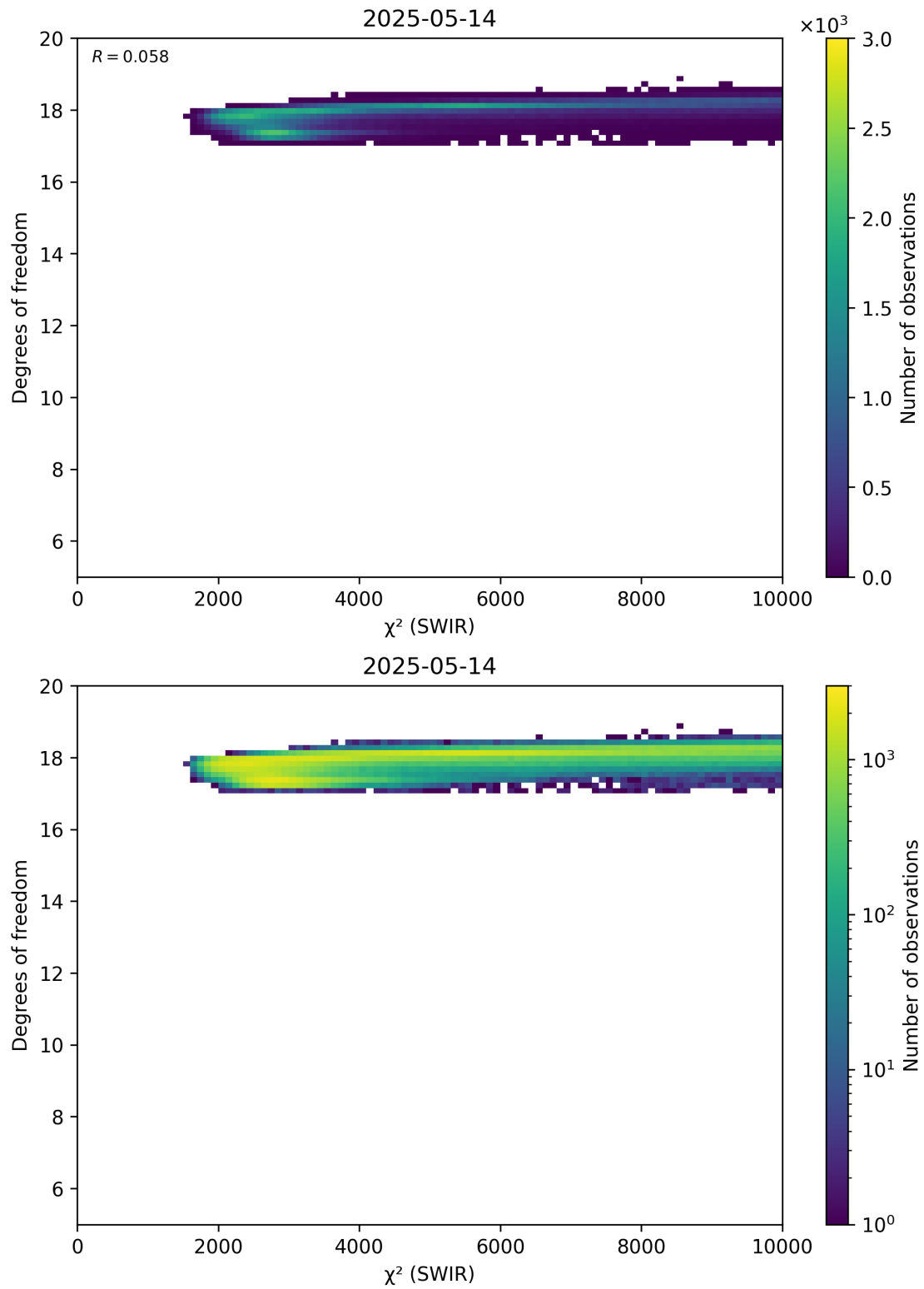
Figure 48: Scatter density plot of “ \chi^2 (SWIR)” against “Degrees of freedom” for 2025-05-13 to 2025-05-15.
