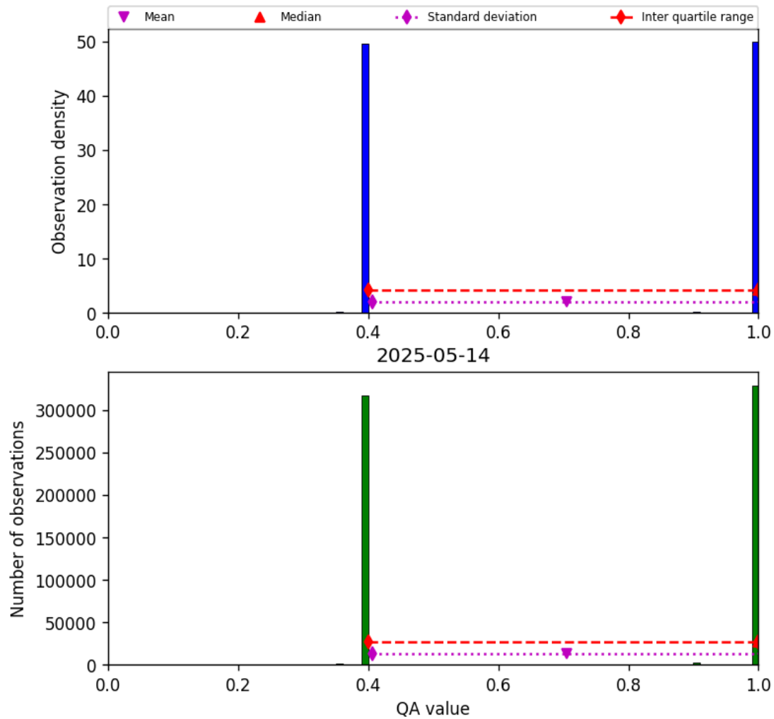
Figure 22: Histogram of “QA value” for 2025-05-13 to 2025-05-15
