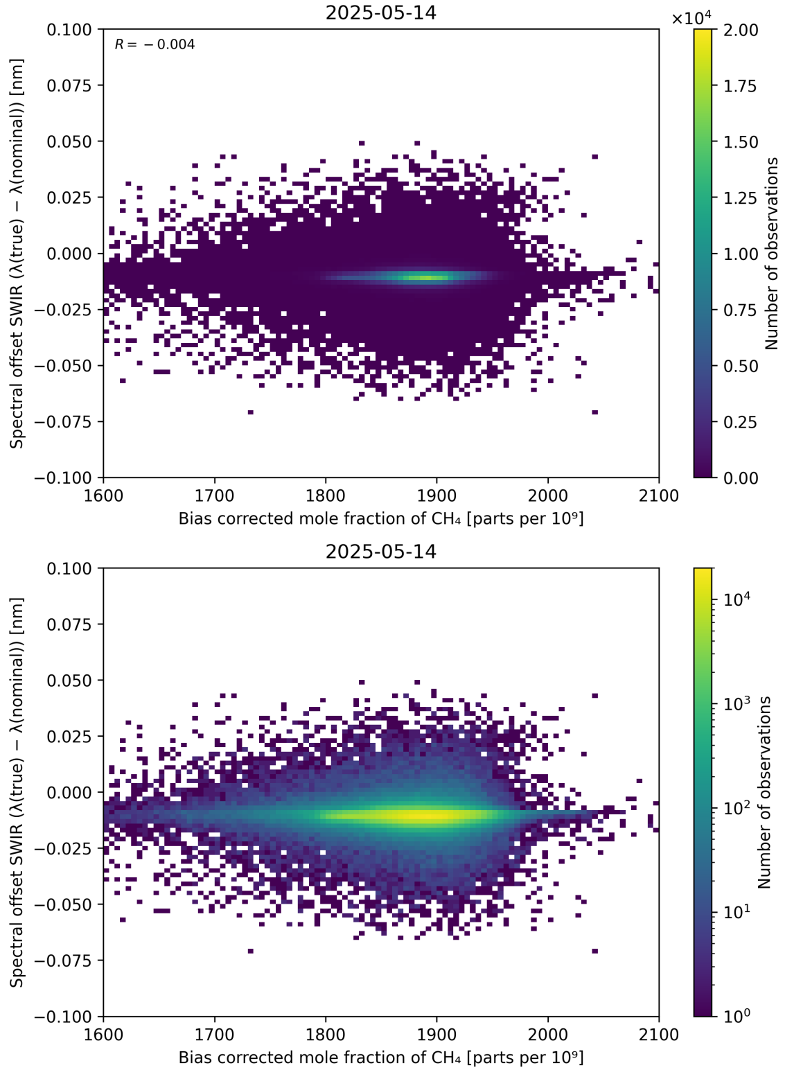
Figure 69: Scatter density plot of “Bias corrected mole fraction of \text{CH}_4 ” against “Spectral offset SWIR ( \lambda_{\text{true}} - \lambda_{\text{nominal}} )” for 2025-05-13 to 2025-05-15.
