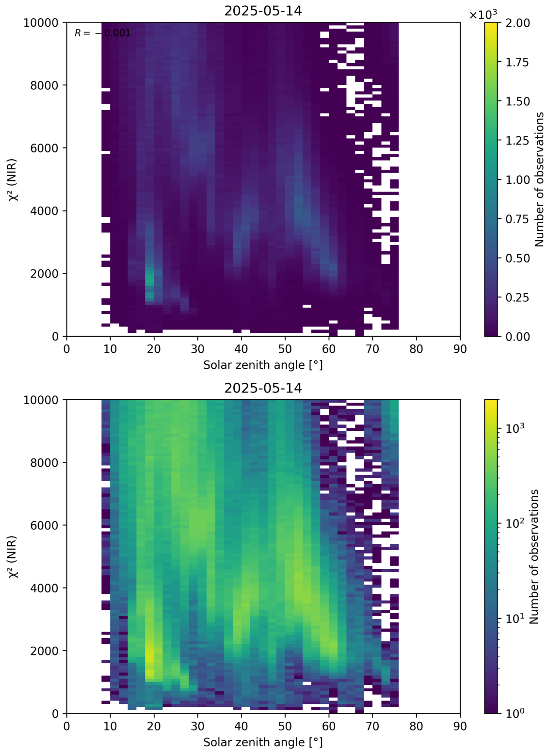
Figure 94: Scatter density plot of “Solar zenith angle” against “ \chi^2 (NIR)” for 2025-05-13 to 2025-05-15.
