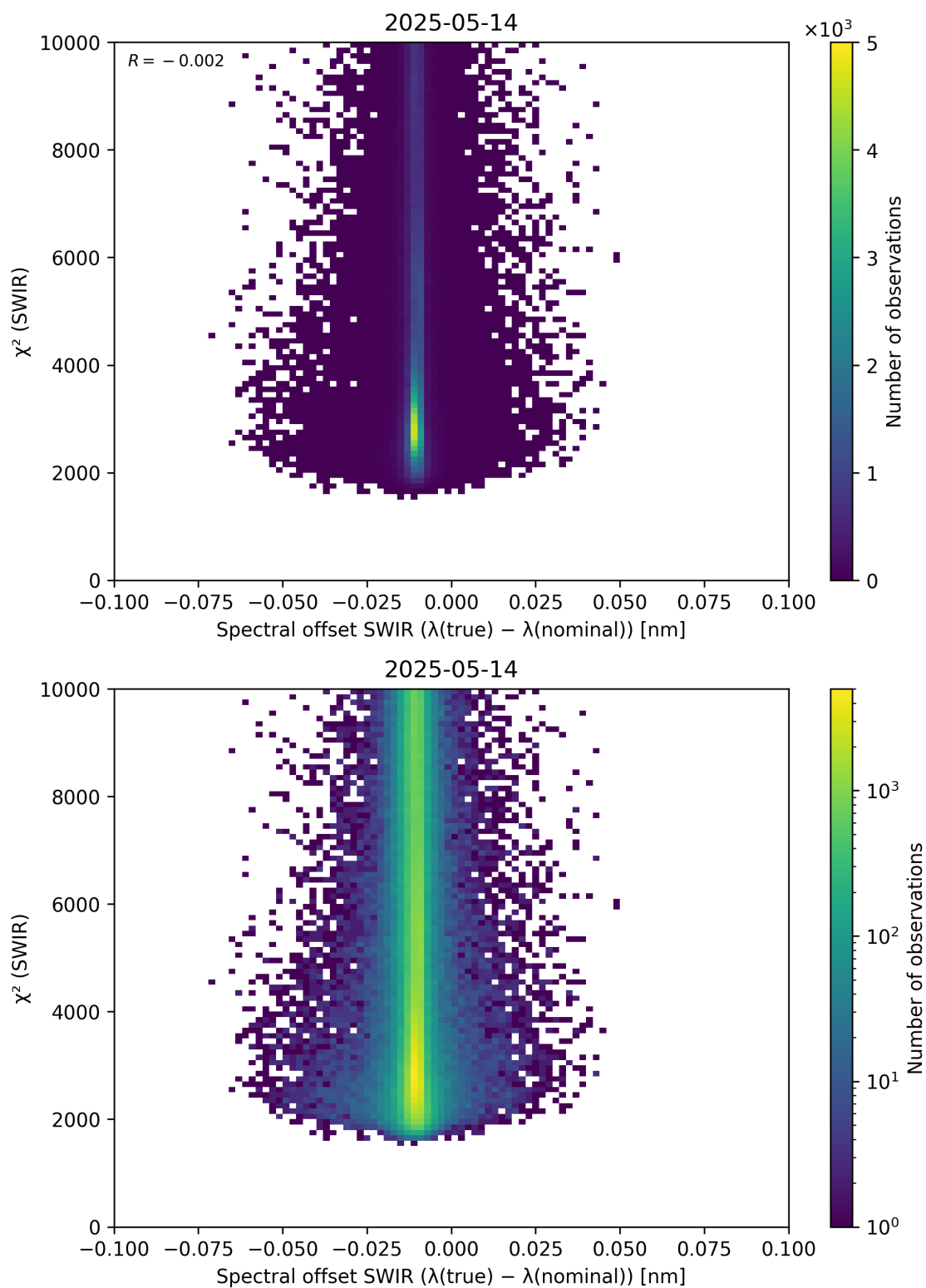
Figure 118: Scatter density plot of “Spectral offset SWIR ( \lambda_{\text{true}} - \lambda_{\text{nominal}} )” against “ \chi^2 (SWIR)” for 2025-05-13 to 2025-05-15.
