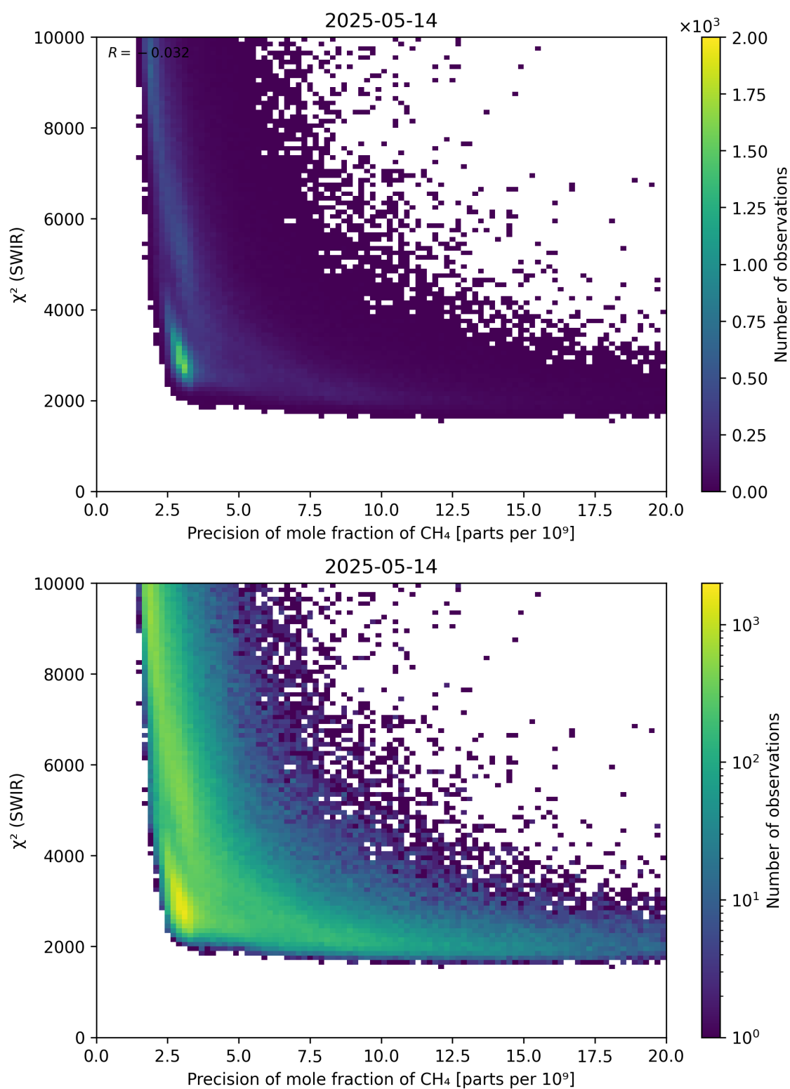
Figure 79: Scatter density plot of “Precision of mole fraction of \text{CH}_4 ” against “ \chi^2 (SWIR)” for 2025-05-13 to 2025-05-15.
