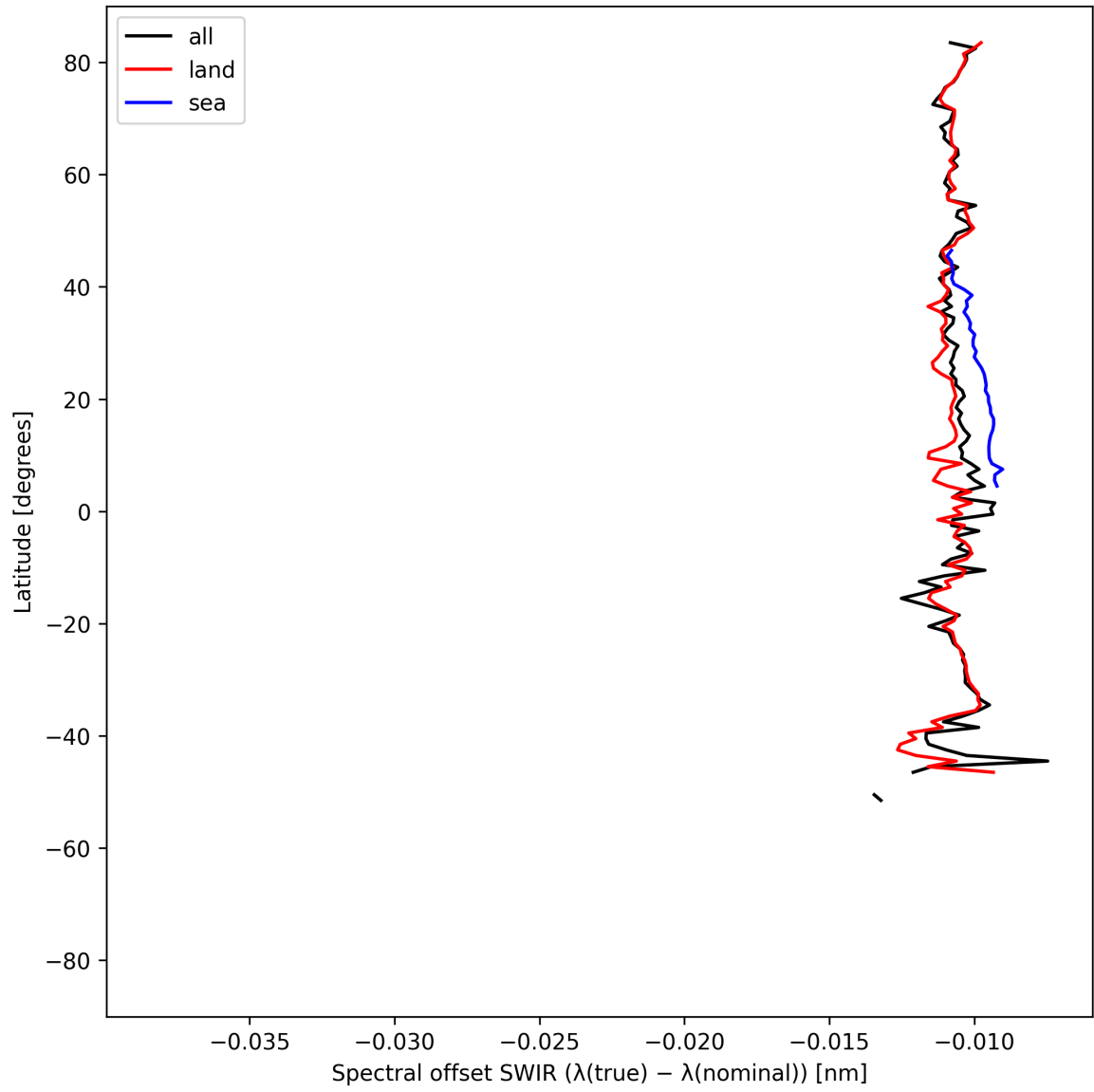
Figure 16: Zonal average of “Spectral offset SWIR ( \lambda_{\text{true}} - \lambda_{\text{nominal}} )” for 2025-05-13 to 2025-05-15.
