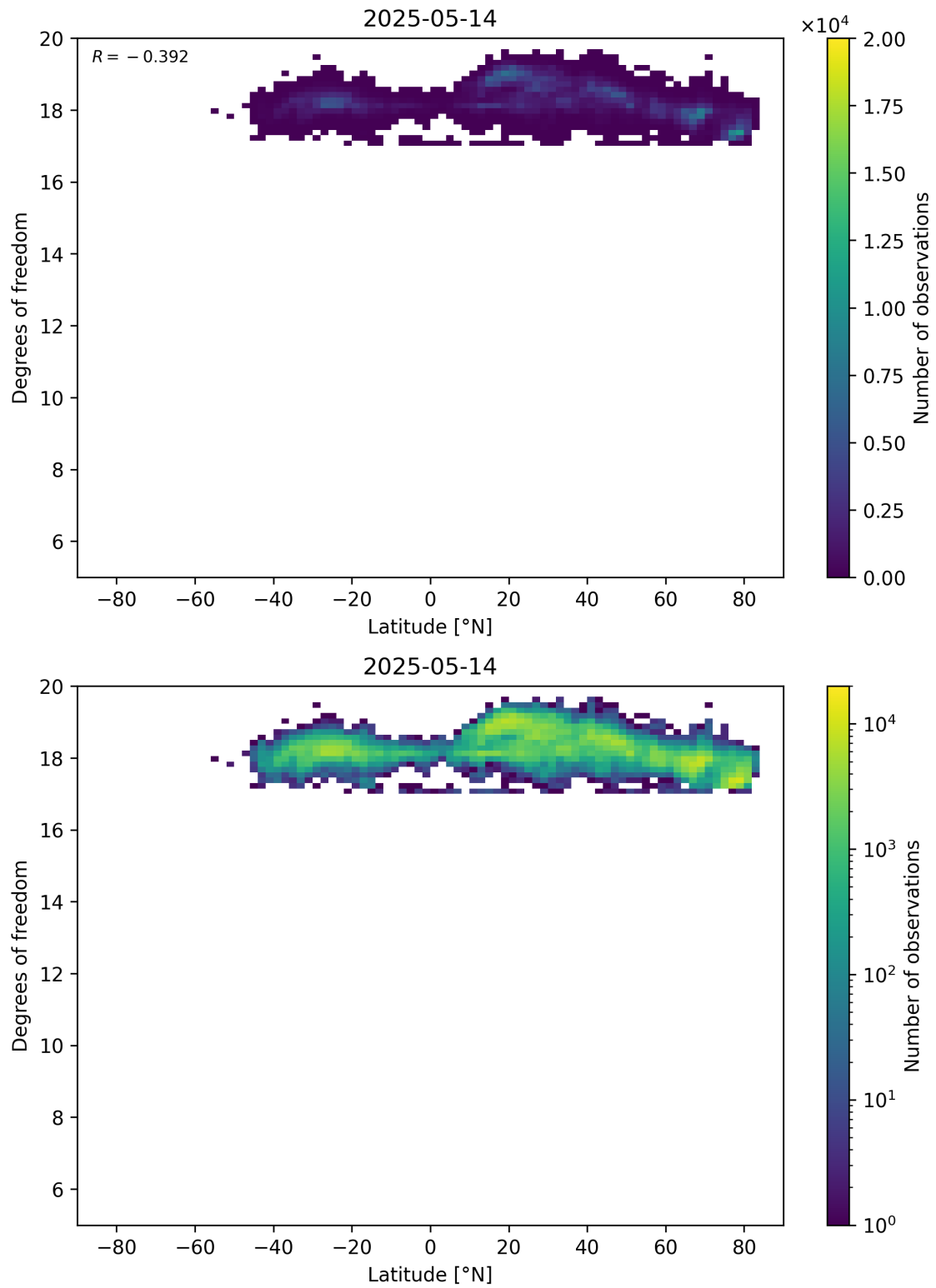
Figure 55: Scatter density plot of “Latitude” against “Degrees of freedom” for 2025-05-13 to 2025-05-15.
