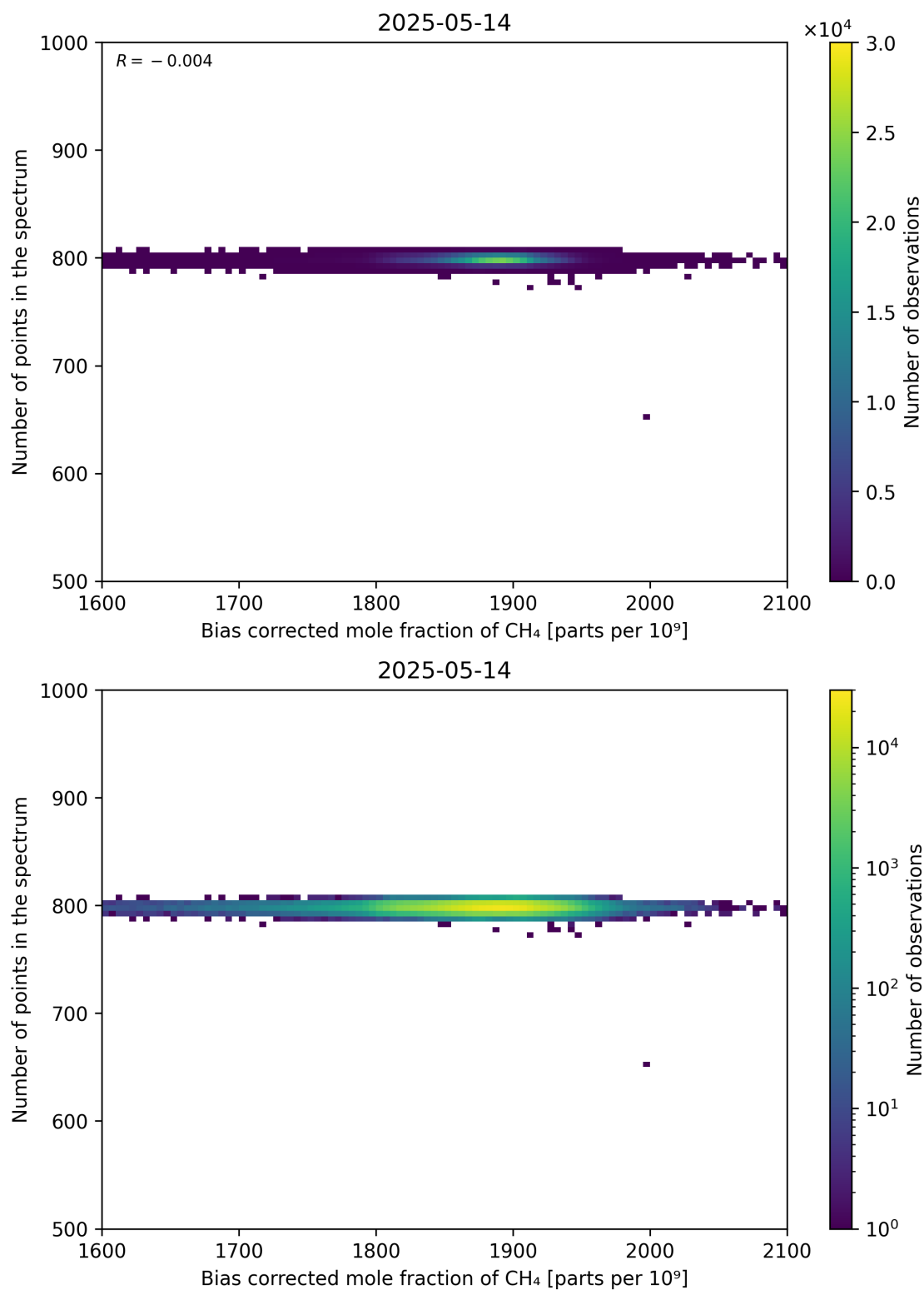
Figure 68: Scatter density plot of “Bias corrected mole fraction of CH 4 ” against “Number of points in the spectrum” for 2025-05-13 to 2025-05-15.
