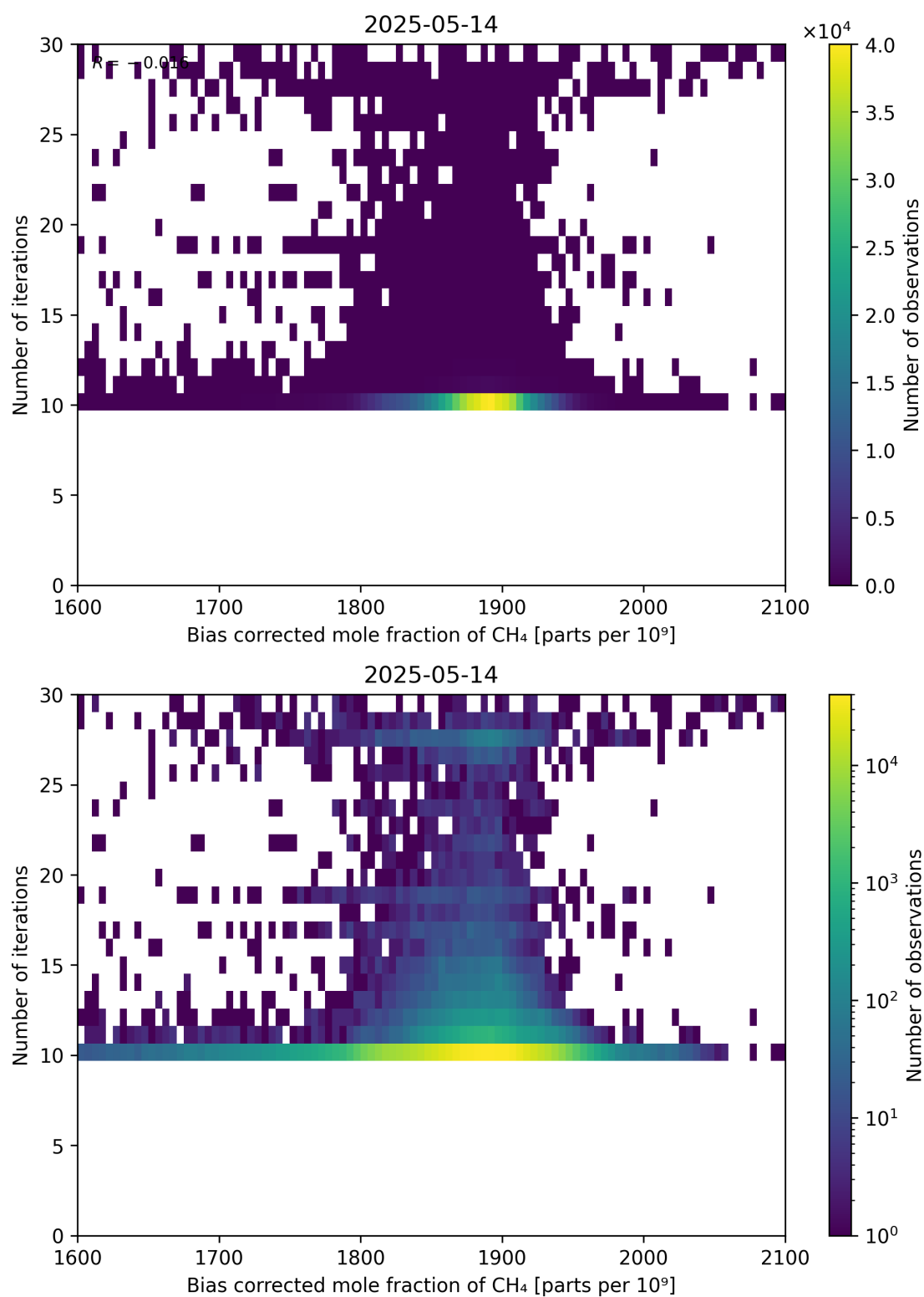
Figure 67: Scatter density plot of “Bias corrected mole fraction of \text{CH}_4 ” against “Number of iterations” for 2025-05-13 to 2025-05-15.
