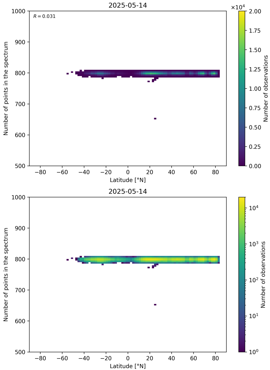
Figure 61: Scatter density plot of “Latitude” against “Number of points in the spectrum” for 2025-05-13 to 2025-05-15.
