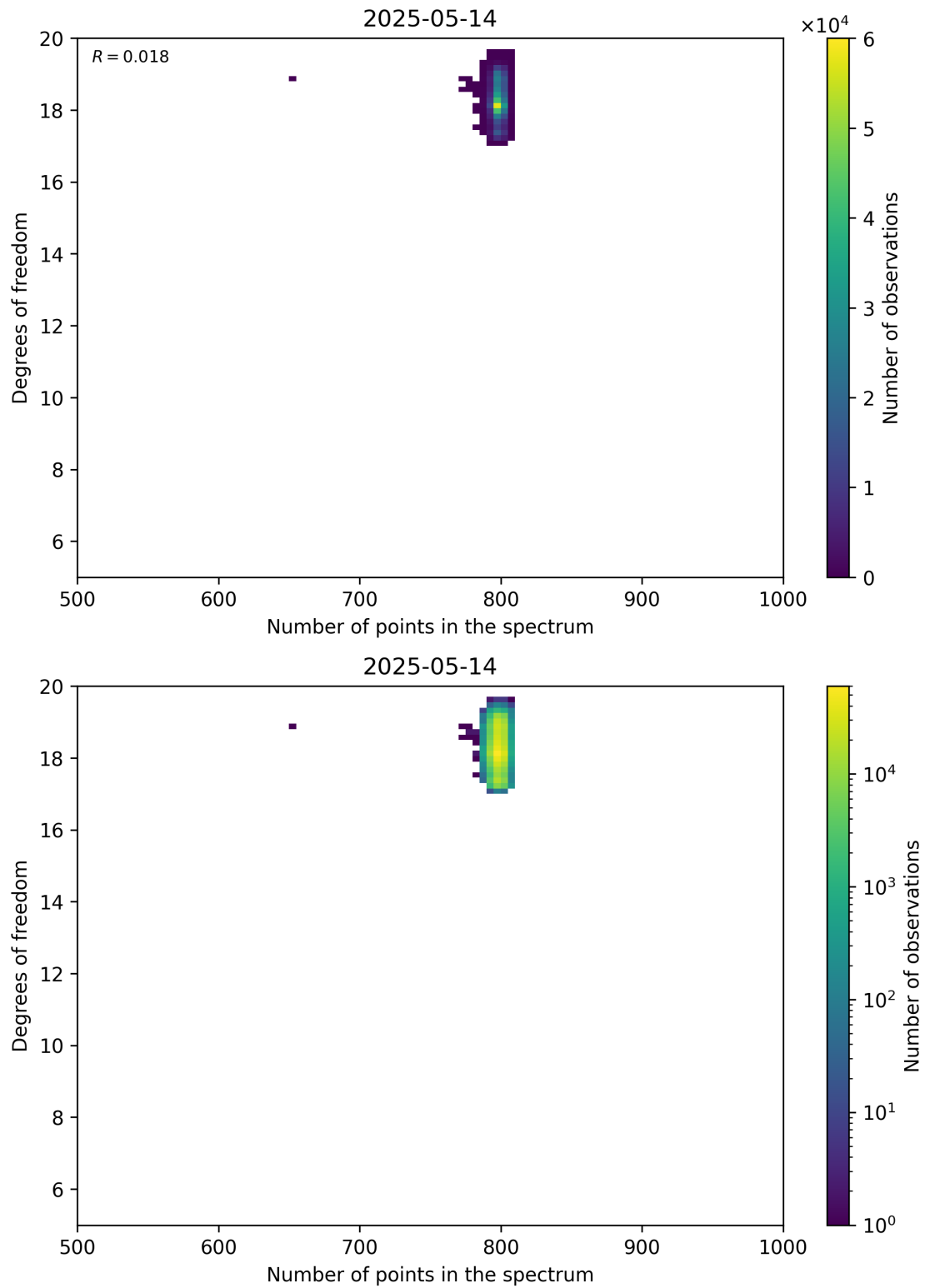
Figure 90: Scatter density plot of “Number of points in the spectrum” against “Degrees of freedom” for 2025-05-13 to 2025-05-15.
