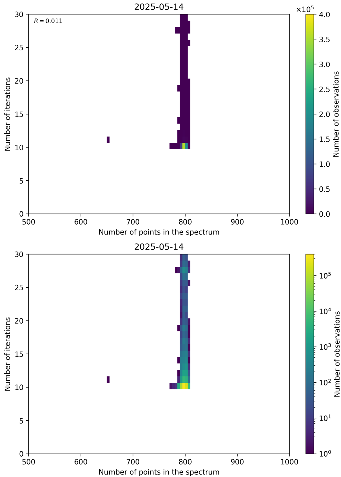
Figure 92: Scatter density plot of “Number of points in the spectrum” against “Number of iterations” for 2025-05-13 to 2025-05-15.
