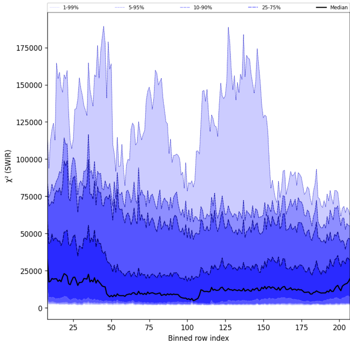
Figure 39: Along track statistics of “ \chi^2 (SWIR)” for 2025-05-13 to 2025-05-15
