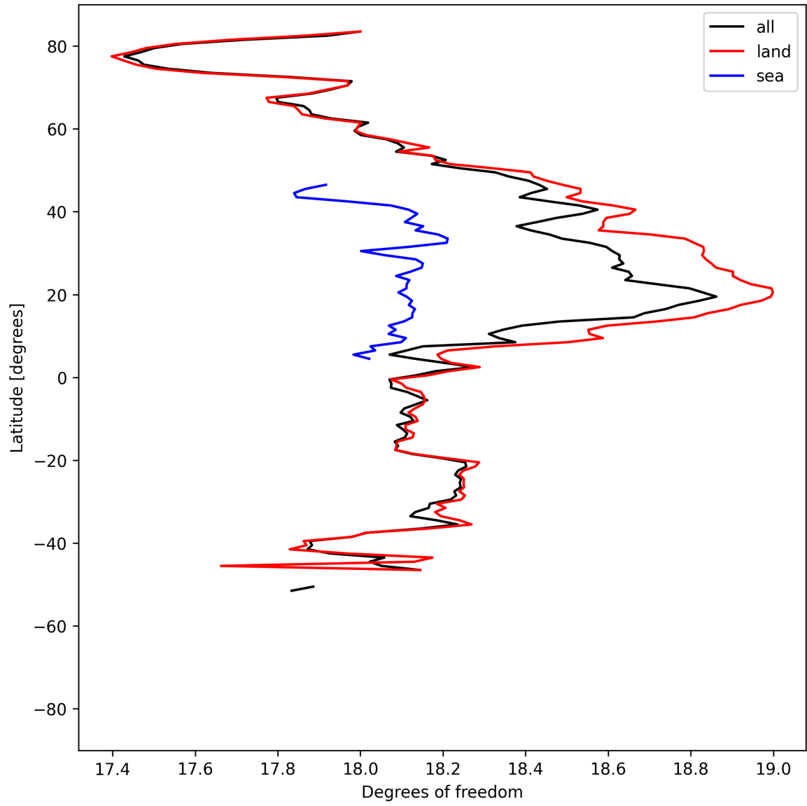
Figure 19: Zonal average of “Degrees of freedom” for 2025-05-13 to 2025-05-15.
