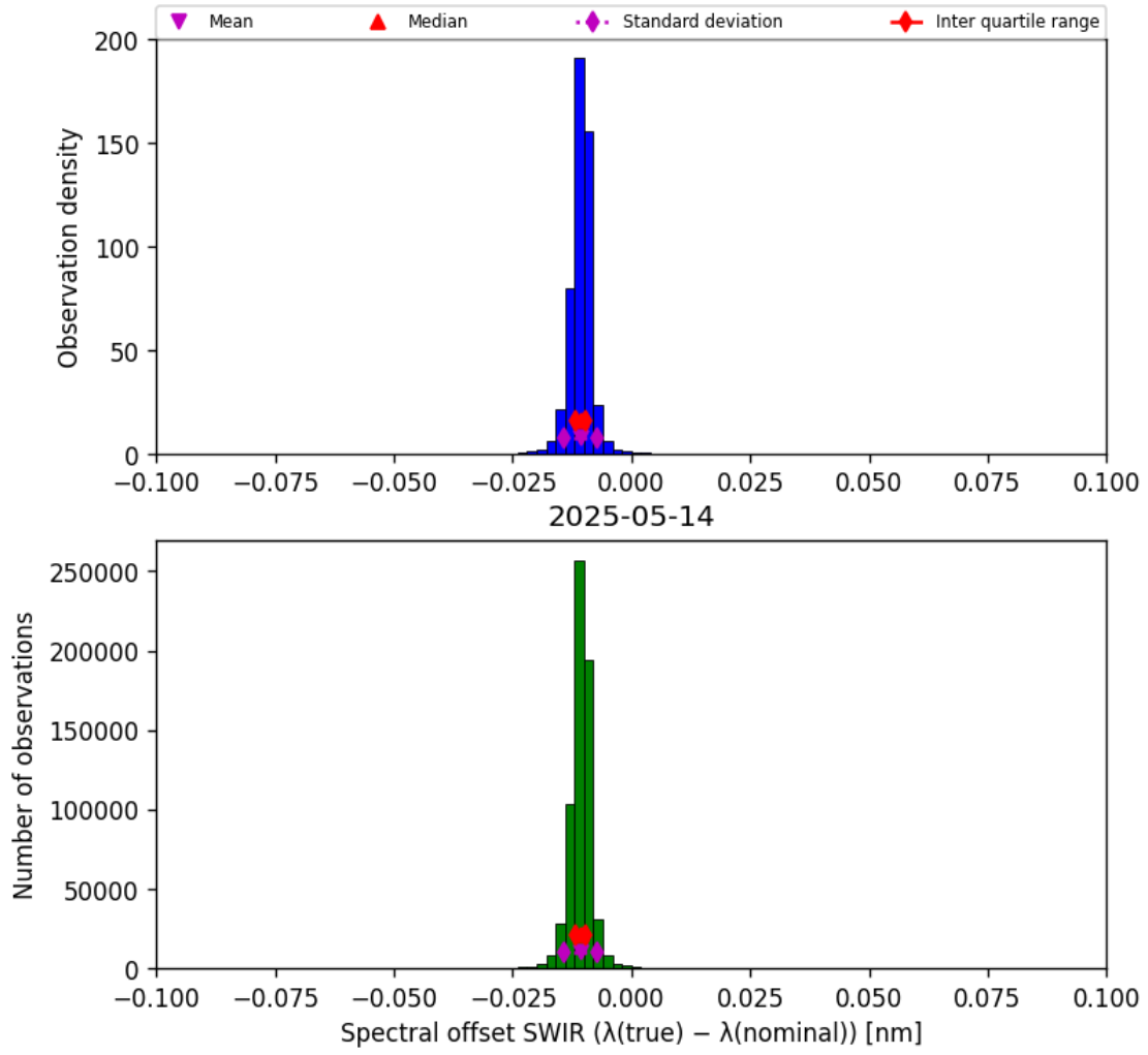
Figure 27: Histogram of “Spectral offset SWIR ( \lambda_{\text{true}} - \lambda_{\text{nominal}} )” for 2025-05-13 to 2025-05-15
