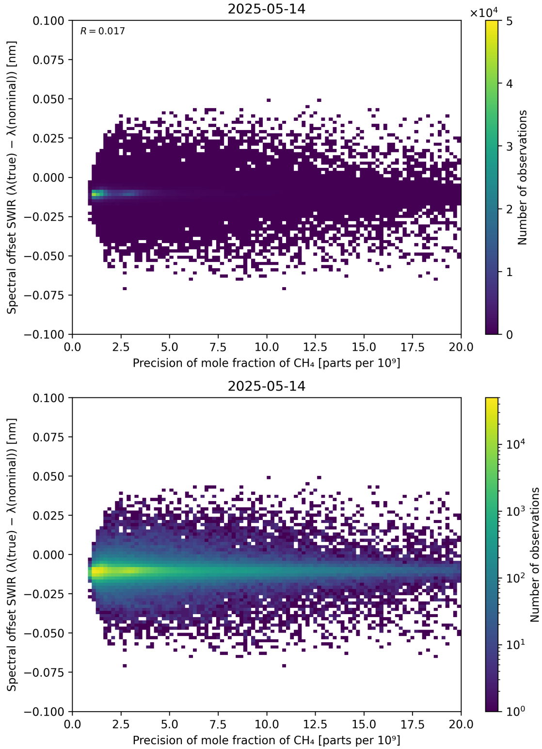
Figure 85: Scatter density plot of “Precision of mole fraction of CH 4 ” against “Spectral offset SWIR ( \lambda_{\text{true}} - \lambda_{\text{nominal}} )” for 2025-05-13 to 2025-05-15.
