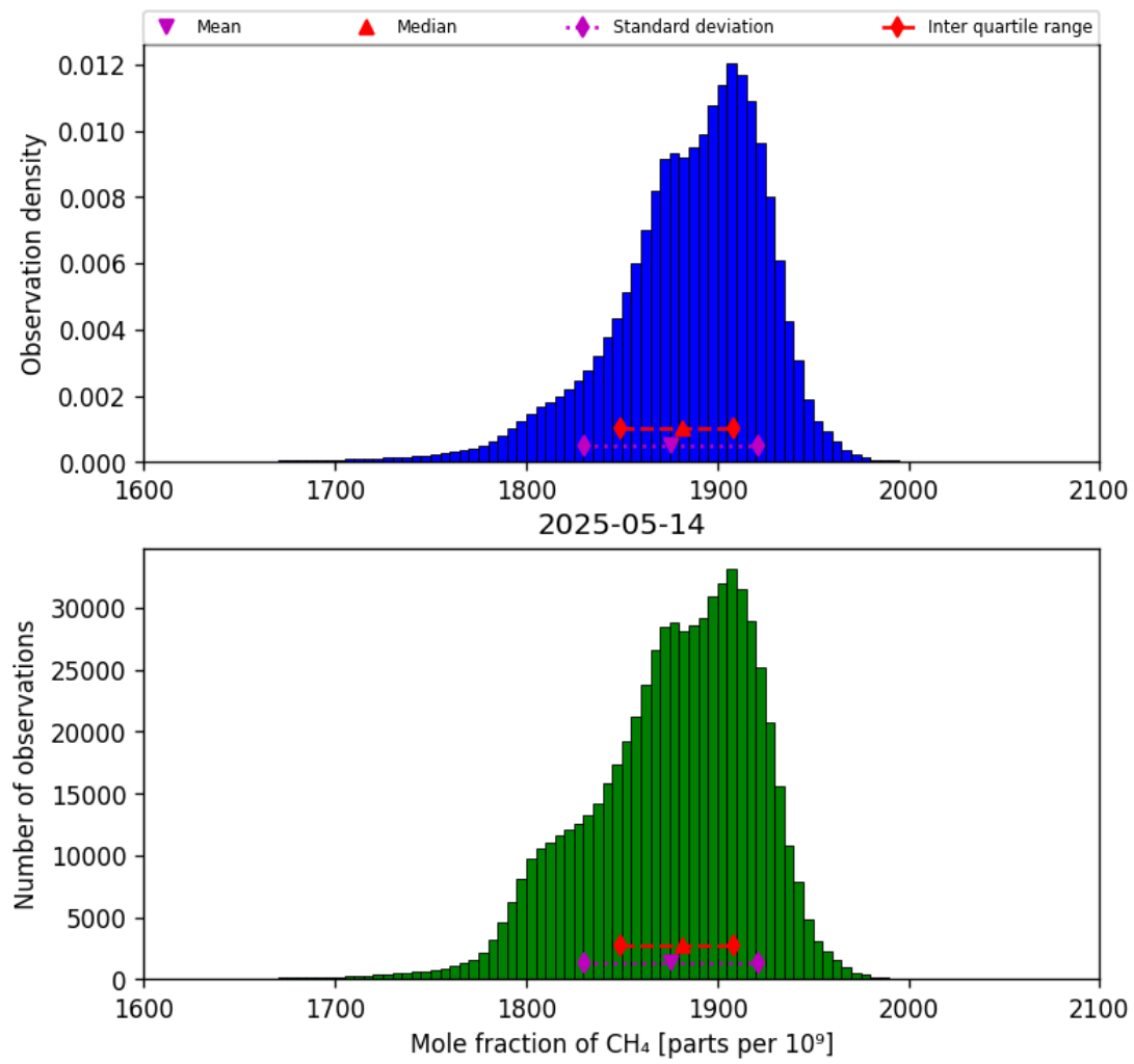
Figure 23: Histogram of “Mole fraction of CH 4 ” for 2025-05-13 to 2025-05-15
