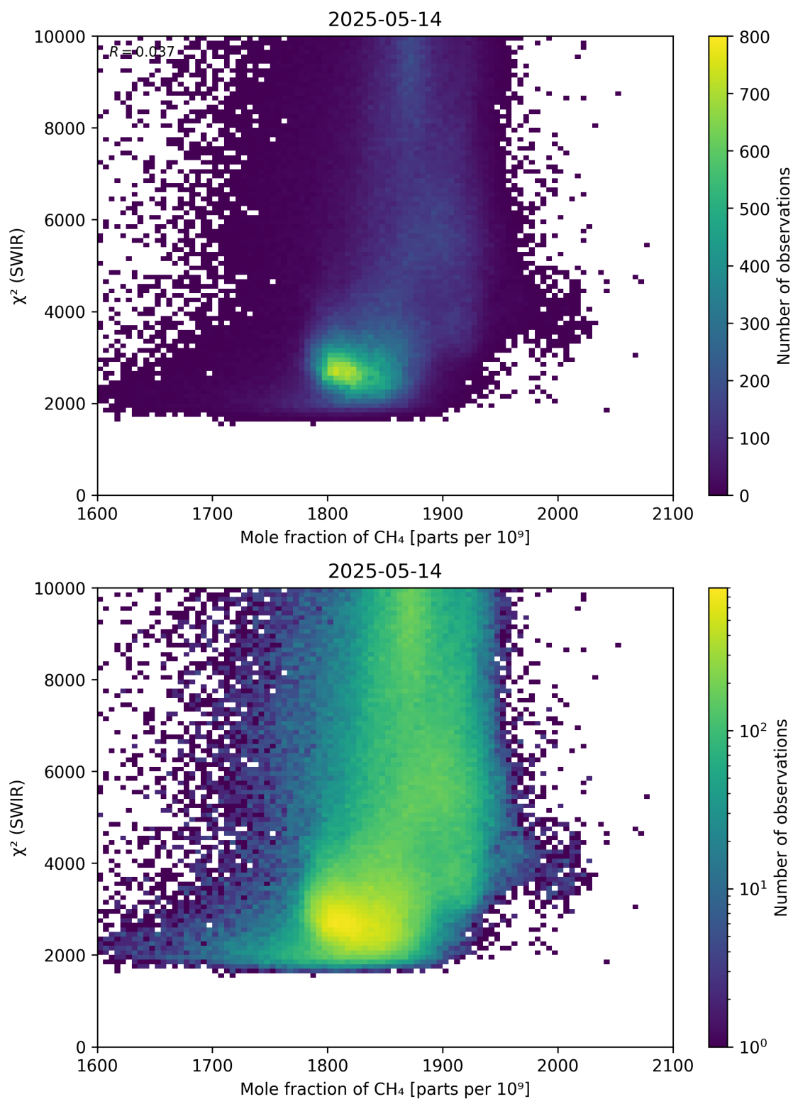
Figure 71: Scatter density plot of “Mole fraction of CH 4 ” against “ \chi^2 (SWIR)” for 2025-05-13 to 2025-05-15.
