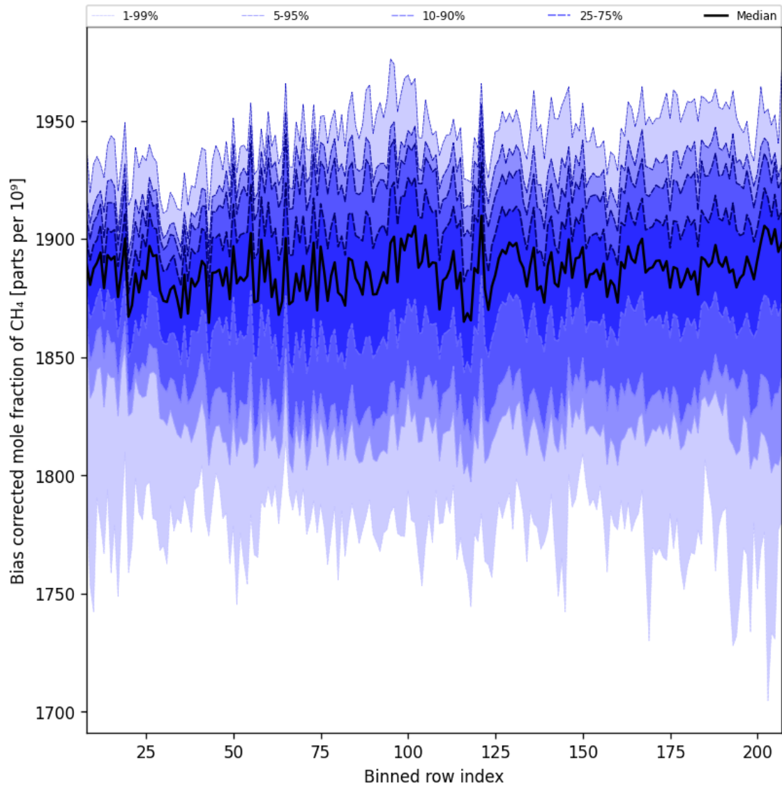
Figure 36: Along track statistics of “Bias corrected mole fraction of CH 4 ” for 2025-05-13 to 2025-05-15
