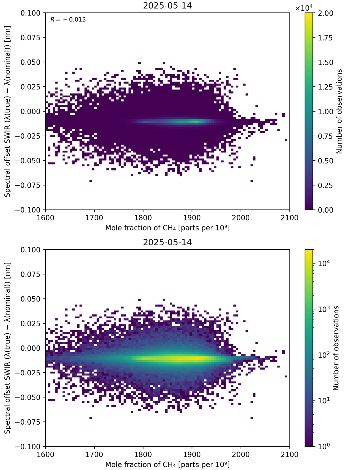
Figure 86: Scatter density plot of “Mole fraction of CH 4 ” against “Spectral offset SWIR ( \lambda_{\text{true}} - \lambda_{\text{nominal}} )” for 2025-05-13 to 2025-05-15.
