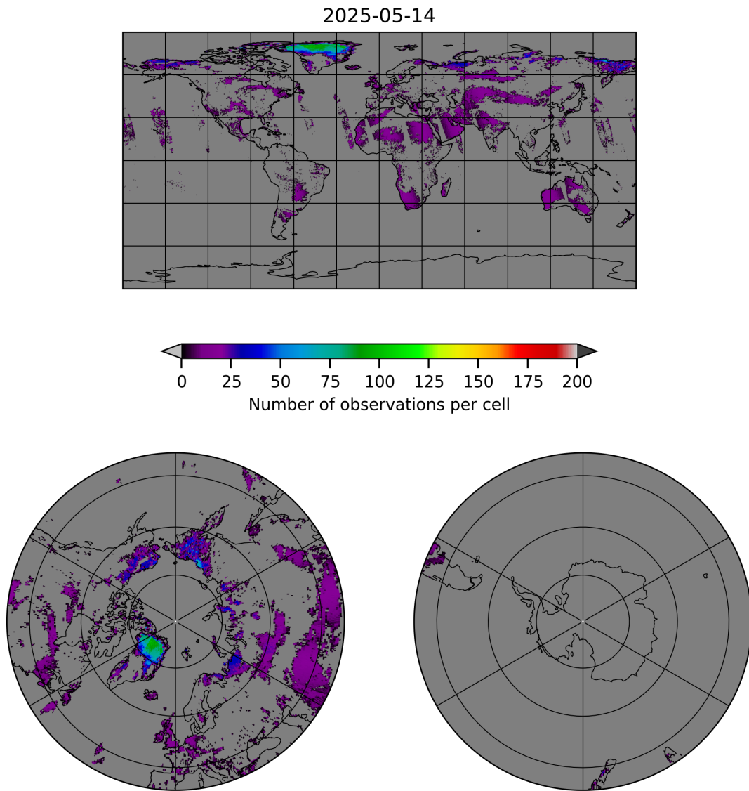
Figure 10: Map of the number of observations for 2025-05-13 to 2025-05-15
