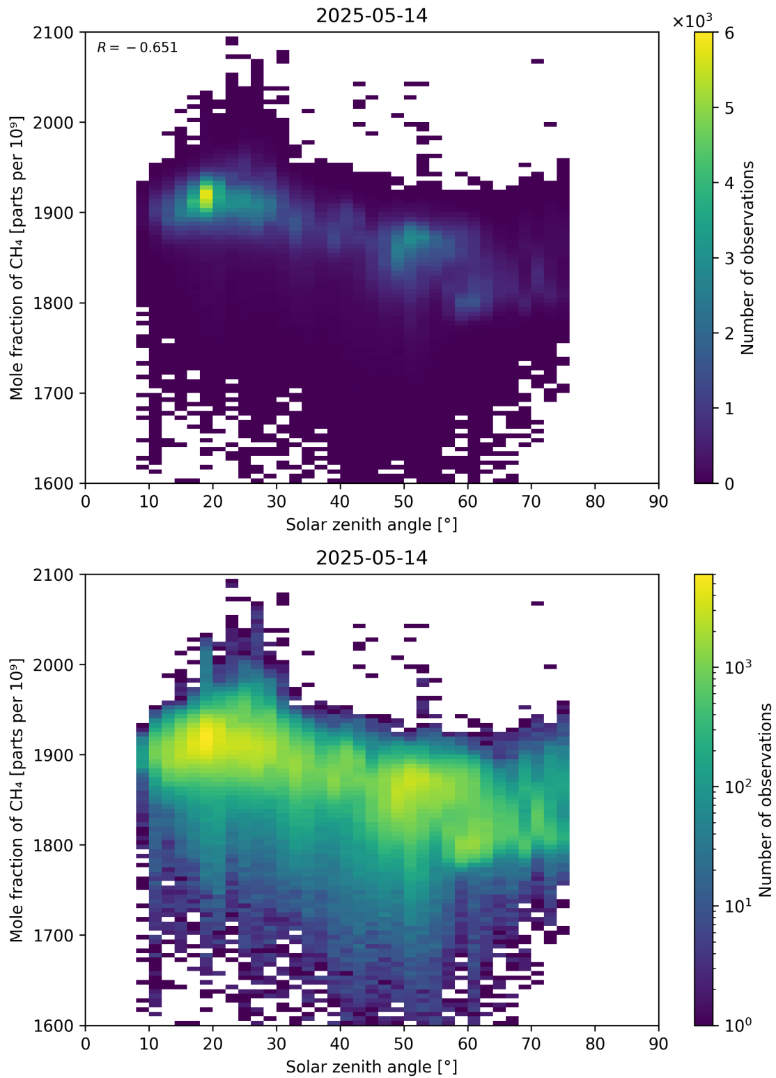
Figure 99: Scatter density plot of “Solar zenith angle” against “Mole fraction of \text{CH}_4 ” for 2025-05-13 to 2025-05-15.
