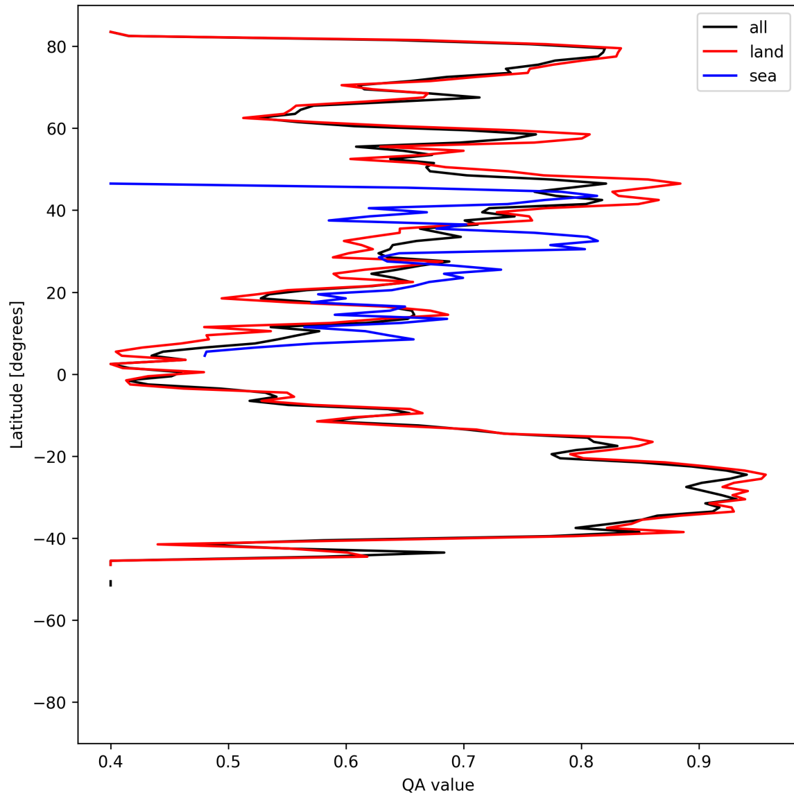
Figure 11: Zonal average of “QA value” for 2025-05-13 to 2025-05-15.
