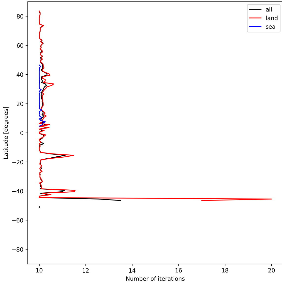
Figure 20: Zonal average of “Number of iterations” for 2025-05-13 to 2025-05-15.
