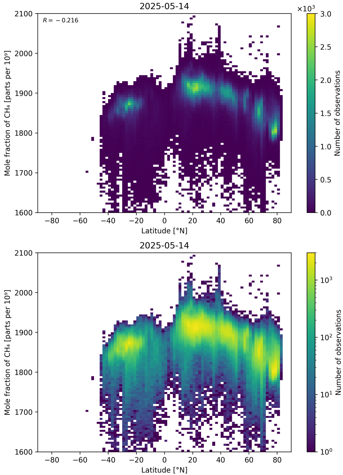
Figure 57: Scatter density plot of “Latitude” against “Mole fraction of CH 4 ” for 2025-05-13 to 2025-05-15.
