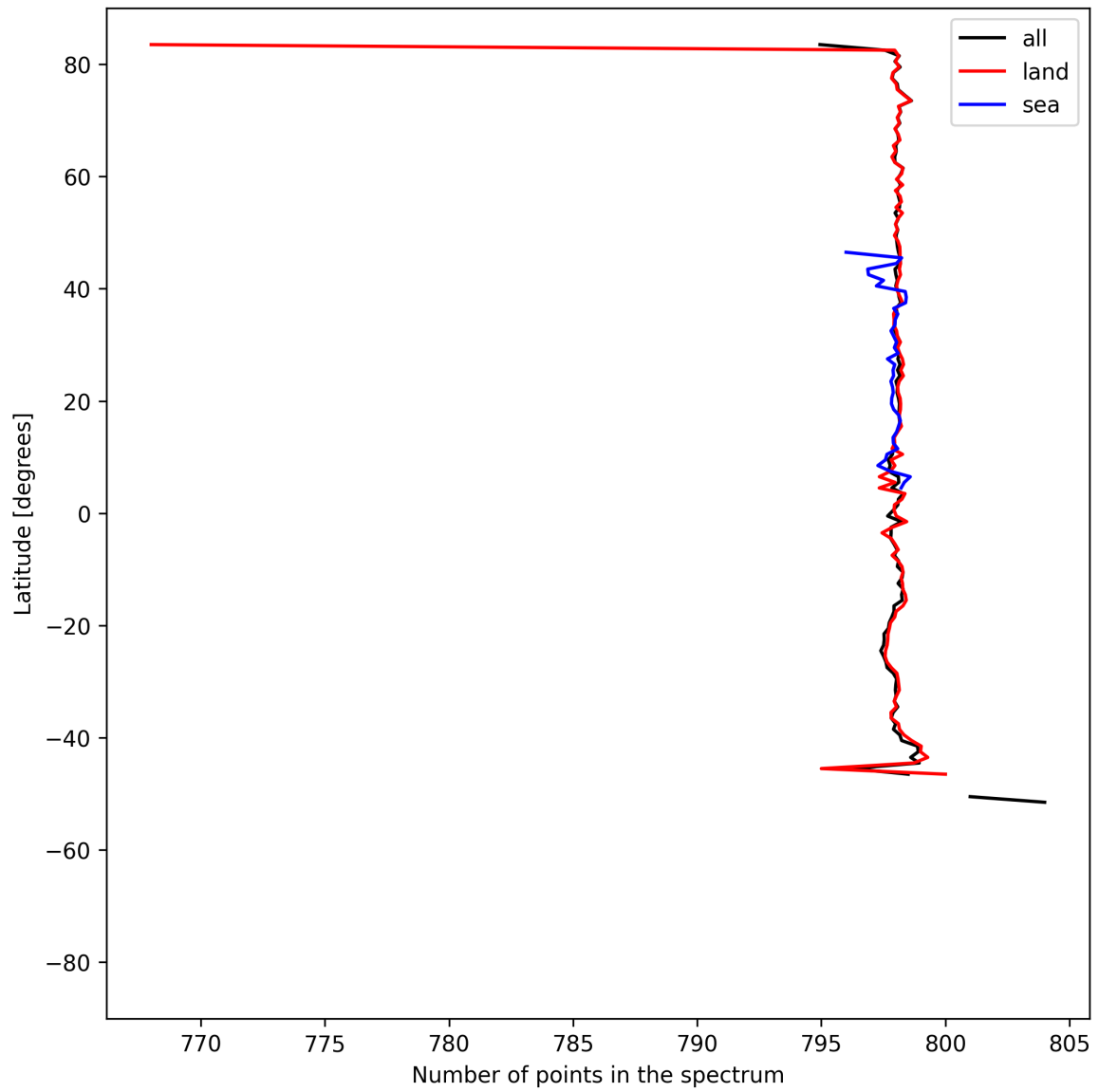
Figure 15: Zonal average of “Number of points in the spectrum” for 2025-05-13 to 2025-05-15.
