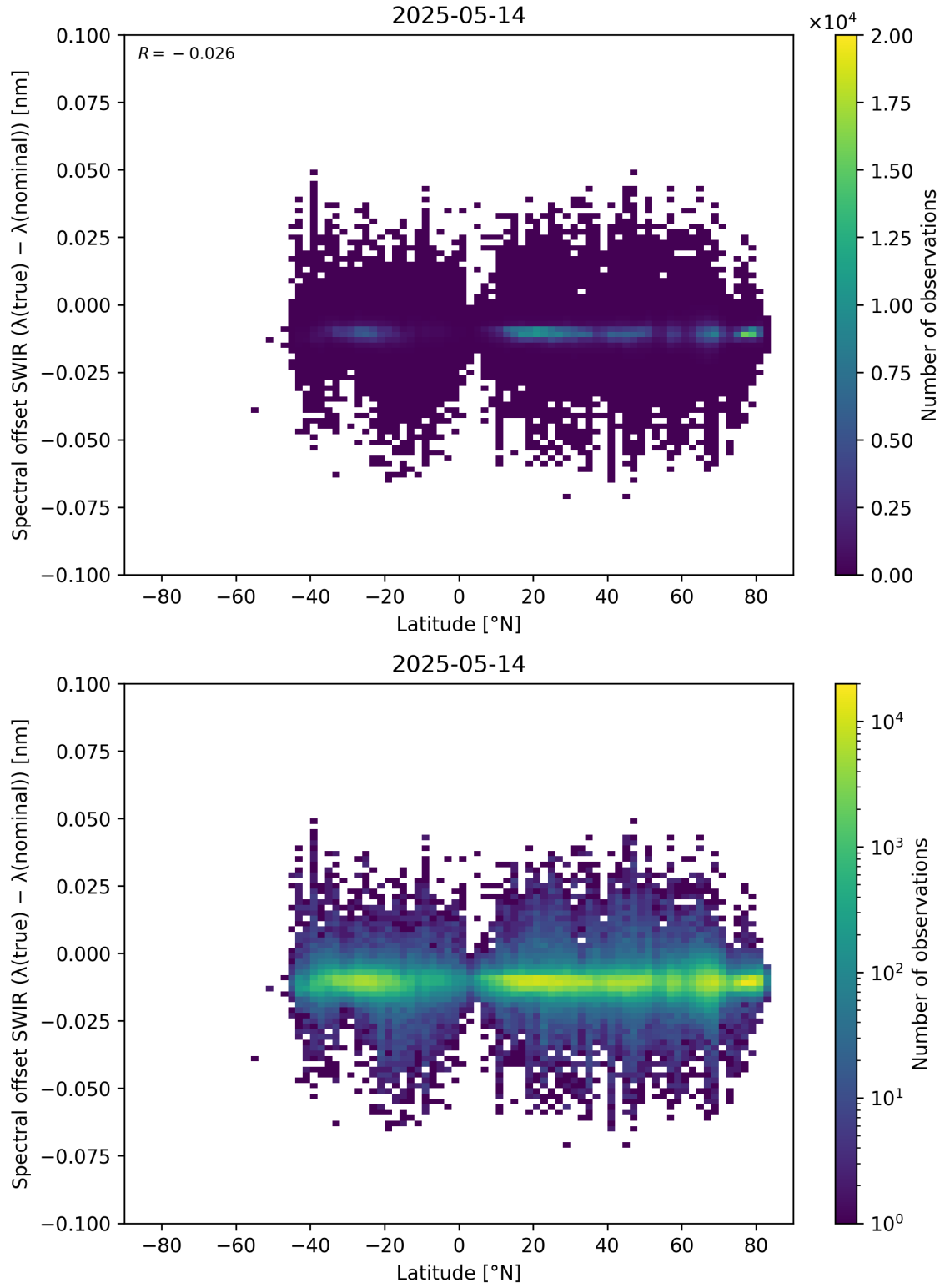
Figure 62: Scatter density plot of “Latitude” against “Spectral offset SWIR ( \lambda_{\text{true}} - \lambda_{\text{nominal}} )” for 2025-05-13 to 2025-05-15.
