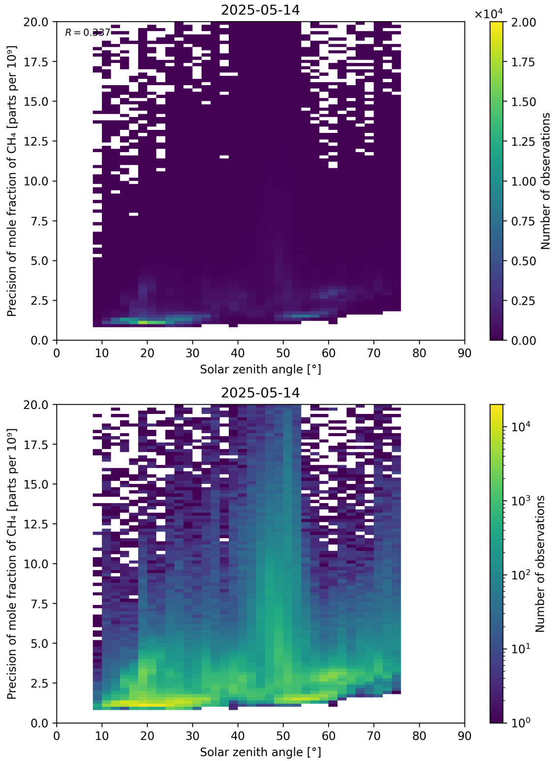
Figure 101: Scatter density plot of “Solar zenith angle” against “Precision of mole fraction of CH 4 ” for 2025-05-13 to 2025-05-15.
