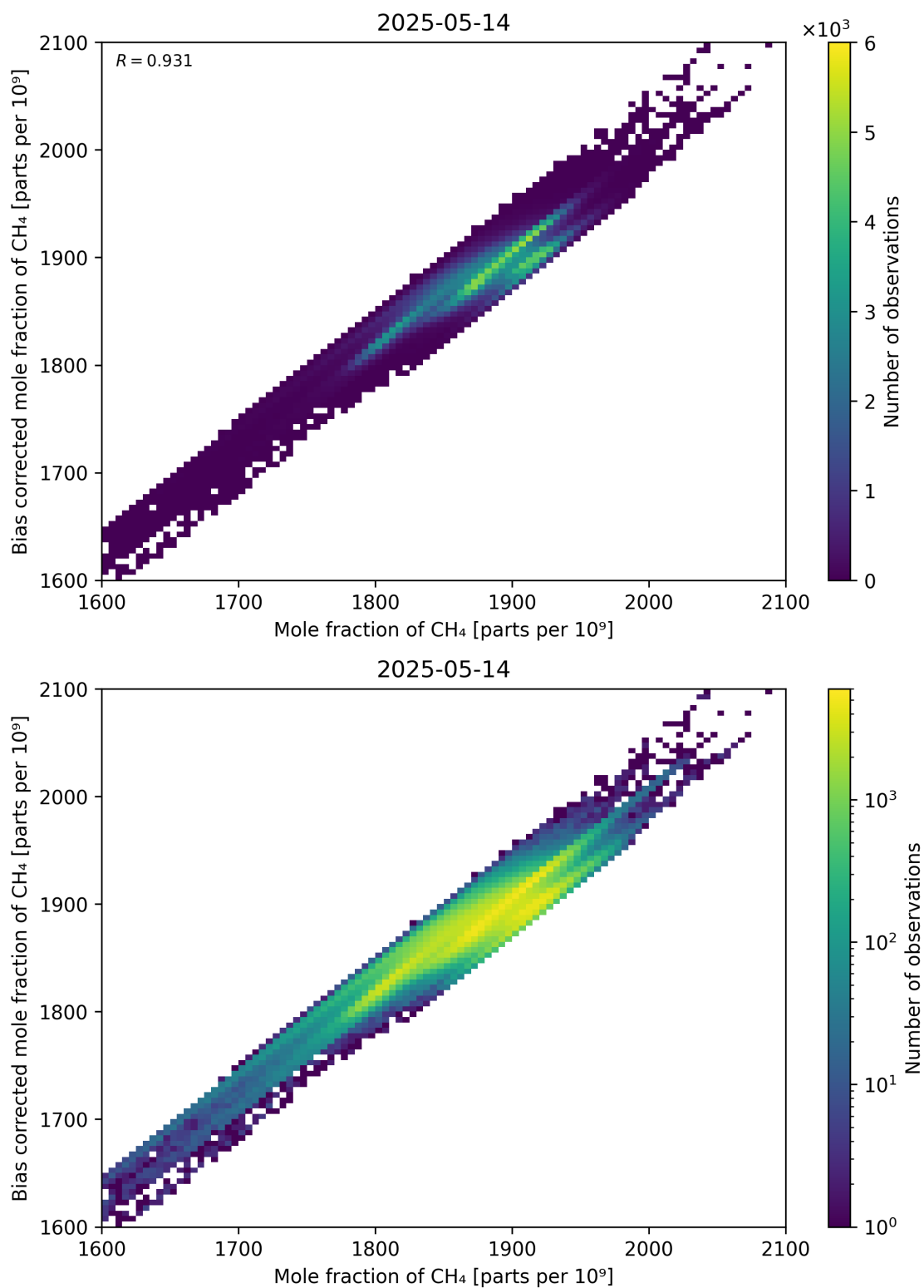
Figure 74: Scatter density plot of “Mole fraction of CH 4 ” against “Bias corrected mole fraction of CH 4 ” for 2025-05-13 to 2025-05-15.
