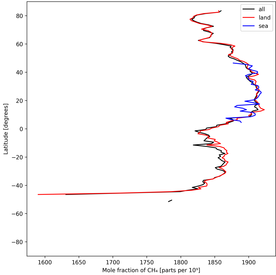
Figure 12: Zonal average of “Mole fraction of CH 4 ” for 2025-05-13 to 2025-05-15.
