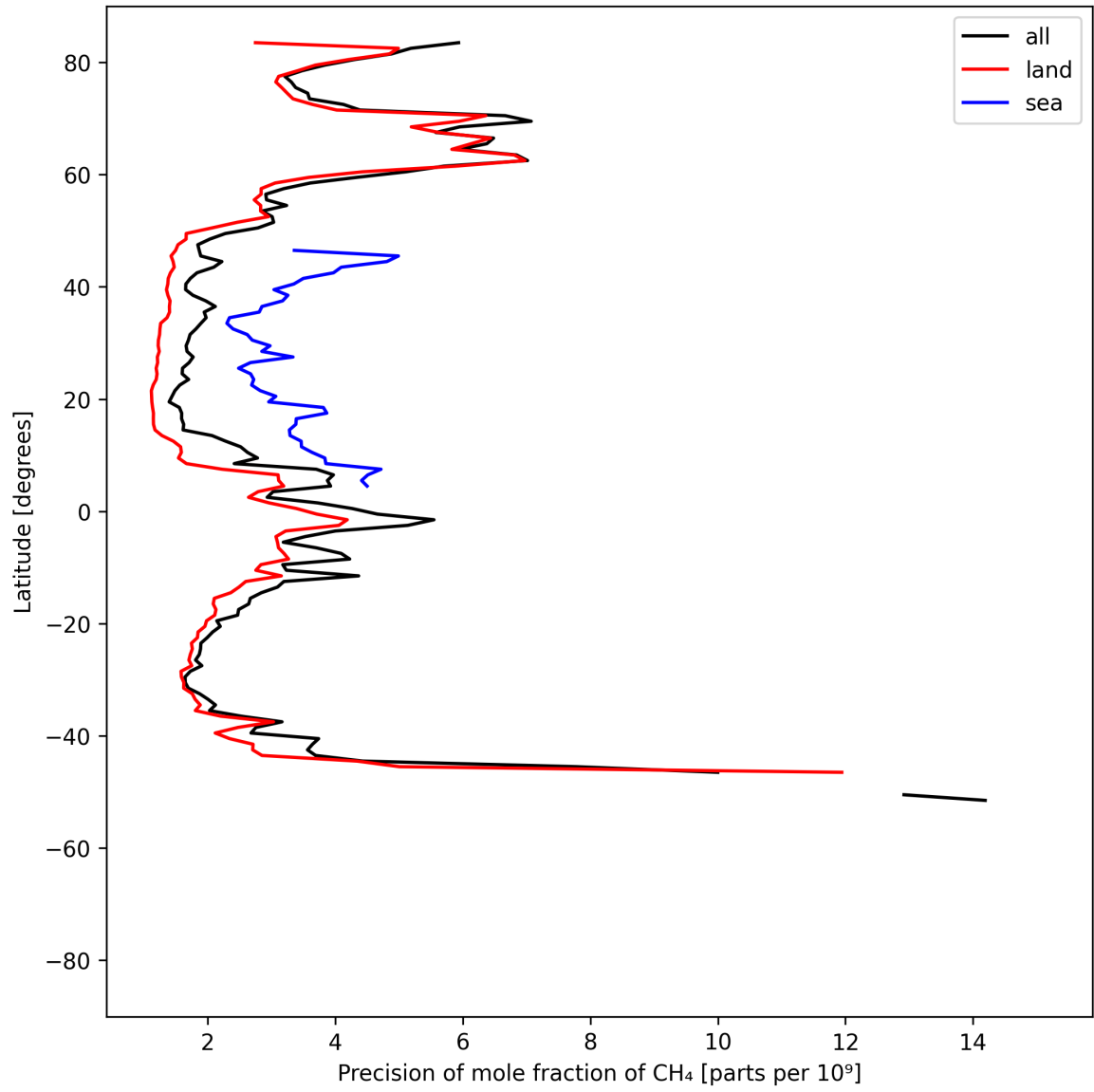
Figure 13: Zonal average of “Precision of mole fraction of CH 4 ” for 2025-05-13 to 2025-05-15.
