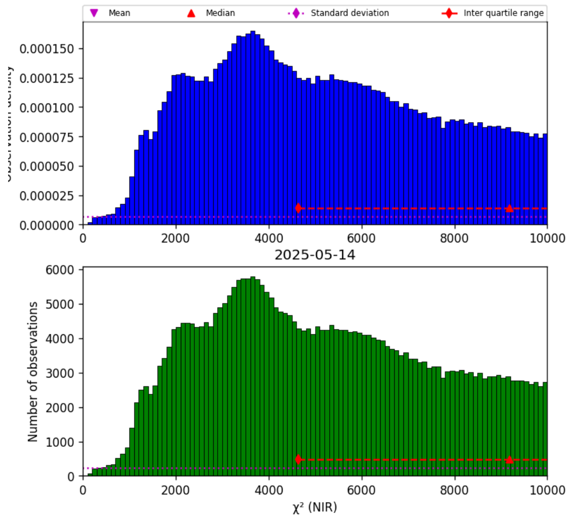
Figure 29: Histogram of “ \chi^2 (NIR)” for 2025-05-13 to 2025-05-15
