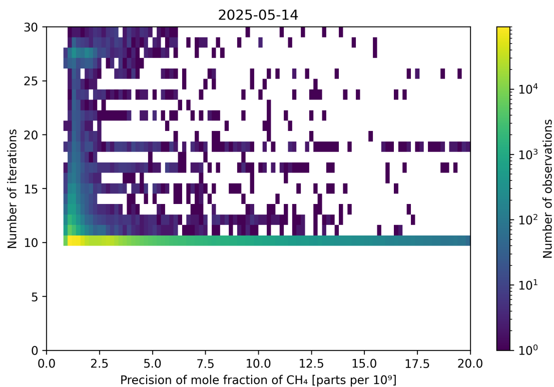
Figure 83: Scatter density plot of “Precision of mole fraction of CH 4 ” against “Number of iterations” for 2025-05-13 to 2025-05-15.
