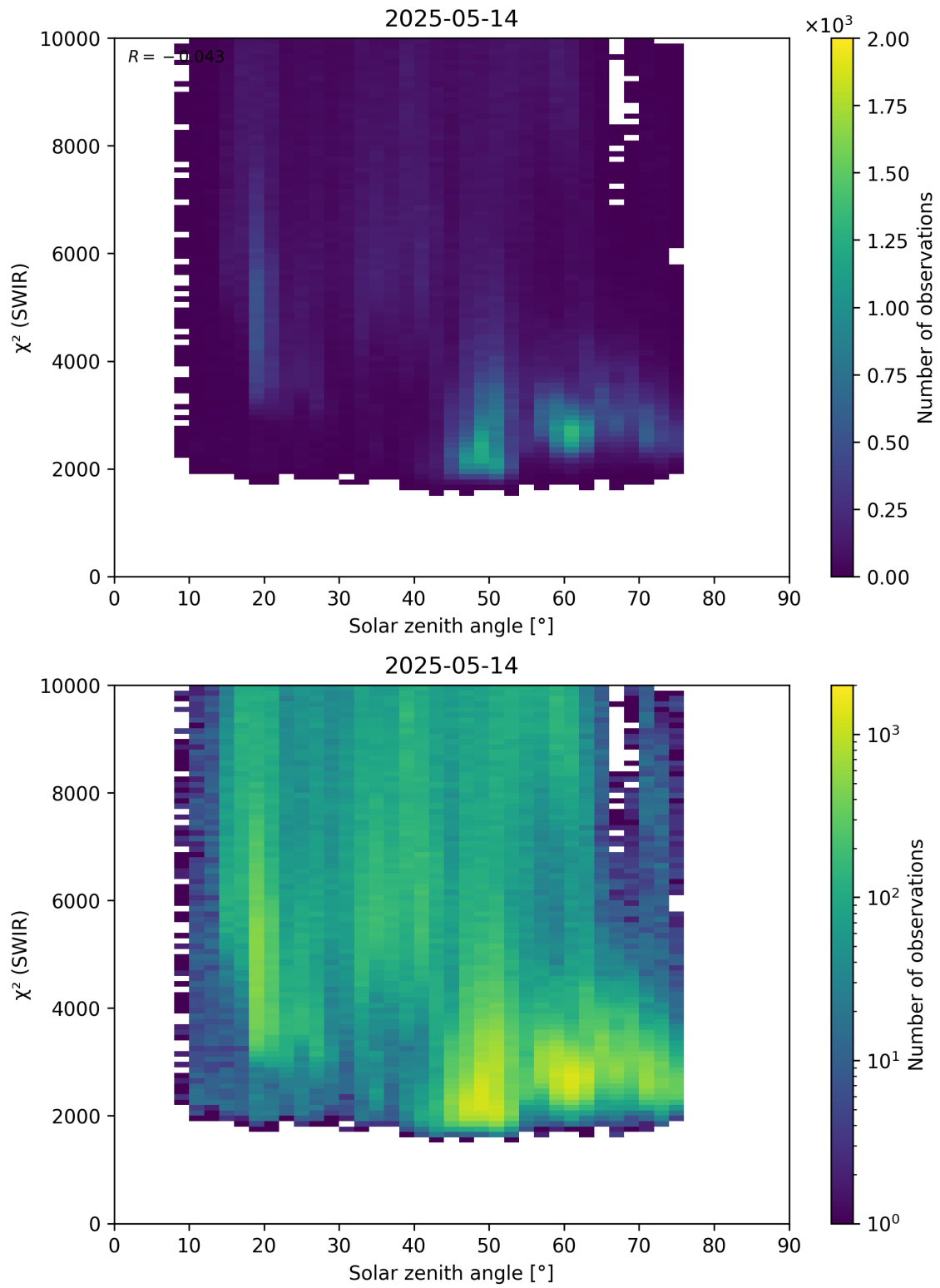
Figure 95: Scatter density plot of “Solar zenith angle” against “ \chi^2 (SWIR)” for 2025-05-13 to 2025-05-15.
