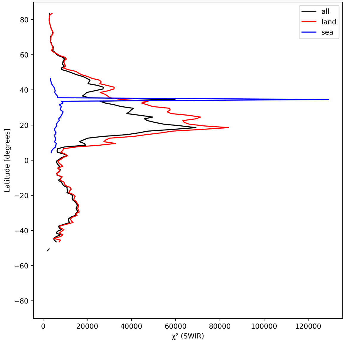
Figure 17: Zonal average of “ \chi^2 (SWIR)” for 2025-05-13 to 2025-05-15.
