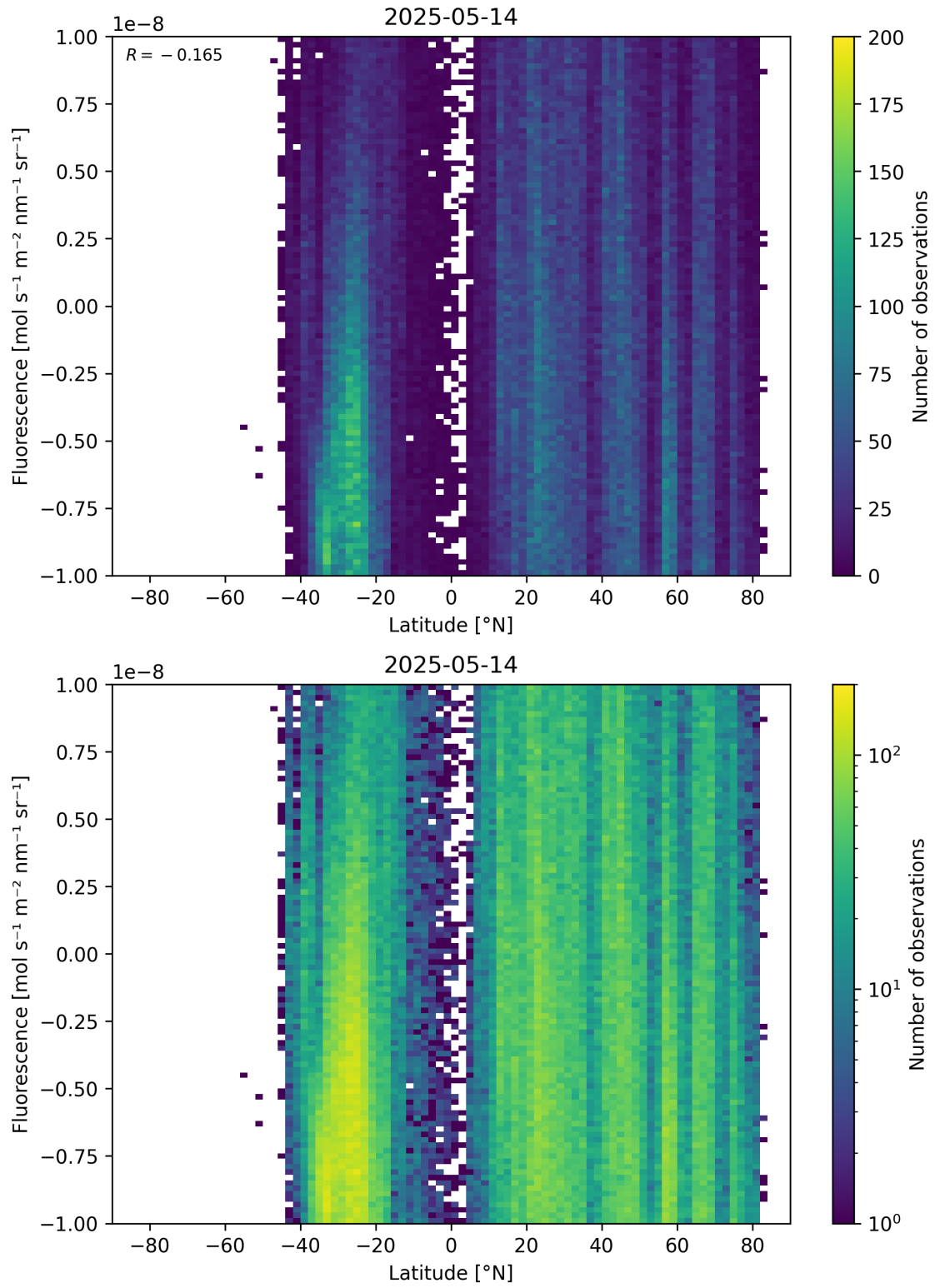
Figure 56: Scatter density plot of “Latitude” against “Fluorescence” for 2025-05-13 to 2025-05-15.
