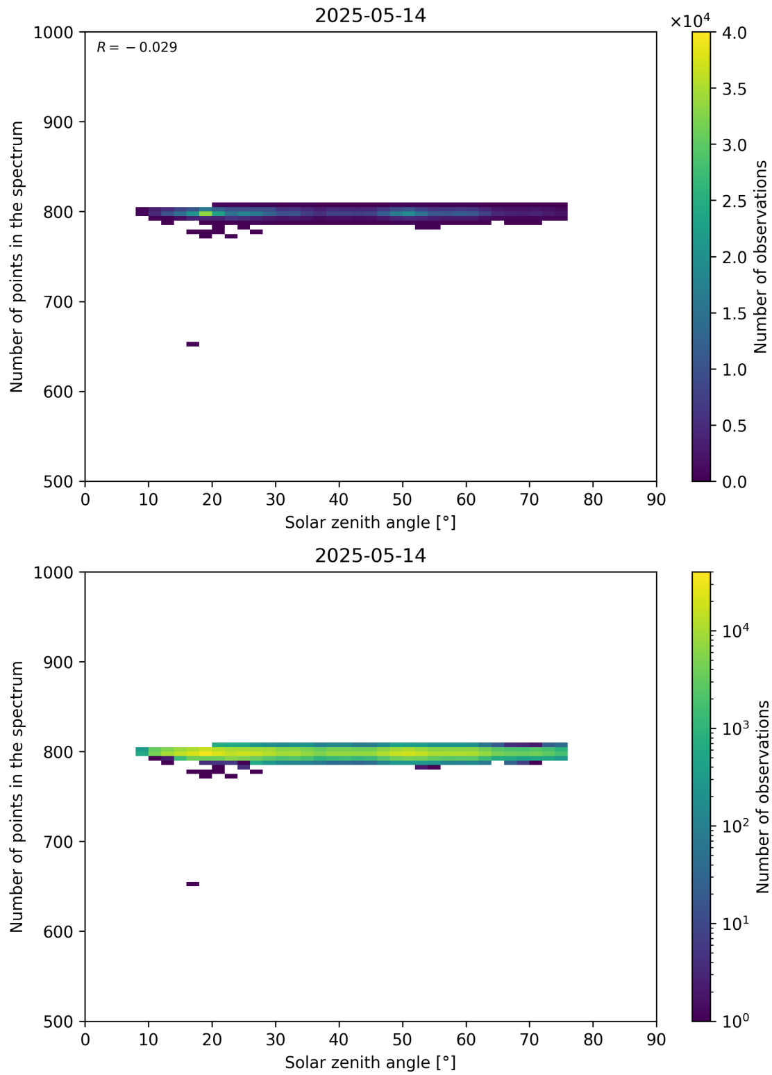
Figure 103: Scatter density plot of “Solar zenith angle” against “Number of points in the spectrum” for 2025-05-13 to 2025-05-15.
