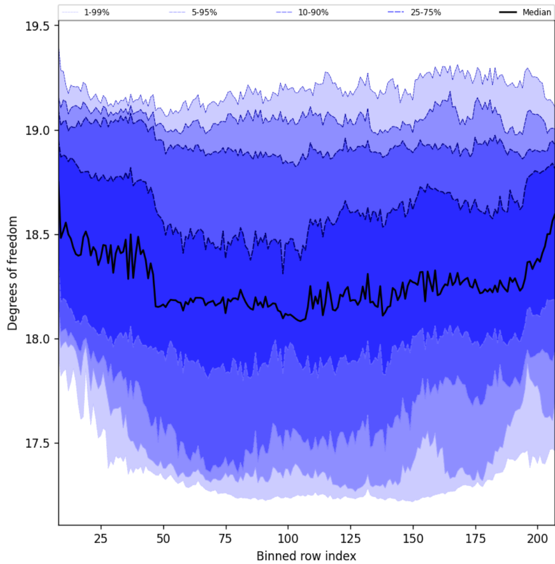
Figure 41: Along track statistics of “Degrees of freedom” for 2025-05-13 to 2025-05-15
