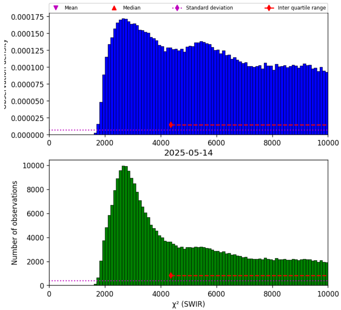
Figure 28: Histogram of “ \chi^2 (SWIR)” for 2025-05-13 to 2025-05-15
