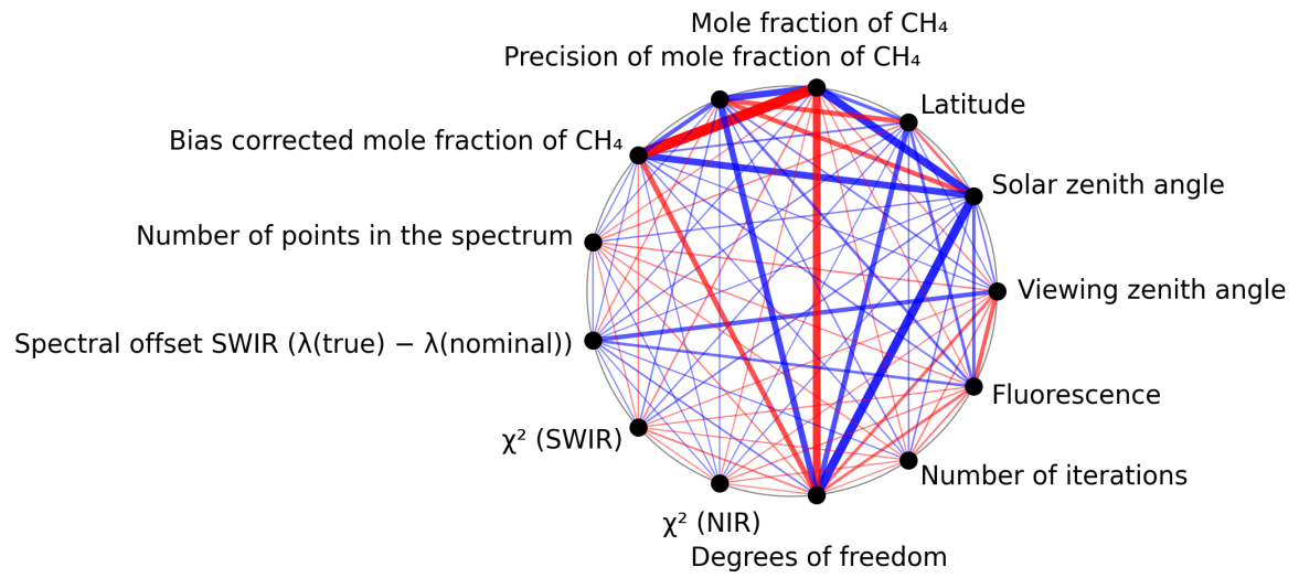
Figure 1: Map of correlation graph for 2025-05-13 to 2025-05-15.
