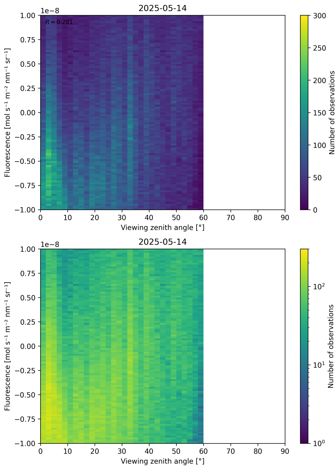
Figure 108: Scatter density plot of “Viewing zenith angle” against “Fluorescence” for 2025-05-13 to 2025-05-15.
