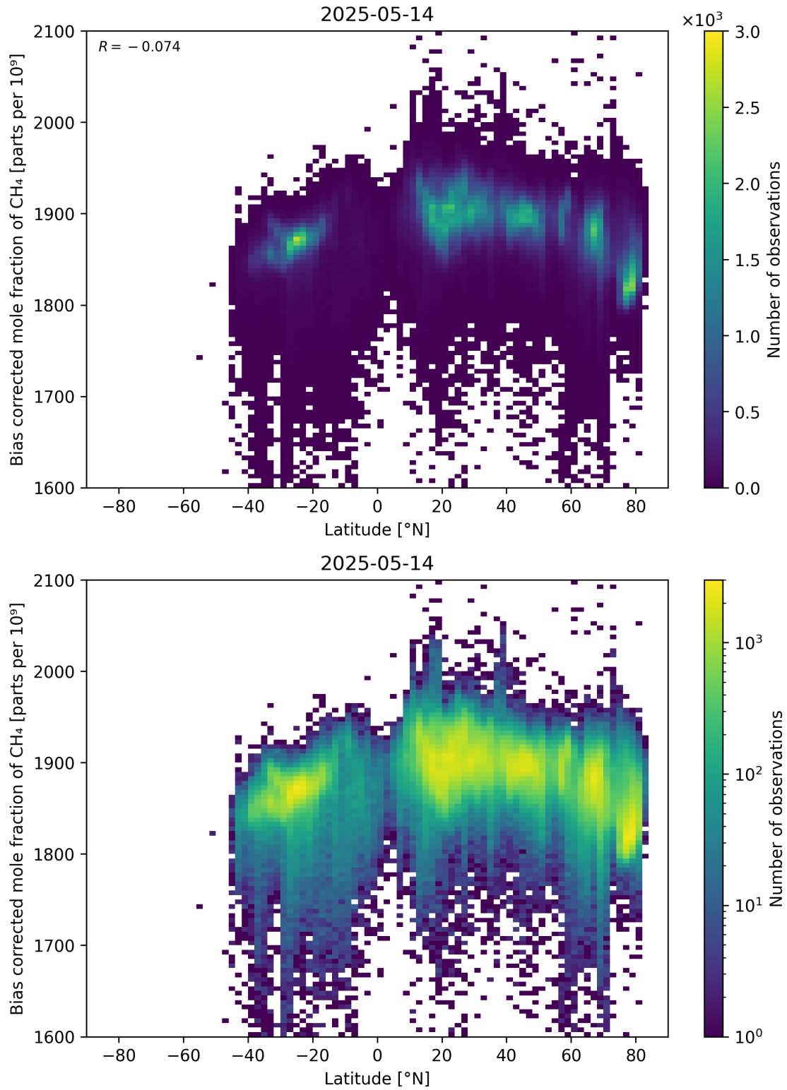
Figure 58: Scatter density plot of “Latitude” against “Bias corrected mole fraction of \text{CH}_4 ” for 2025-05-13 to 2025-05-15.
