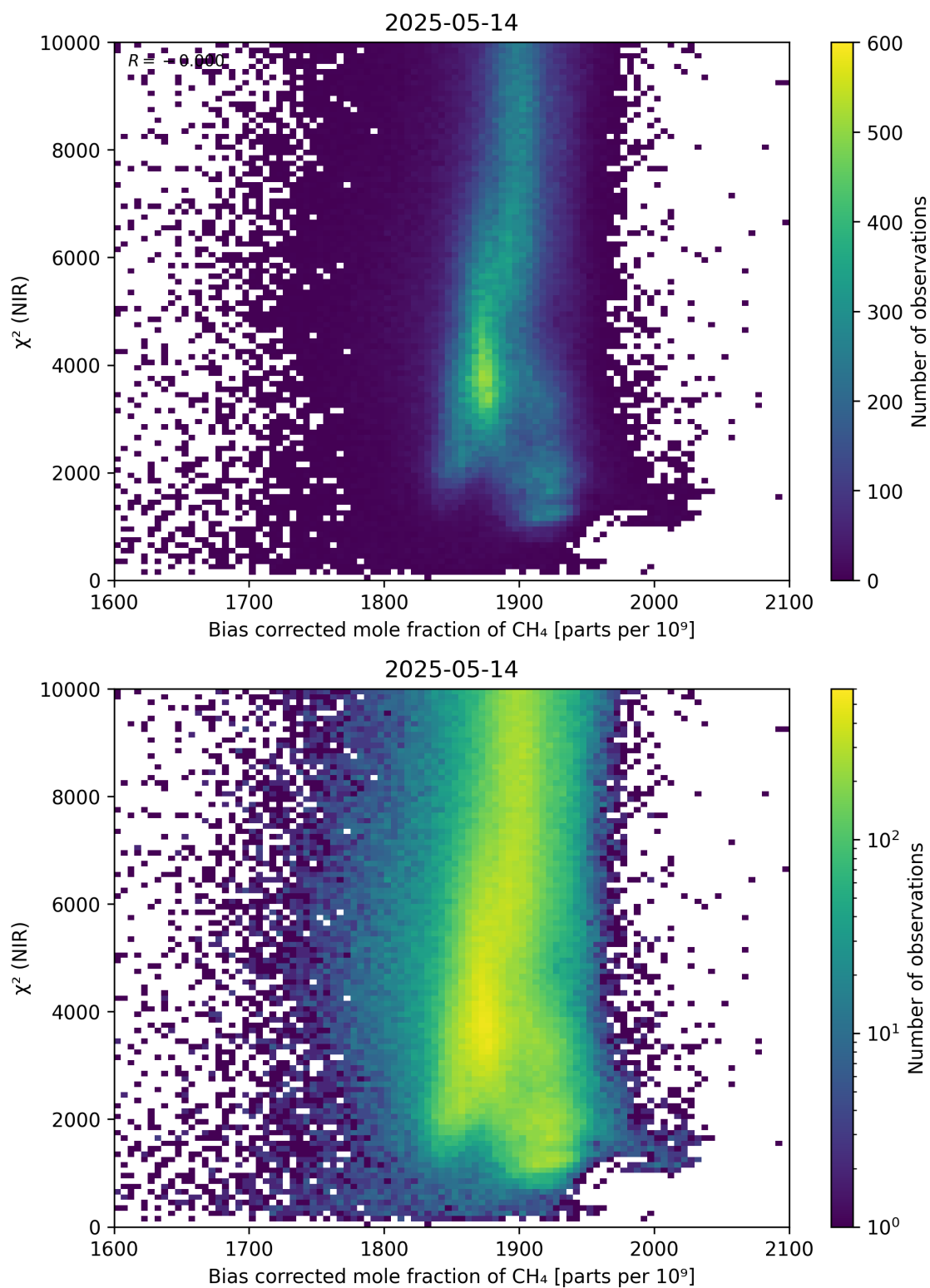
Figure 63: Scatter density plot of “Bias corrected mole fraction of CH 4 ” against “ \chi^2 (NIR)” for 2025-05-13 to 2025-05-15.
