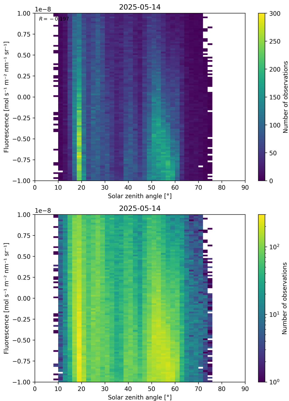
Figure 97: Scatter density plot of “Solar zenith angle” against “Fluorescence” for 2025-05-13 to 2025-05-15.
