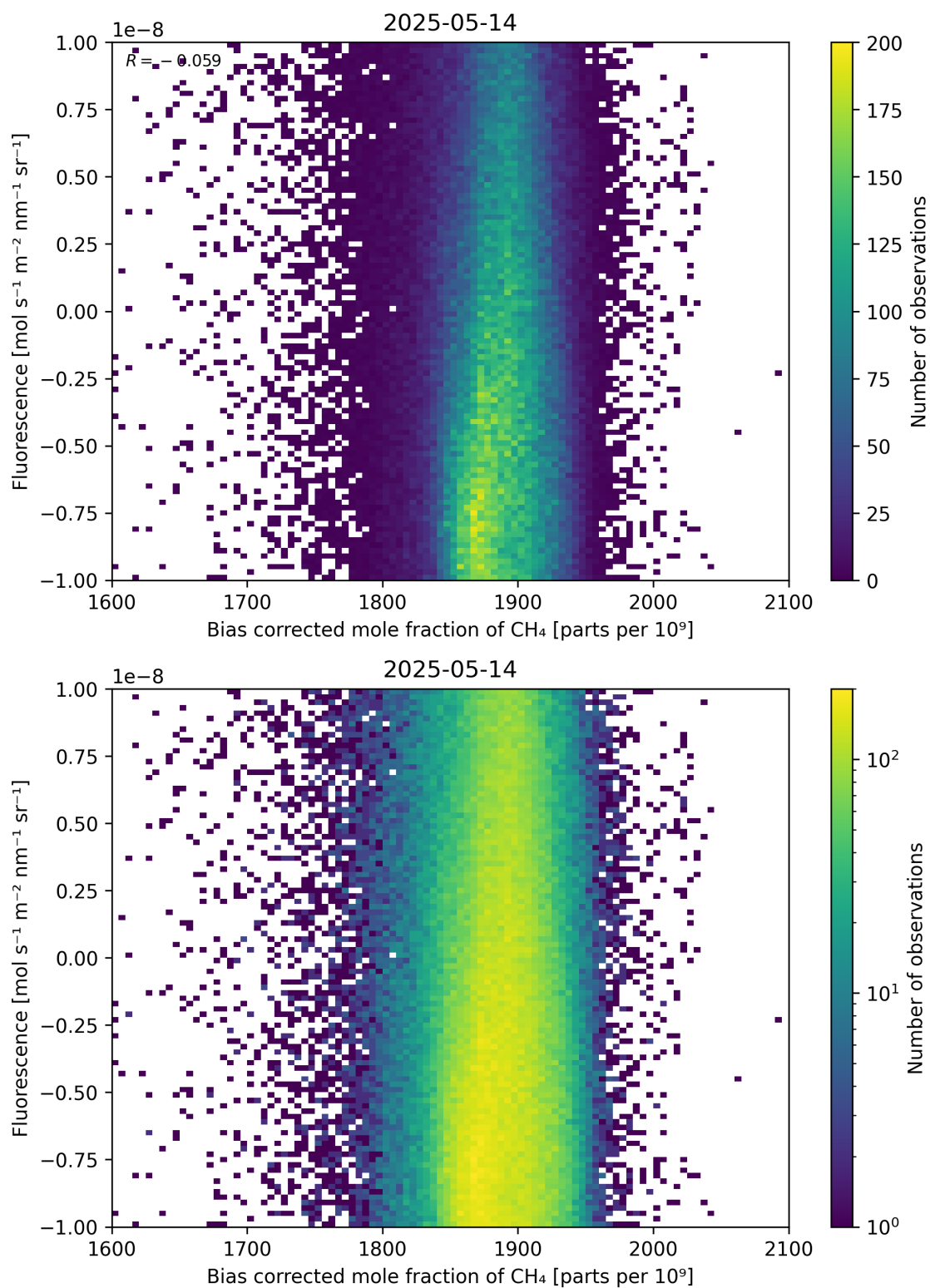
Figure 66: Scatter density plot of “Bias corrected mole fraction of \text{CH}_4 ” against “Fluorescence” for 2025-05-13 to 2025-05-15.
