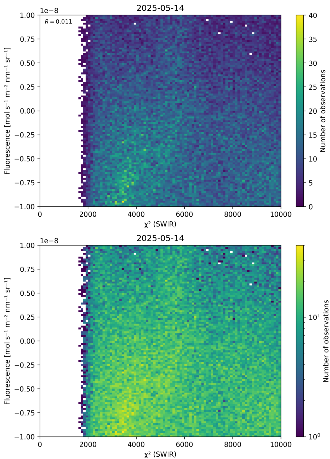
Figure 49: Scatter density plot of “ \chi^2 (SWIR)” against “Fluorescence” for 2025-05-13 to 2025-05-15.
