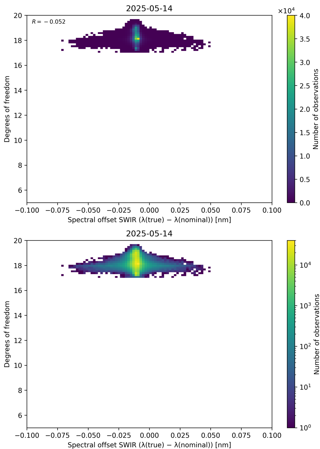
Figure 119: Scatter density plot of “Spectral offset SWIR ( \lambda_{\text{true}} - \lambda_{\text{nominal}} )” against “Degrees of freedom” for 2025-05-13 to 2025-05-15.
