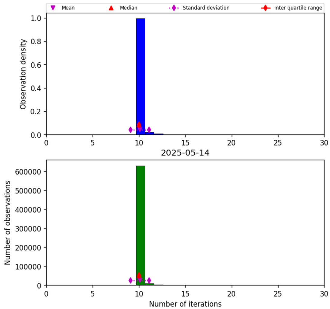
Figure 31: Histogram of “Number of iterations” for 2025-05-13 to 2025-05-15
