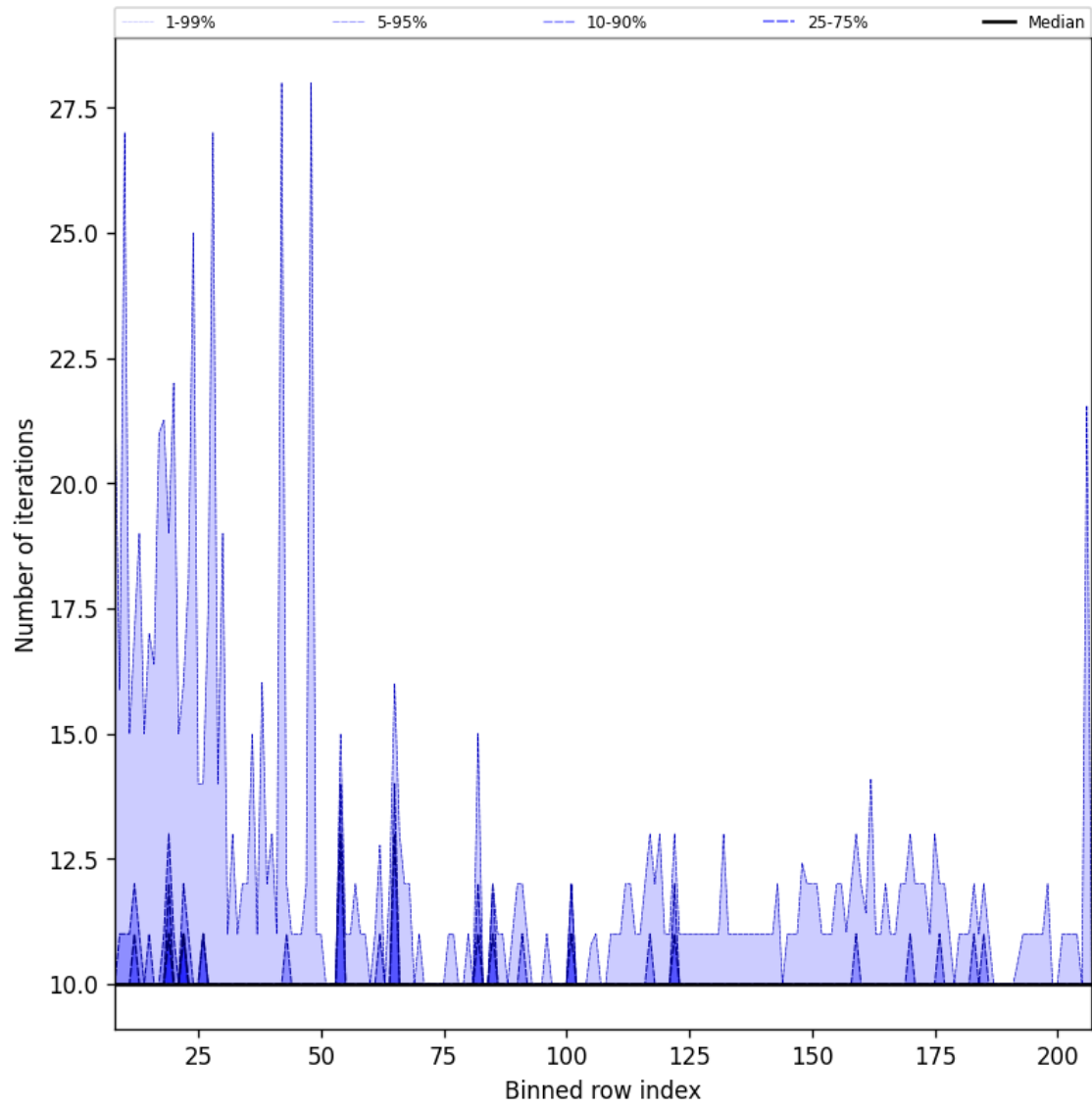
Figure 42: Along track statistics of “Number of iterations” for 2025-05-13 to 2025-05-15
