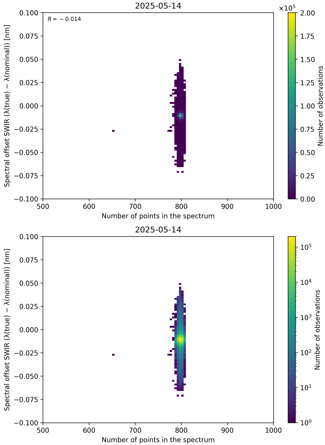
Figure 93: Scatter density plot of “Number of points in the spectrum” against “Spectral offset SWIR ( \lambda_{\text{true}} - \lambda_{\text{nominal}} )” for 2025-05-13 to 2025-05-15.
