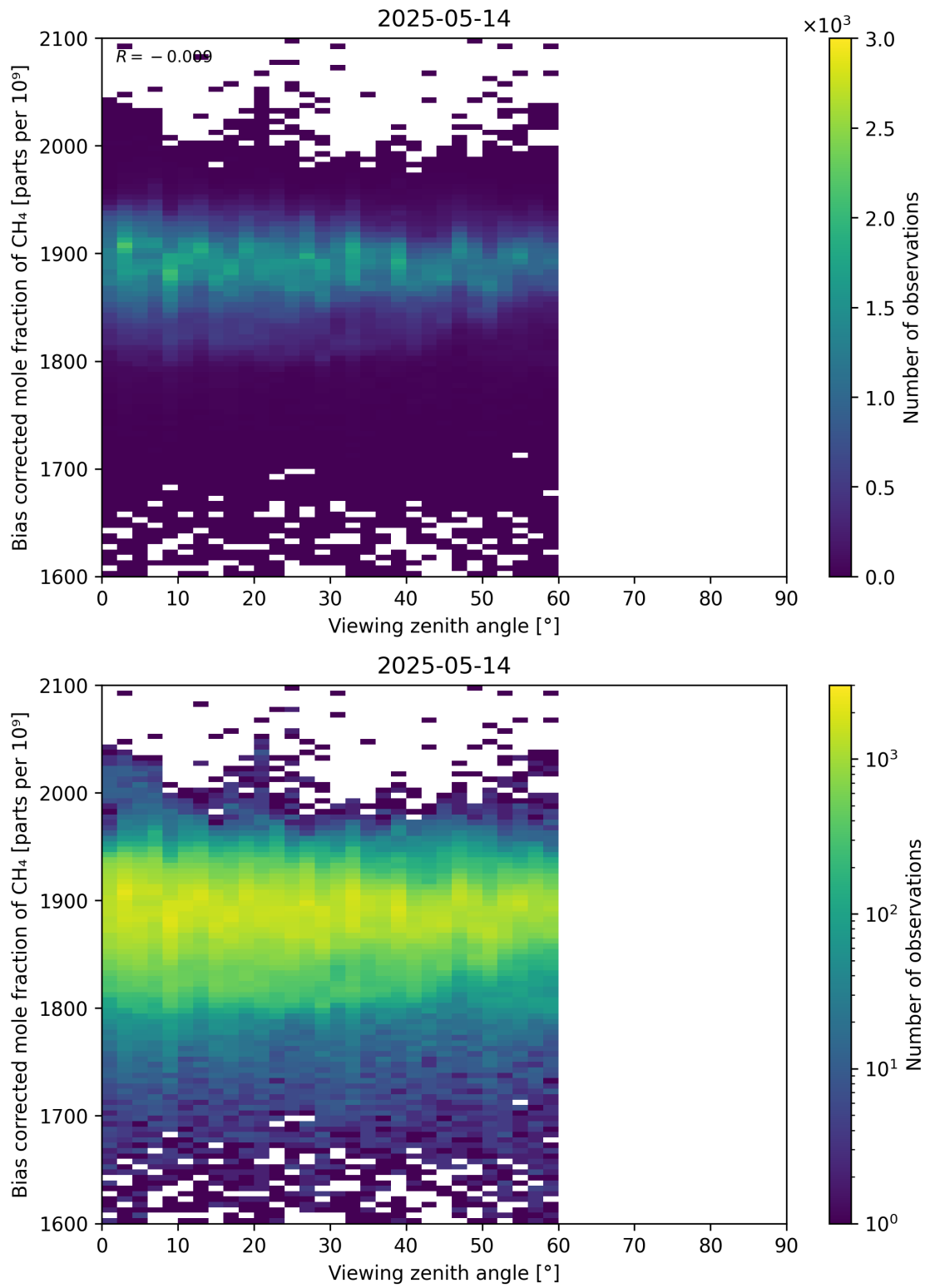
Figure 111: Scatter density plot of “Viewing zenith angle” against “Bias corrected mole fraction of CH 4 ” for 2025-05-13 to 2025-05-15.
