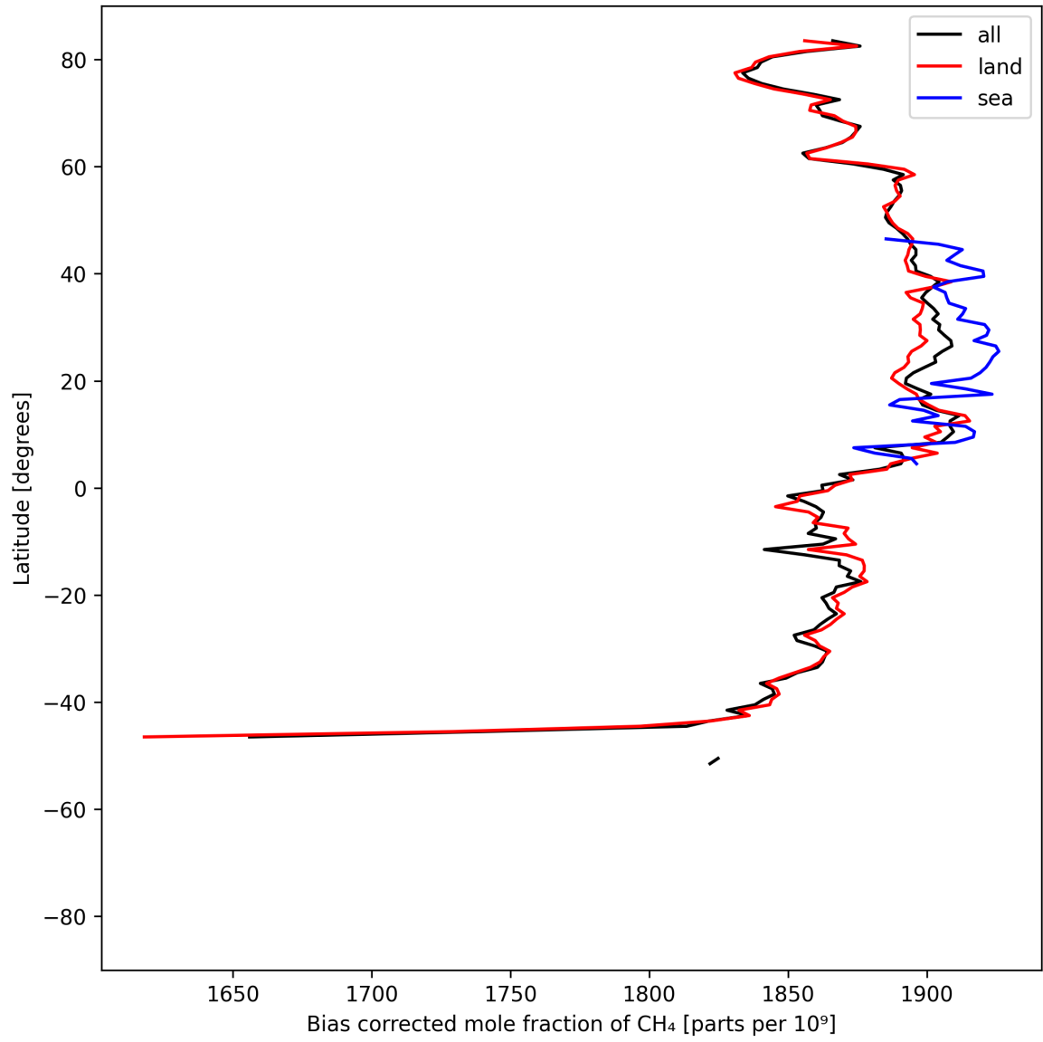
Figure 14: Zonal average of “Bias corrected mole fraction of \text{CH}_4 ” for 2025-05-13 to 2025-05-15.
