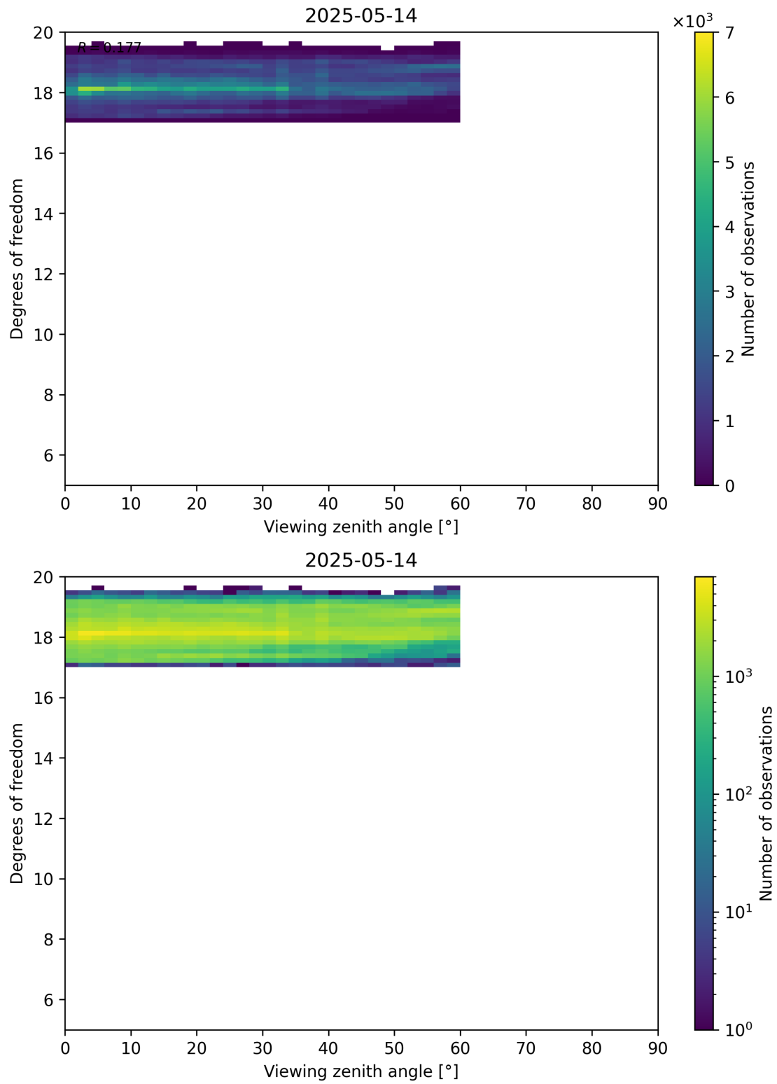
Figure 107: Scatter density plot of “Viewing zenith angle” against “Degrees of freedom” for 2025-05-13 to 2025-05-15.
