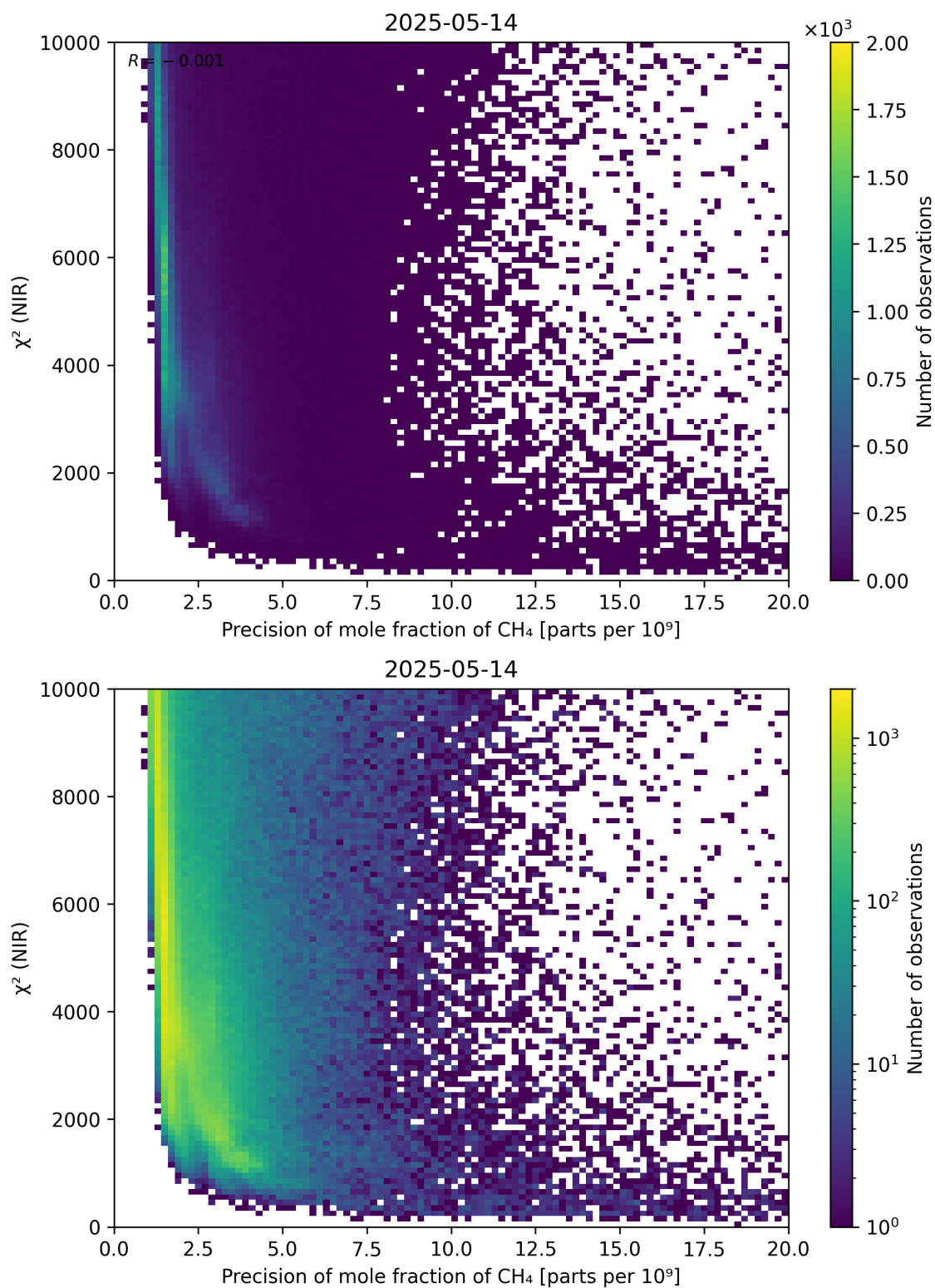
Figure 78: Scatter density plot of “Precision of mole fraction of \text{CH}_4 ” against “ \chi^2 (NIR)” for 2025-05-13 to 2025-05-15.
