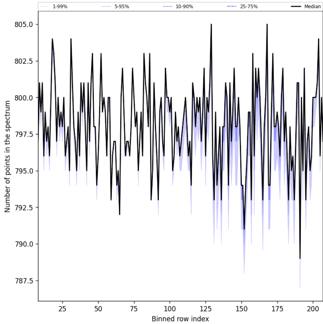
Figure 37: Along track statistics of “Number of points in the spectrum” for 2025-05-13 to 2025-05-15
