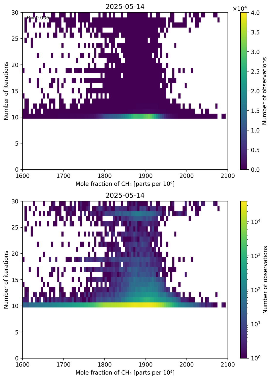
Figure 76: Scatter density plot of “Mole fraction of CH 4 ” against “Number of iterations” for 2025-05-13 to 2025-05-15.
