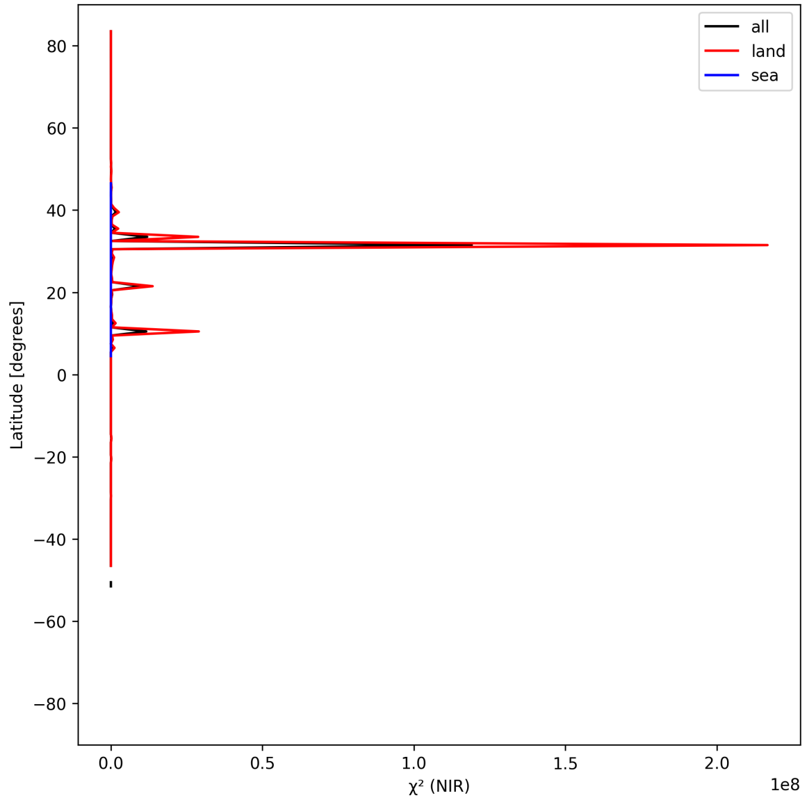
Figure 18: Zonal average of “ \chi^2 (NIR)” for 2025-05-13 to 2025-05-15.
