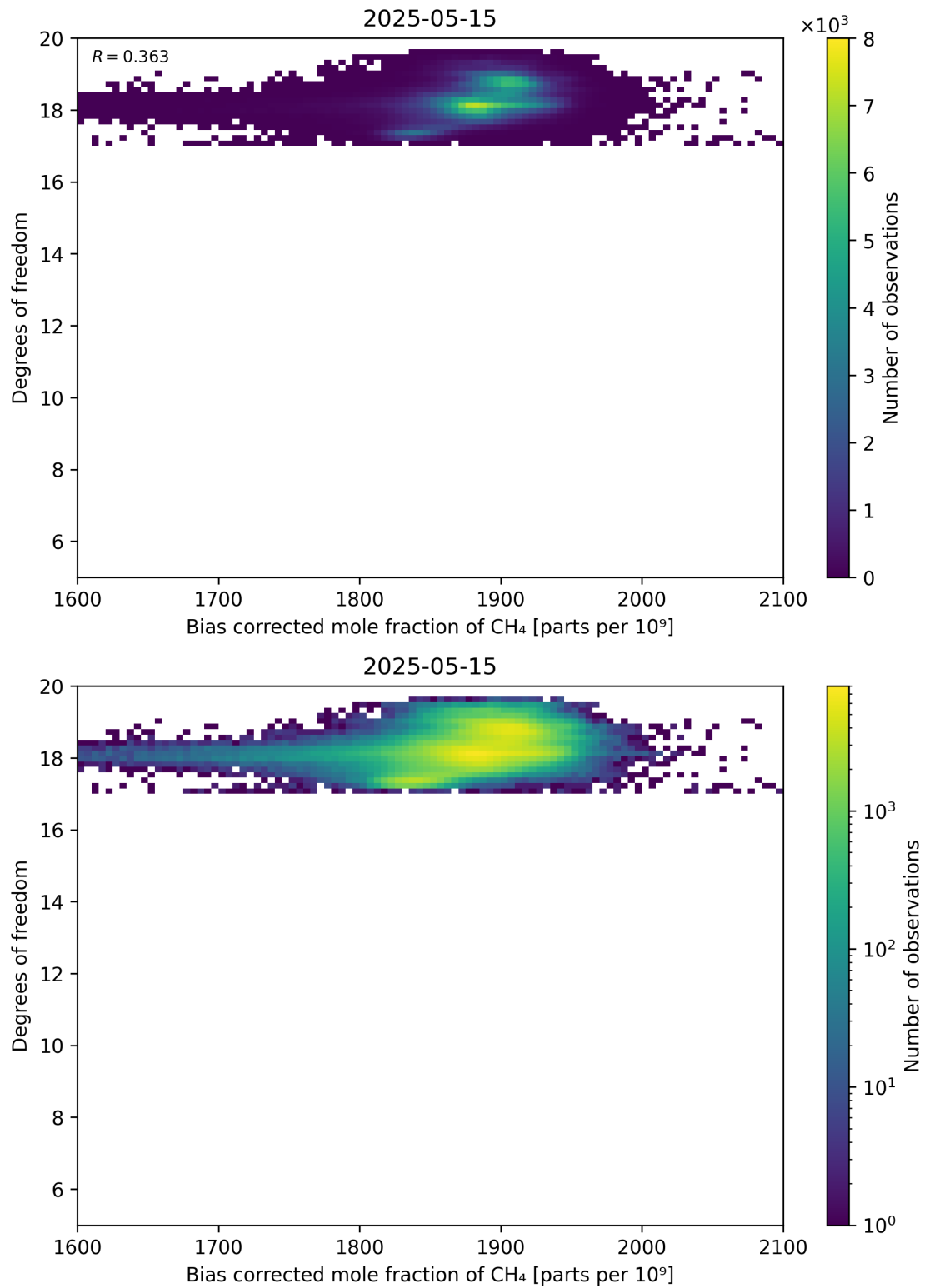
Figure 65: Scatter density plot of “Bias corrected mole fraction of CH 4 ” against “Degrees of freedom” for 2025-05-15 to 2025-05-16.
