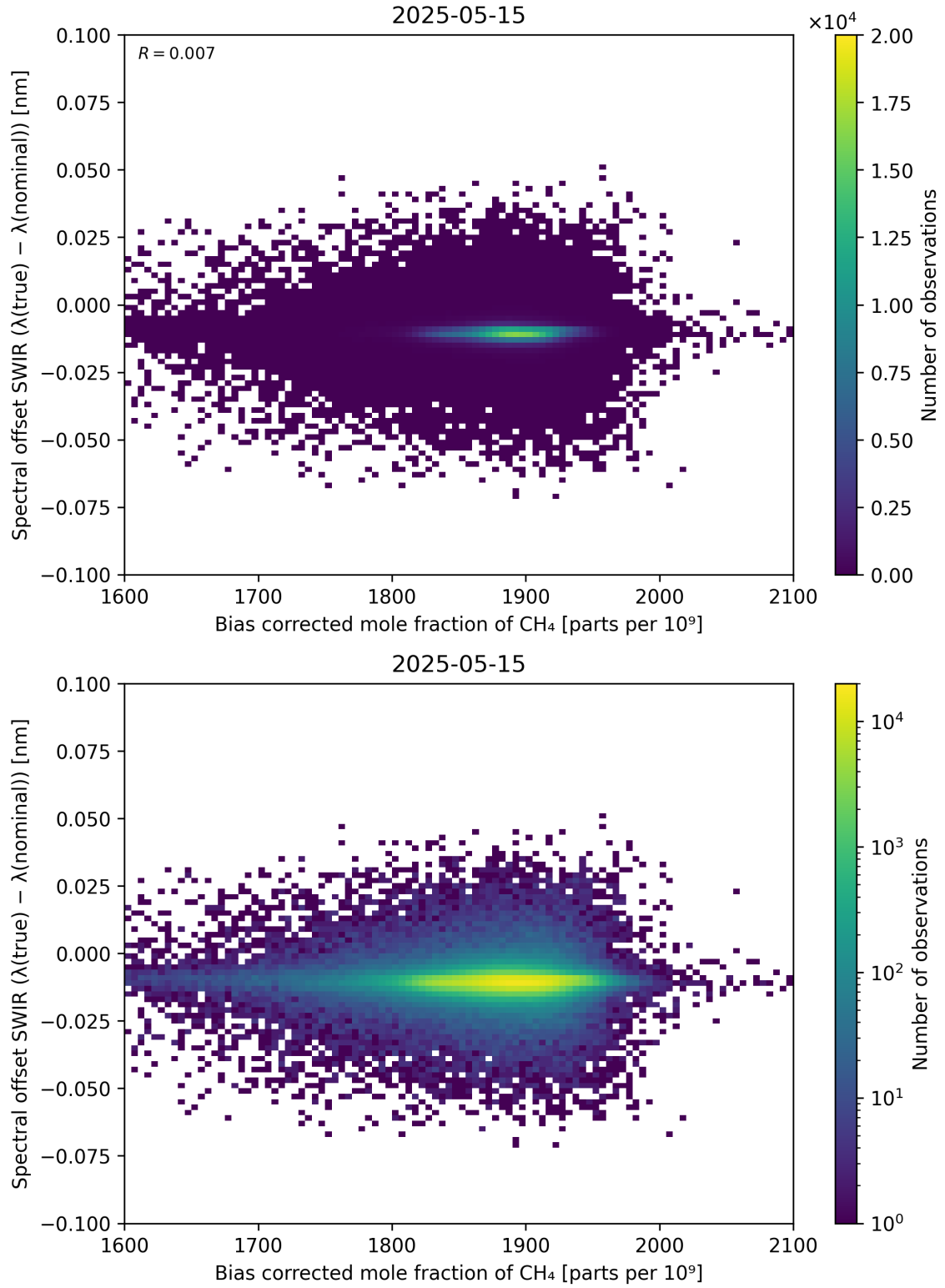
Figure 69: Scatter density plot of “Bias corrected mole fraction of \text{CH}_4 ” against “Spectral offset SWIR ( \lambda_{\text{true}} - \lambda_{\text{nominal}} )” for 2025-05-15 to 2025-05-16.
