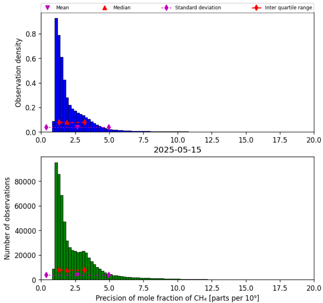
Figure 24: Histogram of “Precision of mole fraction of CH 4 ” for 2025-05-15 to 2025-05-16
