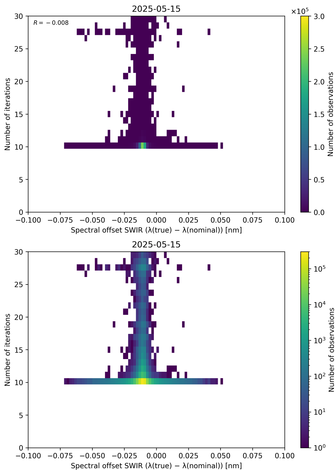
Figure 121: Scatter density plot of “Spectral offset SWIR ( \lambda_{\text{true}} - \lambda_{\text{nominal}} )” against “Number of iterations” for 2025-05-15 to 2025-05-16.
