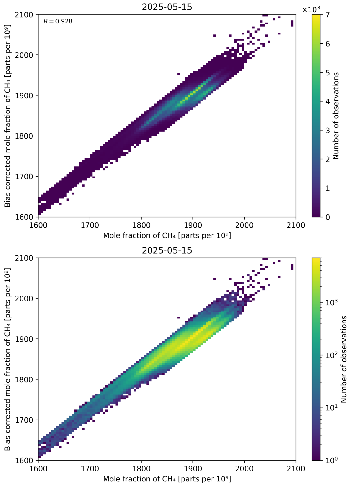
Figure 74: Scatter density plot of “Mole fraction of CH 4 ” against “Bias corrected mole fraction of CH 4 ” for 2025-05-15 to 2025-05-16.
