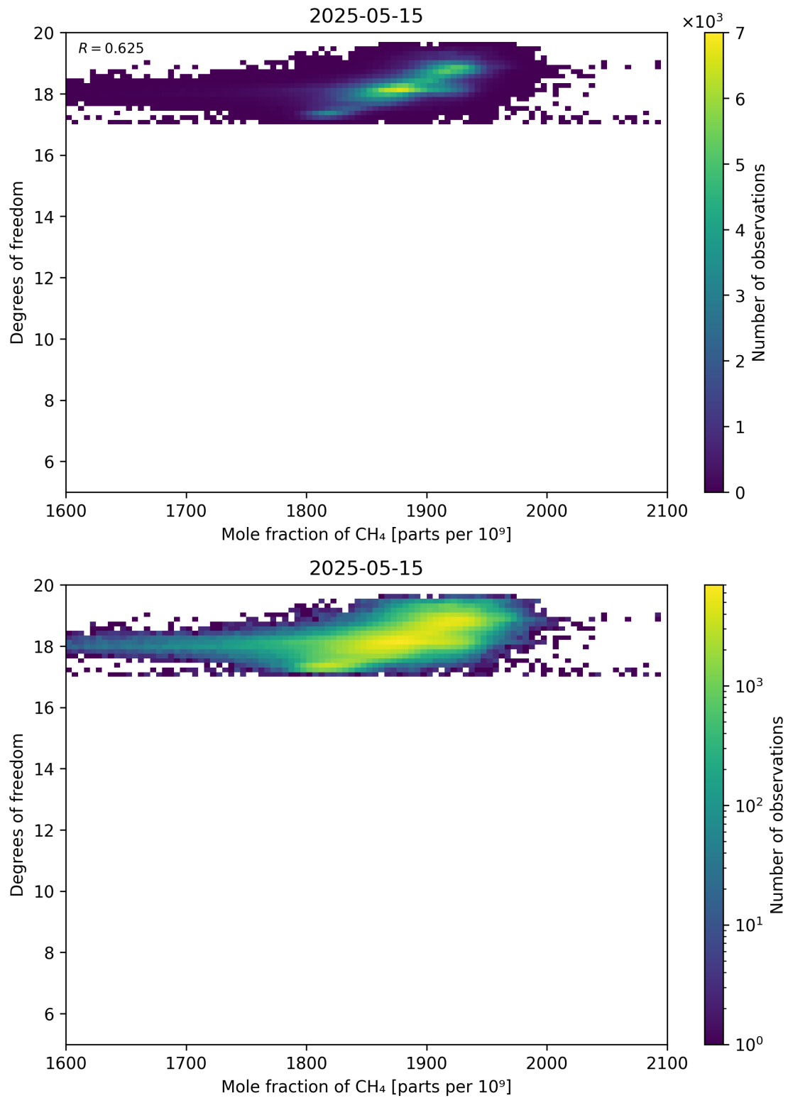
Figure 72: Scatter density plot of “Mole fraction of CH 4 ” against “Degrees of freedom” for 2025-05-15 to 2025-05-16.
