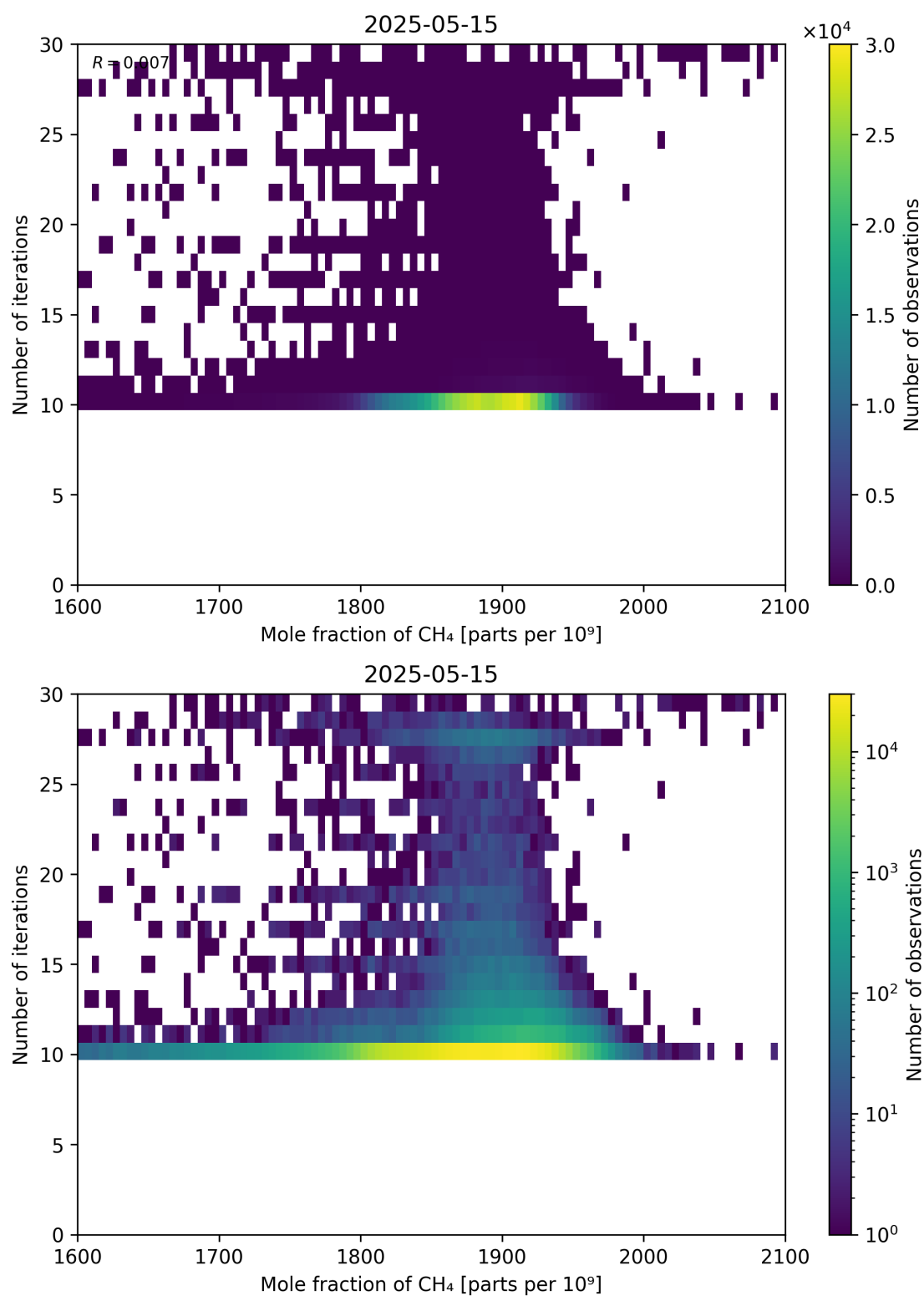
Figure 76: Scatter density plot of “Mole fraction of CH 4 ” against “Number of iterations” for 2025-05-15 to 2025-05-16.
