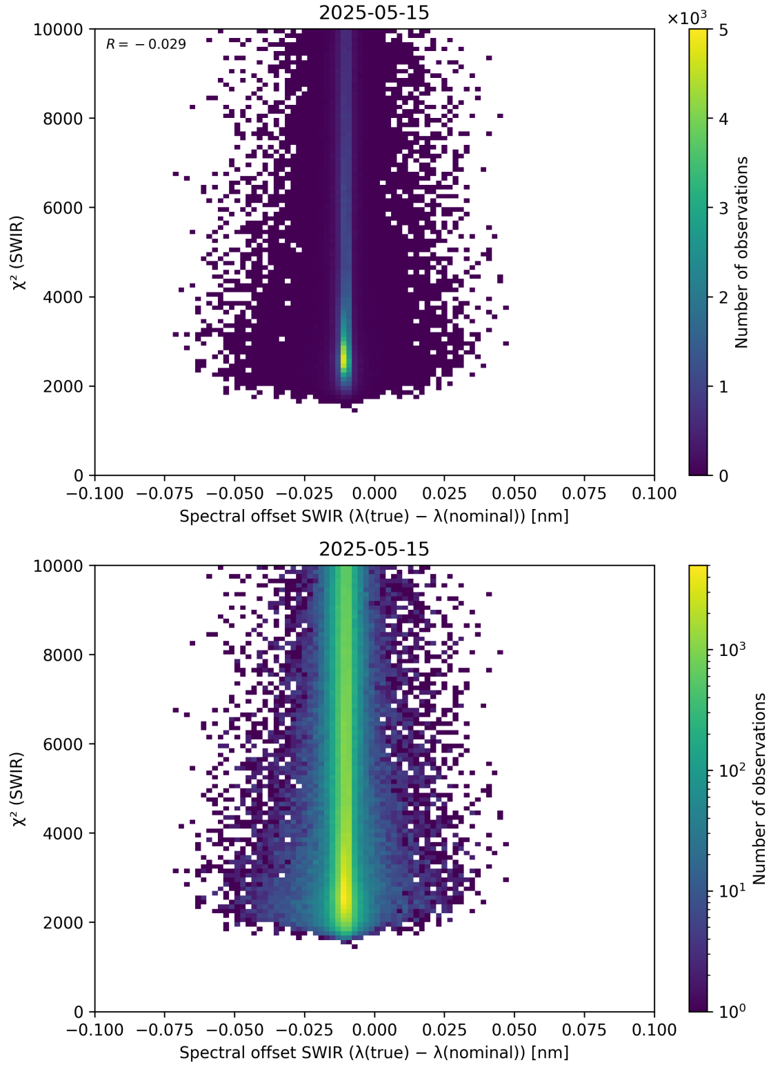
Figure 118: Scatter density plot of “Spectral offset SWIR ( \lambda_{\text{true}} - \lambda_{\text{nominal}} )” against “ \chi^2 (SWIR)” for 2025-05-15 to 2025-05-16.
