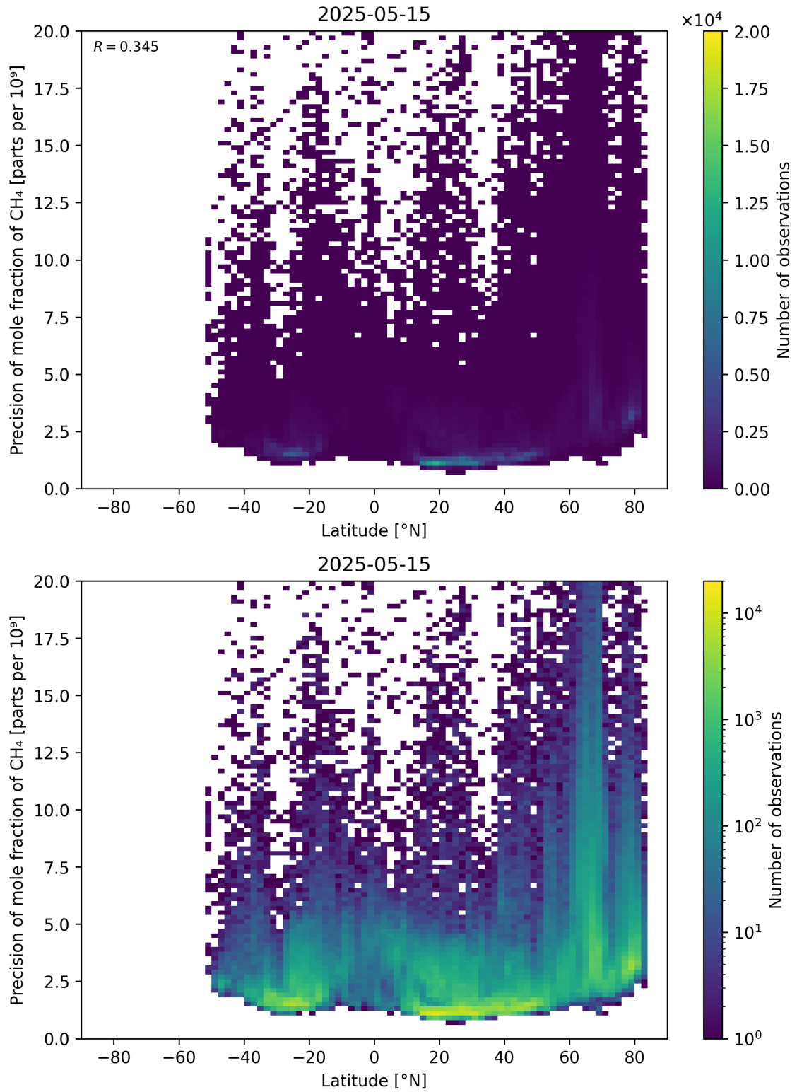
Figure 59: Scatter density plot of “Latitude” against “Precision of mole fraction of \text{CH}_4 ” for 2025-05-15 to 2025-05-16.
