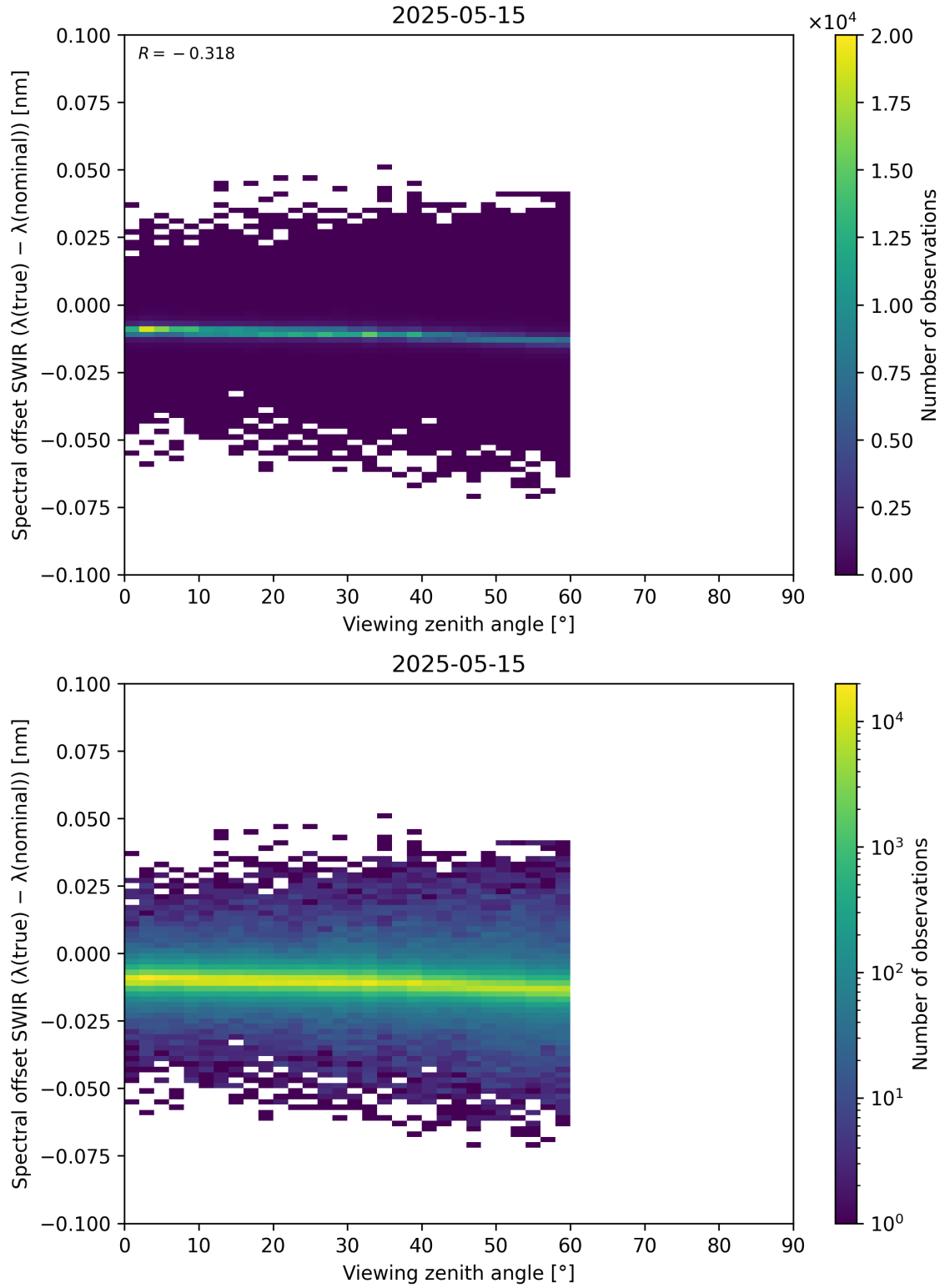
Figure 116: Scatter density plot of “Viewing zenith angle” against “Spectral offset SWIR ( \lambda_{\text{true}} - \lambda_{\text{nominal}} )” for 2025-05-15 to 2025-05-16.
