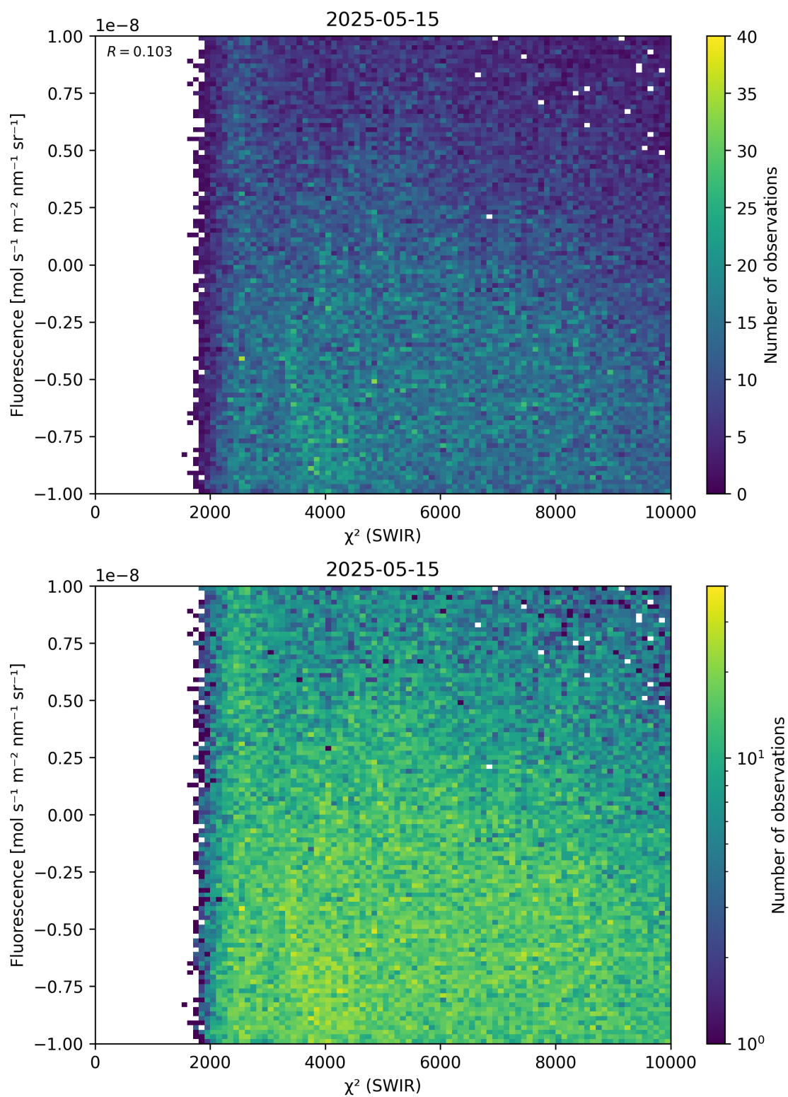
Figure 49: Scatter density plot of “ \chi^2 (SWIR)” against “Fluorescence” for 2025-05-15 to 2025-05-16.
