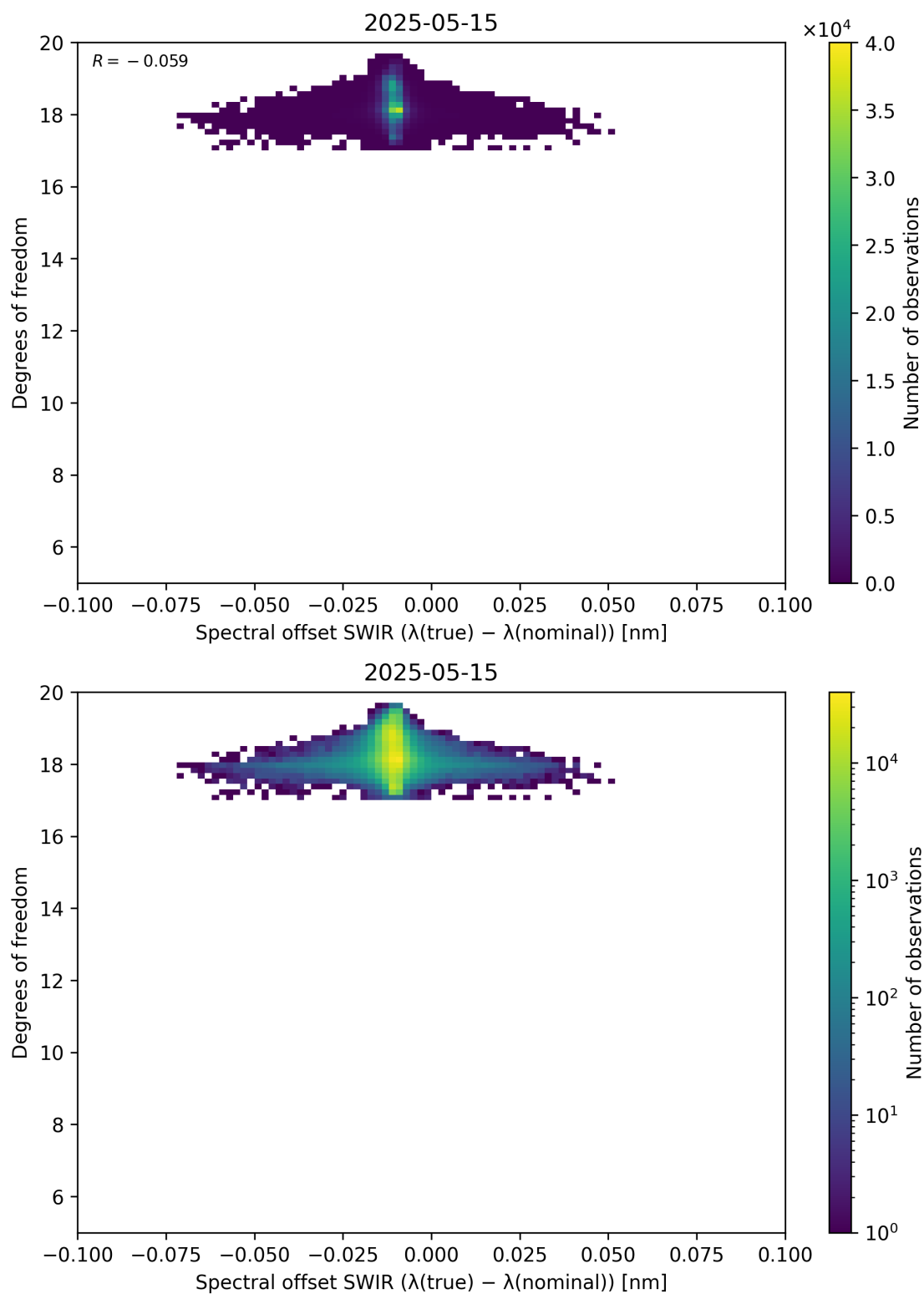
Figure 119: Scatter density plot of “Spectral offset SWIR ( \lambda_{\text{true}} - \lambda_{\text{nominal}} )” against “Degrees of freedom” for 2025-05-15 to 2025-05-16.
