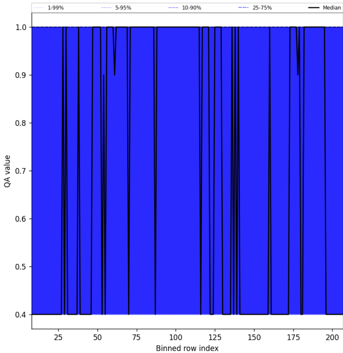
Figure 33: Along track statistics of “QA value” for 2025-05-15 to 2025-05-16
