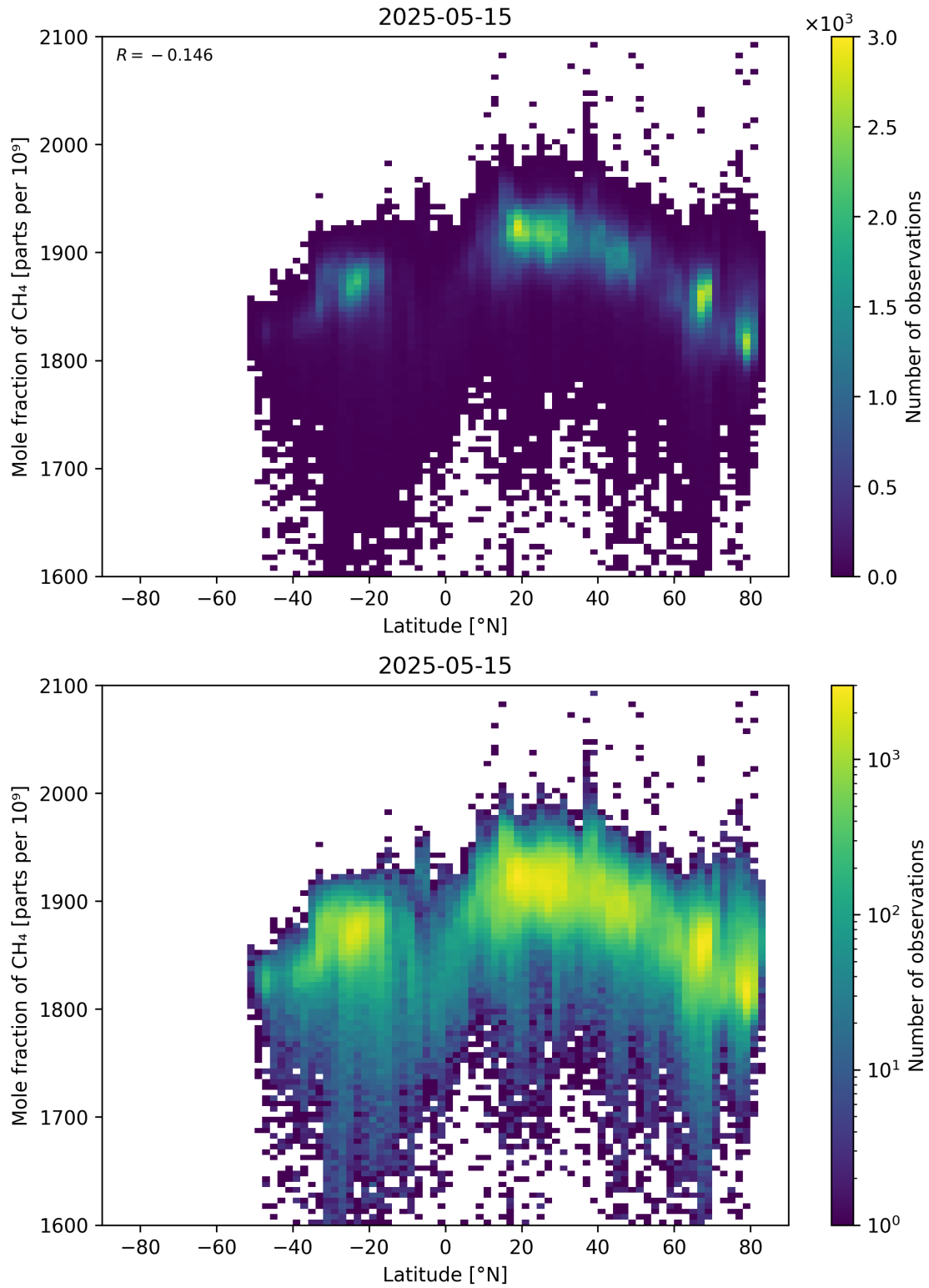
Figure 57: Scatter density plot of “Latitude” against “Mole fraction of CH 4 ” for 2025-05-15 to 2025-05-16.
