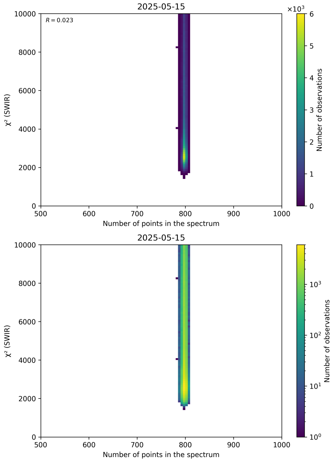
Figure 89: Scatter density plot of “Number of points in the spectrum” against “ \chi^2 (SWIR)” for 2025-05-15 to 2025-05-16.
