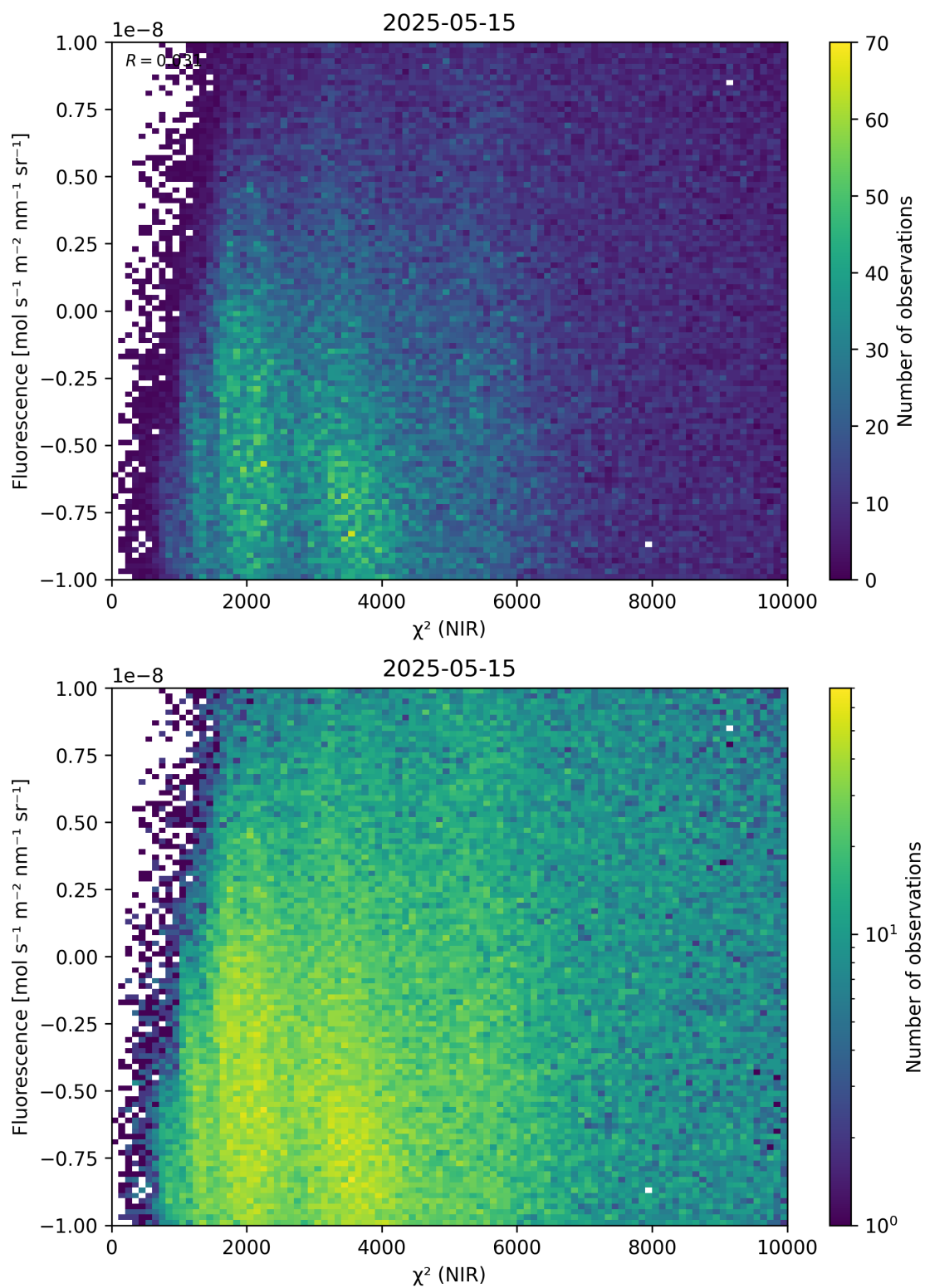
Figure 45: Scatter density plot of “ \chi^2 (NIR)” against “Fluorescence” for 2025-05-15 to 2025-05-16.
