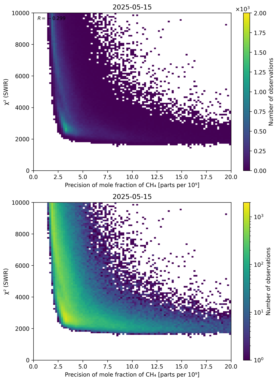
Figure 79: Scatter density plot of “Precision of mole fraction of \text{CH}_4 ” against “ \chi^2 (SWIR)” for 2025-05-15 to 2025-05-16.
