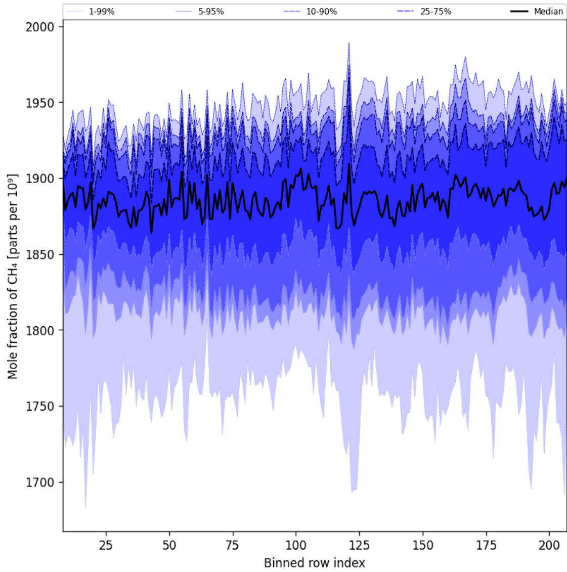
Figure 34: Along track statistics of “Mole fraction of CH 4 ” for 2025-05-15 to 2025-05-16
