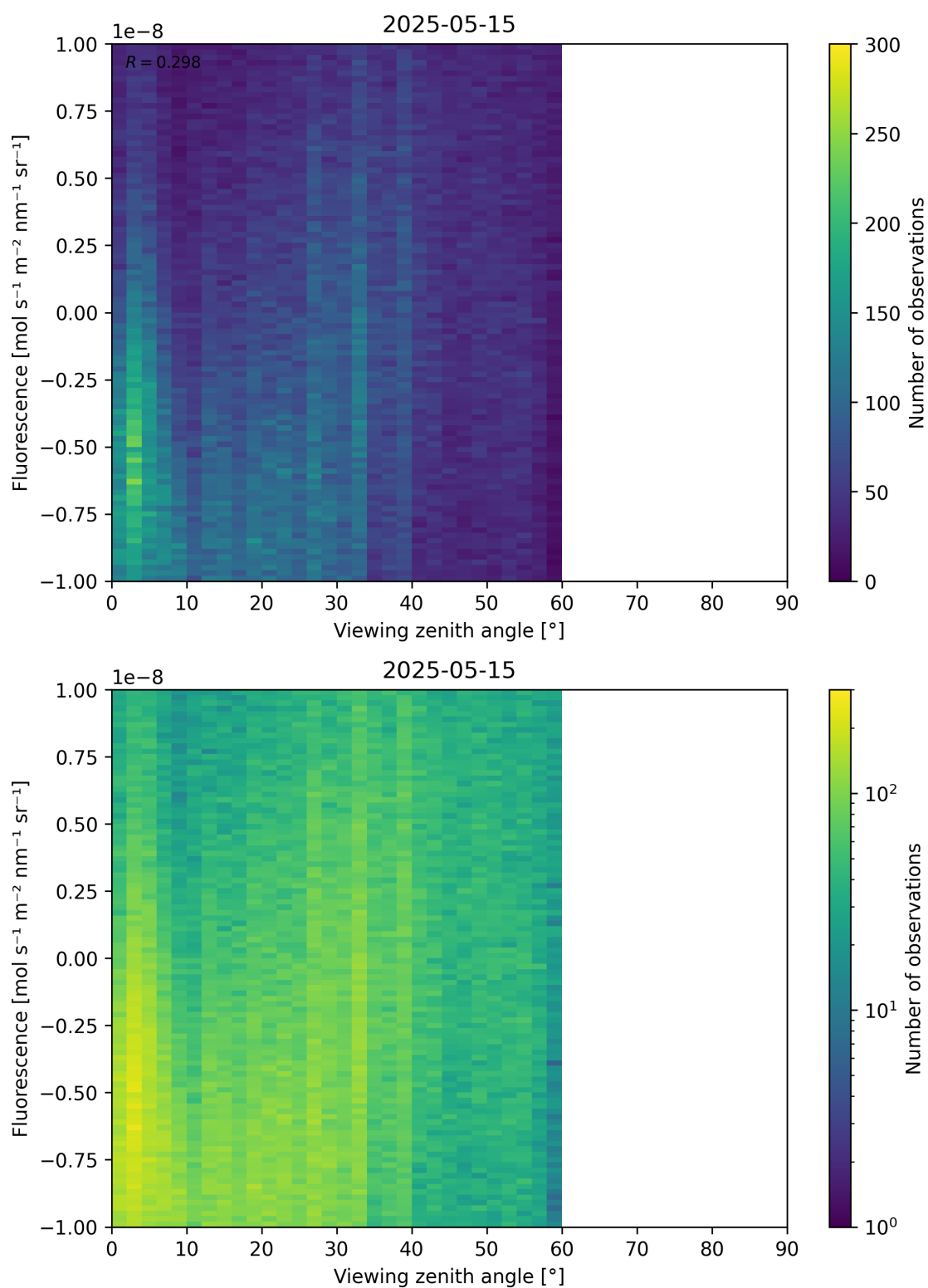
Figure 108: Scatter density plot of “Viewing zenith angle” against “Fluorescence” for 2025-05-15 to 2025-05-16.
