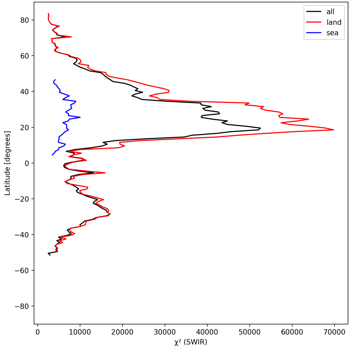
Figure 17: Zonal average of “ \chi^2 (SWIR)” for 2025-05-15 to 2025-05-16.
