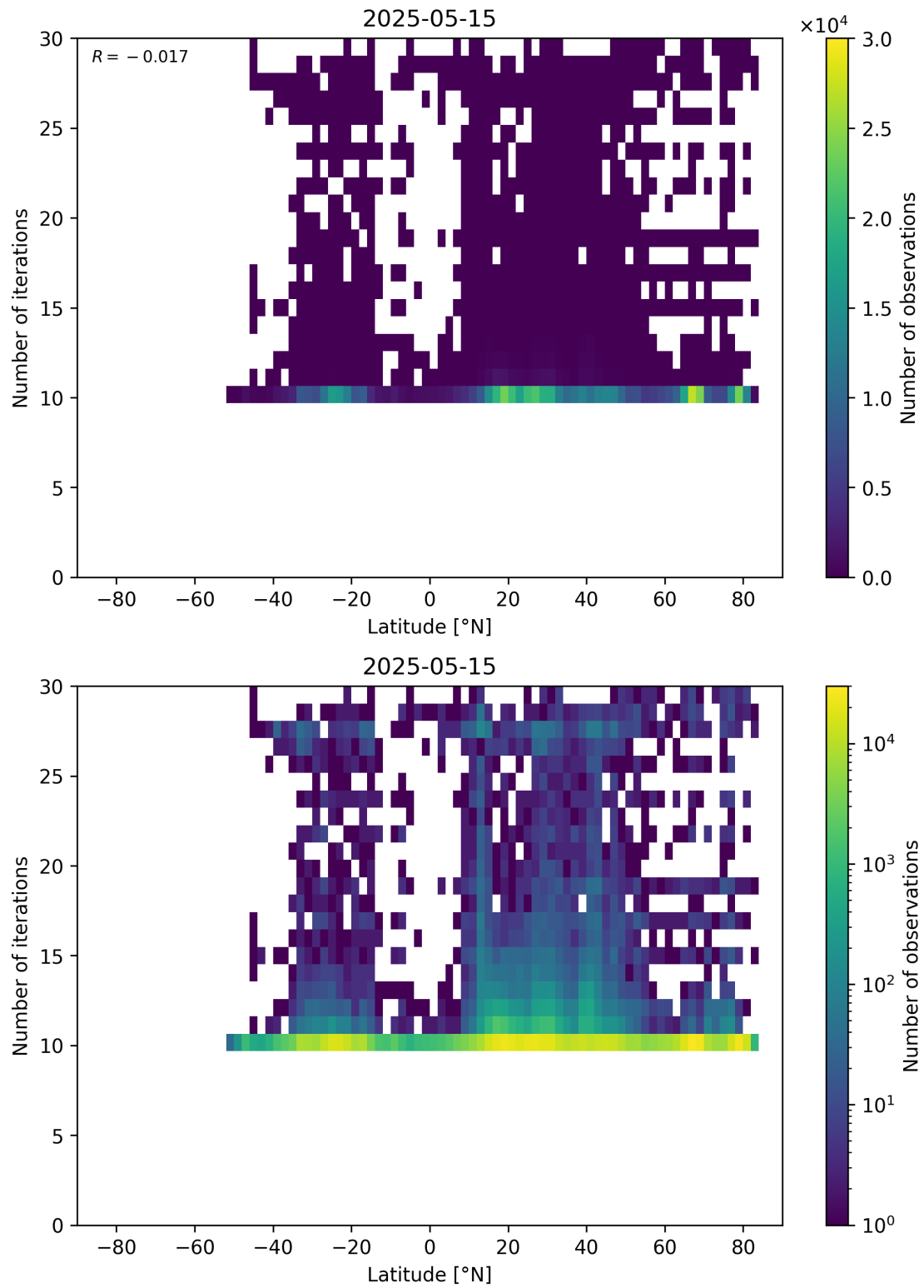
Figure 60: Scatter density plot of “Latitude” against “Number of iterations” for 2025-05-15 to 2025-05-16.
