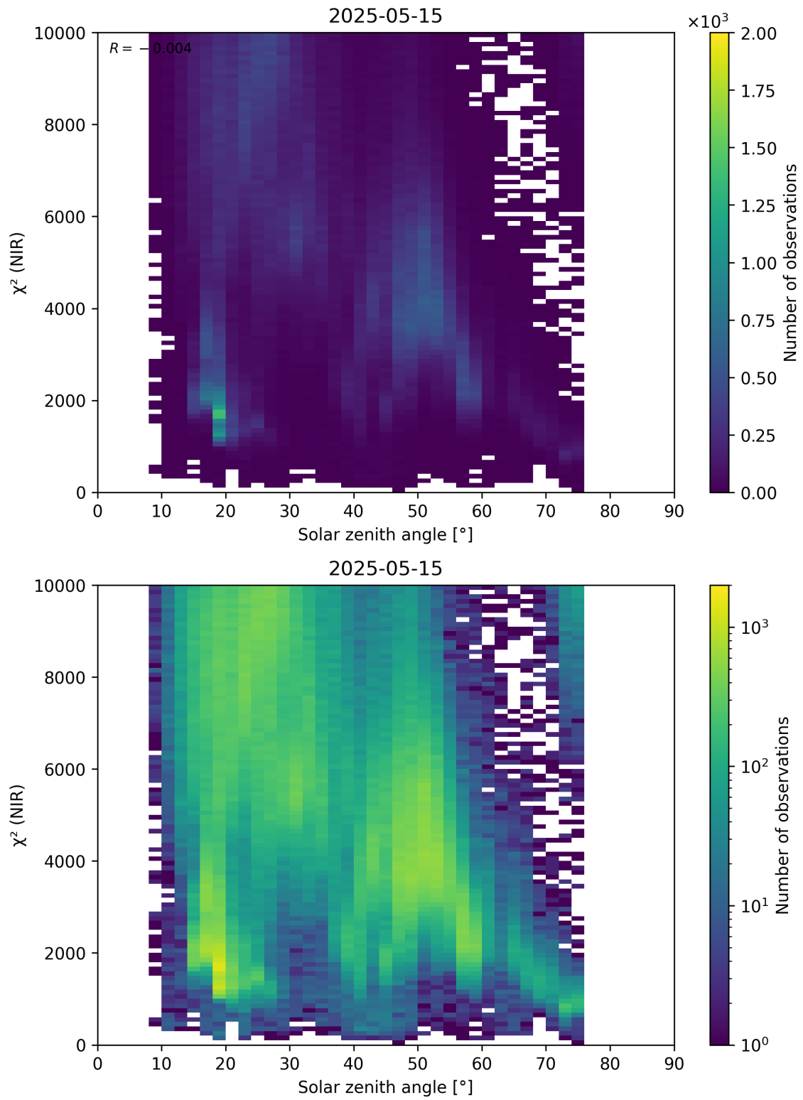
Figure 94: Scatter density plot of “Solar zenith angle” against “ \chi^2 (NIR)” for 2025-05-15 to 2025-05-16.
