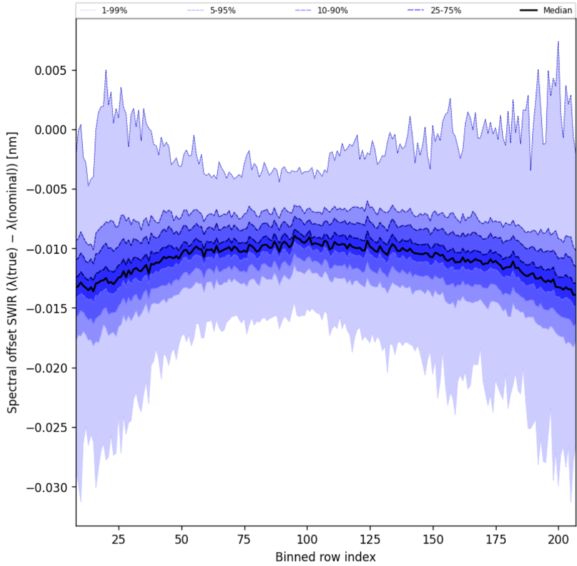
Figure 38: Along track statistics of “Spectral offset SWIR ( \lambda_{\text{true}} - \lambda_{\text{nominal}} )” for 2025-05-15 to 2025-05-16
