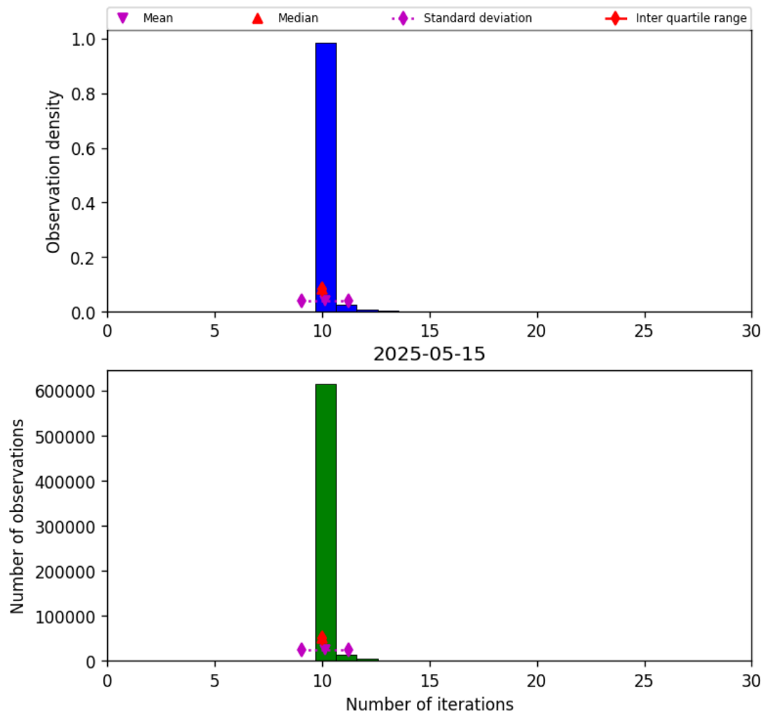
Figure 31: Histogram of “Number of iterations” for 2025-05-15 to 2025-05-16
