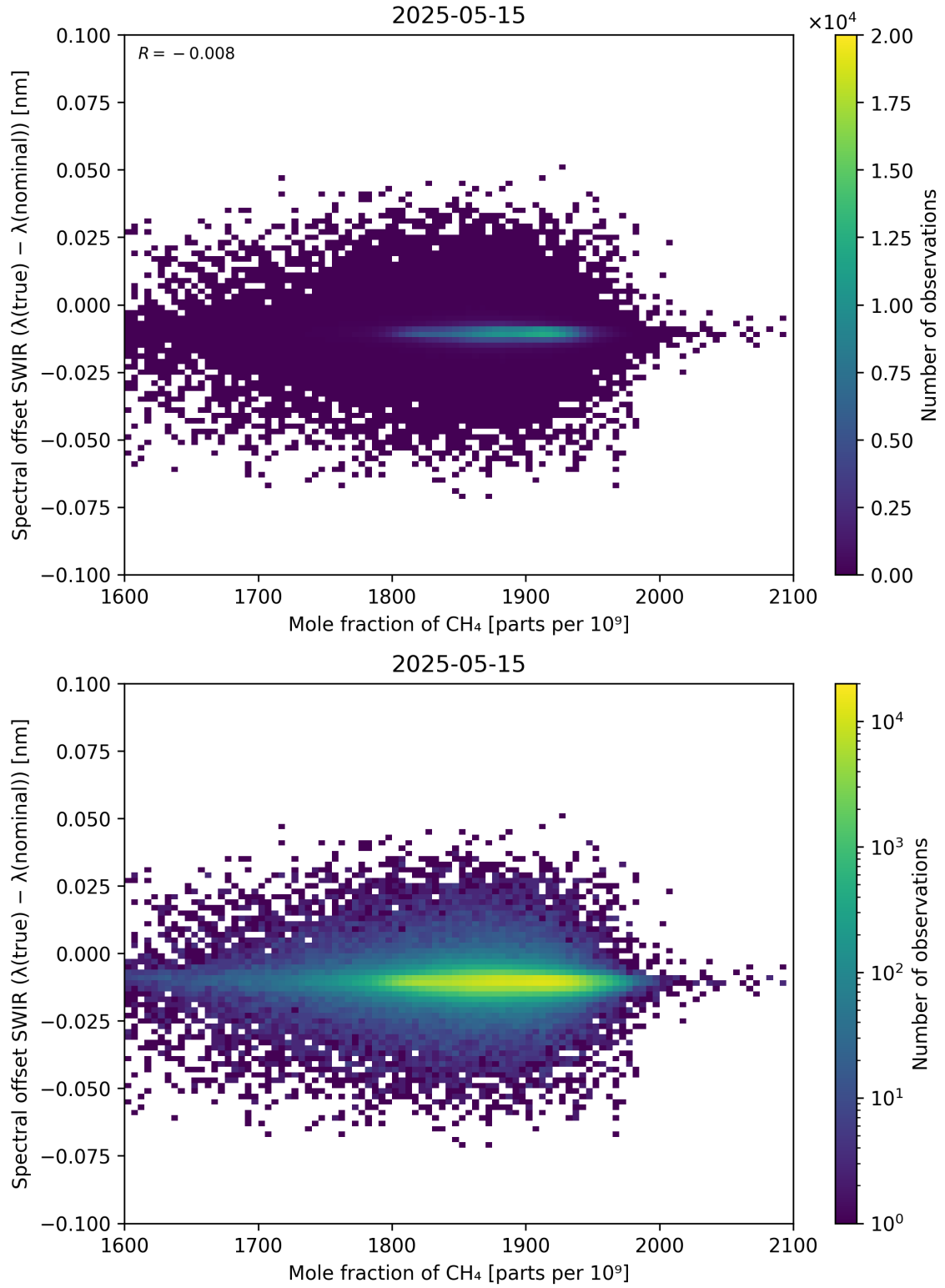
Figure 86: Scatter density plot of “Mole fraction of CH 4 ” against “Spectral offset SWIR ( \lambda_{\text{true}} - \lambda_{\text{nominal}} )” for 2025-05-15 to 2025-05-16.
