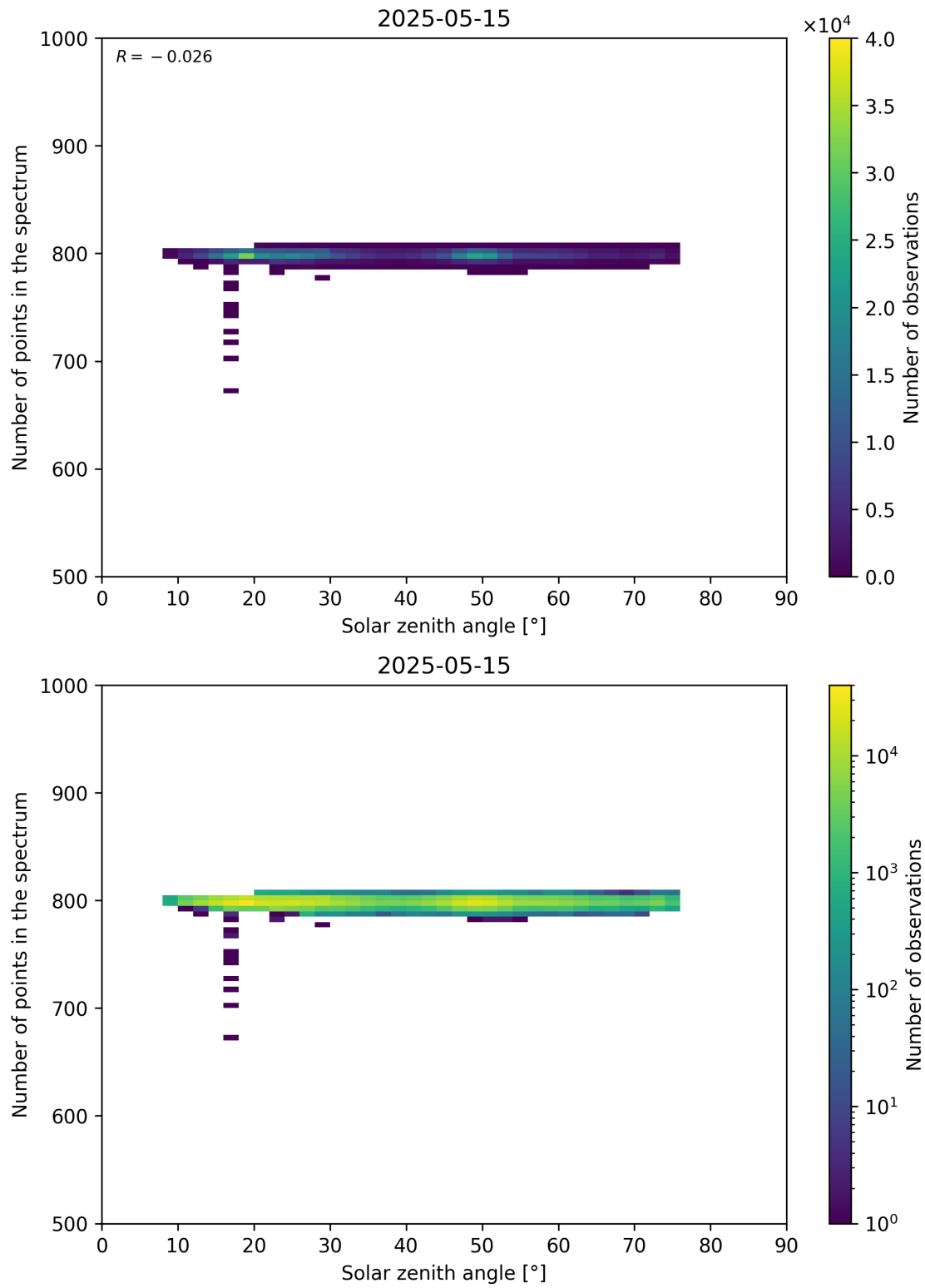
Figure 103: Scatter density plot of “Solar zenith angle” against “Number of points in the spectrum” for 2025-05-15 to 2025-05-16.
