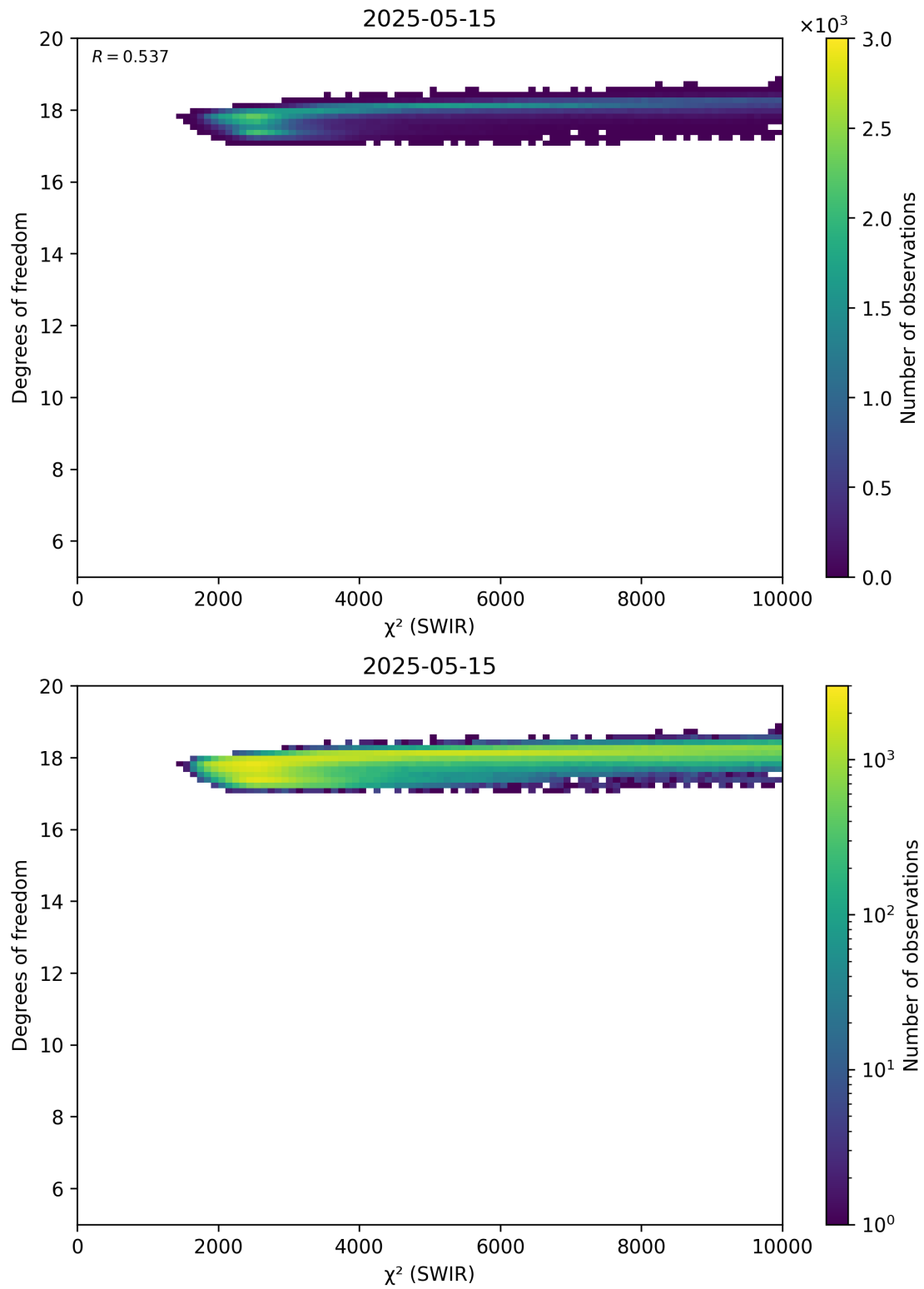
Figure 48: Scatter density plot of “ \chi^2 (SWIR)” against “Degrees of freedom” for 2025-05-15 to 2025-05-16.
