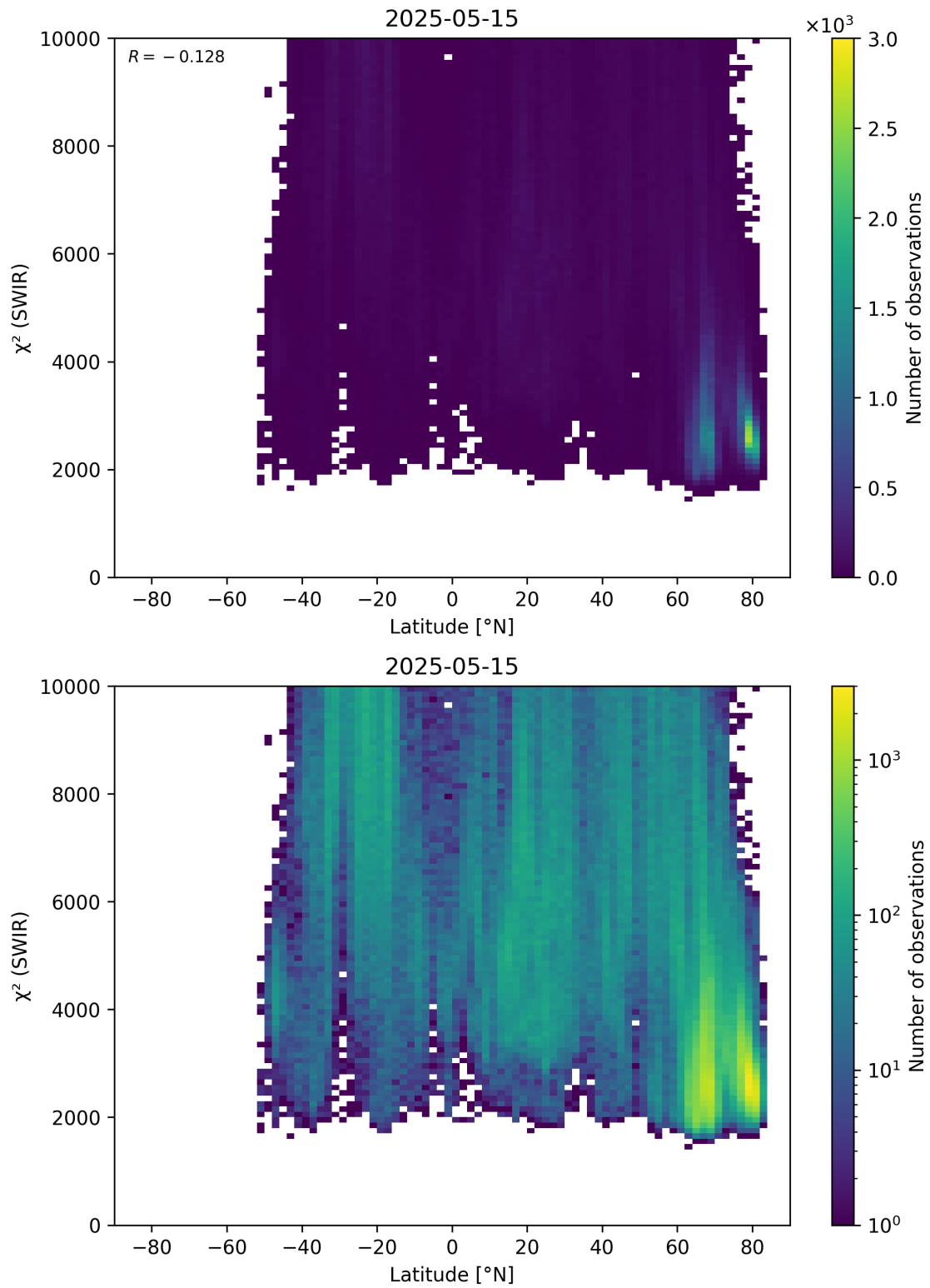
Figure 54: Scatter density plot of “Latitude” against “ \chi^2 (SWIR)” for 2025-05-15 to 2025-05-16.
