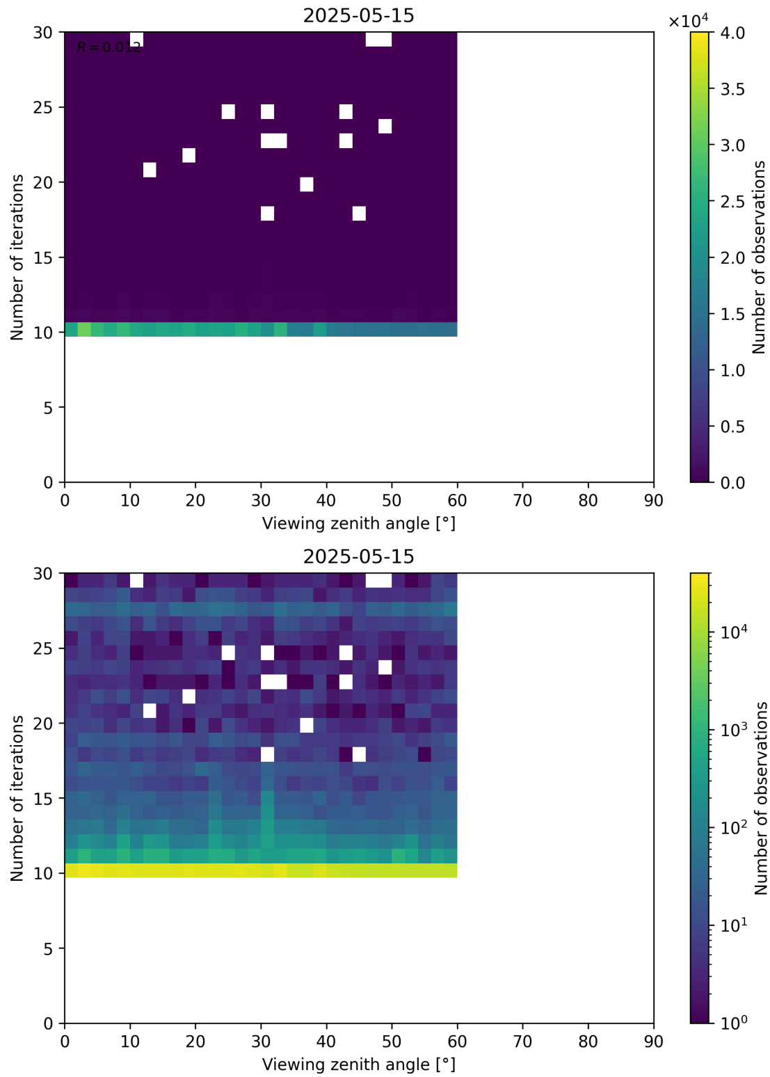
Figure 113: Scatter density plot of “Viewing zenith angle” against “Number of iterations” for 2025-05-15 to 2025-05-16.
