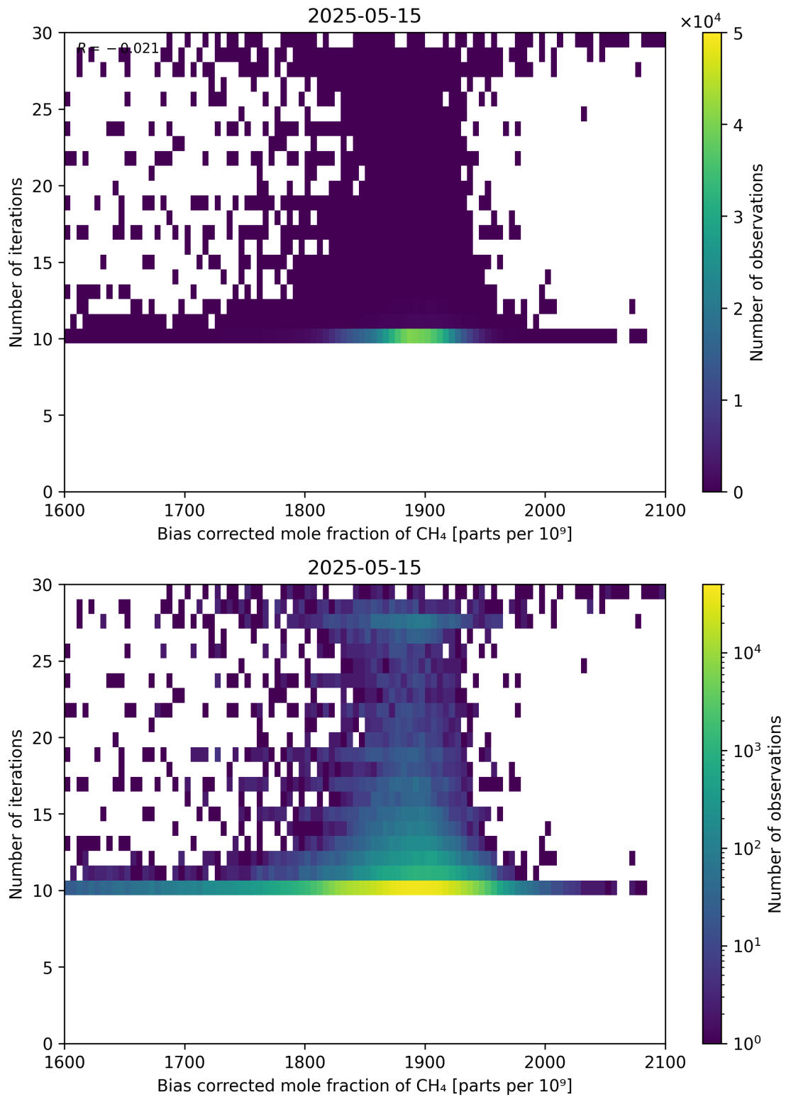
Figure 67: Scatter density plot of “Bias corrected mole fraction of CH 4 ” against “Number of iterations” for 2025-05-15 to 2025-05-16.
