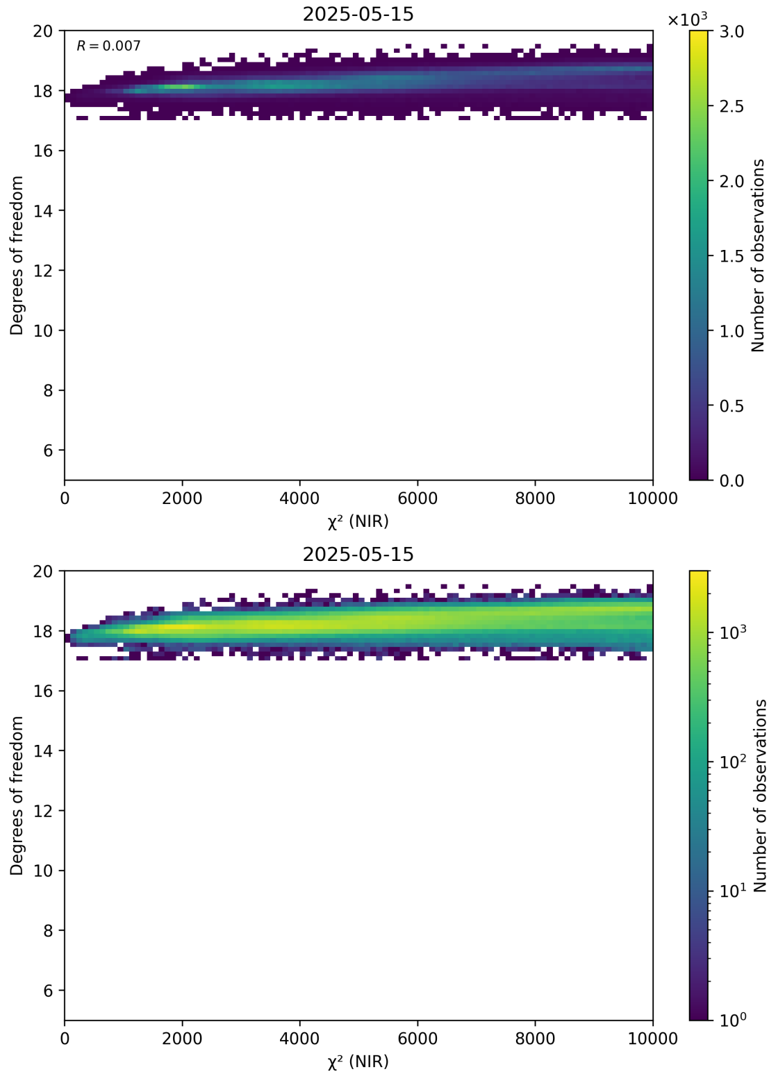
Figure 44: Scatter density plot of “ \chi^2 (NIR)” against “Degrees of freedom” for 2025-05-15 to 2025-05-16.
