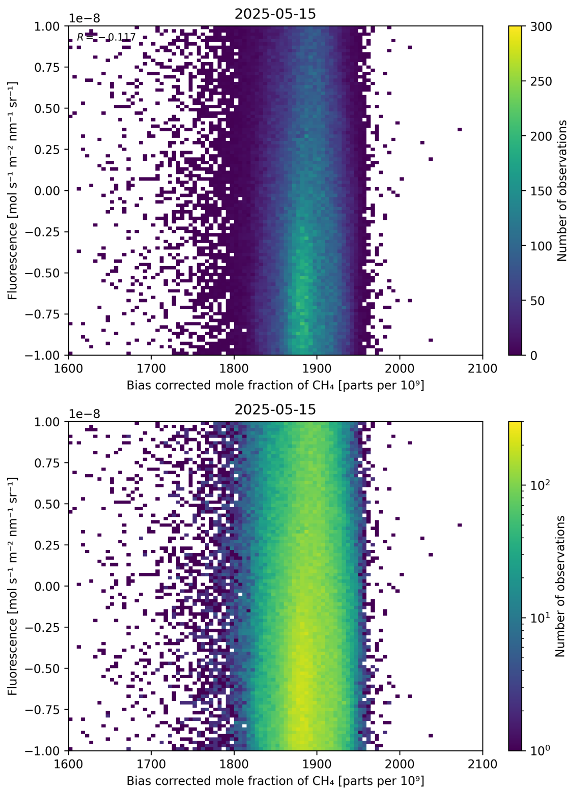
Figure 66: Scatter density plot of “Bias corrected mole fraction of \text{CH}_4 ” against “Fluorescence” for 2025-05-15 to 2025-05-16.
