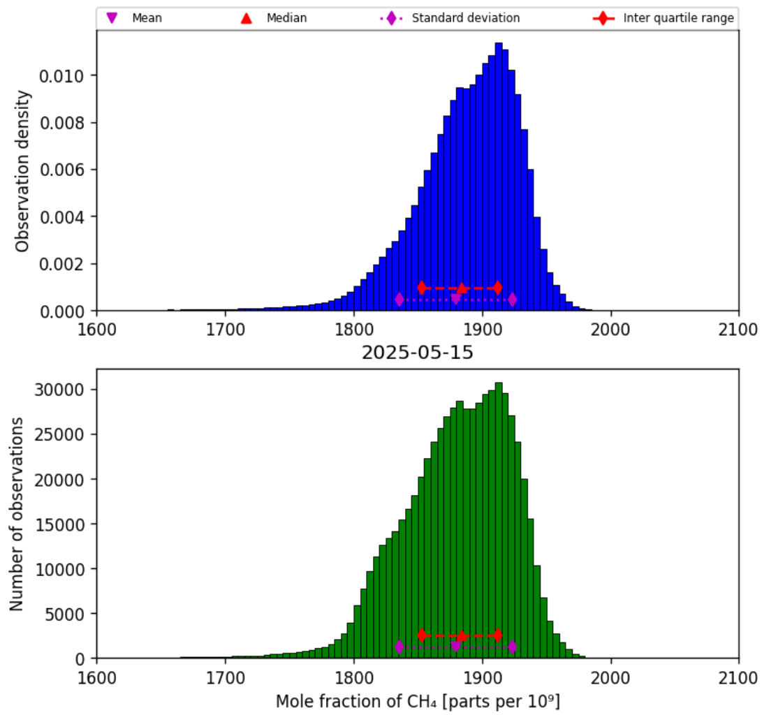
Figure 23: Histogram of “Mole fraction of CH 4 ” for 2025-05-15 to 2025-05-16
