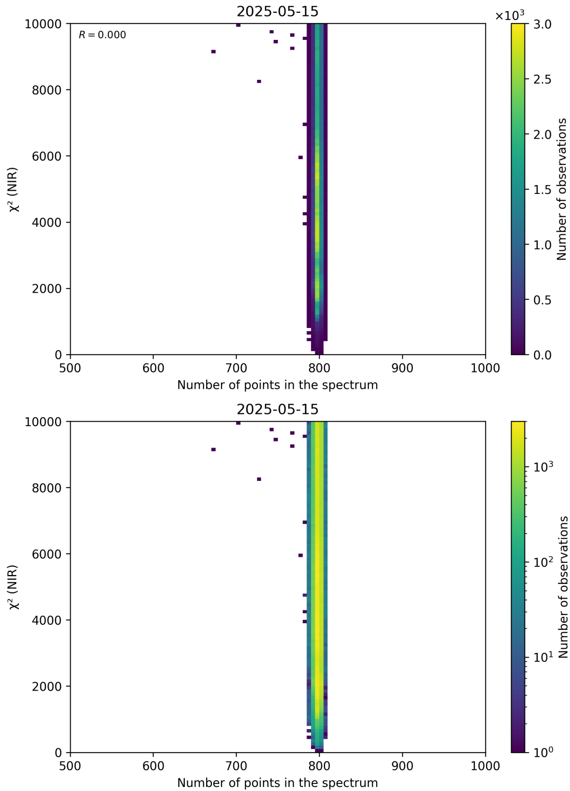
Figure 88: Scatter density plot of “Number of points in the spectrum” against “ \chi^2 (NIR)” for 2025-05-15 to 2025-05-16.
