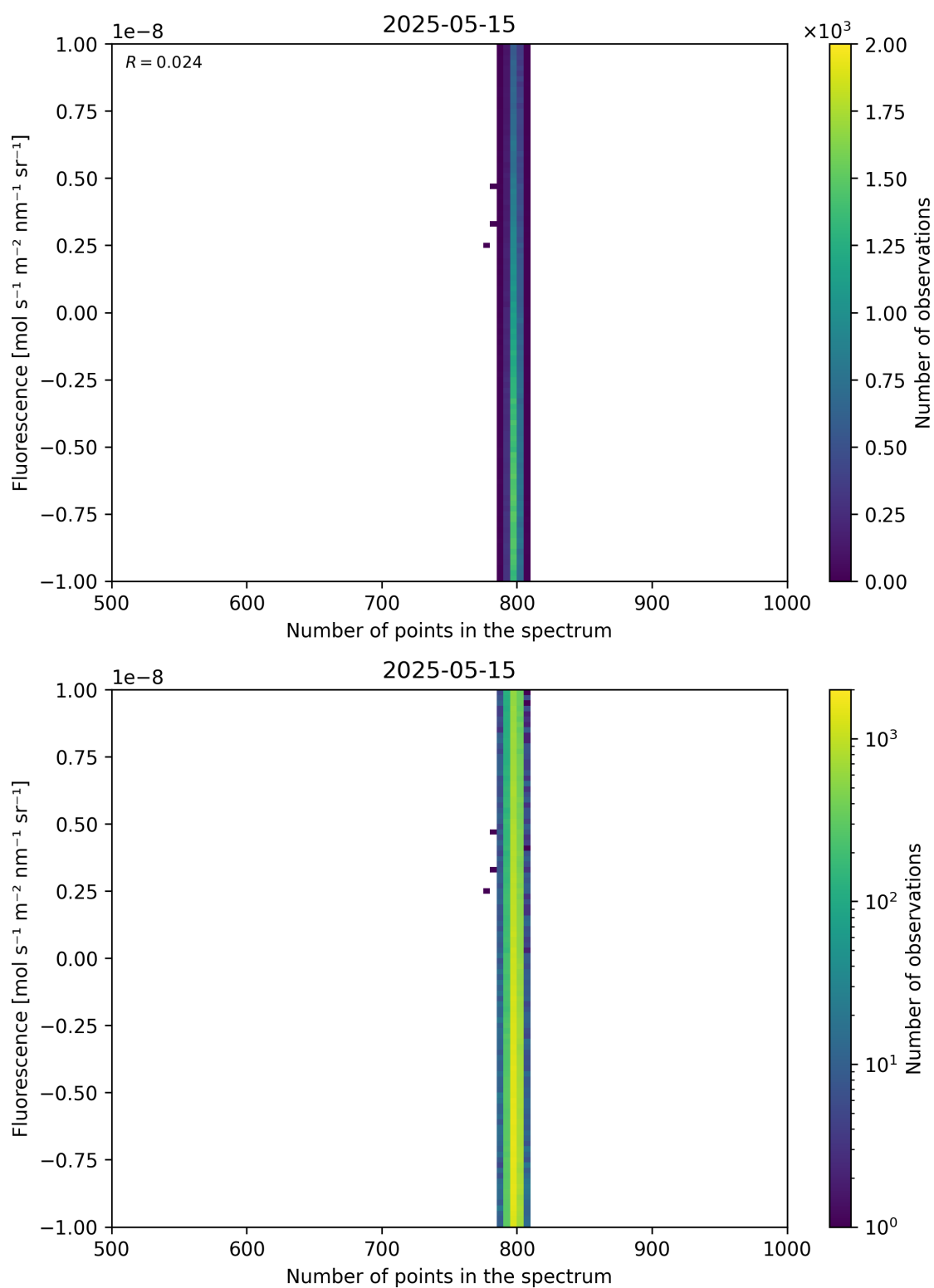
Figure 91: Scatter density plot of “Number of points in the spectrum” against “Fluorescence” for 2025-05-15 to 2025-05-16.
