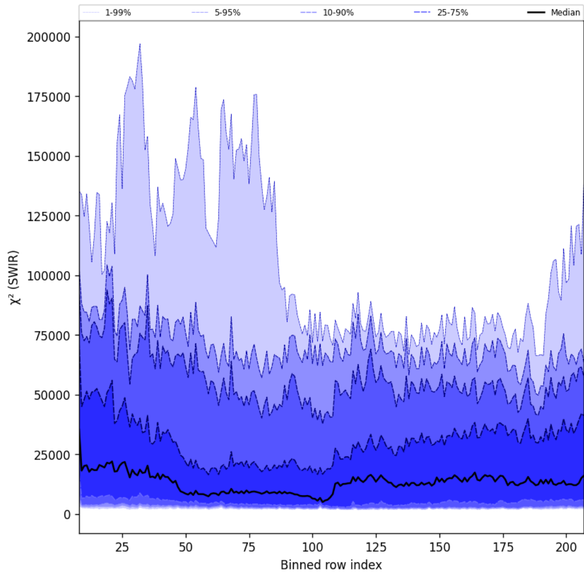
Figure 39: Along track statistics of “ \chi^2 (SWIR)” for 2025-05-15 to 2025-05-16
