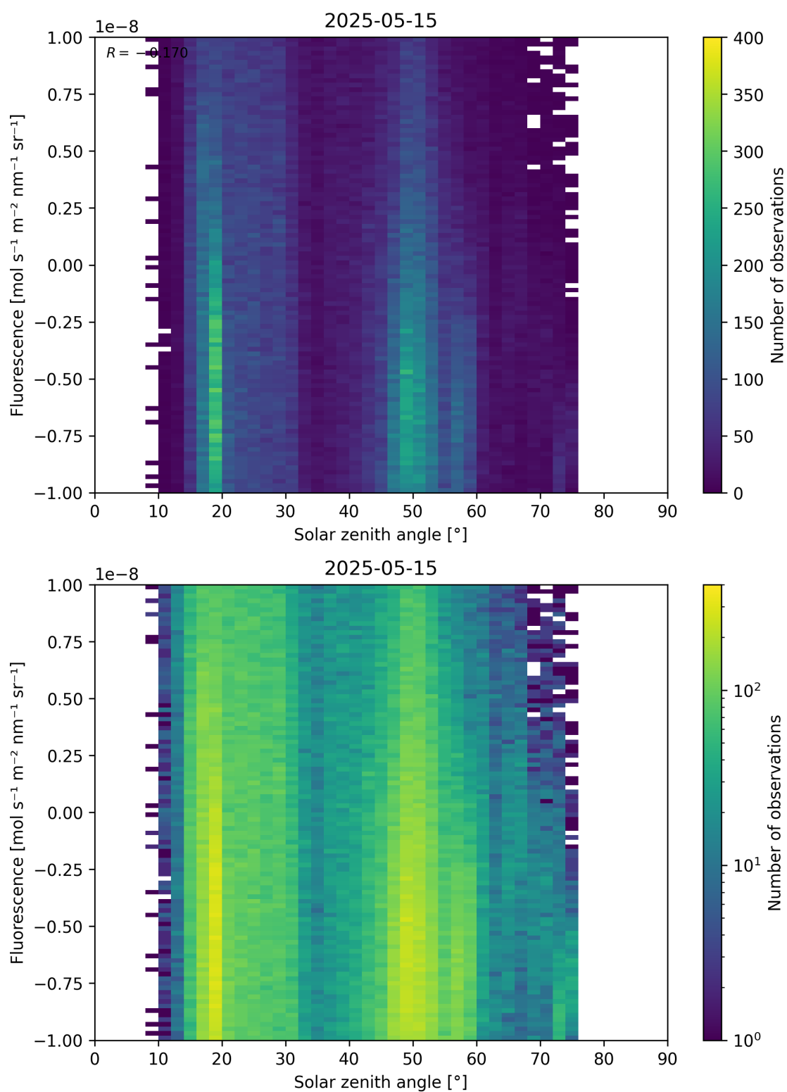
Figure 97: Scatter density plot of “Solar zenith angle” against “Fluorescence” for 2025-05-15 to 2025-05-16.
