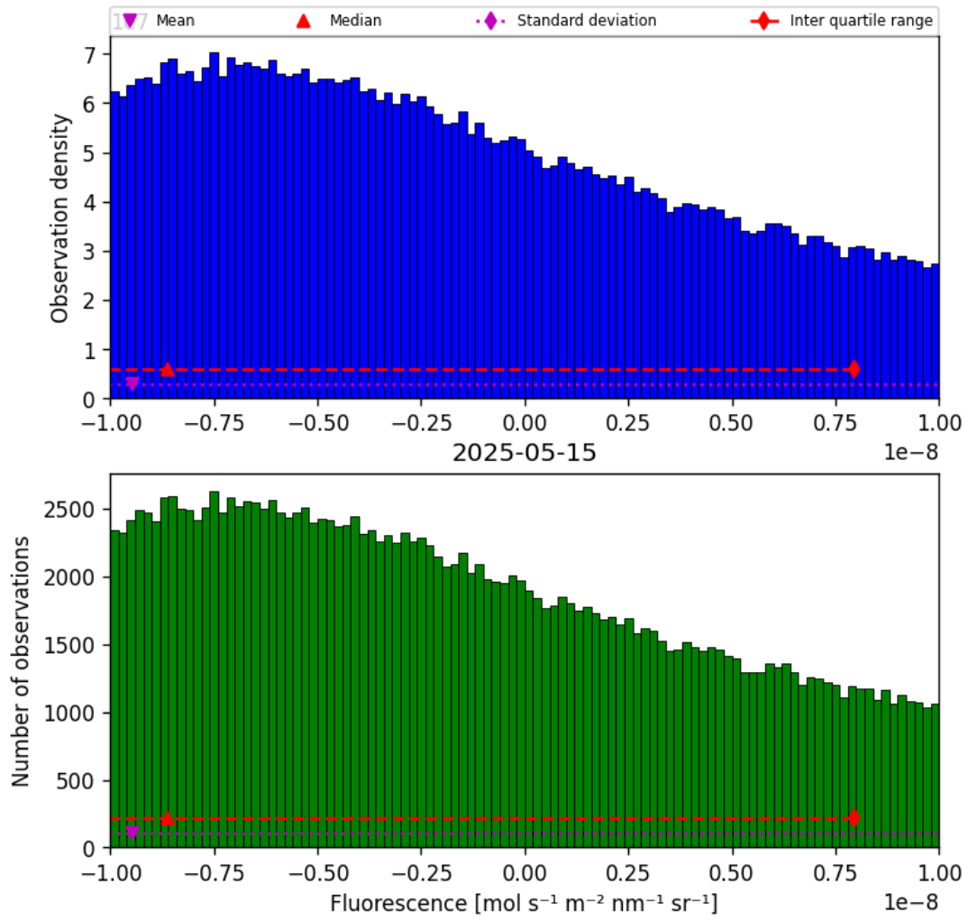
Figure 32: Histogram of “Fluorescence” for 2025-05-15 to 2025-05-16
