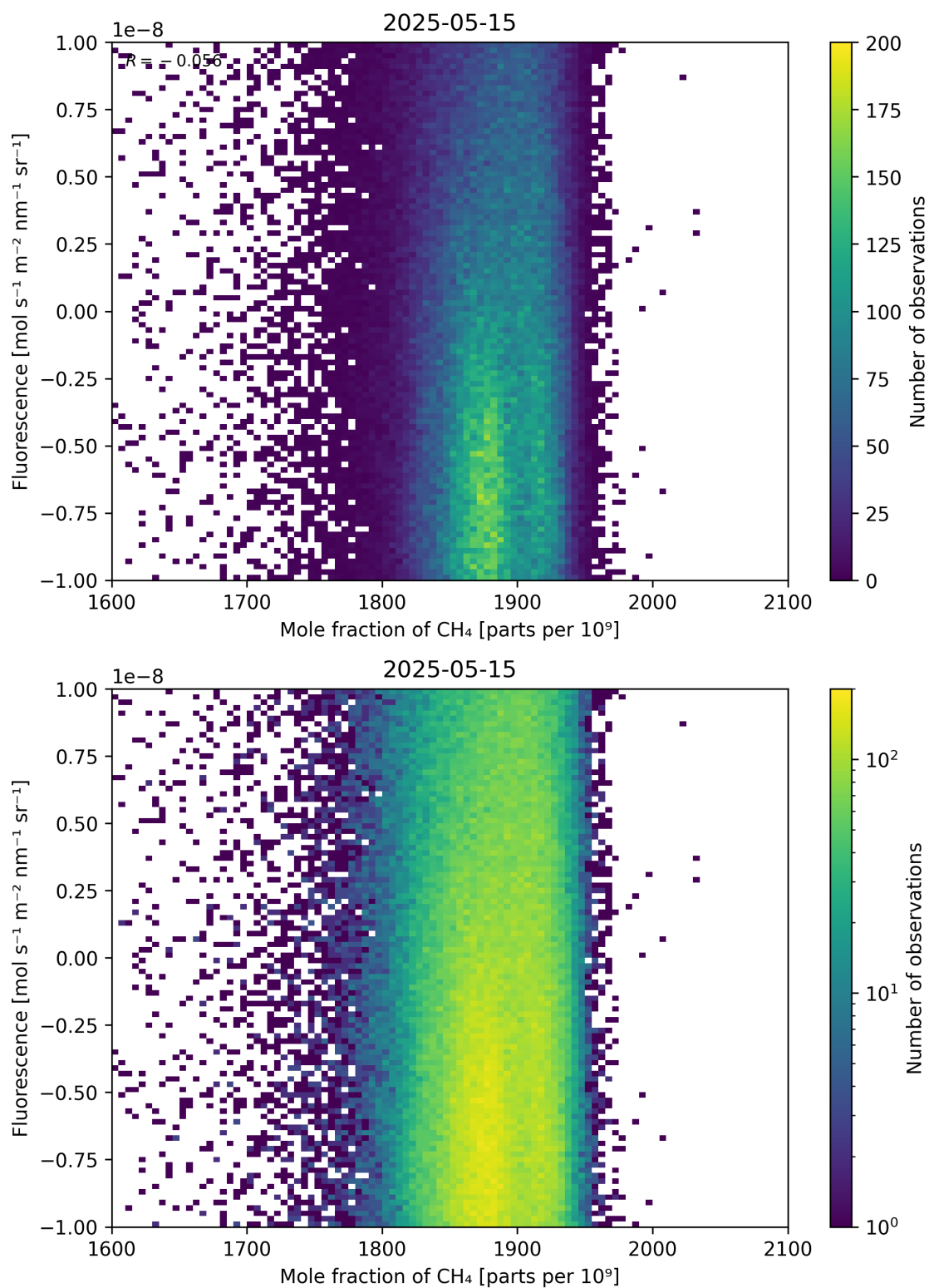
Figure 73: Scatter density plot of “Mole fraction of \text{CH}_4 ” against “Fluorescence” for 2025-05-15 to 2025-05-16.
