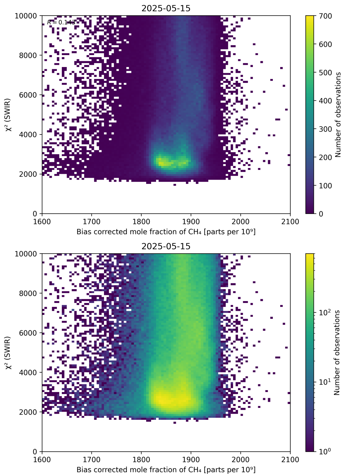
Figure 64: Scatter density plot of “Bias corrected mole fraction of \text{CH}_4 ” against “ \chi^2 (SWIR)” for 2025-05-15 to 2025-05-16.
