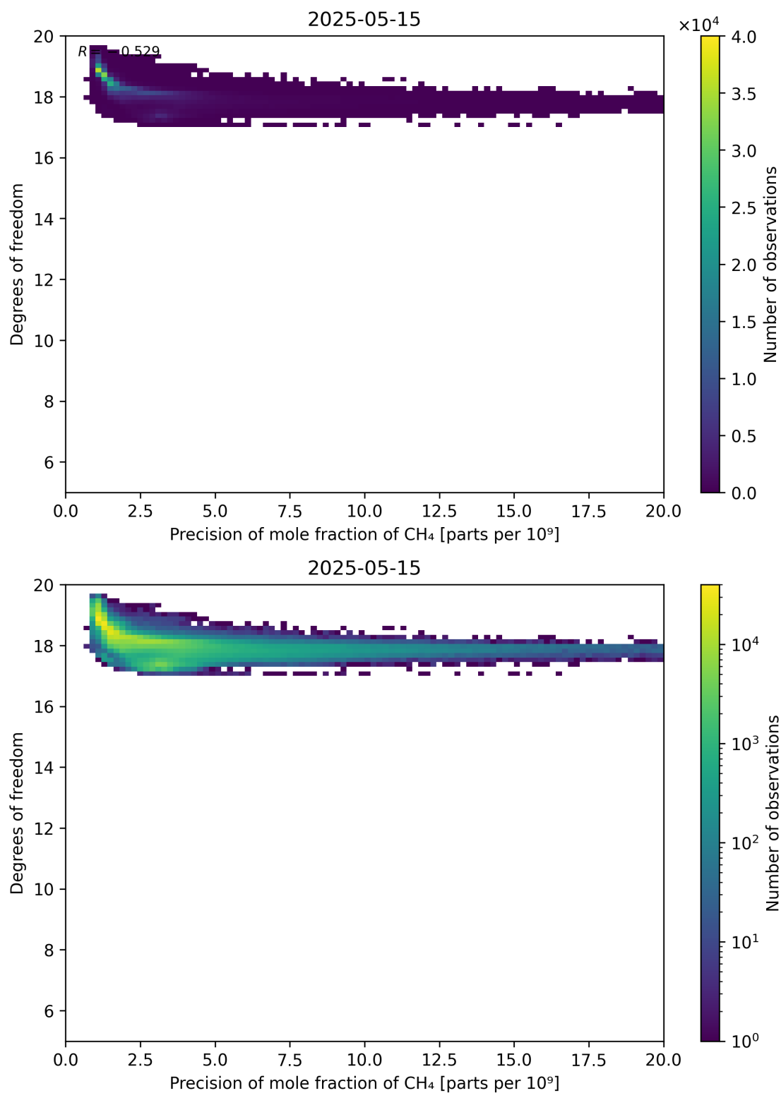
Figure 80: Scatter density plot of “Precision of mole fraction of CH 4 ” against “Degrees of freedom” for 2025-05-15 to 2025-05-16.
