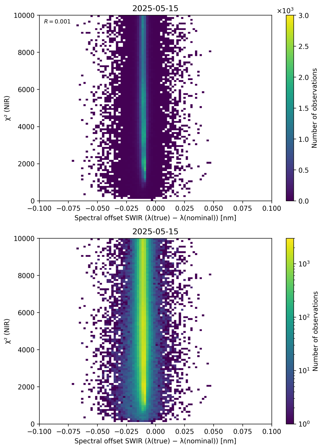
Figure 117: Scatter density plot of “Spectral offset SWIR ( \lambda_{\text{true}} - \lambda_{\text{nominal}} )” against “ \chi^2 (NIR)” for 2025-05-15 to 2025-05-16.
