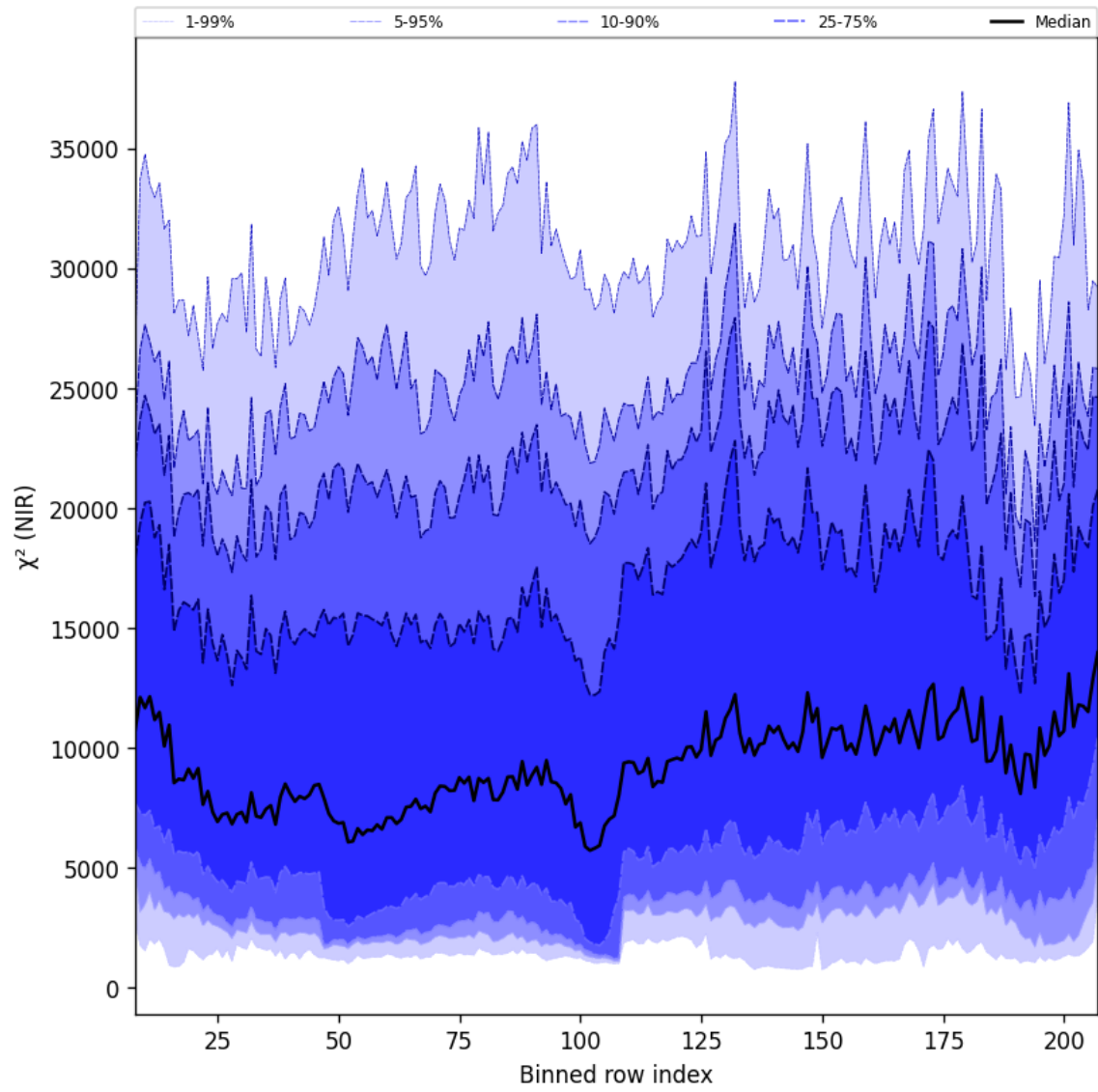
Figure 40: Along track statistics of “ \chi^2 (NIR)” for 2025-05-15 to 2025-05-16
