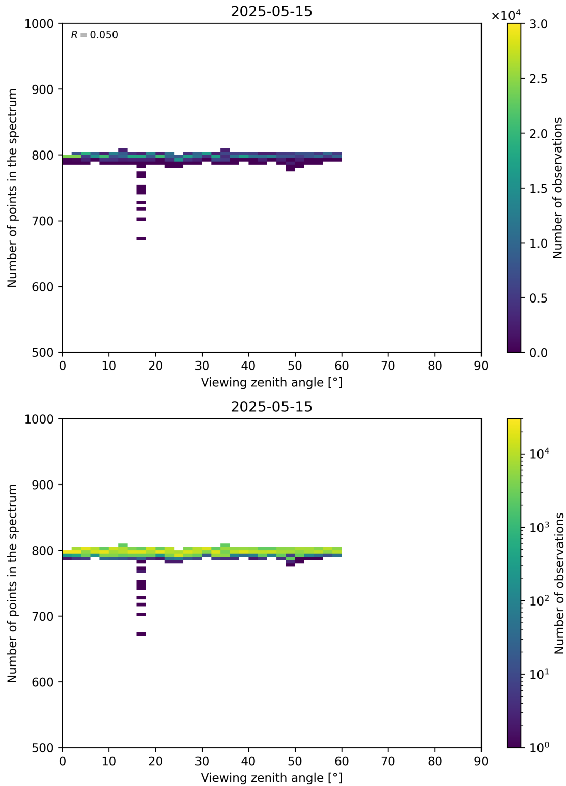
Figure 114: Scatter density plot of “Viewing zenith angle” against “Number of points in the spectrum” for 2025-05-15 to 2025-05-16.
