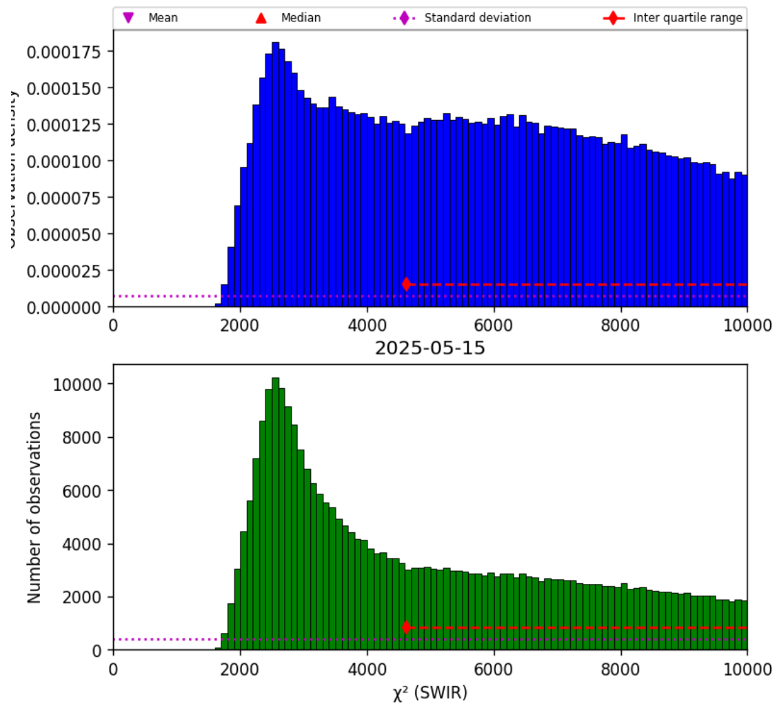
Figure 28: Histogram of “ \chi^2 (SWIR)” for 2025-05-15 to 2025-05-16
