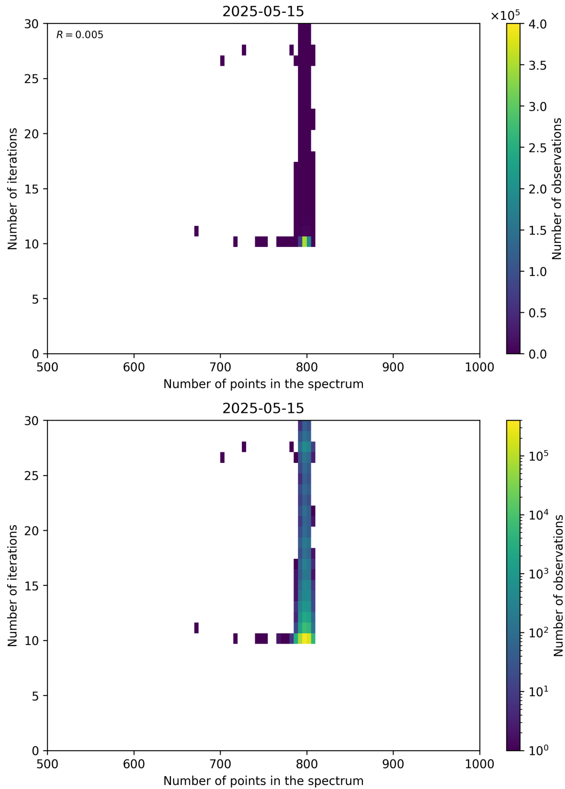
Figure 92: Scatter density plot of “Number of points in the spectrum” against “Number of iterations” for 2025-05-15 to 2025-05-16.
