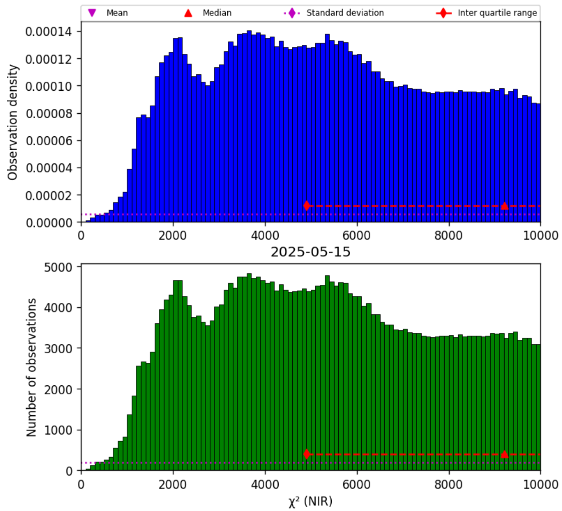
Figure 29: Histogram of “ \chi^2 (NIR)” for 2025-05-15 to 2025-05-16
