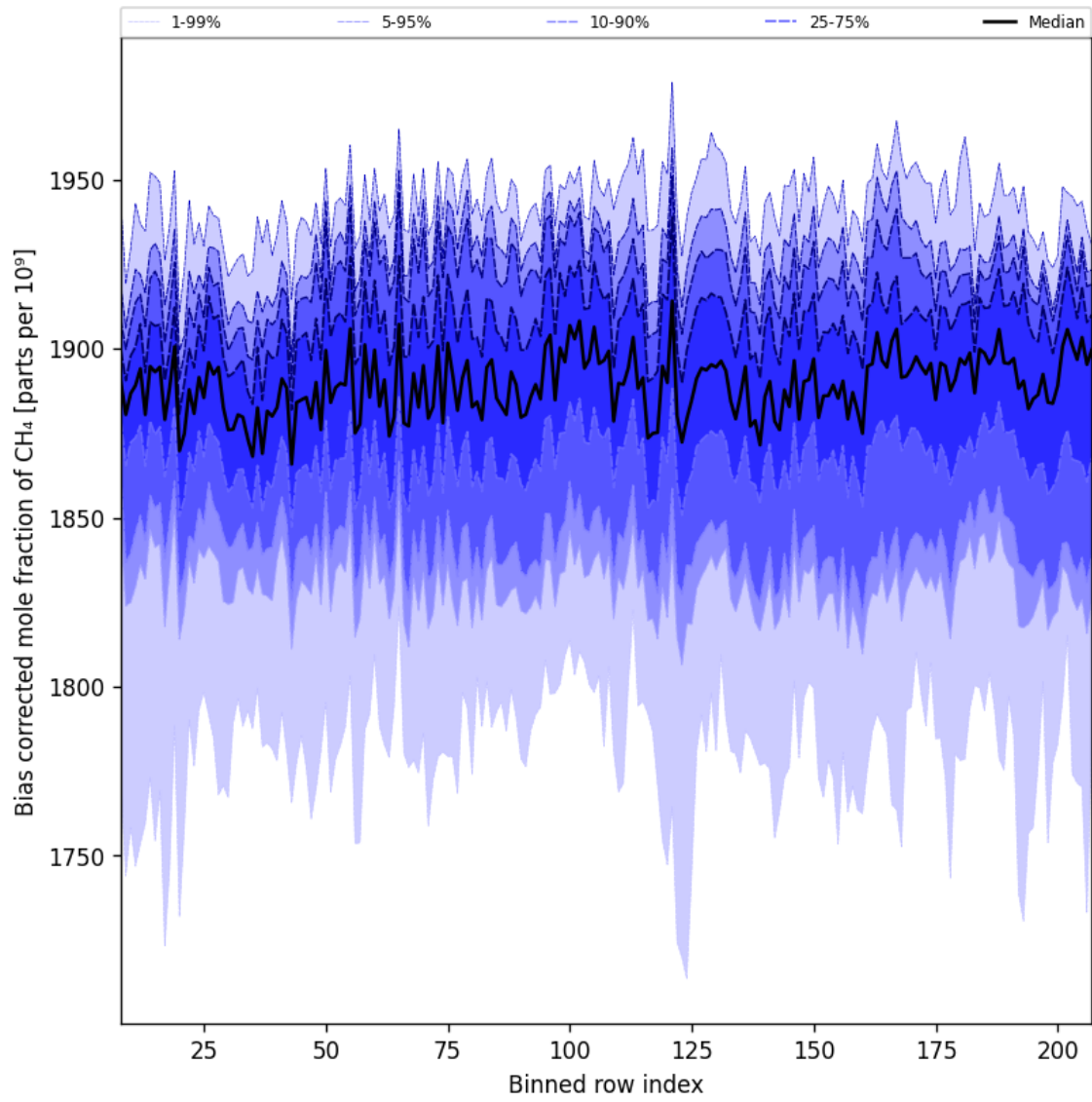
Figure 36: Along track statistics of “Bias corrected mole fraction of CH 4 ” for 2025-05-15 to 2025-05-16
