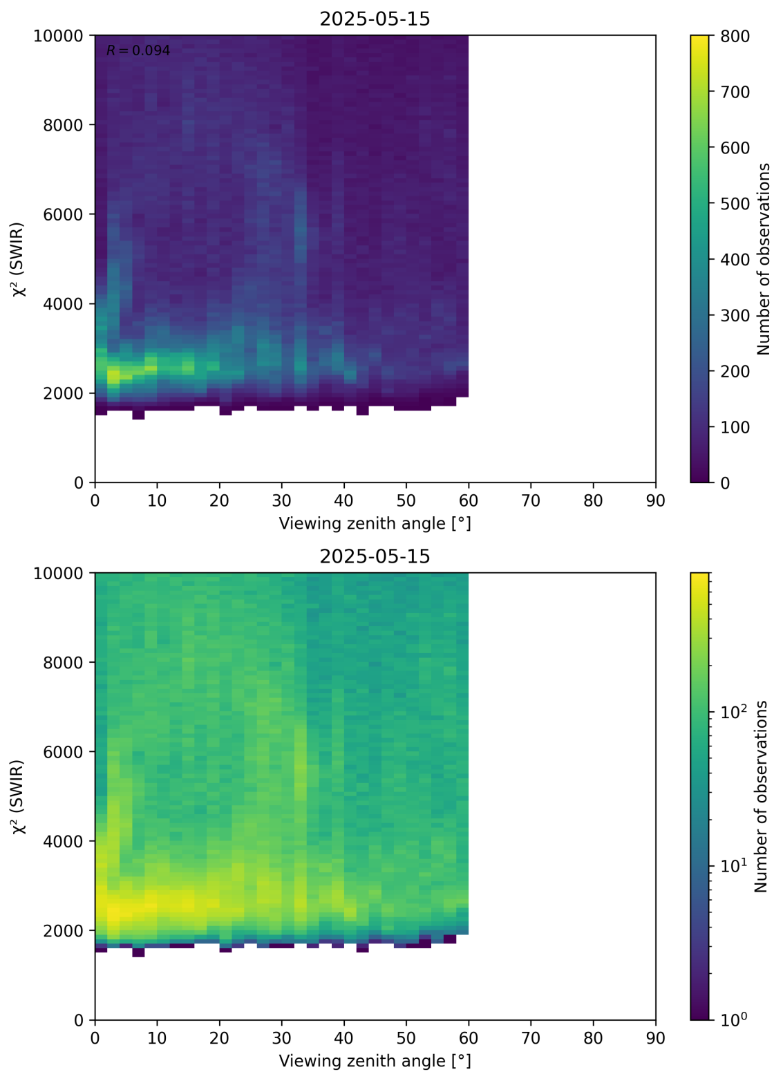
Figure 106: Scatter density plot of “Viewing zenith angle” against “ \chi^2 (SWIR)” for 2025-05-15 to 2025-05-16.
