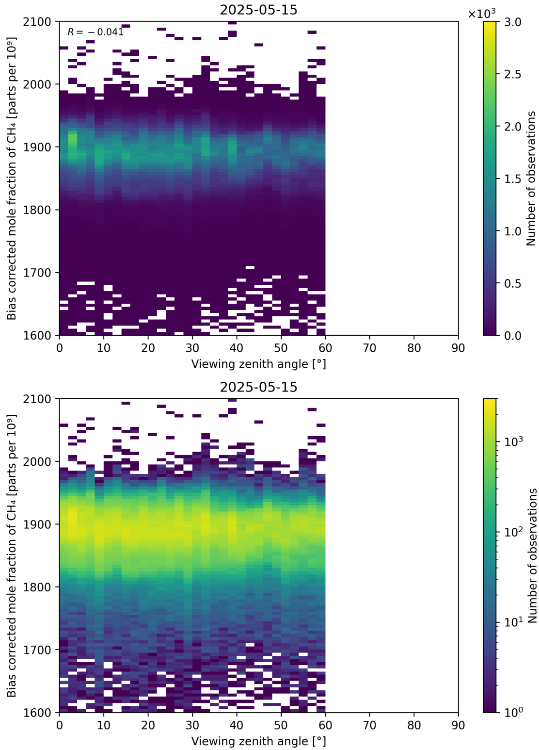
Figure 111: Scatter density plot of “Viewing zenith angle” against “Bias corrected mole fraction of CH 4 ” for 2025-05-15 to 2025-05-16.
