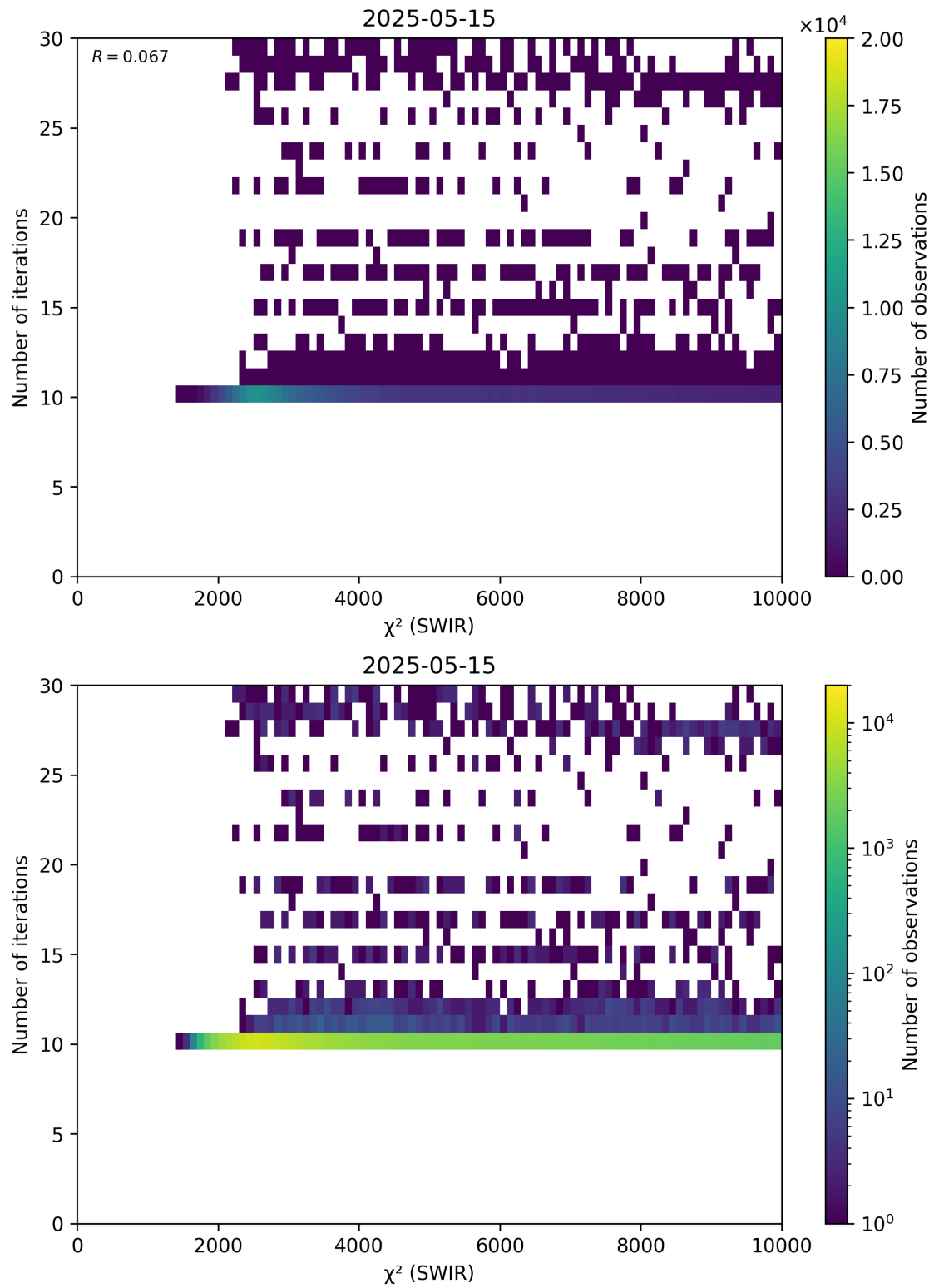
Figure 50: Scatter density plot of “ \chi^2 (SWIR)” against “Number of iterations” for 2025-05-15 to 2025-05-16.
