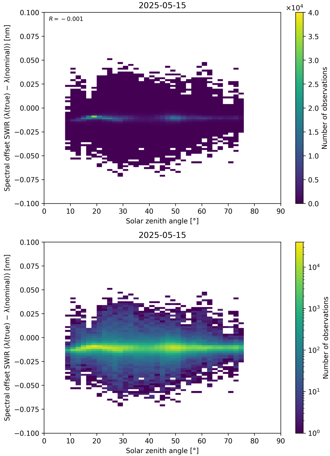
Figure 104: Scatter density plot of “Solar zenith angle” against “Spectral offset SWIR ( \lambda_{\text{true}} - \lambda_{\text{nominal}} )” for 2025-05-15 to 2025-05-16.
