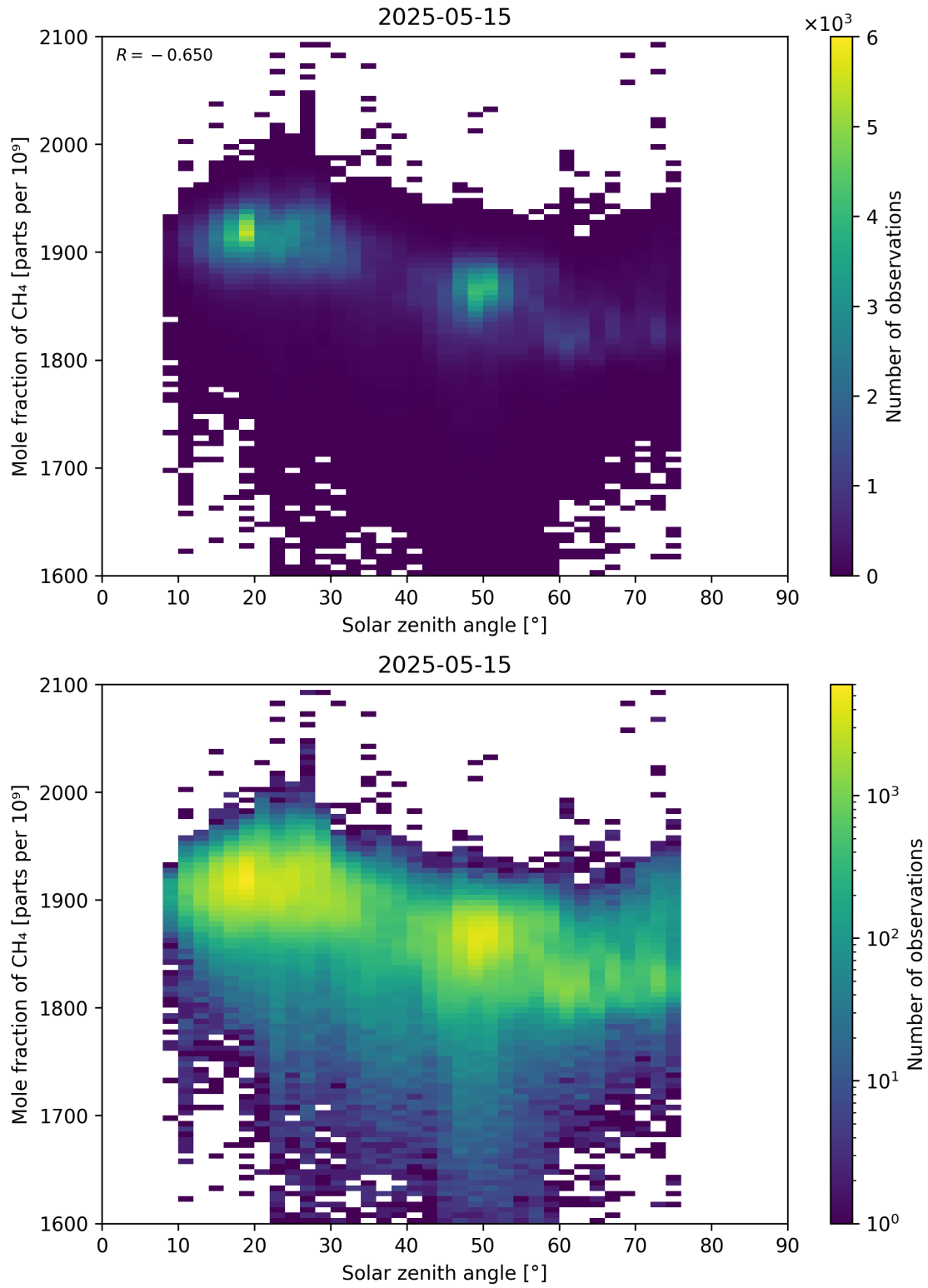
Figure 99: Scatter density plot of “Solar zenith angle” against “Mole fraction of CH 4 ” for 2025-05-15 to 2025-05-16.
