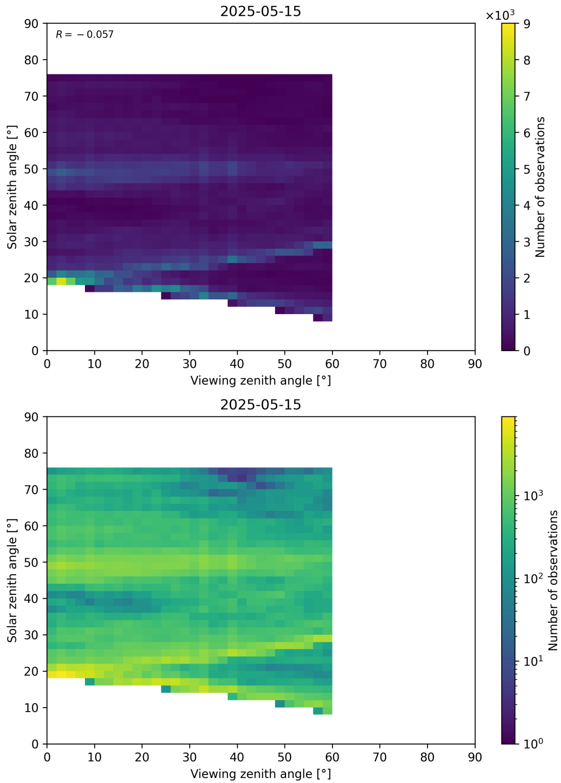
Figure 115: Scatter density plot of “Viewing zenith angle” against “Solar zenith angle” for 2025-05-15 to 2025-05-16.
