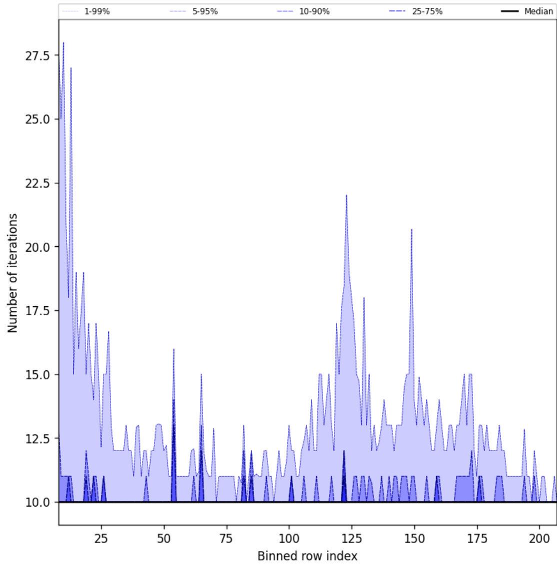
Figure 42: Along track statistics of “Number of iterations” for 2025-05-15 to 2025-05-16
