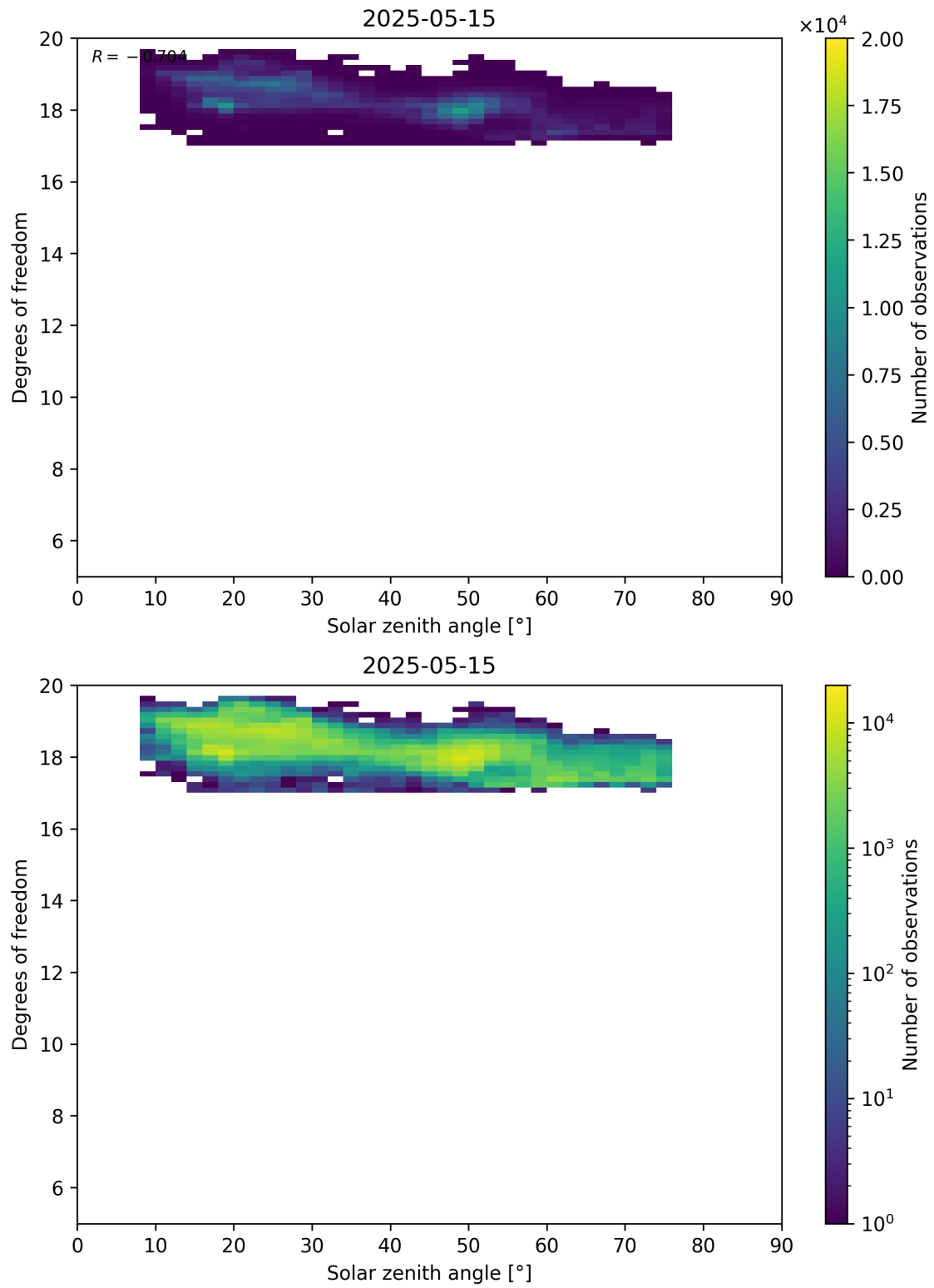
Figure 96: Scatter density plot of “Solar zenith angle” against “Degrees of freedom” for 2025-05-15 to 2025-05-16.
