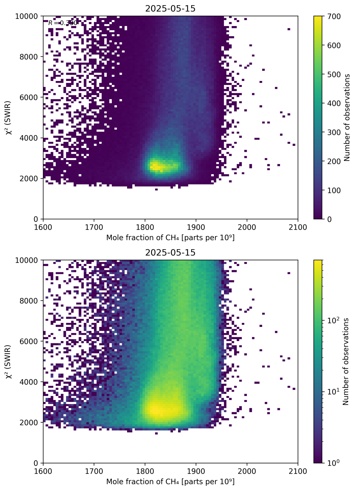
Figure 71: Scatter density plot of “Mole fraction of CH 4 ” against “ \chi^2 (SWIR)” for 2025-05-15 to 2025-05-16.
