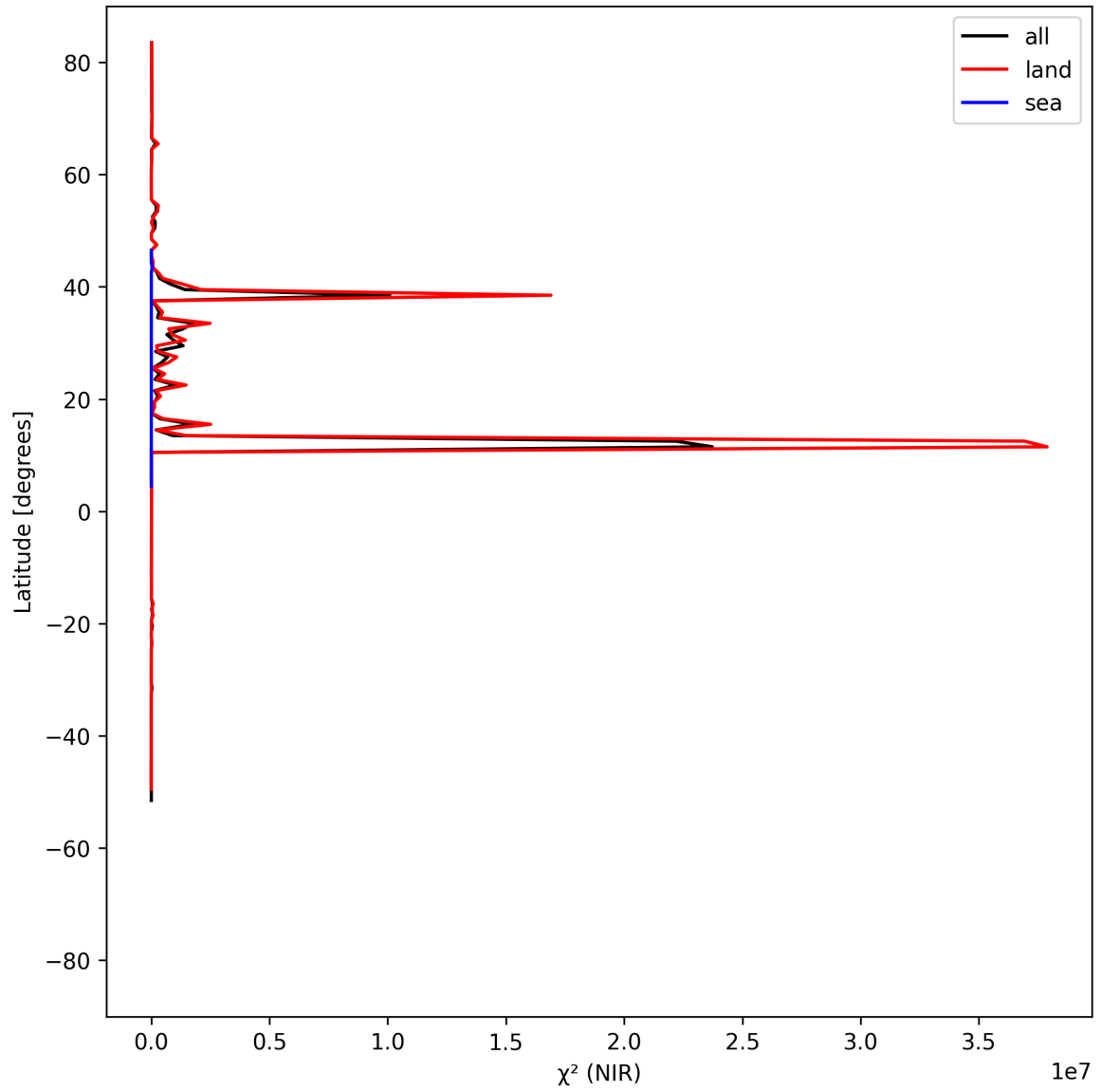
Figure 18: Zonal average of “ \chi^2 (NIR)” for 2025-05-15 to 2025-05-16.
