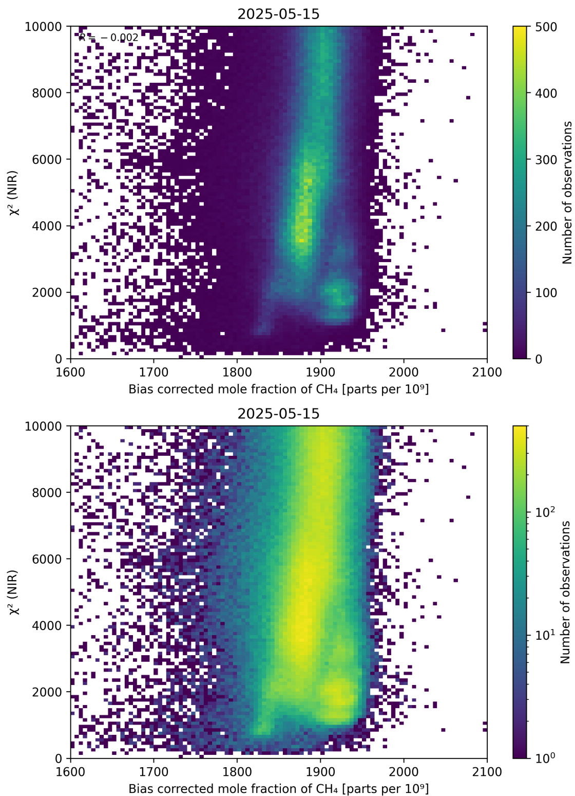
Figure 63: Scatter density plot of “Bias corrected mole fraction of CH 4 ” against “ \chi^2 (NIR)” for 2025-05-15 to 2025-05-16.
