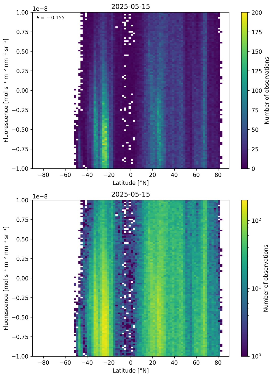
Figure 56: Scatter density plot of “Latitude” against “Fluorescence” for 2025-05-15 to 2025-05-16.
