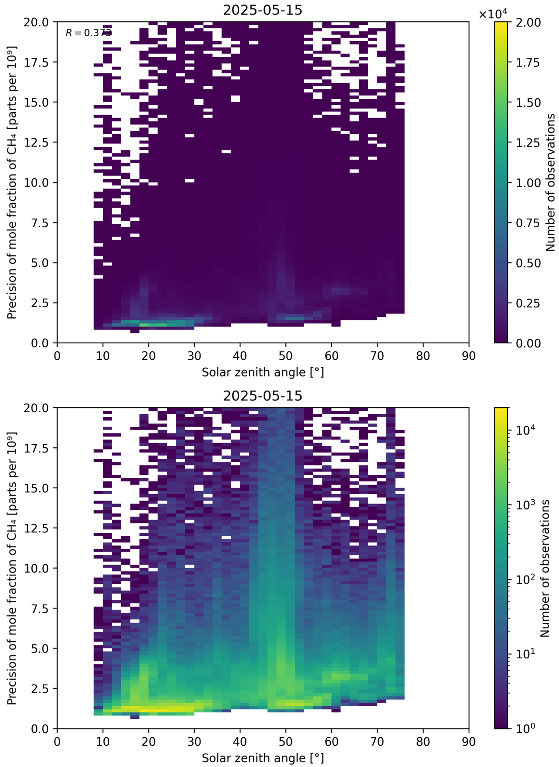
Figure 101: Scatter density plot of “Solar zenith angle” against “Precision of mole fraction of CH 4 ” for 2025-05-15 to 2025-05-16.
