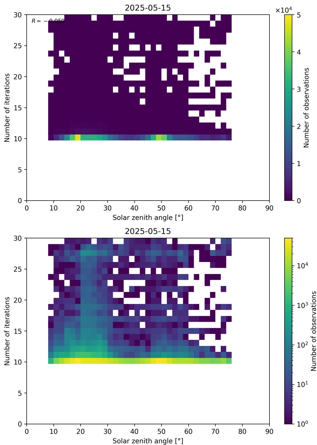
Figure 102: Scatter density plot of “Solar zenith angle” against “Number of iterations” for 2025-05-15 to 2025-05-16.
