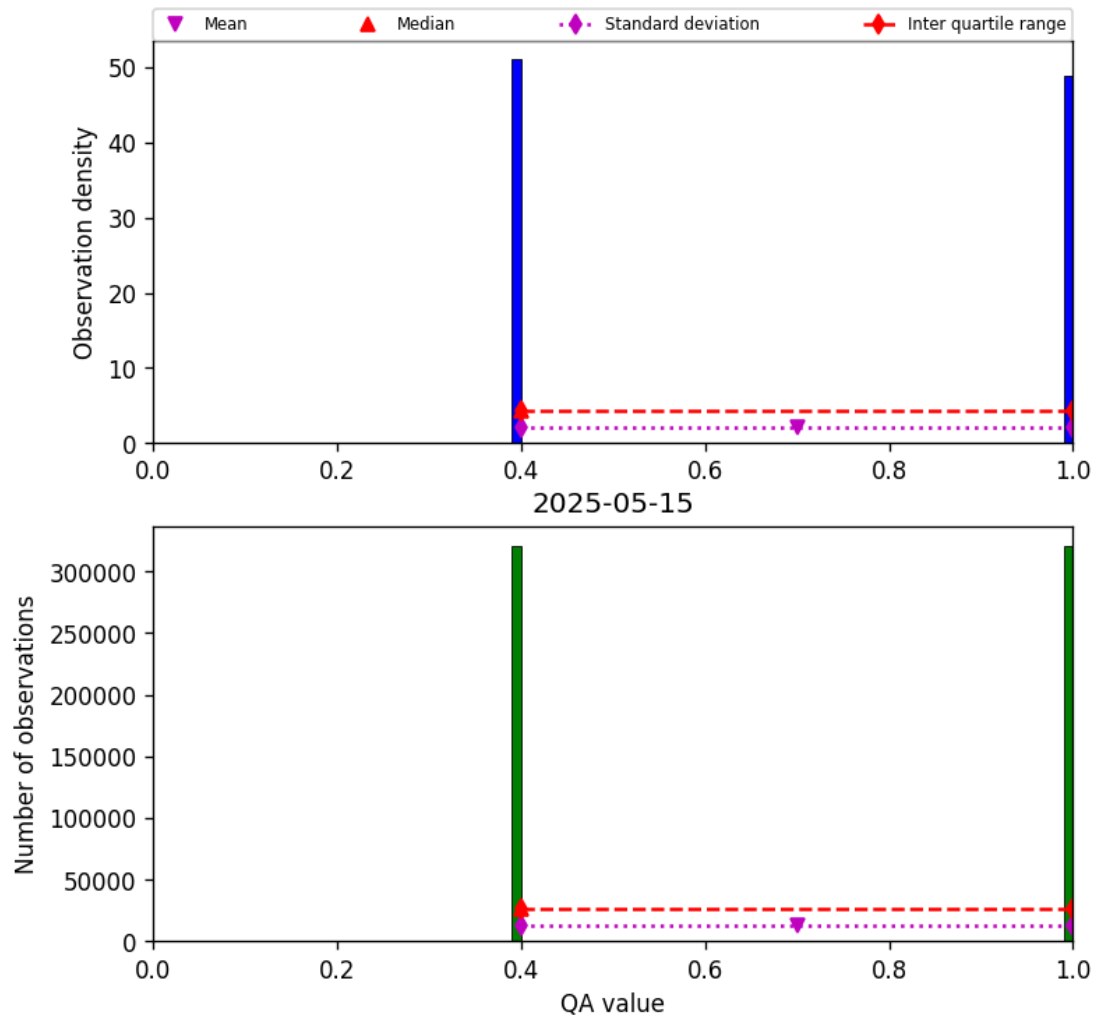
Figure 22: Histogram of “QA value” for 2025-05-15 to 2025-05-16
