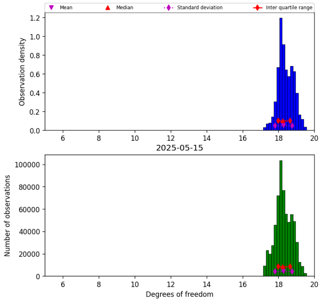
Figure 30: Histogram of “Degrees of freedom” for 2025-05-15 to 2025-05-16
