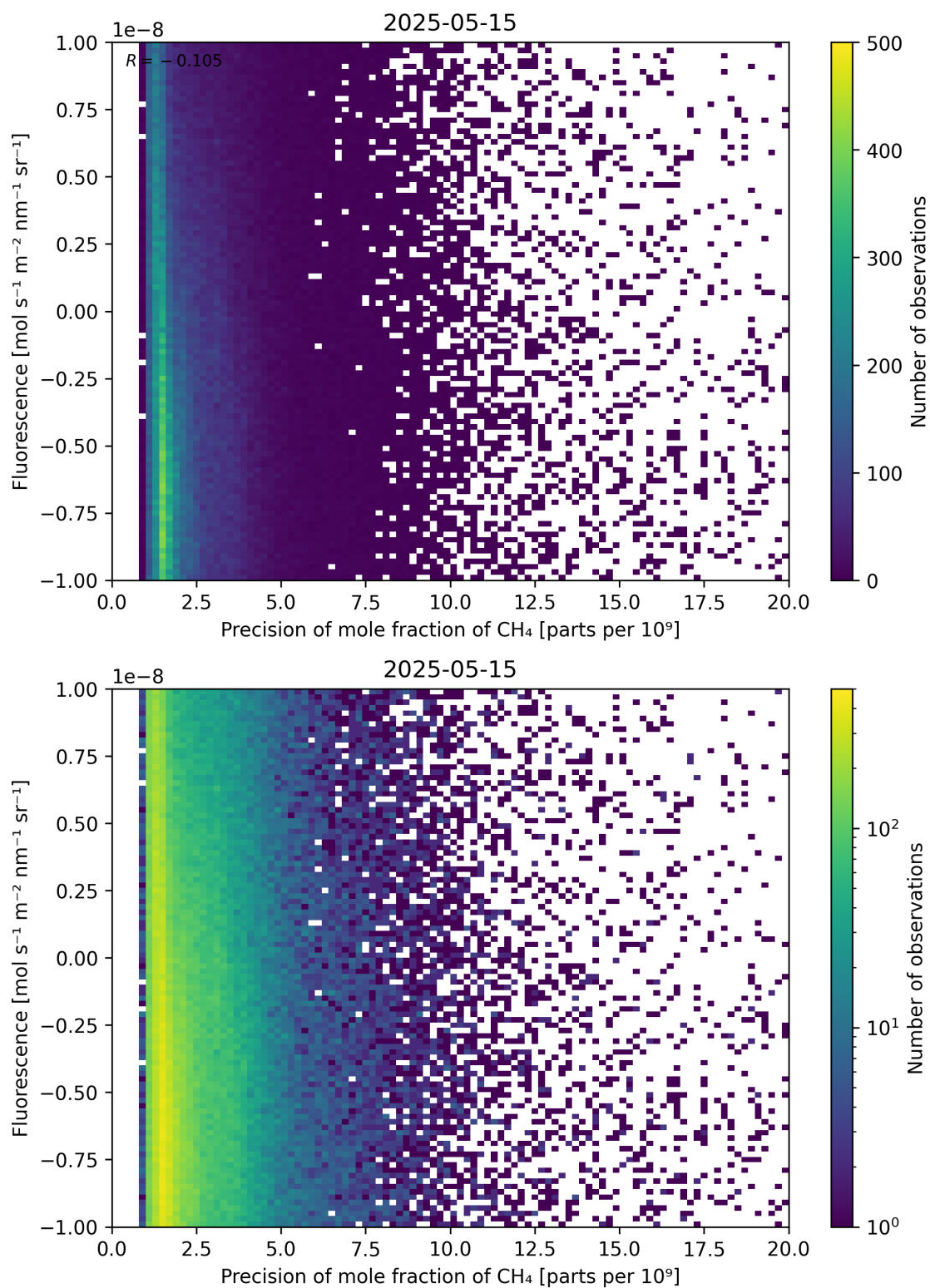
Figure 81: Scatter density plot of “Precision of mole fraction of CH 4 ” against “Fluorescence” for 2025-05-15 to 2025-05-16.
