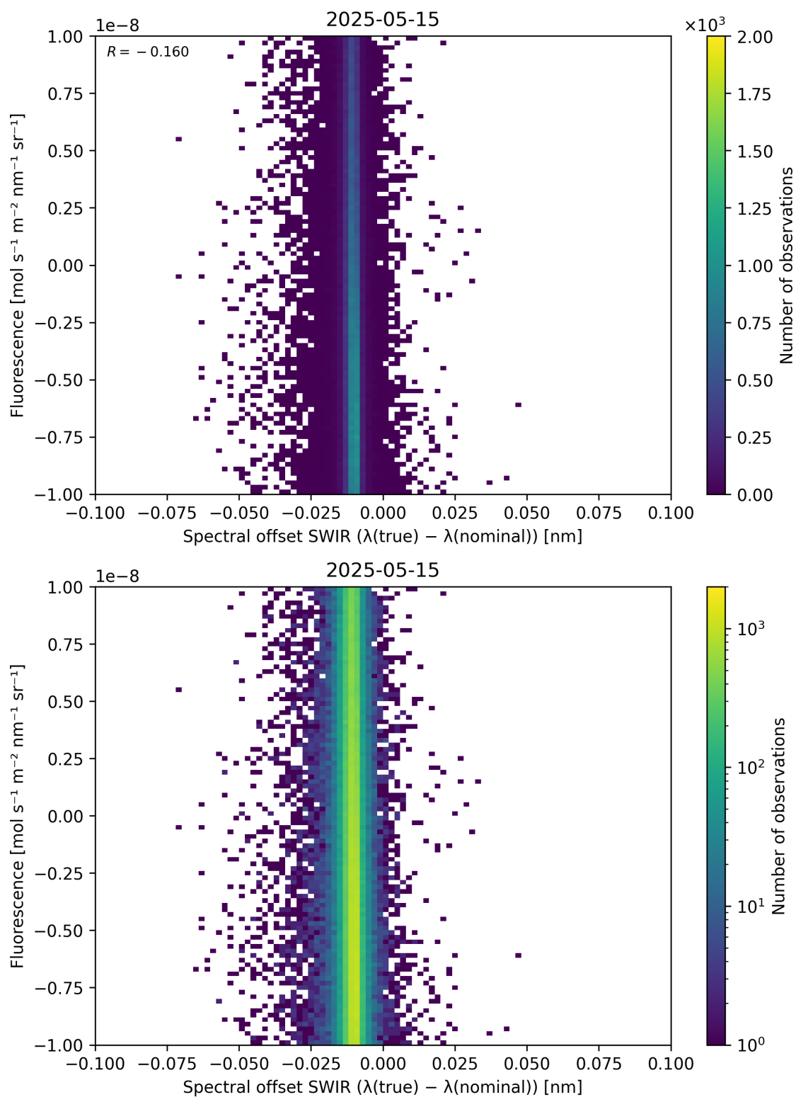
Figure 120: Scatter density plot of “Spectral offset SWIR ( \lambda_{\text{true}} - \lambda_{\text{nominal}} )” against “Fluorescence” for 2025-05-15 to 2025-05-16.
