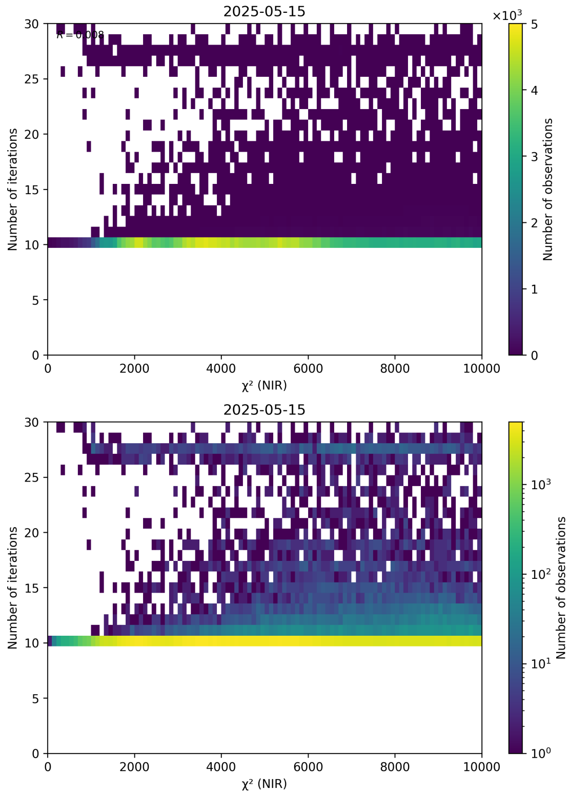
Figure 46: Scatter density plot of “ \chi^2 (NIR)” against “Number of iterations” for 2025-05-15 to 2025-05-16.
