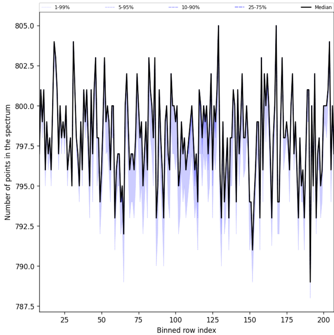
Figure 37: Along track statistics of “Number of points in the spectrum” for 2025-05-15 to 2025-05-16
