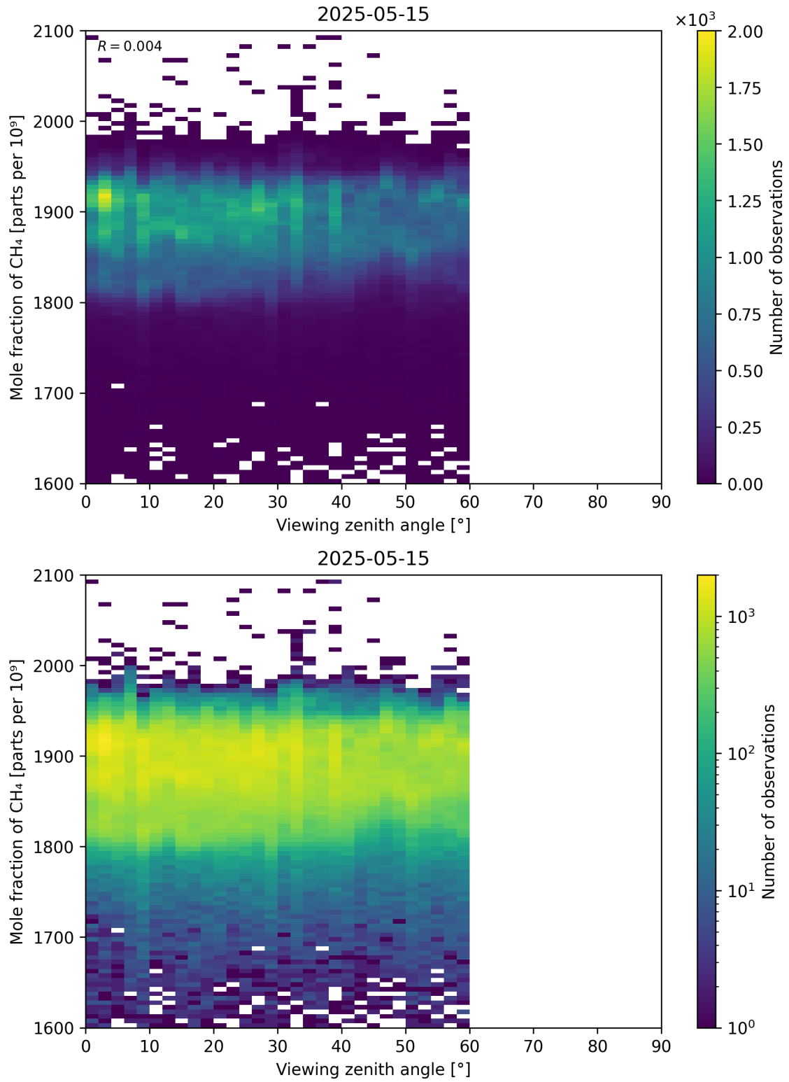
Figure 110: Scatter density plot of “Viewing zenith angle” against “Mole fraction of CH 4 ” for 2025-05-15 to 2025-05-16.
