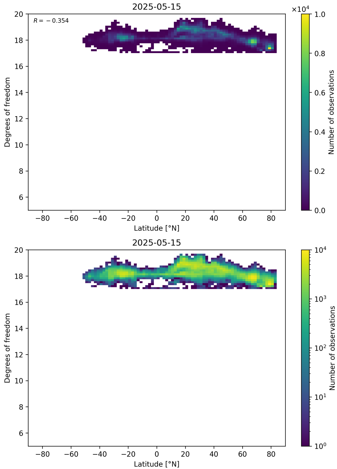
Figure 55: Scatter density plot of “Latitude” against “Degrees of freedom” for 2025-05-15 to 2025-05-16.
