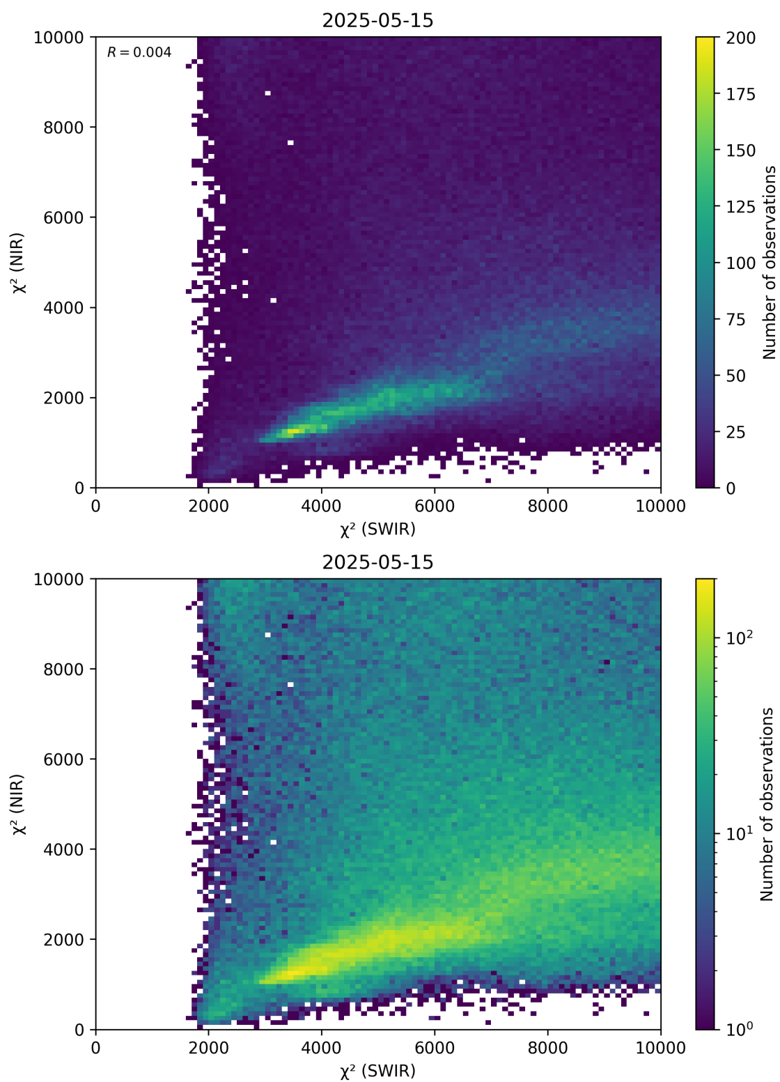
Figure 47: Scatter density plot of “ \chi^2 (SWIR)” against “ \chi^2 (NIR)” for 2025-05-15 to 2025-05-16.
