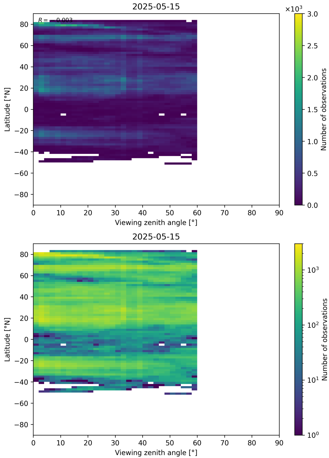
Figure 109: Scatter density plot of “Viewing zenith angle” against “Latitude” for 2025-05-15 to 2025-05-16.
