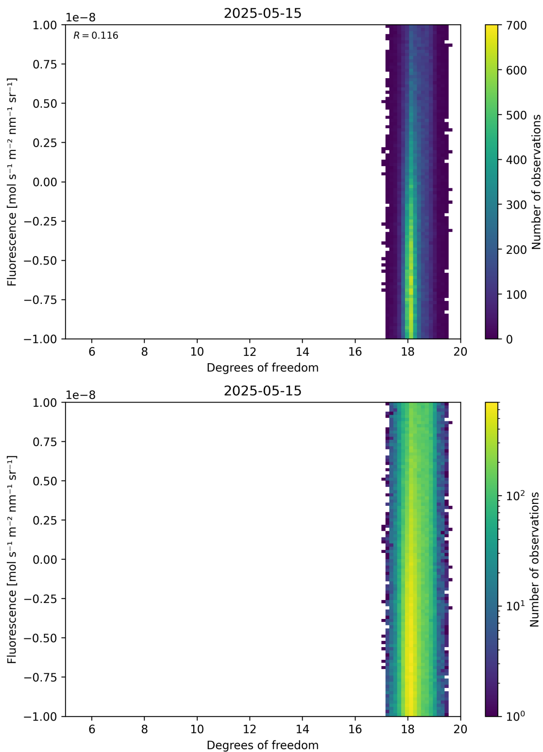
Figure 51: Scatter density plot of “Degrees of freedom” against “Fluorescence” for 2025-05-15 to 2025-05-16.
