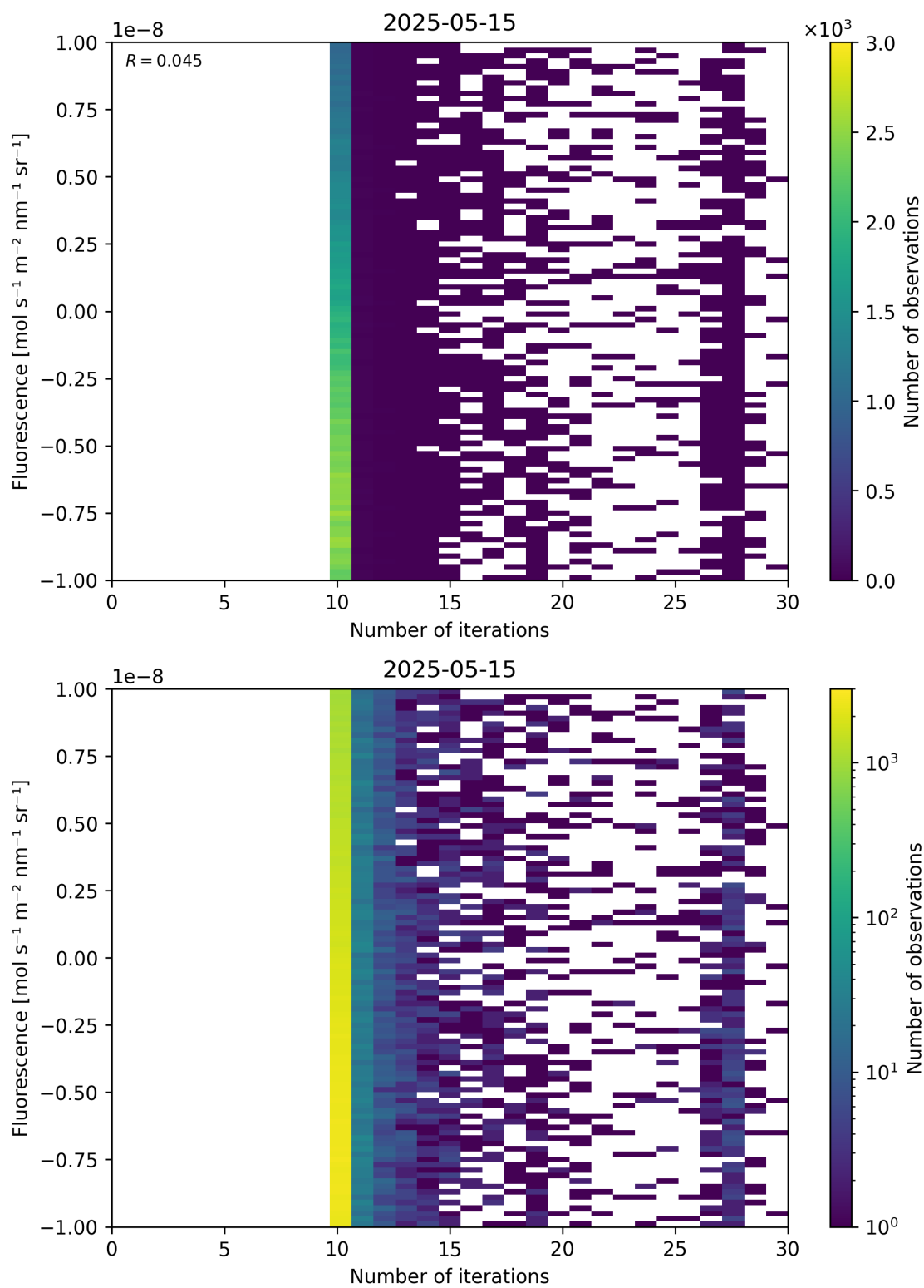
Figure 87: Scatter density plot of “Number of iterations” against “Fluorescence” for 2025-05-15 to 2025-05-16.
