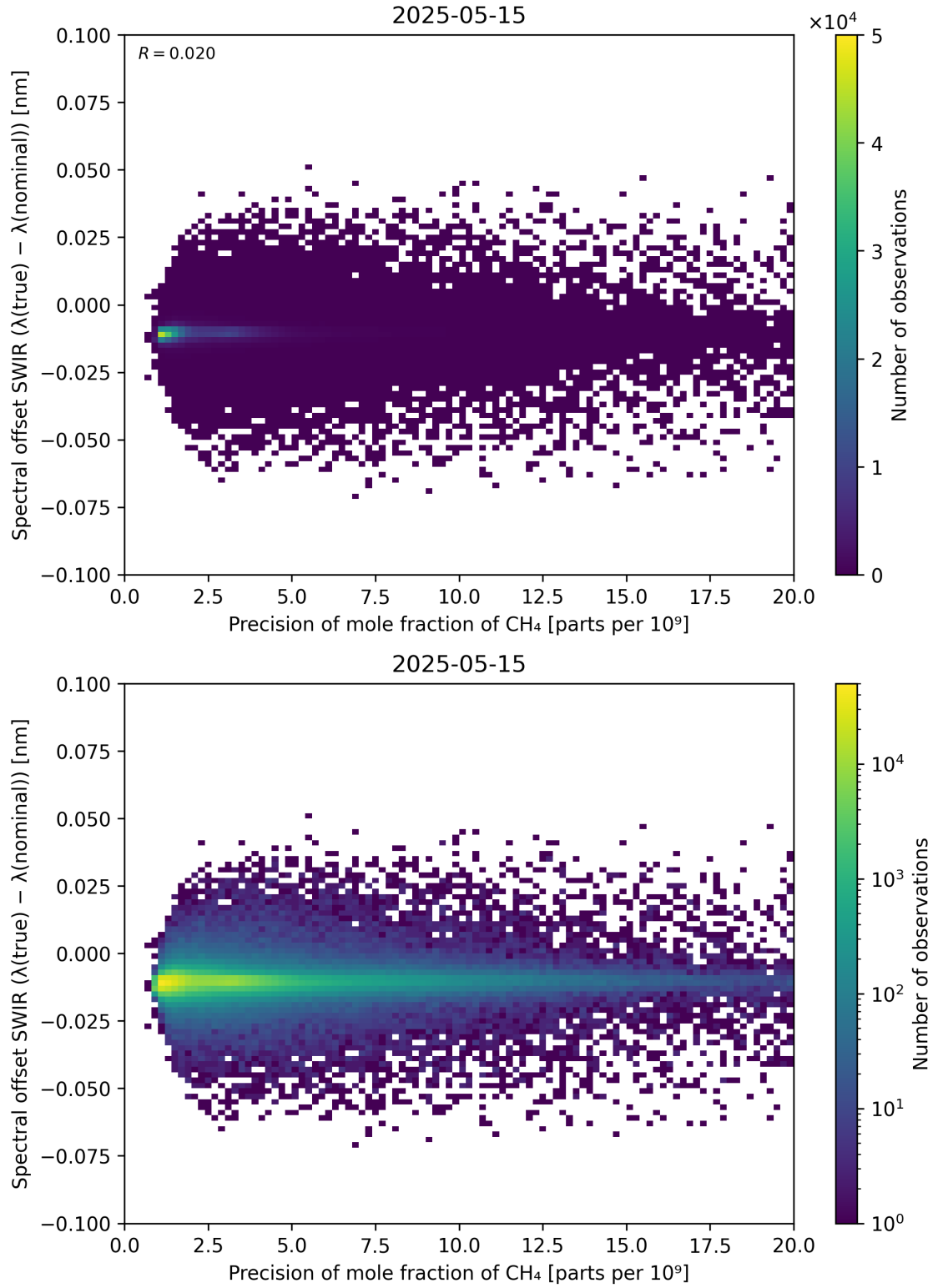
Figure 85: Scatter density plot of “Precision of mole fraction of CH 4 ” against “Spectral offset SWIR ( \lambda_{\text{true}} - \lambda_{\text{nominal}} )” for 2025-05-15 to 2025-05-16.
