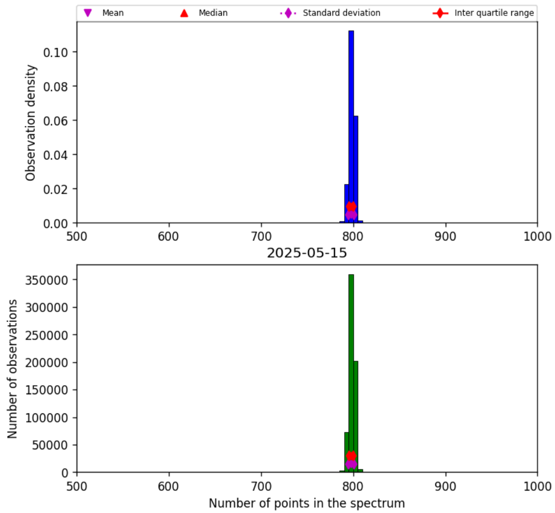
Figure 26: Histogram of “Number of points in the spectrum” for 2025-05-15 to 2025-05-16
