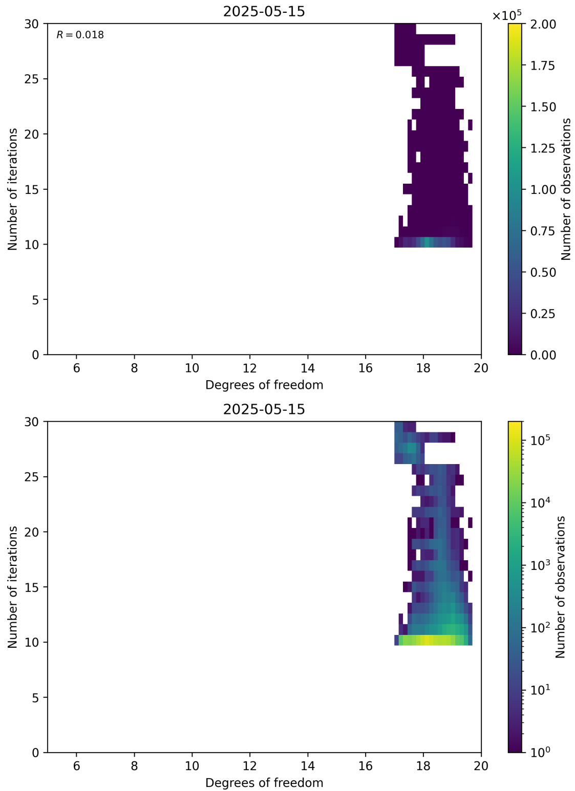
Figure 52: Scatter density plot of “Degrees of freedom” against “Number of iterations” for 2025-05-15 to 2025-05-16.
