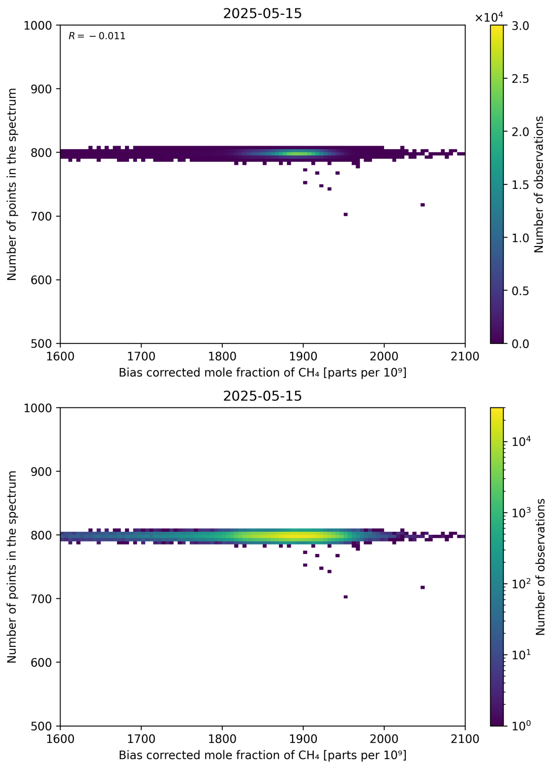
Figure 68: Scatter density plot of “Bias corrected mole fraction of CH 4 ” against “Number of points in the spectrum” for 2025-05-15 to 2025-05-16.
