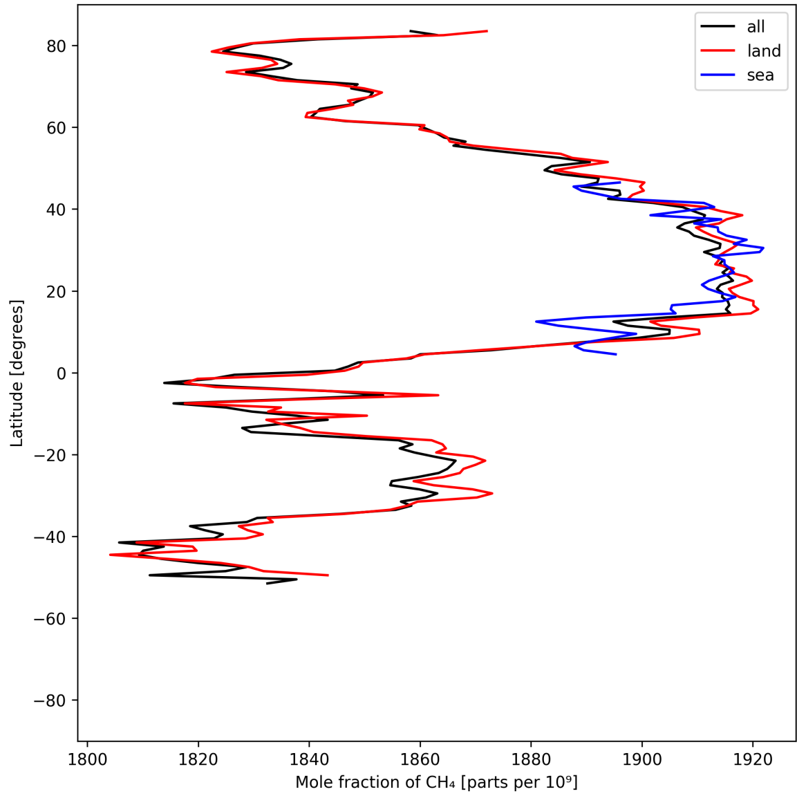
Figure 12: Zonal average of “Mole fraction of \text{CH}_4 ” for 2025-05-15 to 2025-05-16.
