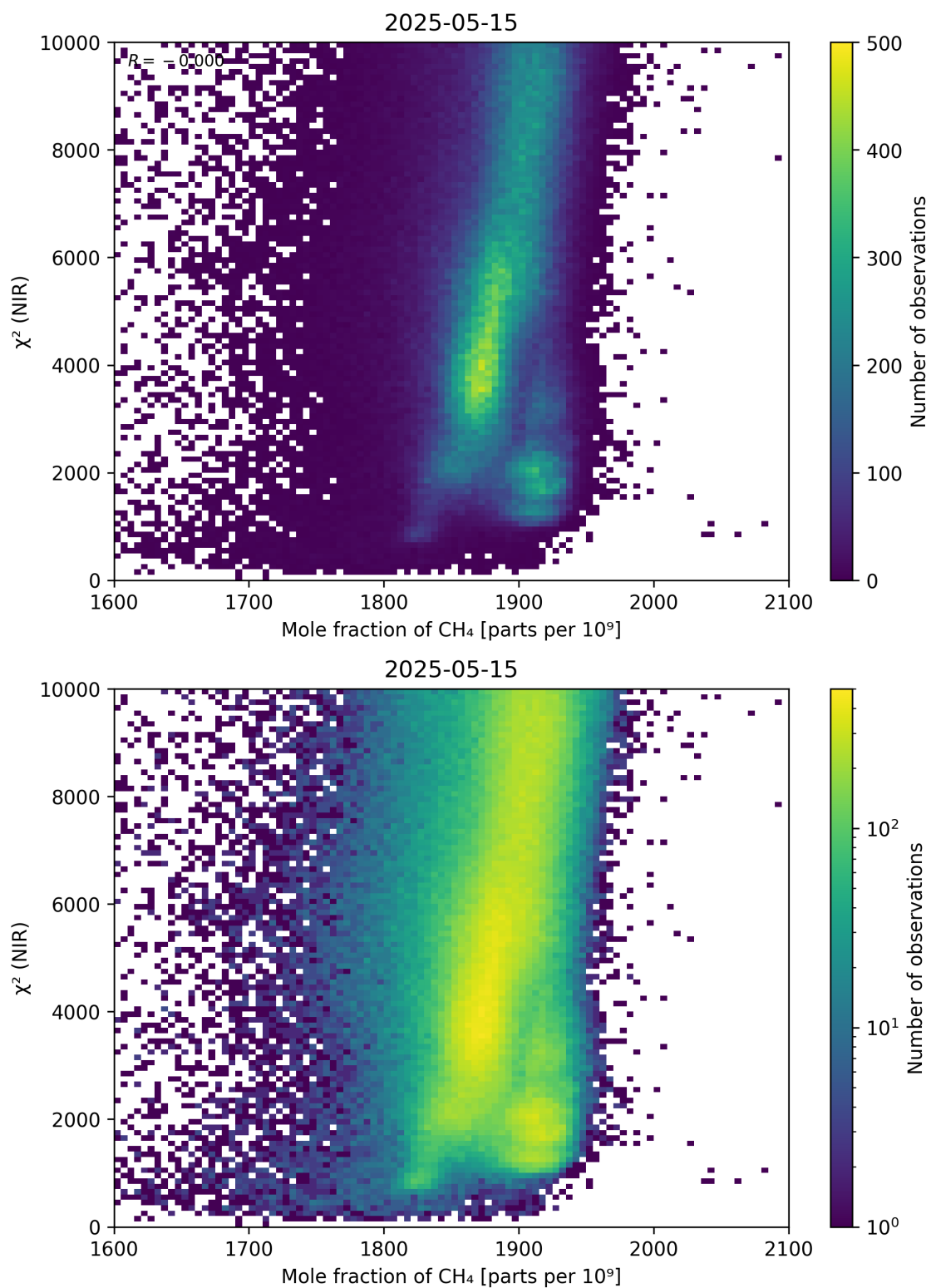
Figure 70: Scatter density plot of “Mole fraction of \text{CH}_4 ” against “ \chi^2 (NIR)” for 2025-05-15 to 2025-05-16.
