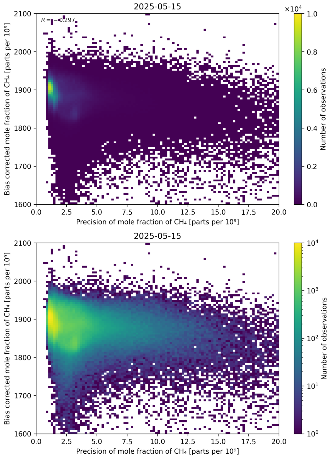
Figure 82: Scatter density plot of “Precision of mole fraction of CH 4 ” against “Bias corrected mole fraction of CH 4 ” for 2025-05-15 to 2025-05-16.
