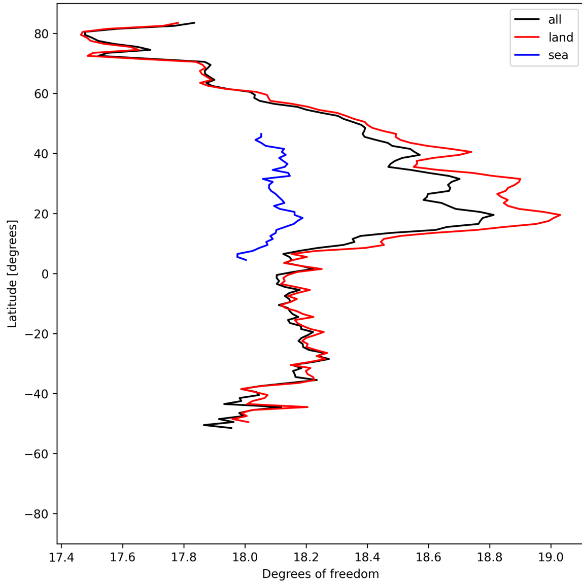
Figure 19: Zonal average of “Degrees of freedom” for 2025-05-15 to 2025-05-16.
