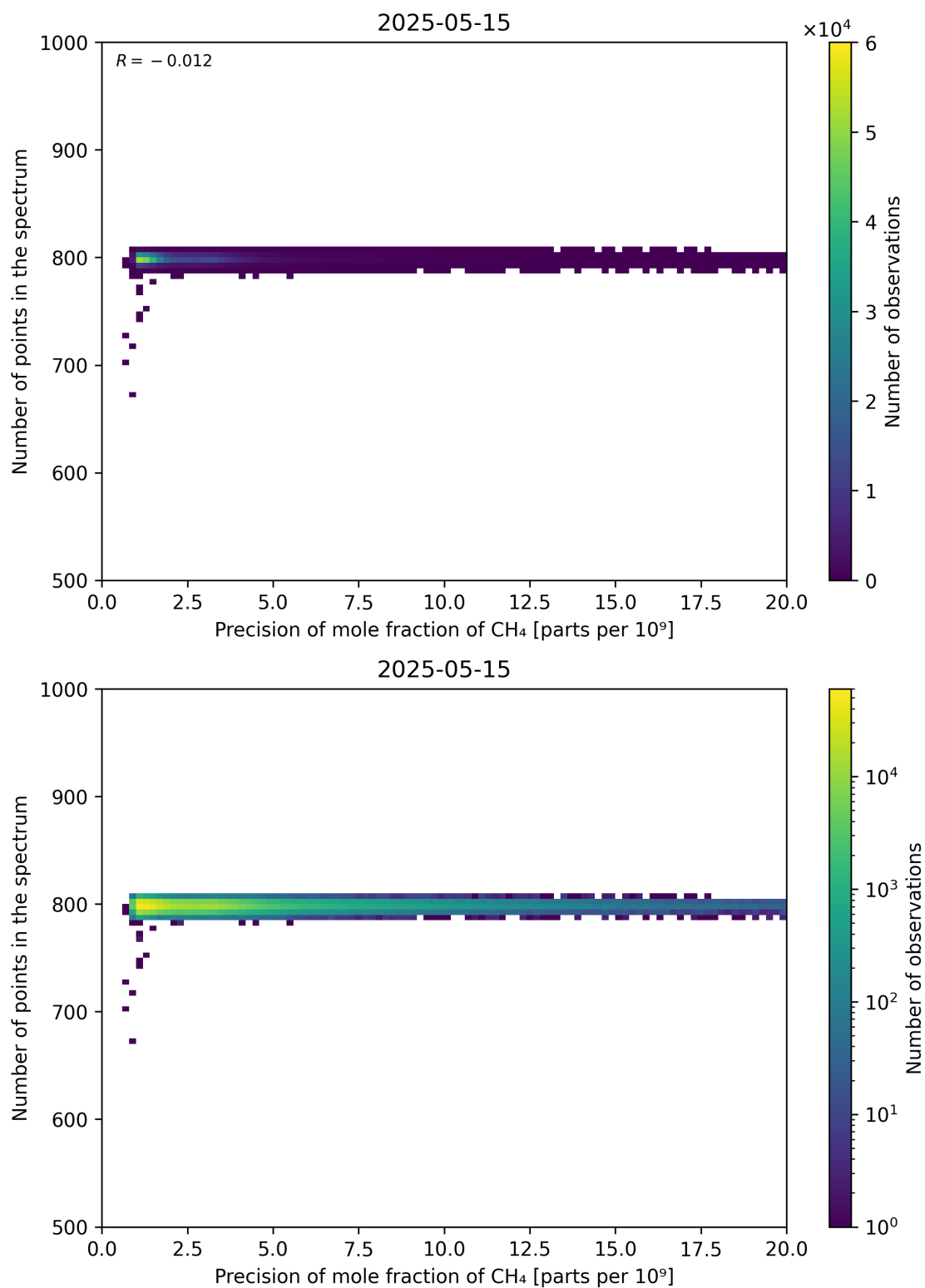
Figure 84: Scatter density plot of “Precision of mole fraction of CH 4 ” against “Number of points in the spectrum” for 2025-05-15 to 2025-05-16.
