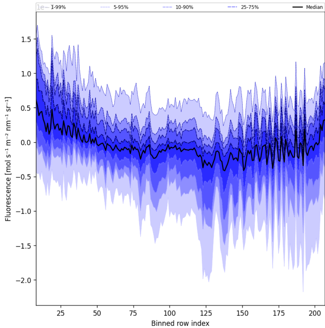
Figure 43: Along track statistics of “Fluorescence” for 2025-05-15 to 2025-05-16
