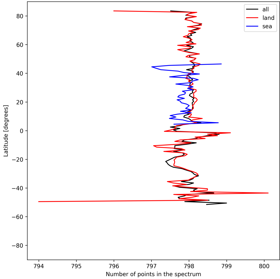
Figure 15: Zonal average of “Number of points in the spectrum” for 2025-05-15 to 2025-05-16.
