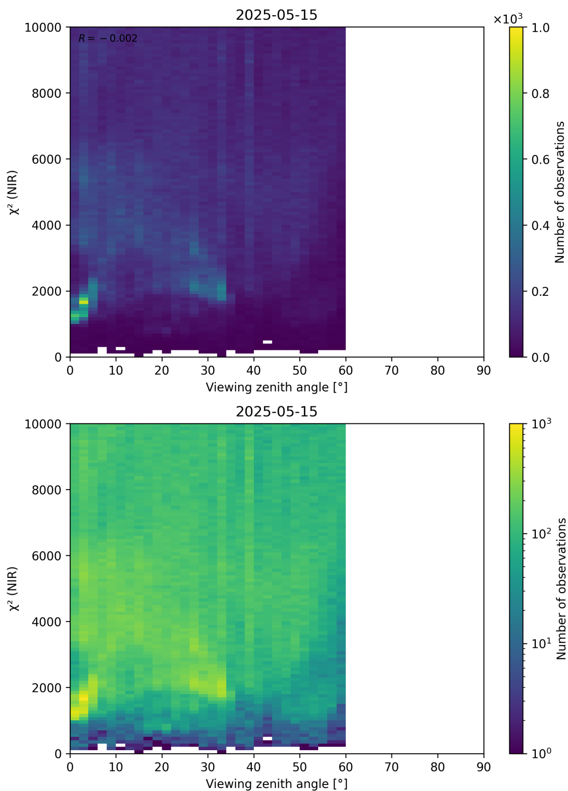
Figure 105: Scatter density plot of “Viewing zenith angle” against “ \chi^2 (NIR)” for 2025-05-15 to 2025-05-16.
