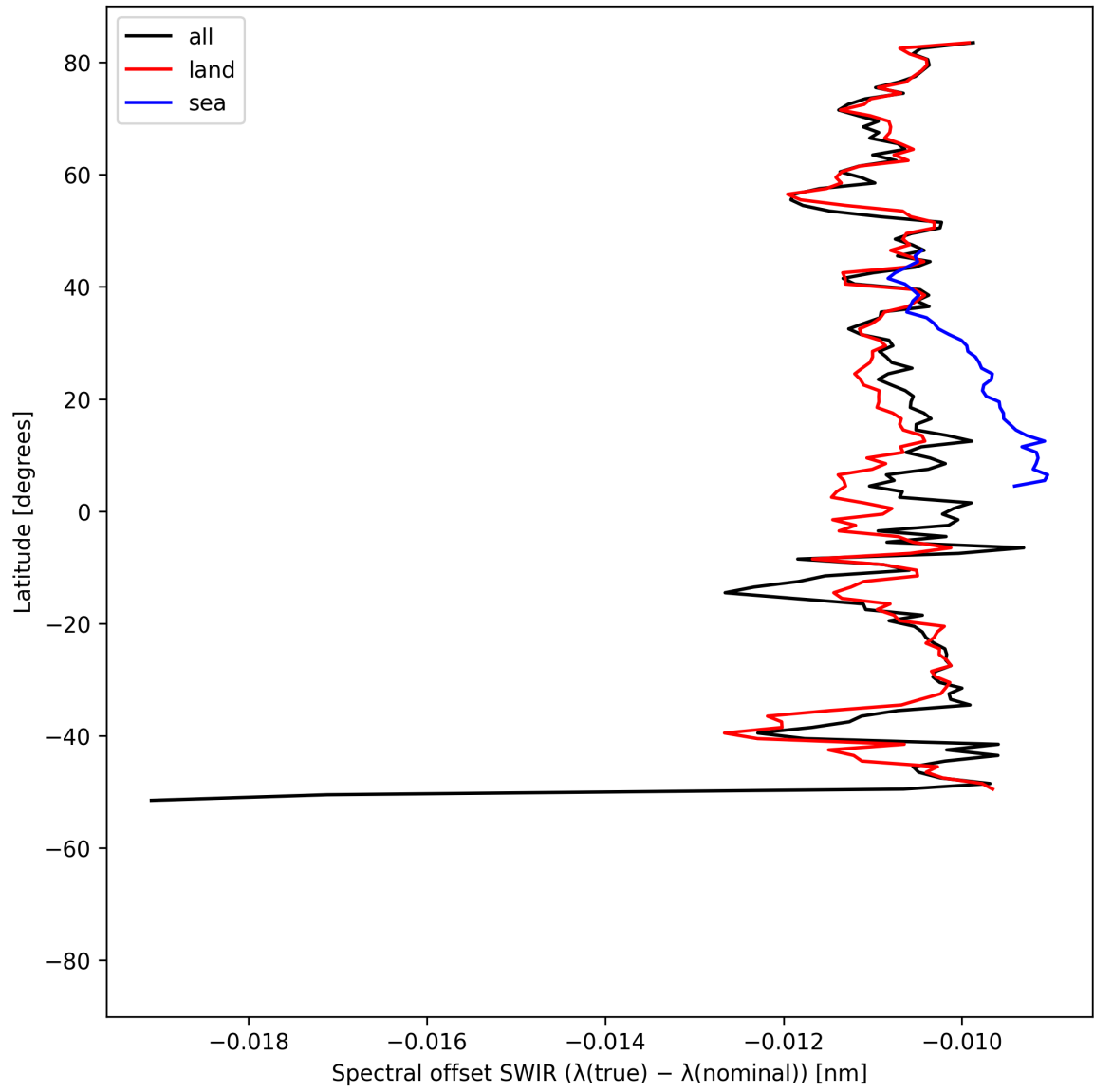
Figure 16: Zonal average of “Spectral offset SWIR ( \lambda_{\text{true}} - \lambda_{\text{nominal}} )” for 2025-05-15 to 2025-05-16.
