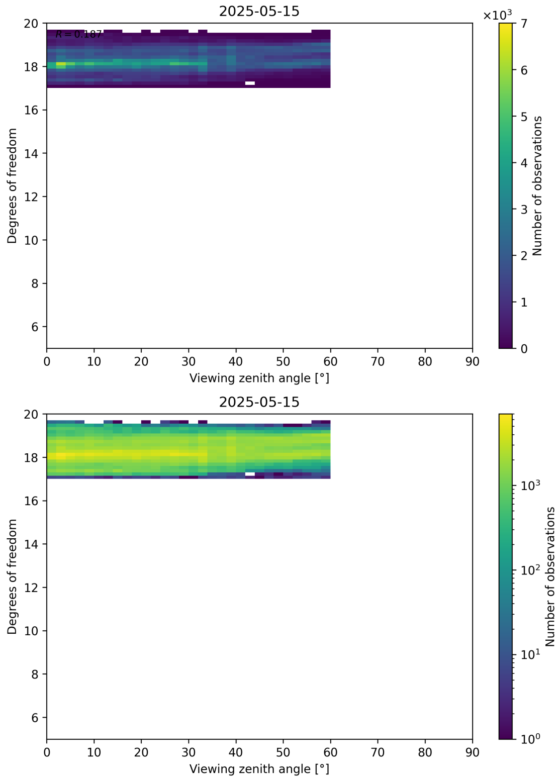
Figure 107: Scatter density plot of “Viewing zenith angle” against “Degrees of freedom” for 2025-05-15 to 2025-05-16.
