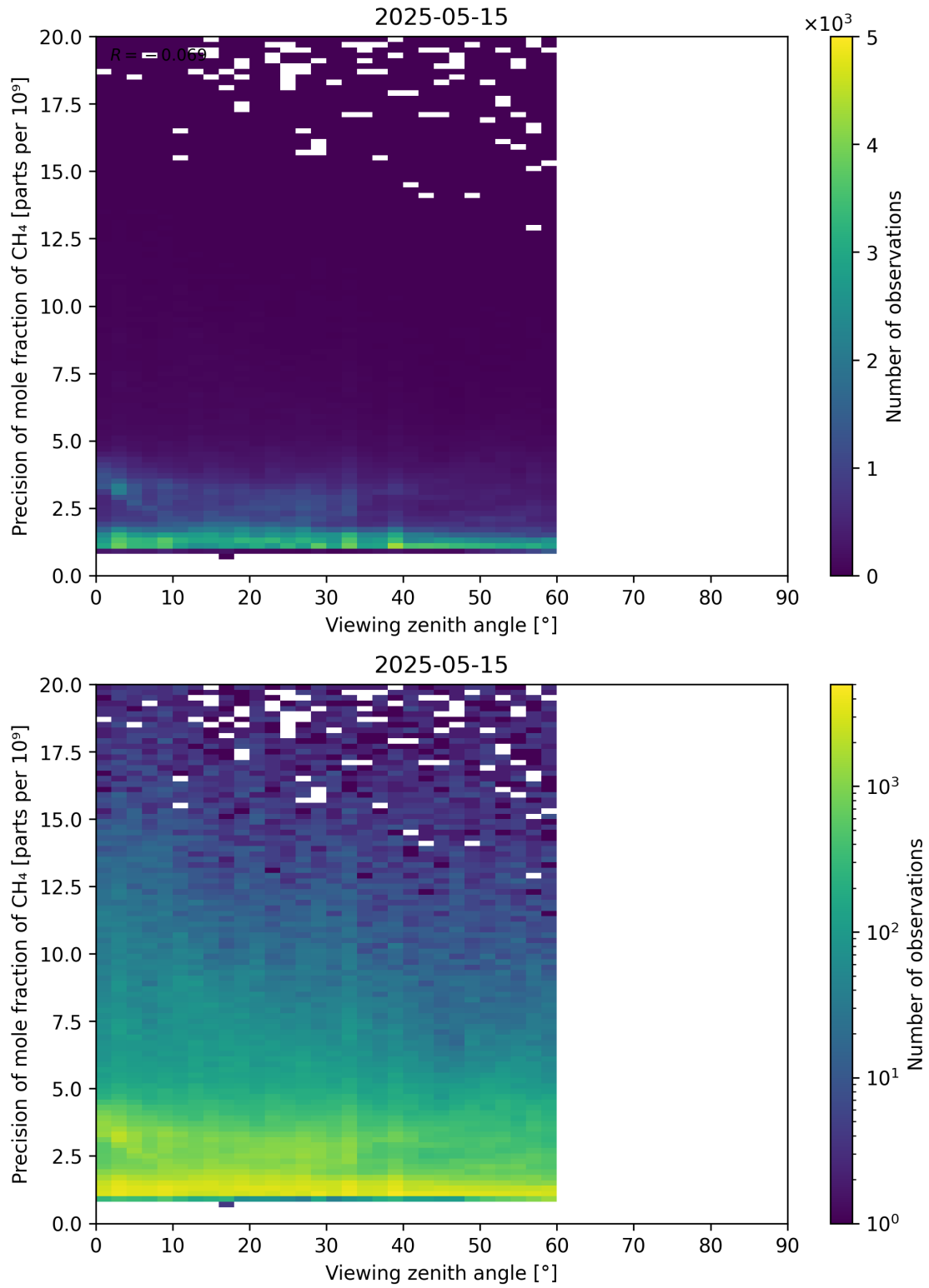
Figure 112: Scatter density plot of “Viewing zenith angle” against “Precision of mole fraction of CH 4 ” for 2025-05-15 to 2025-05-16.
