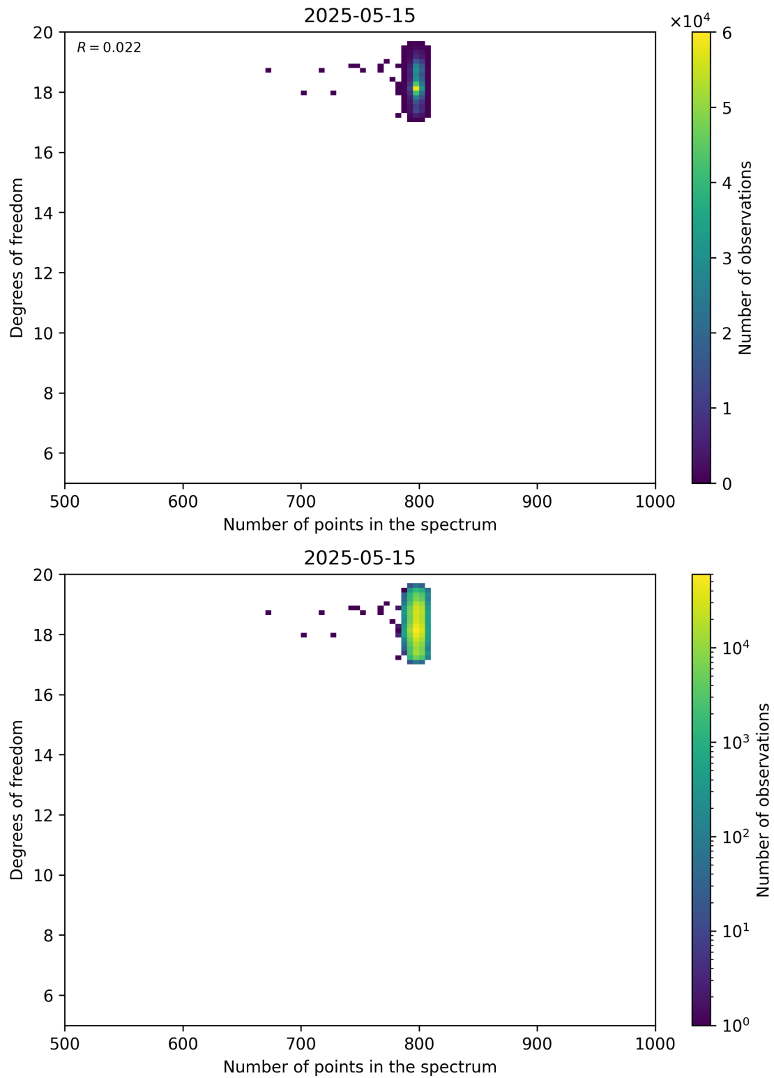
Figure 90: Scatter density plot of “Number of points in the spectrum” against “Degrees of freedom” for 2025-05-15 to 2025-05-16.
