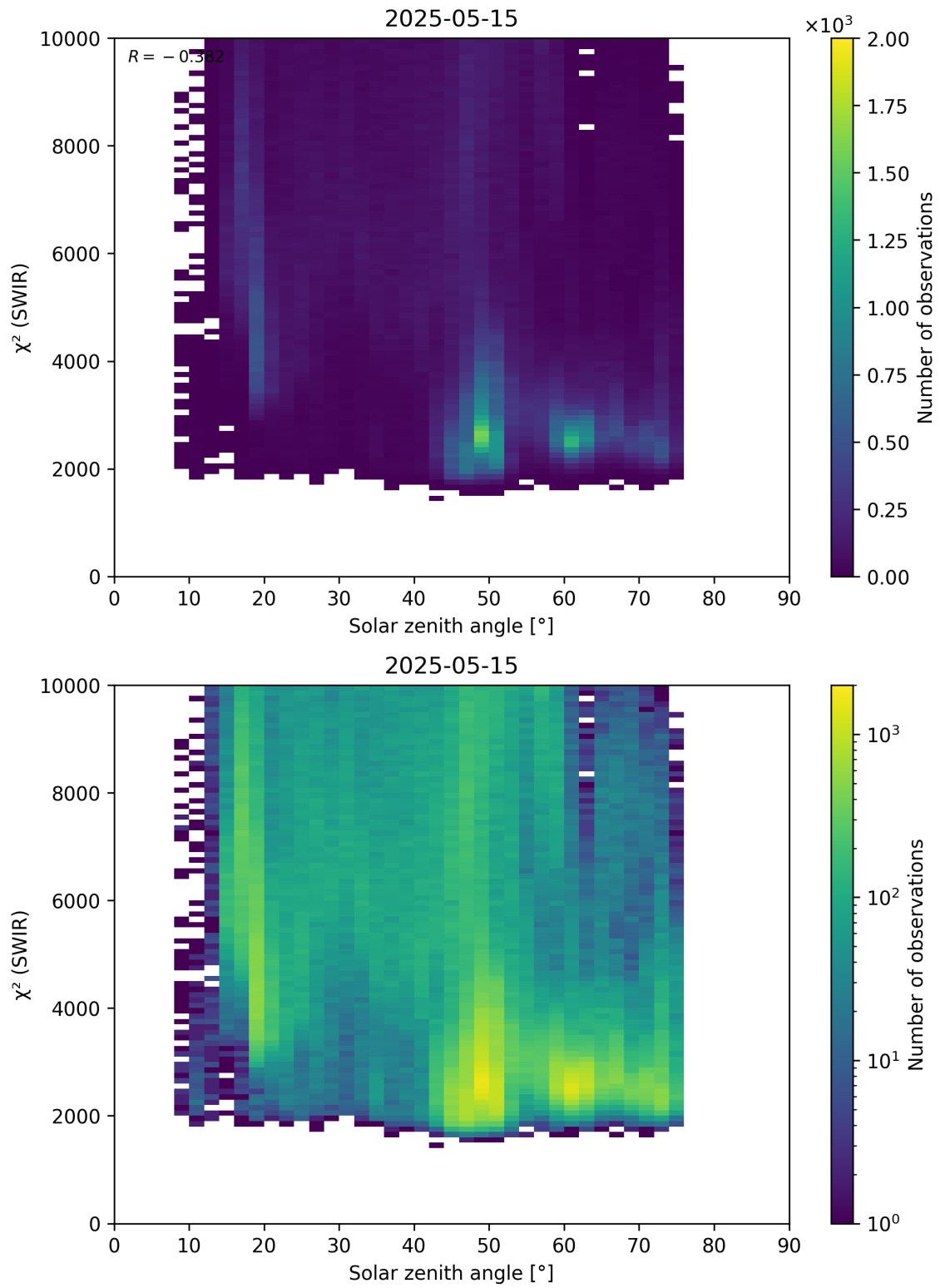
Figure 95: Scatter density plot of “Solar zenith angle” against “ \chi^2 (SWIR)” for 2025-05-15 to 2025-05-16.
