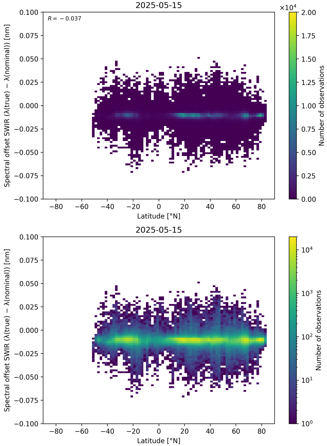
Figure 62: Scatter density plot of “Latitude” against “Spectral offset SWIR ( \lambda_{\text{true}} - \lambda_{\text{nominal}} )” for 2025-05-15 to 2025-05-16.
