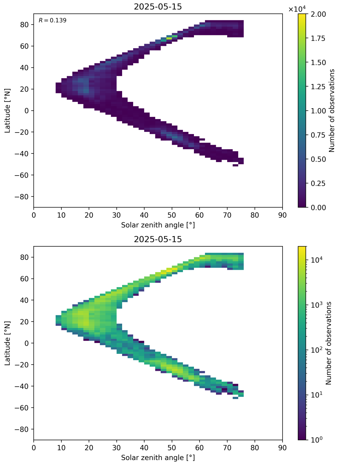
Figure 98: Scatter density plot of “Solar zenith angle” against “Latitude” for 2025-05-15 to 2025-05-16.
