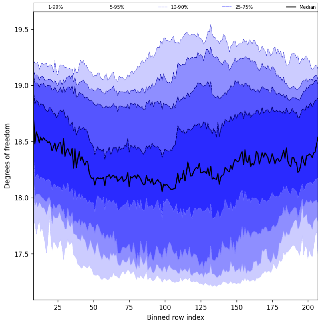
Figure 41: Along track statistics of “Degrees of freedom” for 2025-05-15 to 2025-05-16
