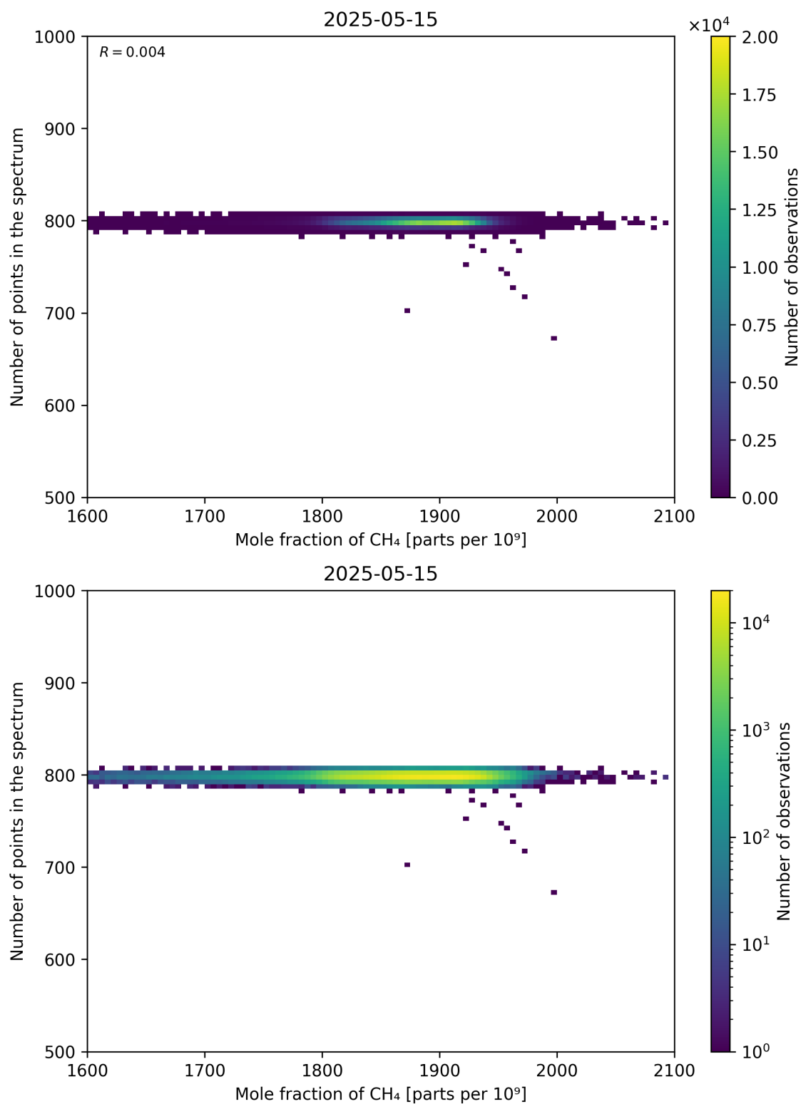
Figure 77: Scatter density plot of “Mole fraction of CH 4 ” against “Number of points in the spectrum” for 2025-05-15 to 2025-05-16.
