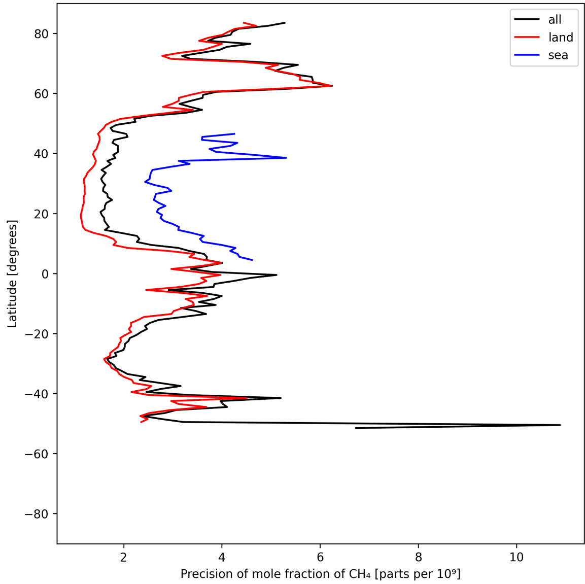
Figure 13: Zonal average of “Precision of mole fraction of CH 4 ” for 2025-05-15 to 2025-05-16.
