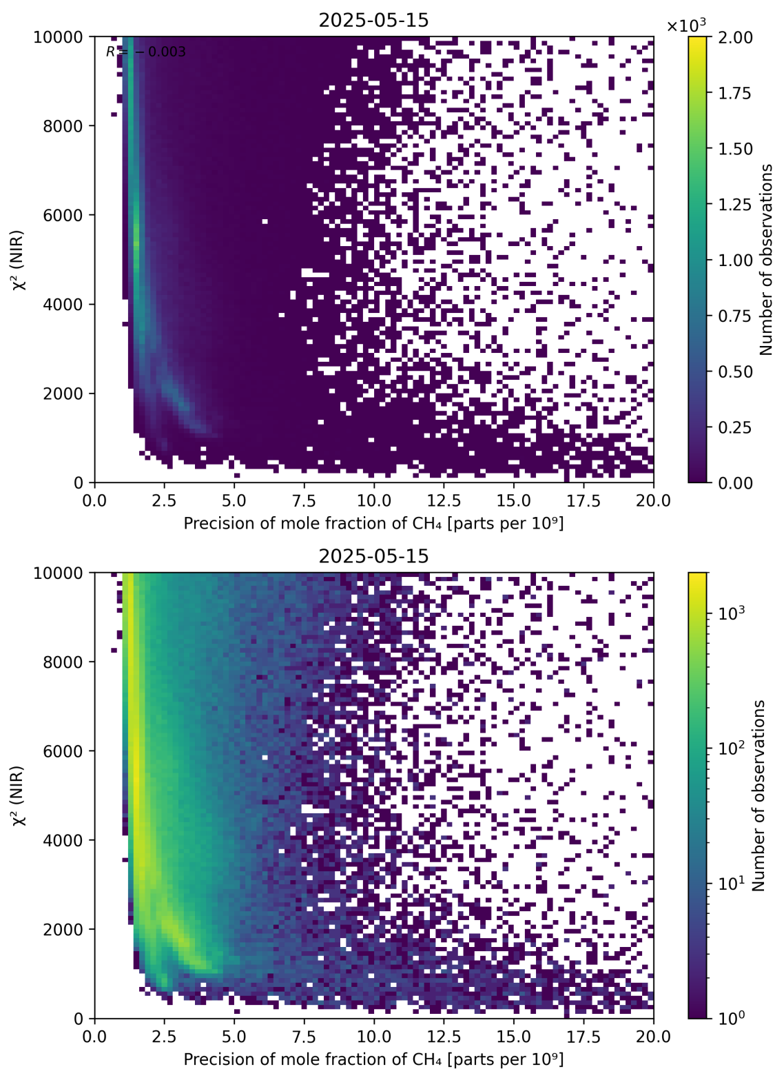
Figure 78: Scatter density plot of “Precision of mole fraction of CH 4 ” against “ \chi^2 (NIR)” for 2025-05-15 to 2025-05-16.
