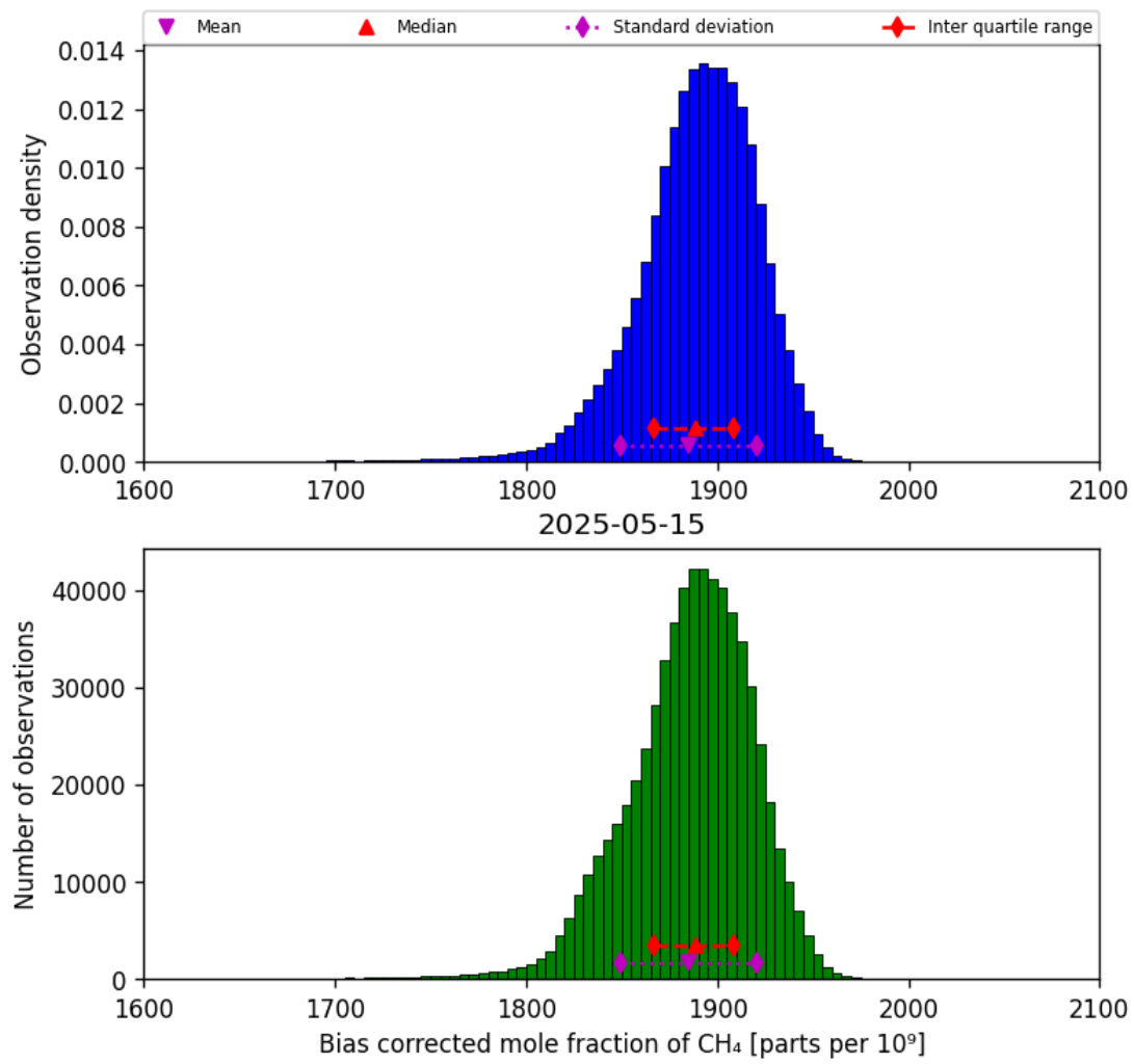
Figure 25: Histogram of “Bias corrected mole fraction of CH 4 ” for 2025-05-15 to 2025-05-16
