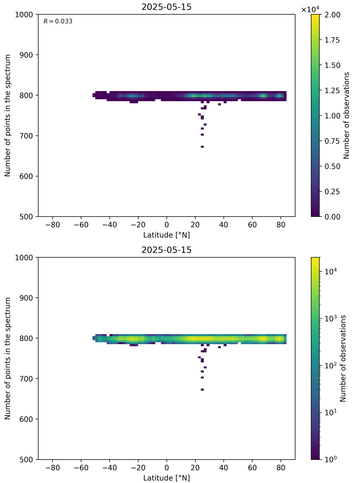
Figure 61: Scatter density plot of “Latitude” against “Number of points in the spectrum” for 2025-05-15 to 2025-05-16.
