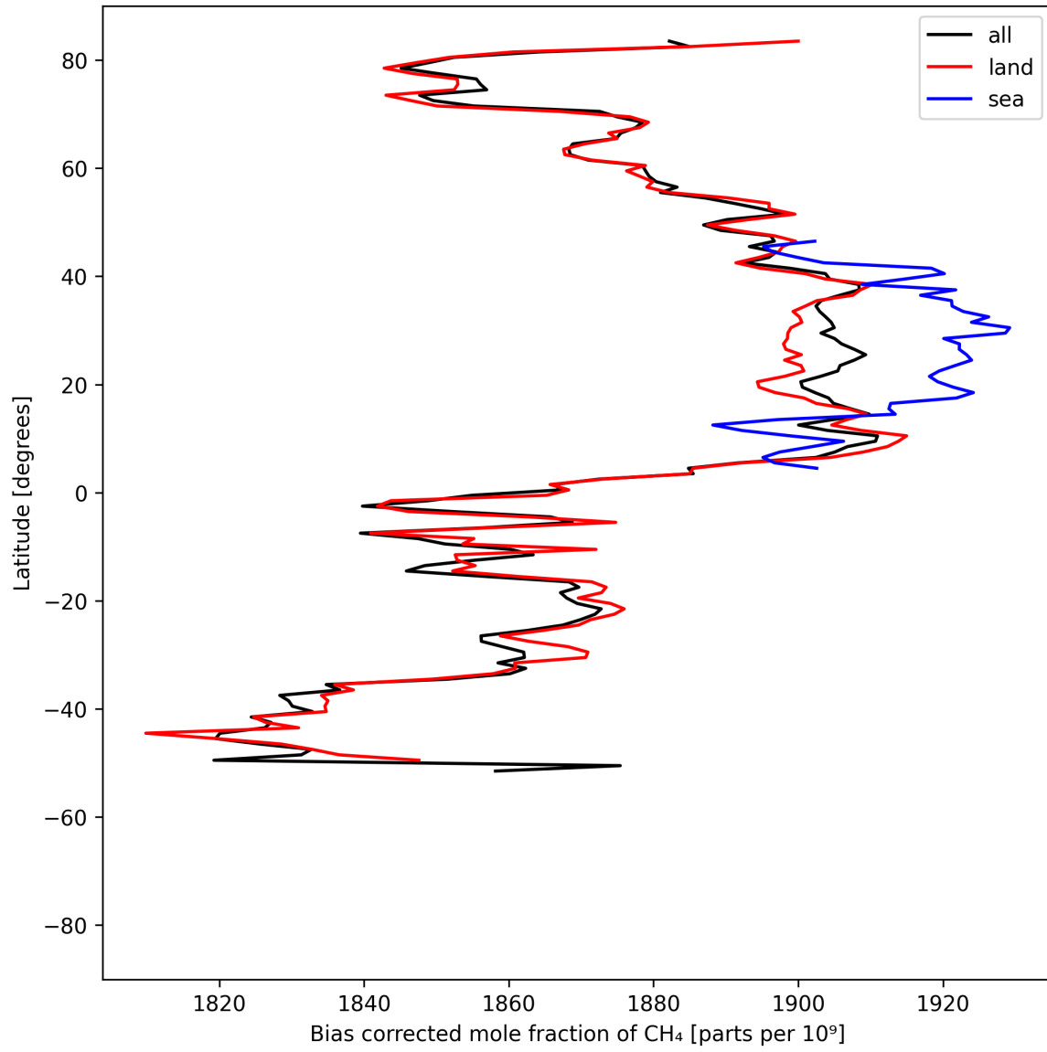
Figure 14: Zonal average of “Bias corrected mole fraction of CH 4 ” for 2025-05-15 to 2025-05-16.
