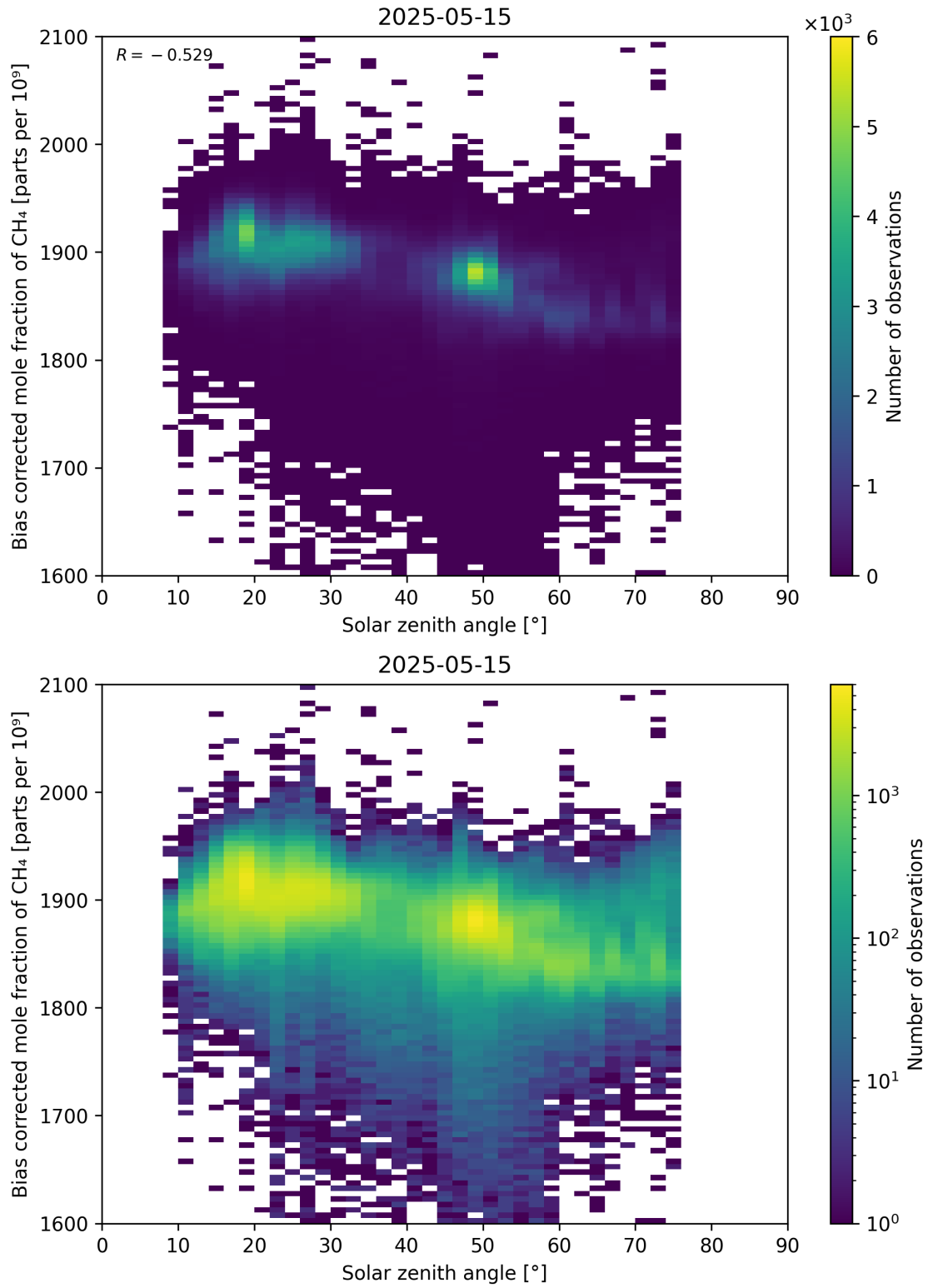
Figure 100: Scatter density plot of “Solar zenith angle” against “Bias corrected mole fraction of CH 4 ” for 2025-05-15 to 2025-05-16.
