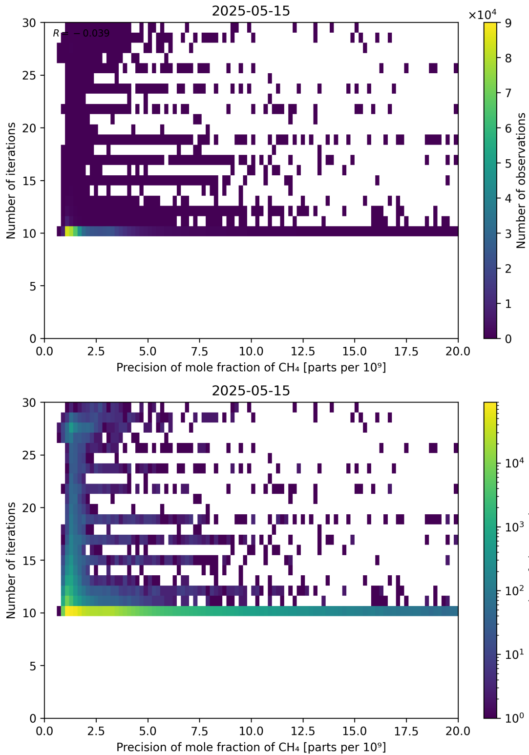
Figure 83: Scatter density plot of “Precision of mole fraction of CH 4 ” against “Number of iterations” for 2025-05-15 to 2025-05-16.
