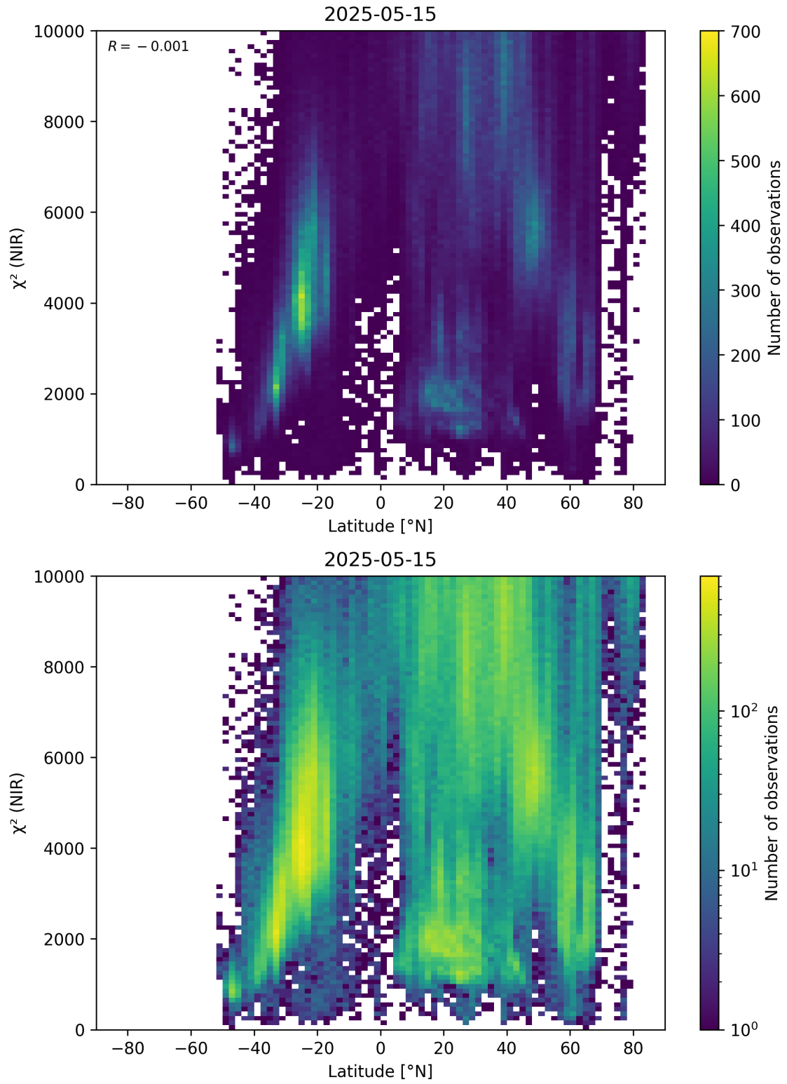
Figure 53: Scatter density plot of “Latitude” against “ \chi^2 (NIR)” for 2025-05-15 to 2025-05-16.
