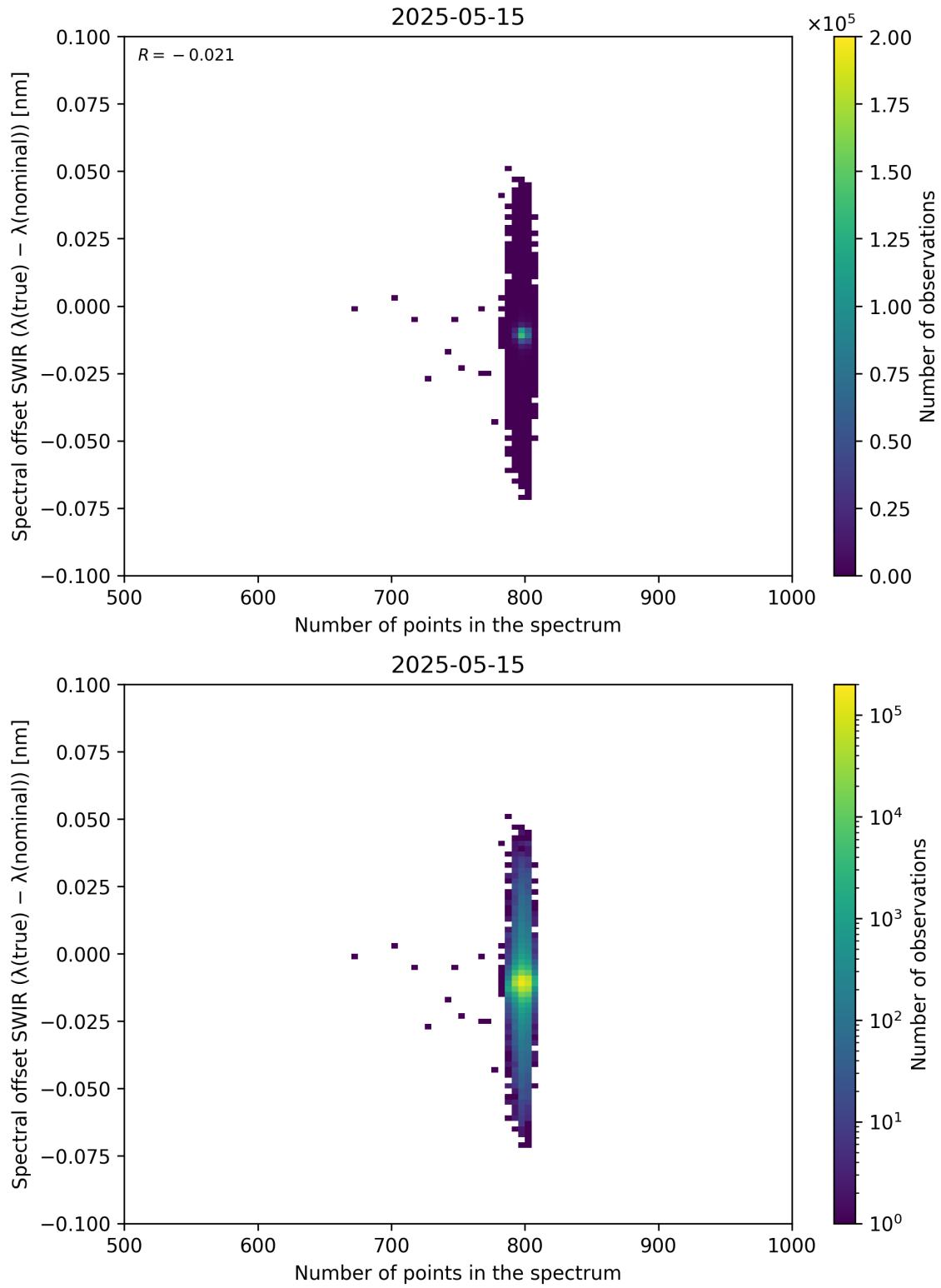
Figure 93: Scatter density plot of “Number of points in the spectrum” against “Spectral offset SWIR ( \lambda_{\text{true}} - \lambda_{\text{nominal}} )” for 2025-05-15 to 2025-05-16.
