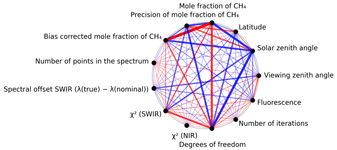
Figure 1: Map of correlation graph for 2025-05-15 to 2025-05-16.
