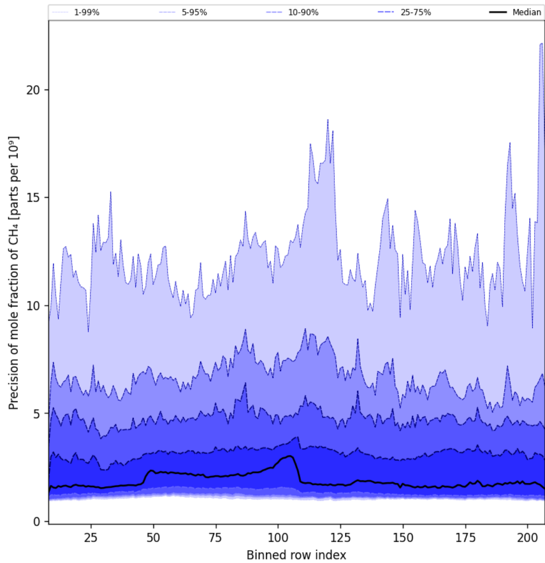
Figure 35: Along track statistics of “Precision of mole fraction of CH 4 ” for 2025-05-15 to 2025-05-16
