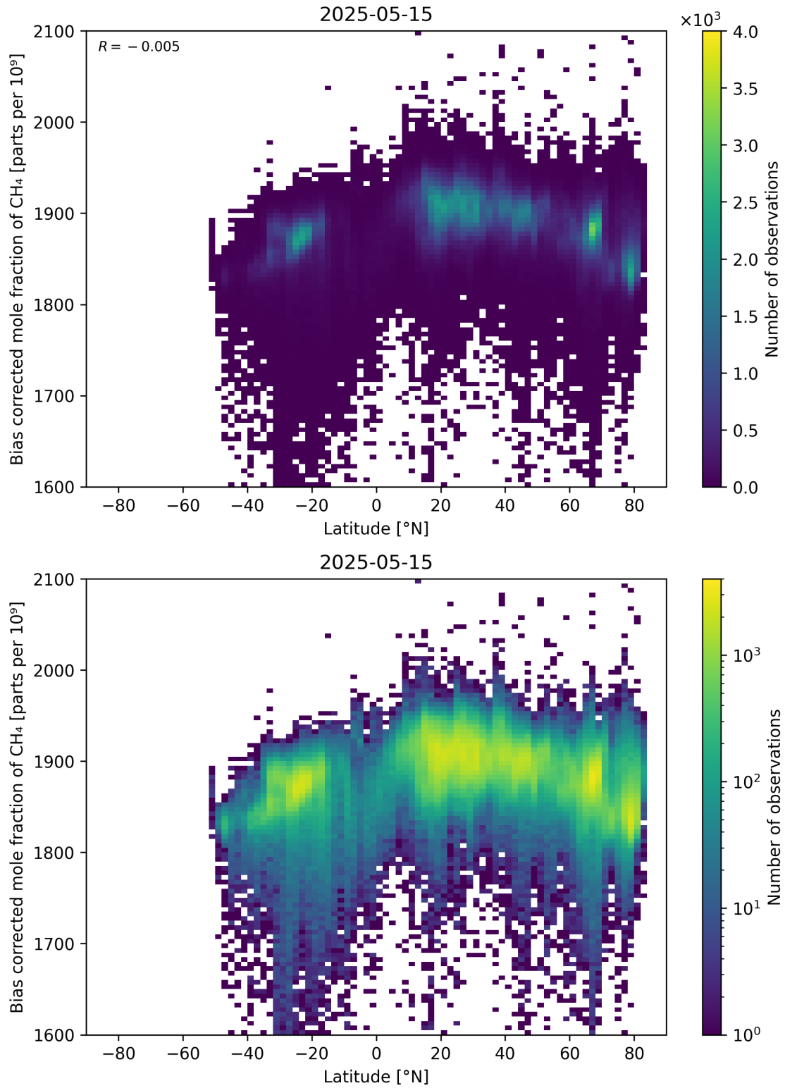
Figure 58: Scatter density plot of “Latitude” against “Bias corrected mole fraction of CH 4 ” for 2025-05-15 to 2025-05-16.
