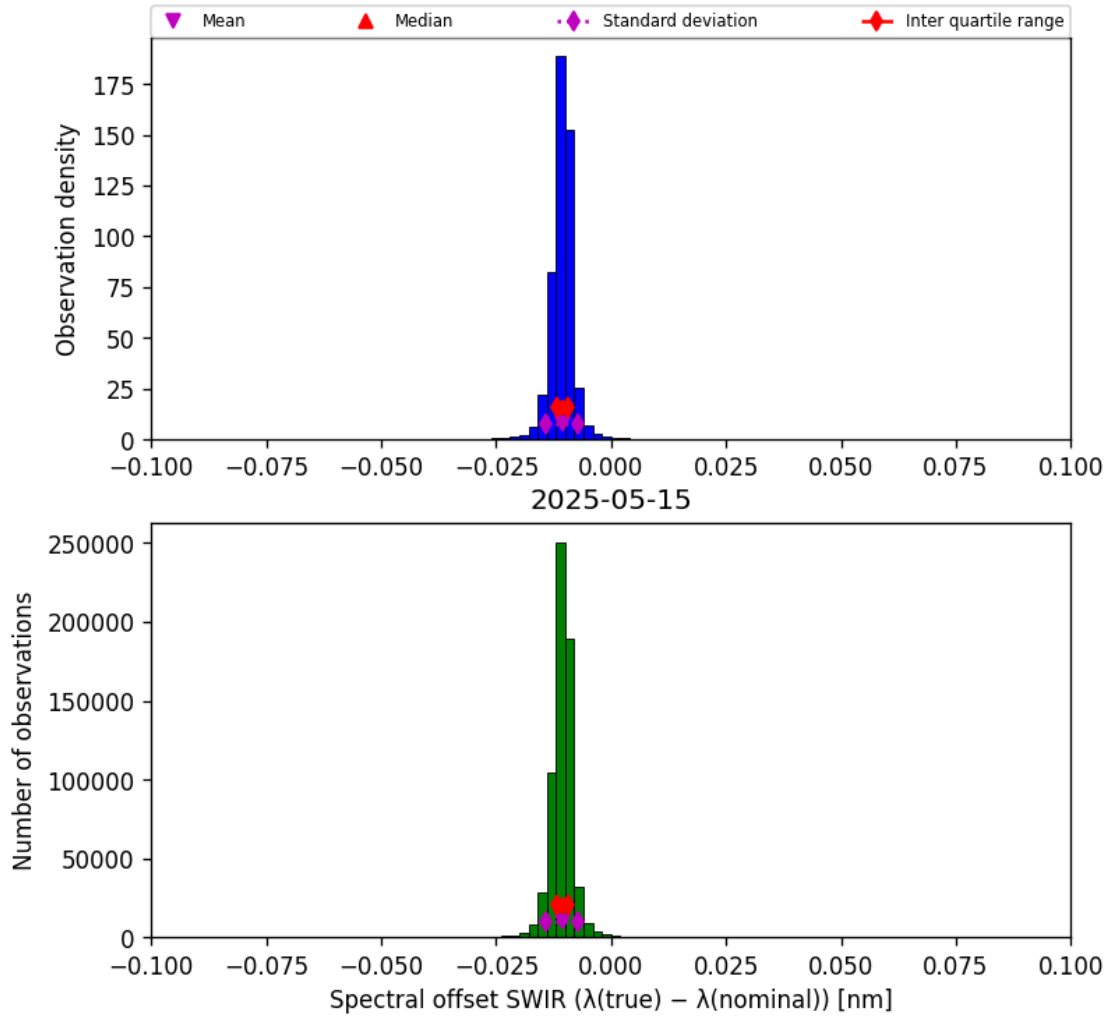
Figure 27: Histogram of “Spectral offset SWIR ( \lambda_{\text{true}} - \lambda_{\text{nominal}} )” for 2025-05-15 to 2025-05-16
