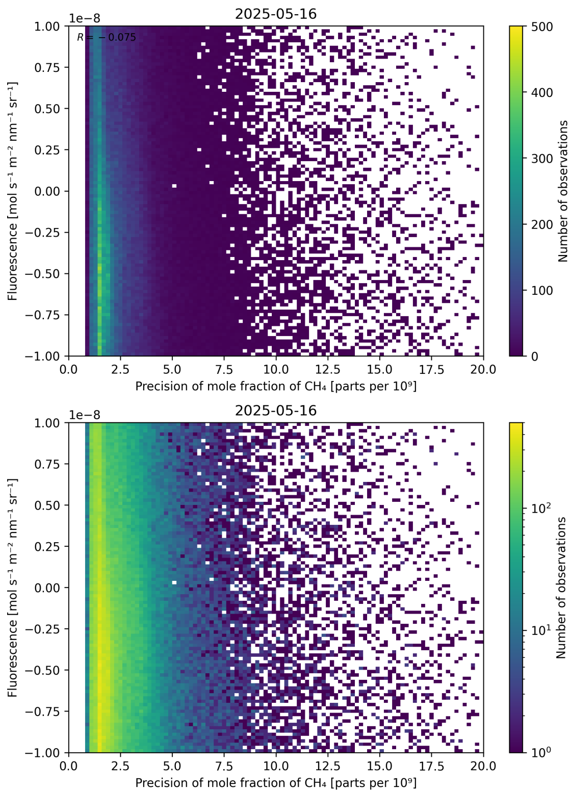
Figure 81: Scatter density plot of “Precision of mole fraction of CH 4 ” against “Fluorescence” for 2025-05-15 to 2025-05-17.
