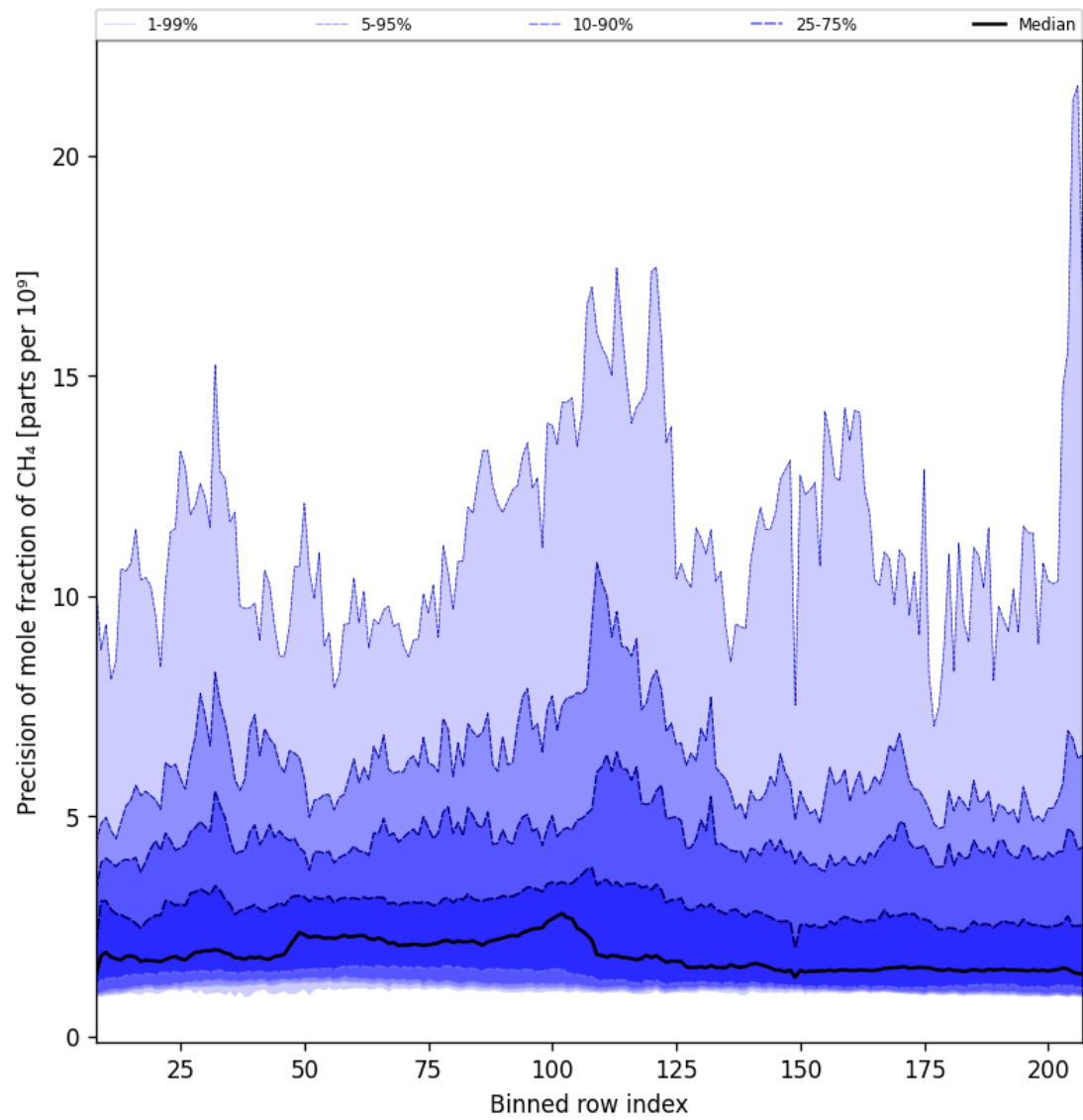
Figure 35: Along track statistics of “Precision of mole fraction of CH 4 ” for 2025-05-15 to 2025-05-17
