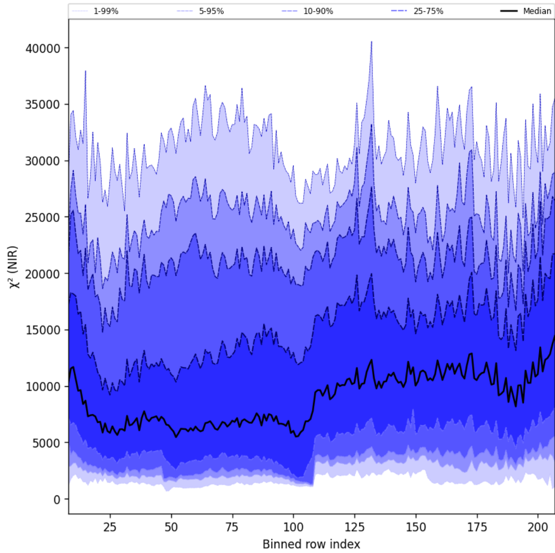
Figure 40: Along track statistics of “ \chi^2 (NIR)” for 2025-05-15 to 2025-05-17
