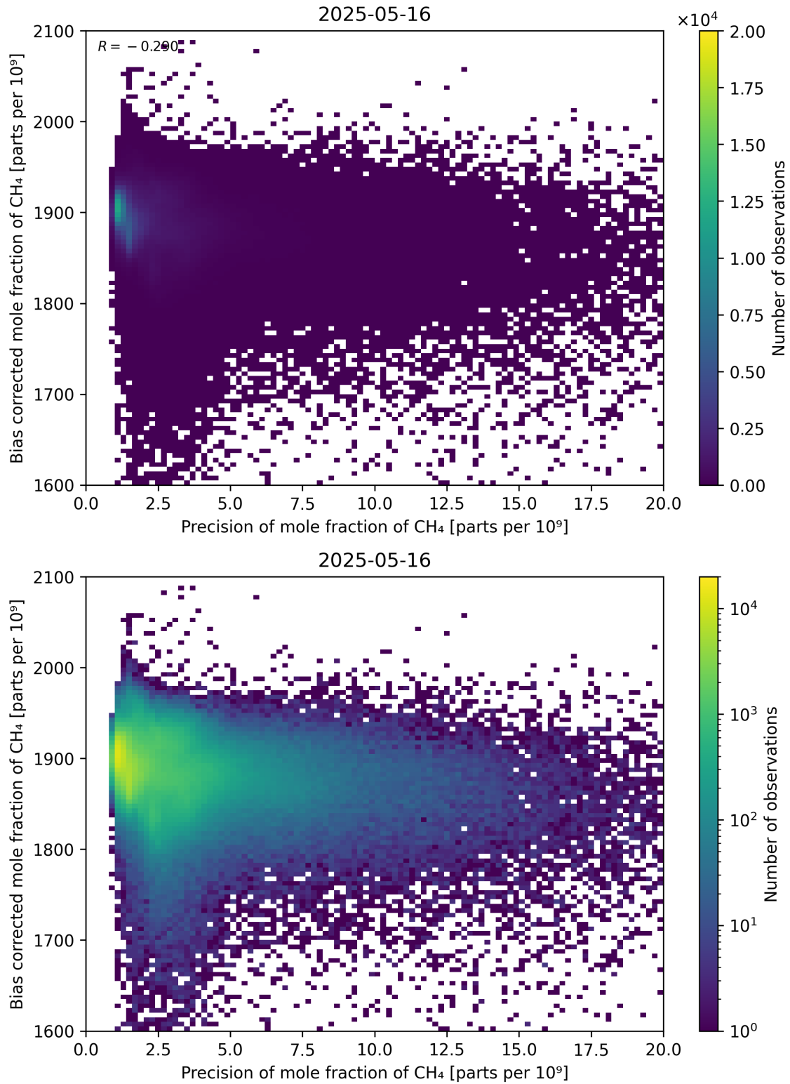
Figure 82: Scatter density plot of “Precision of mole fraction of CH 4 ” against “Bias corrected mole fraction of CH 4 ” for 2025-05-15 to 2025-05-17.
