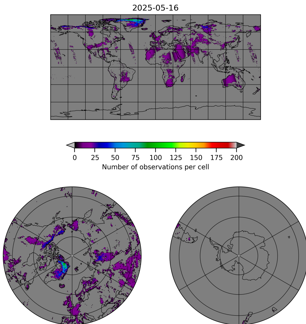
Figure 10: Map of the number of observations for 2025-05-15 to 2025-05-17
