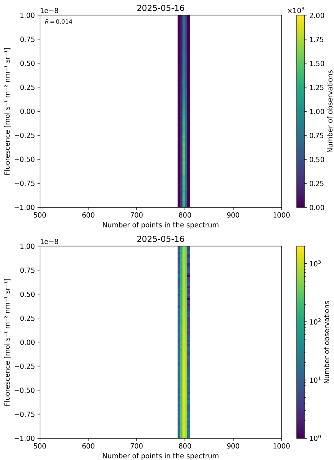
Figure 91: Scatter density plot of “Number of points in the spectrum” against “Fluorescence” for 2025-05-15 to 2025-05-17.
