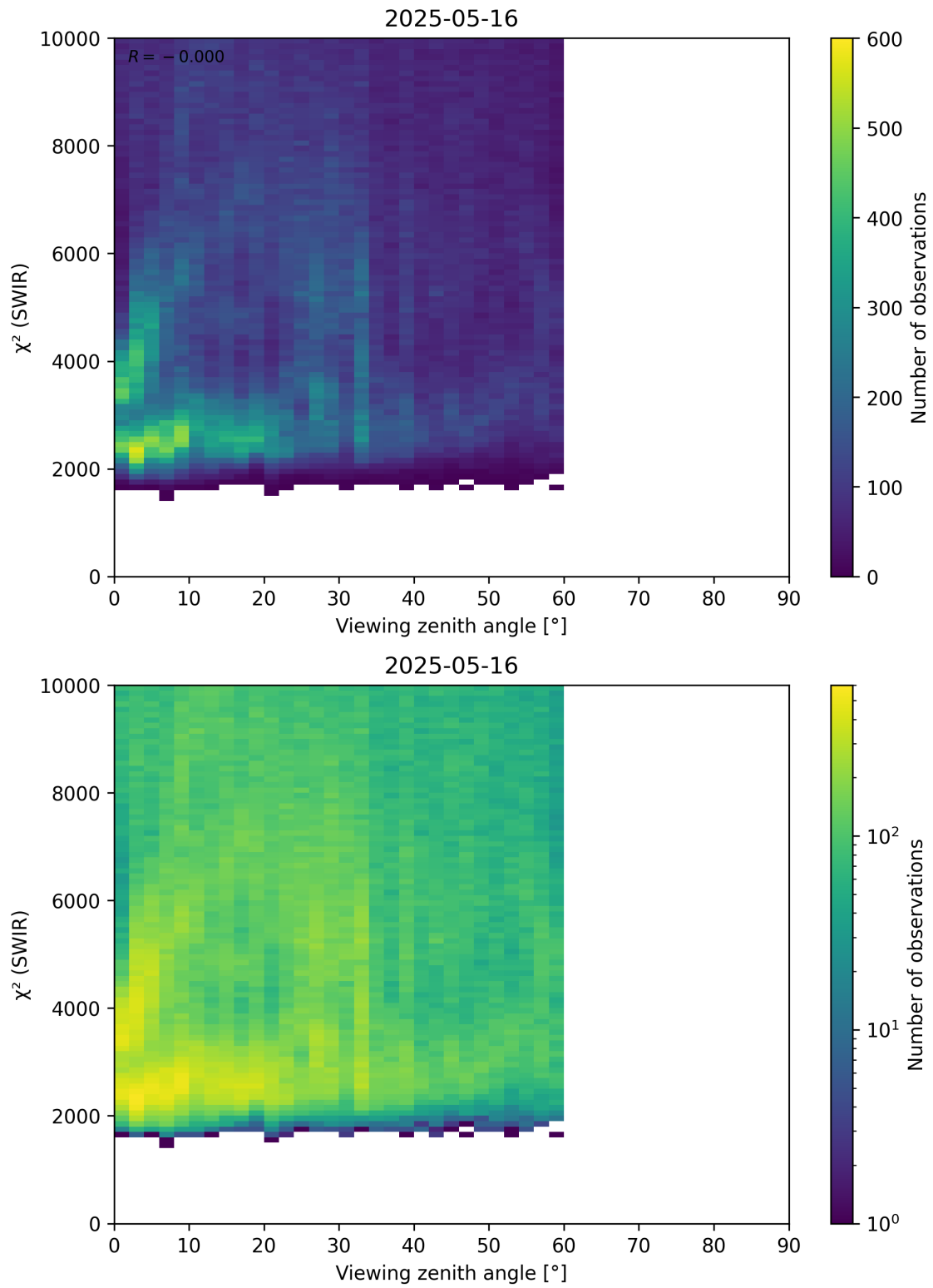
Figure 106: Scatter density plot of “Viewing zenith angle” against “ \chi^2 (SWIR)” for 2025-05-15 to 2025-05-17.
