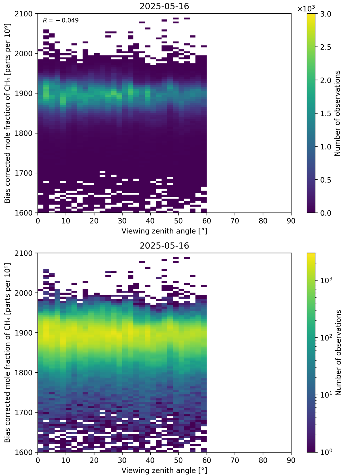
Figure 111: Scatter density plot of “Viewing zenith angle” against “Bias corrected mole fraction of CH 4 ” for 2025-05-15 to 2025-05-17.
