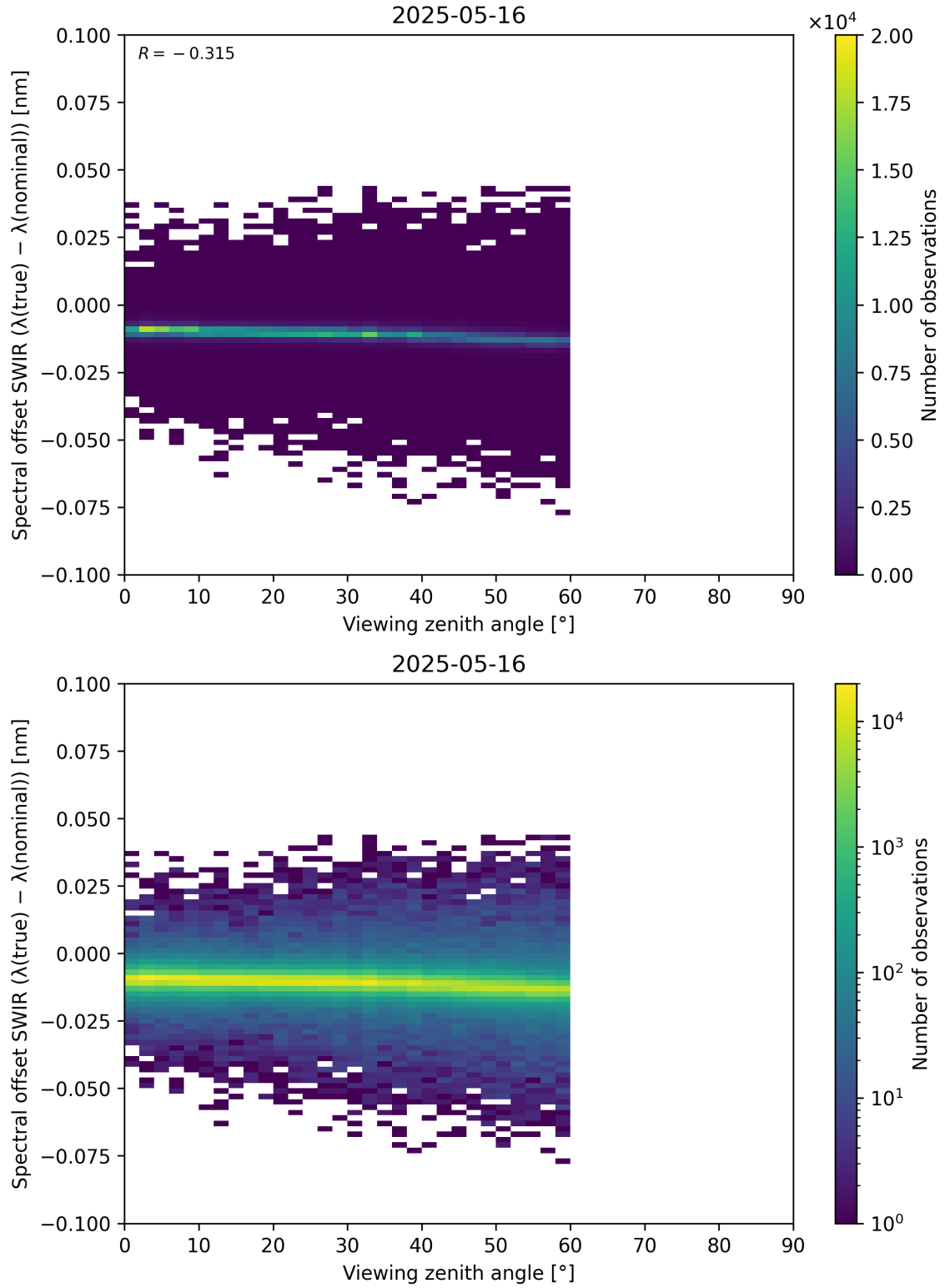
Figure 116: Scatter density plot of “Viewing zenith angle” against “Spectral offset SWIR ( \lambda_{\text{true}} - \lambda_{\text{nominal}} )” for 2025-05-15 to 2025-05-17.
