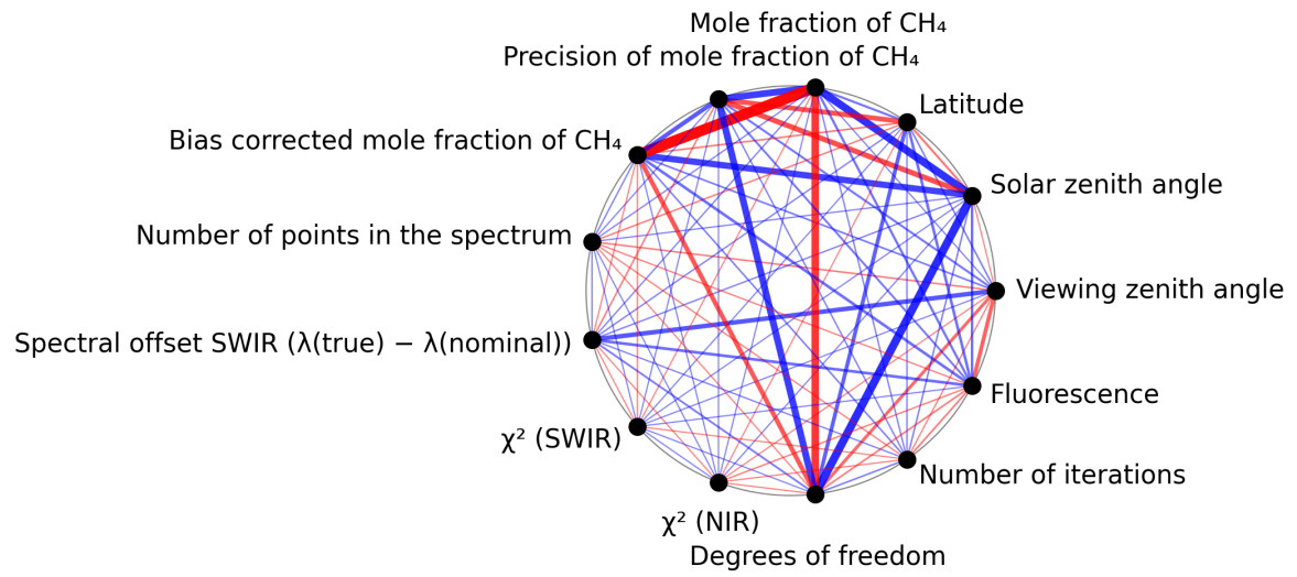
Figure 1: Map of correlation graph for 2025-05-15 to 2025-05-17.
