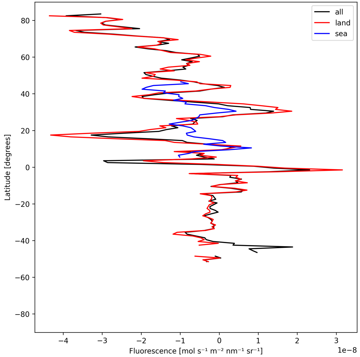
Figure 21: Zonal average of “Fluorescence” for 2025-05-15 to 2025-05-17.
