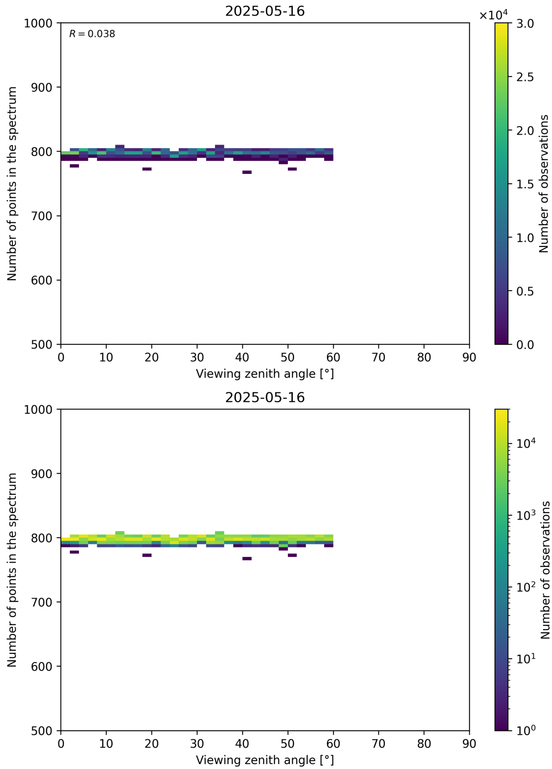
Figure 114: Scatter density plot of “Viewing zenith angle” against “Number of points in the spectrum” for 2025-05-15 to 2025-05-17.
