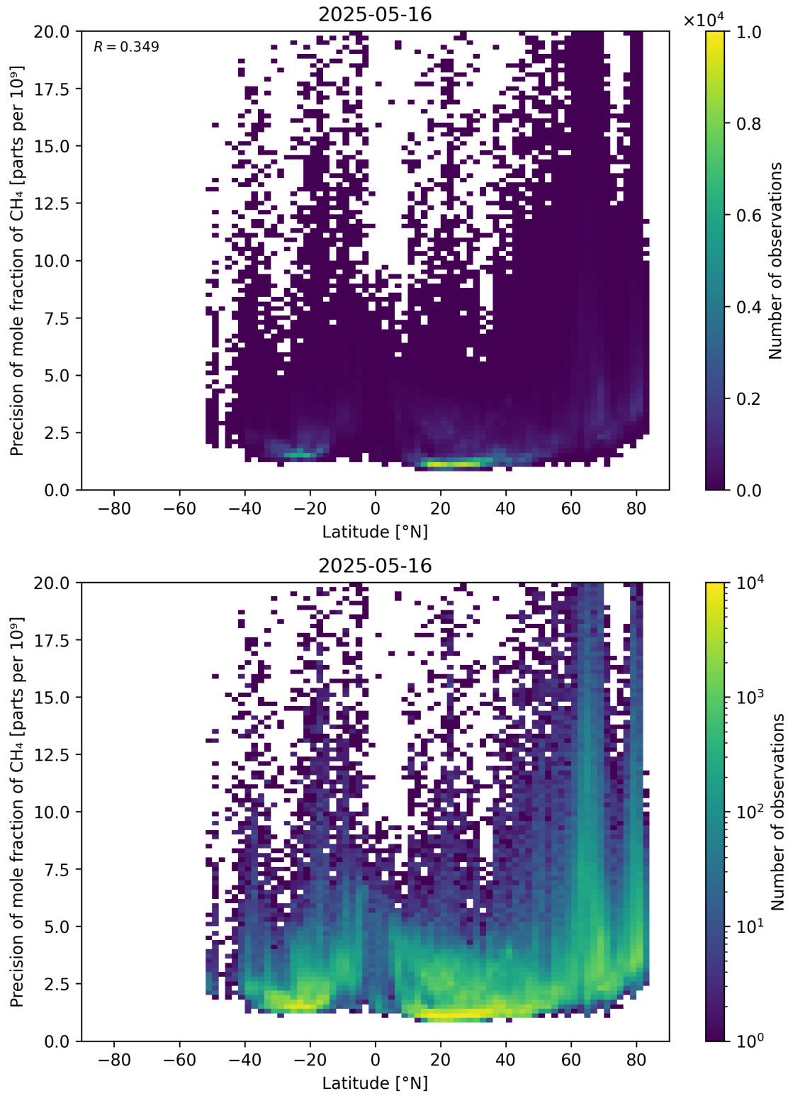
Figure 59: Scatter density plot of “Latitude” against “Precision of mole fraction of \text{CH}_4 ” for 2025-05-15 to 2025-05-17.
