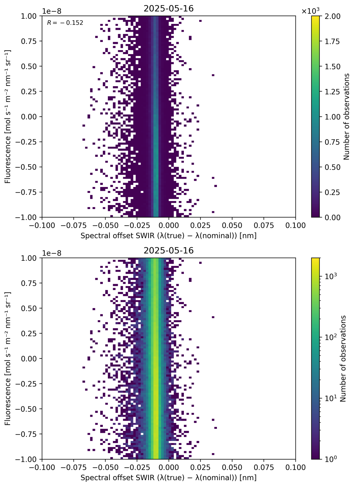
Figure 120: Scatter density plot of “Spectral offset SWIR ( \lambda_{\text{true}} - \lambda_{\text{nominal}} )” against “Fluorescence” for 2025-05-15 to 2025-05-17.
