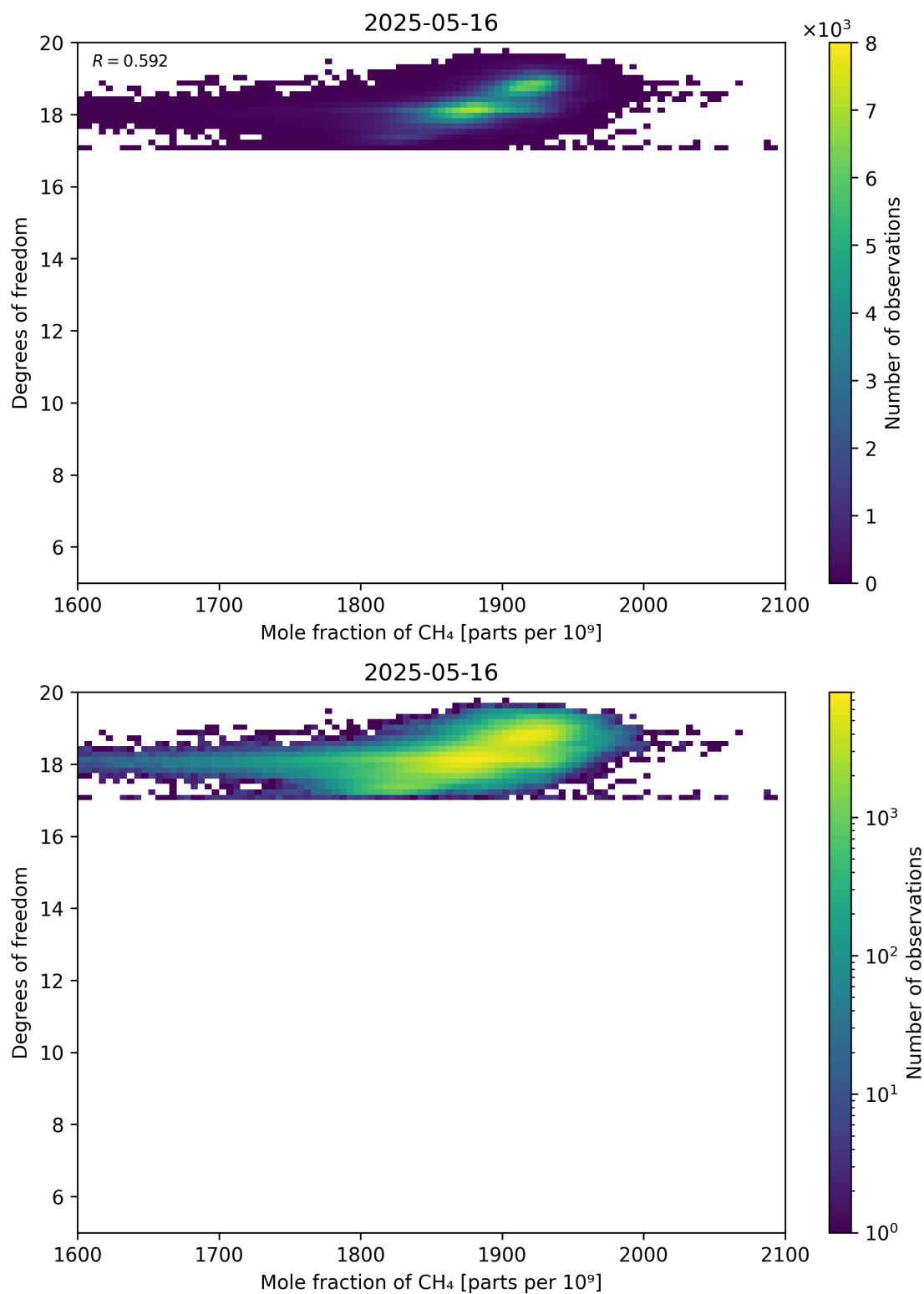
Figure 72: Scatter density plot of “Mole fraction of CH 4 ” against “Degrees of freedom” for 2025-05-15 to 2025-05-17.
