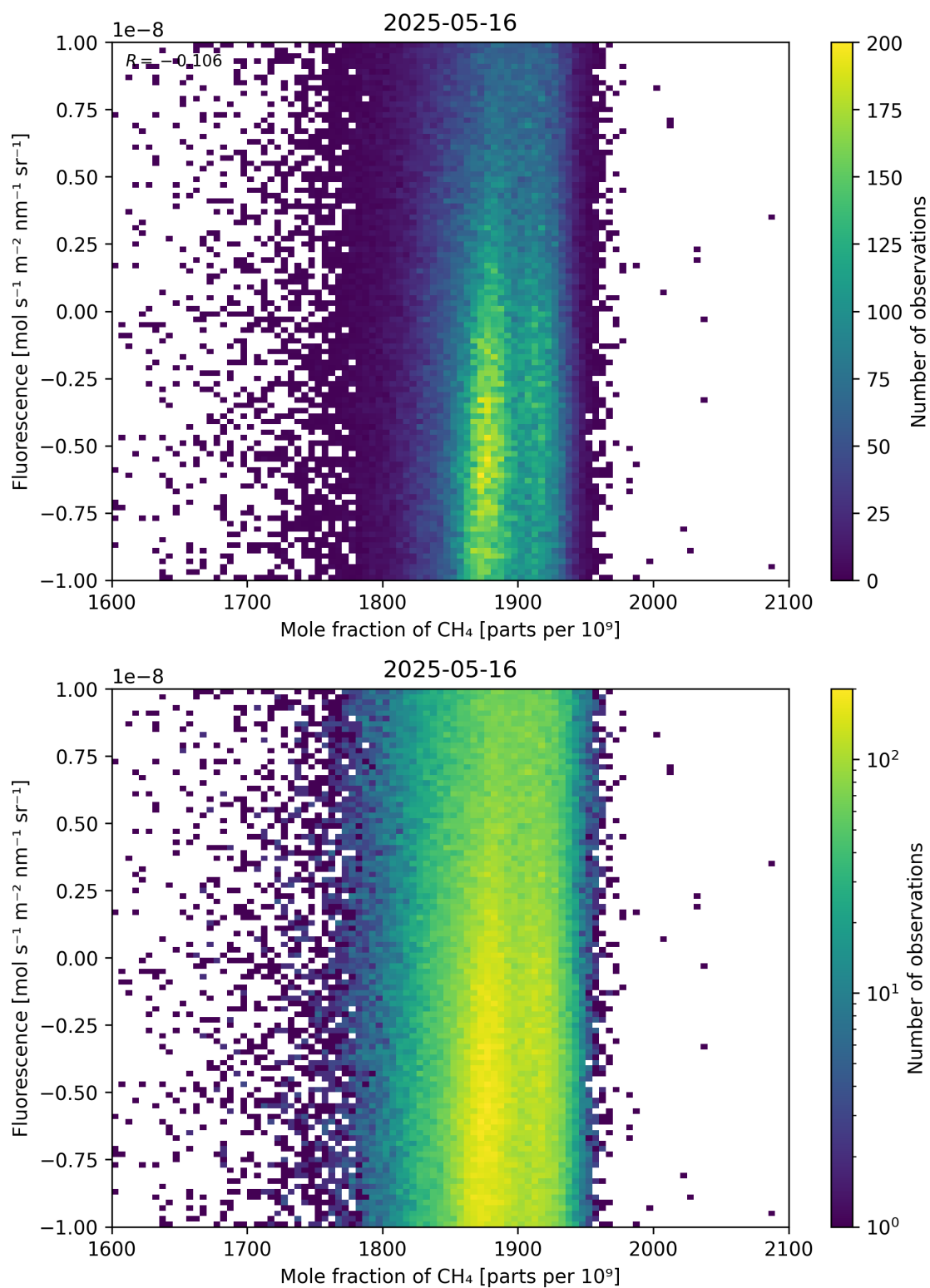
Figure 73: Scatter density plot of “Mole fraction of \text{CH}_4 ” against “Fluorescence” for 2025-05-15 to 2025-05-17.
