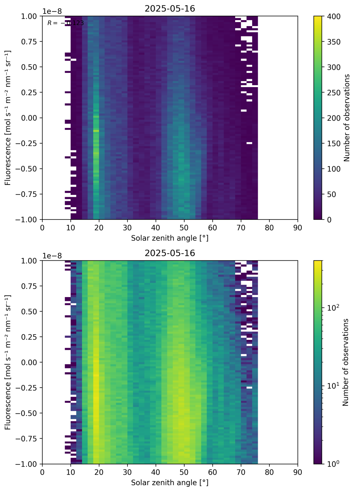
Figure 97: Scatter density plot of “Solar zenith angle” against “Fluorescence” for 2025-05-15 to 2025-05-17.
