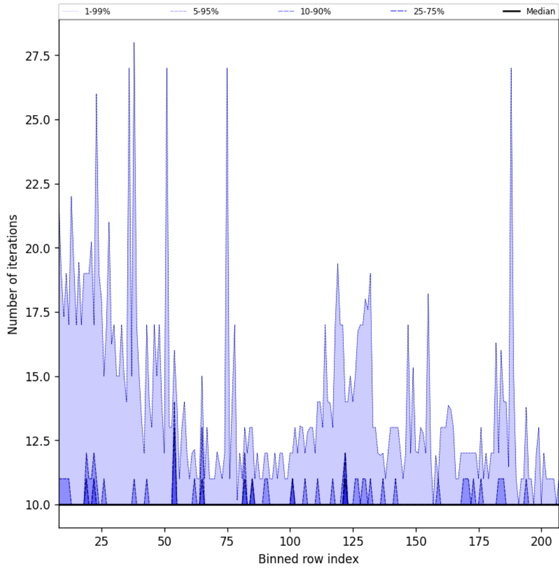
Figure 42: Along track statistics of “Number of iterations” for 2025-05-15 to 2025-05-17
