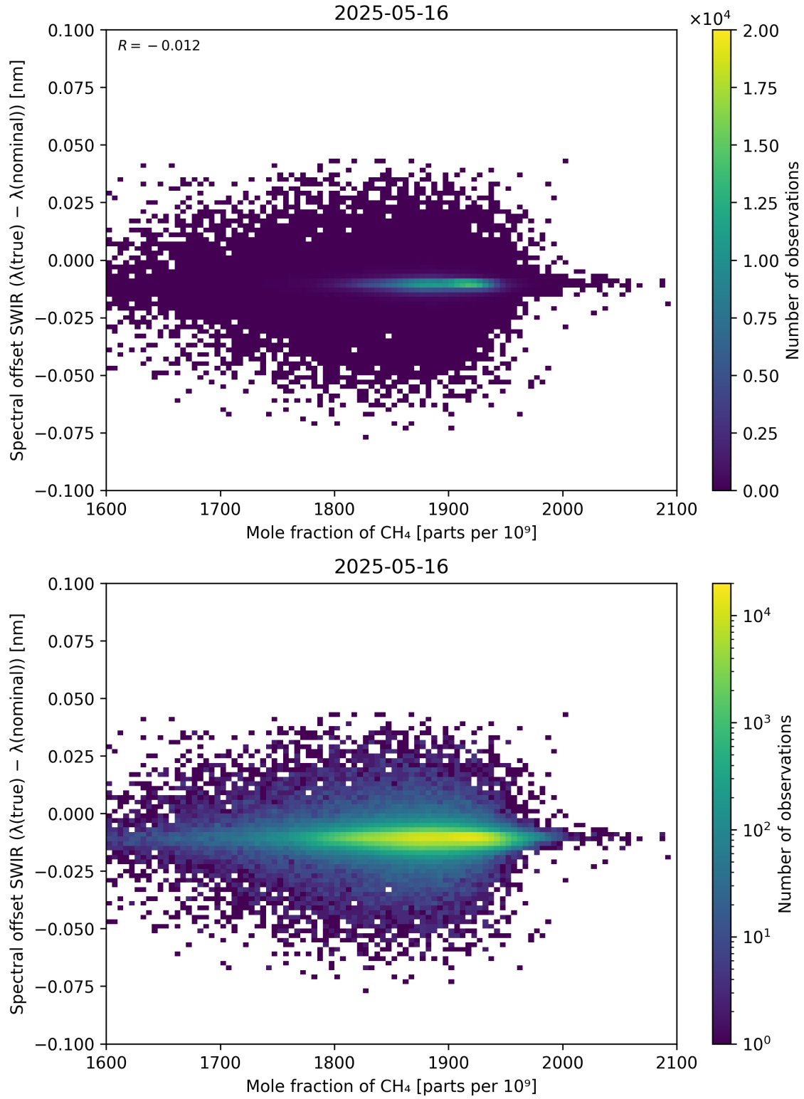
Figure 86: Scatter density plot of “Mole fraction of CH 4 ” against “Spectral offset SWIR ( \lambda_{\text{true}} - \lambda_{\text{nominal}} )” for 2025-05-15 to 2025-05-17.
