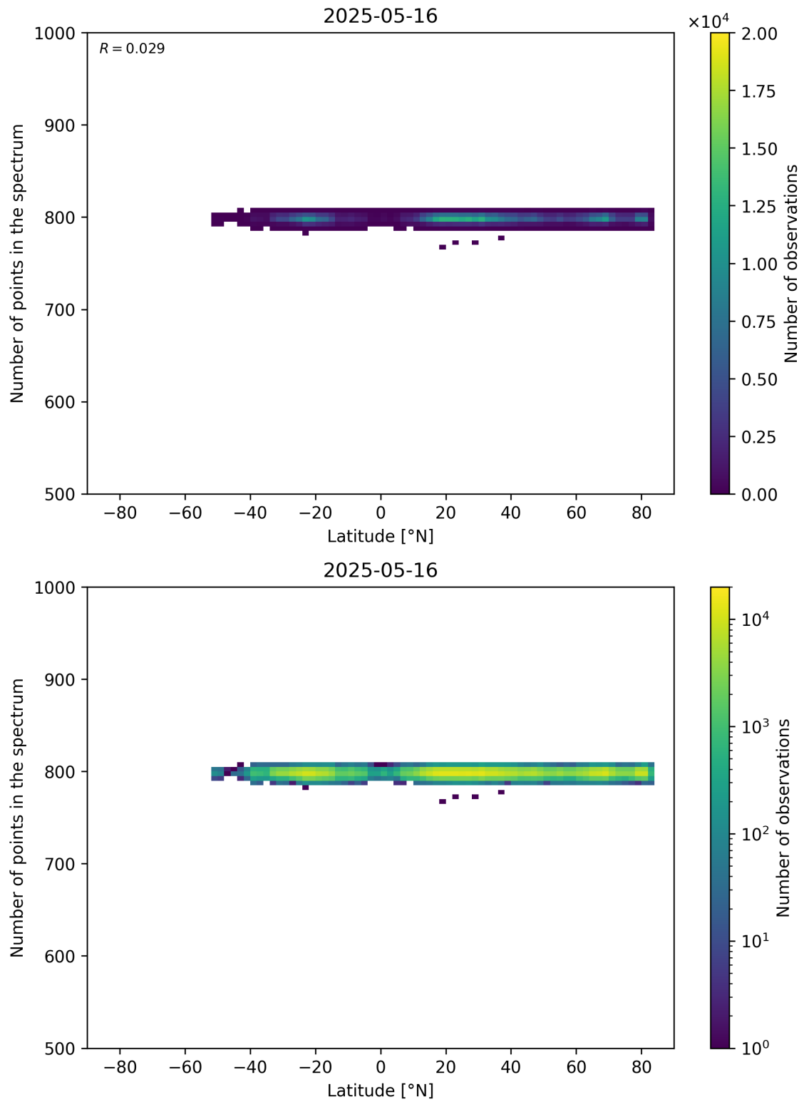
Figure 61: Scatter density plot of “Latitude” against “Number of points in the spectrum” for 2025-05-15 to 2025-05-17.
