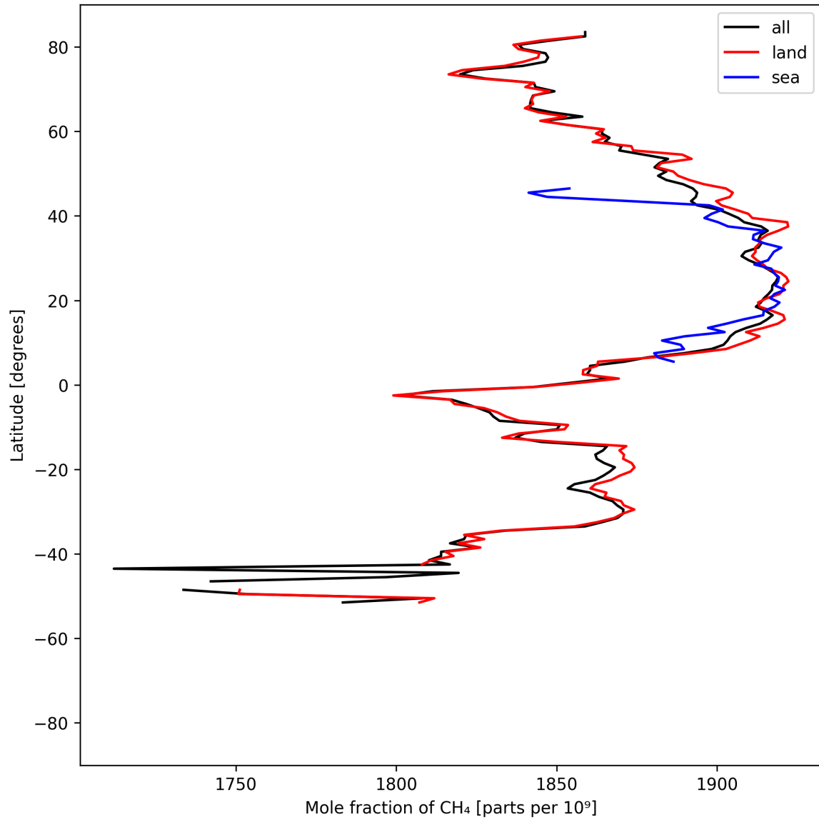
Figure 12: Zonal average of “Mole fraction of CH 4 ” for 2025-05-15 to 2025-05-17.
