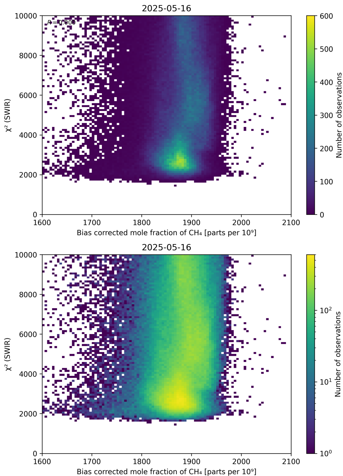
Figure 64: Scatter density plot of “Bias corrected mole fraction of \text{CH}_4 ” against “ \chi^2 (SWIR)” for 2025-05-15 to 2025-05-17.
