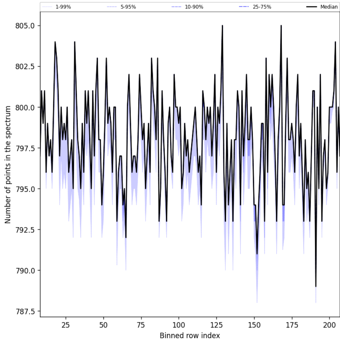
Figure 37: Along track statistics of “Number of points in the spectrum” for 2025-05-15 to 2025-05-17
