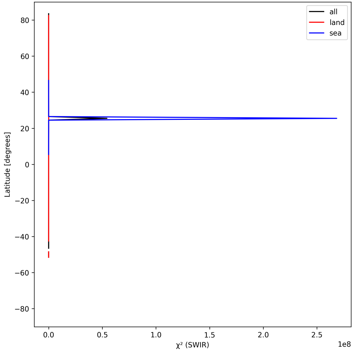
Figure 17: Zonal average of “ \chi^2 (SWIR)” for 2025-05-15 to 2025-05-17.
