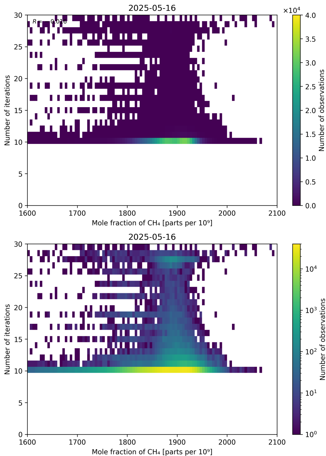
Figure 76: Scatter density plot of “Mole fraction of CH 4 ” against “Number of iterations” for 2025-05-15 to 2025-05-17.
