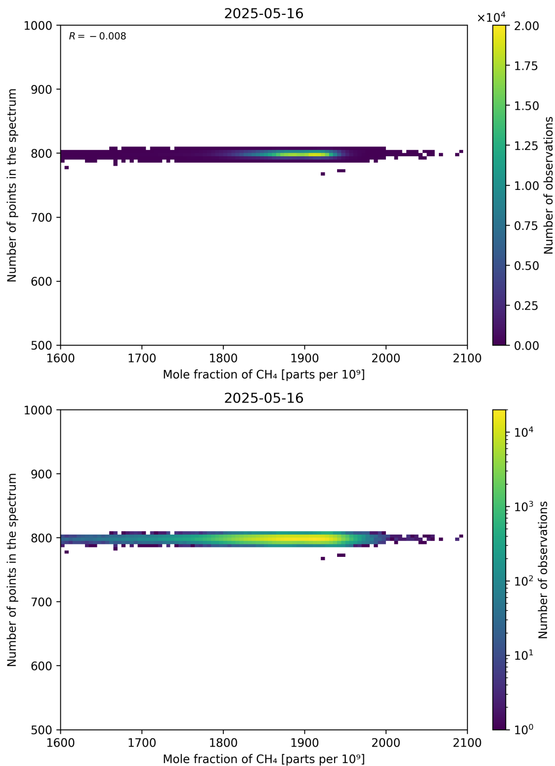
Figure 77: Scatter density plot of “Mole fraction of CH 4 ” against “Number of points in the spectrum” for 2025-05-15 to 2025-05-17.
