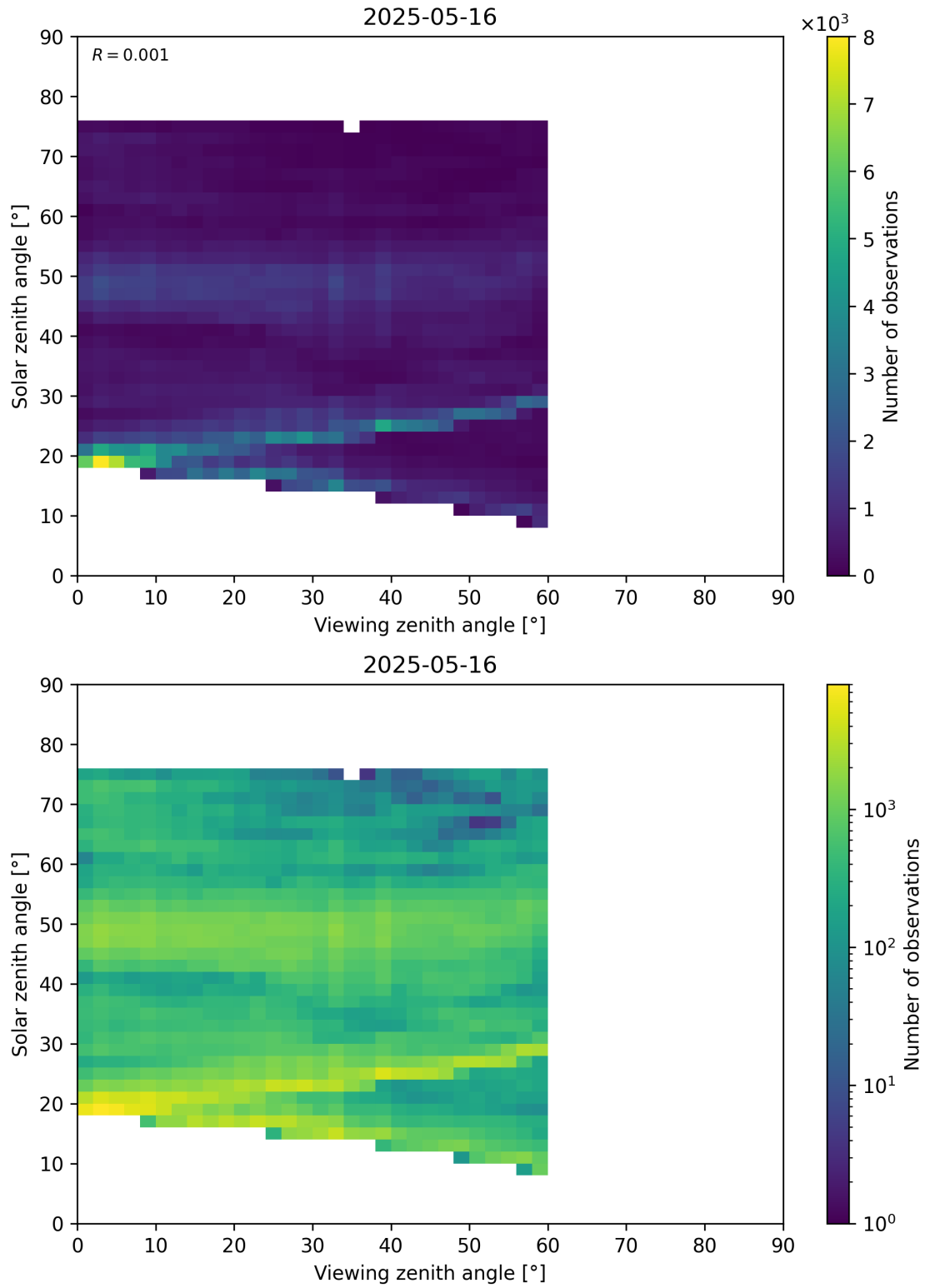
Figure 115: Scatter density plot of “Viewing zenith angle” against “Solar zenith angle” for 2025-05-15 to 2025-05-17.
