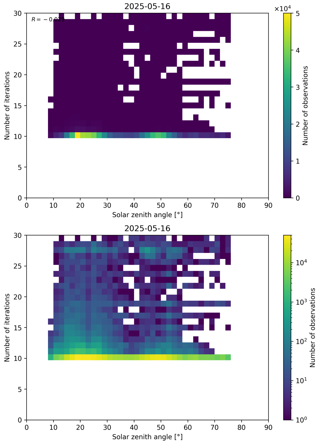
Figure 102: Scatter density plot of “Solar zenith angle” against “Number of iterations” for 2025-05-15 to 2025-05-17.
