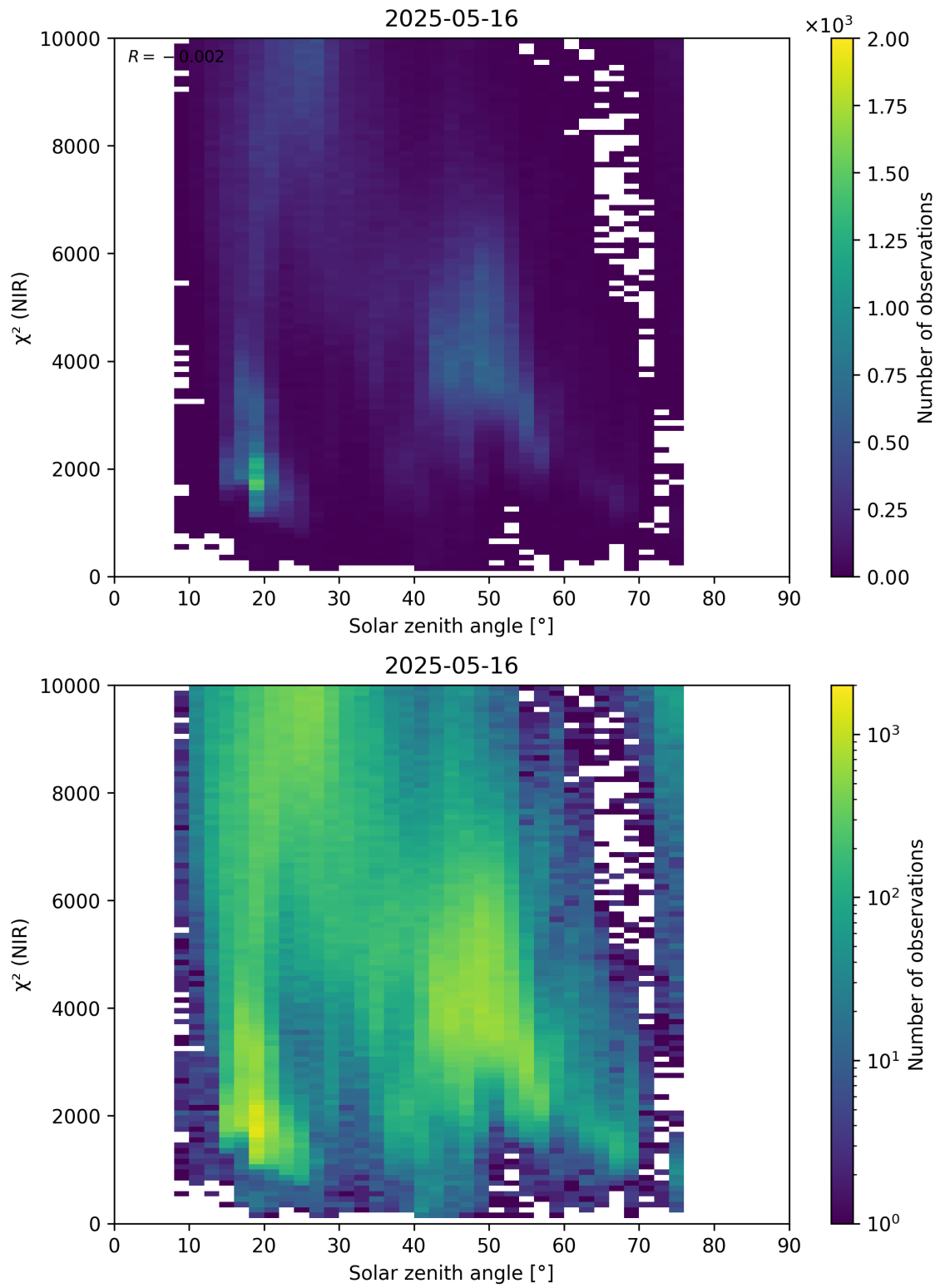
Figure 94: Scatter density plot of “Solar zenith angle” against “ \chi^2 (NIR)” for 2025-05-15 to 2025-05-17.
