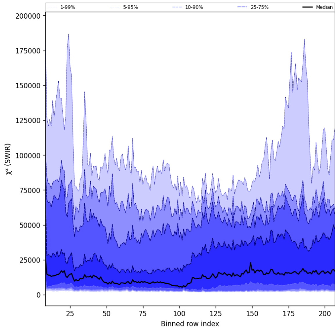
Figure 39: Along track statistics of “ \chi^2 (SWIR)” for 2025-05-15 to 2025-05-17
