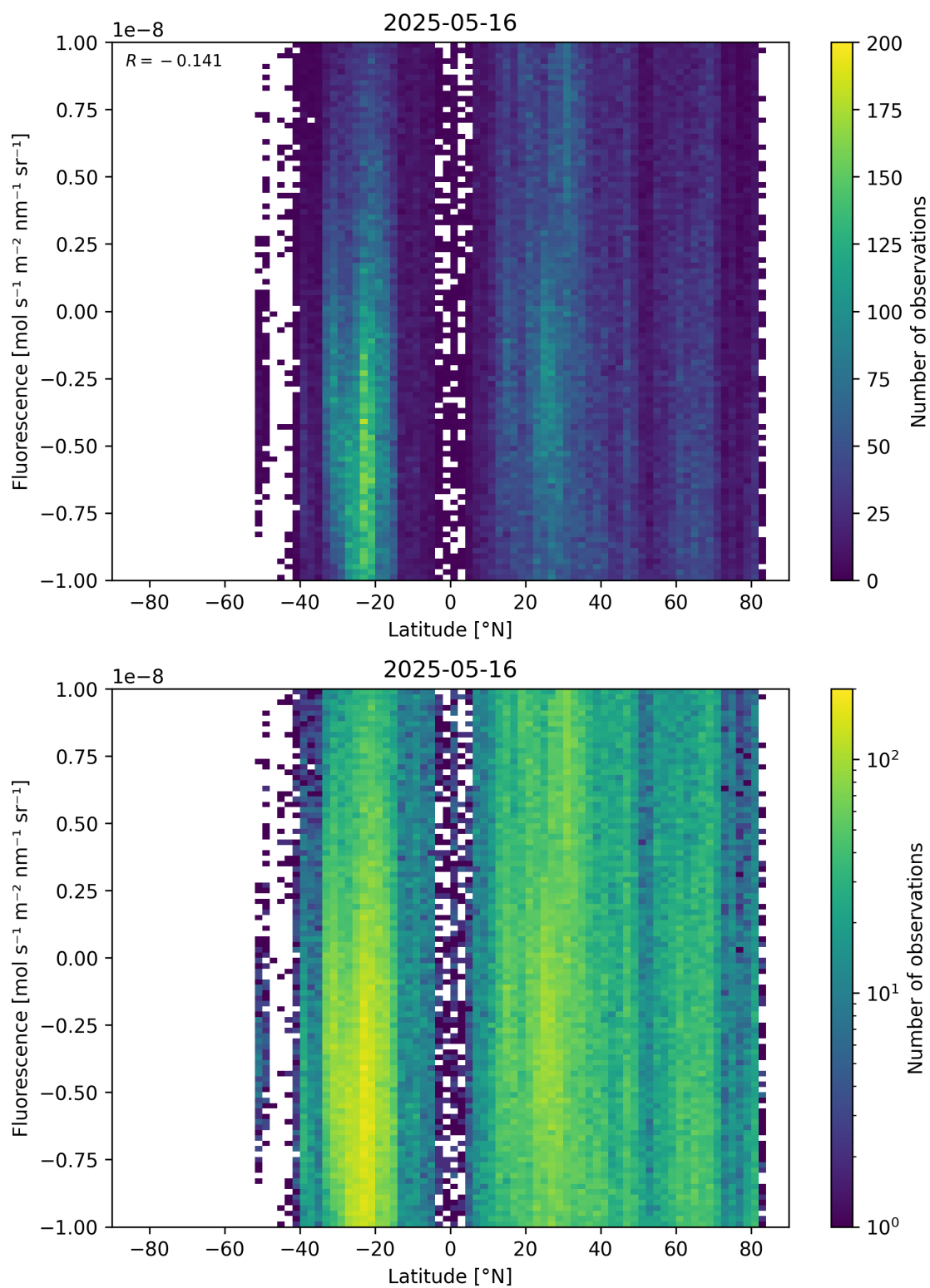
Figure 56: Scatter density plot of “Latitude” against “Fluorescence” for 2025-05-15 to 2025-05-17.
