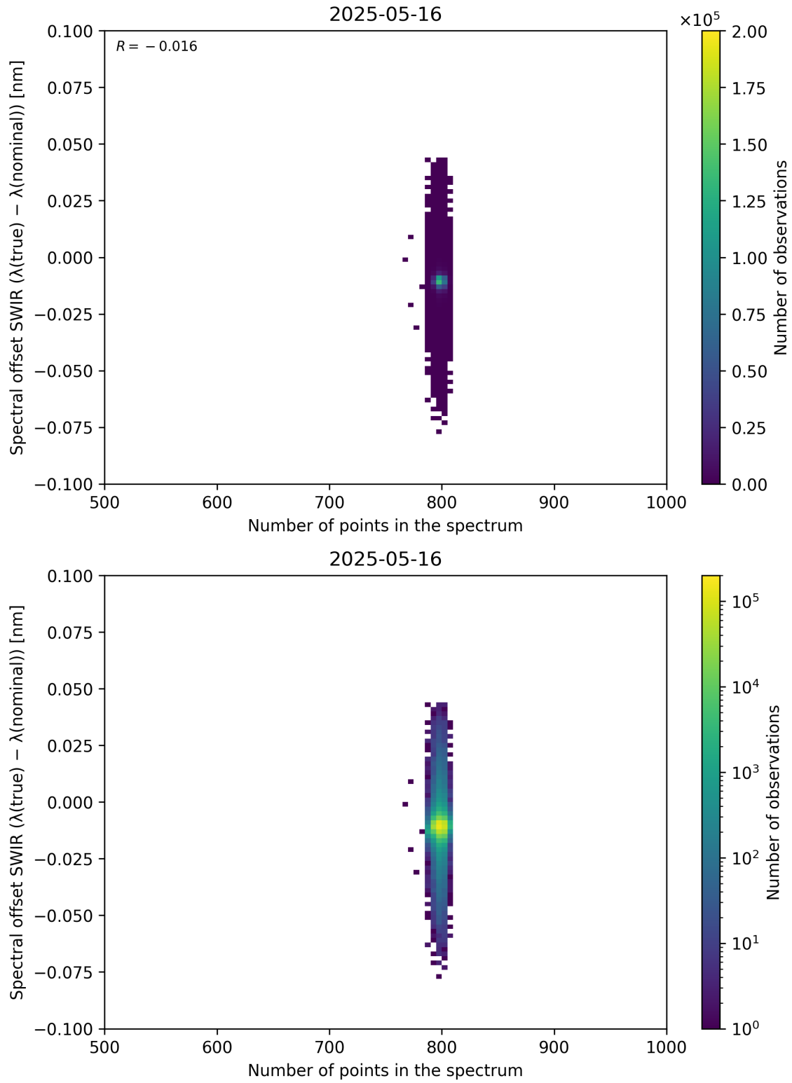
Figure 93: Scatter density plot of “Number of points in the spectrum” against “Spectral offset SWIR ( \lambda_{\text{true}} - \lambda_{\text{nominal}} )” for 2025-05-15 to 2025-05-17.
