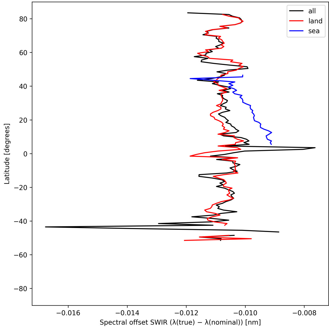
Figure 16: Zonal average of “Spectral offset SWIR ( \lambda_{\text{true}} - \lambda_{\text{nominal}} )” for 2025-05-15 to 2025-05-17.
