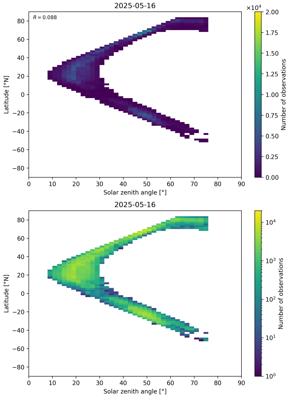
Figure 98: Scatter density plot of “Solar zenith angle” against “Latitude” for 2025-05-15 to 2025-05-17.
