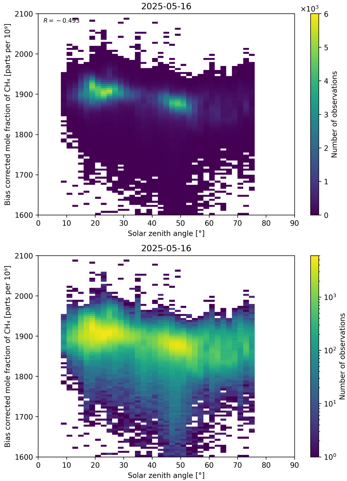
Figure 100: Scatter density plot of “Solar zenith angle” against “Bias corrected mole fraction of CH 4 ” for 2025-05-15 to 2025-05-17.
