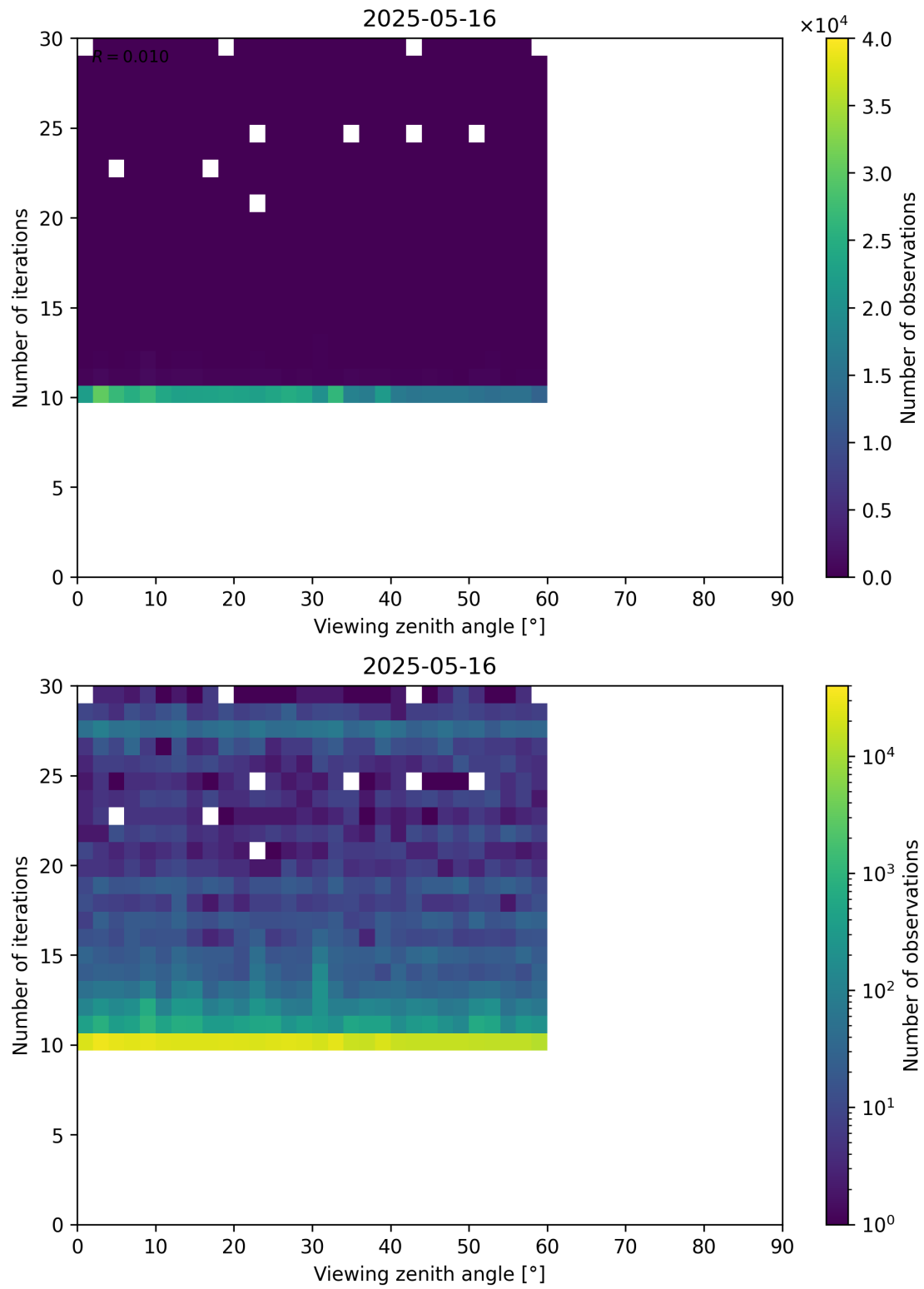
Figure 113: Scatter density plot of “Viewing zenith angle” against “Number of iterations” for 2025-05-15 to 2025-05-17.
