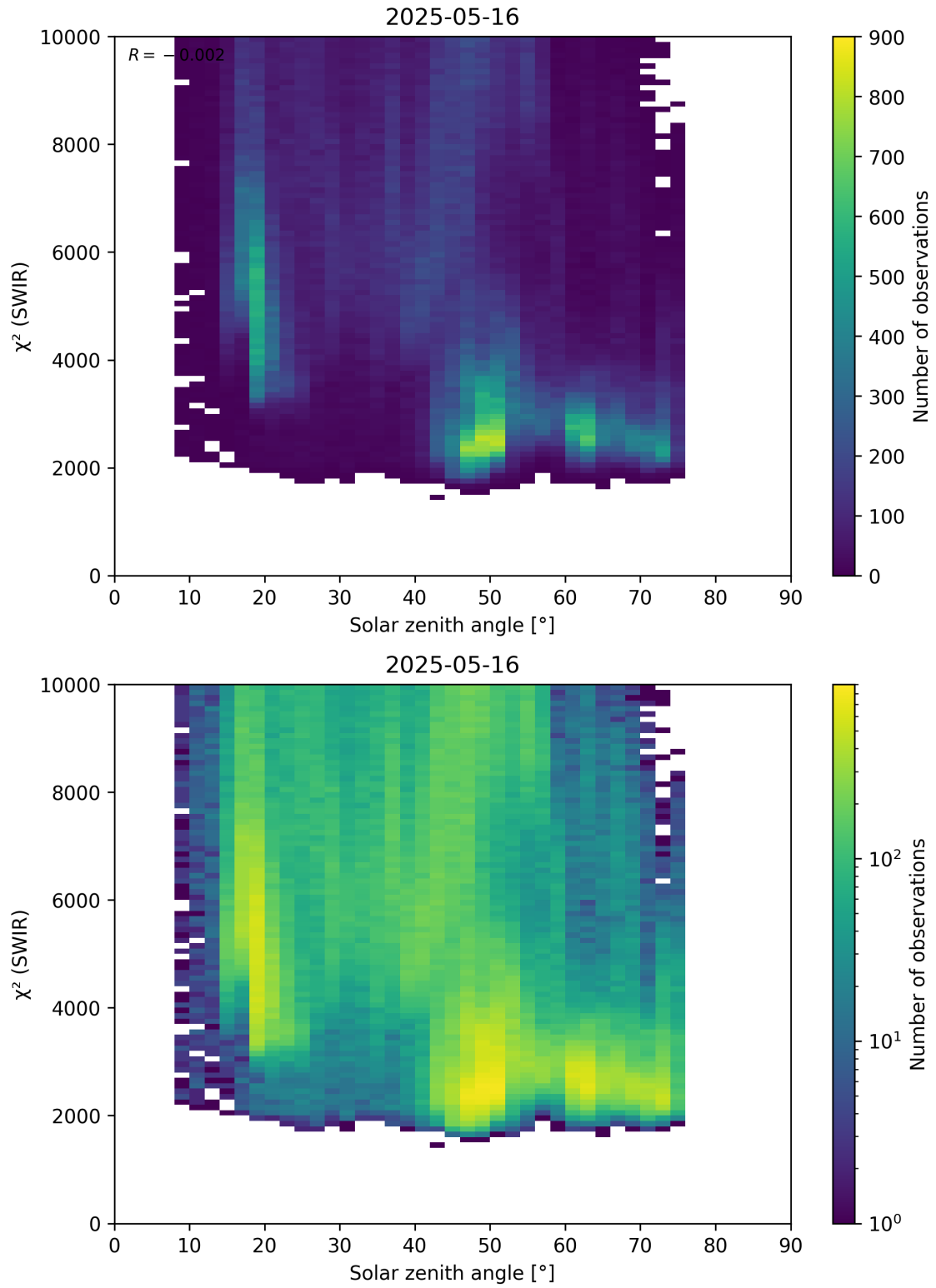
Figure 95: Scatter density plot of “Solar zenith angle” against “ \chi^2 (SWIR)” for 2025-05-15 to 2025-05-17.
