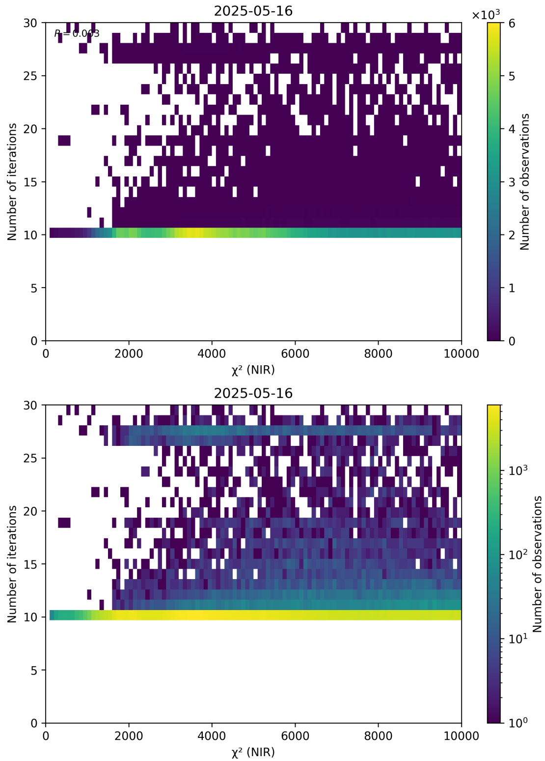
Figure 46: Scatter density plot of “ \chi^2 (NIR)” against “Number of iterations” for 2025-05-15 to 2025-05-17.
