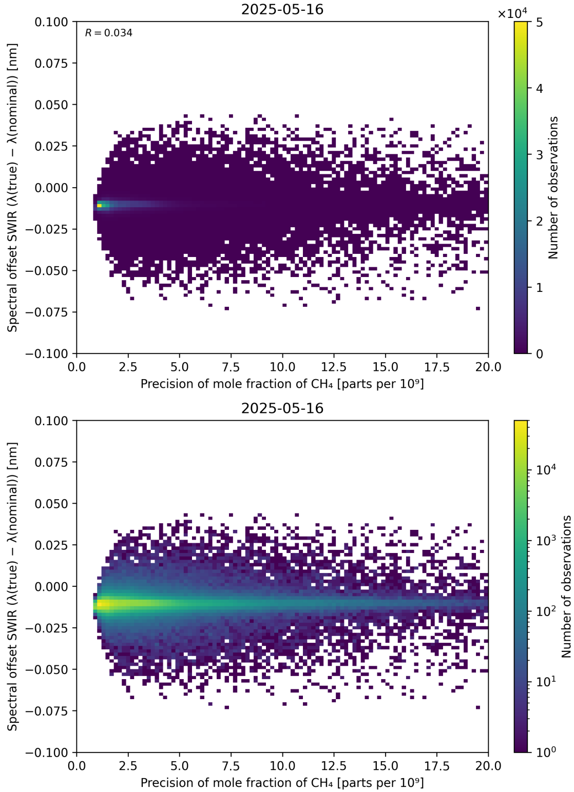
Figure 85: Scatter density plot of “Precision of mole fraction of CH 4 ” against “Spectral offset SWIR ( \lambda_{\text{true}} - \lambda_{\text{nominal}} )” for 2025-05-15 to 2025-05-17.
