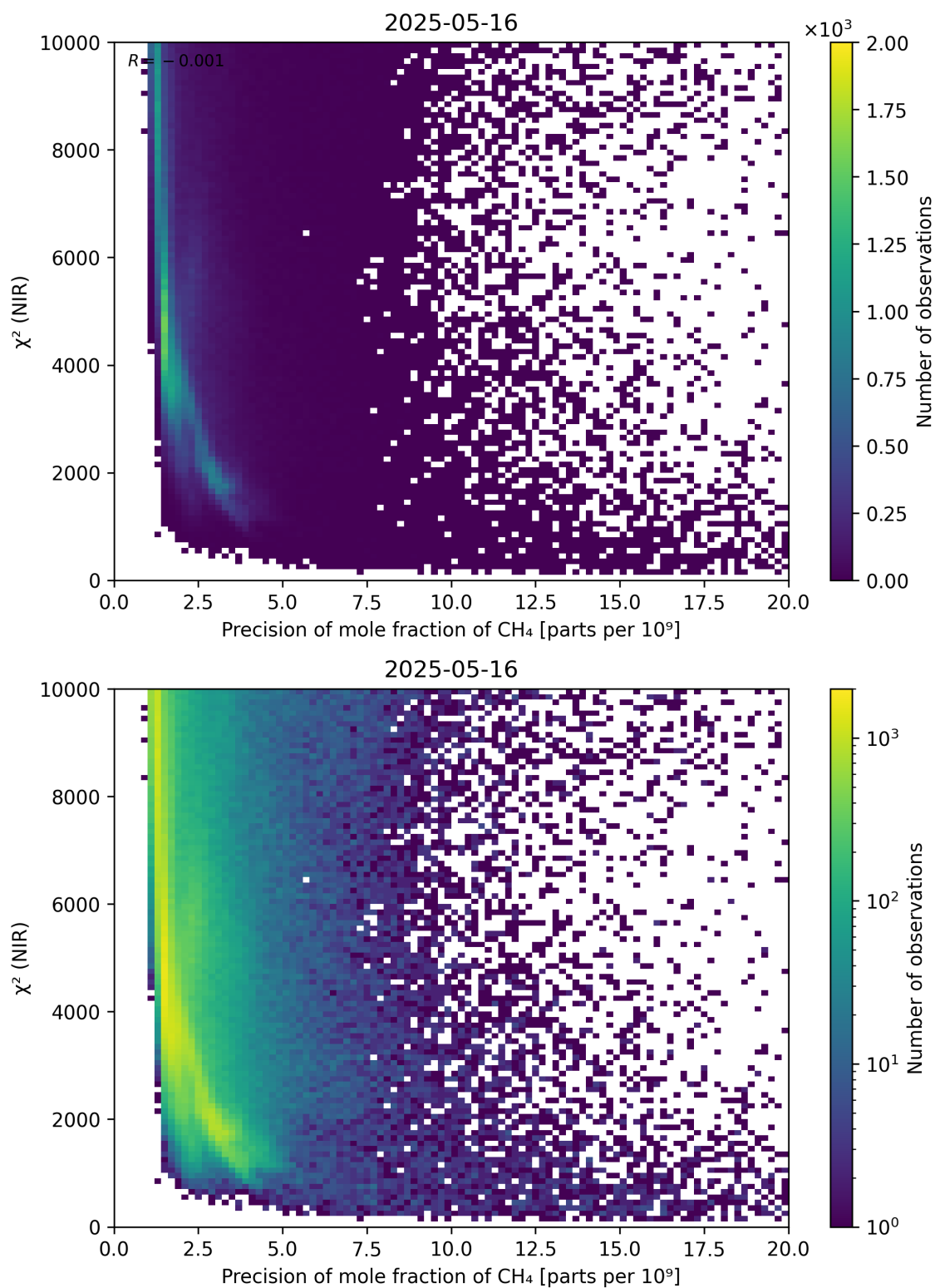
Figure 78: Scatter density plot of “Precision of mole fraction of \text{CH}_4 ” against “ \chi^2 (NIR)” for 2025-05-15 to 2025-05-17.
