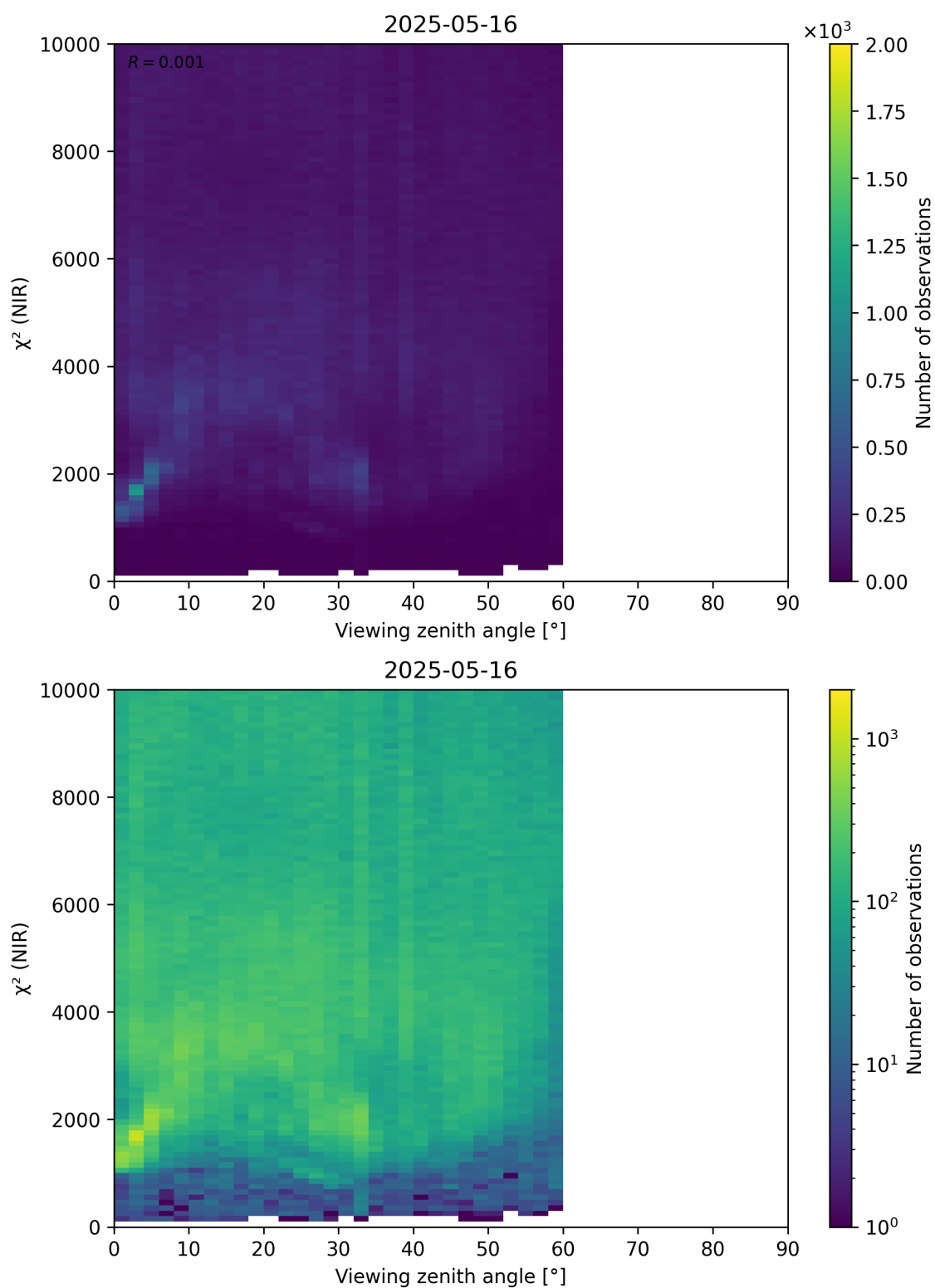
Figure 105: Scatter density plot of “Viewing zenith angle” against “ \chi^2 (NIR)” for 2025-05-15 to 2025-05-17.
