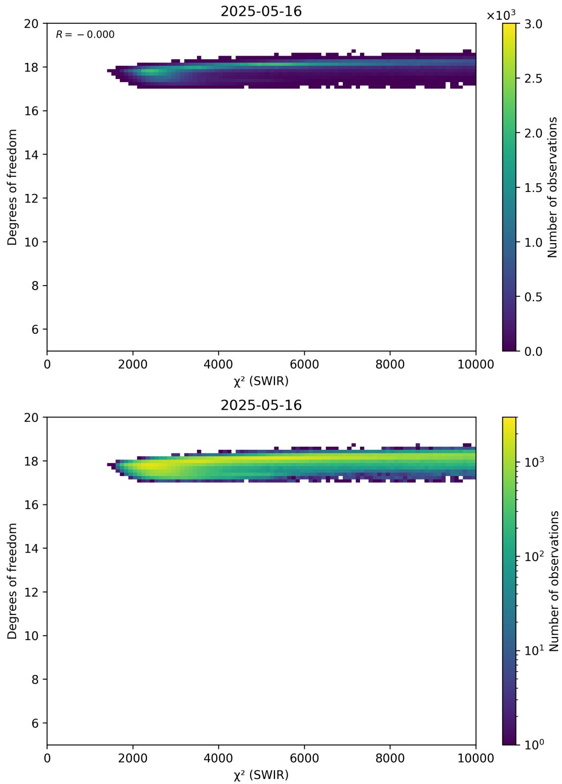
Figure 48: Scatter density plot of “ \chi^2 (SWIR)” against “Degrees of freedom” for 2025-05-15 to 2025-05-17.
