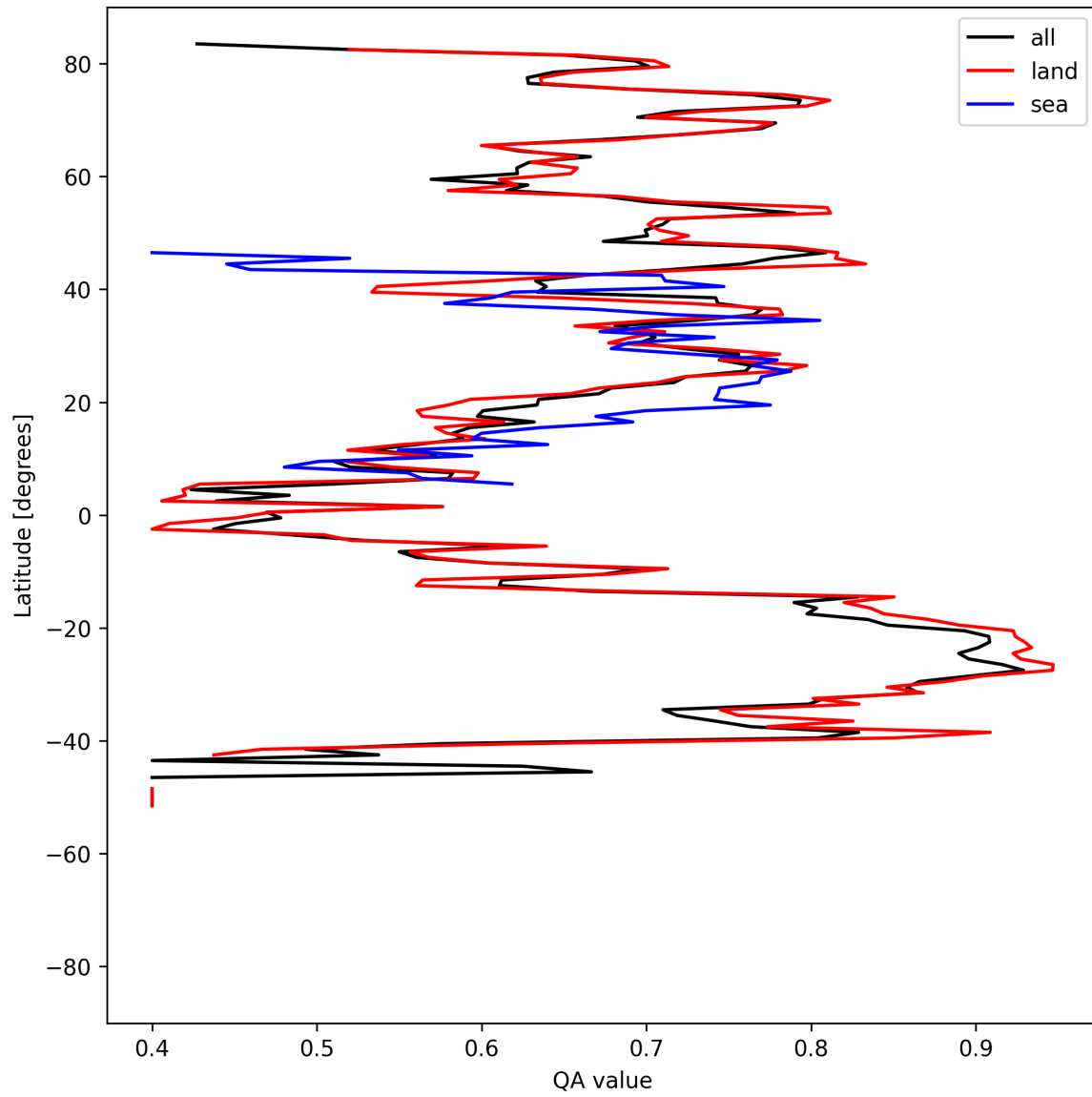
Figure 11: Zonal average of “QA value” for 2025-05-15 to 2025-05-17.
