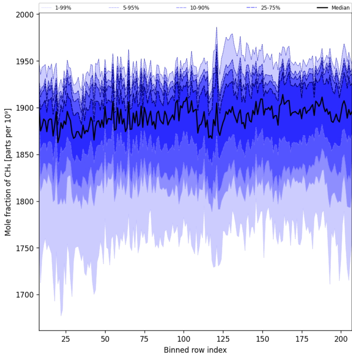
Figure 34: Along track statistics of “Mole fraction of CH 4 ” for 2025-05-15 to 2025-05-17
