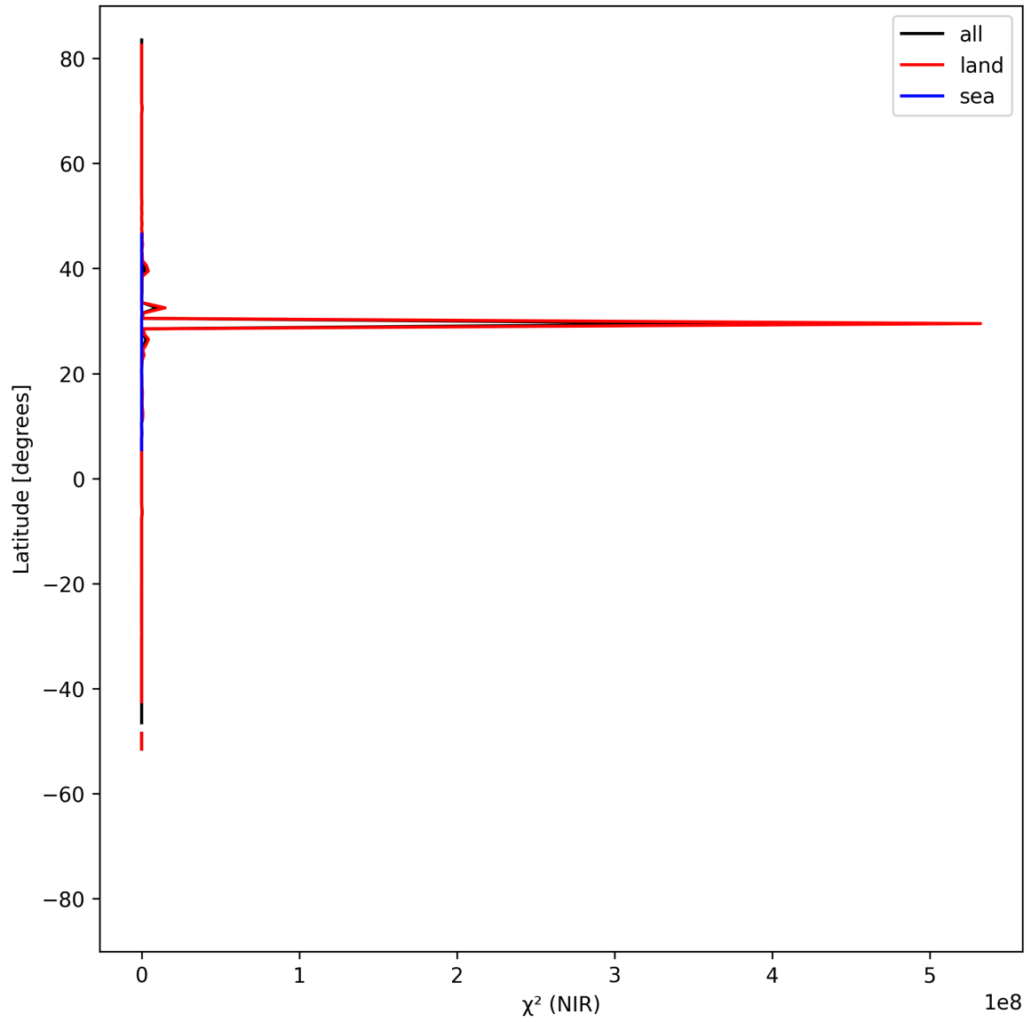
Figure 18: Zonal average of “ \chi^2 (NIR)” for 2025-05-15 to 2025-05-17.
