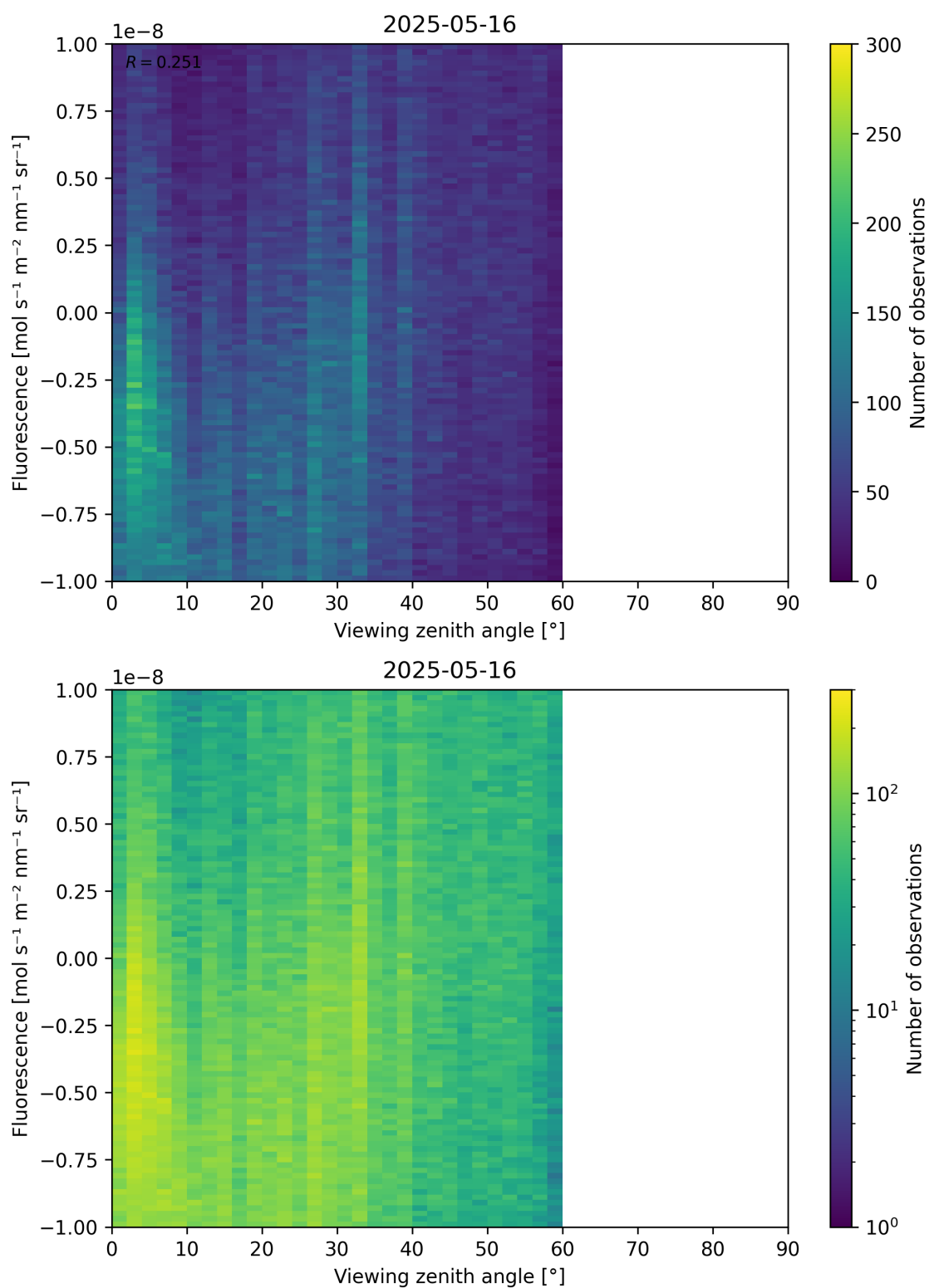
Figure 108: Scatter density plot of “Viewing zenith angle” against “Fluorescence” for 2025-05-15 to 2025-05-17.
