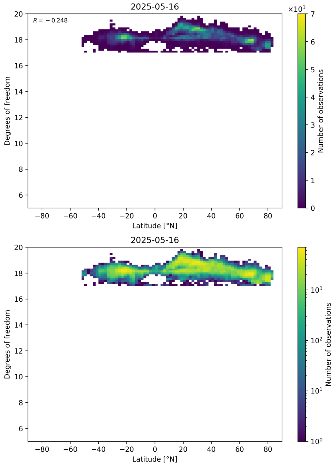
Figure 55: Scatter density plot of “Latitude” against “Degrees of freedom” for 2025-05-15 to 2025-05-17.
