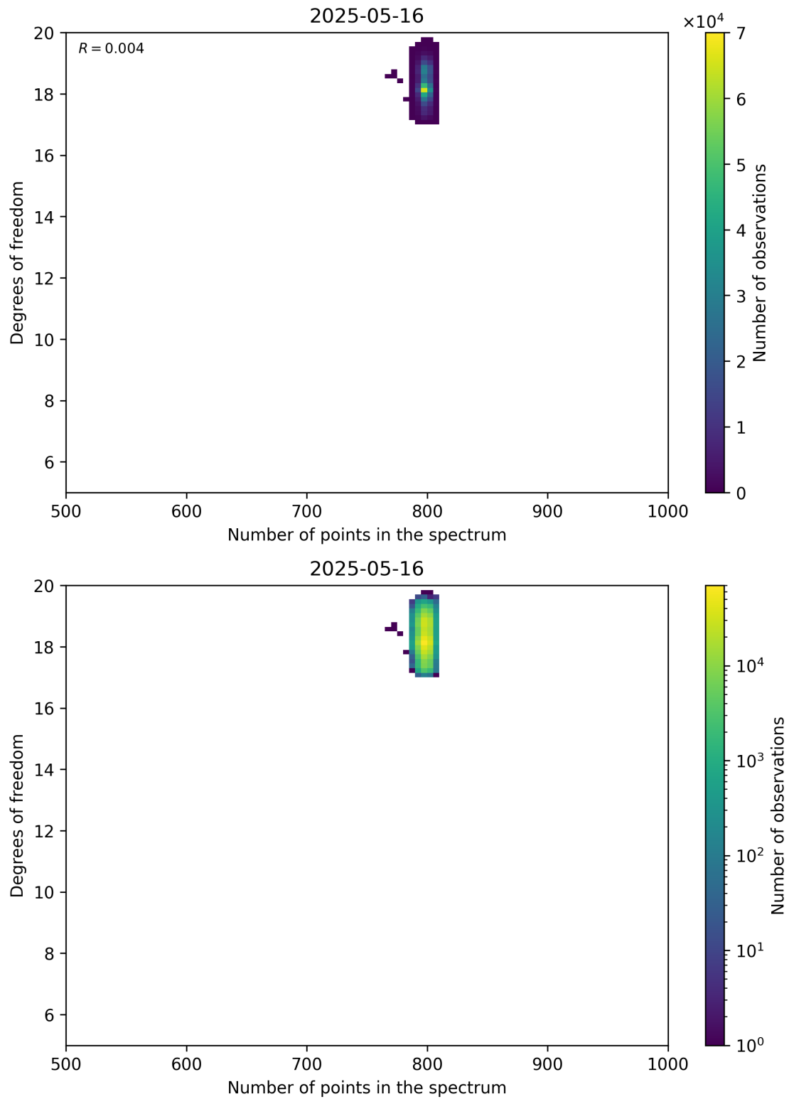
Figure 90: Scatter density plot of “Number of points in the spectrum” against “Degrees of freedom” for 2025-05-15 to 2025-05-17.
