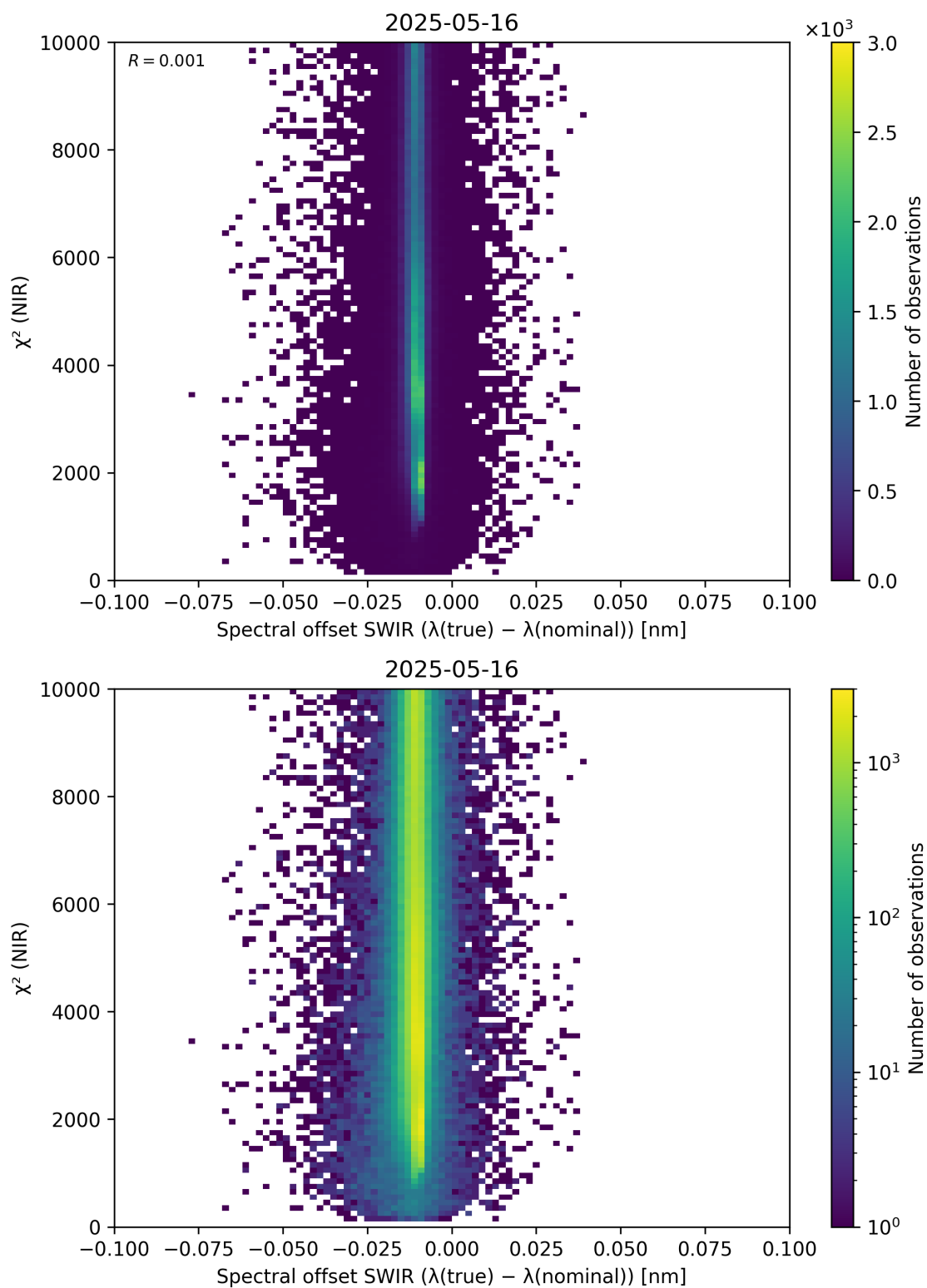
Figure 117: Scatter density plot of “Spectral offset SWIR ( \lambda_{\text{true}} - \lambda_{\text{nominal}} )” against “ \chi^2 (NIR)” for 2025-05-15 to 2025-05-17.
