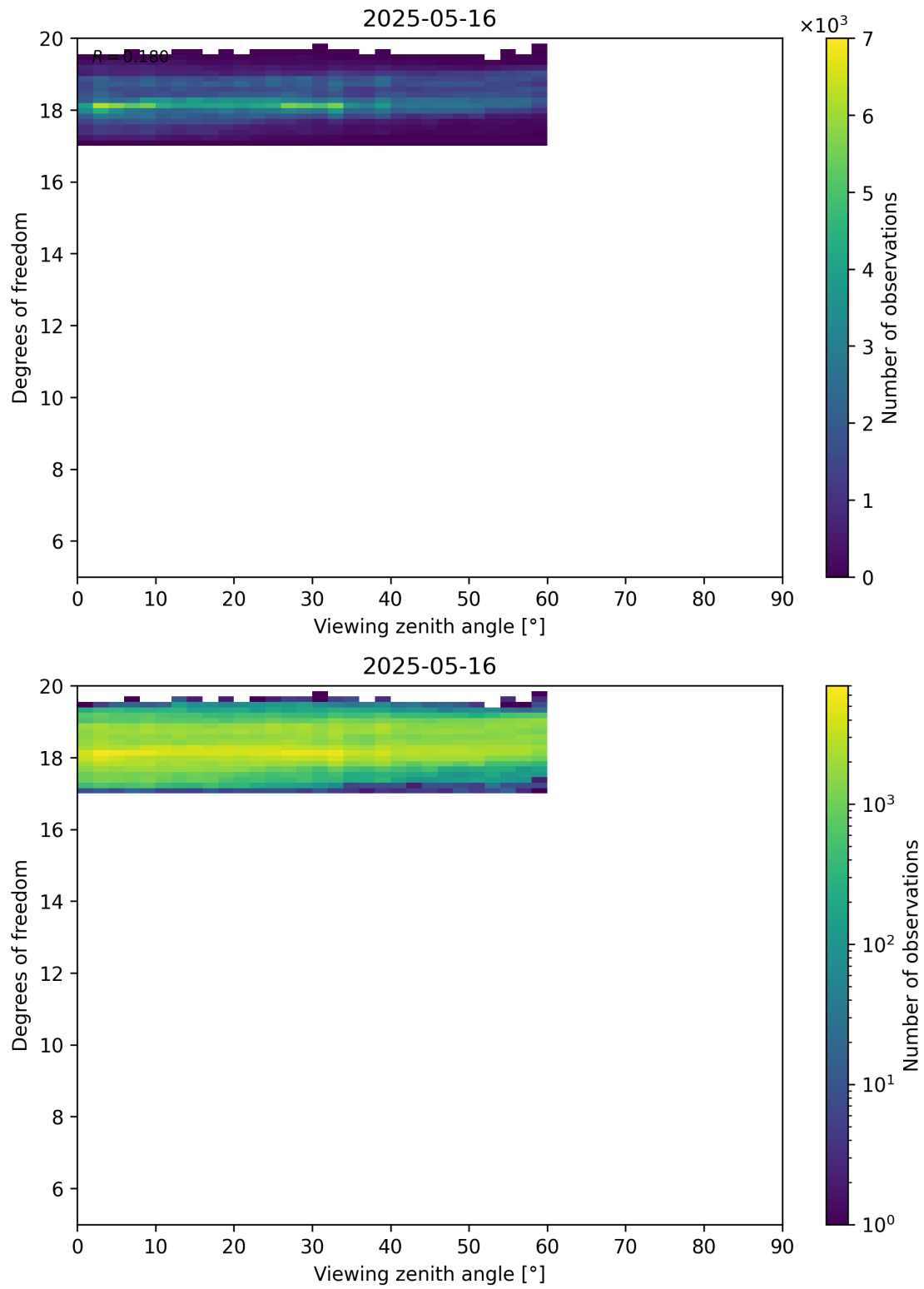
Figure 107: Scatter density plot of “Viewing zenith angle” against “Degrees of freedom” for 2025-05-15 to 2025-05-17.
