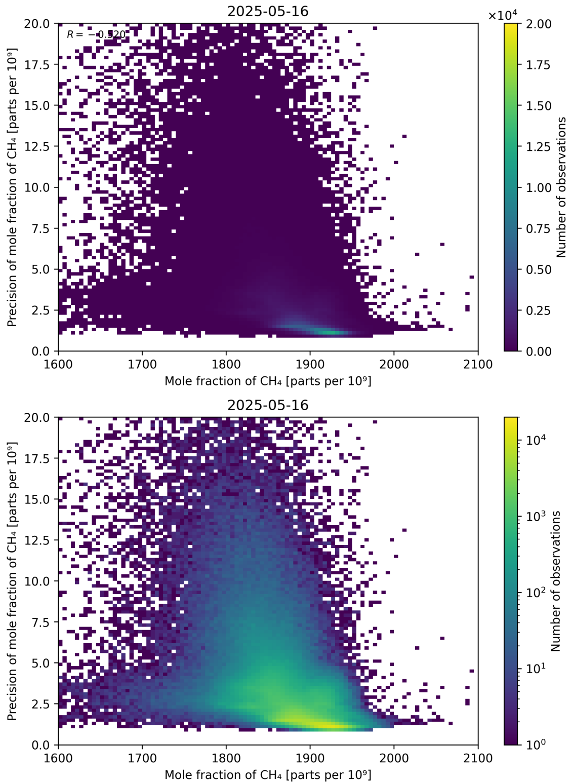
Figure 75: Scatter density plot of “Mole fraction of CH 4 ” against “Precision of mole fraction of CH 4 ” for 2025-05-15 to 2025-05-17.
