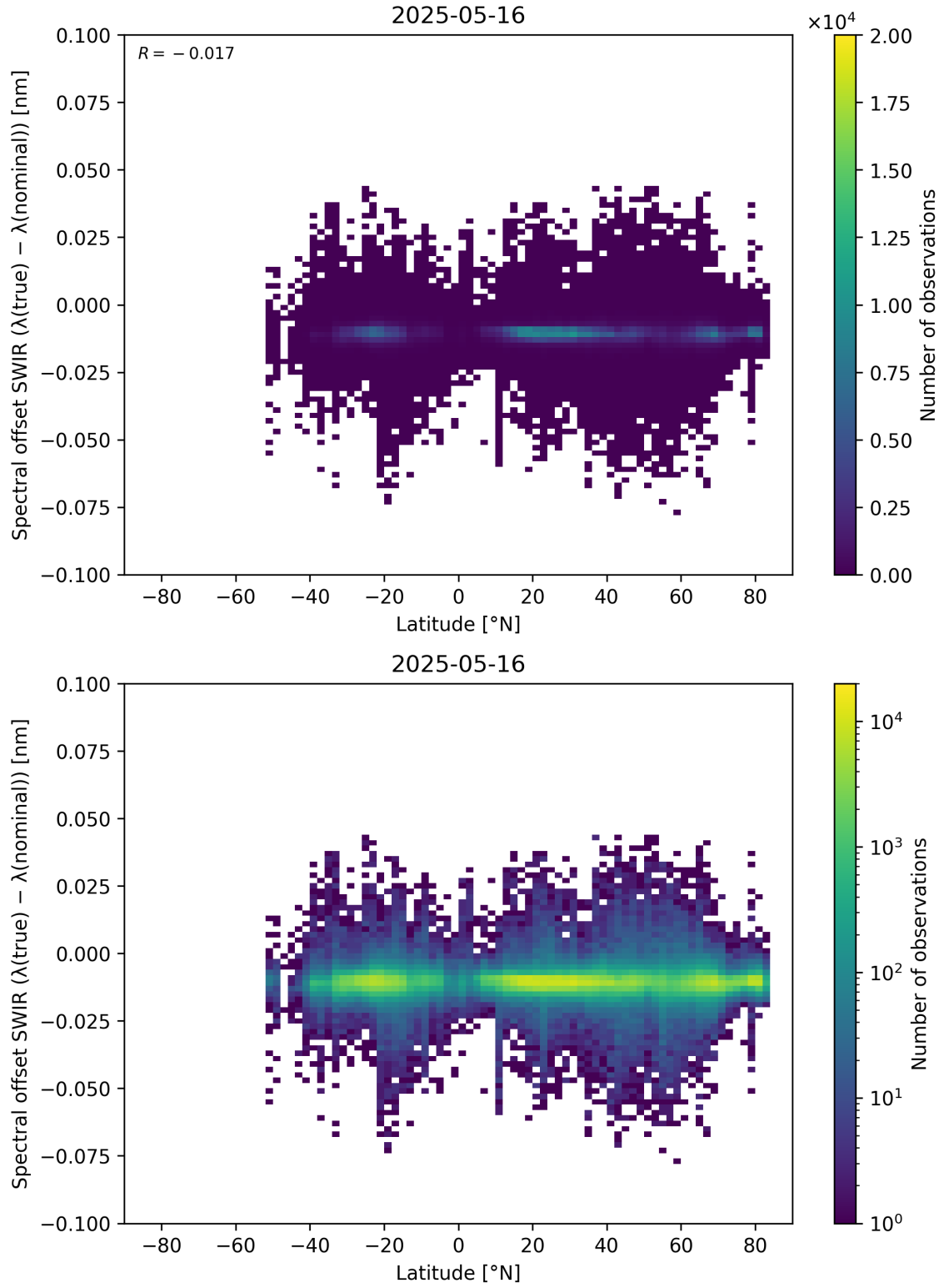
Figure 62: Scatter density plot of “Latitude” against “Spectral offset SWIR ( \lambda_{\text{true}} - \lambda_{\text{nominal}} )” for 2025-05-15 to 2025-05-17.
