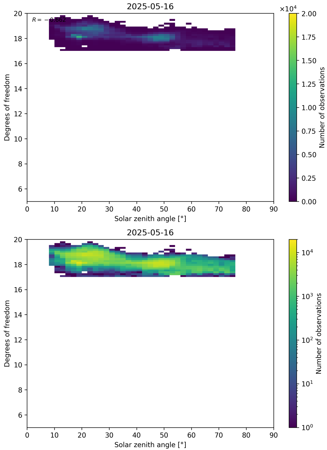
Figure 96: Scatter density plot of “Solar zenith angle” against “Degrees of freedom” for 2025-05-15 to 2025-05-17.
