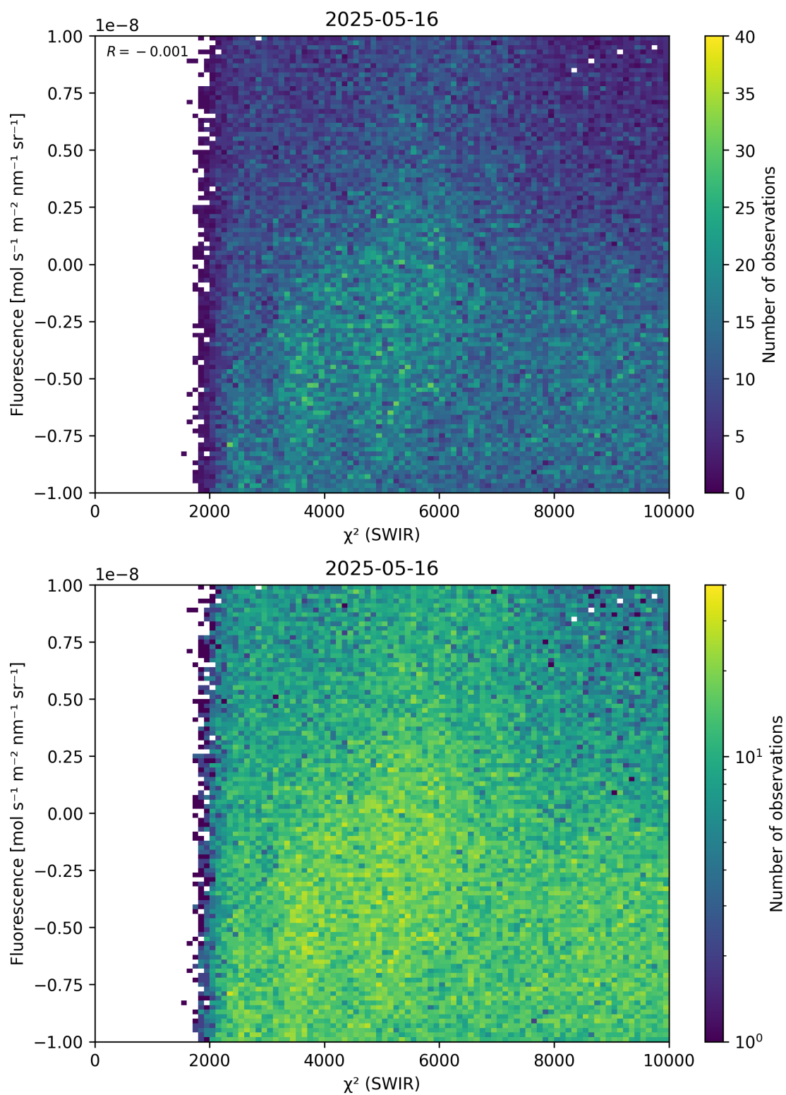
Figure 49: Scatter density plot of “ \chi^2 (SWIR)” against “Fluorescence” for 2025-05-15 to 2025-05-17.
