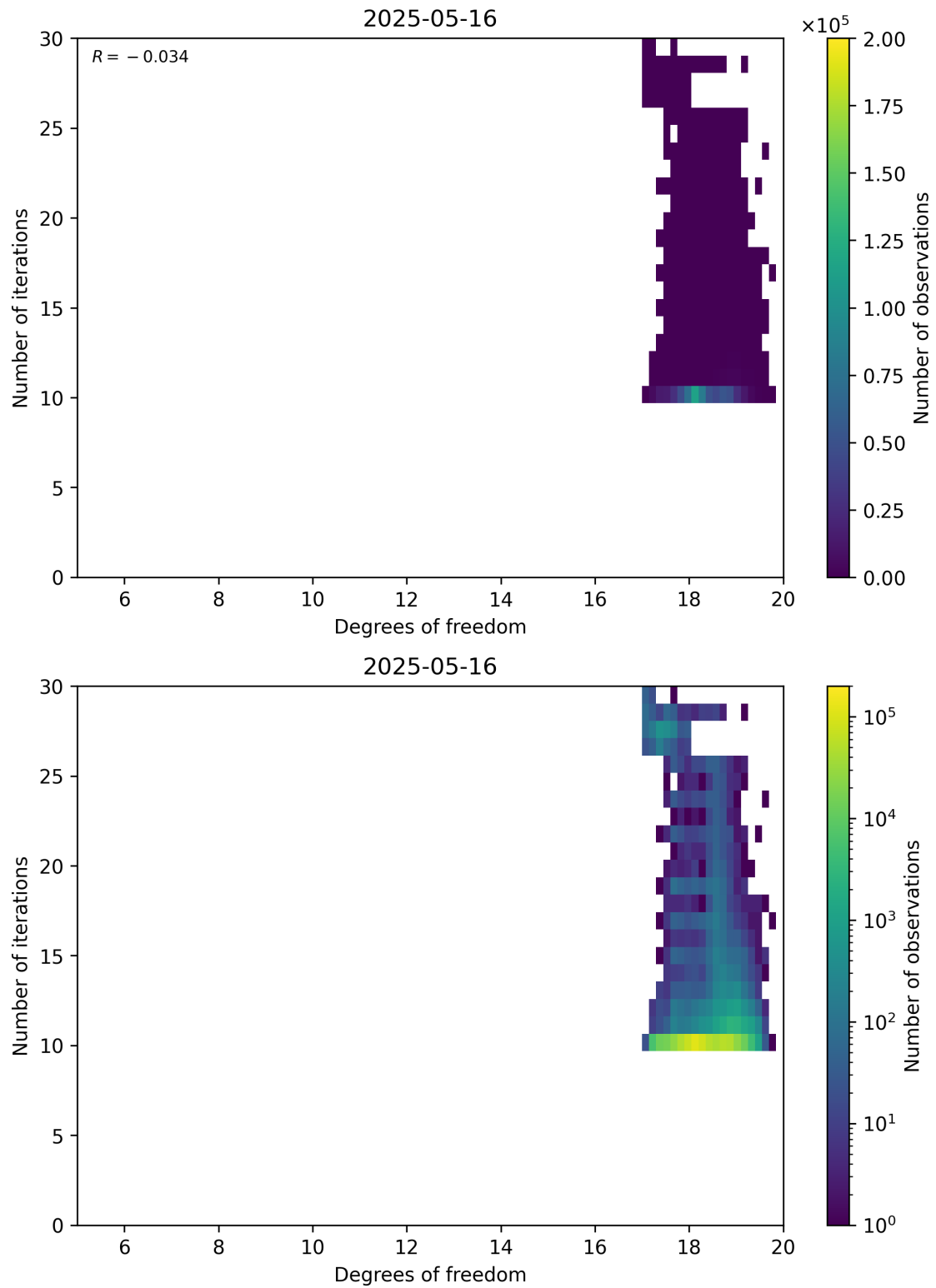
Figure 52: Scatter density plot of “Degrees of freedom” against “Number of iterations” for 2025-05-15 to 2025-05-17.
