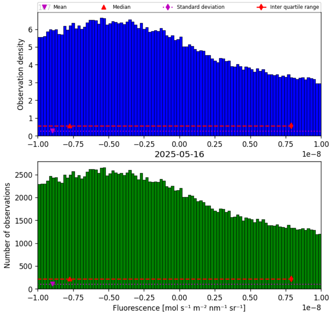
Figure 32: Histogram of “Fluorescence” for 2025-05-15 to 2025-05-17
