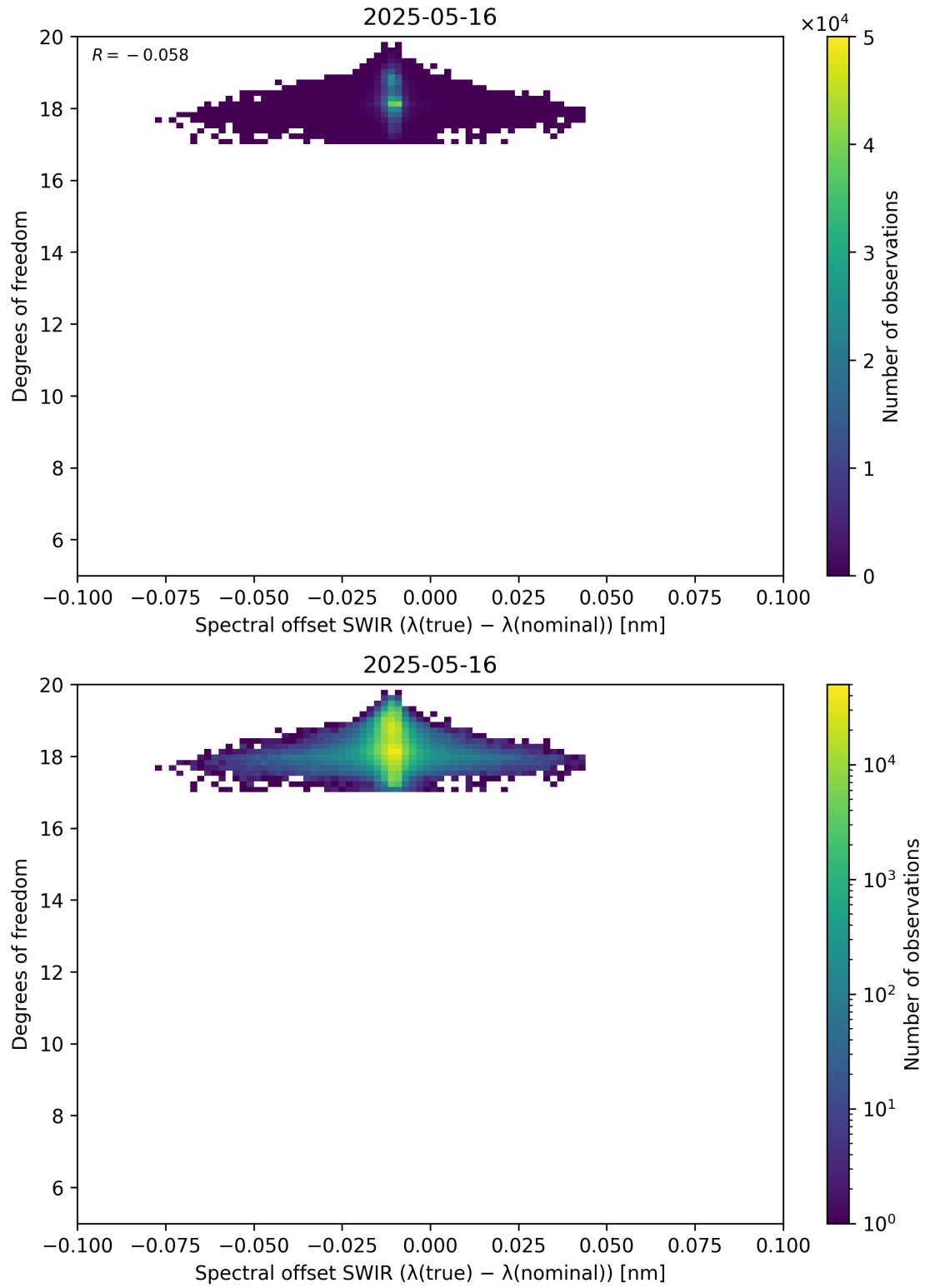
Figure 119: Scatter density plot of “Spectral offset SWIR ( \lambda_{\text{true}} - \lambda_{\text{nominal}} )” against “Degrees of freedom” for 2025-05-15 to 2025-05-17.
