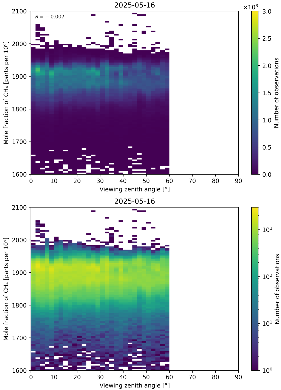
Figure 110: Scatter density plot of “Viewing zenith angle” against “Mole fraction of CH 4 ” for 2025-05-15 to 2025-05-17.
