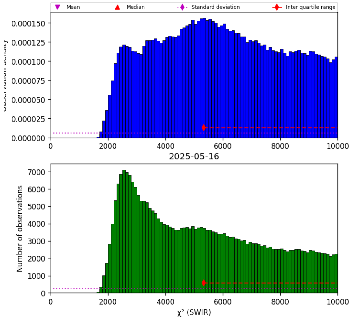
Figure 28: Histogram of “ \chi^2 (SWIR)” for 2025-05-15 to 2025-05-17
