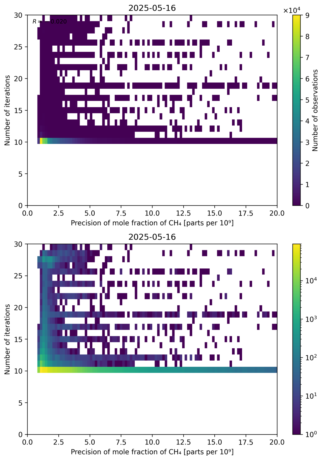
Figure 83: Scatter density plot of “Precision of mole fraction of CH 4 ” against “Number of iterations” for 2025-05-15 to 2025-05-17.
