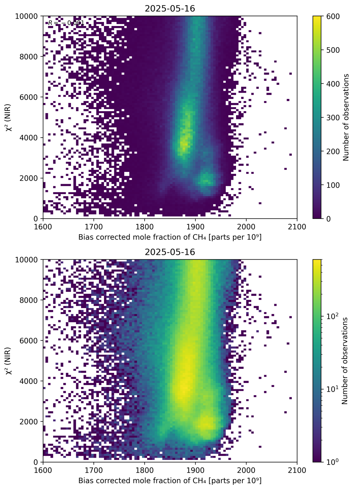
Figure 63: Scatter density plot of “Bias corrected mole fraction of \text{CH}_4 ” against “ \chi^2 (NIR)” for 2025-05-15 to 2025-05-17.
