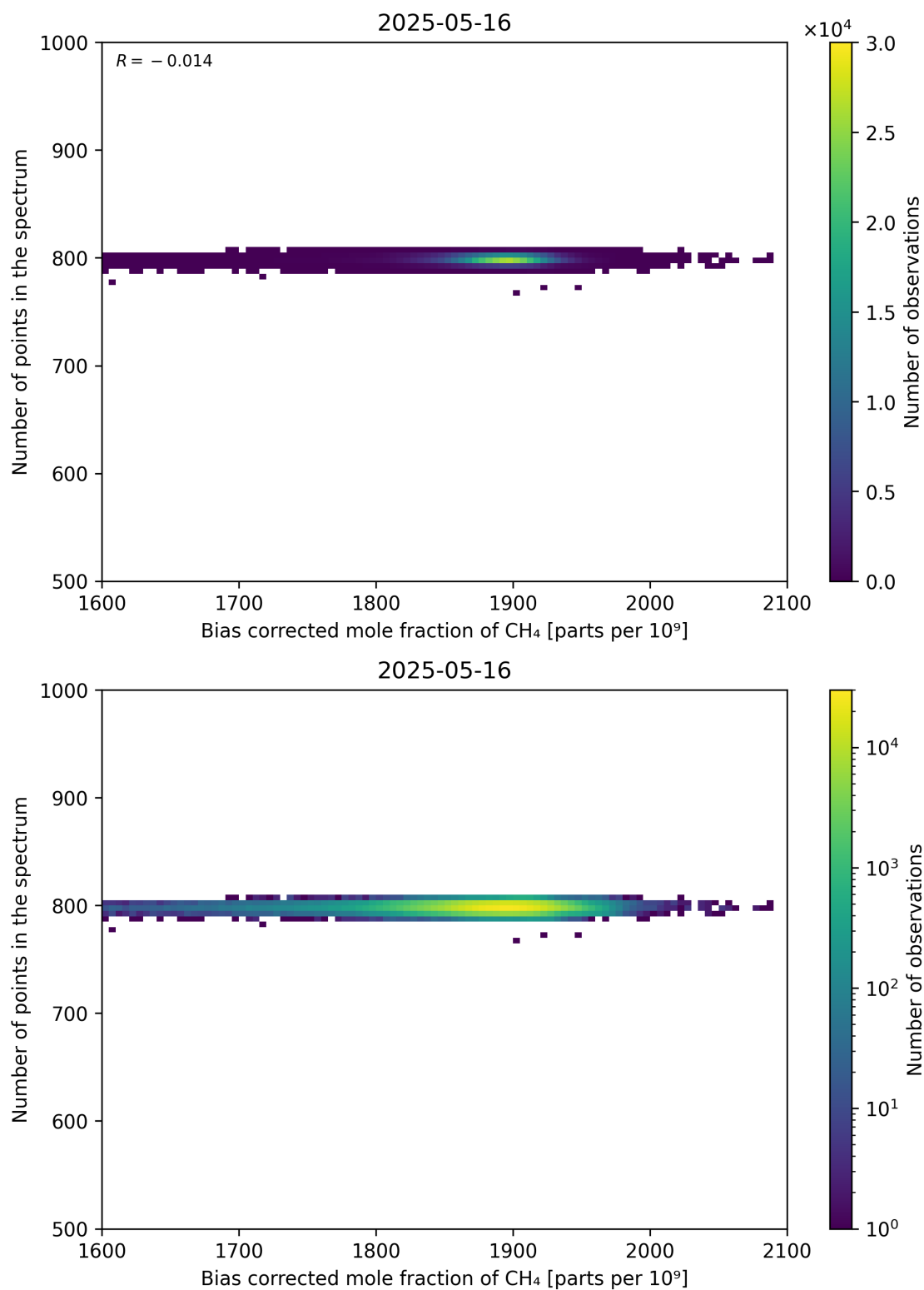
Figure 68: Scatter density plot of “Bias corrected mole fraction of CH 4 ” against “Number of points in the spectrum” for 2025-05-15 to 2025-05-17.
