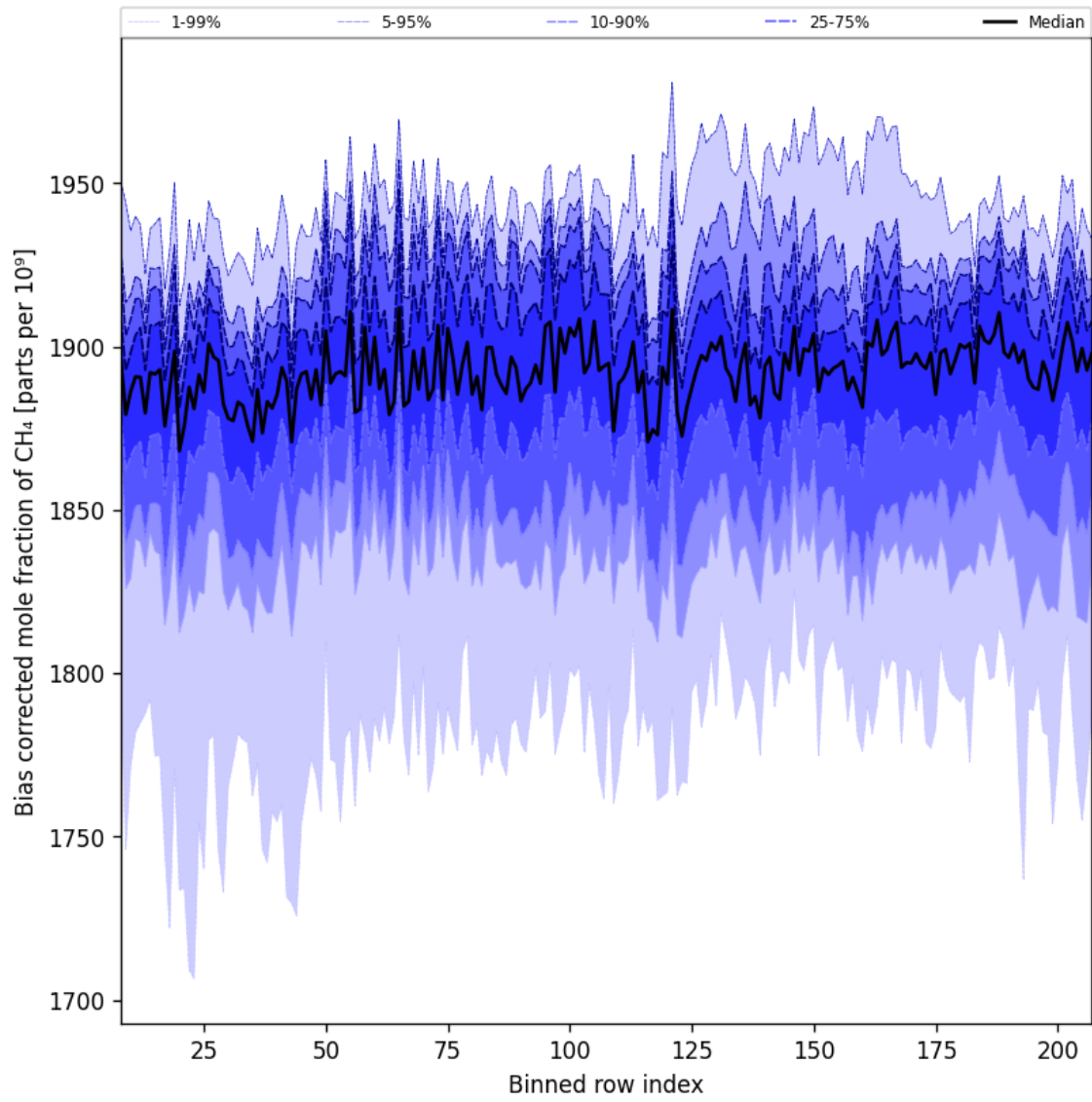
Figure 36: Along track statistics of “Bias corrected mole fraction of CH 4 ” for 2025-05-15 to 2025-05-17
