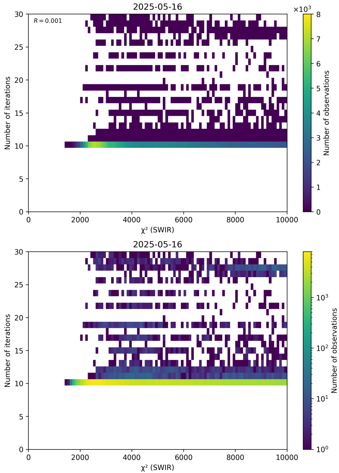
Figure 50: Scatter density plot of “ \chi^2 (SWIR)” against “Number of iterations” for 2025-05-15 to 2025-05-17.
