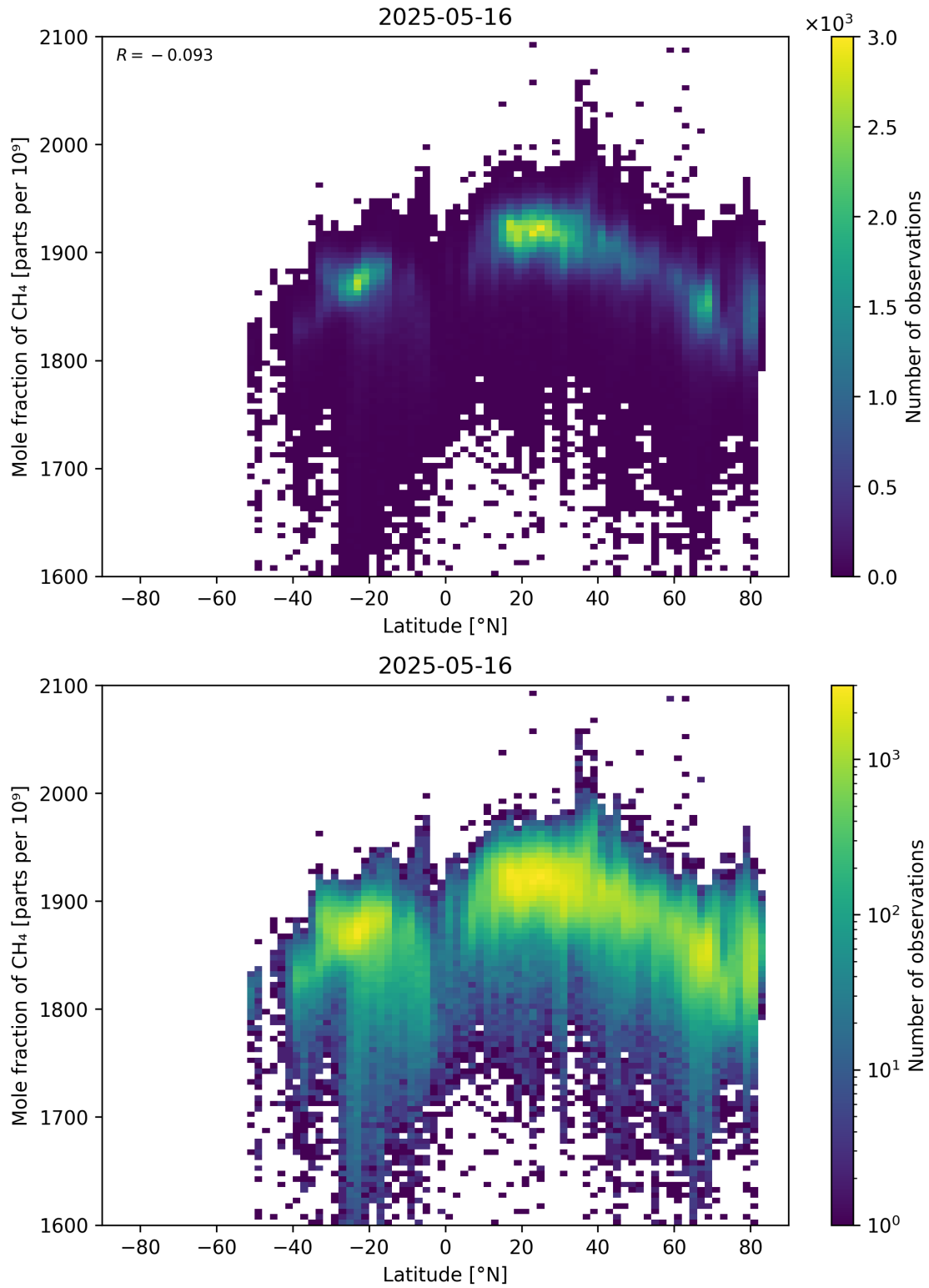
Figure 57: Scatter density plot of “Latitude” against “Mole fraction of CH 4 ” for 2025-05-15 to 2025-05-17.
