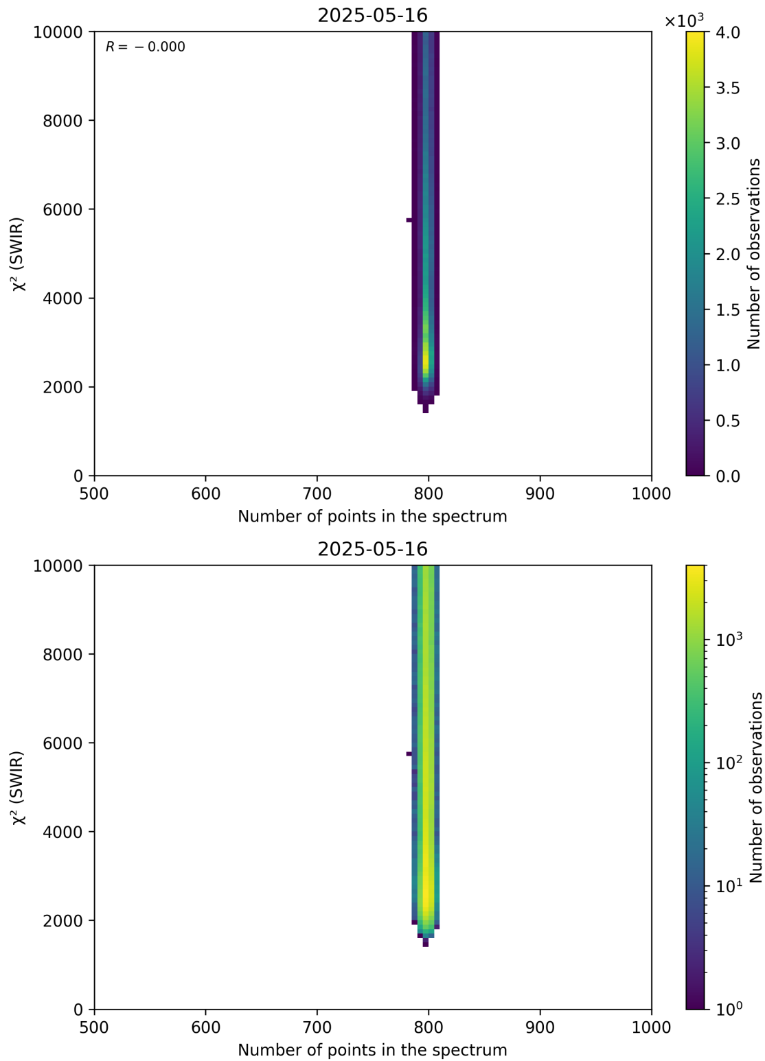
Figure 89: Scatter density plot of “Number of points in the spectrum” against “ \chi^2 (SWIR)” for 2025-05-15 to 2025-05-17.
