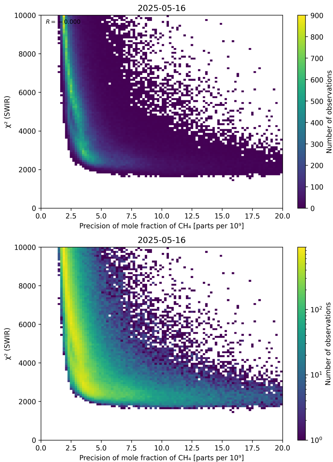
Figure 79: Scatter density plot of “Precision of mole fraction of CH 4 ” against “ \chi^2 (SWIR)” for 2025-05-15 to 2025-05-17.
