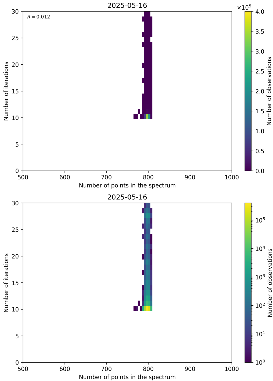
Figure 92: Scatter density plot of “Number of points in the spectrum” against “Number of iterations” for 2025-05-15 to 2025-05-17.
