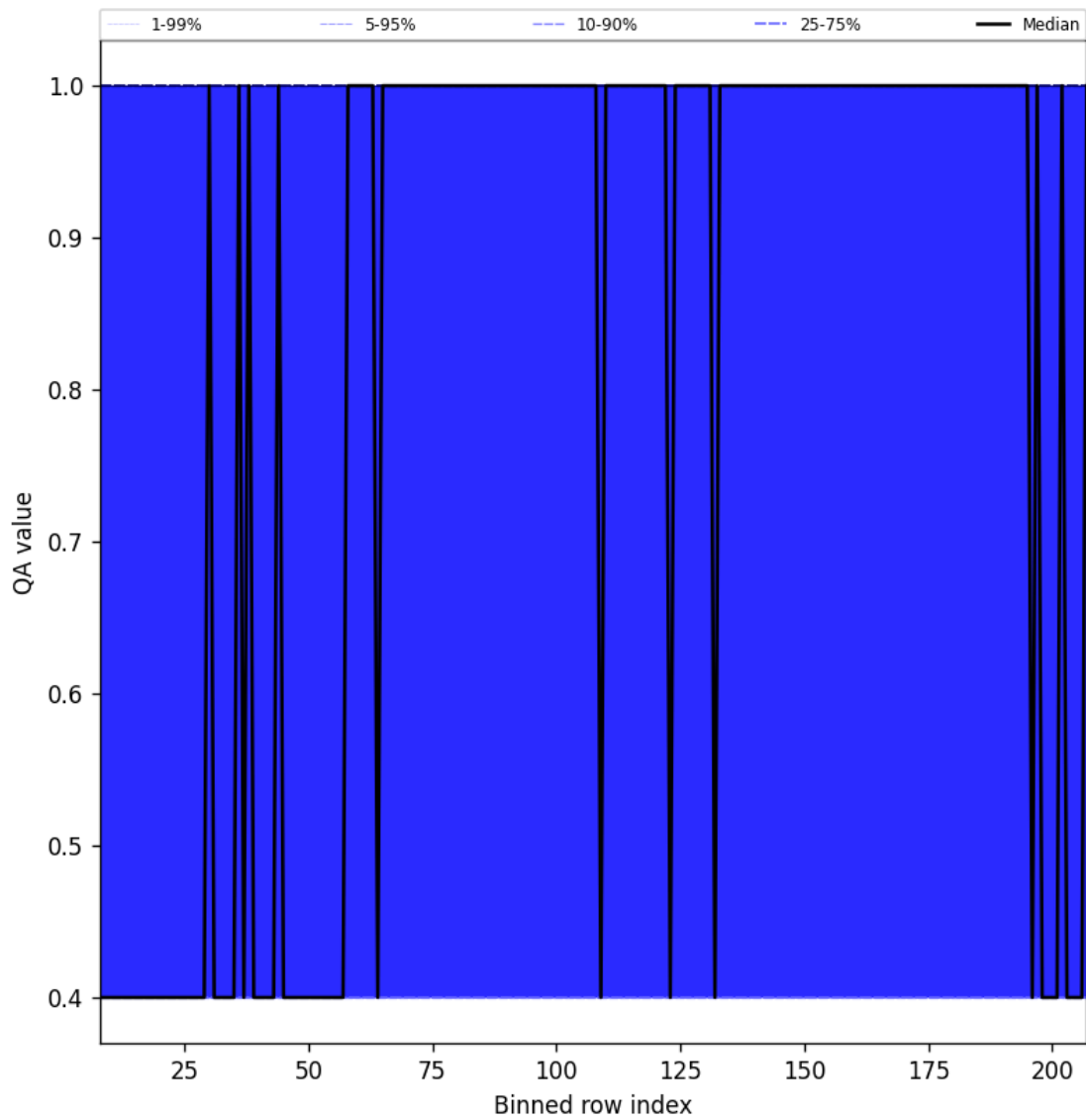
Figure 33: Along track statistics of “QA value” for 2025-05-15 to 2025-05-17
