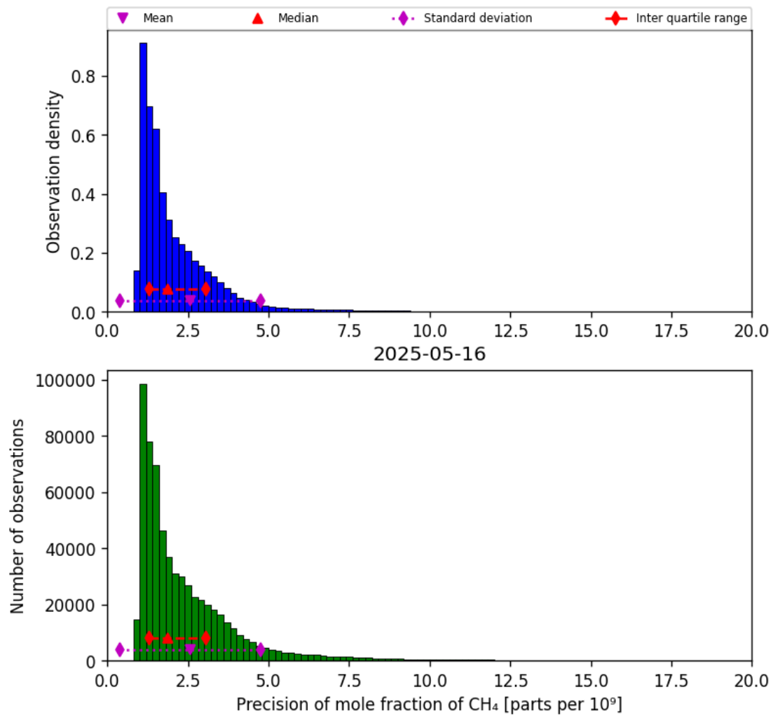
Figure 24: Histogram of “Precision of mole fraction of CH 4 ” for 2025-05-15 to 2025-05-17
