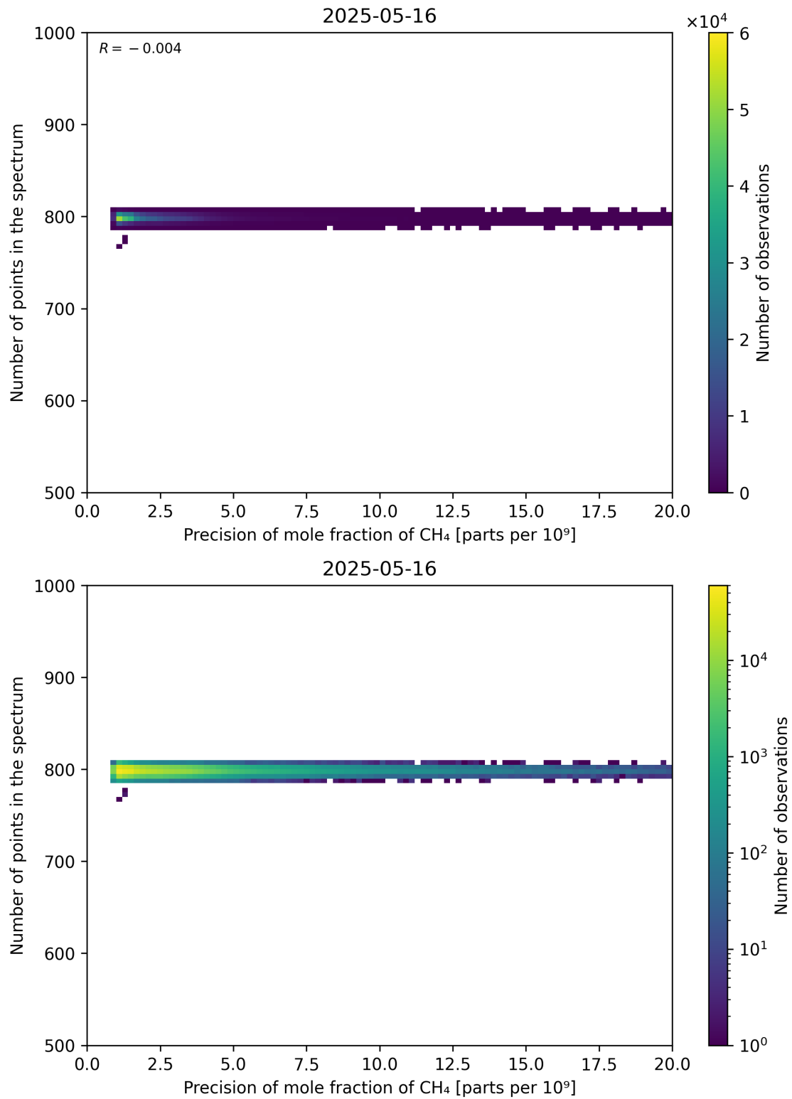
Figure 84: Scatter density plot of “Precision of mole fraction of CH 4 ” against “Number of points in the spectrum” for 2025-05-15 to 2025-05-17.
