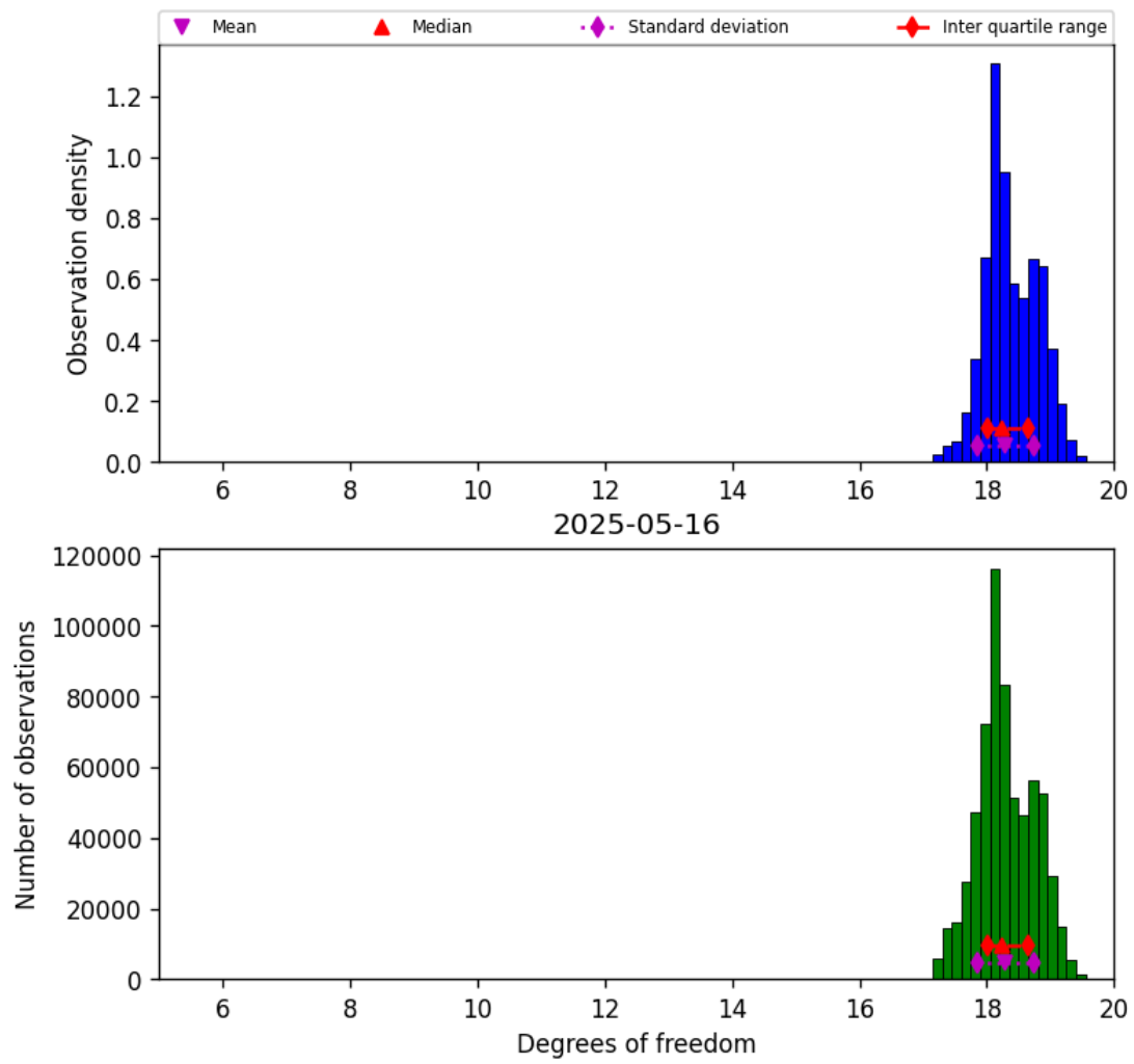
Figure 30: Histogram of “Degrees of freedom” for 2025-05-15 to 2025-05-17
