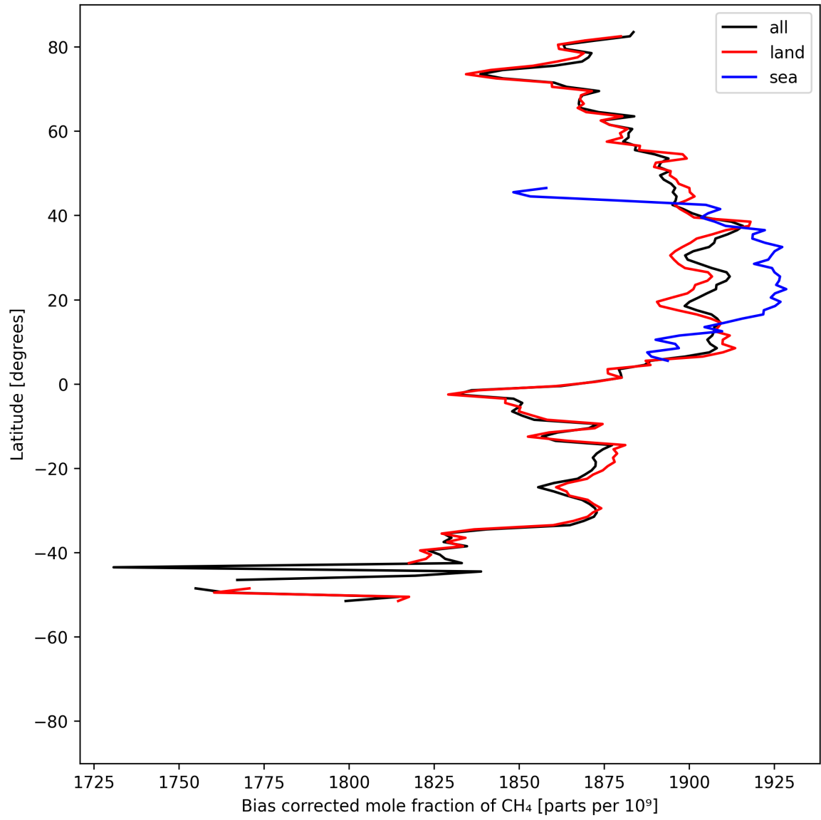
Figure 14: Zonal average of “Bias corrected mole fraction of CH 4 ” for 2025-05-15 to 2025-05-17.
