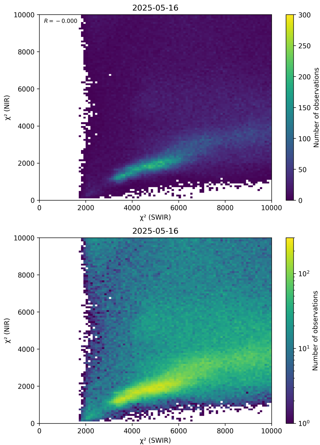
Figure 47: Scatter density plot of “ \chi^2 (SWIR)” against “ \chi^2 (NIR)” for 2025-05-15 to 2025-05-17.
