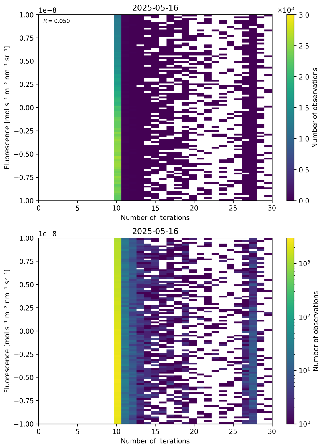
Figure 87: Scatter density plot of “Number of iterations” against “Fluorescence” for 2025-05-15 to 2025-05-17.
