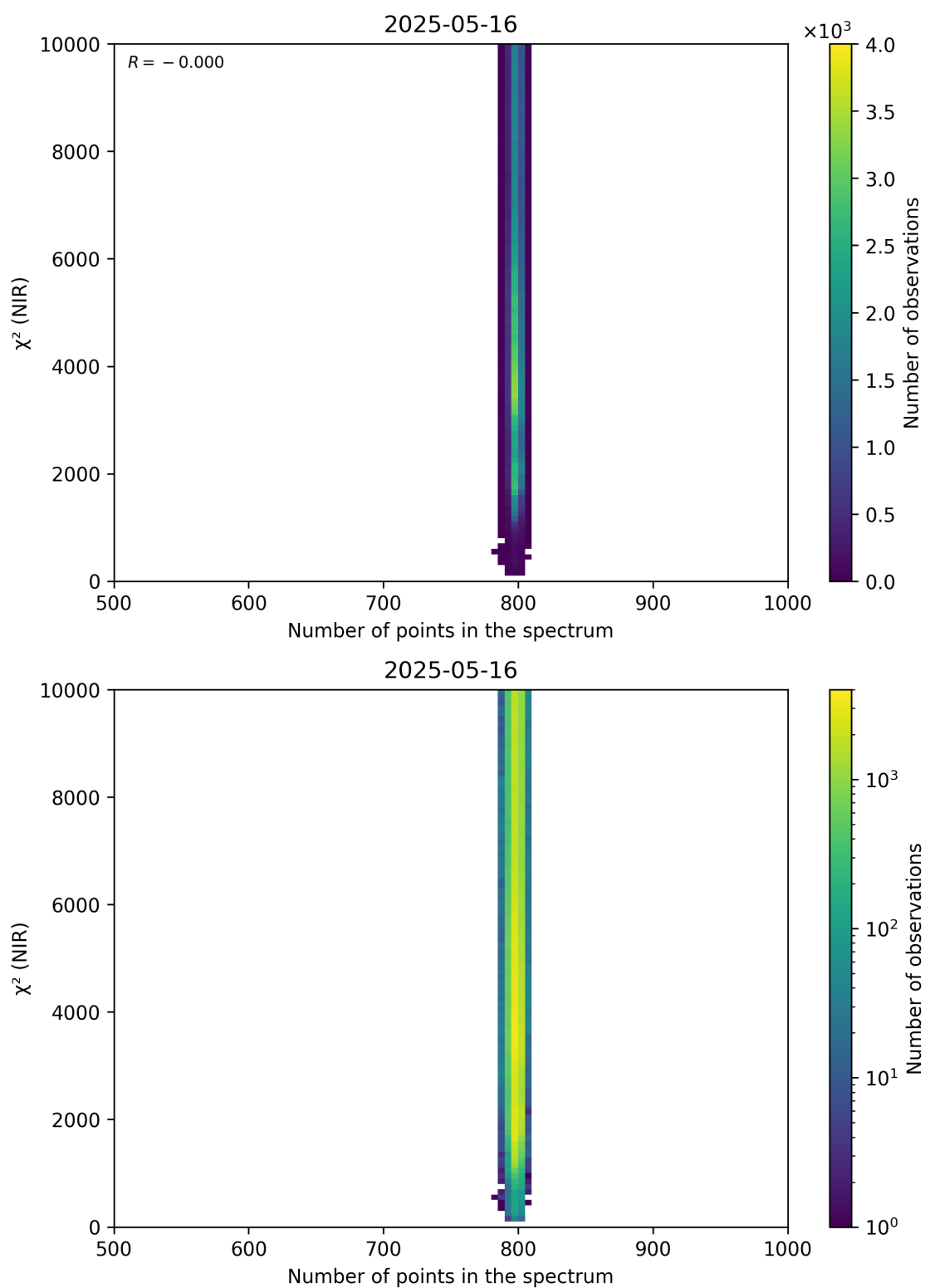
Figure 88: Scatter density plot of “Number of points in the spectrum” against “ \chi^2 (NIR)” for 2025-05-15 to 2025-05-17.
