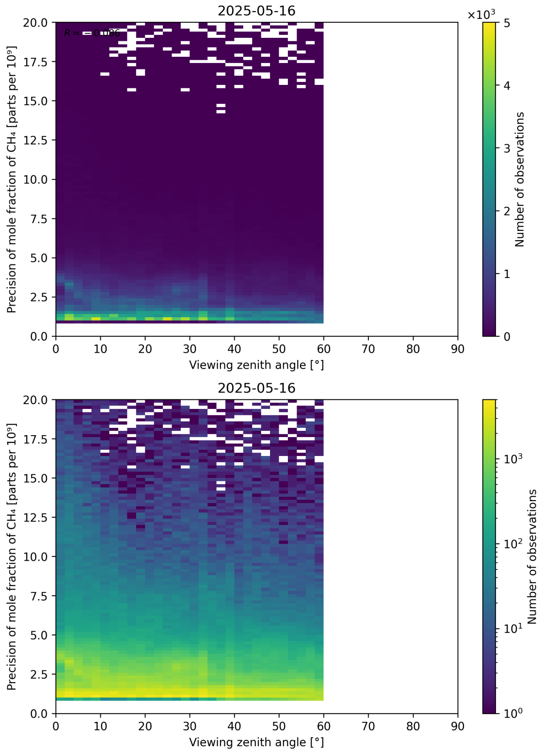
Figure 112: Scatter density plot of “Viewing zenith angle” against “Precision of mole fraction of CH 4 ” for 2025-05-15 to 2025-05-17.
