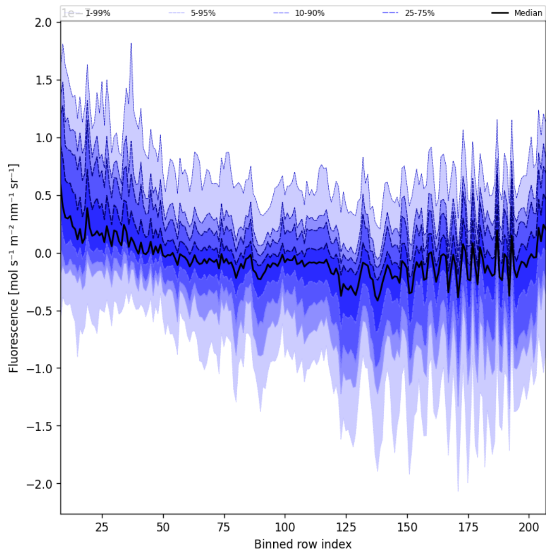
Figure 43: Along track statistics of “Fluorescence” for 2025-05-15 to 2025-05-17
