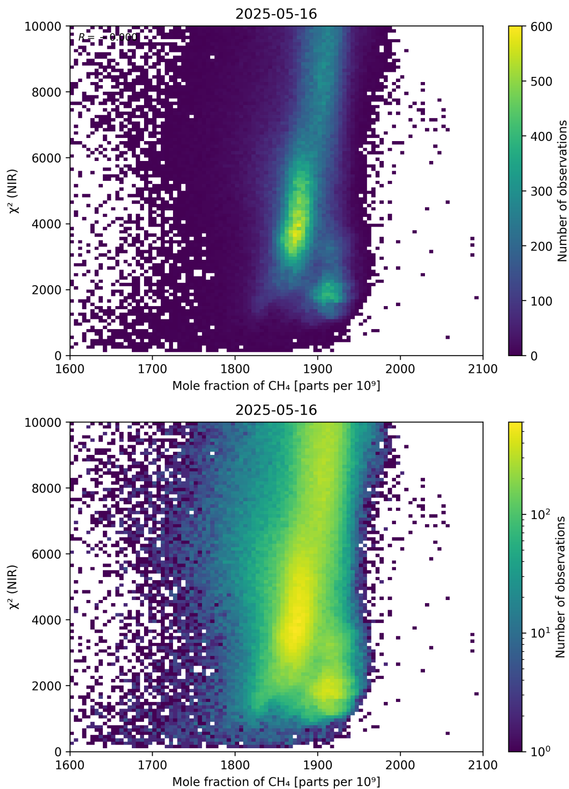
Figure 70: Scatter density plot of “Mole fraction of \text{CH}_4 ” against “ \chi^2 (NIR)” for 2025-05-15 to 2025-05-17.
