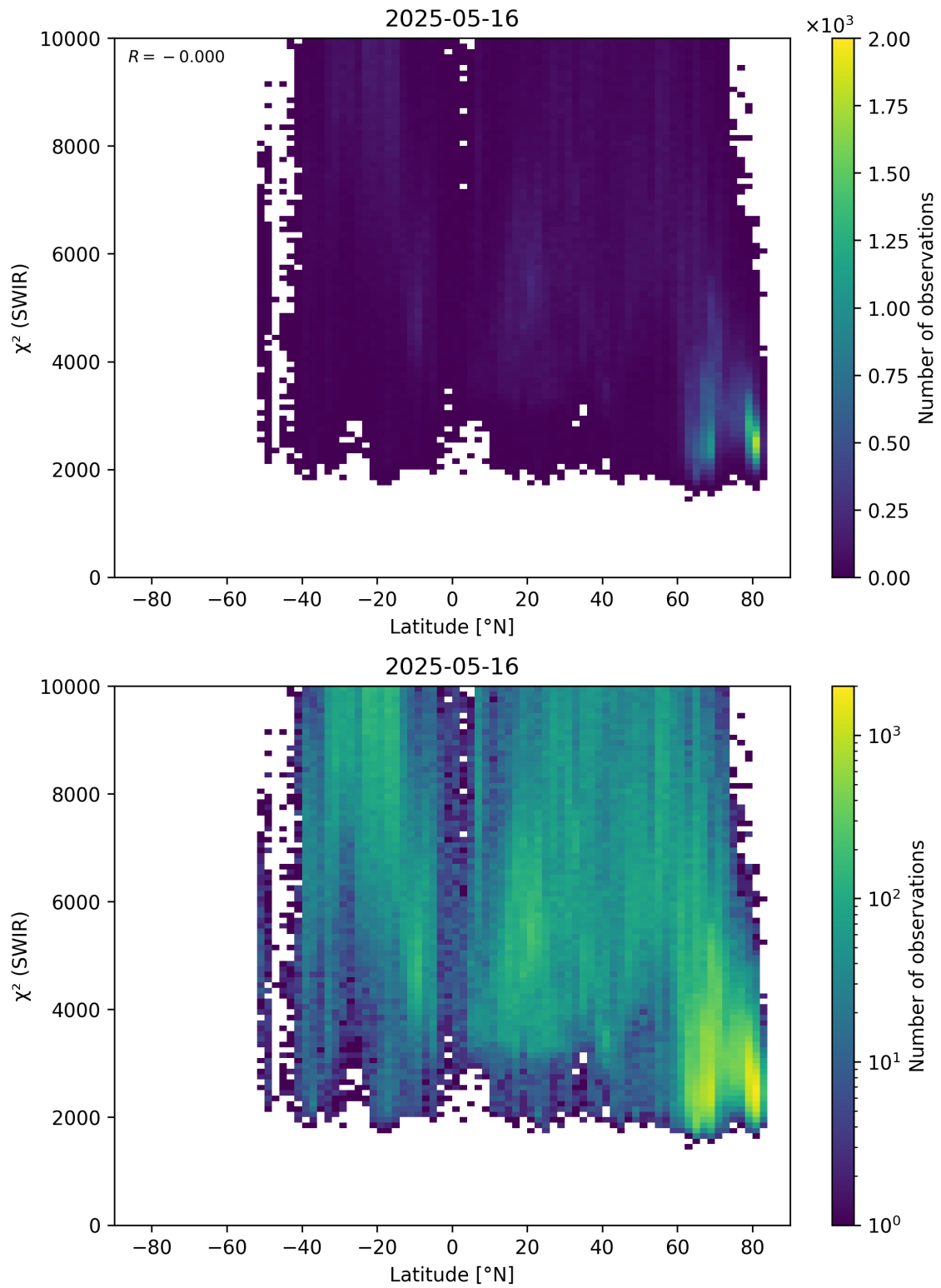
Figure 54: Scatter density plot of “Latitude” against “ \chi^2 (SWIR)” for 2025-05-15 to 2025-05-17.
