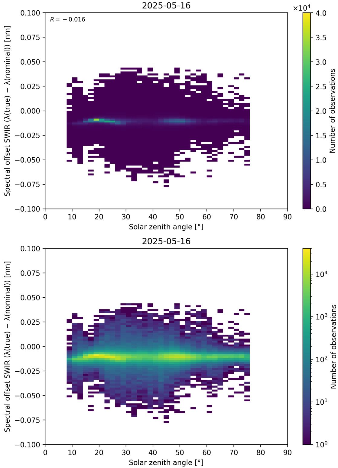
Figure 104: Scatter density plot of “Solar zenith angle” against “Spectral offset SWIR ( \lambda_{\text{true}} - \lambda_{\text{nominal}} )” for 2025-05-15 to 2025-05-17.
