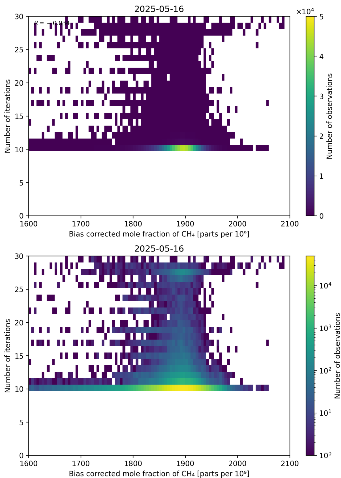
Figure 67: Scatter density plot of “Bias corrected mole fraction of CH 4 ” against “Number of iterations” for 2025-05-15 to 2025-05-17.
