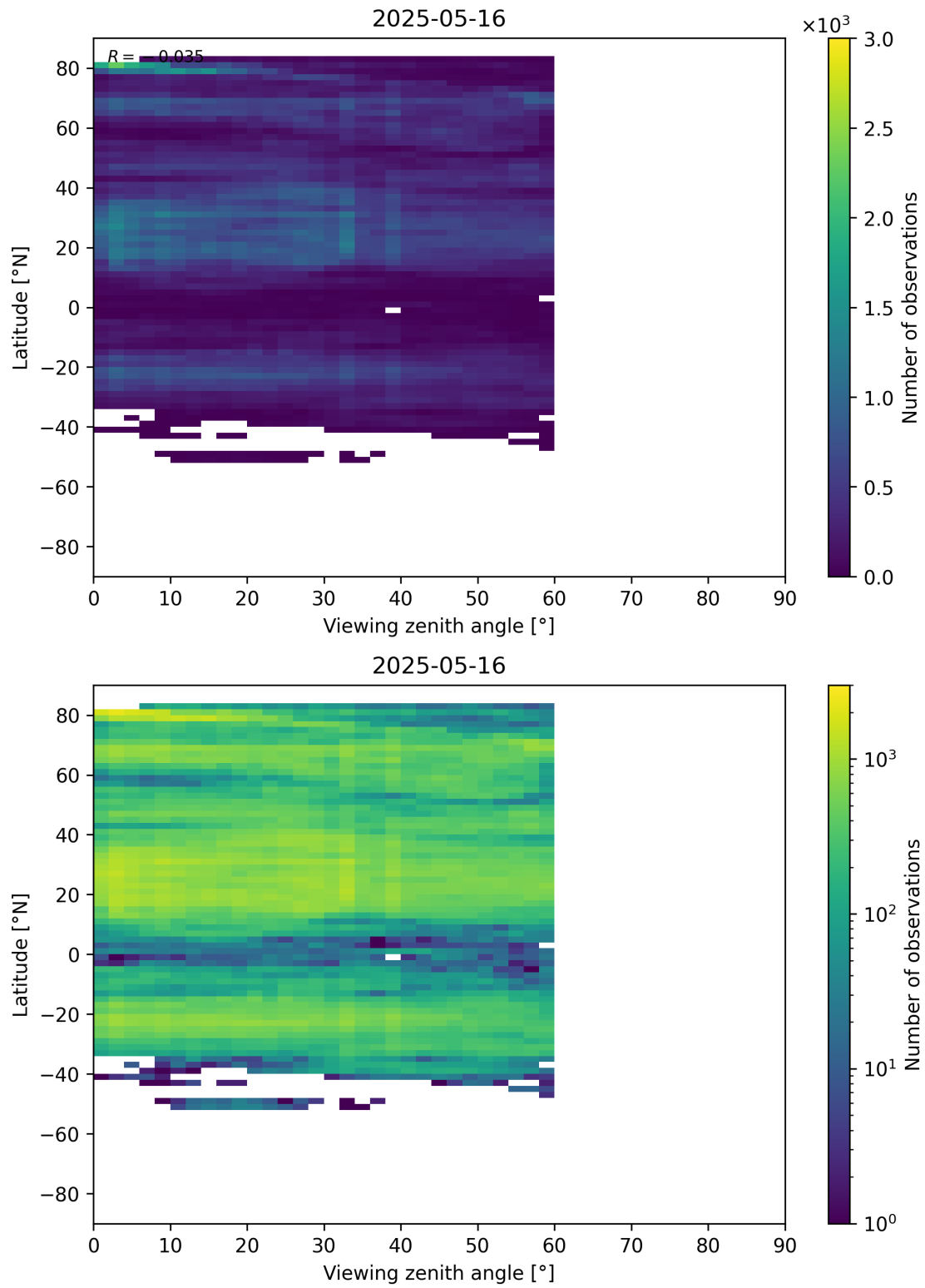
Figure 109: Scatter density plot of “Viewing zenith angle” against “Latitude” for 2025-05-15 to 2025-05-17.
