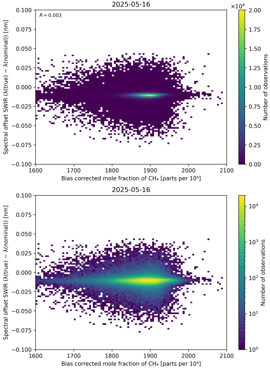
Figure 69: Scatter density plot of “Bias corrected mole fraction of \text{CH}_4 ” against “Spectral offset SWIR ( \lambda_{\text{true}} - \lambda_{\text{nominal}} )” for 2025-05-15 to 2025-05-17.
