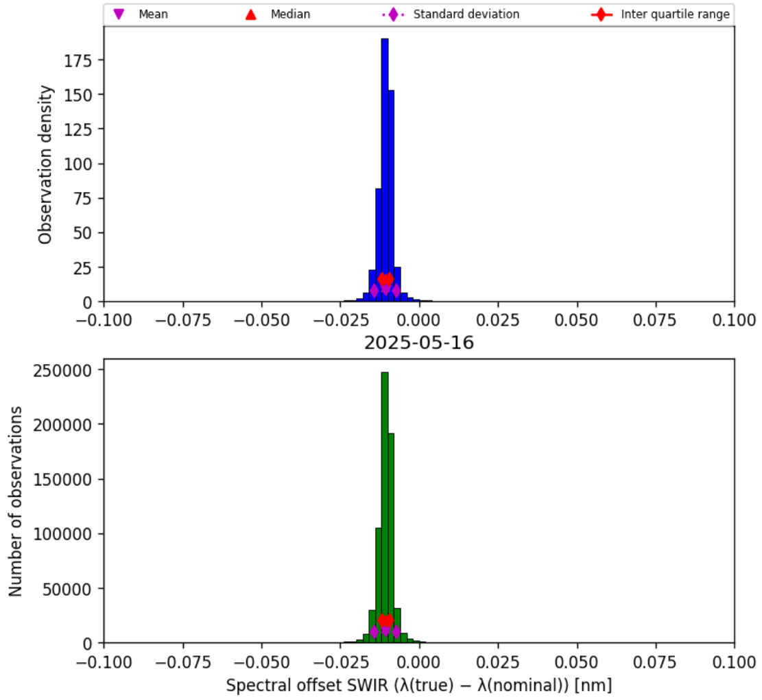
Figure 27: Histogram of “Spectral offset SWIR ( \lambda_{\text{true}} - \lambda_{\text{nominal}} )” for 2025-05-15 to 2025-05-17
