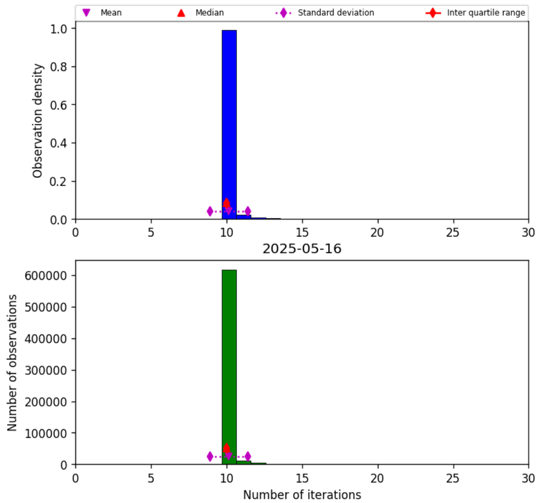
Figure 31: Histogram of “Number of iterations” for 2025-05-15 to 2025-05-17
