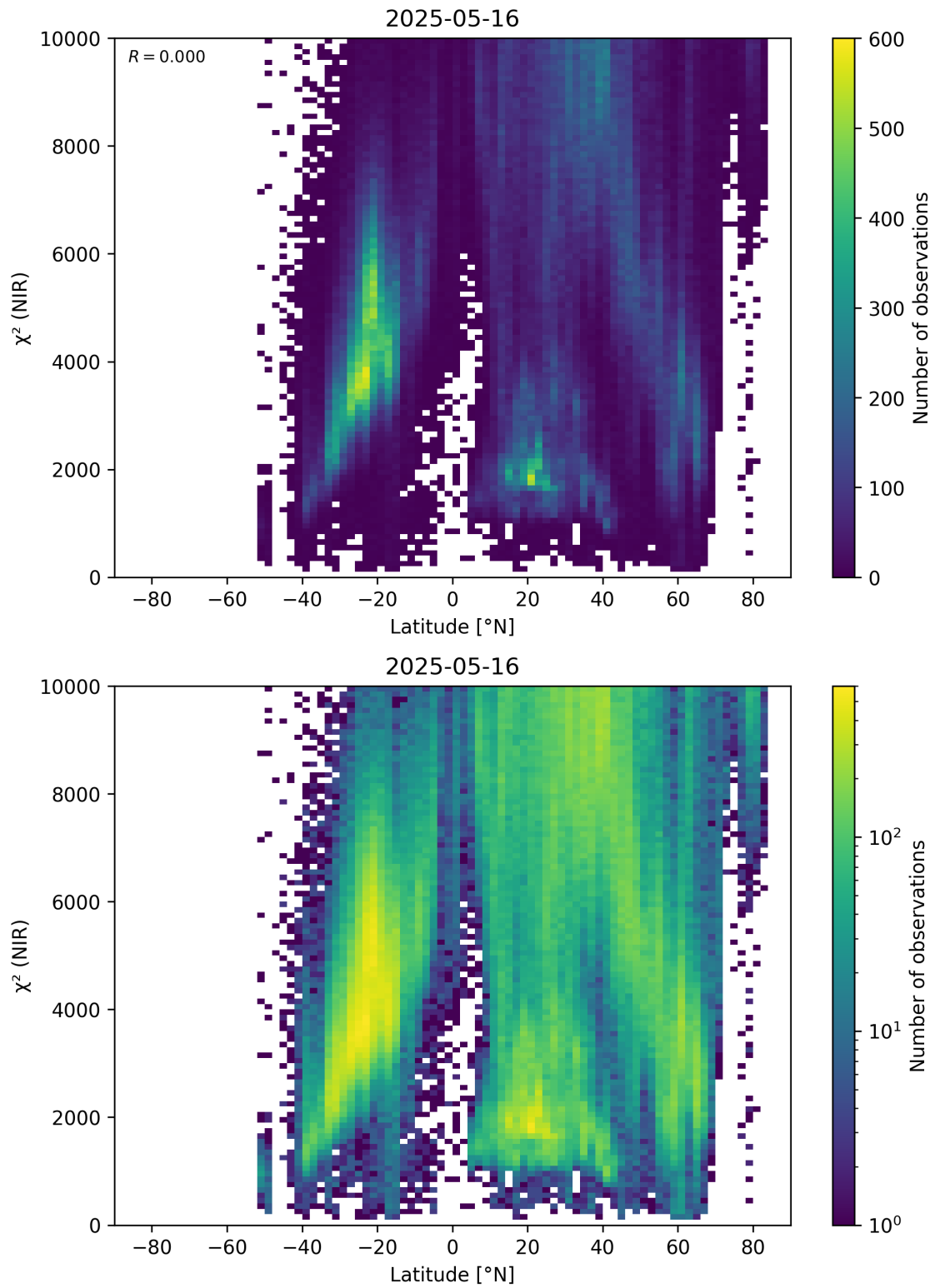
Figure 53: Scatter density plot of “Latitude” against “ \chi^2 (NIR)” for 2025-05-15 to 2025-05-17.
