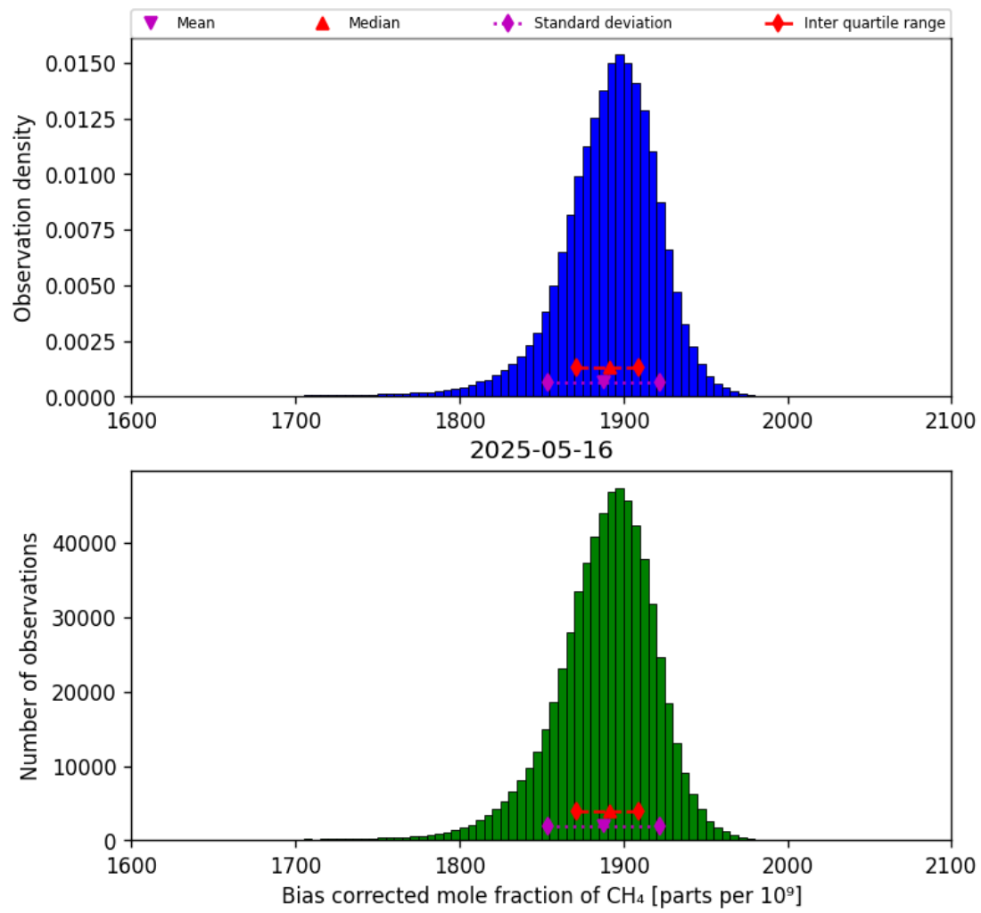
Figure 25: Histogram of “Bias corrected mole fraction of CH 4 ” for 2025-05-15 to 2025-05-17
