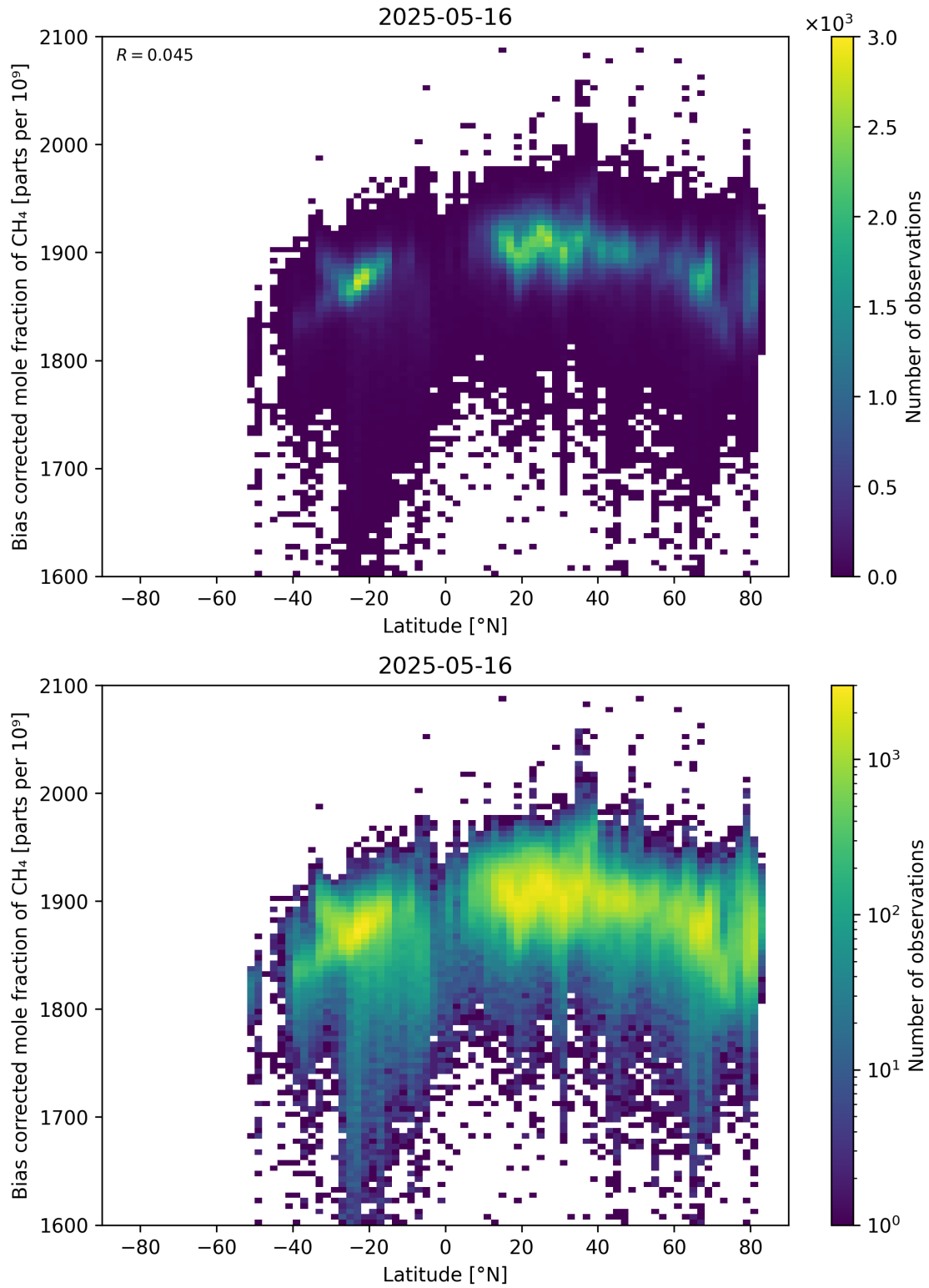
Figure 58: Scatter density plot of “Latitude” against “Bias corrected mole fraction of CH 4 ” for 2025-05-15 to 2025-05-17.
