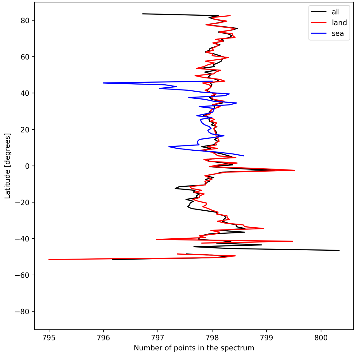
Figure 15: Zonal average of “Number of points in the spectrum” for 2025-05-15 to 2025-05-17.
