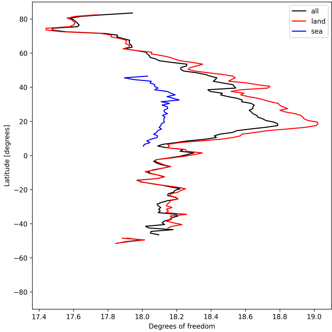
Figure 19: Zonal average of “Degrees of freedom” for 2025-05-15 to 2025-05-17.
