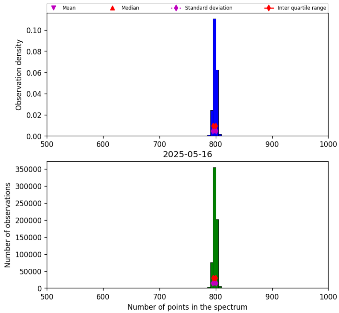
Figure 26: Histogram of “Number of points in the spectrum” for 2025-05-15 to 2025-05-17
