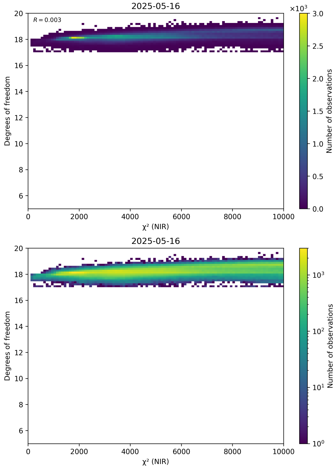
Figure 44: Scatter density plot of “ \chi^2 (NIR)” against “Degrees of freedom” for 2025-05-15 to 2025-05-17.
