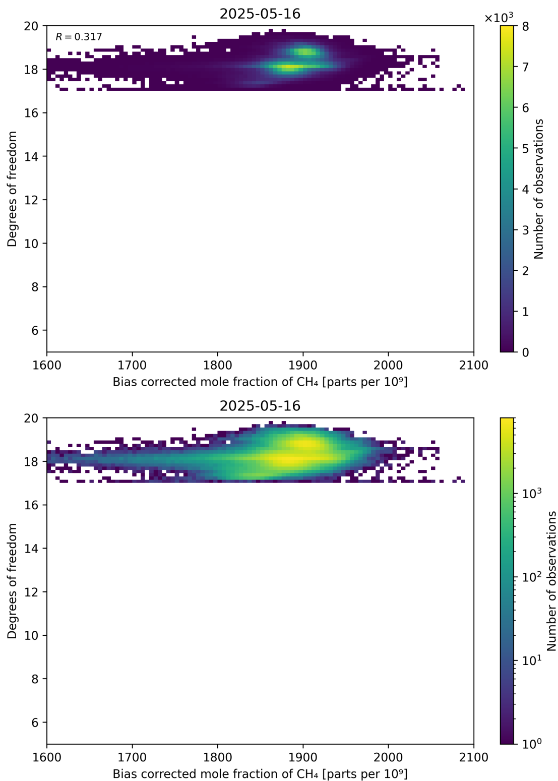
Figure 65: Scatter density plot of “Bias corrected mole fraction of CH 4 ” against “Degrees of freedom” for 2025-05-15 to 2025-05-17.
