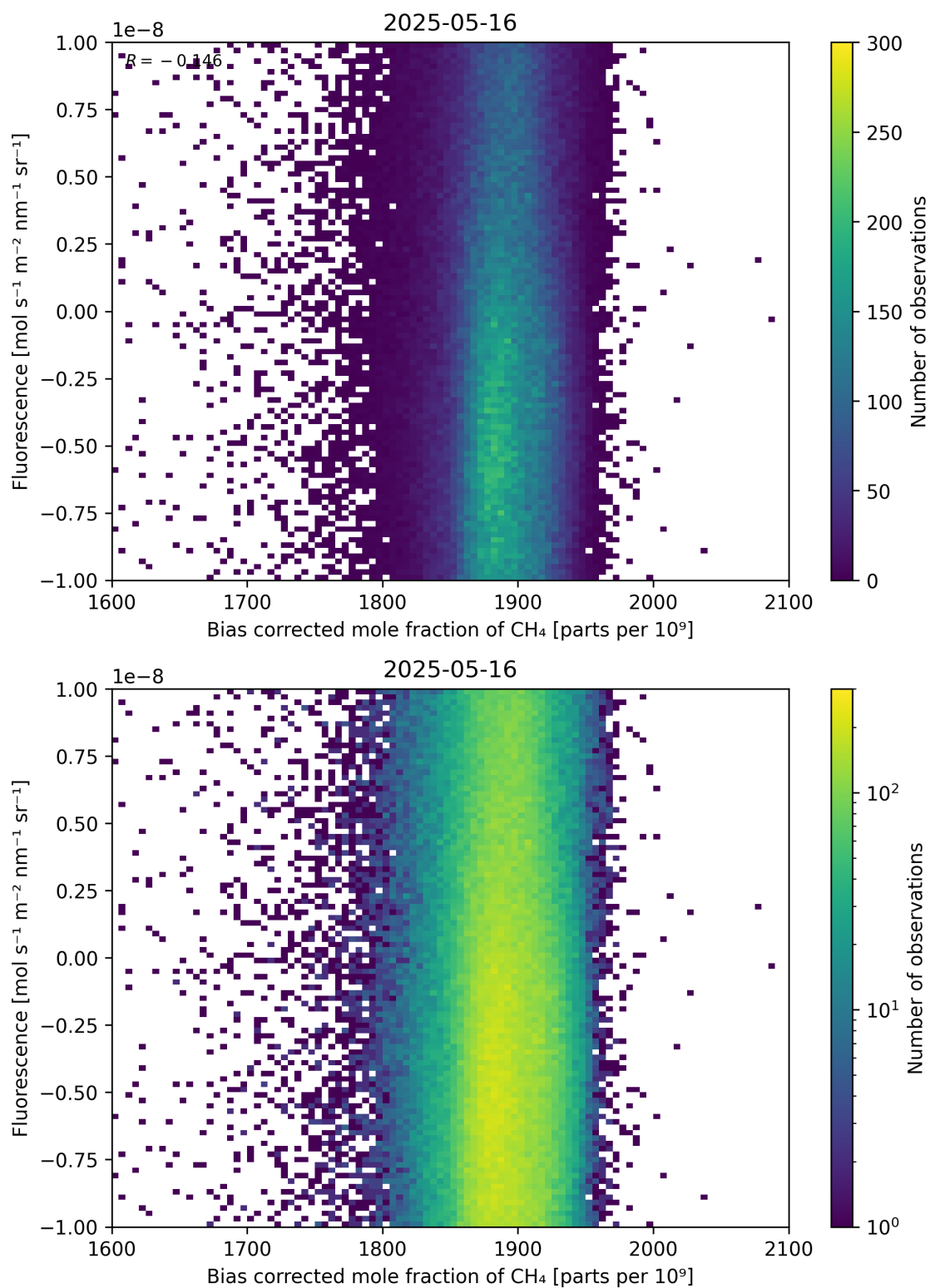
Figure 66: Scatter density plot of “Bias corrected mole fraction of \text{CH}_4 ” against “Fluorescence” for 2025-05-15 to 2025-05-17.
