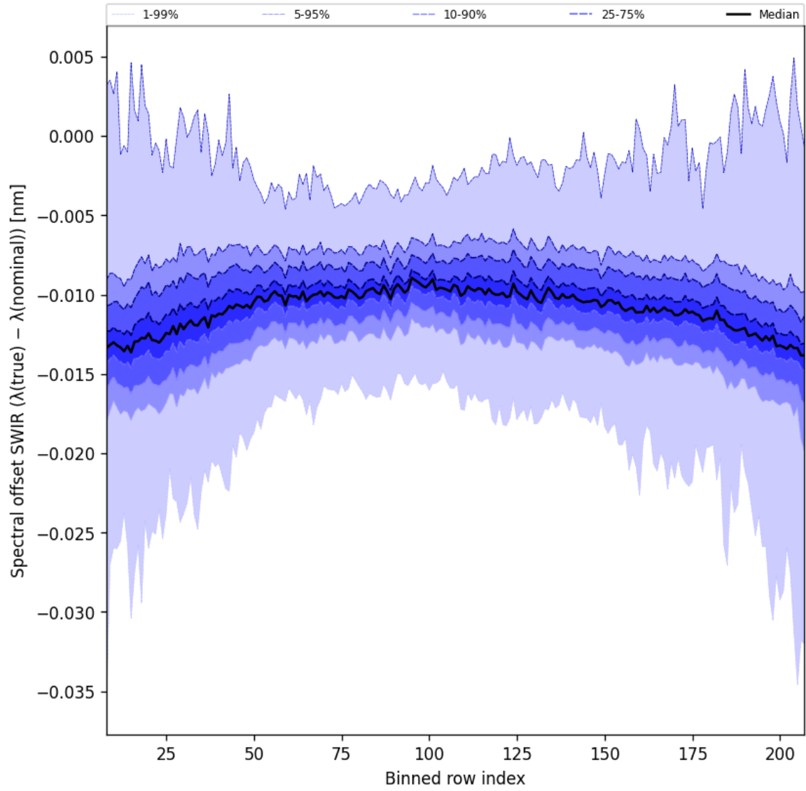
Figure 38: Along track statistics of “Spectral offset SWIR ( \lambda_{\text{true}} - \lambda_{\text{nominal}} )” for 2025-05-15 to 2025-05-17
