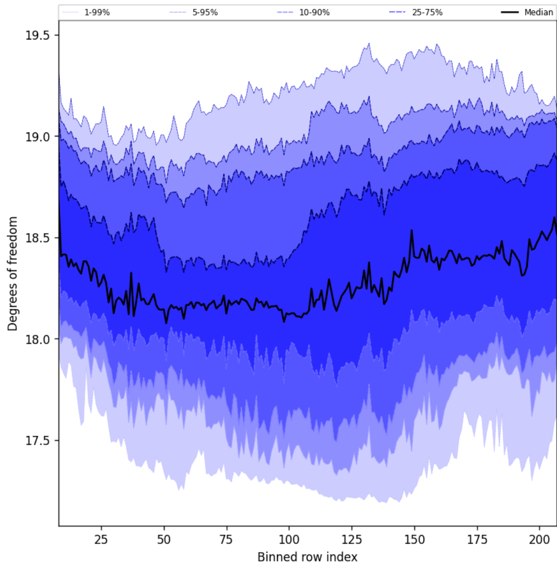
Figure 41: Along track statistics of “Degrees of freedom” for 2025-05-15 to 2025-05-17
