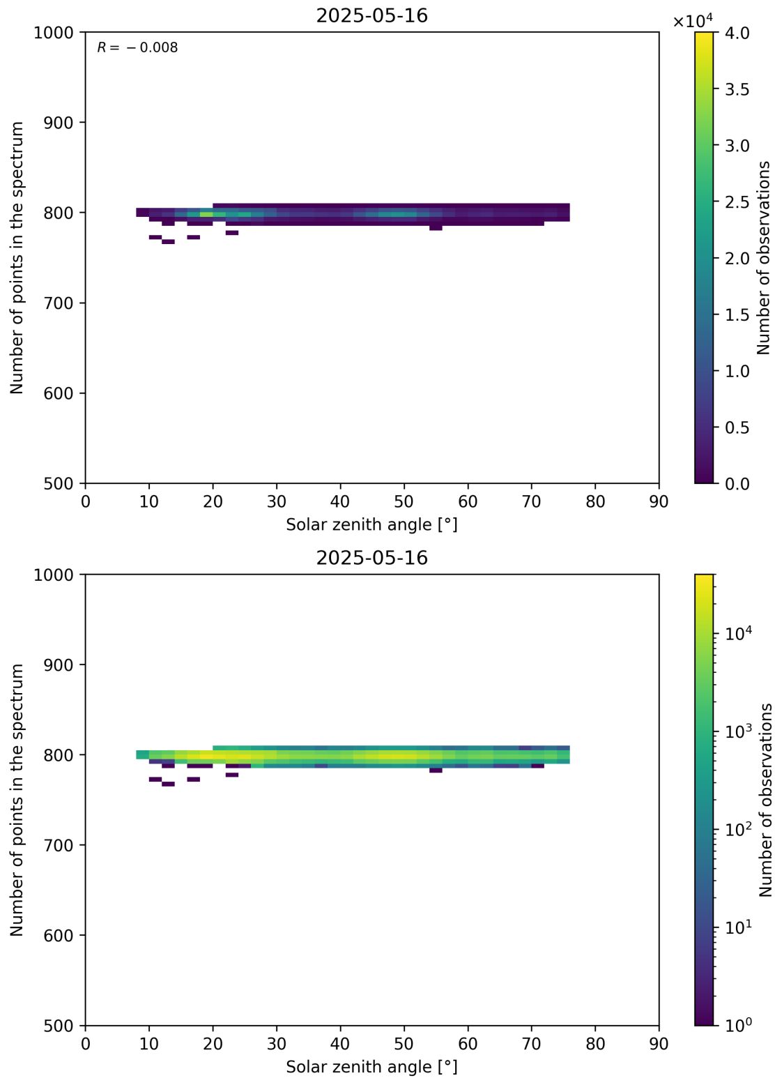
Figure 103: Scatter density plot of “Solar zenith angle” against “Number of points in the spectrum” for 2025-05-15 to 2025-05-17.
