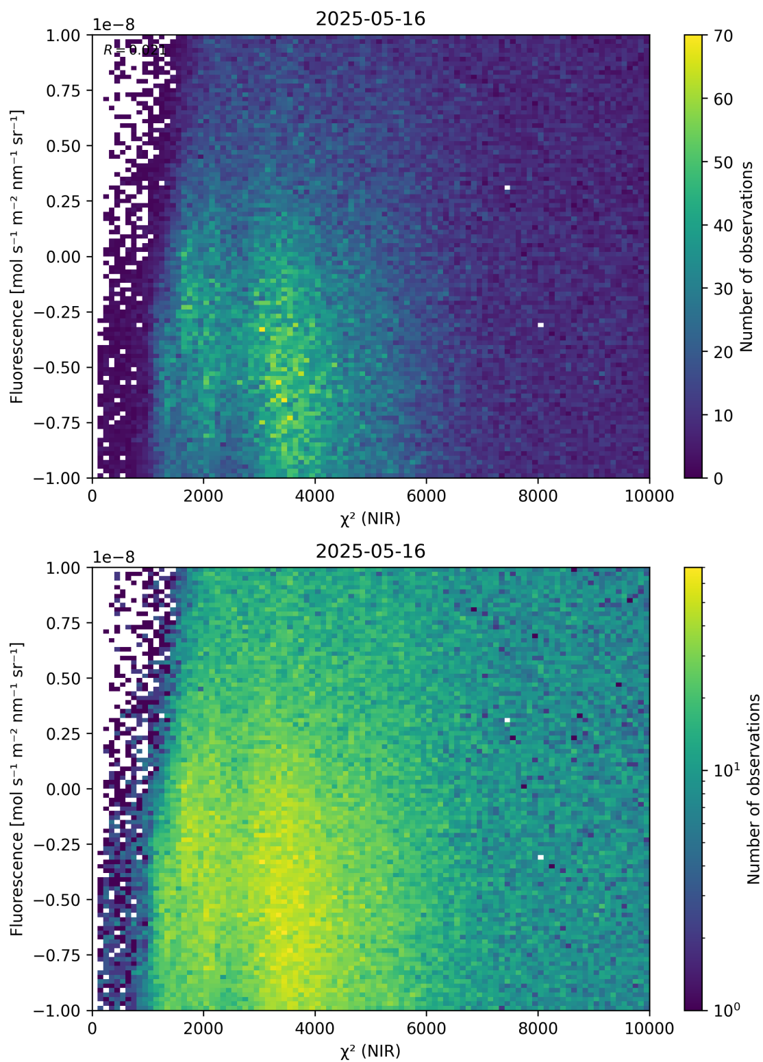
Figure 45: Scatter density plot of “ \chi^2 (NIR)” against “Fluorescence” for 2025-05-15 to 2025-05-17.
