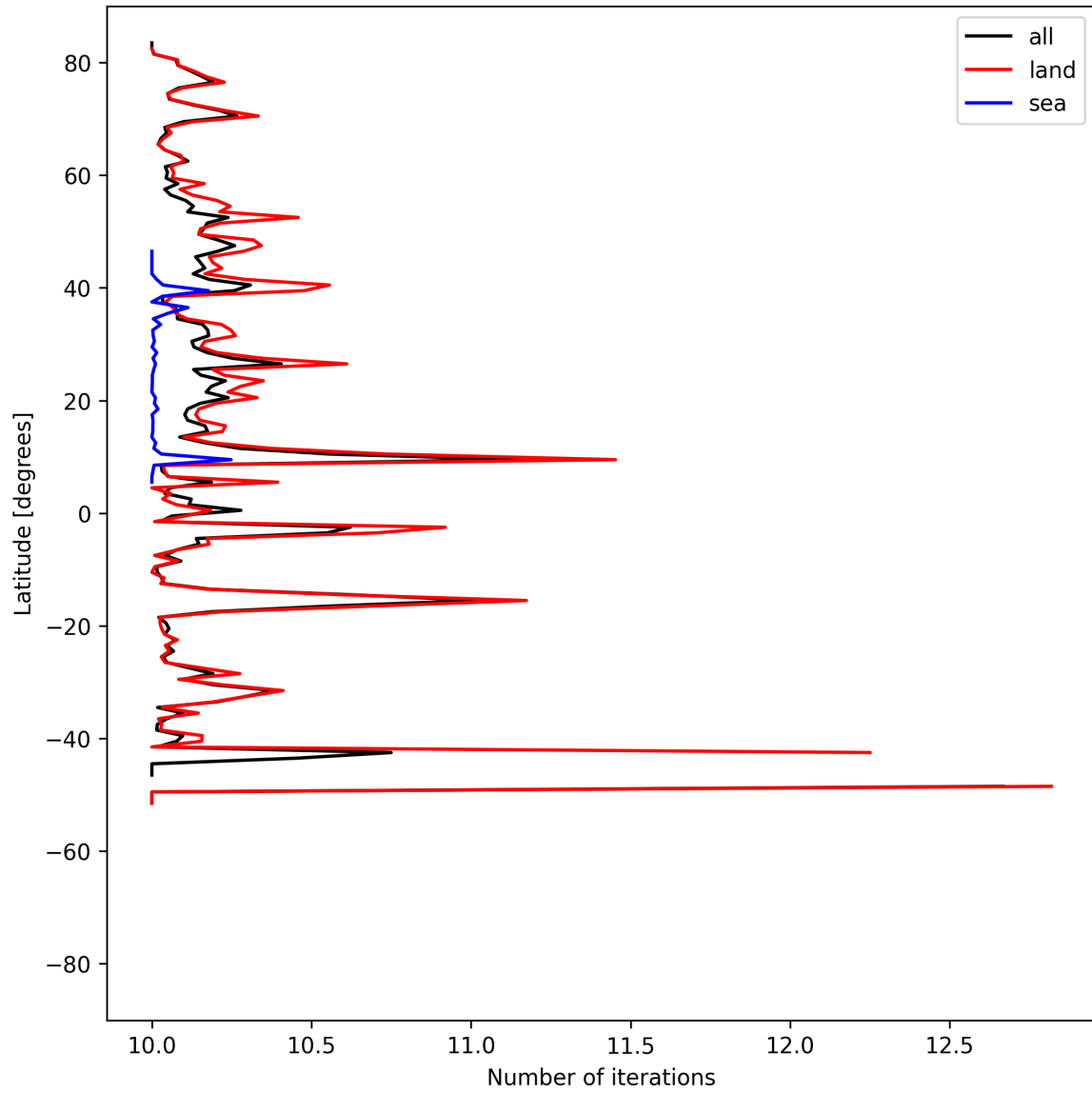
Figure 20: Zonal average of “Number of iterations” for 2025-05-15 to 2025-05-17.
