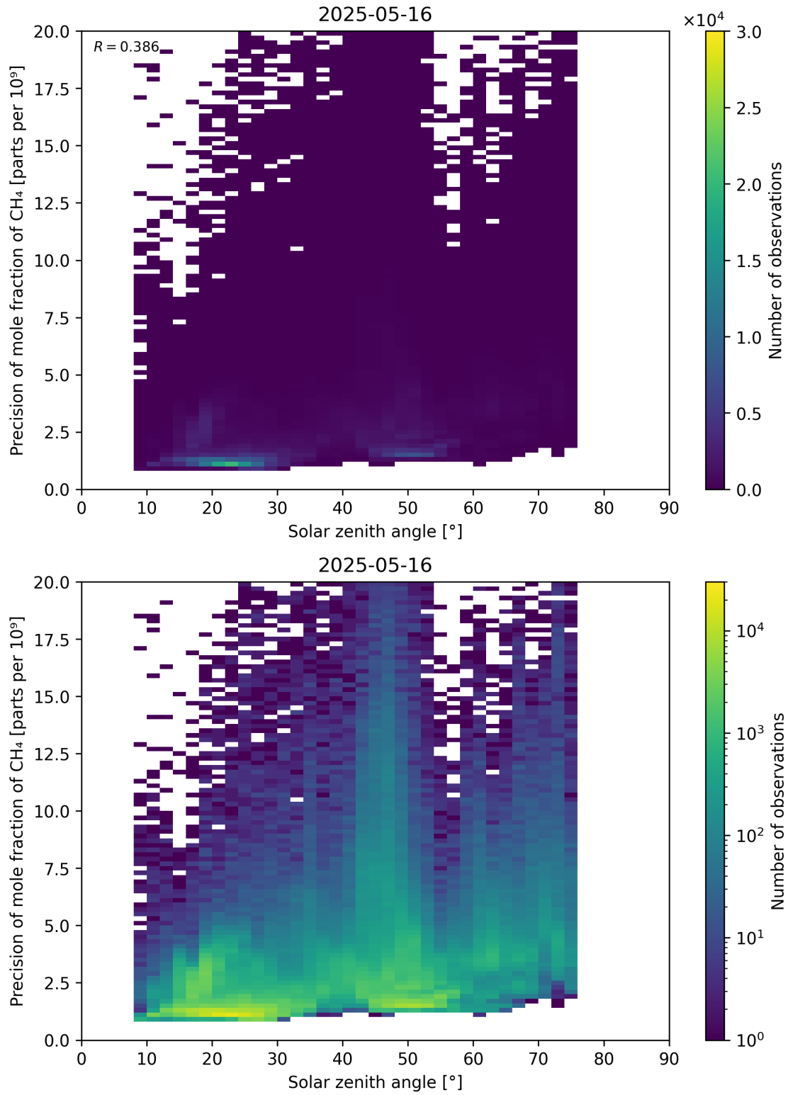
Figure 101: Scatter density plot of “Solar zenith angle” against “Precision of mole fraction of CH 4 ” for 2025-05-15 to 2025-05-17.
