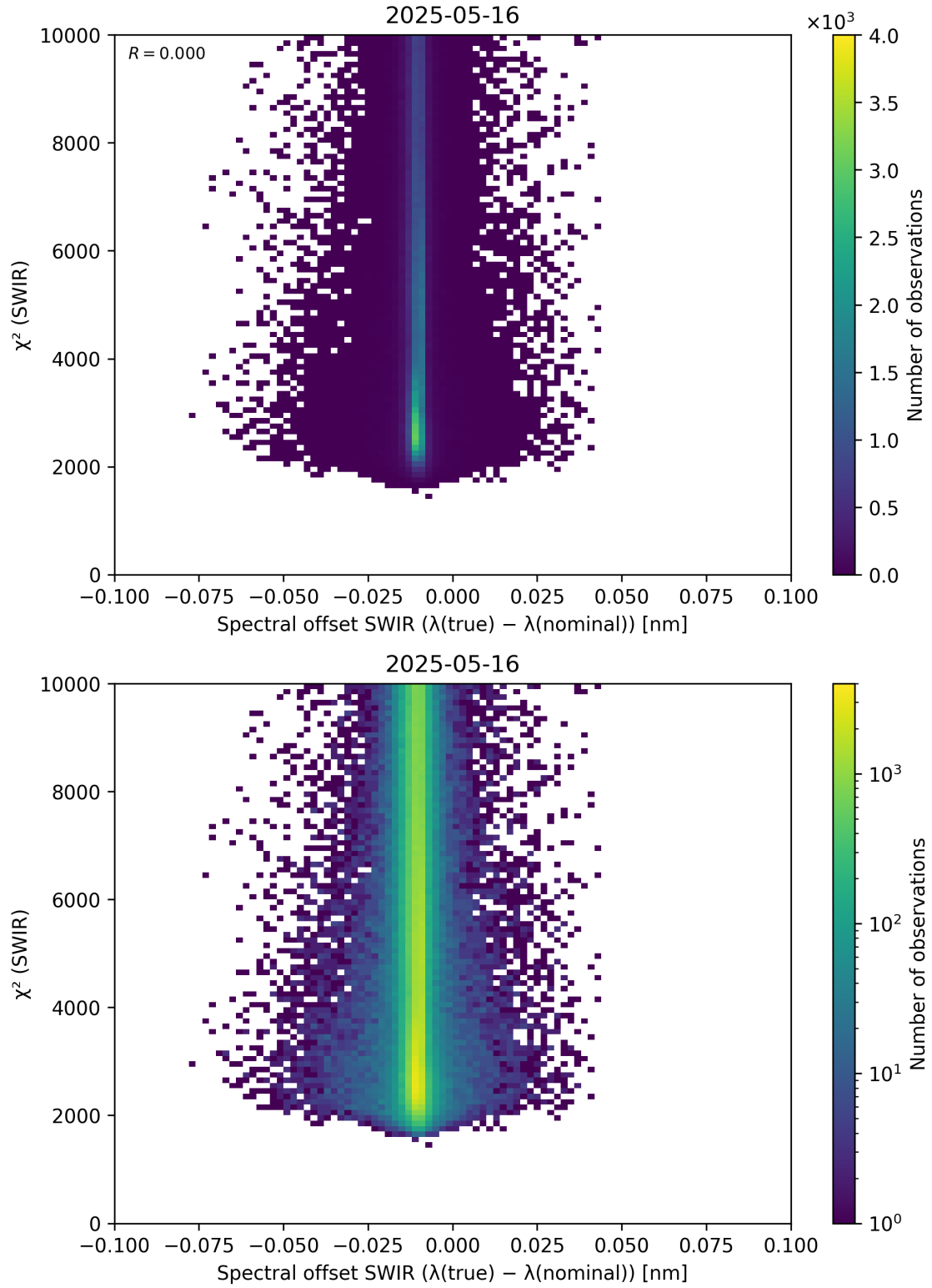
Figure 118: Scatter density plot of “Spectral offset SWIR ( \lambda_{\text{true}} - \lambda_{\text{nominal}} )” against “ \chi^2 (SWIR)” for 2025-05-15 to 2025-05-17.
