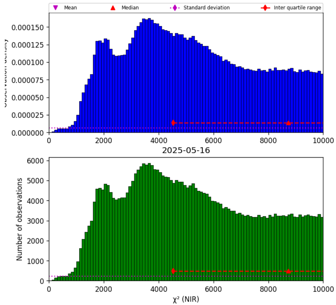
Figure 29: Histogram of “ \chi^2 (NIR)” for 2025-05-15 to 2025-05-17
