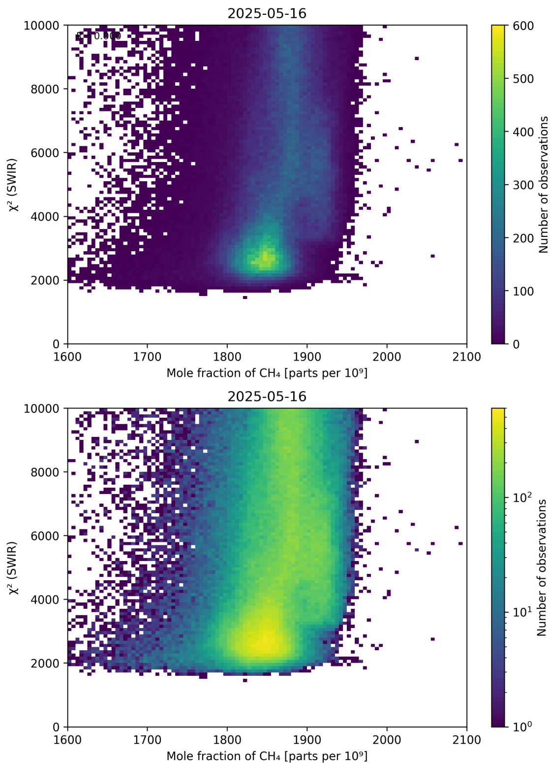
Figure 71: Scatter density plot of “Mole fraction of CH 4 ” against “ \chi^2 (SWIR)” for 2025-05-15 to 2025-05-17.
