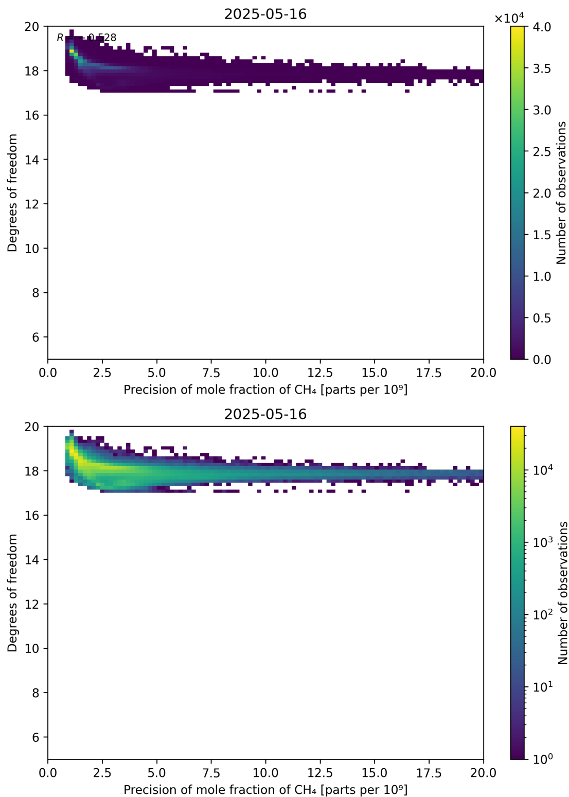
Figure 80: Scatter density plot of “Precision of mole fraction of CH 4 ” against “Degrees of freedom” for 2025-05-15 to 2025-05-17.
