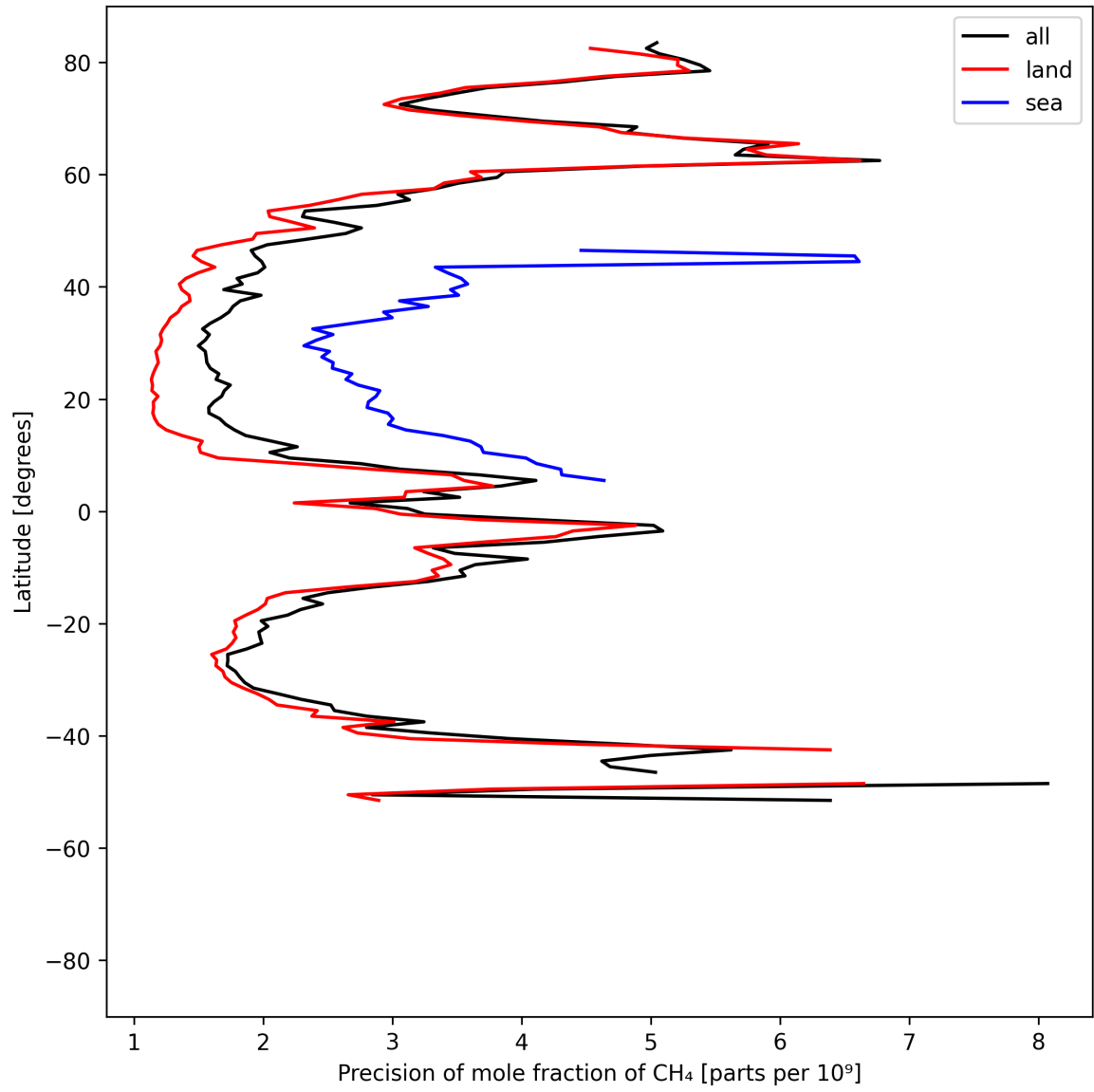
Figure 13: Zonal average of “Precision of mole fraction of CH 4 ” for 2025-05-15 to 2025-05-17.
