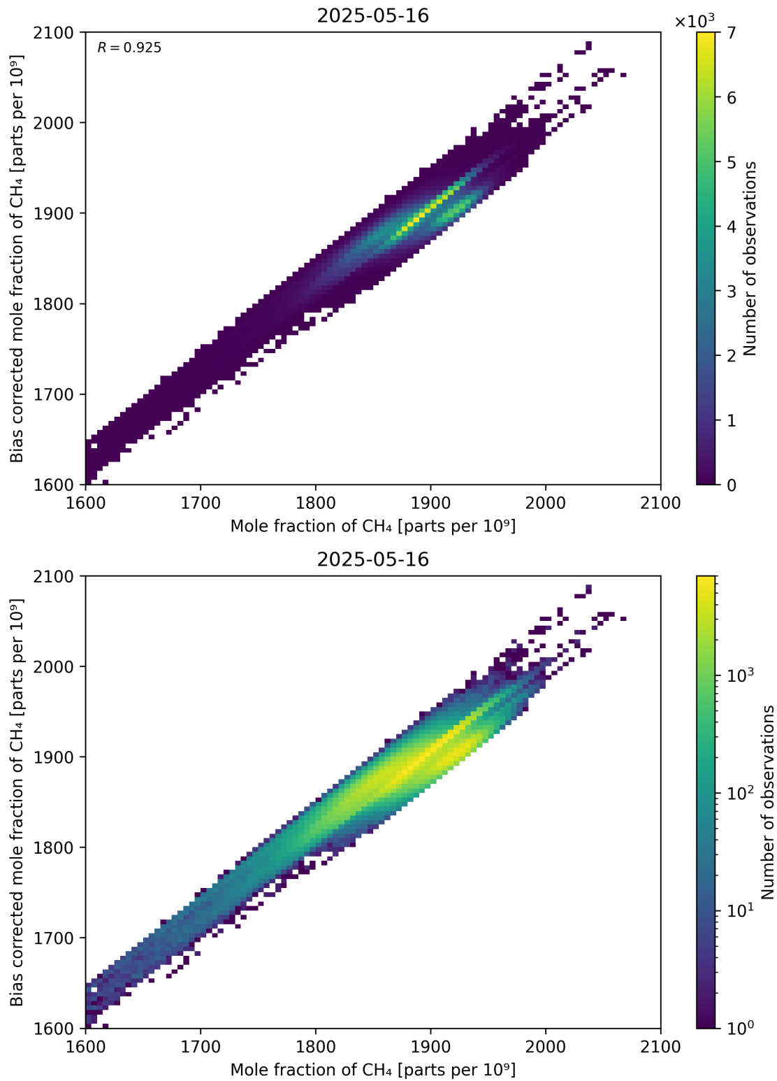
Figure 74: Scatter density plot of “Mole fraction of CH 4 ” against “Bias corrected mole fraction of CH 4 ” for 2025-05-15 to 2025-05-17.
