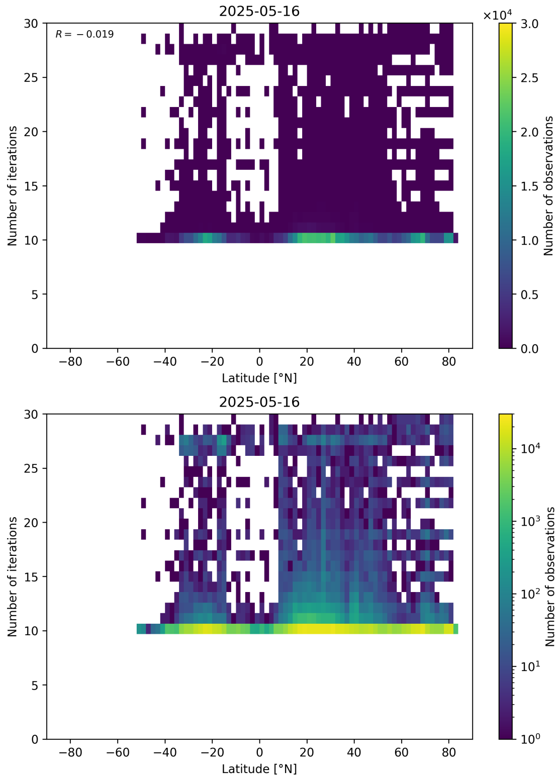
Figure 60: Scatter density plot of “Latitude” against “Number of iterations” for 2025-05-15 to 2025-05-17.
