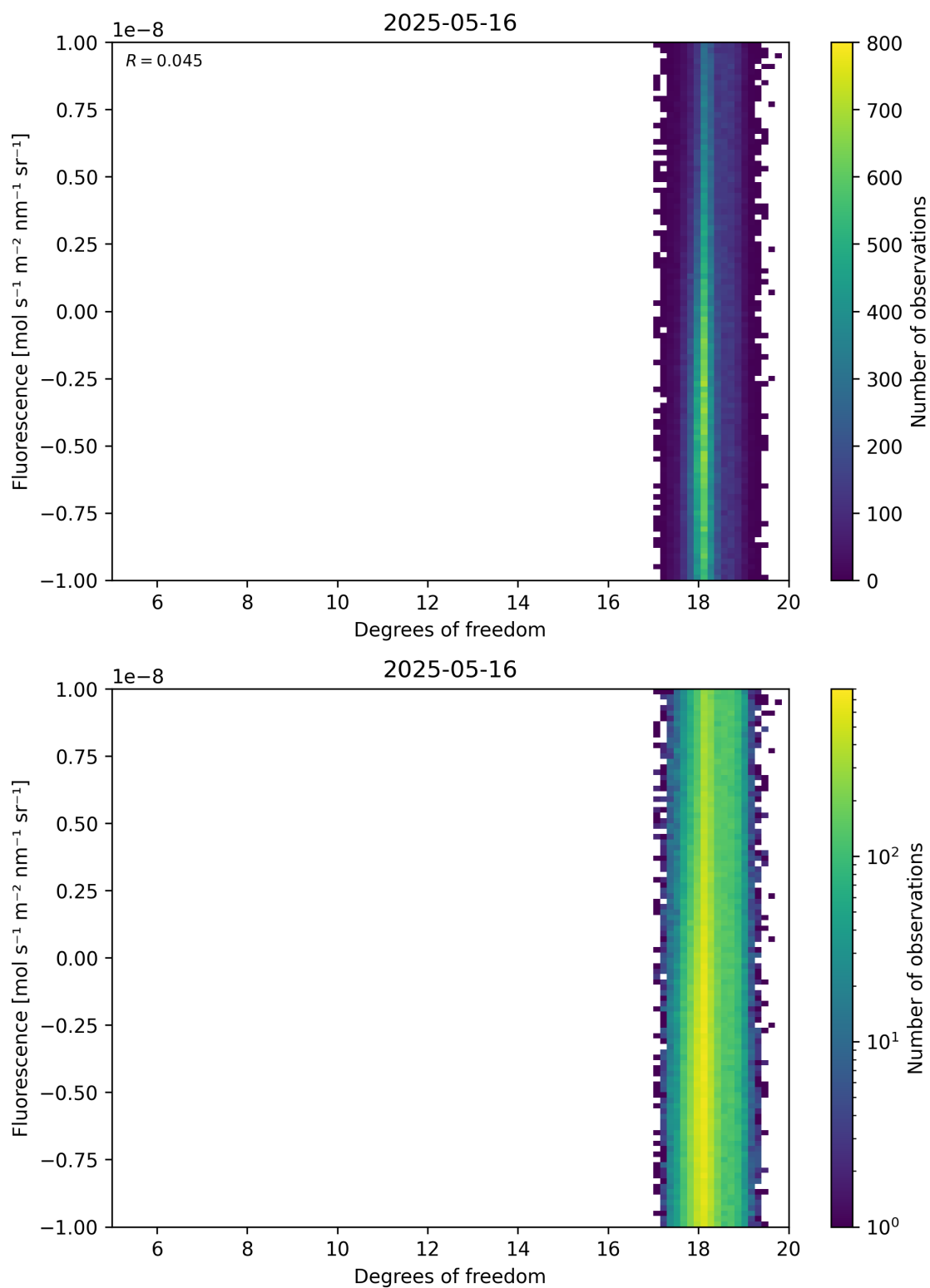
Figure 51: Scatter density plot of “Degrees of freedom” against “Fluorescence” for 2025-05-15 to 2025-05-17.
