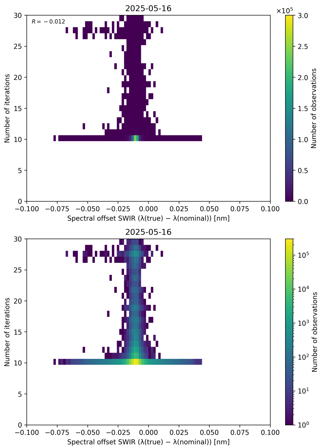
Figure 121: Scatter density plot of “Spectral offset SWIR ( \lambda_{\text{true}} - \lambda_{\text{nominal}} )” against “Number of iterations” for 2025-05-15 to 2025-05-17.
