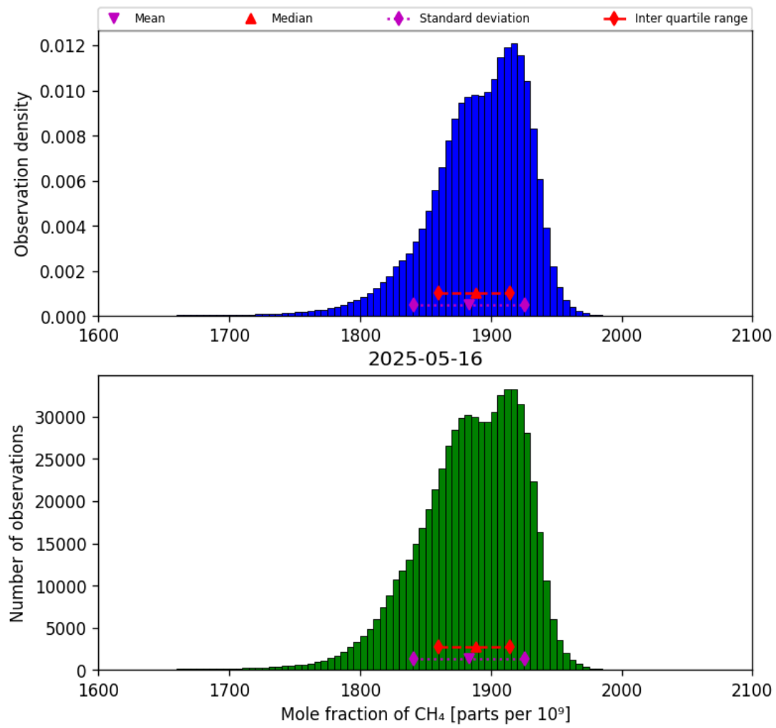
Figure 23: Histogram of “Mole fraction of CH 4 ” for 2025-05-15 to 2025-05-17
