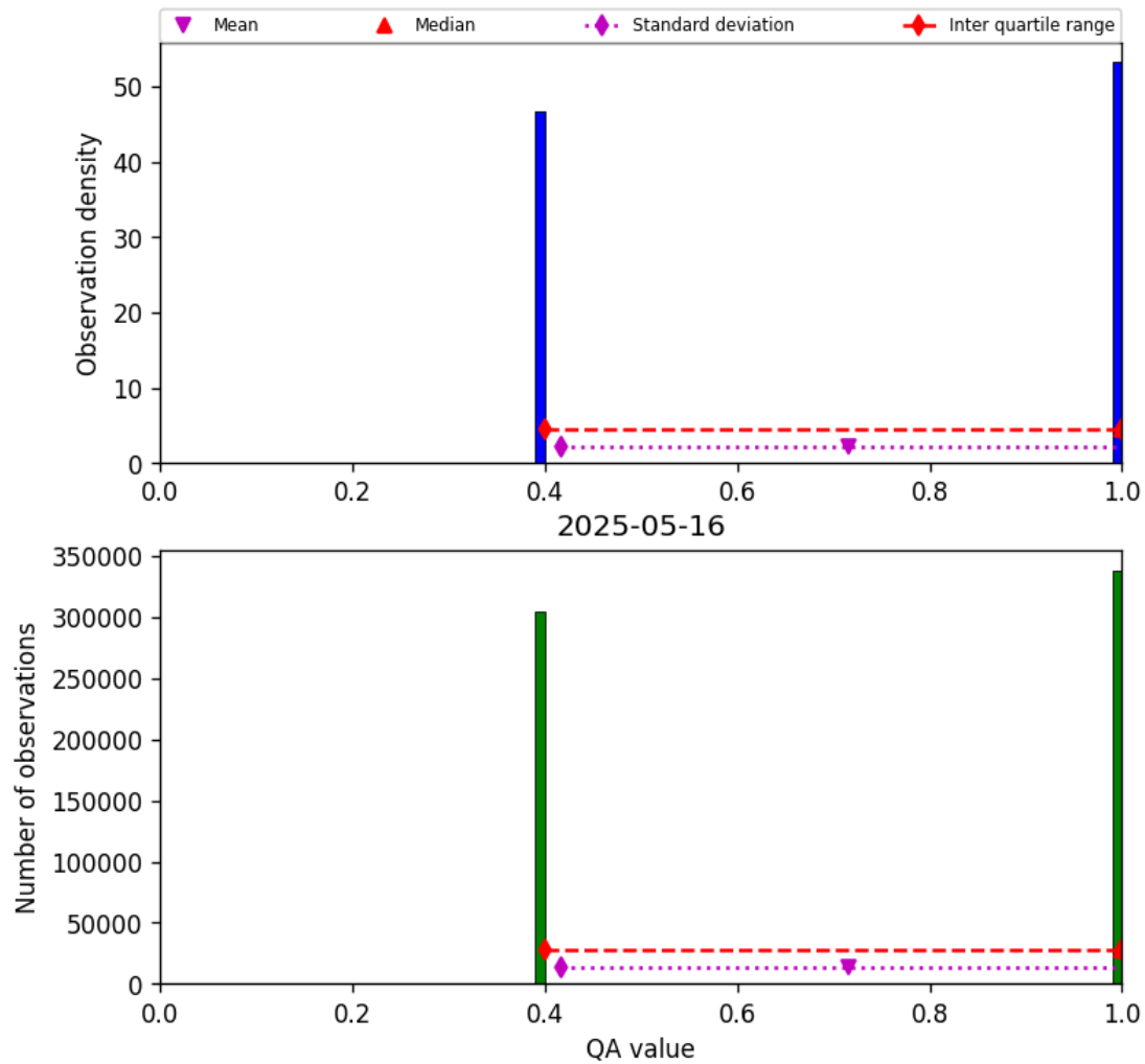
Figure 22: Histogram of “QA value” for 2025-05-15 to 2025-05-17
