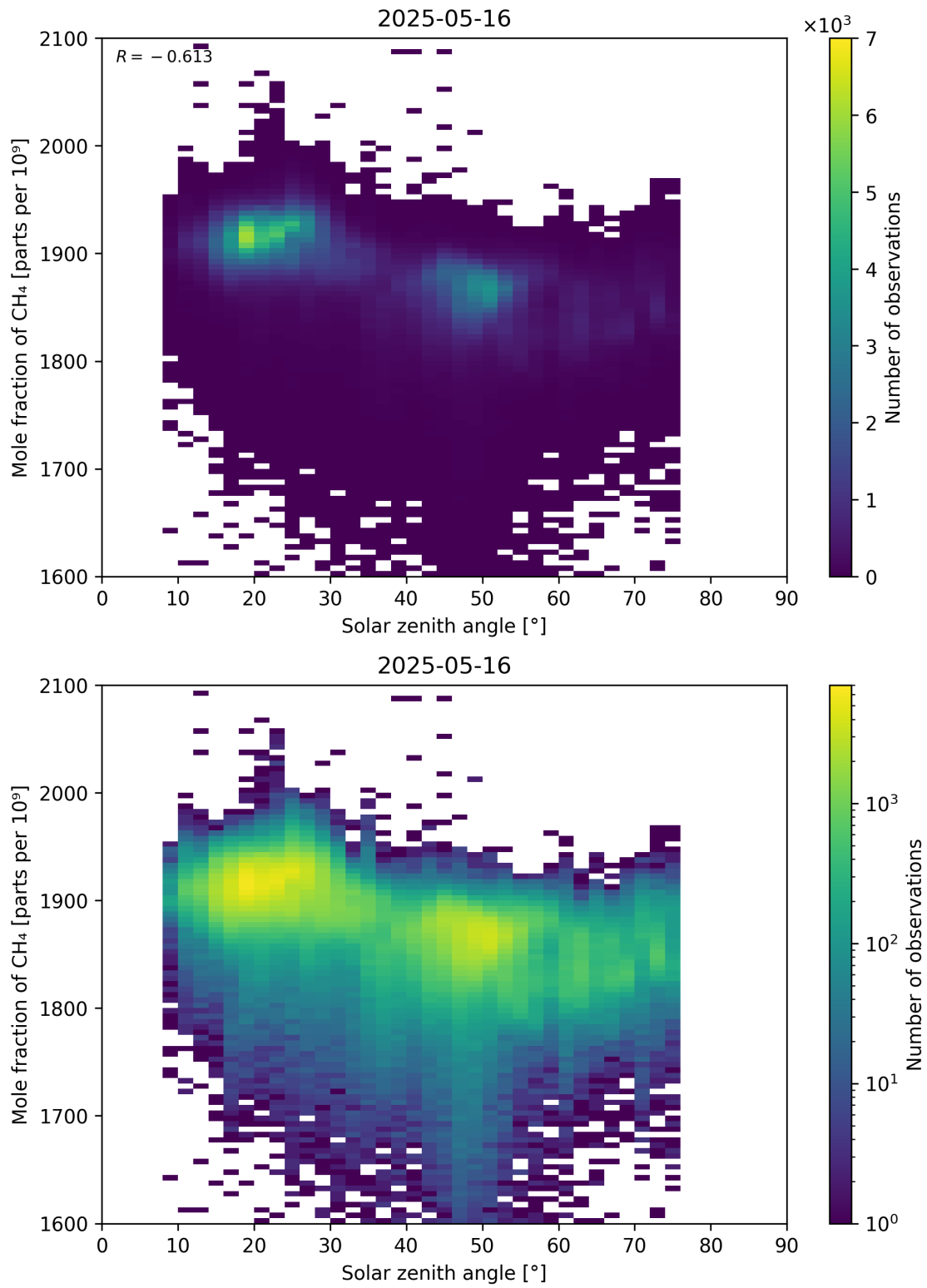
Figure 99: Scatter density plot of “Solar zenith angle” against “Mole fraction of CH 4 ” for 2025-05-15 to 2025-05-17.
