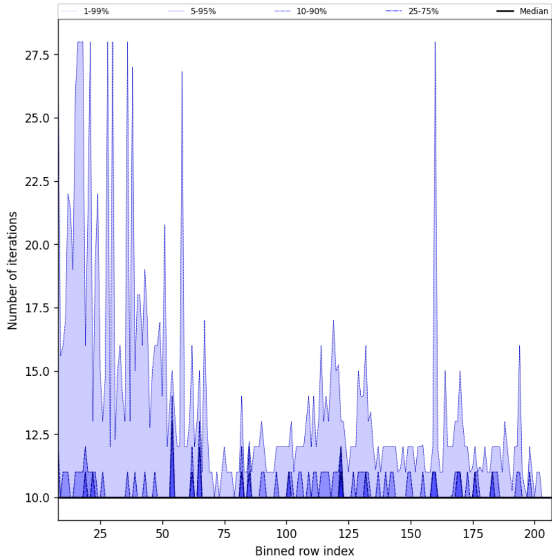
Figure 42: Along track statistics of “Number of iterations” for 2025-05-16 to 2025-05-18
