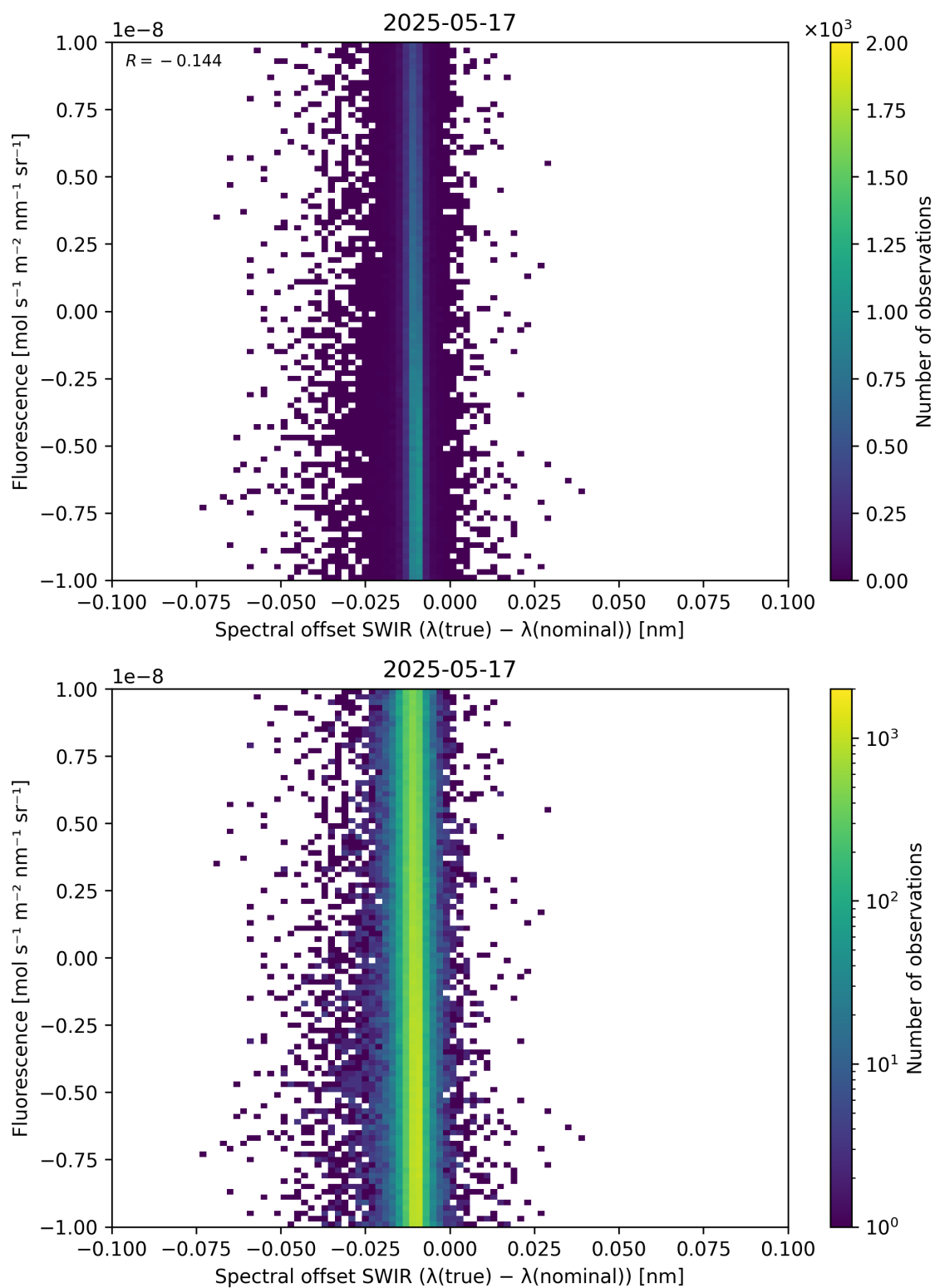
Figure 120: Scatter density plot of “Spectral offset SWIR ( \lambda_{\text{true}} - \lambda_{\text{nominal}} )” against “Fluorescence” for 2025-05-16 to 2025-05-18.
