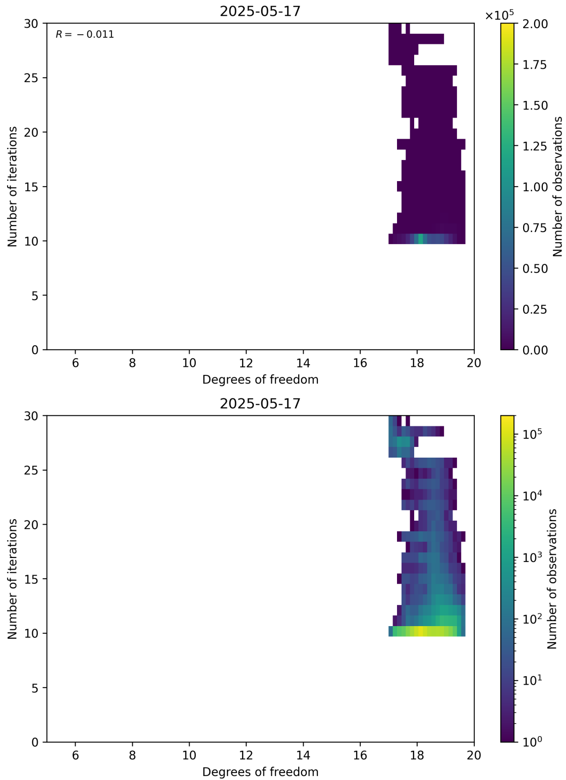
Figure 52: Scatter density plot of “Degrees of freedom” against “Number of iterations” for 2025-05-16 to 2025-05-18.
