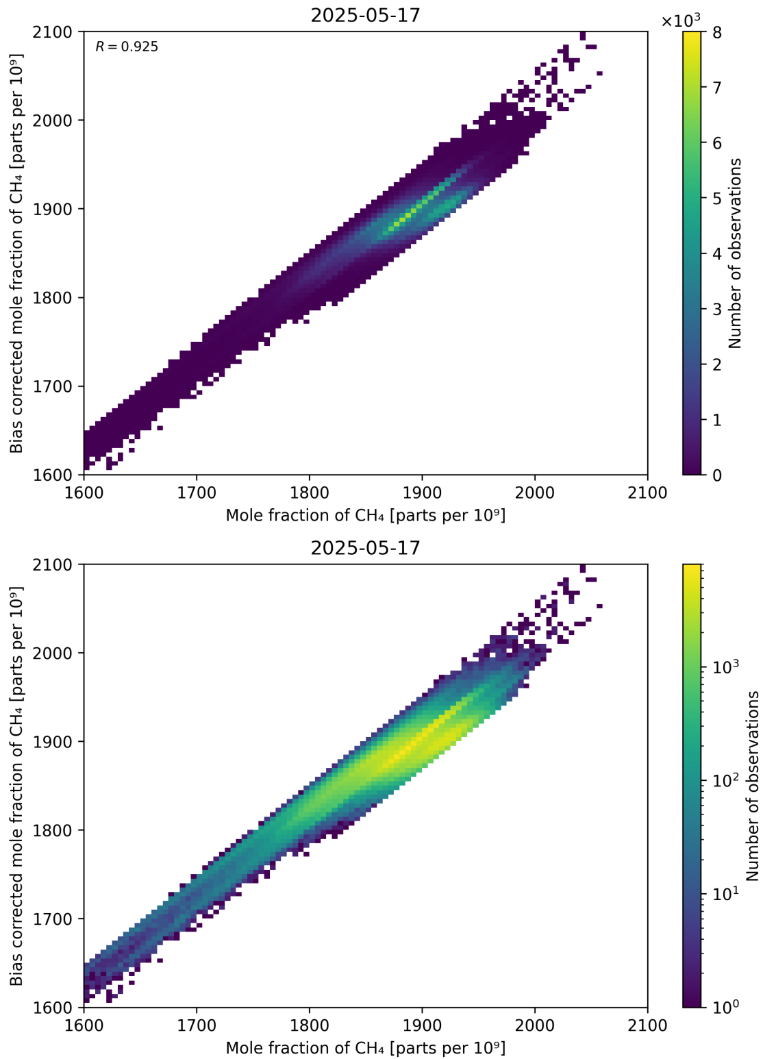
Figure 74: Scatter density plot of “Mole fraction of CH 4 ” against “Bias corrected mole fraction of CH 4 ” for 2025-05-16 to 2025-05-18.
