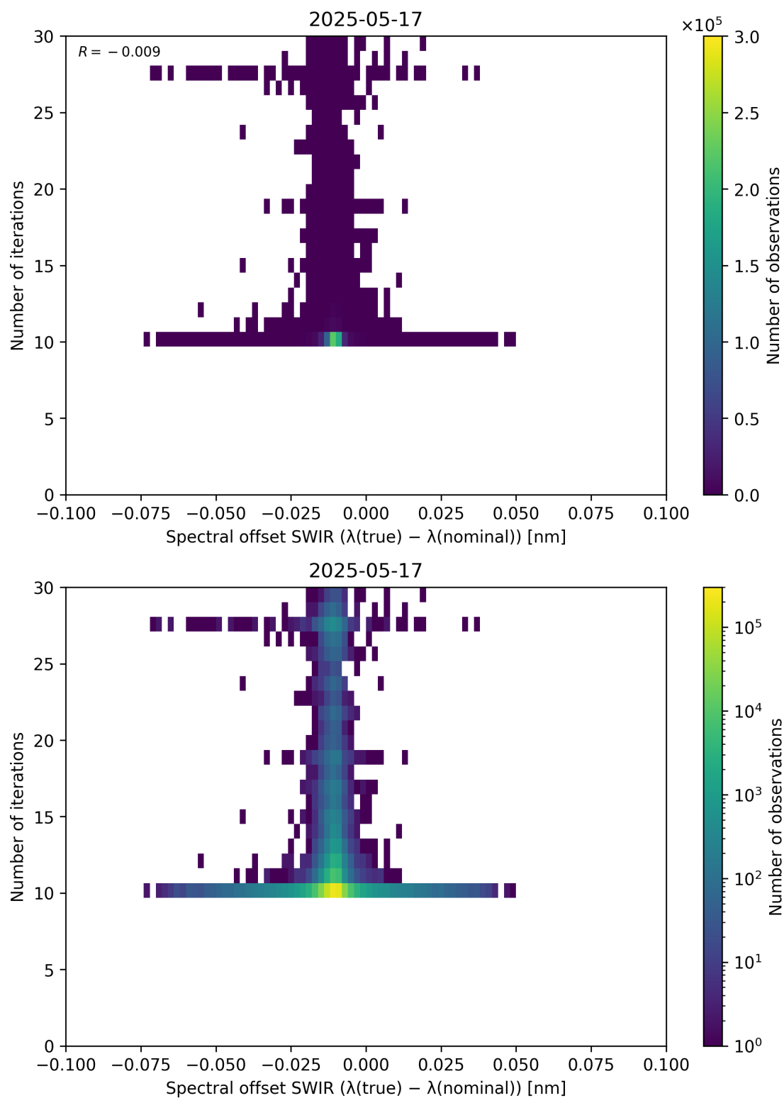
Figure 121: Scatter density plot of “Spectral offset SWIR ( \lambda_{\text{true}} - \lambda_{\text{nominal}} )” against “Number of iterations” for 2025-05-16 to 2025-05-18.
