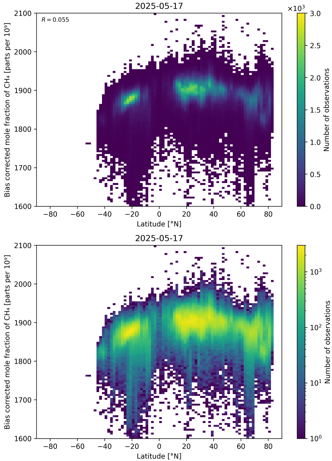
Figure 58: Scatter density plot of “Latitude” against “Bias corrected mole fraction of \text{CH}_4 ” for 2025-05-16 to 2025-05-18.
