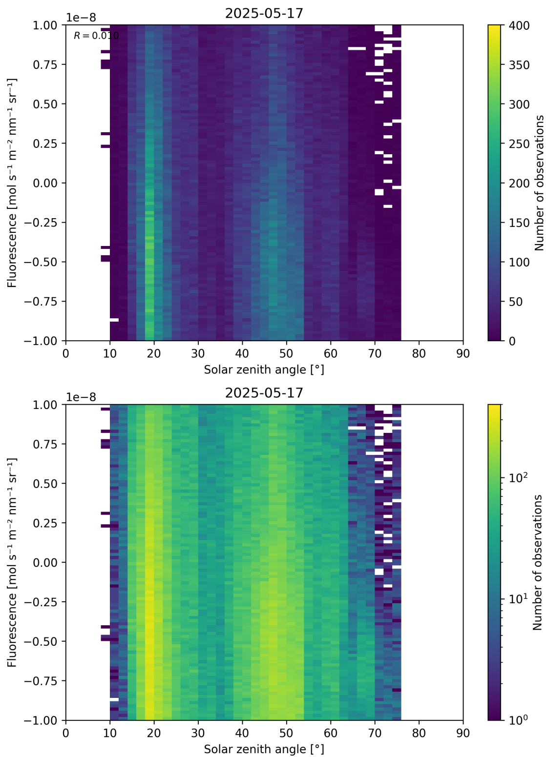
Figure 97: Scatter density plot of “Solar zenith angle” against “Fluorescence” for 2025-05-16 to 2025-05-18.
