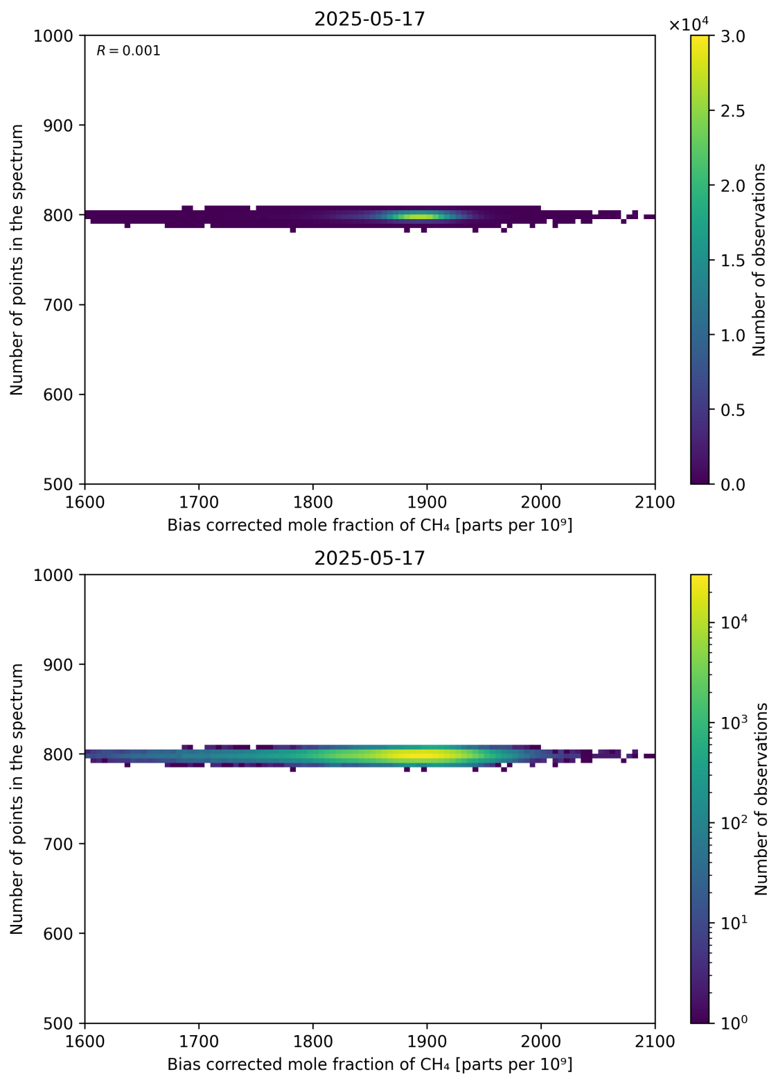
Figure 68: Scatter density plot of “Bias corrected mole fraction of CH 4 ” against “Number of points in the spectrum” for 2025-05-16 to 2025-05-18.
