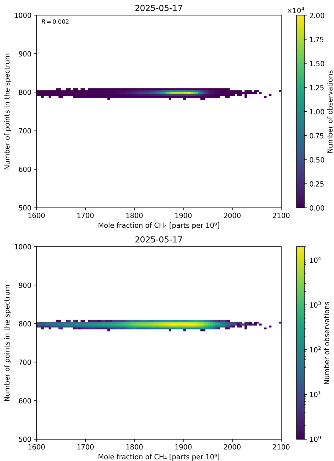
Figure 77: Scatter density plot of “Mole fraction of CH 4 ” against “Number of points in the spectrum” for 2025-05-16 to 2025-05-18.
