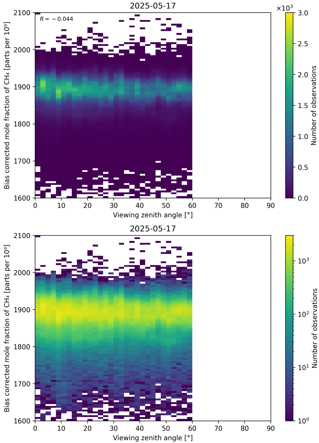
Figure 111: Scatter density plot of “Viewing zenith angle” against “Bias corrected mole fraction of CH 4 ” for 2025-05-16 to 2025-05-18.
