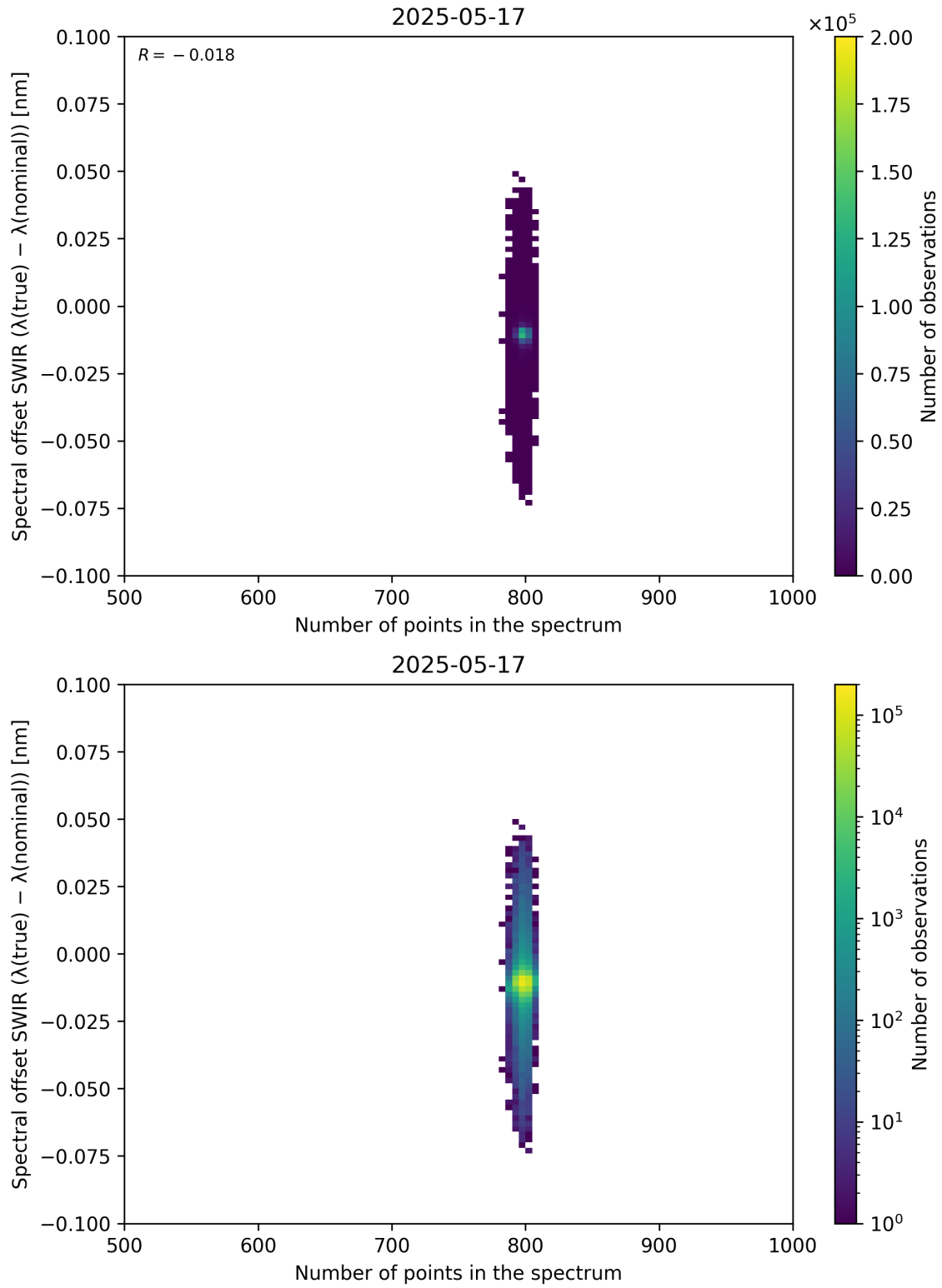
Figure 93: Scatter density plot of “Number of points in the spectrum” against “Spectral offset SWIR ( \lambda_{\text{true}} - \lambda_{\text{nominal}} )” for 2025-05-16 to 2025-05-18.
