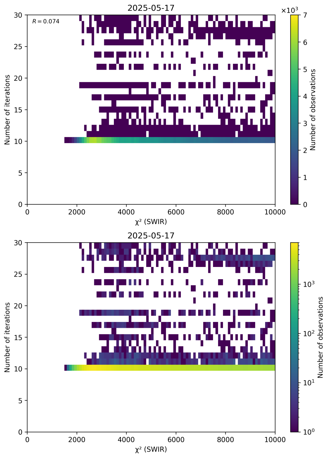
Figure 50: Scatter density plot of “ \chi^2 (SWIR)” against “Number of iterations” for 2025-05-16 to 2025-05-18.
