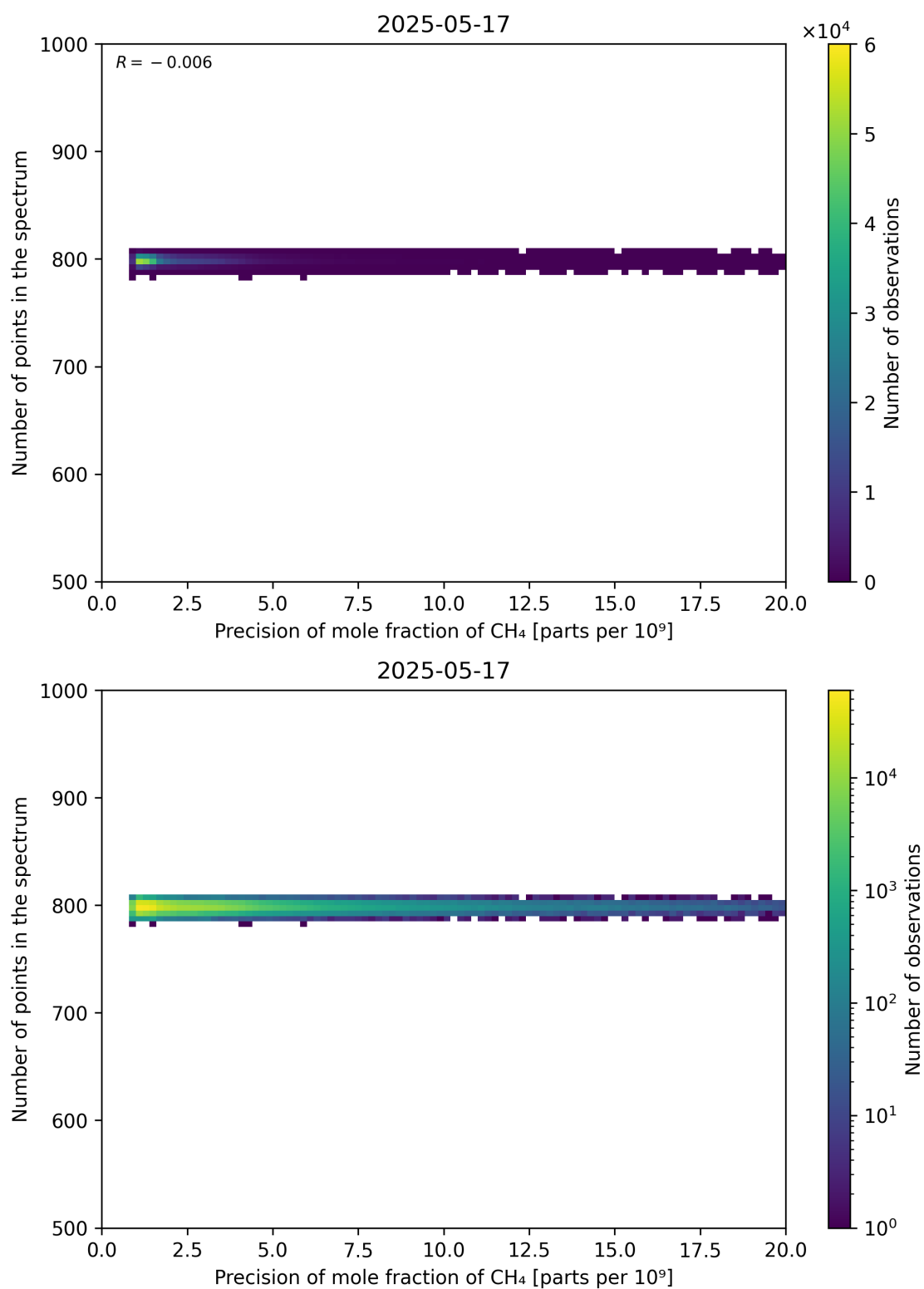
Figure 84: Scatter density plot of “Precision of mole fraction of CH 4 ” against “Number of points in the spectrum” for 2025-05-16 to 2025-05-18.
