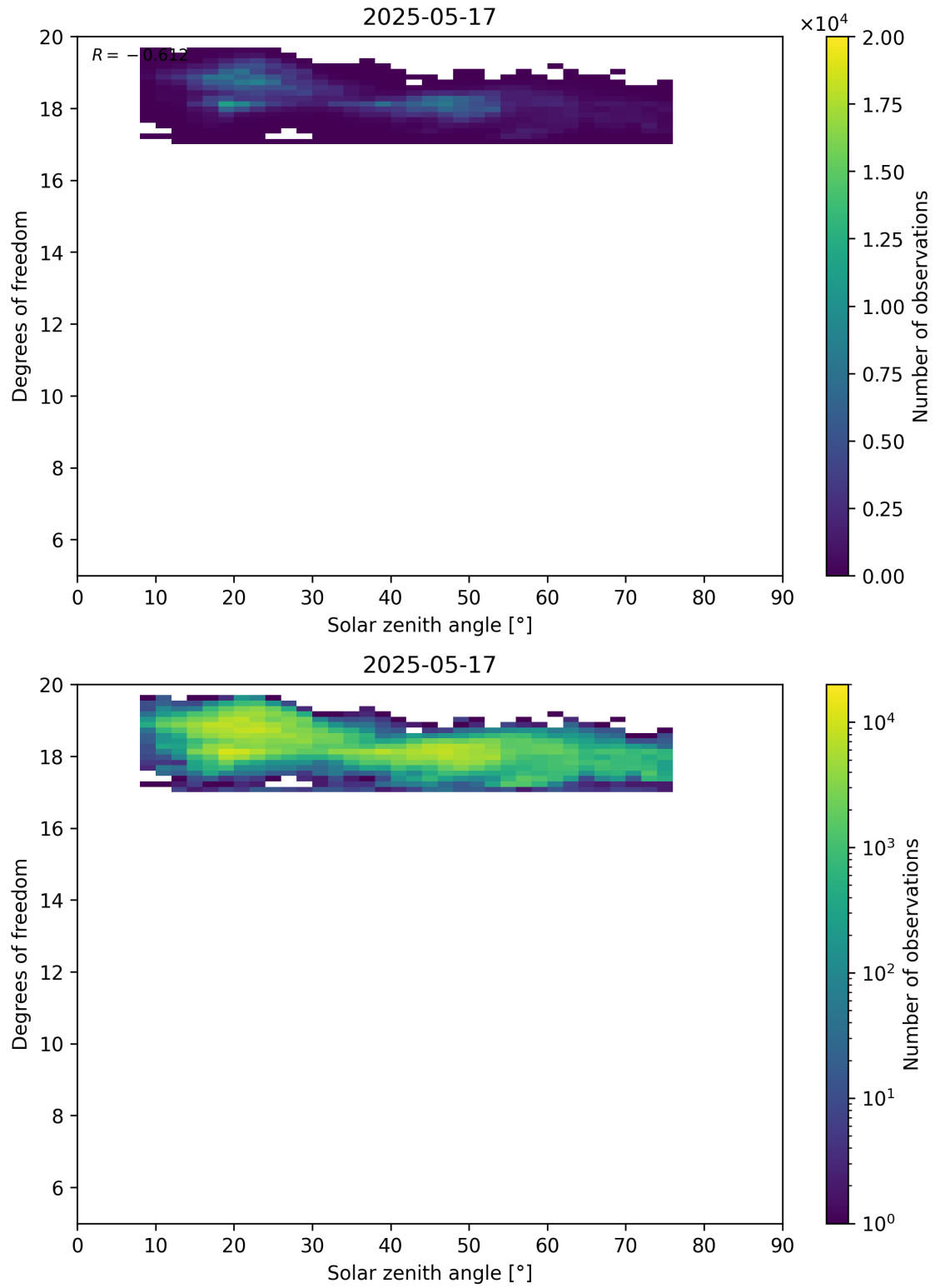
Figure 96: Scatter density plot of “Solar zenith angle” against “Degrees of freedom” for 2025-05-16 to 2025-05-18.
