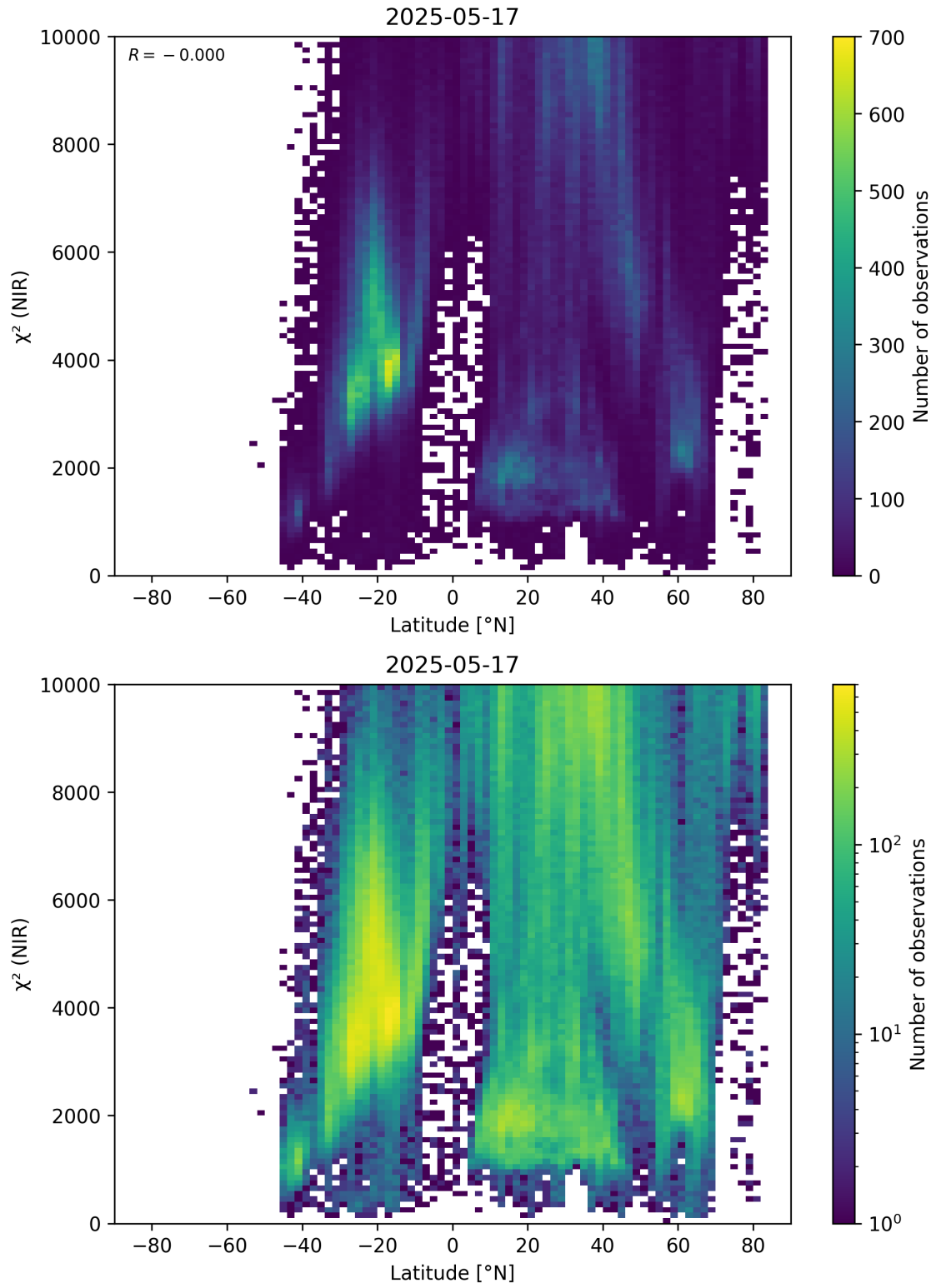
Figure 53: Scatter density plot of “Latitude” against “ \chi^2 (NIR)” for 2025-05-16 to 2025-05-18.
