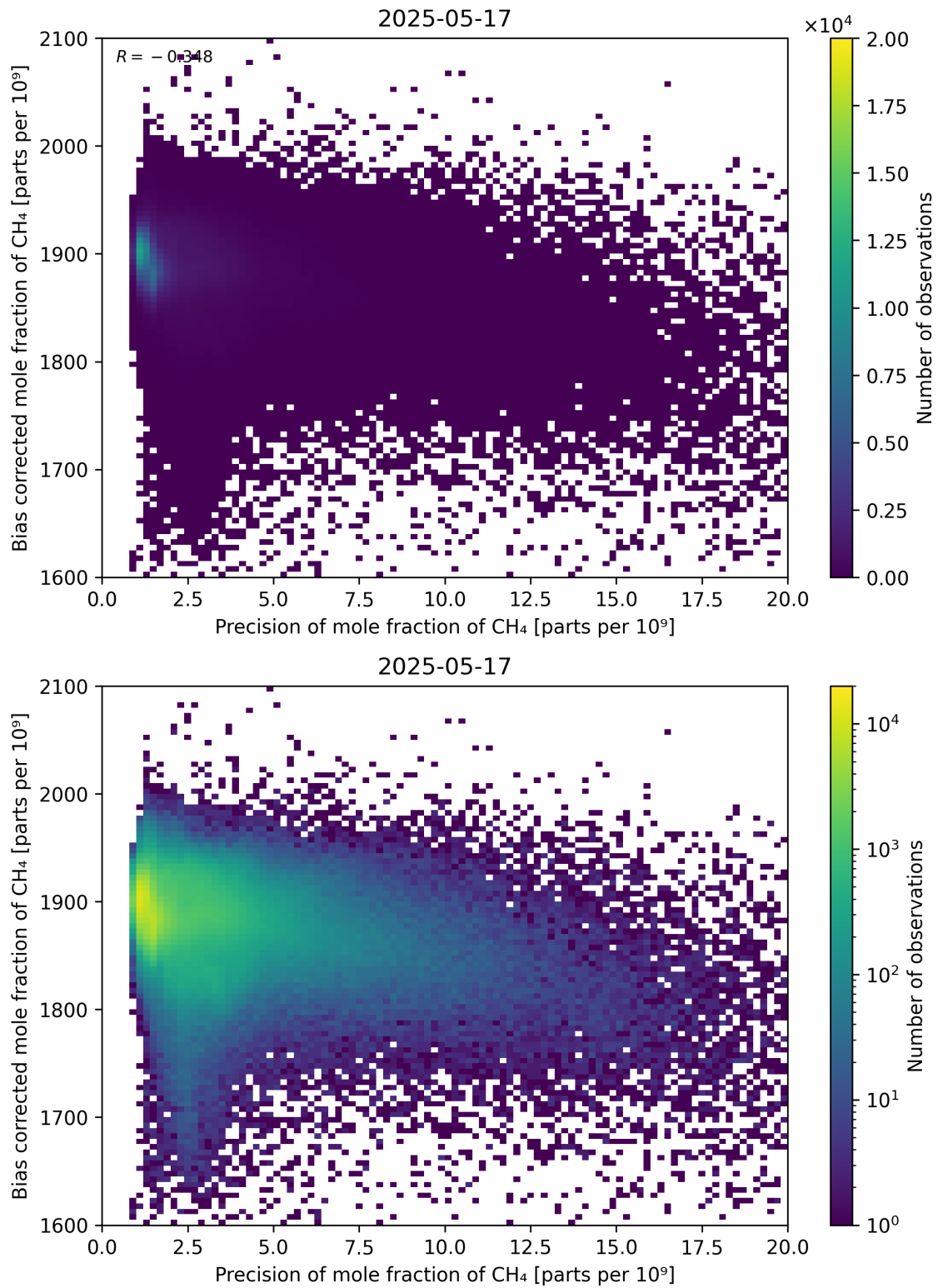
Figure 82: Scatter density plot of “Precision of mole fraction of CH 4 ” against “Bias corrected mole fraction of CH 4 ” for 2025-05-16 to 2025-05-18.
