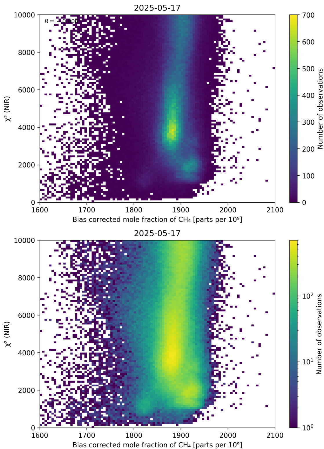
Figure 63: Scatter density plot of “Bias corrected mole fraction of \text{CH}_4 ” against “ \chi^2 (NIR)” for 2025-05-16 to 2025-05-18.
