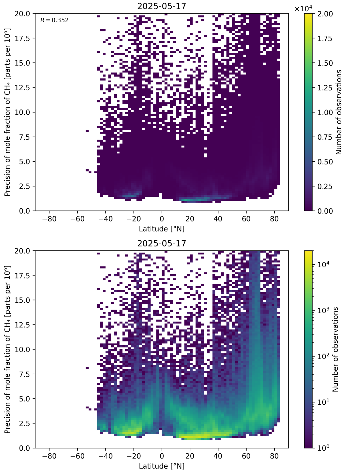
Figure 59: Scatter density plot of “Latitude” against “Precision of mole fraction of \text{CH}_4 ” for 2025-05-16 to 2025-05-18.
