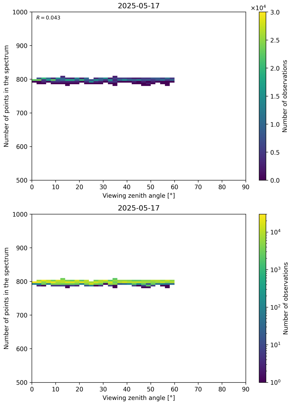
Figure 114: Scatter density plot of “Viewing zenith angle” against “Number of points in the spectrum” for 2025-05-16 to 2025-05-18.
