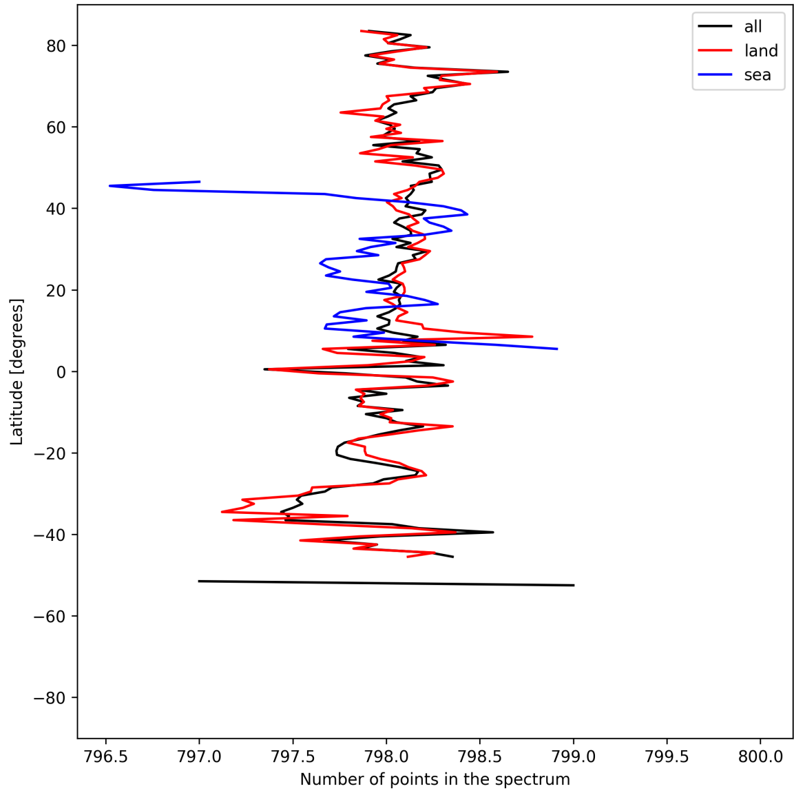
Figure 15: Zonal average of “Number of points in the spectrum” for 2025-05-16 to 2025-05-18.
