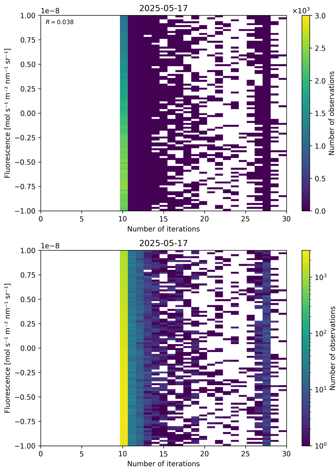
Figure 87: Scatter density plot of "Number of iterations" against "Fluorescence" for 2025-05-16 to 2025-05-18.
