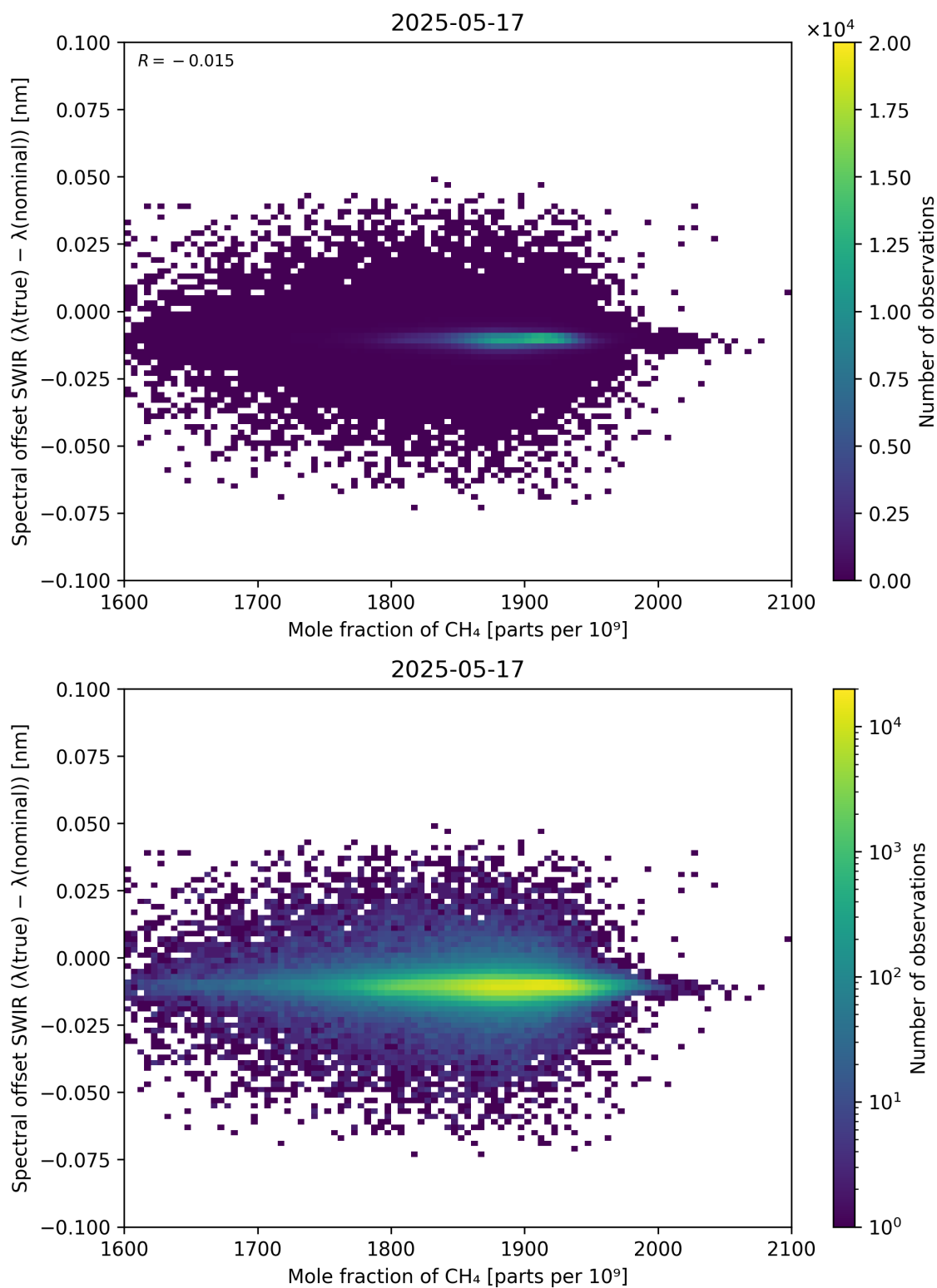
Figure 86: Scatter density plot of “Mole fraction of CH 4 ” against “Spectral offset SWIR ( \lambda_{\text{true}} - \lambda_{\text{nominal}} )” for 2025-05-16 to 2025-05-18.
