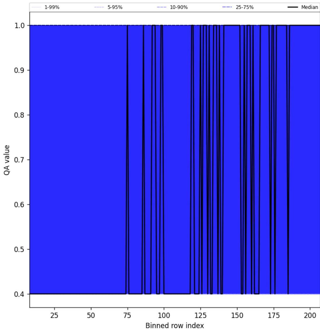
Figure 33: Along track statistics of “QA value” for 2025-05-16 to 2025-05-18
