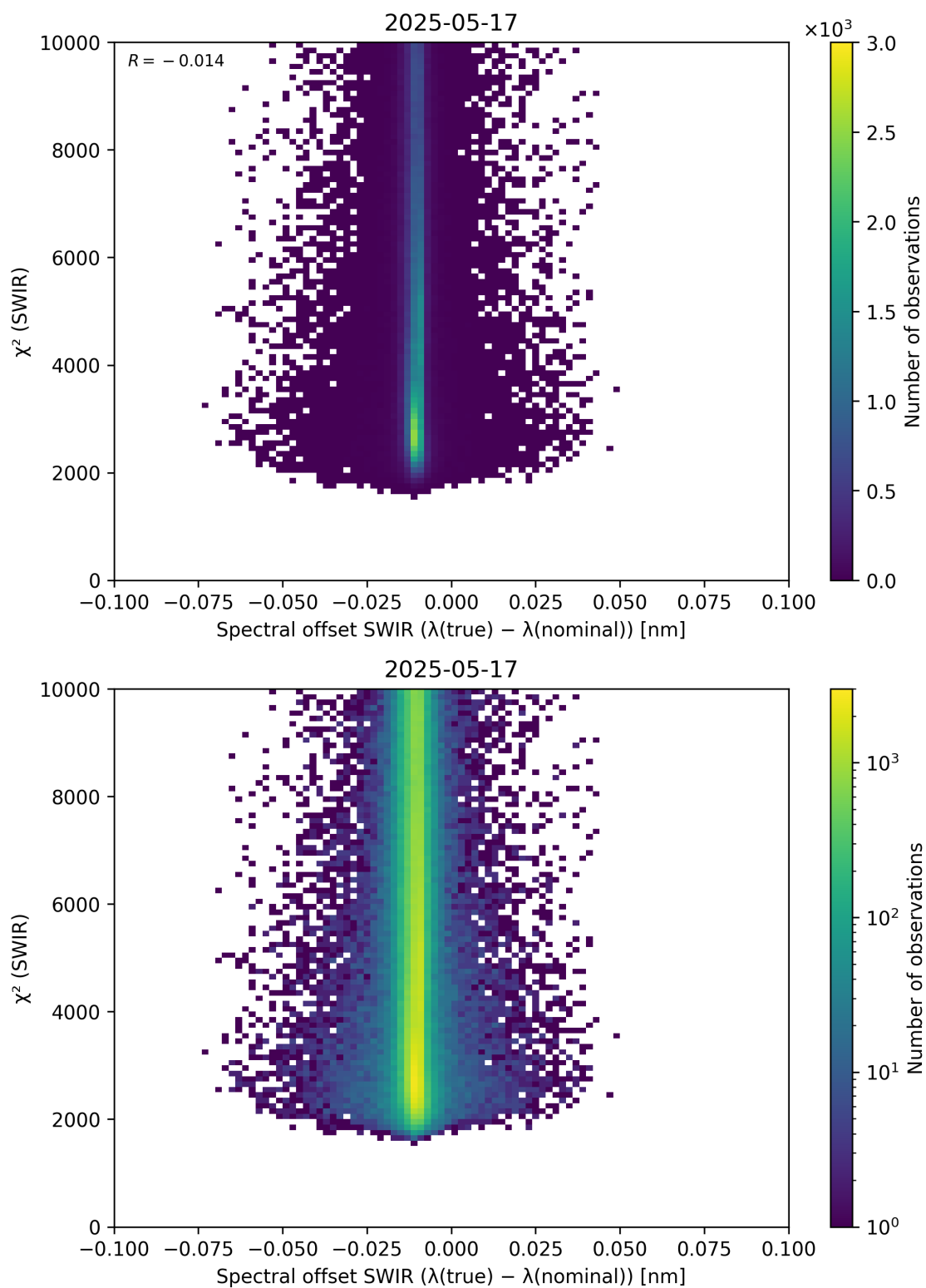
Figure 118: Scatter density plot of “Spectral offset SWIR ( \lambda_{\text{true}} - \lambda_{\text{nominal}} )” against “ \chi^2 (SWIR)” for 2025-05-16 to 2025-05-18.
