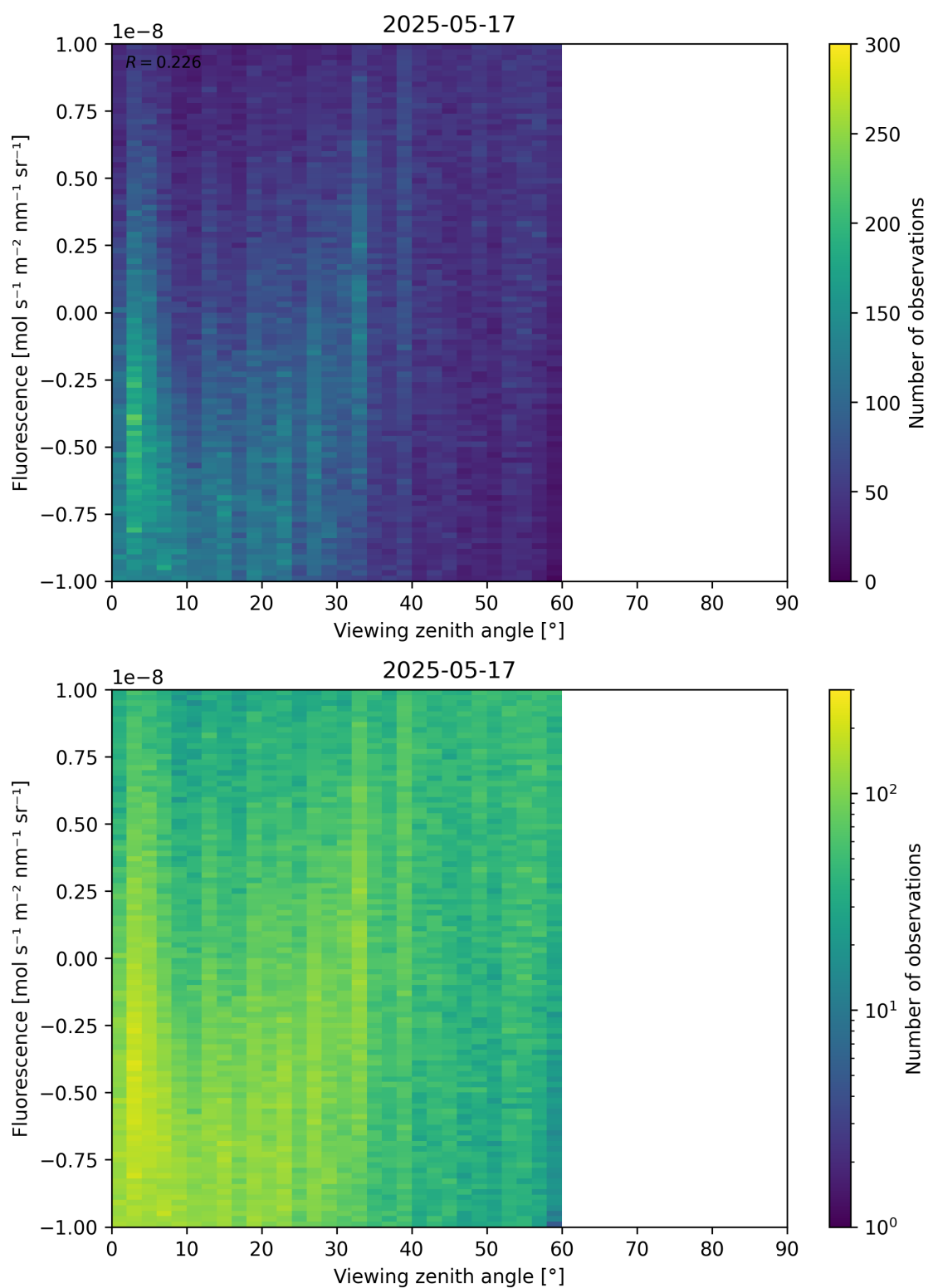
Figure 108: Scatter density plot of “Viewing zenith angle” against “Fluorescence” for 2025-05-16 to 2025-05-18.
