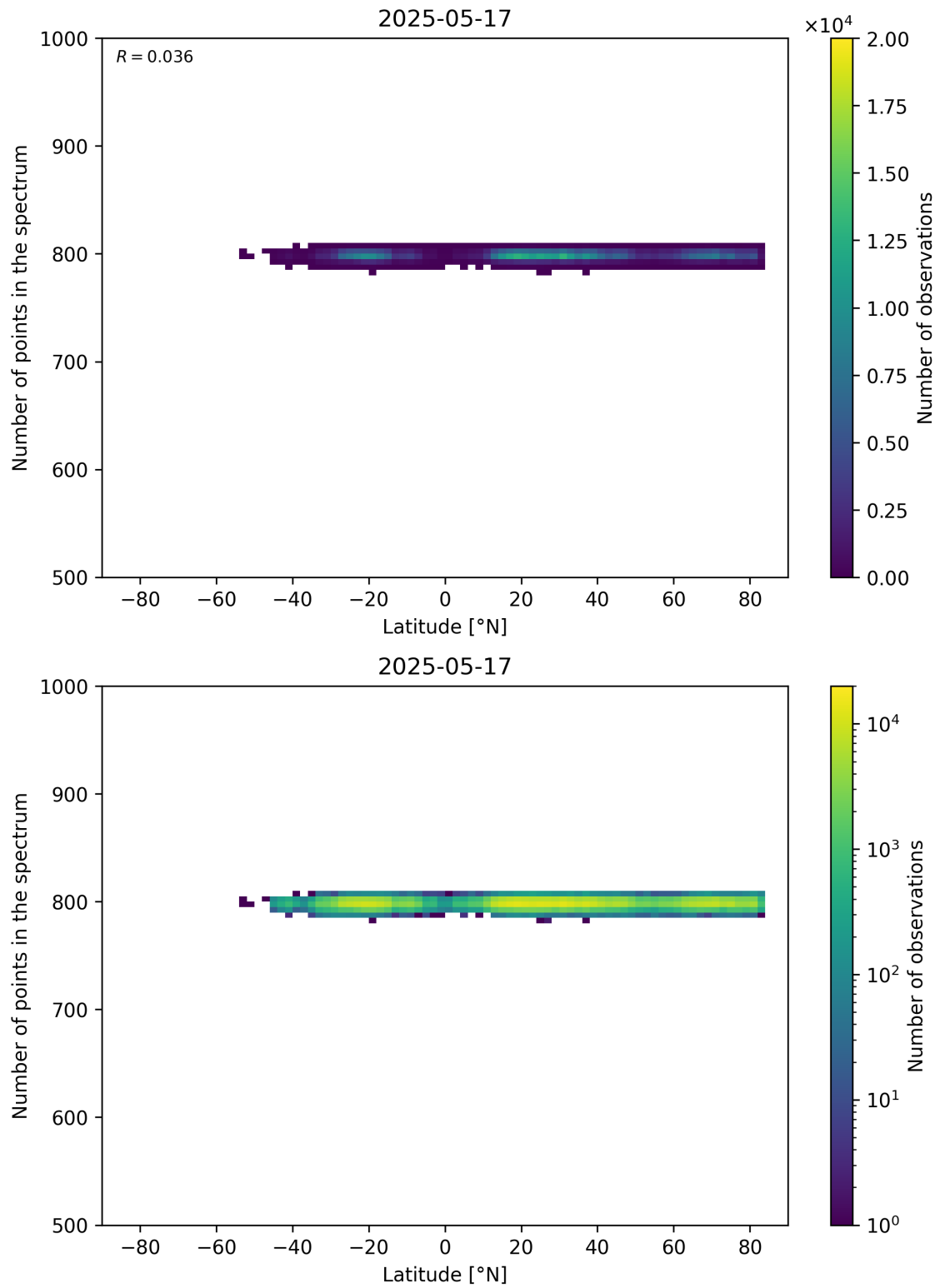
Figure 61: Scatter density plot of “Latitude” against “Number of points in the spectrum” for 2025-05-16 to 2025-05-18.
