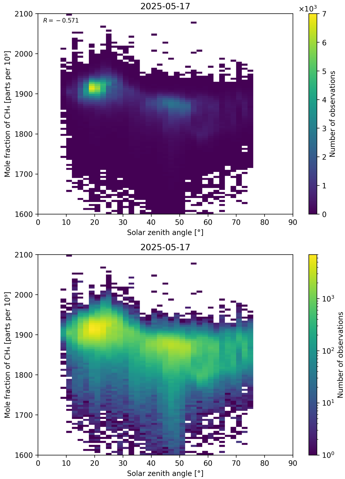
Figure 99: Scatter density plot of “Solar zenith angle” against “Mole fraction of \text{CH}_4 ” for 2025-05-16 to 2025-05-18.
