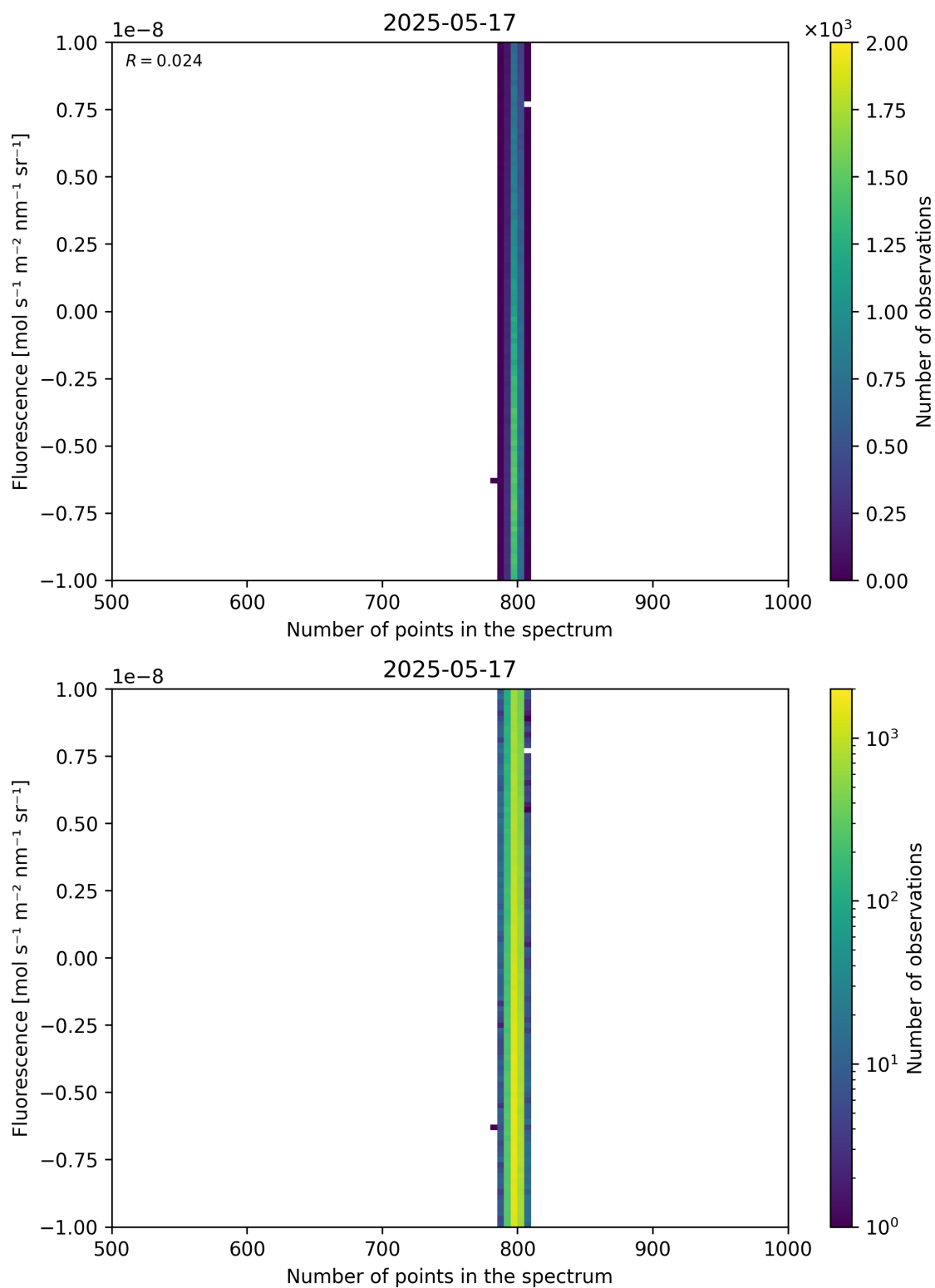
Figure 91: Scatter density plot of “Number of points in the spectrum” against “Fluorescence” for 2025-05-16 to 2025-05-18.
