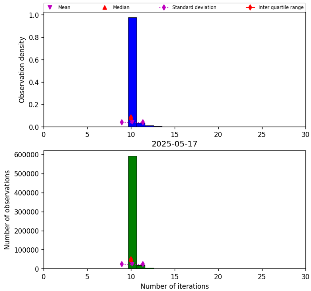
Figure 31: Histogram of “Number of iterations” for 2025-05-16 to 2025-05-18
