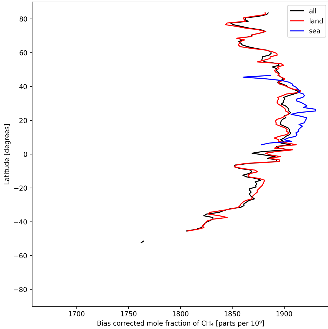
Figure 14: Zonal average of “Bias corrected mole fraction of CH 4 ” for 2025-05-16 to 2025-05-18.
