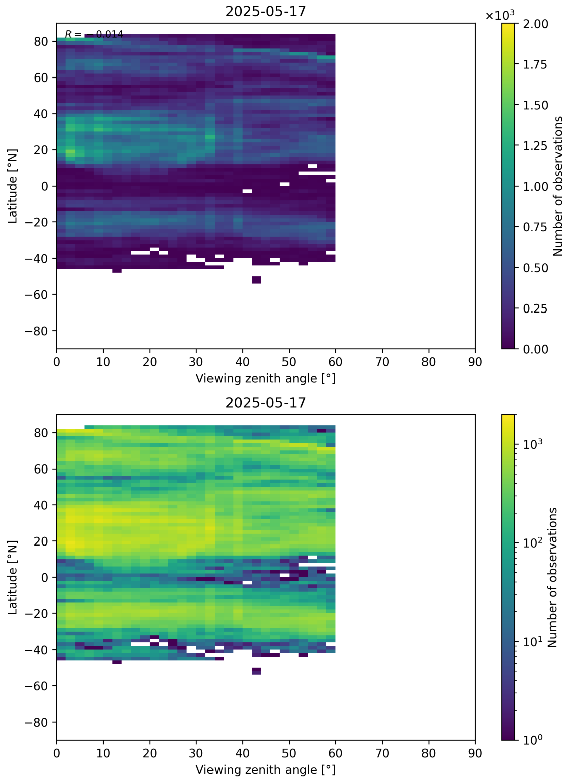
Figure 109: Scatter density plot of “Viewing zenith angle” against “Latitude” for 2025-05-16 to 2025-05-18.
