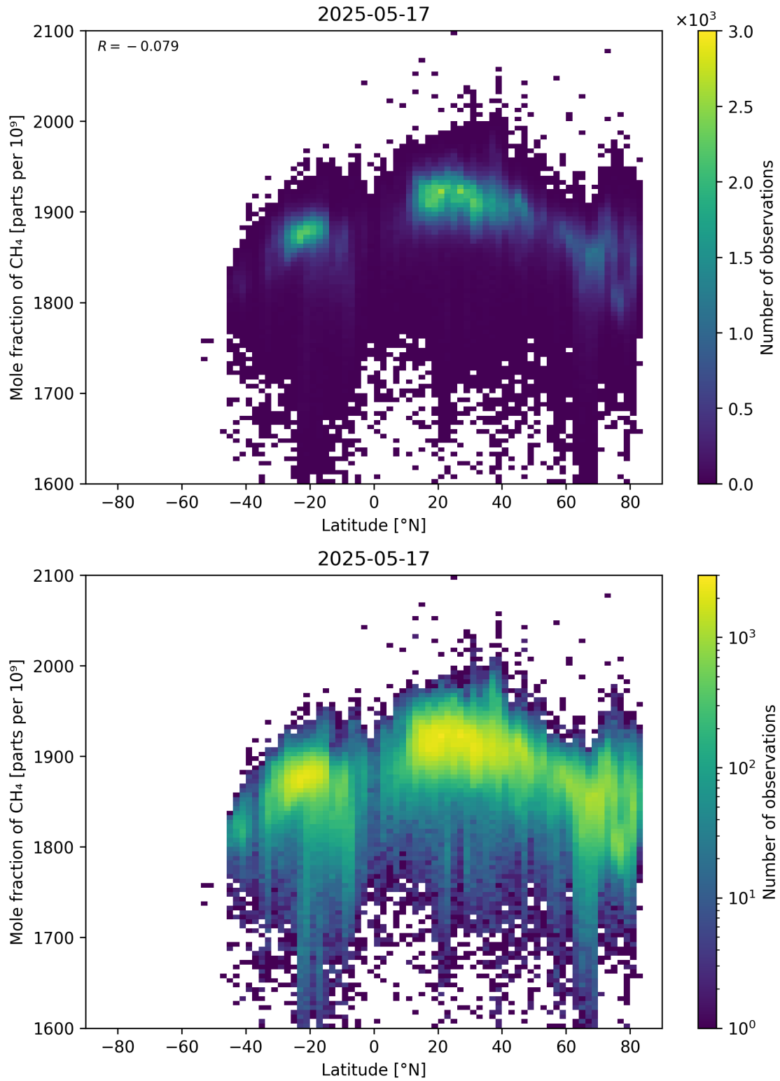
Figure 57: Scatter density plot of “Latitude” against “Mole fraction of CH 4 ” for 2025-05-16 to 2025-05-18.
