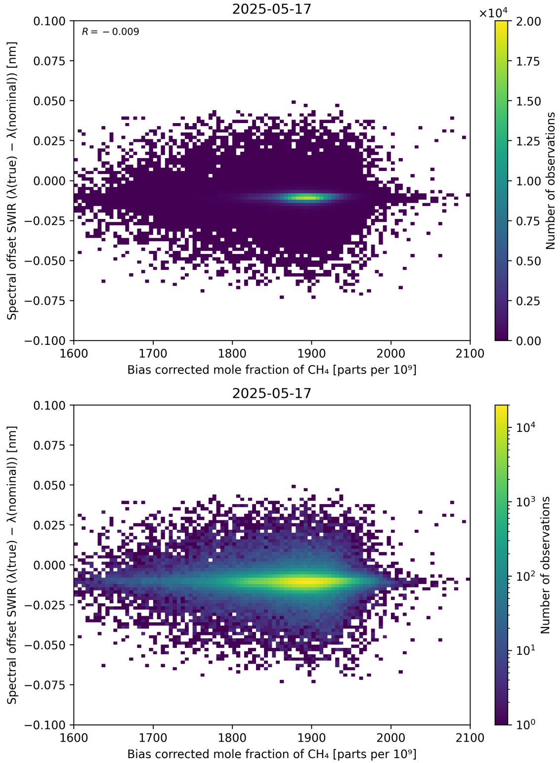
Figure 69: Scatter density plot of “Bias corrected mole fraction of CH 4 ” against “Spectral offset SWIR ( \lambda_{\text{true}} - \lambda_{\text{nominal}} )” for 2025-05-16 to 2025-05-18.
