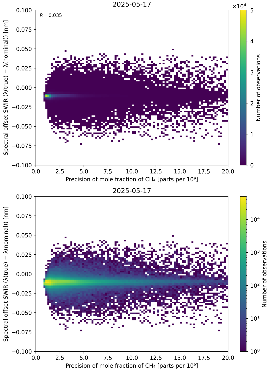
Figure 85: Scatter density plot of “Precision of mole fraction of CH 4 ” against “Spectral offset SWIR ( \lambda_{\text{true}} - \lambda_{\text{nominal}} )” for 2025-05-16 to 2025-05-18.
