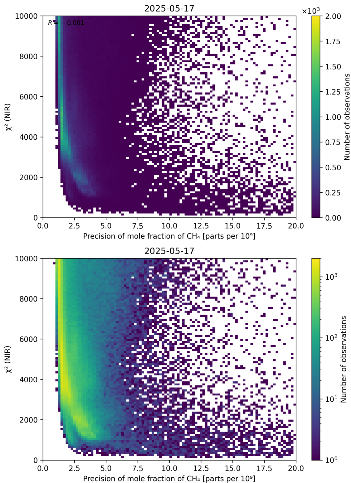
Figure 78: Scatter density plot of “Precision of mole fraction of \text{CH}_4 ” against “ \chi^2 (NIR)” for 2025-05-16 to 2025-05-18.
