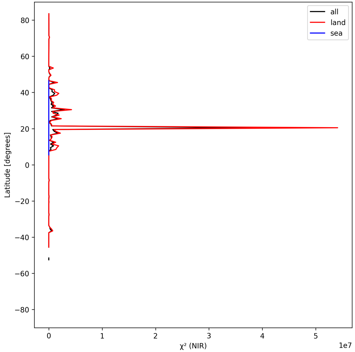
Figure 18: Zonal average of “ \chi^2 (NIR)” for 2025-05-16 to 2025-05-18.
