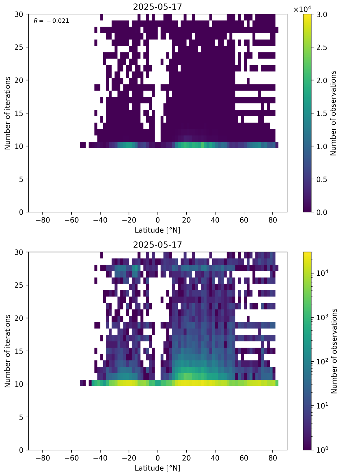
Figure 60: Scatter density plot of “Latitude” against “Number of iterations” for 2025-05-16 to 2025-05-18.
