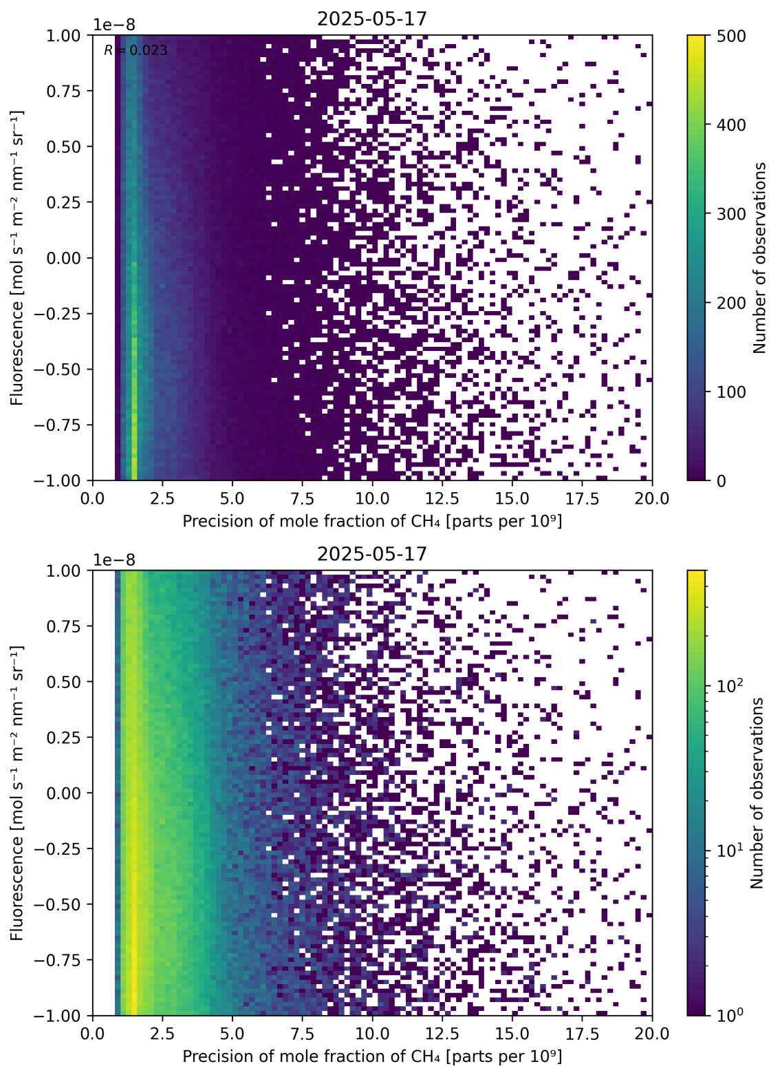
Figure 81: Scatter density plot of “Precision of mole fraction of \text{CH}_4 ” against “Fluorescence” for 2025-05-16 to 2025-05-18.
