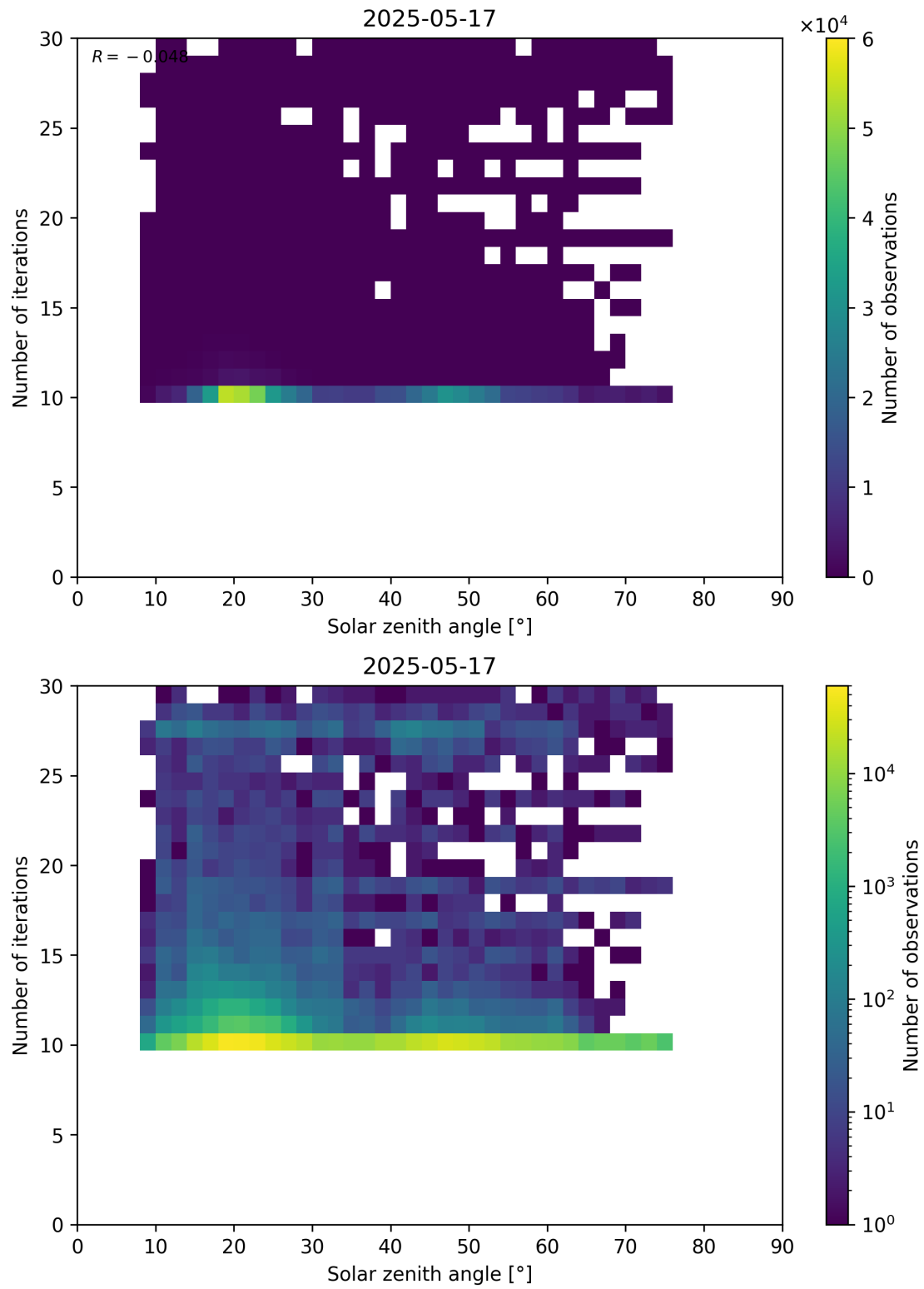
Figure 102: Scatter density plot of “Solar zenith angle” against “Number of iterations” for 2025-05-16 to 2025-05-18.
