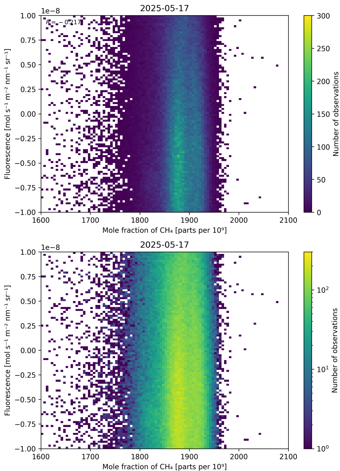
Figure 73: Scatter density plot of “Mole fraction of \text{CH}_4 ” against “Fluorescence” for 2025-05-16 to 2025-05-18.
