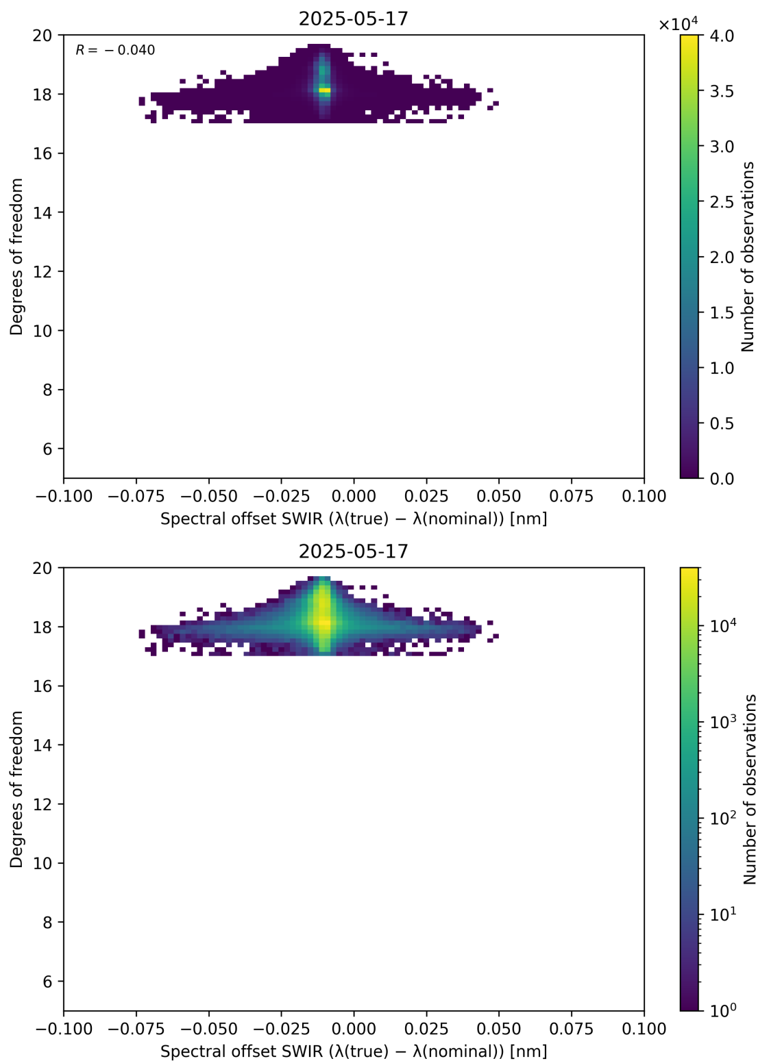
Figure 119: Scatter density plot of “Spectral offset SWIR ( \lambda_{\text{true}} - \lambda_{\text{nominal}} )” against “Degrees of freedom” for 2025-05-16 to 2025-05-18.
