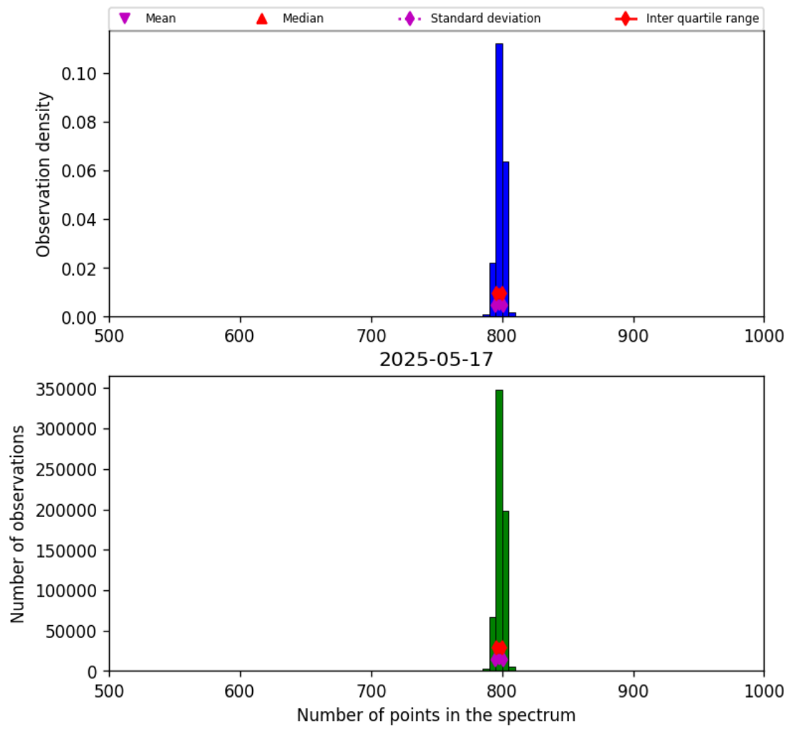
Figure 26: Histogram of “Number of points in the spectrum” for 2025-05-16 to 2025-05-18
