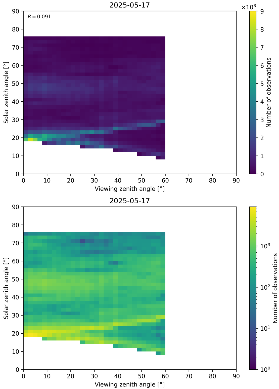
Figure 115: Scatter density plot of “Viewing zenith angle” against “Solar zenith angle” for 2025-05-16 to 2025-05-18.
