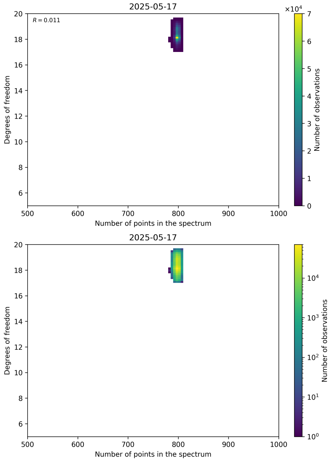
Figure 90: Scatter density plot of “Number of points in the spectrum” against “Degrees of freedom” for 2025-05-16 to 2025-05-18.
