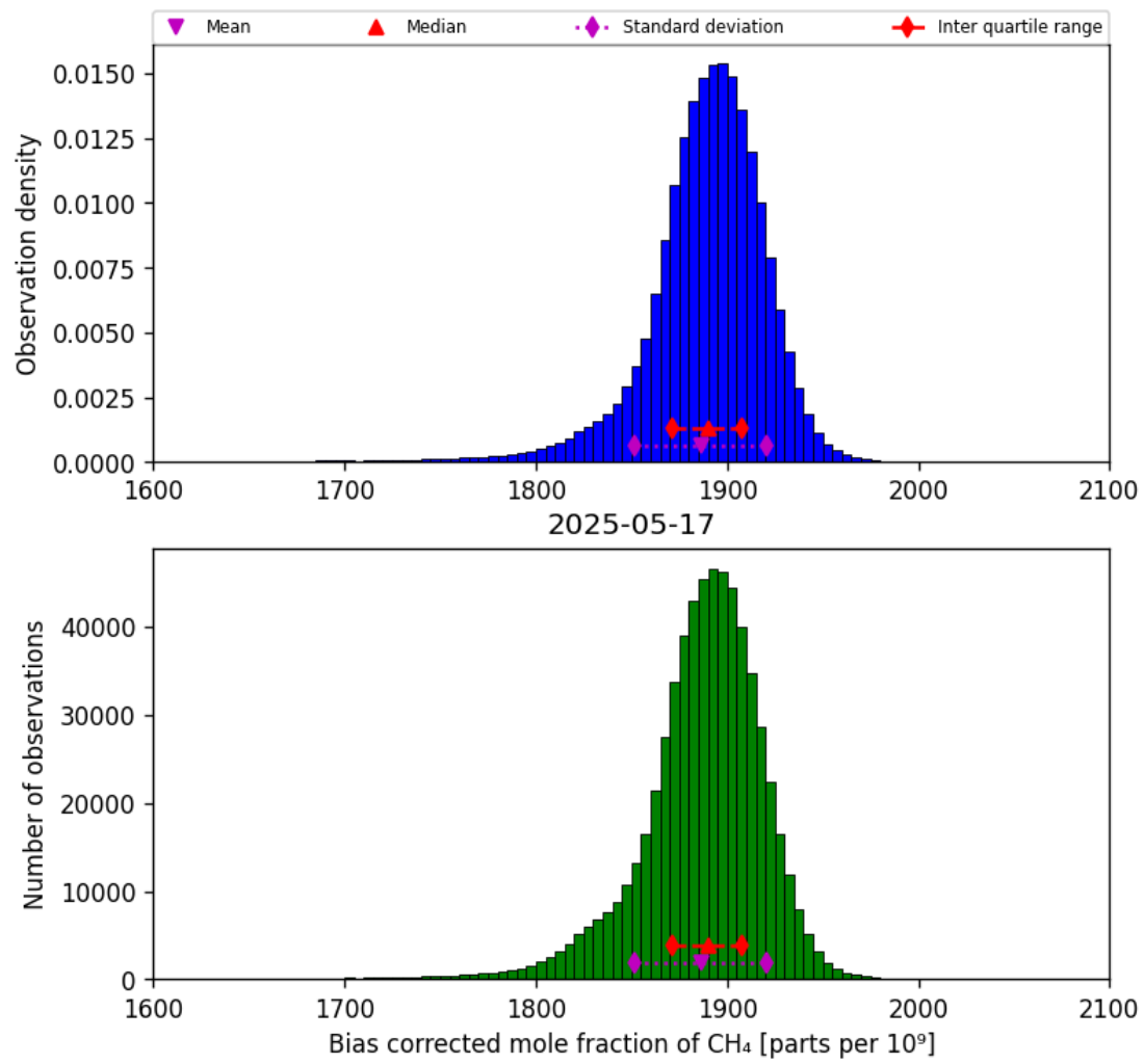
Figure 25: Histogram of “Bias corrected mole fraction of CH 4 ” for 2025-05-16 to 2025-05-18
