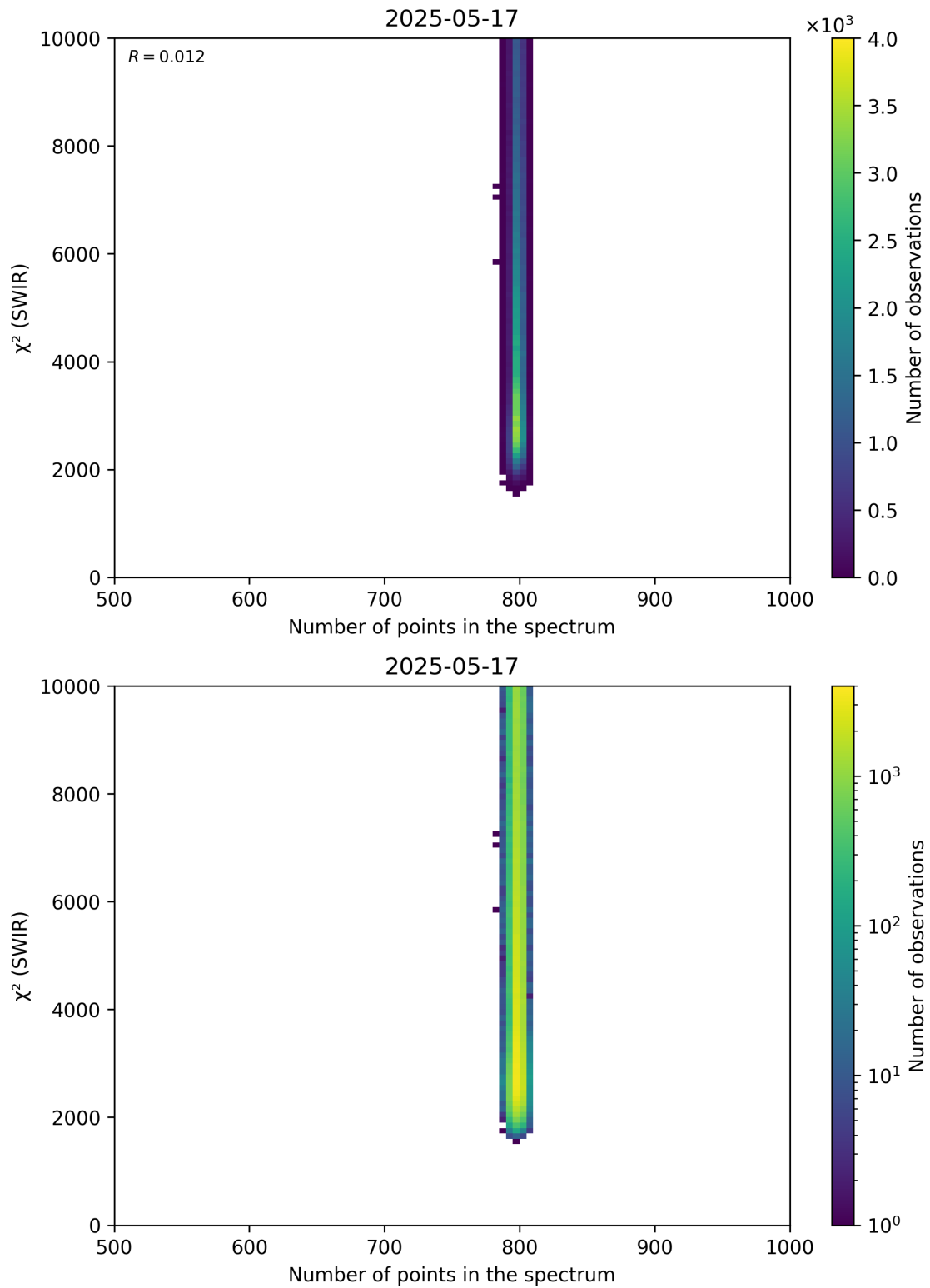
Figure 89: Scatter density plot of “Number of points in the spectrum” against “ \chi^2 (SWIR)” for 2025-05-16 to 2025-05-18.
