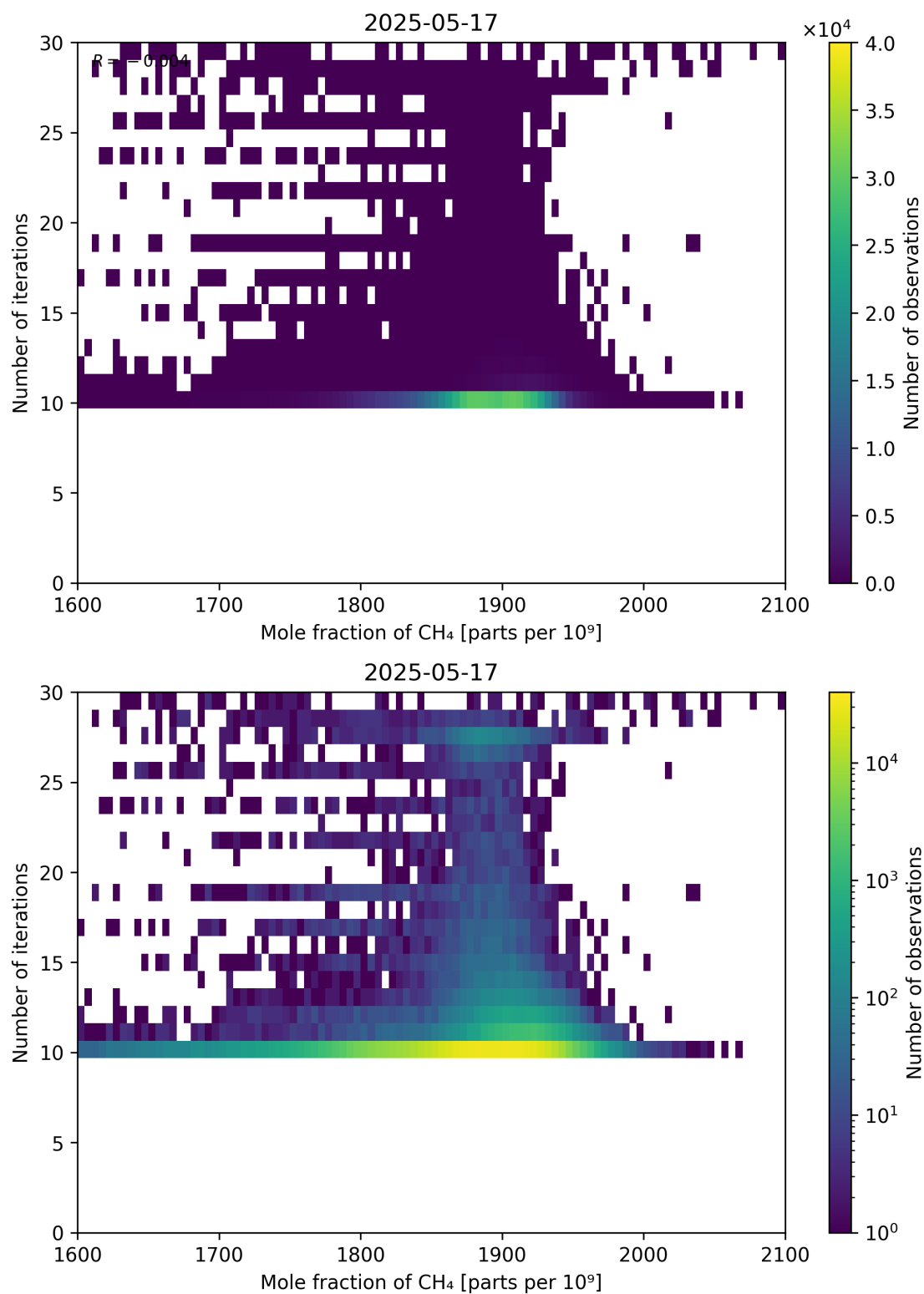
Figure 76: Scatter density plot of “Mole fraction of CH 4 ” against “Number of iterations” for 2025-05-16 to 2025-05-18.
