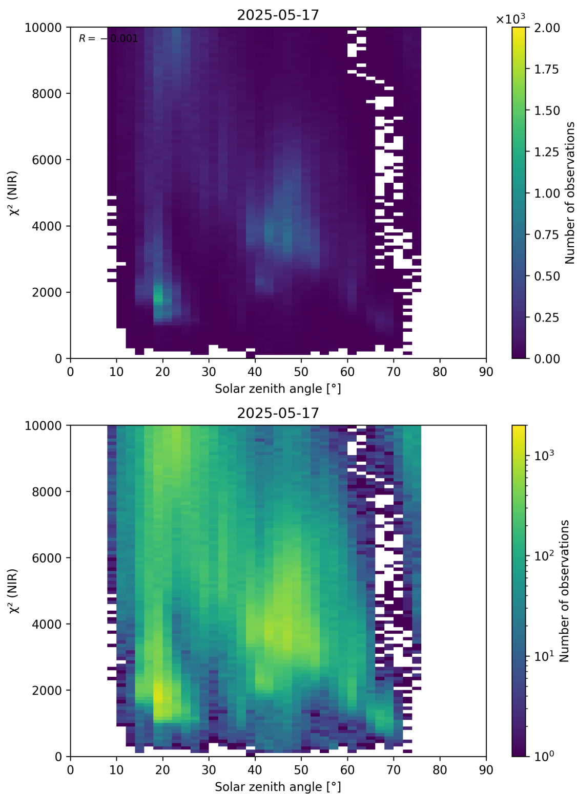
Figure 94: Scatter density plot of “Solar zenith angle” against “ \chi^2 (NIR)” for 2025-05-16 to 2025-05-18.
