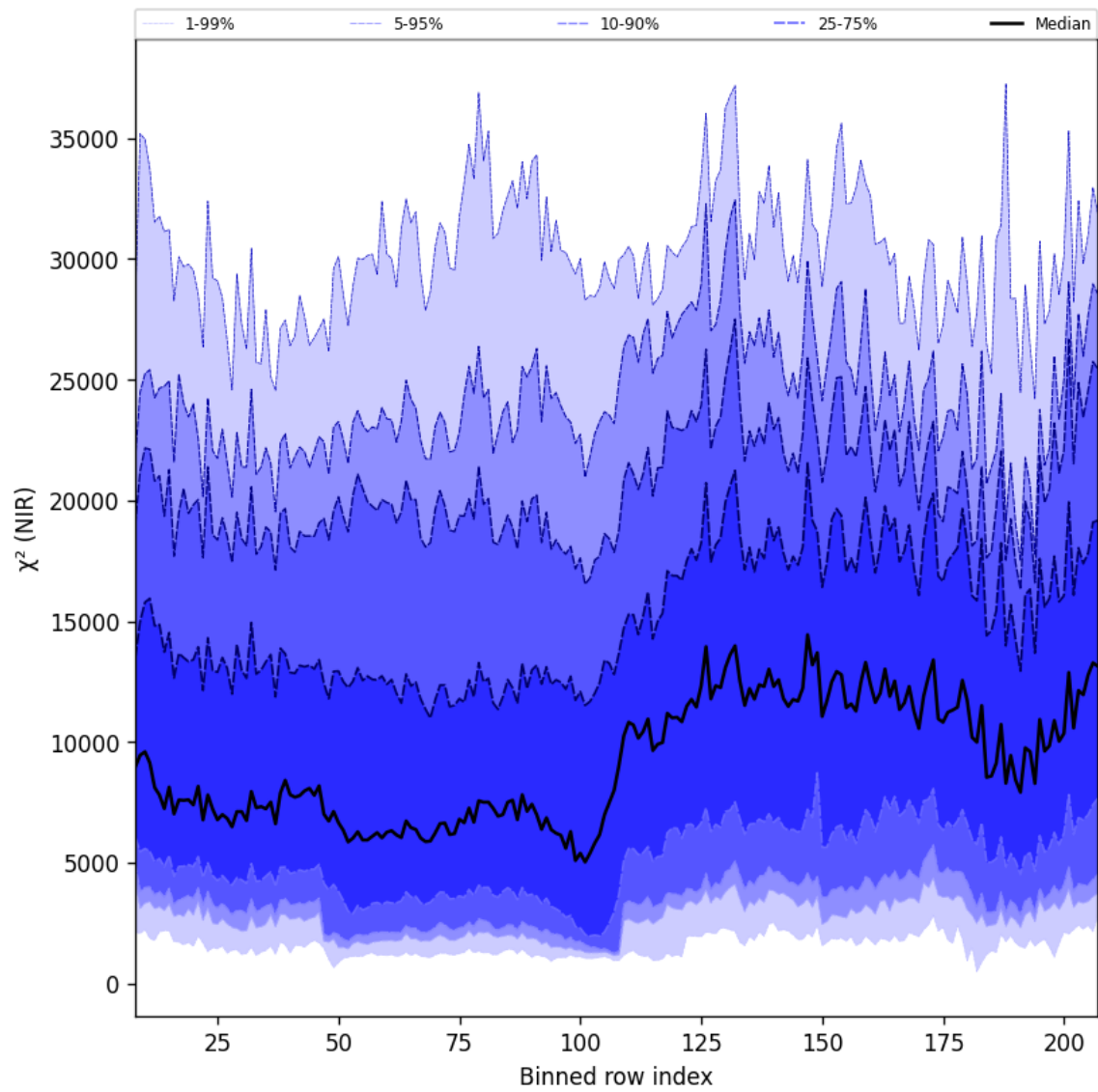
Figure 40: Along track statistics of “ \chi^2 (NIR)” for 2025-05-16 to 2025-05-18
