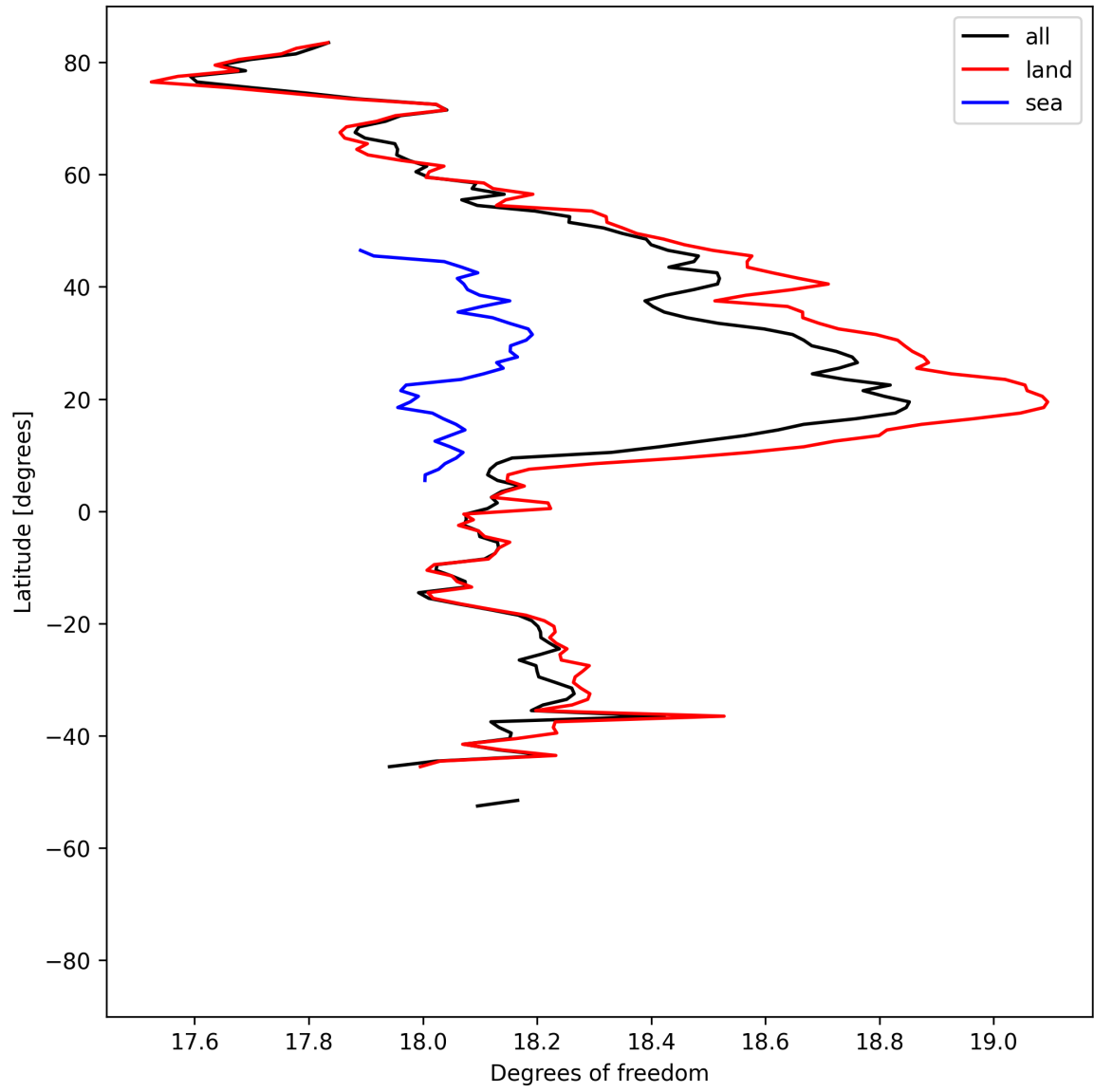
Figure 19: Zonal average of “Degrees of freedom” for 2025-05-16 to 2025-05-18.
