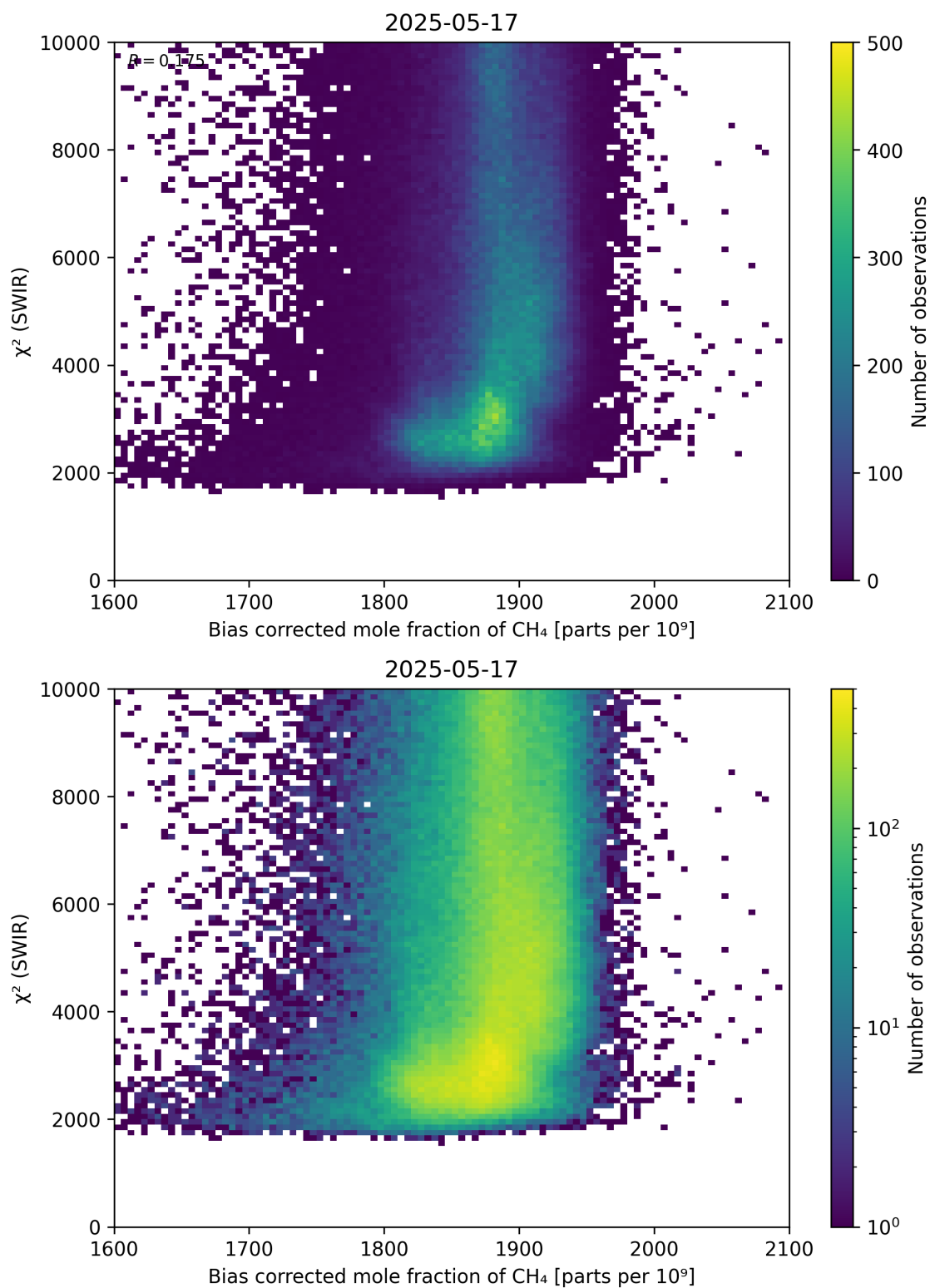
Figure 64: Scatter density plot of “Bias corrected mole fraction of \text{CH}_4 ” against “ \chi^2 (SWIR)” for 2025-05-16 to 2025-05-18.
