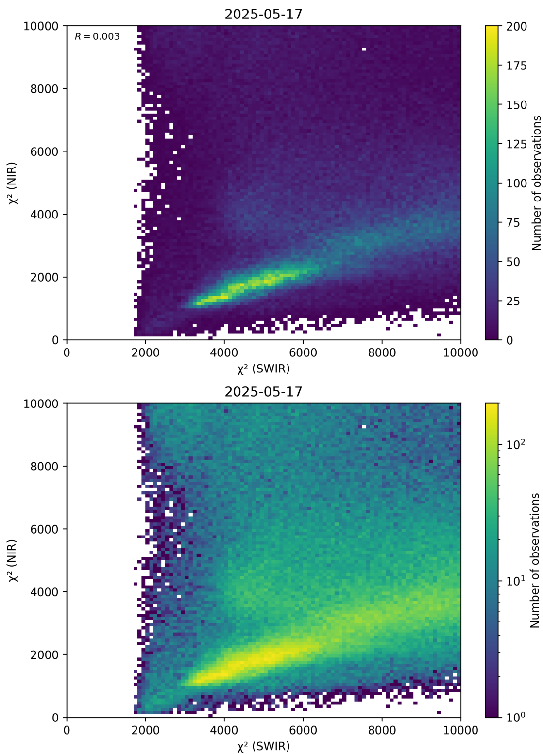
Figure 47: Scatter density plot of “ \chi^2 (SWIR)” against “ \chi^2 (NIR)” for 2025-05-16 to 2025-05-18.
