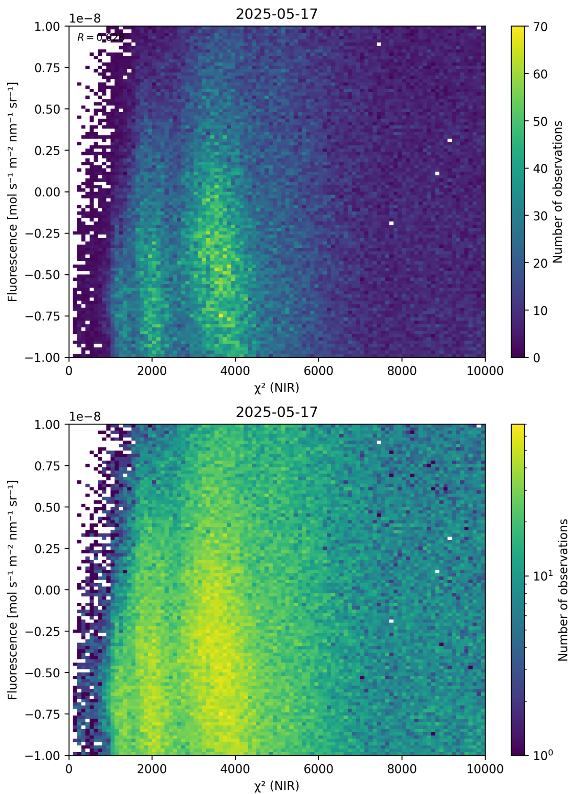
Figure 45: Scatter density plot of “ \chi^2 (NIR)” against “Fluorescence” for 2025-05-16 to 2025-05-18.
