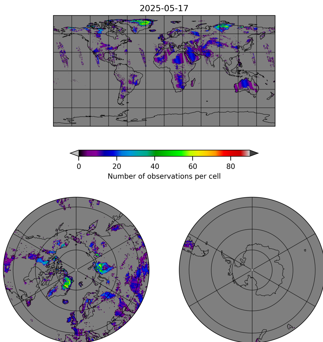
Figure 10: Map of the number of observations for 2025-05-16 to 2025-05-18
