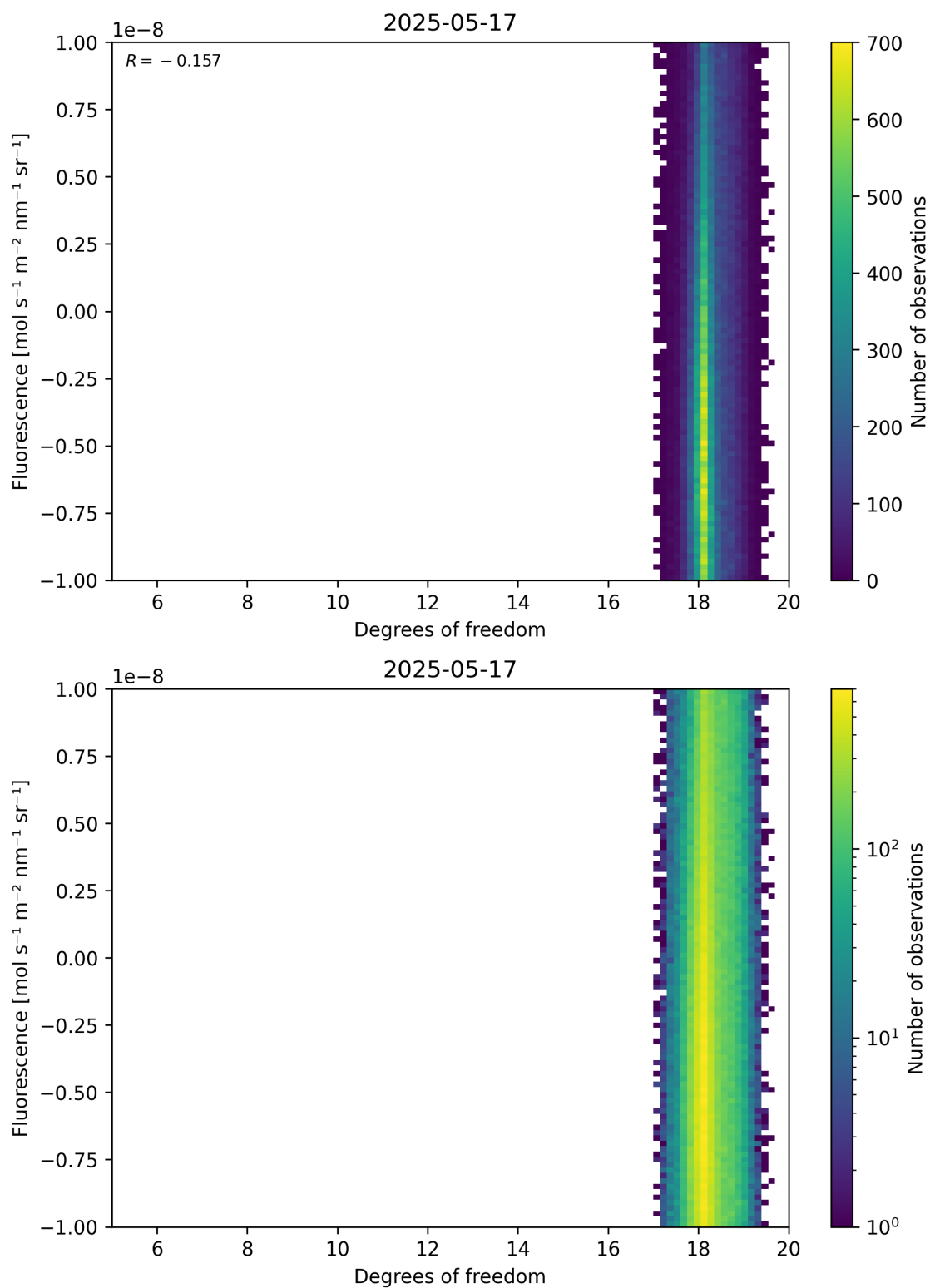
Figure 51: Scatter density plot of “Degrees of freedom” against “Fluorescence” for 2025-05-16 to 2025-05-18.
