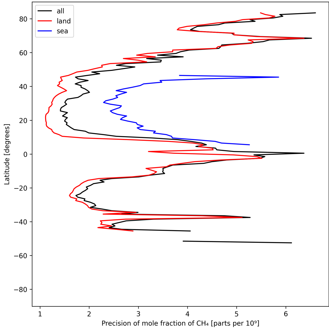
Figure 13: Zonal average of “Precision of mole fraction of CH 4 ” for 2025-05-16 to 2025-05-18.
