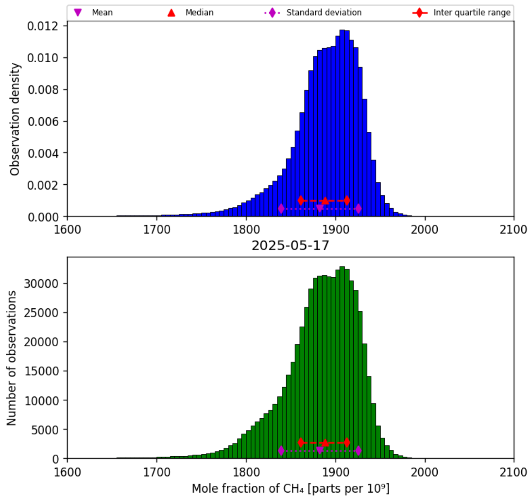
Figure 23: Histogram of “Mole fraction of CH 4 ” for 2025-05-16 to 2025-05-18
