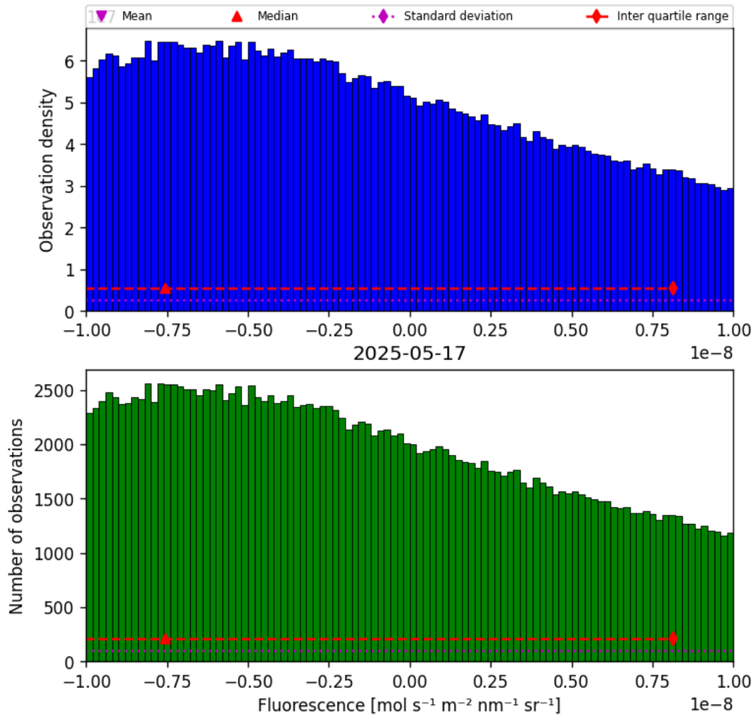
Figure 32: Histogram of “Fluorescence” for 2025-05-16 to 2025-05-18
