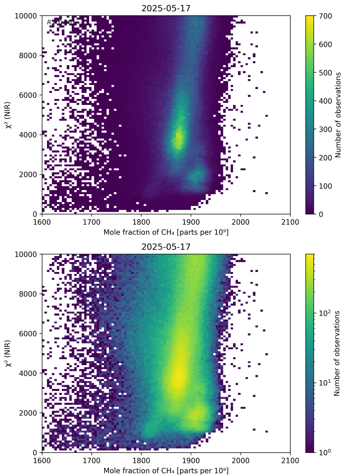
Figure 70: Scatter density plot of “Mole fraction of CH 4 ” against “ \chi^2 (NIR)” for 2025-05-16 to 2025-05-18.
