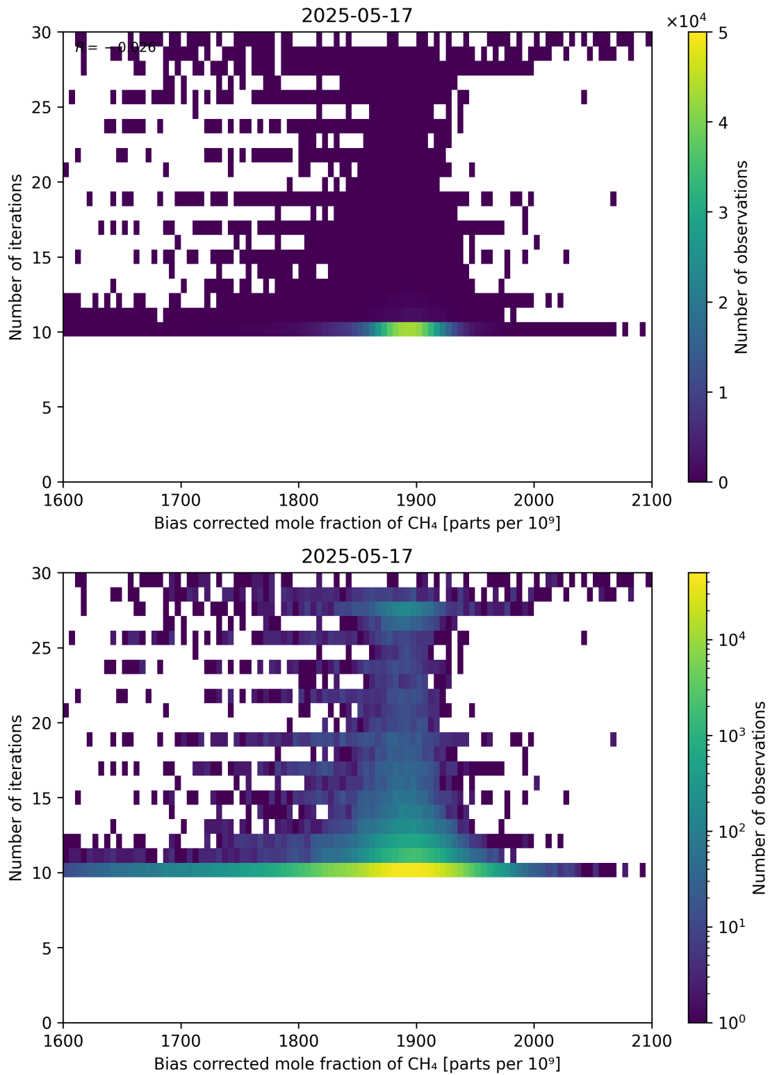
Figure 67: Scatter density plot of “Bias corrected mole fraction of CH 4 ” against “Number of iterations” for 2025-05-16 to 2025-05-18.
