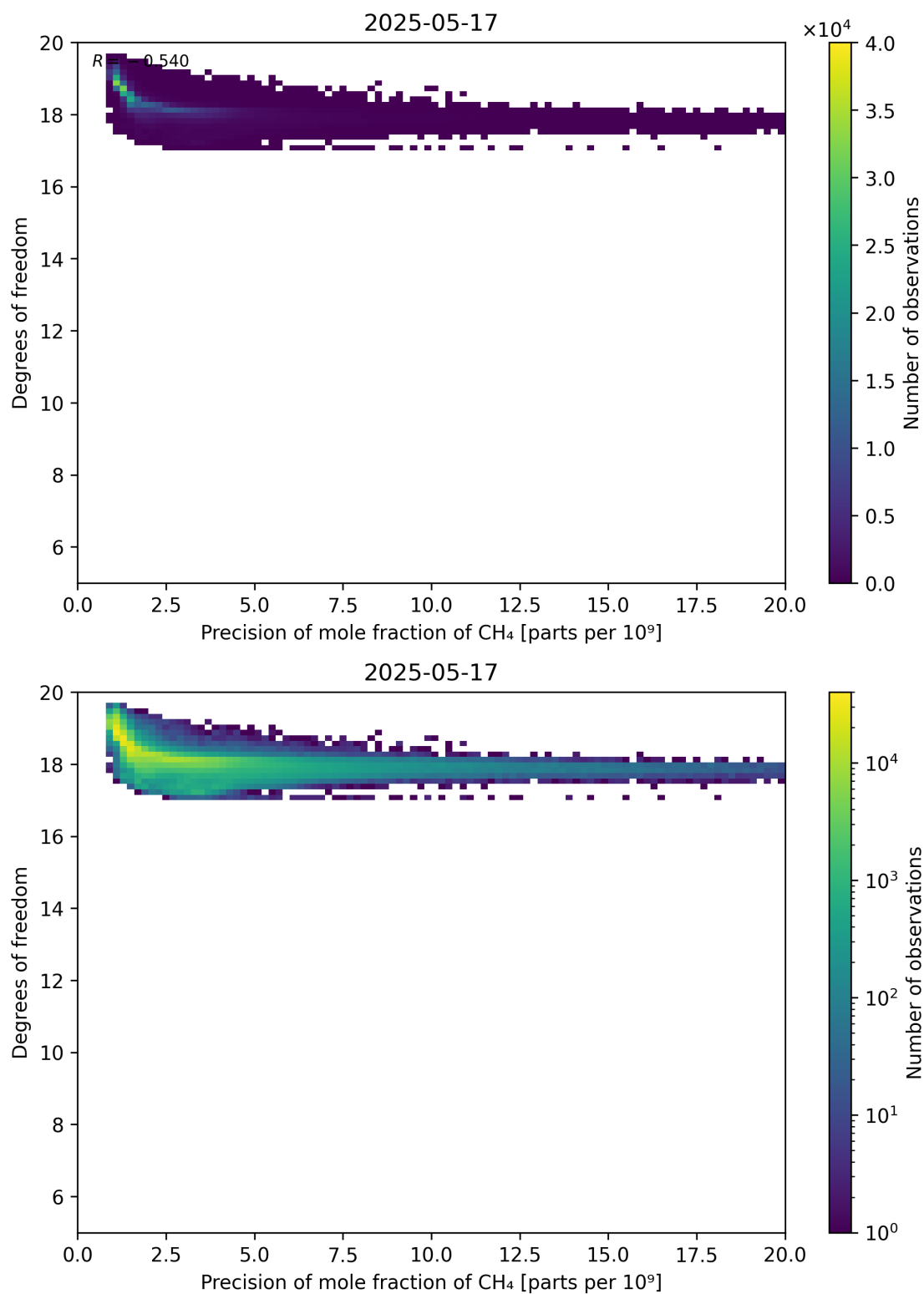
Figure 80: Scatter density plot of “Precision of mole fraction of CH 4 ” against “Degrees of freedom” for 2025-05-16 to 2025-05-18.
