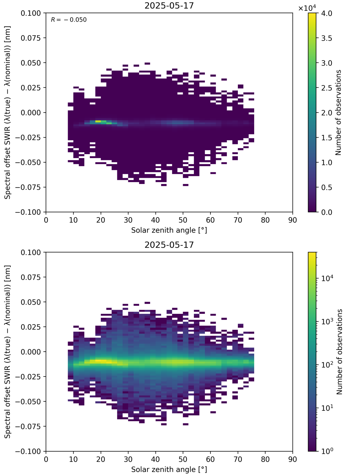
Figure 104: Scatter density plot of “Solar zenith angle” against “Spectral offset SWIR ( \lambda_{\text{true}} - \lambda_{\text{nominal}} )” for 2025-05-16 to 2025-05-18.
