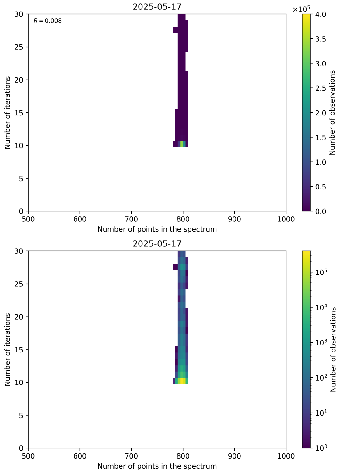
Figure 92: Scatter density plot of “Number of points in the spectrum” against “Number of iterations” for 2025-05-16 to 2025-05-18.
