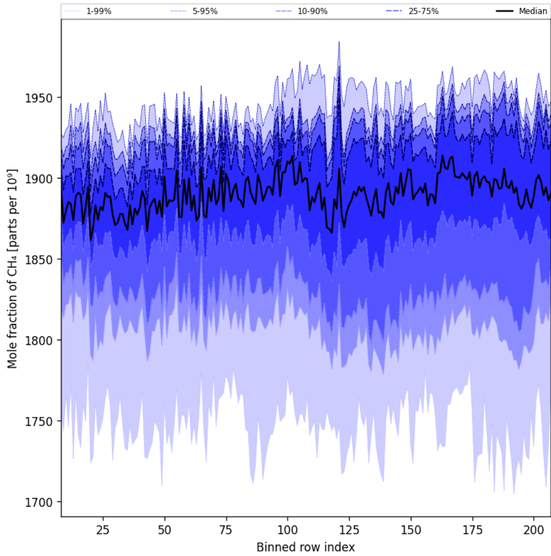
Figure 34: Along track statistics of “Mole fraction of CH 4 ” for 2025-05-16 to 2025-05-18
