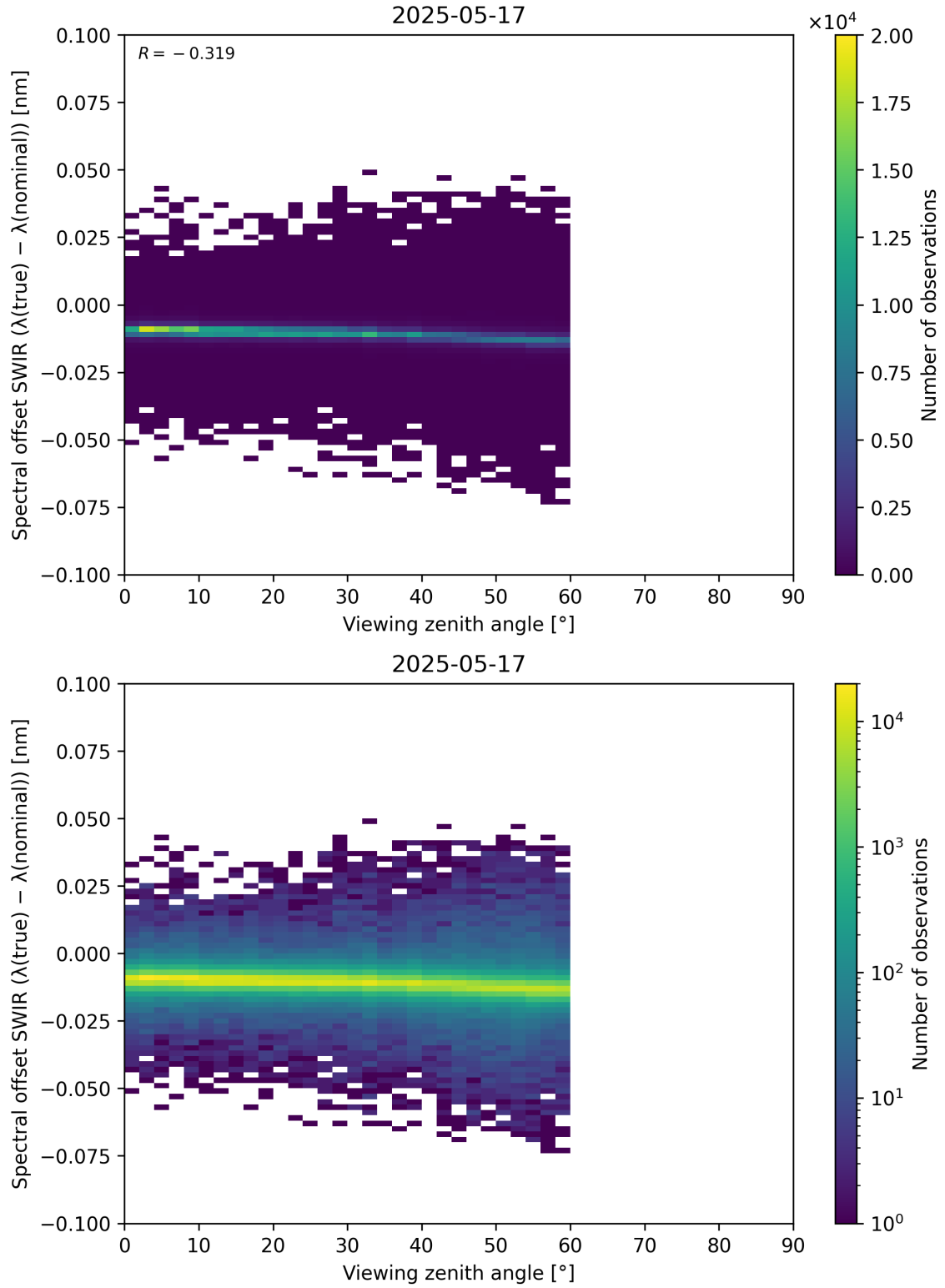
Figure 116: Scatter density plot of “Viewing zenith angle” against “Spectral offset SWIR ( \lambda_{\text{true}} - \lambda_{\text{nominal}} )” for 2025-05-16 to 2025-05-18.
