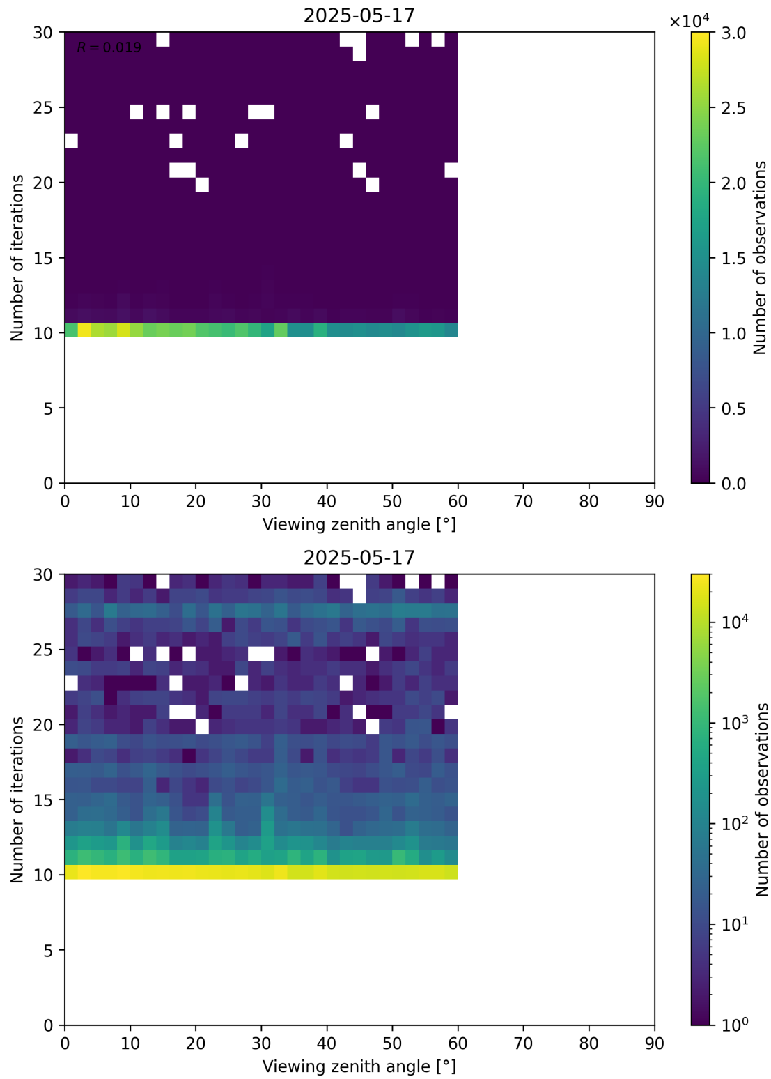
Figure 113: Scatter density plot of “Viewing zenith angle” against “Number of iterations” for 2025-05-16 to 2025-05-18.
