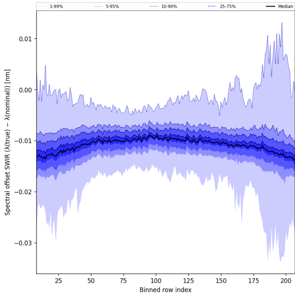
Figure 38: Along track statistics of “Spectral offset SWIR ( \lambda_{\text{true}} - \lambda_{\text{nominal}} )” for 2025-05-16 to 2025-05-18
