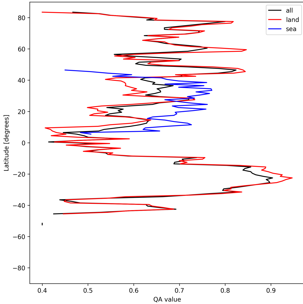
Figure 11: Zonal average of “QA value” for 2025-05-16 to 2025-05-18.
