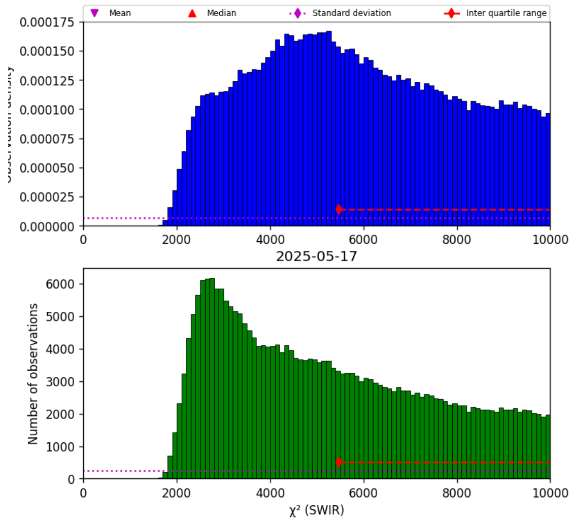
Figure 28: Histogram of “ \chi^2 (SWIR)” for 2025-05-16 to 2025-05-18
