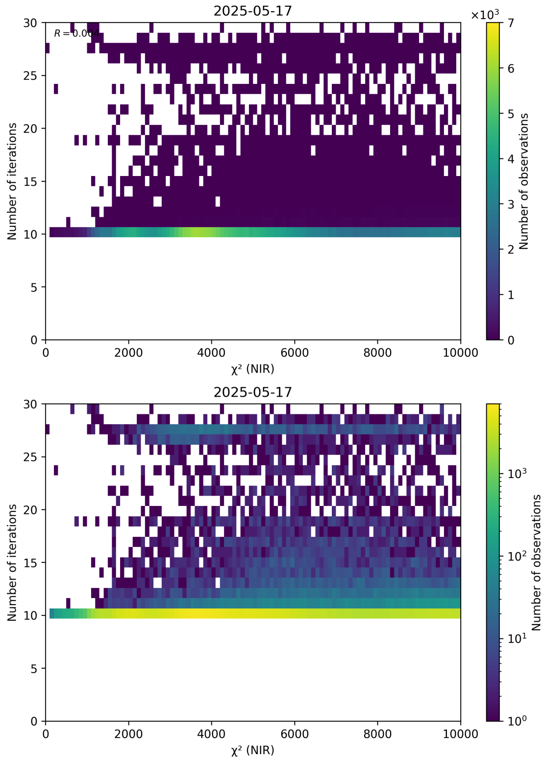
Figure 46: Scatter density plot of “ \chi^2 (NIR)” against “Number of iterations” for 2025-05-16 to 2025-05-18.
