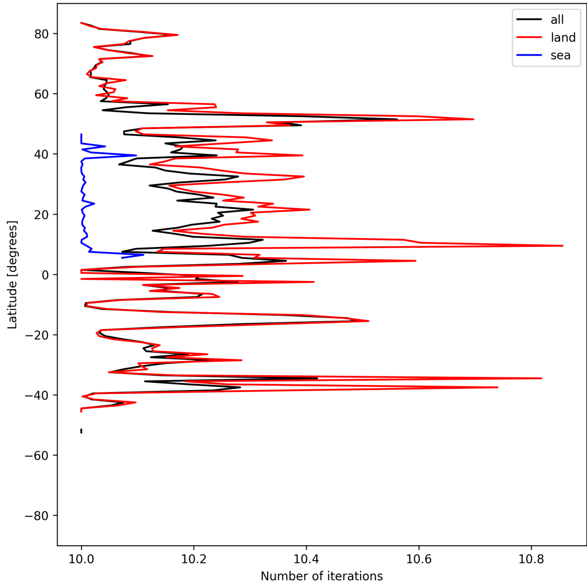
Figure 20: Zonal average of “Number of iterations” for 2025-05-16 to 2025-05-18.
