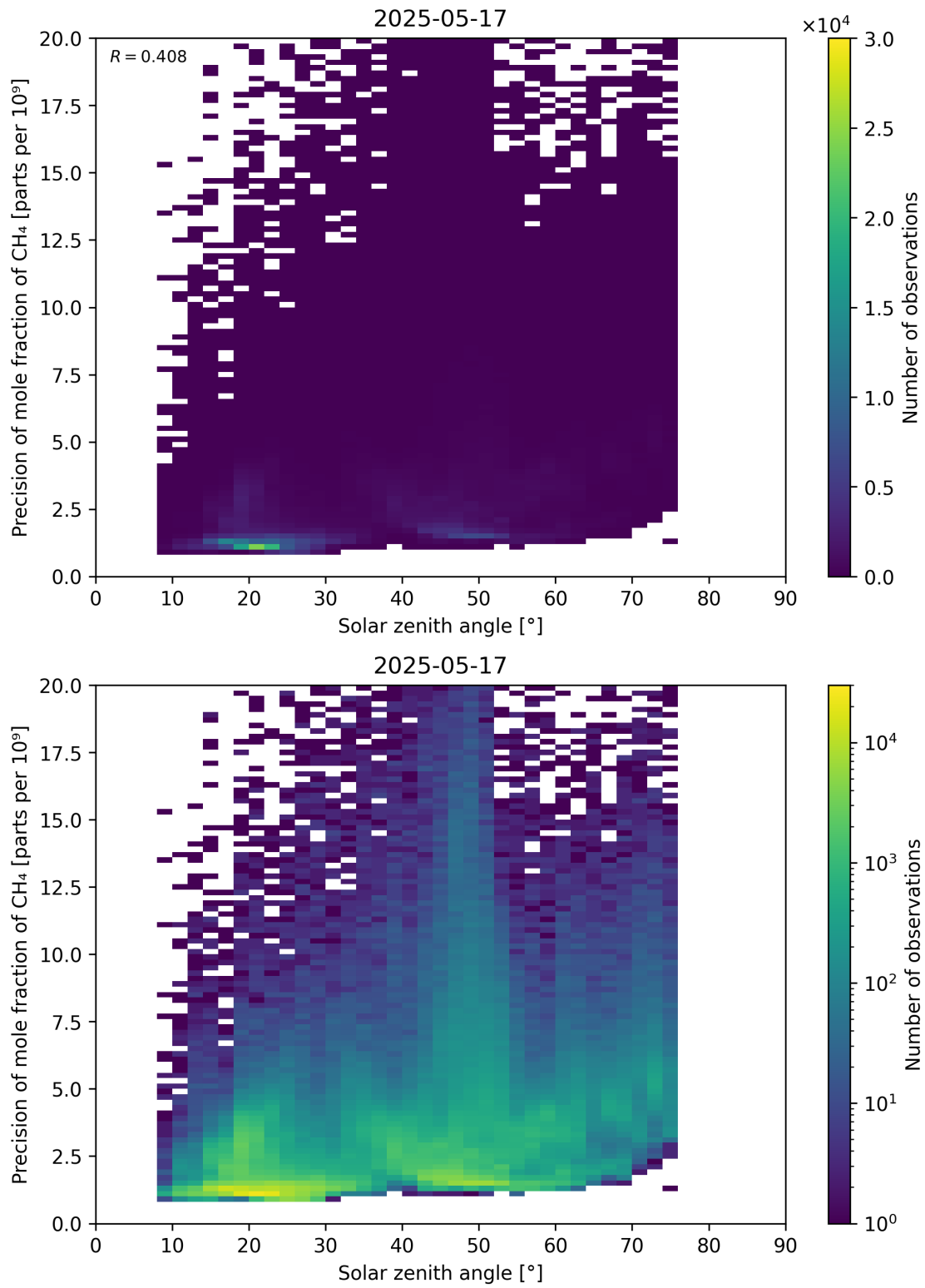
Figure 101: Scatter density plot of “Solar zenith angle” against “Precision of mole fraction of \text{CH}_4 ” for 2025-05-16 to 2025-05-18.
