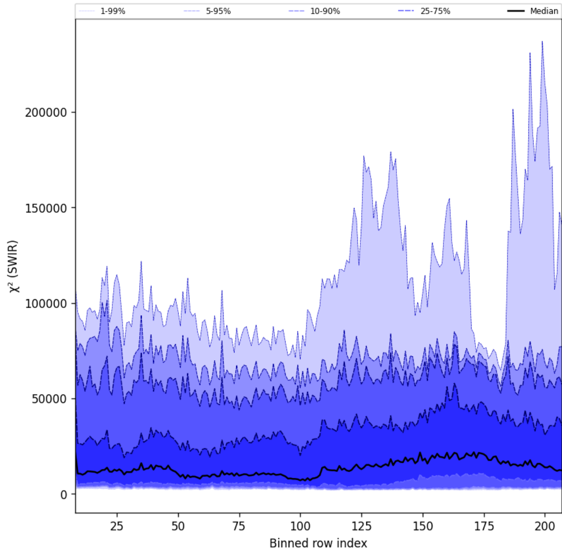
Figure 39: Along track statistics of “ \chi^2 (SWIR)” for 2025-05-16 to 2025-05-18
