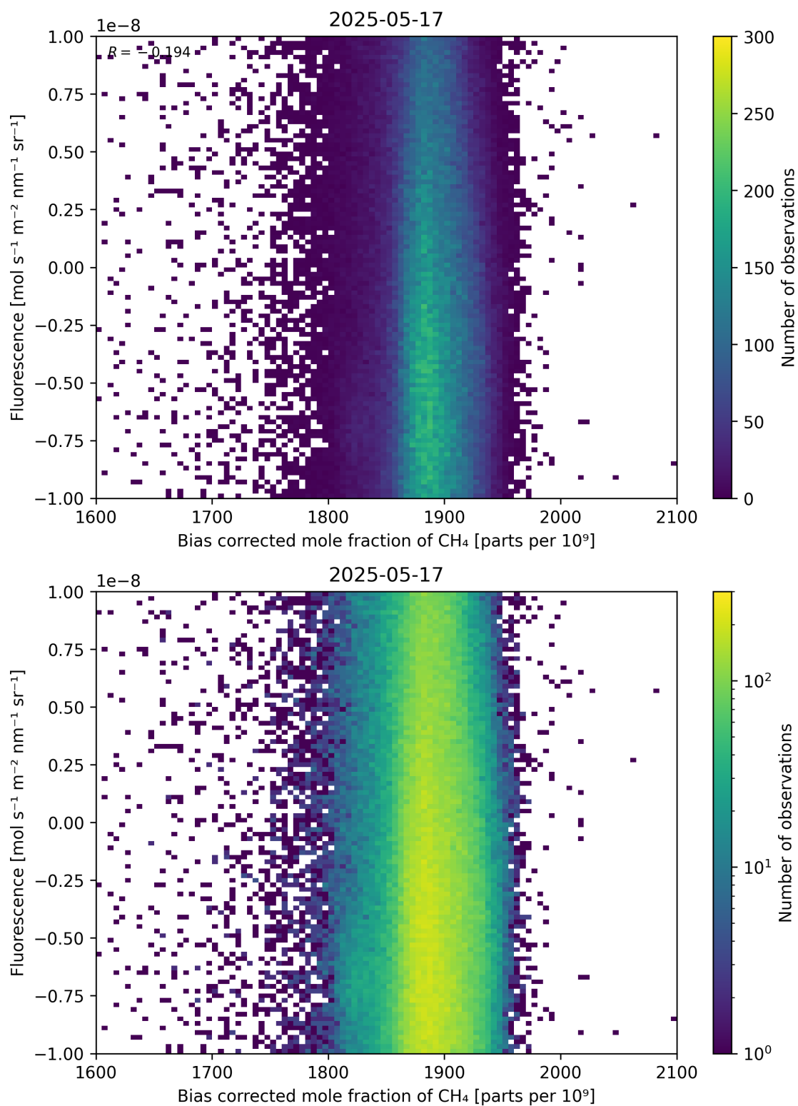
Figure 66: Scatter density plot of “Bias corrected mole fraction of \text{CH}_4 ” against “Fluorescence” for 2025-05-16 to 2025-05-18.
