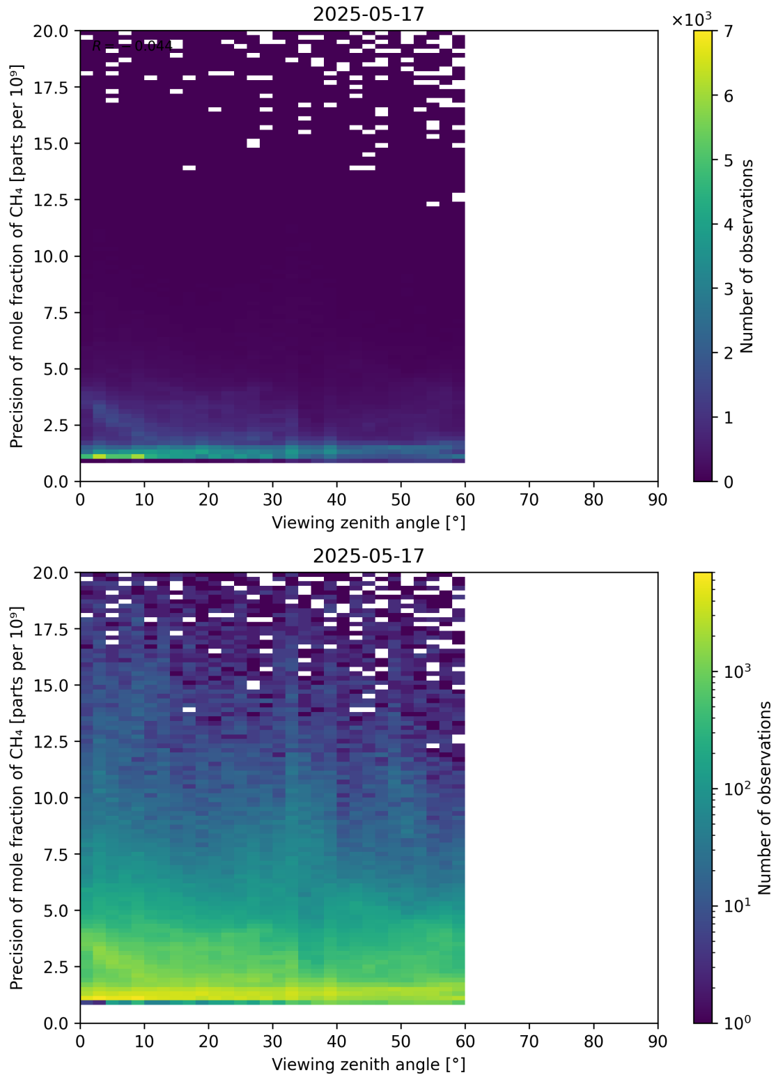
Figure 112: Scatter density plot of “Viewing zenith angle” against “Precision of mole fraction of CH 4 ” for 2025-05-16 to 2025-05-18.
