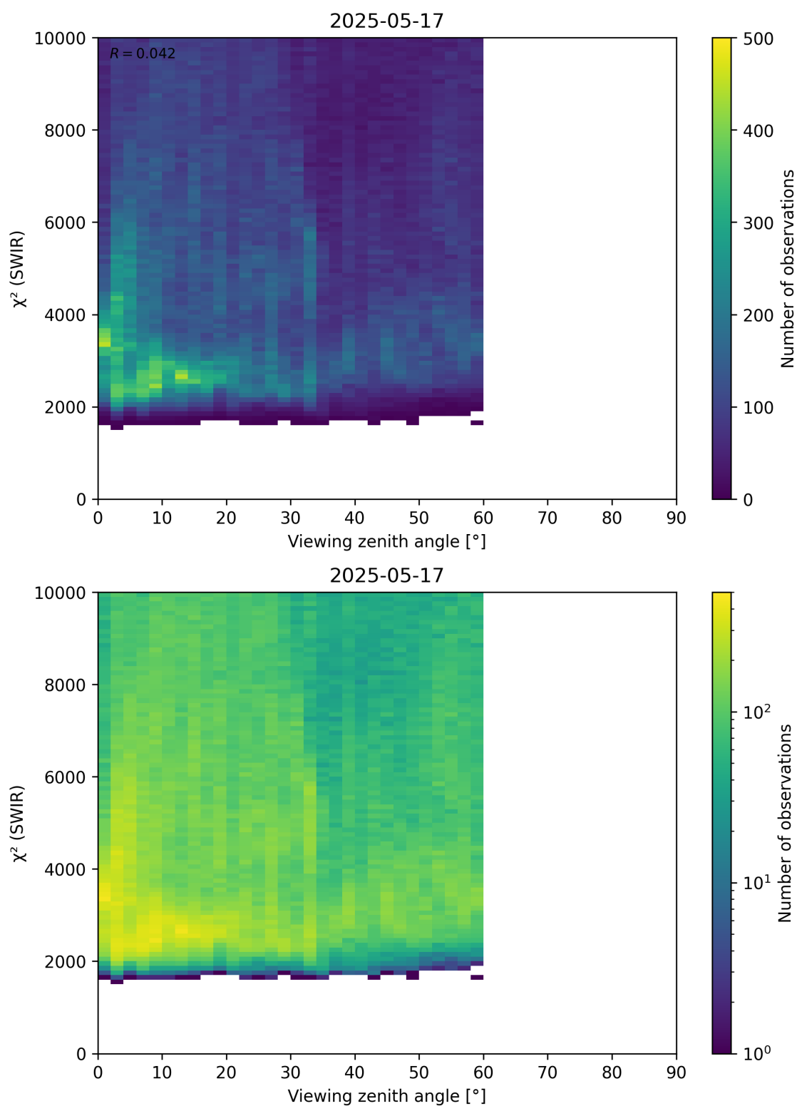
Figure 106: Scatter density plot of “Viewing zenith angle” against “ \chi^2 (SWIR)” for 2025-05-16 to 2025-05-18.
