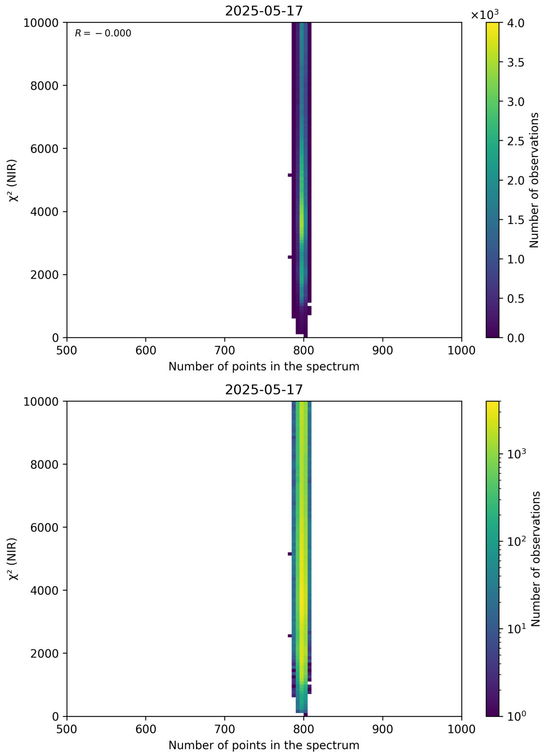
Figure 88: Scatter density plot of “Number of points in the spectrum” against “ \chi^2 (NIR)” for 2025-05-16 to 2025-05-18.
