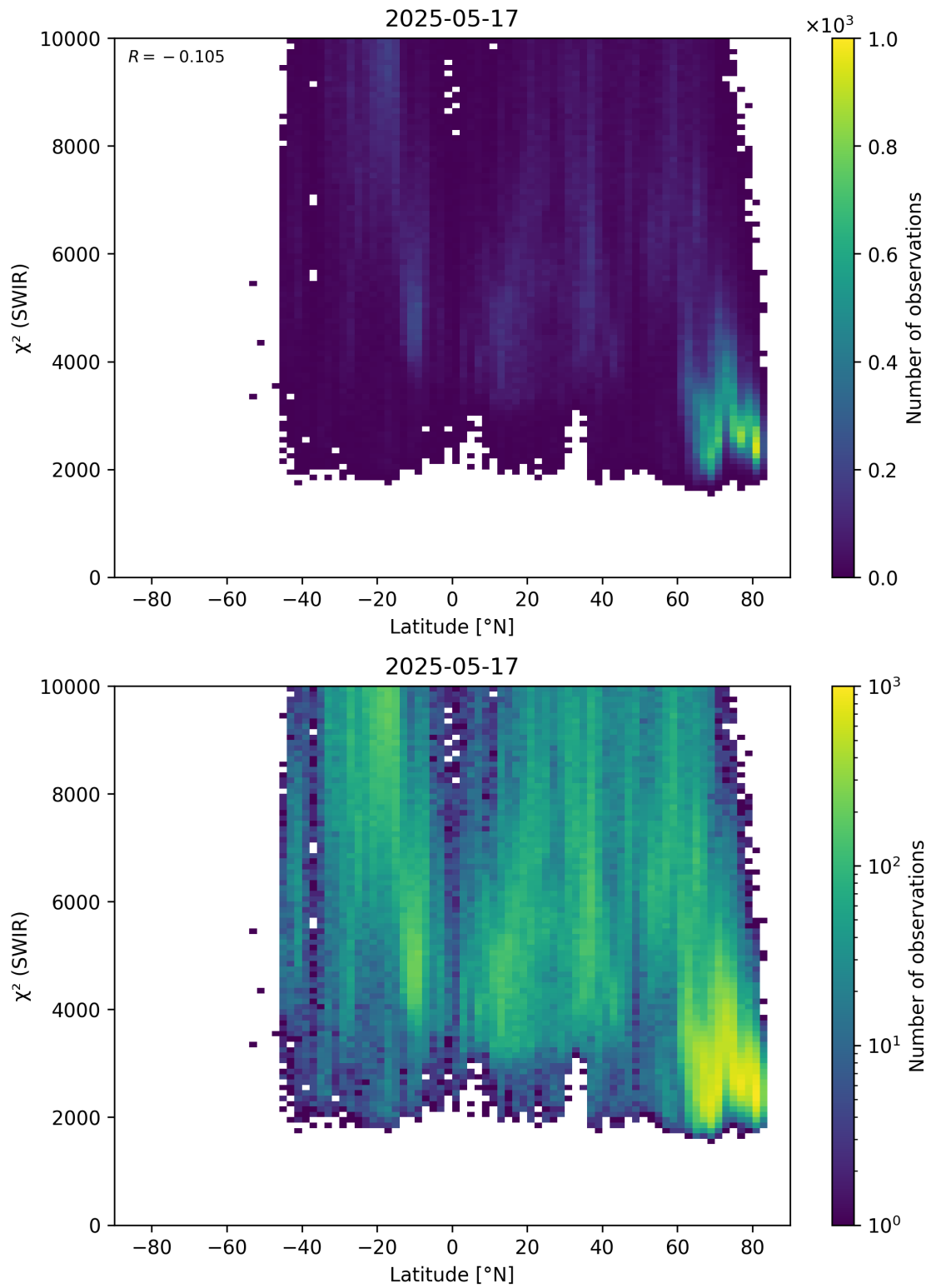
Figure 54: Scatter density plot of “Latitude” against “ \chi^2 (SWIR)” for 2025-05-16 to 2025-05-18.
