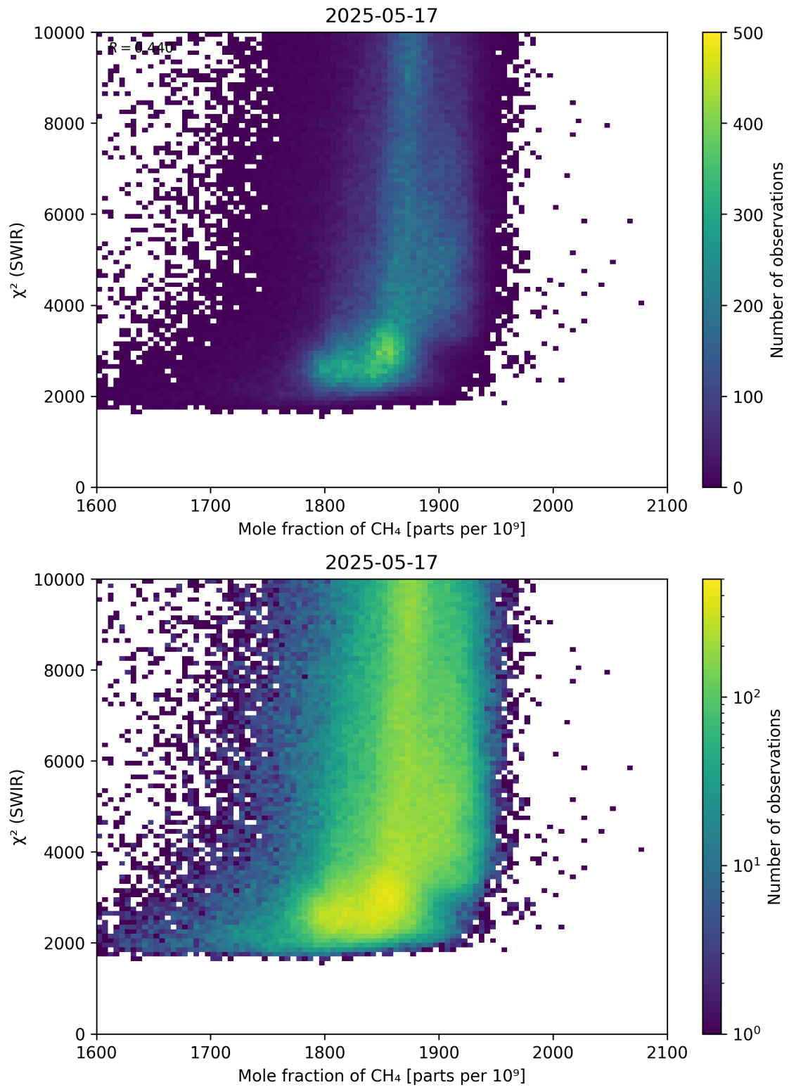
Figure 71: Scatter density plot of “Mole fraction of \text{CH}_4 ” against “ \chi^2 (SWIR)” for 2025-05-16 to 2025-05-18.
