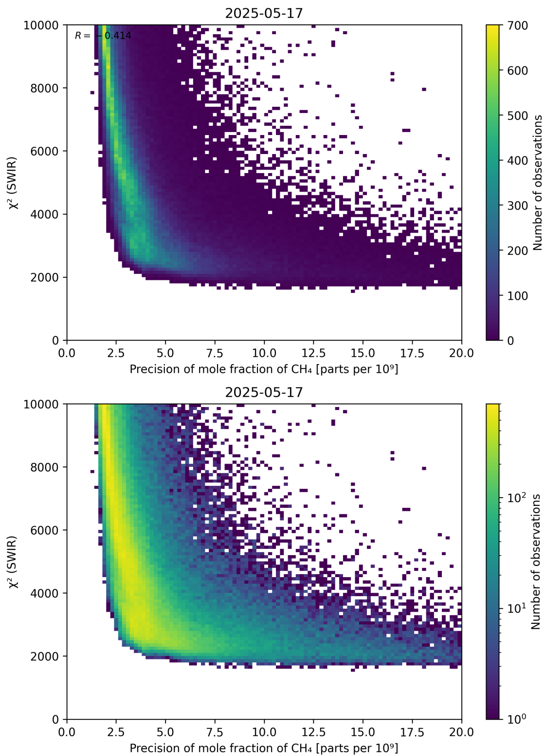
Figure 79: Scatter density plot of “Precision of mole fraction of \text{CH}_4 ” against “ \chi^2 (SWIR)” for 2025-05-16 to 2025-05-18.
