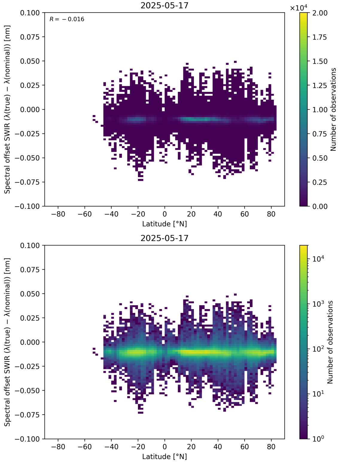
Figure 62: Scatter density plot of “Latitude” against “Spectral offset SWIR ( \lambda_{\text{true}} - \lambda_{\text{nominal}} )” for 2025-05-16 to 2025-05-18.
