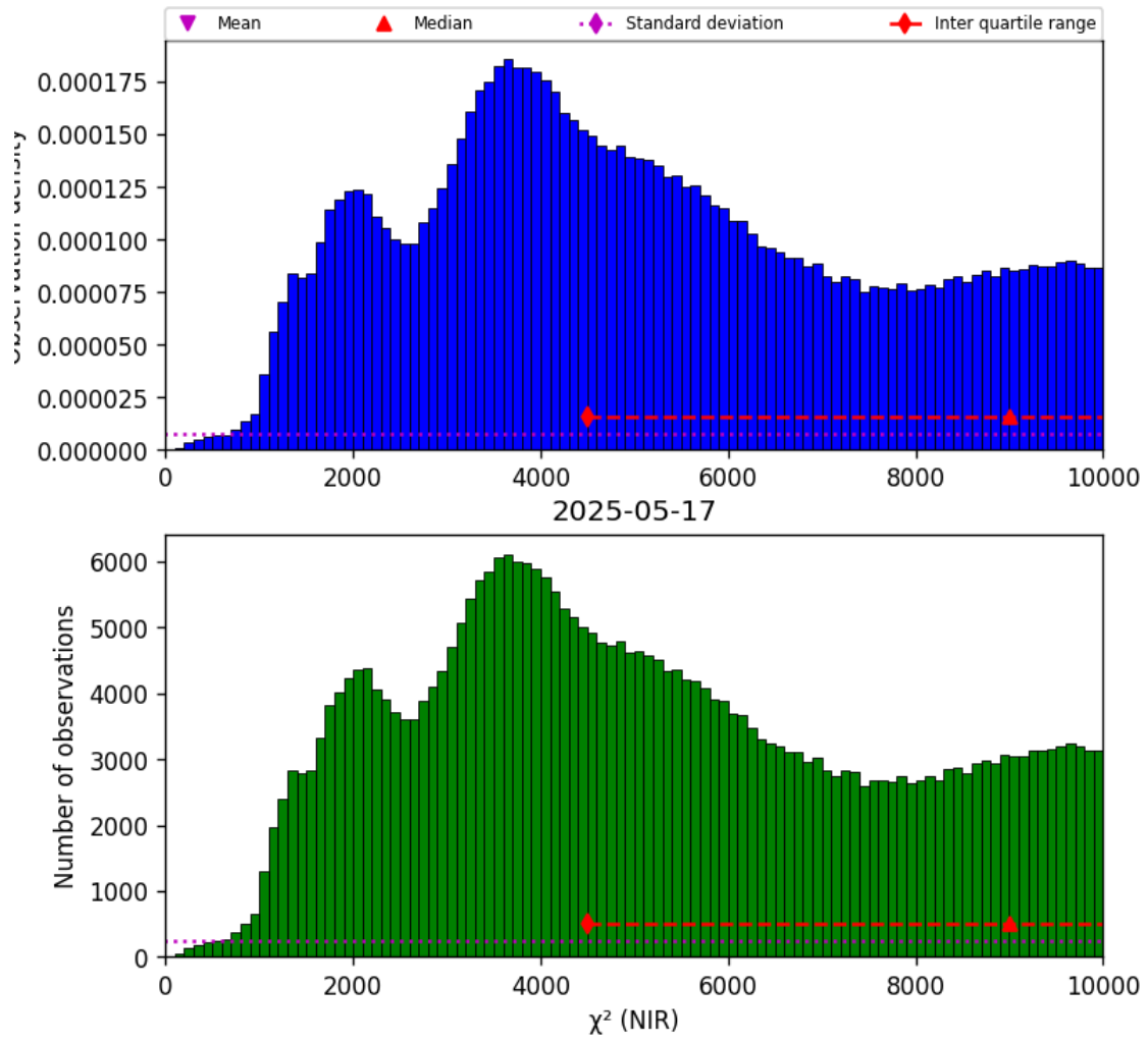
Figure 29: Histogram of “ \chi^2 (NIR)” for 2025-05-16 to 2025-05-18
