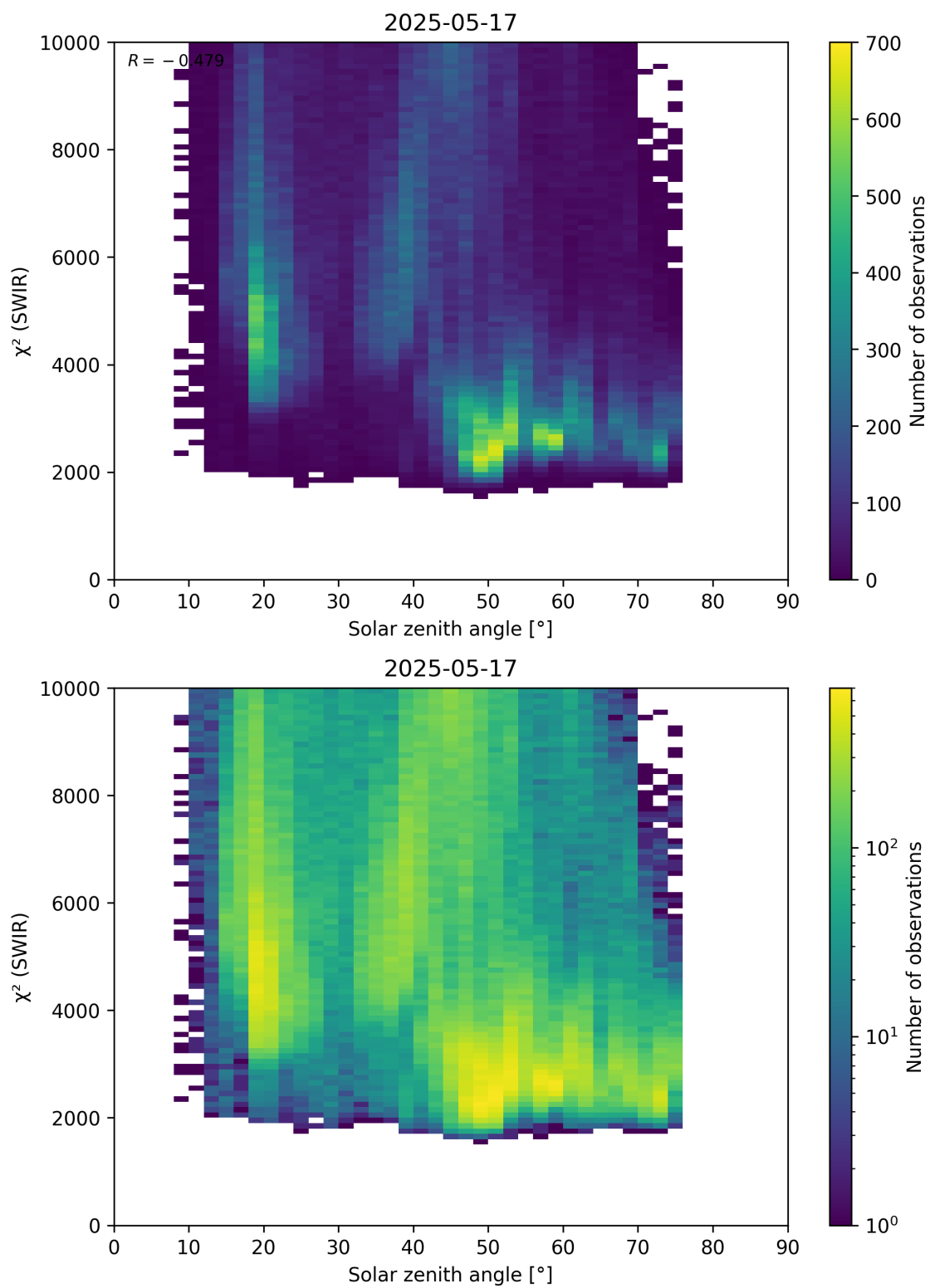
Figure 95: Scatter density plot of “Solar zenith angle” against “ \chi^2 (SWIR)” for 2025-05-16 to 2025-05-18.
