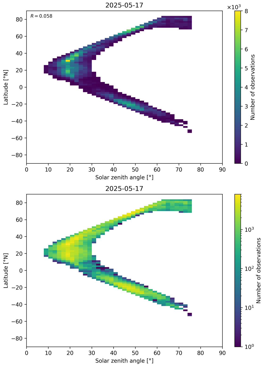
Figure 98: Scatter density plot of “Solar zenith angle” against “Latitude” for 2025-05-16 to 2025-05-18.
