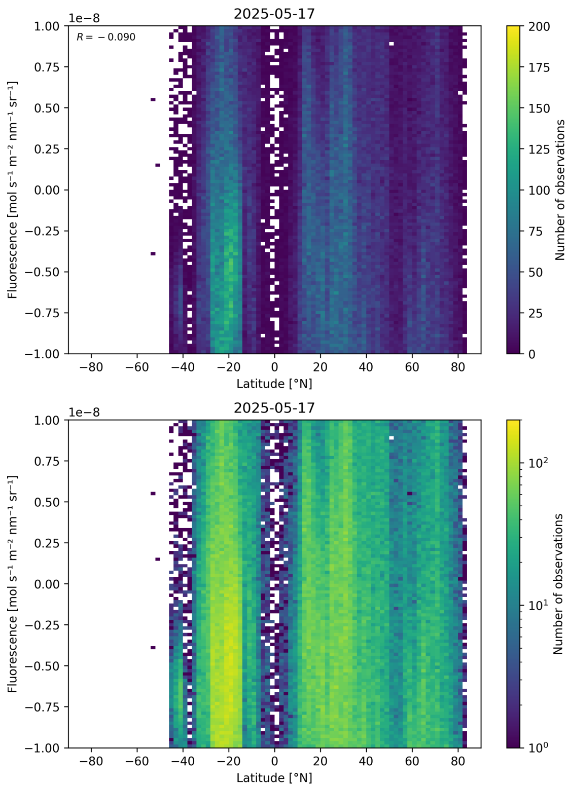
Figure 56: Scatter density plot of “Latitude” against “Fluorescence” for 2025-05-16 to 2025-05-18.
