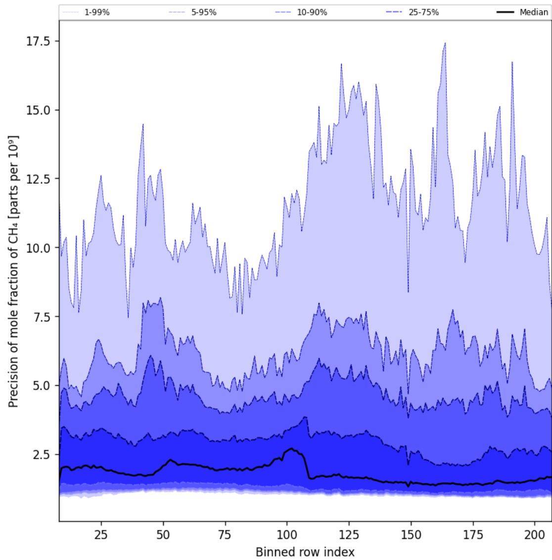
Figure 35: Along track statistics of “Precision of mole fraction of CH 4 ” for 2025-05-16 to 2025-05-18
