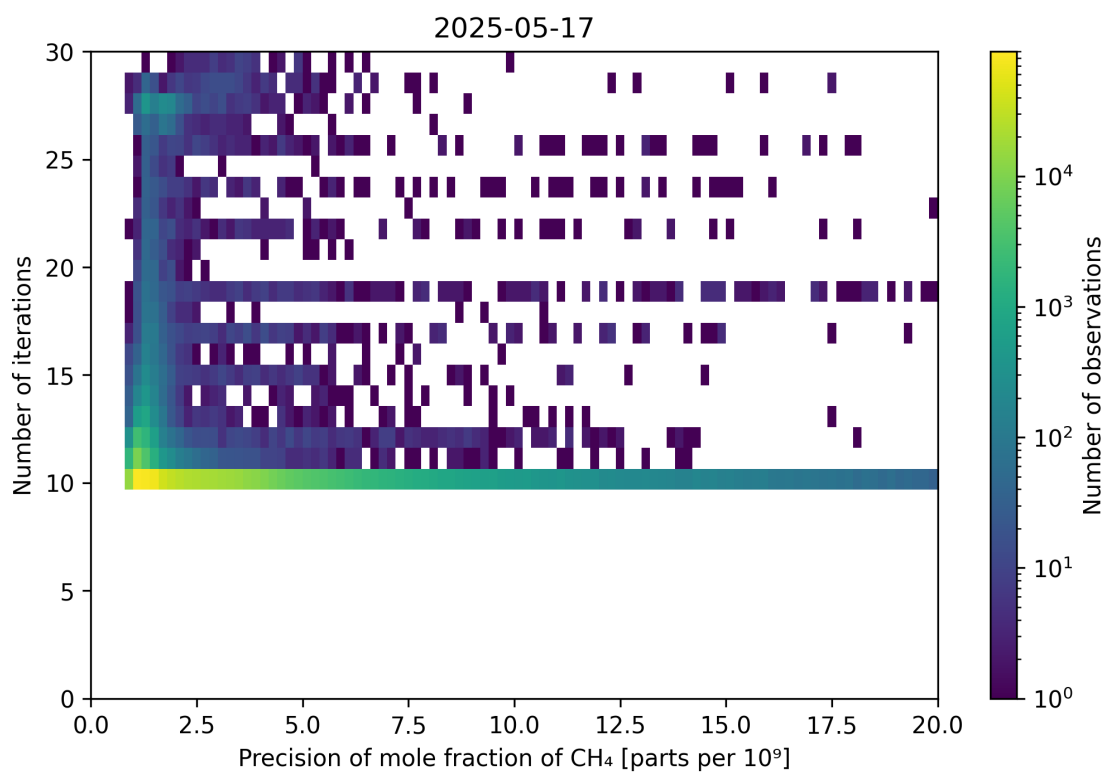
Figure 83: Scatter density plot of “Precision of mole fraction of CH 4 ” against “Number of iterations” for 2025-05-16 to 2025-05-18.
