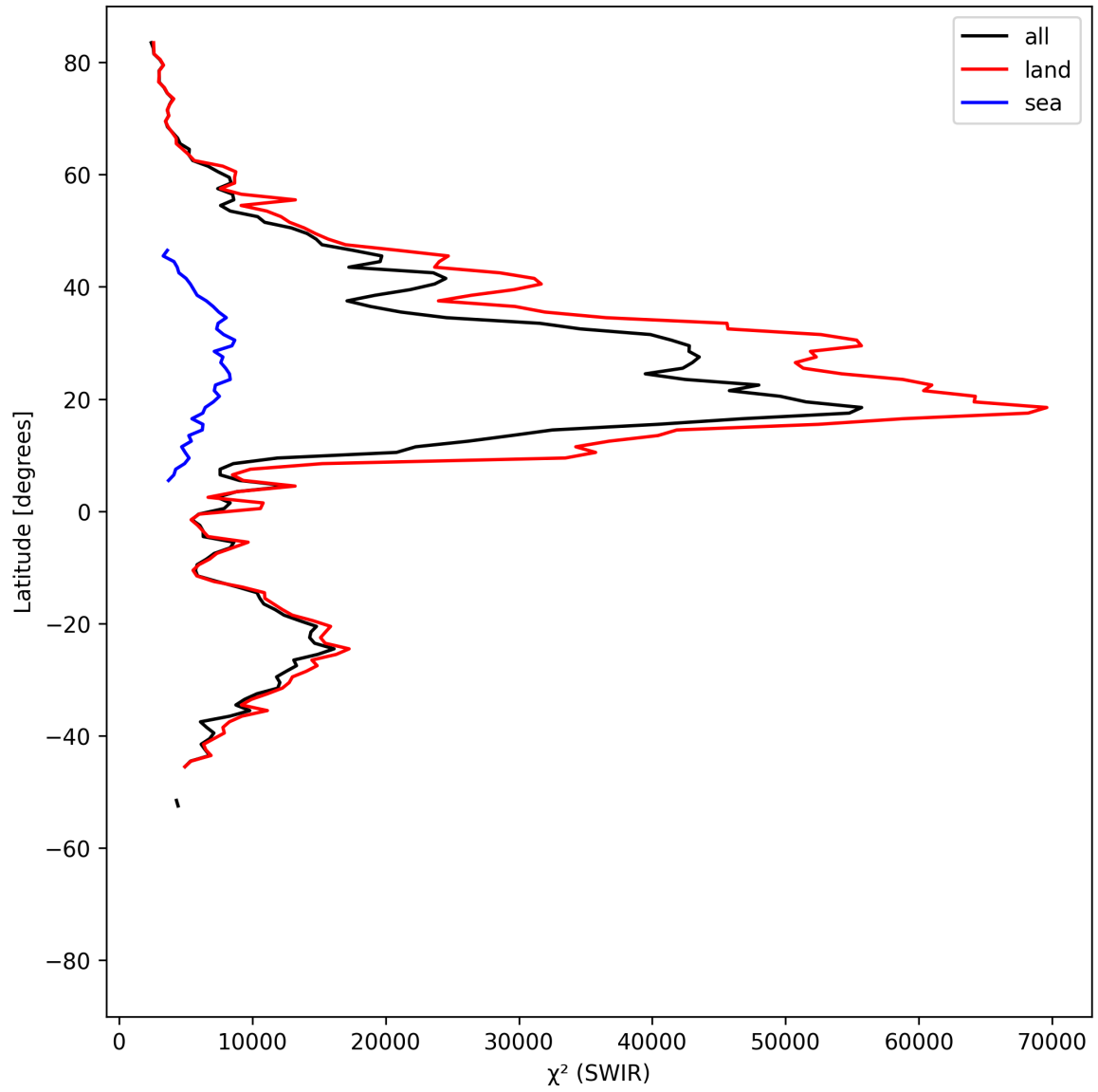
Figure 17: Zonal average of “ \chi^2 (SWIR)” for 2025-05-16 to 2025-05-18.
