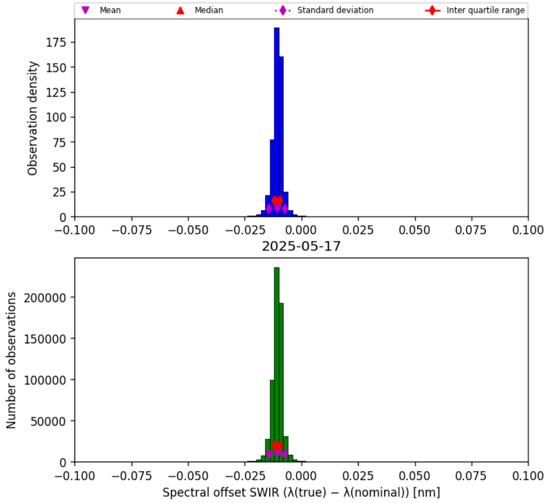
Figure 27: Histogram of “Spectral offset SWIR ( \lambda_{\text{true}} - \lambda_{\text{nominal}} )” for 2025-05-16 to 2025-05-18
