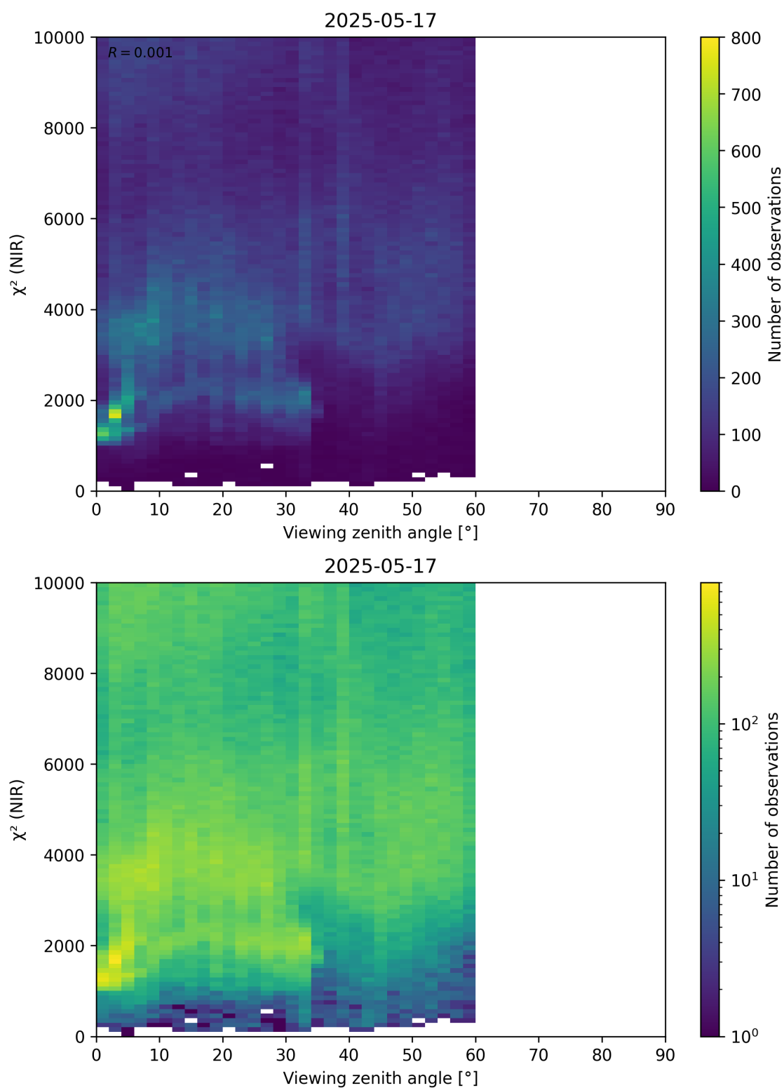
Figure 105: Scatter density plot of “Viewing zenith angle” against “ \chi^2 (NIR)” for 2025-05-16 to 2025-05-18.
