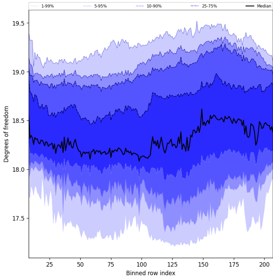
Figure 41: Along track statistics of “Degrees of freedom” for 2025-05-16 to 2025-05-18
