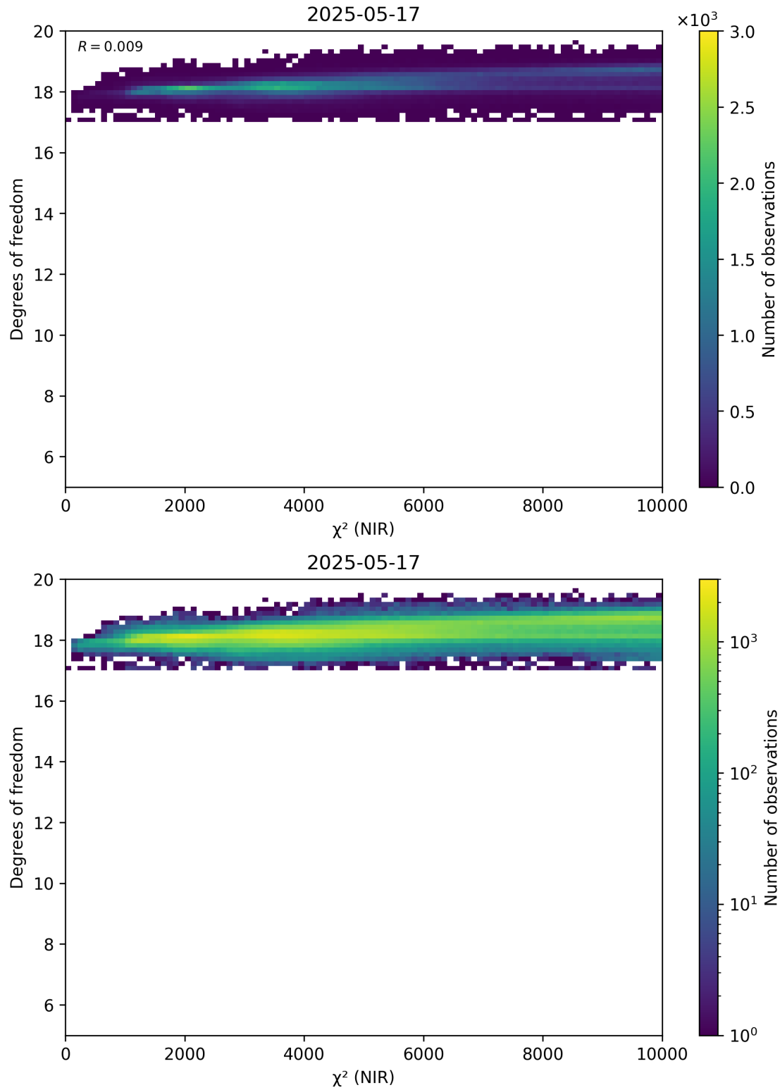
Figure 44: Scatter density plot of “ \chi^2 (NIR)” against “Degrees of freedom” for 2025-05-16 to 2025-05-18.
