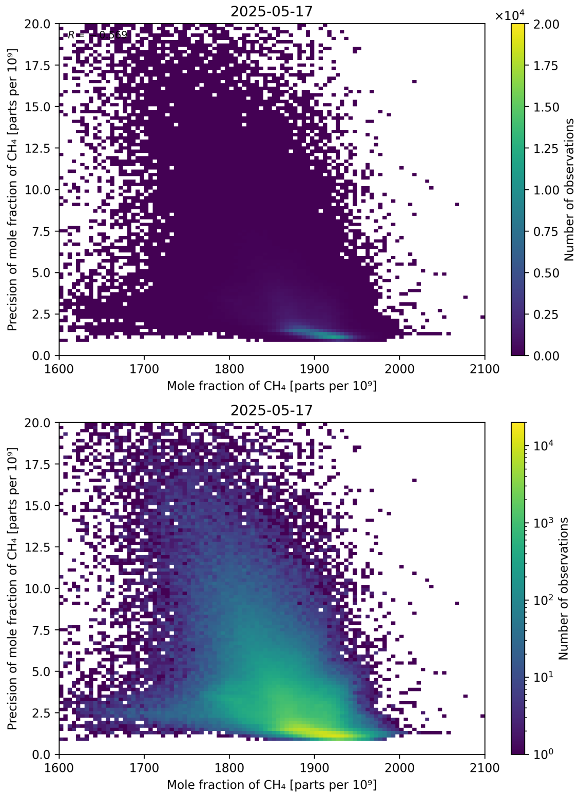
Figure 75: Scatter density plot of “Mole fraction of CH 4 ” against “Precision of mole fraction of CH 4 ” for 2025-05-16 to 2025-05-18.
