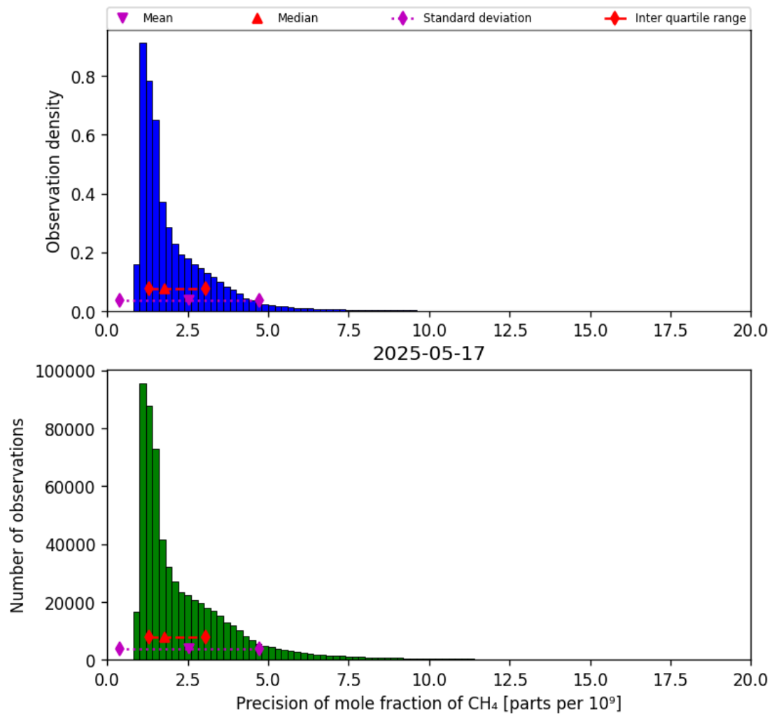
Figure 24: Histogram of “Precision of mole fraction of CH 4 ” for 2025-05-16 to 2025-05-18
