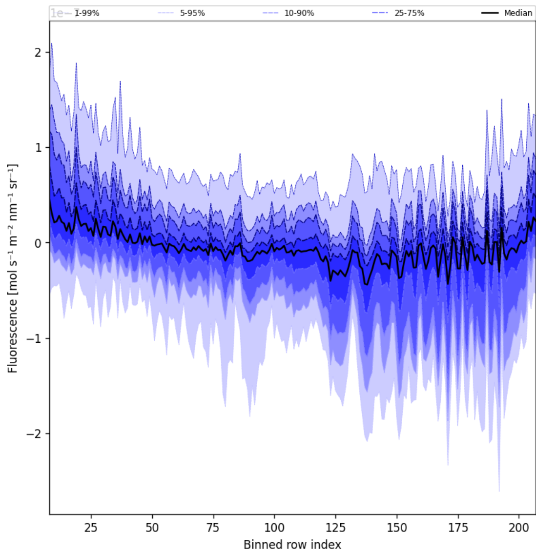
Figure 43: Along track statistics of “Fluorescence” for 2025-05-16 to 2025-05-18
