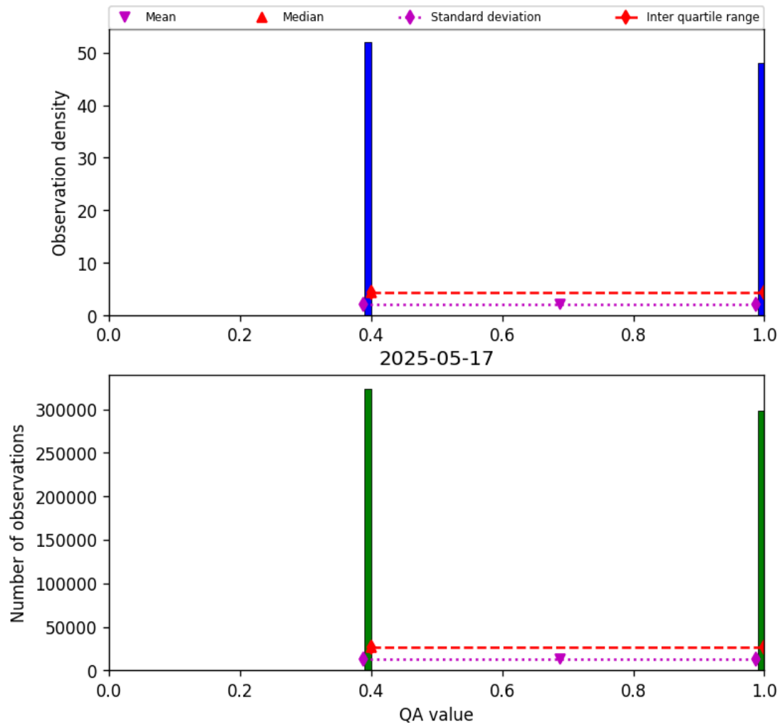
Figure 22: Histogram of “QA value” for 2025-05-16 to 2025-05-18
