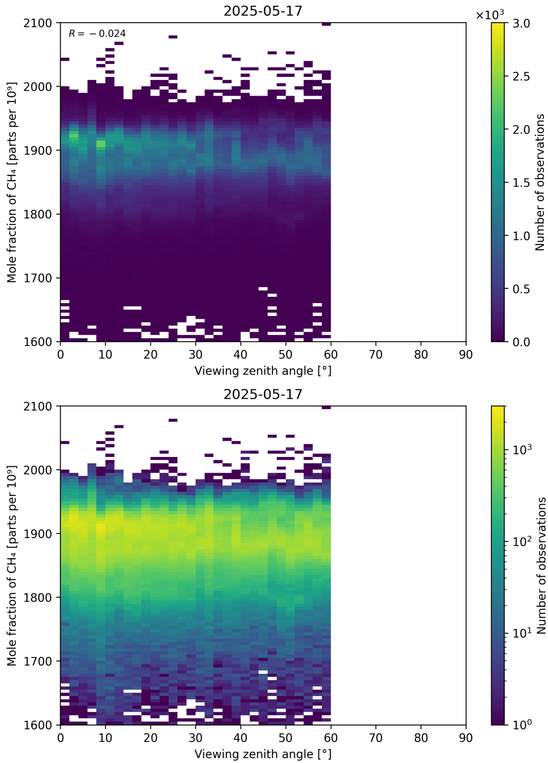
Figure 110: Scatter density plot of “Viewing zenith angle” against “Mole fraction of CH 4 ” for 2025-05-16 to 2025-05-18.
