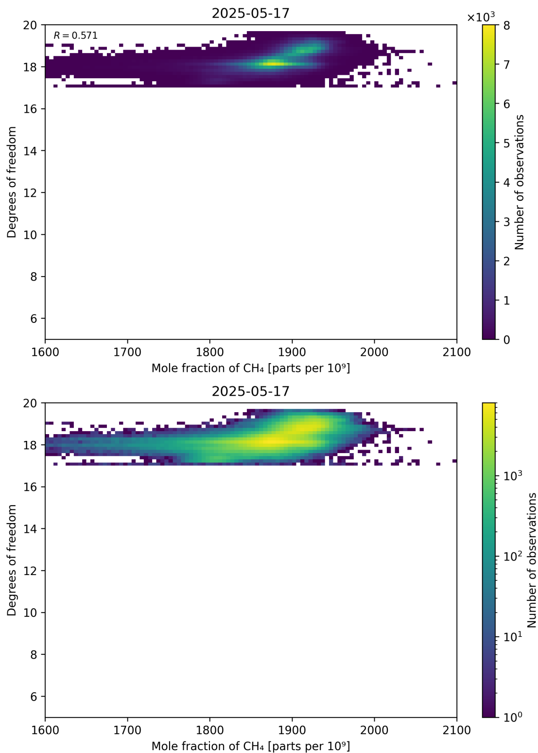
Figure 72: Scatter density plot of “Mole fraction of CH 4 ” against “Degrees of freedom” for 2025-05-16 to 2025-05-18.
