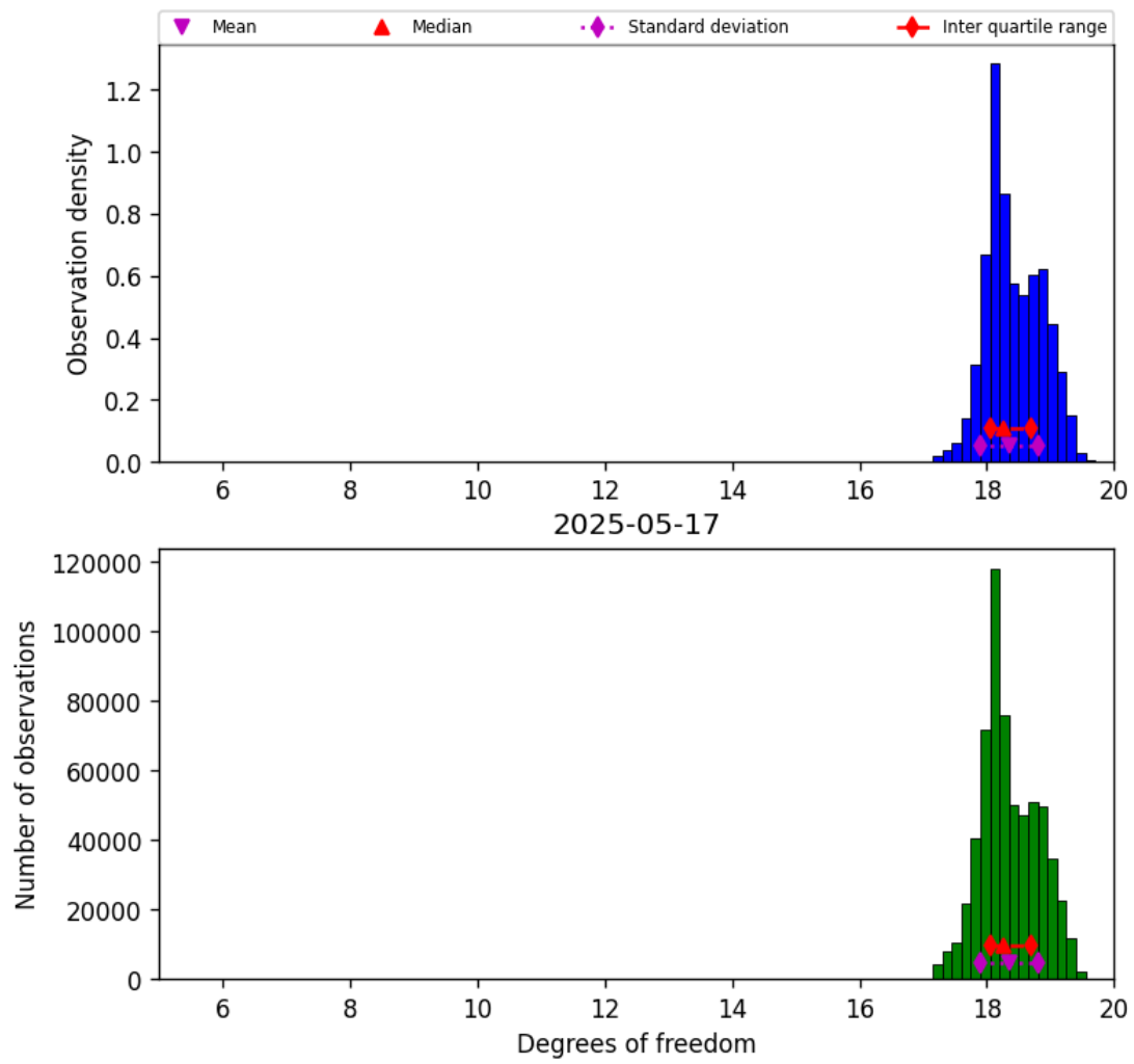
Figure 30: Histogram of “Degrees of freedom” for 2025-05-16 to 2025-05-18
