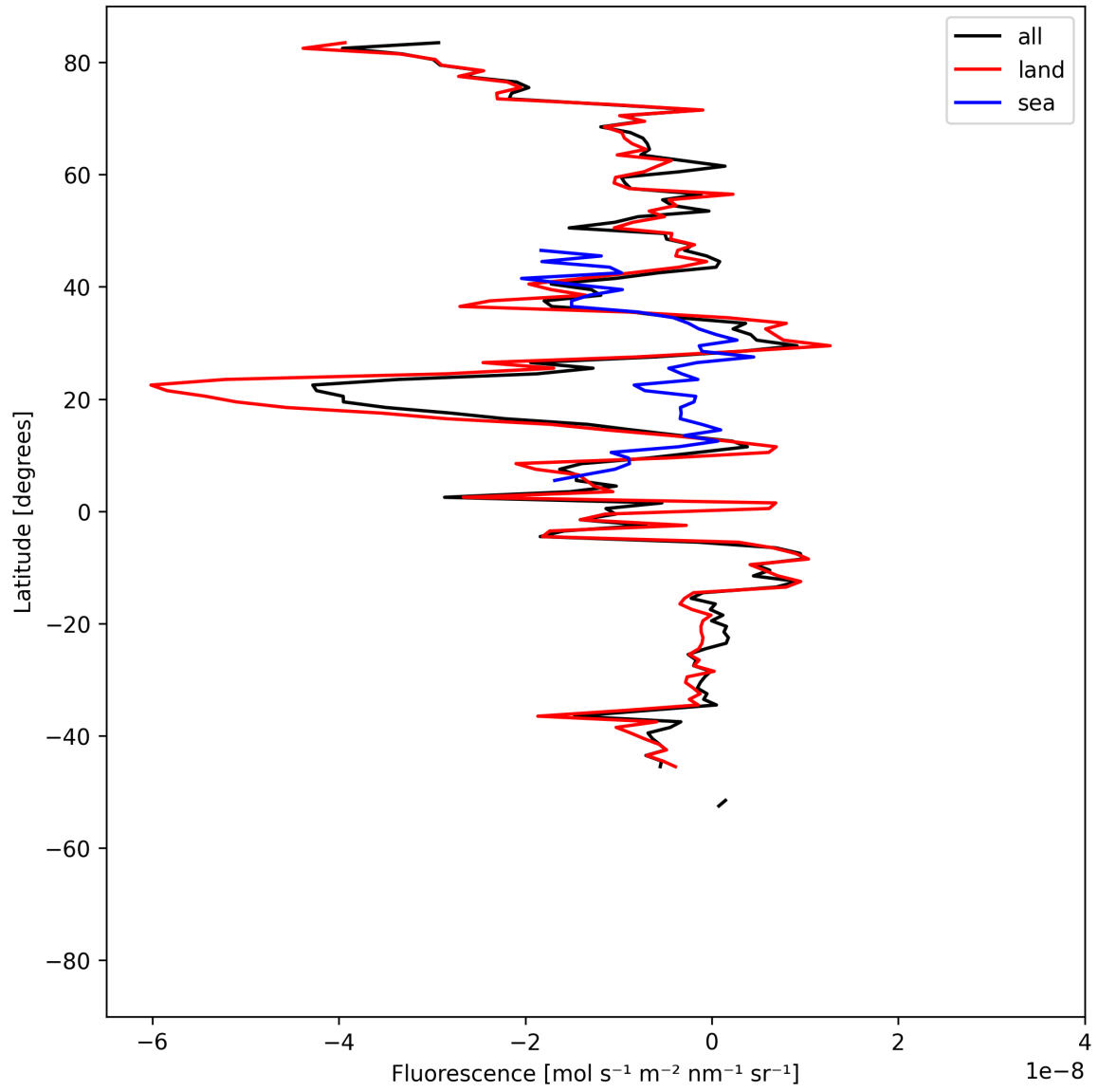
Figure 21: Zonal average of “Fluorescence” for 2025-05-16 to 2025-05-18.
