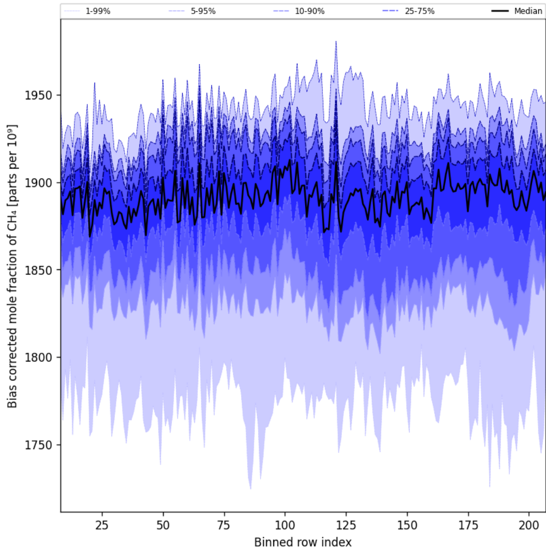
Figure 36: Along track statistics of “Bias corrected mole fraction of CH 4 ” for 2025-05-16 to 2025-05-18
