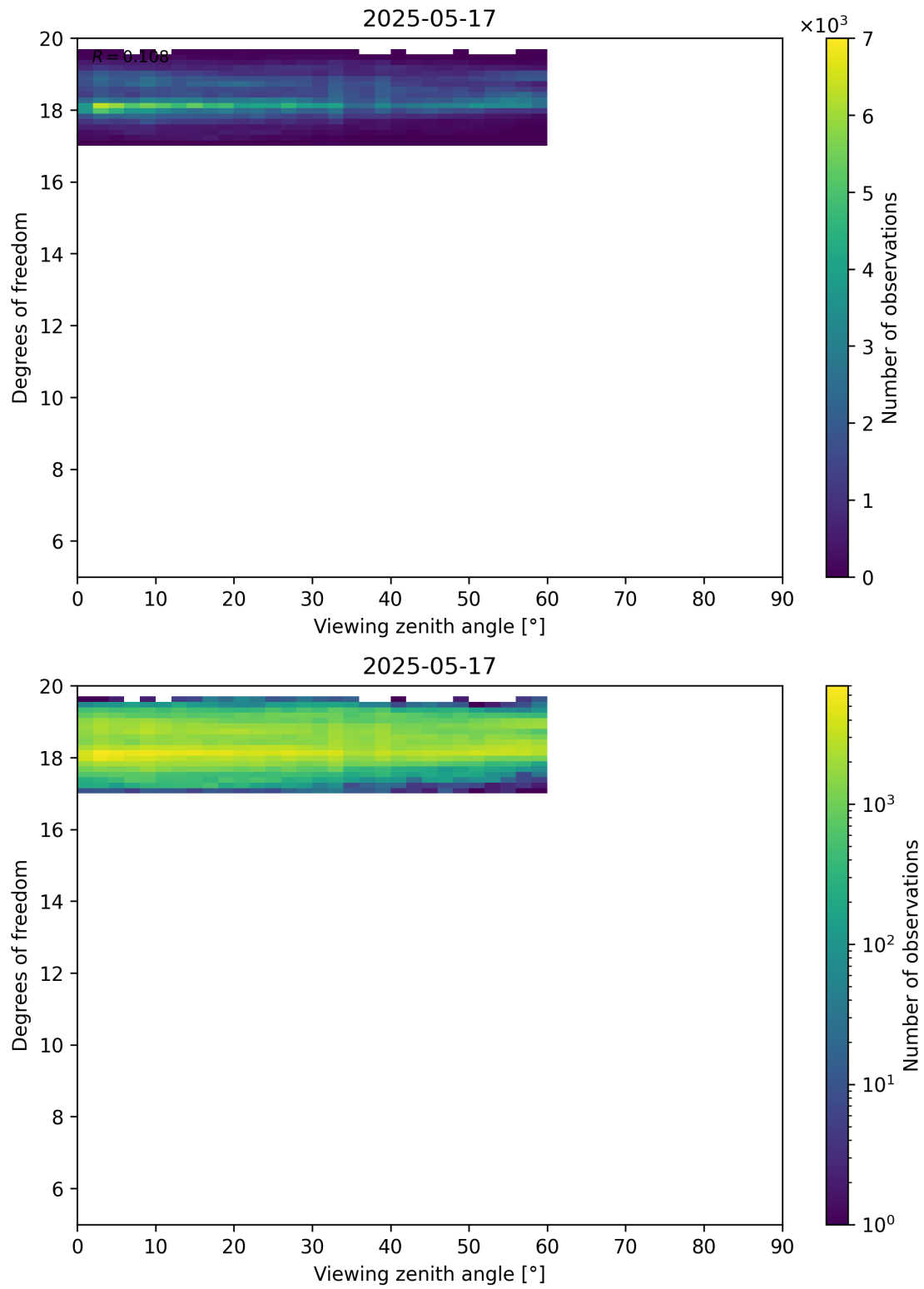
Figure 107: Scatter density plot of “Viewing zenith angle” against “Degrees of freedom” for 2025-05-16 to 2025-05-18.
