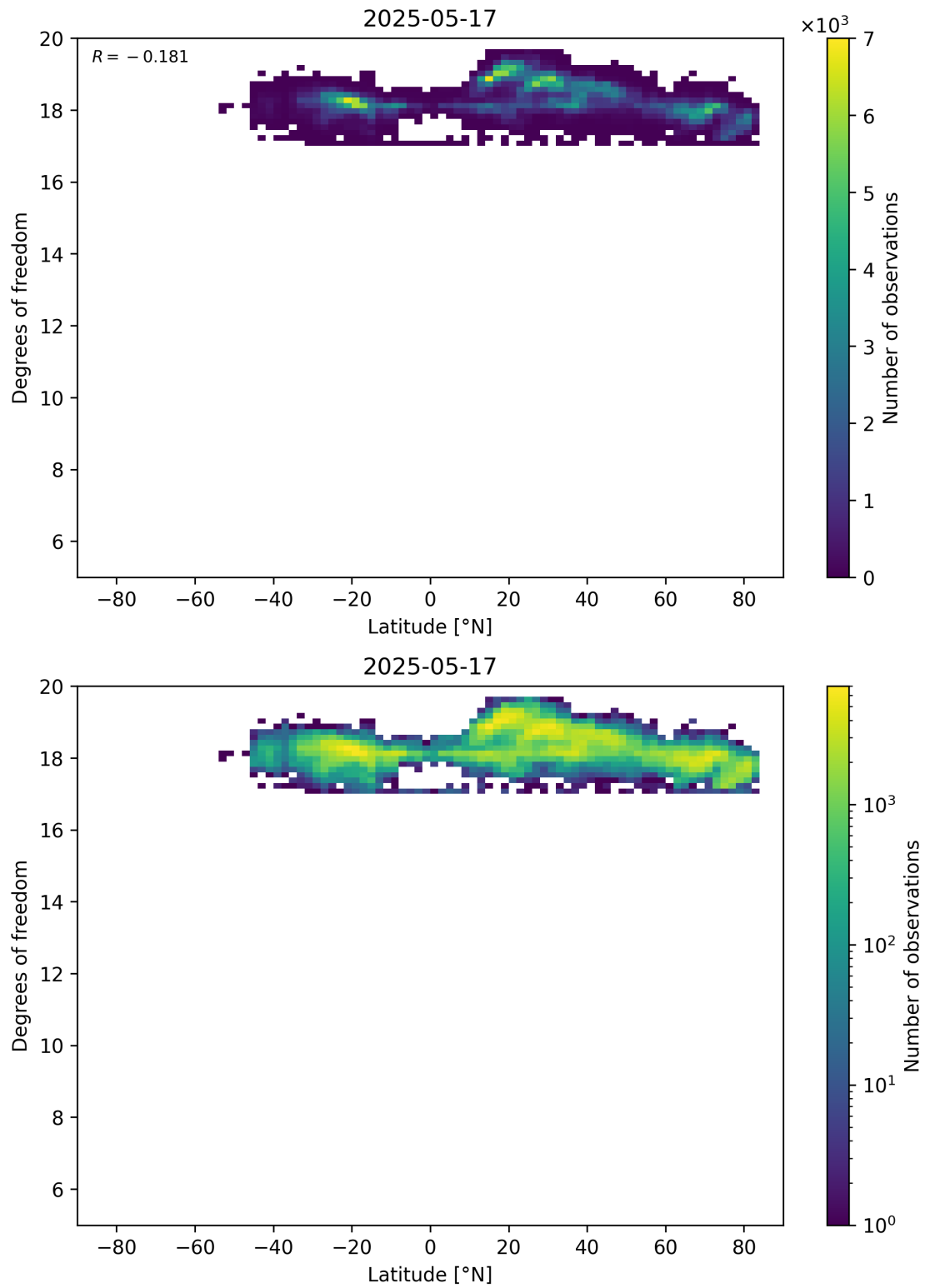
Figure 55: Scatter density plot of “Latitude” against “Degrees of freedom” for 2025-05-16 to 2025-05-18.
