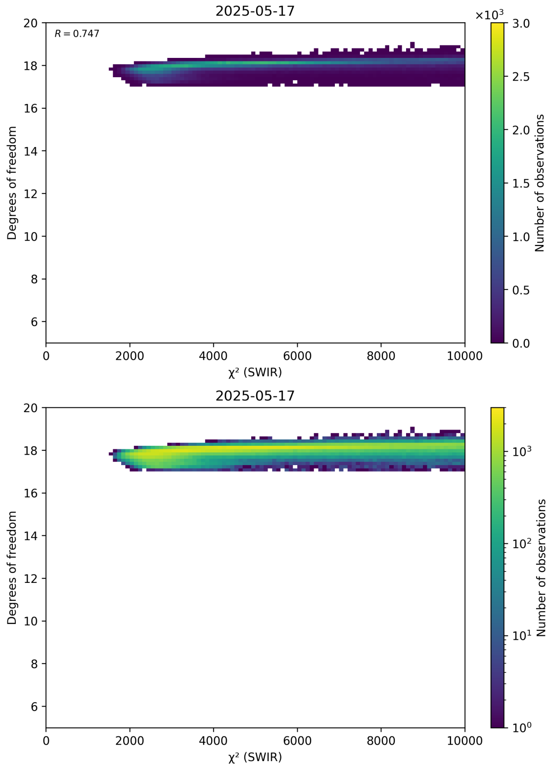
Figure 48: Scatter density plot of “ \chi^2 (SWIR)” against “Degrees of freedom” for 2025-05-16 to 2025-05-18.
