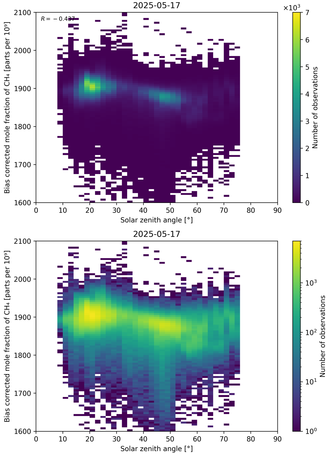
Figure 100: Scatter density plot of “Solar zenith angle” against “Bias corrected mole fraction of CH 4 ” for 2025-05-16 to 2025-05-18.
