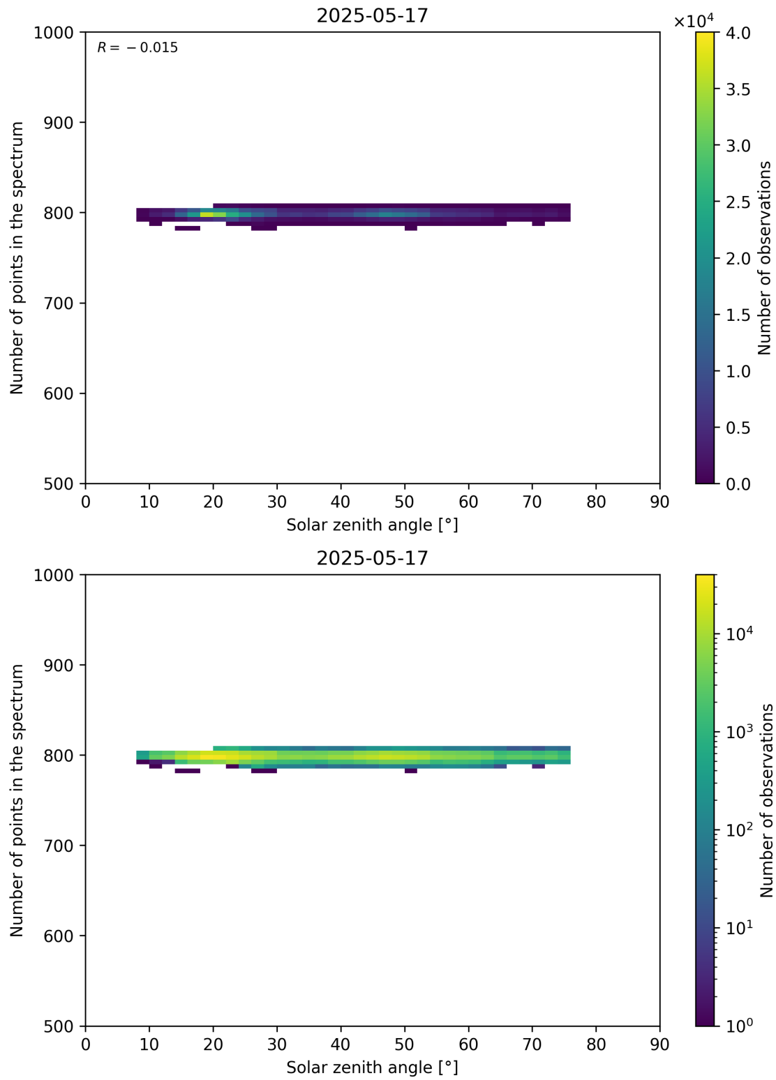
Figure 103: Scatter density plot of “Solar zenith angle” against “Number of points in the spectrum” for 2025-05-16 to 2025-05-18.
