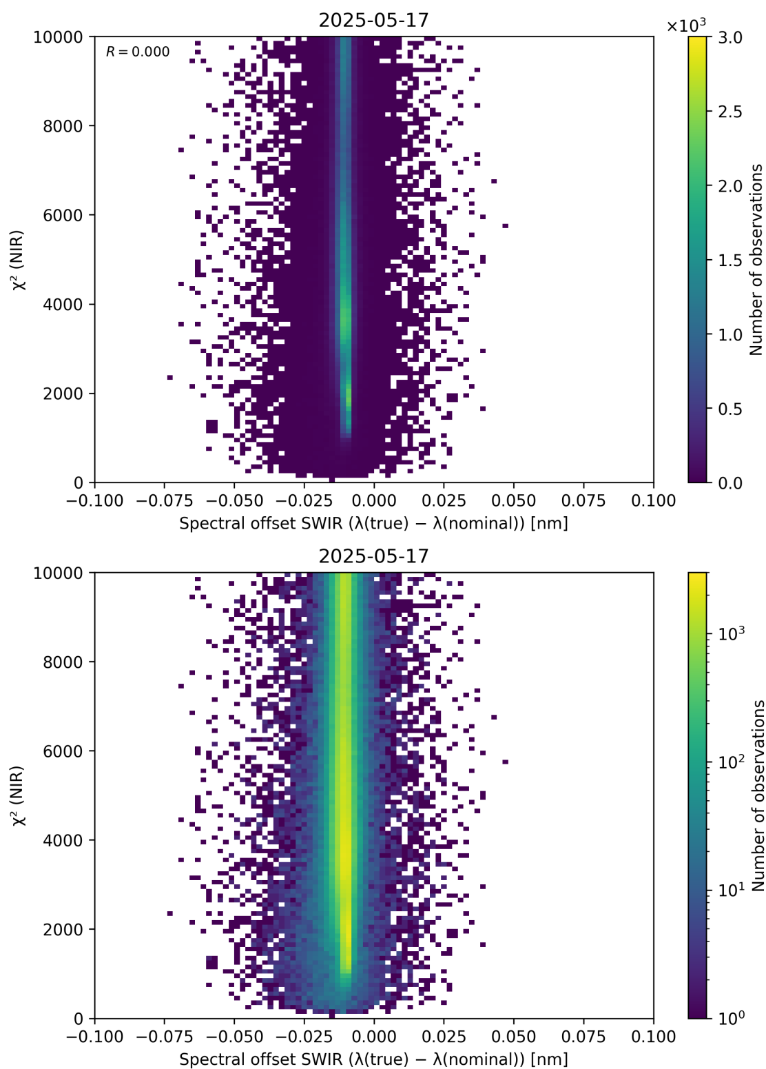
Figure 117: Scatter density plot of “Spectral offset SWIR ( \lambda_{\text{true}} - \lambda_{\text{nominal}} )” against “ \chi^2 (NIR)” for 2025-05-16 to 2025-05-18.
