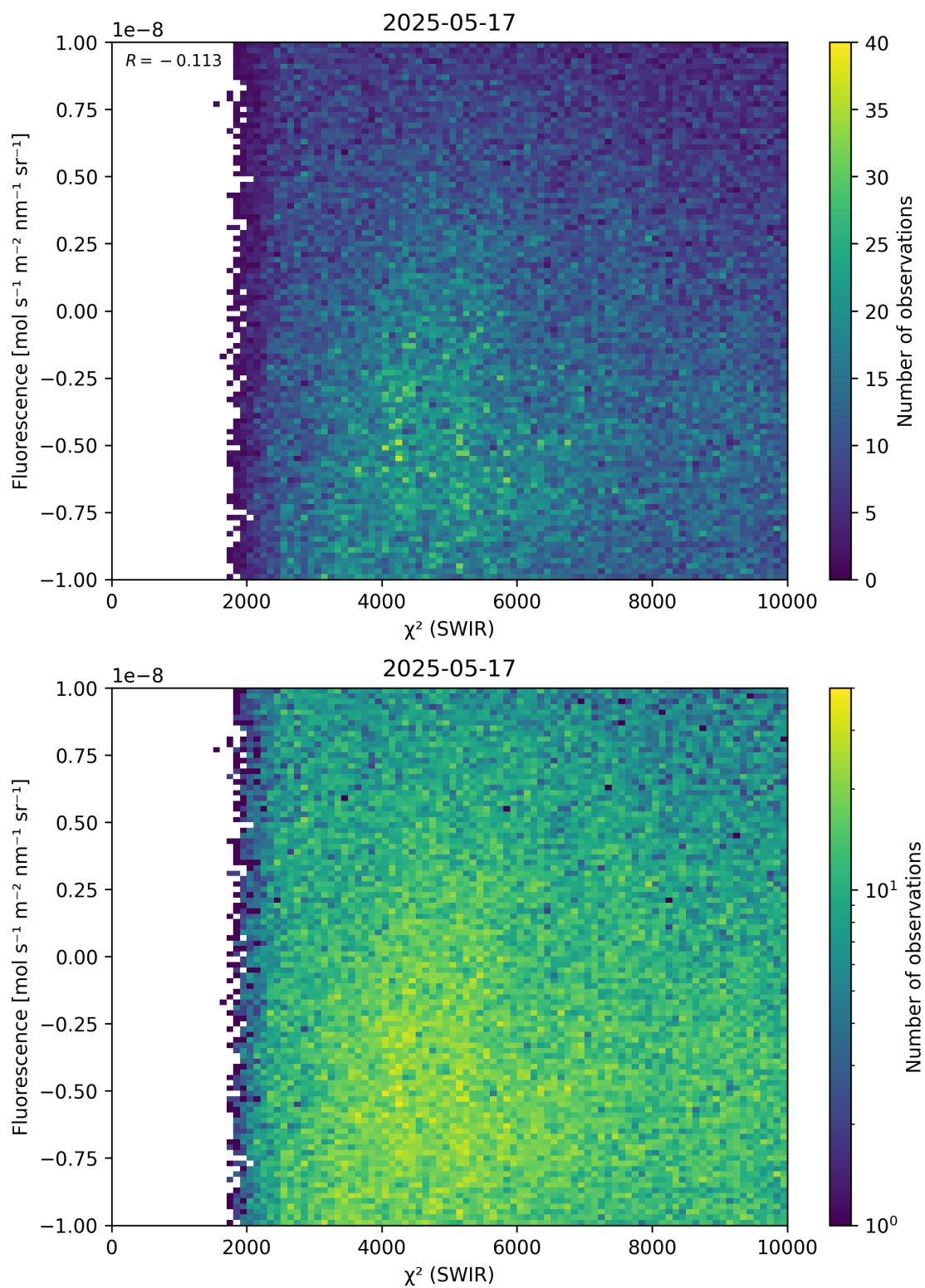
Figure 49: Scatter density plot of “ \chi^2 (SWIR)” against “Fluorescence” for 2025-05-16 to 2025-05-18.
