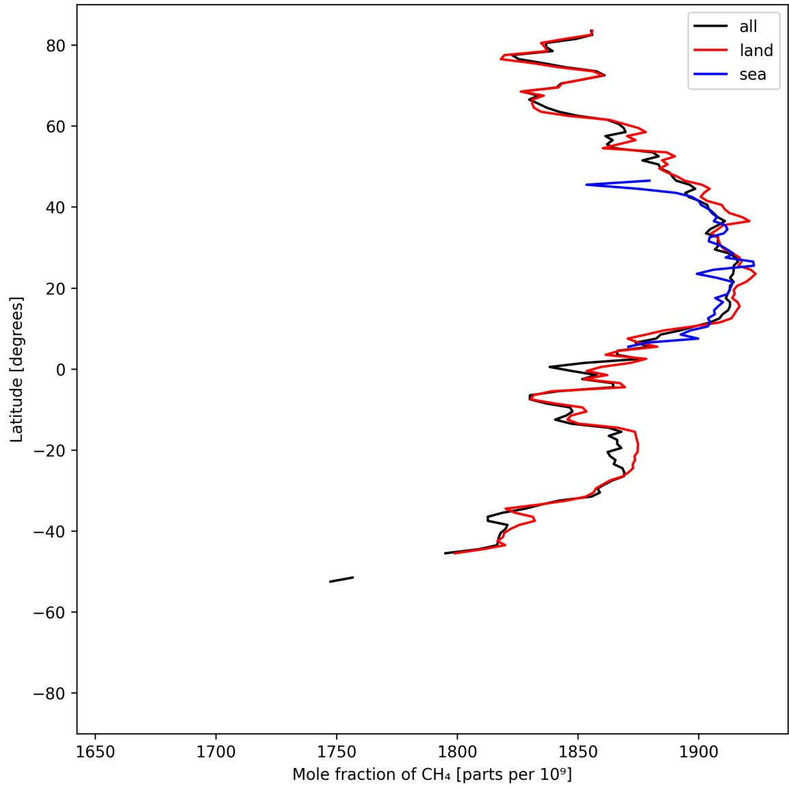
Figure 12: Zonal average of “Mole fraction of CH 4 ” for 2025-05-16 to 2025-05-18.
