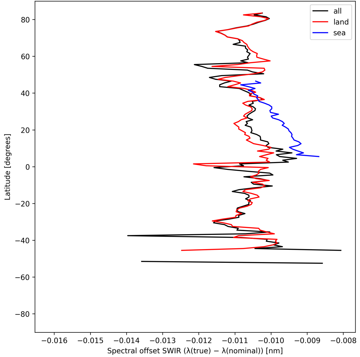
Figure 16: Zonal average of “Spectral offset SWIR ( \lambda_{\text{true}} - \lambda_{\text{nominal}} )” for 2025-05-16 to 2025-05-18.
