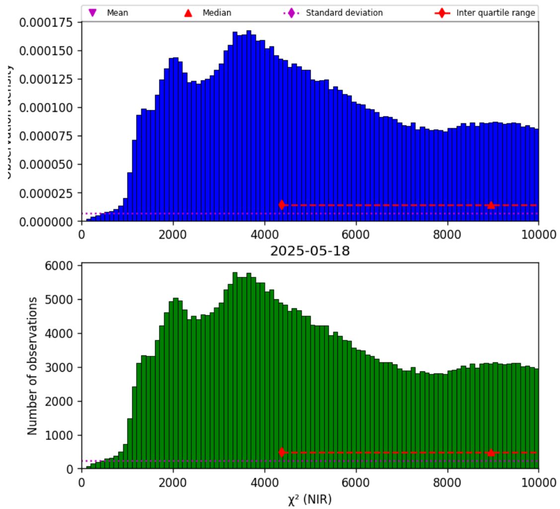
Figure 29: Histogram of “ \chi^2 (NIR)” for 2025-05-17 to 2025-05-19
