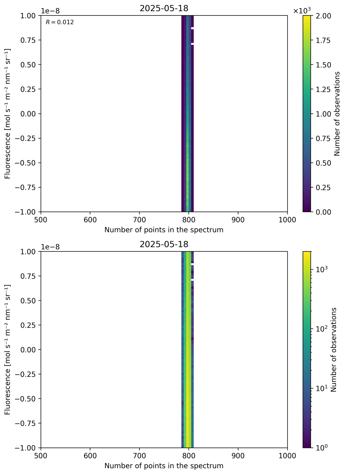
Figure 91: Scatter density plot of “Number of points in the spectrum” against “Fluorescence” for 2025-05-17 to 2025-05-19.
