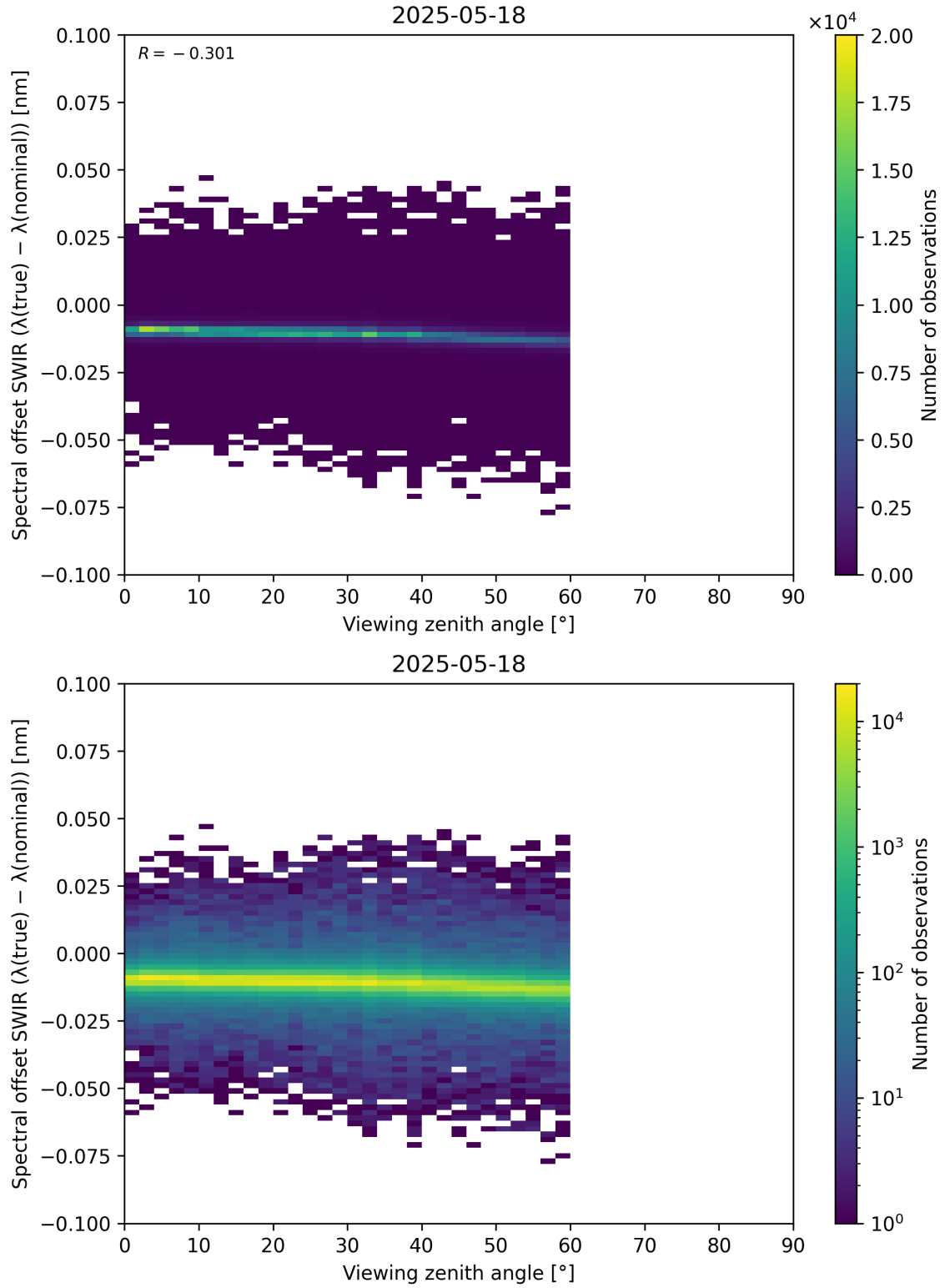
Figure 116: Scatter density plot of “Viewing zenith angle” against “Spectral offset SWIR ( \lambda_{\text{true}} - \lambda_{\text{nominal}} )” for 2025-05-17 to 2025-05-19.
