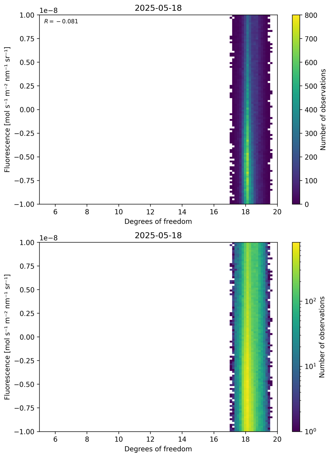
Figure 51: Scatter density plot of “Degrees of freedom” against “Fluorescence” for 2025-05-17 to 2025-05-19.
