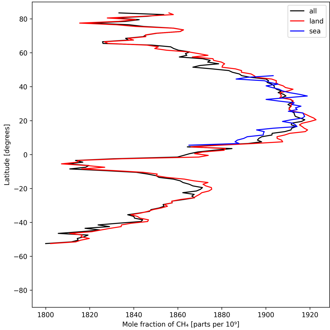
Figure 12: Zonal average of “Mole fraction of \text{CH}_4 ” for 2025-05-17 to 2025-05-19.
