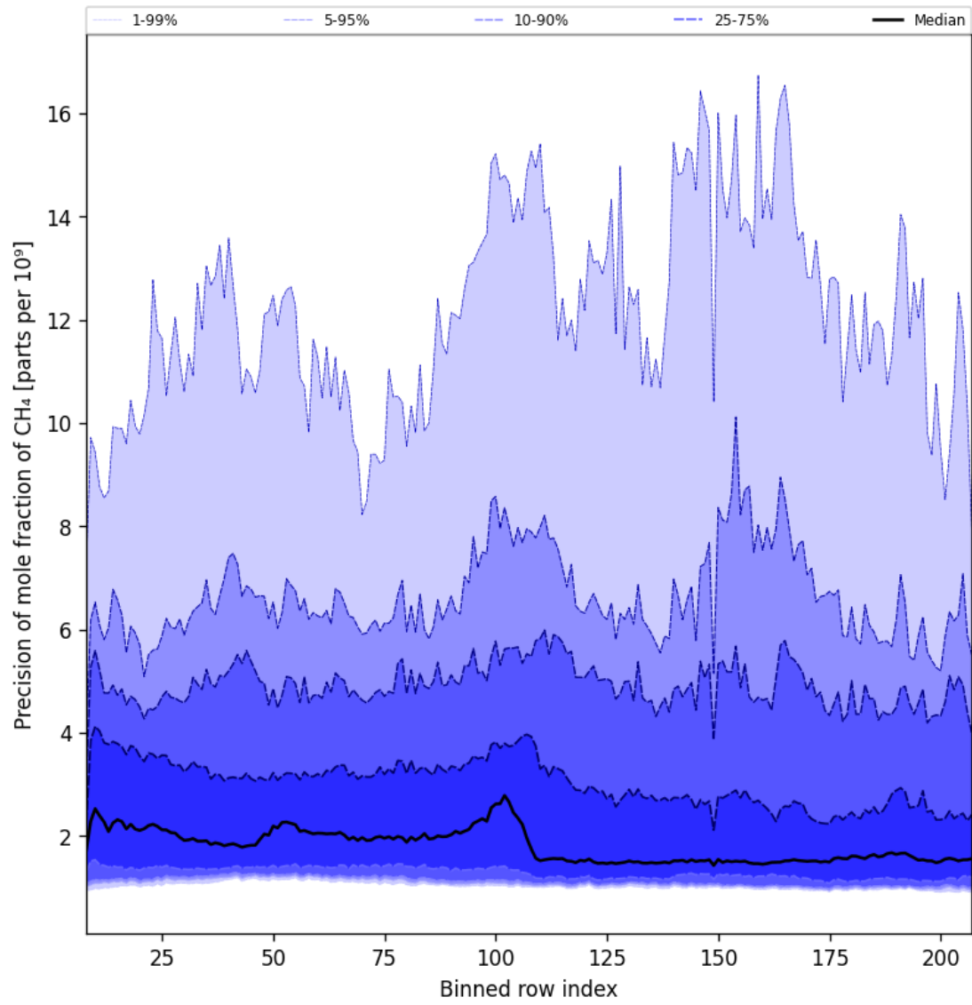
Figure 35: Along track statistics of “Precision of mole fraction of CH 4 ” for 2025-05-17 to 2025-05-19
