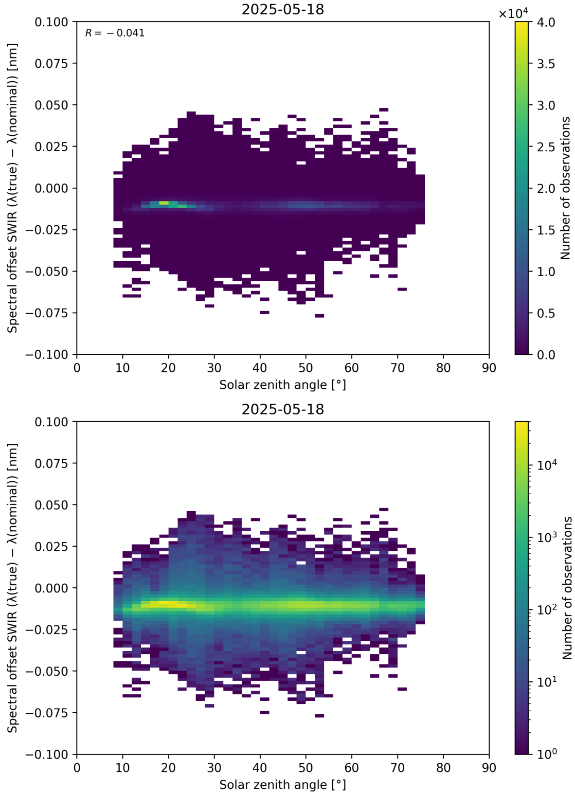
Figure 104: Scatter density plot of “Solar zenith angle” against “Spectral offset SWIR ( \lambda_{\text{true}} - \lambda_{\text{nominal}} )” for 2025-05-17 to 2025-05-19.
