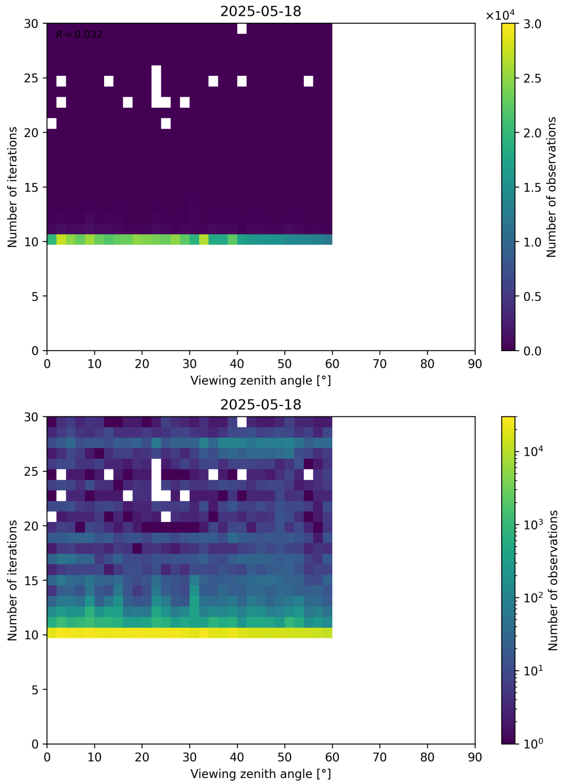
Figure 113: Scatter density plot of “Viewing zenith angle” against “Number of iterations” for 2025-05-17 to 2025-05-19.
