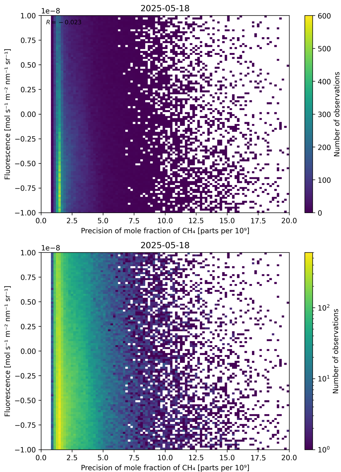
Figure 81: Scatter density plot of “Precision of mole fraction of \text{CH}_4 ” against “Fluorescence” for 2025-05-17 to 2025-05-19.
