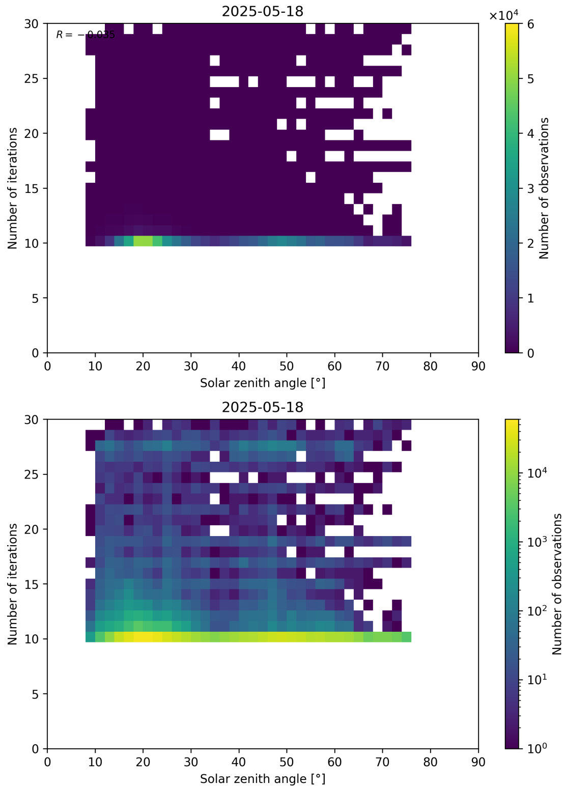
Figure 102: Scatter density plot of “Solar zenith angle” against “Number of iterations” for 2025-05-17 to 2025-05-19.
