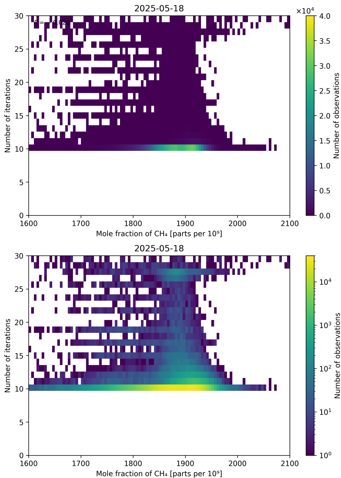
Figure 76: Scatter density plot of “Mole fraction of CH 4 ” against “Number of iterations” for 2025-05-17 to 2025-05-19.
