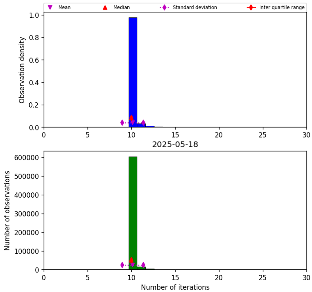
Figure 31: Histogram of “Number of iterations” for 2025-05-17 to 2025-05-19
