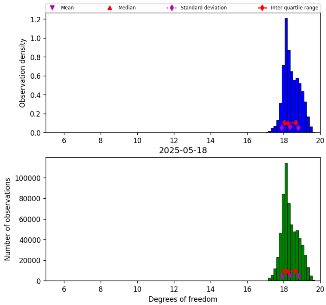
Figure 30: Histogram of “Degrees of freedom” for 2025-05-17 to 2025-05-19
