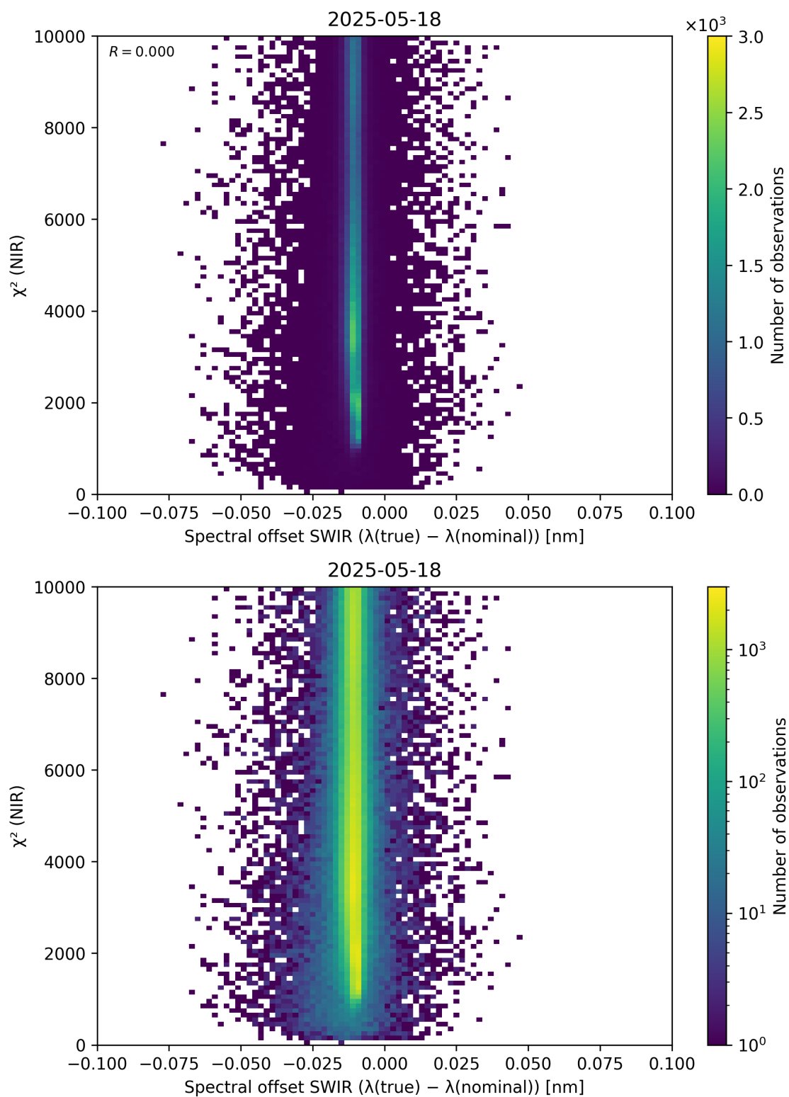
Figure 117: Scatter density plot of “Spectral offset SWIR ( \lambda_{\text{true}} - \lambda_{\text{nominal}} )” against “ \chi^2 (NIR)” for 2025-05-17 to 2025-05-19.
