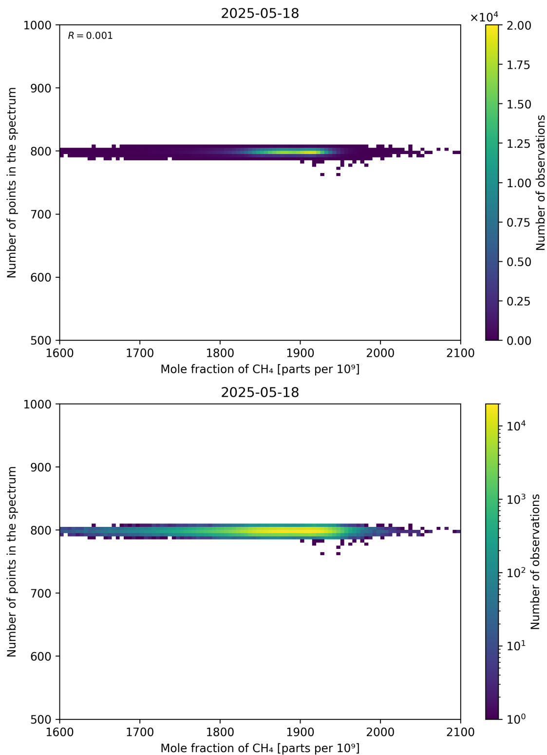
Figure 77: Scatter density plot of “Mole fraction of CH 4 ” against “Number of points in the spectrum” for 2025-05-17 to 2025-05-19.
