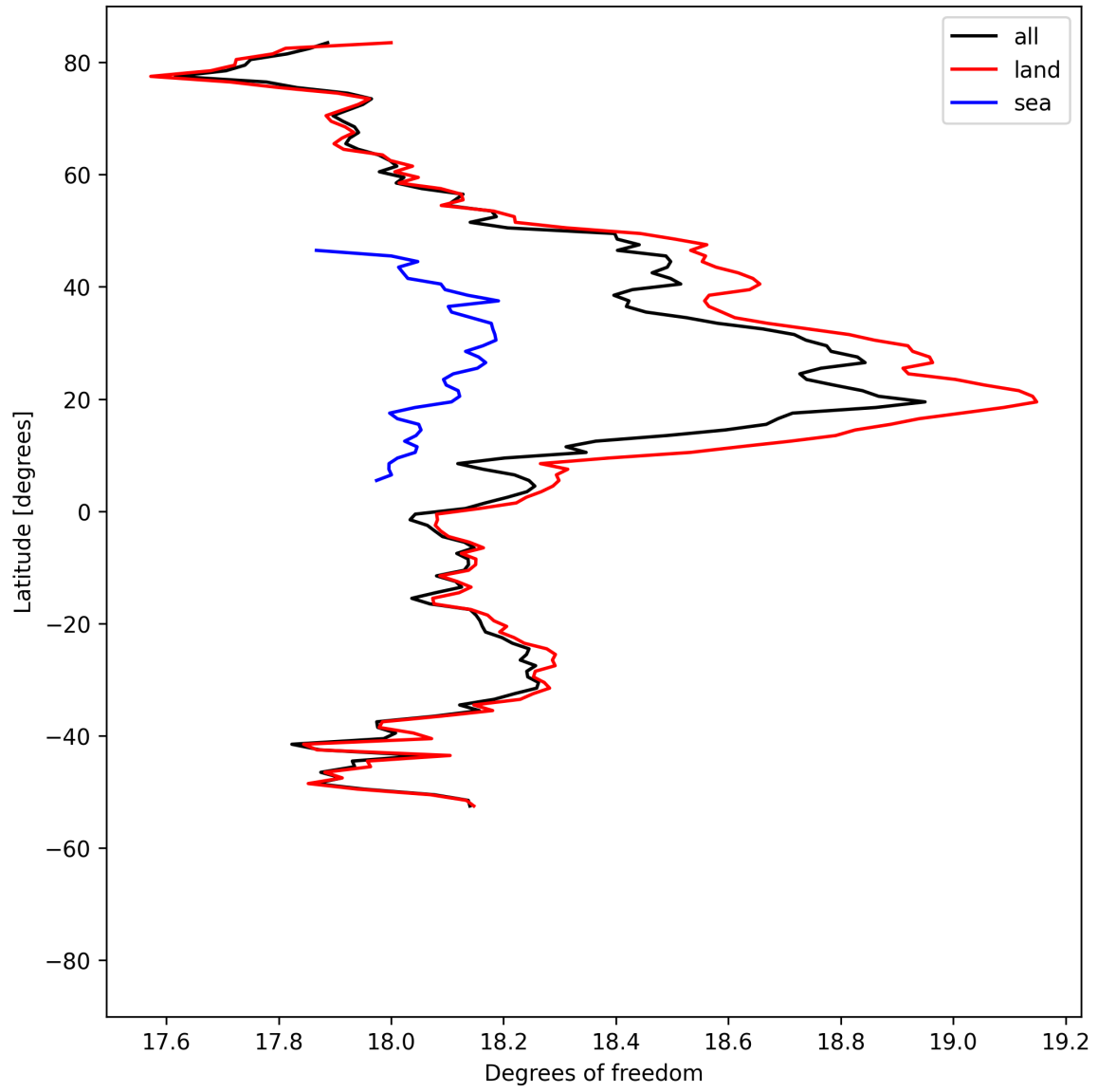
Figure 19: Zonal average of “Degrees of freedom” for 2025-05-17 to 2025-05-19.
