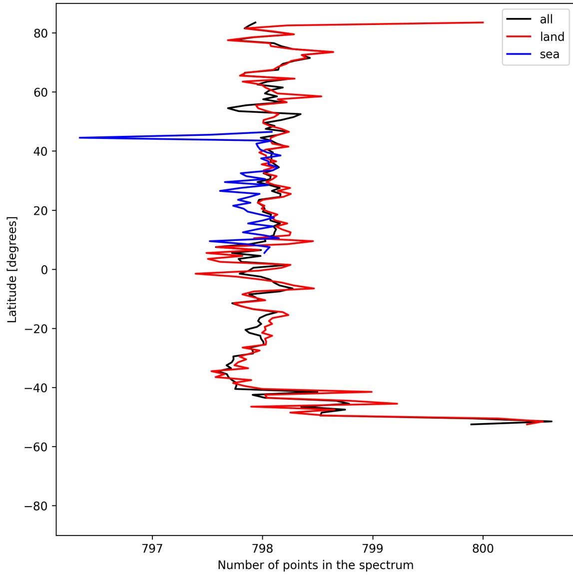
Figure 15: Zonal average of “Number of points in the spectrum” for 2025-05-17 to 2025-05-19.
