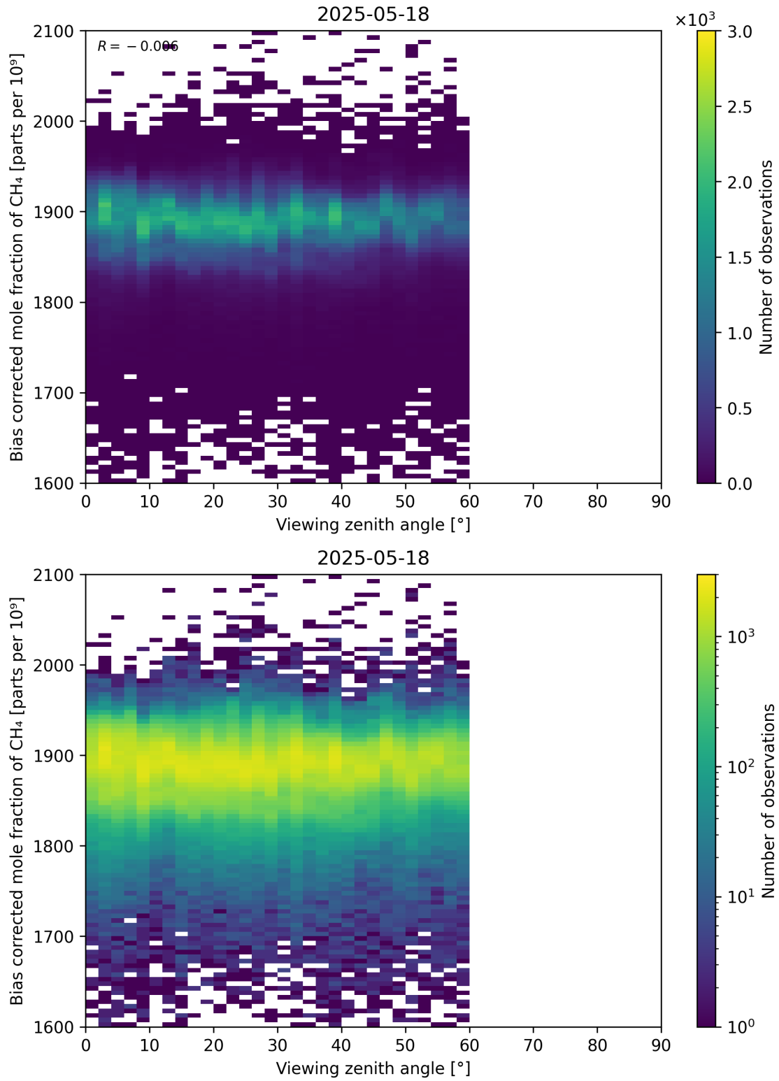
Figure 111: Scatter density plot of “Viewing zenith angle” against “Bias corrected mole fraction of CH 4 ” for 2025-05-17 to 2025-05-19.
