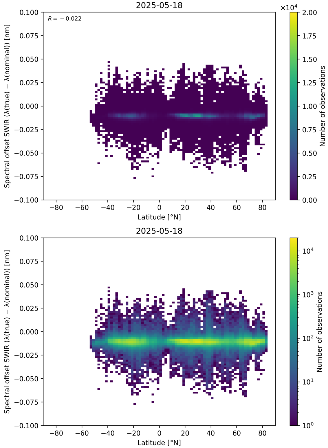
Figure 62: Scatter density plot of “Latitude” against “Spectral offset SWIR ( \lambda_{\text{true}} - \lambda_{\text{nominal}} )” for 2025-05-17 to 2025-05-19.
