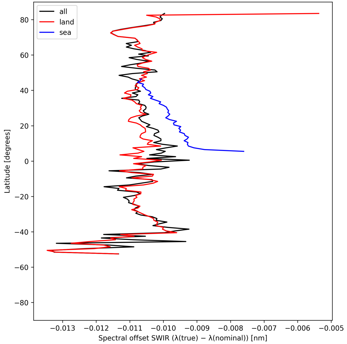
Figure 16: Zonal average of “Spectral offset SWIR ( \lambda_{\text{true}} - \lambda_{\text{nominal}} )” for 2025-05-17 to 2025-05-19.
