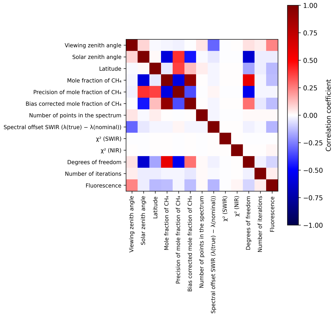
Figure 2: Map of correlation matrix for 2025-05-17 to 2025-05-19.
