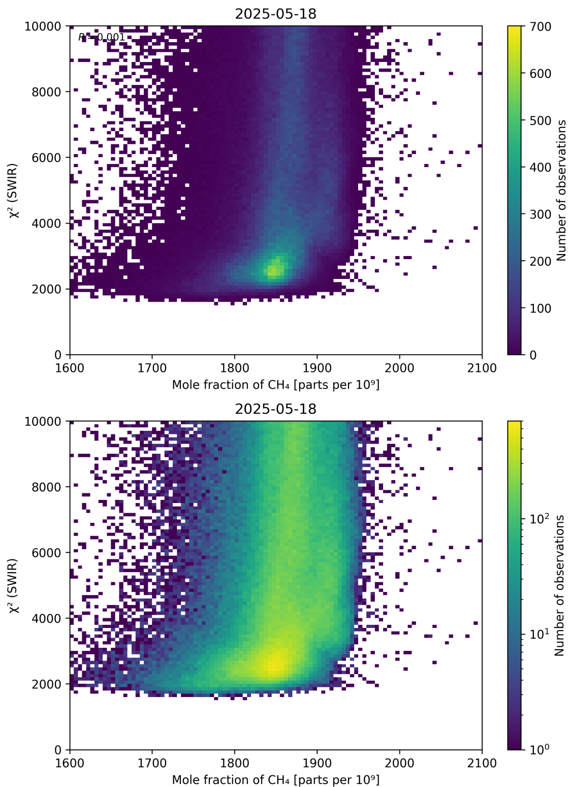
Figure 71: Scatter density plot of “Mole fraction of CH 4 ” against “ \chi^2 (SWIR)” for 2025-05-17 to 2025-05-19.
