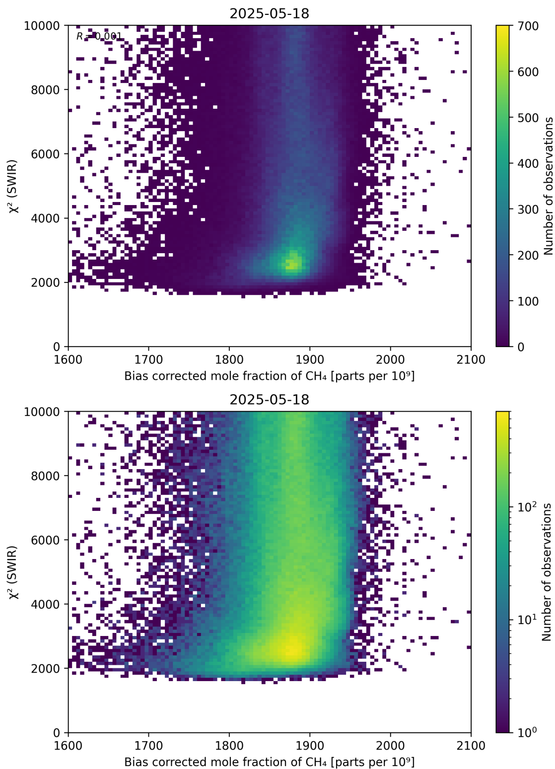
Figure 64: Scatter density plot of “Bias corrected mole fraction of \text{CH}_4 ” against “ \chi^2 (SWIR)” for 2025-05-17 to 2025-05-19.
