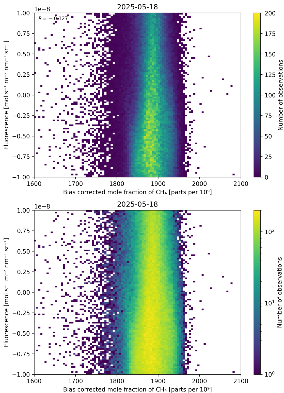
Figure 66: Scatter density plot of “Bias corrected mole fraction of \text{CH}_4 ” against “Fluorescence” for 2025-05-17 to 2025-05-19.
