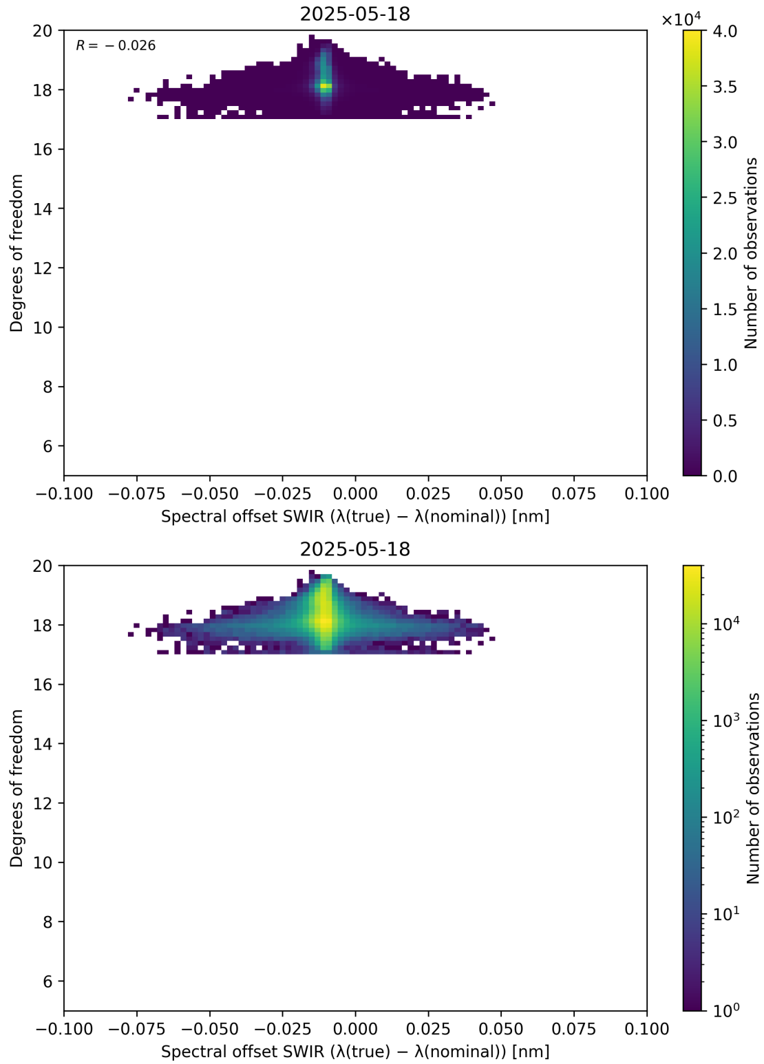
Figure 119: Scatter density plot of “Spectral offset SWIR ( \lambda_{\text{true}} - \lambda_{\text{nominal}} )” against “Degrees of freedom” for 2025-05-17 to 2025-05-19.
