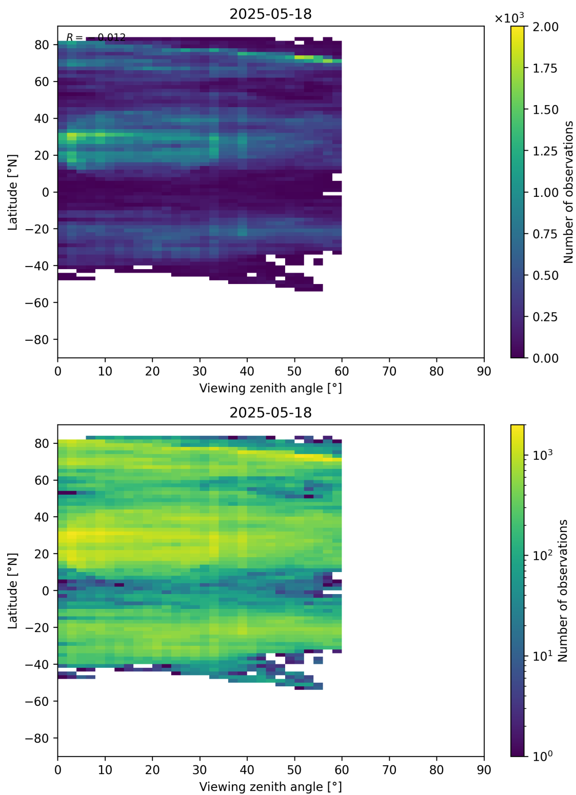
Figure 109: Scatter density plot of “Viewing zenith angle” against “Latitude” for 2025-05-17 to 2025-05-19.
