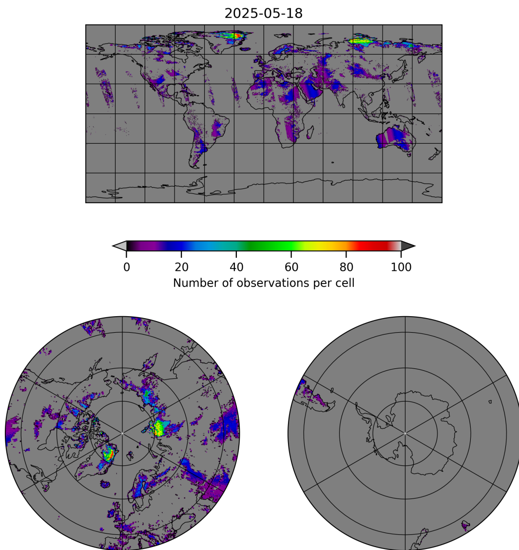
Figure 10: Map of the number of observations for 2025-05-17 to 2025-05-19
