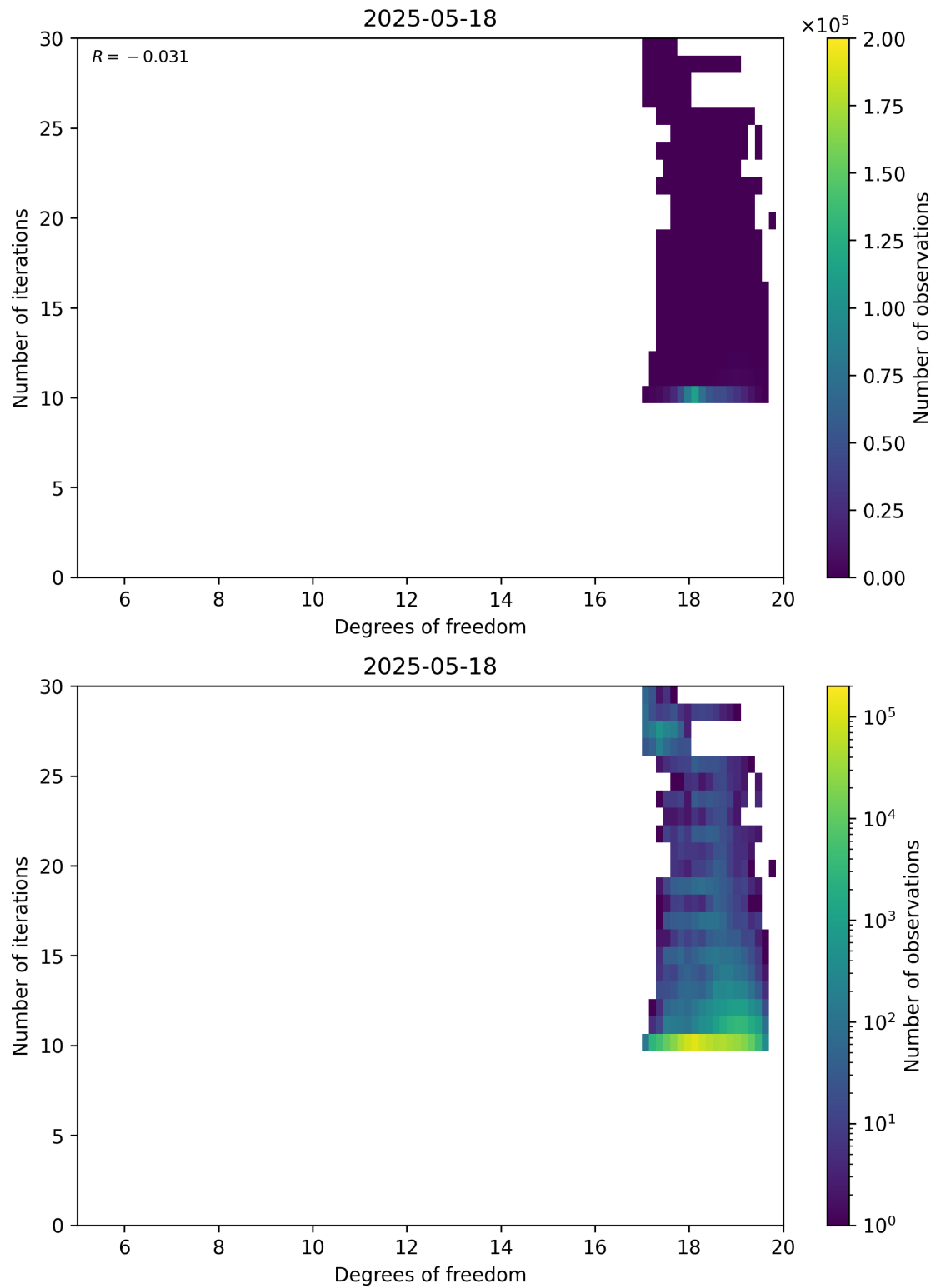
Figure 52: Scatter density plot of “Degrees of freedom” against “Number of iterations” for 2025-05-17 to 2025-05-19.
