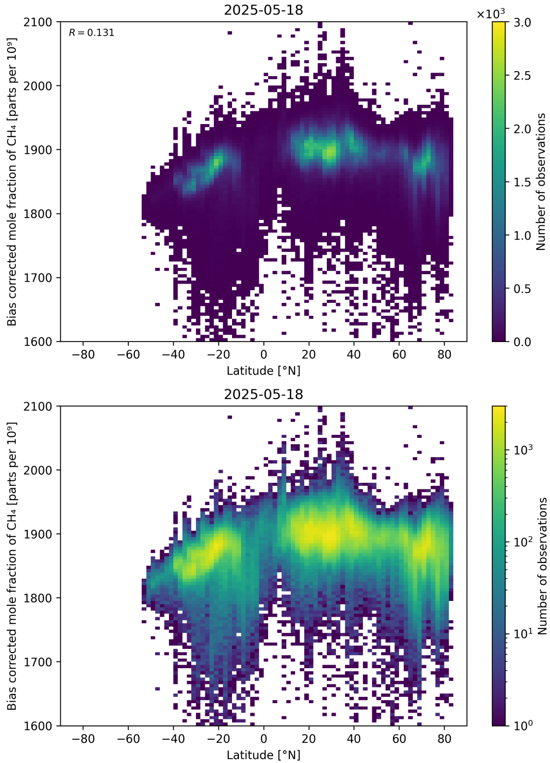
Figure 58: Scatter density plot of “Latitude” against “Bias corrected mole fraction of CH 4 ” for 2025-05-17 to 2025-05-19.
