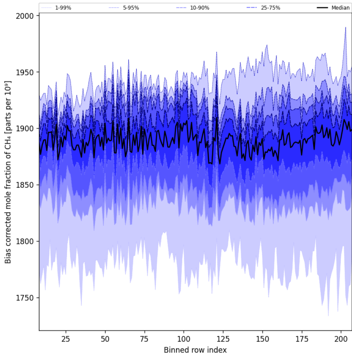
Figure 36: Along track statistics of “Bias corrected mole fraction of CH 4 ” for 2025-05-17 to 2025-05-19
