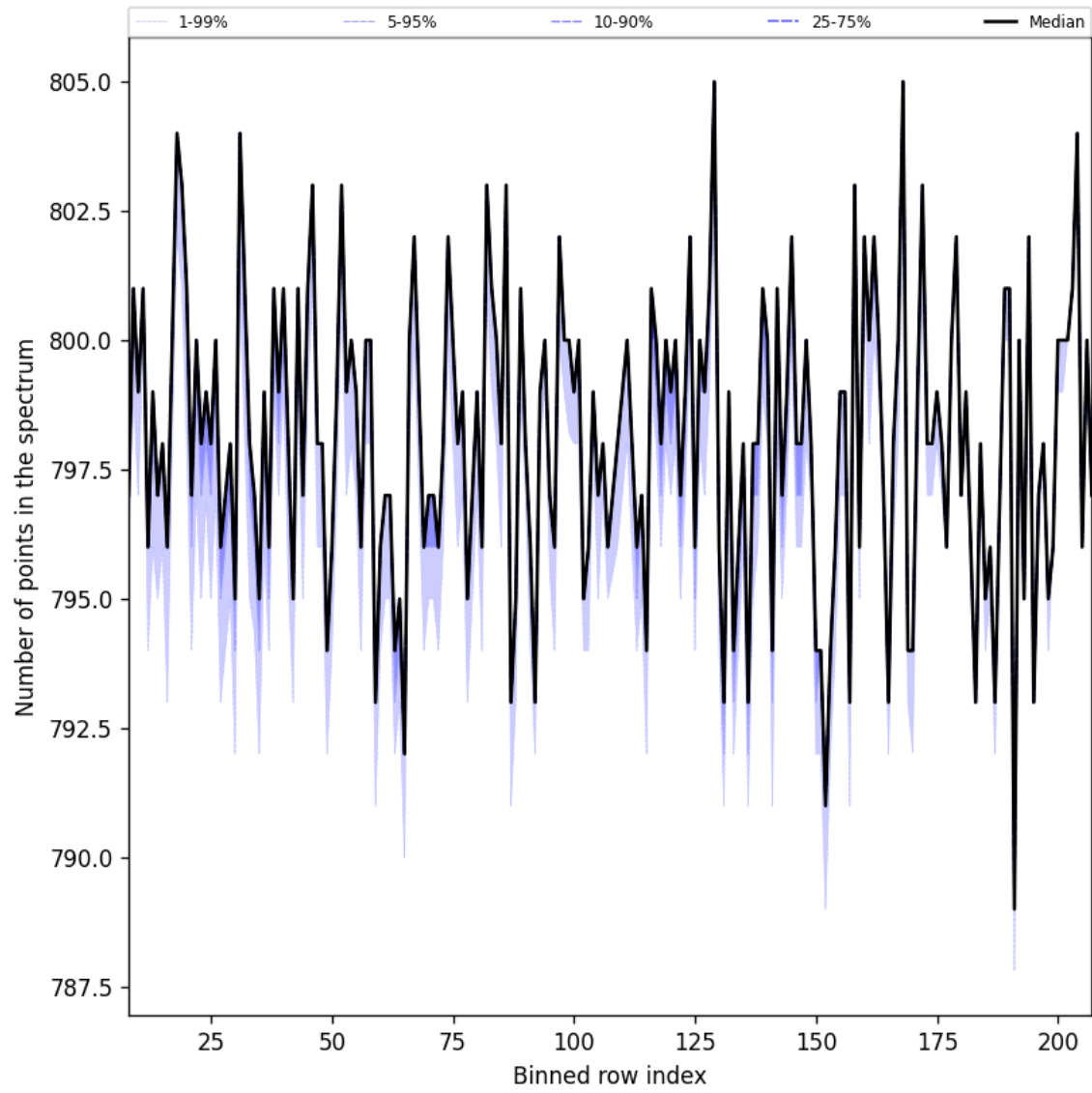
Figure 37: Along track statistics of “Number of points in the spectrum” for 2025-05-17 to 2025-05-19
