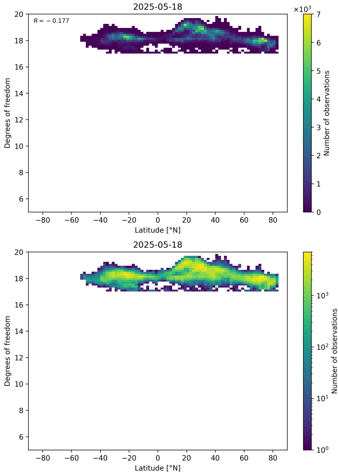
Figure 55: Scatter density plot of “Latitude” against “Degrees of freedom” for 2025-05-17 to 2025-05-19.
