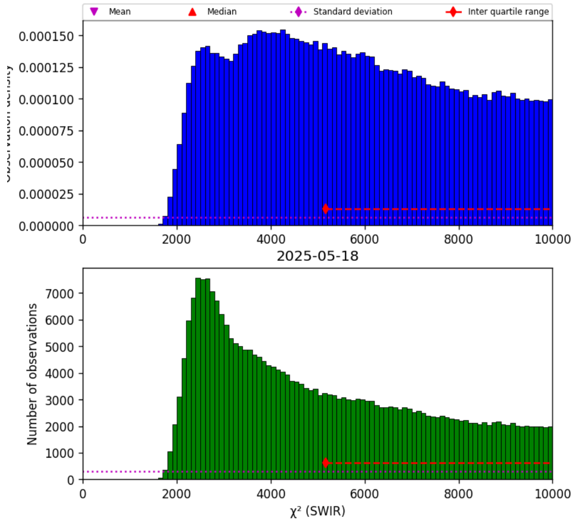
Figure 28: Histogram of “ \chi^2 (SWIR)” for 2025-05-17 to 2025-05-19
