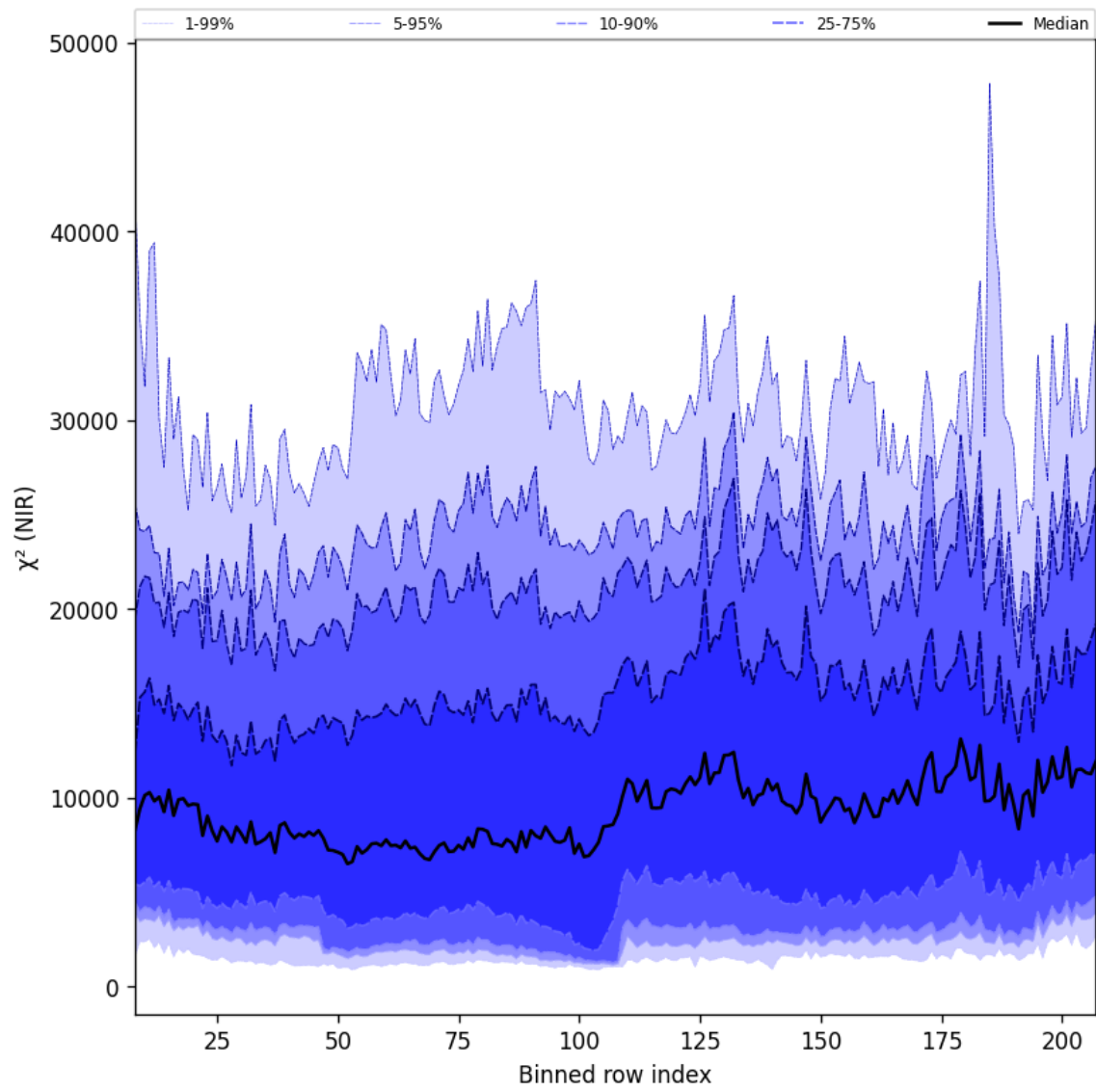
Figure 40: Along track statistics of “ \chi^2 (NIR)” for 2025-05-17 to 2025-05-19
