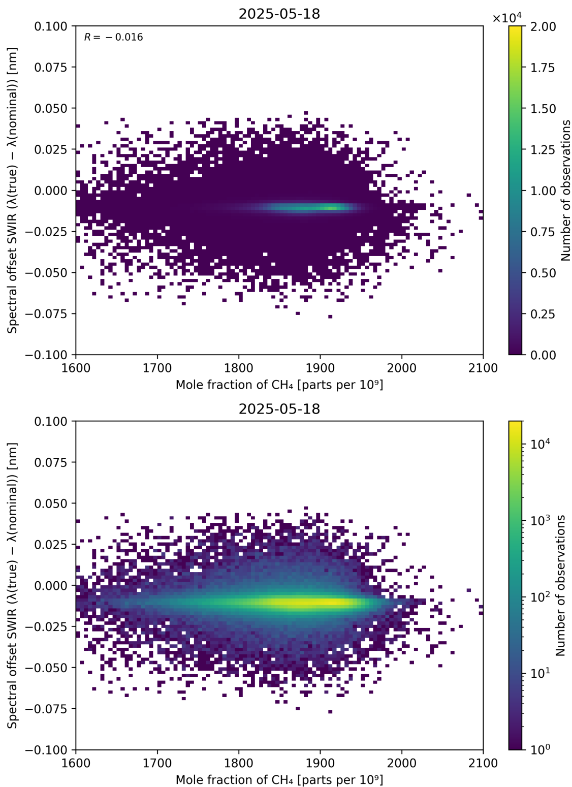
Figure 86: Scatter density plot of “Mole fraction of CH 4 ” against “Spectral offset SWIR ( \lambda_{\text{true}} - \lambda_{\text{nominal}} )” for 2025-05-17 to 2025-05-19.
