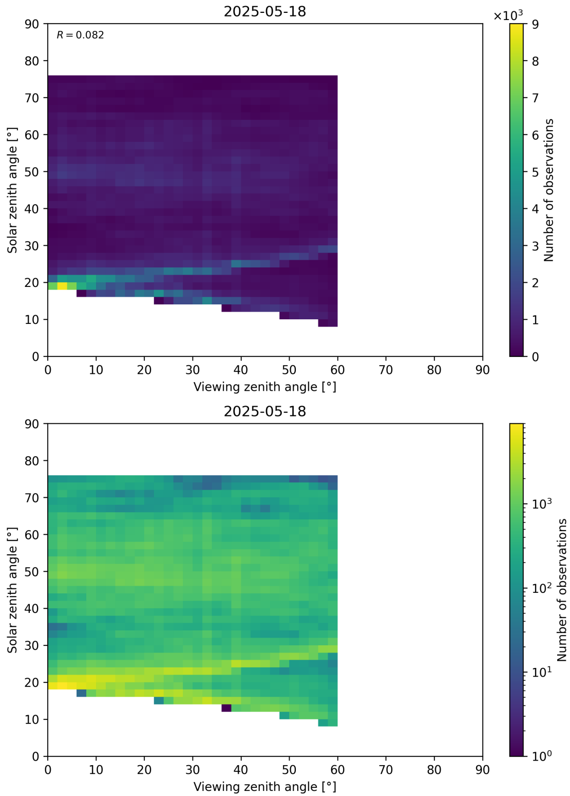
Figure 115: Scatter density plot of “Viewing zenith angle” against “Solar zenith angle” for 2025-05-17 to 2025-05-19.
