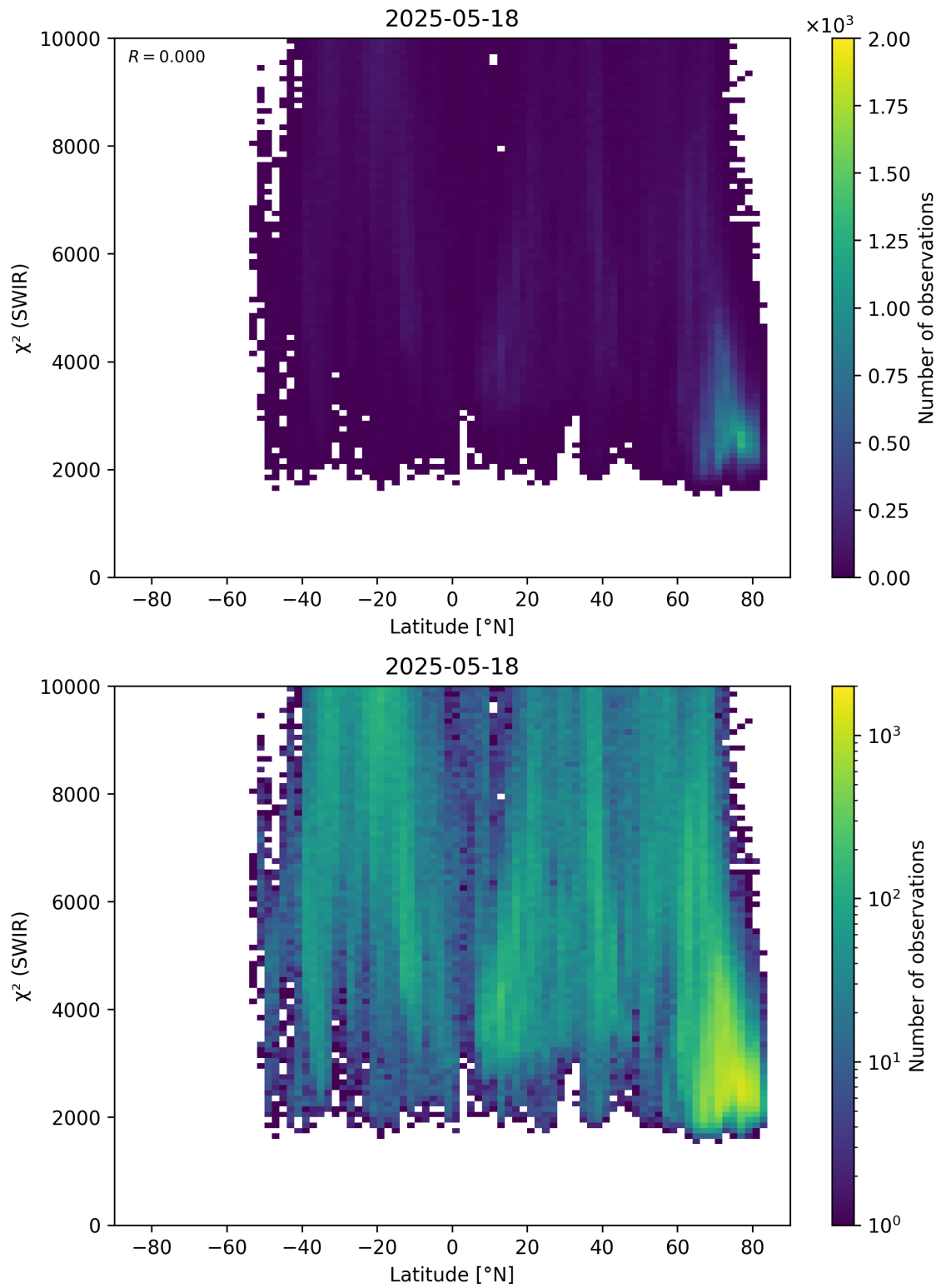
Figure 54: Scatter density plot of “Latitude” against “ \chi^2 (SWIR)” for 2025-05-17 to 2025-05-19.
