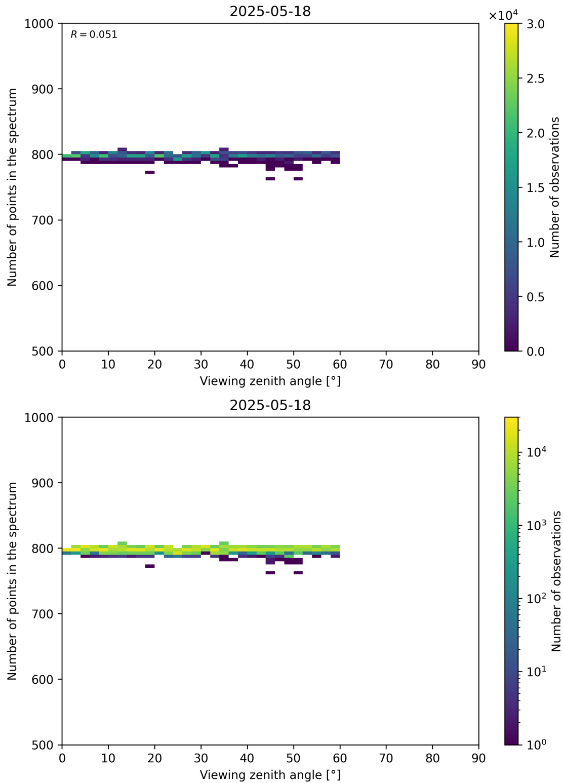
Figure 114: Scatter density plot of “Viewing zenith angle” against “Number of points in the spectrum” for 2025-05-17 to 2025-05-19.
