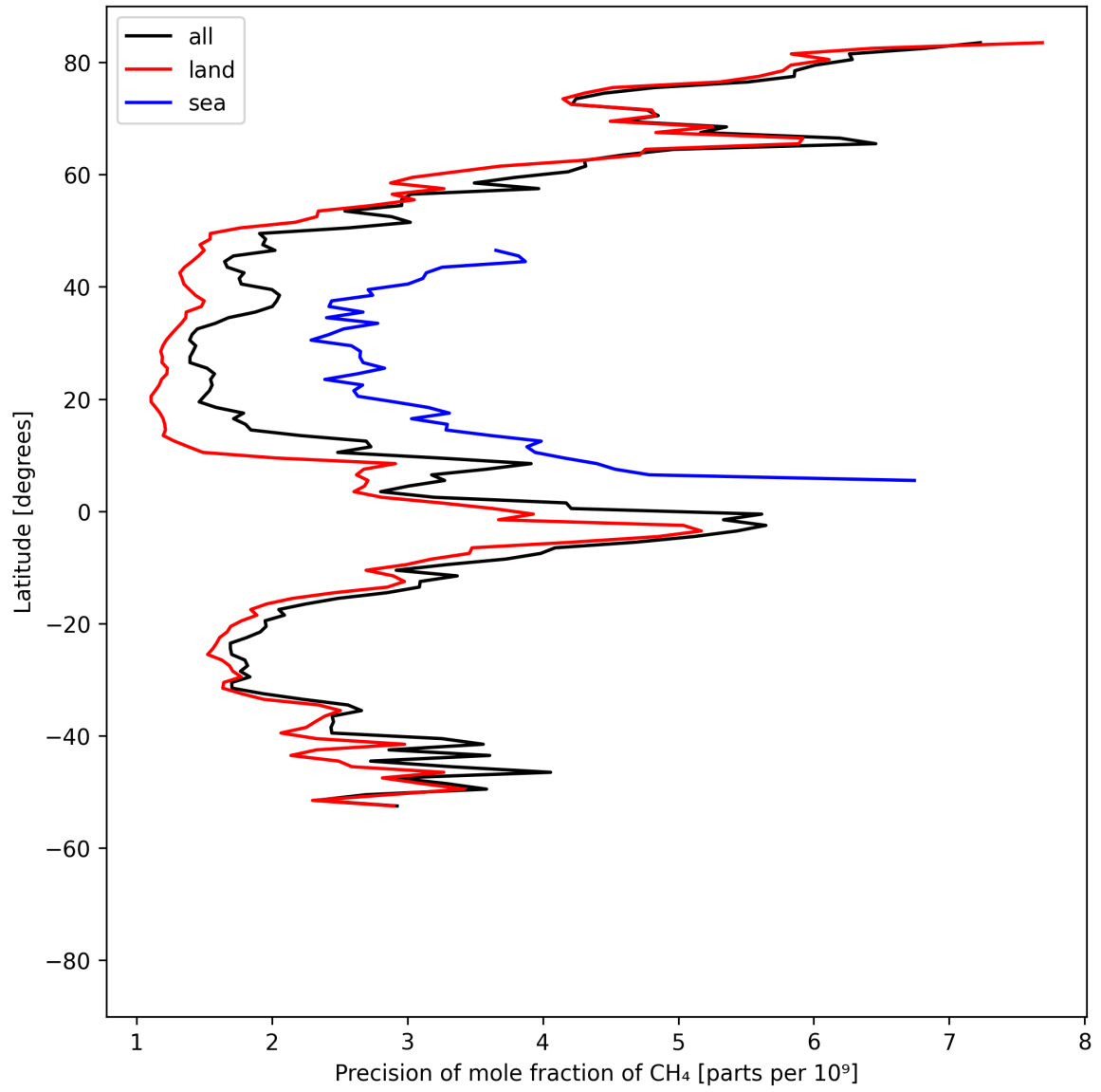
Figure 13: Zonal average of “Precision of mole fraction of CH 4 ” for 2025-05-17 to 2025-05-19.
