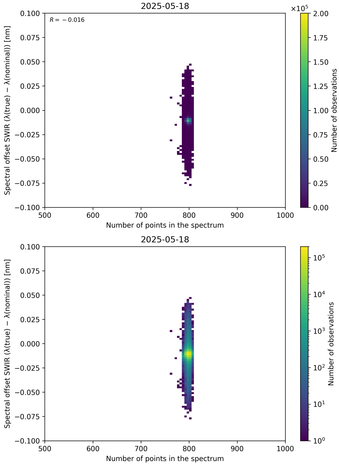
Figure 93: Scatter density plot of “Number of points in the spectrum” against “Spectral offset SWIR ( \lambda_{\text{true}} - \lambda_{\text{nominal}} )” for 2025-05-17 to 2025-05-19.
