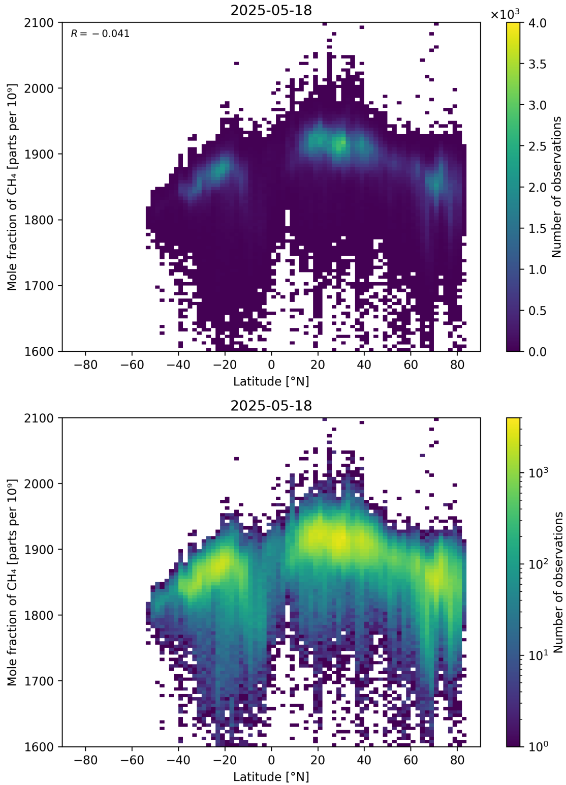
Figure 57: Scatter density plot of “Latitude” against “Mole fraction of CH 4 ” for 2025-05-17 to 2025-05-19.
