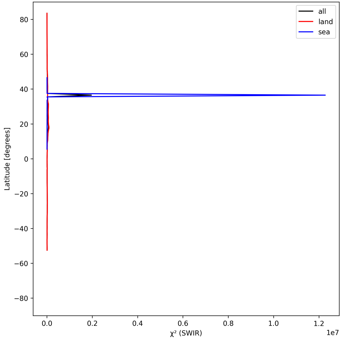
Figure 17: Zonal average of “ \chi^2 (SWIR)” for 2025-05-17 to 2025-05-19.
