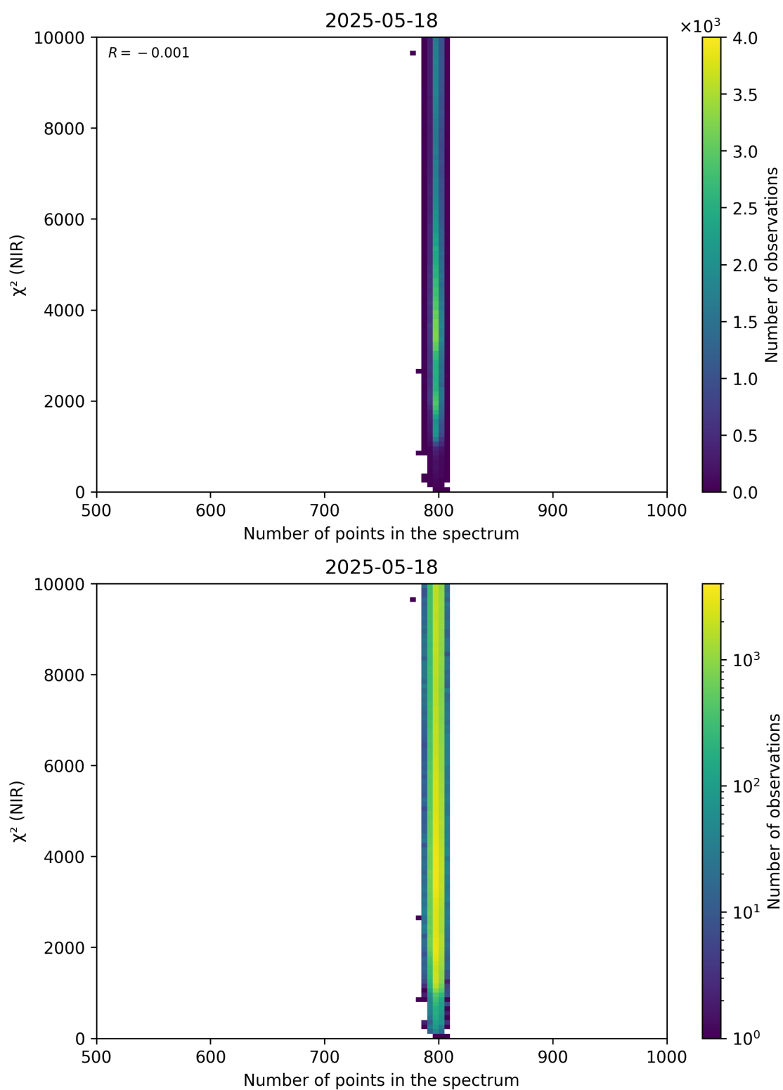
Figure 88: Scatter density plot of “Number of points in the spectrum” against “ \chi^2 (NIR)” for 2025-05-17 to 2025-05-19.
