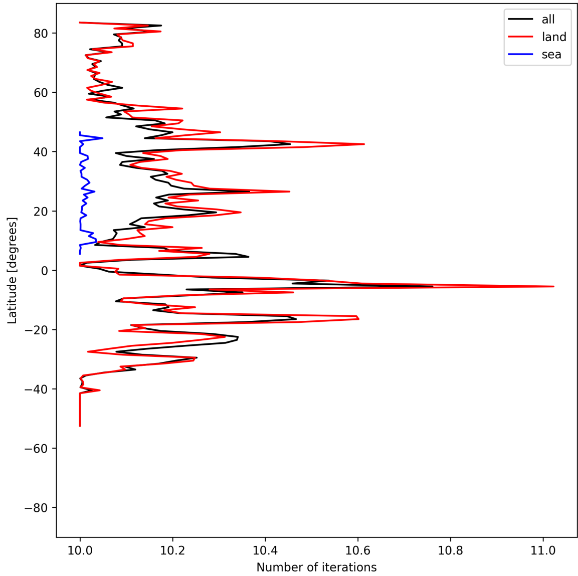
Figure 20: Zonal average of “Number of iterations” for 2025-05-17 to 2025-05-19.
