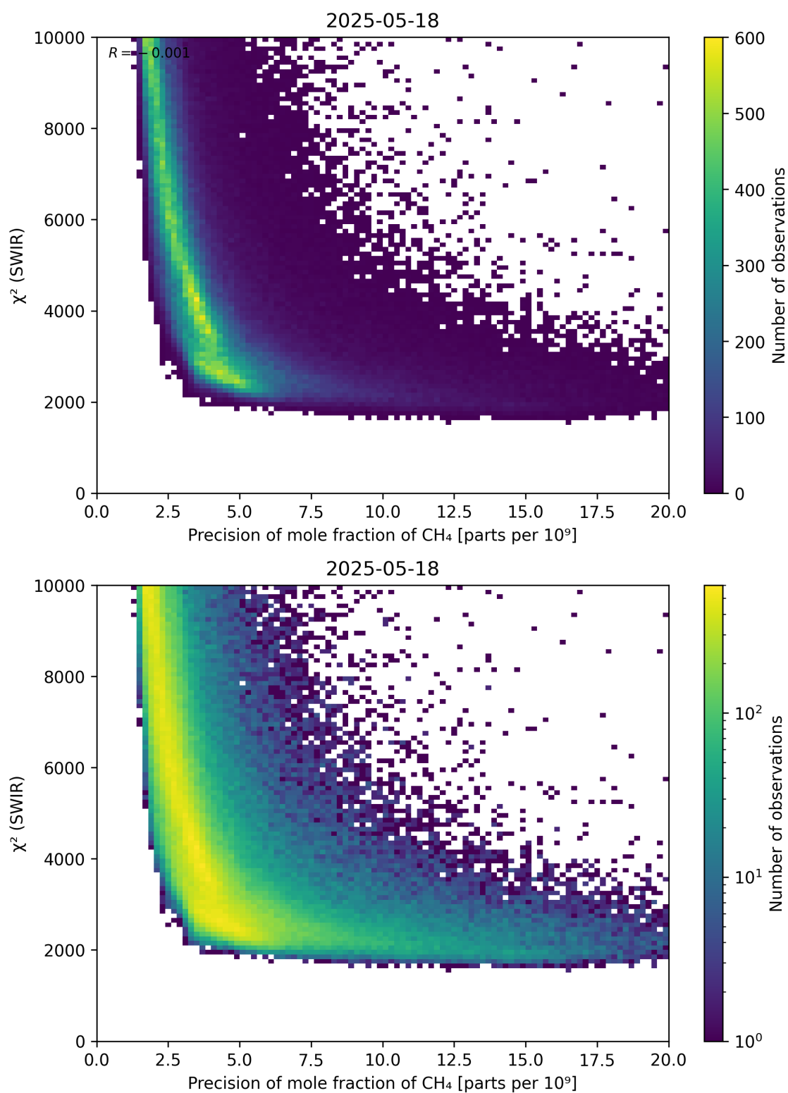
Figure 79: Scatter density plot of “Precision of mole fraction of \text{CH}_4 ” against “ \chi^2 (SWIR)” for 2025-05-17 to 2025-05-19.
