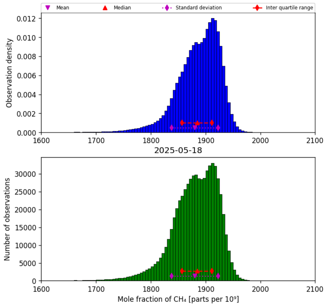
Figure 23: Histogram of “Mole fraction of CH 4 ” for 2025-05-17 to 2025-05-19
