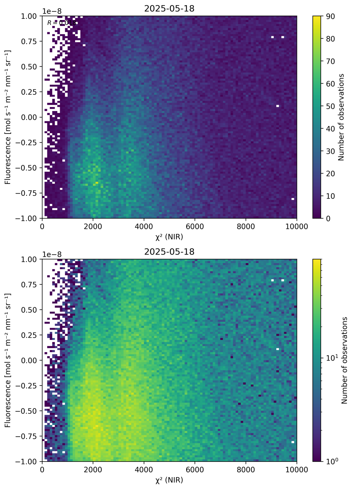
Figure 45: Scatter density plot of “ \chi^2 (NIR)” against “Fluorescence” for 2025-05-17 to 2025-05-19.
