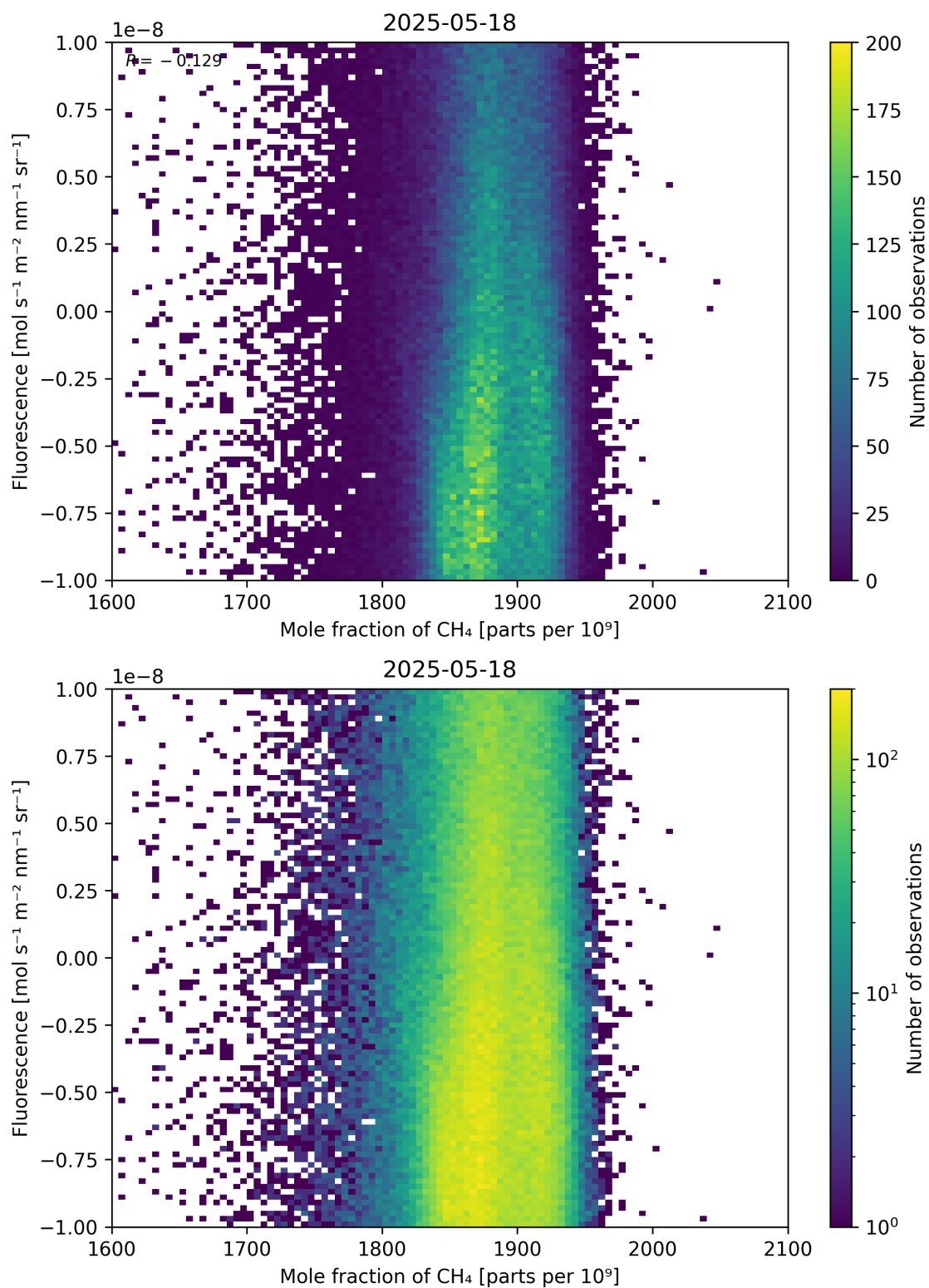
Figure 73: Scatter density plot of “Mole fraction of CH 4 ” against “Fluorescence” for 2025-05-17 to 2025-05-19.
