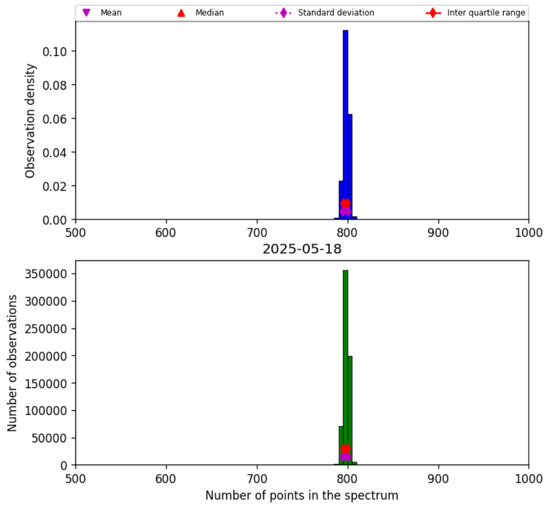
Figure 26: Histogram of “Number of points in the spectrum” for 2025-05-17 to 2025-05-19
