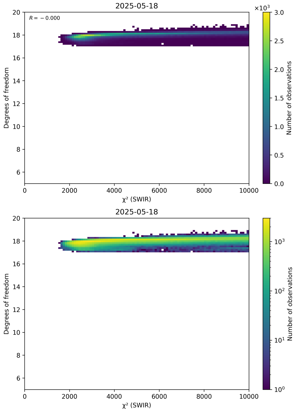
Figure 48: Scatter density plot of “ \chi^2 (SWIR)” against “Degrees of freedom” for 2025-05-17 to 2025-05-19.
