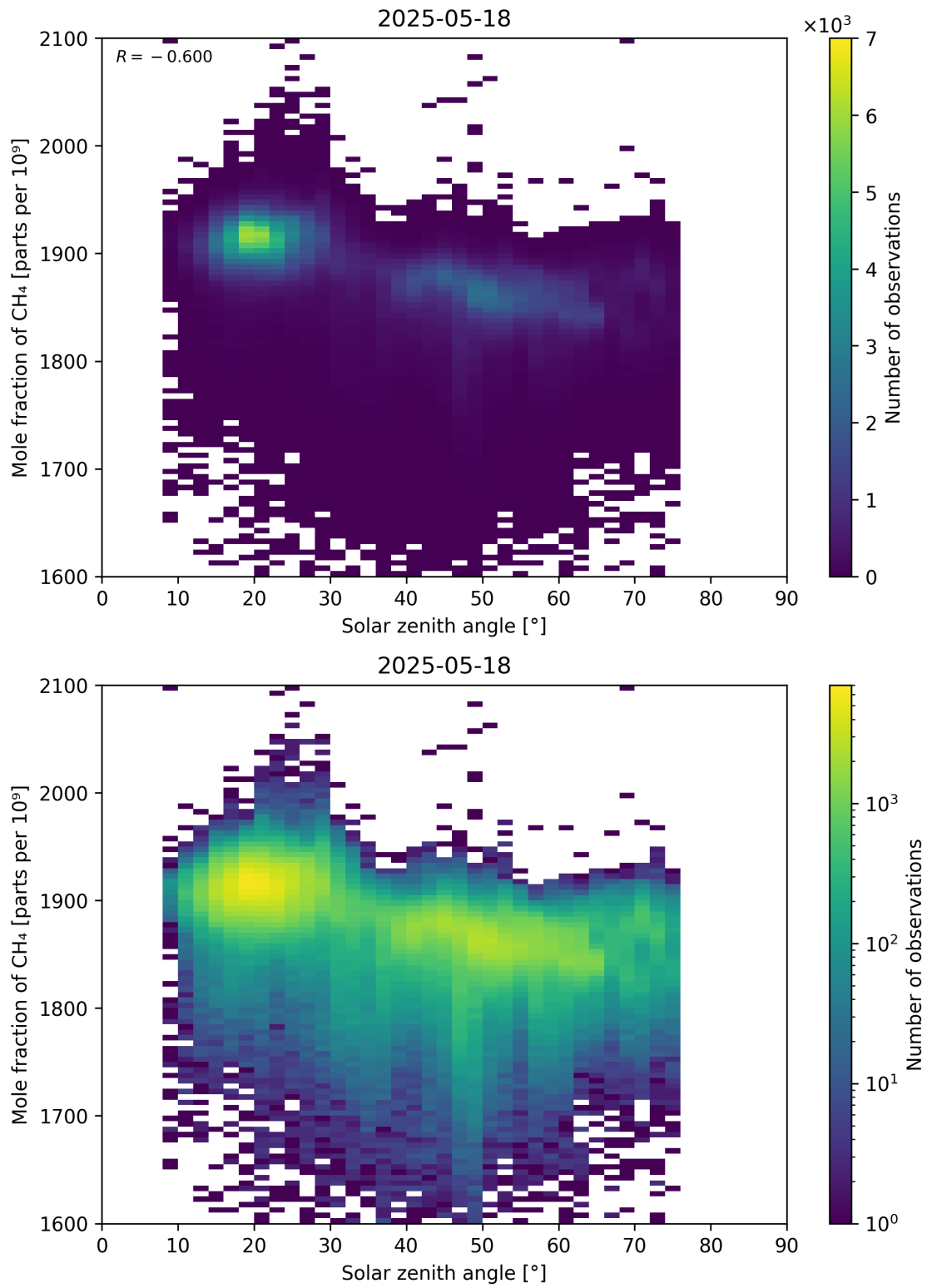
Figure 99: Scatter density plot of “Solar zenith angle” against “Mole fraction of CH 4 ” for 2025-05-17 to 2025-05-19.
