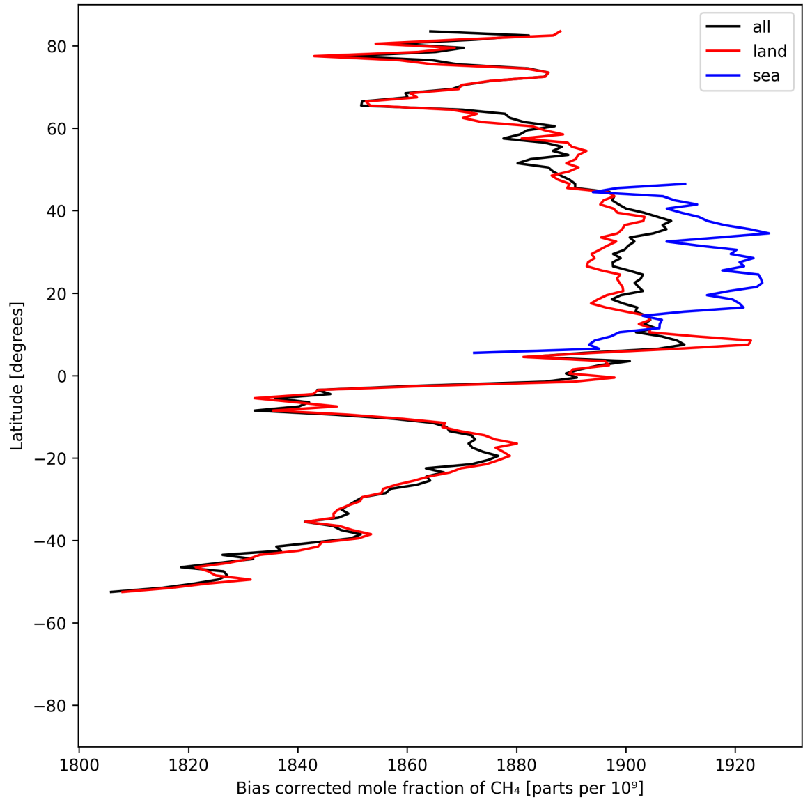
Figure 14: Zonal average of “Bias corrected mole fraction of CH 4 ” for 2025-05-17 to 2025-05-19.
