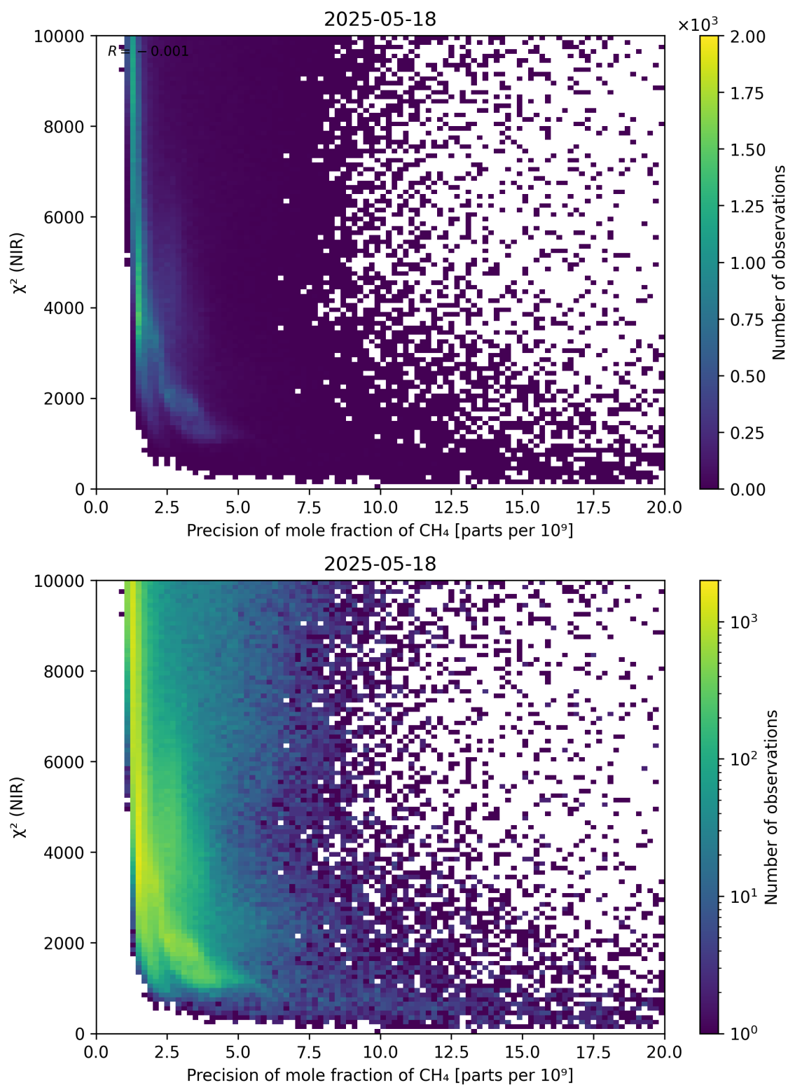
Figure 78: Scatter density plot of “Precision of mole fraction of \text{CH}_4 ” against “ \chi^2 (NIR)” for 2025-05-17 to 2025-05-19.
