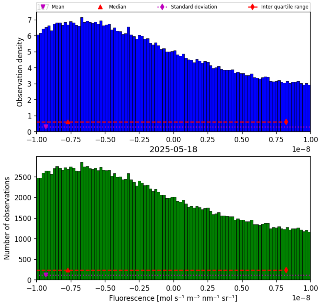
Figure 32: Histogram of “Fluorescence” for 2025-05-17 to 2025-05-19
