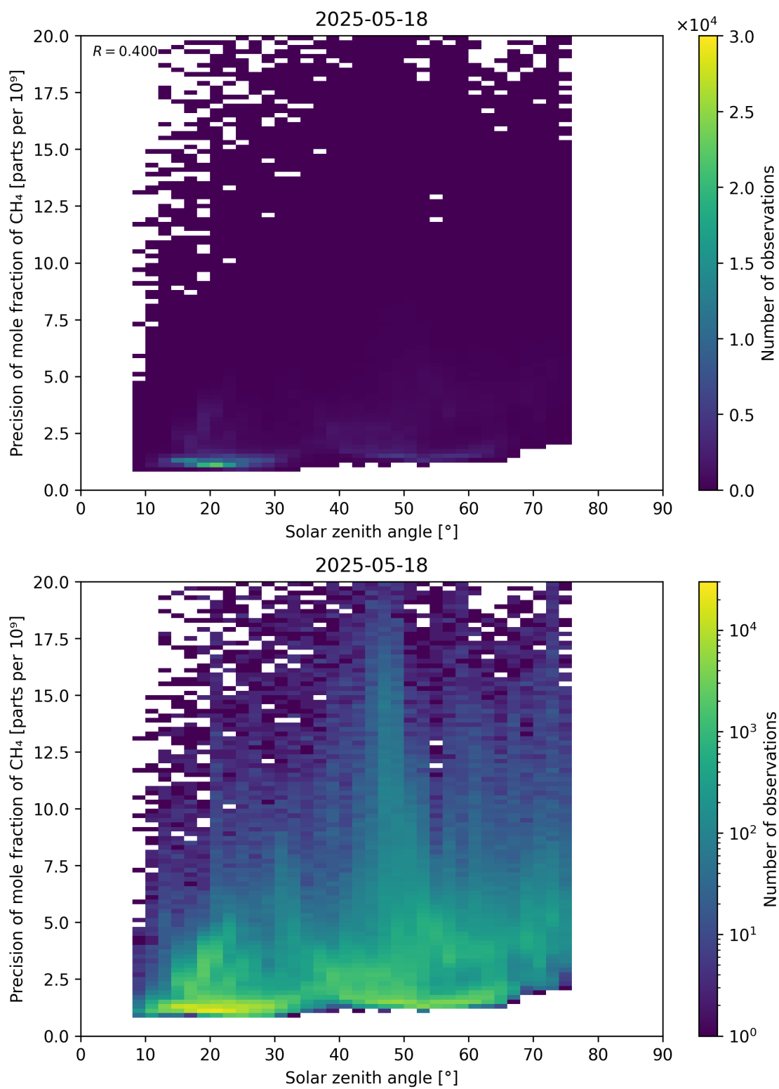
Figure 101: Scatter density plot of “Solar zenith angle” against “Precision of mole fraction of CH 4 ” for 2025-05-17 to 2025-05-19.
