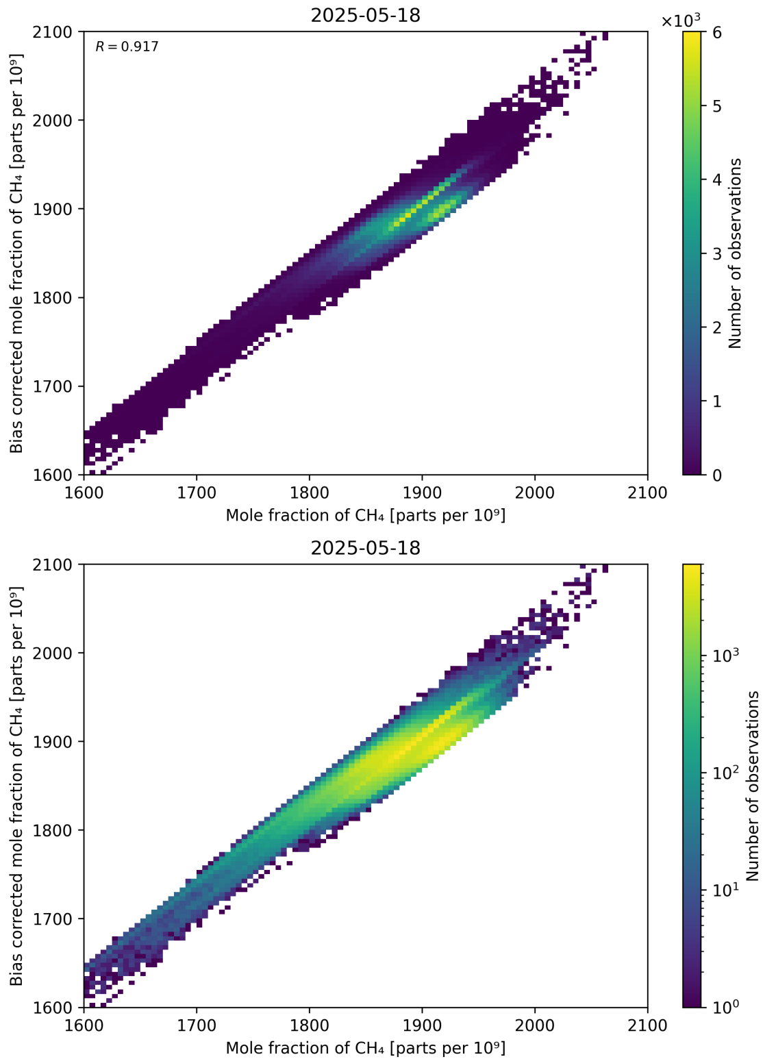
Figure 74: Scatter density plot of “Mole fraction of CH 4 ” against “Bias corrected mole fraction of CH 4 ” for 2025-05-17 to 2025-05-19.
