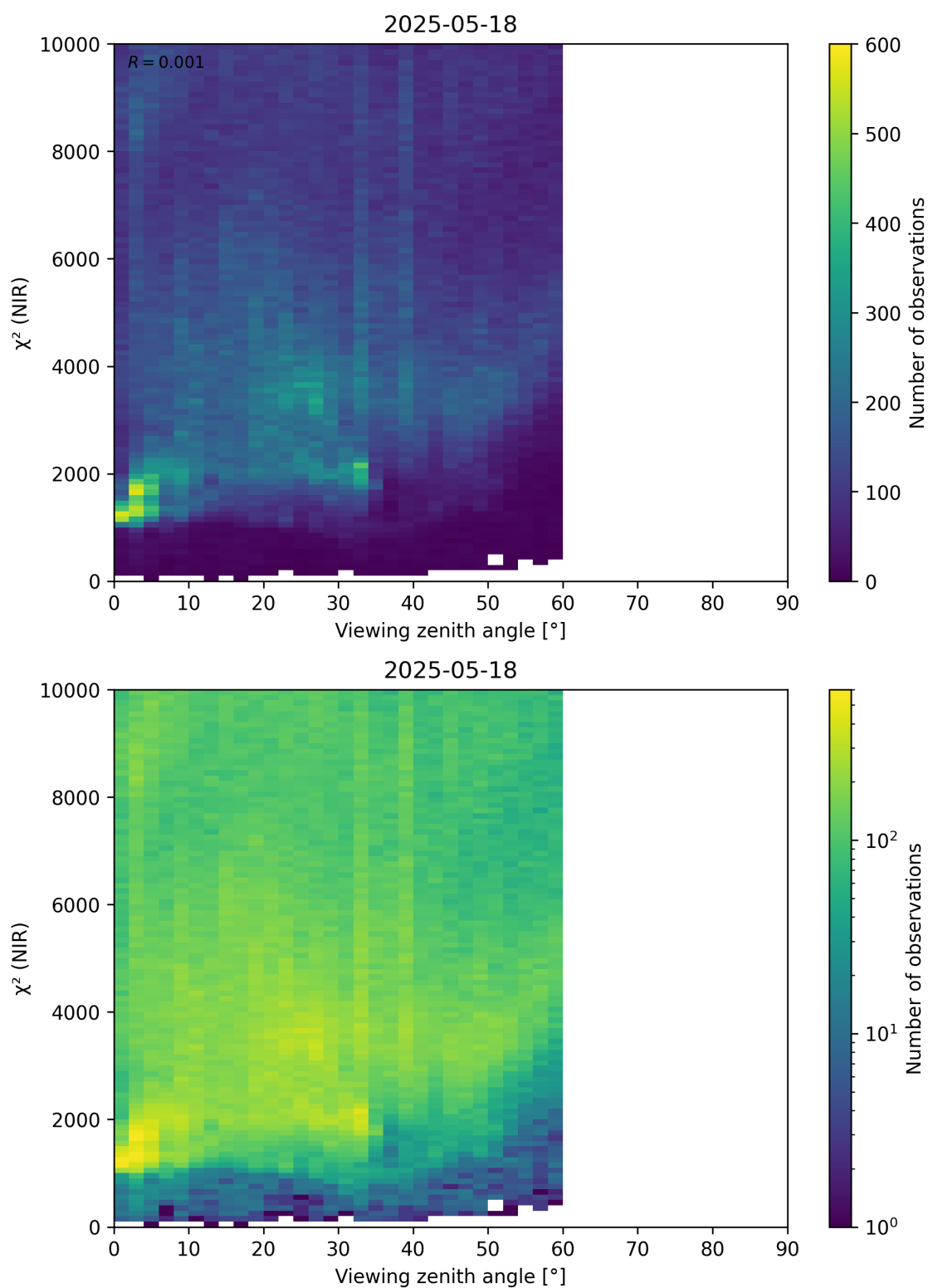
Figure 105: Scatter density plot of “Viewing zenith angle” against “ \chi^2 (NIR)” for 2025-05-17 to 2025-05-19.
