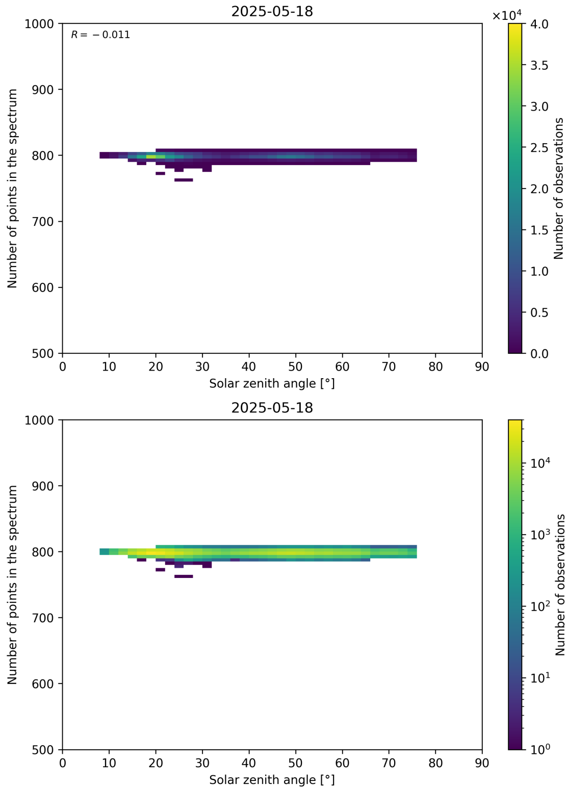
Figure 103: Scatter density plot of “Solar zenith angle” against “Number of points in the spectrum” for 2025-05-17 to 2025-05-19.
