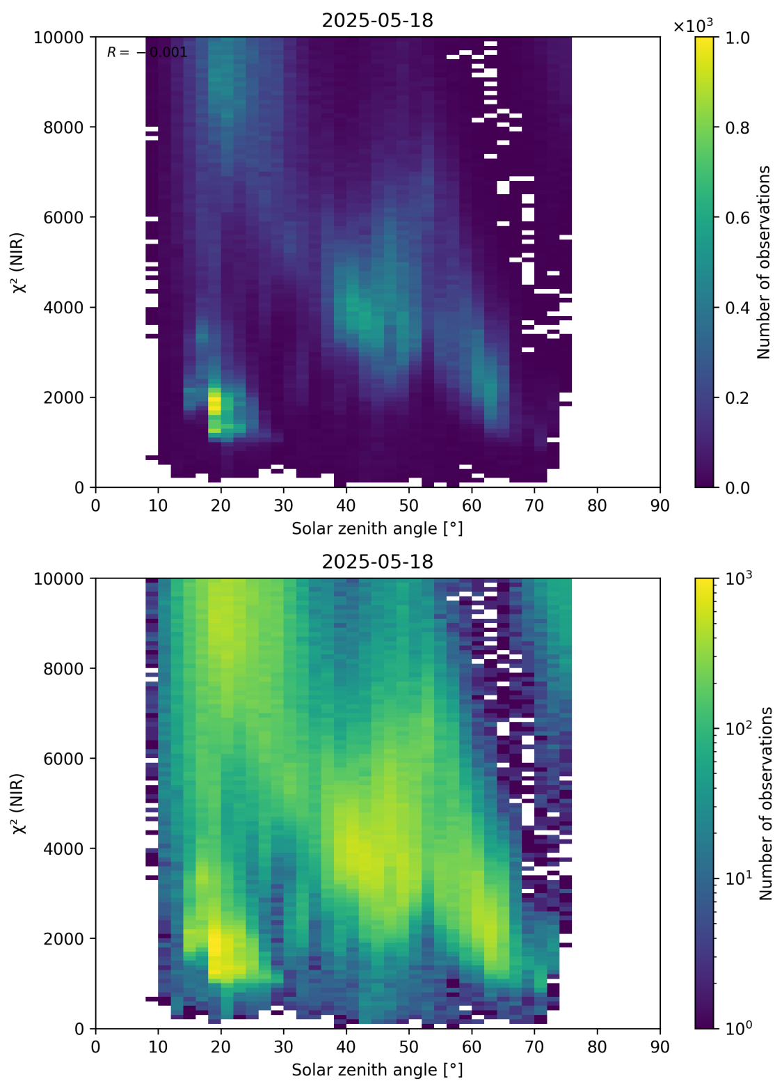
Figure 94: Scatter density plot of “Solar zenith angle” against “ \chi^2 (NIR)” for 2025-05-17 to 2025-05-19.
