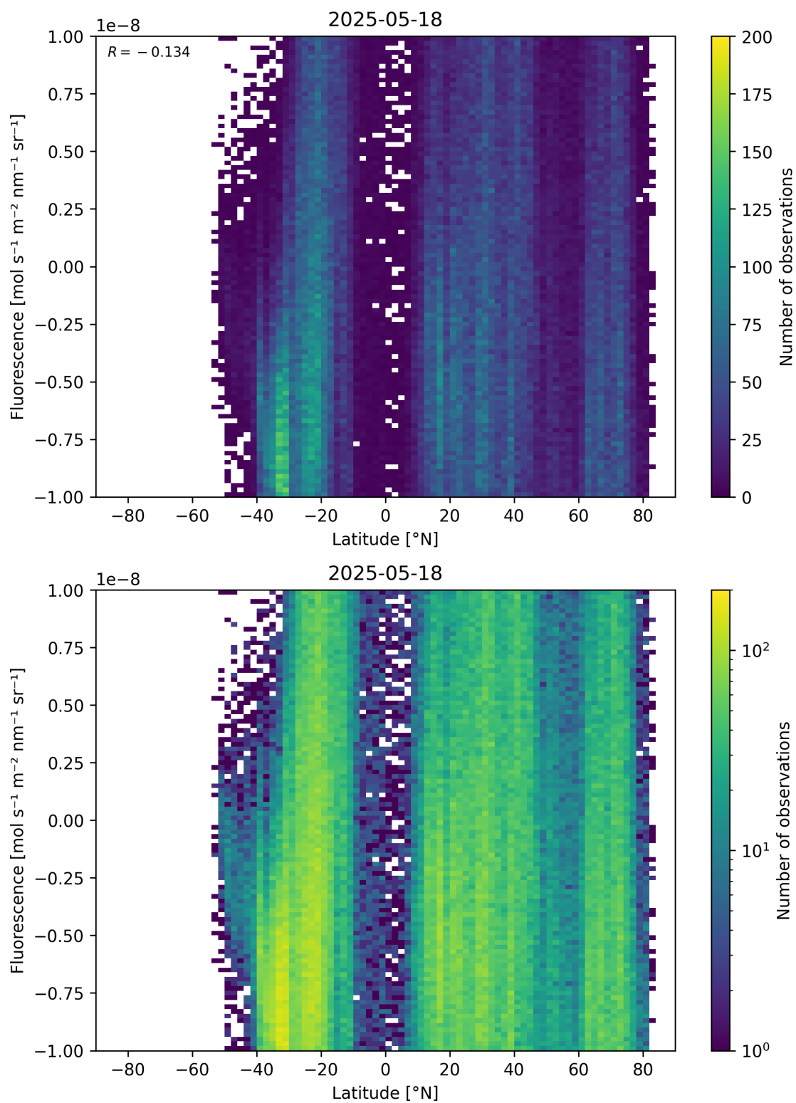
Figure 56: Scatter density plot of “Latitude” against “Fluorescence” for 2025-05-17 to 2025-05-19.
