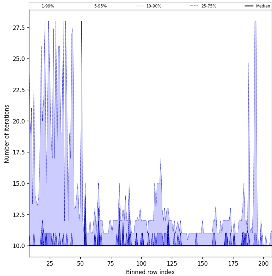
Figure 42: Along track statistics of “Number of iterations” for 2025-05-17 to 2025-05-19
