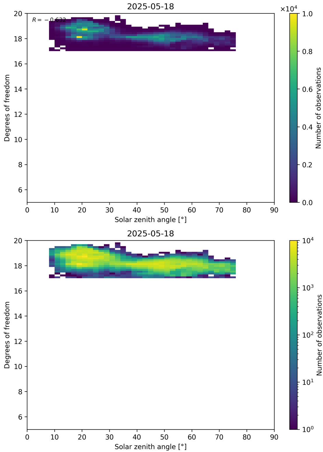
Figure 96: Scatter density plot of “Solar zenith angle” against “Degrees of freedom” for 2025-05-17 to 2025-05-19.
