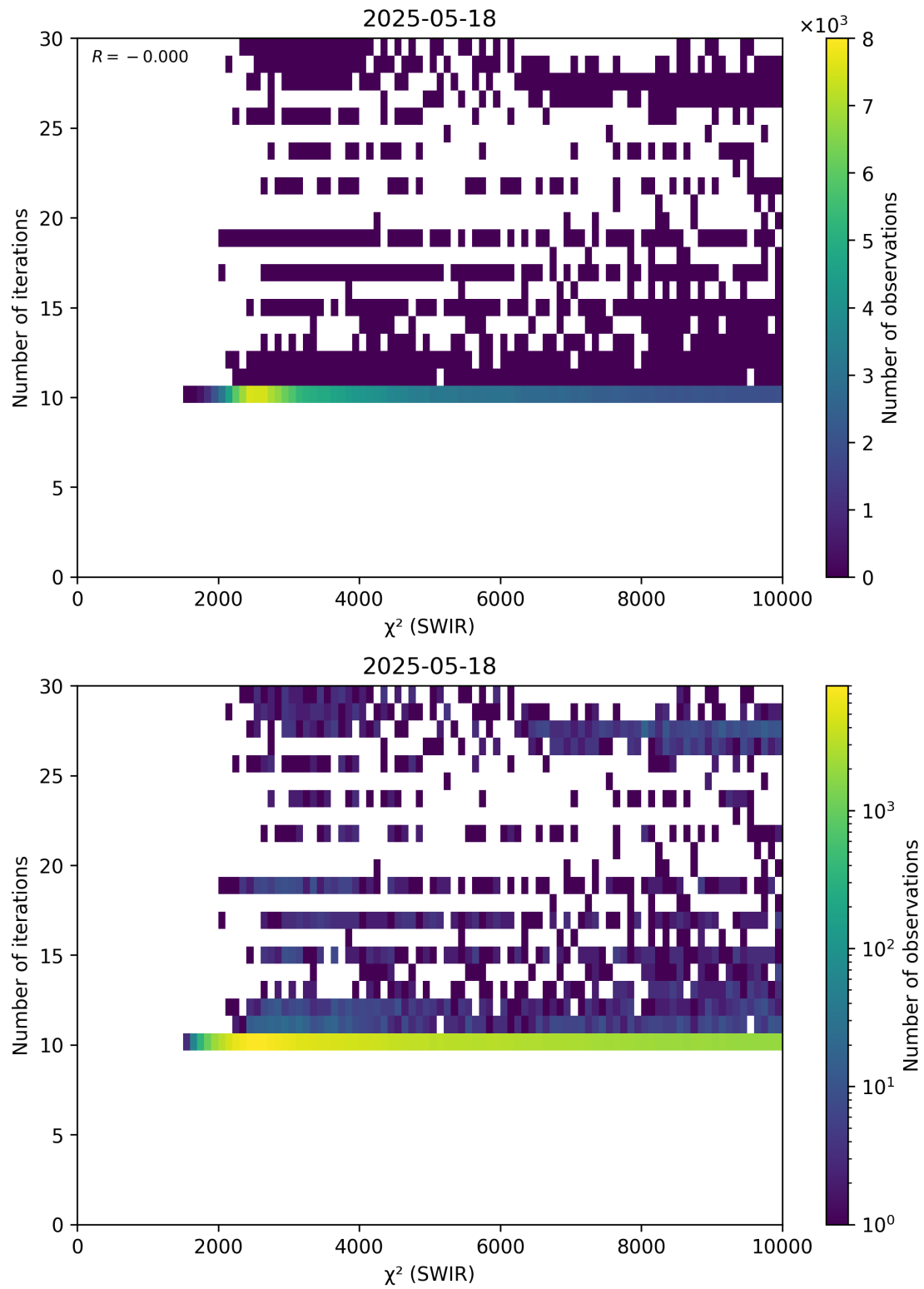
Figure 50: Scatter density plot of “ \chi^2 (SWIR)” against “Number of iterations” for 2025-05-17 to 2025-05-19.
