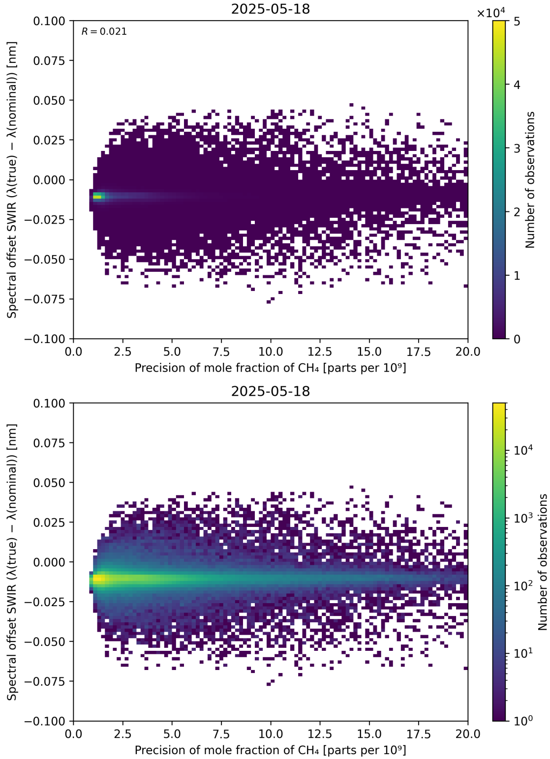
Figure 85: Scatter density plot of “Precision of mole fraction of CH 4 ” against “Spectral offset SWIR ( \lambda_{\text{true}} - \lambda_{\text{nominal}} )” for 2025-05-17 to 2025-05-19.
