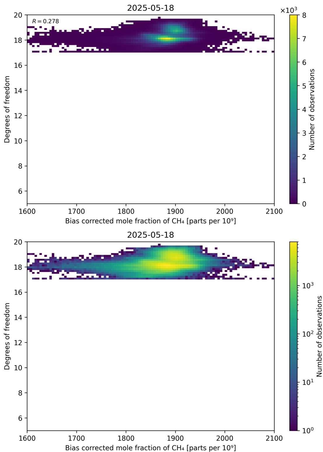
Figure 65: Scatter density plot of “Bias corrected mole fraction of CH 4 ” against “Degrees of freedom” for 2025-05-17 to 2025-05-19.
