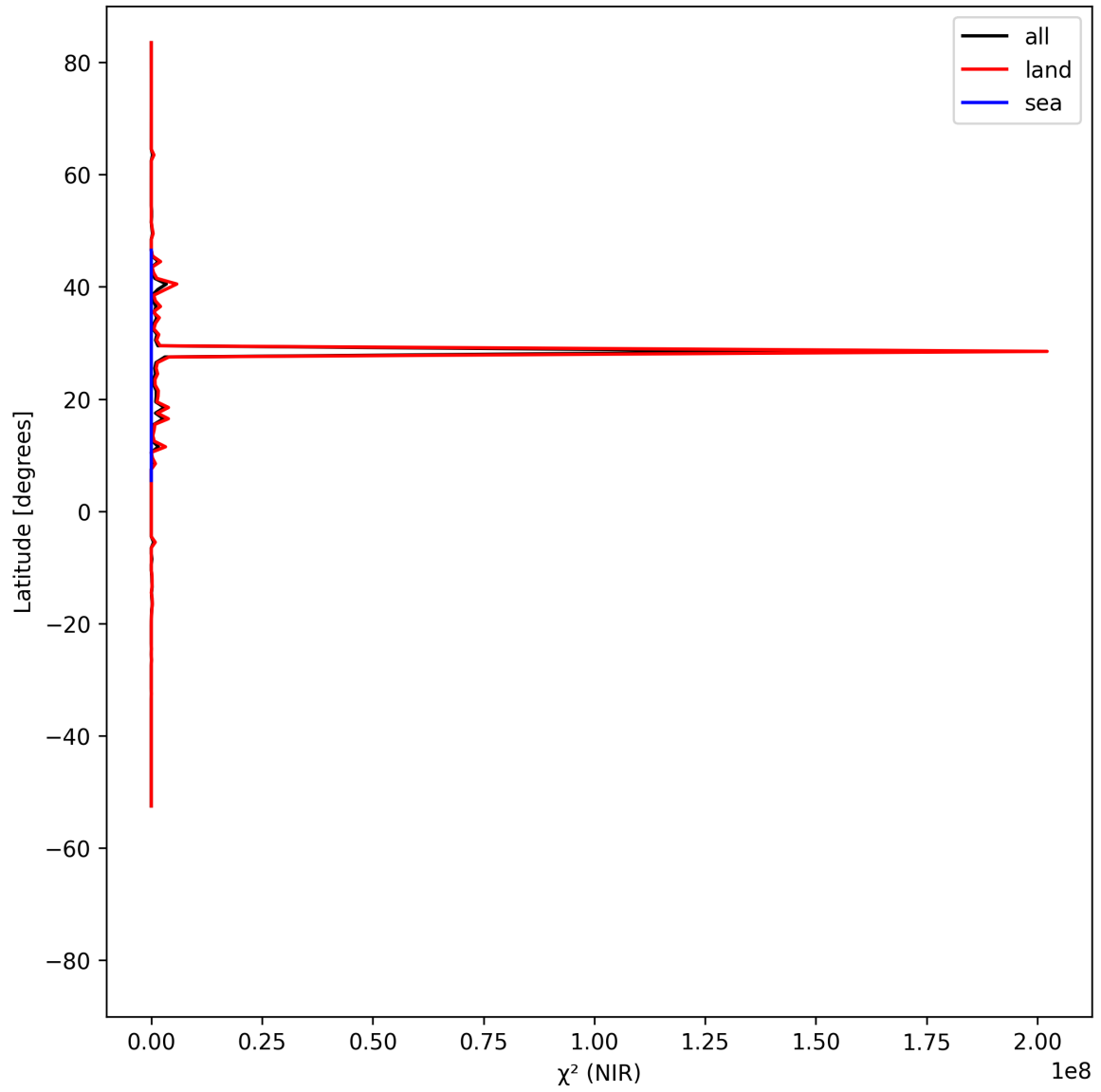
Figure 18: Zonal average of “ \chi^2 (NIR)” for 2025-05-17 to 2025-05-19.
