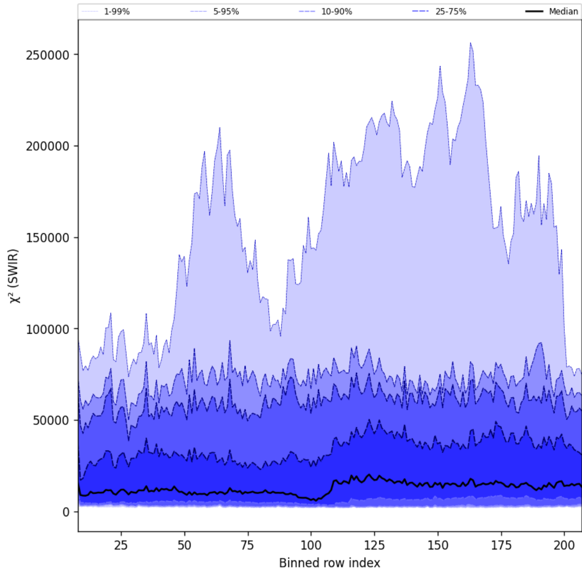
Figure 39: Along track statistics of “ \chi^2 (SWIR)” for 2025-05-17 to 2025-05-19
