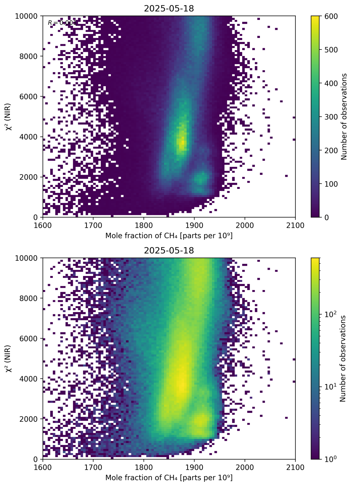
Figure 70: Scatter density plot of “Mole fraction of \text{CH}_4 ” against “ \chi^2 (NIR)” for 2025-05-17 to 2025-05-19.
