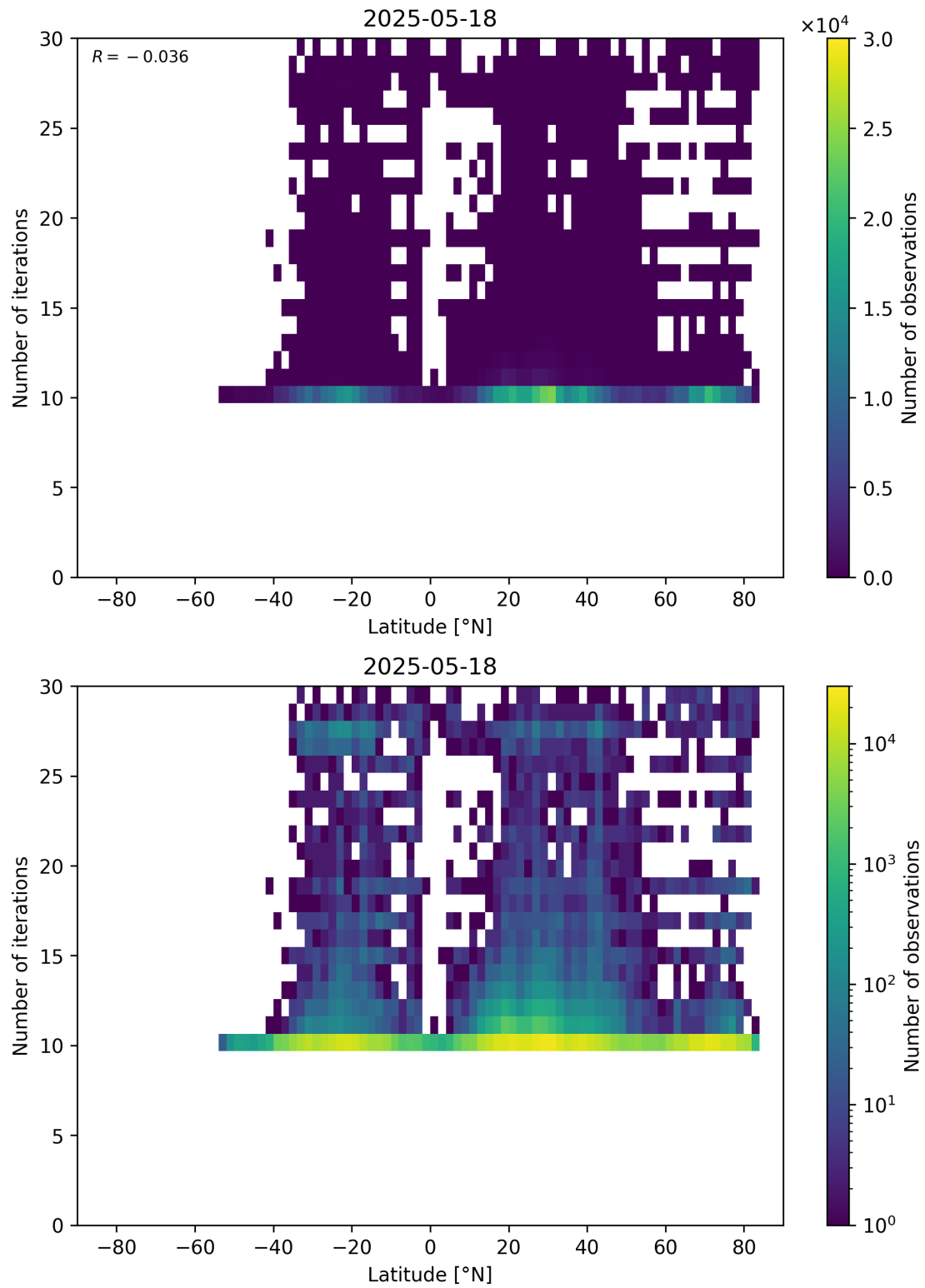
Figure 60: Scatter density plot of “Latitude” against “Number of iterations” for 2025-05-17 to 2025-05-19.
