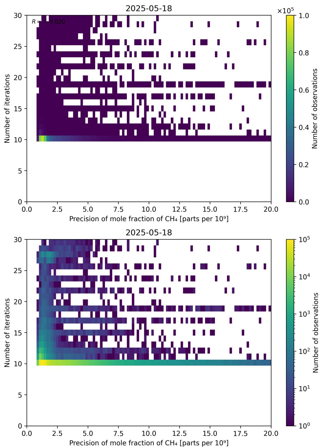
Figure 83: Scatter density plot of “Precision of mole fraction of CH 4 ” against “Number of iterations” for 2025-05-17 to 2025-05-19.
