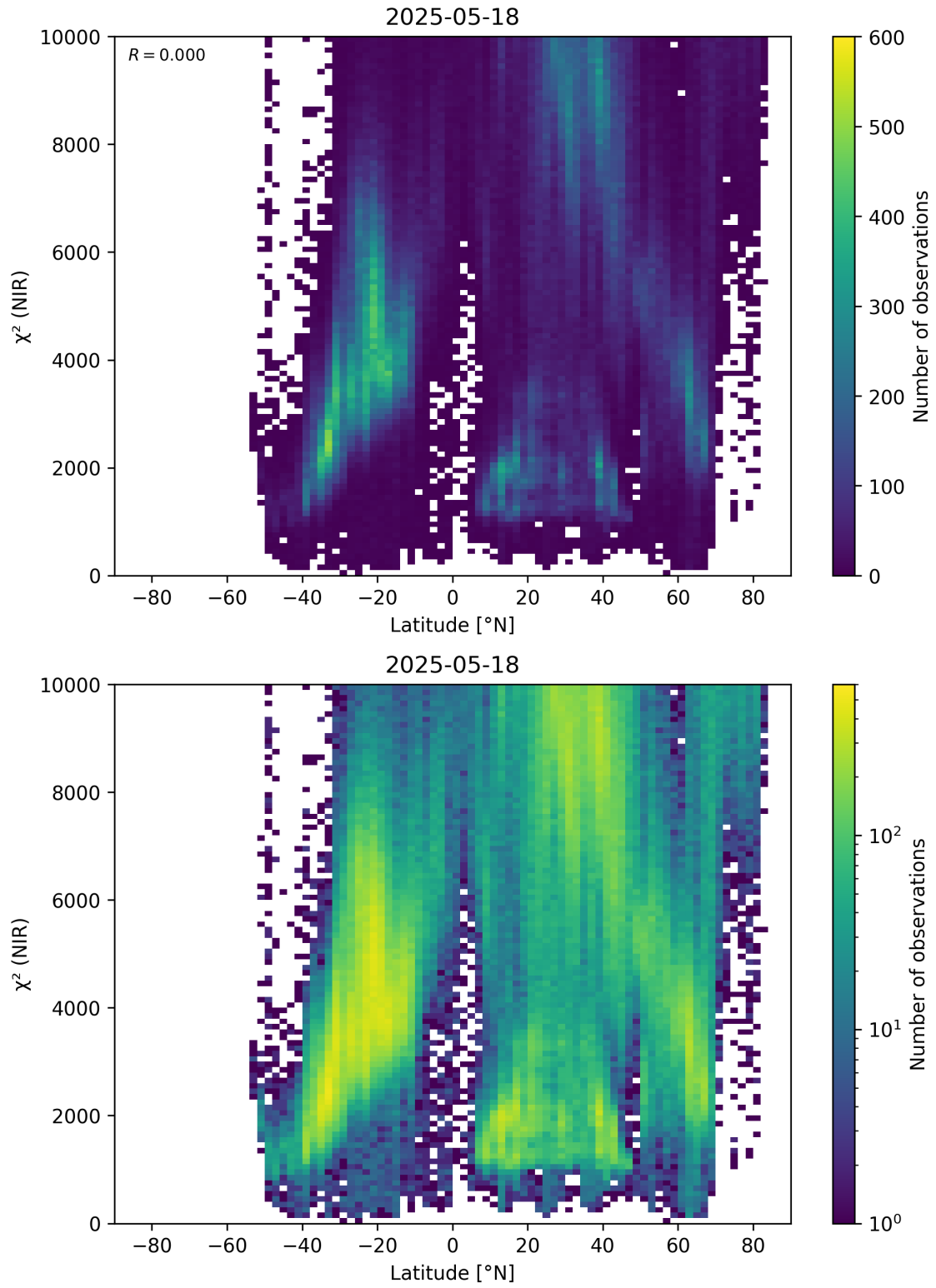
Figure 53: Scatter density plot of “Latitude” against “ \chi^2 (NIR)” for 2025-05-17 to 2025-05-19.
