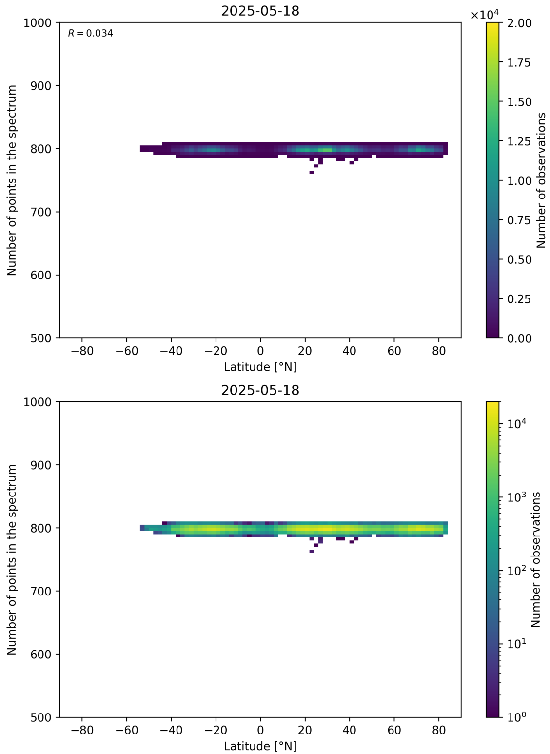
Figure 61: Scatter density plot of “Latitude” against “Number of points in the spectrum” for 2025-05-17 to 2025-05-19.
