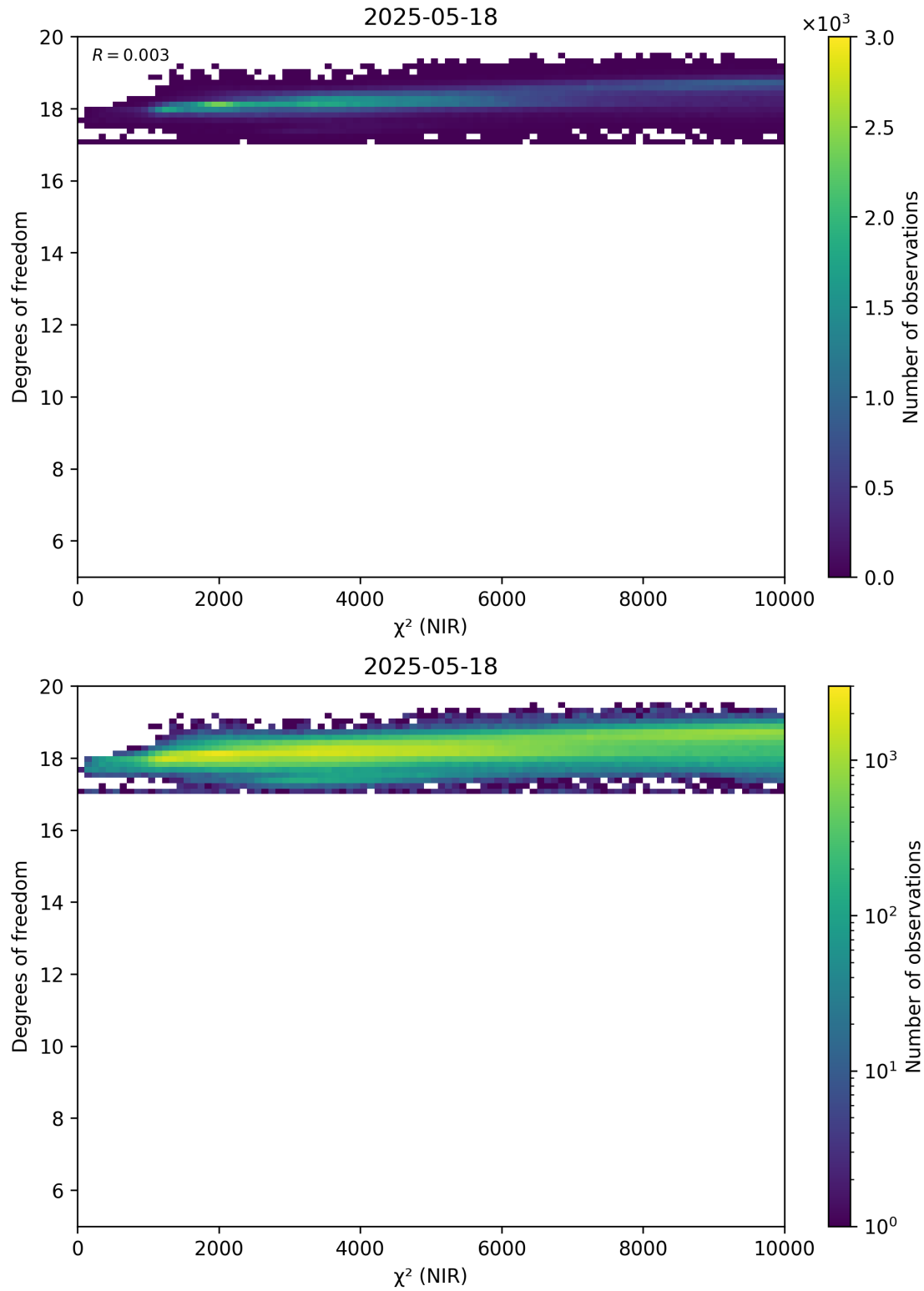
Figure 44: Scatter density plot of “ \chi^2 (NIR)” against “Degrees of freedom” for 2025-05-17 to 2025-05-19.
