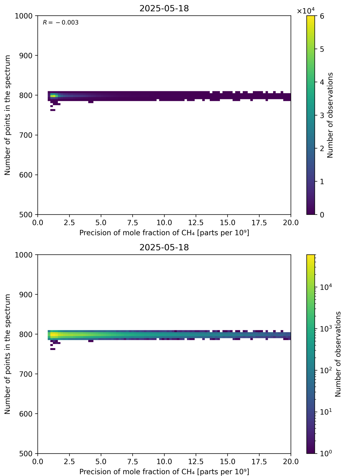
Figure 84: Scatter density plot of “Precision of mole fraction of CH 4 ” against “Number of points in the spectrum” for 2025-05-17 to 2025-05-19.
