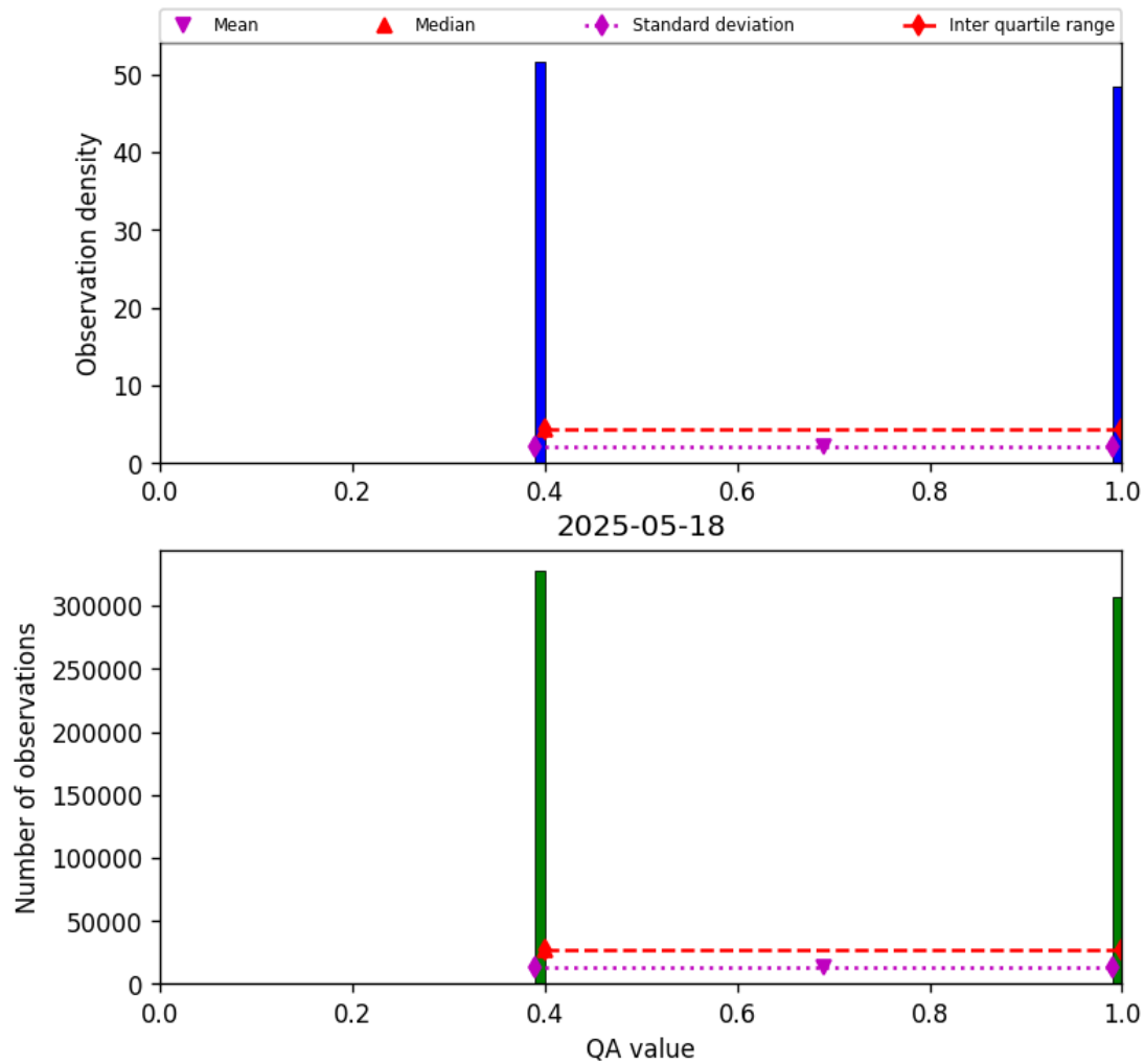
Figure 22: Histogram of “QA value” for 2025-05-17 to 2025-05-19
