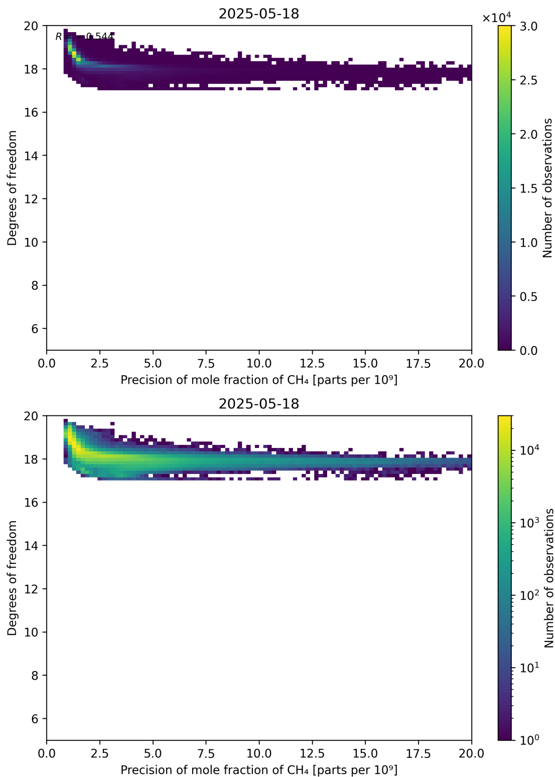
Figure 80: Scatter density plot of “Precision of mole fraction of CH 4 ” against “Degrees of freedom” for 2025-05-17 to 2025-05-19.
