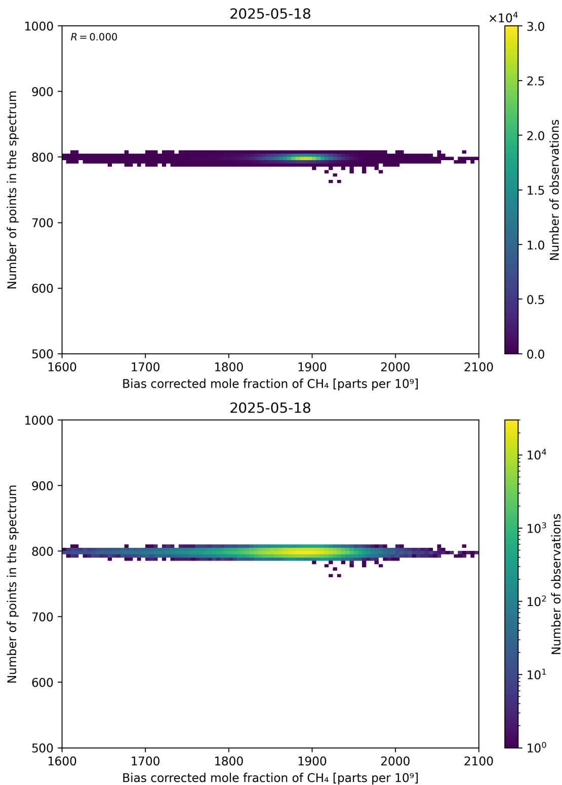
Figure 68: Scatter density plot of “Bias corrected mole fraction of \text{CH}_4 ” against “Number of points in the spectrum” for 2025-05-17 to 2025-05-19.
