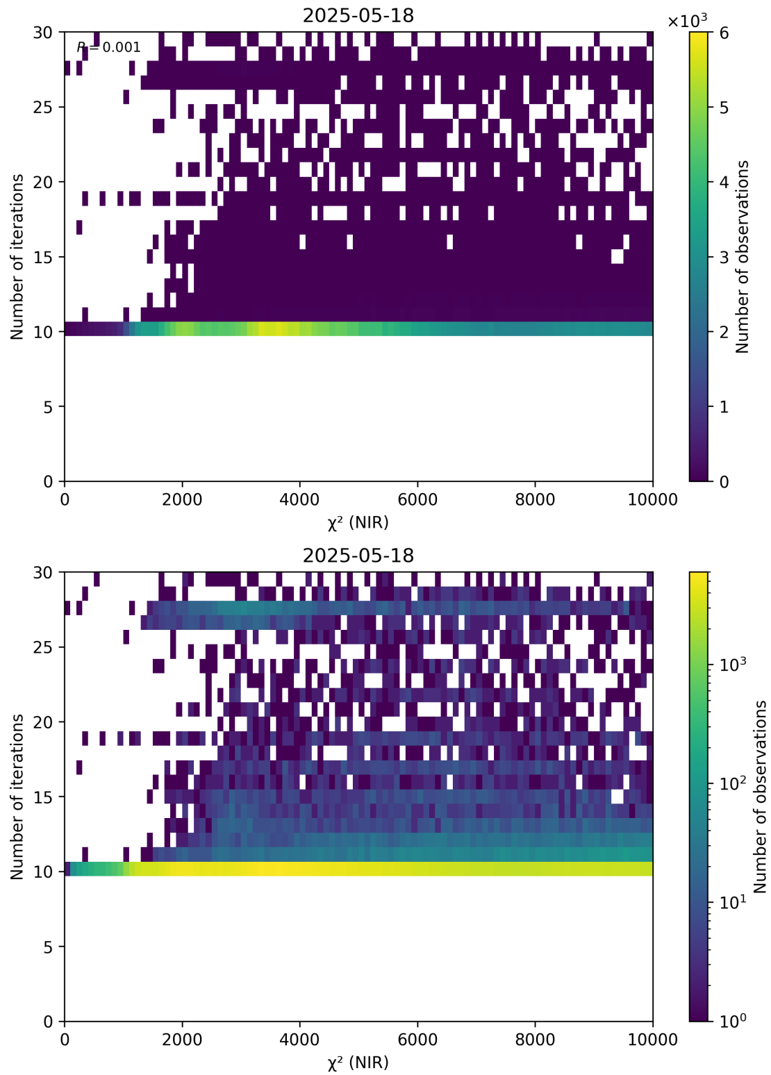
Figure 46: Scatter density plot of “ \chi^2 (NIR)” against “Number of iterations” for 2025-05-17 to 2025-05-19.
