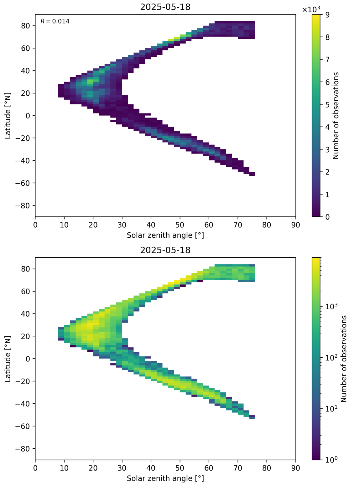
Figure 98: Scatter density plot of “Solar zenith angle” against “Latitude” for 2025-05-17 to 2025-05-19.
