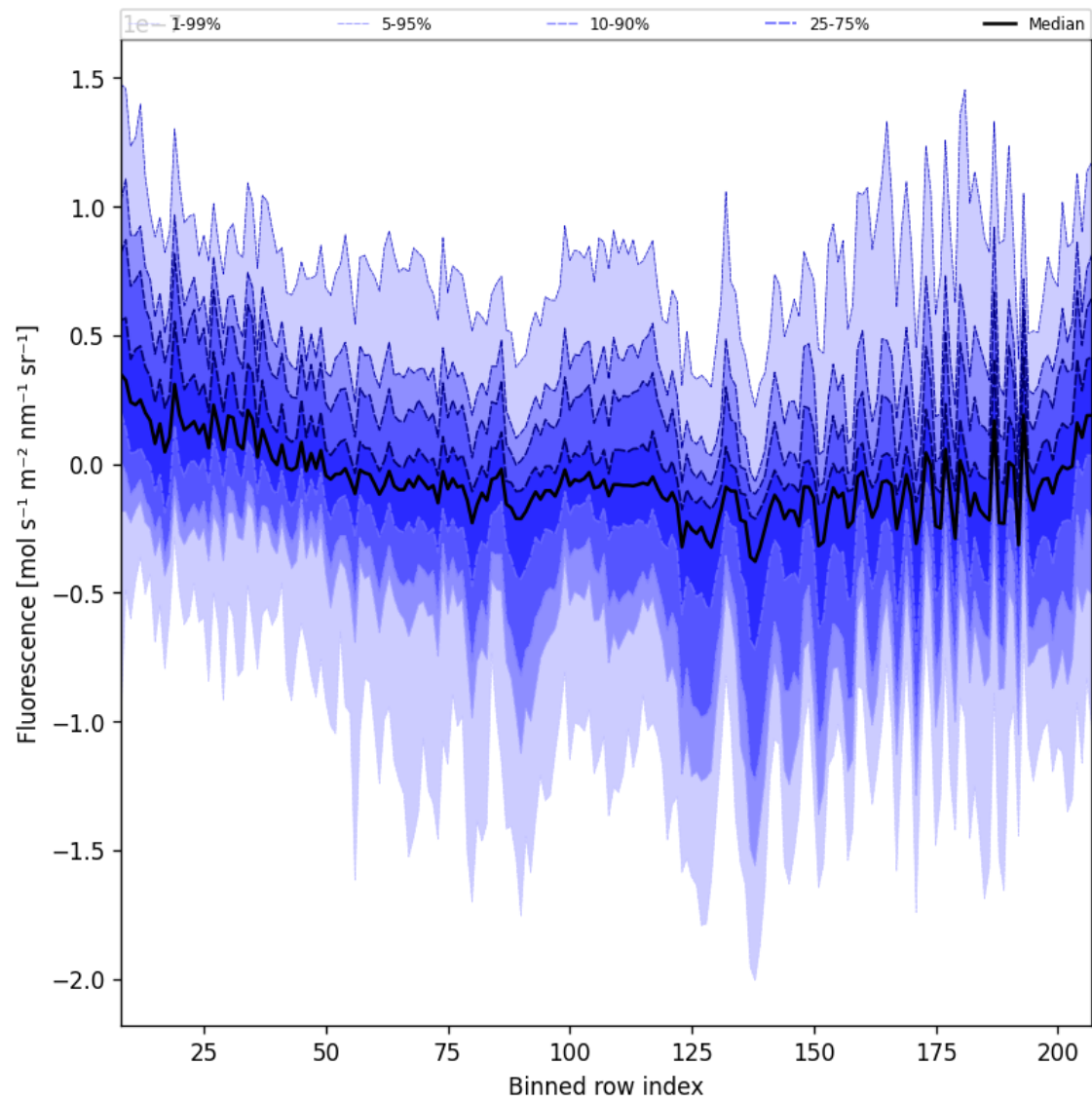
Figure 43: Along track statistics of “Fluorescence” for 2025-05-17 to 2025-05-19
