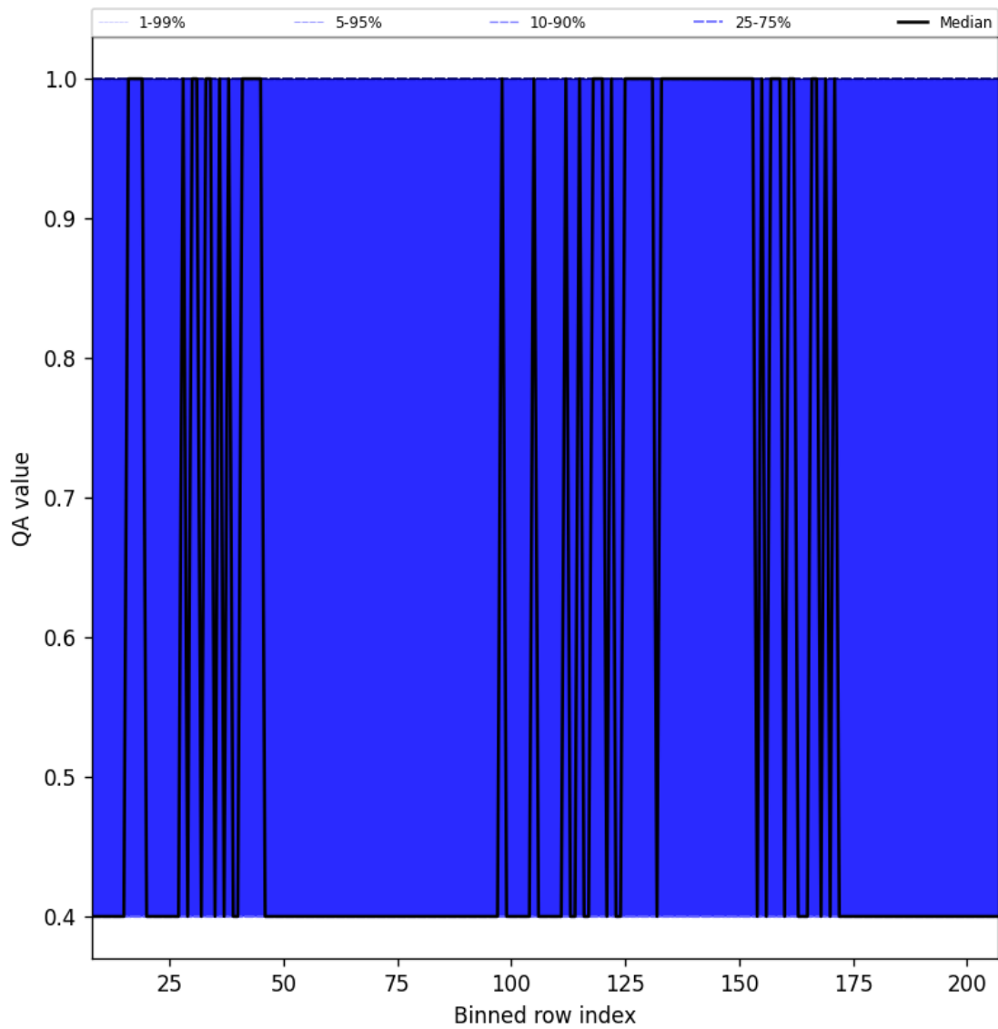
Figure 33: Along track statistics of “QA value” for 2025-05-17 to 2025-05-19
