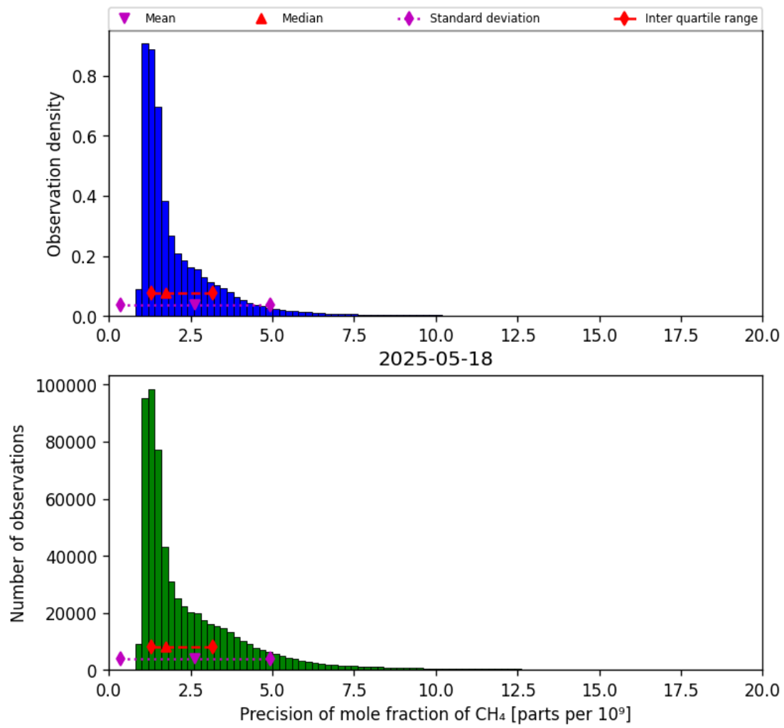
Figure 24: Histogram of “Precision of mole fraction of CH 4 ” for 2025-05-17 to 2025-05-19
