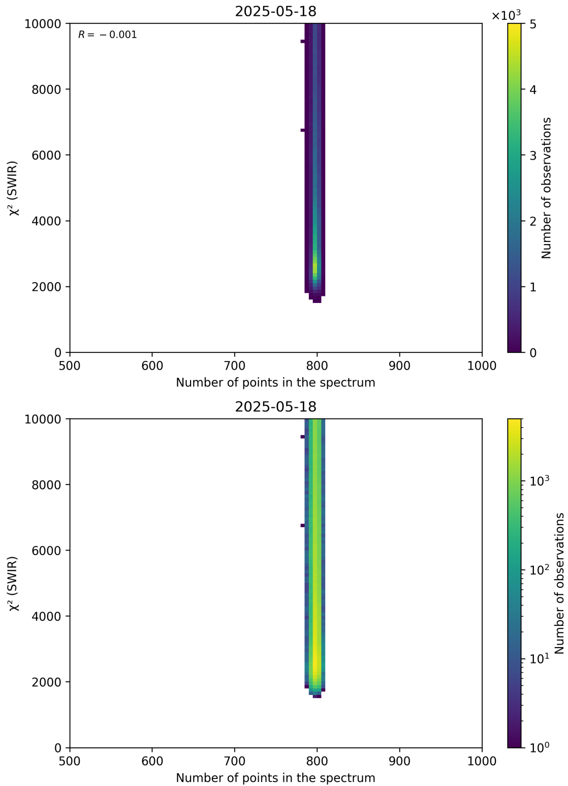
Figure 89: Scatter density plot of “Number of points in the spectrum” against “ \chi^2 (SWIR)” for 2025-05-17 to 2025-05-19.
