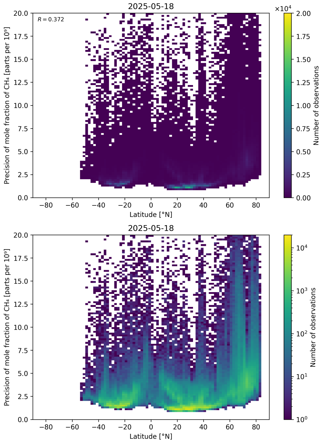
Figure 59: Scatter density plot of “Latitude” against “Precision of mole fraction of \text{CH}_4 ” for 2025-05-17 to 2025-05-19.
