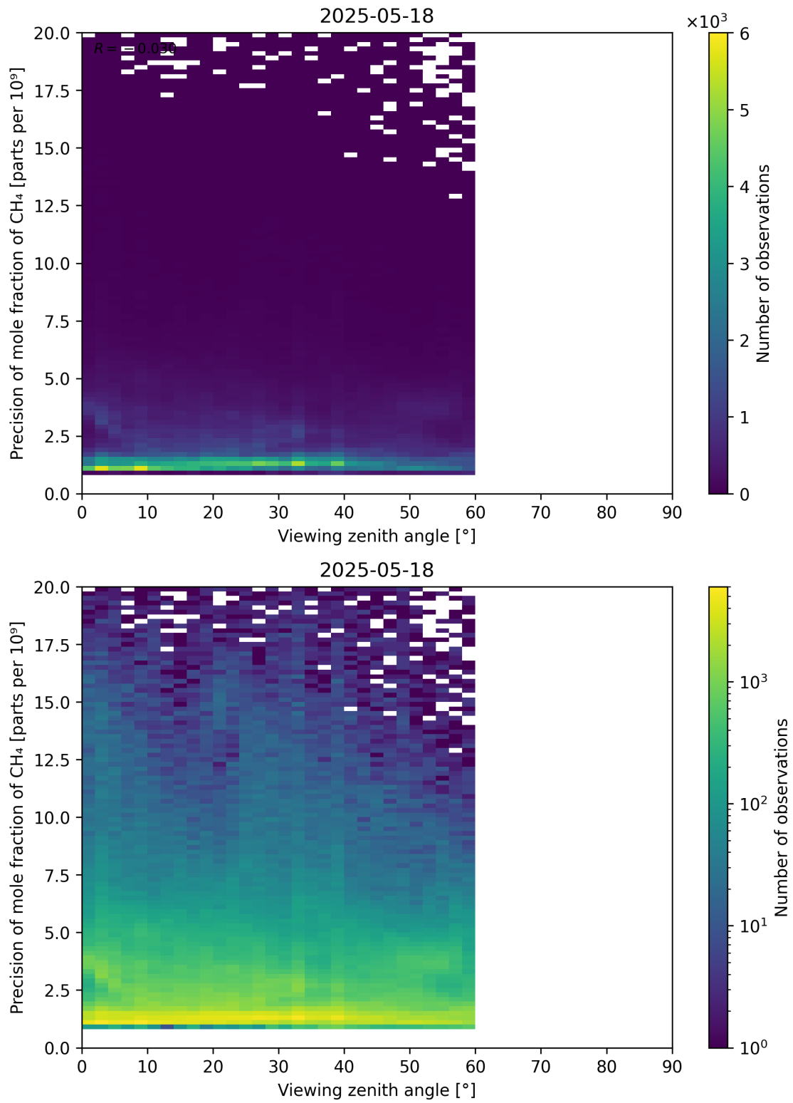
Figure 112: Scatter density plot of “Viewing zenith angle” against “Precision of mole fraction of CH 4 ” for 2025-05-17 to 2025-05-19.
