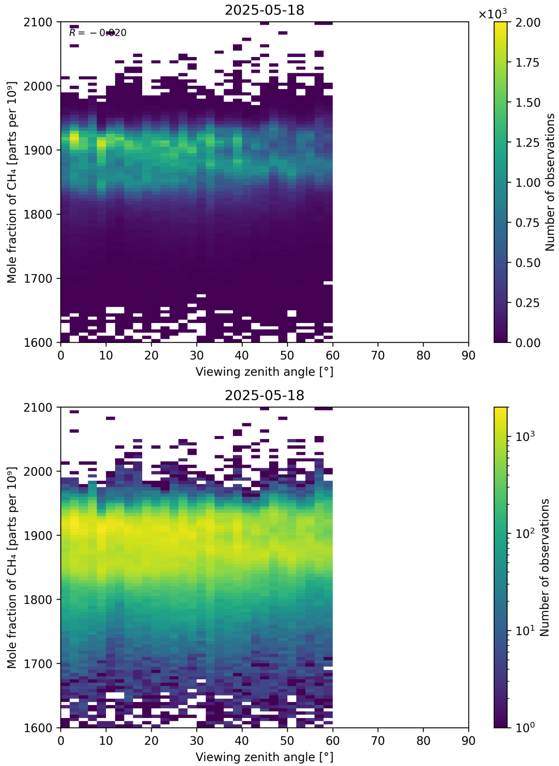
Figure 110: Scatter density plot of “Viewing zenith angle” against “Mole fraction of CH 4 ” for 2025-05-17 to 2025-05-19.
