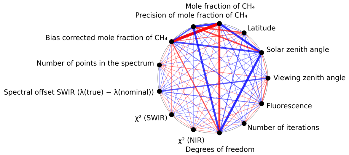
Figure 1: Map of correlation graph for 2025-05-17 to 2025-05-19.
