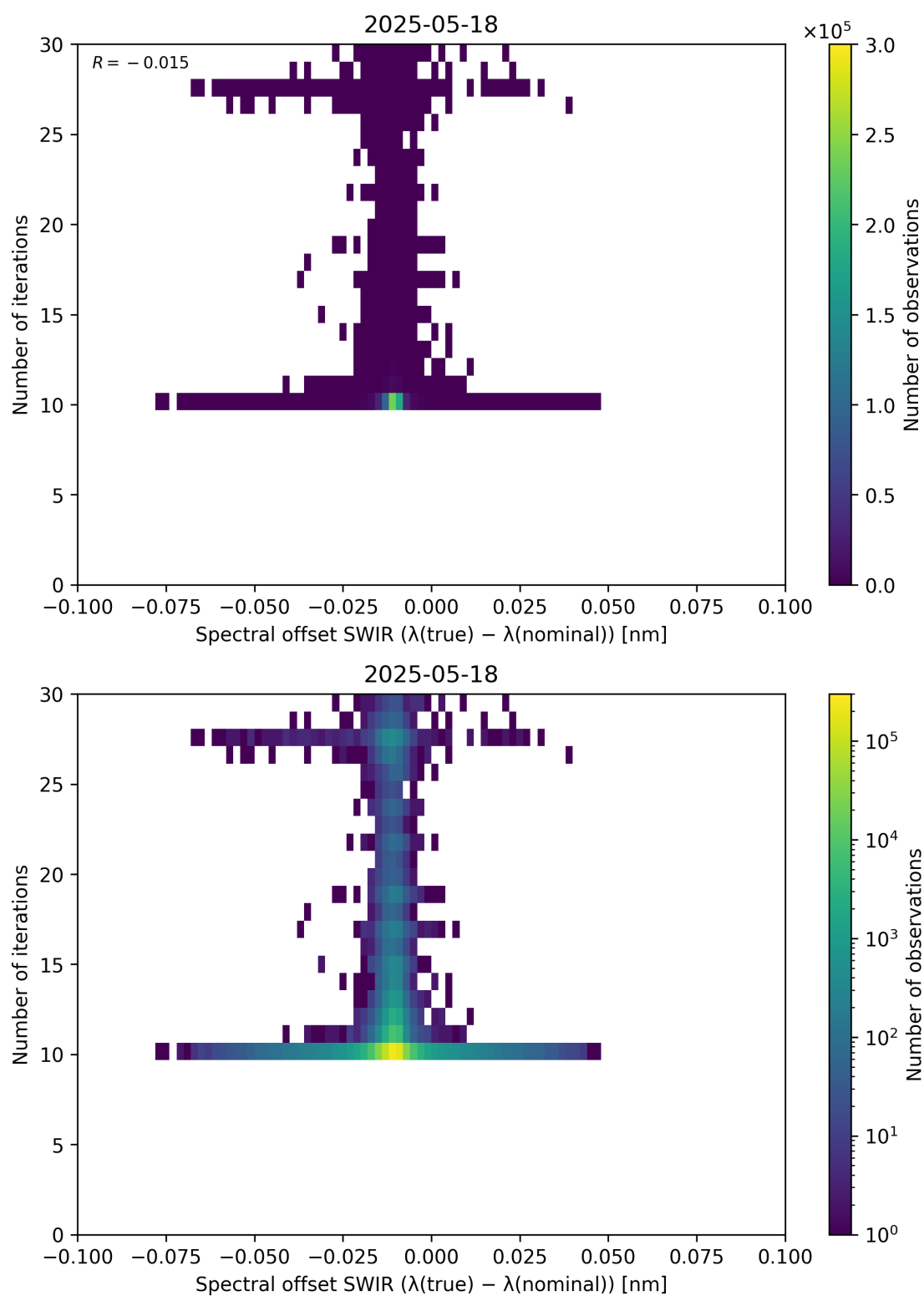
Figure 121: Scatter density plot of “Spectral offset SWIR ( \lambda_{\text{true}} - \lambda_{\text{nominal}} )” against “Number of iterations” for 2025-05-17 to 2025-05-19.
