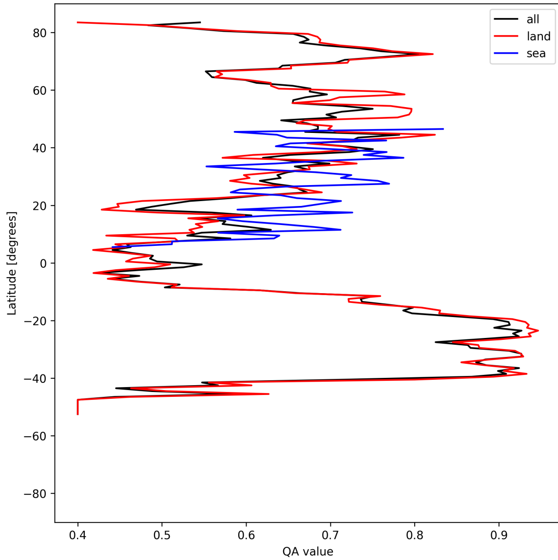
Figure 11: Zonal average of “QA value” for 2025-05-17 to 2025-05-19.
