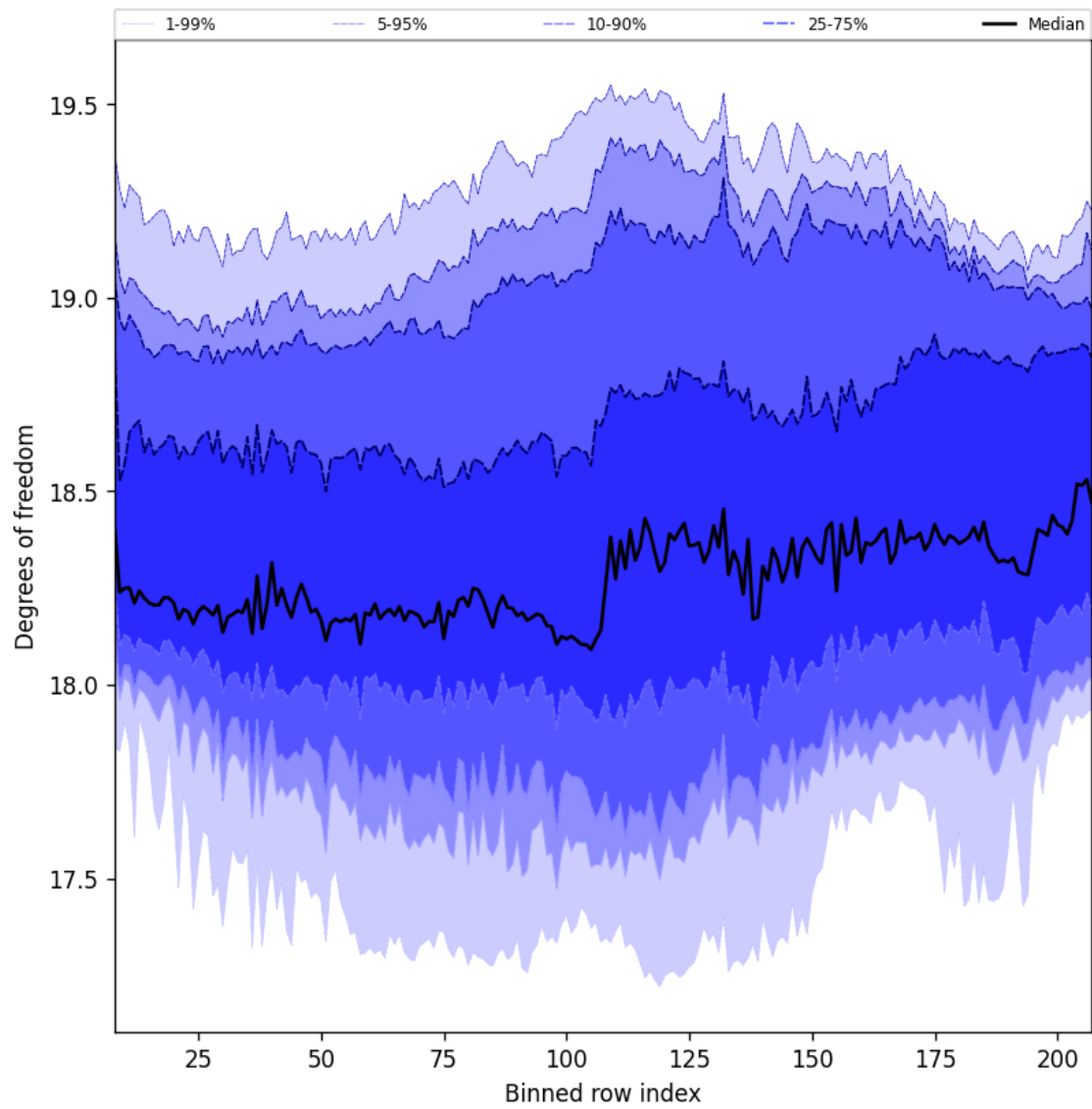
Figure 41: Along track statistics of “Degrees of freedom” for 2025-05-17 to 2025-05-19
