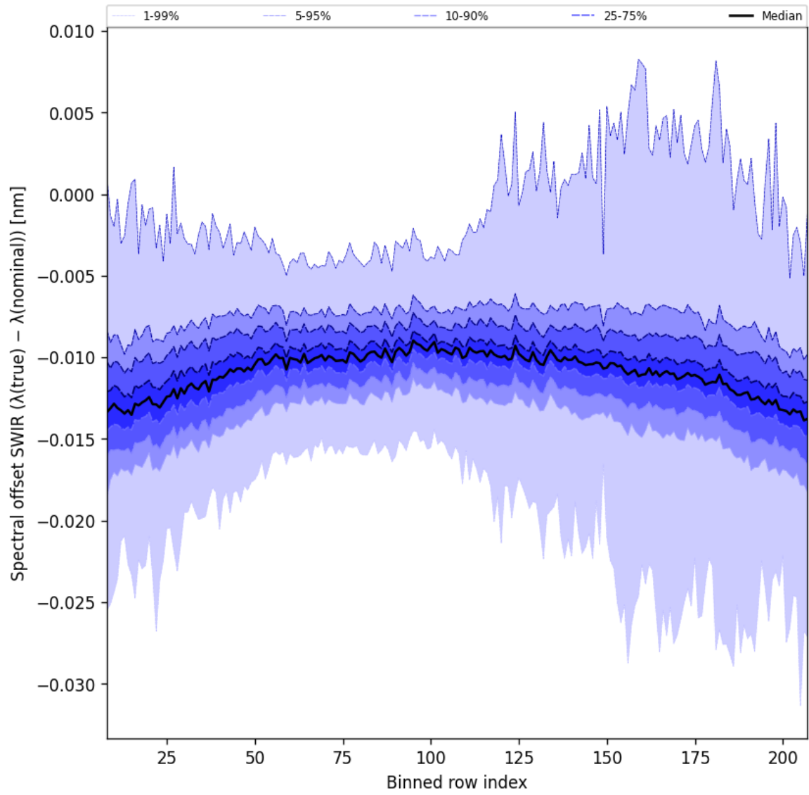
Figure 38: Along track statistics of “Spectral offset SWIR ( \lambda_{\text{true}} - \lambda_{\text{nominal}} )” for 2025-05-17 to 2025-05-19
