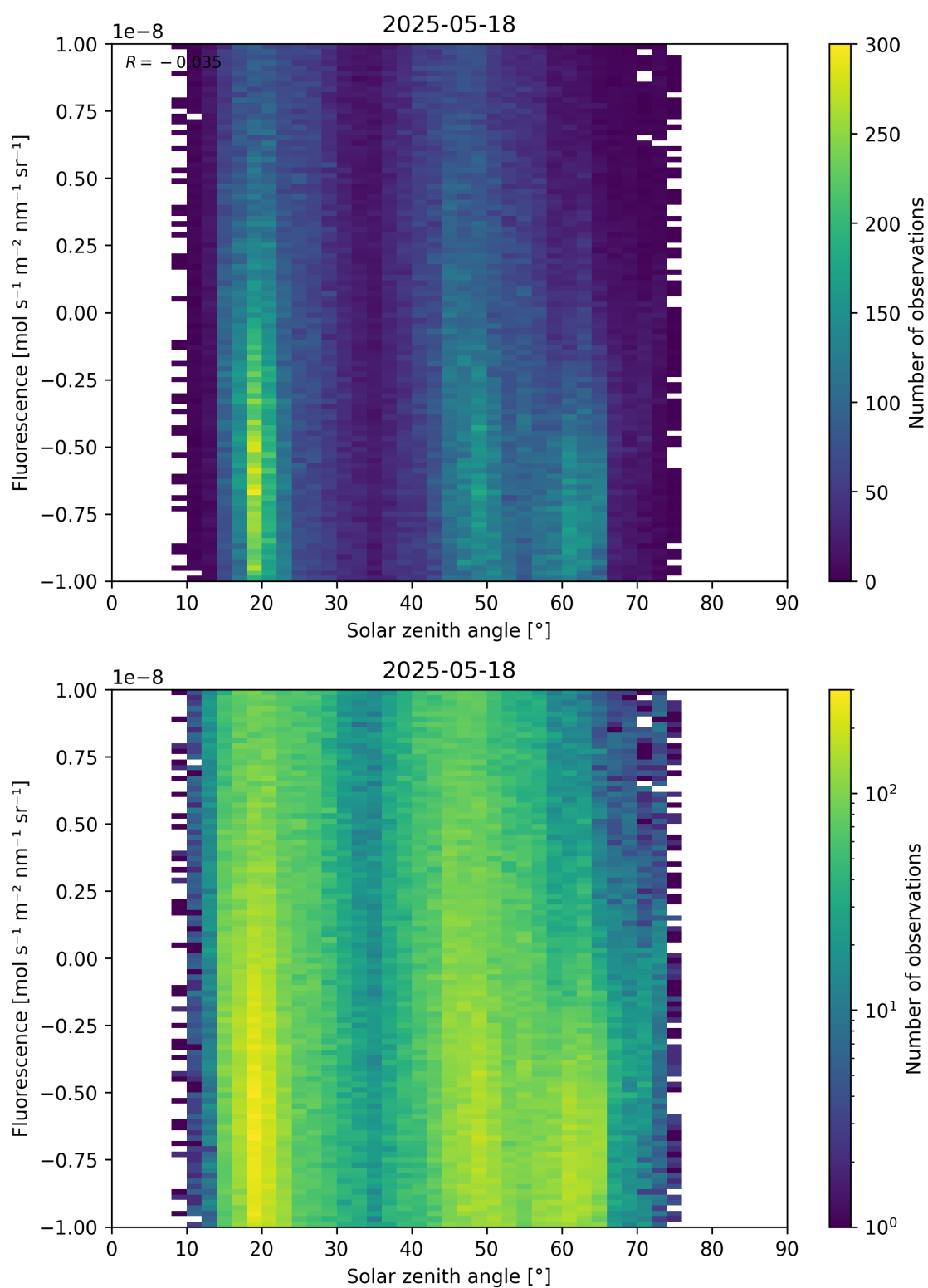
Figure 97: Scatter density plot of “Solar zenith angle” against “Fluorescence” for 2025-05-17 to 2025-05-19.
