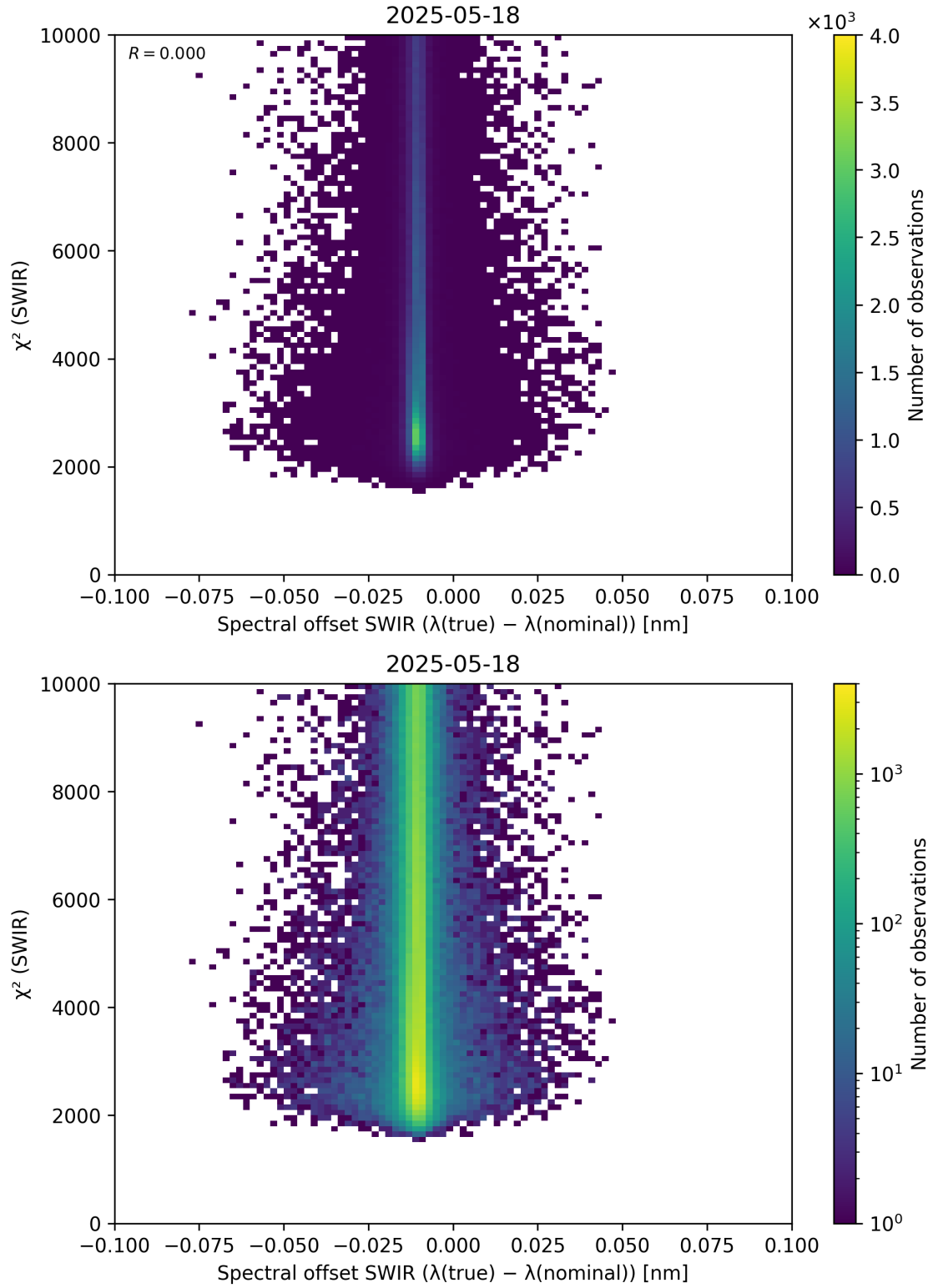
Figure 118: Scatter density plot of “Spectral offset SWIR ( \lambda_{\text{true}} - \lambda_{\text{nominal}} )” against “ \chi^2 (SWIR)” for 2025-05-17 to 2025-05-19.
