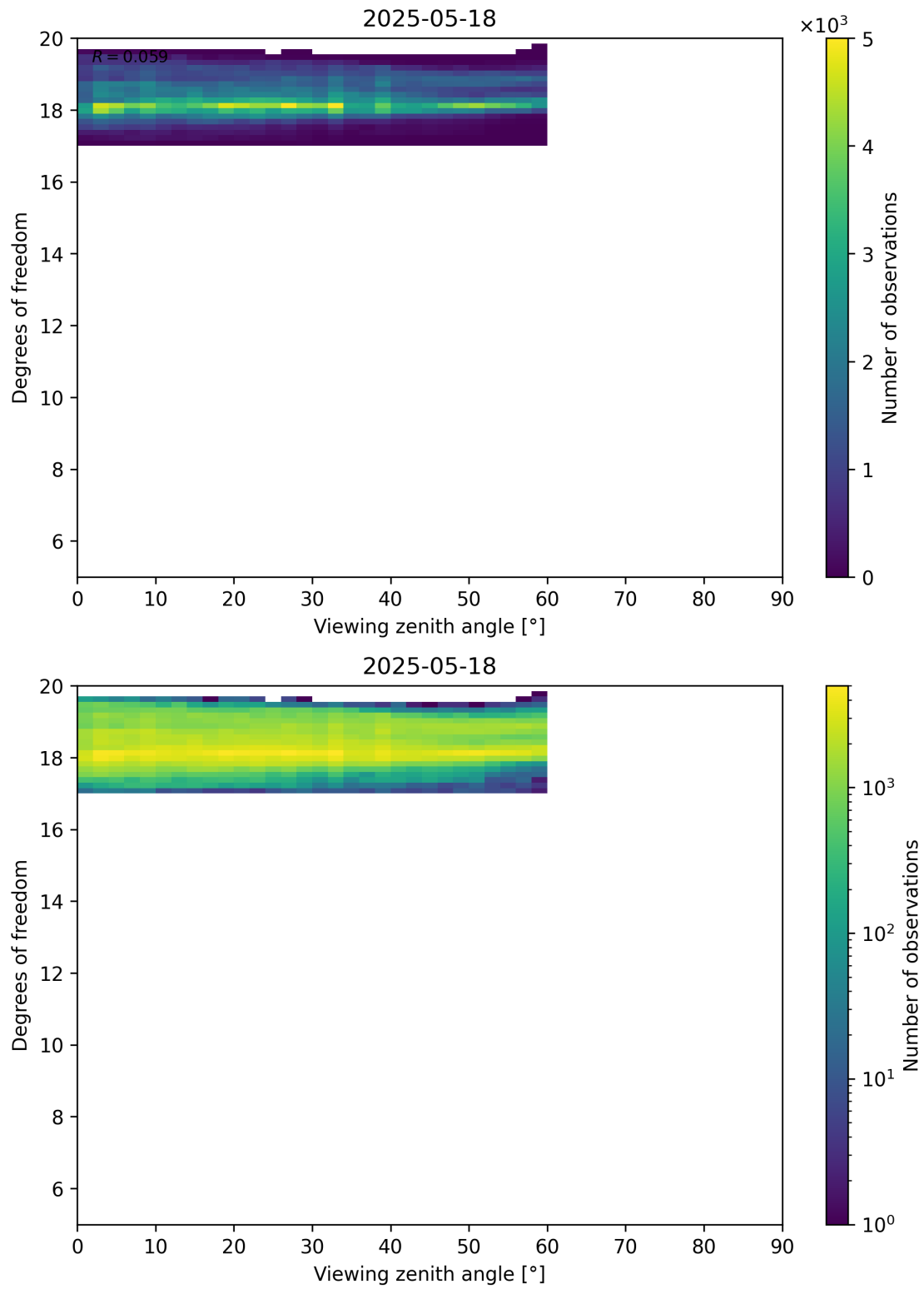
Figure 107: Scatter density plot of “Viewing zenith angle” against “Degrees of freedom” for 2025-05-17 to 2025-05-19.
