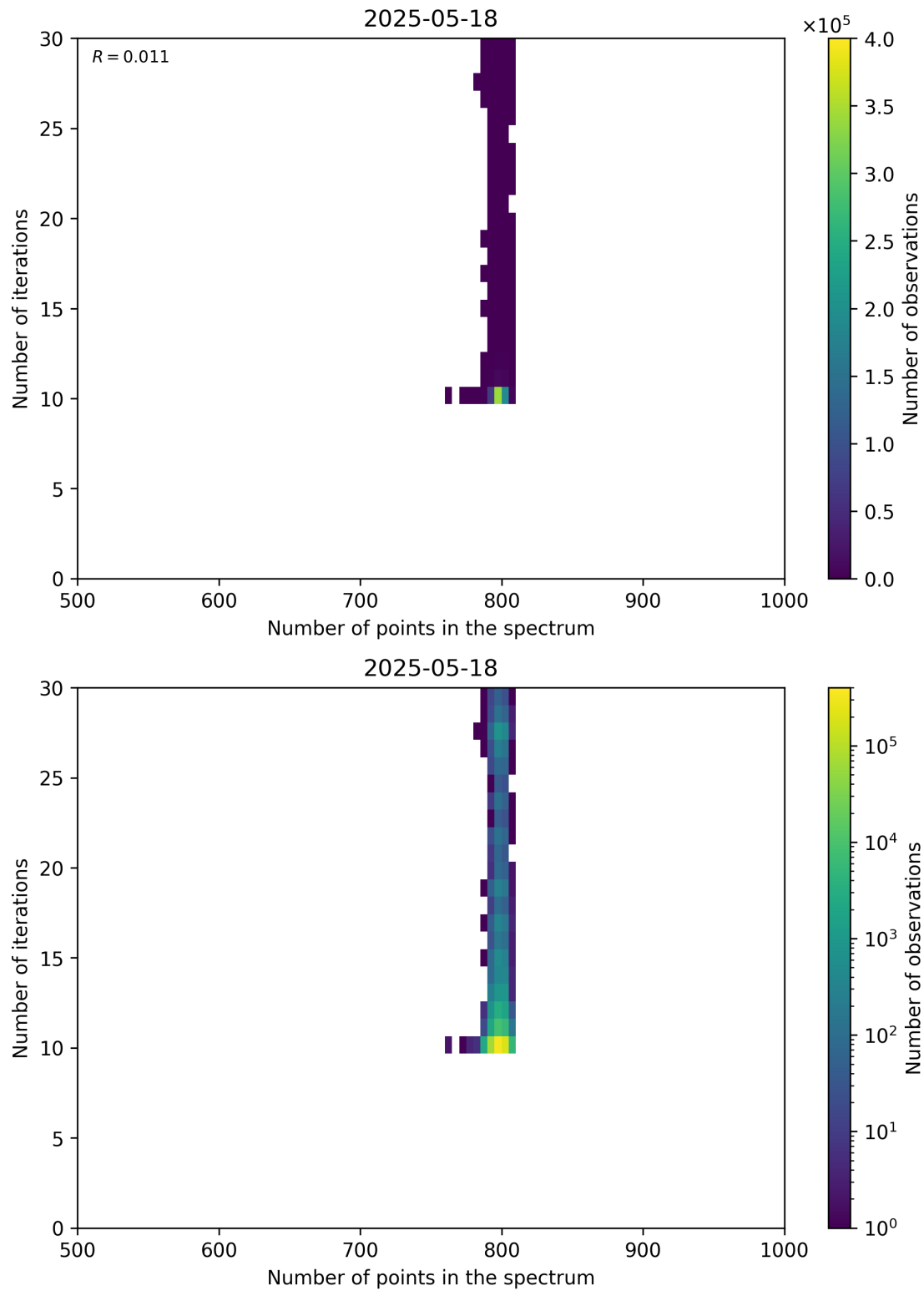
Figure 92: Scatter density plot of “Number of points in the spectrum” against “Number of iterations” for 2025-05-17 to 2025-05-19.
