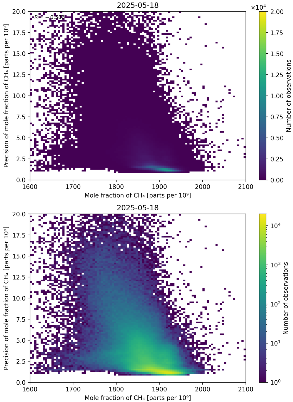
Figure 75: Scatter density plot of “Mole fraction of CH 4 ” against “Precision of mole fraction of CH 4 ” for 2025-05-17 to 2025-05-19.
