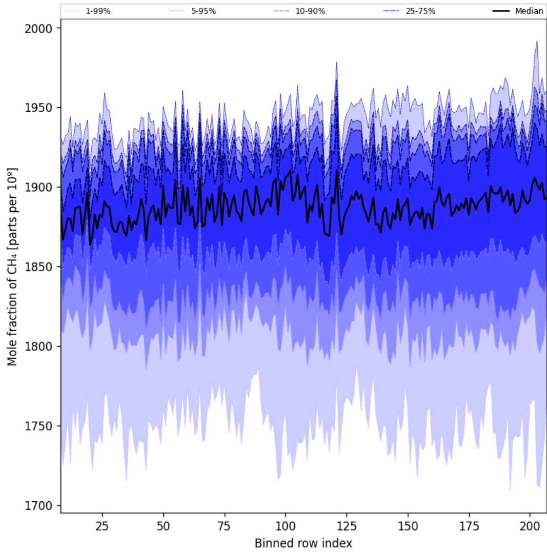
Figure 34: Along track statistics of “Mole fraction of CH 4 ” for 2025-05-17 to 2025-05-19
