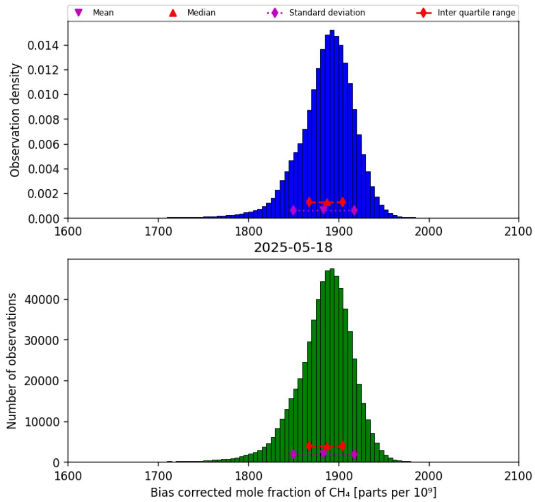
Figure 25: Histogram of “Bias corrected mole fraction of CH 4 ” for 2025-05-17 to 2025-05-19
