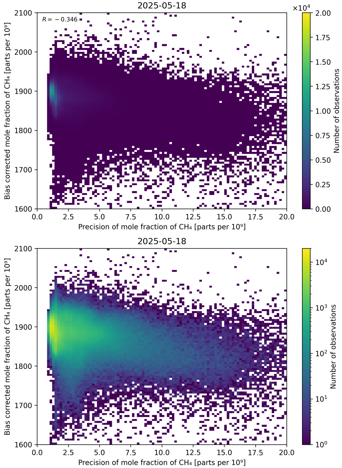
Figure 82: Scatter density plot of “Precision of mole fraction of CH 4 ” against “Bias corrected mole fraction of CH 4 ” for 2025-05-17 to 2025-05-19.
