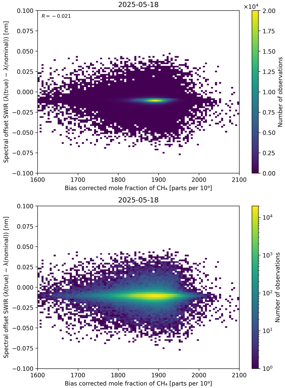
Figure 69: Scatter density plot of “Bias corrected mole fraction of \text{CH}_4 ” against “Spectral offset SWIR ( \lambda_{\text{true}} - \lambda_{\text{nominal}} )” for 2025-05-17 to 2025-05-19.
