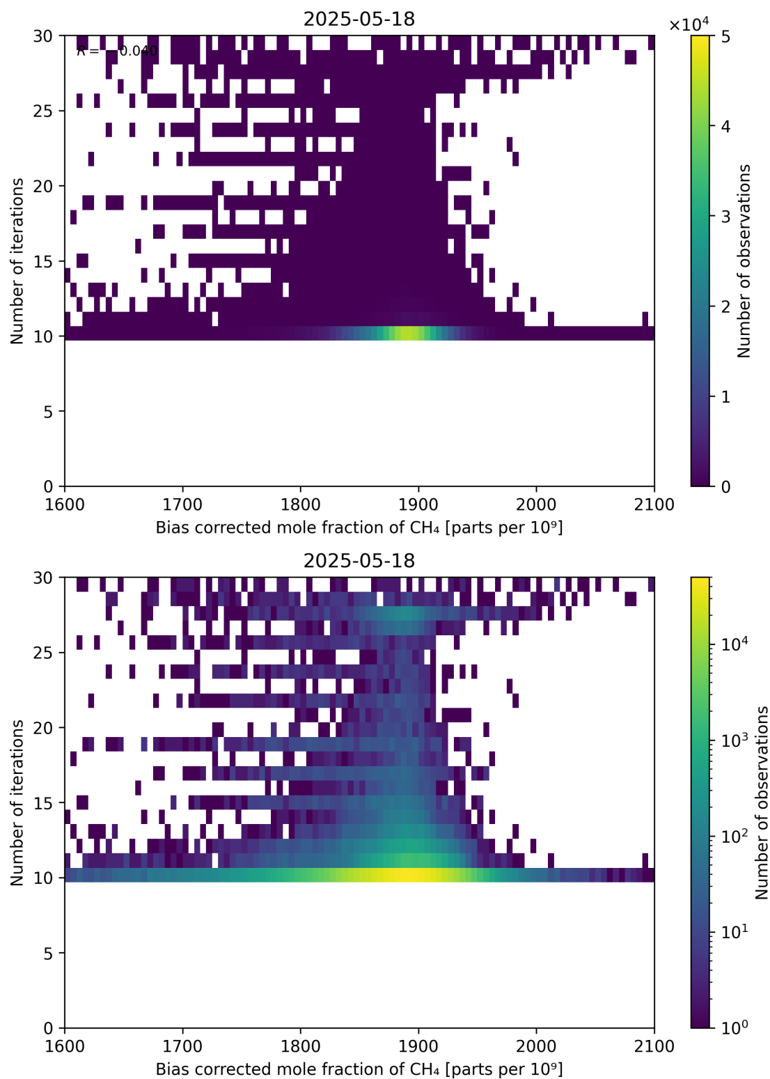
Figure 67: Scatter density plot of “Bias corrected mole fraction of CH 4 ” against “Number of iterations” for 2025-05-17 to 2025-05-19.
