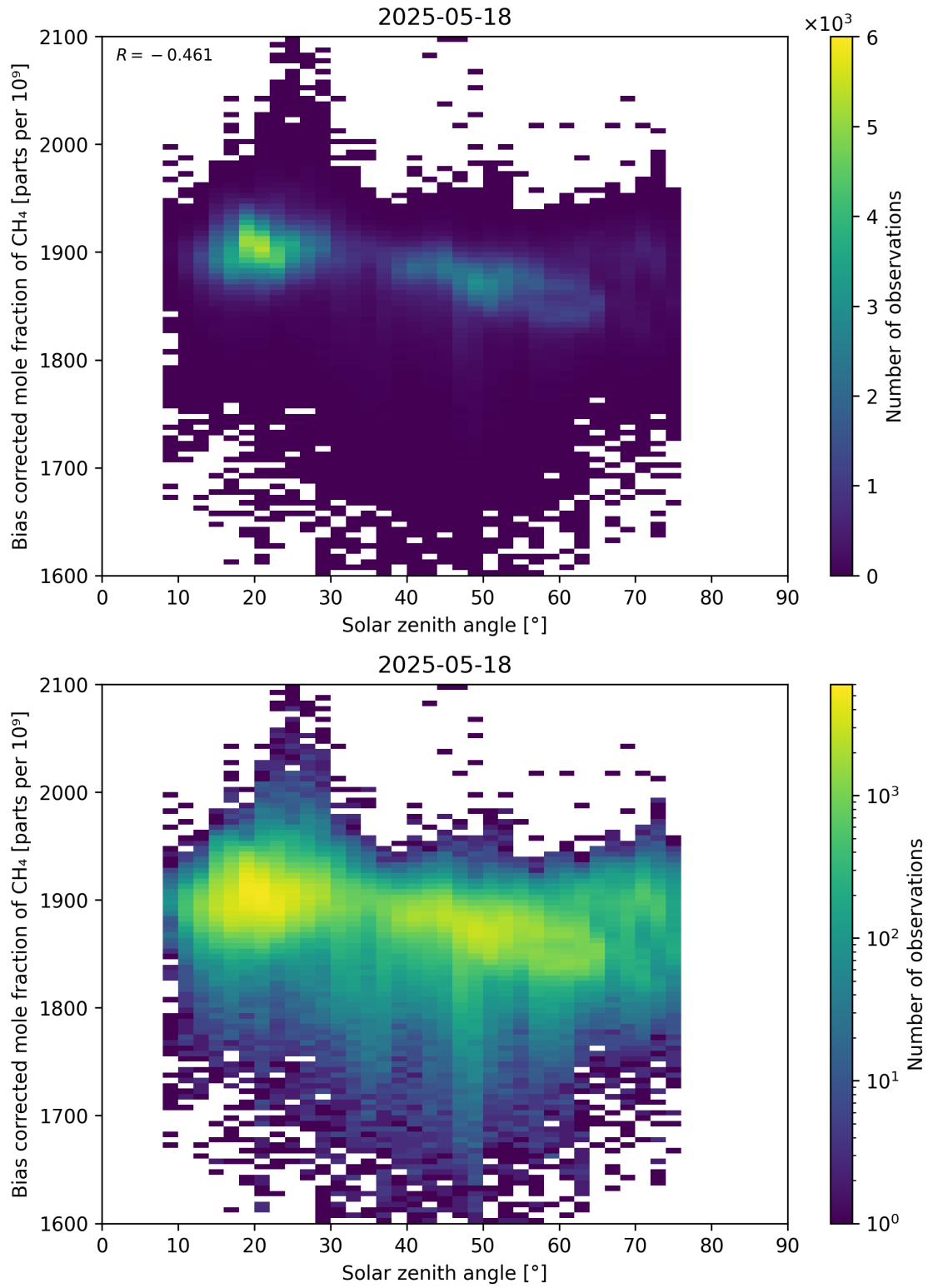
Figure 100: Scatter density plot of “Solar zenith angle” against “Bias corrected mole fraction of CH 4 ” for 2025-05-17 to 2025-05-19.
