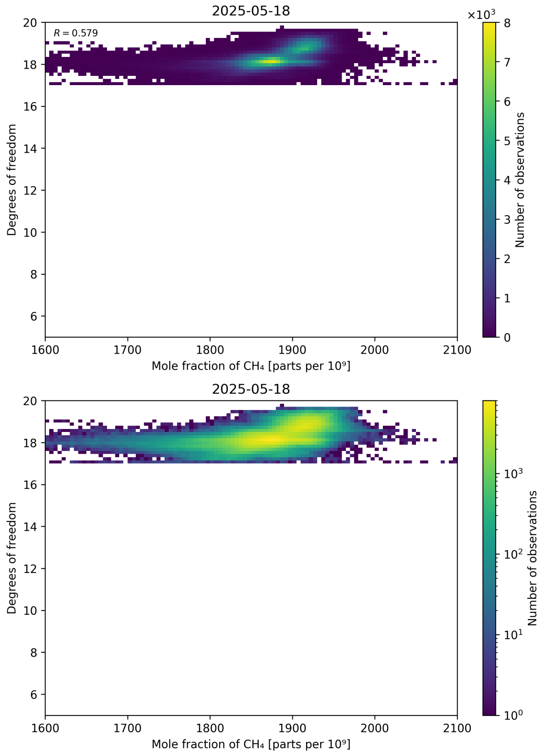
Figure 72: Scatter density plot of “Mole fraction of CH 4 ” against “Degrees of freedom” for 2025-05-17 to 2025-05-19.
