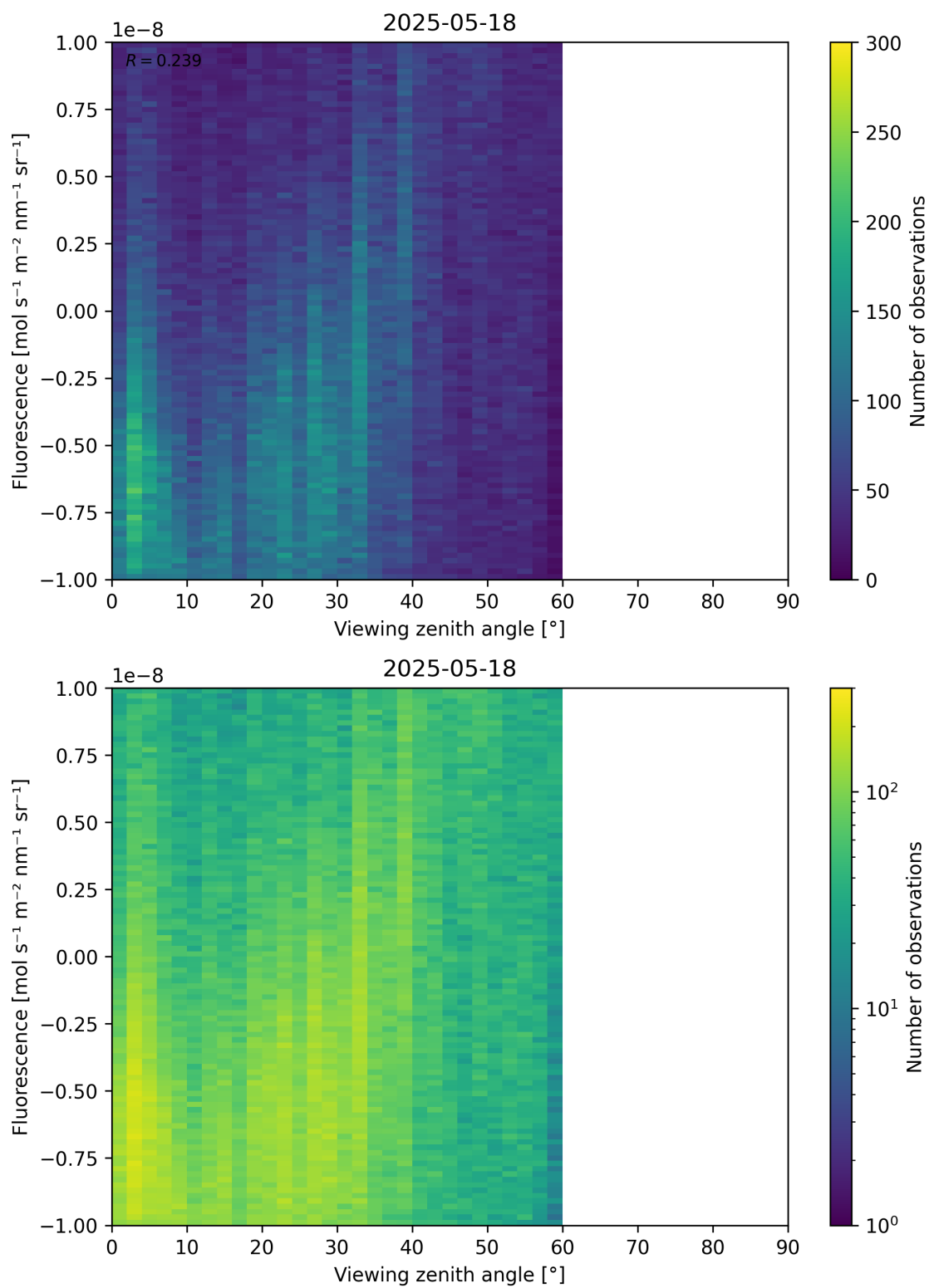
Figure 108: Scatter density plot of “Viewing zenith angle” against “Fluorescence” for 2025-05-17 to 2025-05-19.
