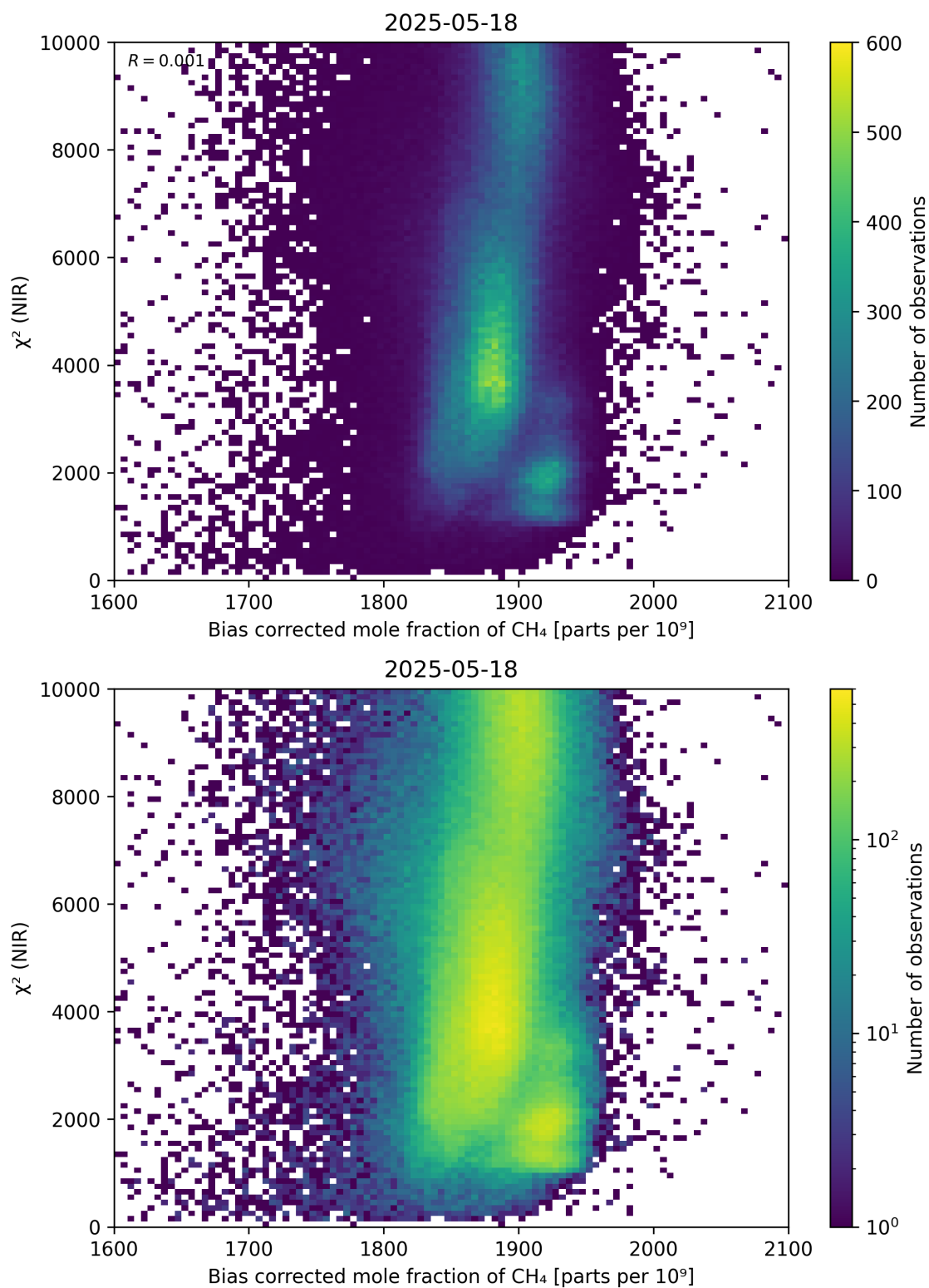
Figure 63: Scatter density plot of “Bias corrected mole fraction of CH 4 ” against “ \chi^2 (NIR)” for 2025-05-17 to 2025-05-19.
