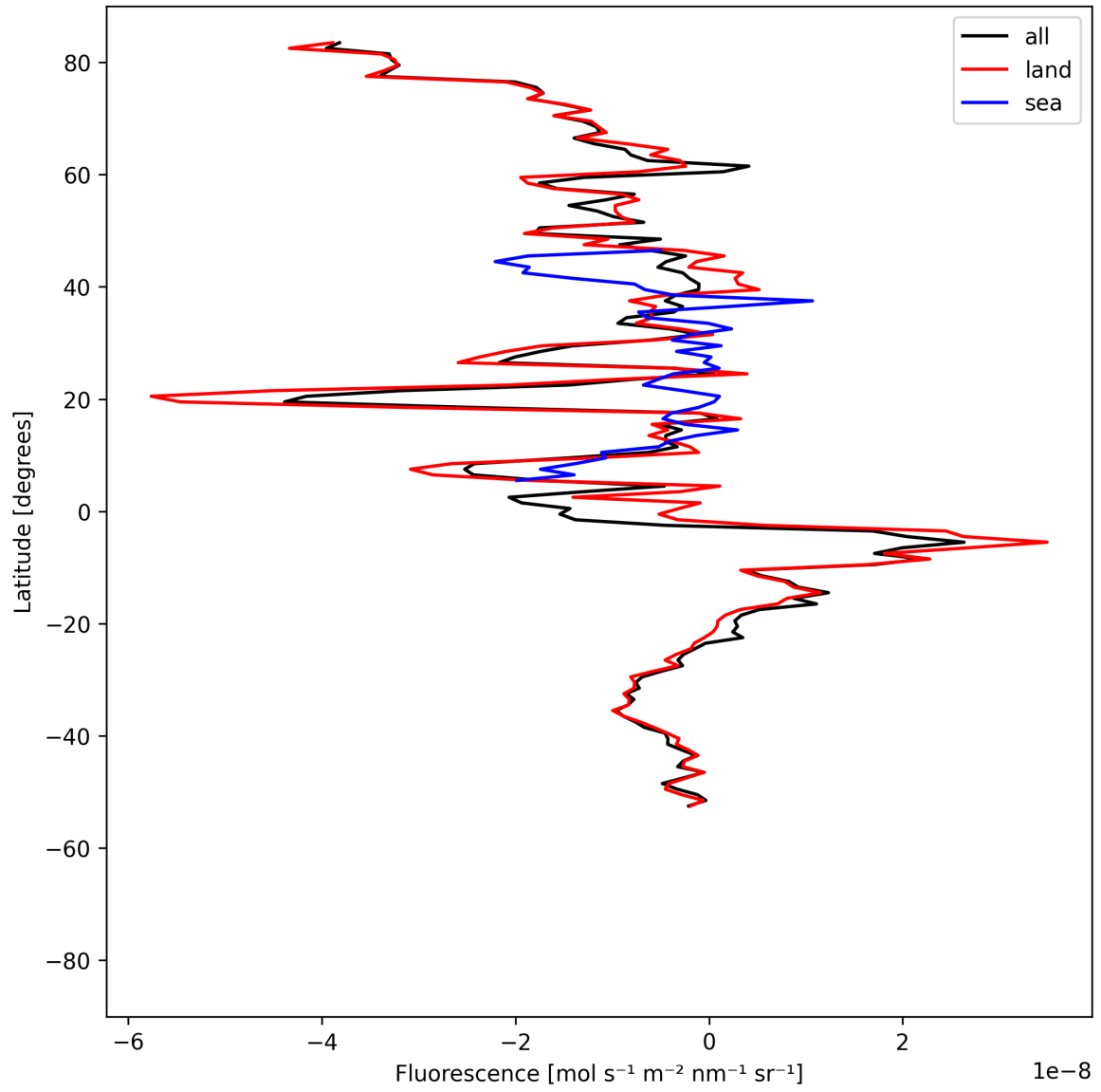
Figure 21: Zonal average of “Fluorescence” for 2025-05-17 to 2025-05-19.
