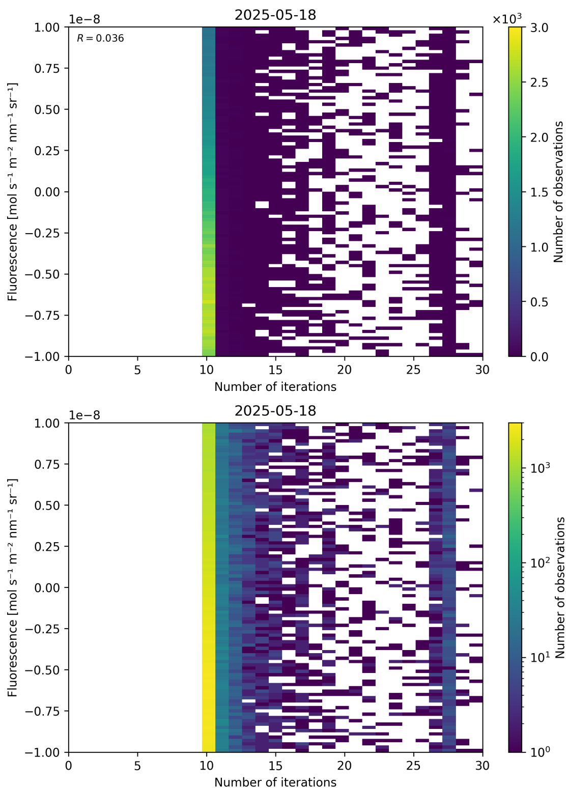
Figure 87: Scatter density plot of “Number of iterations” against “Fluorescence” for 2025-05-17 to 2025-05-19.
