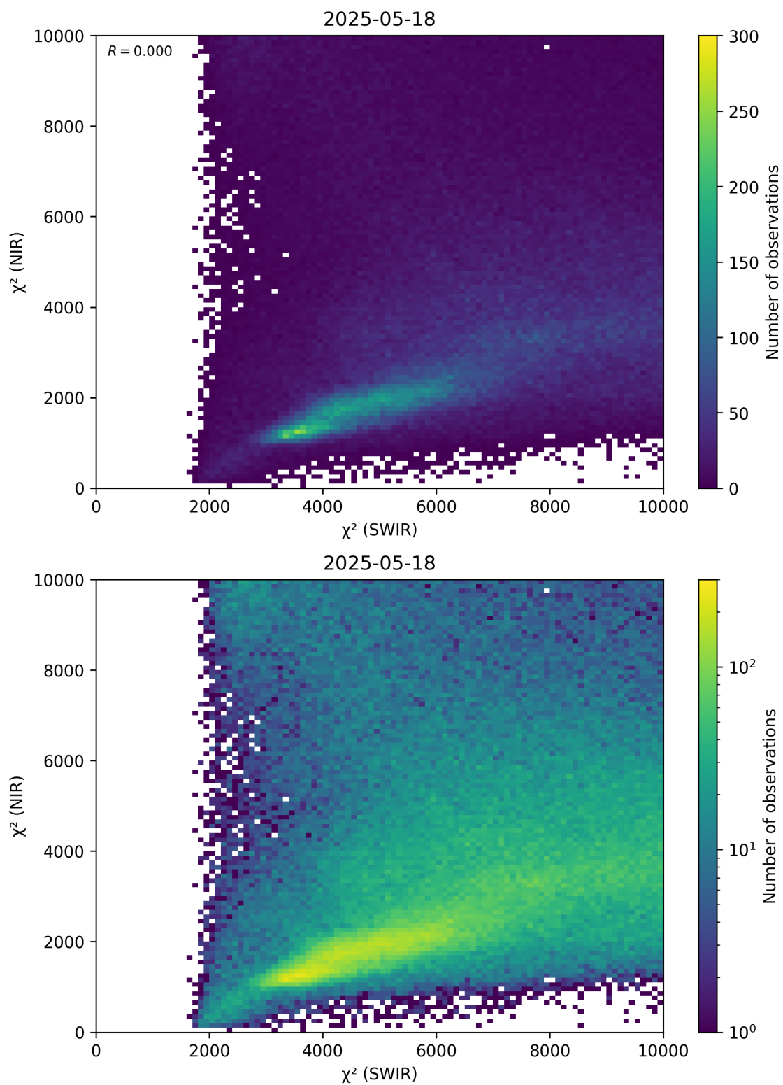
Figure 47: Scatter density plot of “ \chi^2 (SWIR)” against “ \chi^2 (NIR)” for 2025-05-17 to 2025-05-19.
