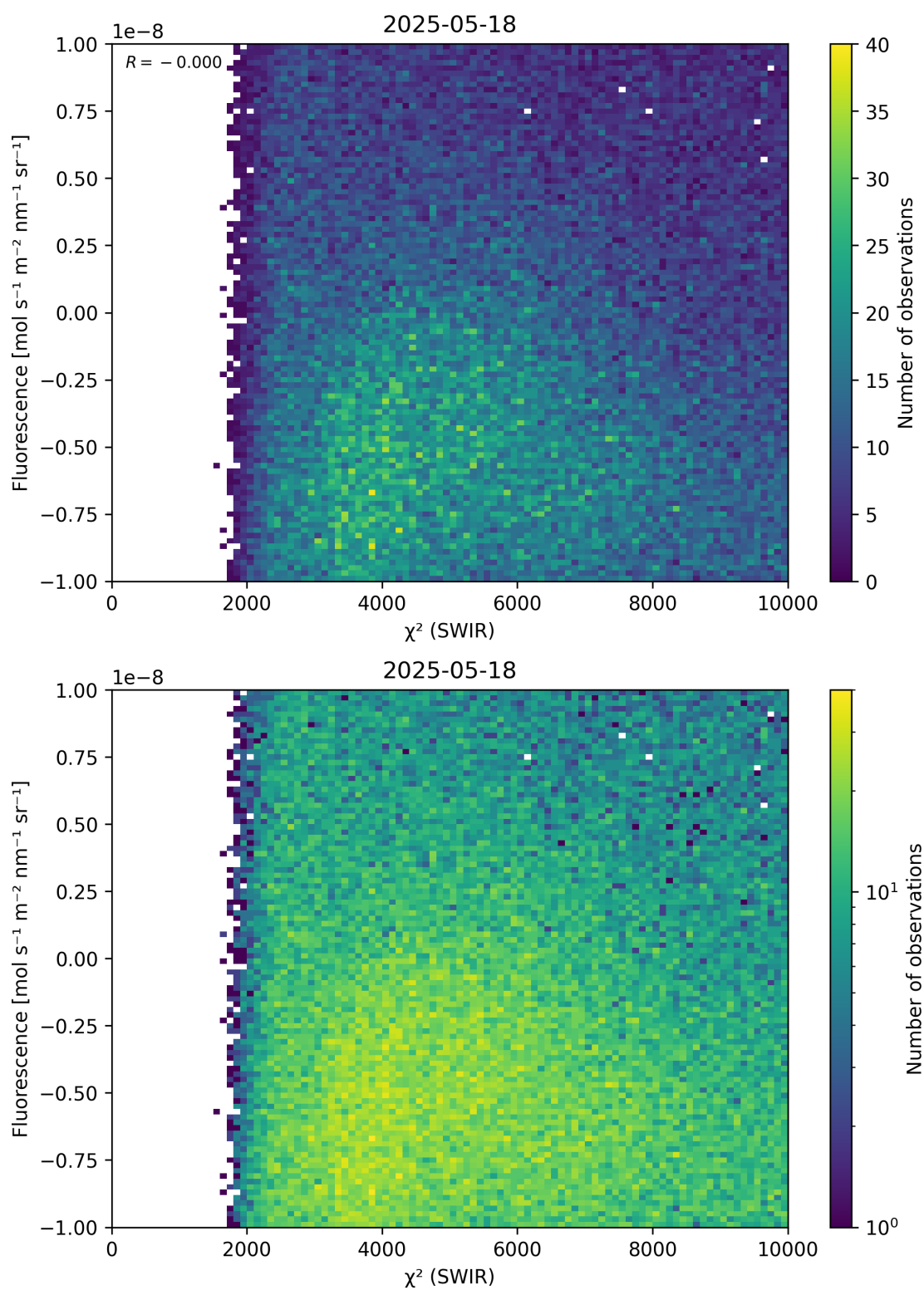
Figure 49: Scatter density plot of “ \chi^2 (SWIR)” against “Fluorescence” for 2025-05-17 to 2025-05-19.
