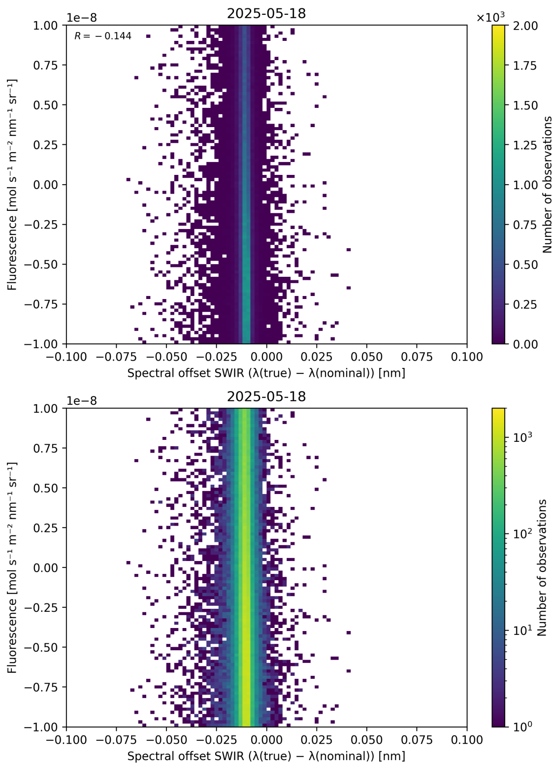
Figure 120: Scatter density plot of “Spectral offset SWIR ( \lambda_{\text{true}} - \lambda_{\text{nominal}} )” against “Fluorescence” for 2025-05-17 to 2025-05-19.
