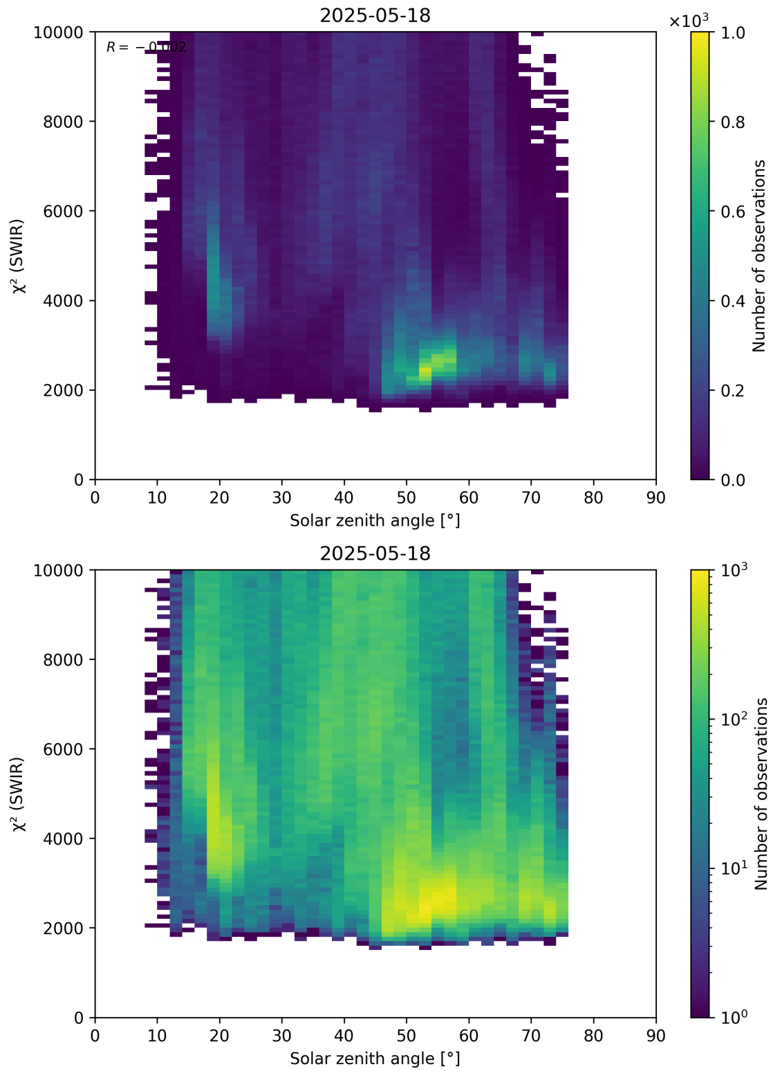
Figure 95: Scatter density plot of “Solar zenith angle” against “ \chi^2 (SWIR)” for 2025-05-17 to 2025-05-19.
