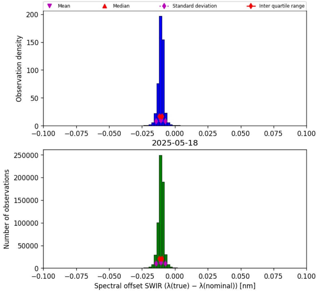
Figure 27: Histogram of “Spectral offset SWIR ( \lambda_{\text{true}} - \lambda_{\text{nominal}} )” for 2025-05-17 to 2025-05-19
