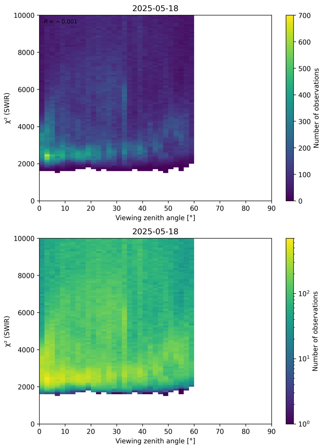
Figure 106: Scatter density plot of “Viewing zenith angle” against “ \chi^2 (SWIR)” for 2025-05-17 to 2025-05-19.
