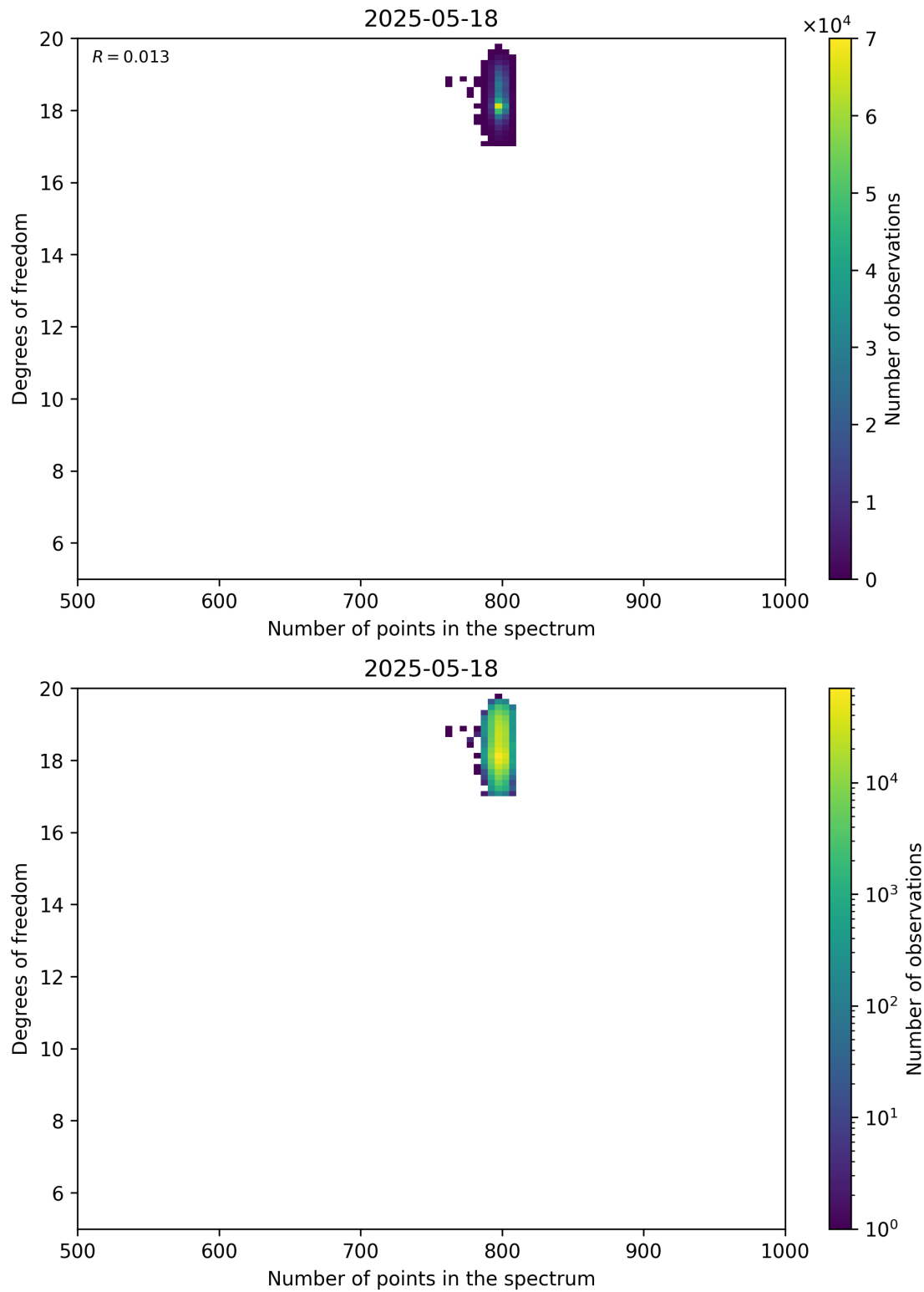
Figure 90: Scatter density plot of “Number of points in the spectrum” against “Degrees of freedom” for 2025-05-17 to 2025-05-19.
