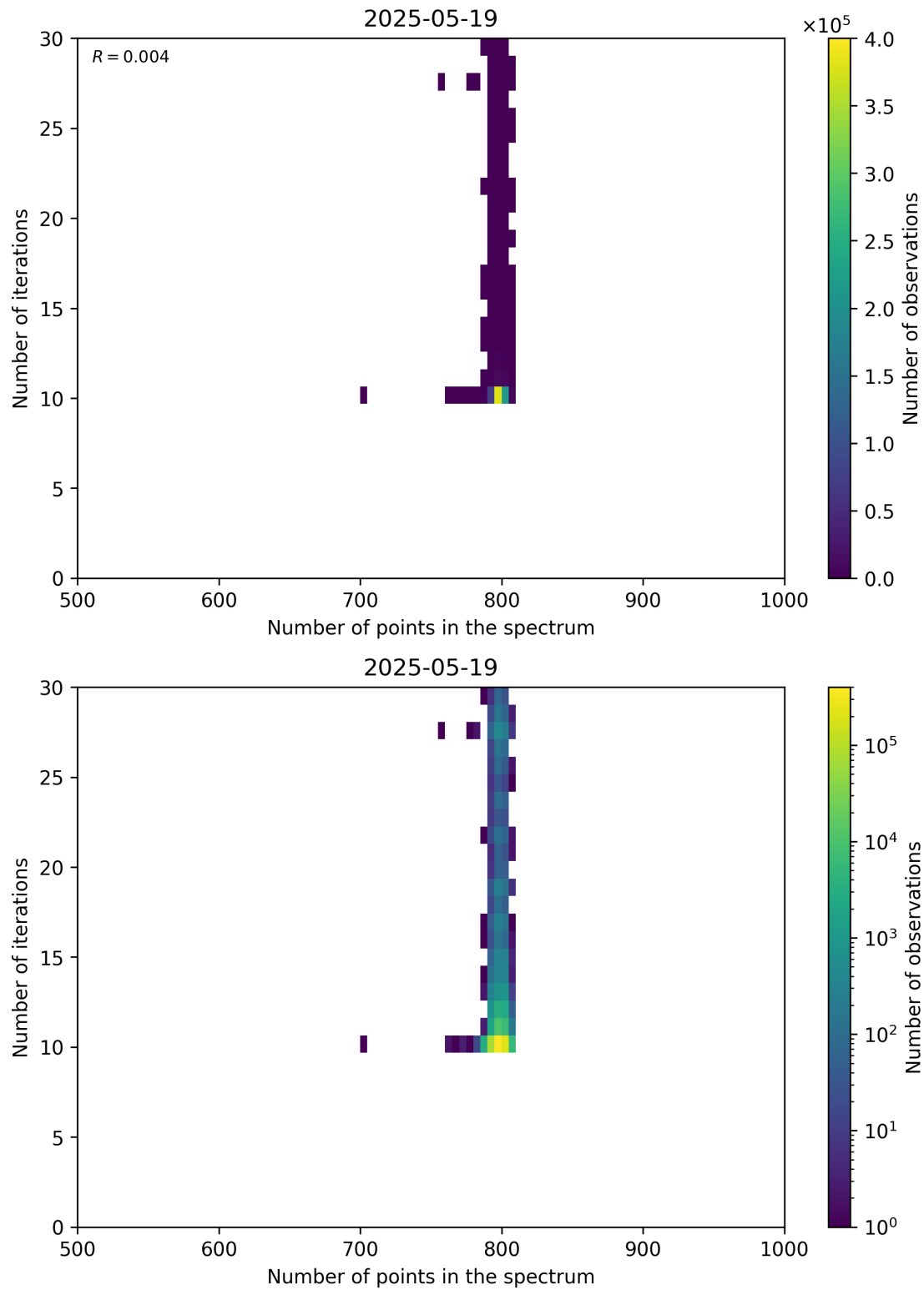
Figure 92: Scatter density plot of “Number of points in the spectrum” against “Number of iterations” for 2025-05-18 to 2025-05-20.
