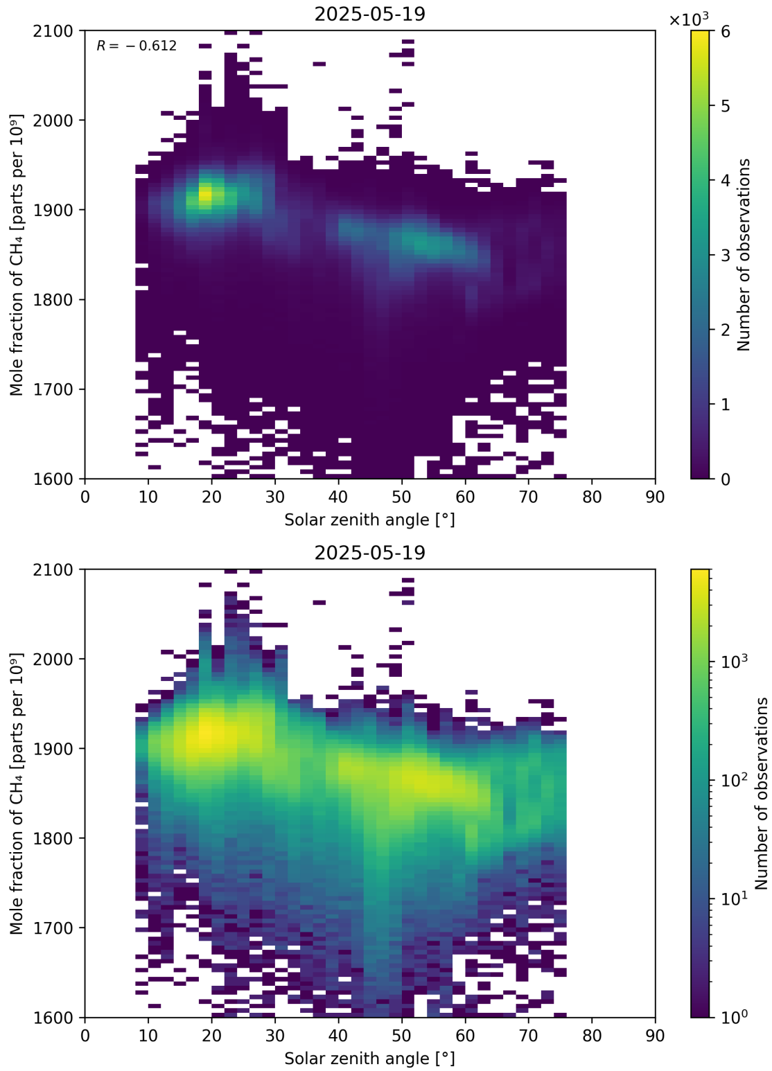
Figure 99: Scatter density plot of “Solar zenith angle” against “Mole fraction of CH 4 ” for 2025-05-18 to 2025-05-20.
