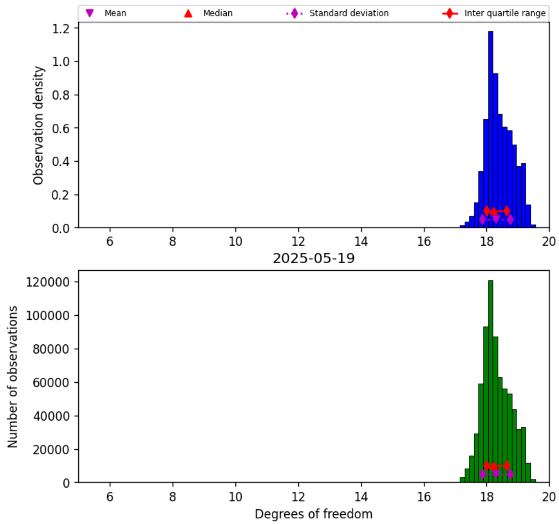
Figure 30: Histogram of “Degrees of freedom” for 2025-05-18 to 2025-05-20
