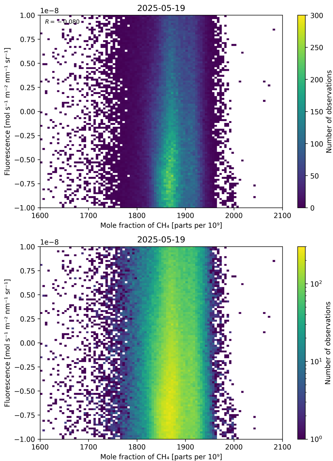
Figure 73: Scatter density plot of “Mole fraction of \text{CH}_4 ” against “Fluorescence” for 2025-05-18 to 2025-05-20.
