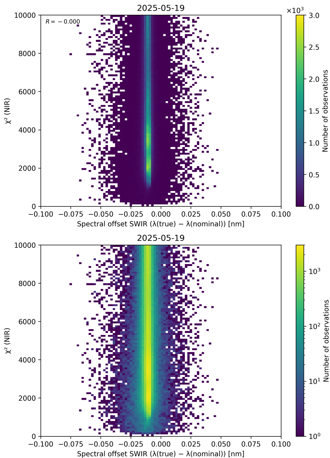
Figure 117: Scatter density plot of “Spectral offset SWIR ( \lambda_{\text{true}} - \lambda_{\text{nominal}} )” against “ \chi^2 (NIR)” for 2025-05-18 to 2025-05-20.
