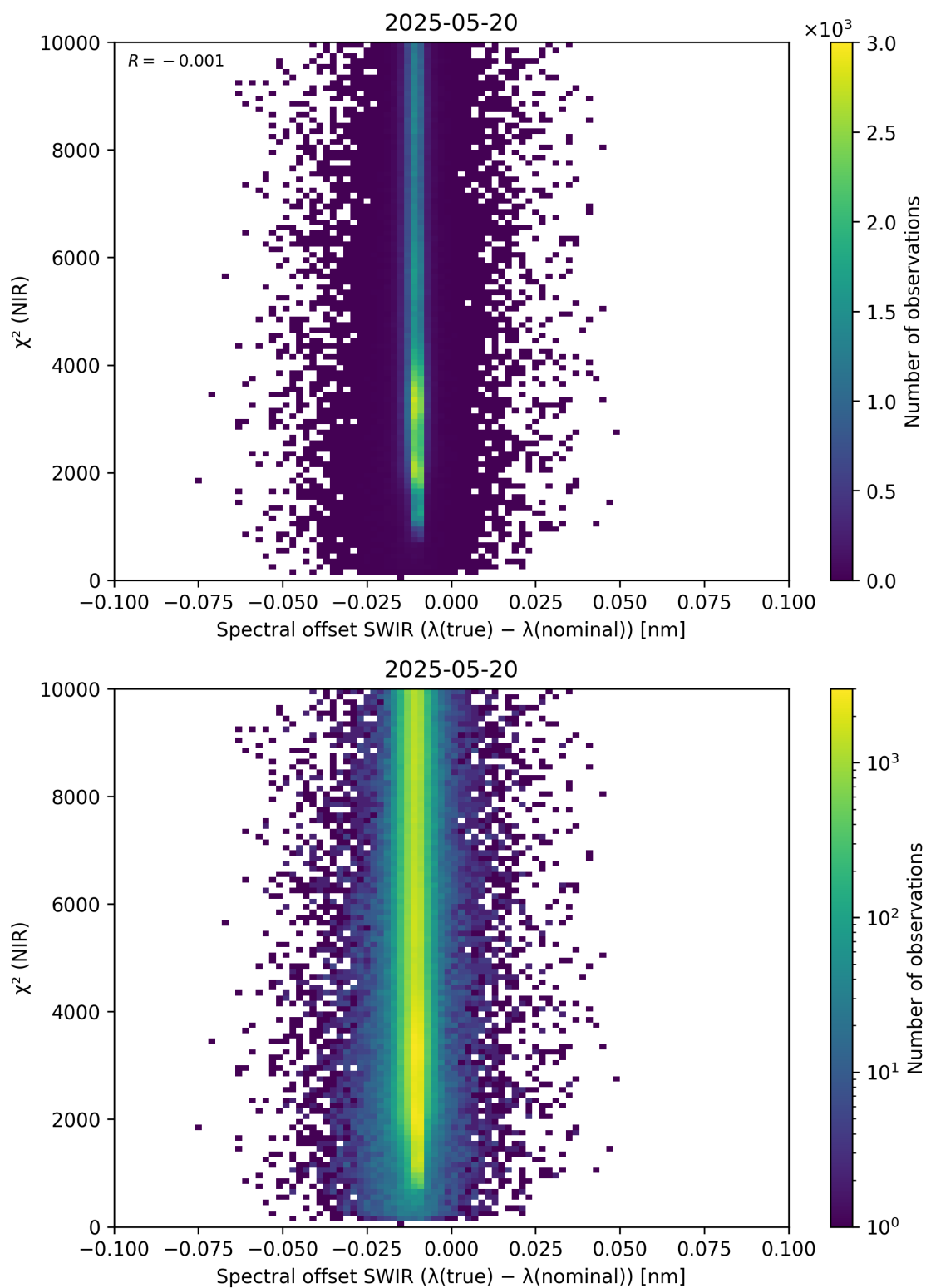
Figure 117: Scatter density plot of “Spectral offset SWIR ( \lambda_{\text{true}} - \lambda_{\text{nominal}} )” against “ \chi^2 (NIR)” for 2025-05-19 to 2025-05-21.
