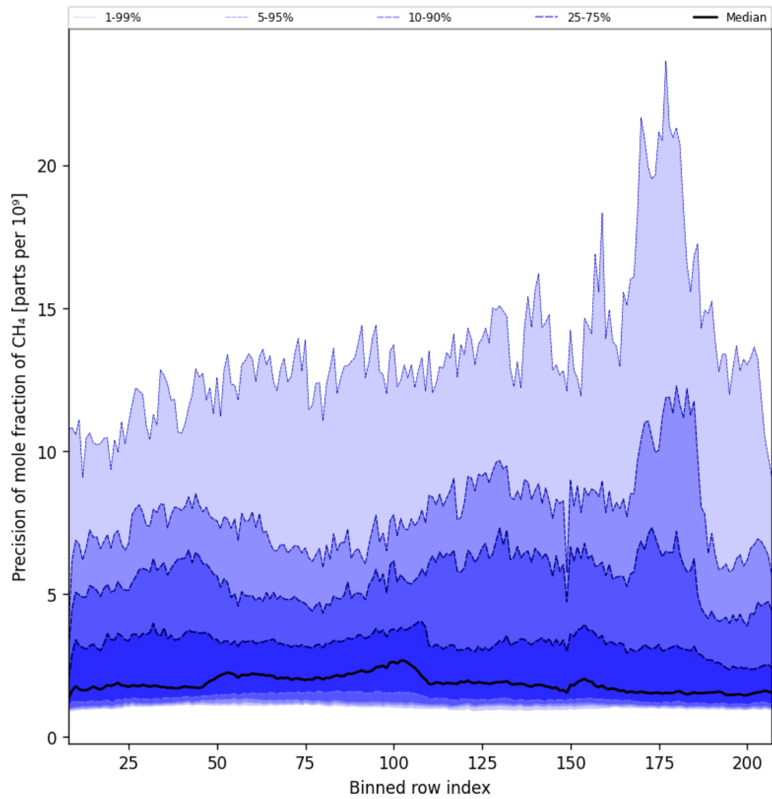
Figure 35: Along track statistics of “Precision of mole fraction of CH 4 ” for 2025-05-19 to 2025-05-21
