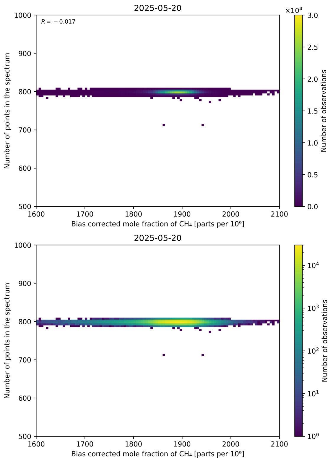
Figure 68: Scatter density plot of “Bias corrected mole fraction of CH 4 ” against “Number of points in the spectrum” for 2025-05-19 to 2025-05-21.
