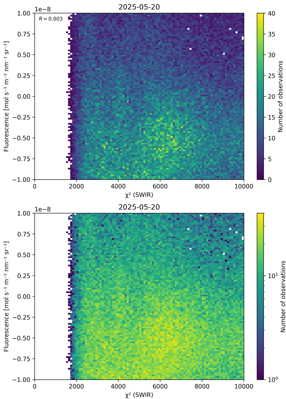
Figure 49: Scatter density plot of “ \chi^2 (SWIR)” against “Fluorescence” for 2025-05-19 to 2025-05-21.
