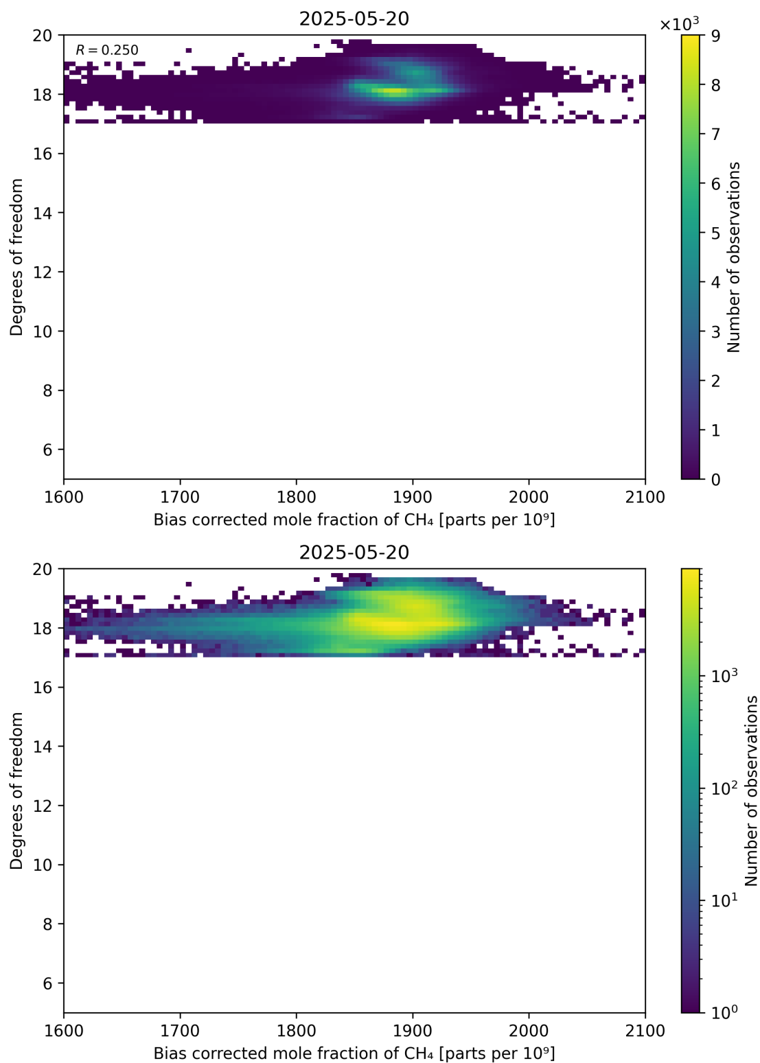
Figure 65: Scatter density plot of “Bias corrected mole fraction of CH 4 ” against “Degrees of freedom” for 2025-05-19 to 2025-05-21.
