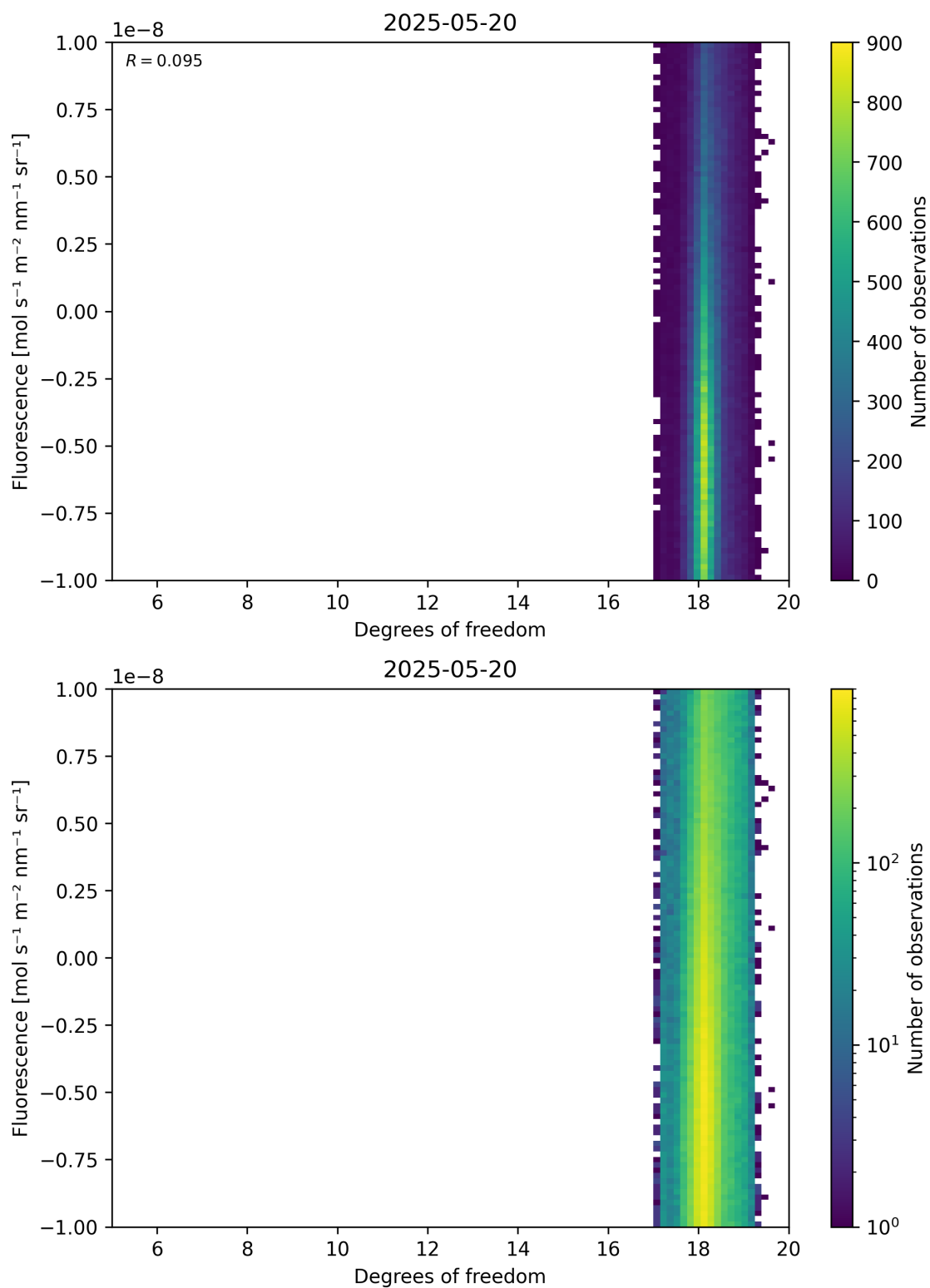
Figure 51: Scatter density plot of “Degrees of freedom” against “Fluorescence” for 2025-05-19 to 2025-05-21.
