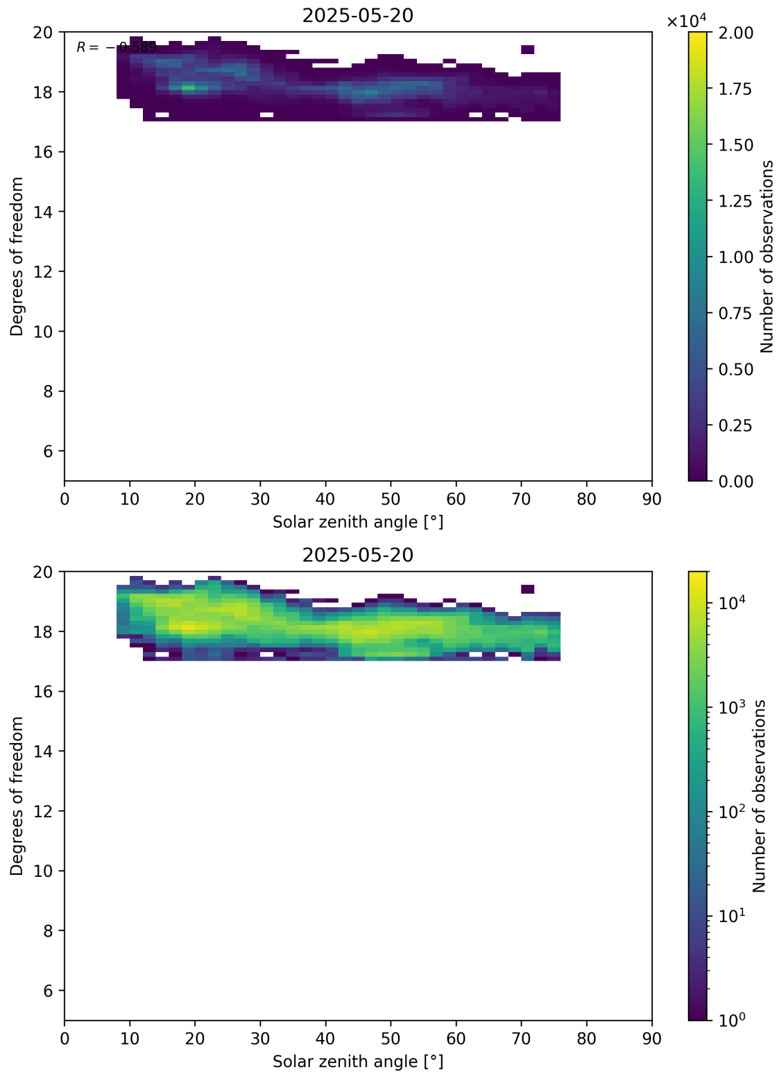
Figure 96: Scatter density plot of “Solar zenith angle” against “Degrees of freedom” for 2025-05-19 to 2025-05-21.
