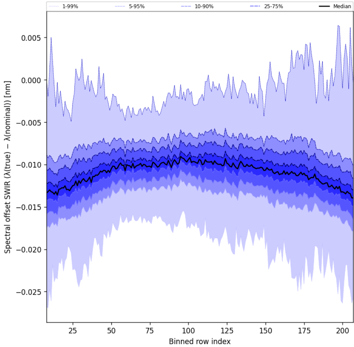
Figure 38: Along track statistics of “Spectral offset SWIR ( \lambda_{\text{true}} - \lambda_{\text{nominal}} )” for 2025-05-19 to 2025-05-21
