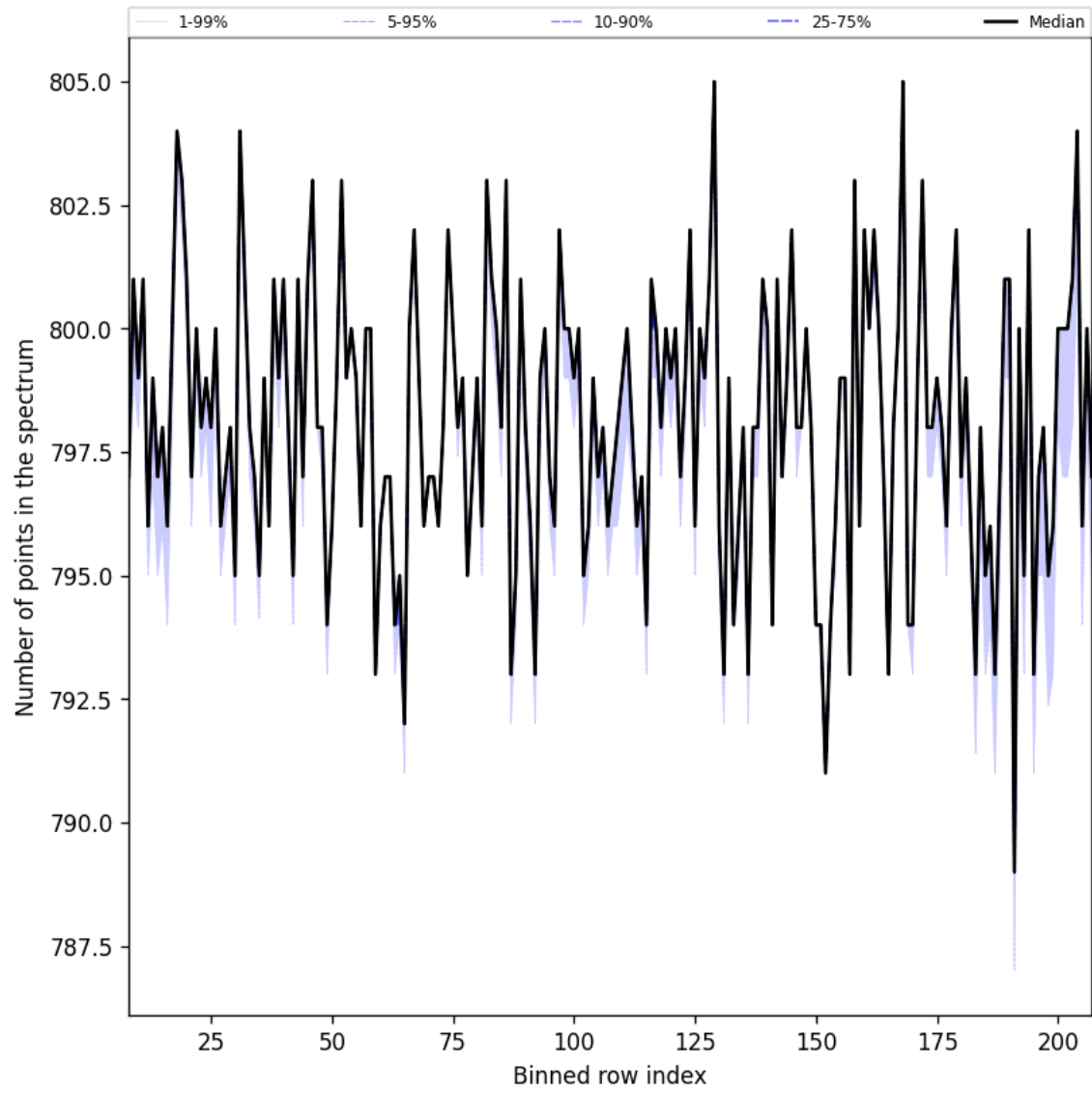
Figure 37: Along track statistics of “Number of points in the spectrum” for 2025-05-19 to 2025-05-21
