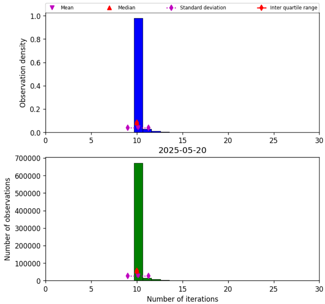
Figure 31: Histogram of “Number of iterations” for 2025-05-19 to 2025-05-21
