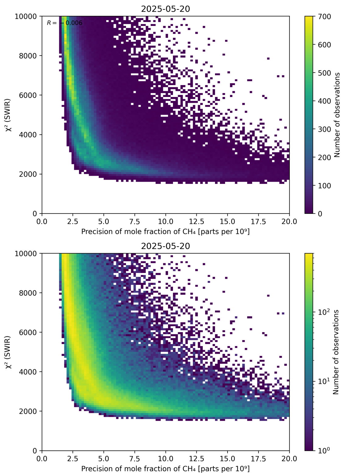
Figure 79: Scatter density plot of “Precision of mole fraction of \text{CH}_4 ” against “ \chi^2 (SWIR)” for 2025-05-19 to 2025-05-21.
