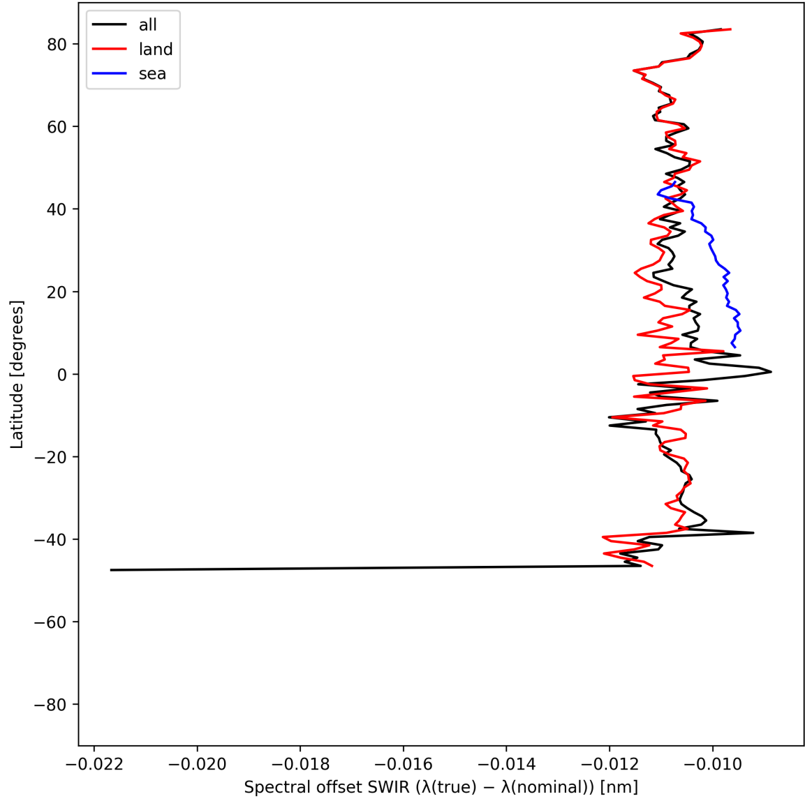
Figure 16: Zonal average of “Spectral offset SWIR ( \lambda_{\text{true}} - \lambda_{\text{nominal}} )” for 2025-05-19 to 2025-05-21.
