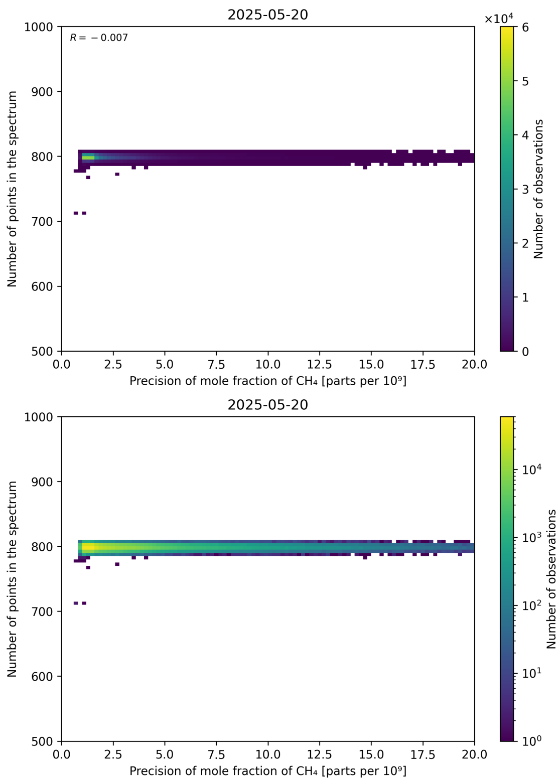
Figure 84: Scatter density plot of “Precision of mole fraction of CH 4 ” against “Number of points in the spectrum” for 2025-05-19 to 2025-05-21.
