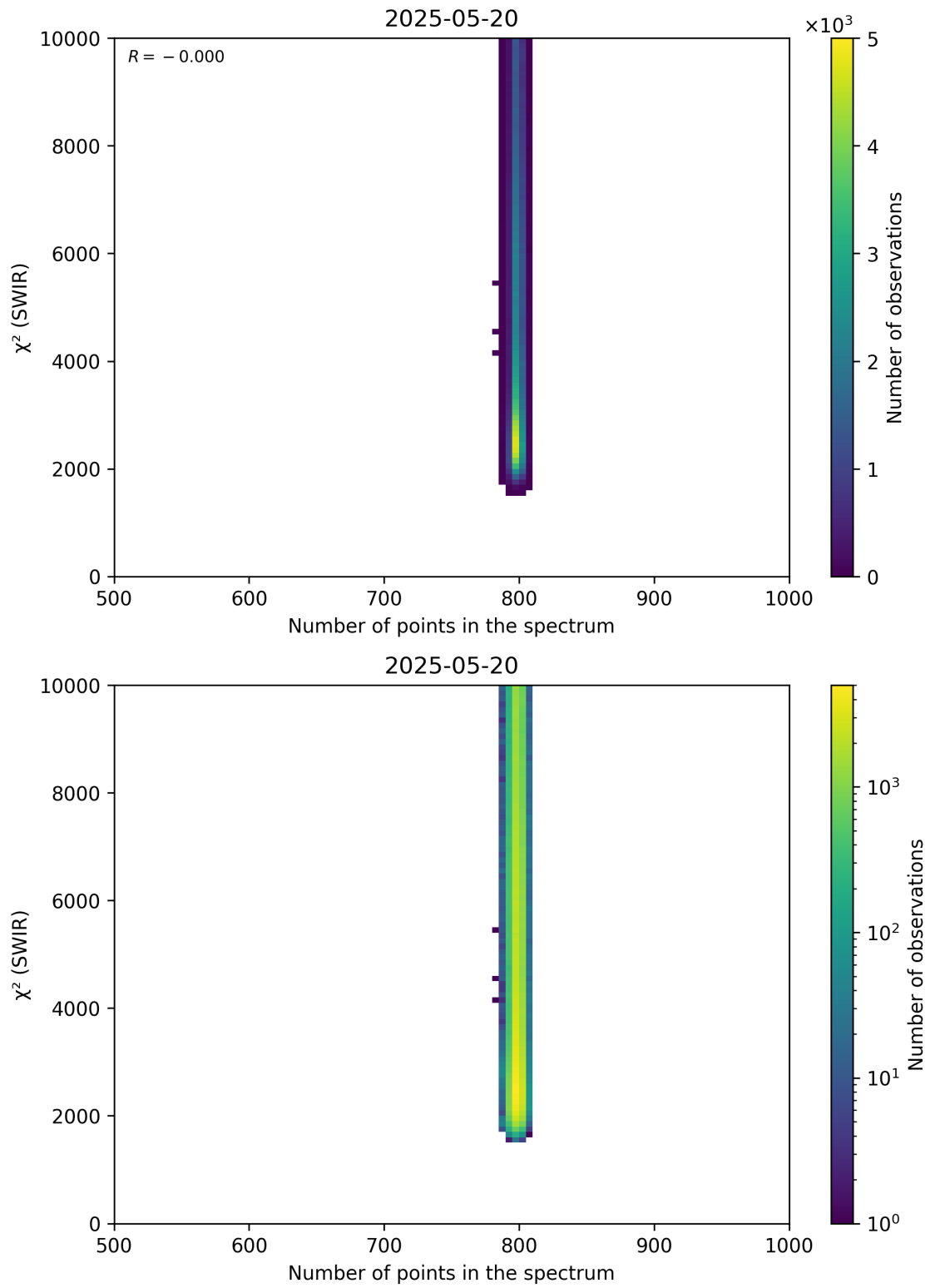
Figure 89: Scatter density plot of “Number of points in the spectrum” against “ \chi^2 (SWIR)” for 2025-05-19 to 2025-05-21.
