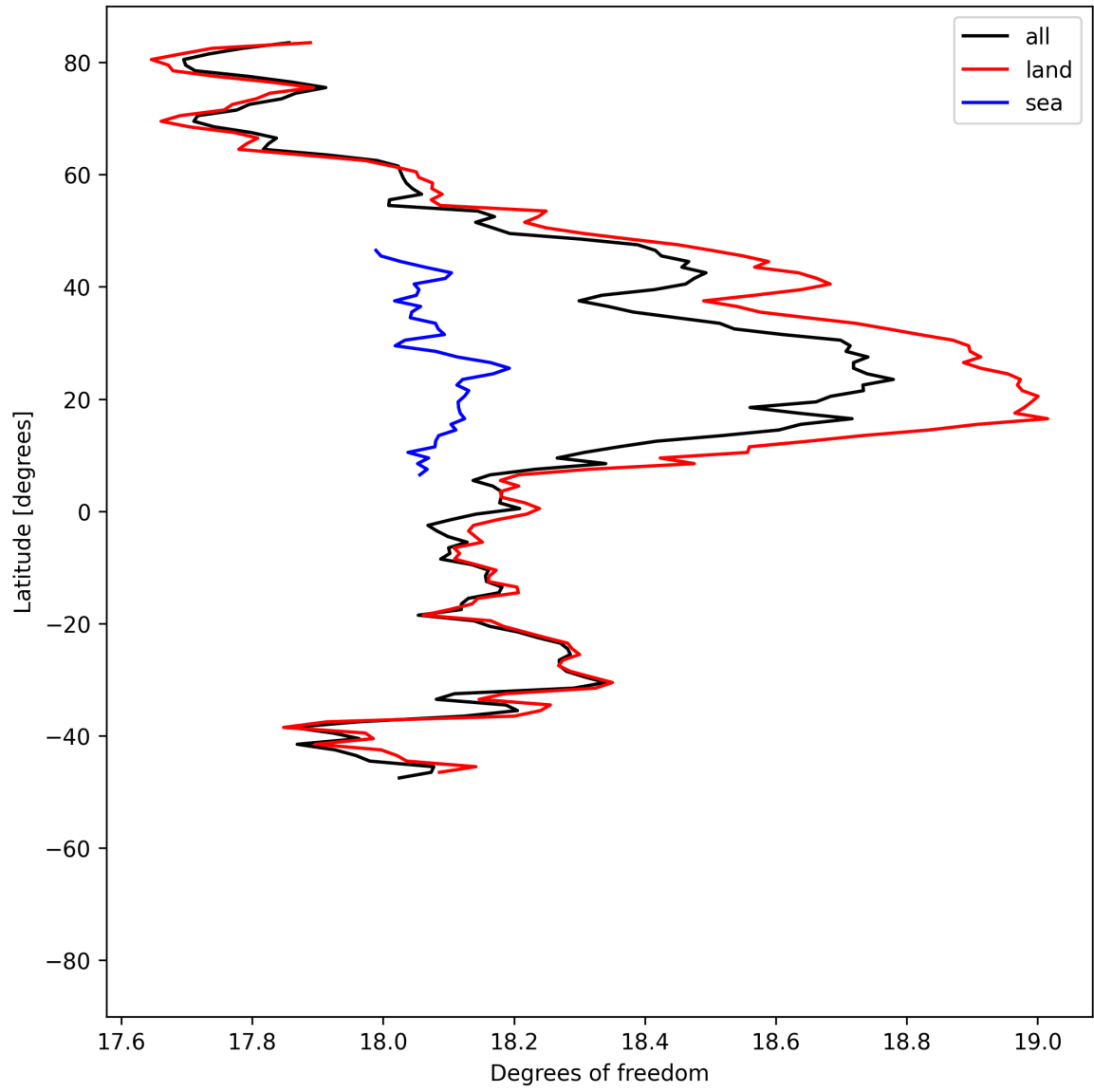
Figure 19: Zonal average of “Degrees of freedom” for 2025-05-19 to 2025-05-21.
