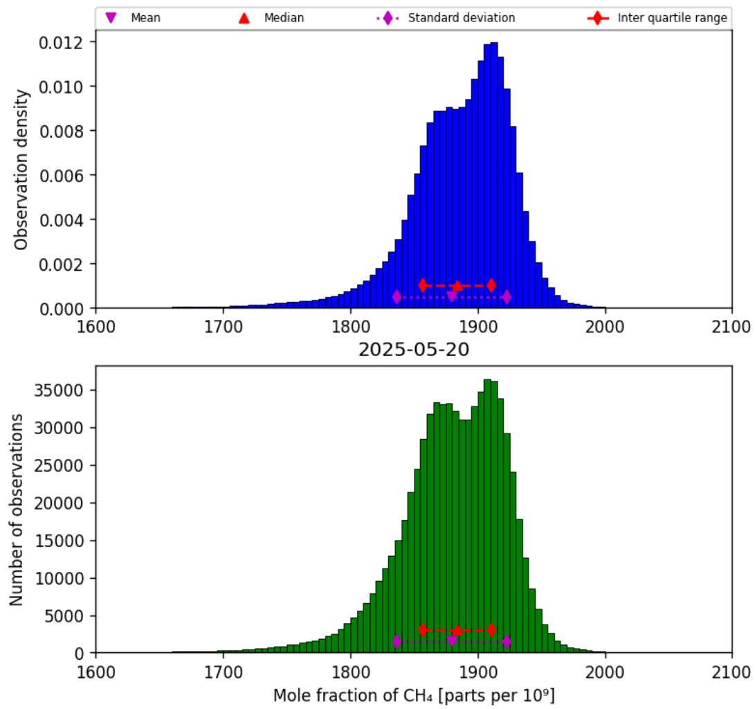
Figure 23: Histogram of “Mole fraction of CH 4 ” for 2025-05-19 to 2025-05-21
