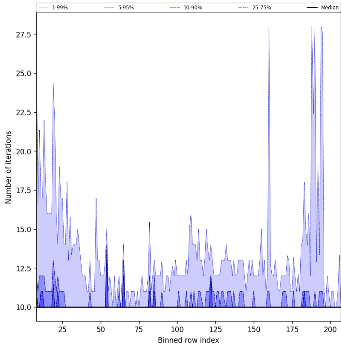
Figure 42: Along track statistics of “Number of iterations” for 2025-05-19 to 2025-05-21
