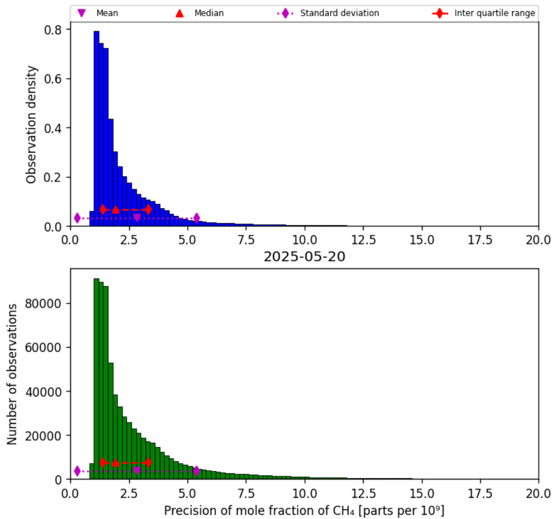
Figure 24: Histogram of “Precision of mole fraction of CH 4 ” for 2025-05-19 to 2025-05-21
