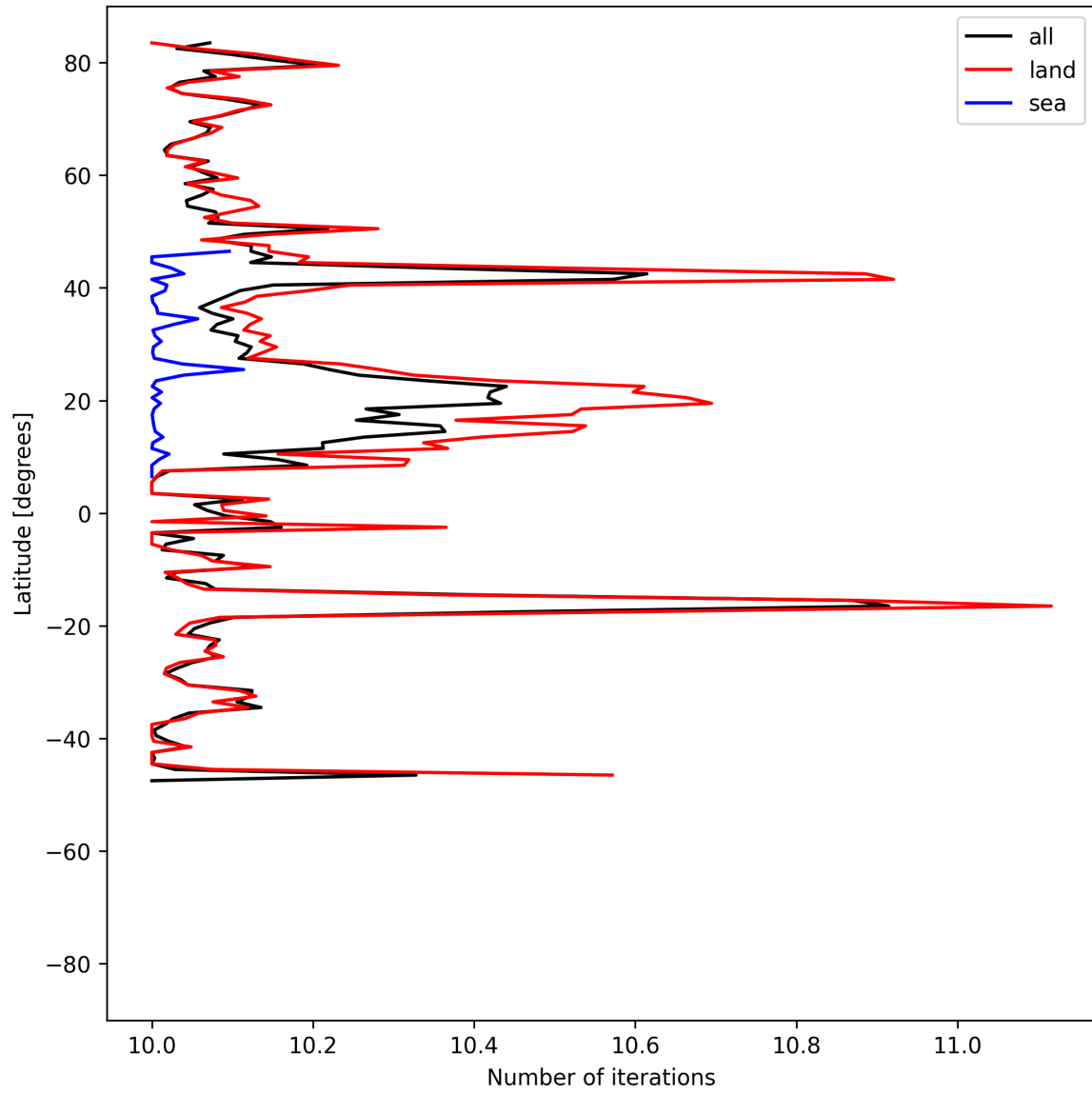
Figure 20: Zonal average of “Number of iterations” for 2025-05-19 to 2025-05-21.
