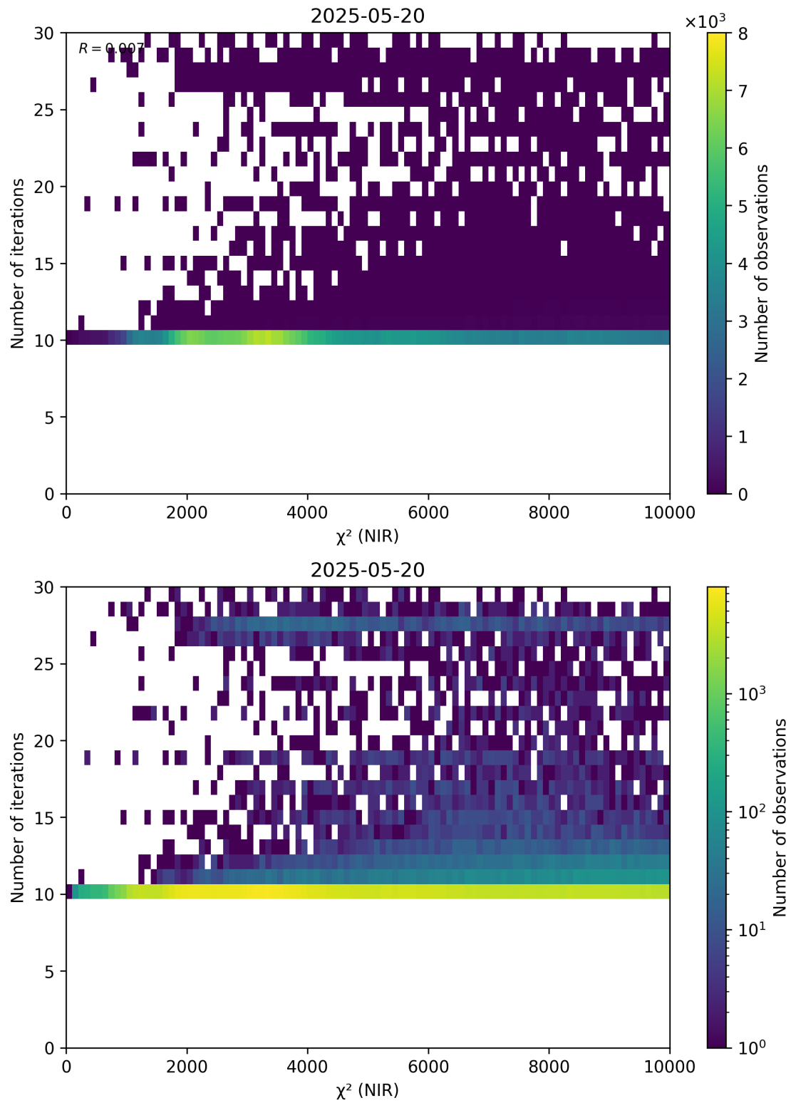
Figure 46: Scatter density plot of “ \chi^2 (NIR)” against “Number of iterations” for 2025-05-19 to 2025-05-21.
