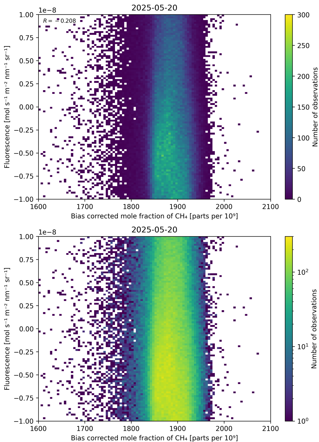
Figure 66: Scatter density plot of “Bias corrected mole fraction of \text{CH}_4 ” against “Fluorescence” for 2025-05-19 to 2025-05-21.
