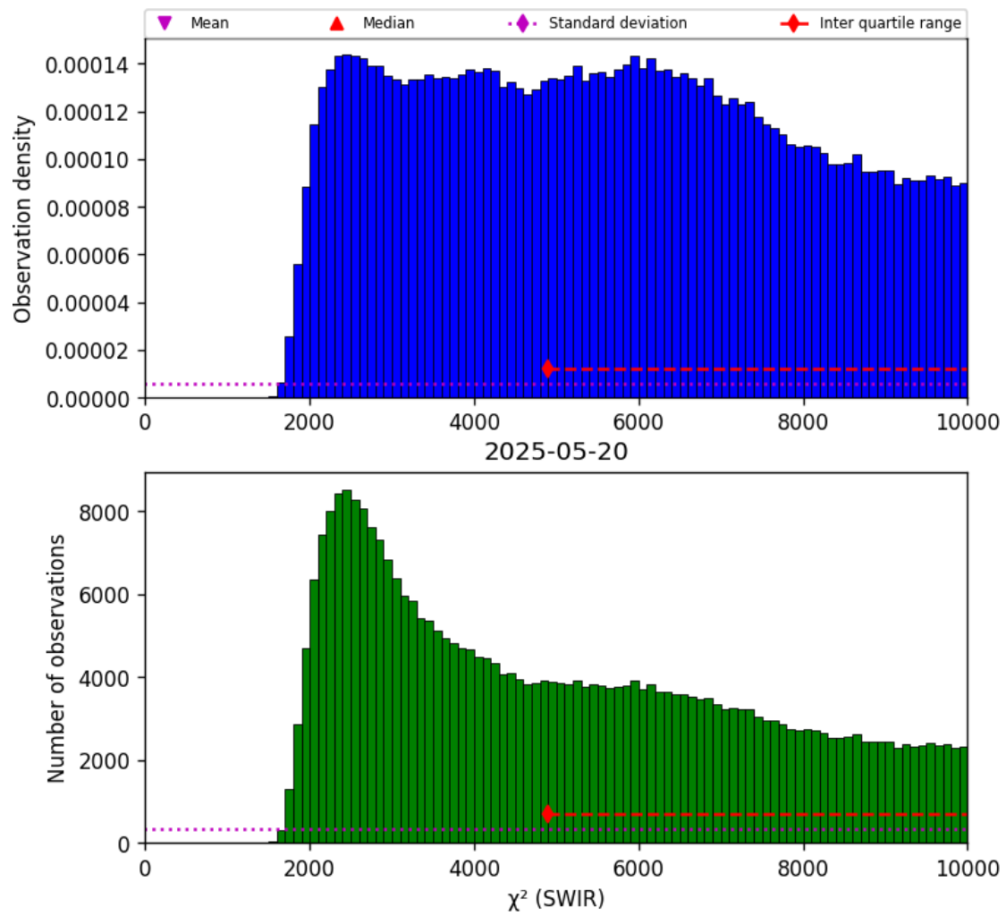
Figure 28: Histogram of “ \chi^2 (SWIR)” for 2025-05-19 to 2025-05-21
