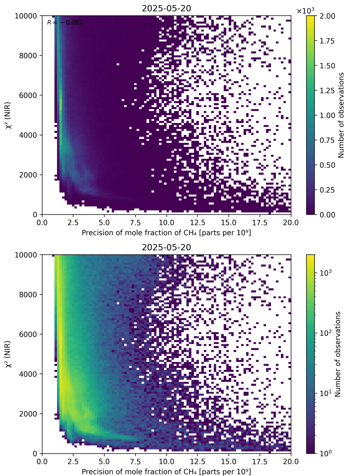
Figure 78: Scatter density plot of “Precision of mole fraction of CH 4 ” against “ \chi^2 (NIR)” for 2025-05-19 to 2025-05-21.
