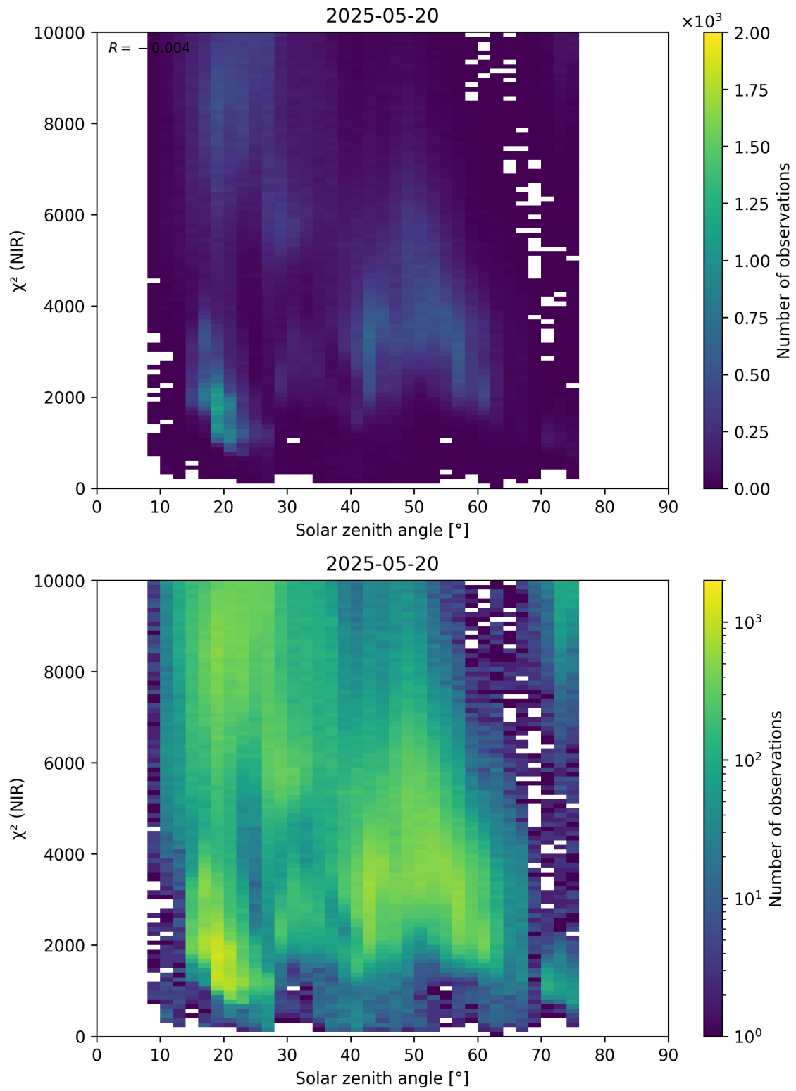
Figure 94: Scatter density plot of “Solar zenith angle” against “ \chi^2 (NIR)” for 2025-05-19 to 2025-05-21.
