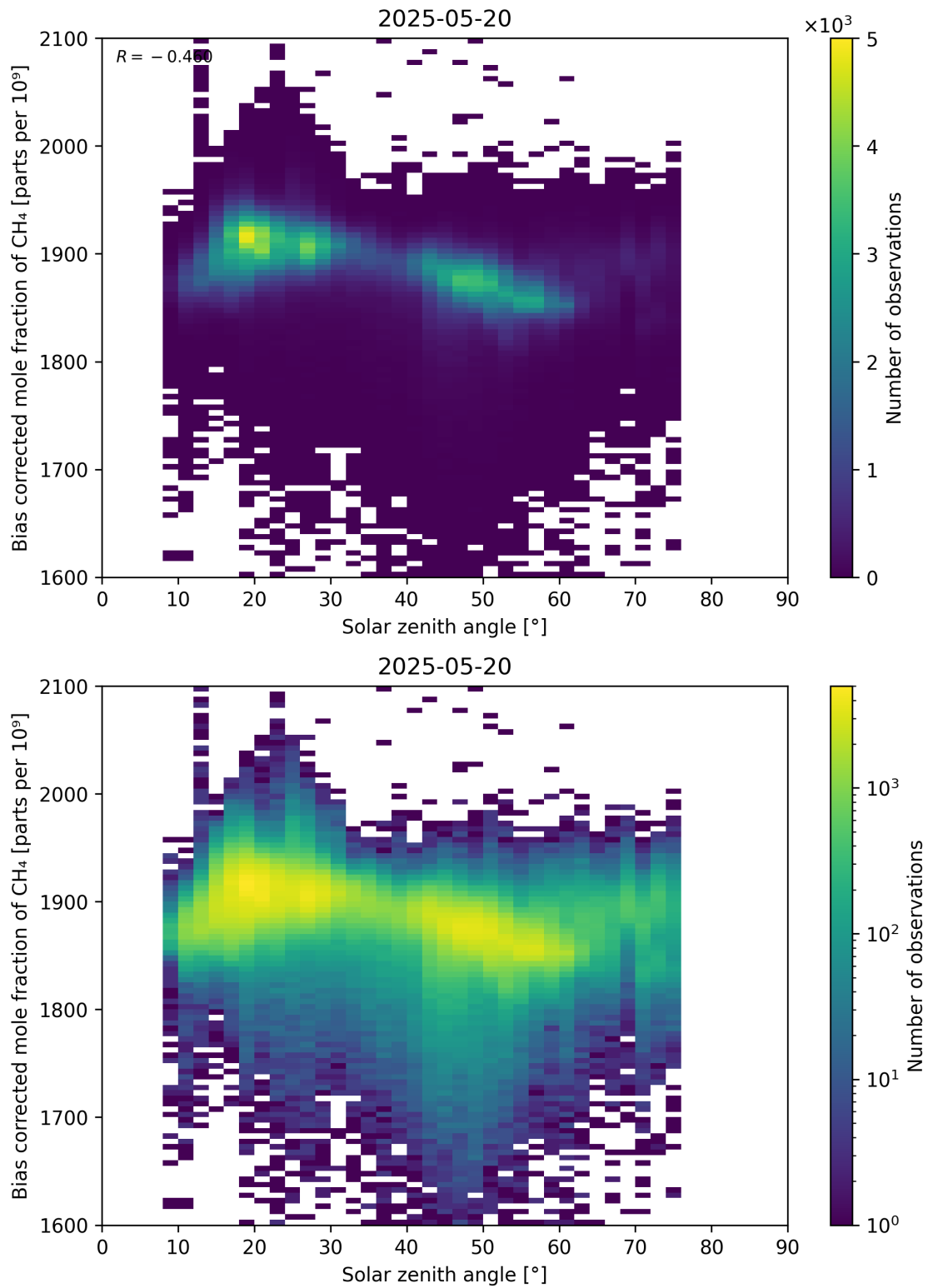
Figure 100: Scatter density plot of “Solar zenith angle” against “Bias corrected mole fraction of CH 4 ” for 2025-05-19 to 2025-05-21.
