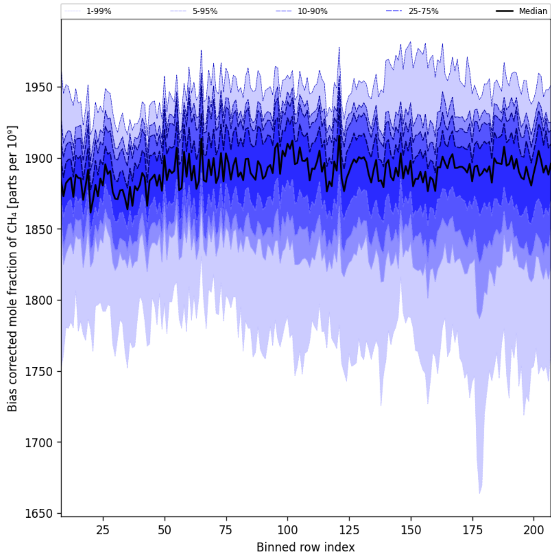
Figure 36: Along track statistics of “Bias corrected mole fraction of CH 4 ” for 2025-05-19 to 2025-05-21
