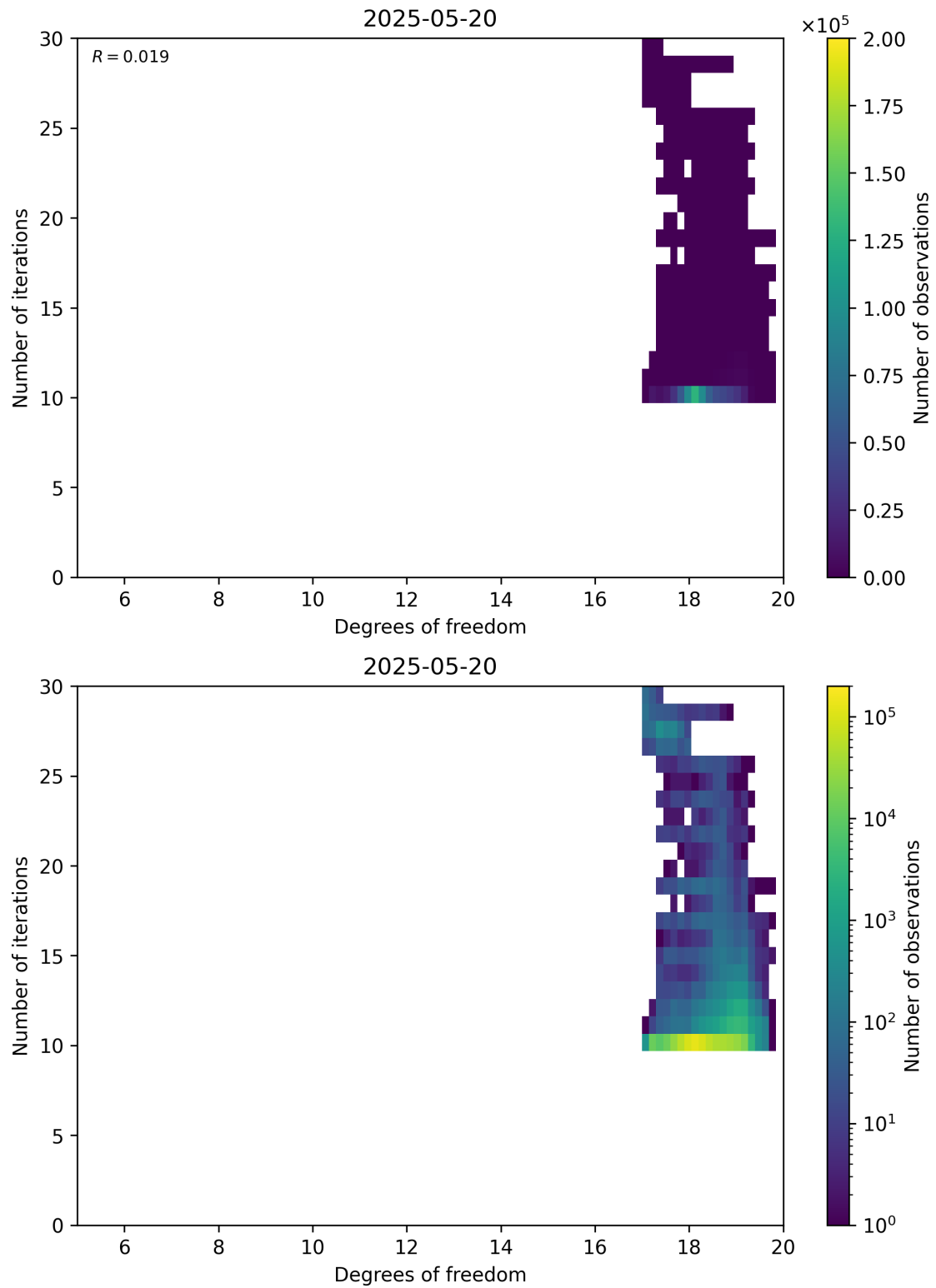
Figure 52: Scatter density plot of “Degrees of freedom” against “Number of iterations” for 2025-05-19 to 2025-05-21.
