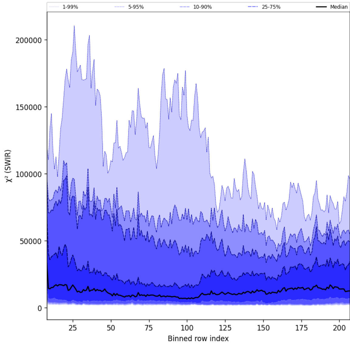
Figure 39: Along track statistics of “ \chi^2 (SWIR)” for 2025-05-19 to 2025-05-21
