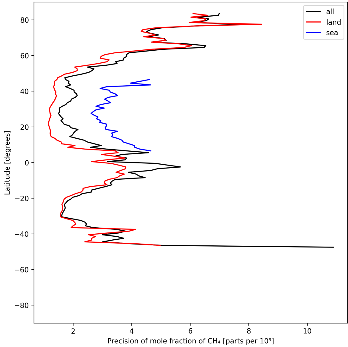
Figure 13: Zonal average of “Precision of mole fraction of CH 4 ” for 2025-05-19 to 2025-05-21.
