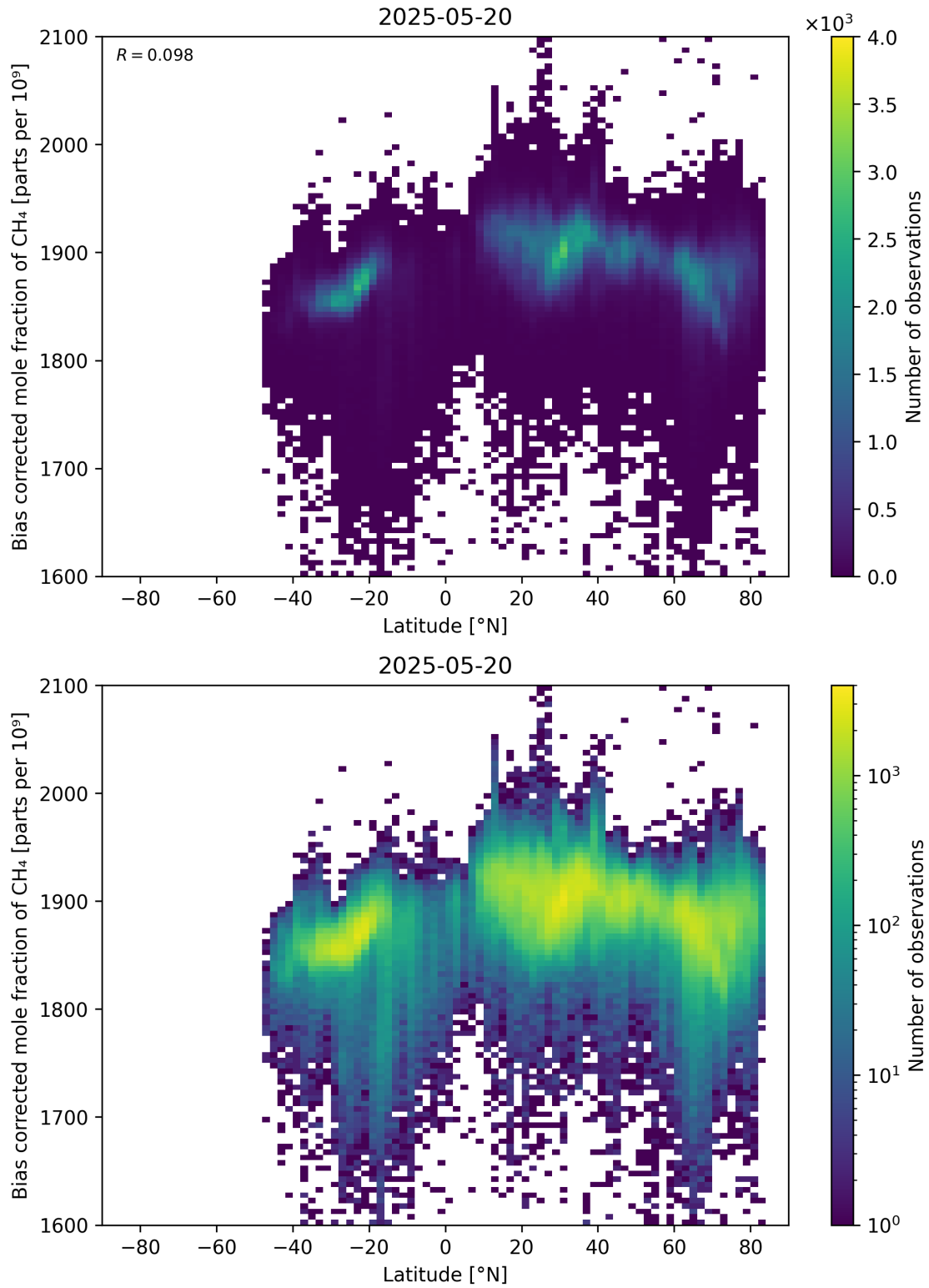
Figure 58: Scatter density plot of “Latitude” against “Bias corrected mole fraction of CH 4 ” for 2025-05-19 to 2025-05-21.
