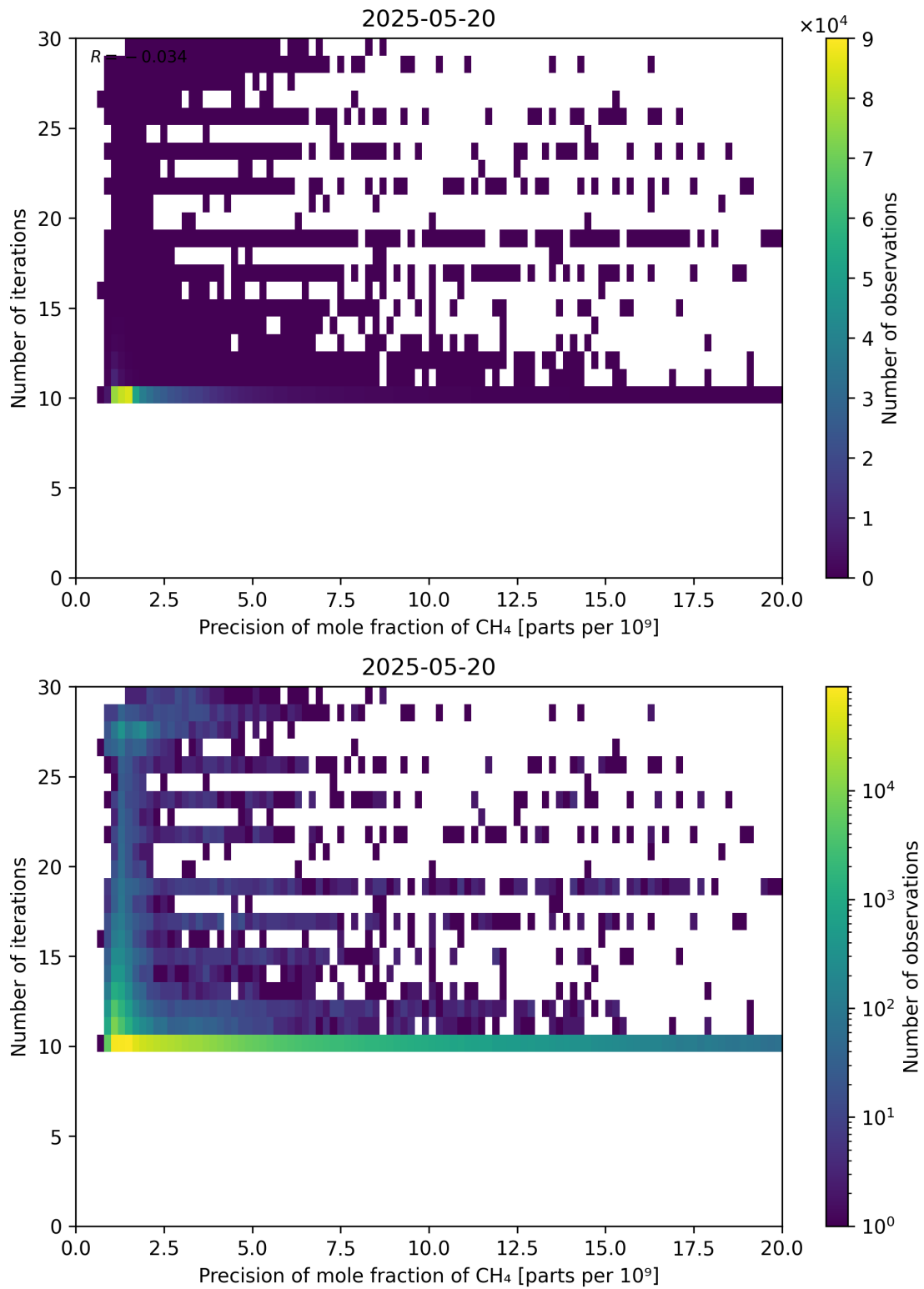
Figure 83: Scatter density plot of “Precision of mole fraction of CH 4 ” against “Number of iterations” for 2025-05-19 to 2025-05-21.
