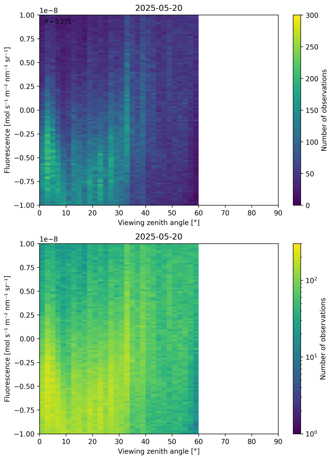
Figure 108: Scatter density plot of “Viewing zenith angle” against “Fluorescence” for 2025-05-19 to 2025-05-21.
