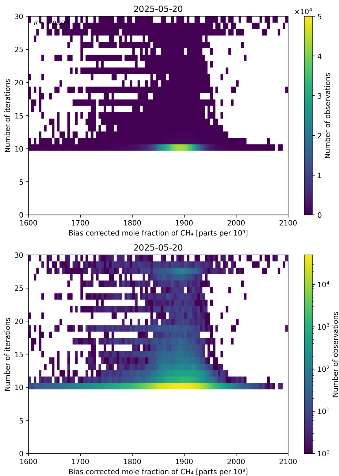
Figure 67: Scatter density plot of “Bias corrected mole fraction of CH 4 ” against “Number of iterations” for 2025-05-19 to 2025-05-21.
