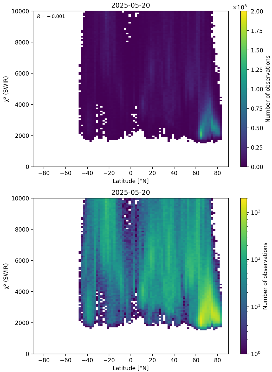
Figure 54: Scatter density plot of “Latitude” against “ \chi^2 (SWIR)” for 2025-05-19 to 2025-05-21.
