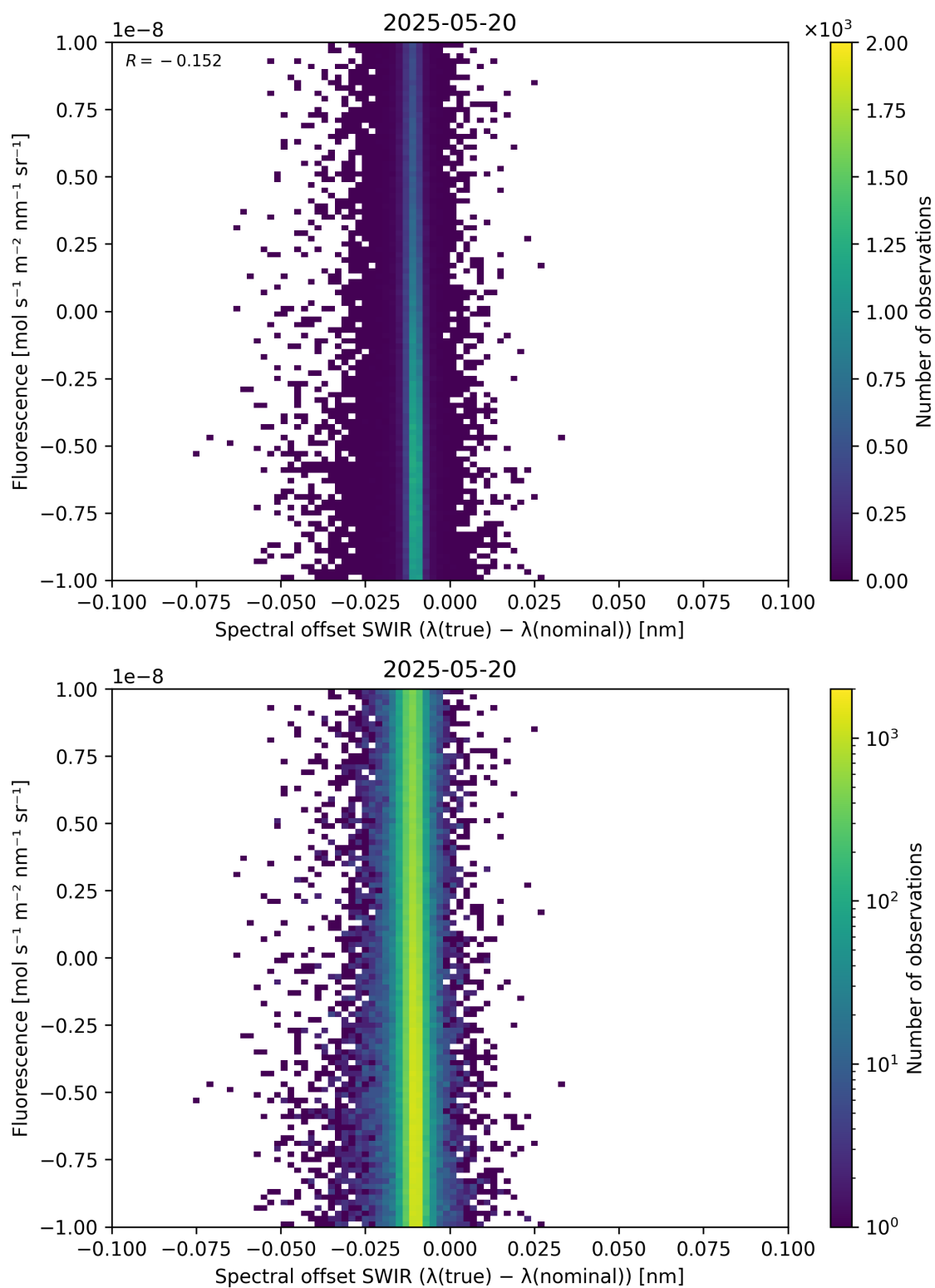
Figure 120: Scatter density plot of “Spectral offset SWIR ( \lambda_{\text{true}} - \lambda_{\text{nominal}} )” against “Fluorescence” for 2025-05-19 to 2025-05-21.
