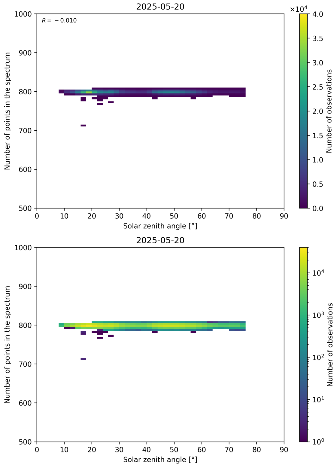
Figure 103: Scatter density plot of “Solar zenith angle” against “Number of points in the spectrum” for 2025-05-19 to 2025-05-21.
