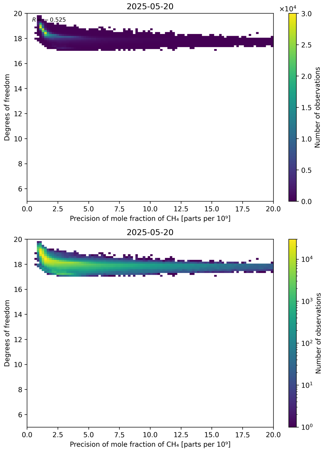
Figure 80: Scatter density plot of “Precision of mole fraction of CH 4 ” against “Degrees of freedom” for 2025-05-19 to 2025-05-21.
