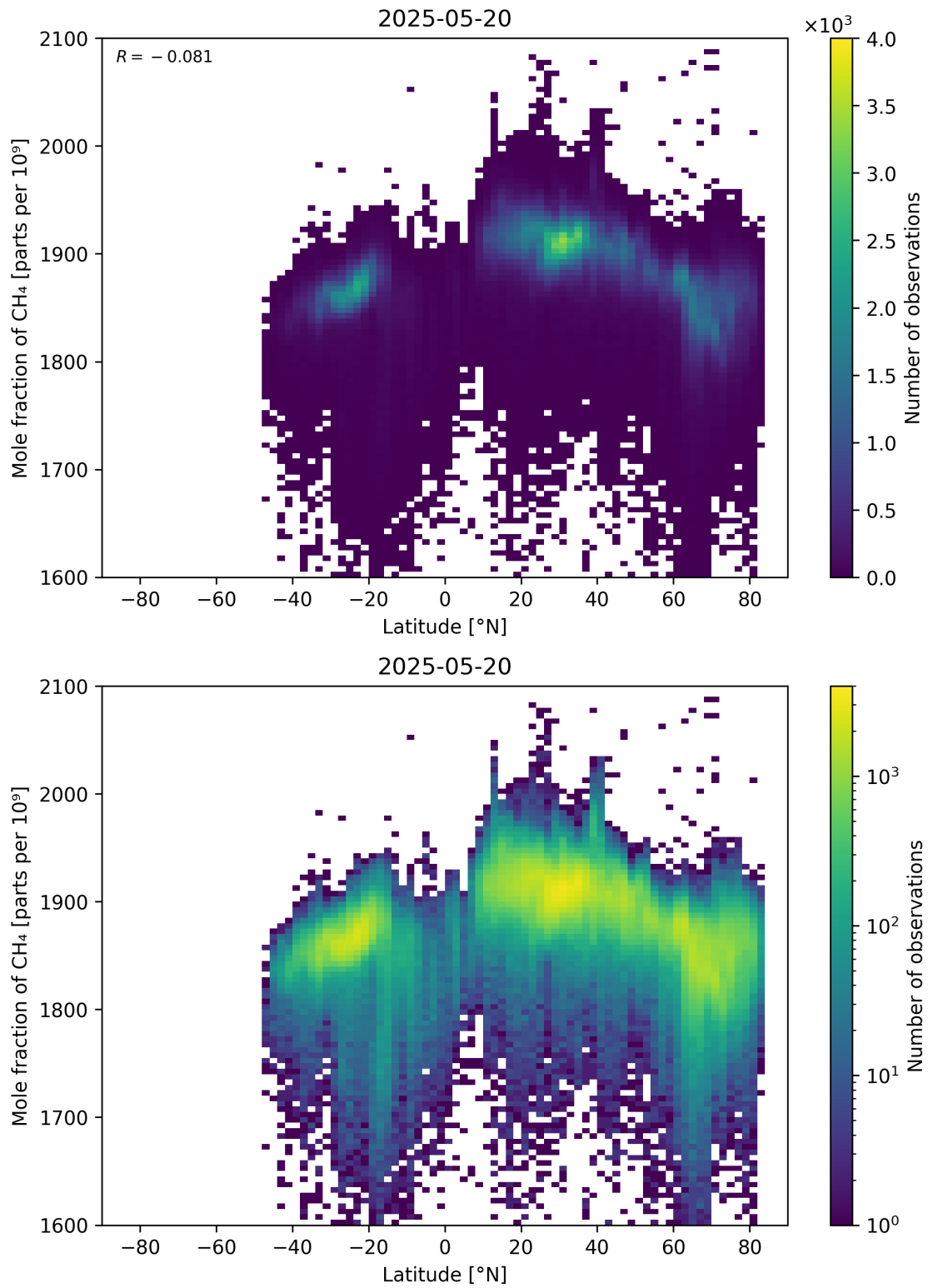
Figure 57: Scatter density plot of “Latitude” against “Mole fraction of CH 4 ” for 2025-05-19 to 2025-05-21.
