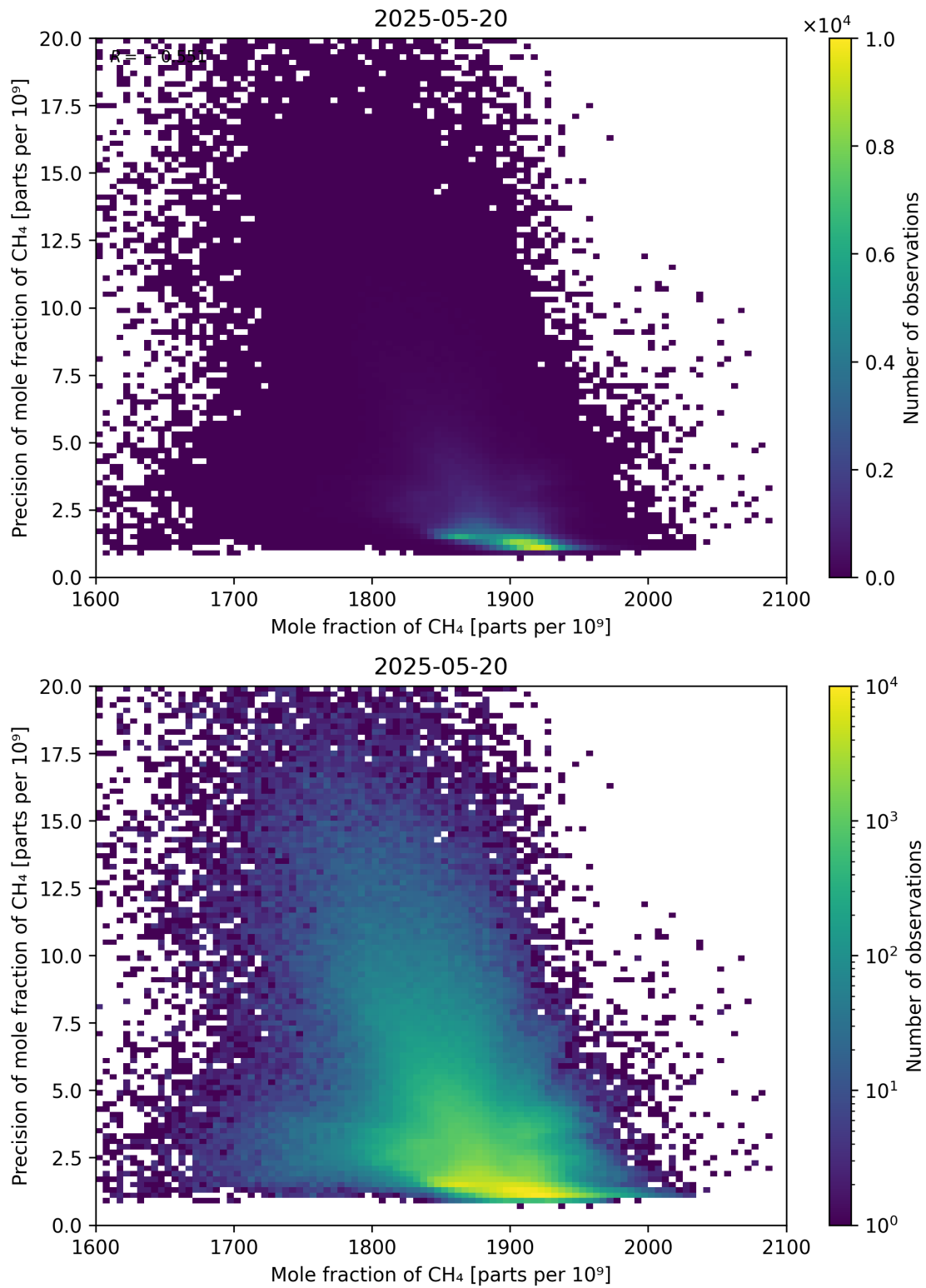
Figure 75: Scatter density plot of “Mole fraction of CH 4 ” against “Precision of mole fraction of CH 4 ” for 2025-05-19 to 2025-05-21.
