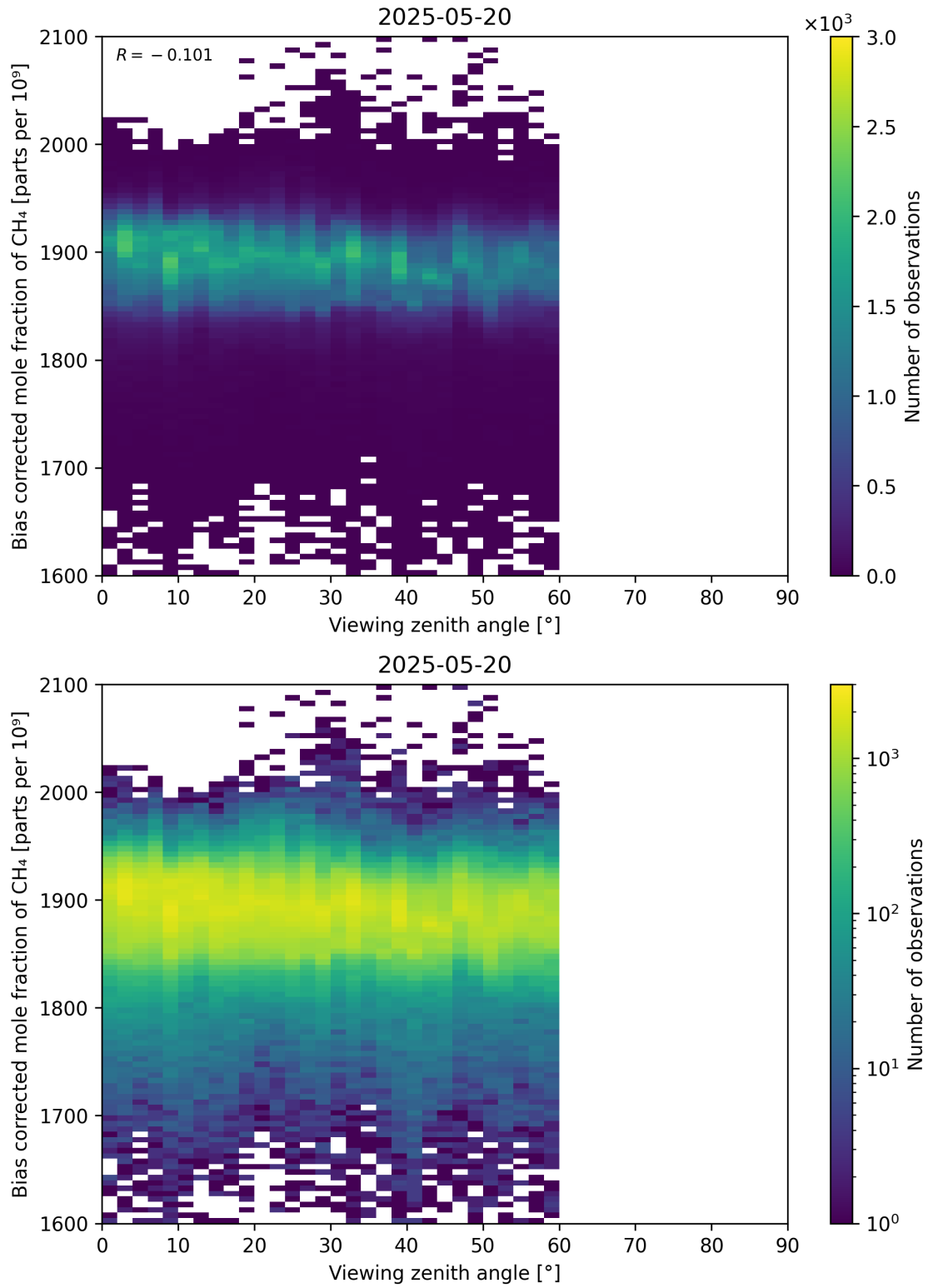
Figure 111: Scatter density plot of “Viewing zenith angle” against “Bias corrected mole fraction of CH 4 ” for 2025-05-19 to 2025-05-21.
