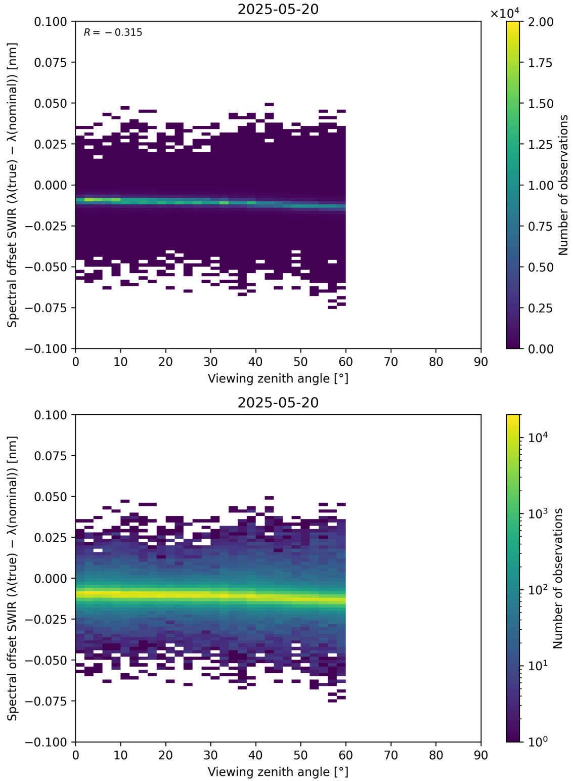
Figure 116: Scatter density plot of “Viewing zenith angle” against “Spectral offset SWIR ( \lambda_{\text{true}} - \lambda_{\text{nominal}} )” for 2025-05-19 to 2025-05-21.
