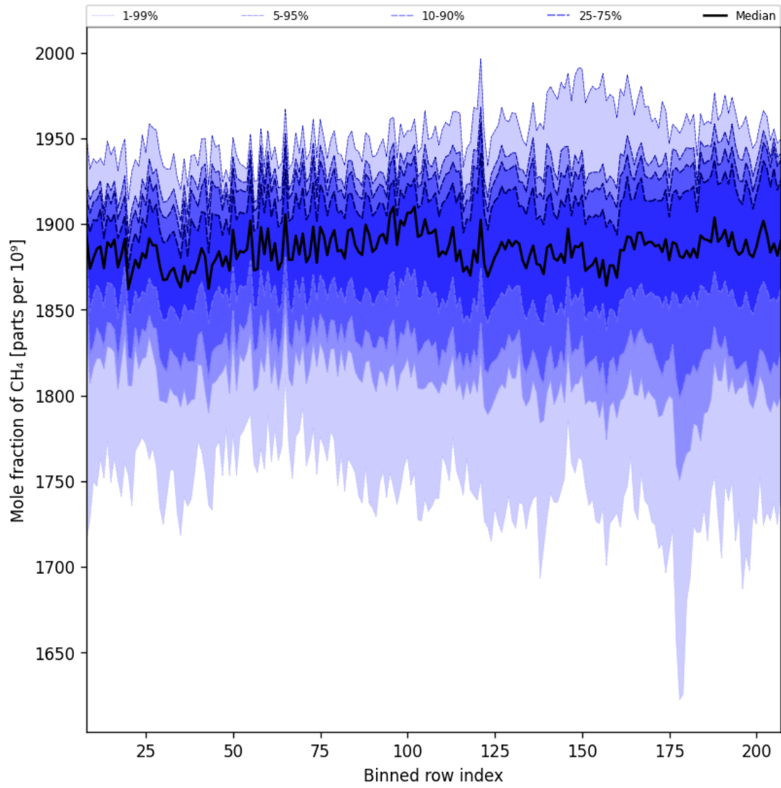
Figure 34: Along track statistics of “Mole fraction of CH 4 ” for 2025-05-19 to 2025-05-21
