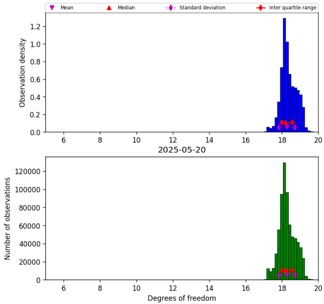
Figure 30: Histogram of “Degrees of freedom” for 2025-05-19 to 2025-05-21
