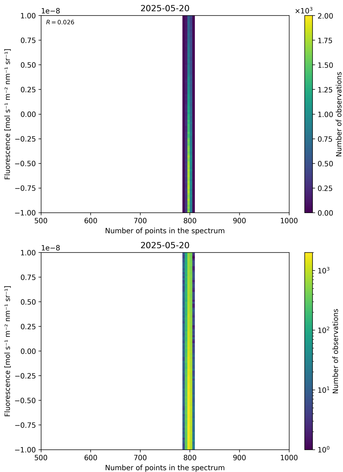
Figure 91: Scatter density plot of “Number of points in the spectrum” against “Fluorescence” for 2025-05-19 to 2025-05-21.
