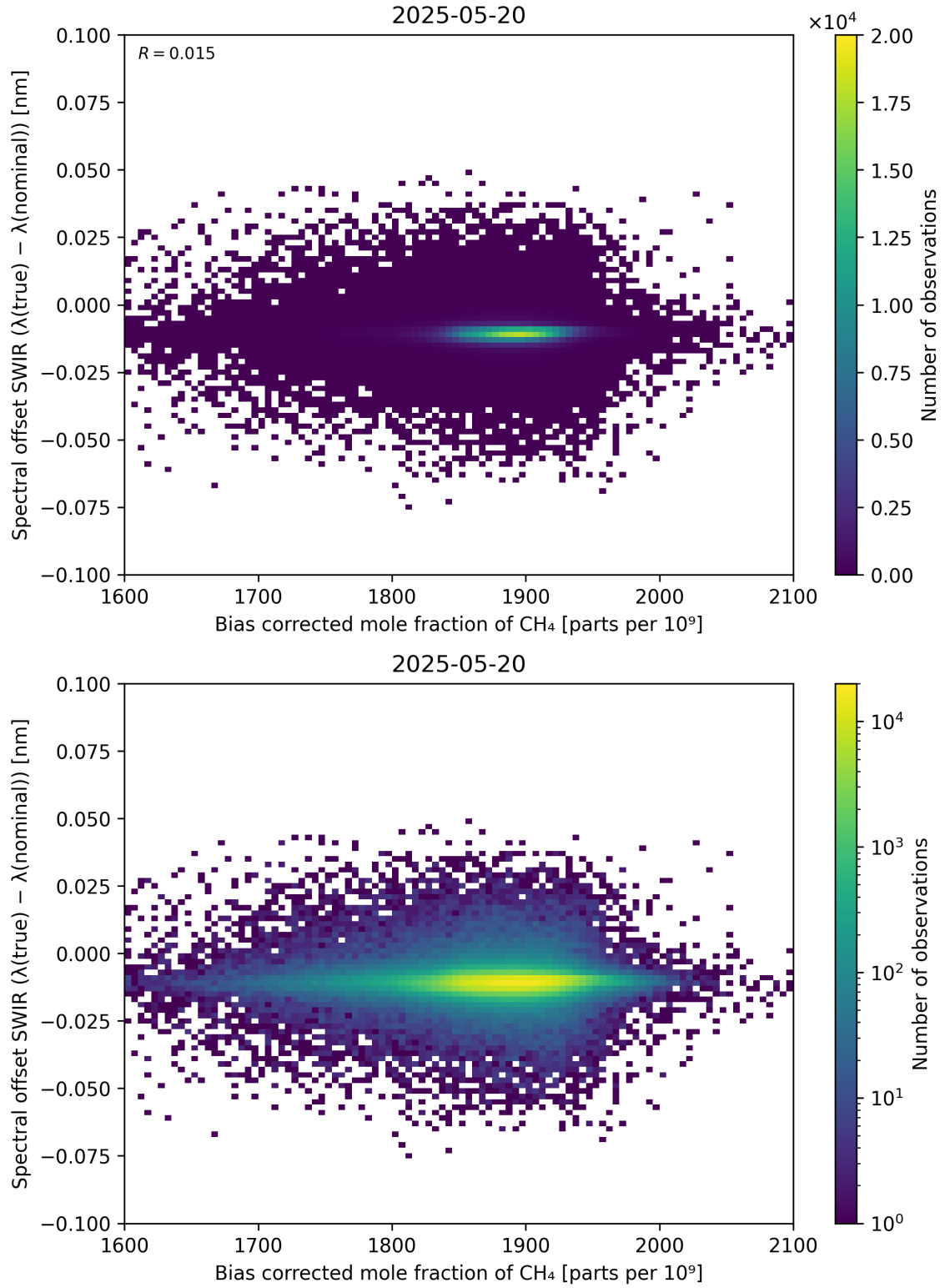
Figure 69: Scatter density plot of “Bias corrected mole fraction of \text{CH}_4 ” against “Spectral offset SWIR ( \lambda_{\text{true}} - \lambda_{\text{nominal}} )” for 2025-05-19 to 2025-05-21.
