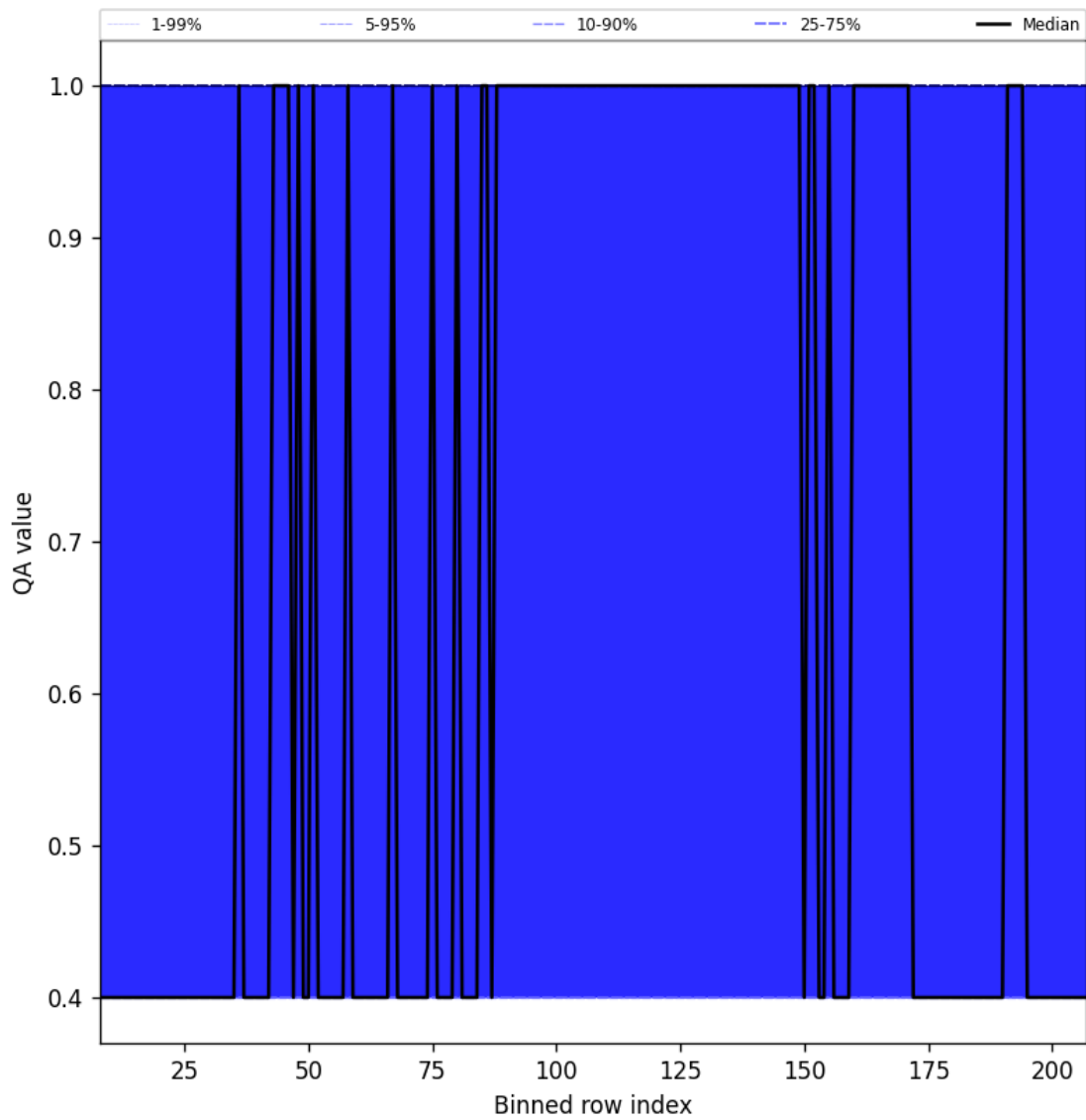
Figure 33: Along track statistics of “QA value” for 2025-05-19 to 2025-05-21
