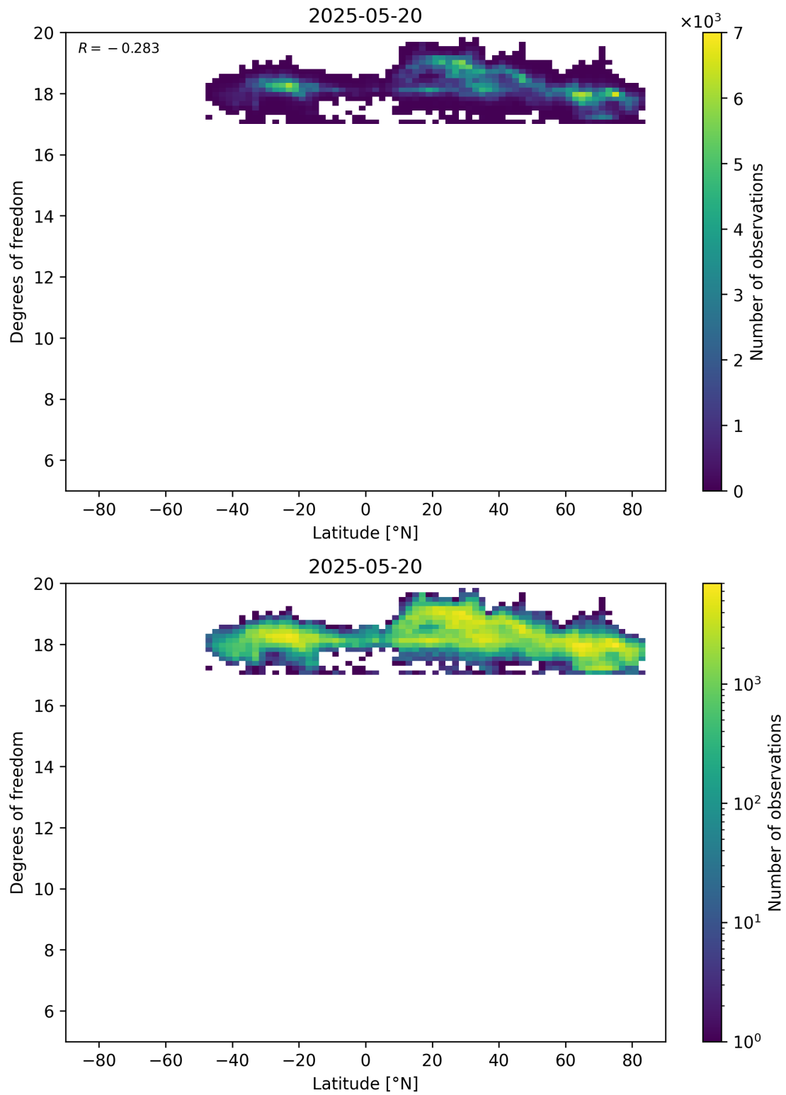
Figure 55: Scatter density plot of “Latitude” against “Degrees of freedom” for 2025-05-19 to 2025-05-21.
