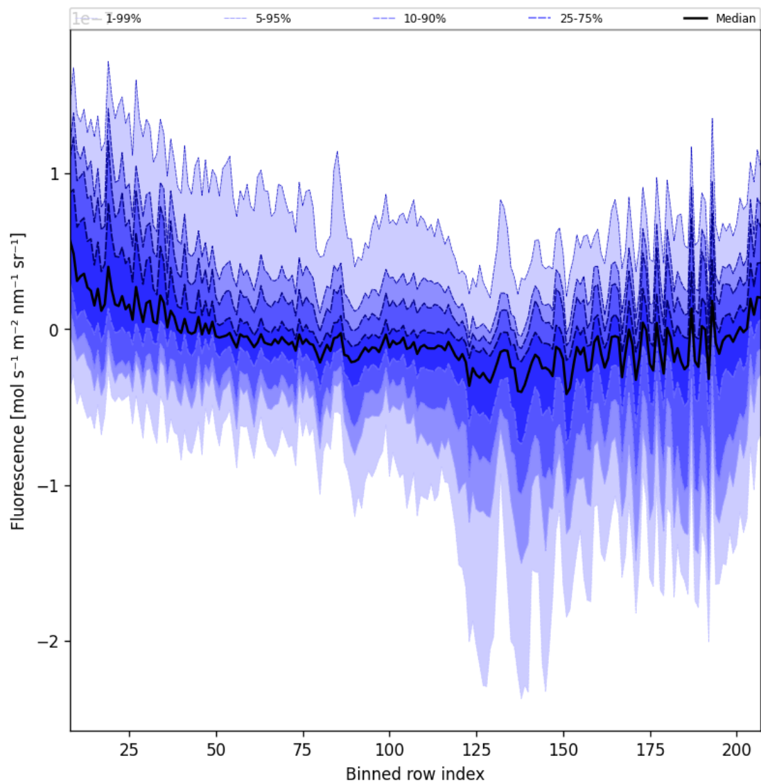
Figure 43: Along track statistics of “Fluorescence” for 2025-05-19 to 2025-05-21
