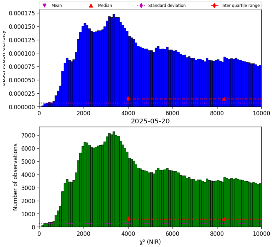
Figure 29: Histogram of “ \chi^2 (NIR)” for 2025-05-19 to 2025-05-21
