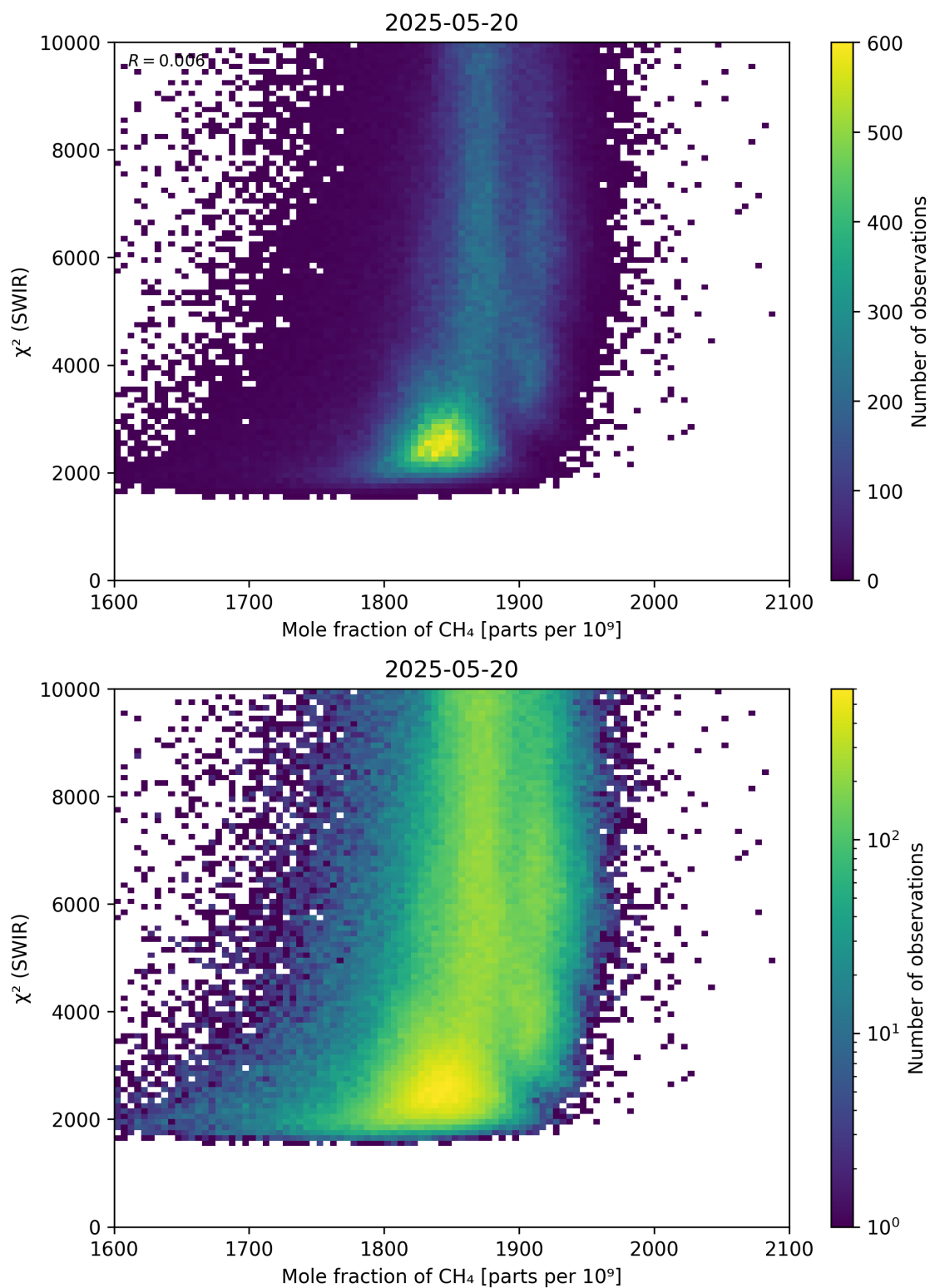
Figure 71: Scatter density plot of “Mole fraction of \text{CH}_4 ” against “ \chi^2 (SWIR)” for 2025-05-19 to 2025-05-21.
