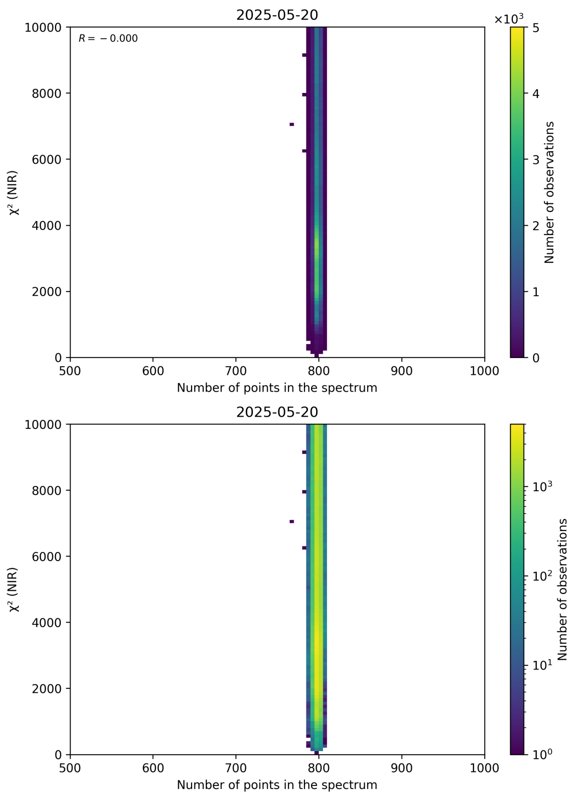
Figure 88: Scatter density plot of “Number of points in the spectrum” against “ \chi^2 (NIR)” for 2025-05-19 to 2025-05-21.
