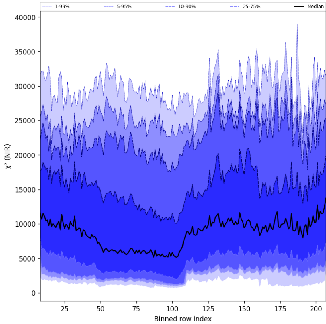
Figure 40: Along track statistics of " \chi^2 (NIR)" for 2025-05-19 to 2025-05-21
