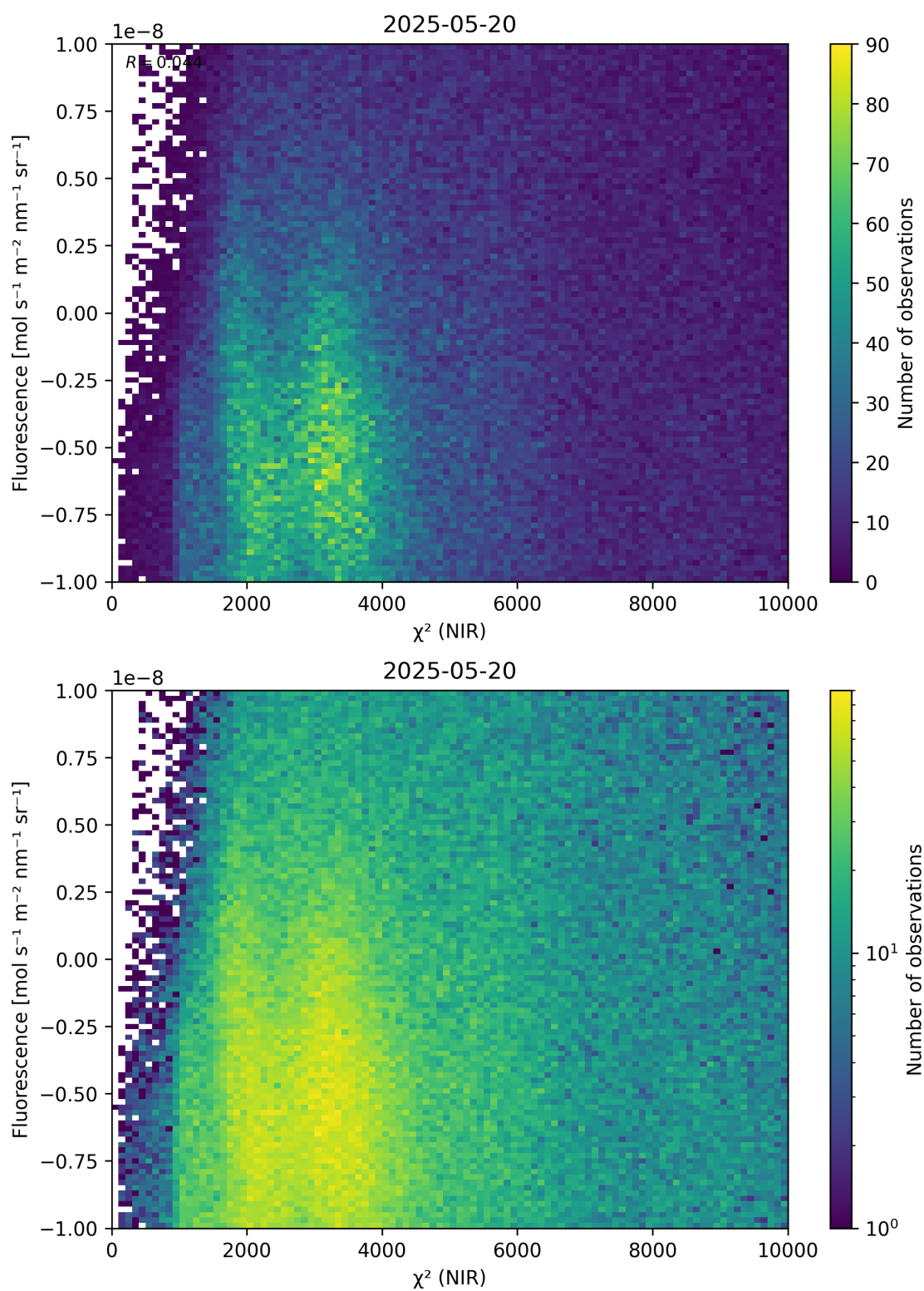
Figure 45: Scatter density plot of “ \chi^2 (NIR)” against “Fluorescence” for 2025-05-19 to 2025-05-21.
