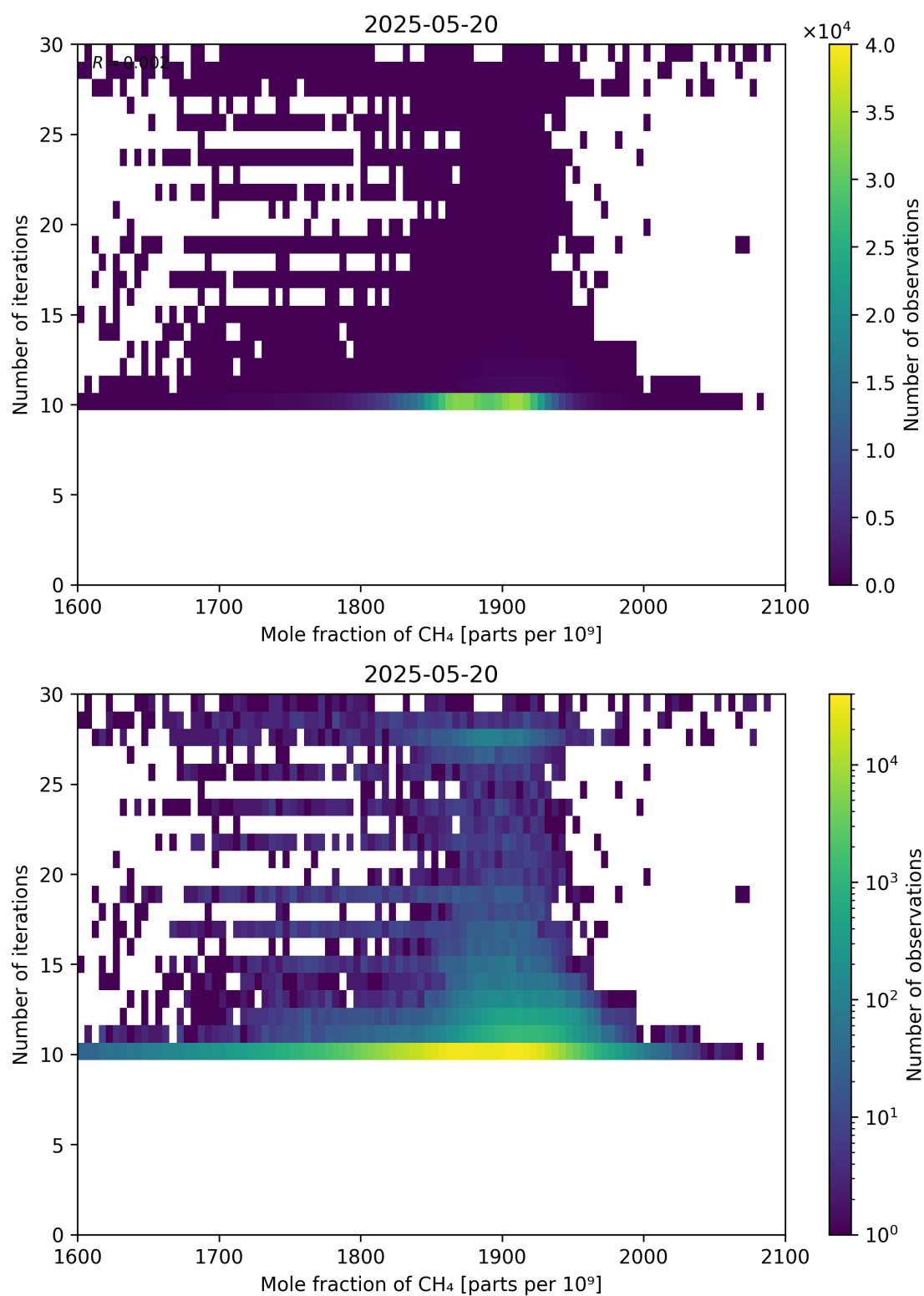
Figure 76: Scatter density plot of “Mole fraction of CH 4 ” against “Number of iterations” for 2025-05-19 to 2025-05-21.
