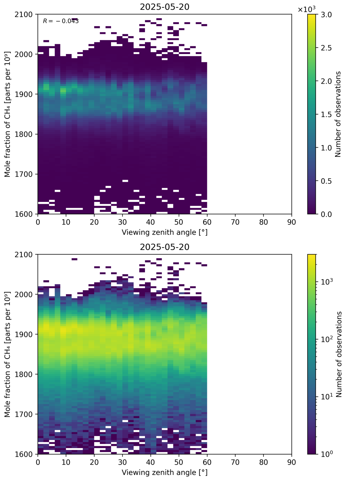
Figure 110: Scatter density plot of “Viewing zenith angle” against “Mole fraction of CH 4 ” for 2025-05-19 to 2025-05-21.
