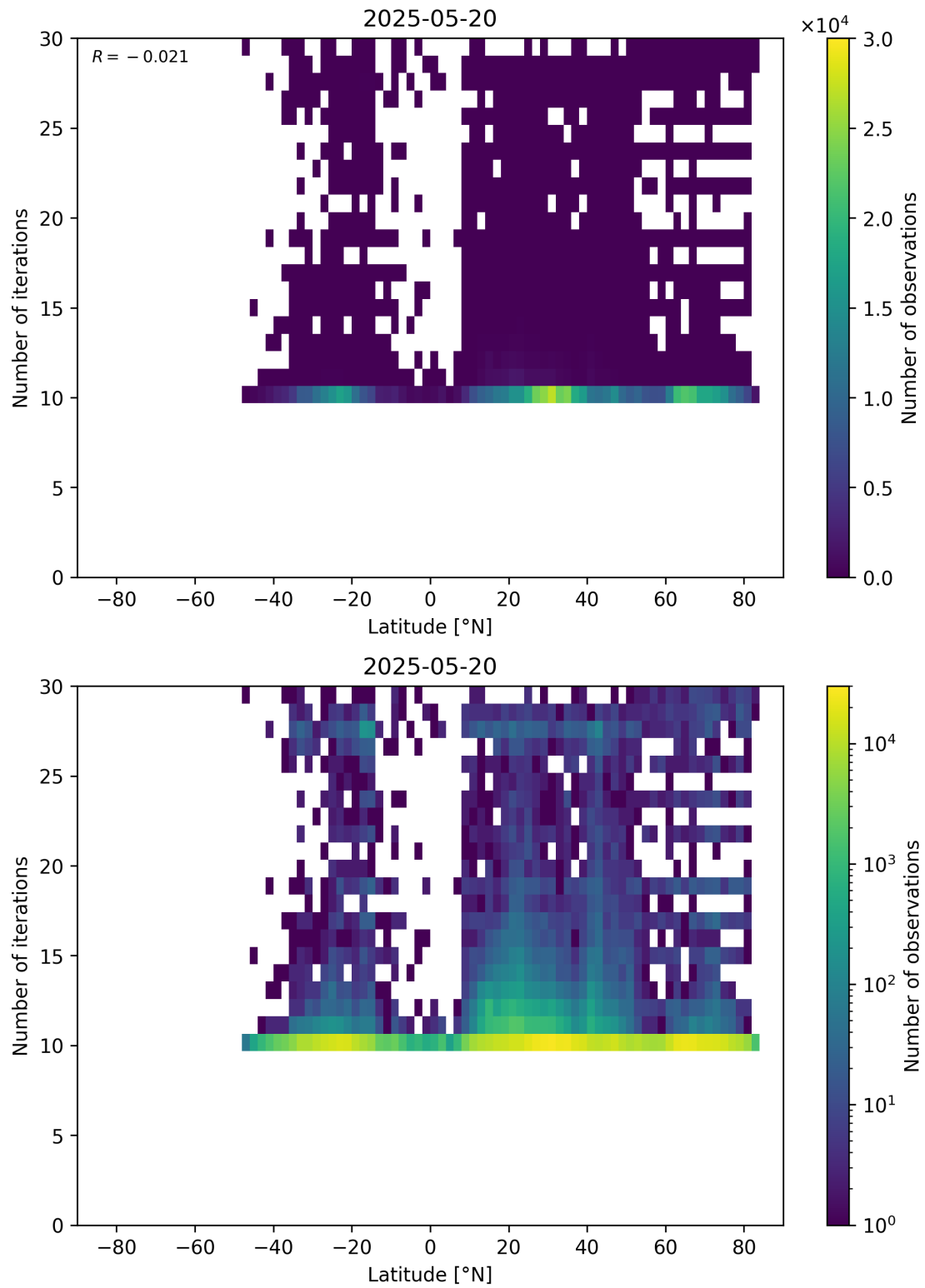
Figure 60: Scatter density plot of “Latitude” against “Number of iterations” for 2025-05-19 to 2025-05-21.
