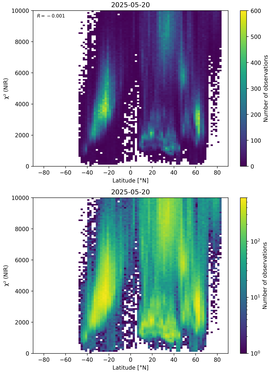
Figure 53: Scatter density plot of “Latitude” against “ \chi^2 (NIR)” for 2025-05-19 to 2025-05-21.
