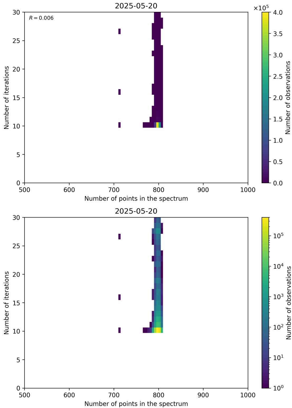
Figure 92: Scatter density plot of “Number of points in the spectrum” against “Number of iterations” for 2025-05-19 to 2025-05-21.
