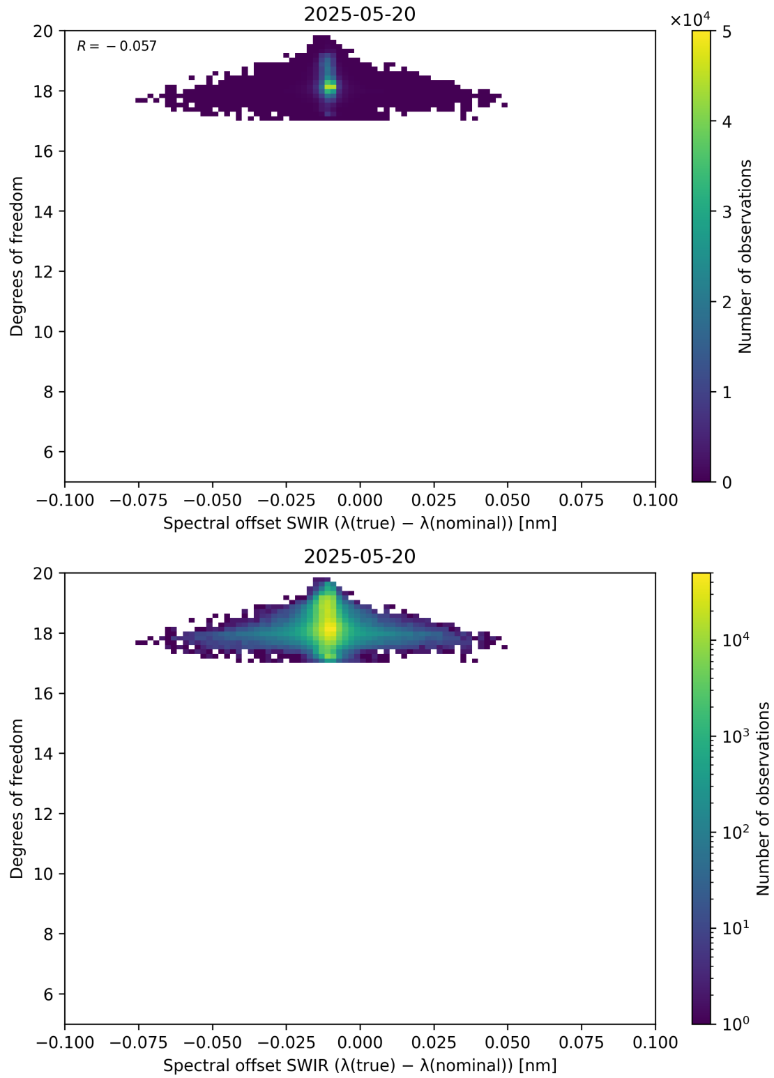
Figure 119: Scatter density plot of “Spectral offset SWIR ( \lambda_{\text{true}} - \lambda_{\text{nominal}} )” against “Degrees of freedom” for 2025-05-19 to 2025-05-21.
