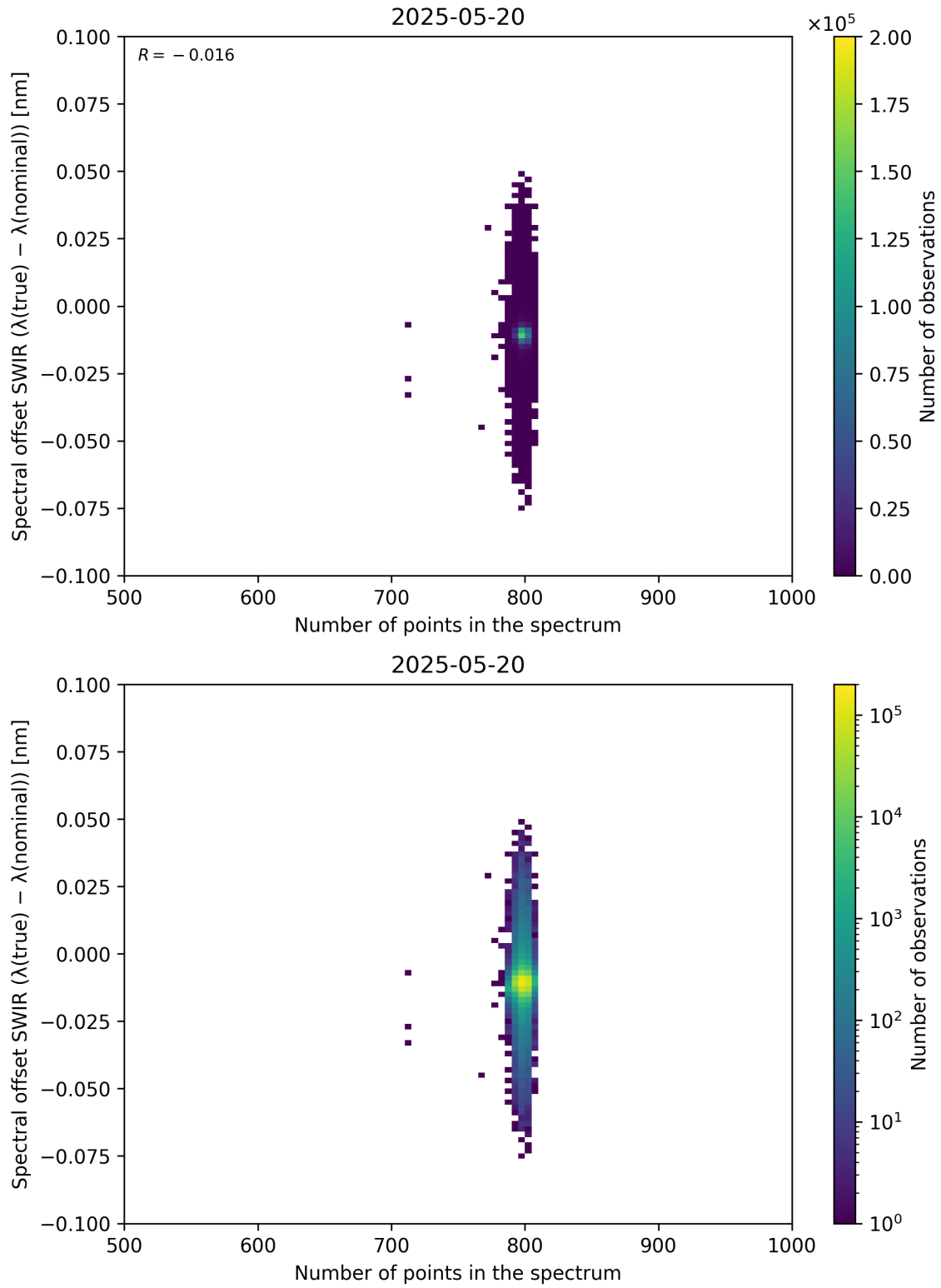
Figure 93: Scatter density plot of “Number of points in the spectrum” against “Spectral offset SWIR ( \lambda_{\text{true}} - \lambda_{\text{nominal}} )” for 2025-05-19 to 2025-05-21.
