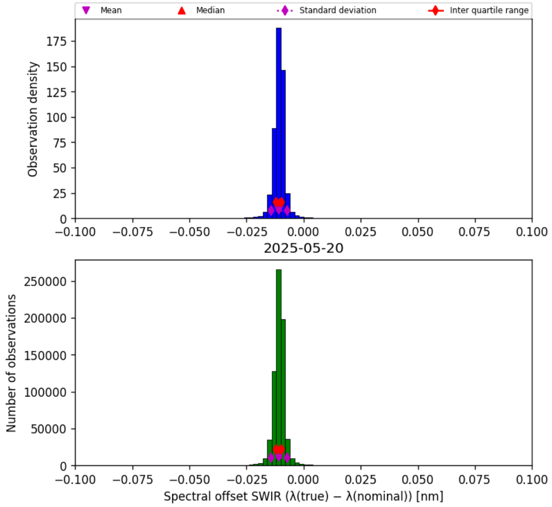
Figure 27: Histogram of “Spectral offset SWIR ( \lambda_{\text{true}} - \lambda_{\text{nominal}} )” for 2025-05-19 to 2025-05-21
