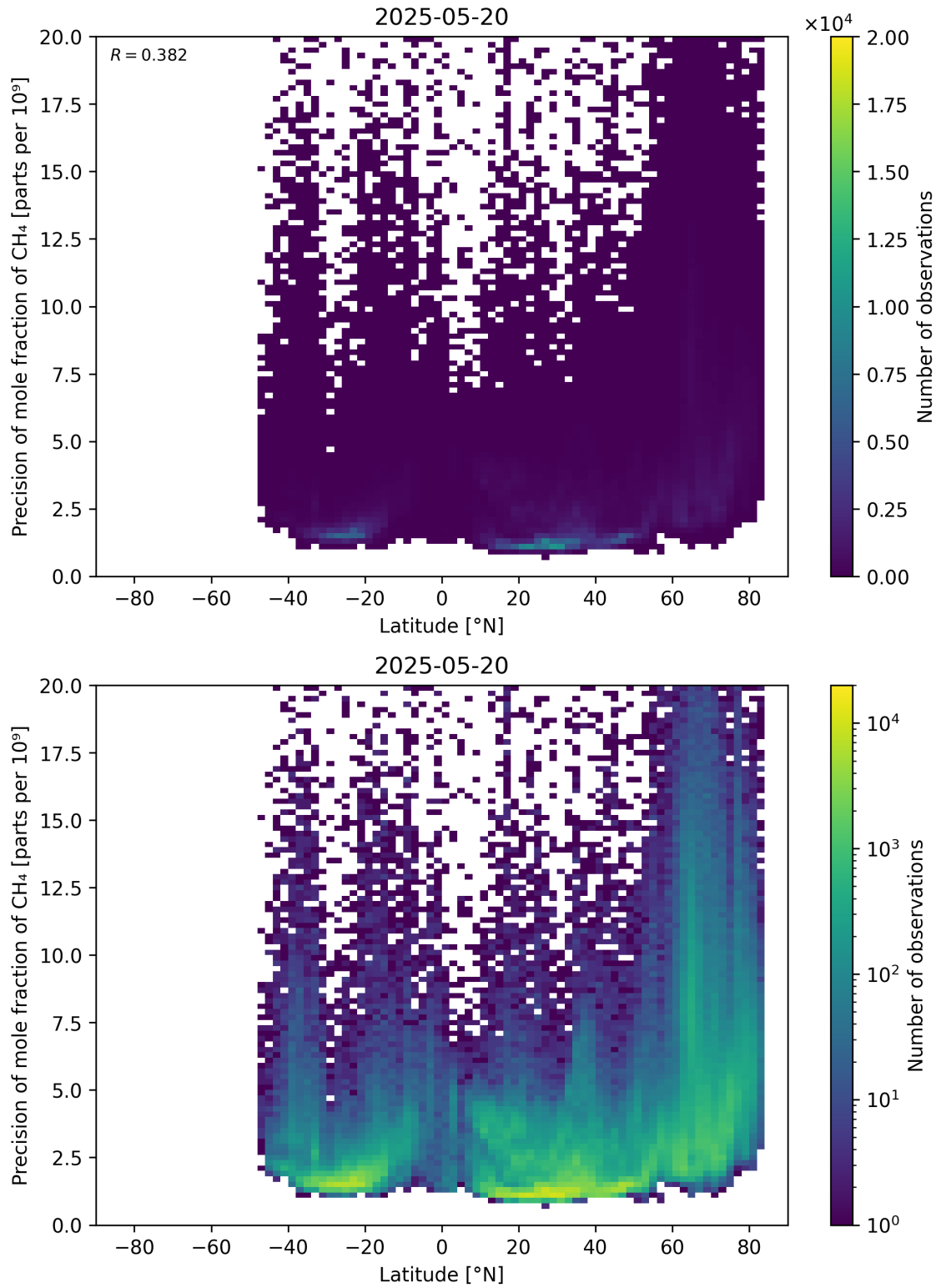
Figure 59: Scatter density plot of “Latitude” against “Precision of mole fraction of \text{CH}_4 ” for 2025-05-19 to 2025-05-21.
