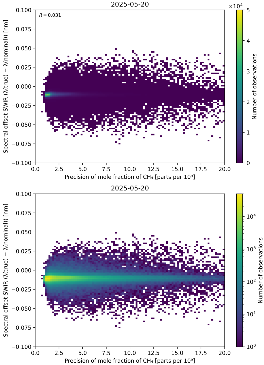
Figure 85: Scatter density plot of “Precision of mole fraction of CH 4 ” against “Spectral offset SWIR ( \lambda_{\text{true}} - \lambda_{\text{nominal}} )” for 2025-05-19 to 2025-05-21.
