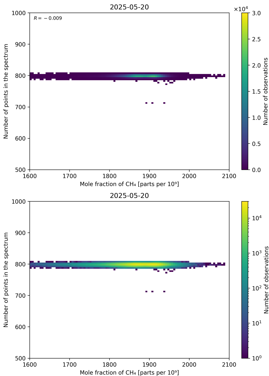
Figure 77: Scatter density plot of “Mole fraction of CH 4 ” against “Number of points in the spectrum” for 2025-05-19 to 2025-05-21.
