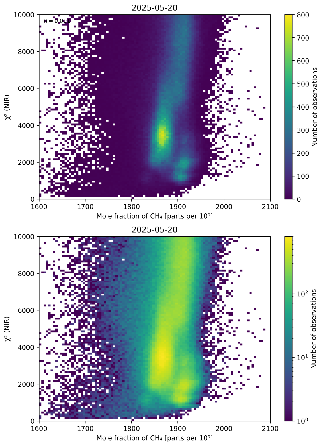
Figure 70: Scatter density plot of “Mole fraction of \text{CH}_4 ” against “ \chi^2 (NIR)” for 2025-05-19 to 2025-05-21.
