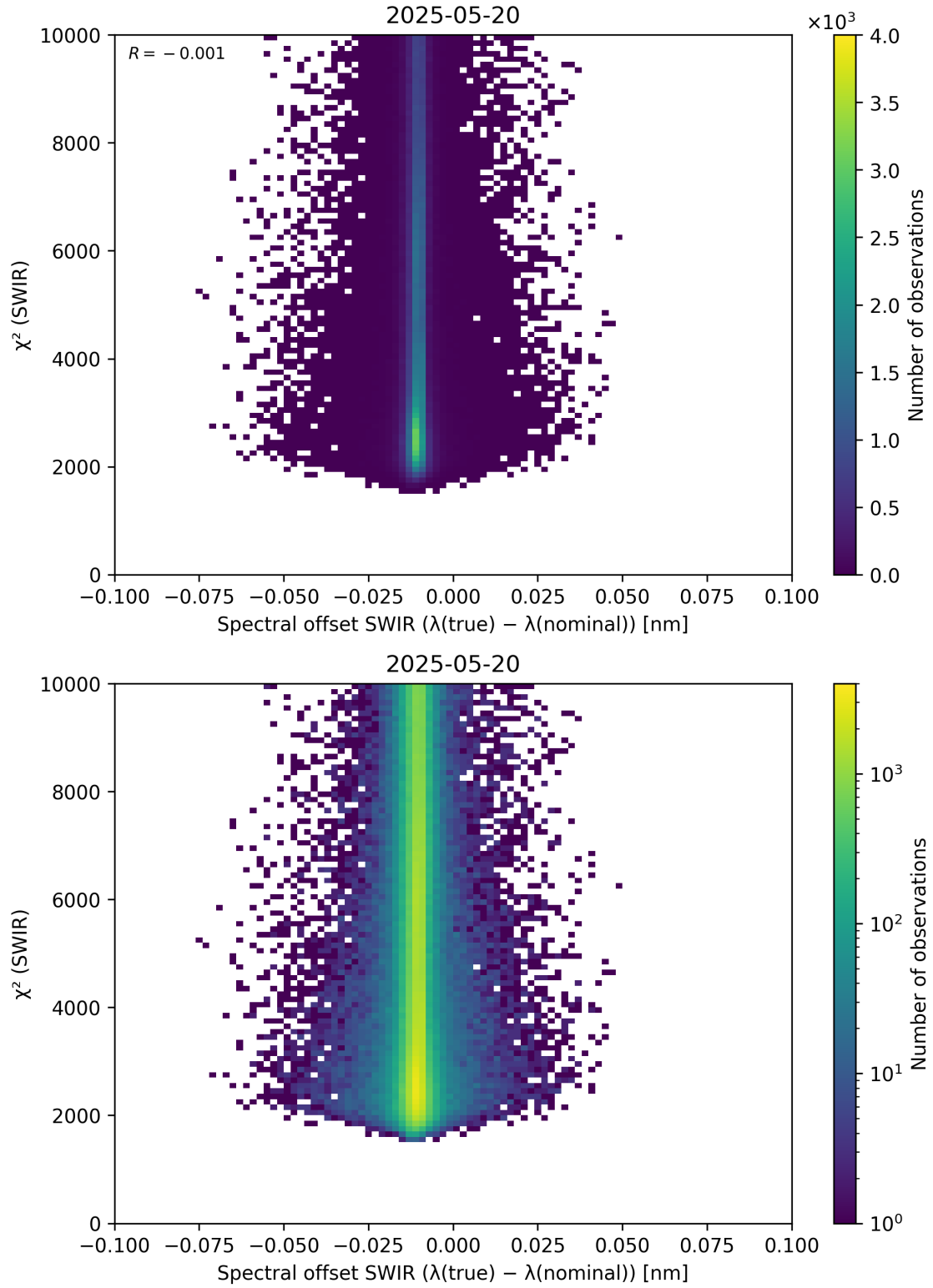
Figure 118: Scatter density plot of “Spectral offset SWIR ( \lambda_{\text{true}} - \lambda_{\text{nominal}} )” against “ \chi^2 (SWIR)” for 2025-05-19 to 2025-05-21.
