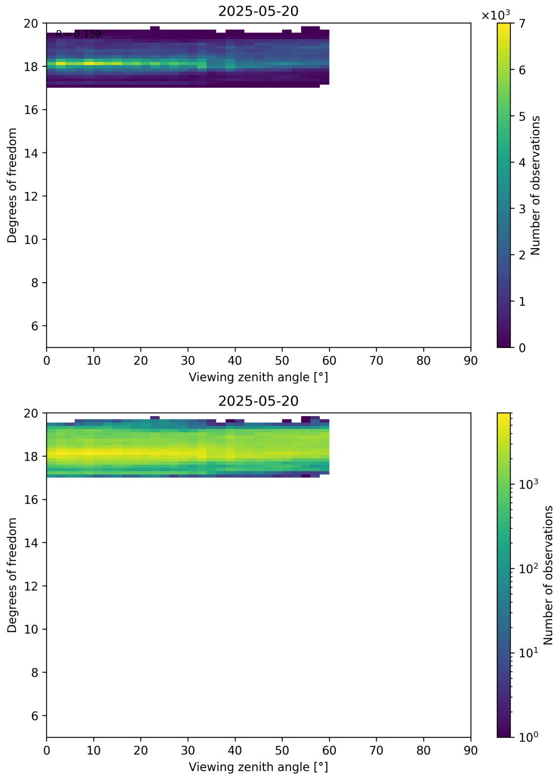
Figure 107: Scatter density plot of “Viewing zenith angle” against “Degrees of freedom” for 2025-05-19 to 2025-05-21.
