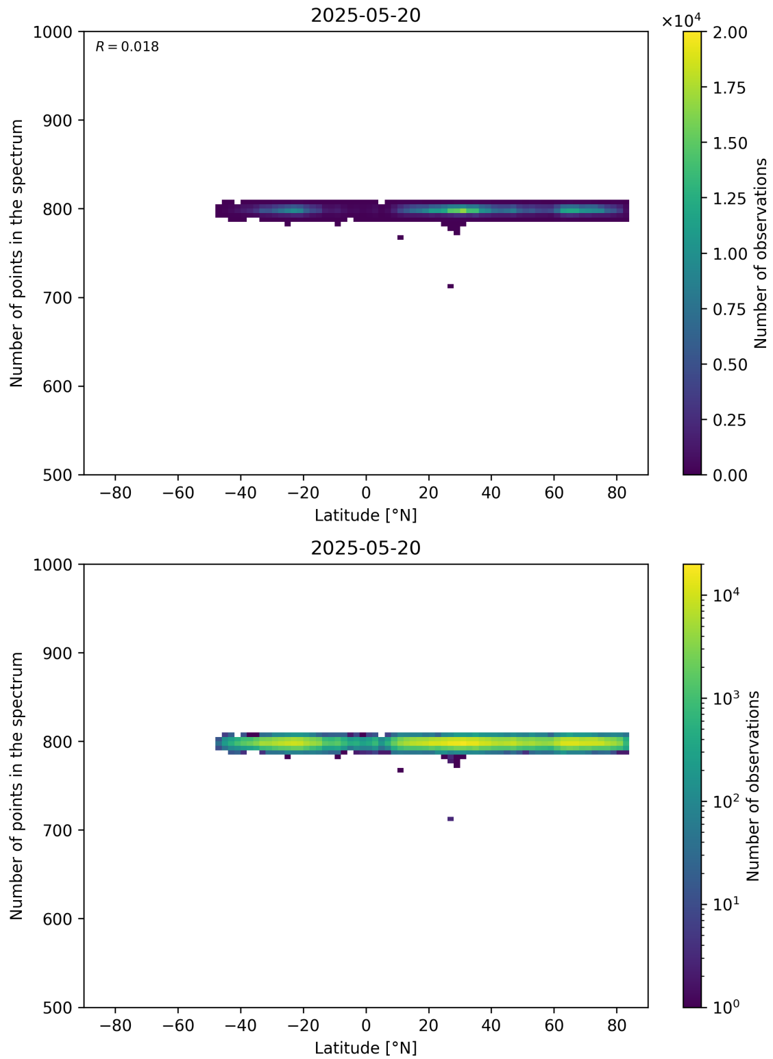
Figure 61: Scatter density plot of “Latitude” against “Number of points in the spectrum” for 2025-05-19 to 2025-05-21.
