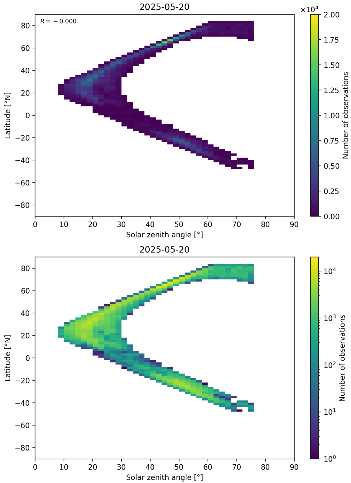
Figure 98: Scatter density plot of “Solar zenith angle” against “Latitude” for 2025-05-19 to 2025-05-21.
