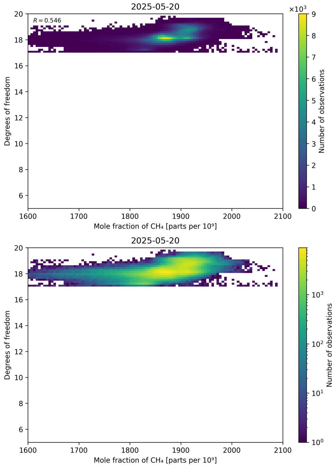
Figure 72: Scatter density plot of “Mole fraction of CH 4 ” against “Degrees of freedom” for 2025-05-19 to 2025-05-21.
