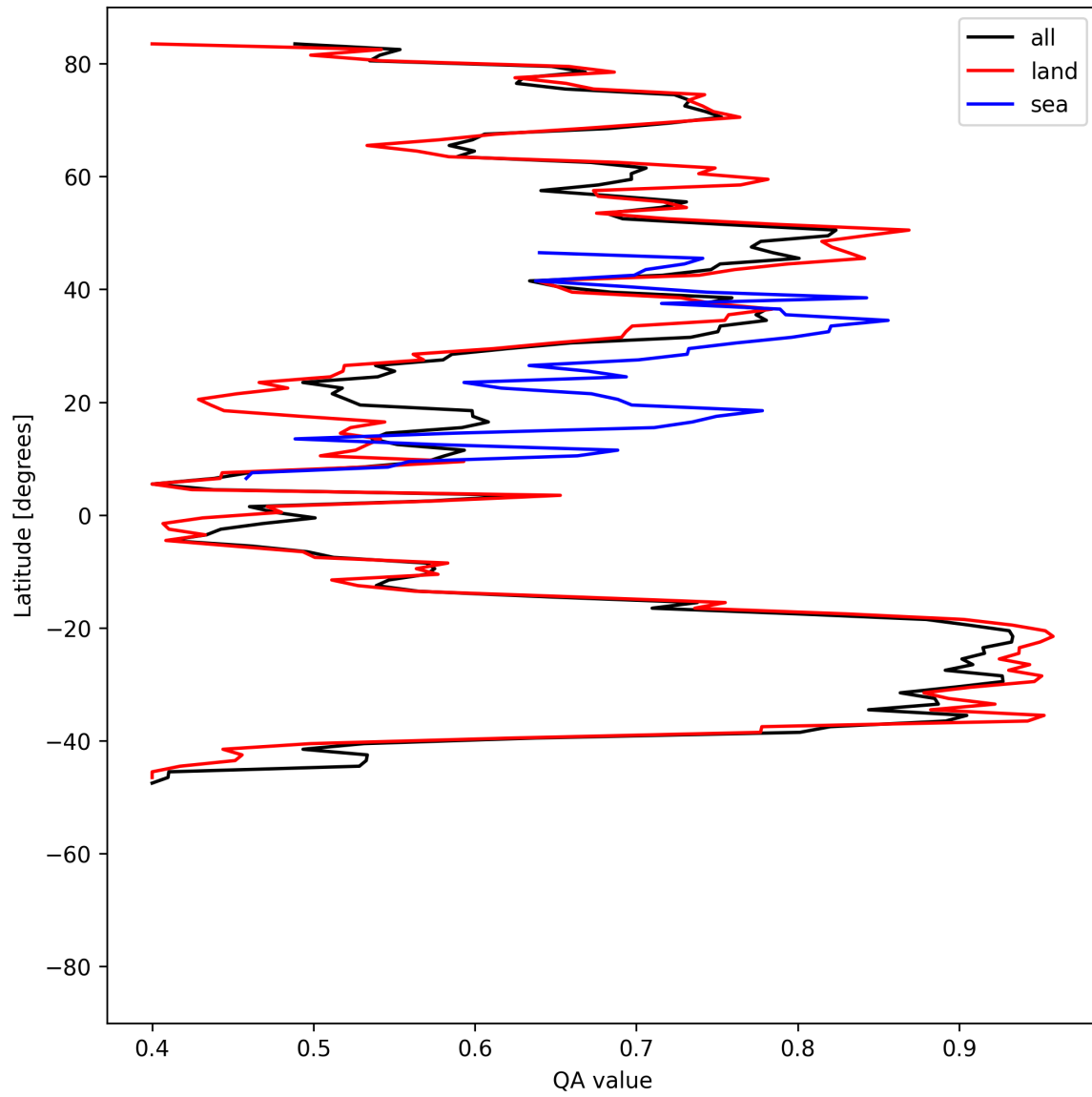
Figure 11: Zonal average of “QA value” for 2025-05-19 to 2025-05-21.
