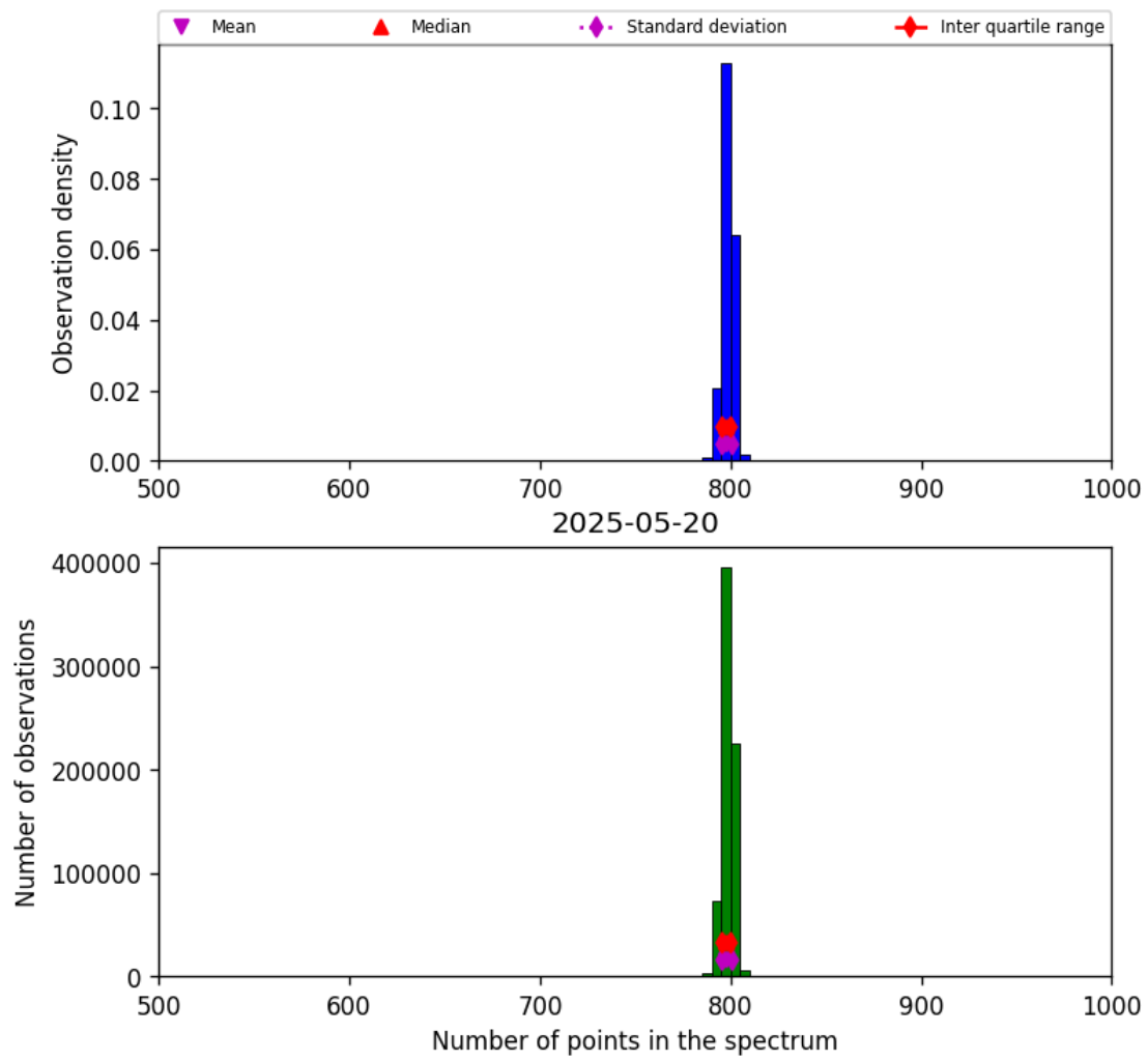
Figure 26: Histogram of “Number of points in the spectrum” for 2025-05-19 to 2025-05-21
