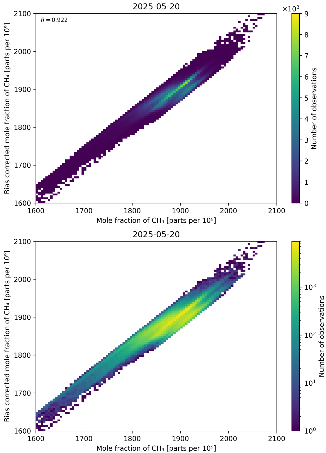
Figure 74: Scatter density plot of “Mole fraction of CH 4 ” against “Bias corrected mole fraction of CH 4 ” for 2025-05-19 to 2025-05-21.
