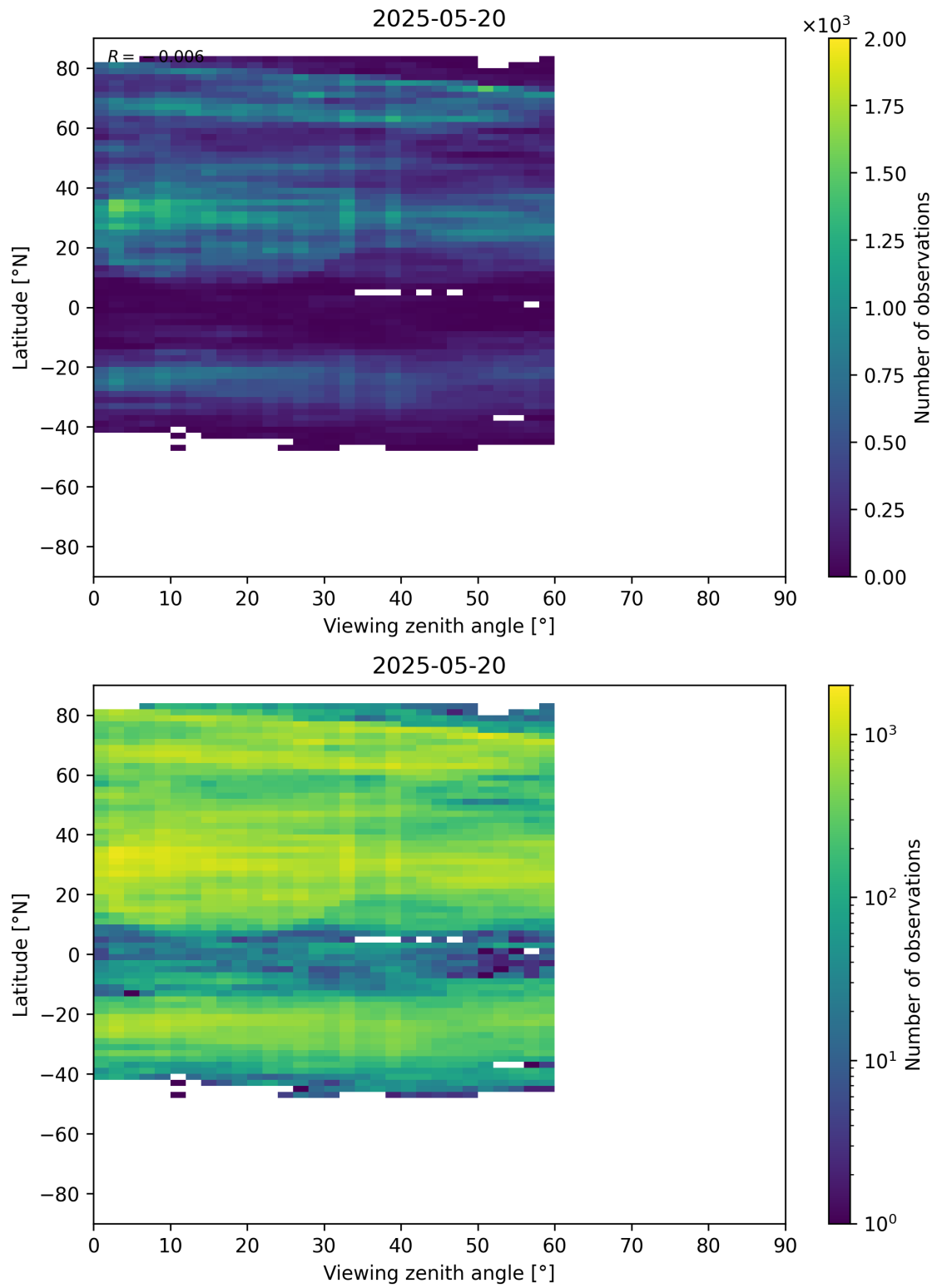
Figure 109: Scatter density plot of “Viewing zenith angle” against “Latitude” for 2025-05-19 to 2025-05-21.
