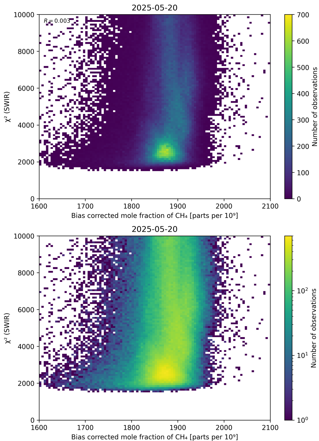
Figure 64: Scatter density plot of “Bias corrected mole fraction of \text{CH}_4 ” against “ \chi^2 (SWIR)” for 2025-05-19 to 2025-05-21.
