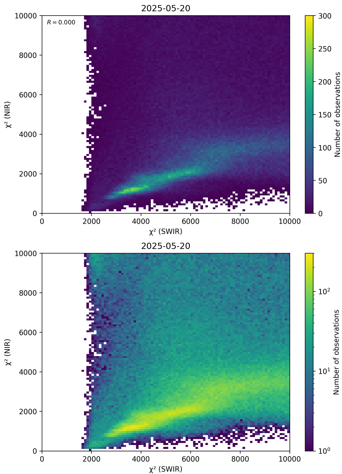
Figure 47: Scatter density plot of “ \chi^2 (SWIR)” against “ \chi^2 (NIR)” for 2025-05-19 to 2025-05-21.
