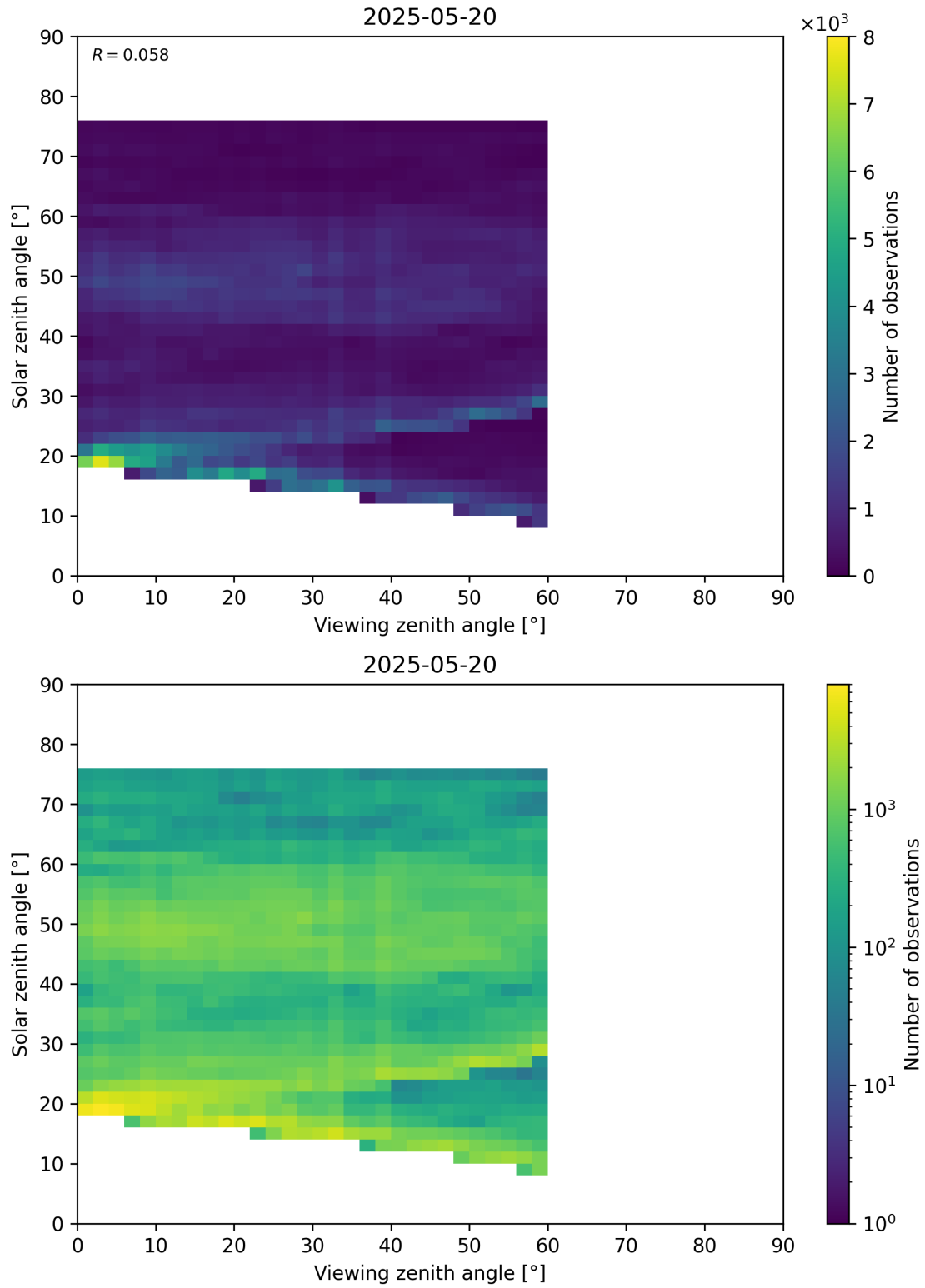
Figure 115: Scatter density plot of “Viewing zenith angle” against “Solar zenith angle” for 2025-05-19 to 2025-05-21.
