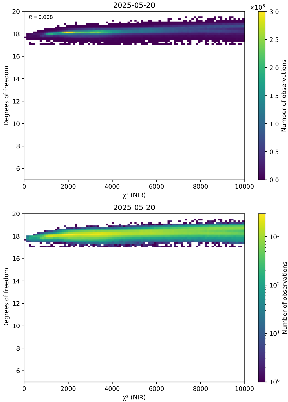
Figure 44: Scatter density plot of “ \chi^2 (NIR)” against “Degrees of freedom” for 2025-05-19 to 2025-05-21.
