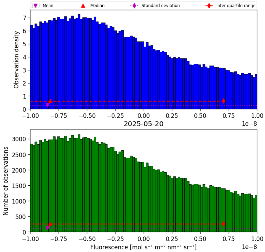
Figure 32: Histogram of “Fluorescence” for 2025-05-19 to 2025-05-21
