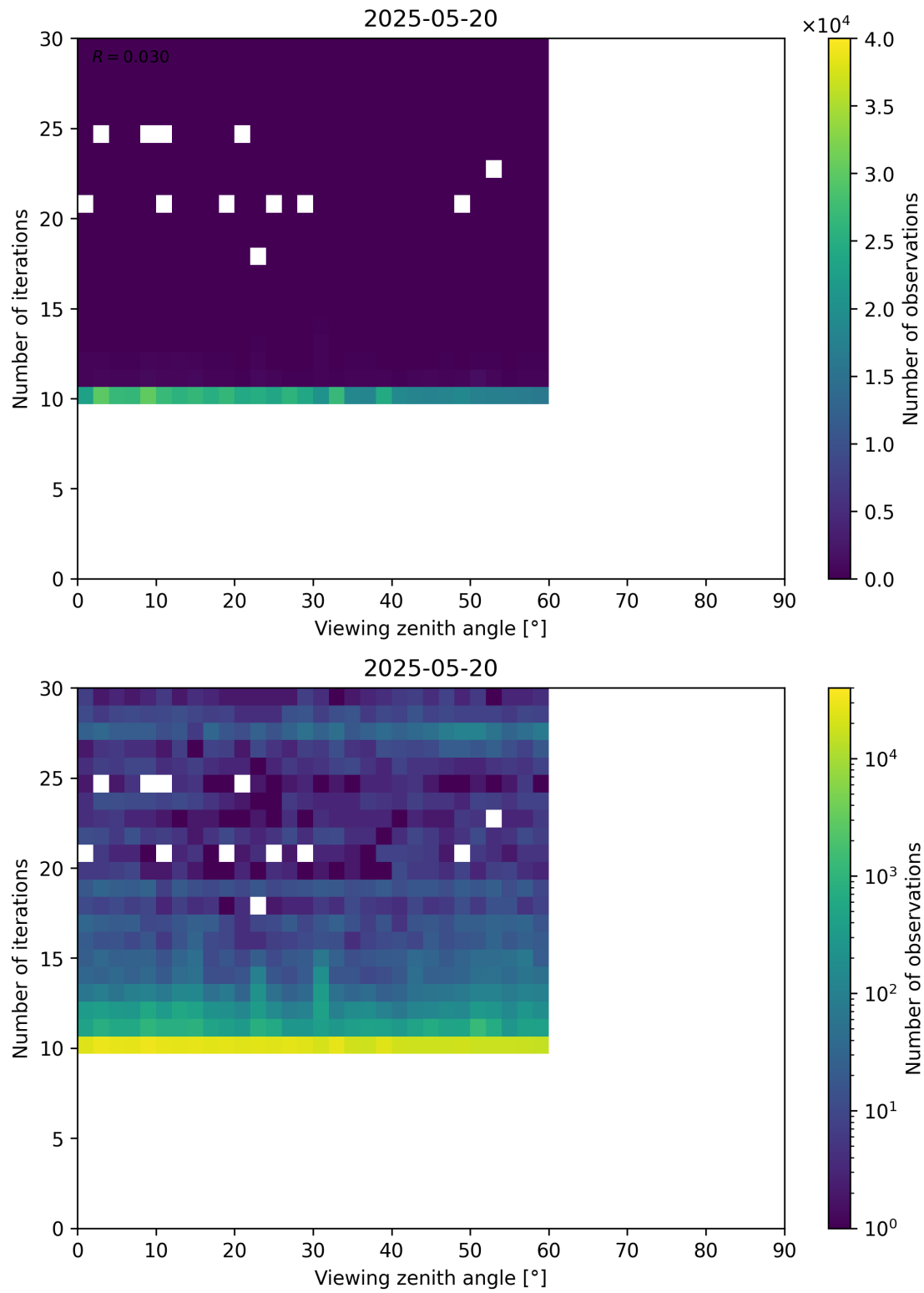
Figure 113: Scatter density plot of “Viewing zenith angle” against “Number of iterations” for 2025-05-19 to 2025-05-21.
