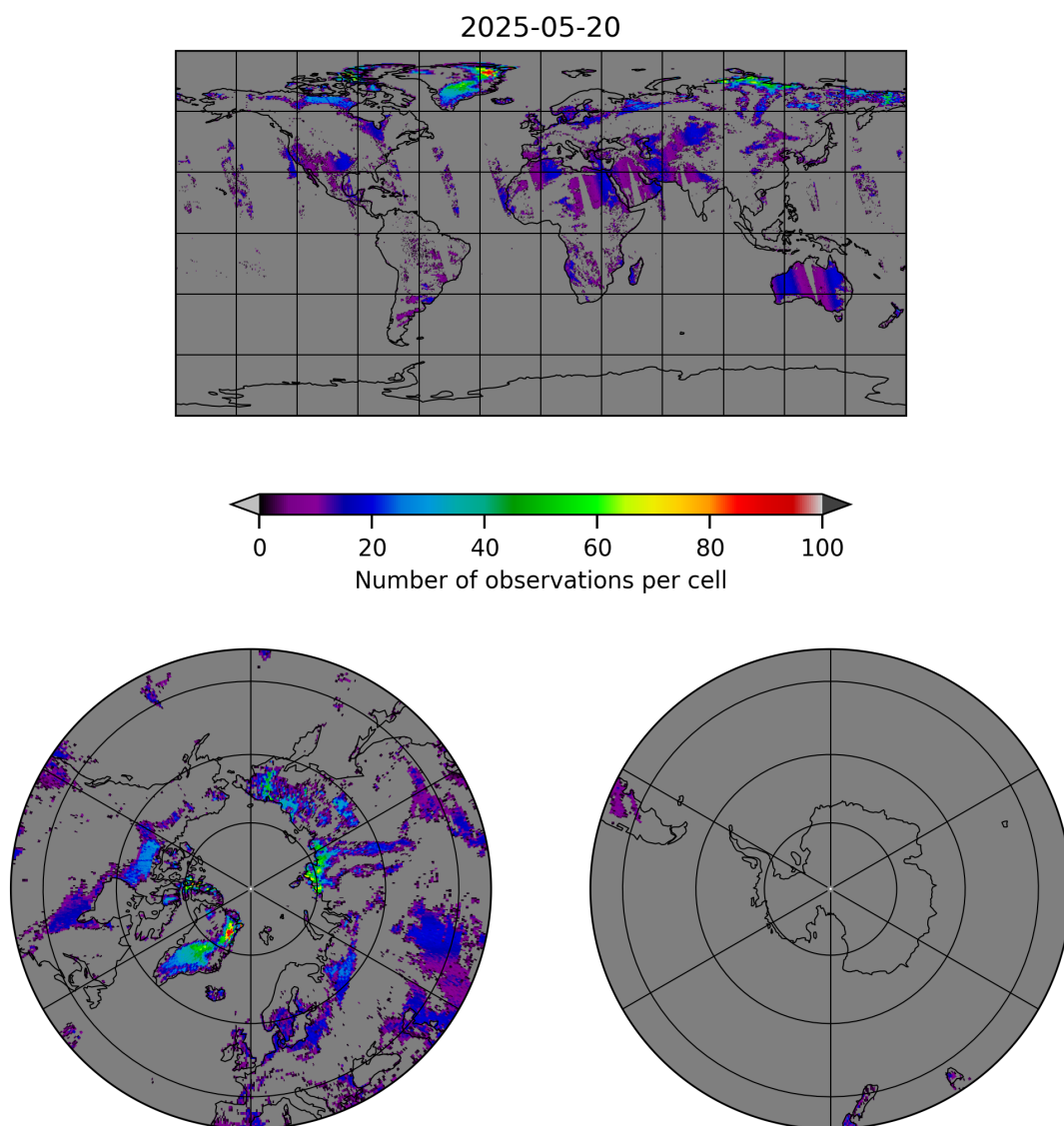
Figure 10: Map of the number of observations for 2025-05-19 to 2025-05-21
