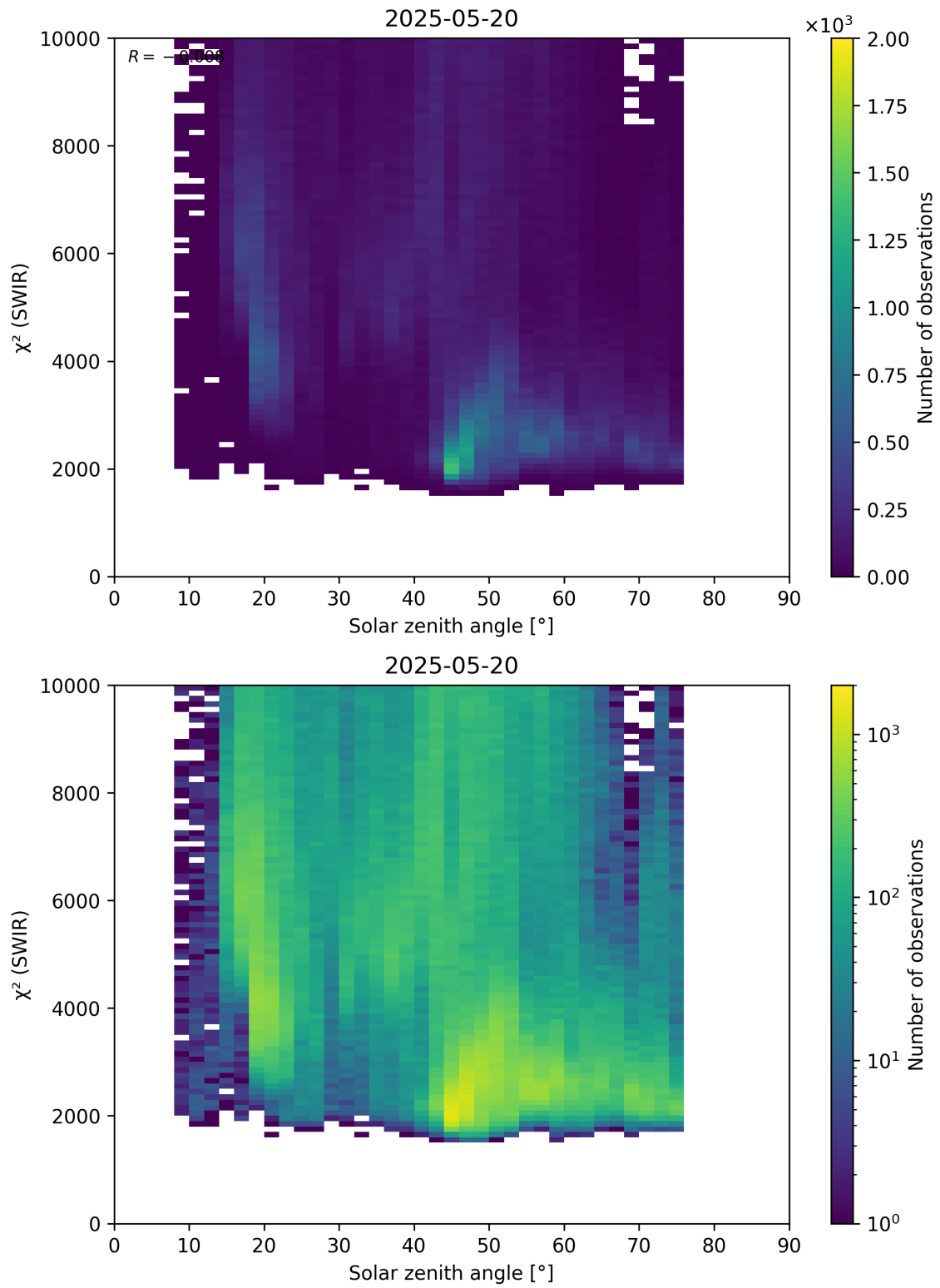
Figure 95: Scatter density plot of “Solar zenith angle” against “ \chi^2 (SWIR)” for 2025-05-19 to 2025-05-21.
