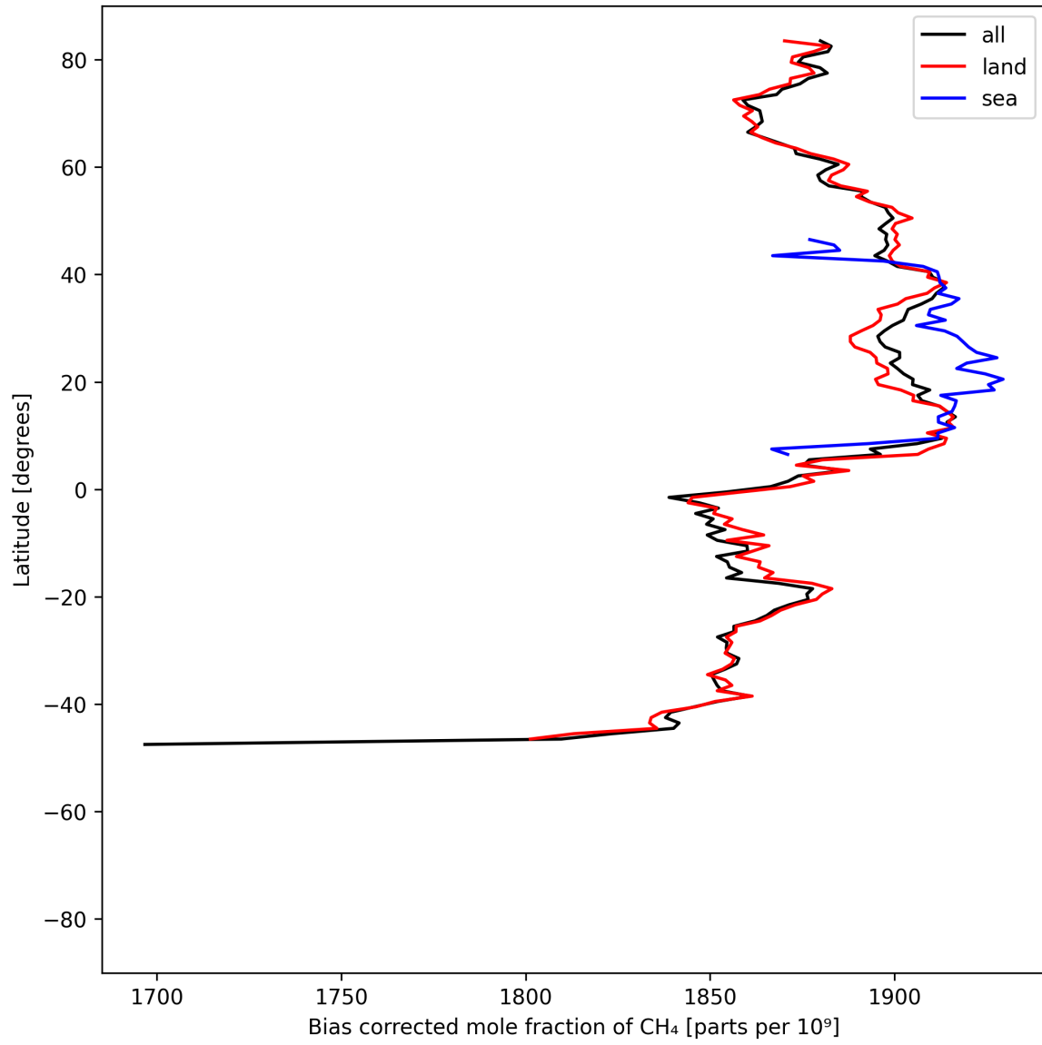
Figure 14: Zonal average of “Bias corrected mole fraction of \text{CH}_4 ” for 2025-05-19 to 2025-05-21.
