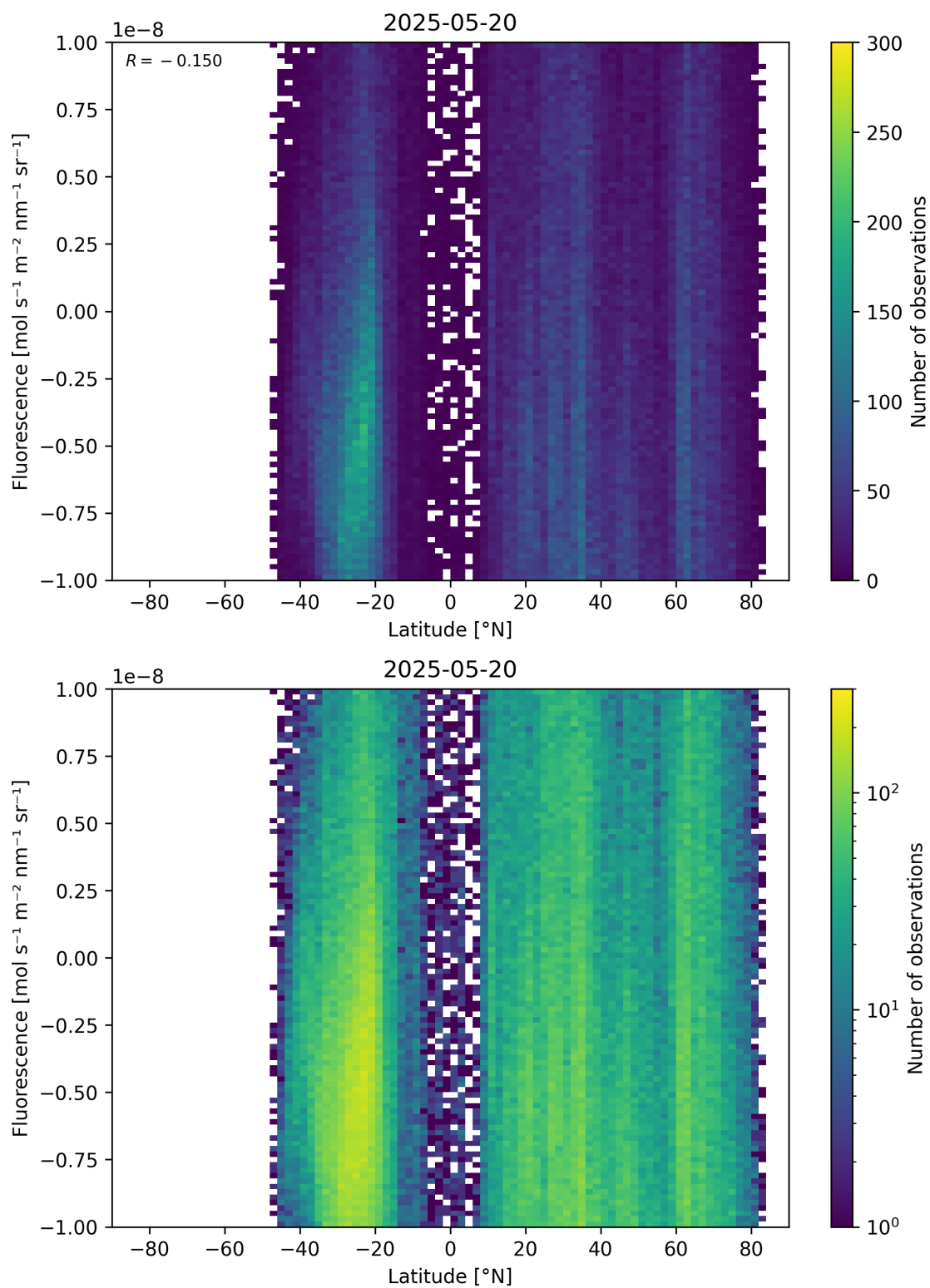
Figure 56: Scatter density plot of “Latitude” against “Fluorescence” for 2025-05-19 to 2025-05-21.
