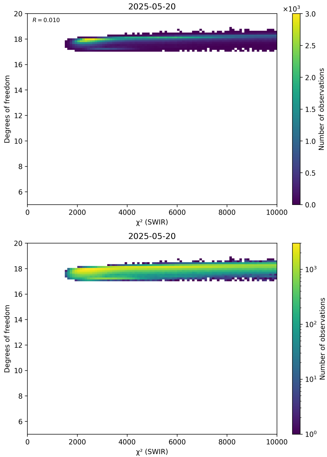
Figure 48: Scatter density plot of “ \chi^2 (SWIR)” against “Degrees of freedom” for 2025-05-19 to 2025-05-21.
