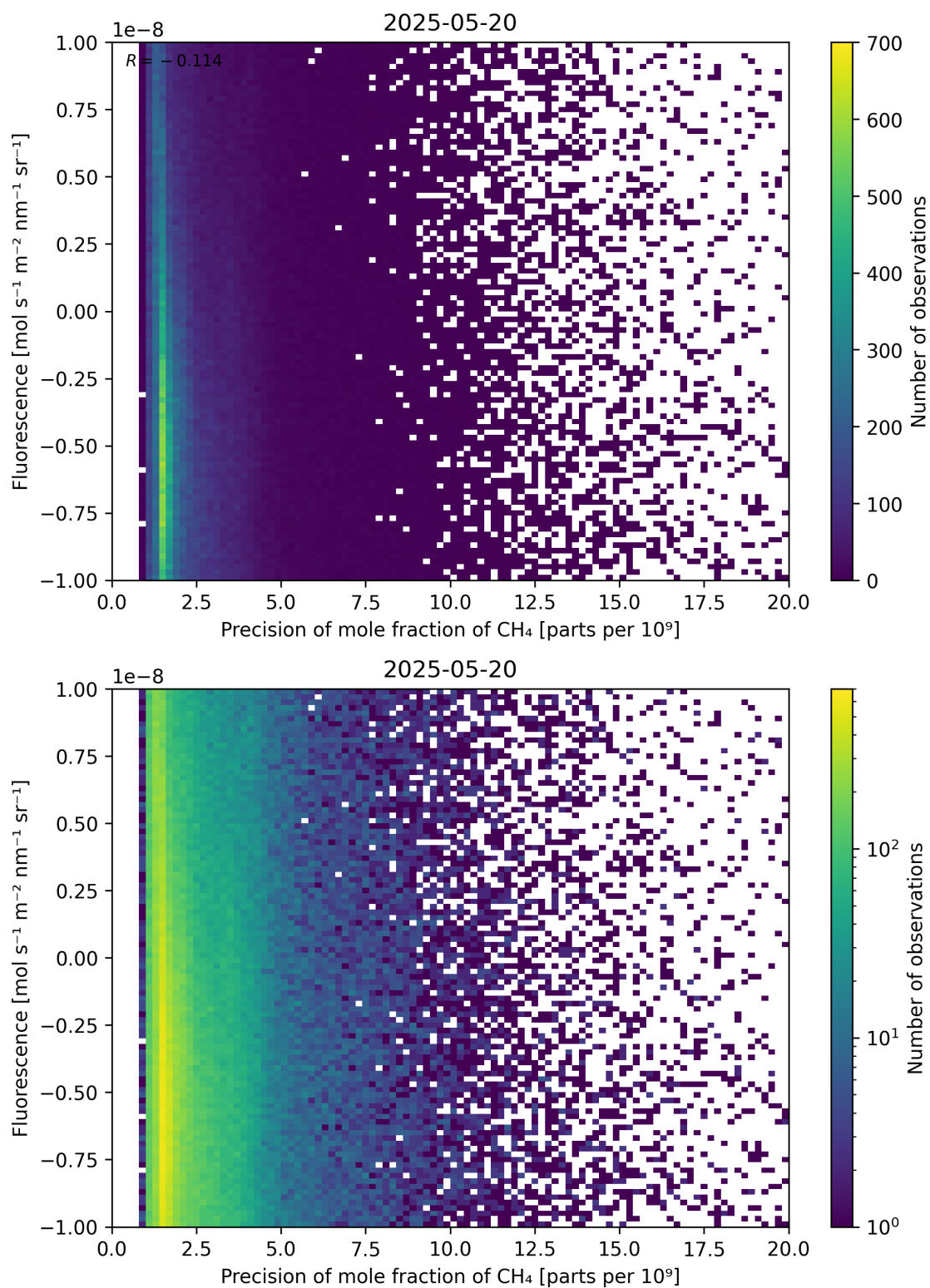
Figure 81: Scatter density plot of “Precision of mole fraction of \text{CH}_4 ” against “Fluorescence” for 2025-05-19 to 2025-05-21.
