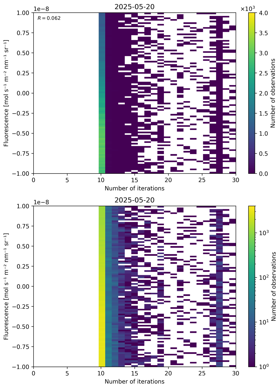
Figure 87: Scatter density plot of “Number of iterations” against “Fluorescence” for 2025-05-19 to 2025-05-21.
