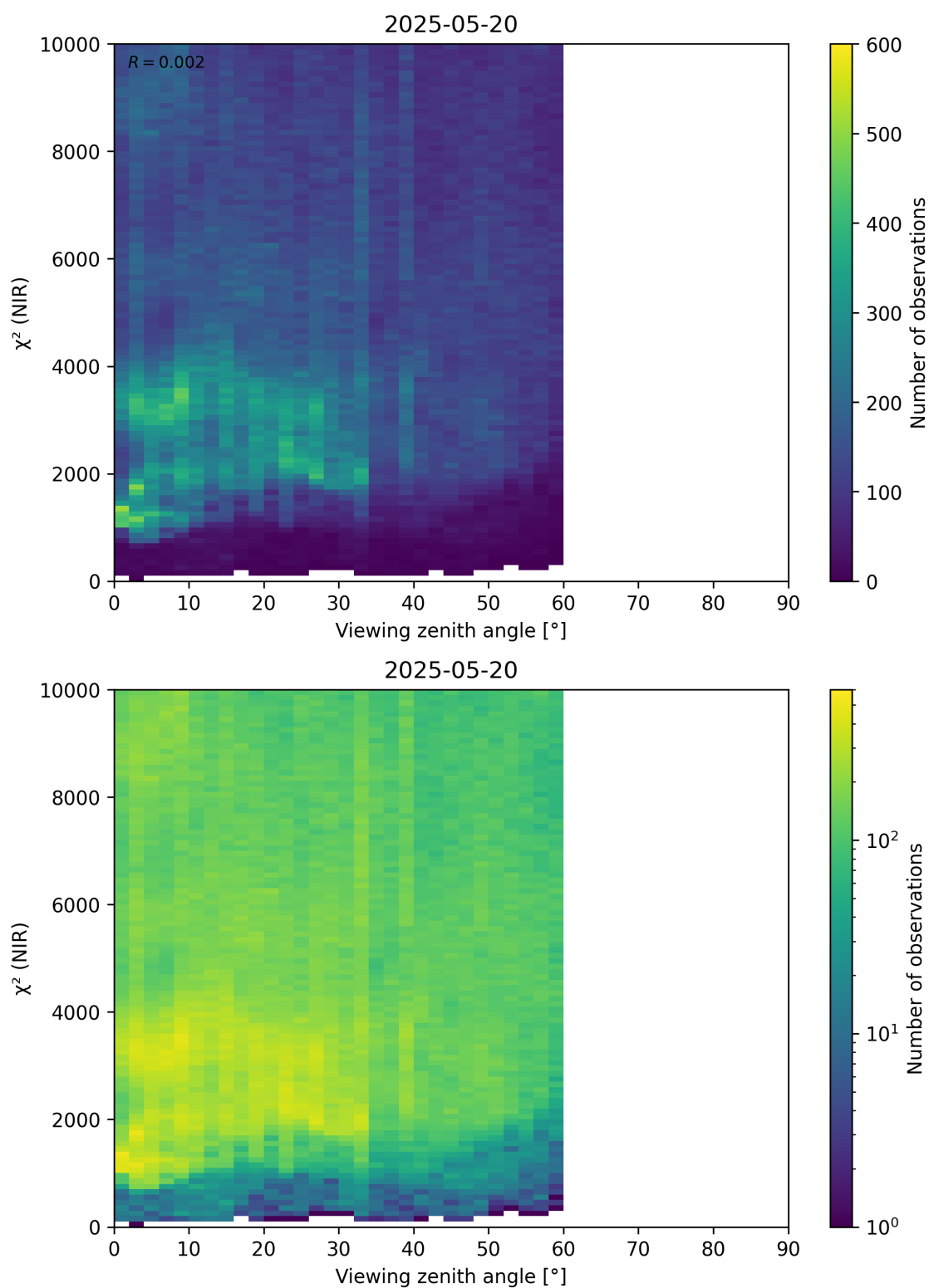
Figure 105: Scatter density plot of “Viewing zenith angle” against “ \chi^2 (NIR)” for 2025-05-19 to 2025-05-21.
