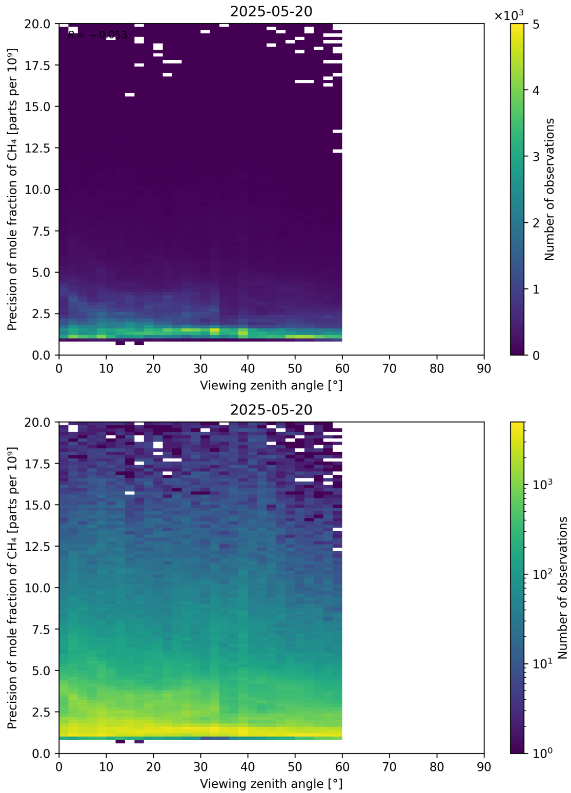
Figure 112: Scatter density plot of “Viewing zenith angle” against “Precision of mole fraction of CH 4 ” for 2025-05-19 to 2025-05-21.
