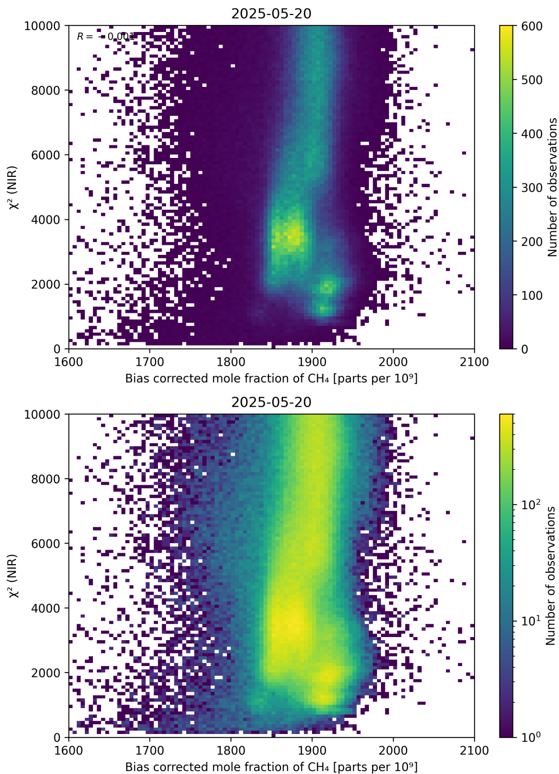
Figure 63: Scatter density plot of “Bias corrected mole fraction of \text{CH}_4 ” against “ \chi^2 (NIR)” for 2025-05-19 to 2025-05-21.
