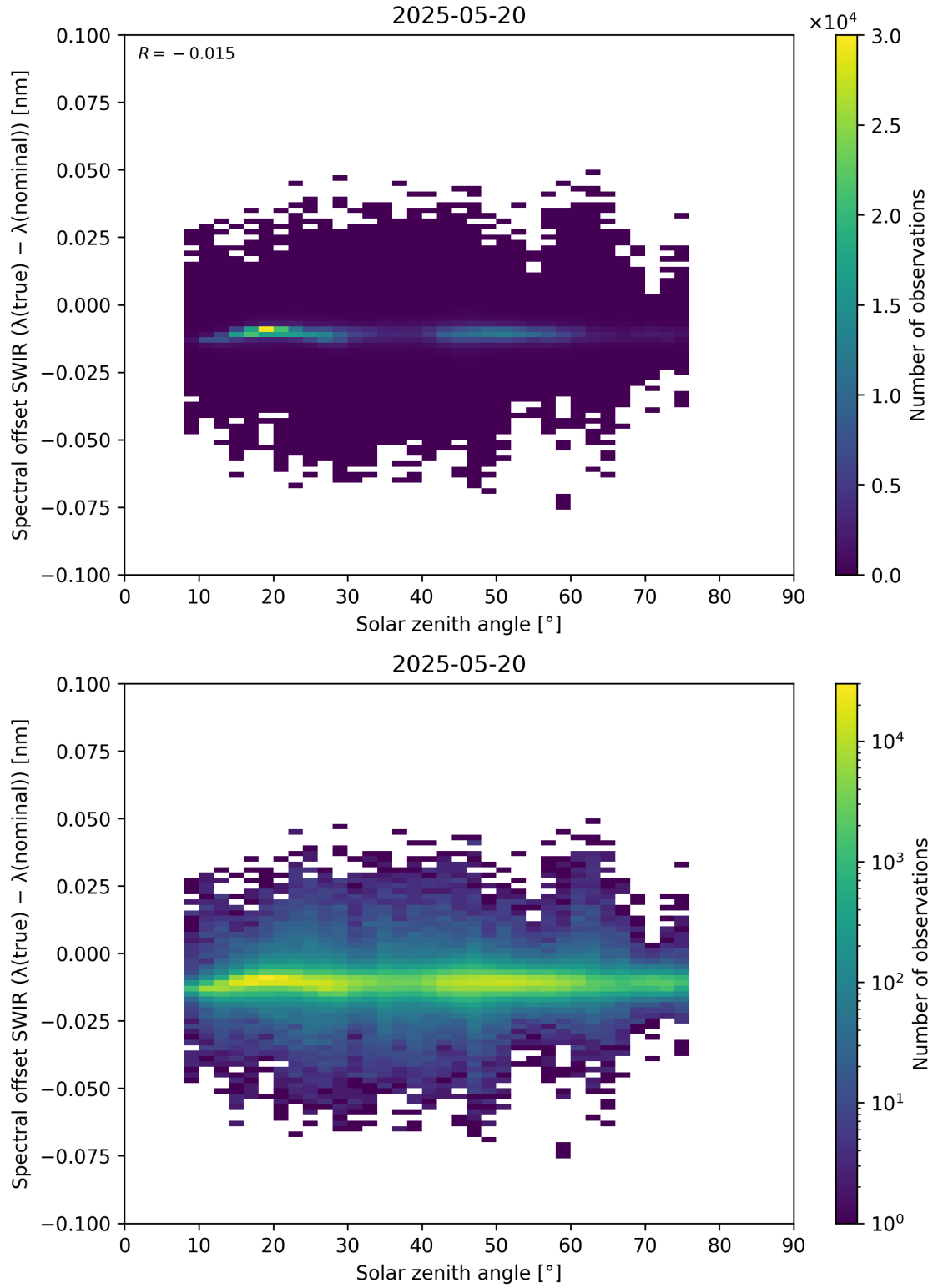
Figure 104: Scatter density plot of “Solar zenith angle” against “Spectral offset SWIR ( \lambda_{\text{true}} - \lambda_{\text{nominal}} )” for 2025-05-19 to 2025-05-21.
