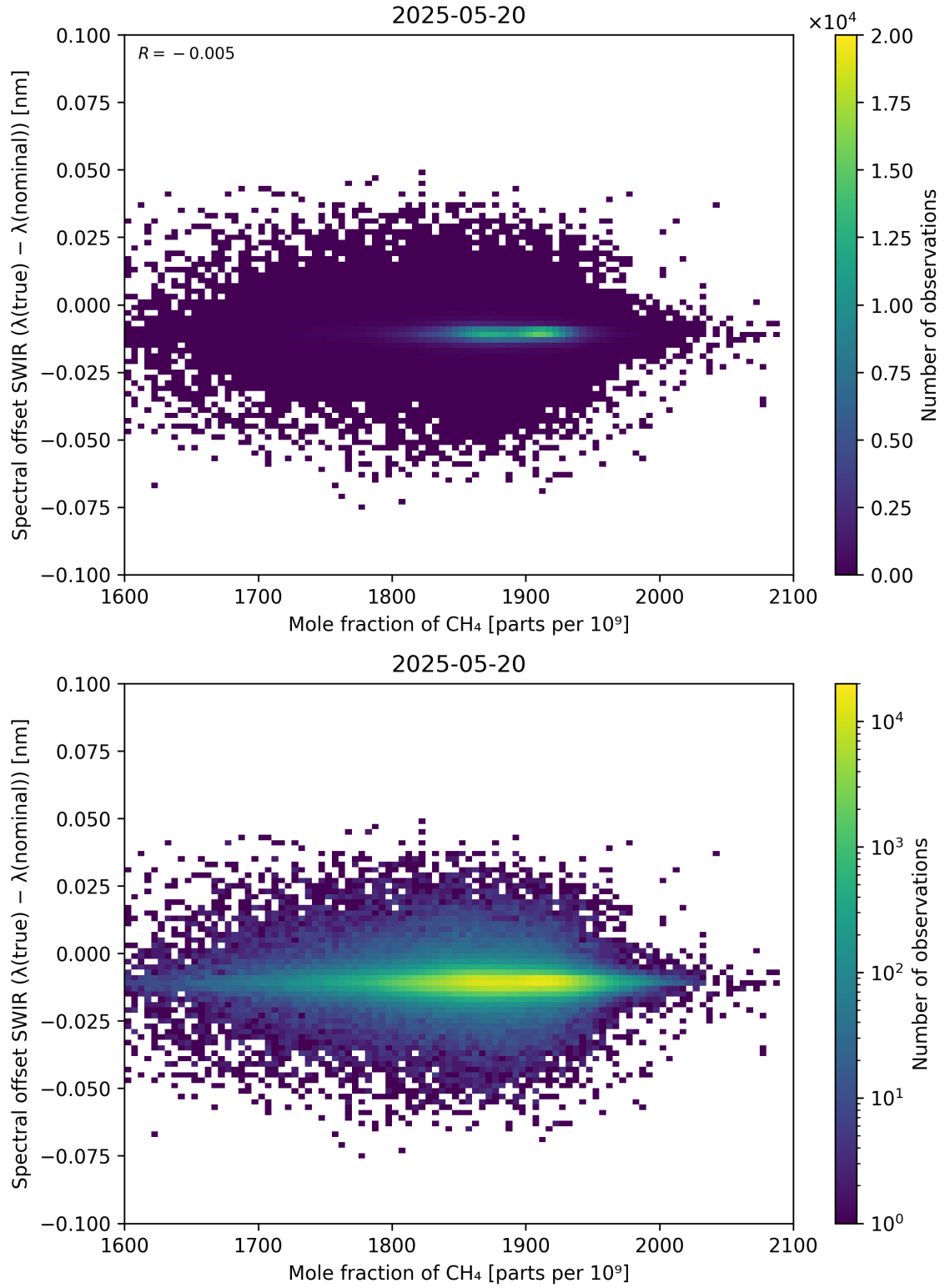
Figure 86: Scatter density plot of “Mole fraction of CH 4 ” against “Spectral offset SWIR ( \lambda_{\text{true}} - \lambda_{\text{nominal}} )” for 2025-05-19 to 2025-05-21.
