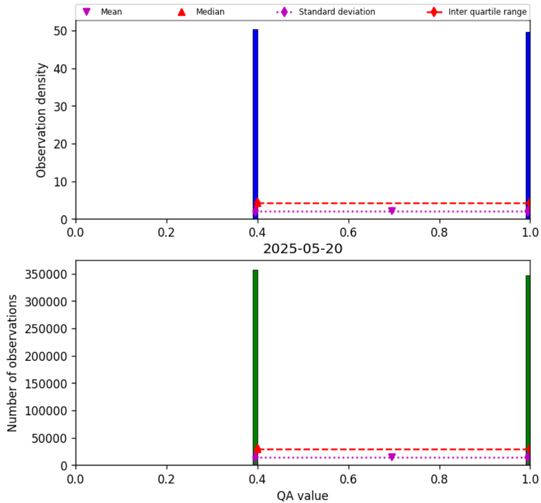
Figure 22: Histogram of “QA value” for 2025-05-19 to 2025-05-21
