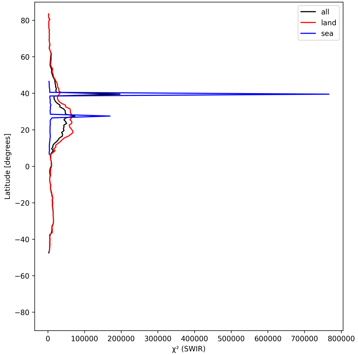
Figure 17: Zonal average of “ \chi^2 (SWIR)” for 2025-05-19 to 2025-05-21.
