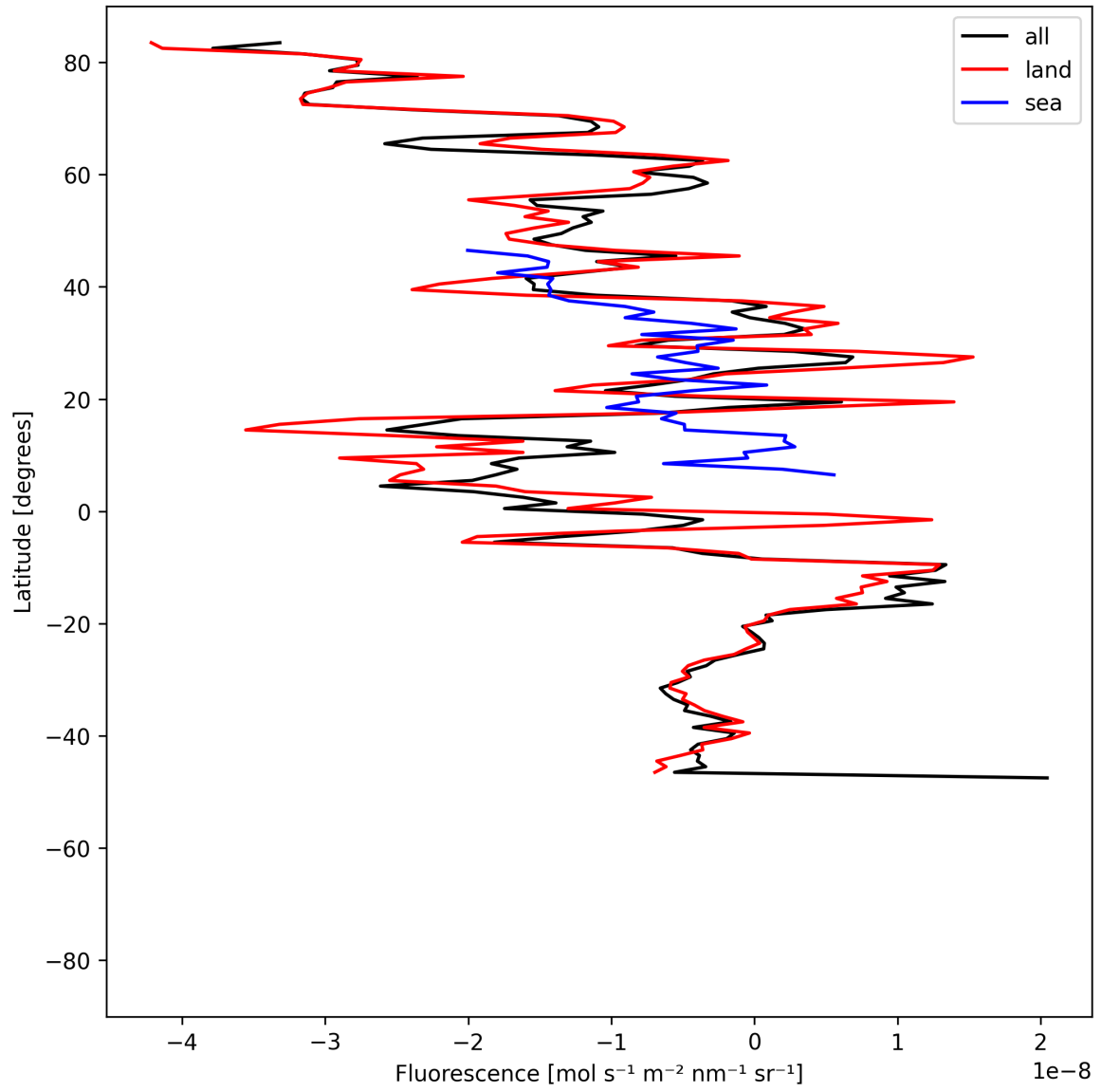
Figure 21: Zonal average of “Fluorescence” for 2025-05-19 to 2025-05-21.
