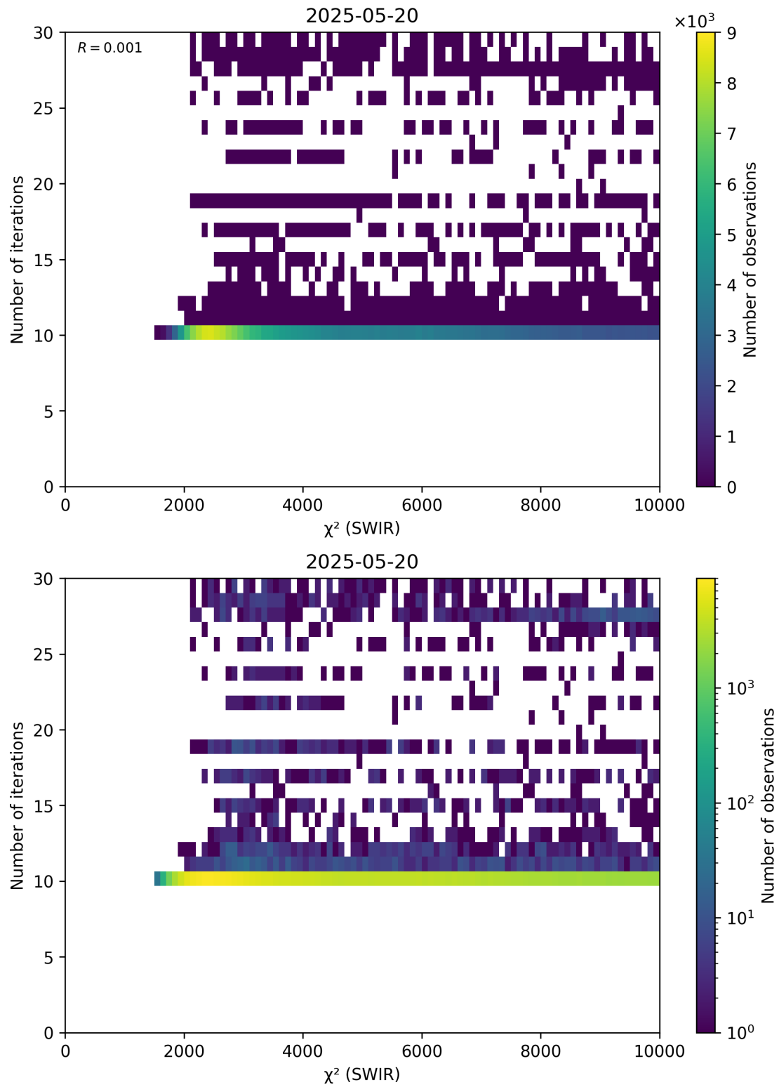
Figure 50: Scatter density plot of “ \chi^2 (SWIR)” against “Number of iterations” for 2025-05-19 to 2025-05-21.
