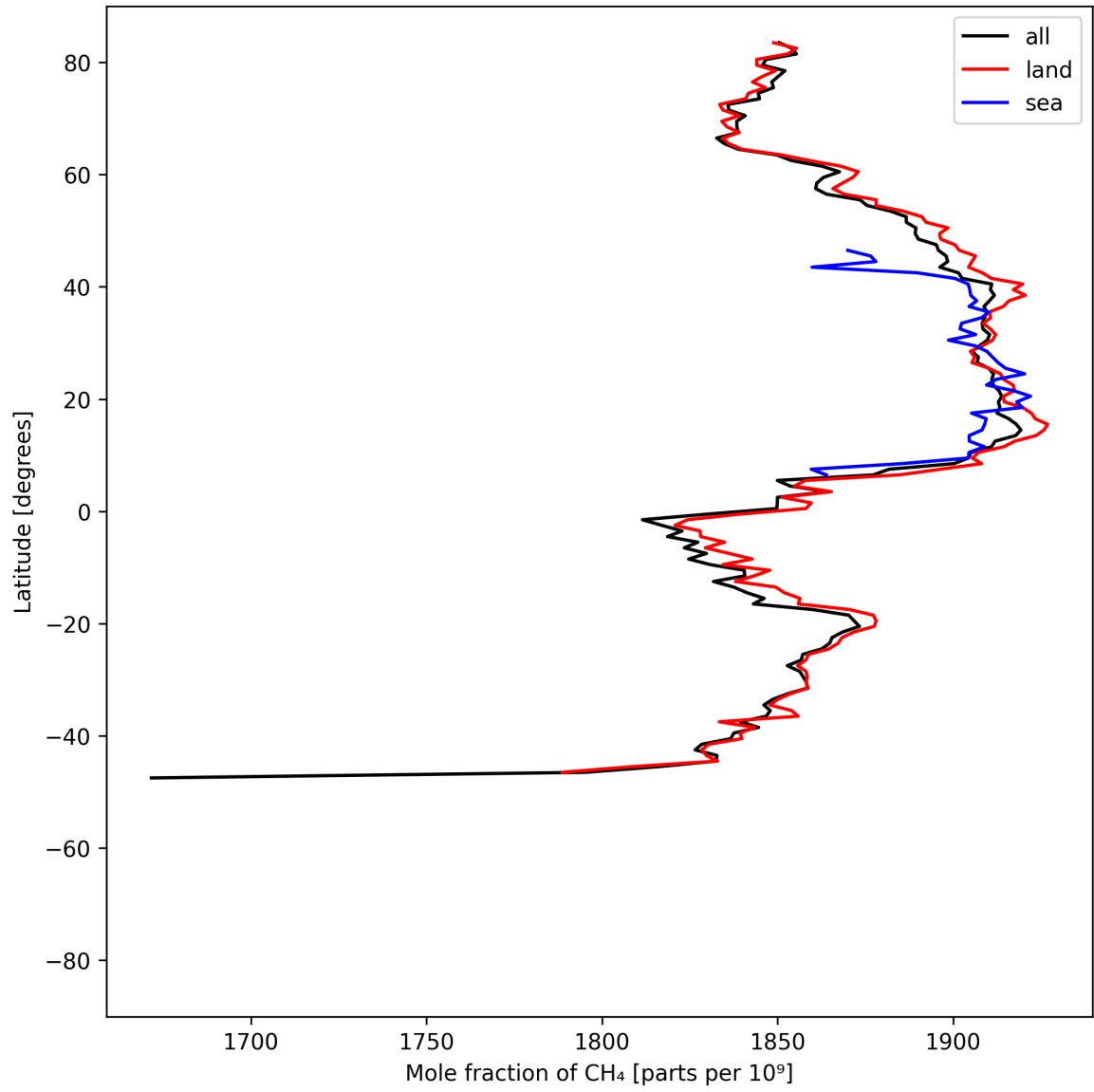
Figure 12: Zonal average of “Mole fraction of CH 4 ” for 2025-05-19 to 2025-05-21.
