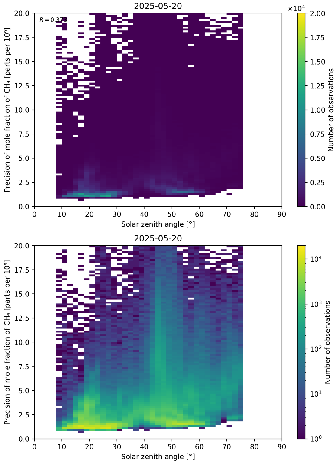
Figure 101: Scatter density plot of “Solar zenith angle” against “Precision of mole fraction of CH 4 ” for 2025-05-19 to 2025-05-21.
