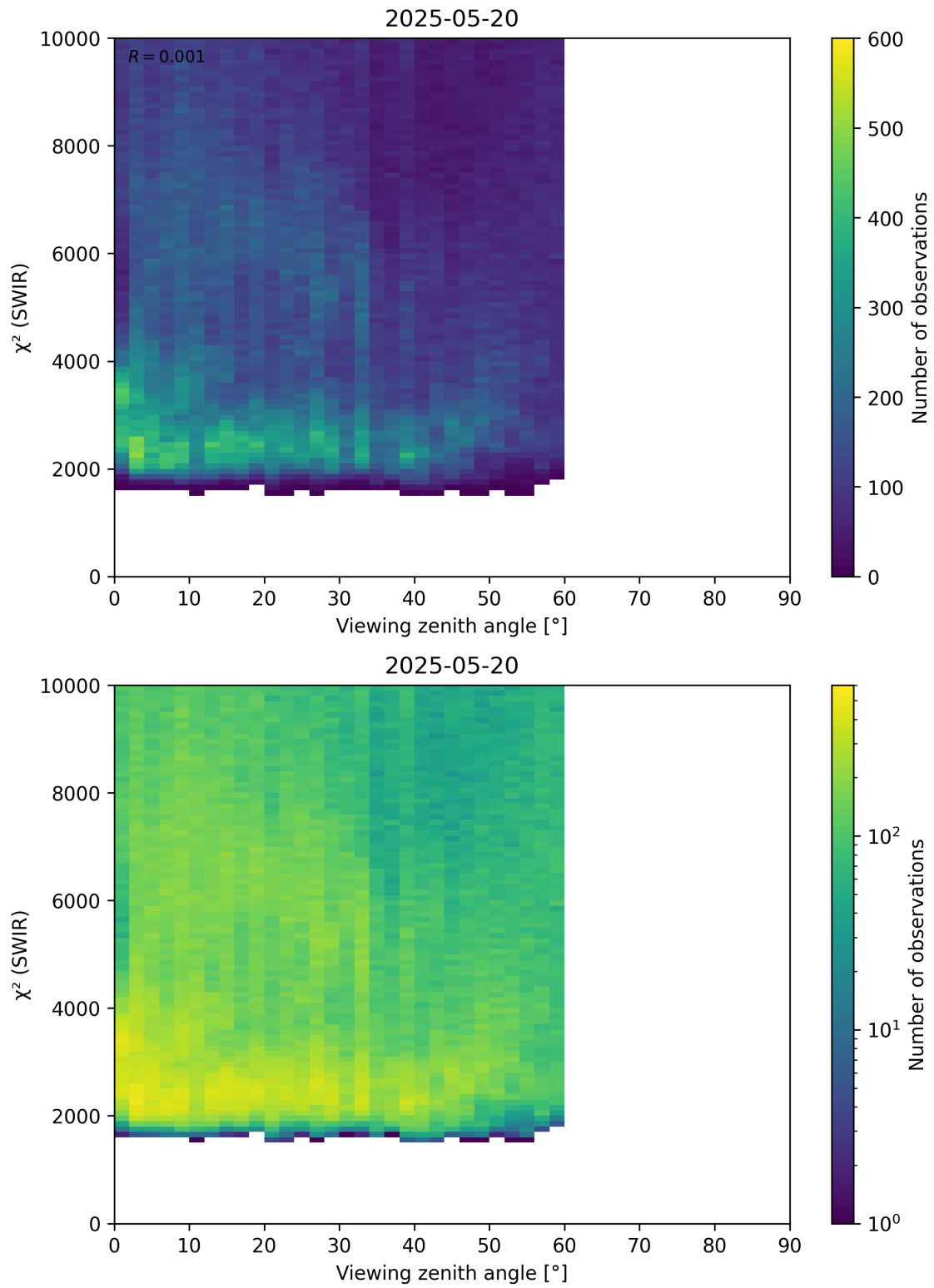
Figure 106: Scatter density plot of “Viewing zenith angle” against “ \chi^2 (SWIR)” for 2025-05-19 to 2025-05-21.
