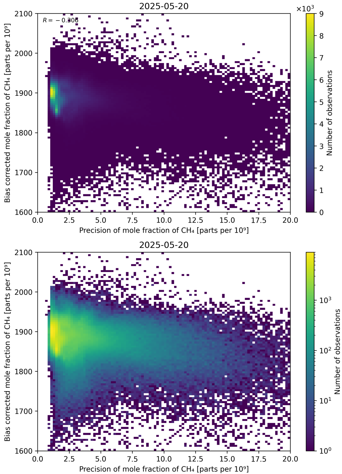
Figure 82: Scatter density plot of “Precision of mole fraction of CH 4 ” against “Bias corrected mole fraction of CH 4 ” for 2025-05-19 to 2025-05-21.
