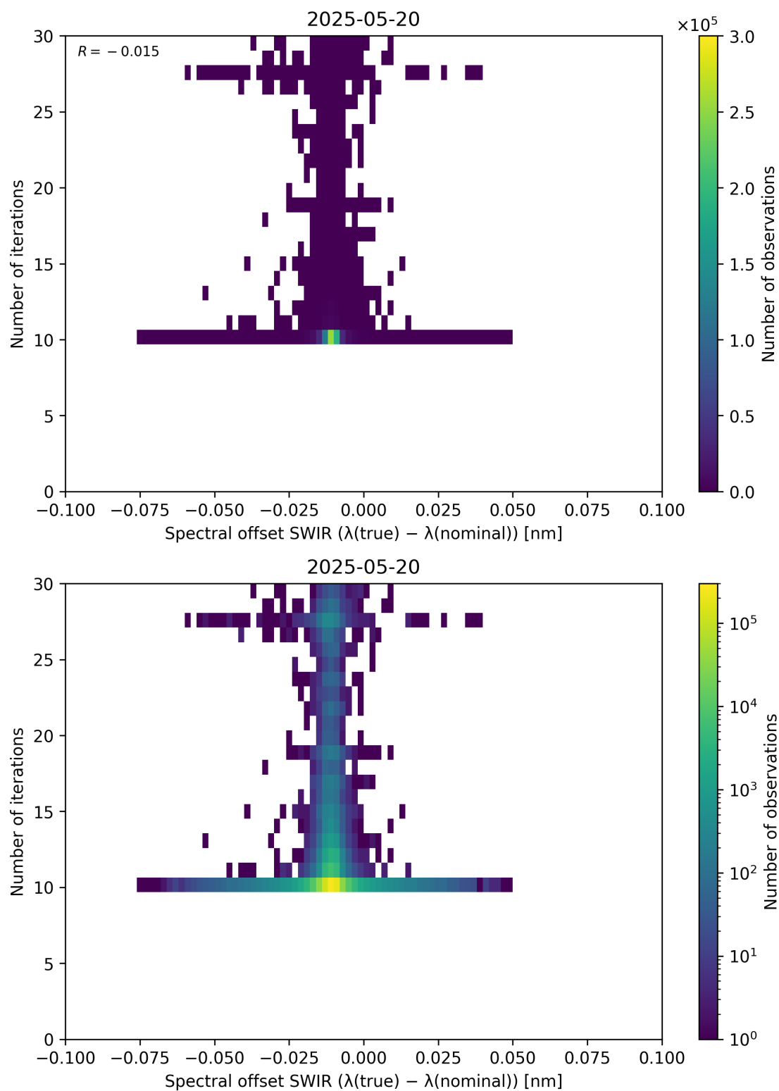
Figure 121: Scatter density plot of “Spectral offset SWIR ( \lambda_{\text{true}} - \lambda_{\text{nominal}} )” against “Number of iterations” for 2025-05-19 to 2025-05-21.
