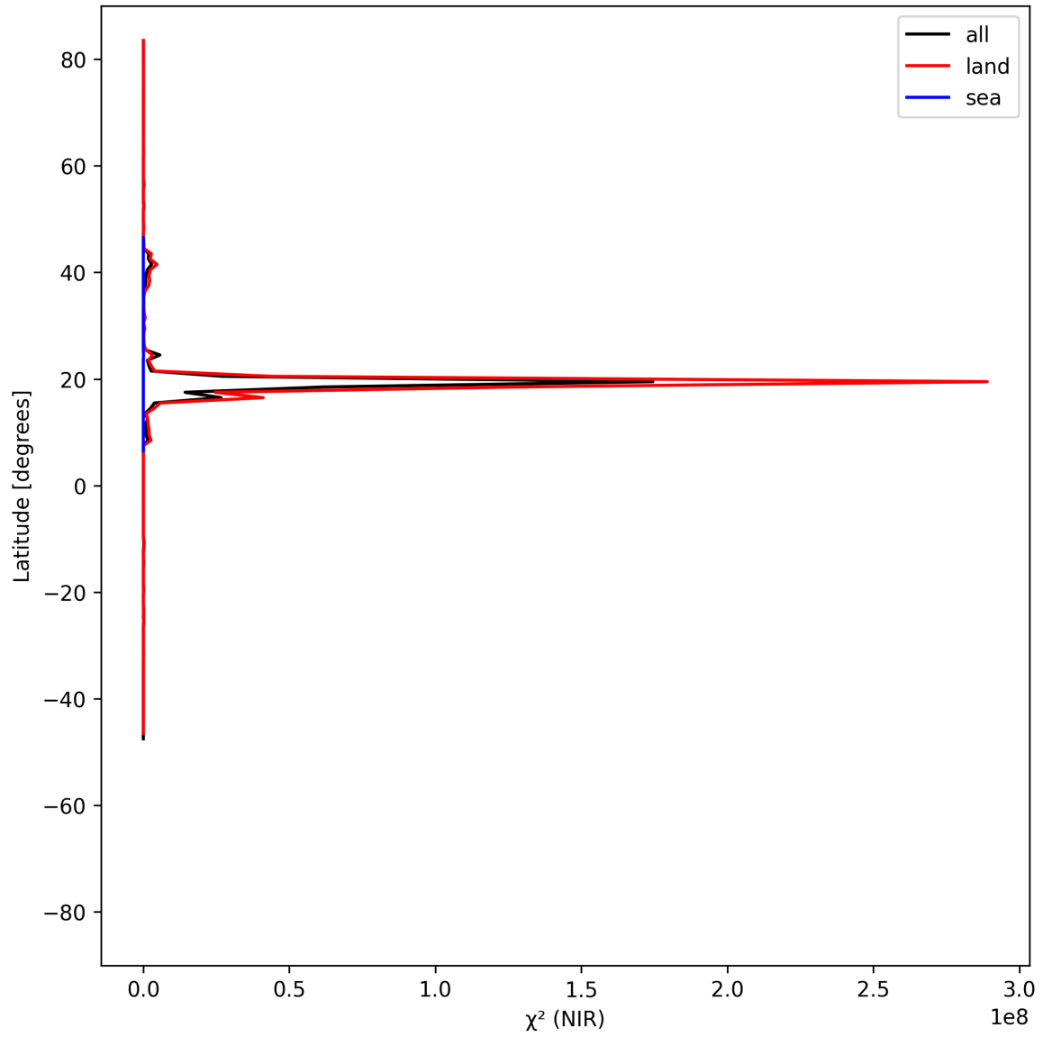
Figure 18: Zonal average of “ \chi^2 (NIR)” for 2025-05-19 to 2025-05-21.
