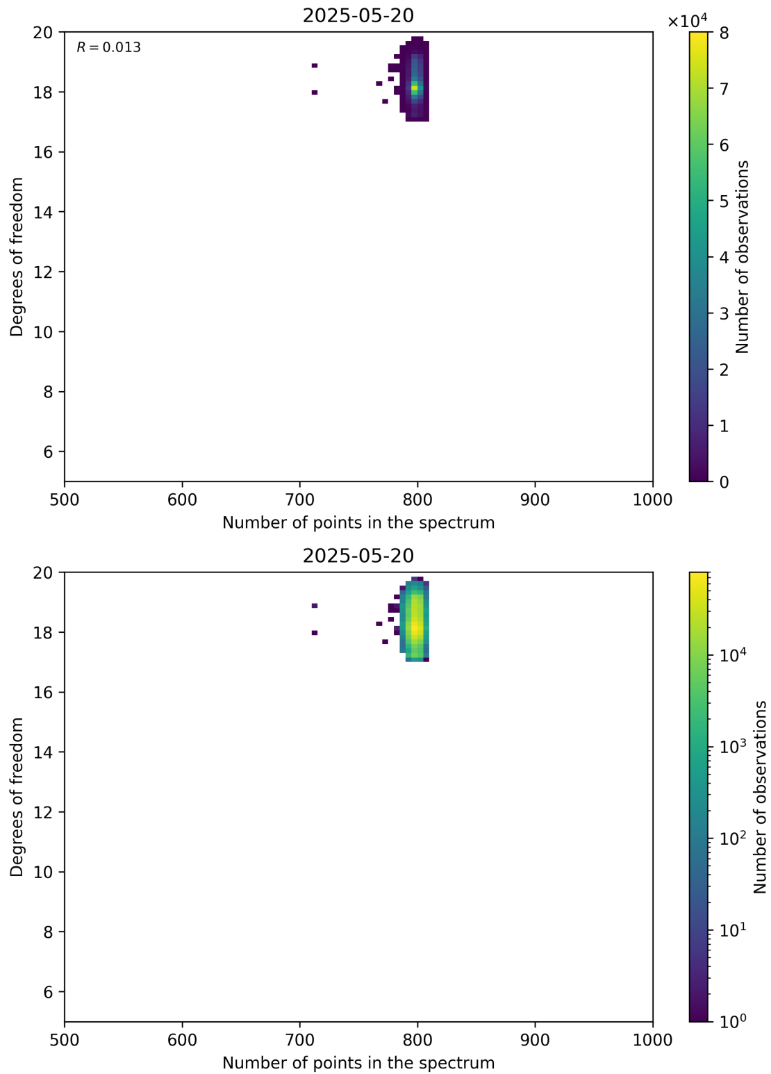
Figure 90: Scatter density plot of “Number of points in the spectrum” against “Degrees of freedom” for 2025-05-19 to 2025-05-21.
