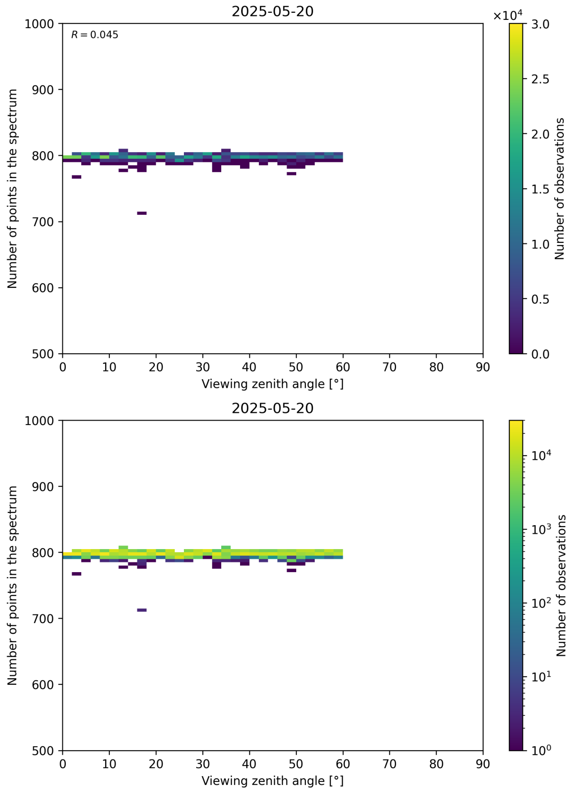
Figure 114: Scatter density plot of “Viewing zenith angle” against “Number of points in the spectrum” for 2025-05-19 to 2025-05-21.
