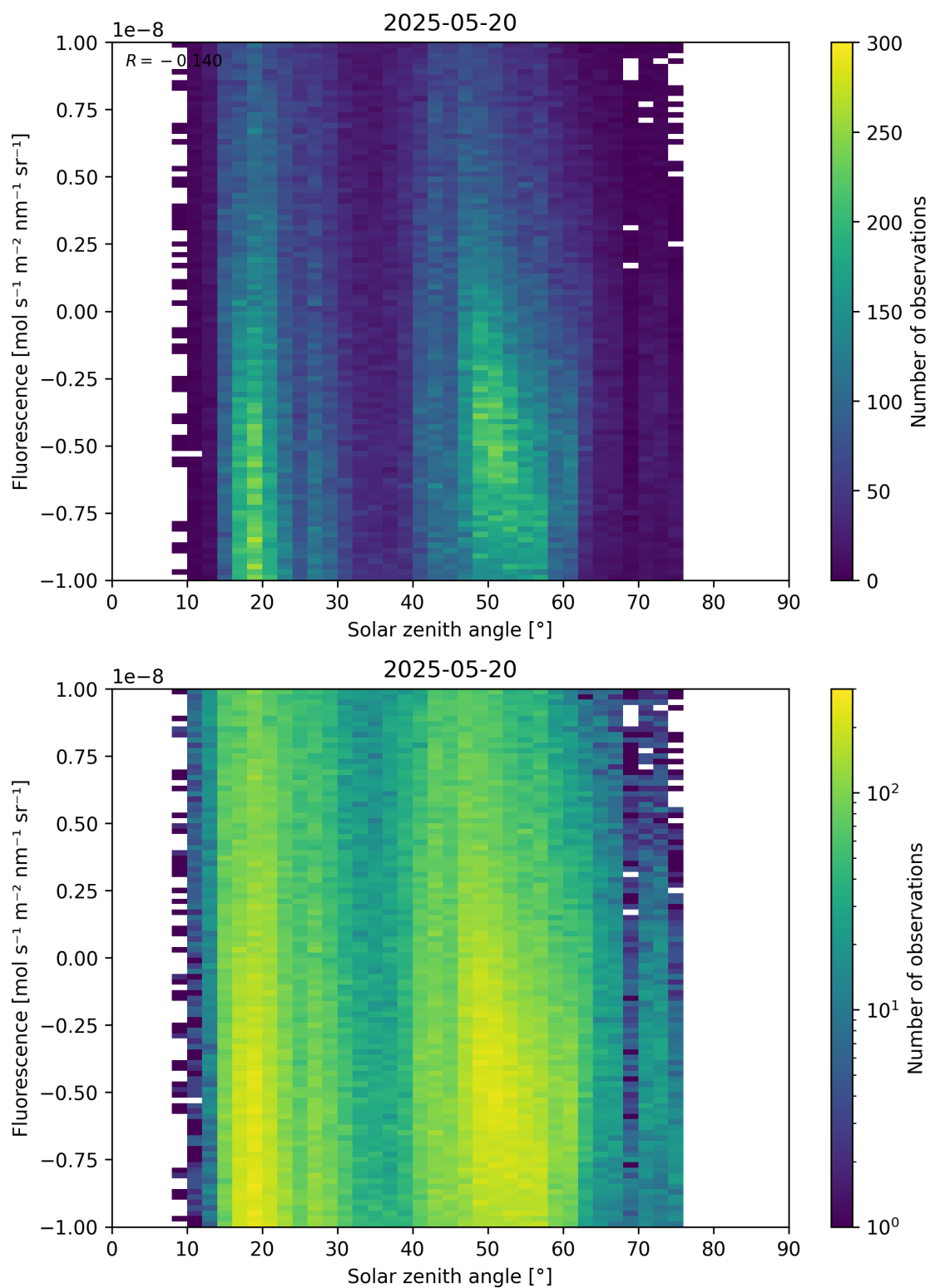
Figure 97: Scatter density plot of “Solar zenith angle” against “Fluorescence” for 2025-05-19 to 2025-05-21.
