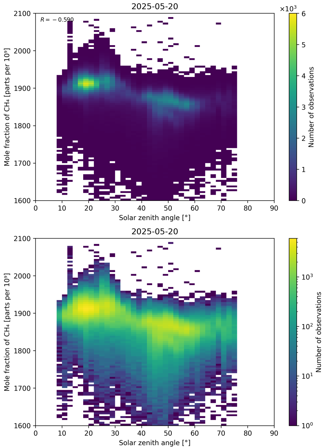
Figure 99: Scatter density plot of “Solar zenith angle” against “Mole fraction of \text{CH}_4 ” for 2025-05-19 to 2025-05-21.
