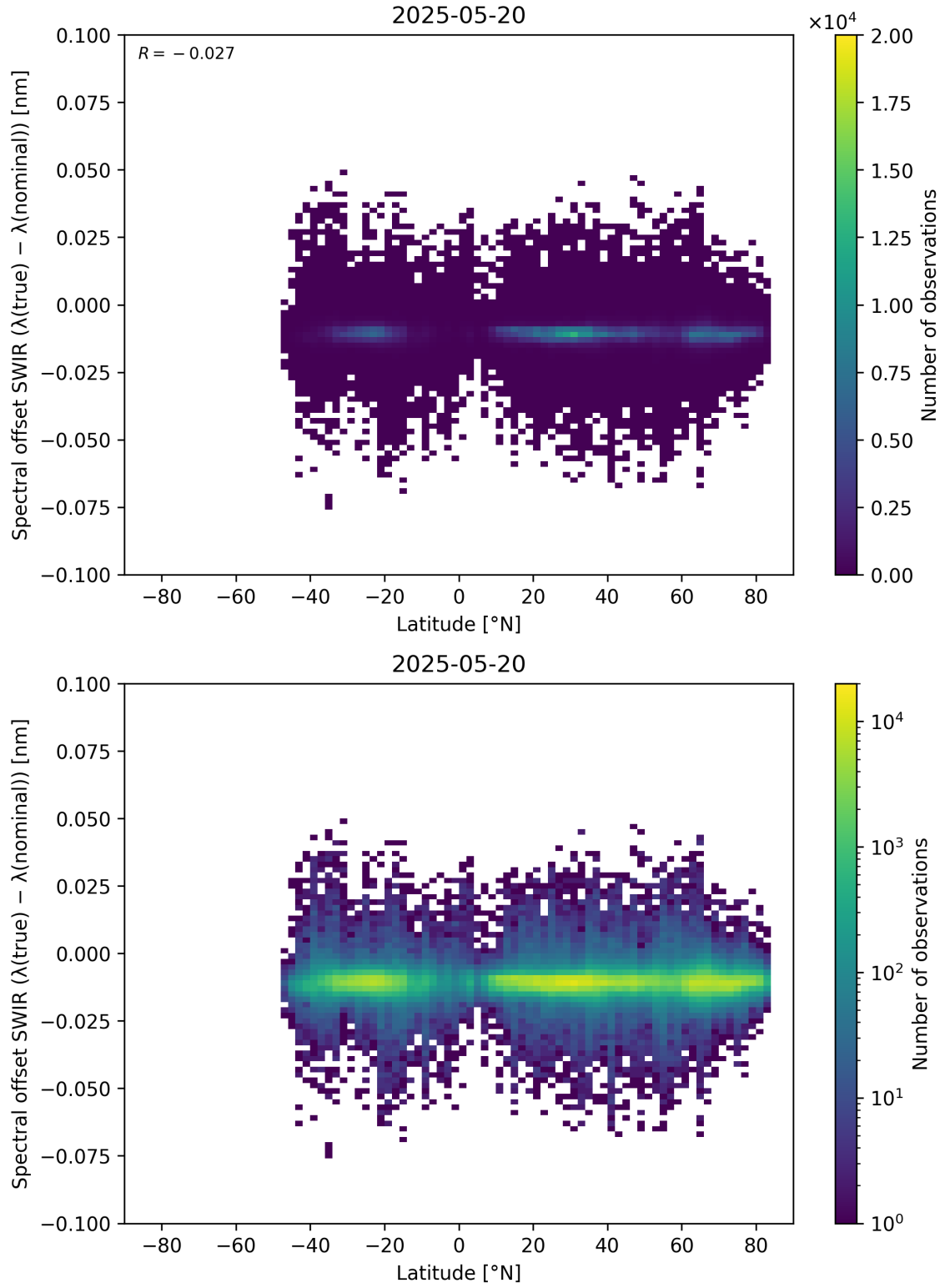
Figure 62: Scatter density plot of “Latitude” against “Spectral offset SWIR ( \lambda_{\text{true}} - \lambda_{\text{nominal}} )” for 2025-05-19 to 2025-05-21.
