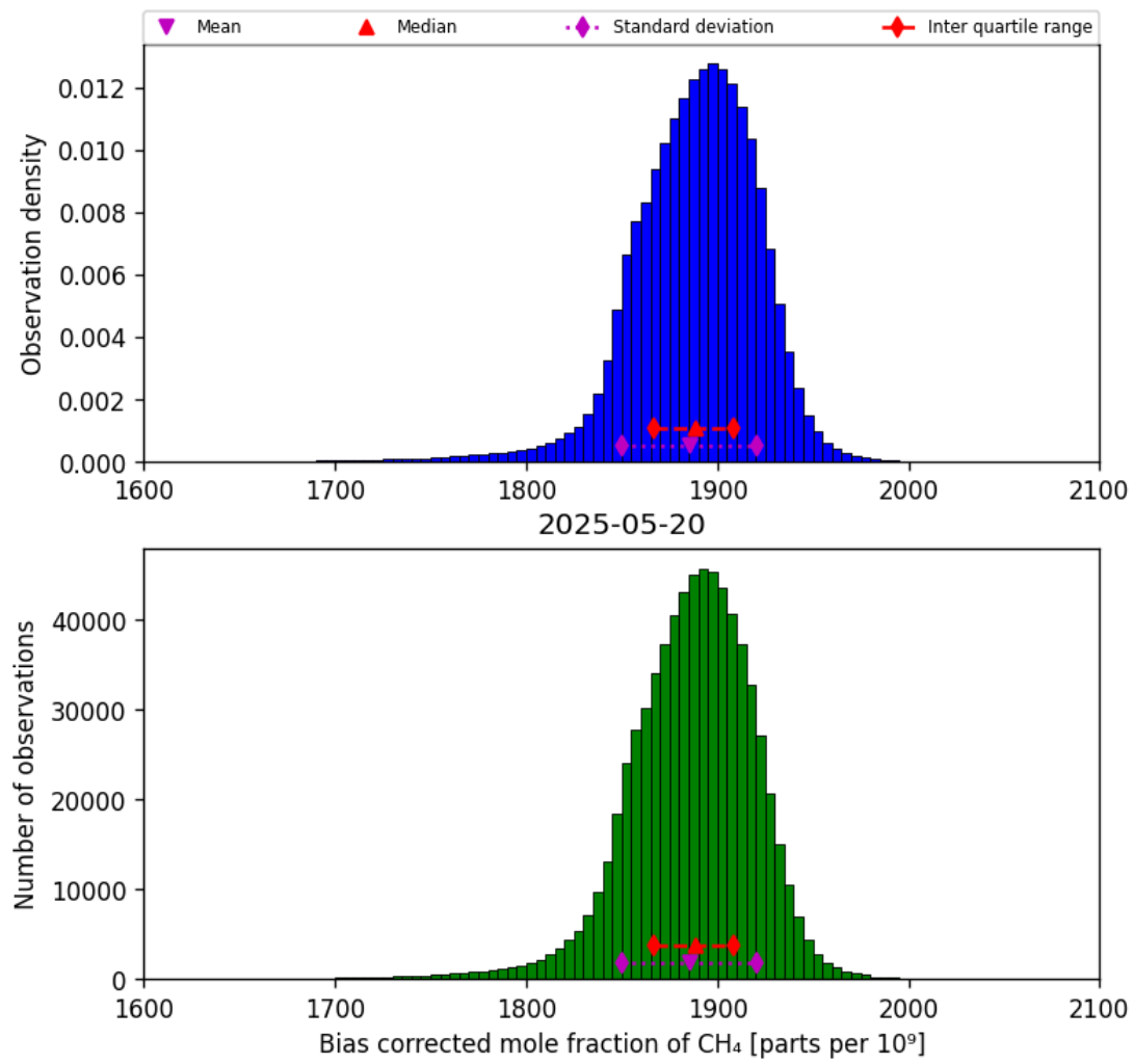
Figure 25: Histogram of “Bias corrected mole fraction of CH 4 ” for 2025-05-19 to 2025-05-21
