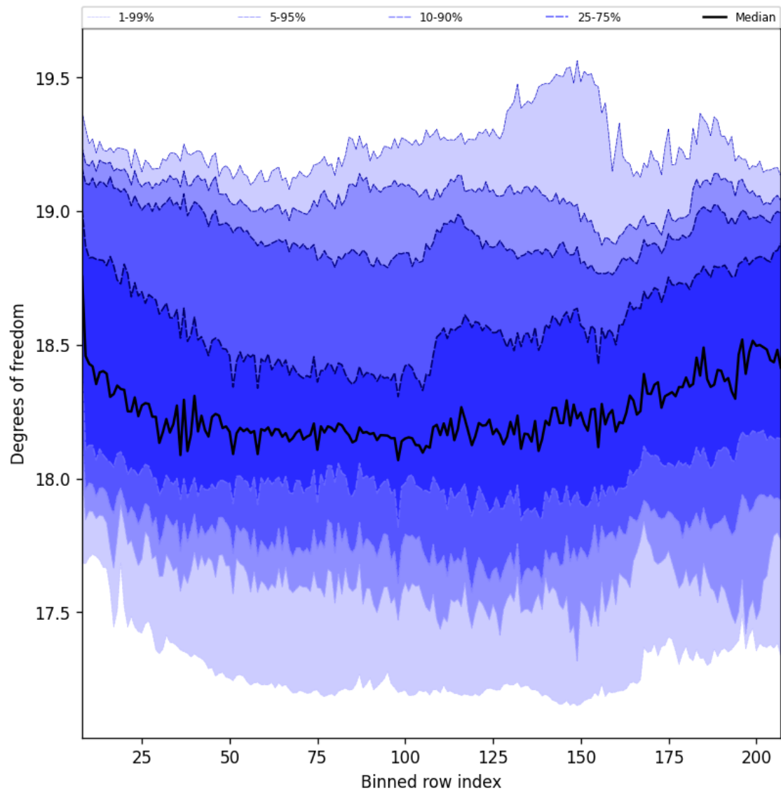
Figure 41: Along track statistics of “Degrees of freedom” for 2025-05-19 to 2025-05-21
