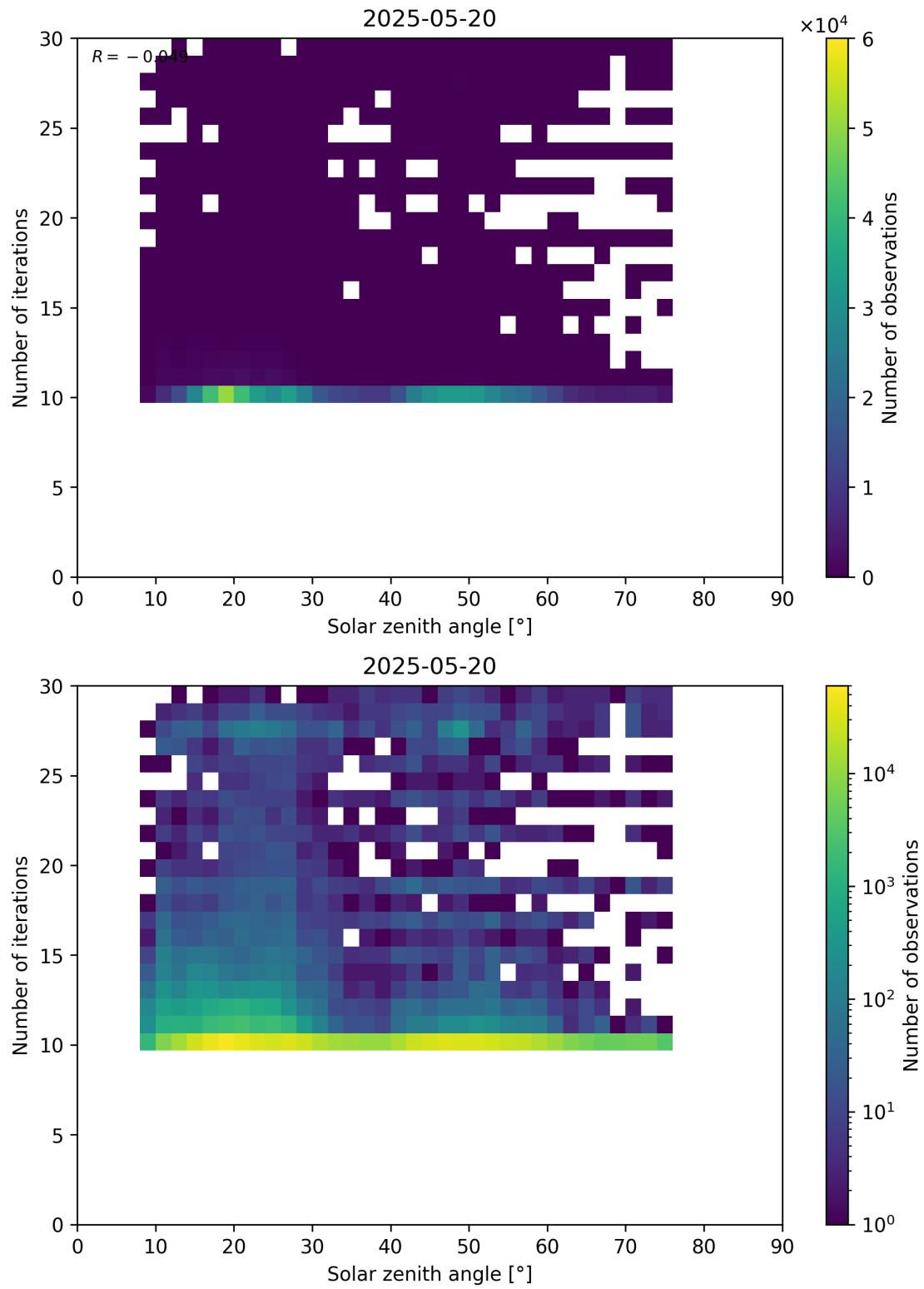
Figure 102: Scatter density plot of “Solar zenith angle” against “Number of iterations” for 2025-05-19 to 2025-05-21.
