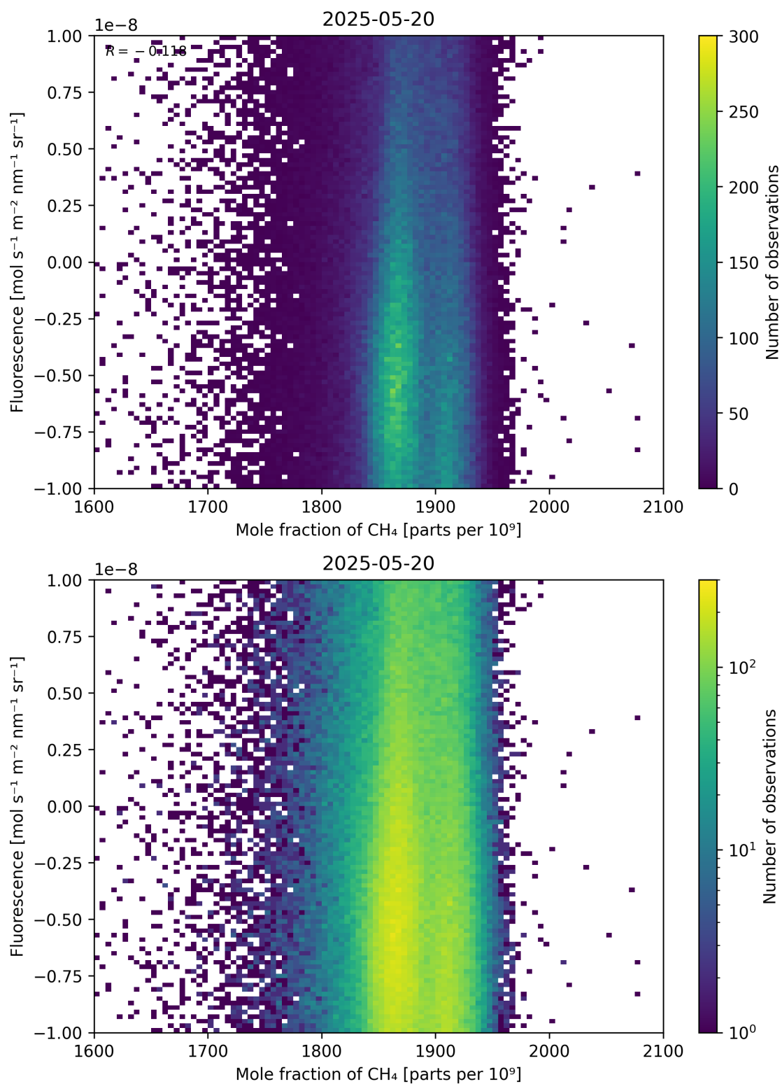
Figure 73: Scatter density plot of “Mole fraction of \text{CH}_4 ” against “Fluorescence” for 2025-05-19 to 2025-05-21.
