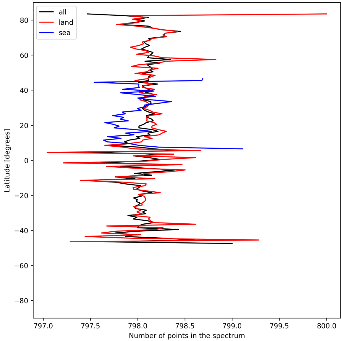
Figure 15: Zonal average of “Number of points in the spectrum” for 2025-05-19 to 2025-05-21.
