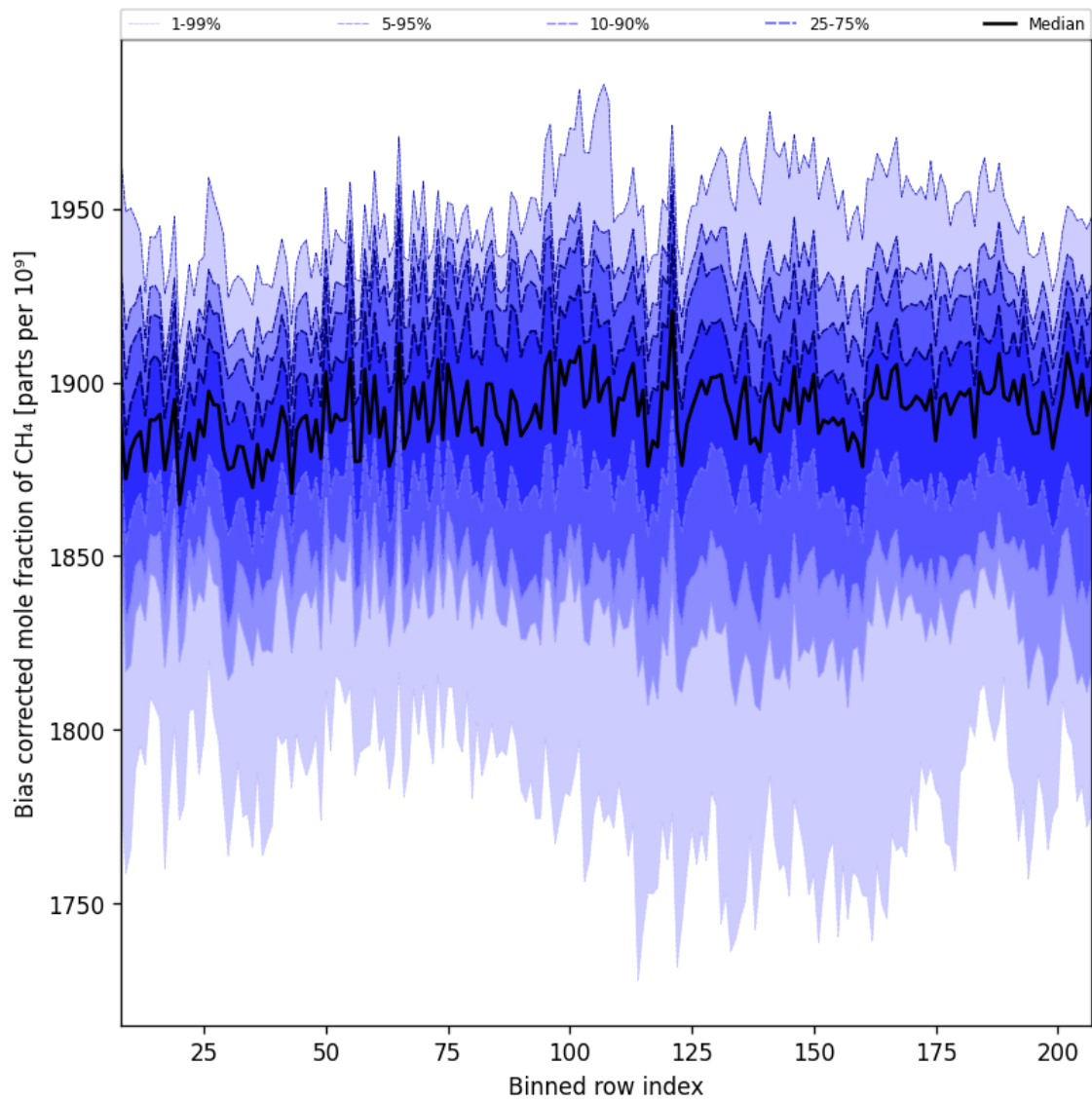
Figure 36: Along track statistics of “Bias corrected mole fraction of CH 4 ” for 2025-05-21 to 2025-05-22
