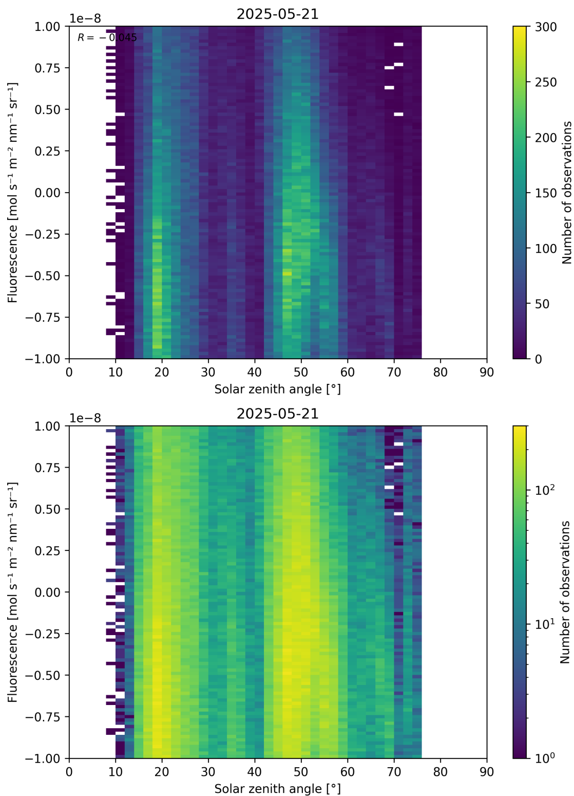
Figure 97: Scatter density plot of “Solar zenith angle” against “Fluorescence” for 2025-05-21 to 2025-05-22.
