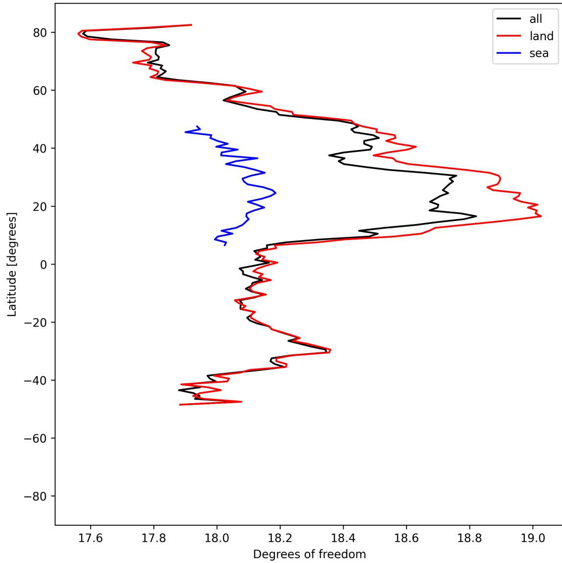
Figure 19: Zonal average of “Degrees of freedom” for 2025-05-21 to 2025-05-22.
