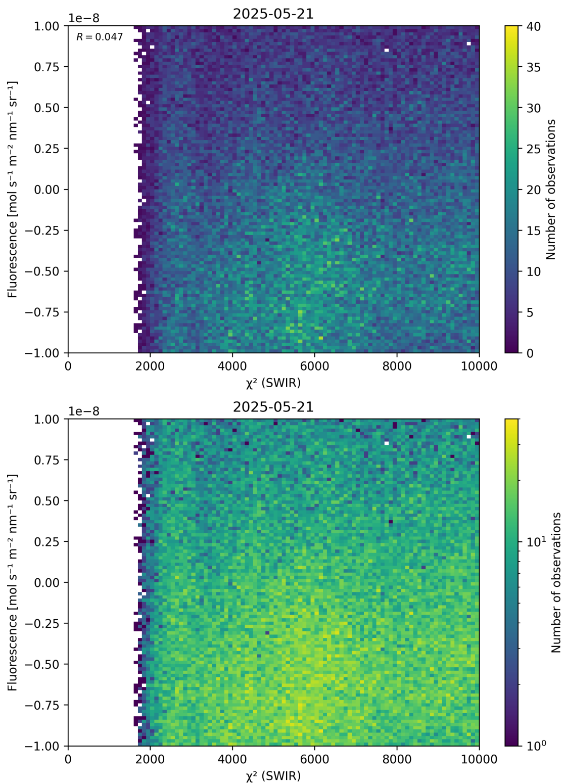
Figure 49: Scatter density plot of “ \chi^2 (SWIR)” against “Fluorescence” for 2025-05-21 to 2025-05-22.
