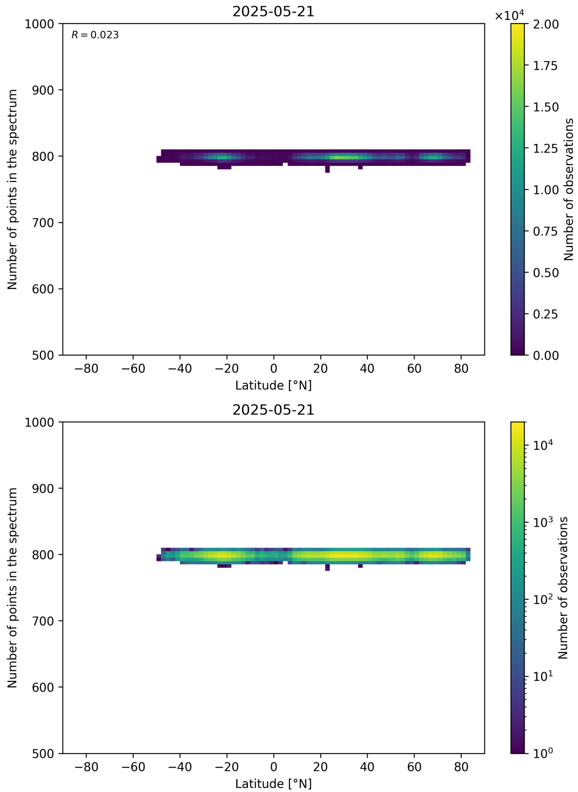
Figure 61: Scatter density plot of “Latitude” against “Number of points in the spectrum” for 2025-05-21 to 2025-05-22.
