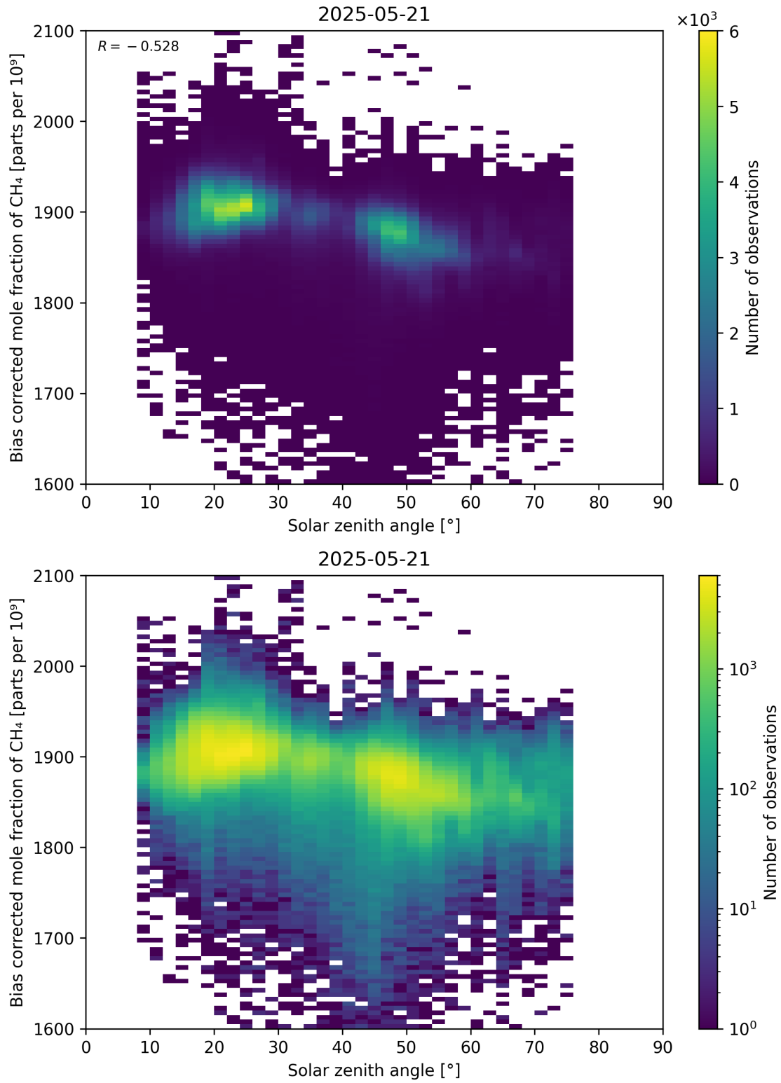
Figure 100: Scatter density plot of “Solar zenith angle” against “Bias corrected mole fraction of CH 4 ” for 2025-05-21 to 2025-05-22.
