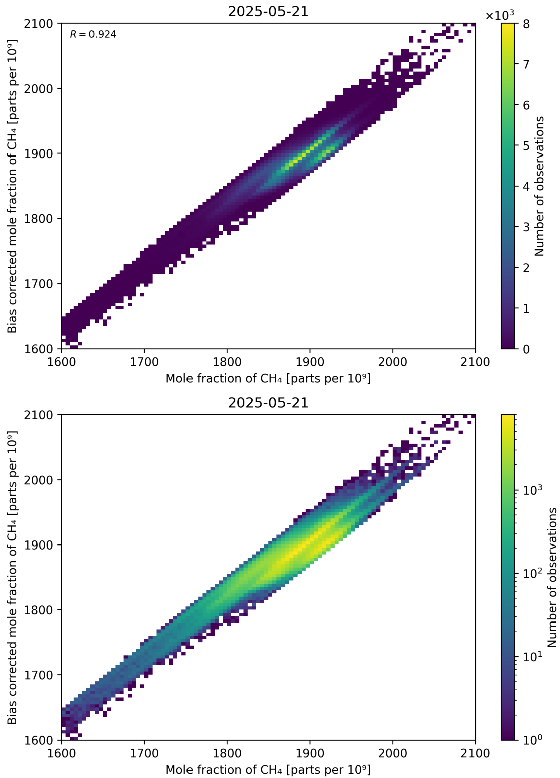
Figure 74: Scatter density plot of “Mole fraction of CH 4 ” against “Bias corrected mole fraction of CH 4 ” for 2025-05-21 to 2025-05-22.
