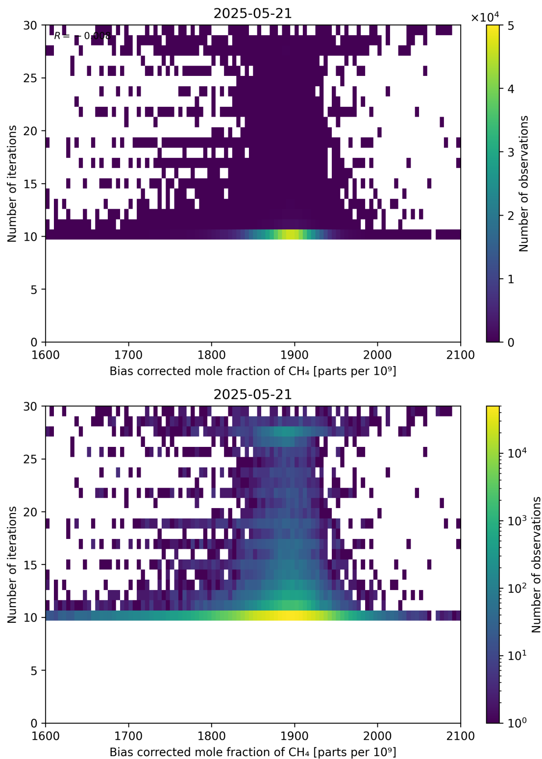
Figure 67: Scatter density plot of “Bias corrected mole fraction of CH 4 ” against “Number of iterations” for 2025-05-21 to 2025-05-22.
