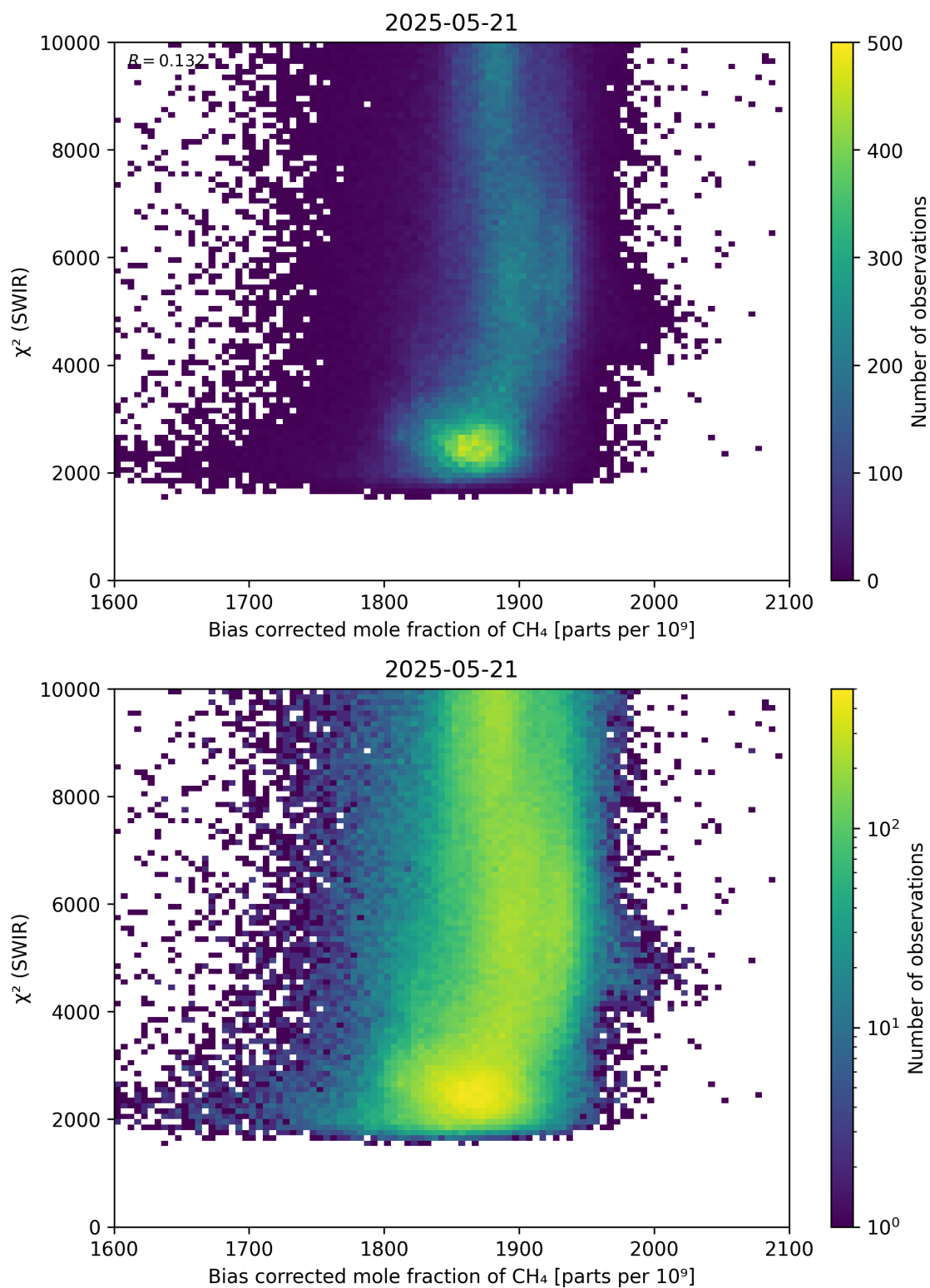
Figure 64: Scatter density plot of “Bias corrected mole fraction of CH 4 ” against “ \chi^2 (SWIR)” for 2025-05-21 to 2025-05-22.
