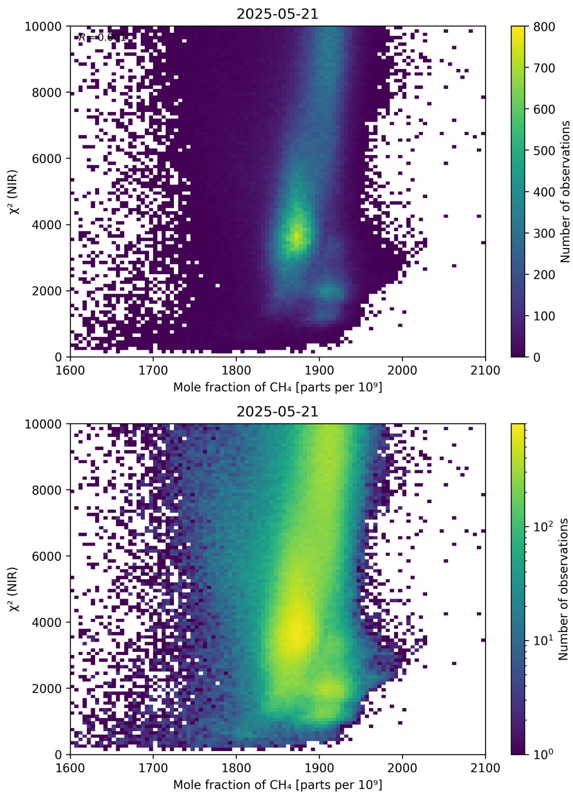
Figure 70: Scatter density plot of “Mole fraction of CH 4 ” against “ \chi^2 (NIR)” for 2025-05-21 to 2025-05-22.
