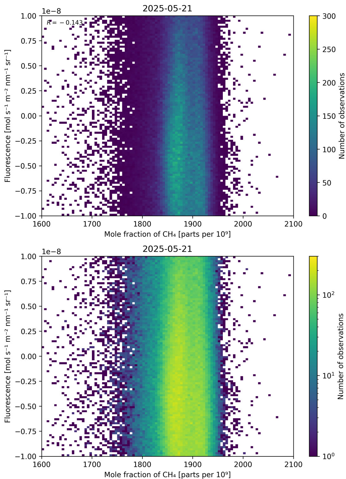
Figure 73: Scatter density plot of “Mole fraction of CH 4 ” against “Fluorescence” for 2025-05-21 to 2025-05-22.
