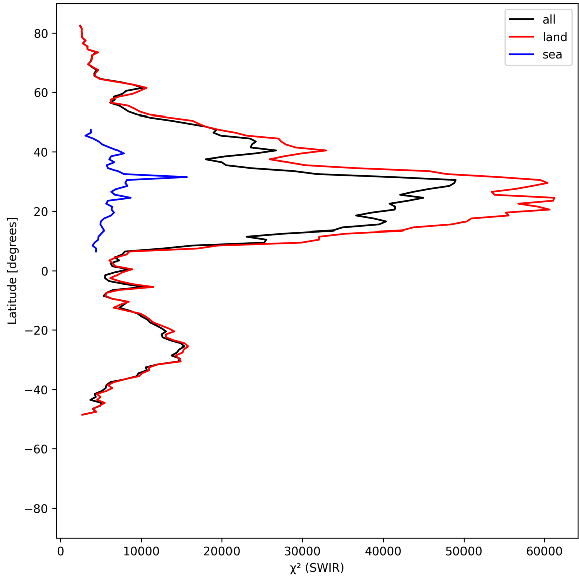
Figure 17: Zonal average of “ \chi^2 (SWIR)” for 2025-05-21 to 2025-05-22.
