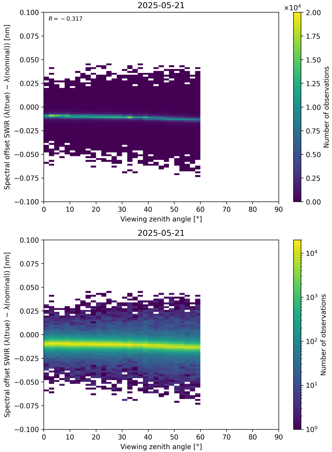
Figure 116: Scatter density plot of “Viewing zenith angle” against “Spectral offset SWIR ( \lambda_{\text{true}} - \lambda_{\text{nominal}} )” for 2025-05-21 to 2025-05-22.
