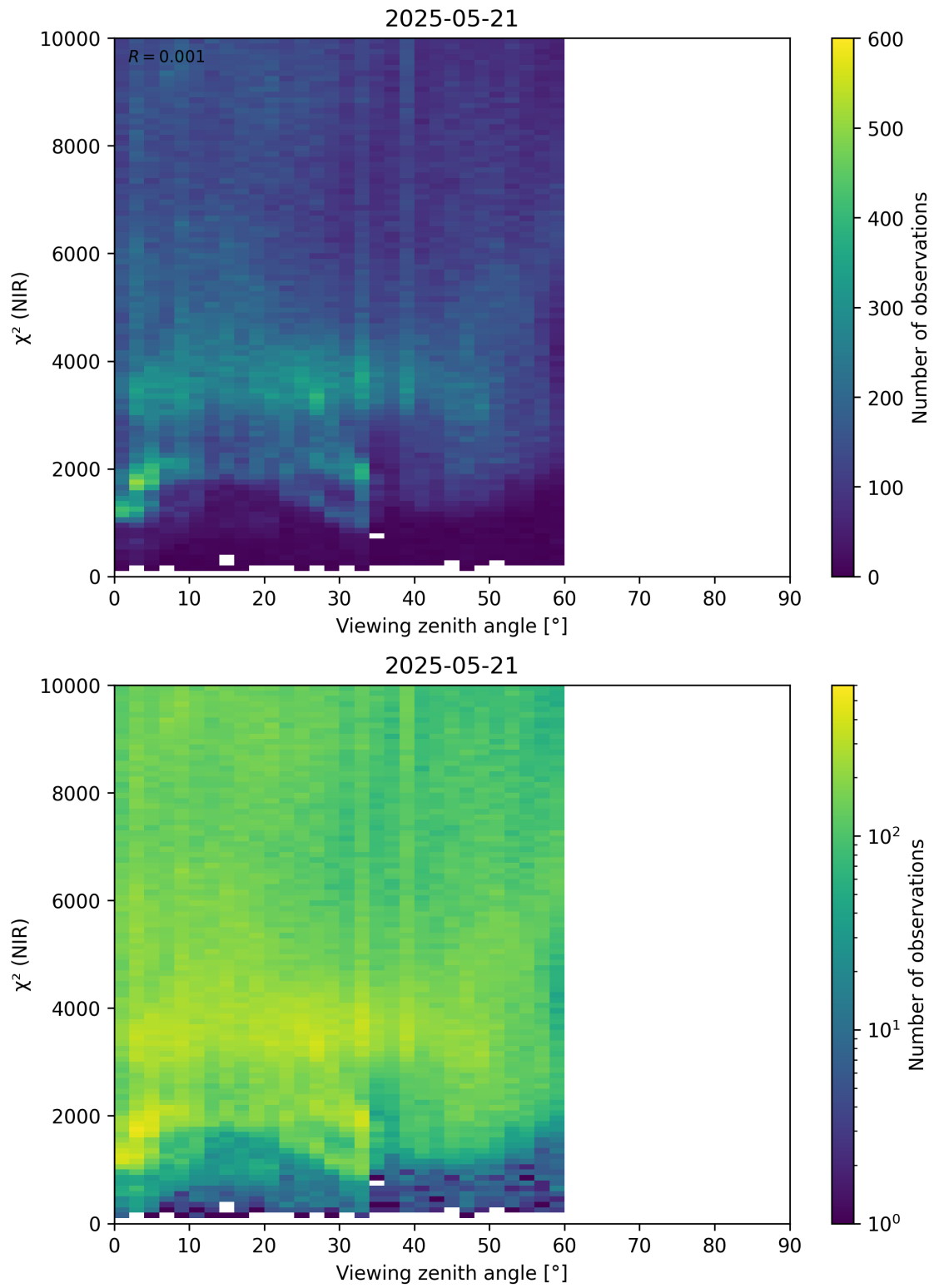
Figure 105: Scatter density plot of “Viewing zenith angle” against “ \chi^2 (NIR)” for 2025-05-21 to 2025-05-22.
