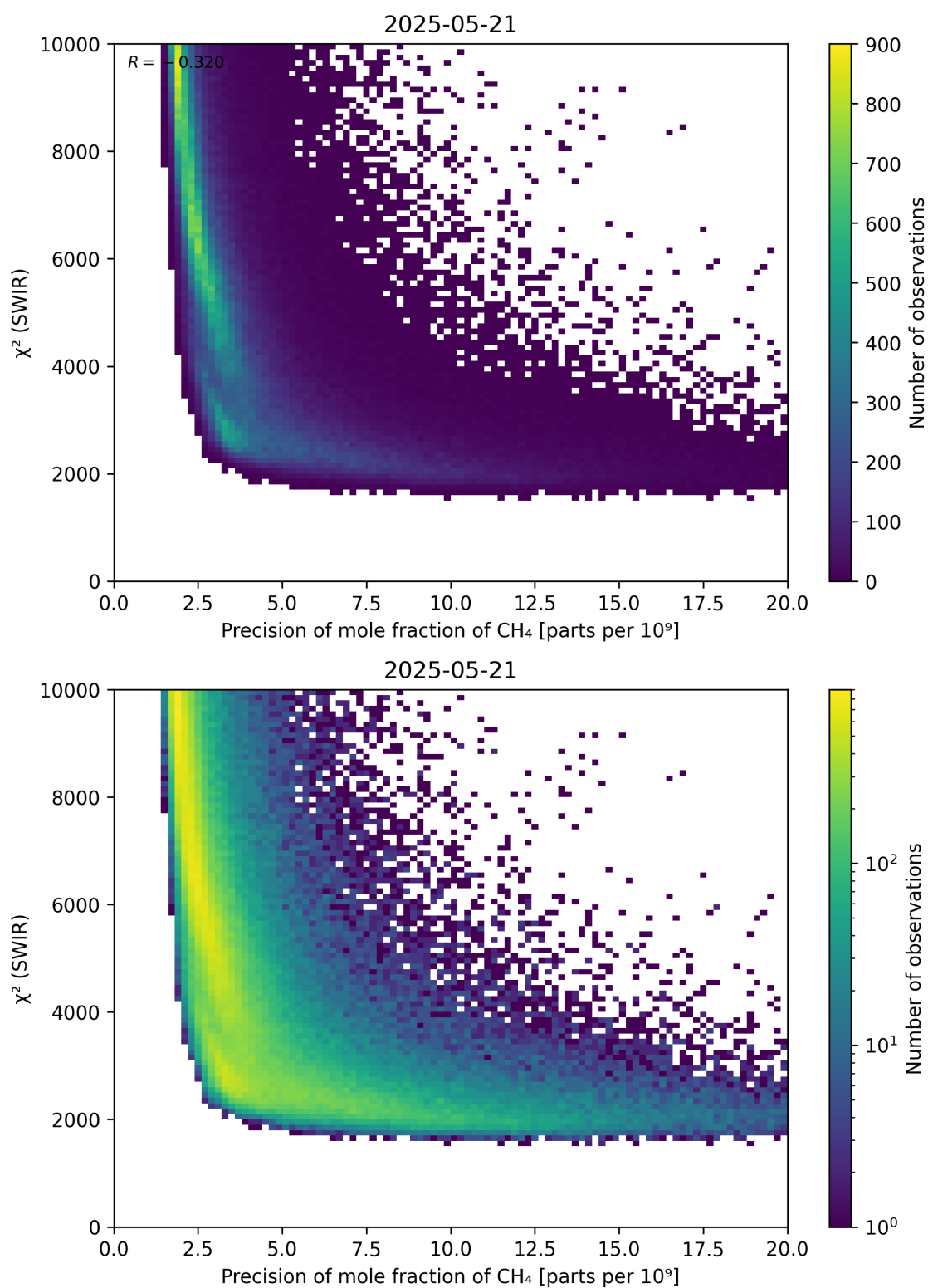
Figure 79: Scatter density plot of “Precision of mole fraction of CH 4 ” against “ \chi^2 (SWIR)” for 2025-05-21 to 2025-05-22.
