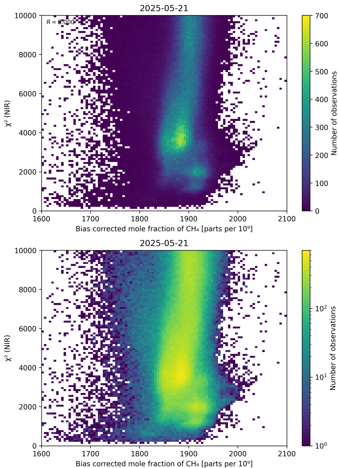
Figure 63: Scatter density plot of “Bias corrected mole fraction of CH 4 ” against “ \chi^2 (NIR)” for 2025-05-21 to 2025-05-22.
