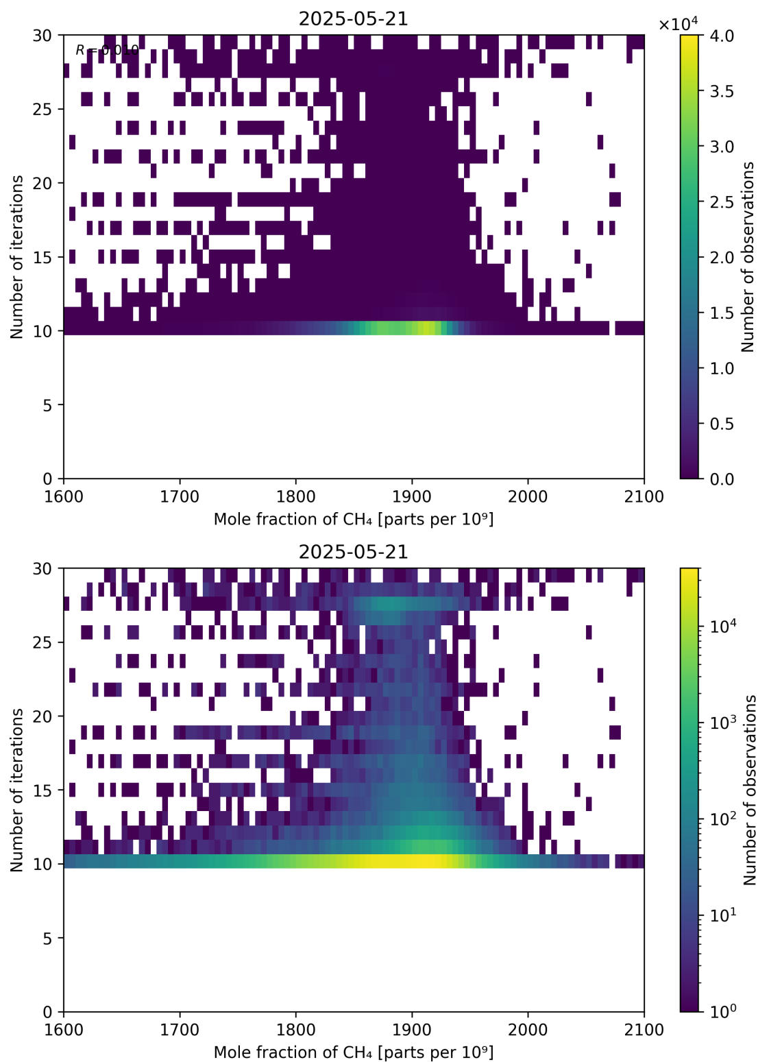
Figure 76: Scatter density plot of “Mole fraction of CH 4 ” against “Number of iterations” for 2025-05-21 to 2025-05-22.
