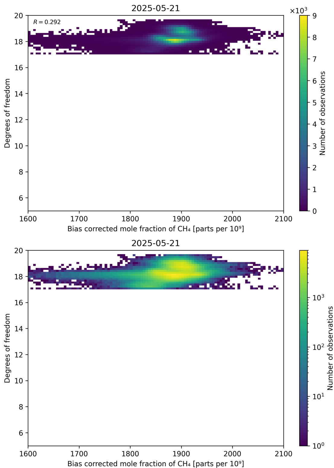
Figure 65: Scatter density plot of “Bias corrected mole fraction of CH 4 ” against “Degrees of freedom” for 2025-05-21 to 2025-05-22.
