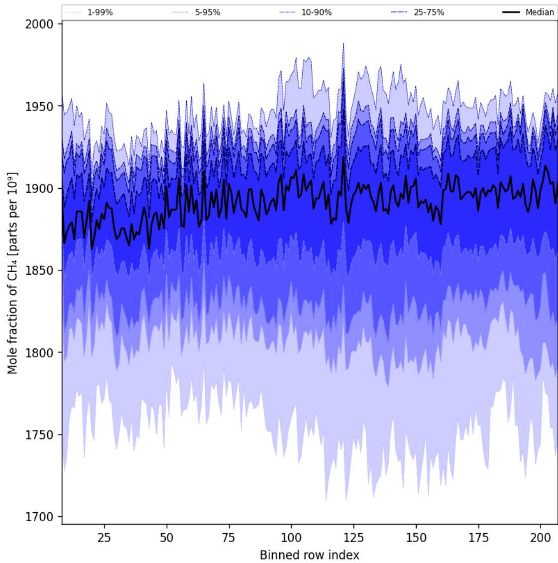
Figure 34: Along track statistics of “Mole fraction of CH 4 ” for 2025-05-21 to 2025-05-22
