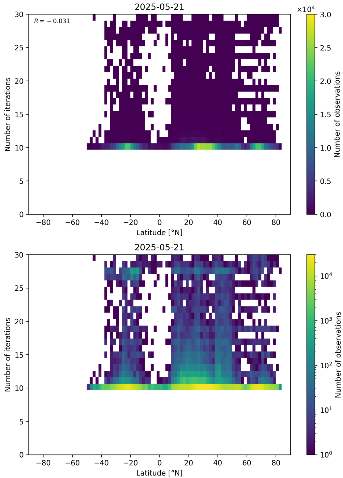
Figure 60: Scatter density plot of “Latitude” against “Number of iterations” for 2025-05-21 to 2025-05-22.
