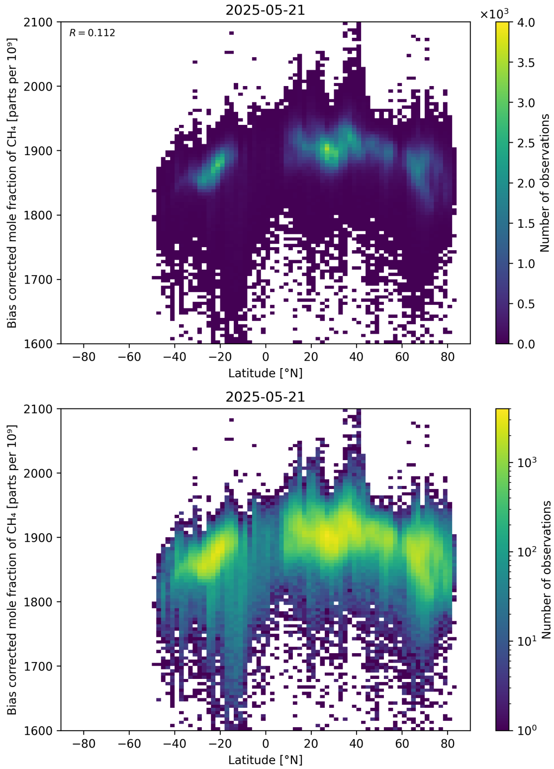
Figure 58: Scatter density plot of “Latitude” against “Bias corrected mole fraction of CH 4 ” for 2025-05-21 to 2025-05-22.
