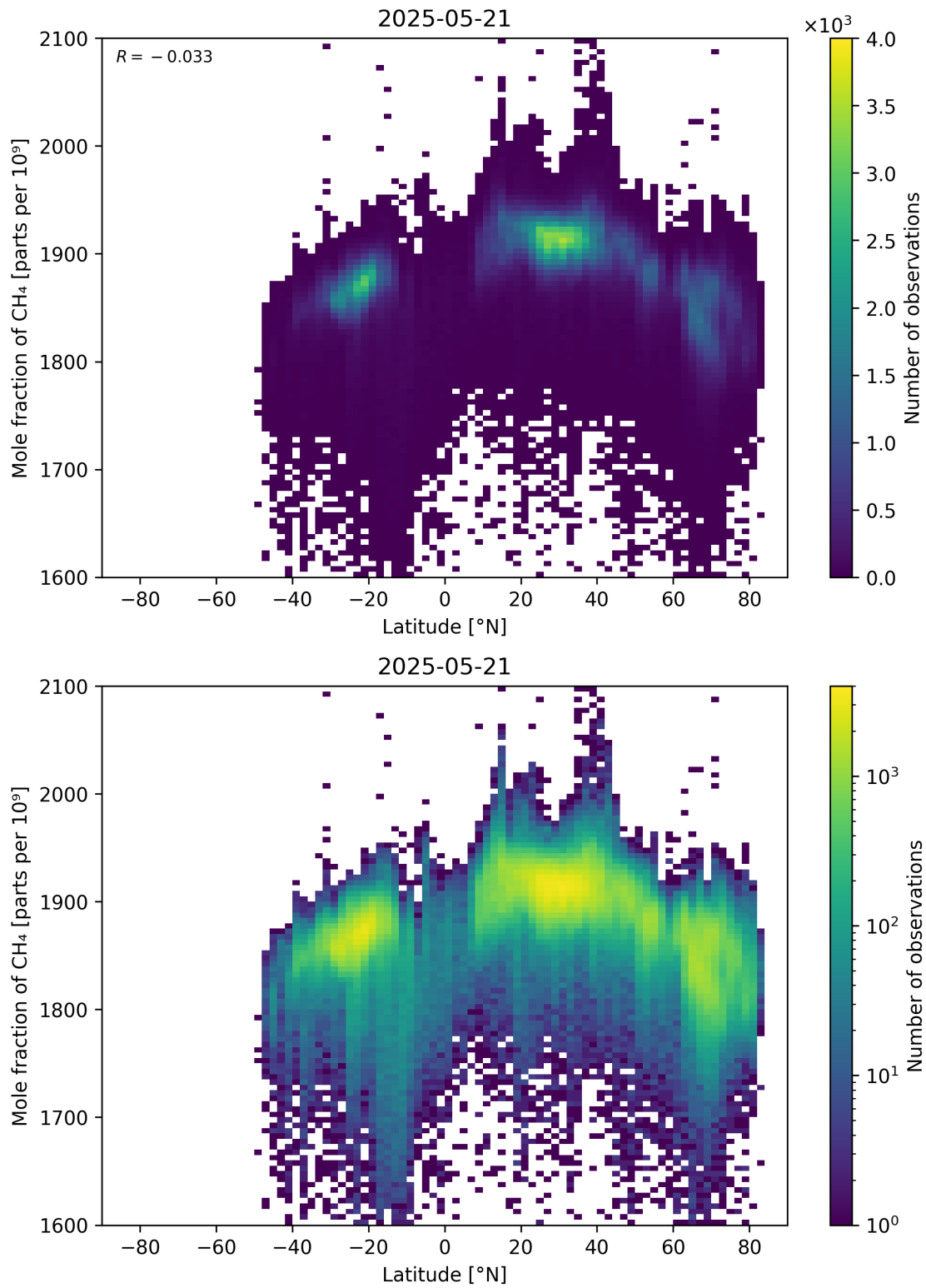
Figure 57: Scatter density plot of “Latitude” against “Mole fraction of CH 4 ” for 2025-05-21 to 2025-05-22.
