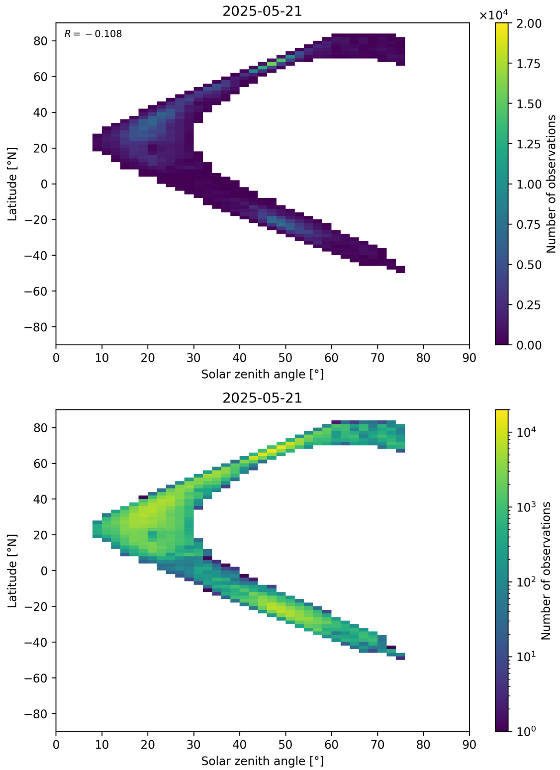
Figure 98: Scatter density plot of “Solar zenith angle” against “Latitude” for 2025-05-21 to 2025-05-22.
