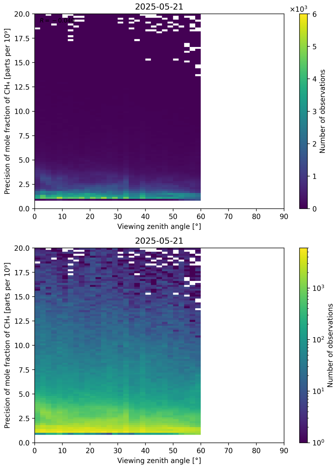
Figure 112: Scatter density plot of “Viewing zenith angle” against “Precision of mole fraction of CH 4 ” for 2025-05-21 to 2025-05-22.
