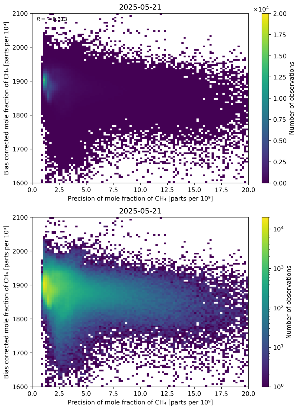
Figure 82: Scatter density plot of “Precision of mole fraction of CH 4 ” against “Bias corrected mole fraction of CH 4 ” for 2025-05-21 to 2025-05-22.
