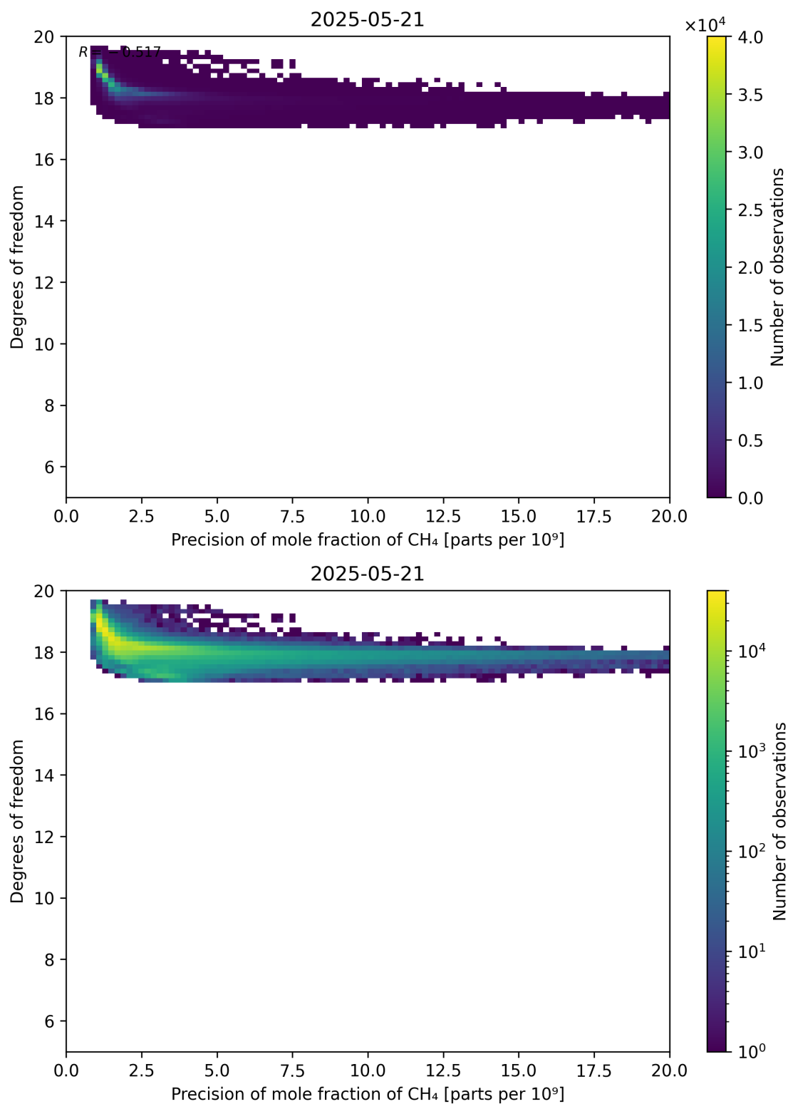
Figure 80: Scatter density plot of “Precision of mole fraction of CH 4 ” against “Degrees of freedom” for 2025-05-21 to 2025-05-22.
