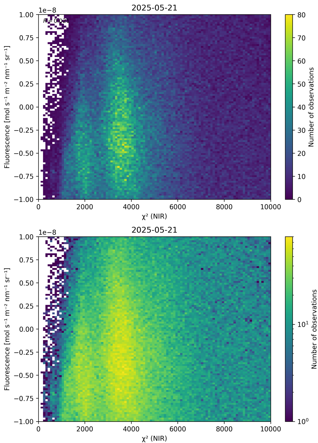
Figure 45: Scatter density plot of “ \chi^2 (NIR)” against “Fluorescence” for 2025-05-21 to 2025-05-22.
