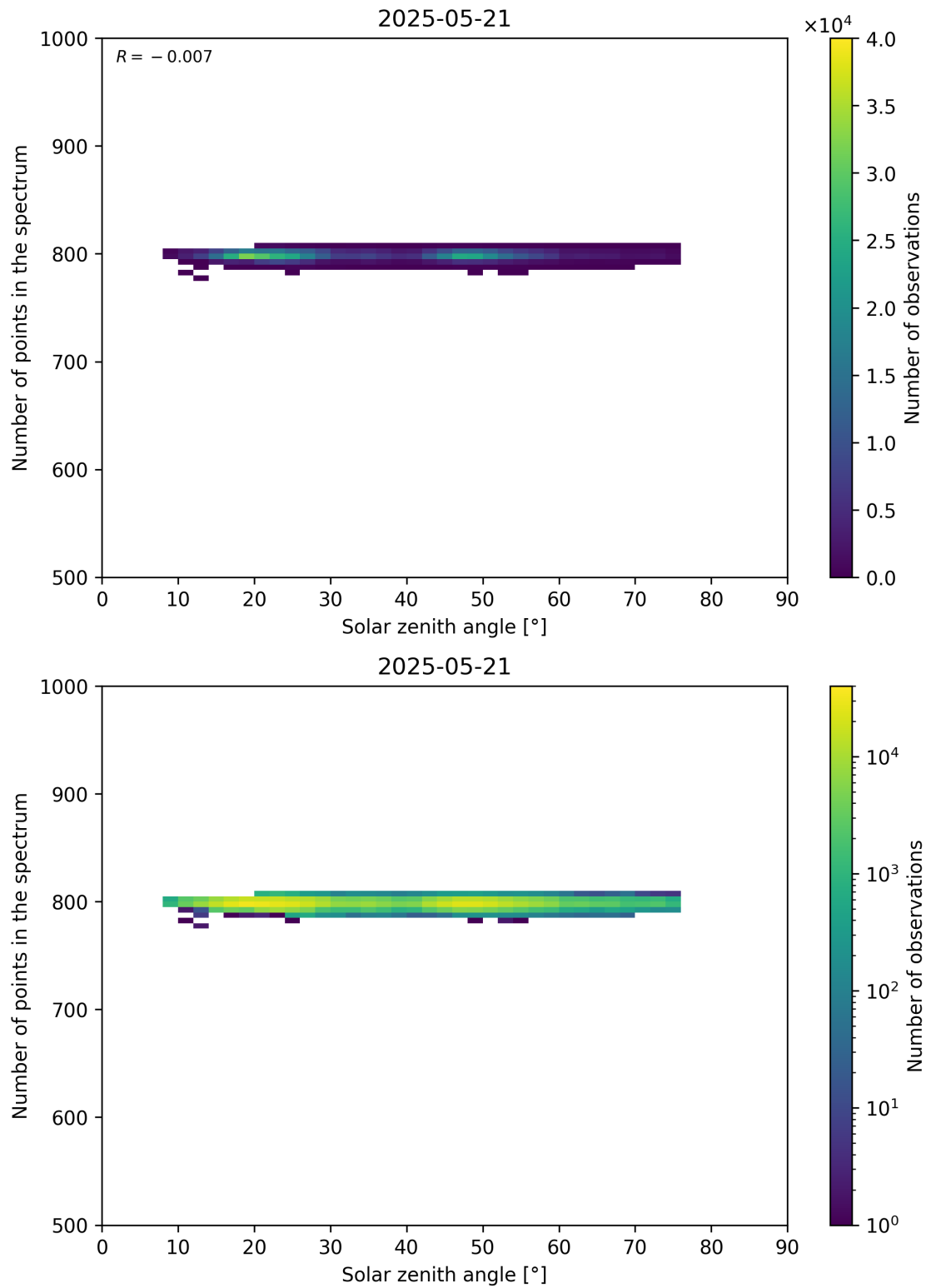
Figure 103: Scatter density plot of “Solar zenith angle” against “Number of points in the spectrum” for 2025-05-21 to 2025-05-22.
