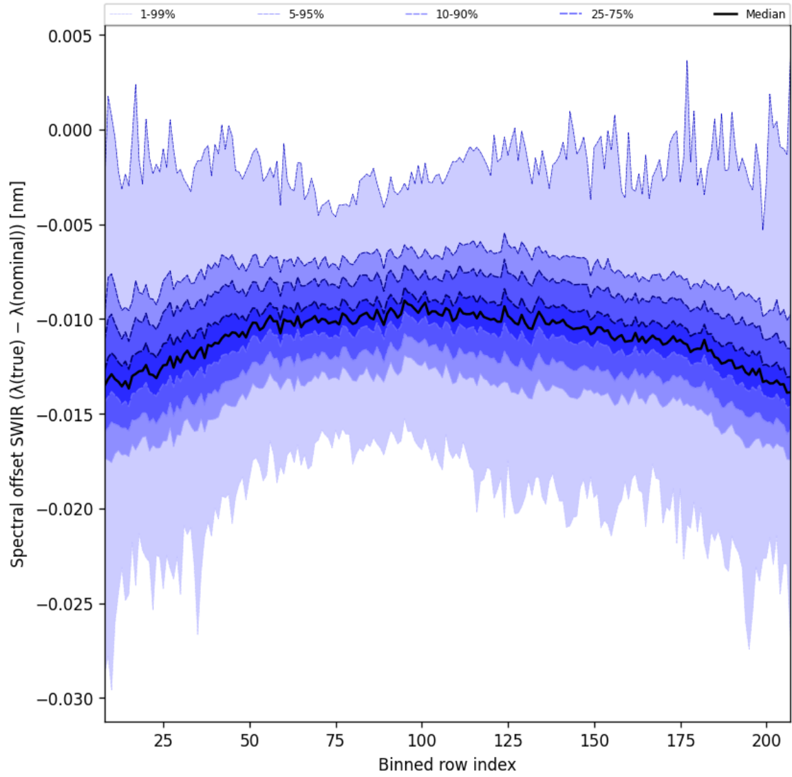
Figure 38: Along track statistics of “Spectral offset SWIR ( \lambda_{\text{true}} - \lambda_{\text{nominal}} )” for 2025-05-21 to 2025-05-22
