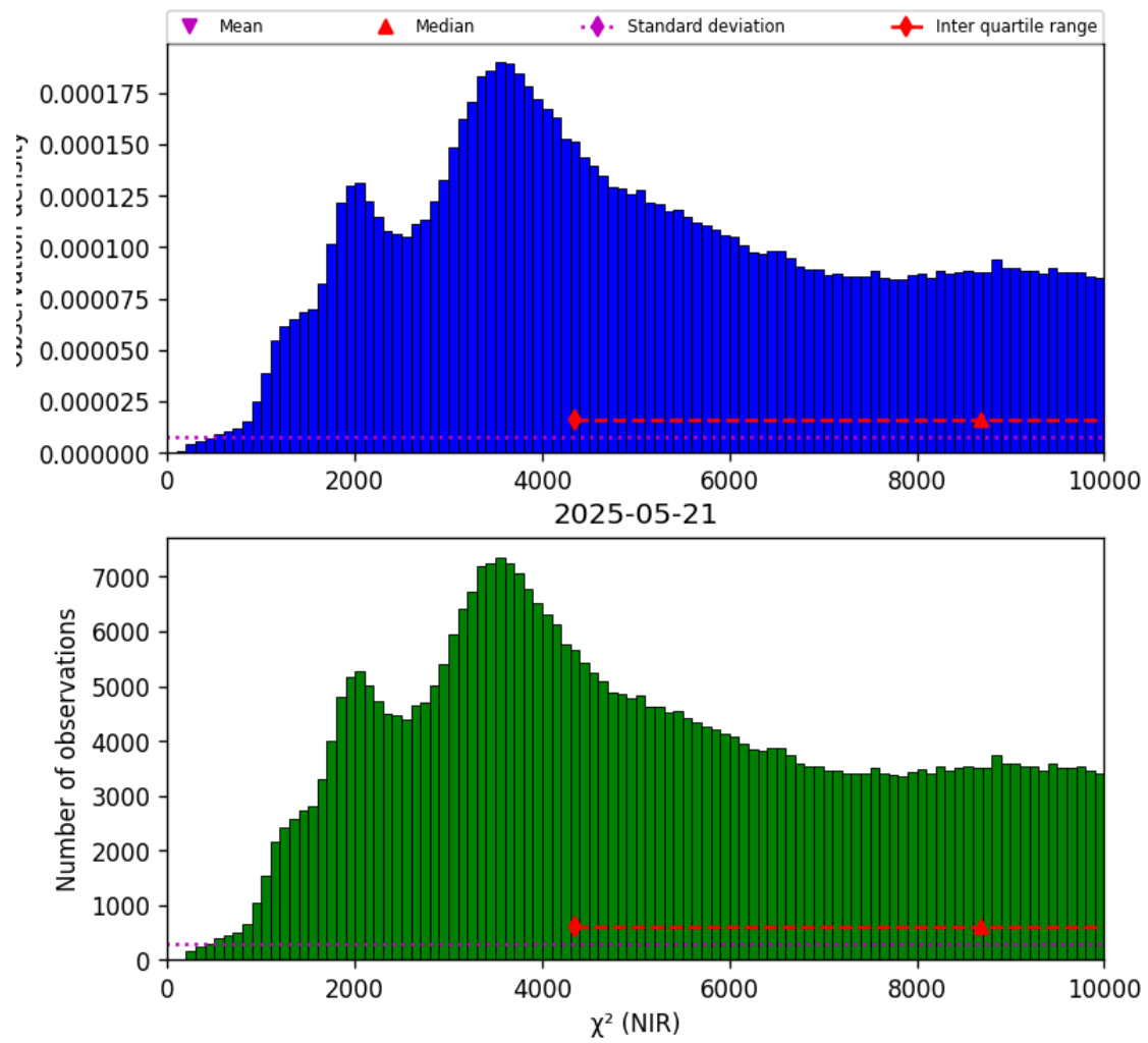
Figure 29: Histogram of “ \chi^2 (NIR)” for 2025-05-21 to 2025-05-22
