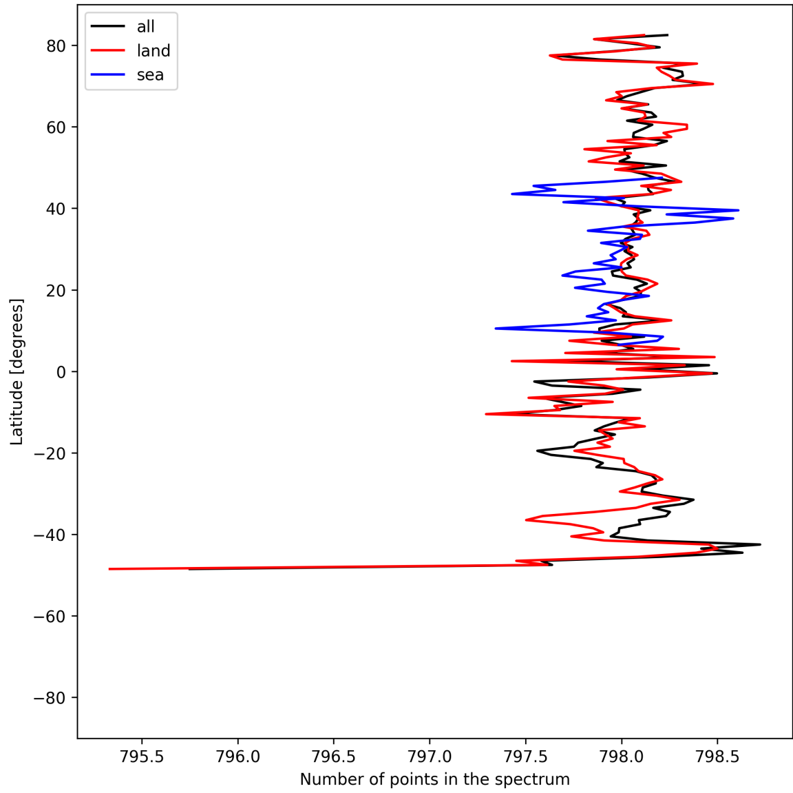
Figure 15: Zonal average of “Number of points in the spectrum” for 2025-05-21 to 2025-05-22.
