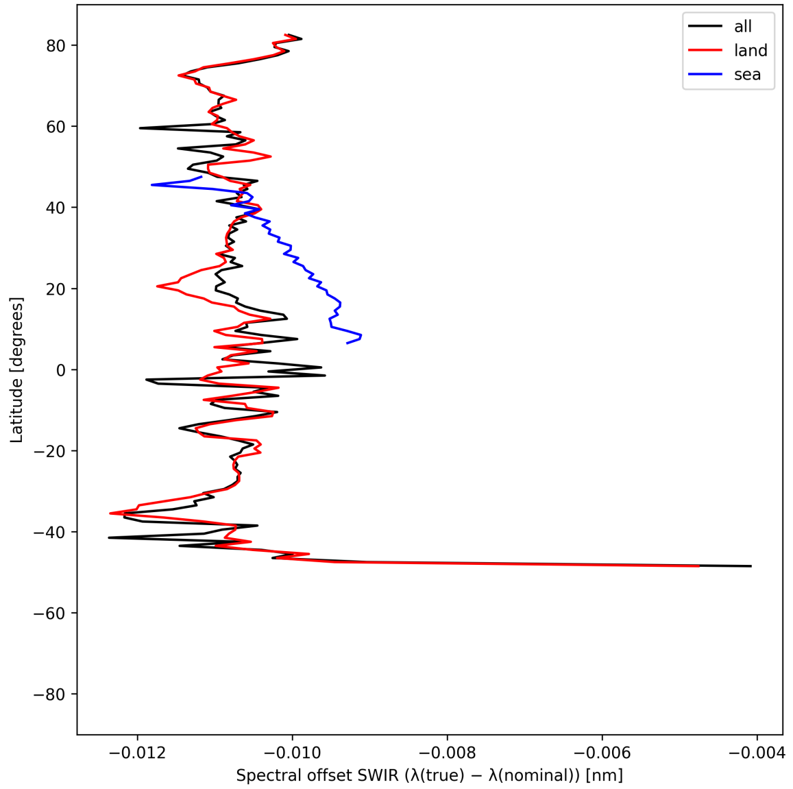
Figure 16: Zonal average of “Spectral offset SWIR ( \lambda_{\text{true}} - \lambda_{\text{nominal}} )” for 2025-05-21 to 2025-05-22.
