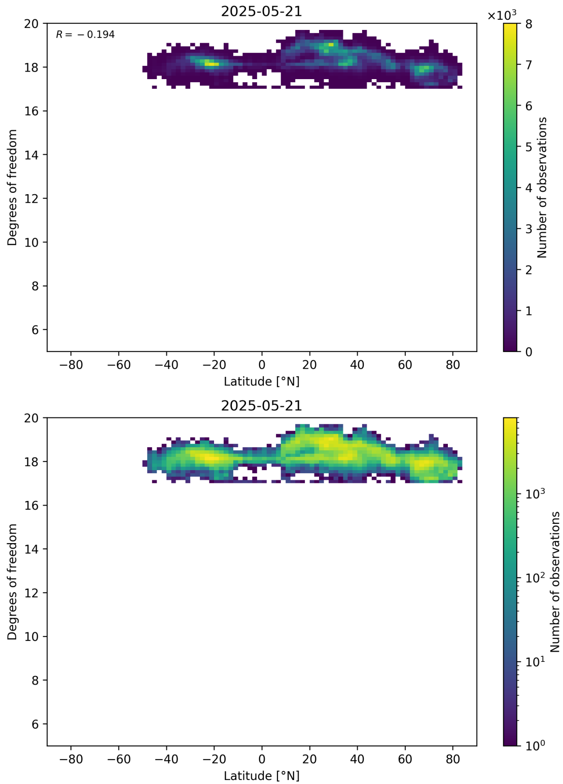
Figure 55: Scatter density plot of “Latitude” against “Degrees of freedom” for 2025-05-21 to 2025-05-22.
