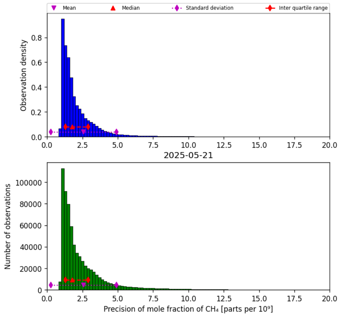
Figure 24: Histogram of “Precision of mole fraction of CH 4 ” for 2025-05-21 to 2025-05-22
