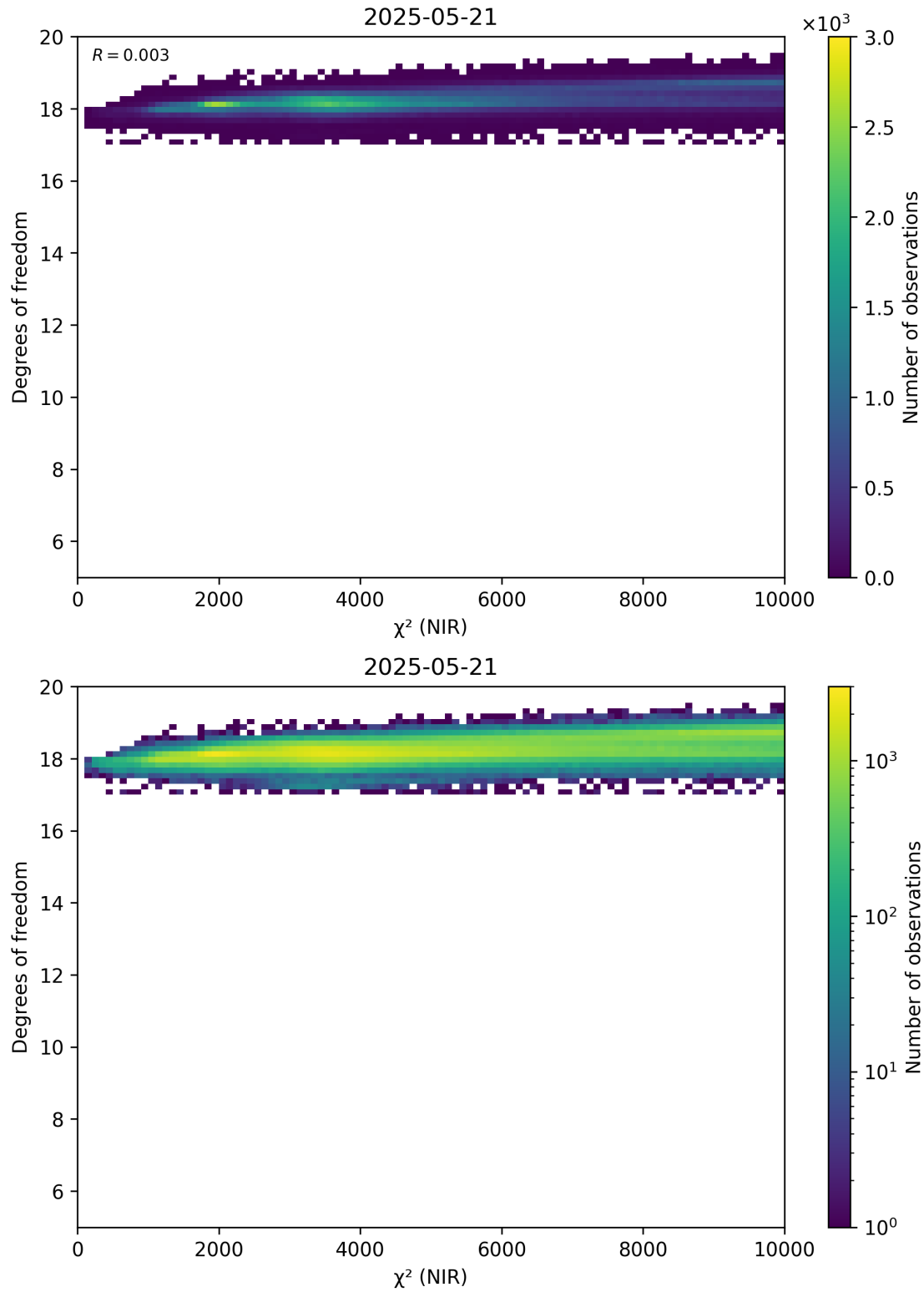
Figure 44: Scatter density plot of “ \chi^2 (NIR)” against “Degrees of freedom” for 2025-05-21 to 2025-05-22.
