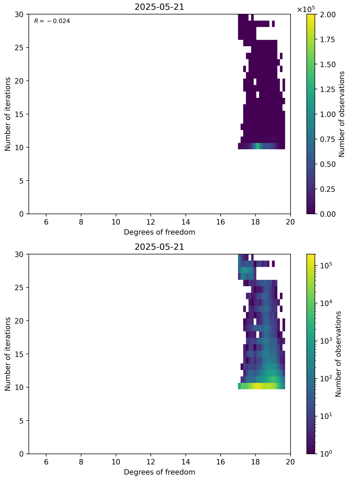
Figure 52: Scatter density plot of “Degrees of freedom” against “Number of iterations” for 2025-05-21 to 2025-05-22.
