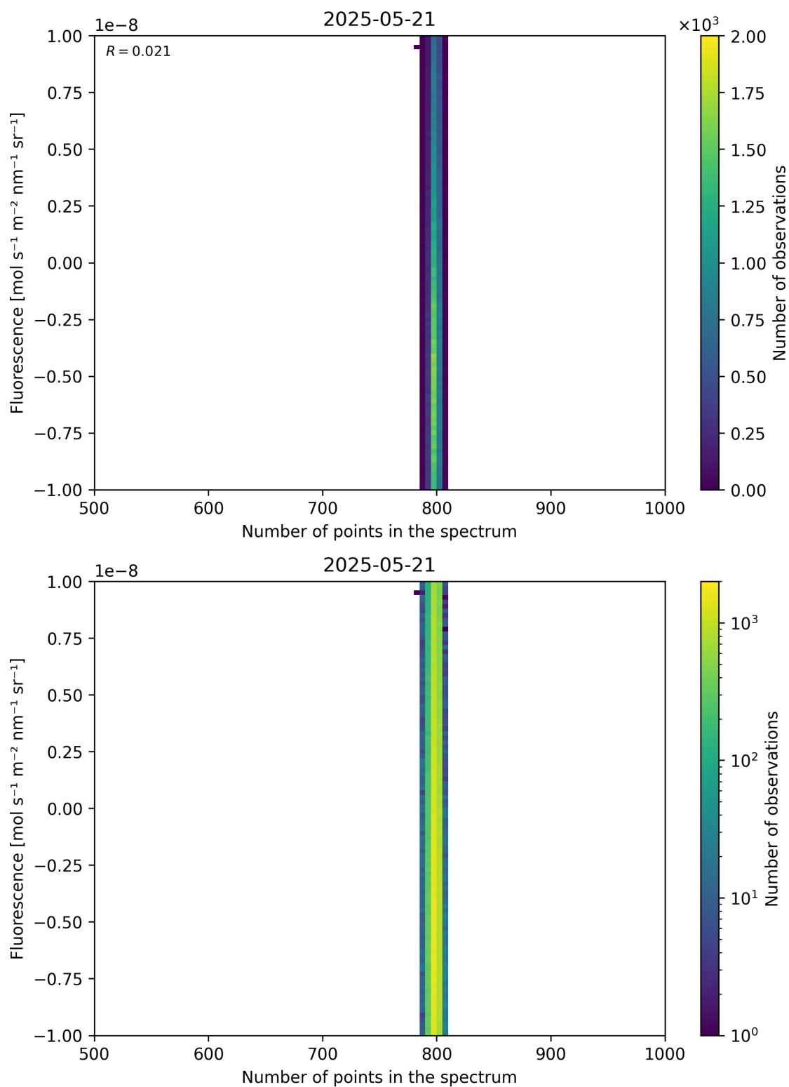
Figure 91: Scatter density plot of “Number of points in the spectrum” against “Fluorescence” for 2025-05-21 to 2025-05-22.
