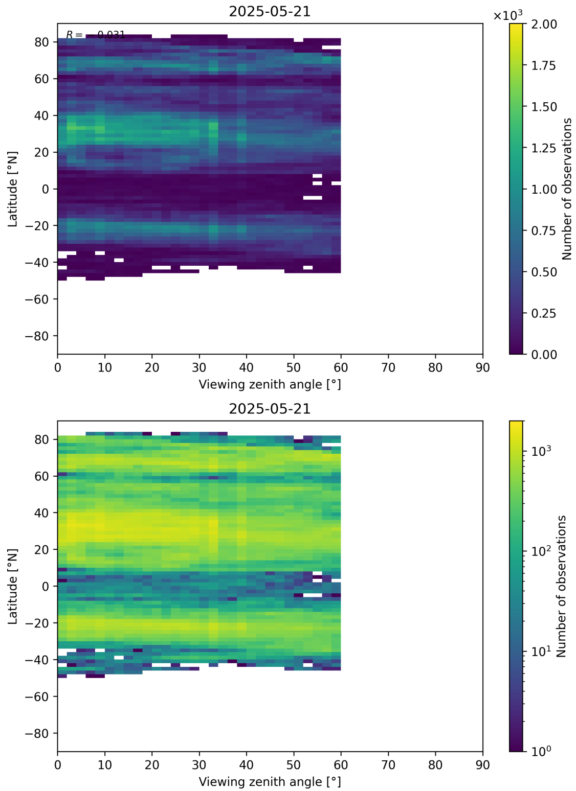
Figure 109: Scatter density plot of “Viewing zenith angle” against “Latitude” for 2025-05-21 to 2025-05-22.
