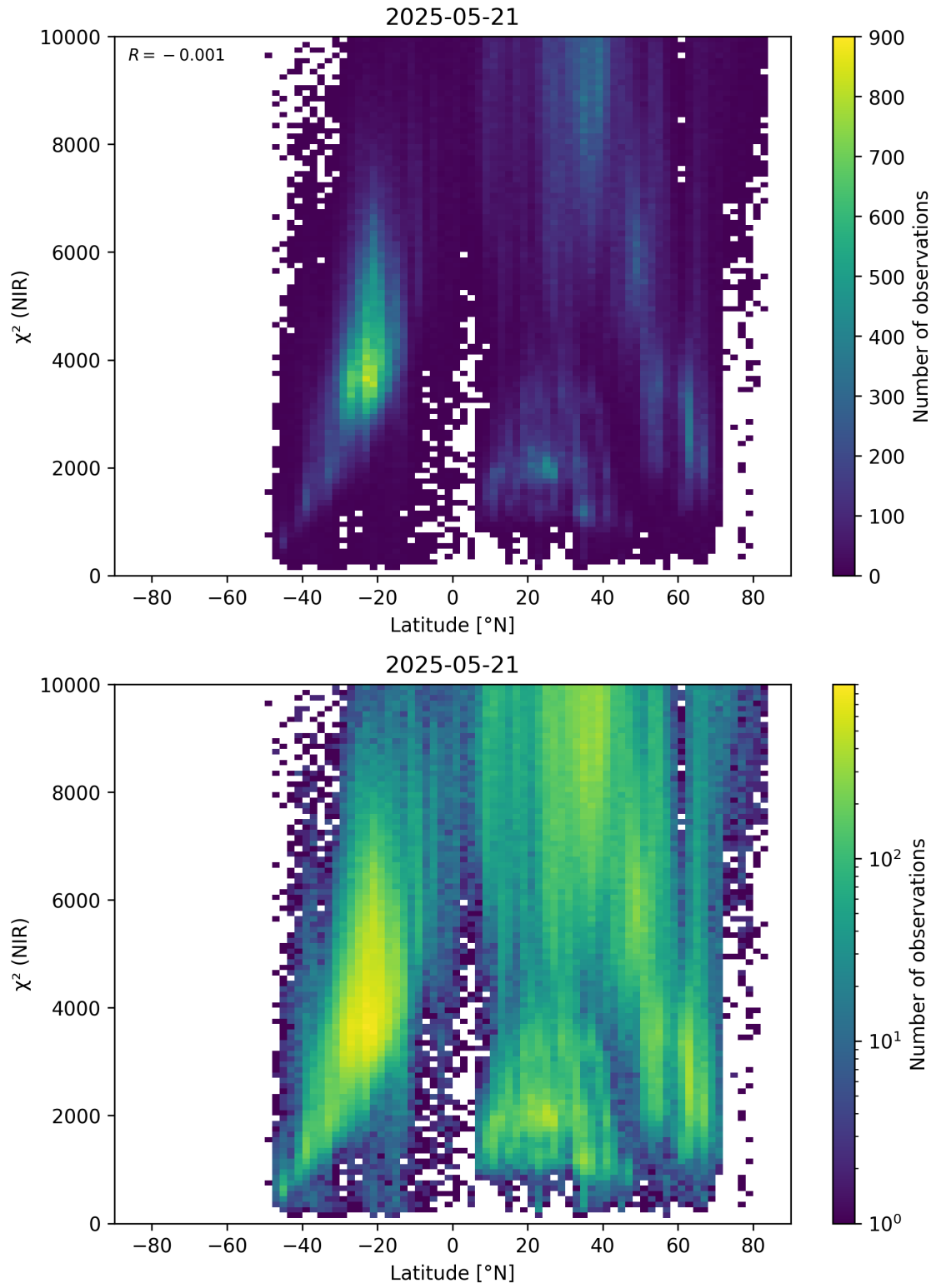
Figure 53: Scatter density plot of “Latitude” against “ \chi^2 (NIR)” for 2025-05-21 to 2025-05-22.
