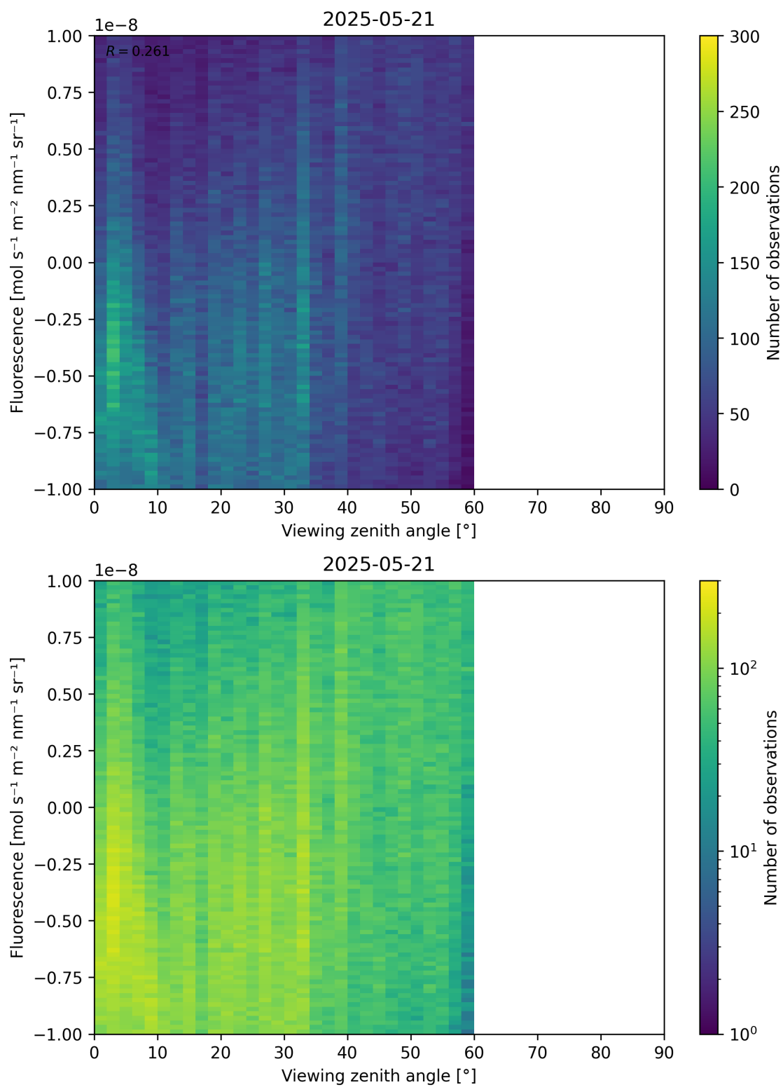
Figure 108: Scatter density plot of “Viewing zenith angle” against “Fluorescence” for 2025-05-21 to 2025-05-22.
