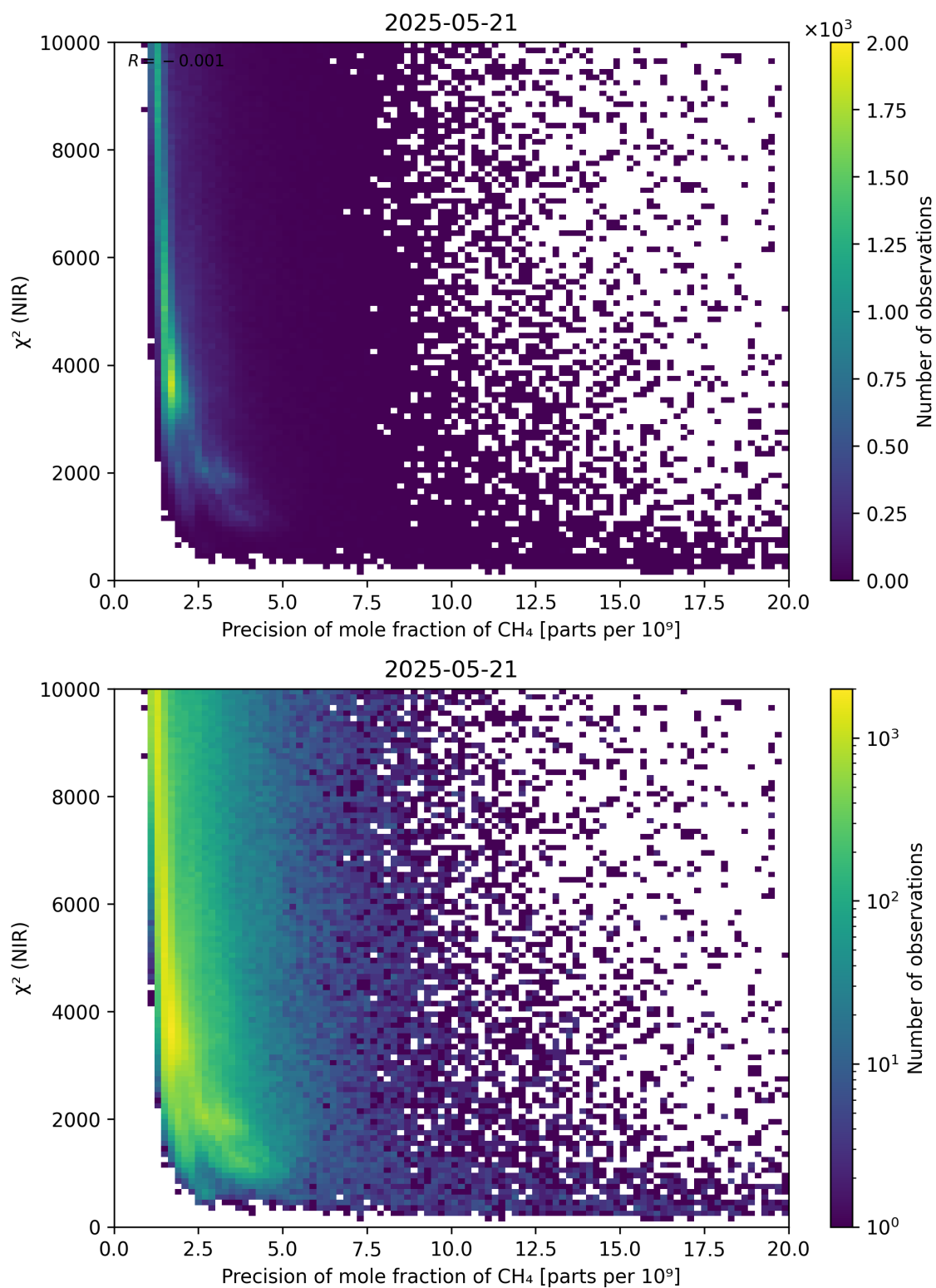
Figure 78: Scatter density plot of “Precision of mole fraction of \text{CH}_4 ” against “ \chi^2 (NIR)” for 2025-05-21 to 2025-05-22.
