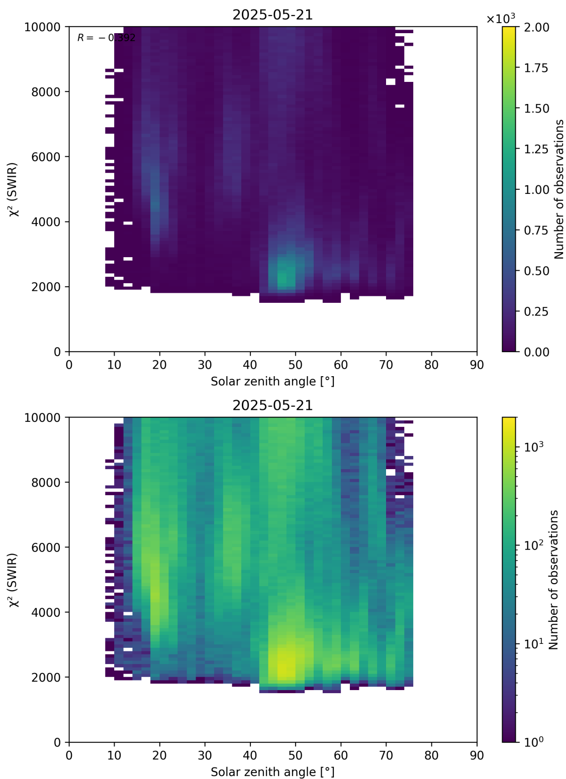
Figure 95: Scatter density plot of “Solar zenith angle” against “ \chi^2 (SWIR)” for 2025-05-21 to 2025-05-22.
