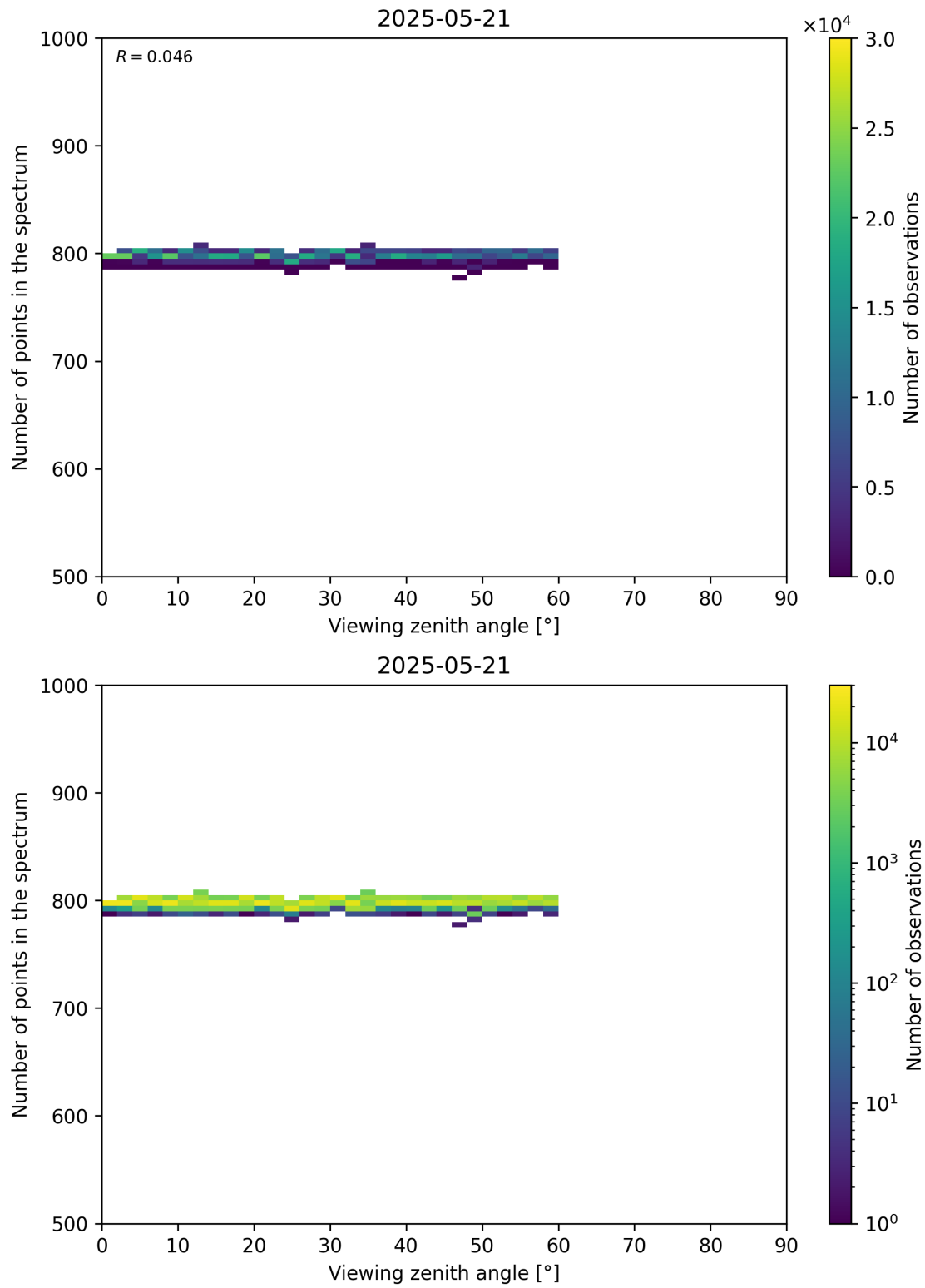
Figure 114: Scatter density plot of “Viewing zenith angle” against “Number of points in the spectrum” for 2025-05-21 to 2025-05-22.
