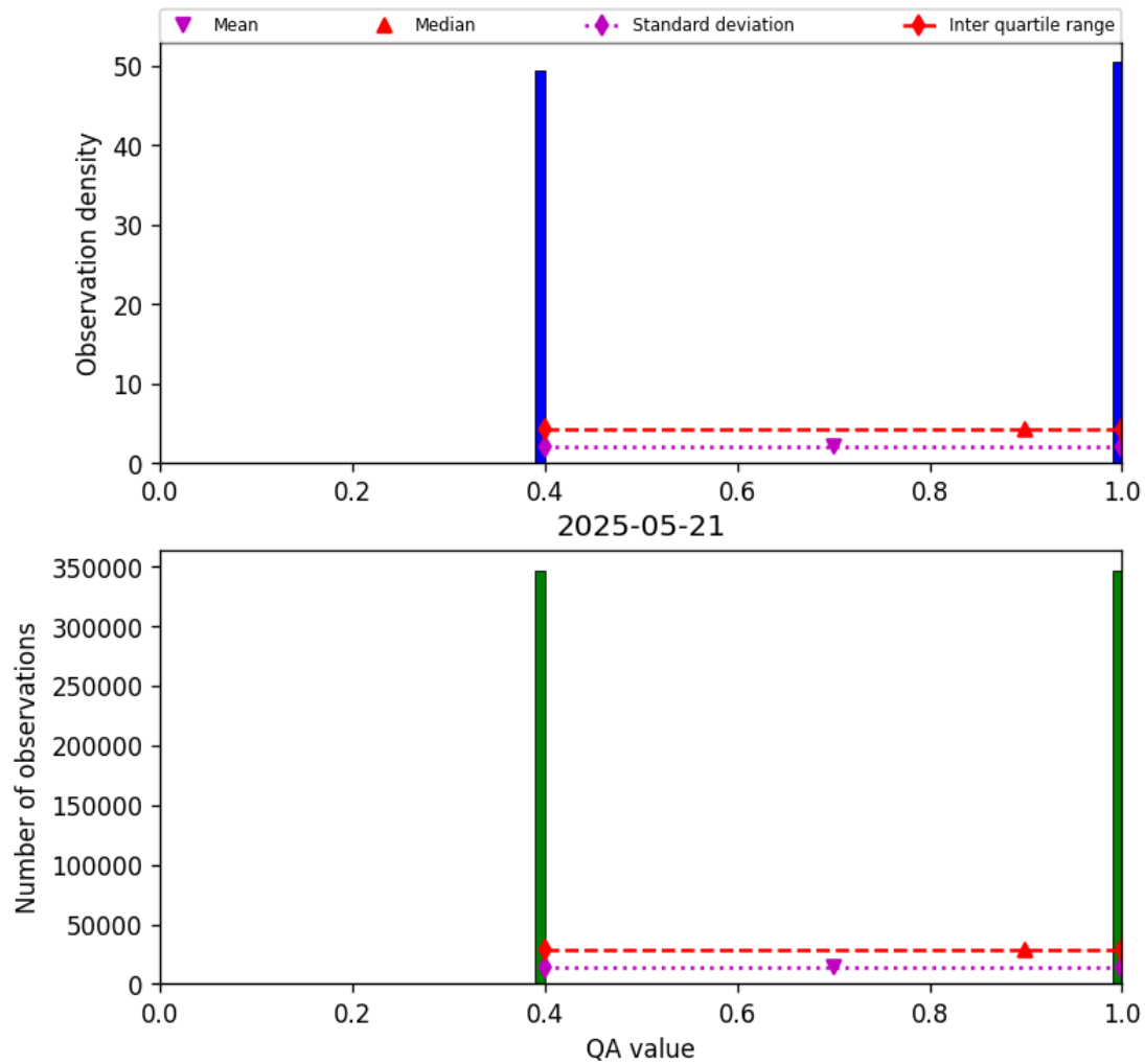
Figure 22: Histogram of “QA value” for 2025-05-21 to 2025-05-22
