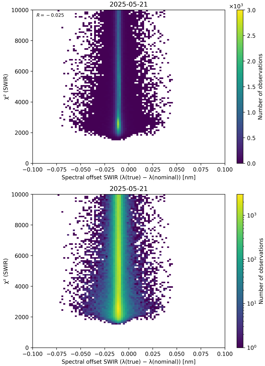
Figure 118: Scatter density plot of “Spectral offset SWIR ( \lambda_{\text{true}} - \lambda_{\text{nominal}} )” against “ \chi^2 (SWIR)” for 2025-05-21 to 2025-05-22.
