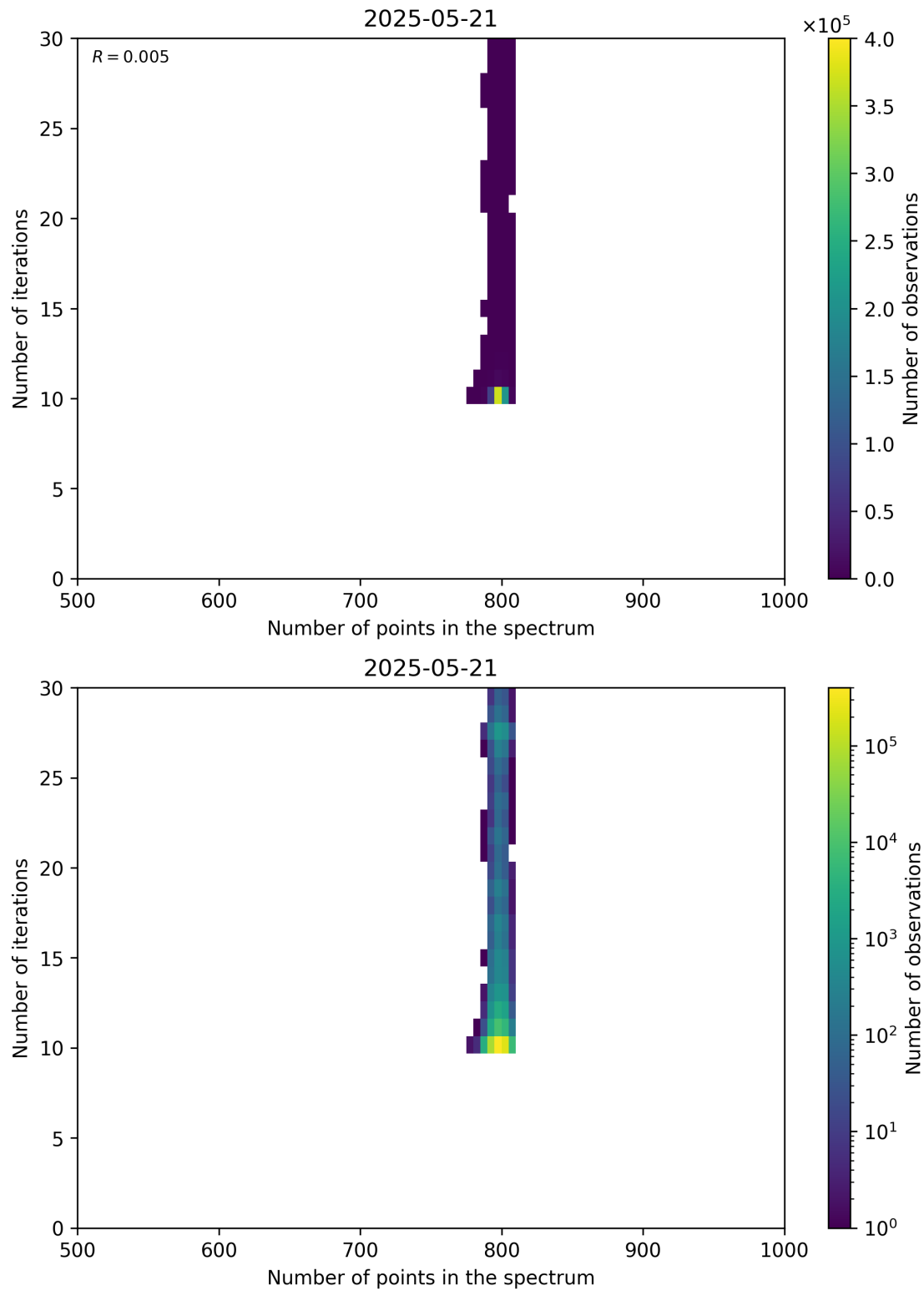
Figure 92: Scatter density plot of “Number of points in the spectrum” against “Number of iterations” for 2025-05-21 to 2025-05-22.
