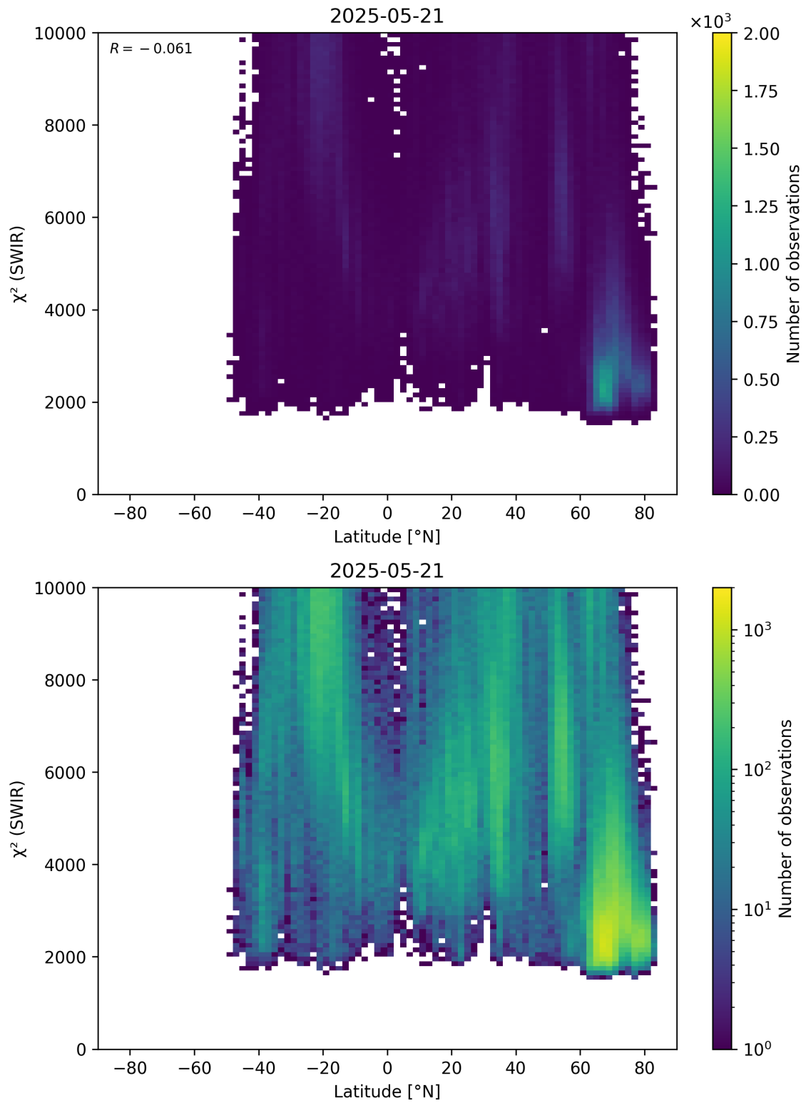
Figure 54: Scatter density plot of “Latitude” against “ \chi^2 (SWIR)” for 2025-05-21 to 2025-05-22.
