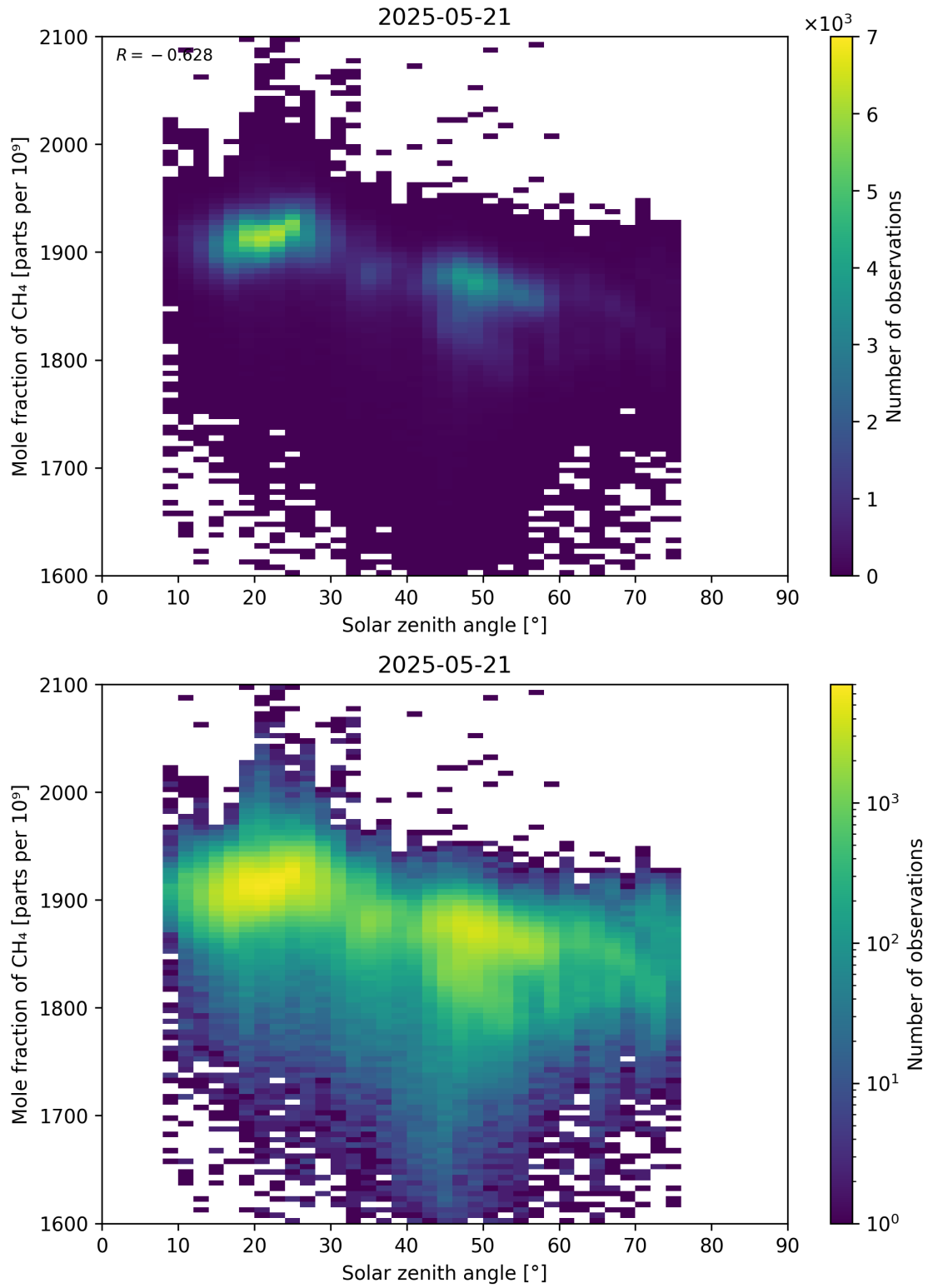
Figure 99: Scatter density plot of “Solar zenith angle” against “Mole fraction of CH 4 ” for 2025-05-21 to 2025-05-22.
