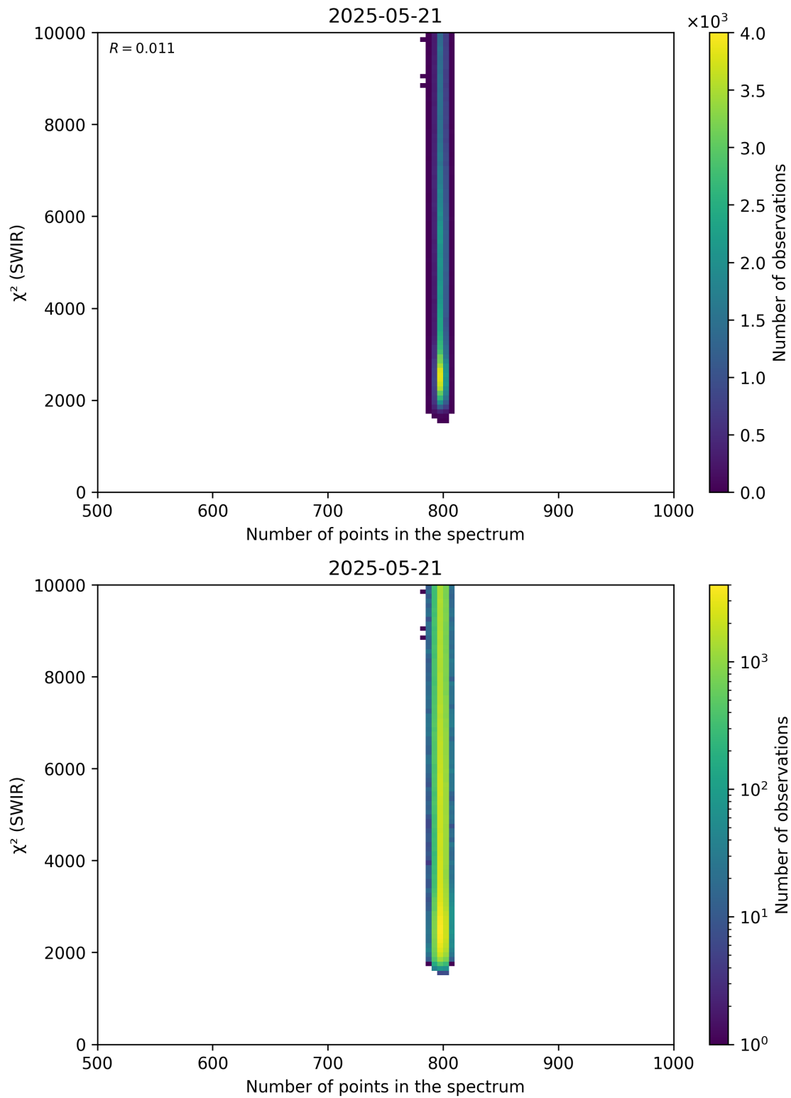
Figure 89: Scatter density plot of “Number of points in the spectrum” against “ \chi^2 (SWIR)” for 2025-05-21 to 2025-05-22.
