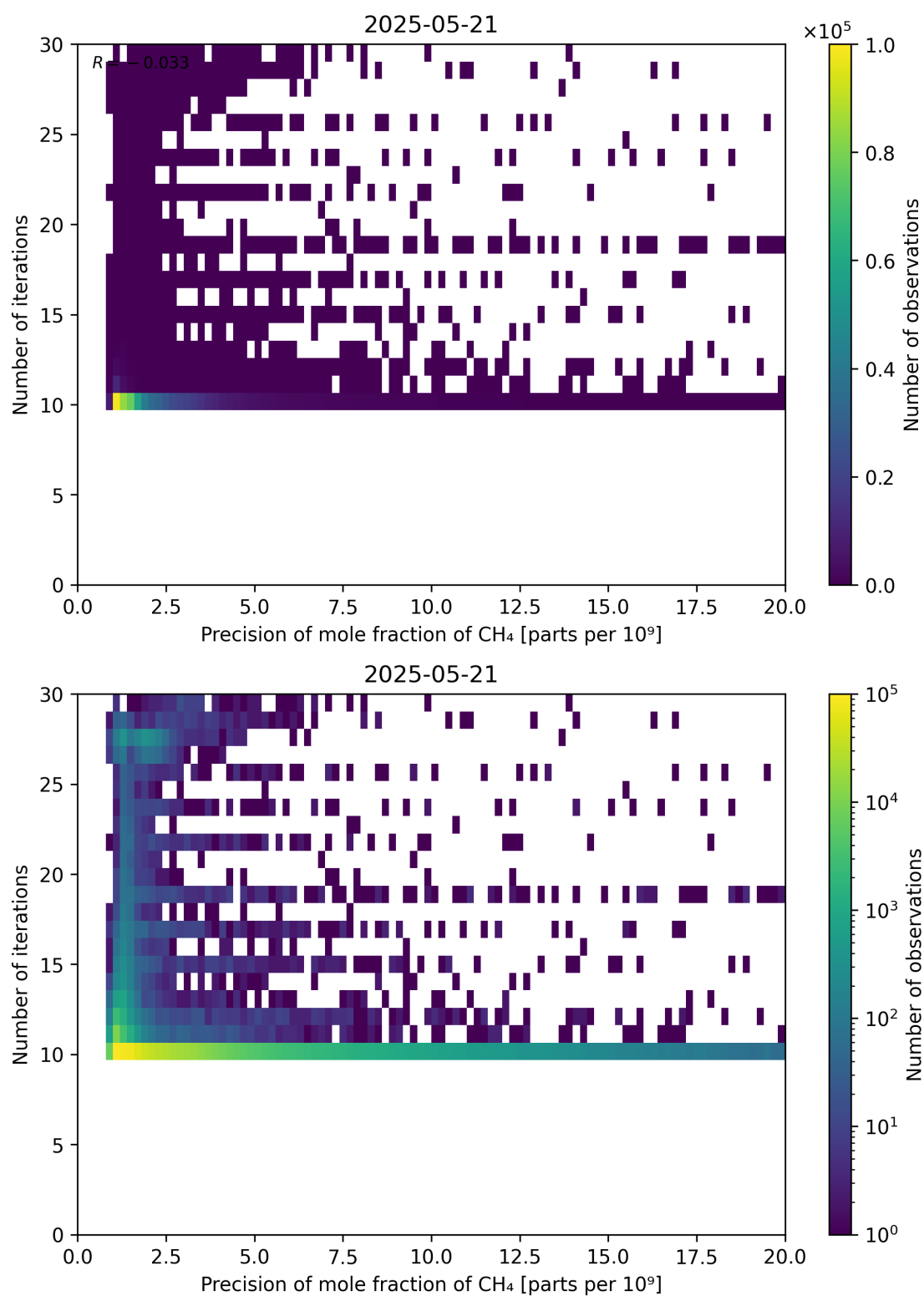
Figure 83: Scatter density plot of “Precision of mole fraction of CH 4 ” against “Number of iterations” for 2025-05-21 to 2025-05-22.
