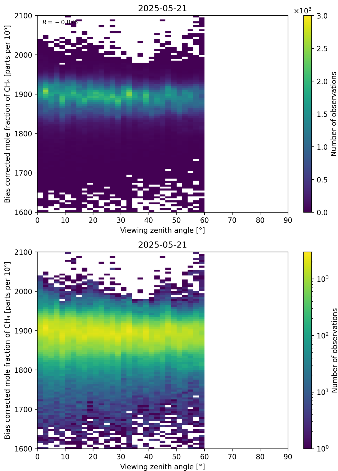
Figure 111: Scatter density plot of “Viewing zenith angle” against “Bias corrected mole fraction of CH 4 ” for 2025-05-21 to 2025-05-22.
