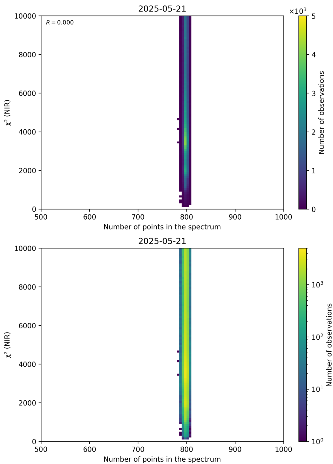
Figure 88: Scatter density plot of “Number of points in the spectrum” against “ \chi^2 (NIR)” for 2025-05-21 to 2025-05-22.
