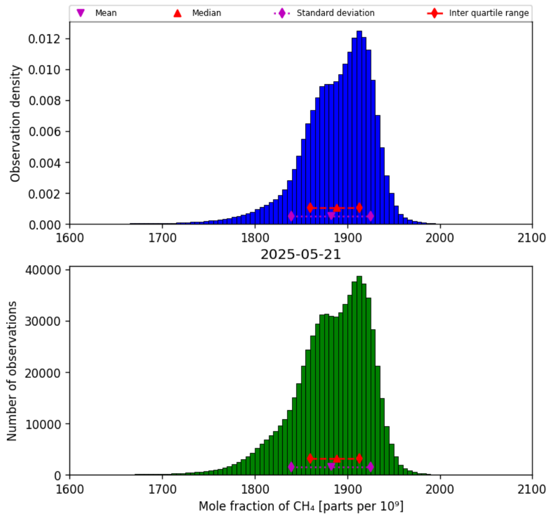
Figure 23: Histogram of “Mole fraction of CH 4 ” for 2025-05-21 to 2025-05-22
