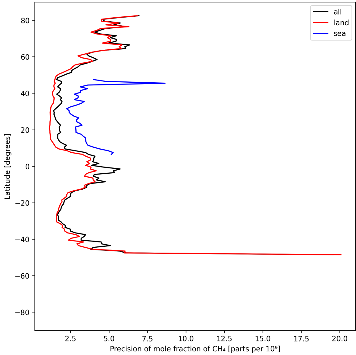
Figure 13: Zonal average of “Precision of mole fraction of CH 4 ” for 2025-05-21 to 2025-05-22.
