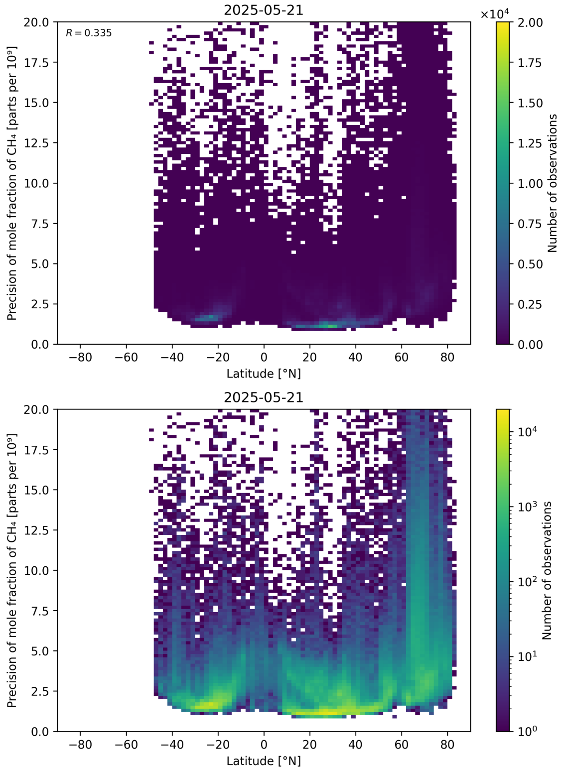
Figure 59: Scatter density plot of “Latitude” against “Precision of mole fraction of \text{CH}_4 ” for 2025-05-21 to 2025-05-22.
