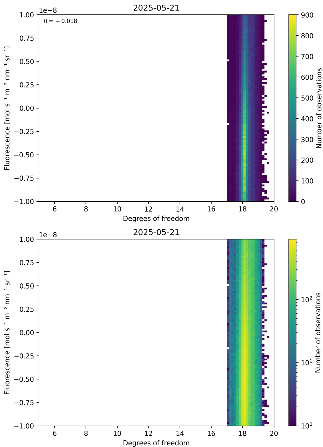
Figure 51: Scatter density plot of “Degrees of freedom” against “Fluorescence” for 2025-05-21 to 2025-05-22.
