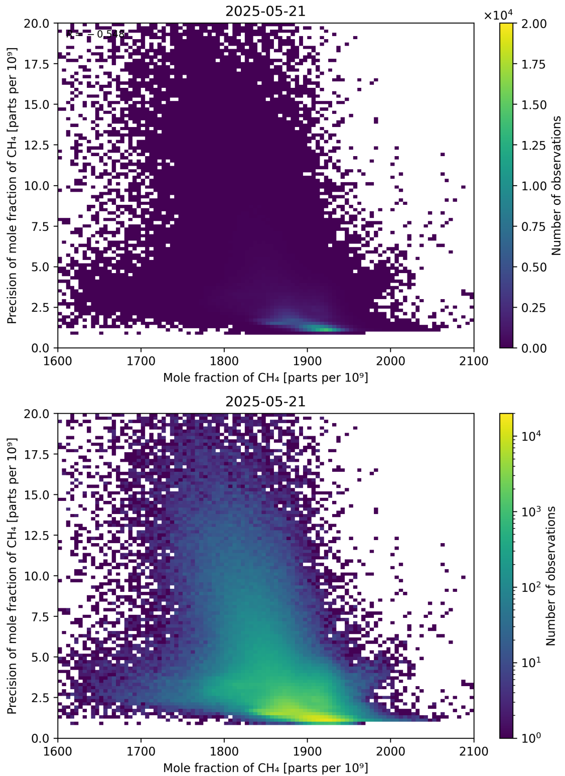
Figure 75: Scatter density plot of “Mole fraction of CH 4 ” against “Precision of mole fraction of CH 4 ” for 2025-05-21 to 2025-05-22.
