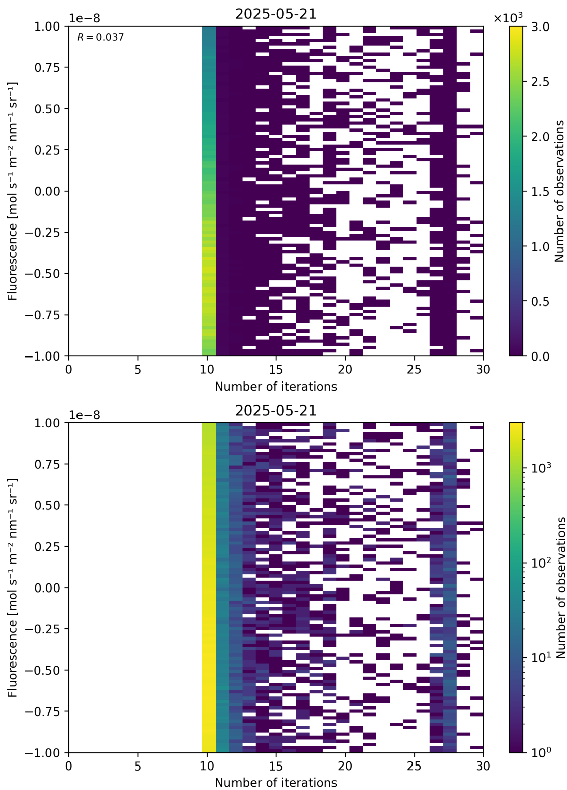
Figure 87: Scatter density plot of “Number of iterations” against “Fluorescence” for 2025-05-21 to 2025-05-22.
