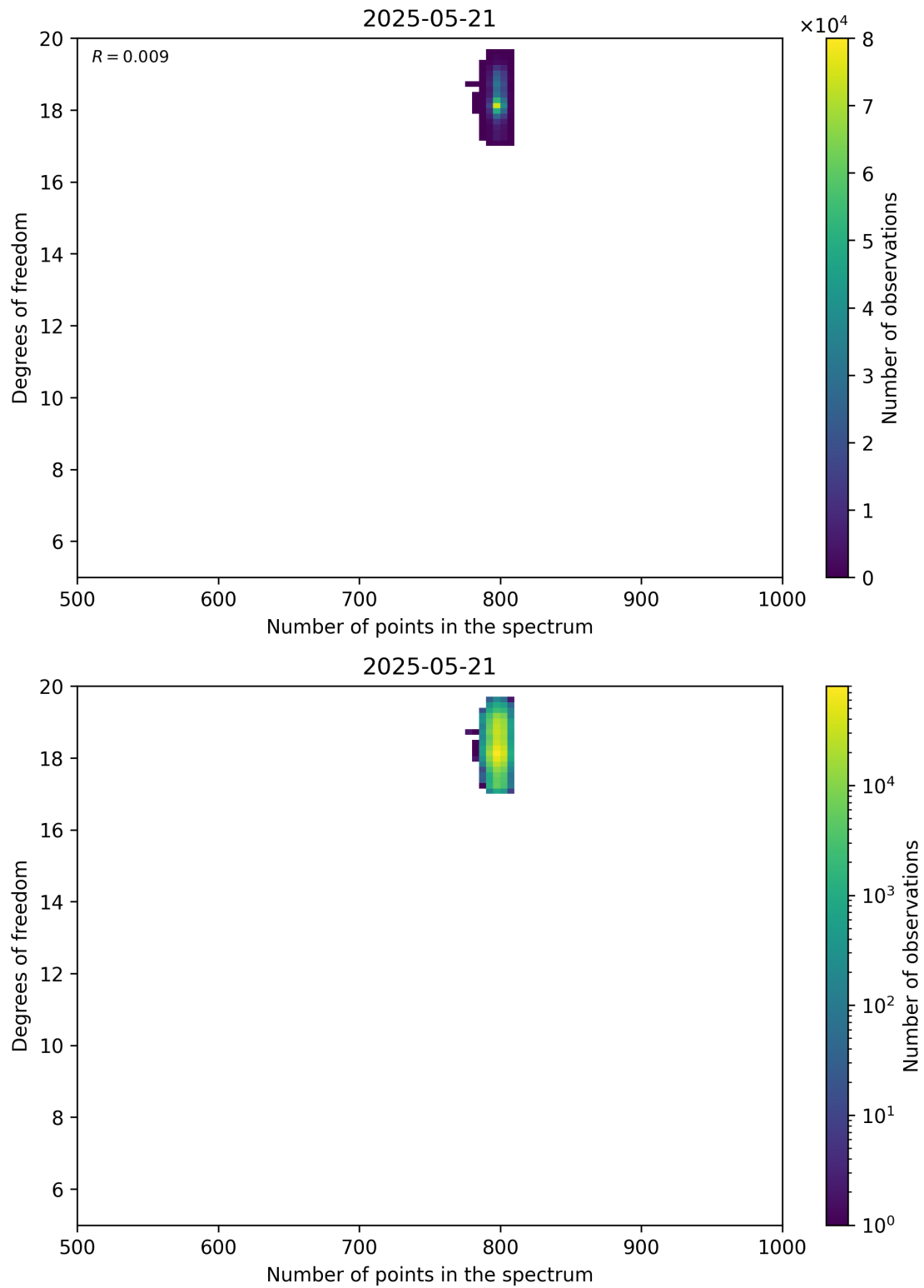
Figure 90: Scatter density plot of “Number of points in the spectrum” against “Degrees of freedom” for 2025-05-21 to 2025-05-22.
