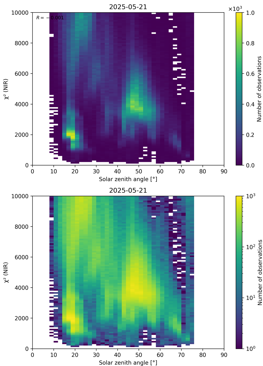
Figure 94: Scatter density plot of “Solar zenith angle” against “ \chi^2 (NIR)” for 2025-05-21 to 2025-05-22.
