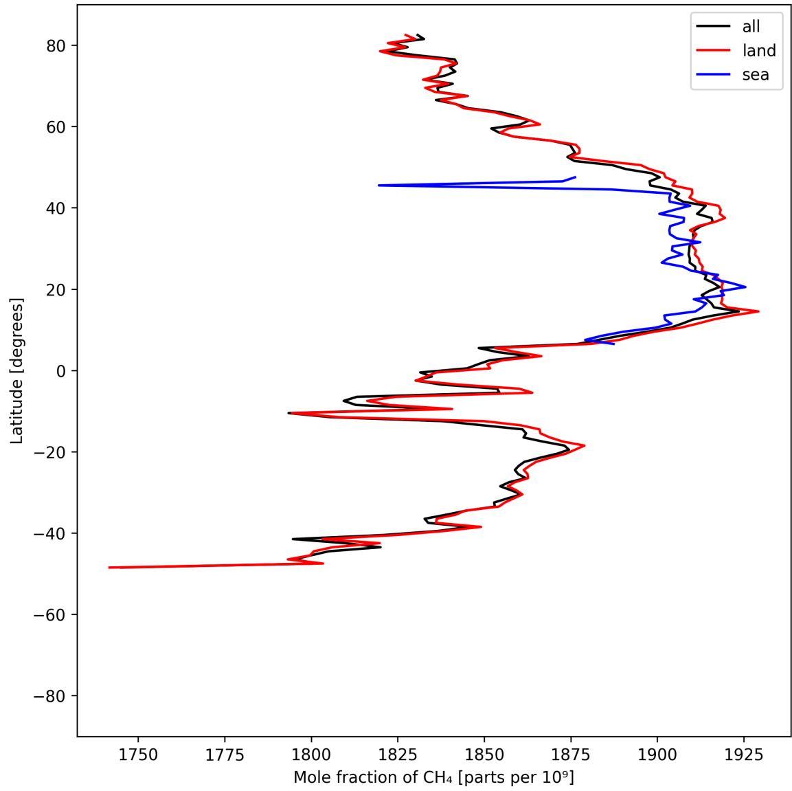
Figure 12: Zonal average of “Mole fraction of CH 4 ” for 2025-05-21 to 2025-05-22.
