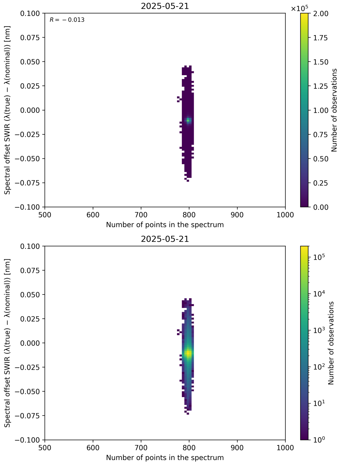
Figure 93: Scatter density plot of “Number of points in the spectrum” against “Spectral offset SWIR ( \lambda_{\text{true}} - \lambda_{\text{nominal}} )” for 2025-05-21 to 2025-05-22.
