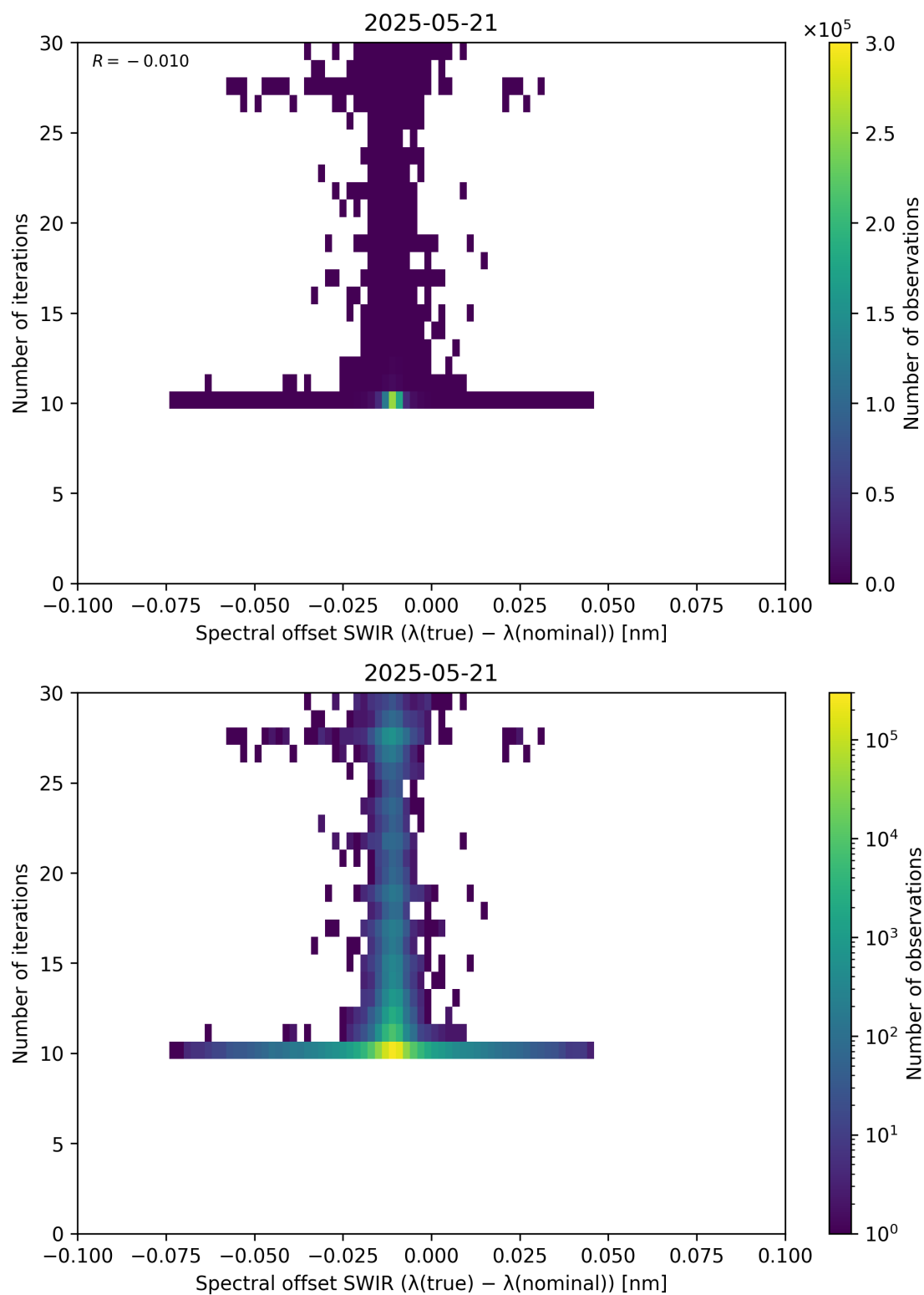
Figure 121: Scatter density plot of “Spectral offset SWIR ( \lambda_{\text{true}} - \lambda_{\text{nominal}} )” against “Number of iterations” for 2025-05-21 to 2025-05-22.
