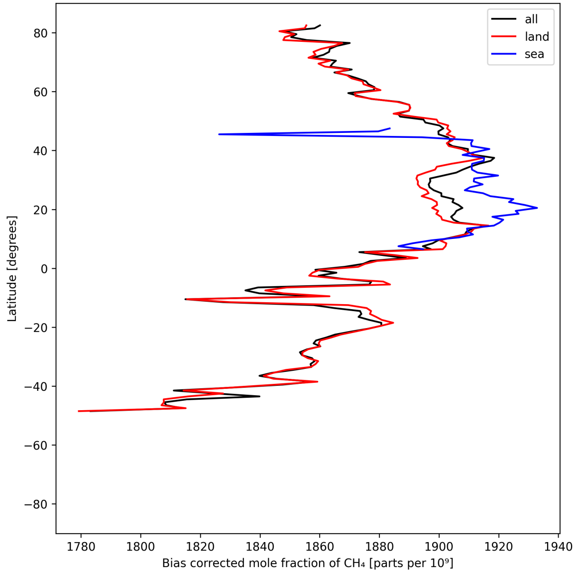
Figure 14: Zonal average of “Bias corrected mole fraction of \text{CH}_4 ” for 2025-05-21 to 2025-05-22.
