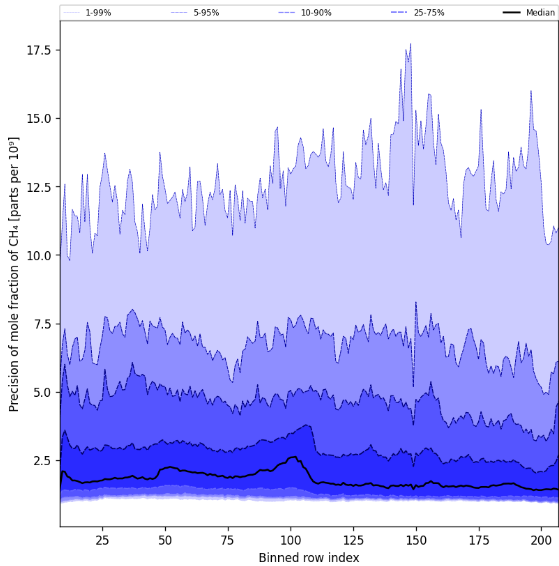
Figure 35: Along track statistics of “Precision of mole fraction of CH 4 ” for 2025-05-21 to 2025-05-22
