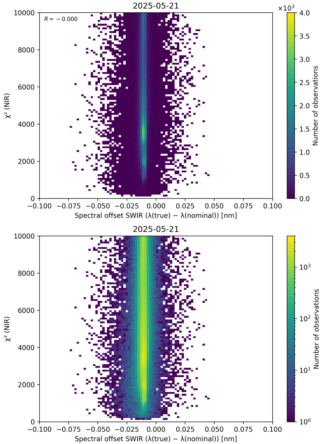
Figure 117: Scatter density plot of “Spectral offset SWIR ( \lambda_{\text{true}} - \lambda_{\text{nominal}} )” against “ \chi^2 (NIR)” for 2025-05-21 to 2025-05-22.
