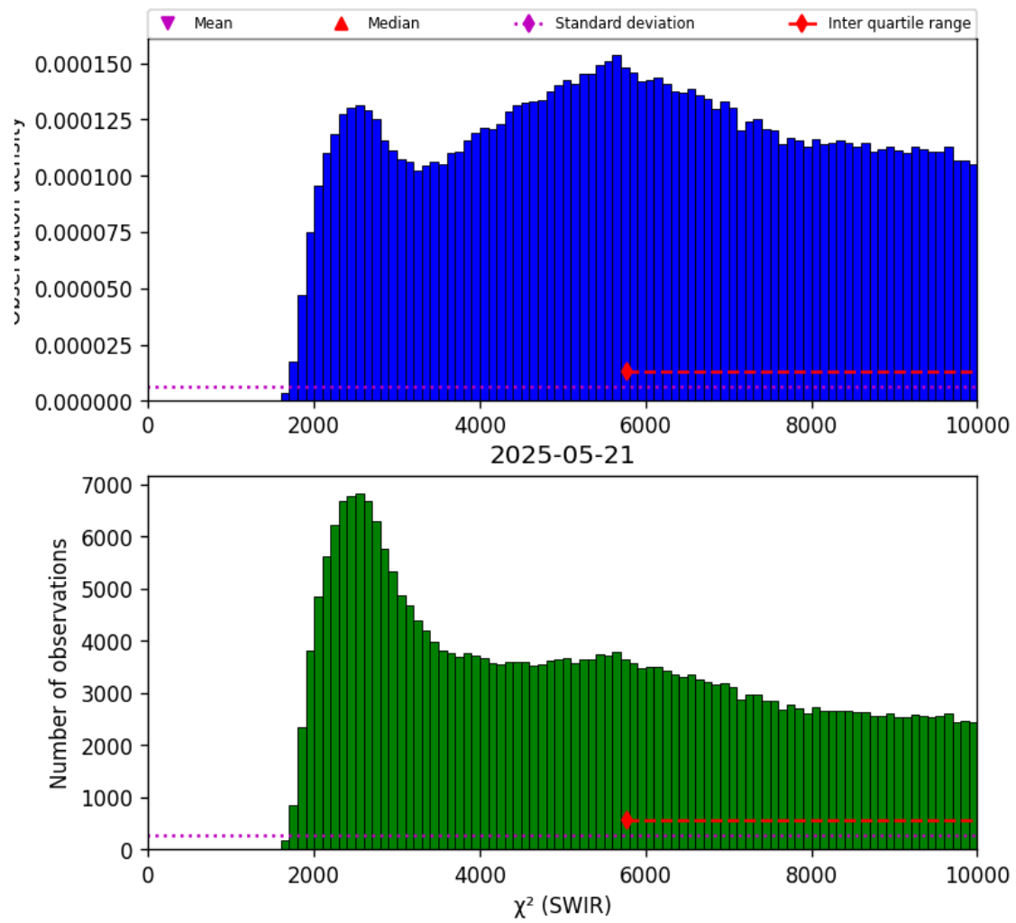
Figure 28: Histogram of “ \chi^2 (SWIR)” for 2025-05-21 to 2025-05-22
