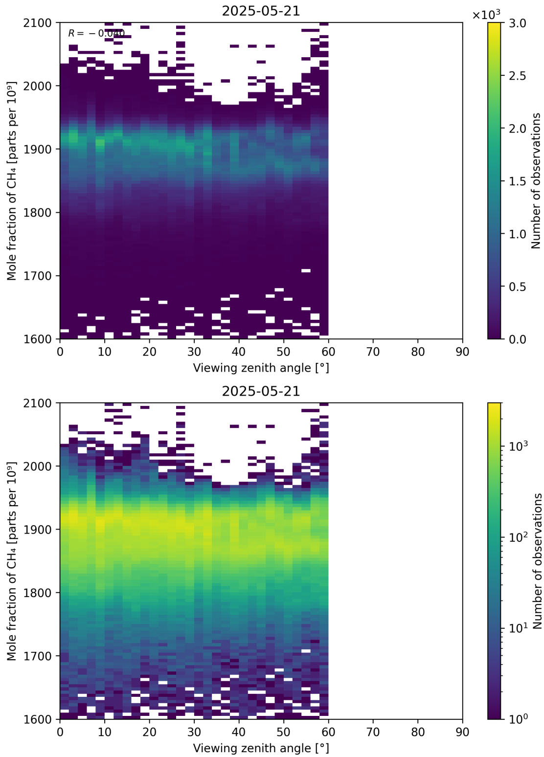
Figure 110: Scatter density plot of “Viewing zenith angle” against “Mole fraction of CH 4 ” for 2025-05-21 to 2025-05-22.
