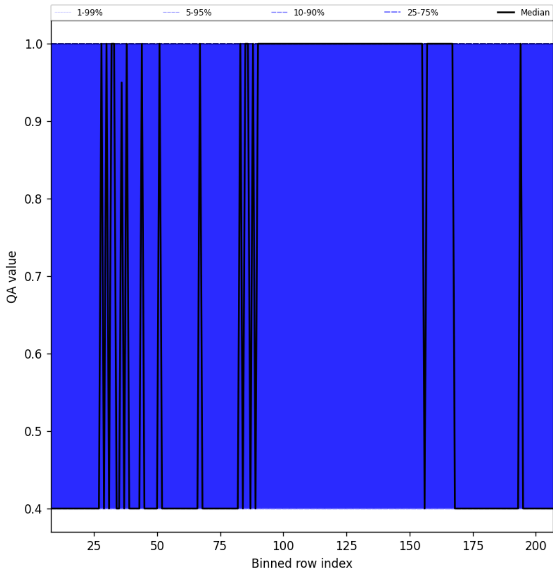
Figure 33: Along track statistics of “QA value” for 2025-05-21 to 2025-05-22
