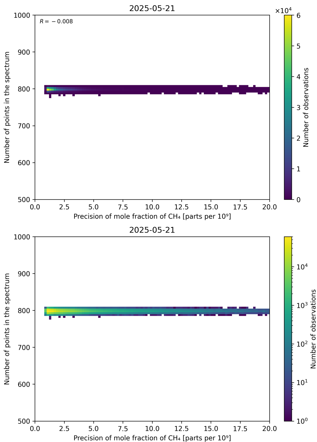
Figure 84: Scatter density plot of “Precision of mole fraction of CH 4 ” against “Number of points in the spectrum” for 2025-05-21 to 2025-05-22.
