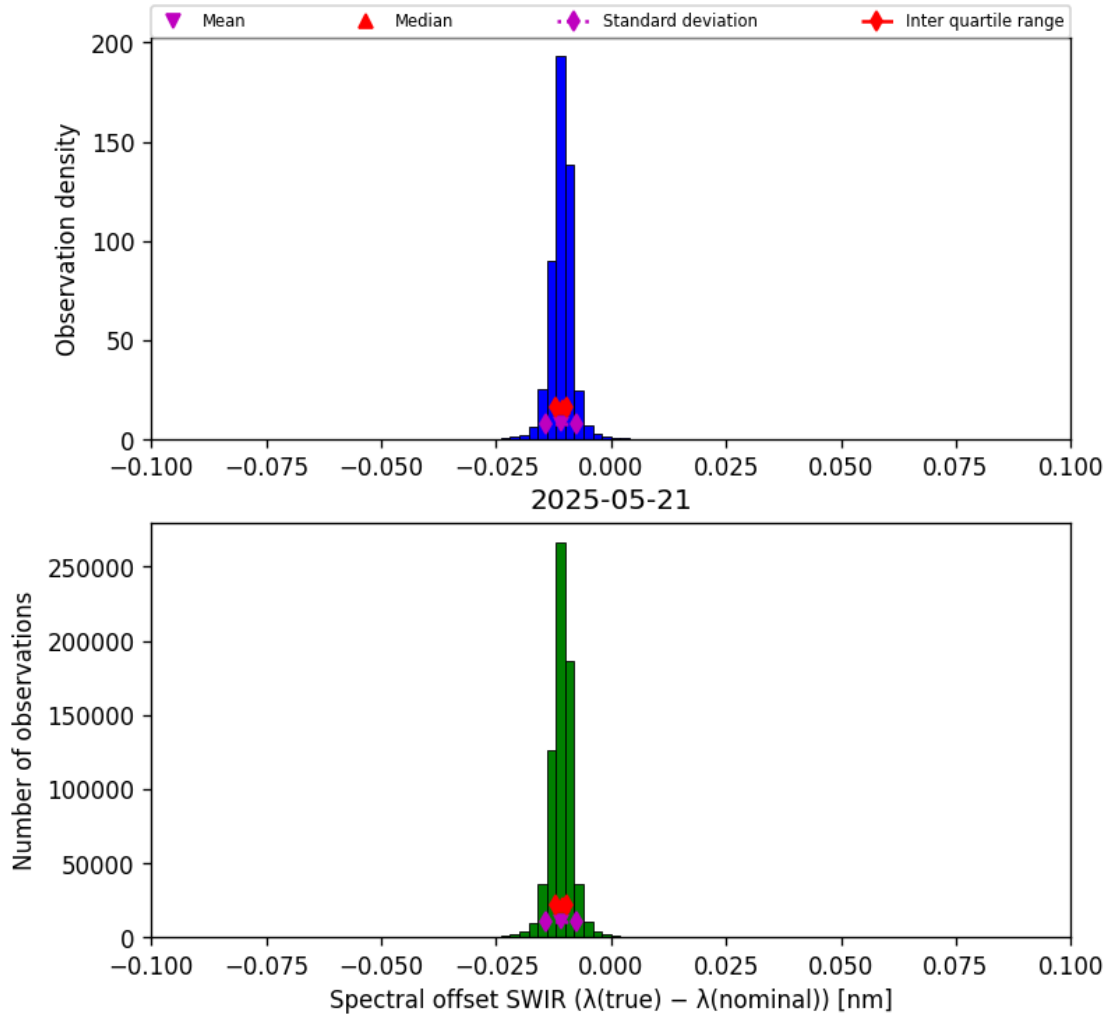
Figure 27: Histogram of “Spectral offset SWIR ( \lambda_{\text{true}} - \lambda_{\text{nominal}} )” for 2025-05-21 to 2025-05-22
