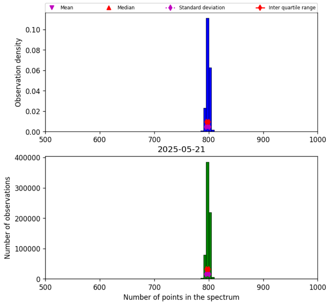
Figure 26: Histogram of “Number of points in the spectrum” for 2025-05-21 to 2025-05-22
