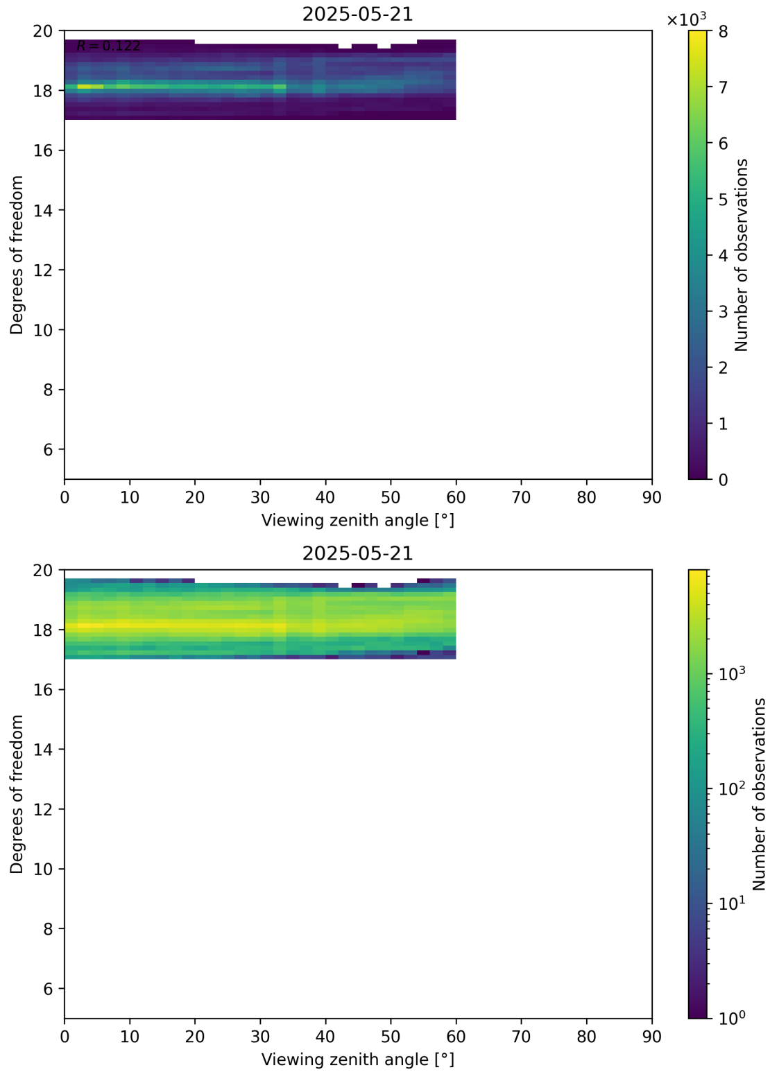
Figure 107: Scatter density plot of “Viewing zenith angle” against “Degrees of freedom” for 2025-05-21 to 2025-05-22.
