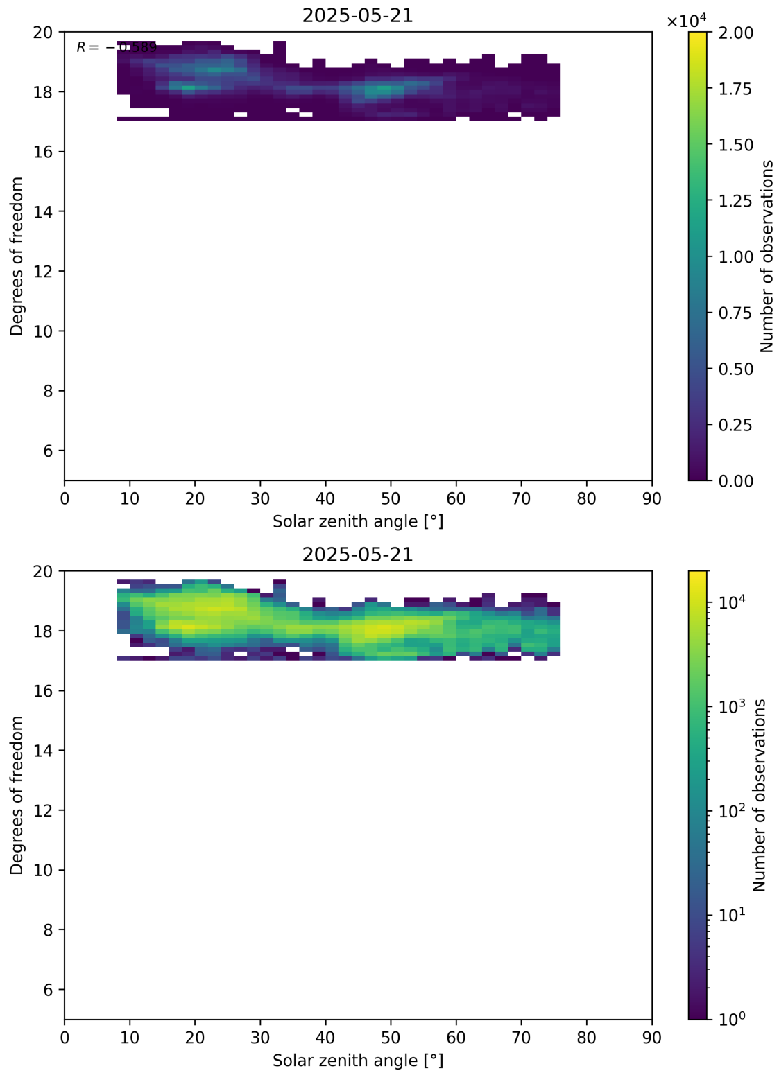
Figure 96: Scatter density plot of “Solar zenith angle” against “Degrees of freedom” for 2025-05-21 to 2025-05-22.
