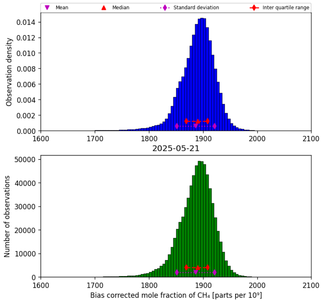
Figure 25: Histogram of “Bias corrected mole fraction of CH 4 ” for 2025-05-21 to 2025-05-22
