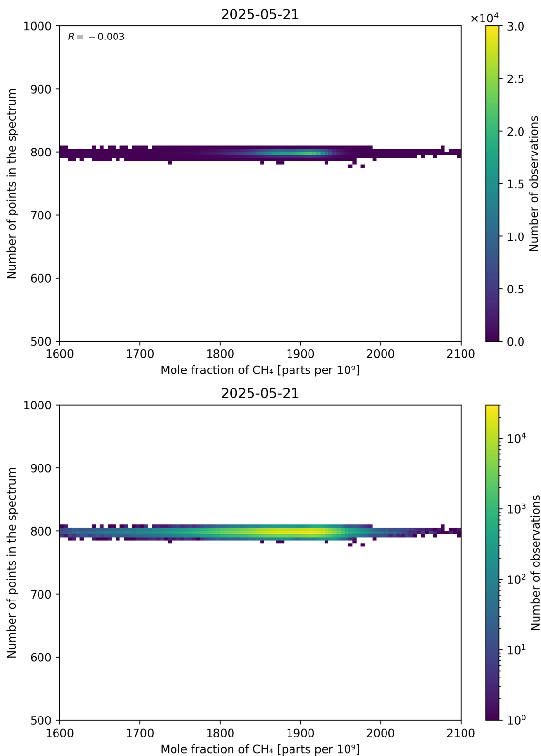
Figure 77: Scatter density plot of “Mole fraction of CH 4 ” against “Number of points in the spectrum” for 2025-05-21 to 2025-05-22.
