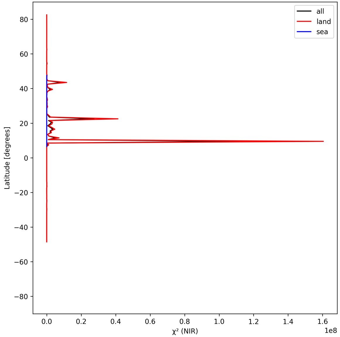
Figure 18: Zonal average of “ \chi^2 (NIR)” for 2025-05-21 to 2025-05-22.
