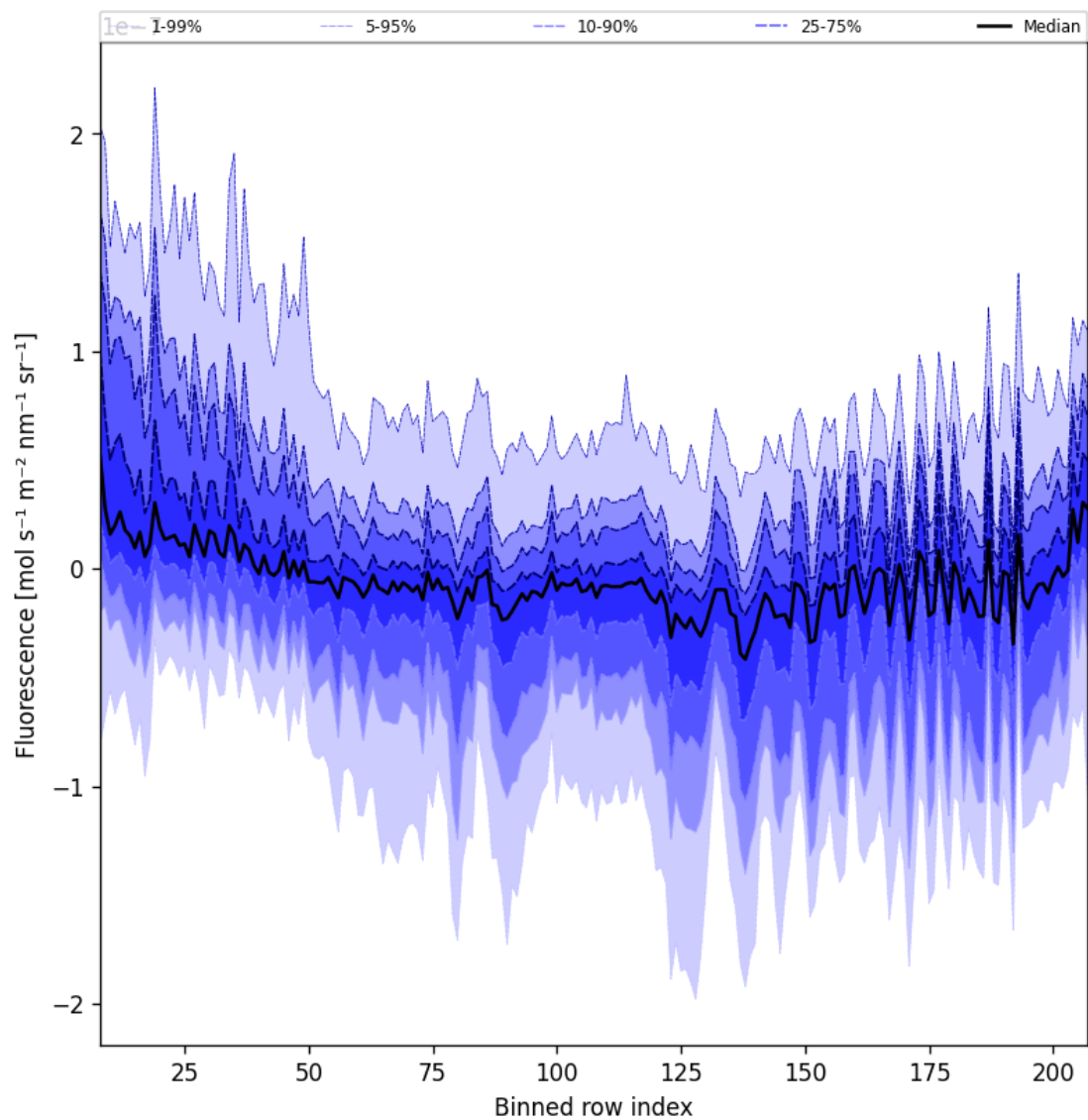
Figure 43: Along track statistics of “Fluorescence” for 2025-05-21 to 2025-05-22
