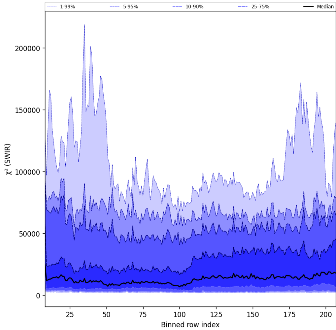
Figure 39: Along track statistics of " \chi^2 (SWIR)" for 2025-05-21 to 2025-05-22
