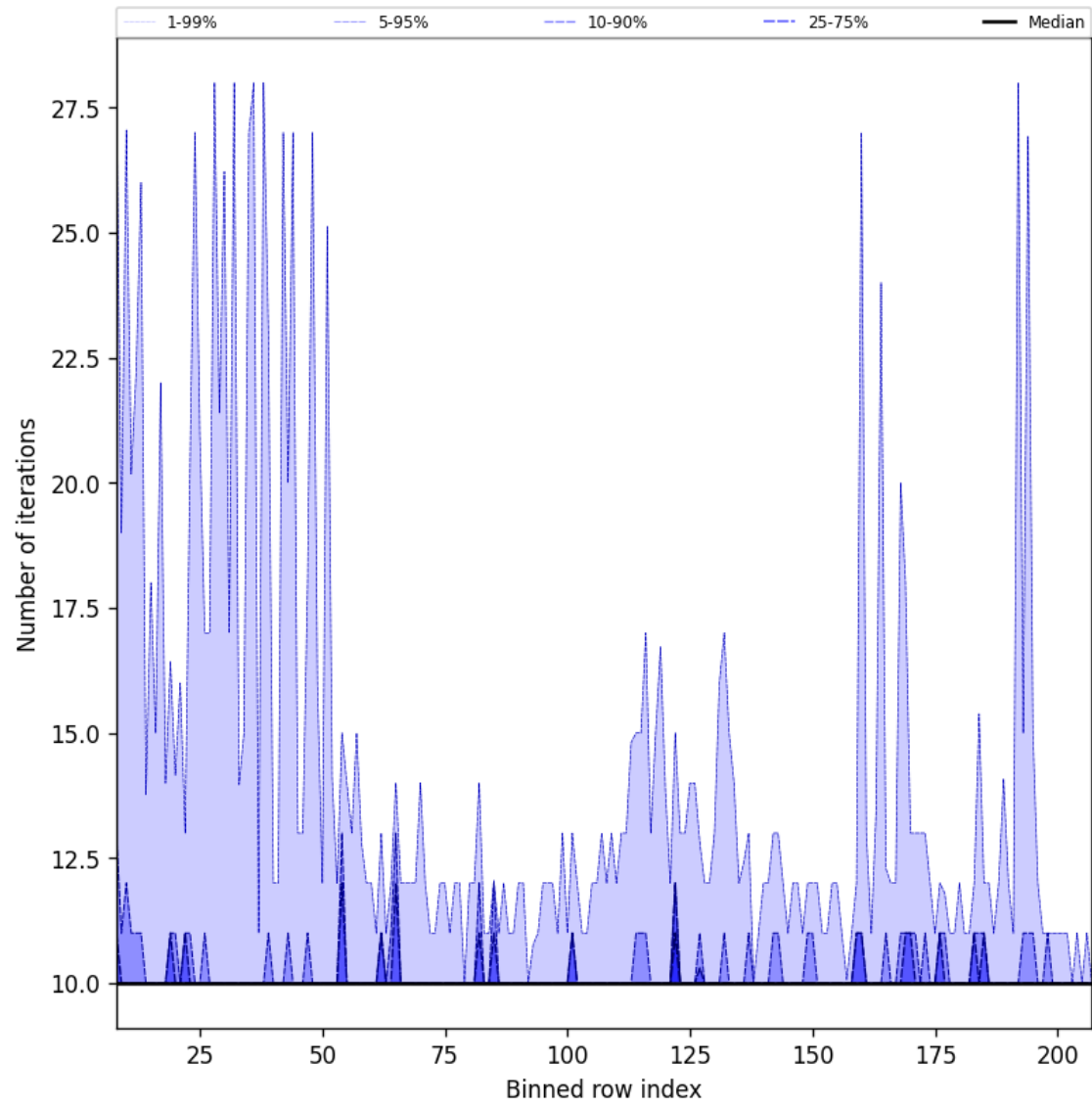
Figure 42: Along track statistics of “Number of iterations” for 2025-05-21 to 2025-05-22
