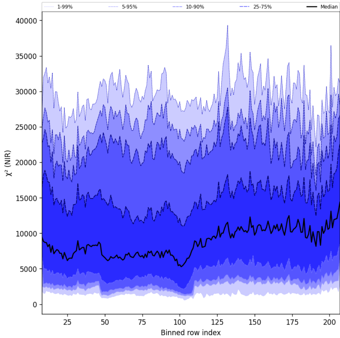
Figure 40: Along track statistics of “ \chi^2 (NIR)” for 2025-05-21 to 2025-05-22
