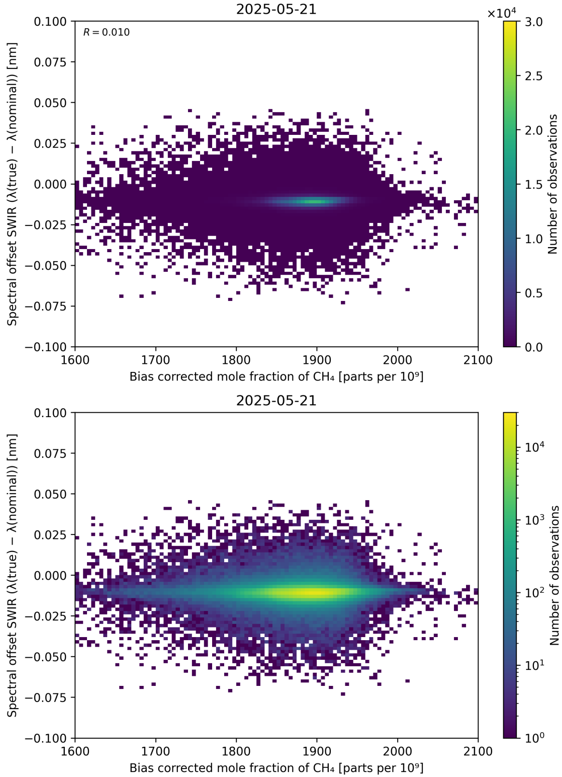
Figure 69: Scatter density plot of “Bias corrected mole fraction of CH 4 ” against “Spectral offset SWIR ( \lambda_{\text{true}} - \lambda_{\text{nominal}} )” for 2025-05-21 to 2025-05-22.
