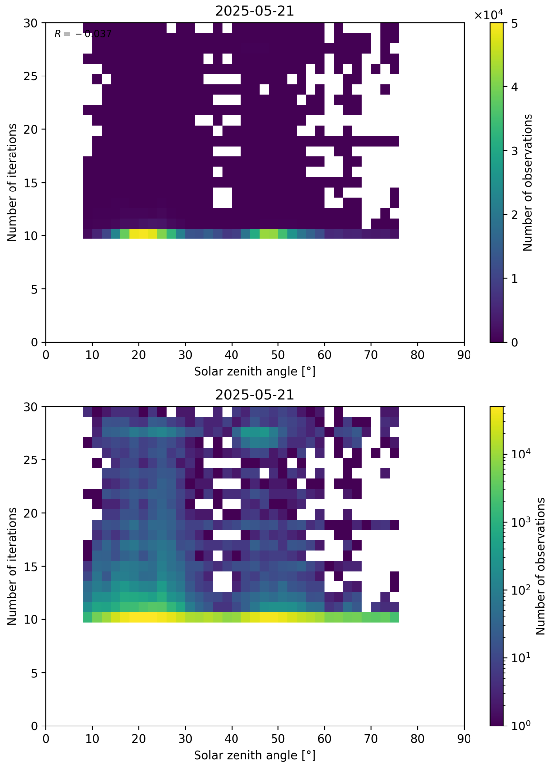
Figure 102: Scatter density plot of “Solar zenith angle” against “Number of iterations” for 2025-05-21 to 2025-05-22.
