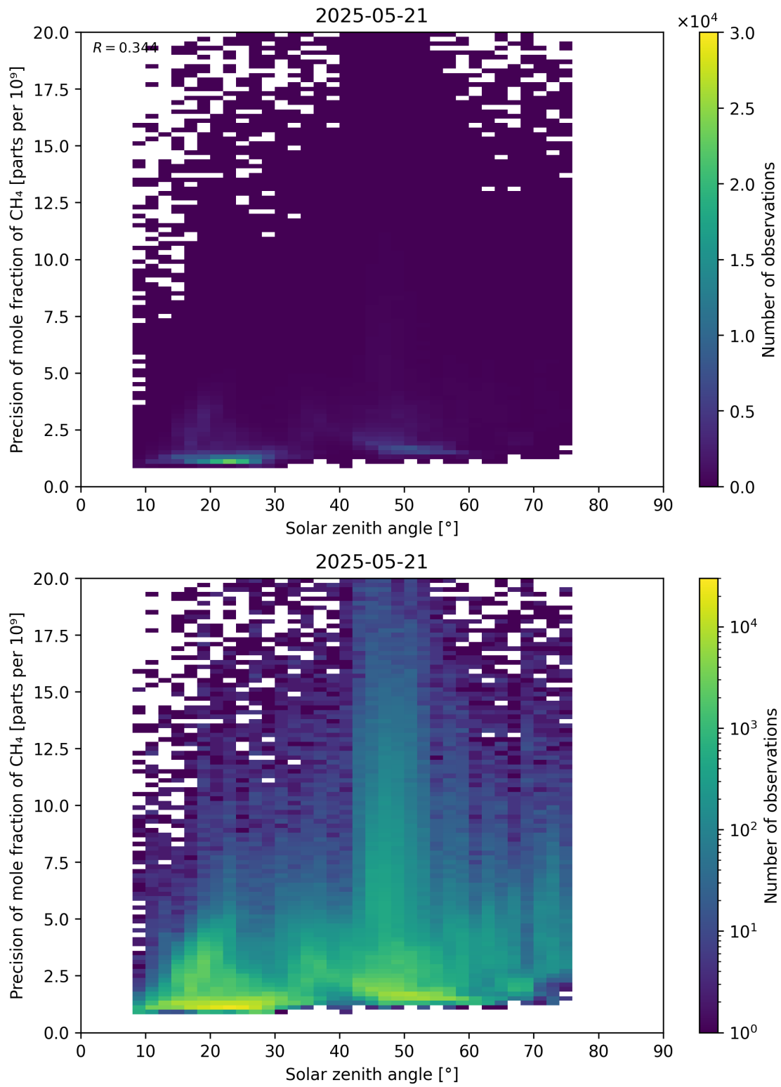
Figure 101: Scatter density plot of “Solar zenith angle” against “Precision of mole fraction of \text{CH}_4 ” for 2025-05-21 to 2025-05-22.
