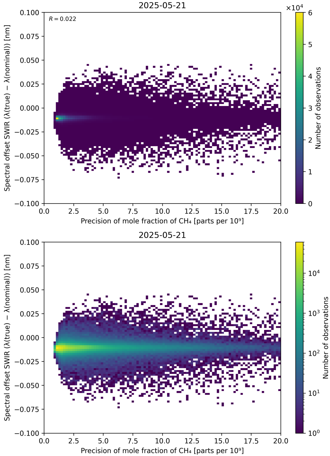
Figure 85: Scatter density plot of “Precision of mole fraction of \text{CH}_4 ” against “Spectral offset SWIR ( \lambda_{\text{true}} - \lambda_{\text{nominal}} )” for 2025-05-21 to 2025-05-22.
