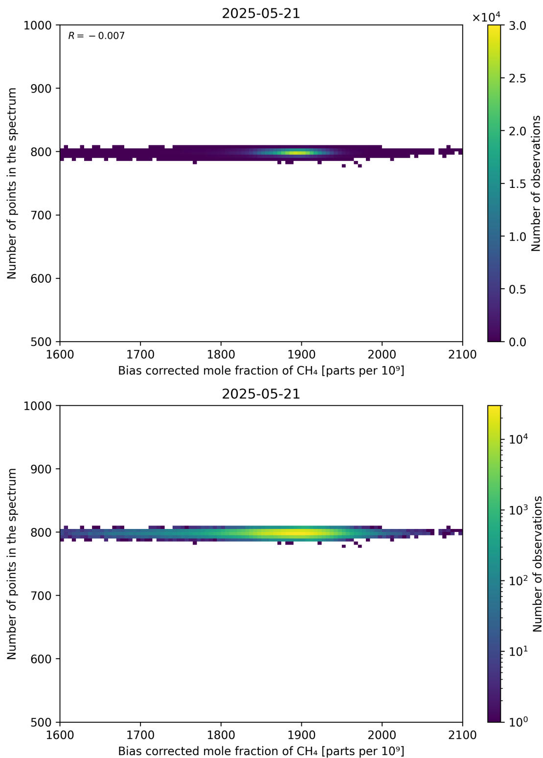
Figure 68: Scatter density plot of “Bias corrected mole fraction of CH 4 ” against “Number of points in the spectrum” for 2025-05-21 to 2025-05-22.
