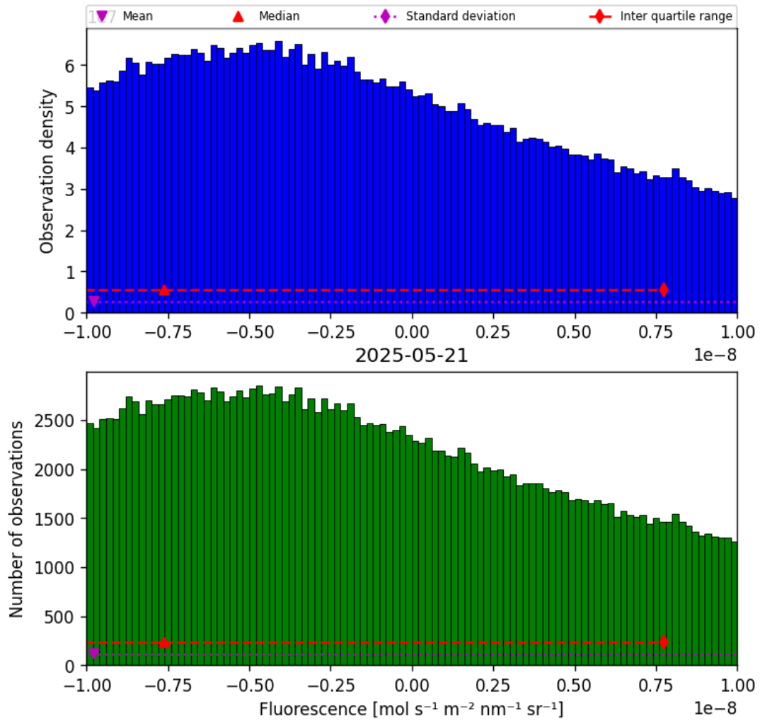
Figure 32: Histogram of “Fluorescence” for 2025-05-21 to 2025-05-22
