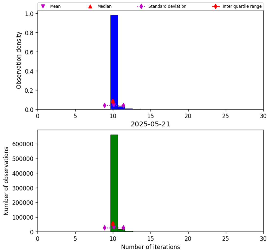
Figure 31: Histogram of “Number of iterations” for 2025-05-21 to 2025-05-22
