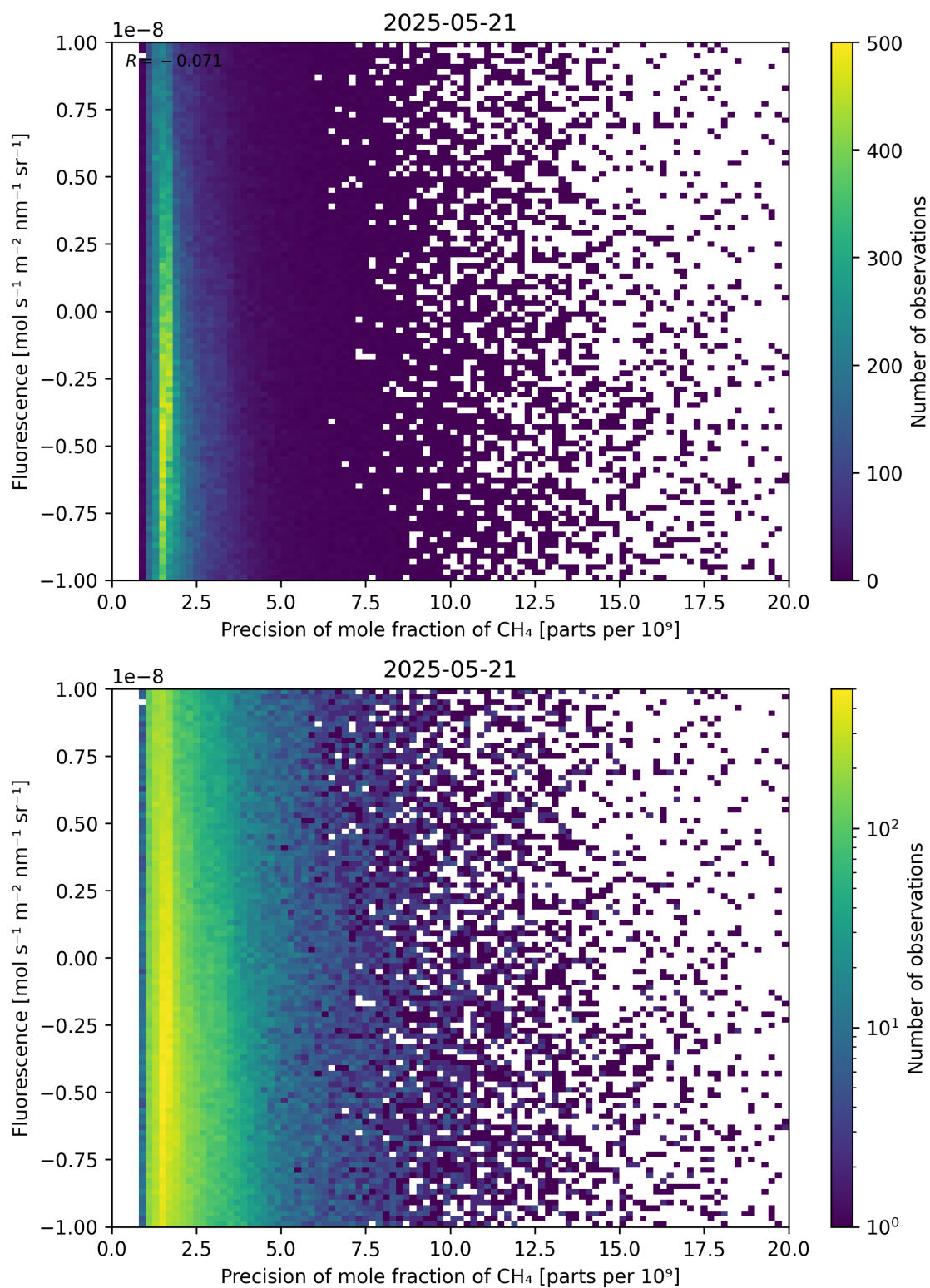
Figure 81: Scatter density plot of “Precision of mole fraction of \text{CH}_4 ” against “Fluorescence” for 2025-05-21 to 2025-05-22.
