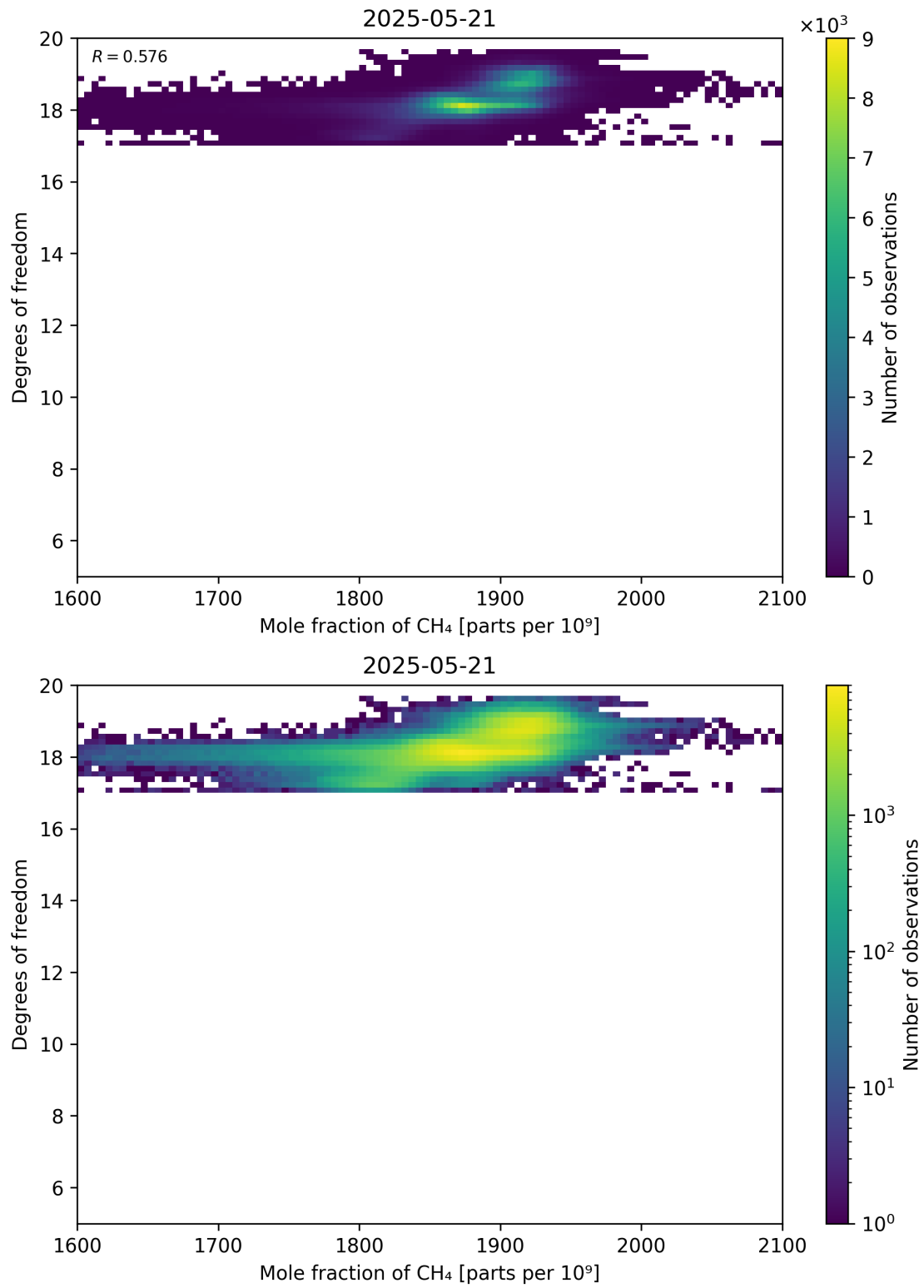
Figure 72: Scatter density plot of “Mole fraction of CH 4 ” against “Degrees of freedom” for 2025-05-21 to 2025-05-22.
