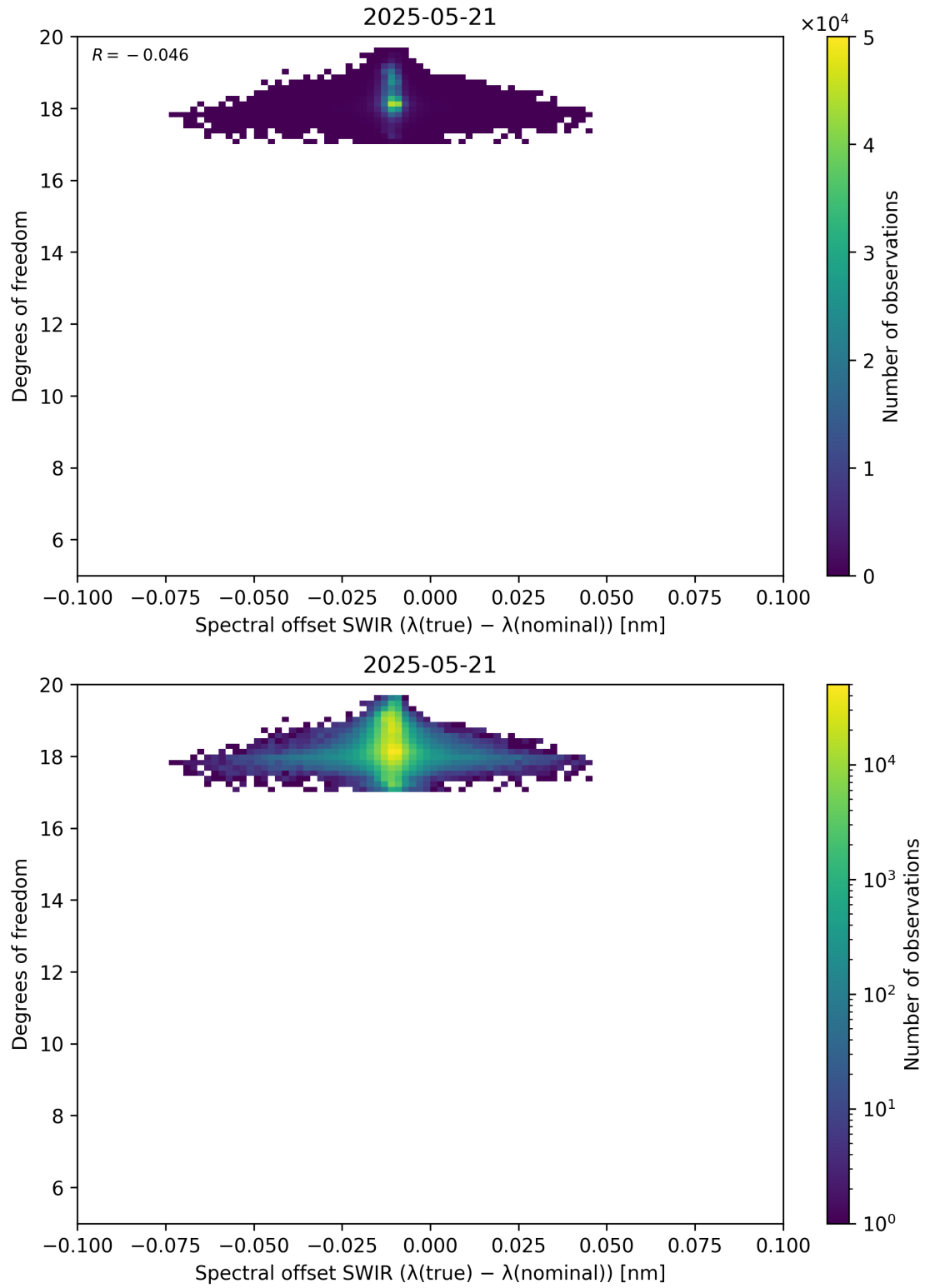
Figure 119: Scatter density plot of “Spectral offset SWIR ( \lambda_{\text{true}} - \lambda_{\text{nominal}} )” against “Degrees of freedom” for 2025-05-21 to 2025-05-22.
