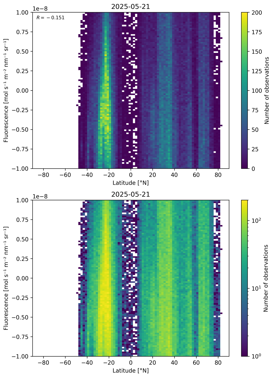
Figure 56: Scatter density plot of “Latitude” against “Fluorescence” for 2025-05-21 to 2025-05-22.
