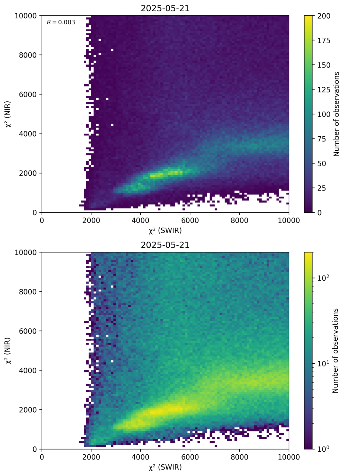
Figure 47: Scatter density plot of “ \chi^2 (SWIR)” against “ \chi^2 (NIR)” for 2025-05-21 to 2025-05-22.
