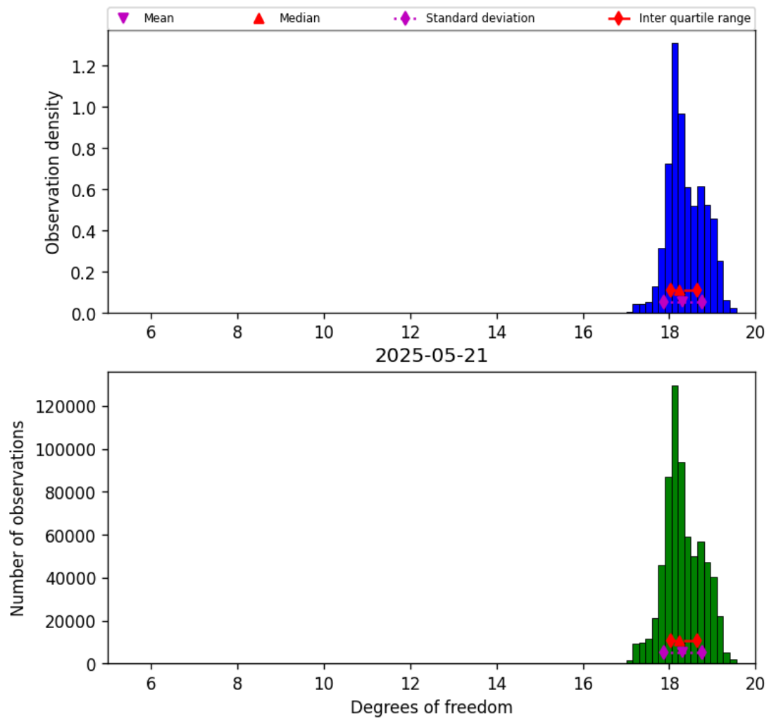
Figure 30: Histogram of “Degrees of freedom” for 2025-05-21 to 2025-05-22
