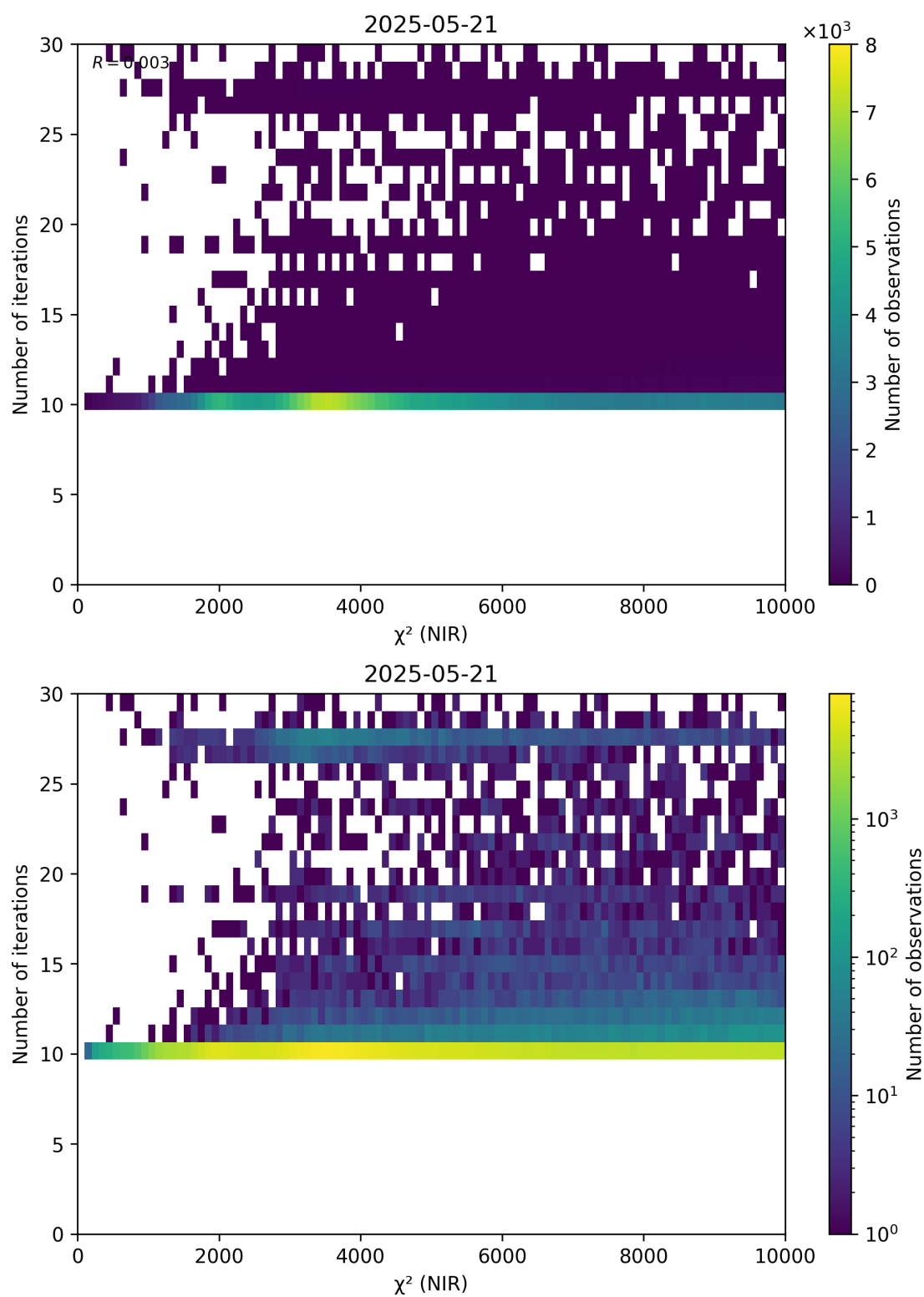
Figure 46: Scatter density plot of “ \chi^2 (NIR)” against “Number of iterations” for 2025-05-21 to 2025-05-22.
