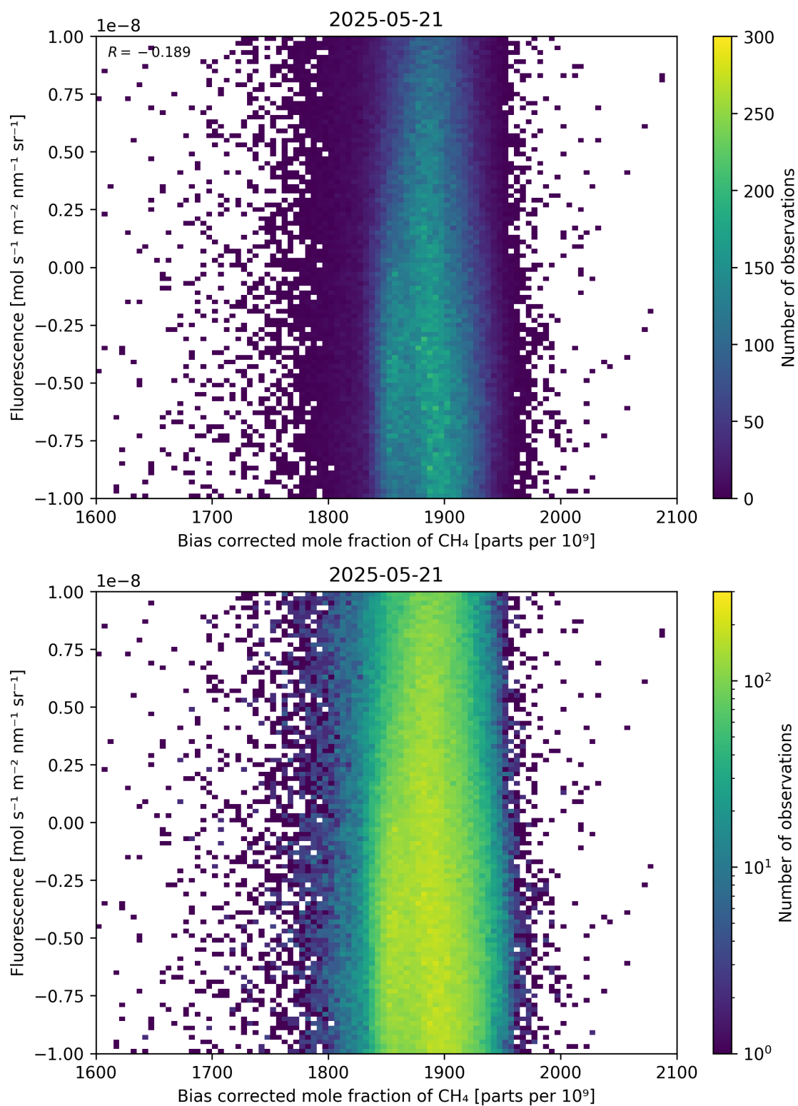
Figure 66: Scatter density plot of “Bias corrected mole fraction of \text{CH}_4 ” against “Fluorescence” for 2025-05-21 to 2025-05-22.
