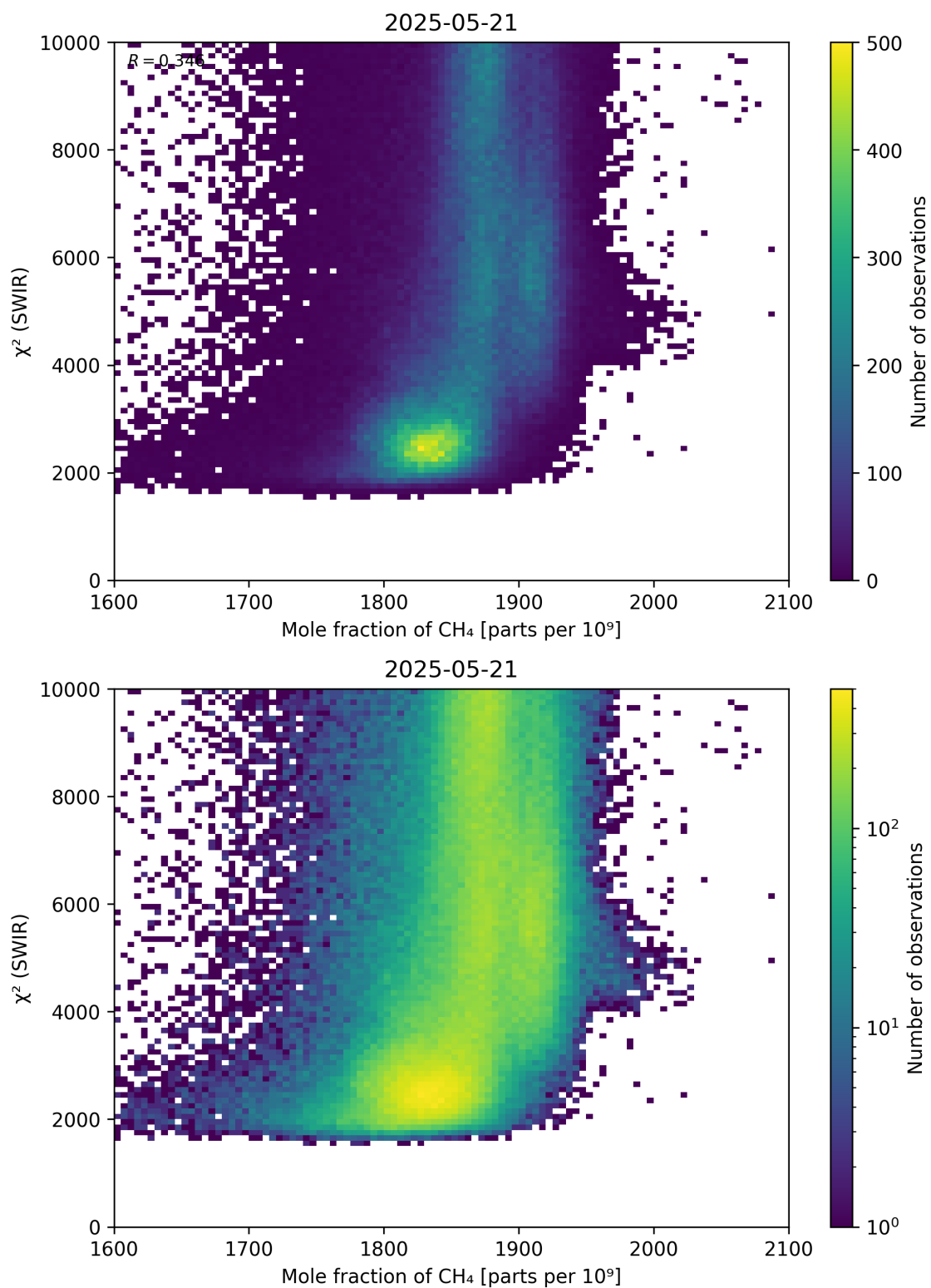
Figure 71: Scatter density plot of “Mole fraction of \text{CH}_4 ” against “ \chi^2 (SWIR)” for 2025-05-21 to 2025-05-22.
