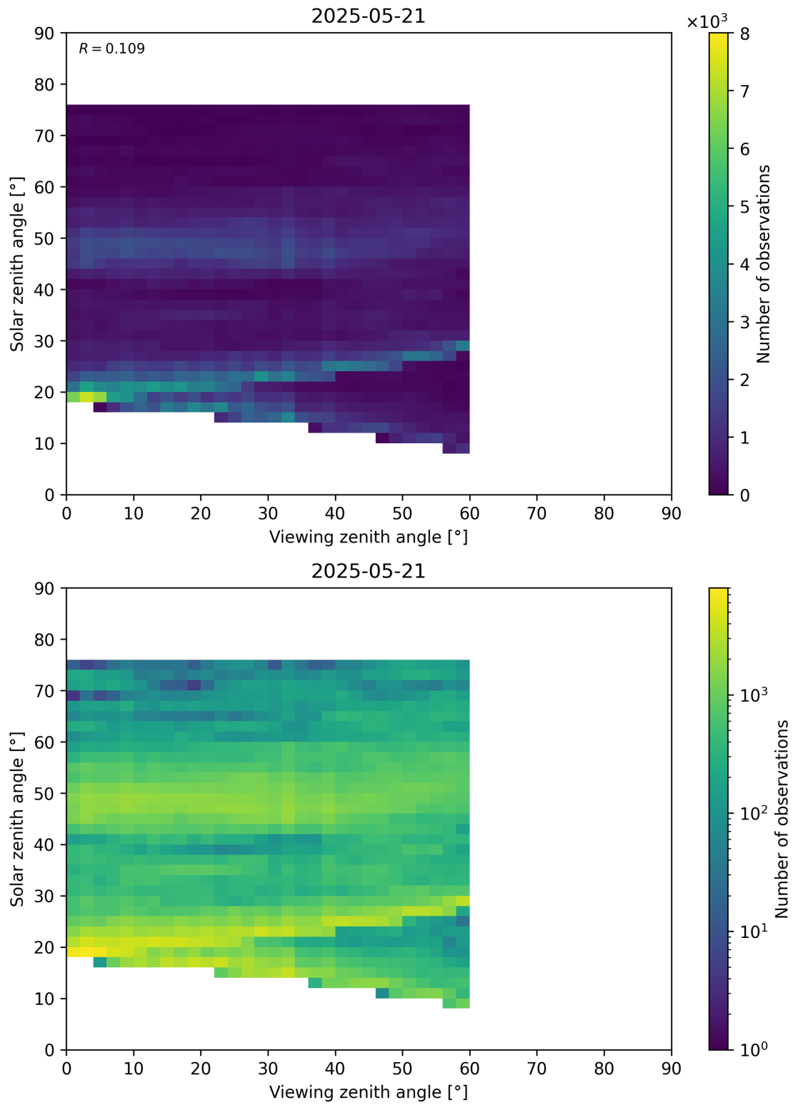
Figure 115: Scatter density plot of “Viewing zenith angle” against “Solar zenith angle” for 2025-05-21 to 2025-05-22.
