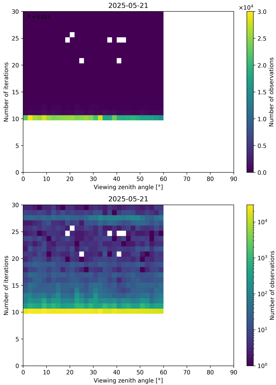
Figure 113: Scatter density plot of “Viewing zenith angle” against “Number of iterations” for 2025-05-21 to 2025-05-22.
