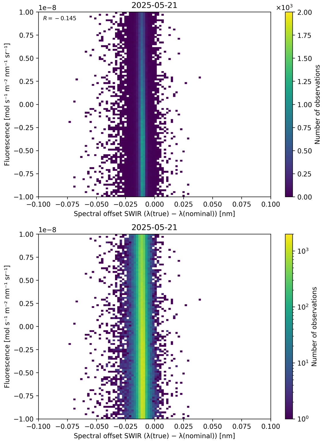
Figure 120: Scatter density plot of “Spectral offset SWIR ( \lambda_{\text{true}} - \lambda_{\text{nominal}} )” against “Fluorescence” for 2025-05-21 to 2025-05-22.
