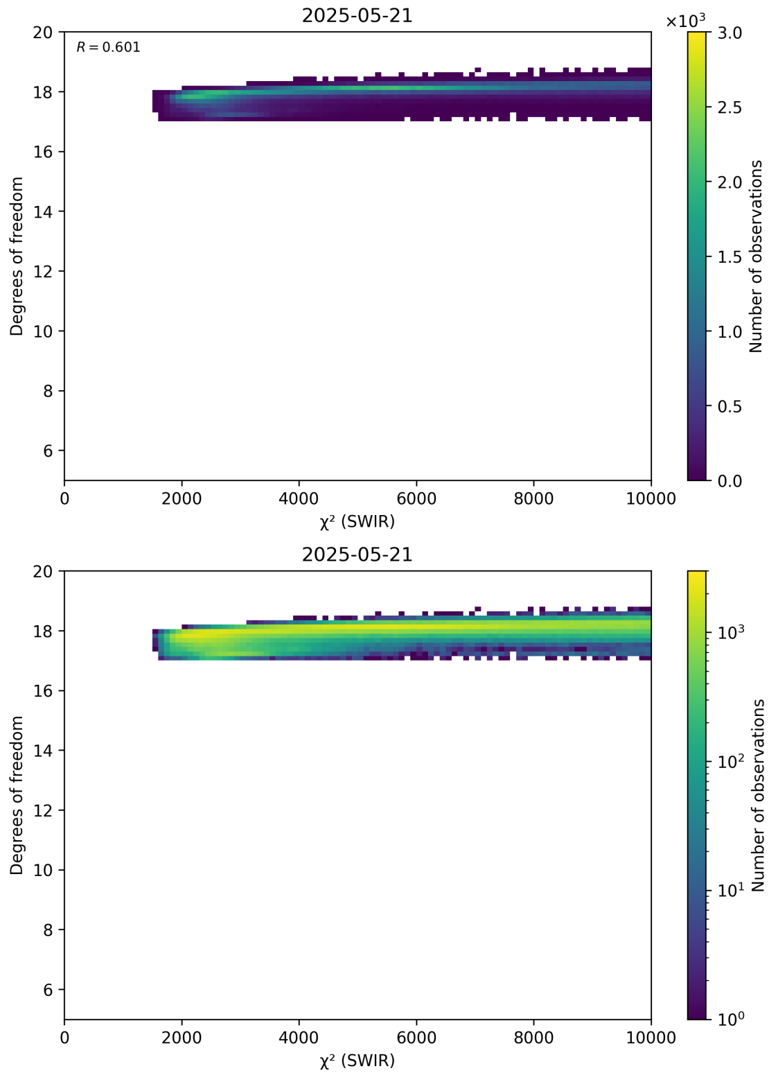
Figure 48: Scatter density plot of “ \chi^2 (SWIR)” against “Degrees of freedom” for 2025-05-21 to 2025-05-22.
