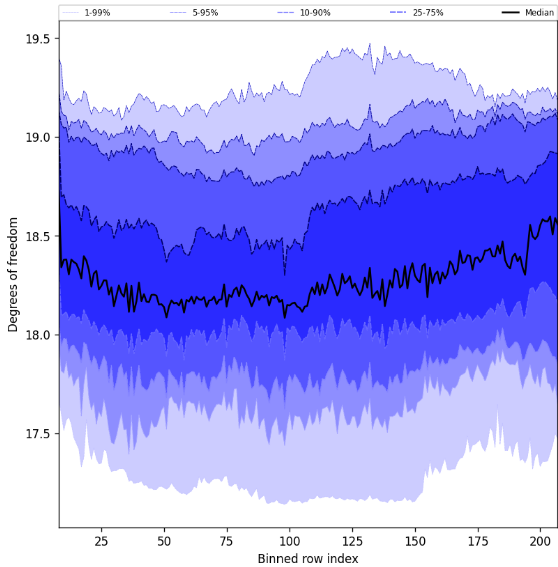
Figure 41: Along track statistics of “Degrees of freedom” for 2025-05-21 to 2025-05-22
