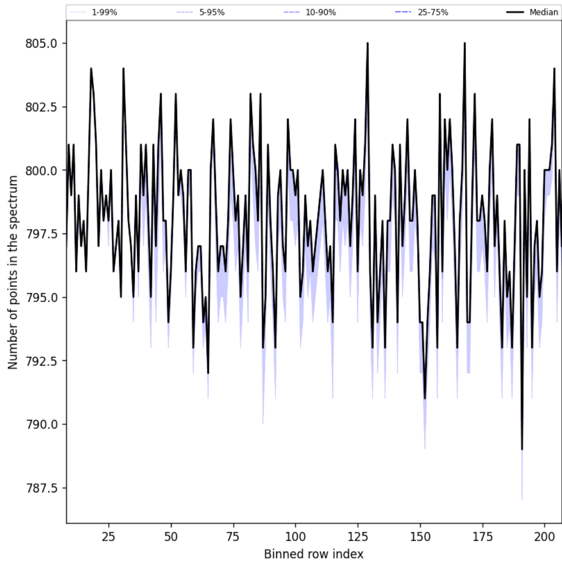
Figure 37: Along track statistics of “Number of points in the spectrum” for 2025-05-21 to 2025-05-22
