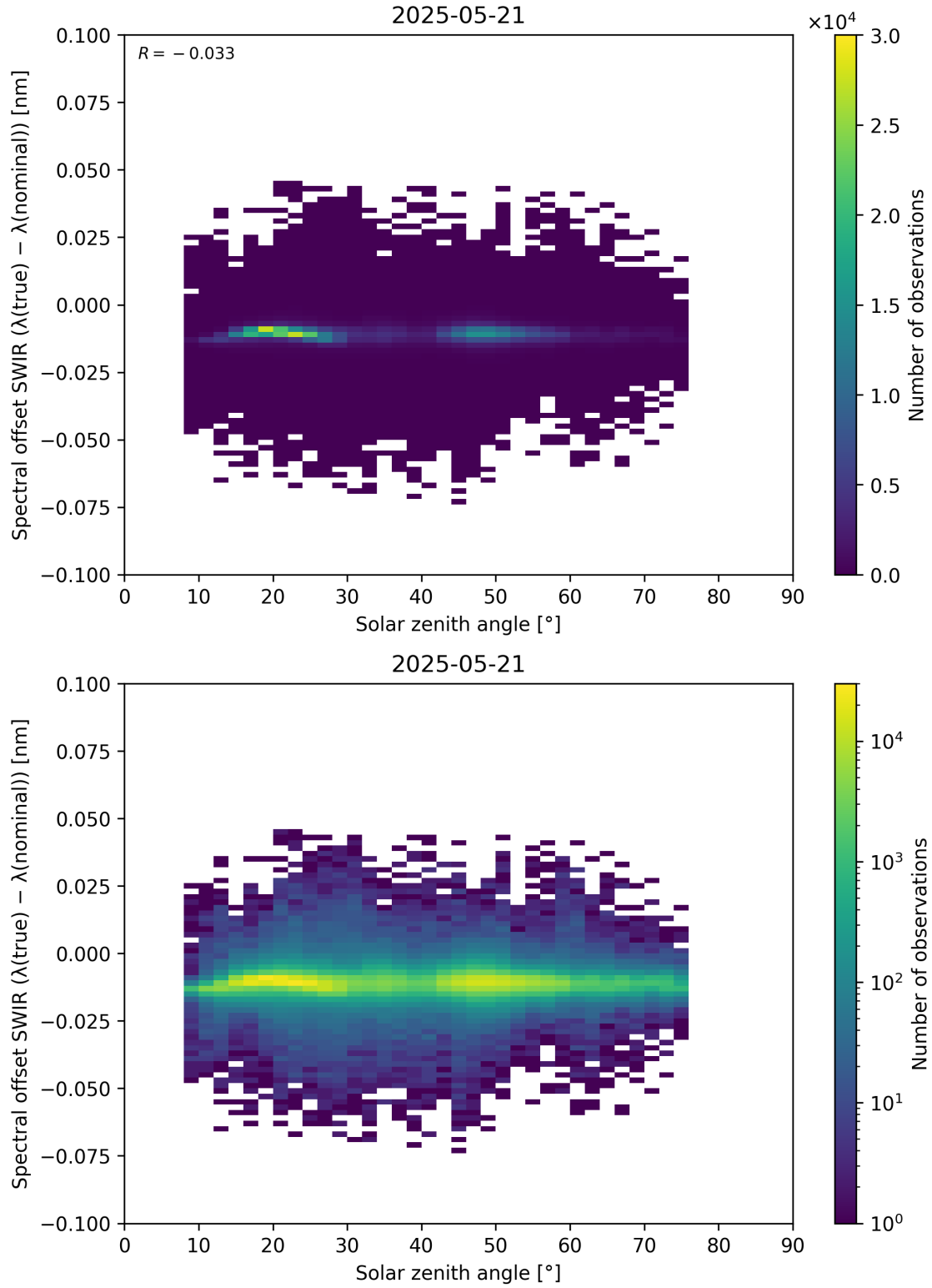
Figure 104: Scatter density plot of “Solar zenith angle” against “Spectral offset SWIR ( \lambda_{\text{true}} - \lambda_{\text{nominal}} )” for 2025-05-21 to 2025-05-22.
