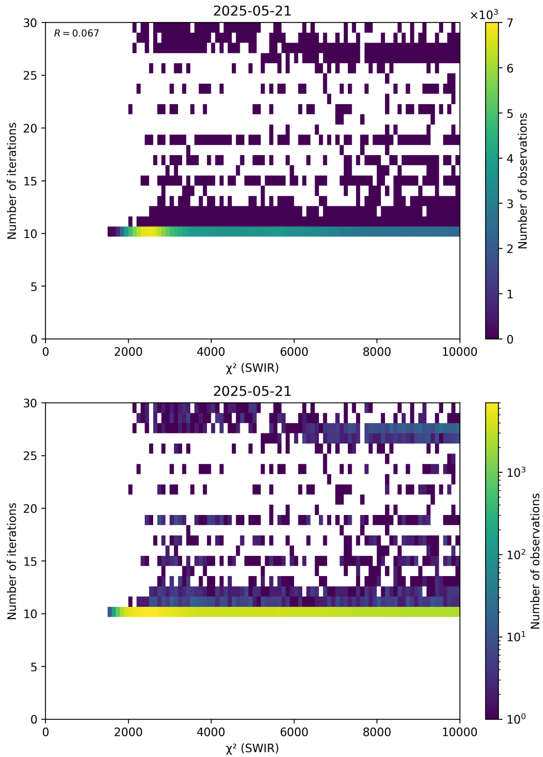
Figure 50: Scatter density plot of “ \chi^2 (SWIR)” against “Number of iterations” for 2025-05-21 to 2025-05-22.
