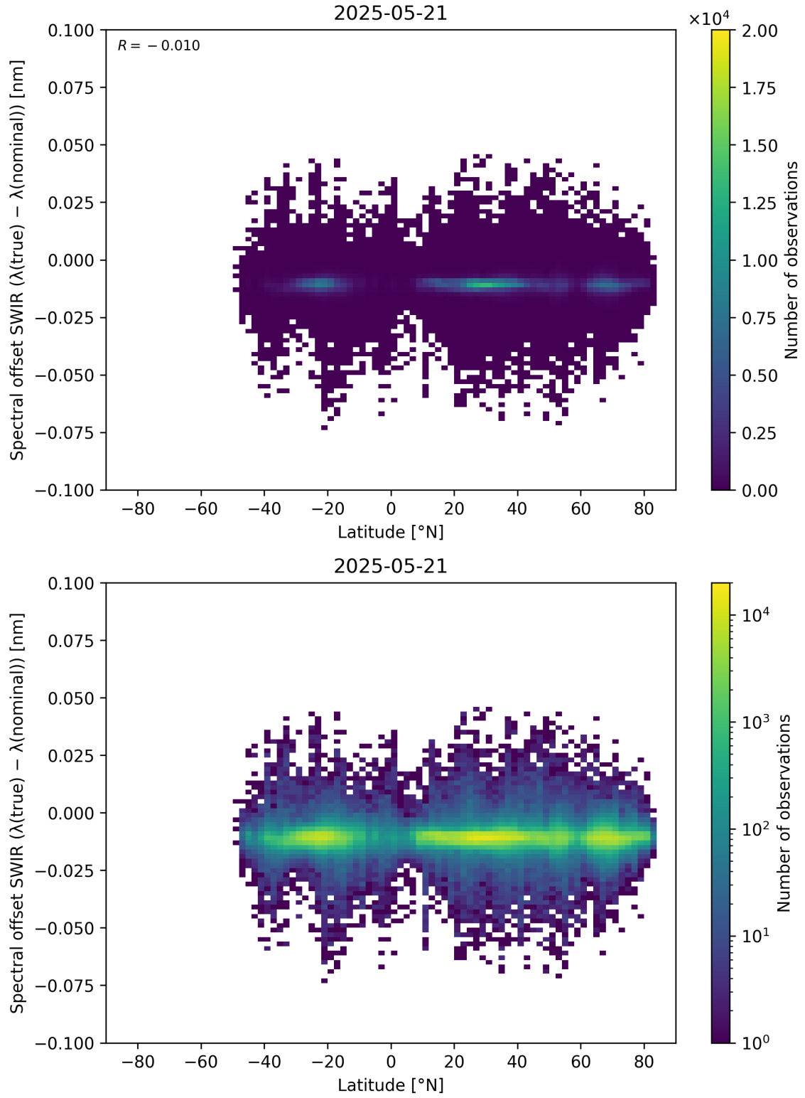
Figure 62: Scatter density plot of “Latitude” against “Spectral offset SWIR ( \lambda_{\text{true}} - \lambda_{\text{nominal}} )” for 2025-05-21 to 2025-05-22.
