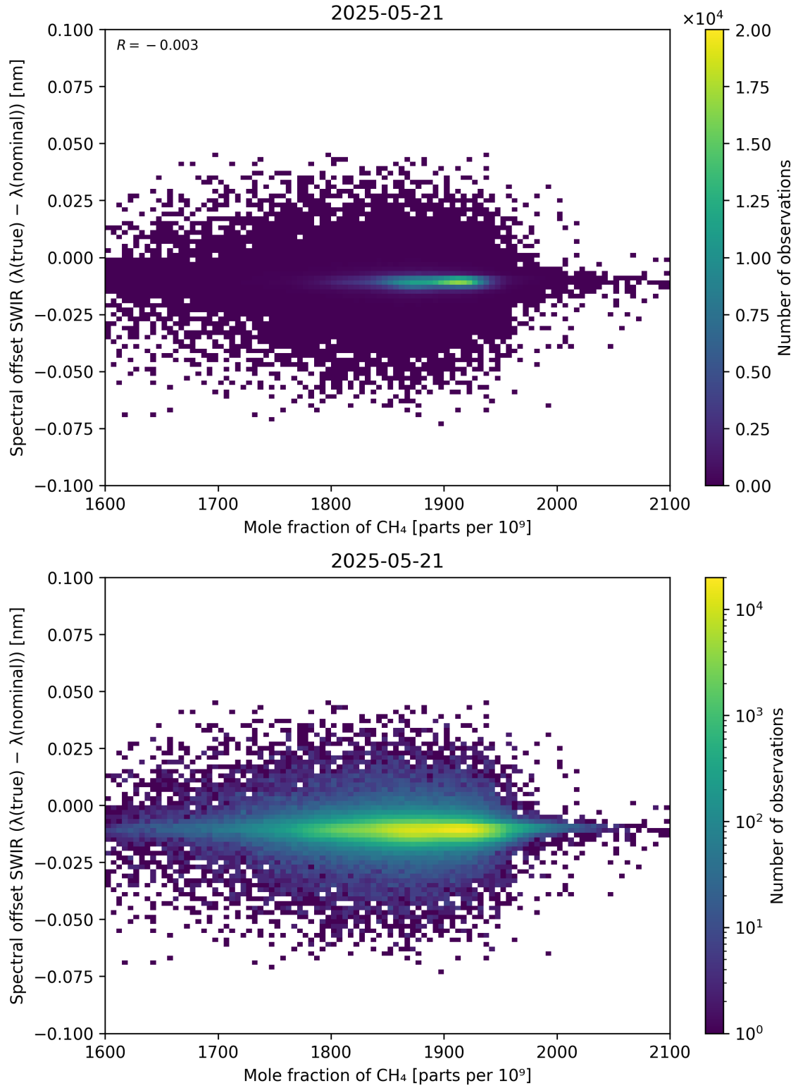
Figure 86: Scatter density plot of “Mole fraction of CH 4 ” against “Spectral offset SWIR ( \lambda_{\text{true}} - \lambda_{\text{nominal}} )” for 2025-05-21 to 2025-05-22.
