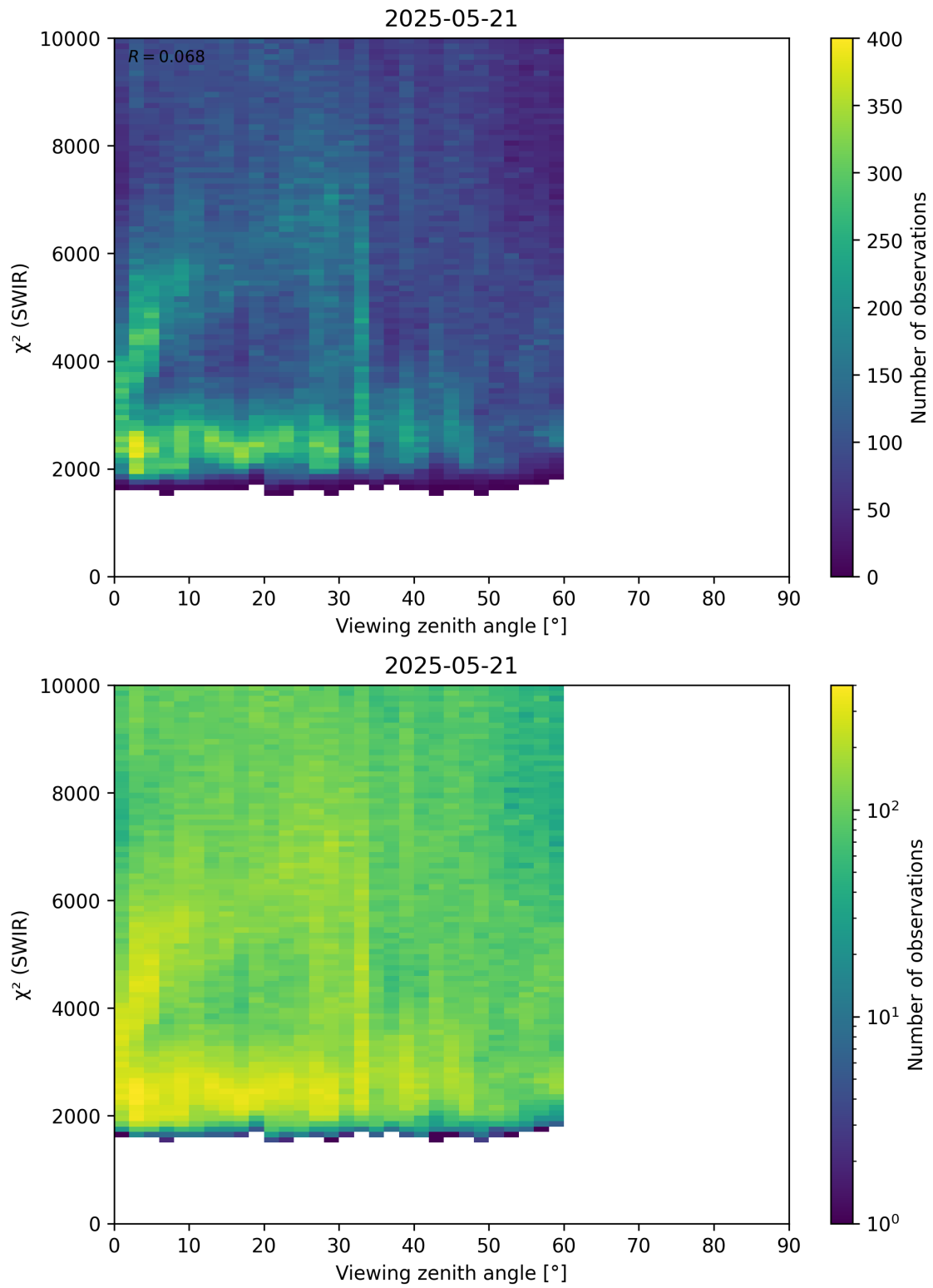
Figure 106: Scatter density plot of “Viewing zenith angle” against “ \chi^2 (SWIR)” for 2025-05-21 to 2025-05-22.
